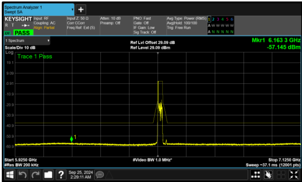
Figure 295 - A (Core 0) 802.11ax HE20 RU26 SP 6535 MHz (CH117)
