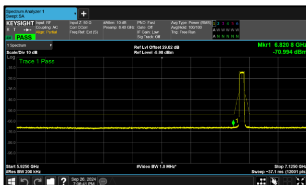
Figure 298 - A (Core 0) 802.11a VLP 6855 MHz (CH181)
