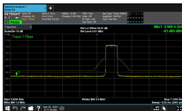
Figure 301 - A (Core 0) 802.11ax HE80 SU VLP 6625 MHz (CH135)
