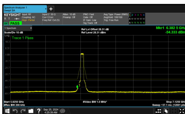
Figure 326 - B (Core 1) 802.11ax HE20 SU SP 6415 MHz (CH93)
