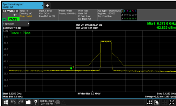
Figure 338 - A (Core 0) 802.11ax HE80 SU LPI 6625 MHz (CH135)
