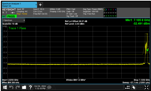
Figure 324 - B (Core 1) 802.11ax HE20 RU52 LPI 7095 MHz (CH229)
