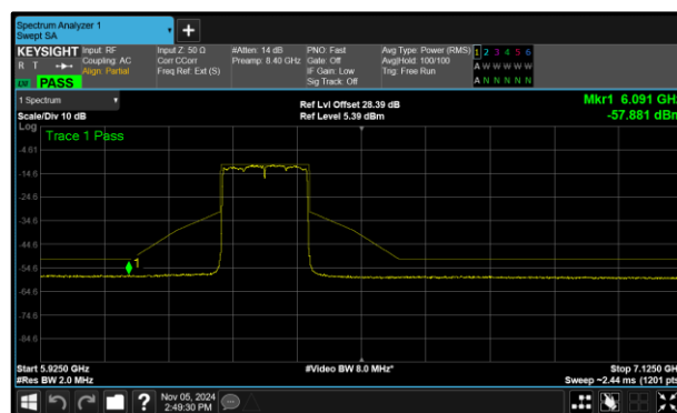
Figure 306 - B (Core 1) 802.11ax HE160 SU LPI 6345 MHz (CH79)
