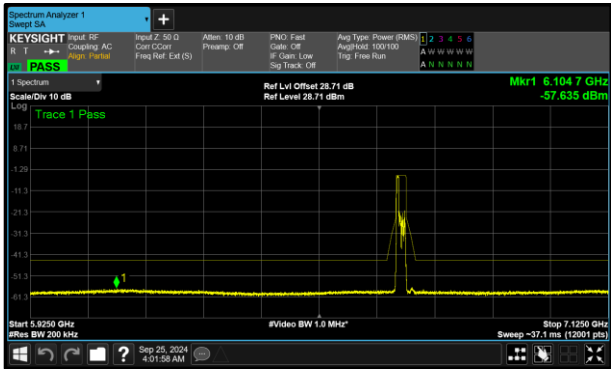
Figure 314 - A (Core 0) 802.11ax HE20 RU52 SP 6695 MHz (CH149)
