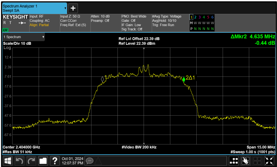
Figure 101 - Core 1 (B) 2404 MHz (CH2) 99% Bandwidth
