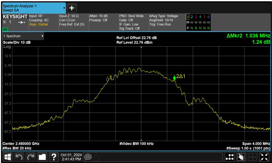
Figure 135 - Core 2 (A) 2480 MHz (CH39) 99% Bandwidth
