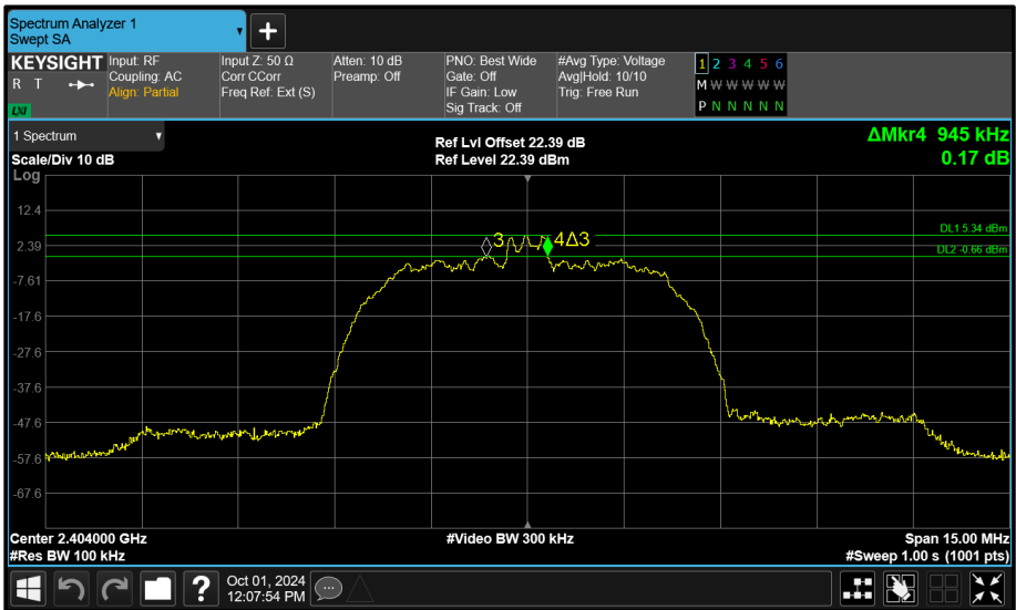
Figure 102 - Core 1 (B) 2404 MHz (CH2) 6 dB Bandwidth
