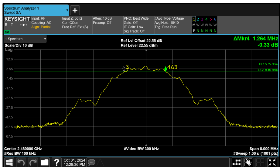
Figure 118 - Core 1 (B) 2480 MHz (CH39) 6 dB Bandwidth
