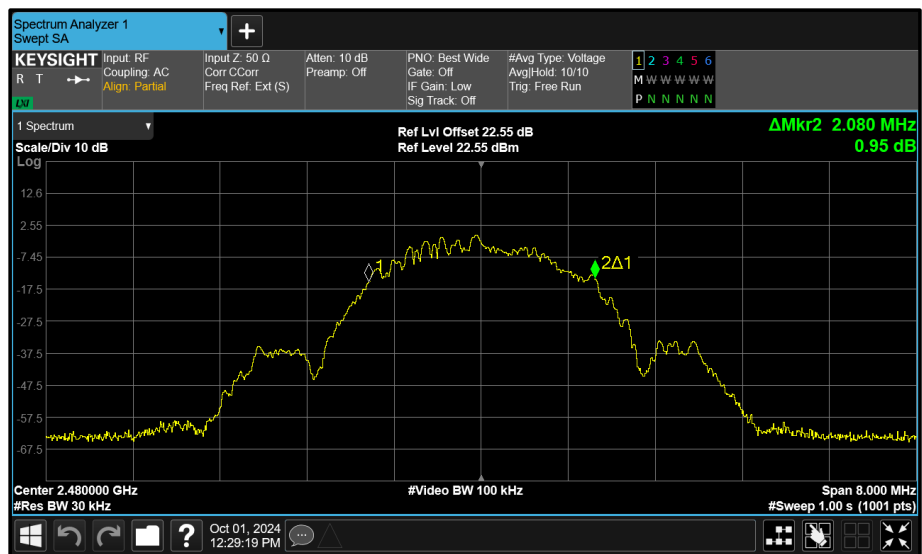
Figure 117 - Core 1 (B) 2480 MHz (CH39) 99% Bandwidth
