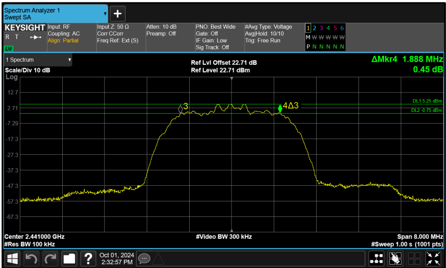
Figure 122 - Core 2 (A) 2441 MHz (CH39) 6 dB Bandwidth
