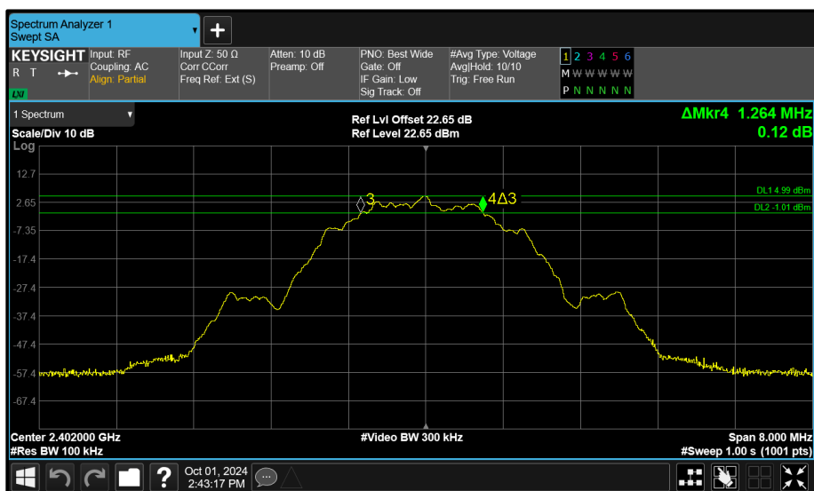
Figure 138 - Core 2 (A) 2402 MHz (CH37) 6 dB Bandwidth
