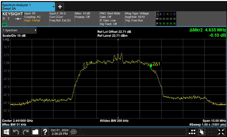
Figure 127 - Core 2 (A) 2441 MHz (CH39) 99% Bandwidth
