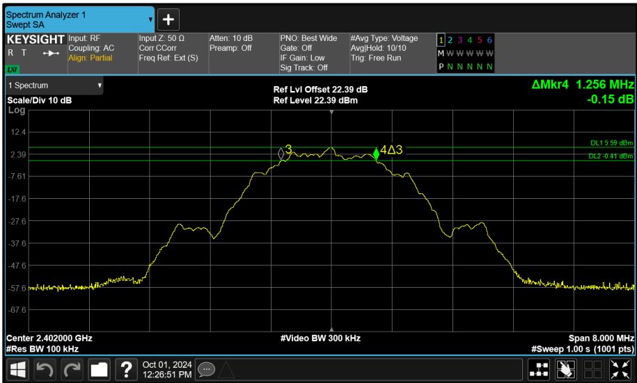
Figure 114 - Core 1 (B) 2402 MHz (CH37) 6 dB Bandwidth
