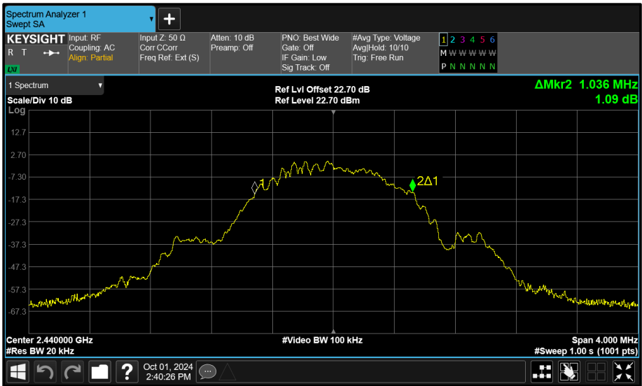
Figure 133 - Core 2 (A) 2440 MHz (CH17) 99% Bandwidth
