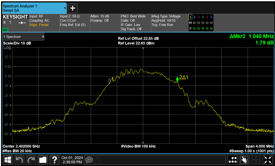
Figure 131 - Core 2 (A) 2402 MHz (CH37) 99% Bandwidth
