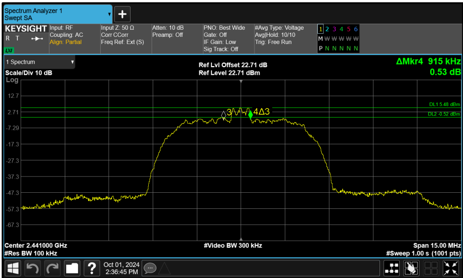
Figure 128 - Core 2 (A) 2441 MHz (CH39) 6 dB Bandwidth
