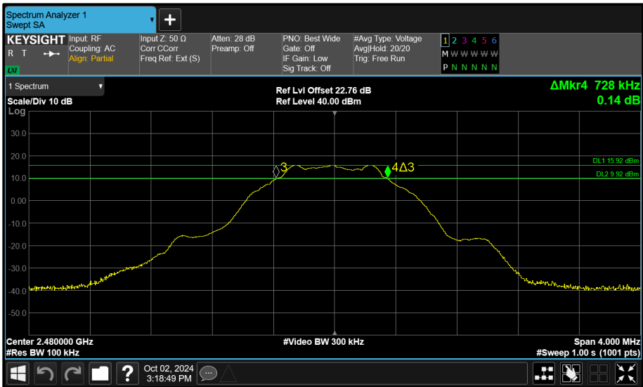
Figure 88 - Core 0 (A) 2480 MHz (CH39) 6 dB Bandwidth
