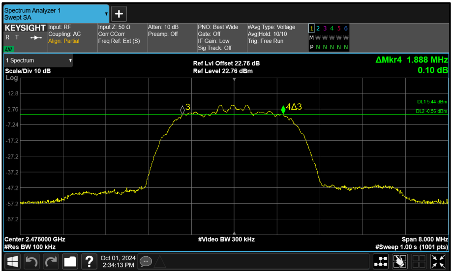
Figure 124 - Core 2 (A) 2476 MHz (CH74) 6 dB Bandwidth
