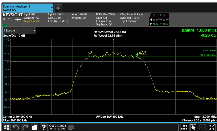
Figure 120 - Core 2 (A) 2404 MHz (CH2) 6 dB Bandwidth
