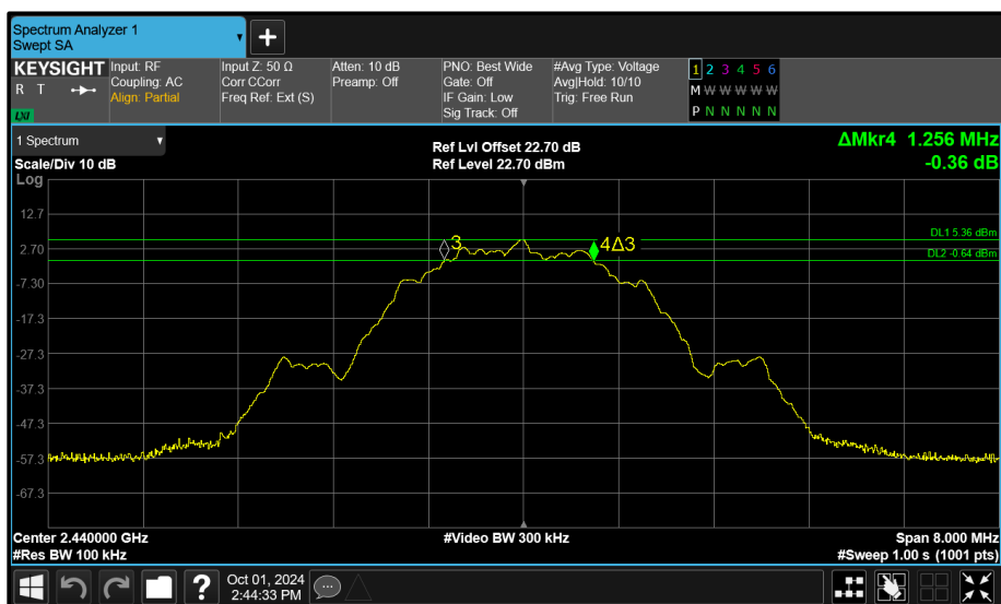
Figure 140 - Core 2 (A) 2440 MHz (CH17) 6 dB Bandwidth
