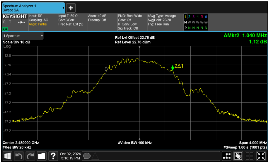
Figure 87 - Core 0 (A) 2480 MHz (CH39) 99% Bandwidth
