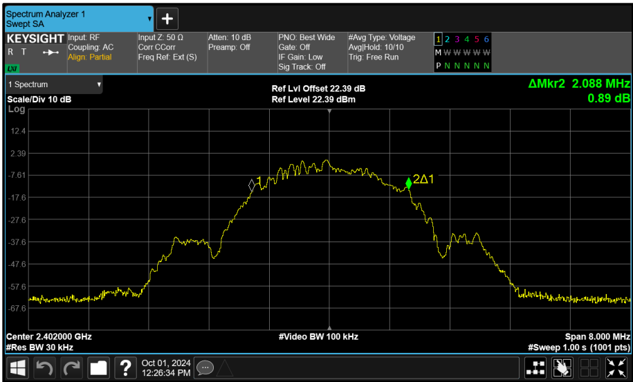
Figure 113 - Core 1 (B) 2402 MHz (CH37) 99% Bandwidth
