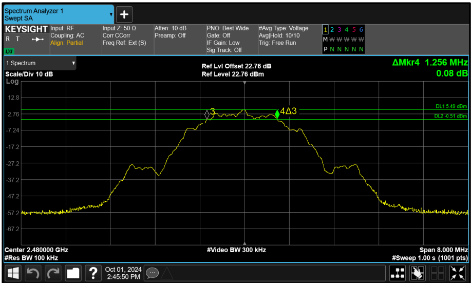
Figure 142 - Core 2 (A) 2480 MHz (CH39) 6 dB Bandwidth
