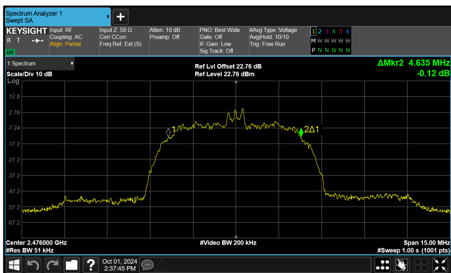
Figure 129 - Core 2 (A) 2476 MHz (CH74) 99% Bandwidth
