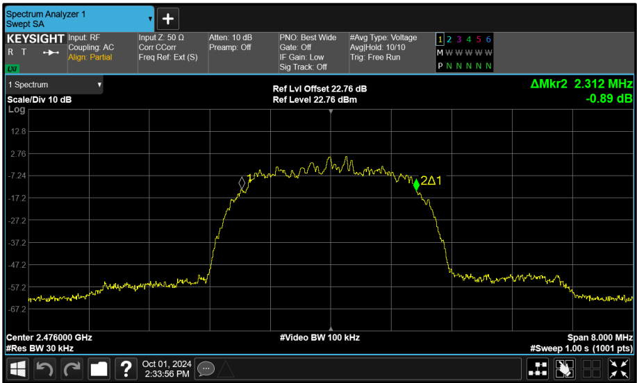
Figure 123 - Core 2 (A) 2476 MHz (CH74) 99% Bandwidth
