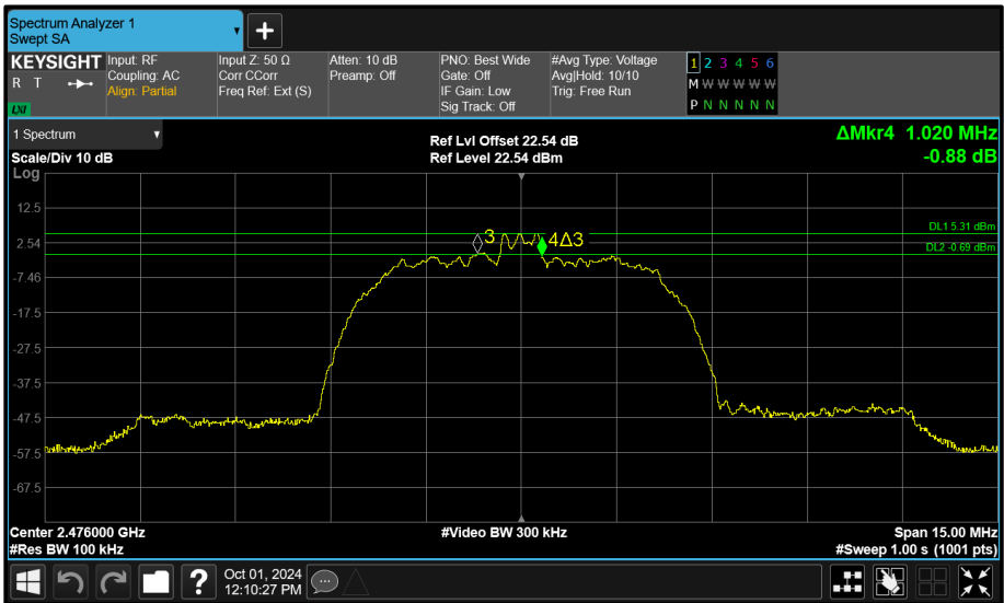
Figure 106 - Core 1 (B) 2476 MHz (CH74) 6 dB Bandwidth
