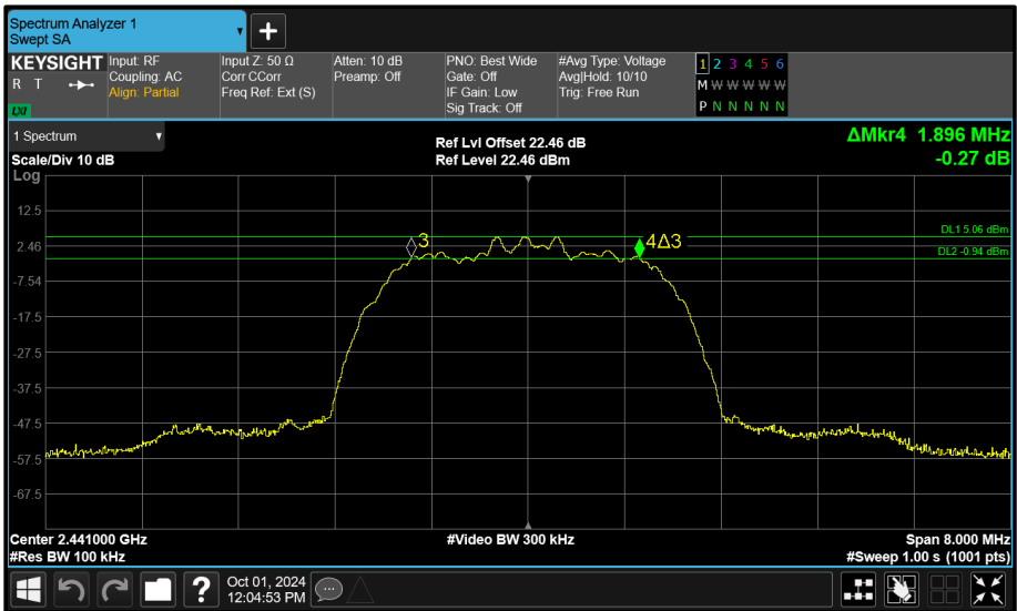
Figure 98 - Core 1 (B) 2441 MHz (CH39) 6 dB Bandwidth
