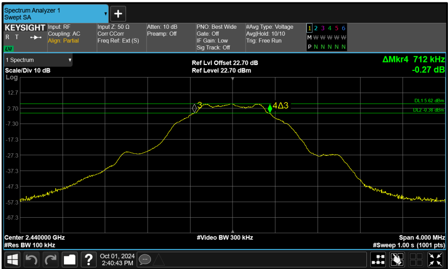
Figure 134 - Core 2 (A) 2440 MHz (CH17) 6 dB Bandwidth
