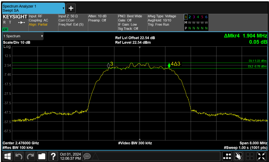
Figure 100 - Core 1 (B) 2476 MHz (CH74) 6 dB Bandwidth
