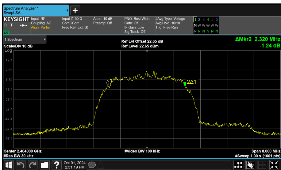
Figure 119 - Core 2 (A) 2404 MHz (CH2) 99% Bandwidth
