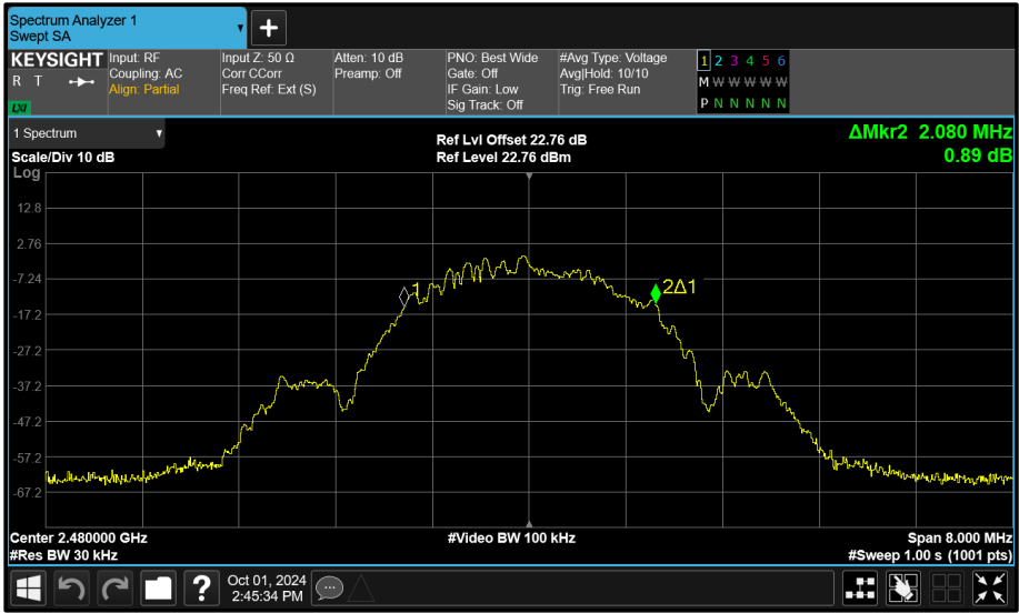
Figure 141 - Core 2 (A) 2480 MHz (CH39) 99% Bandwidth
