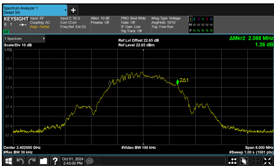
Figure 137 - Core 2 (A) 2402 MHz (CH37) 99% Bandwidth
