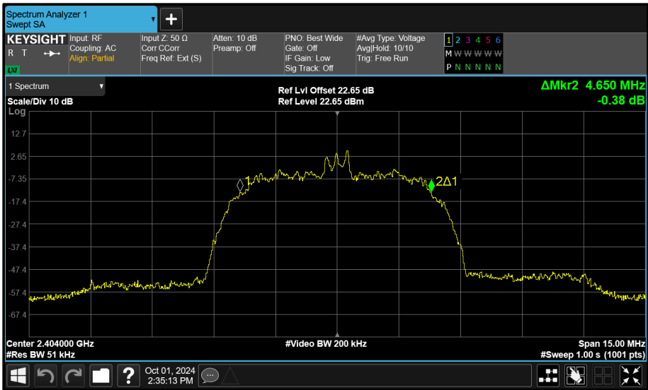
Figure 125 - Core 2 (A) 2404 MHz (CH2) 99% Bandwidth
