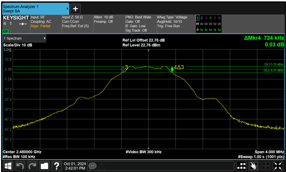
Figure 136 - Core 2 (A) 2480 MHz (CH39) 6 dB Bandwidth
