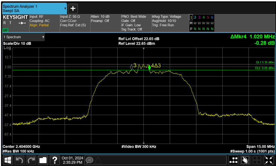
Figure 126 - Core 2 (A) 2404 MHz (CH2) 6 dB Bandwidth
