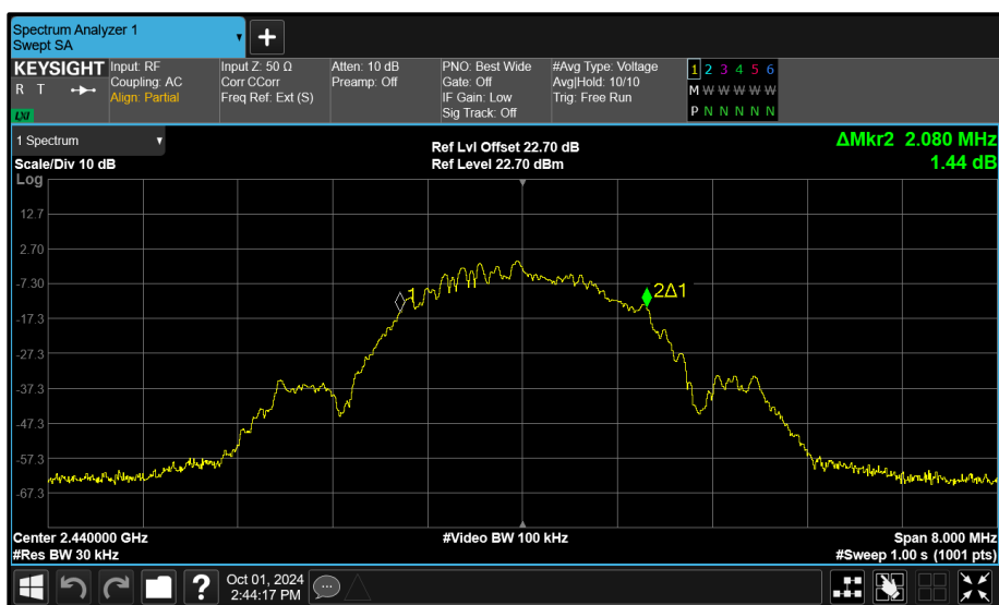
Figure 139 - Core 2 (A) 2440 MHz (CH17) 99% Bandwidth
