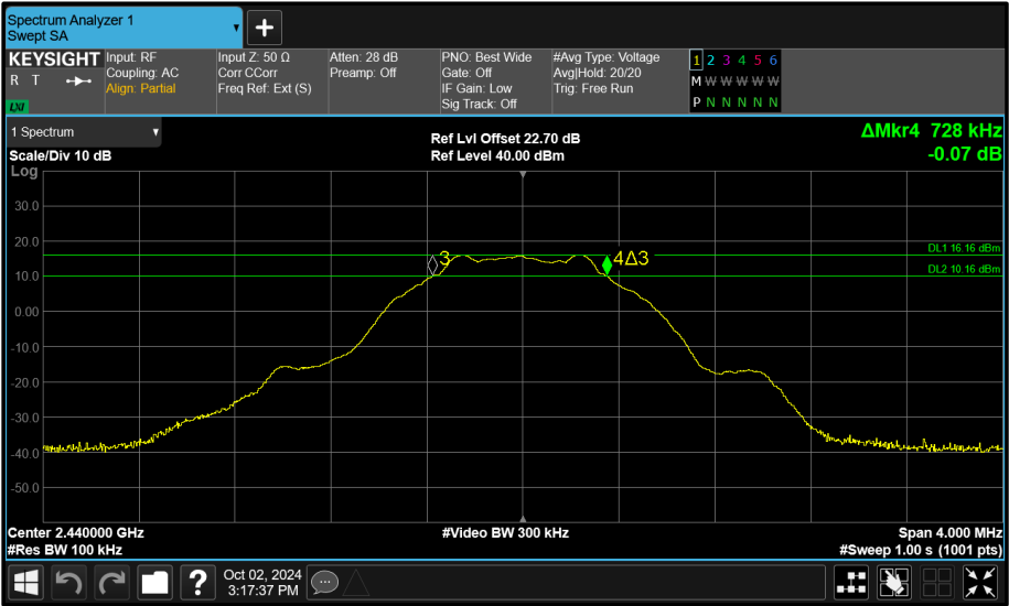
Figure 86 - Core 0 (A) 2440 MHz (CH17) 6 dB Bandwidth
