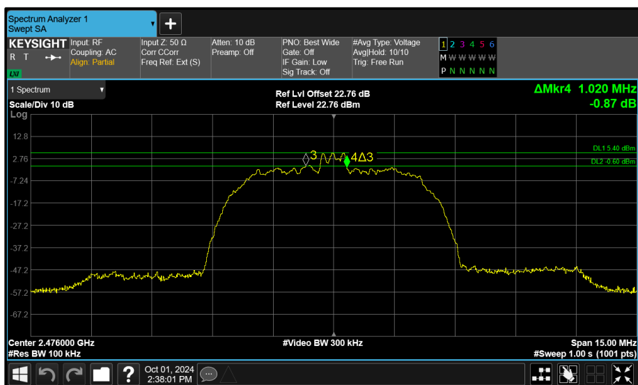
Figure 130 - Core 2 (A) 2476 MHz (CH74) 6 dB Bandwidth
