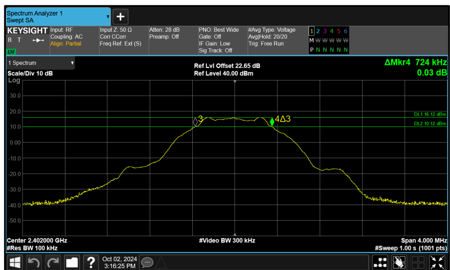
Figure 84 - Core 0 (A) 2402 MHz (CH37) 6 dB Bandwidth
