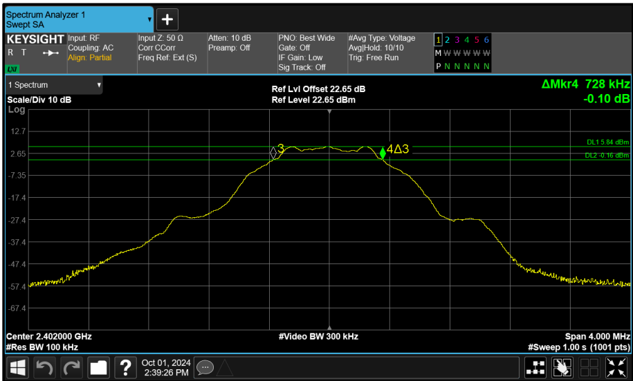
Figure 132 - Core 2 (A) 2402 MHz (CH37) 6 dB Bandwidth
