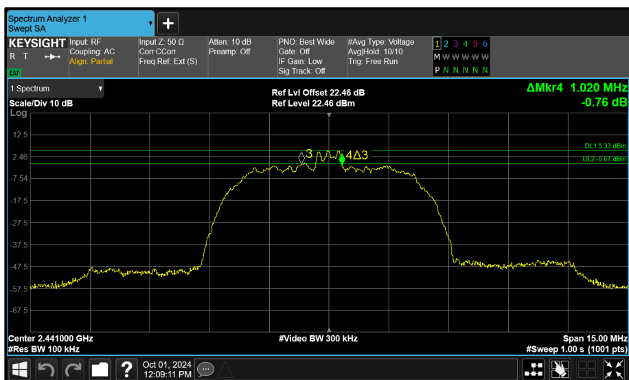
Figure 104 - Core 1 (B) 2441 MHz (CH39) 6 dB Bandwidth
