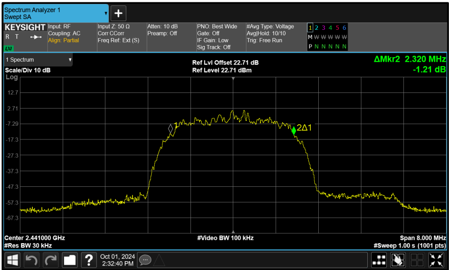
Figure 121 - Core 2 (A) 2441 MHz (CH39) 99% Bandwidth
