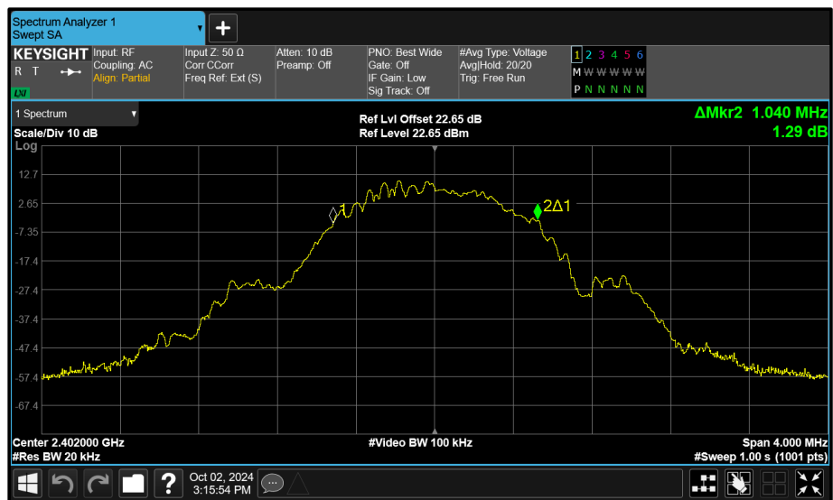
Figure 83 - Core 0 (A) 2402 MHz (CH37) 99% Bandwidth
