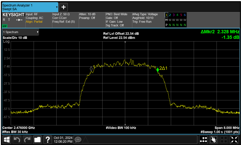
Figure 99 - Core 1 (B) 2476 MHz (CH74) 99% Bandwidth
