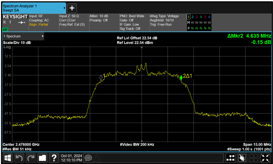
Figure 105 - Core 1 (B) 2476 MHz (CH74) 99% Bandwidth
