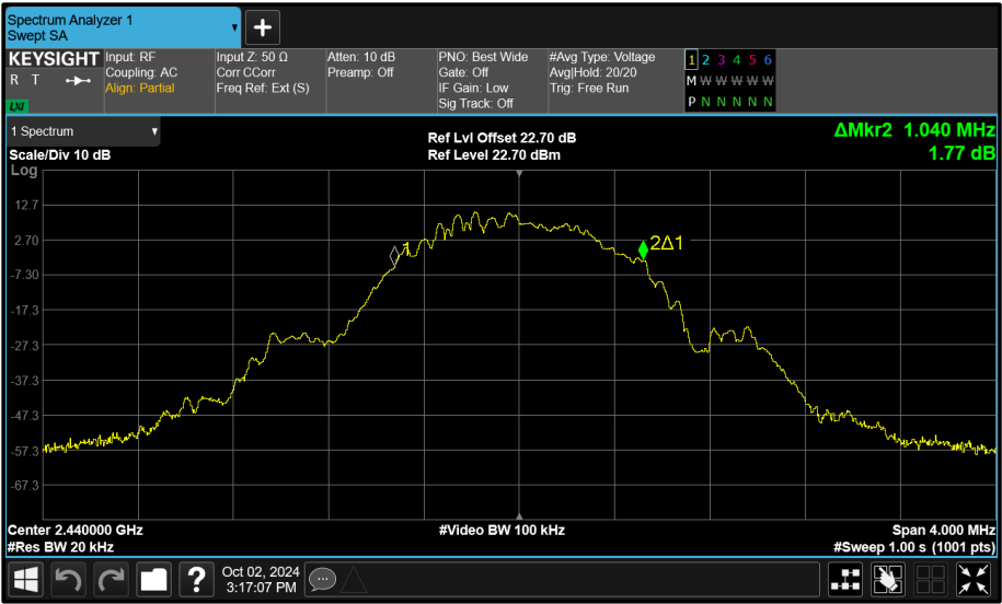
Figure 85 - Core 0 (A) 2440 MHz (CH17) 99% Bandwidth
