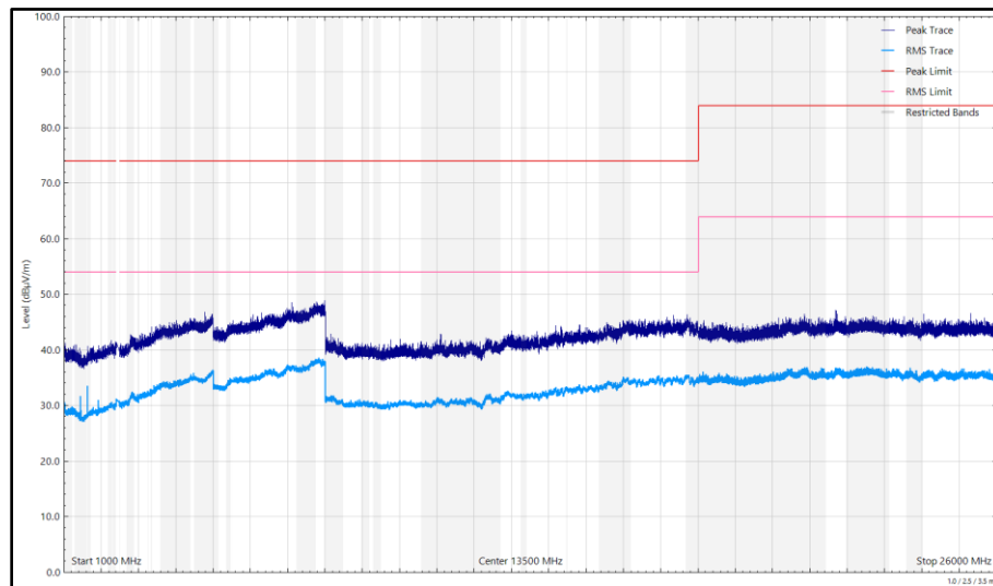
Figure 277 - 2440 MHz (CH17), LE1M, iPA, Core 2, 1 GHz to 26 GHz, Horizontal
