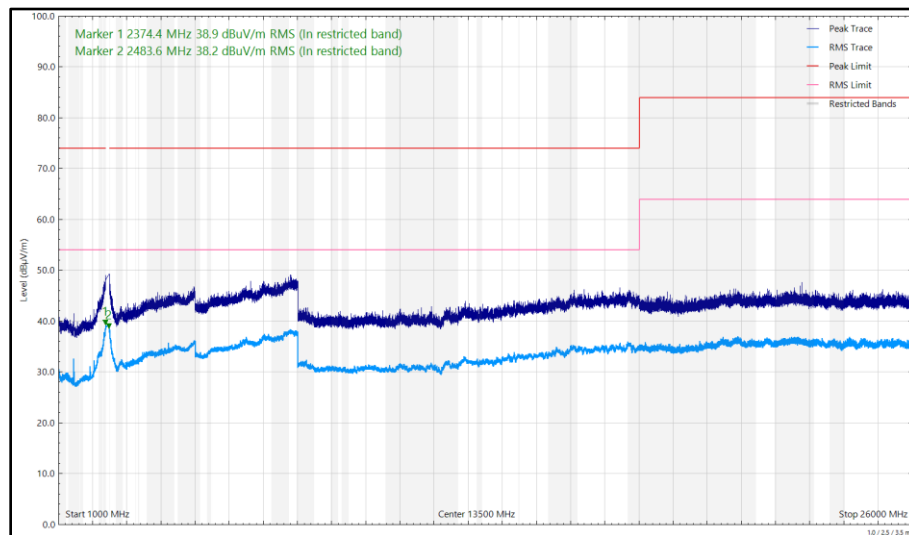
Figure 281 - 2404 MHz (CH37), HDR4, ePA, Core 0 + Core 1, 1 GHz to 26 GHz, Vertical
