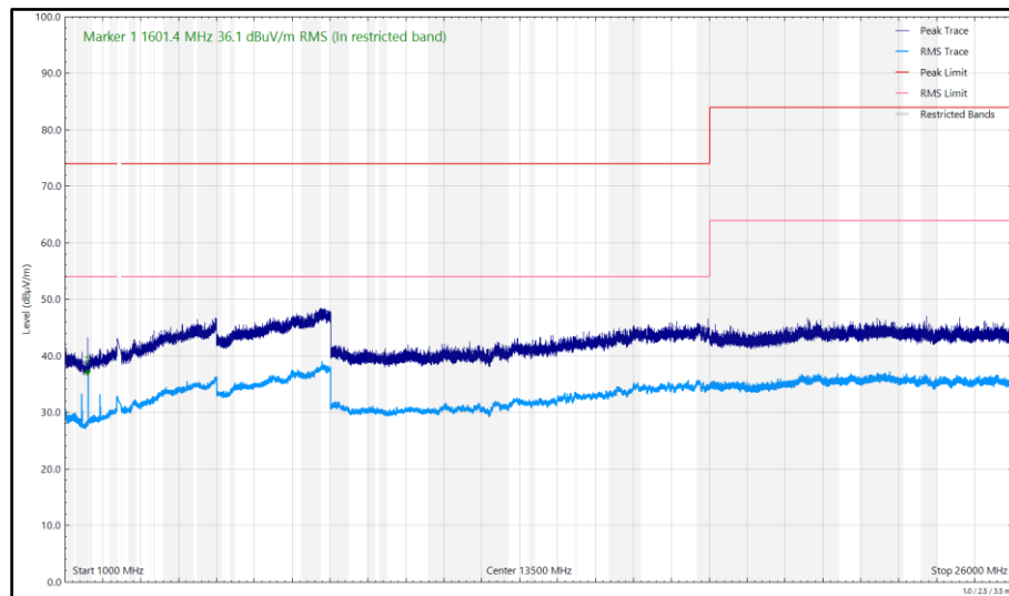
Figure 289 - 2402 MHz (CH37), LE1M, iPA, Core 2, 1 GHz to 26 GHz, Vertical
