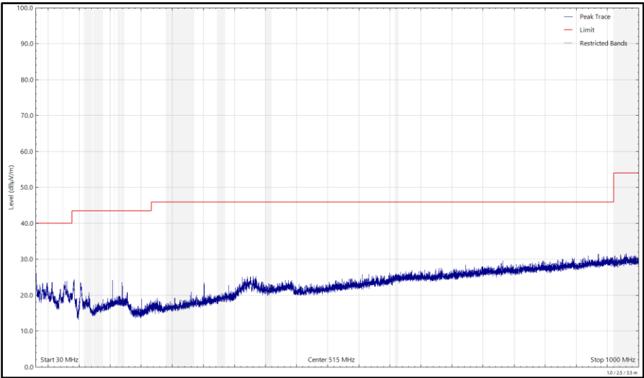
Figure 274 - 2440 MHz (CH17), LE1M, iPA, Core 0 + Core 1, 30 MHz to 1 GHz, Vertical (Peak)
