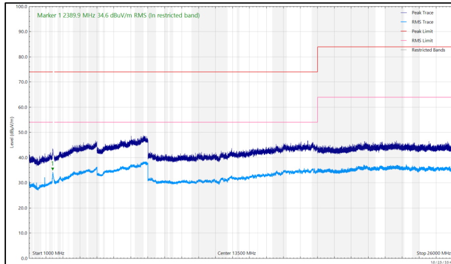
Figure 284 - 2402 MHz (CH37), LE1M, iPA, Core 0 + Core 1, 1 GHz to 26 GHz, Horizontal
