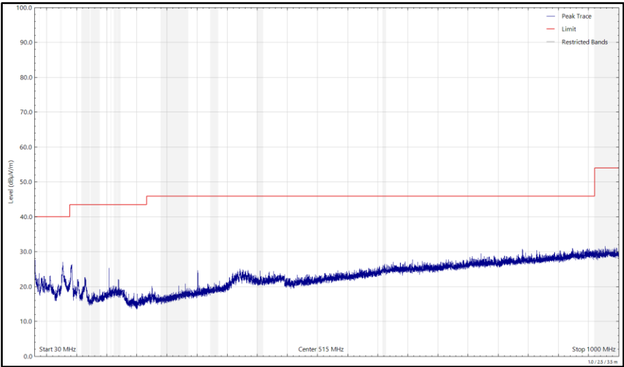
Figure 278 - 2440 MHz (CH17), LE1M, iPA, Core 2, 30 MHz to 1 GHz, Vertical (Peak)
