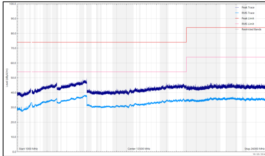
Figure 280 - 2404 MHz (CH37), HDR4, ePA, Core 0 + Core 1, 1 GHz to 26 GHz, Horizontal
