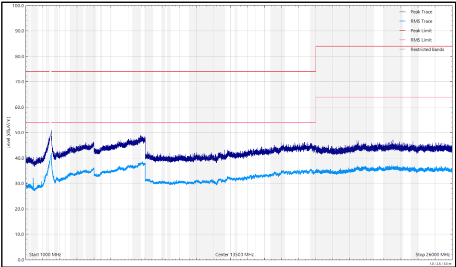
Figure 283 - 2476 MHz (CH39), HDR4, ePA, Core 0 + Core 1, 1 GHz to 26 GHz, Vertical
