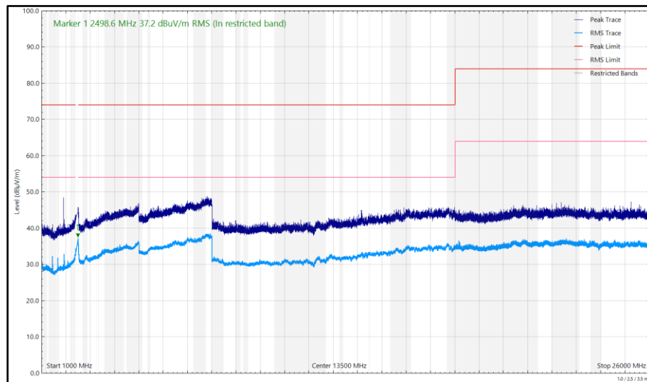
Figure 287 - 2480 MHz (CH39), LE1M, iPA, Core 0 + Core 1, 1 GHz to 26 GHz, Vertical
