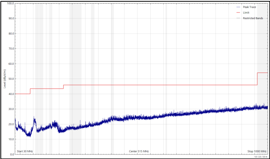
Figure 270 - 2440 MHz (CH17), HDR4, ePA, Core 0 + Core 1, 30 MHz to 1 GHz, Vertical (Peak)
