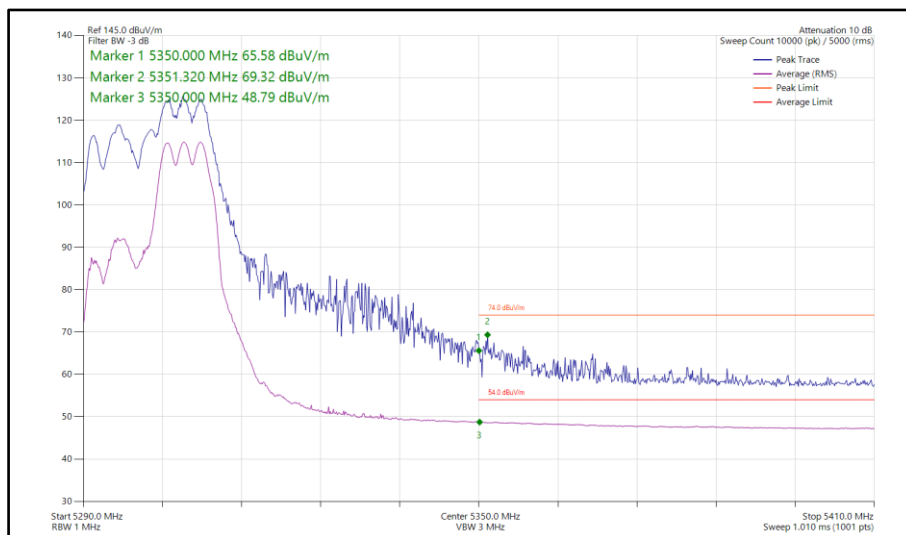
Figure 124 - 802.11ax HE20, RU 106-54, SDM, Core 0-1 - 5300 MHz Band Edge Frequency 5350 MHz
