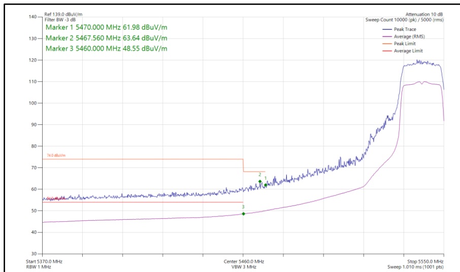
Figure 65 - 802.11n HT20, SISO, Core 1 - 5540 MHz Band Edge Frequency 5460 MHz
