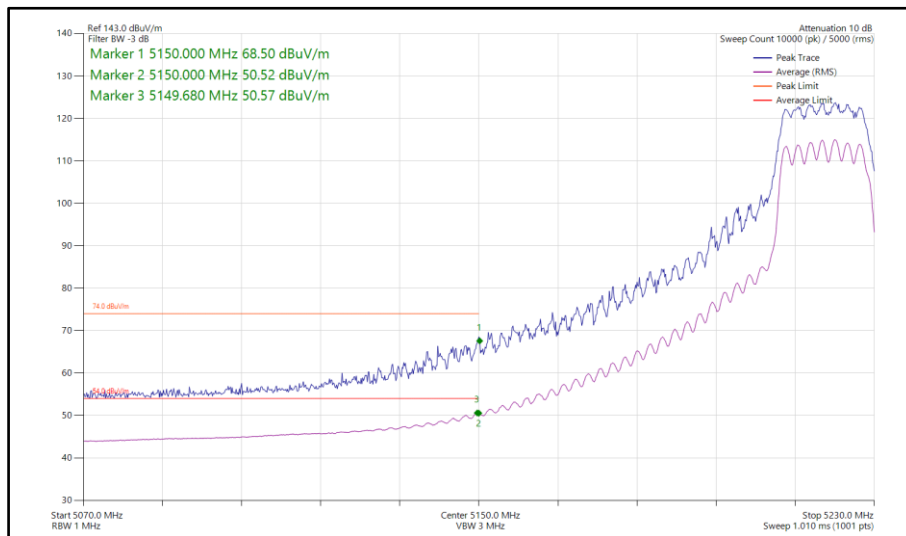
Figure 75 - 802.11n HT20, CDD, Core 0-1 - 5220 MHz Band Edge Frequency 5150 MHz
