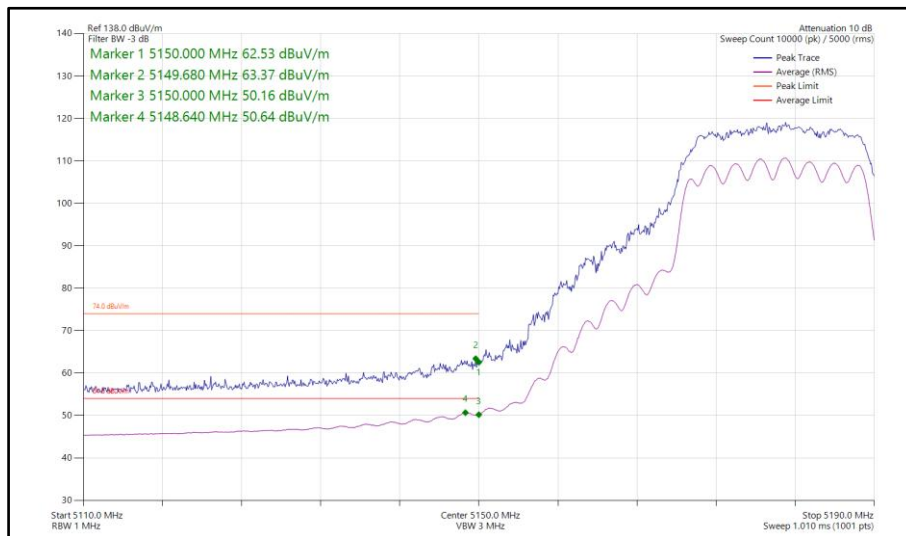
Figure 73 - 802.11n HT20, CDD, Core 0-1 - 5180 MHz Band Edge Frequency 5150 MHz
