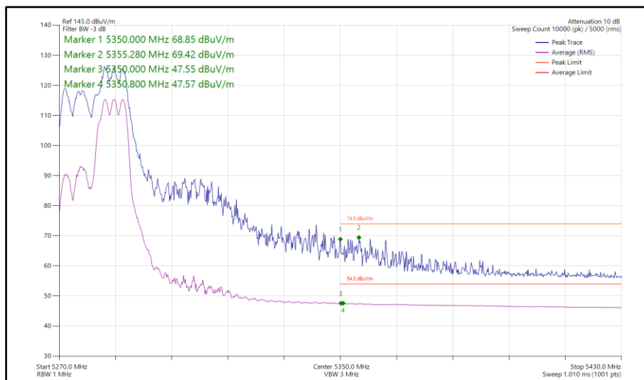
Figure 122 - 802.11ax HE20, RU 106-54, SDM, Core 0-1 - 5280 MHz Band Edge Frequency 5350 MHz
