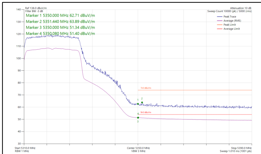
Figure 125 - 802.11ax HE20, SU, SDM, Core 0-1 - 5320 MHz Band Edge Frequency 5350 MHz
