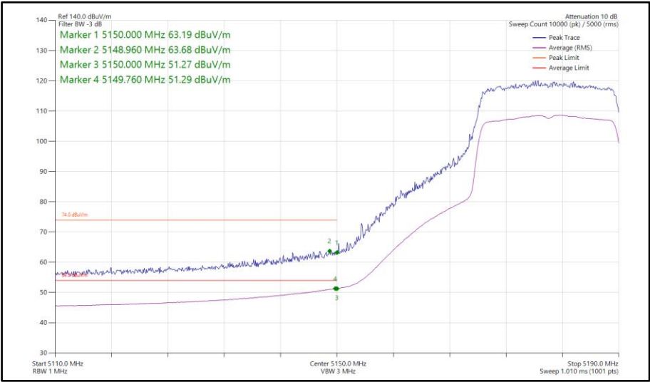
Figure 109 - 802.11ax HE20, SU, SDM, Core 0-1 - 5180 MHz Band Edge Frequency 5150 MHz
