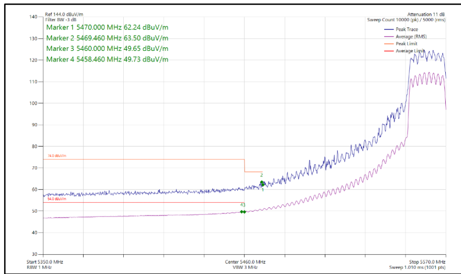
Figure 103 - 802.11ax HE20, SU, CDD, Core 0-1 - 5560 MHz Band Edge Frequency 5460 MHz
