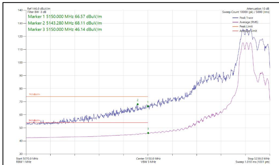
Figure 81 - 802.11ax HE20, RU 106-53, CDD, Core 0-1 - 5220 MHz Band Edge Frequency 5150 MHz
