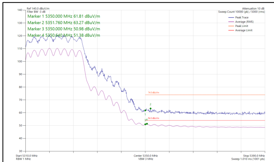
Figure 91 - 802.11ax HE20, SU, CDD, Core 0-1 - 5320 MHz Band Edge Frequency 5350 MHz
