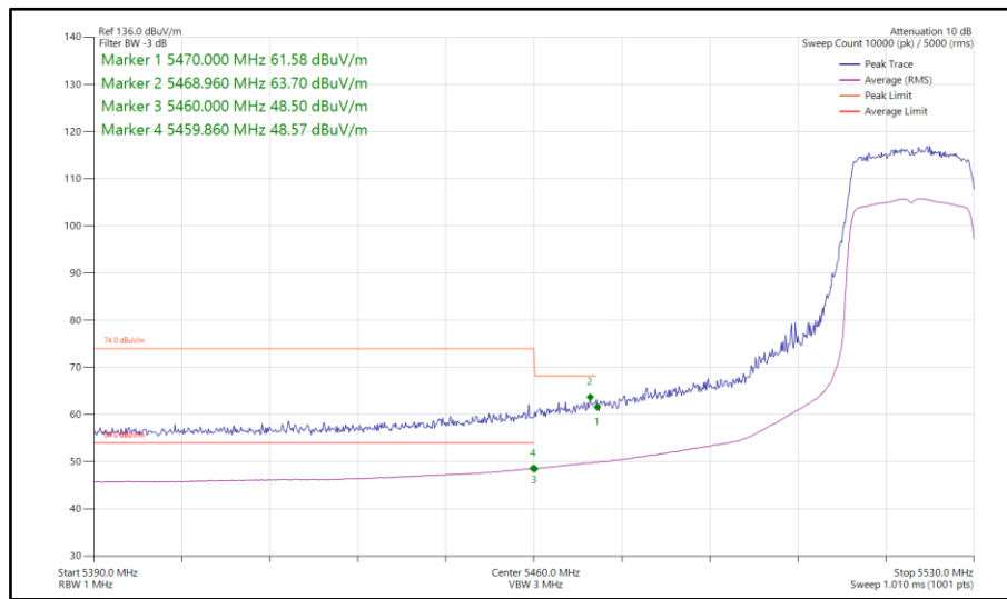
Figure 69 - 802.11ax HE20, SU, SISO, Core 1 - 5520 MHz Band Edge Frequency 5460 MHz
