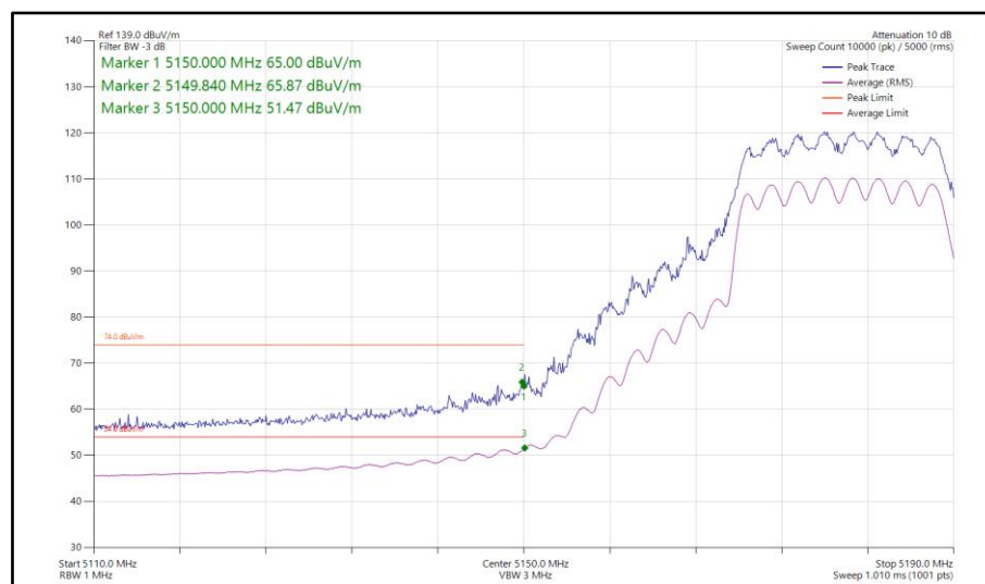
Figure 76 - 802.11ax HE20, SU, CDD, Core 0-1 - 5180 MHz Band Edge Frequency 5150 MHz
