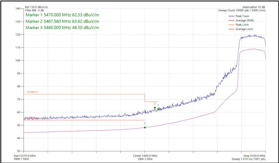
Figure 71 - 802.11ax HE20, SU, SISO, Core 1 - 5540 MHz Band Edge Frequency 5460 MHz
