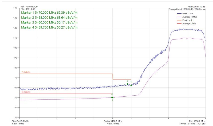
Figure 63 - 802.11n HT20, SISO, Core 1 - 5500 MHz Band Edge Frequency 5460 MHz
