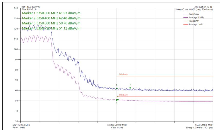
Figure 89 - 802.11ax HE20, SU, CDD, Core 0-1 - 5300 MHz Band Edge Frequency 5350 MHz
