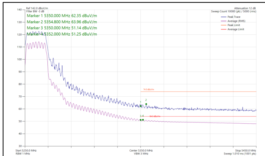
Figure 83 - 802.11n HT20, CDD, Core 0-1 - 5260 MHz Band Edge Frequency 5350 MHz
