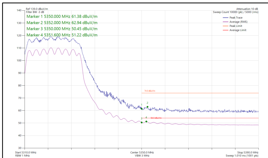
Figure 86 - 802.11n HT20, CDD, Core 0-1 - 5320 MHz Band Edge Frequency 5350 MHz
