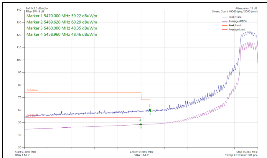
Figure 97 - 802.11n HT20, CDD, Core 0-1 - 5580 MHz Band Edge Frequency 5460 MHz
