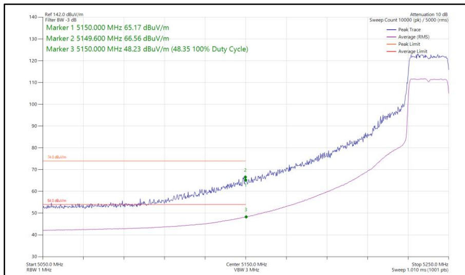
Figure 115 - 802.11ax HE20, SU, SDM, Core 0-1 - 5240 MHz Band Edge Frequency 5150 MHz
