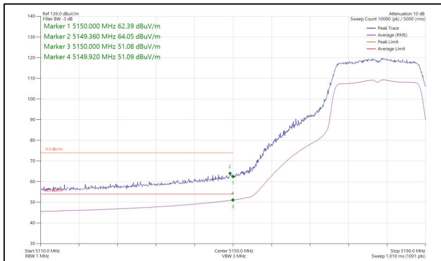
Figure 105 - 802.11n HT20, SDM, Core 0-1 - 5180 MHz Band Edge Frequency 5150 MHz
