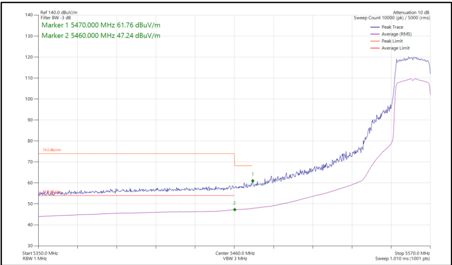
Figure 72 - 802.11ax HE20, SU, SISO, Core 1 - 5560 MHz Band Edge Frequency 5460 MHz
