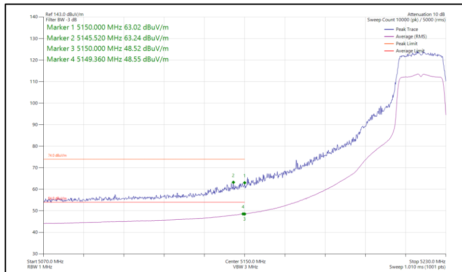
Figure 107 - 802.11n HT20, SDM, Core 0-1 - 5220 MHz Band Edge Frequency 5150 MHz
