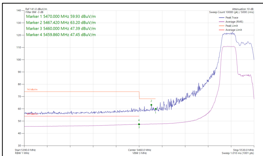
Figure 70 - 802.11ax HE20, RU 106-53, SISO, Core 1 - 5520 MHz Band Edge Frequency 5460 MHz
