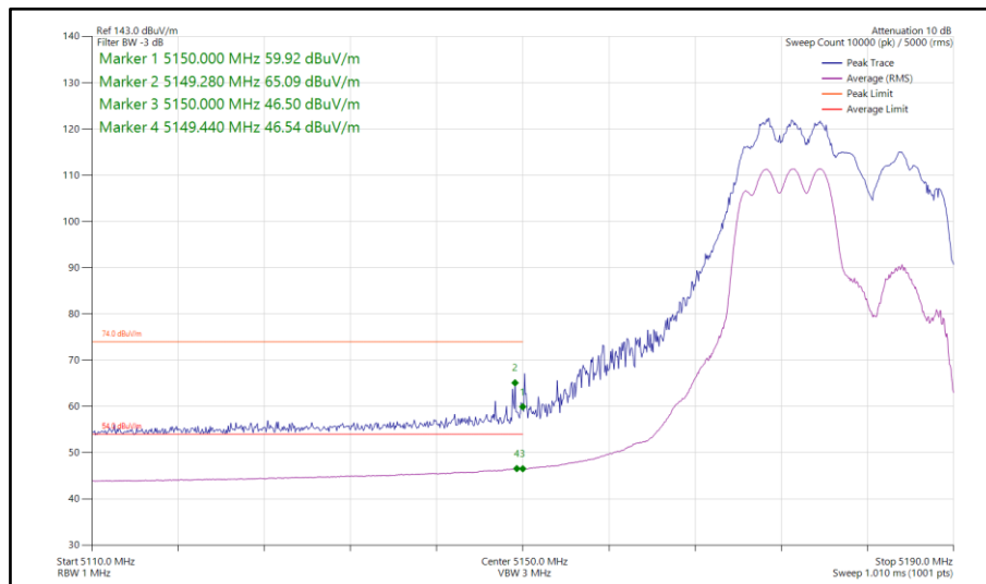
Figure 77 - 802.11ax HE20, RU 106-53, CDD, Core 0-1 - 5180 MHz Band Edge Frequency 5150 MHz
