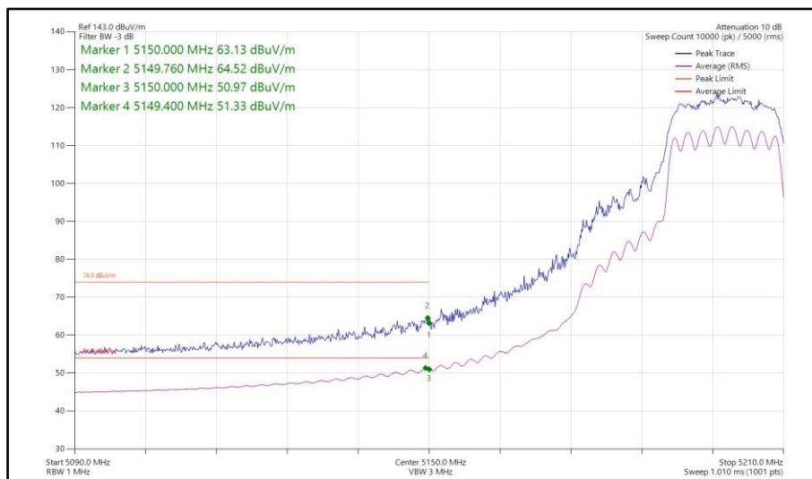
Figure 74 - 802.11n HT20, CDD, Core 0-1 - 5200 MHz Band Edge Frequency 5150 MHz
