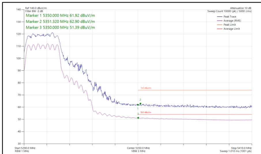
Figure 85 - 802.11n HT20, CDD, Core 0-1 - 5300 MHz Band Edge Frequency 5350 MHz
