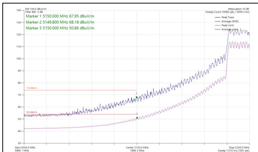
Figure 82 - 802.11ax HE20, SU, CDD, Core 0-1 - 5240 MHz Band Edge Frequency 5150 MHz
