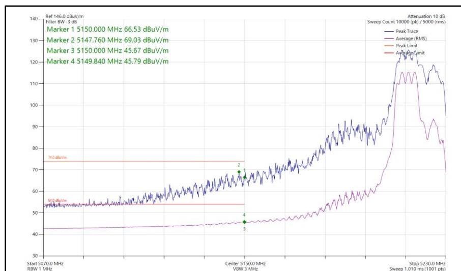
Figure 114 - 802.11ax HE20, RU 106-53, SDM, Core 0-1 - 5220 MHz Band Edge Frequency 5150 MHz
