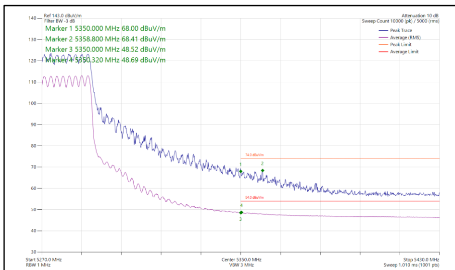
Figure 88 - 802.11ax HE20, SU, CDD, Core 0-1 - 5280 MHz Band Edge Frequency 5350 MHz
