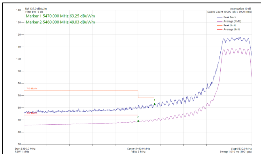
Figure 94 - 802.11n HT20, CDD, Core 0-1 - 5520 MHz Band Edge Frequency 5460 MHz
