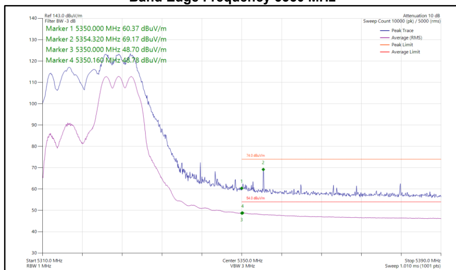
Figure 92 - 802.11ax HE20, RU 106-54, CDD, Core 0-1 - 5320 MHz Band Edge Frequency 5350 MHz
