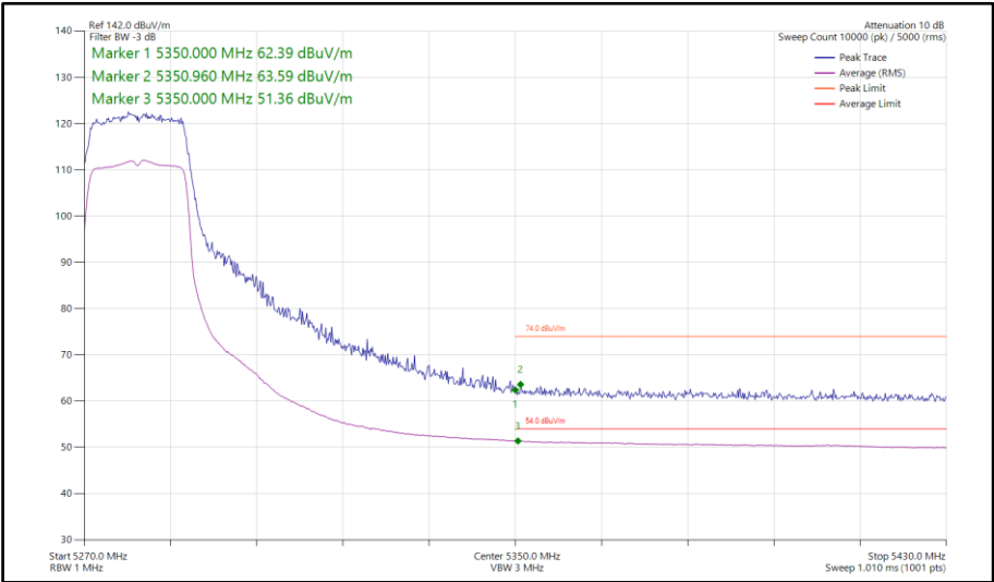
Figure 117 - 802.11n HT20, SDM, Core 0-1 - 5280 MHz Band Edge Frequency 5350 MHz
