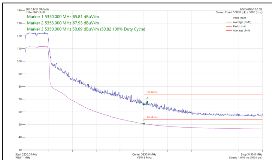
Figure 120 - 802.11ax HE20, SU, SDM, Core 0-1 - 5260 MHz Band Edge Frequency 5350 MHz
