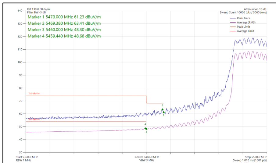
Figure 100 - 802.11ax HE20, SU, CDD, Core 0-1 - 5520 MHz Band Edge Frequency 5460 MHz
