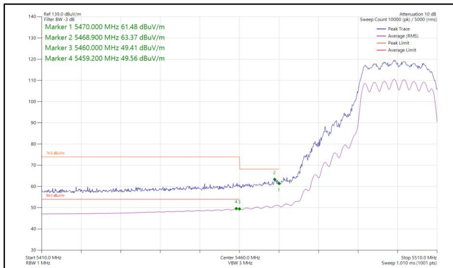
Figure 93 - 802.11n HT20, CDD, Core 0-1 - 5500 MHz Band Edge Frequency 5460 MHz
