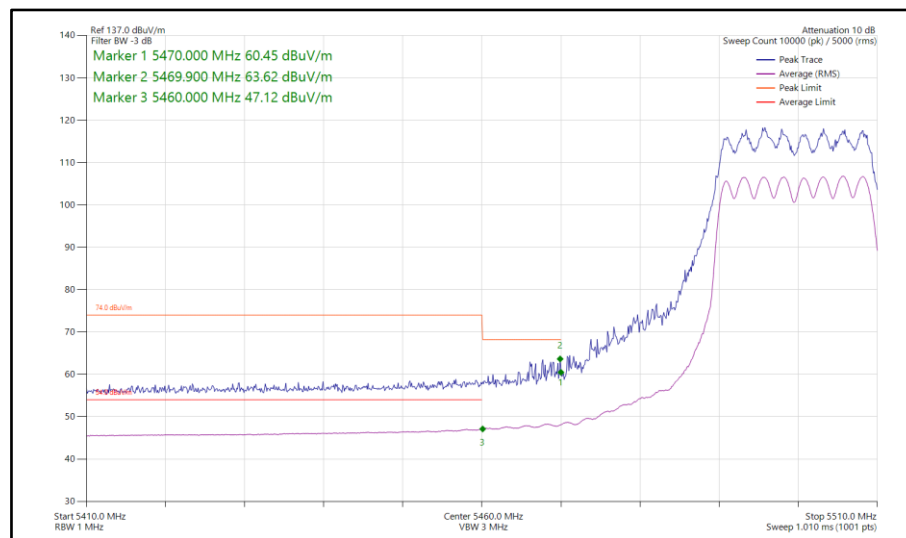
Figure 98 - 802.11ax HE20, SU, CDD, Core 0-1 - 5500 MHz Band Edge Frequency 5460 MHz
