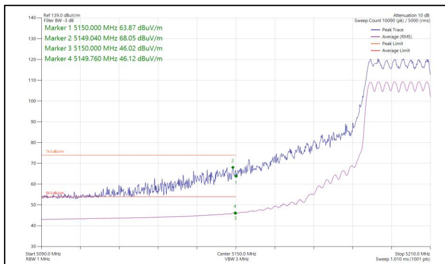
Figure 78 - 802.11ax HE20, SU, CDD, Core 0-1 - 5200 MHz Band Edge Frequency 5150 MHz
