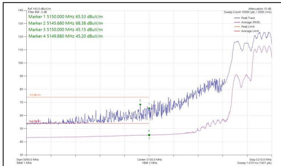
Figure 79 - 802.11ax HE20, RU 106-54, CDD, Core 0-1 - 5200 MHz Band Edge Frequency 5150 MHz
