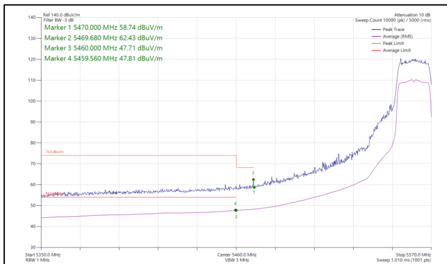
Figure 66 - 802.11n HT20, SISO, Core 1 - 5560 MHz Band Edge Frequency 5460 MHz
