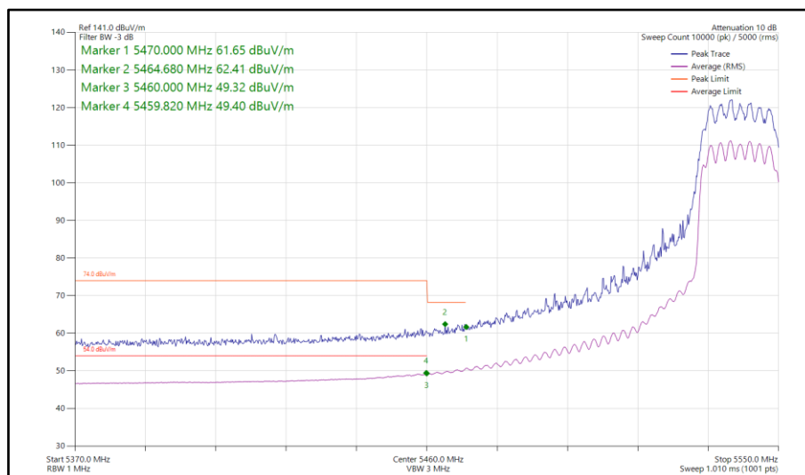
Figure 102 - 802.11ax HE20, SU, CDD, Core 0-1 - 5540 MHz Band Edge Frequency 5460 MHz
