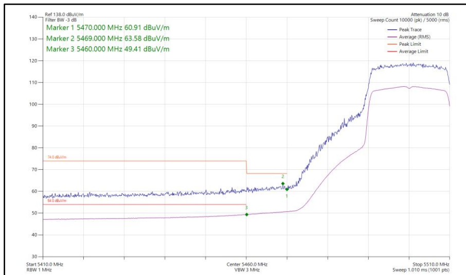
Figure 67 - 802.11ax HE20, SU, SISO, Core 1 - 5500 MHz Band Edge Frequency 5460 MHz
