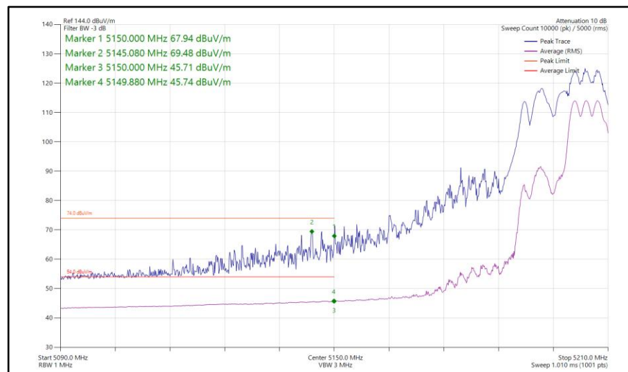
Figure 112 - 802.11ax HE20, RU 106-54, SDM, Core 0-1 - 5200 MHz Band Edge Frequency 5150 MHz
