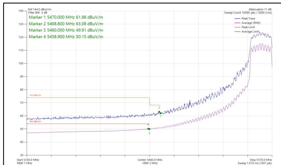
Figure 96 - 802.11n HT20, CDD, Core 0-1 - 5560 MHz Band Edge Frequency 5460 MHz
