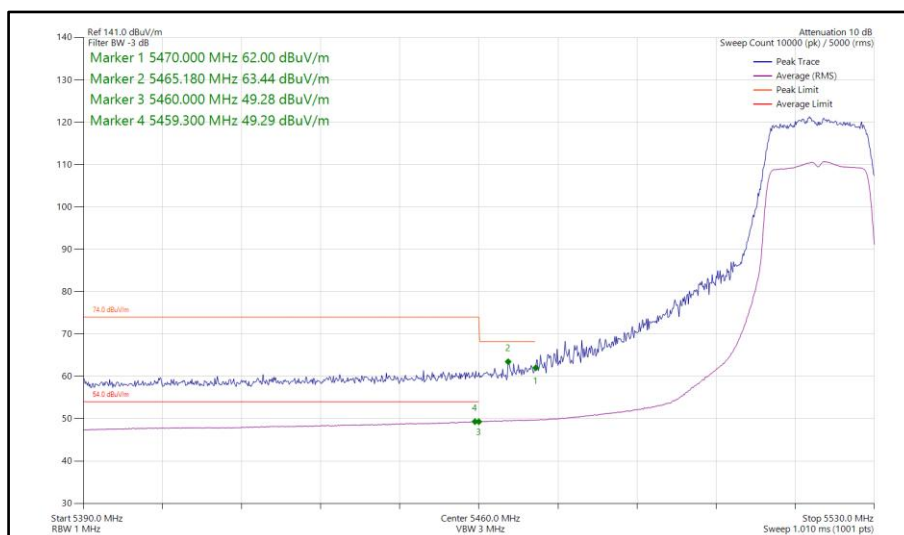
Figure 128 - 802.11n HT20, SDM, Core 0-1 - 5520 MHz Band Edge Frequency 5460 MHz
