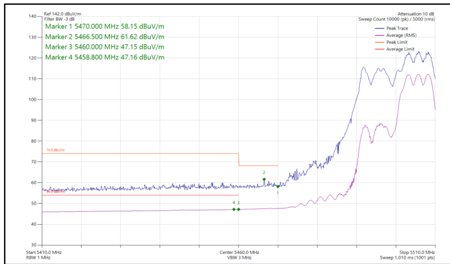
Figure 99 - 802.11ax HE20, RU 106-54, CDD, Core 0-1 - 5500 MHz Band Edge Frequency 5460 MHz
