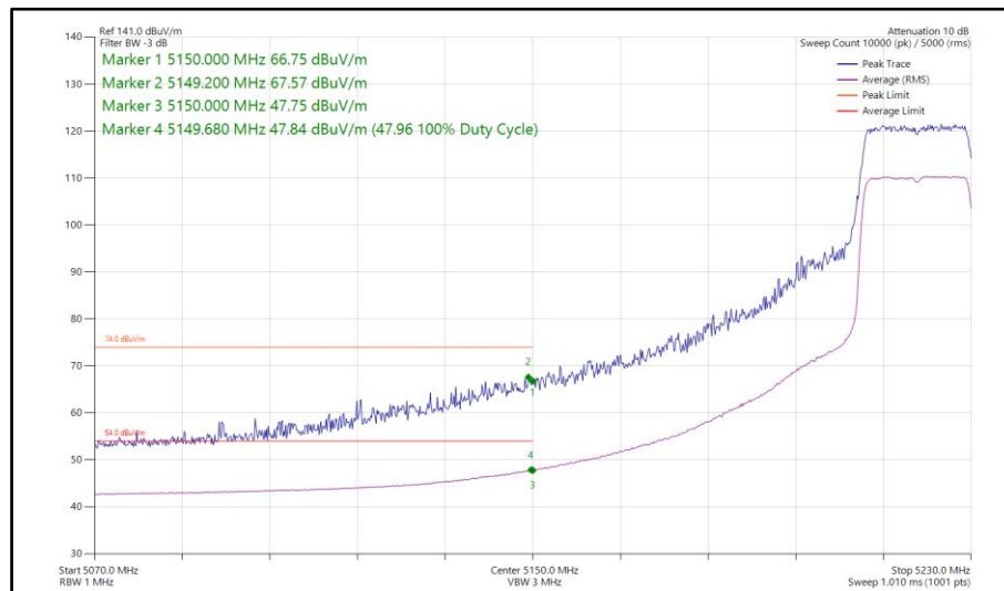
Figure 113 - 802.11ax HE20, SU, SDM, Core 0-1 - 5220 MHz Band Edge Frequency 5150 MHz
