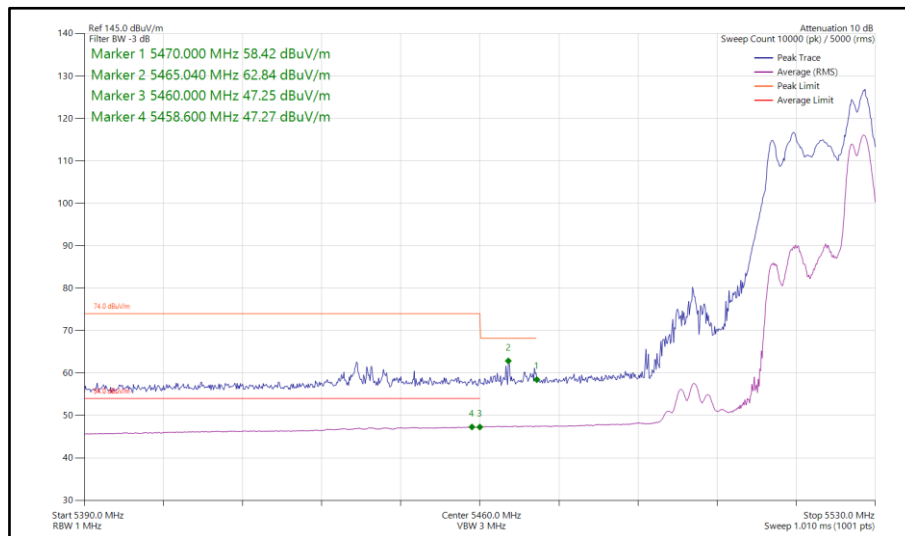
Figure 101 - 802.11ax HE20, RU 52-40, CDD, Core 0-1 - 5520 MHz Band Edge Frequency 5460 MHz
