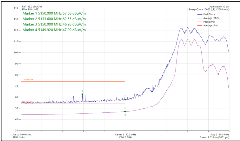
Figure 110 - 802.11ax HE20, RU 106-53, SDM, Core 0-1 - 5180 MHz Band Edge Frequency 5150 MHz
