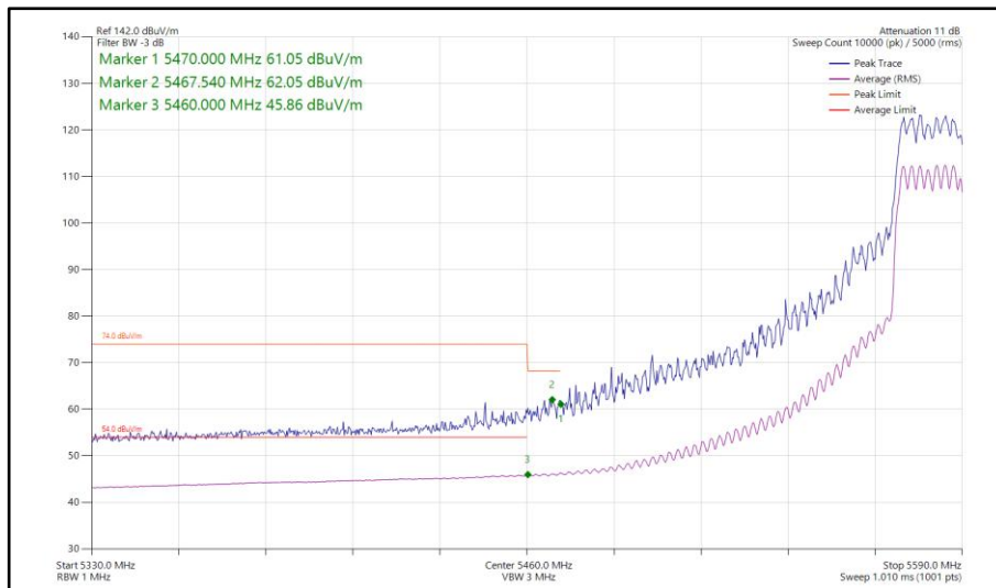
Figure 104 - 802.11ax HE20, SU, CDD, Core 0-1 - 5580 MHz Band Edge Frequency 5460 MHz
