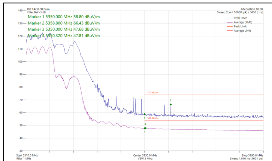
Figure 126 - 802.11ax HE20, RU 106-53, SDM, Core 0-1 - 5320 MHz Band Edge Frequency 5350 MHz
