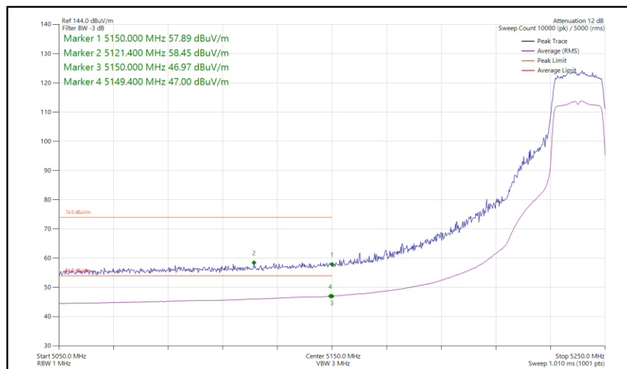
Figure 108 - 802.11n HT20, SDM, Core 0-1 - 5240 MHz Band Edge Frequency 5150 MHz
