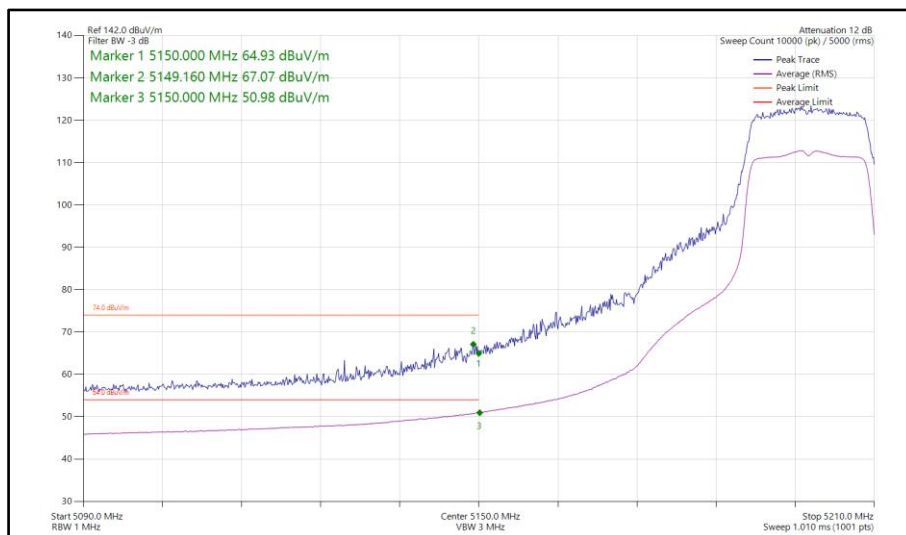
Figure 106 - 802.11n HT20, SDM, Core 0-1 - 5200 MHz Band Edge Frequency 5150 MHz
