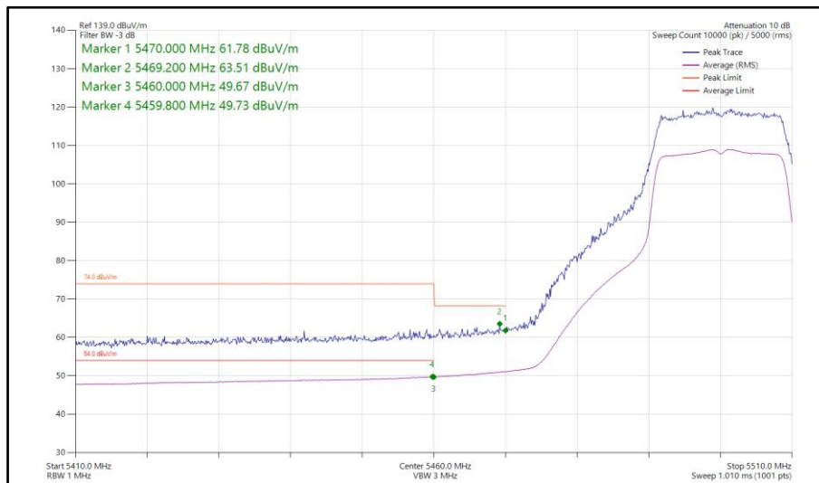
Figure 127 - 802.11n HT20, SDM, Core 0-1 - 5500 MHz Band Edge Frequency 5460 MHz
