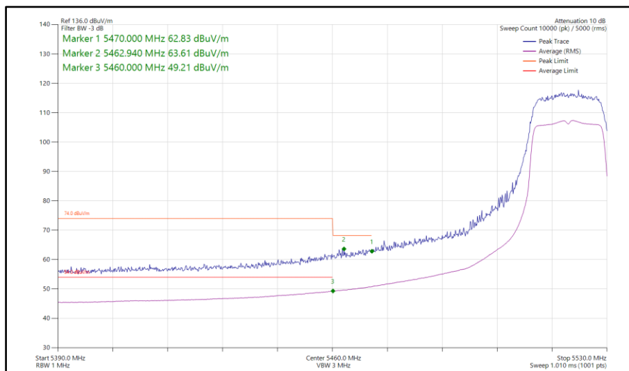
Figure 64 - 802.11n HT20, SISO, Core 1 - 5520 MHz Band Edge Frequency 5460 MHz
