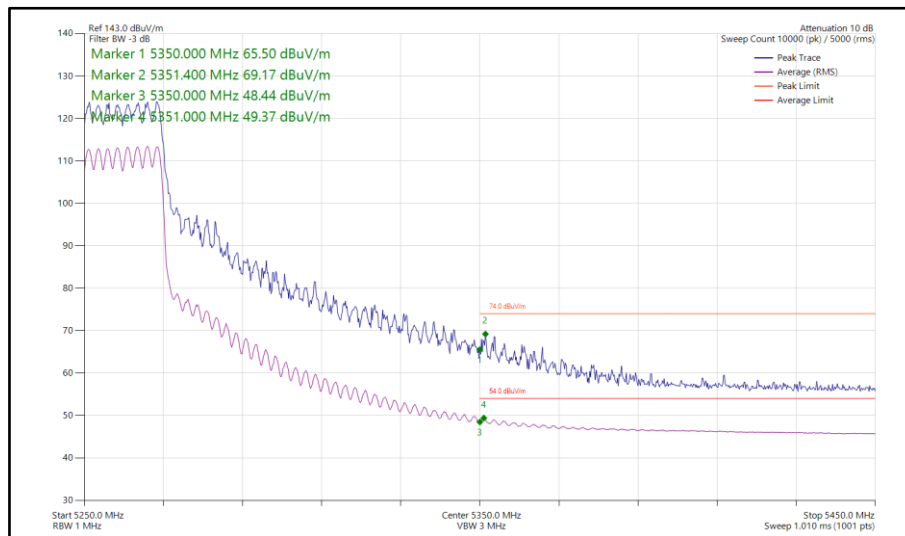
Figure 87 - 802.11ax HE20, SU, CDD, Core 0-1 - 5260 MHz Band Edge Frequency 5350 MHz
