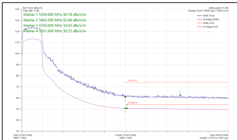
Figure 116 - 802.11n HT20, SDM, Core 0-1 - 5260 MHz Band Edge Frequency 5350 MHz
