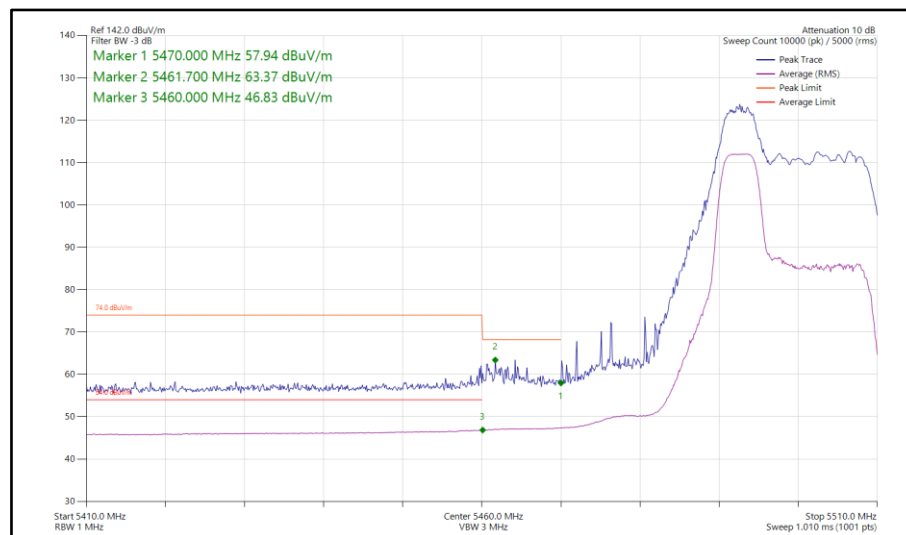
Figure 68 - 802.11ax HE20, RU 52-37, SISO, Core 1 - 5500 MHz Band Edge Frequency 5460 MHz
