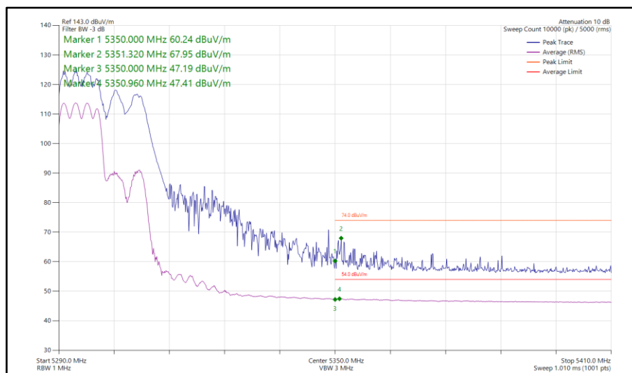
Figure 90 - 802.11ax HE20, RU 106-53, CDD, Core 0-1 - 5300 MHz Band Edge Frequency 5350 MHz
