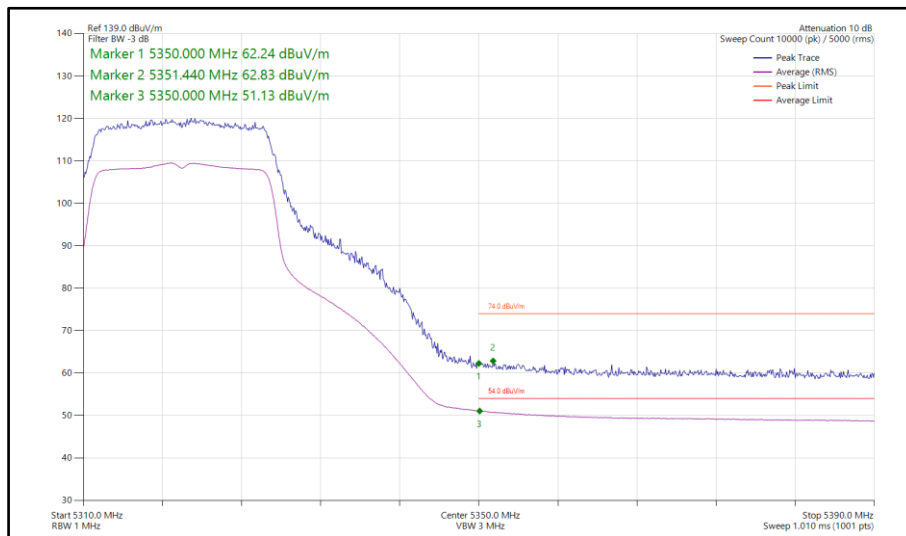
Figure 119 - 802.11n HT20, SDM, Core 0-1 - 5320 MHz Band Edge Frequency 5350 MHz
