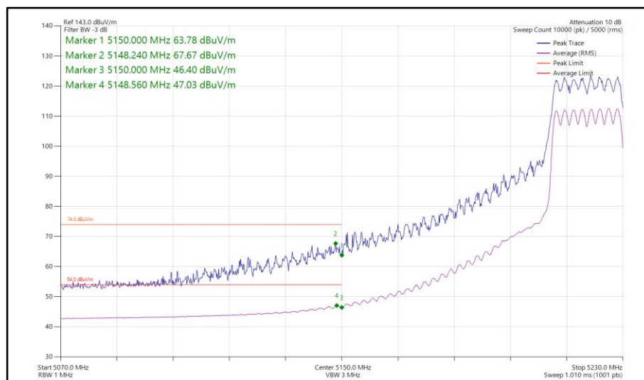
Figure 80 - 802.11ax HE20, SU, CDD, Core 0-1 - 5220 MHz Band Edge Frequency 5150 MHz
