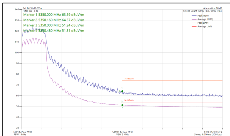
Figure 84 - 802.11n HT20, CDD, Core 0-1 - 5280 MHz Band Edge Frequency 5350 MHz
