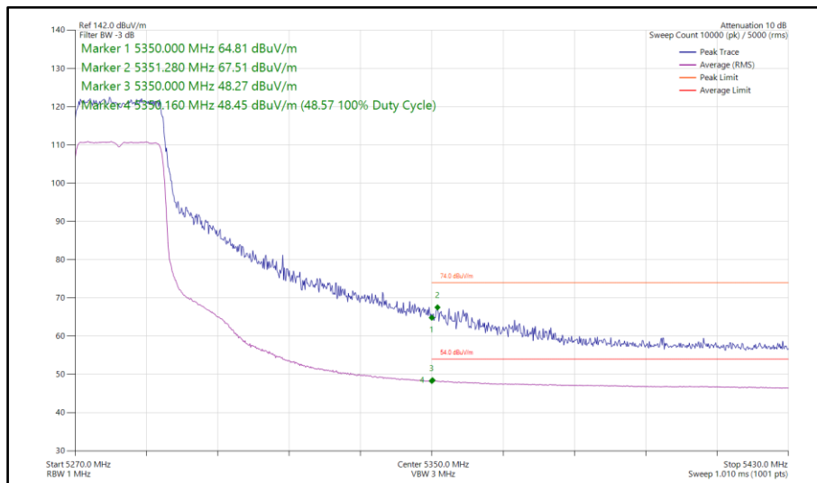
Figure 121 - 802.11ax HE20, SU, SDM, Core 0-1 - 5280 MHz Band Edge Frequency 5350 MHz
