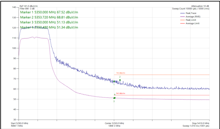
Figure 118 - 802.11n HT20, SDM, Core 0-1 - 5300 MHz Band Edge Frequency 5350 MHz
