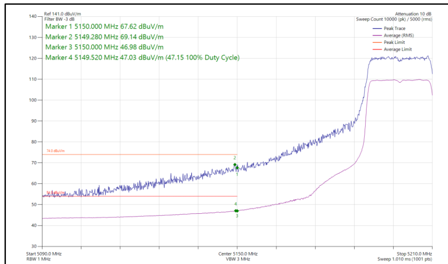
Figure 111 - 802.11ax HE20, SU, SDM, Core 0-1 - 5200 MHz Band Edge Frequency 5150 MHz
