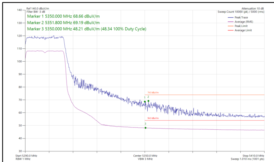
Figure 123 - 802.11ax HE20, SU, SDM, Core 0-1 - 5300 MHz Band Edge Frequency 5350 MHz
