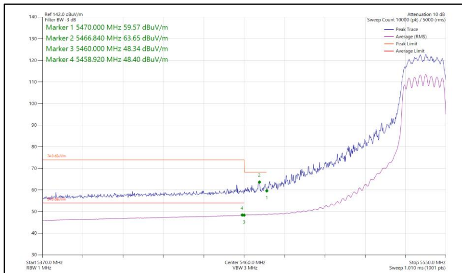
Figure 95 - 802.11n HT20, CDD, Core 0-1 - 5540 MHz Band Edge Frequency 5460 MHz
