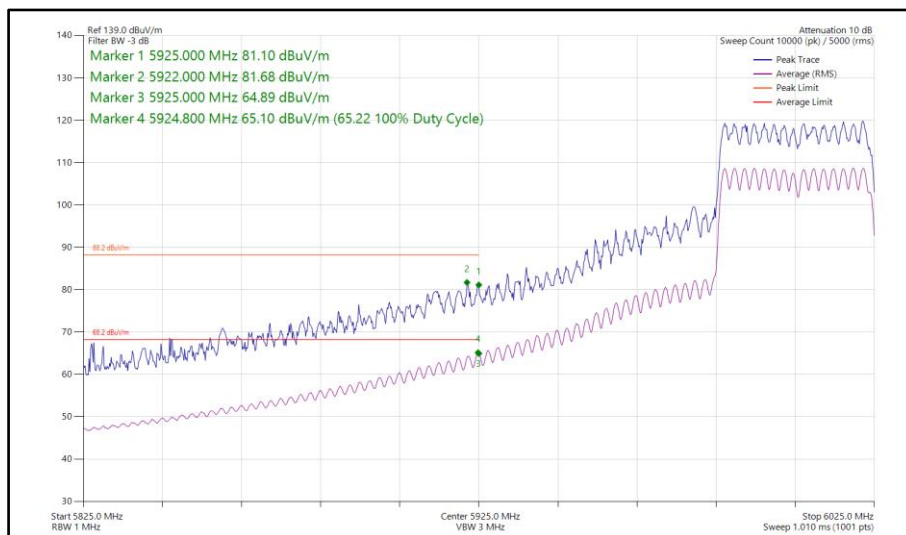
Figure 215 - 802.11ax HE40, SU, SDM, Core 0-1 - 6005 MHz Band Edge Frequency 5925 MHz
