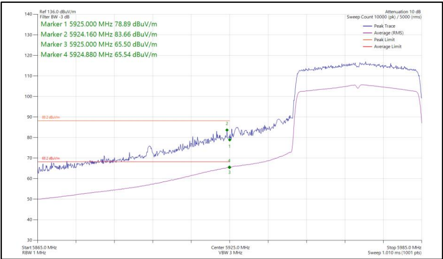
Figure 194 - 802.11ax HE40, SU, SISO, Core 0 - 5965 MHz Band Edge Frequency 5925 MHz
