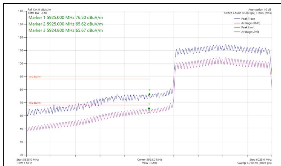
Figure 238 - 802.11ax HE80, SU, SDM, Core 0-1 - 5985 MHz Band Edge Frequency 5925 MHz
