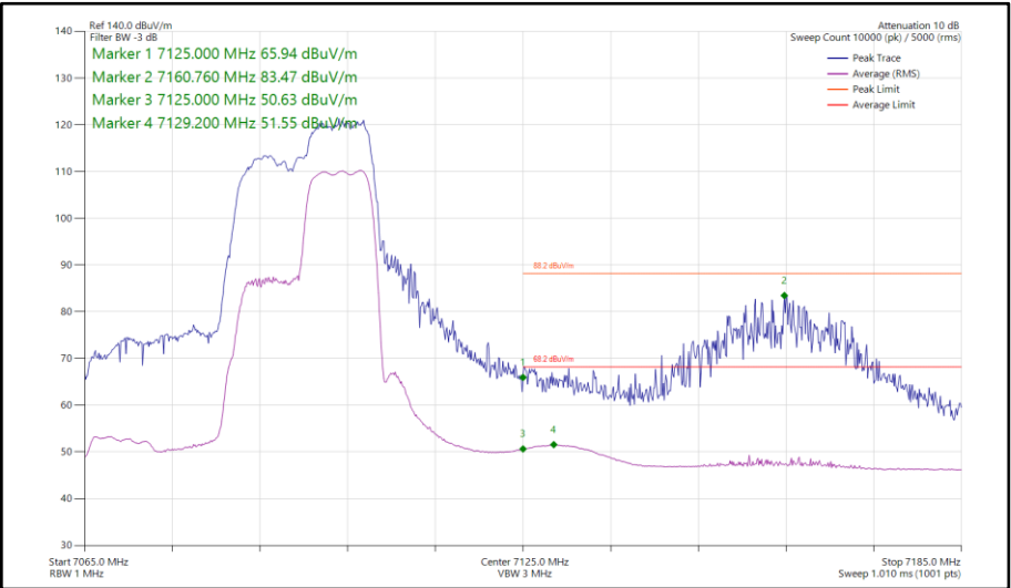
Figure 218 - 802.11ax HE40, RU 106-56, SDM, Core 0-1 - 7085 MHz Band Edge Frequency 7125 MHz
