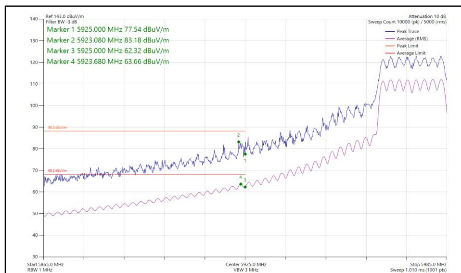
Figure 176 - 802.11ax HE20, SU, CDD, Core 0-1 - 5975 MHz Band Edge Frequency 5925 MHz
