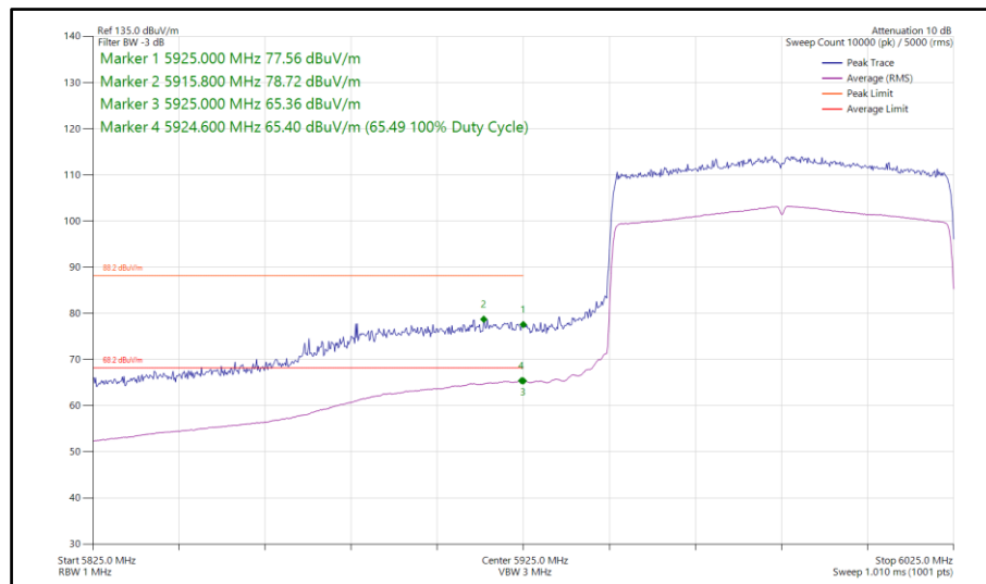
Figure 225 - 802.11ax HE80, SU, SISO, Core 1 - 5985 MHz Band Edge Frequency 5925 MHz
