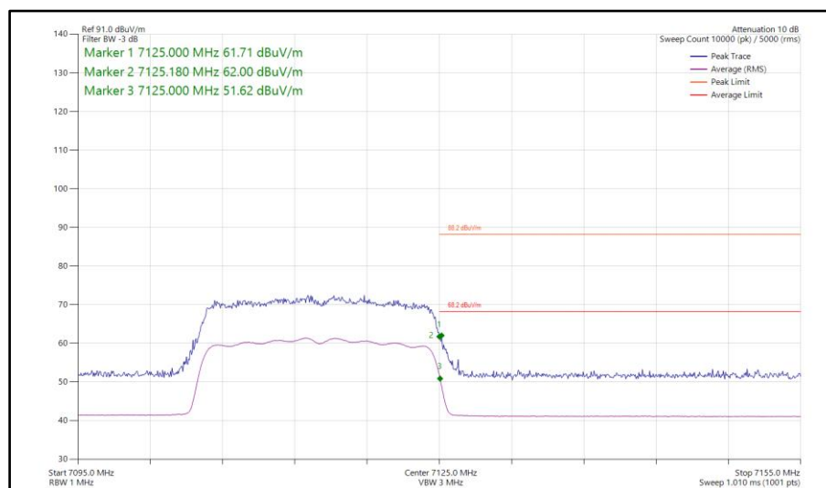
Figure 182 - 802.11ax HE20, SU, CDD, Core 0-1 - 7115 MHz Band Edge Frequency 7125 MHz
