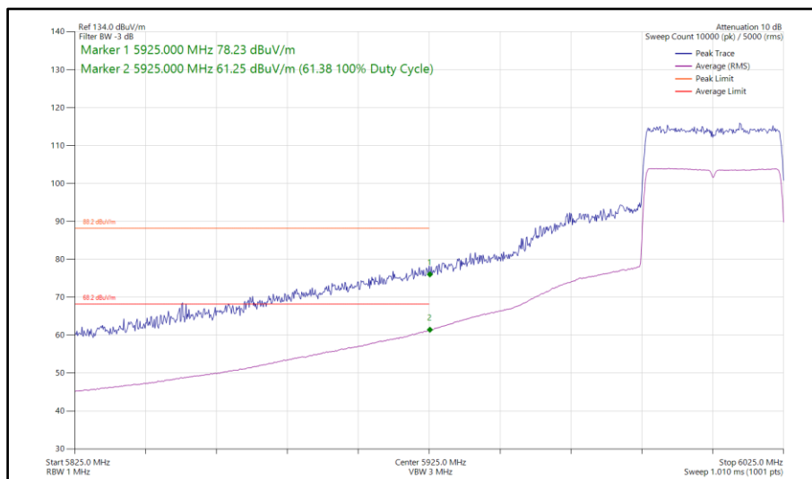
Figure 196 - 802.11ax HE40, SU, SISO, Core 0 - 6005 MHz Band Edge Frequency 5925 MHz
