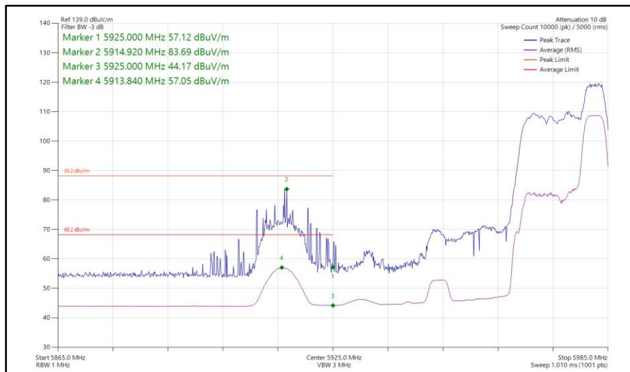
Figure 195 - 802.11ax HE40, RU 52-44, SISO, Core 0 - 5965 MHz Band Edge Frequency 5925 MHz
