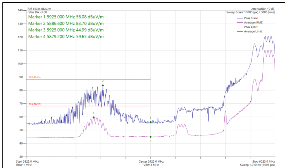
Figure 232 - 802.11ax HE80, RU 106-60, CDD, Core 0-1 - 5985 MHz Band Edge Frequency 5925 MHz
