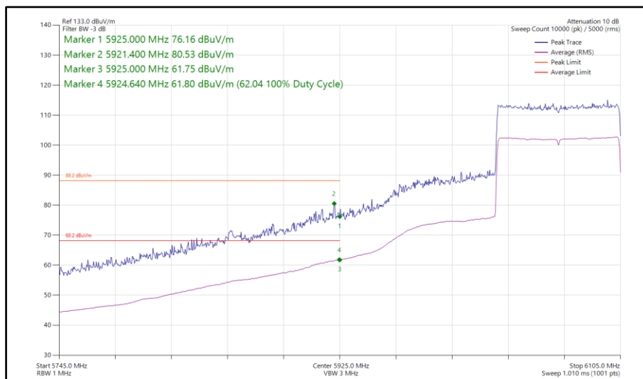
Figure 227 - 802.11ax HE80, SU, SISO, Core 1 - 6065 MHz Band Edge Frequency 5925 MHz
