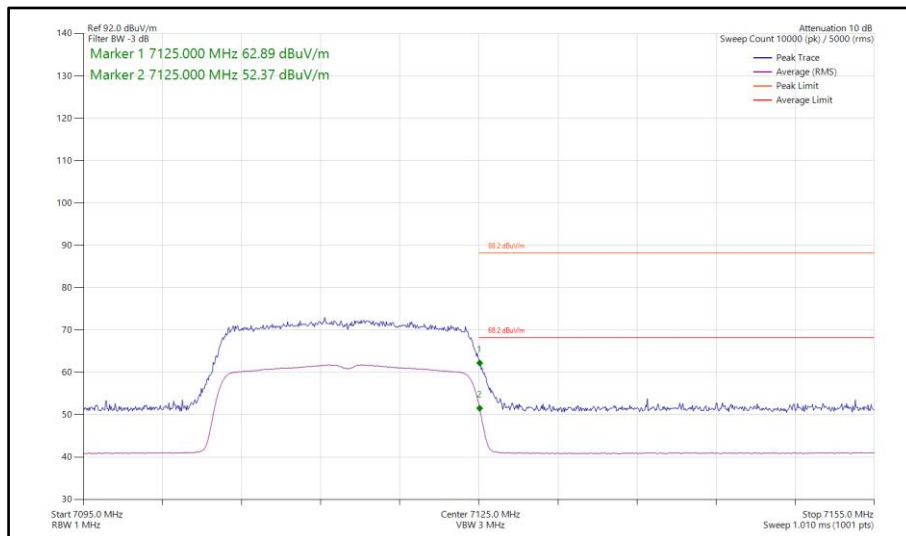
Figure 172 - 802.11ax HE20, SU, SISO, Core 1 - 7115 MHz Band Edge Frequency 7125 MHz
