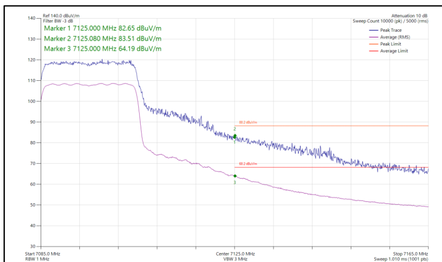
Figure 180 - 802.11ax HE20, SU, CDD, Core 0-1 - 7095 MHz Band Edge Frequency 7125 MHz
