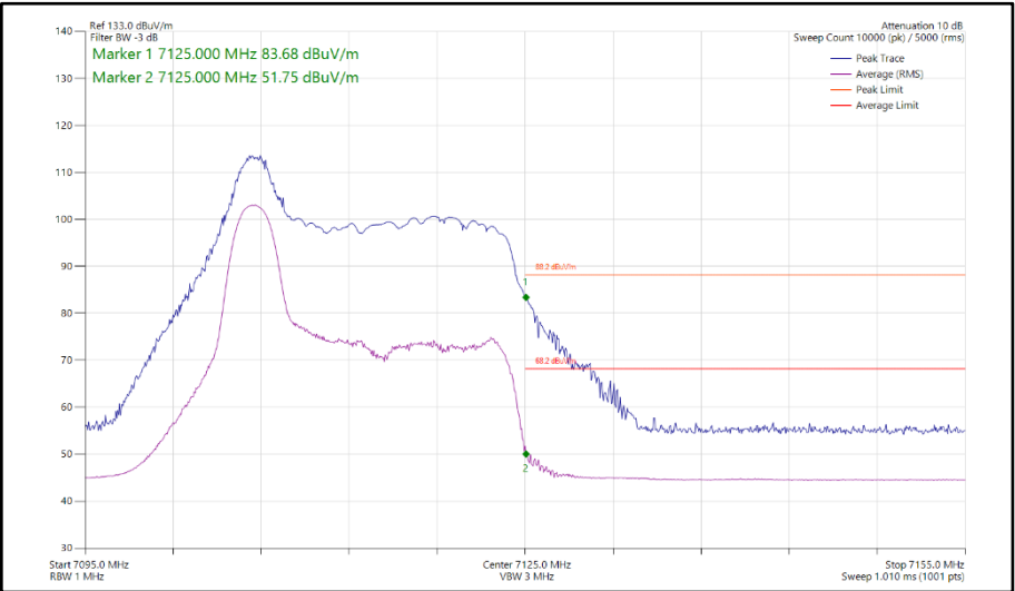
Figure 183 - 802.11ax HE20, RU 26-0, CDD, Core 0-1 - 7115 MHz Band Edge Frequency 7125 MHz
