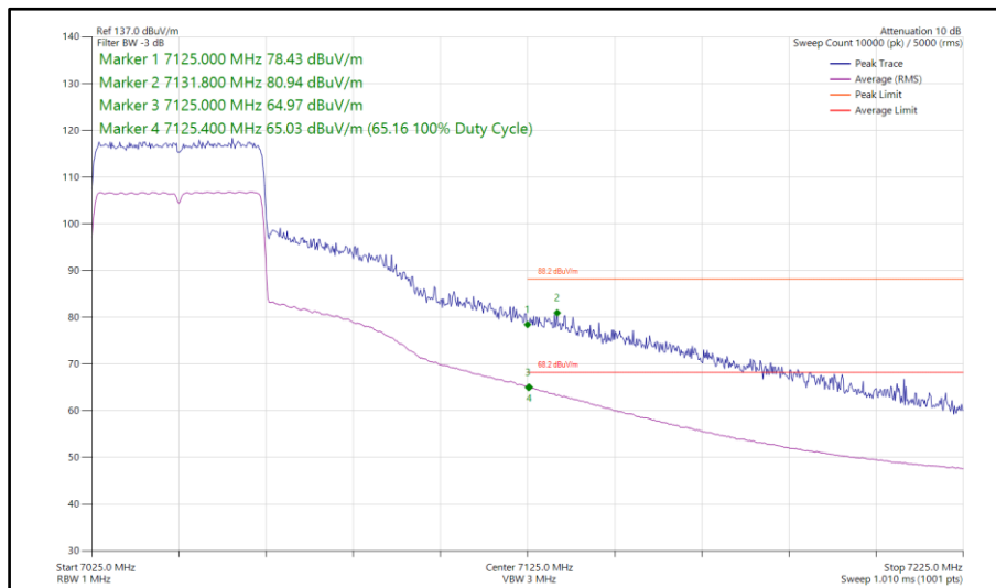
Figure 216 - 802.11ax HE40, SU, SDM, Core 0-1 - 7045 MHz Band Edge Frequency 7125 MHz
