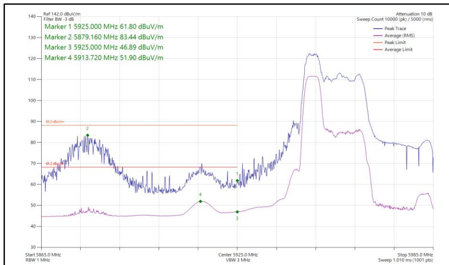
Figure 201 - 802.11ax HE40, RU 52-37, SISO, Core 1 - 5965 MHz Band Edge Frequency 5925 MHz
