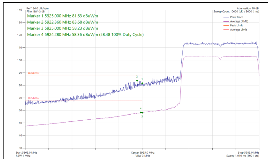
Figure 200 - 802.11ax HE40, SU, SISO, Core 1 - 5965 MHz Band Edge Frequency 5925 MHz
