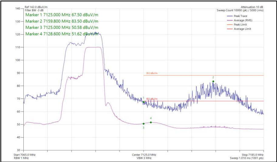
Figure 205 - 802.11ax HE40, RU 106-56, SISO, Core 1 - 7085 MHz Band Edge Frequency 7125 MHz
