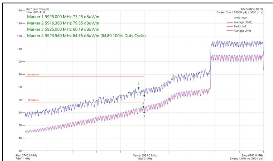
Figure 233 - 802.11ax HE80, SU, CDD, Core 0-1 - 6065 MHz Band Edge Frequency 5925 MHz
