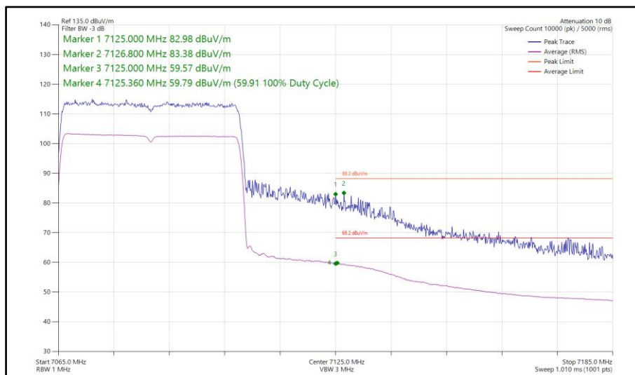
Figure 198 - 802.11ax HE40, SU, SISO, Core 0 - 7085 MHz Band Edge Frequency 7125 MHz
