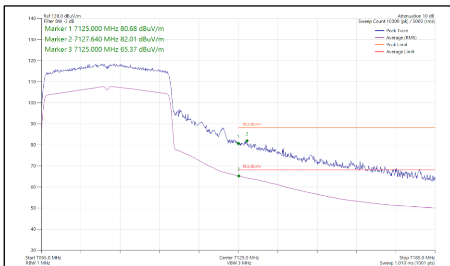
Figure 204 - 802.11ax HE40, SU, SISO, Core 1 - 7085 MHz Band Edge Frequency 7125 MHz
