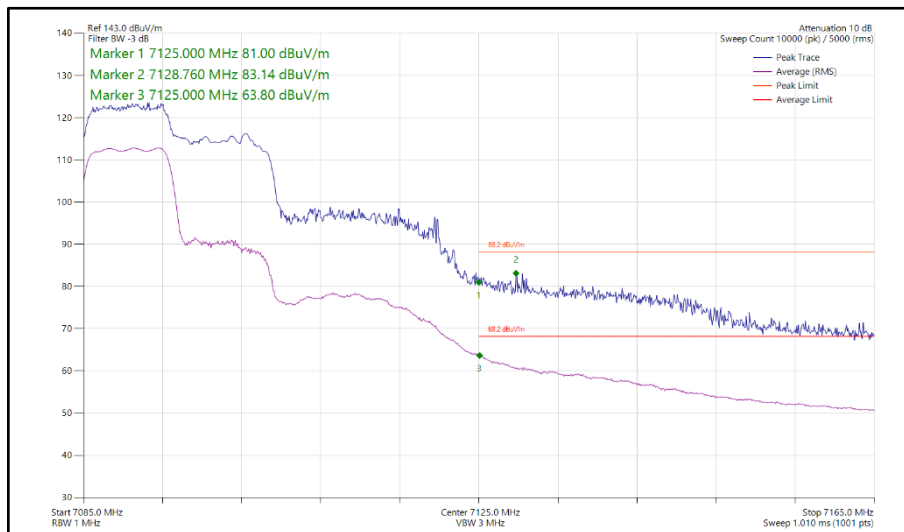
Figure 191 - 802.11ax HE20, RU 106-53, SDM, Core 0-1 - 7095 MHz Band Edge Frequency 7125 MHz
