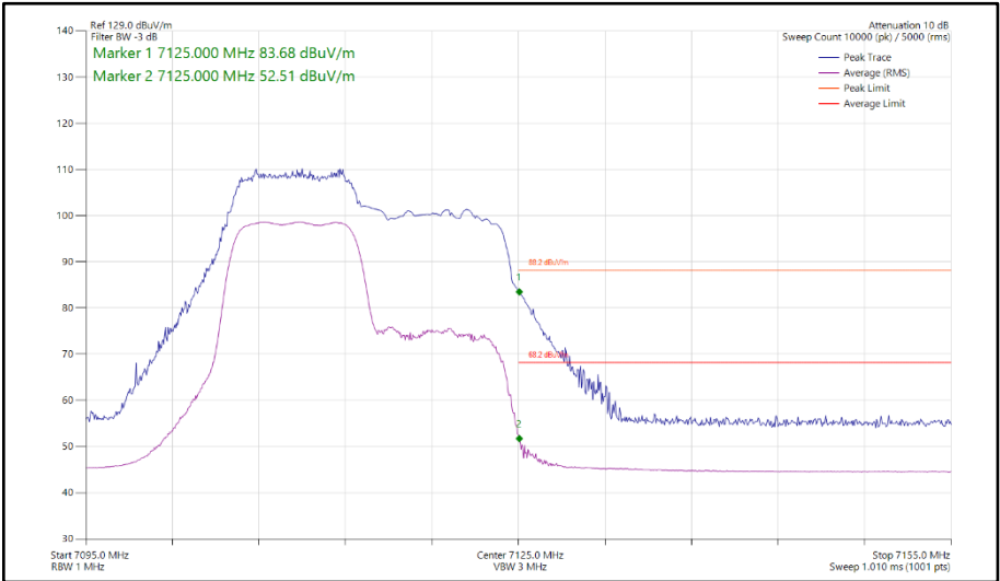
Figure 193 - 802.11ax HE20, RU 106-53, SDM, Core 0-1 - 7115 MHz Band Edge Frequency 7125 MHz
