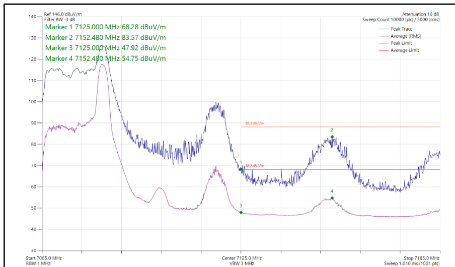
Figure 189 - 802.11ax HE20, RU 26-8, SDM, Core 0-1 - 7075 MHz Band Edge Frequency 7125 MHz
