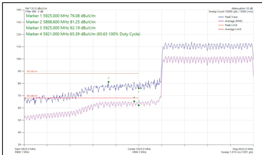
Figure 231 - 802.11ax HE80, SU, CDD, Core 0-1 - 5985 MHz Band Edge Frequency 5925 MHz
