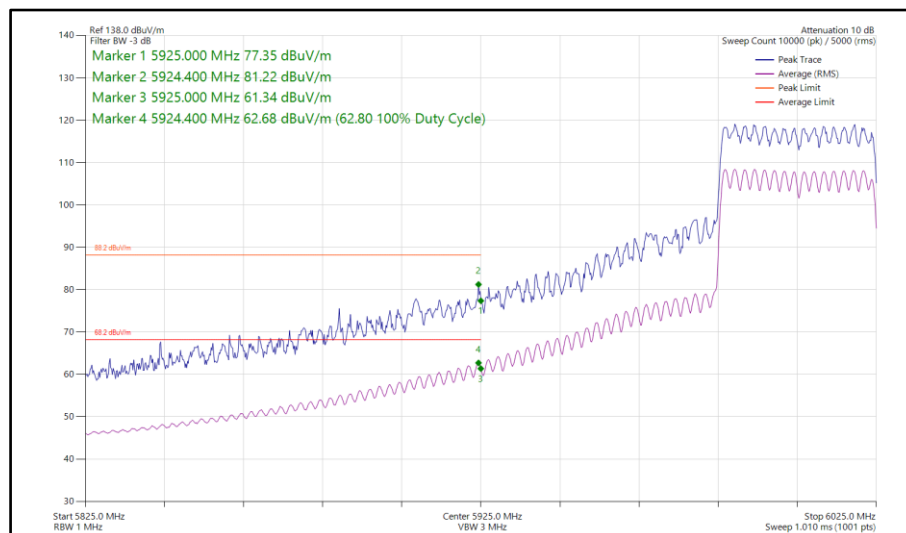
Figure 208 - 802.11ax HE40, SU, CDD, Core 0-1 - 6005 MHz Band Edge Frequency 5925 MHz
