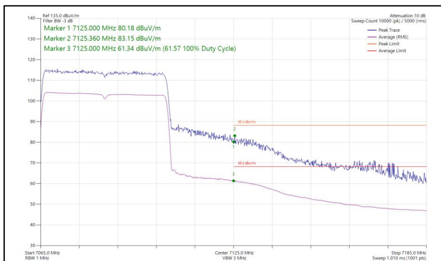
Figure 217 - 802.11ax HE40, SU, SDM, Core 0-1 - 7085 MHz Band Edge Frequency 7125 MHz
