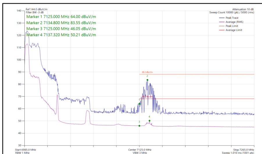
Figure 237 - 802.11ax HE80, RU 52-37, CDD, Core 0-1 - 7025 MHz Band Edge Frequency 7125 MHz
