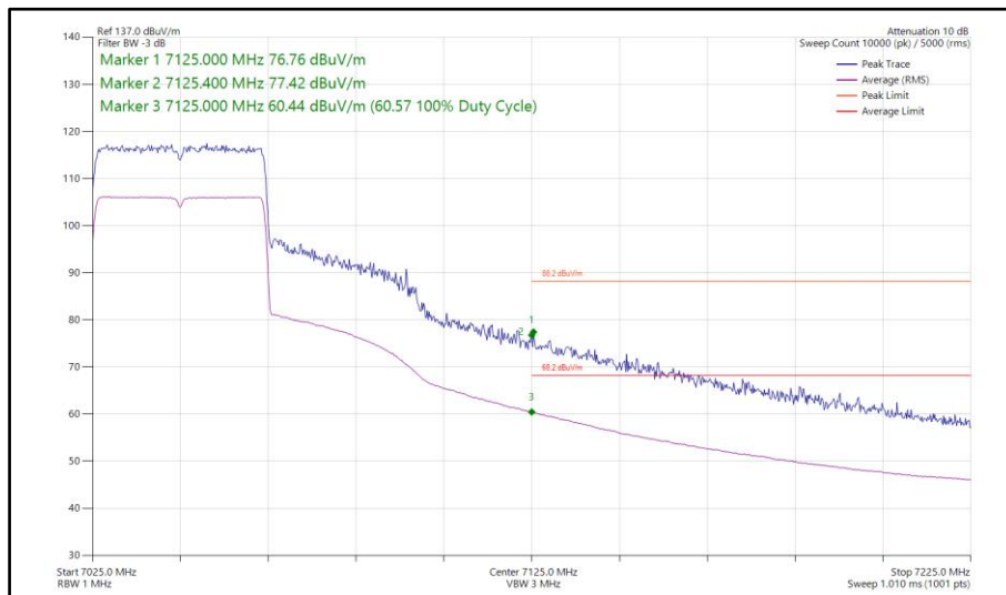
Figure 197 - 802.11ax HE40, SU, SISO, Core 0 - 7045 MHz Band Edge Frequency 7125 MHz
