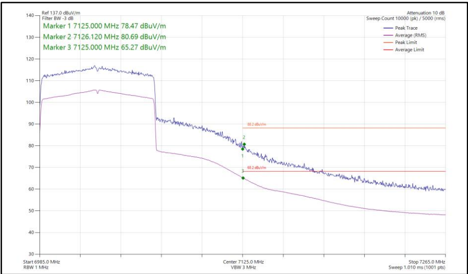
Figure 229 - 802.11ax HE80, SU, SISO, Core 1 - 7025 MHz Band Edge Frequency 7125 MHz
