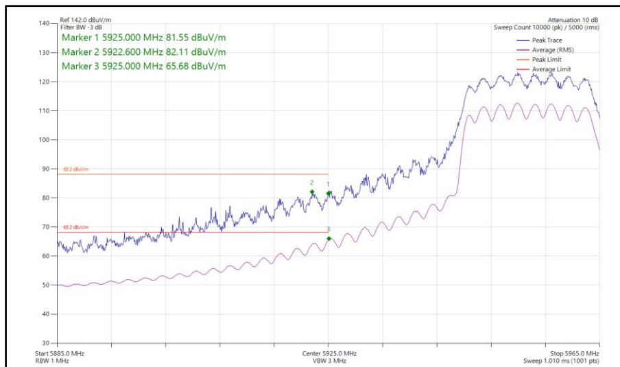
Figure 174 - 802.11ax HE20, SU, CDD, Core 0-1 - 5955 MHz Band Edge Frequency 5925 MHz
