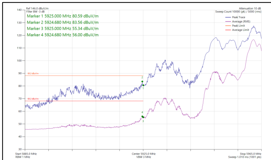
Figure 185 - 802.11ax HE20, RU 52-40, SDM, Core 0-1 - 5955 MHz Band Edge Frequency 5925 MHz
