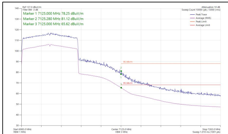
Figure 236 - 802.11ax HE80, SU, CDD, Core 0-1 - 7025 MHz Band Edge Frequency 7125 MHz
