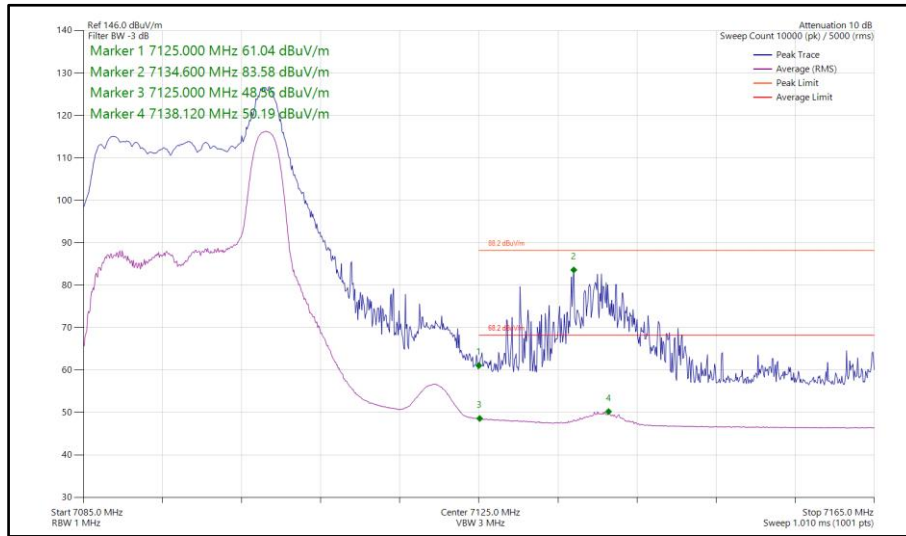
Figure 171 - 802.11ax HE20, RU 26-8, SISO, Core 1 - 7095 MHz Band Edge Frequency 7125 MHz
