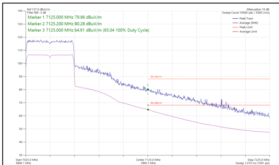
Figure 210 - 802.11ax HE40, SU, CDD, Core 0-1 - 7045 MHz Band Edge Frequency 7125 MHz
