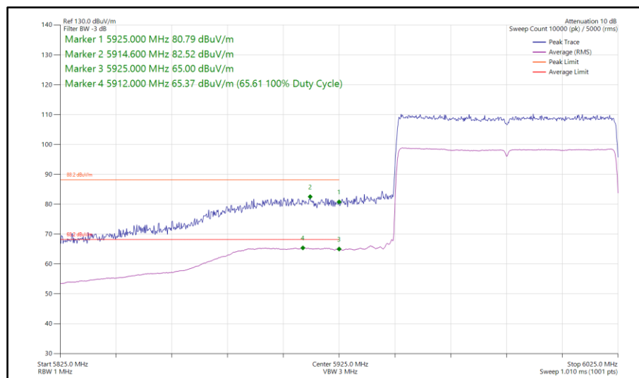
Figure 219 - 802.11ax HE80, SU, SISO, Core 0 - 5985 MHz Band Edge Frequency 5925 MHz
