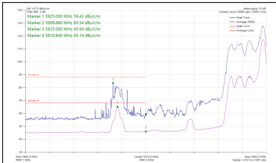
Figure 214 - 802.11ax HE40, RU 26-17, SDM, Core 0-1 - 5965 MHz Band Edge Frequency 5925 MHz
