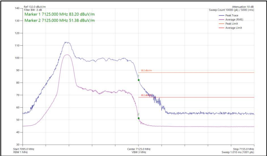
Figure 173 - 802.11ax HE20, RU 26-0, SISO, Core 1 - 7115 MHz Band Edge Frequency 7125 MHz
