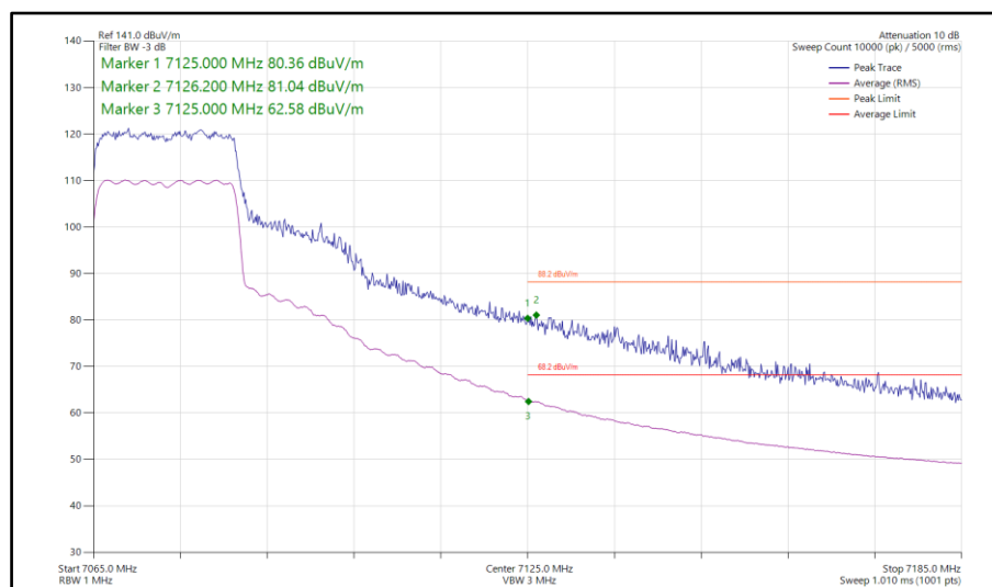
Figure 178 - 802.11ax HE20, SU, CDD, Core 0-1 - 7075 MHz Band Edge Frequency 7125 MHz
