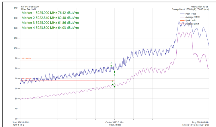
Figure 187 - 802.11ax HE20, RU 106-53, SDM, Core 0-1 - 5975 MHz Band Edge Frequency 5925 MHz
