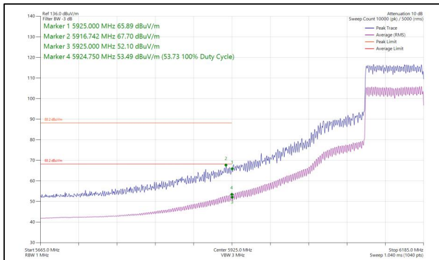
Figure 234 - 802.11ax HE80, SU, CDD, Core 0-1 - 6145 MHz Band Edge Frequency 5925 MHz
