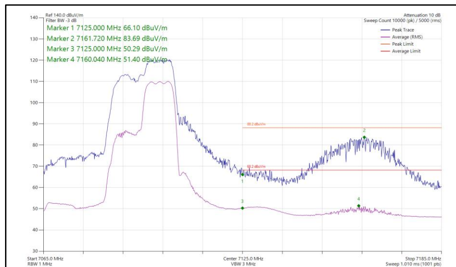
Figure 212 - 802.11ax HE40, RU 106-56, CDD, Core 0-1 - 7085 MHz Band Edge Frequency 7125 MHz
