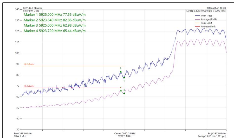
Figure 184 - 802.11ax HE20, SU, SDM, Core 0-1 - 5955 MHz Band Edge Frequency 5925 MHz
