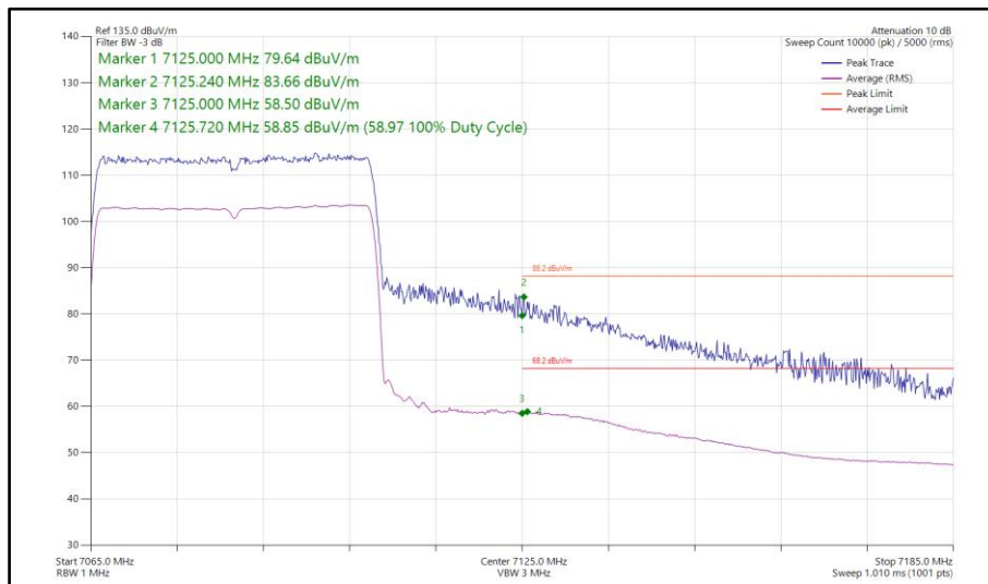
Figure 211 - 802.11ax HE40, SU, CDD, Core 0-1 - 7085 MHz Band Edge Frequency 7125 MHz
