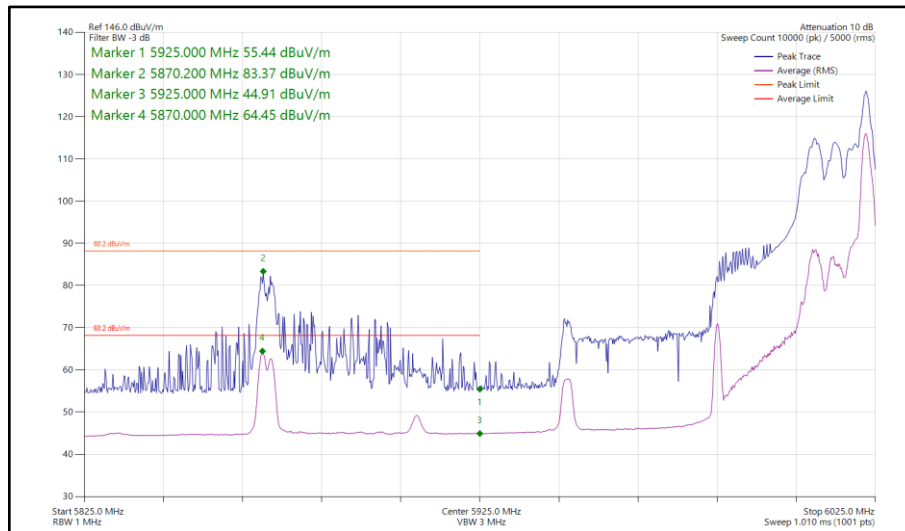
Figure 239 - 802.11ax HE80, RU 26-36, SDM, Core 0-1 - 5985 MHz Band Edge Frequency 5925 MHz
