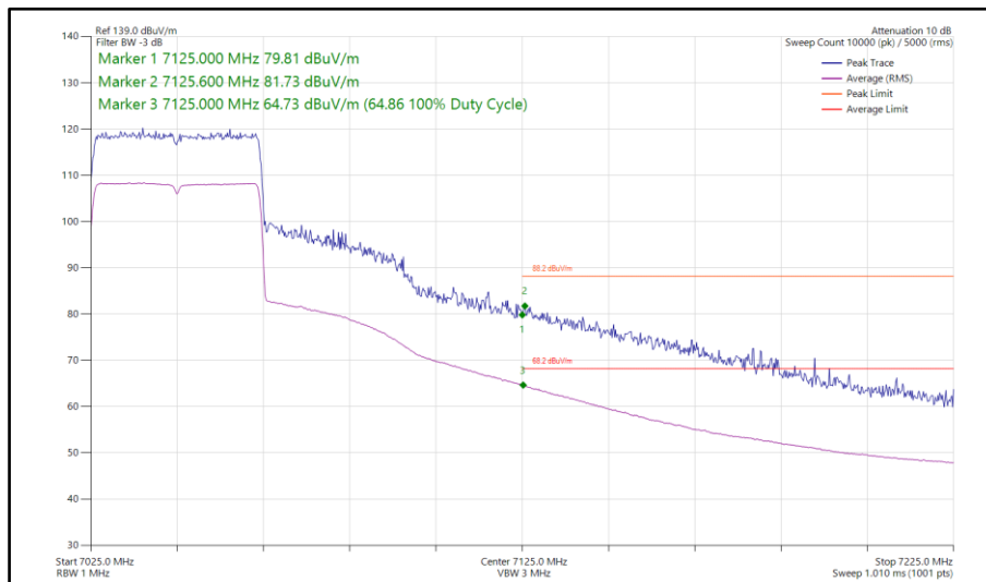
Figure 203 - 802.11ax HE40, SU, SISO, Core 1 - 7045 MHz Band Edge Frequency 7125 MHz
