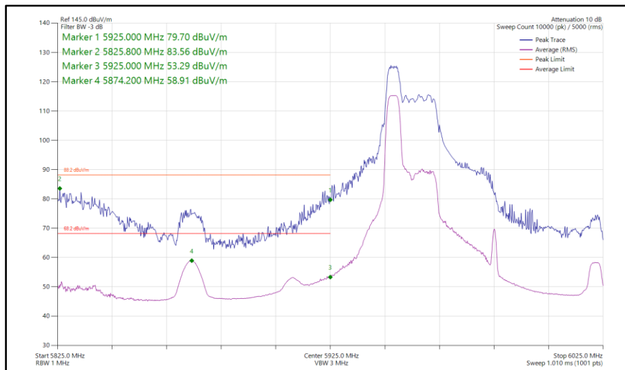
Figure 226 - 802.11ax HE80, RU 52-37, SISO, Core 1 - 5985 MHz Band Edge Frequency 5925 MHz
