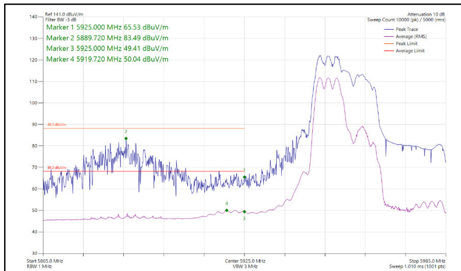
Figure 207 - 802.11ax HE40, RU 106-53, CDD, Core 0-1 - 5965 MHz Band Edge Frequency 5925 MHz
