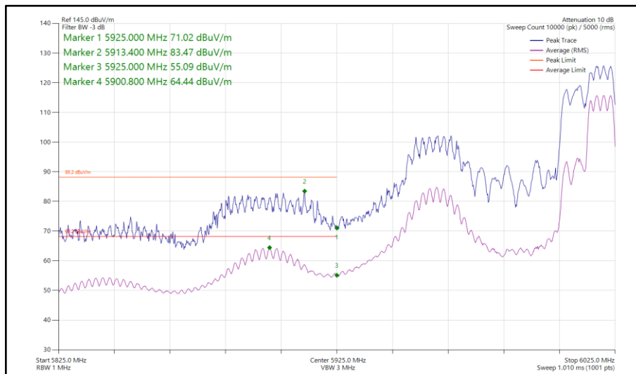
Figure 209 - 802.11ax HE40, RU 106-56, CDD, Core 0-1 - 6005 MHz Band Edge Frequency 5925 MHz
