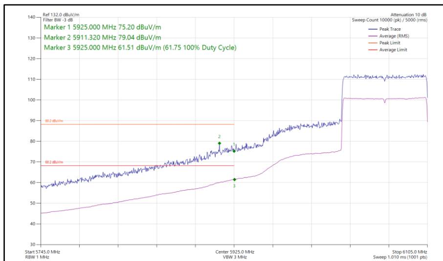
Figure 221 - 802.11ax HE80, SU, SISO, Core 0 - 6065 MHz Band Edge Frequency 5925 MHz
