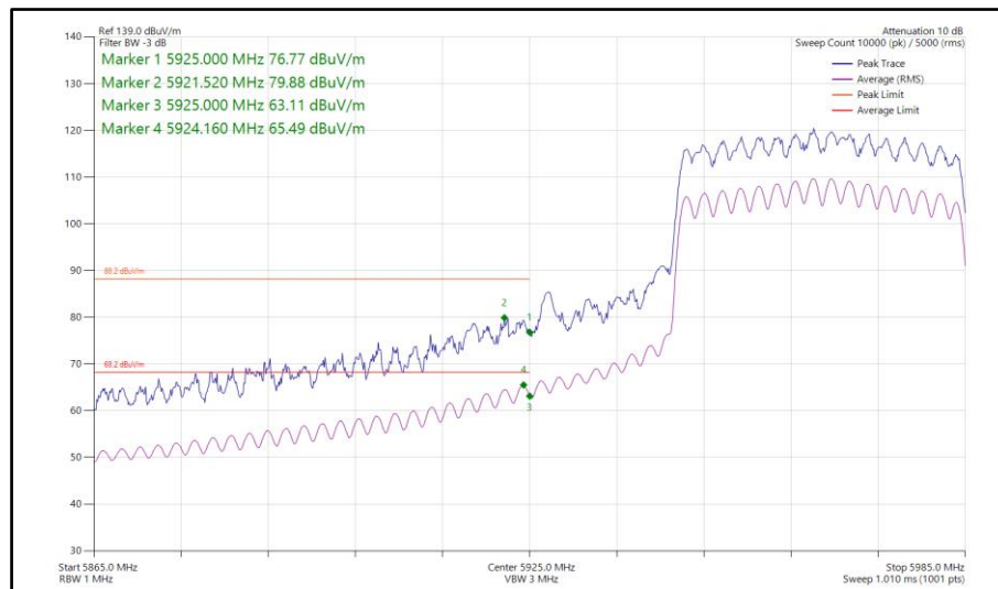
Figure 213 - 802.11ax HE40, SU, SDM, Core 0-1 - 5965 MHz Band Edge Frequency 5925 MHz
