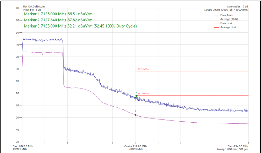
Figure 228 - 802.11ax HE80, SU, SISO, Core 1 - 6945 MHz Band Edge Frequency 7125 MHz
