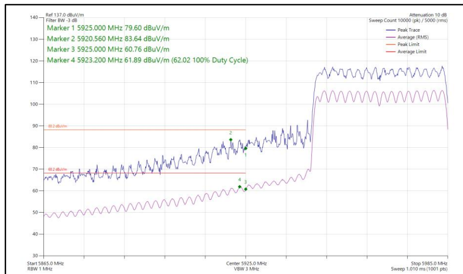
Figure 206 - 802.11ax HE40, SU, CDD, Core 0-1 - 5965 MHz Band Edge Frequency 5925 MHz
