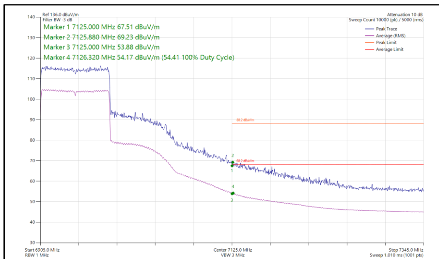
Figure 235 - 802.11ax HE80, SU, CDD, Core 0-1 - 6945 MHz Band Edge Frequency 7125 MHz
