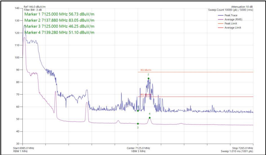
Figure 230 - 802.11ax HE80, RU 26-0, SISO, Core 1 - 7025 MHz Band Edge Frequency 7125 MHz
