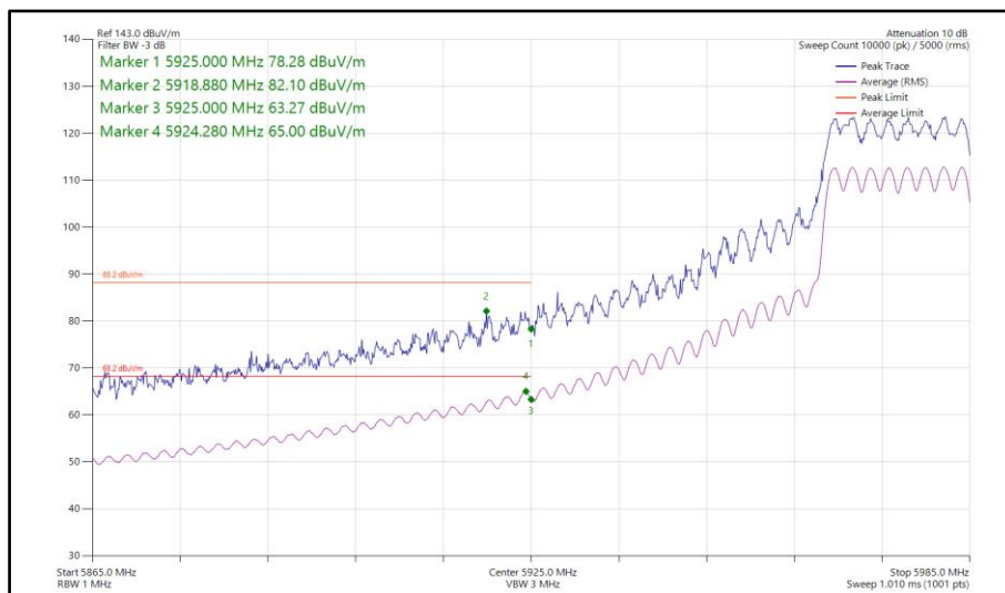
Figure 186 - 802.11ax HE20, SU, SDM, Core 0-1 - 5975 MHz Band Edge Frequency 5925 MHz
