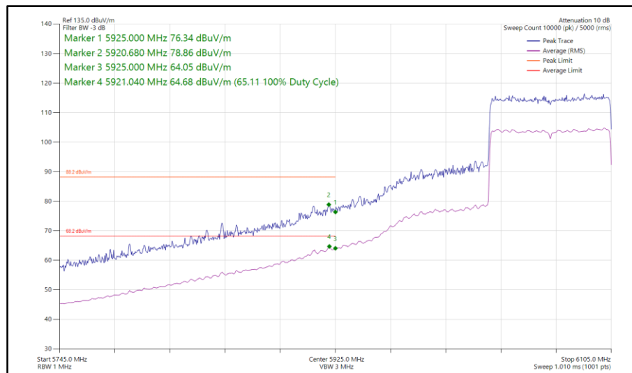
Figure 240 - 802.11ax HE80, SU, SDM, Core 0-1 - 6065 MHz Band Edge Frequency 5925 MHz
