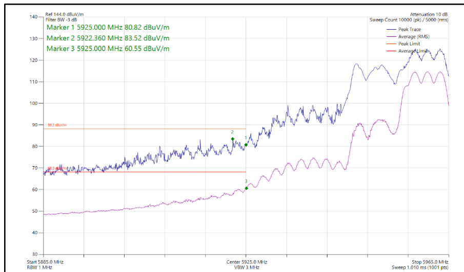
Figure 175 - 802.11ax HE20, RU 106-54, CDD, Core 0-1 - 5955 MHz Band Edge Frequency 5925 MHz
