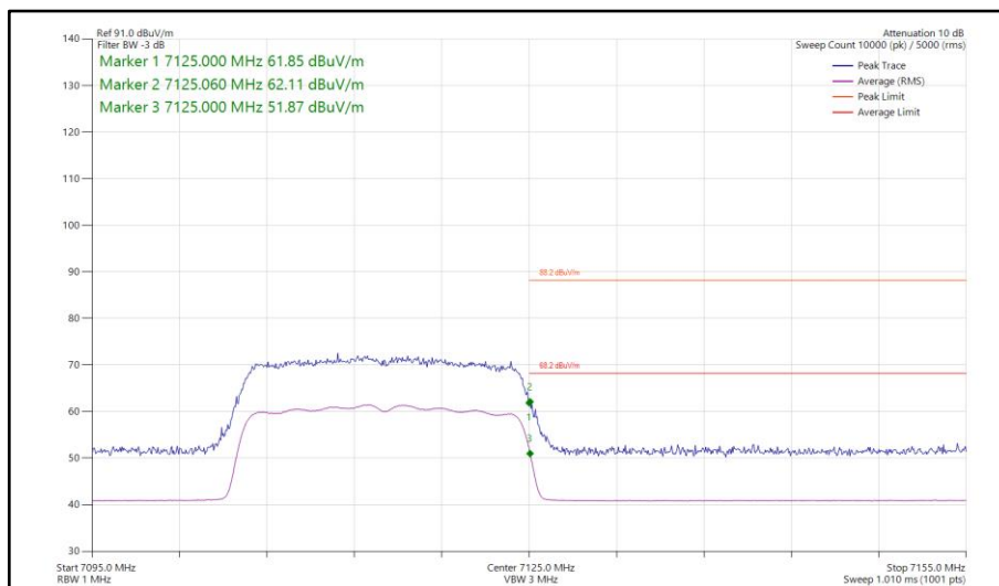
Figure 192 - 802.11ax HE20, SU, SDM, Core 0-1 - 7115 MHz Band Edge Frequency 7125 MHz
