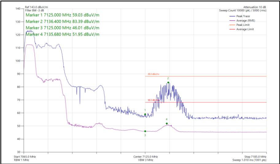
Figure 199 - 802.11ax HE40, RU 52-37, SISO, Core 0 - 7085 MHz Band Edge Frequency 7125 MHz
