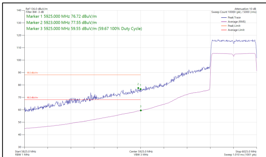
Figure 202 - 802.11ax HE40, SU, SISO, Core 1 - 6005 MHz Band Edge Frequency 5925 MHz
