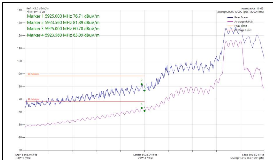
Figure 177 - 802.11ax HE20, RU 106-53, CDD, Core 0-1 - 5975 MHz Band Edge Frequency 5925 MHz
