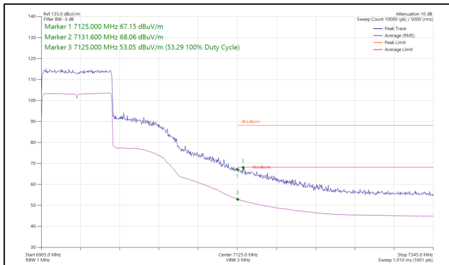
Figure 222 - 802.11ax HE80, SU, SISO, Core 0 - 6945 MHz Band Edge Frequency 7125 MHz
