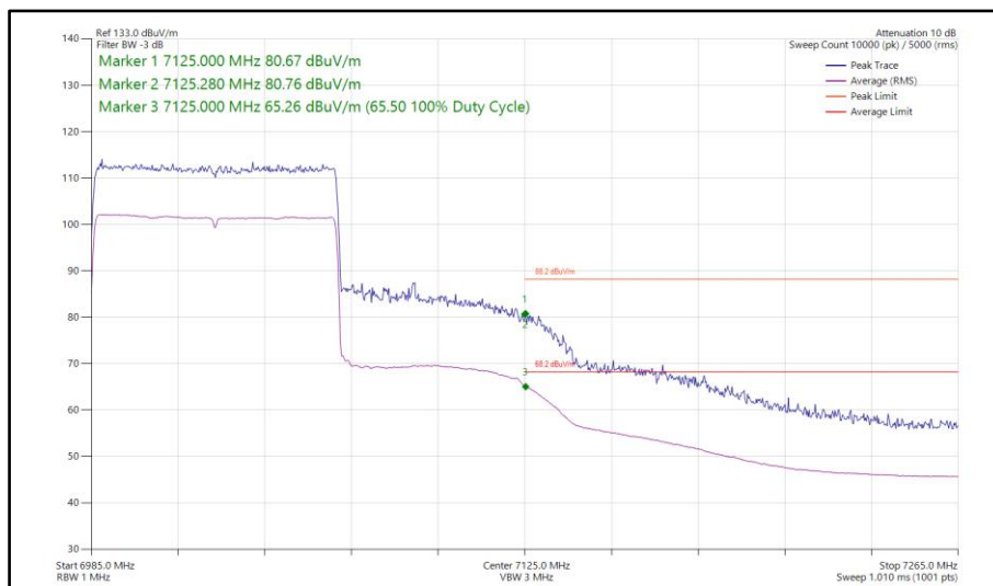
Figure 223 - 802.11ax HE80, SU, SISO, Core 0 - 7025 MHz Band Edge Frequency 7125 MHz
