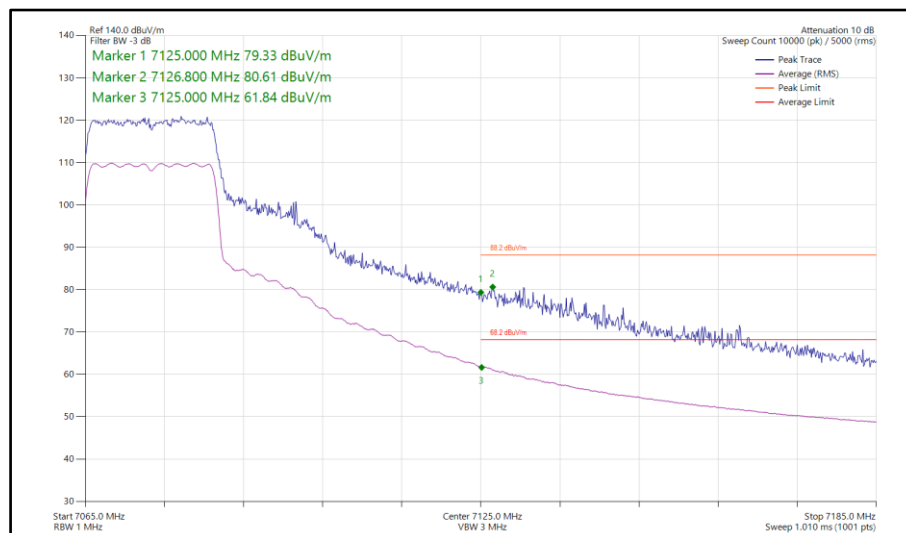
Figure 188 - 802.11ax HE20, SU, SDM, Core 0-1 - 7075 MHz Band Edge Frequency 7125 MHz
