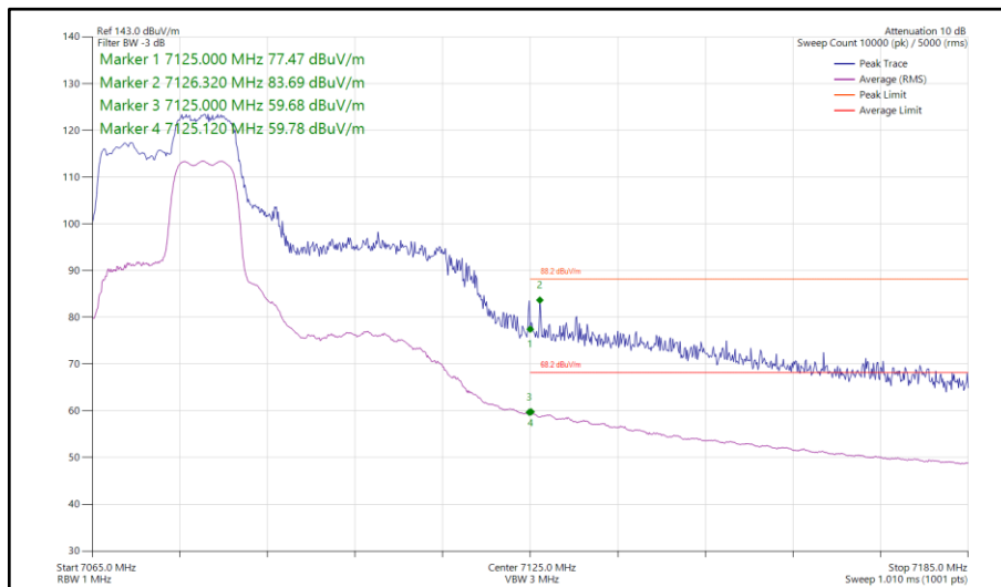
Figure 179 - 802.11ax HE20, RU 106-54, CDD, Core 0-1 - 7075 MHz Band Edge Frequency 7125 MHz
