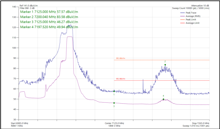
Figure 224 - 802.11ax HE80, RU 106-60, SISO, Core 0 - 7025 MHz Band Edge Frequency 7125 MHz
