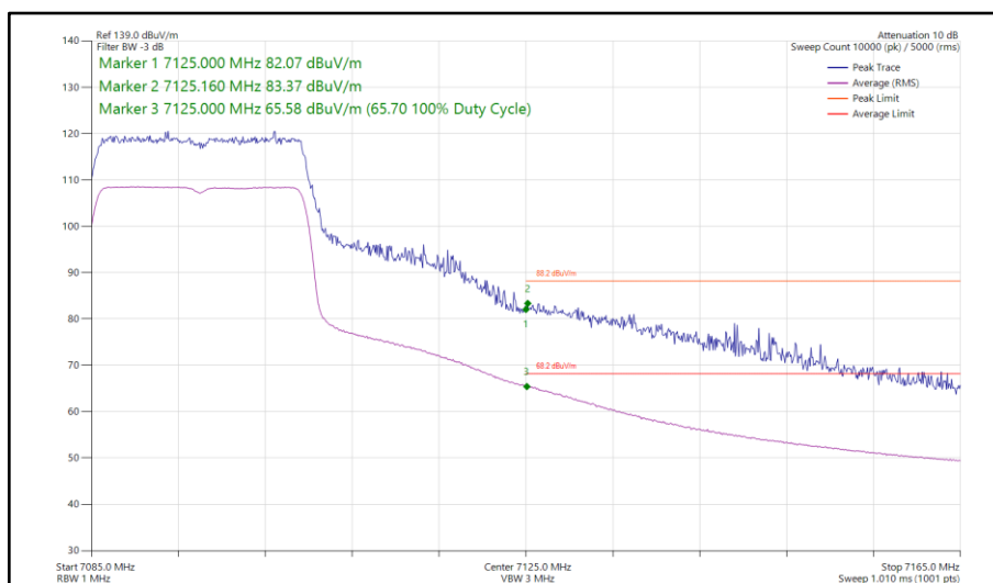
Figure 190 - 802.11ax HE20, SU, SDM, Core 0-1 - 7095 MHz Band Edge Frequency 7125 MHz
