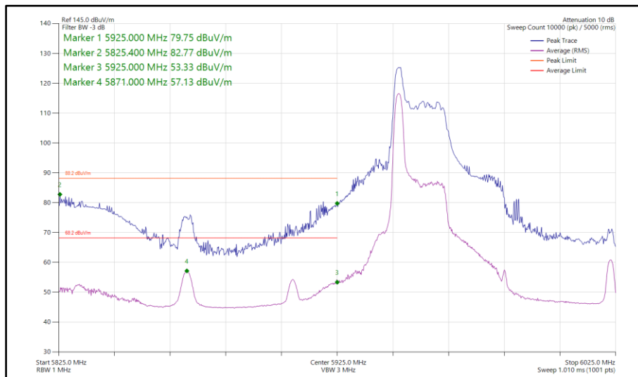
Figure 220 - 802.11ax HE80, RU 26-0, SISO, Core 0 - 5985 MHz Band Edge Frequency 5925 MHz
