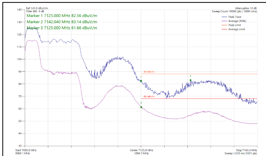
Figure 181 - 802.11ax HE20, RU 52-37, CDD, Core 0-1 - 7095 MHz Band Edge Frequency 7125 MHz
