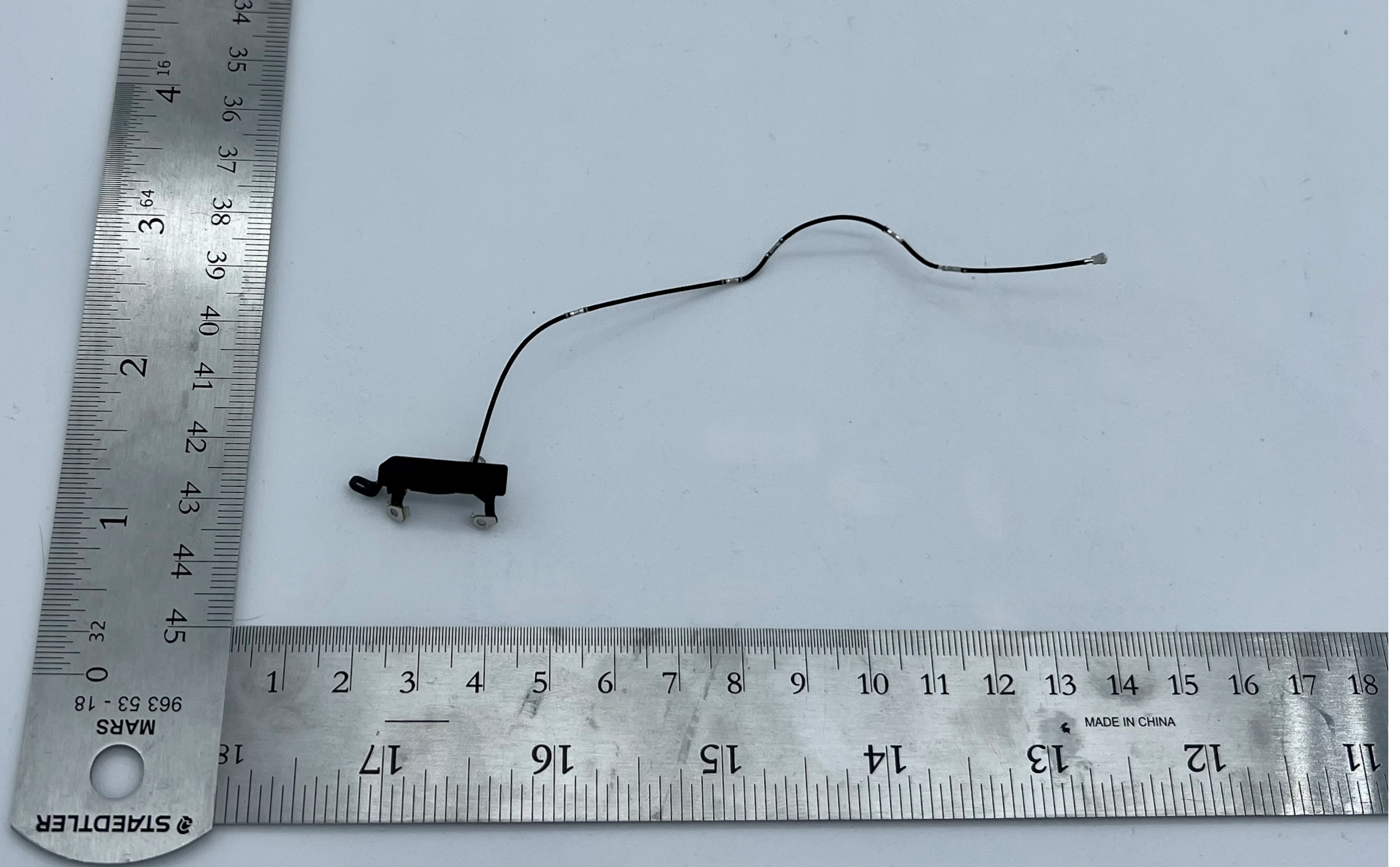
A3416 NB UNII_R - Front
