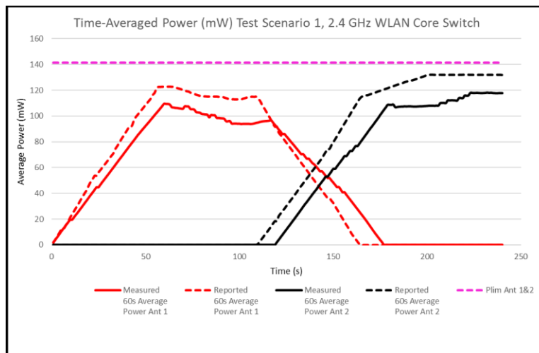
Figure I-2 60s Average Power vs. Time, 2.4 GHz
