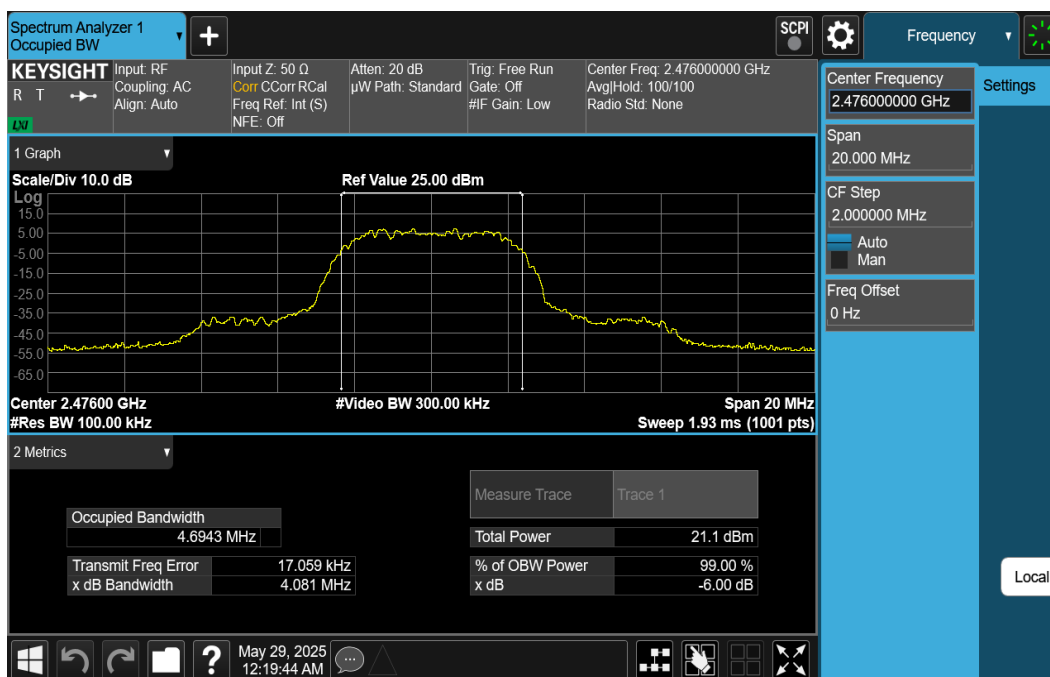
Plot 7-6. 6dB BW & 99% OBW Plot Ant1 (Bluetooth (HDR8), 8Mbps, – Ch. 73)
