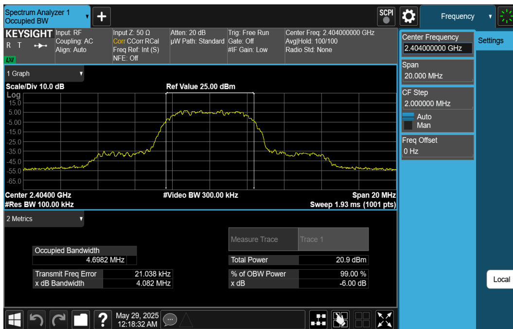
Plot 7-4. 6dB BW & 99% OBW Plot Ant1 (Bluetooth (HDR8), 8Mbps, – Ch. 1)
