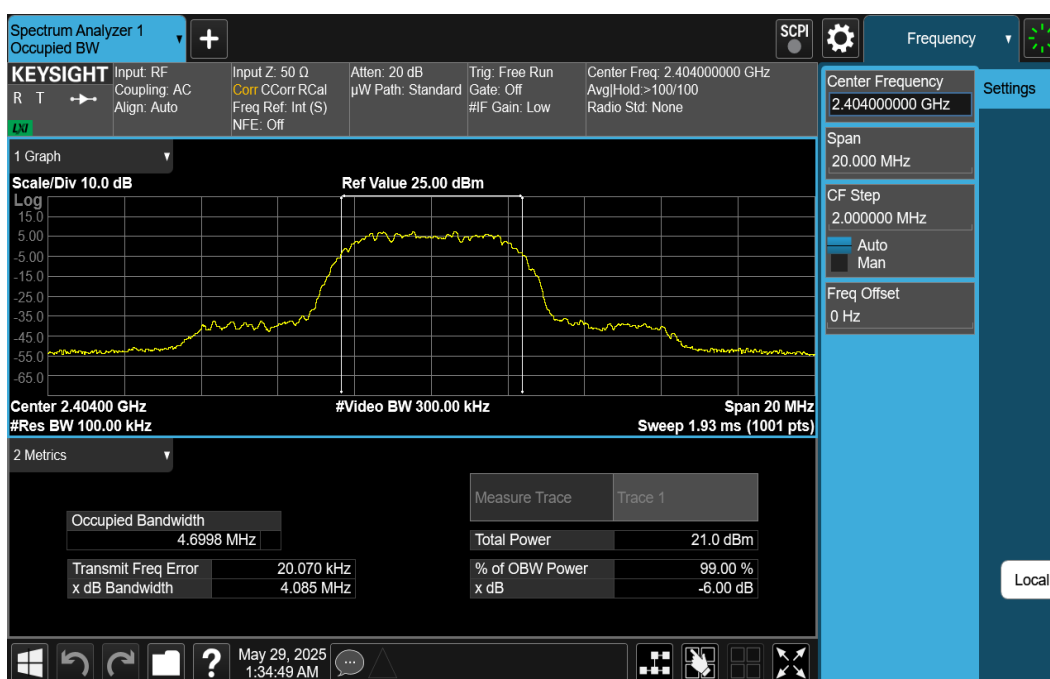
Plot 7-10. 6dB BW & 99% OBW Plot Ant2 (Bluetooth (HDR8), 8Mbps, – Ch. 1)
