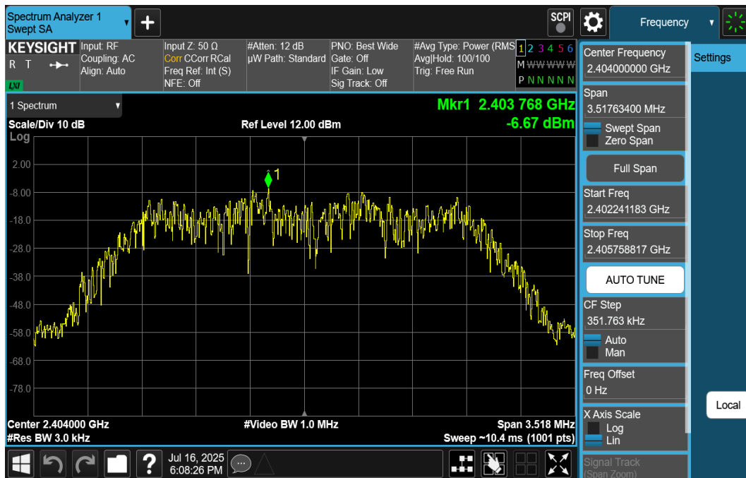
Plot 7-19. Power Spectral Density Plot Ant1 (Bluetooth (HDR4), 4Mbps, ePA – Ch. 1)
