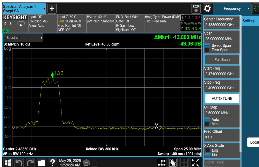
Plot 7-74. Band Edge Plot Ant1 (Bluetooth (HDR4), ePA - Ch. 73)
