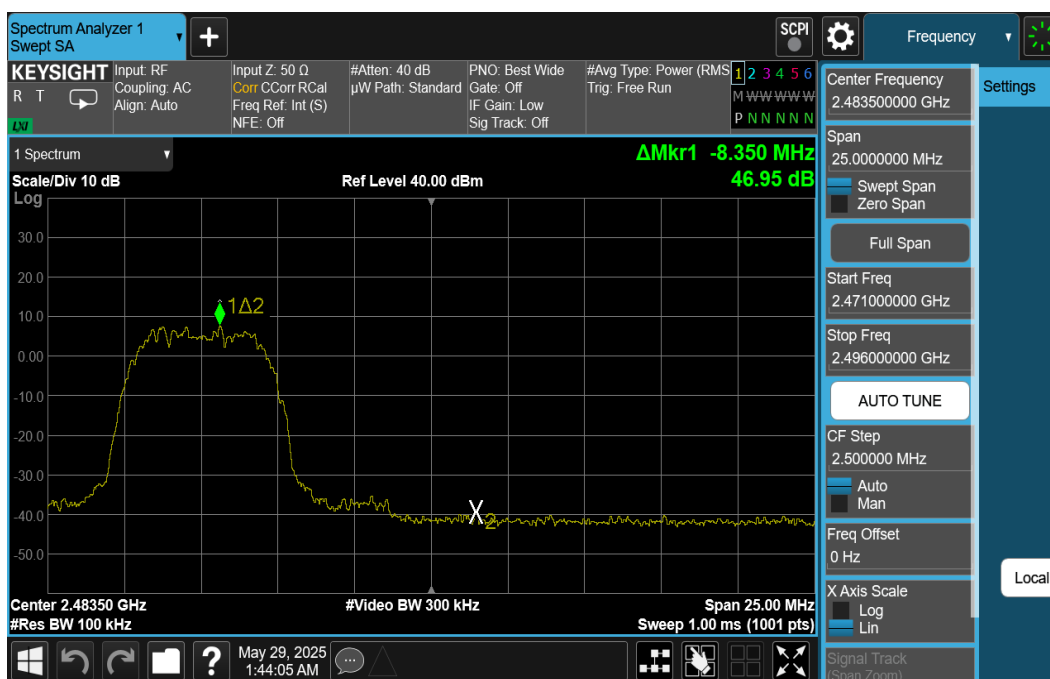
Plot 7-80. Band Edge Plot Ant2 (Bluetooth (HDR8), ePA – Ch. 73)
