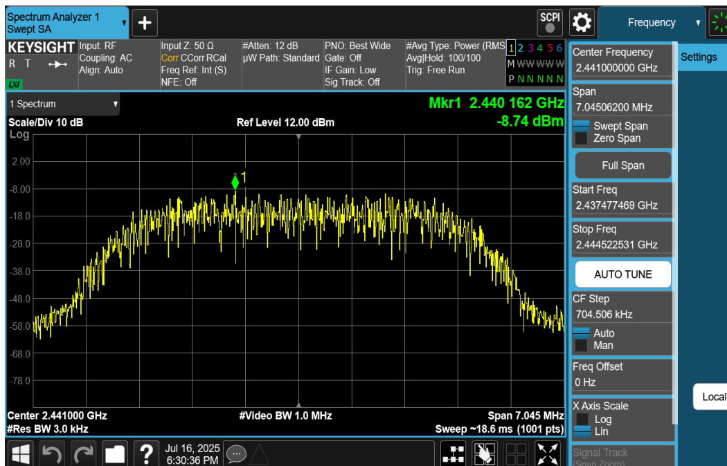
Plot 7-63. Power Spectral Density Plot TxBF Ant1 (Bluetooth (HDR8), 8Mbps, ePA – Ch. 38)
