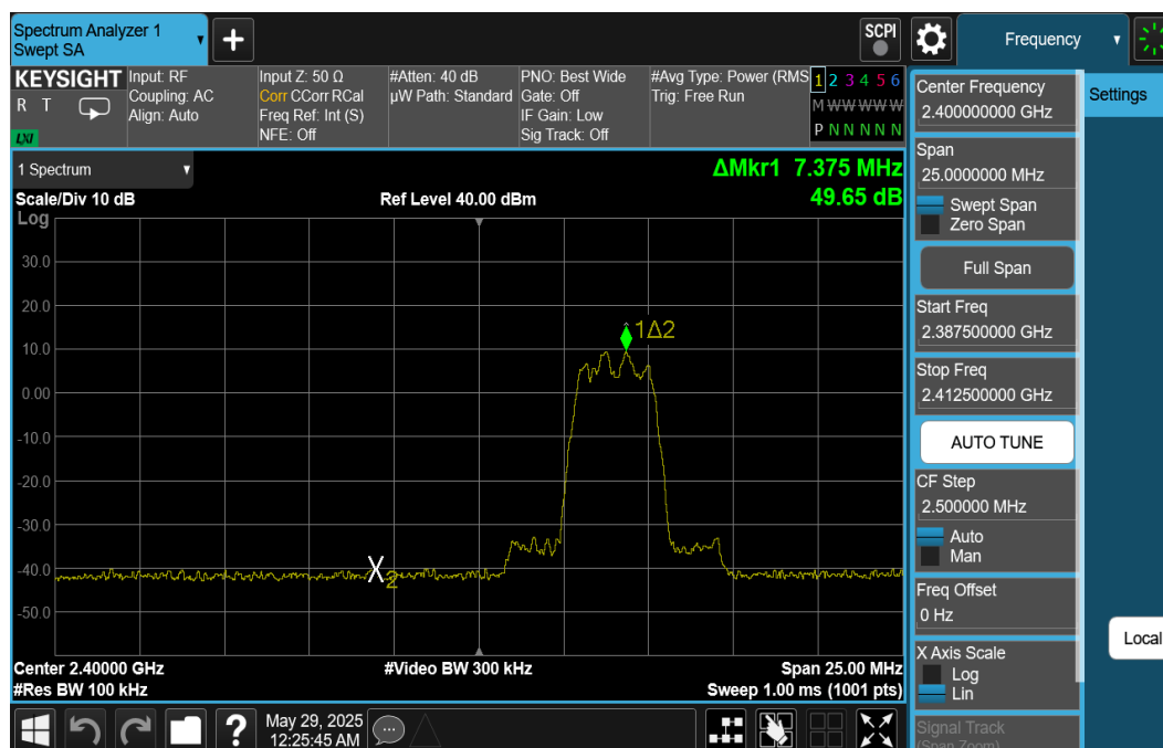
Plot 7-73. Band Edge Plot Ant1 (Bluetooth (HDR4), ePA – Ch. 1)
