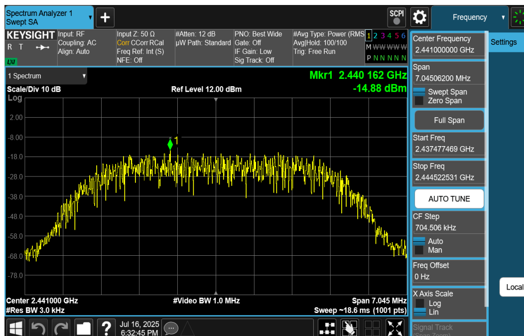
Plot 7-69. Power Spectral Density Plot TxBF Ant1 (Bluetooth (HDR8), 8Mbps, iPA – Ch. 38)
