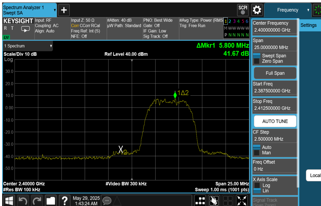
Plot 7-79. Band Edge Plot Ant2 (Bluetooth (HDR8), ePA – Ch. 1)
