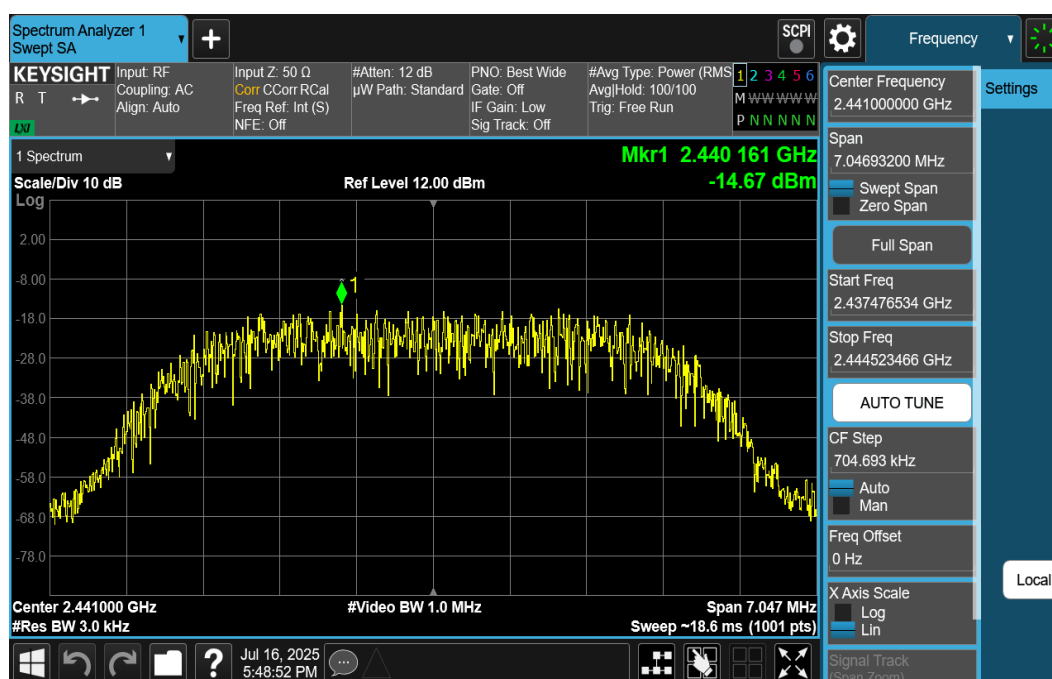
Plot 7-70. Power Spectral Density Plot TxBF Ant2 (Bluetooth (HDR8), 8Mbps, iPA – Ch. 38)
