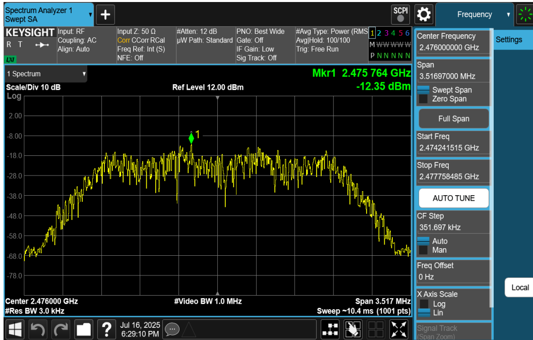
Plot 7-59. Power Spectral Density Plot Tx BF Ant1 (Bluetooth (HDR4), 4Mbps, iPA – Ch. 73)
