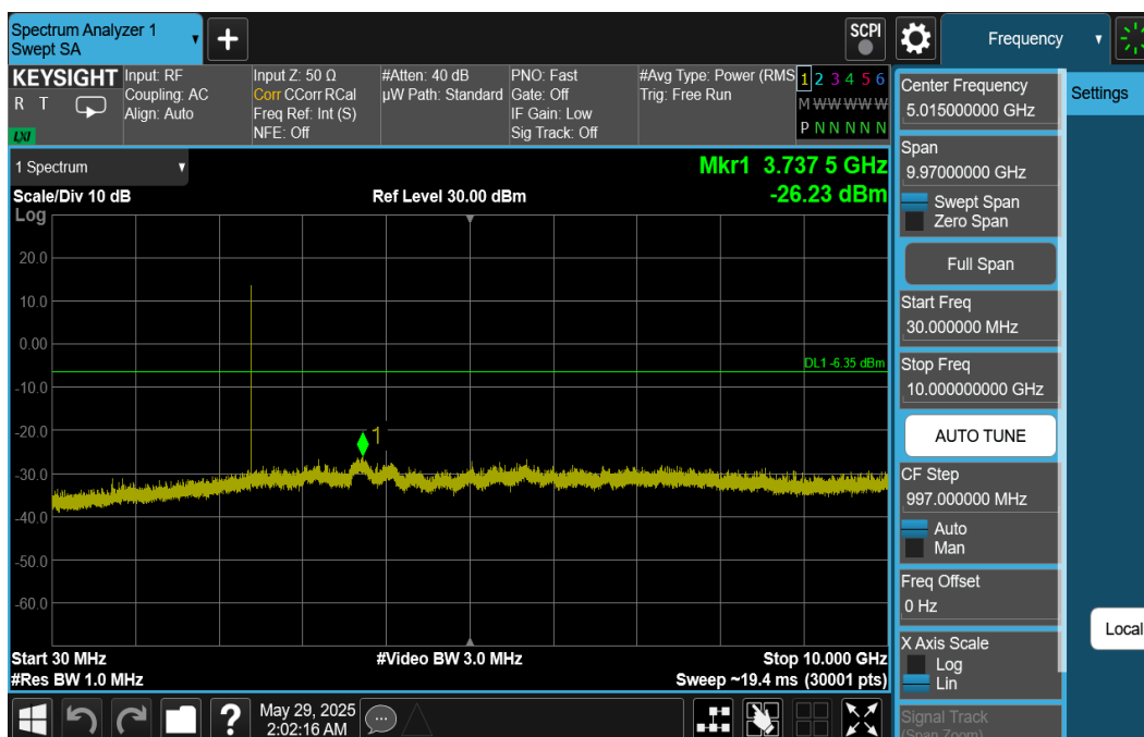
Plot 7-91. Conducted Spurious Plot Ant2 (Bluetooth (HDR4), 4 Mbps, ePA – Ch. 1)
