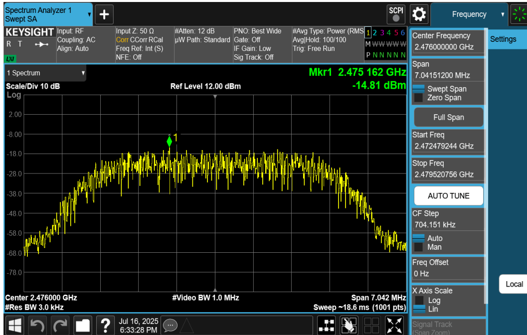
Plot 7-71. Power Spectral Density Plot TxBF Ant1 (Bluetooth (HDR8), 8Mbps, iPA – Ch. 73)
