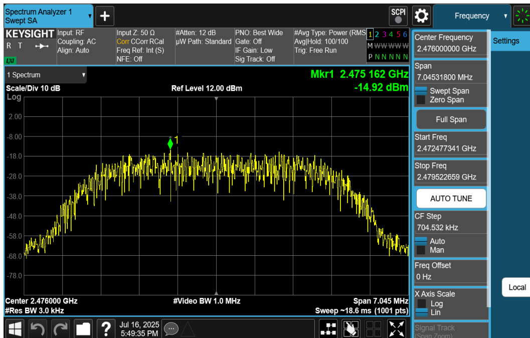
Plot 7-72. Power Spectral Density Plot TxBF Ant2 (Bluetooth (HDR8), 8Mbps, iPA – Ch. 73)
