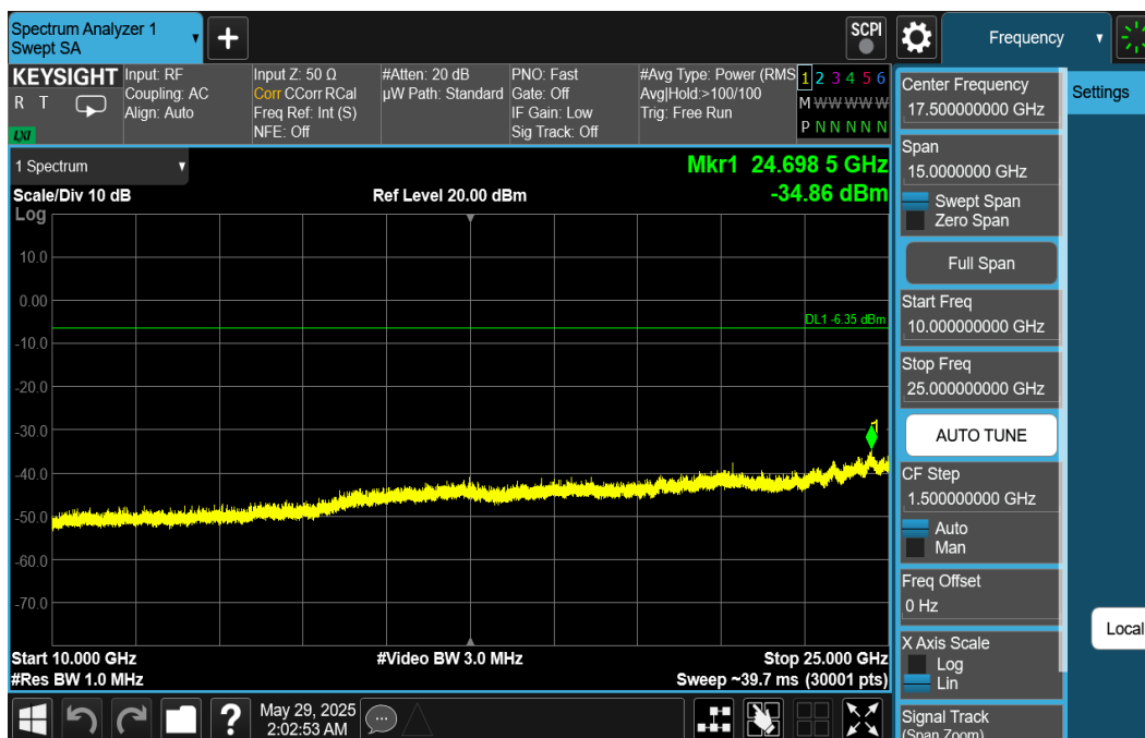
Plot 7-92. Conducted Spurious Plot Ant2 (Bluetooth (HDR4), 4 Mbps, ePA – Ch. 1)
