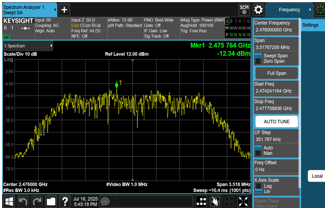
Plot 7-60. Power Spectral Density Plot Tx BF Ant2 (Bluetooth (HDR4), 4Mbps, iPA – Ch. 73)
