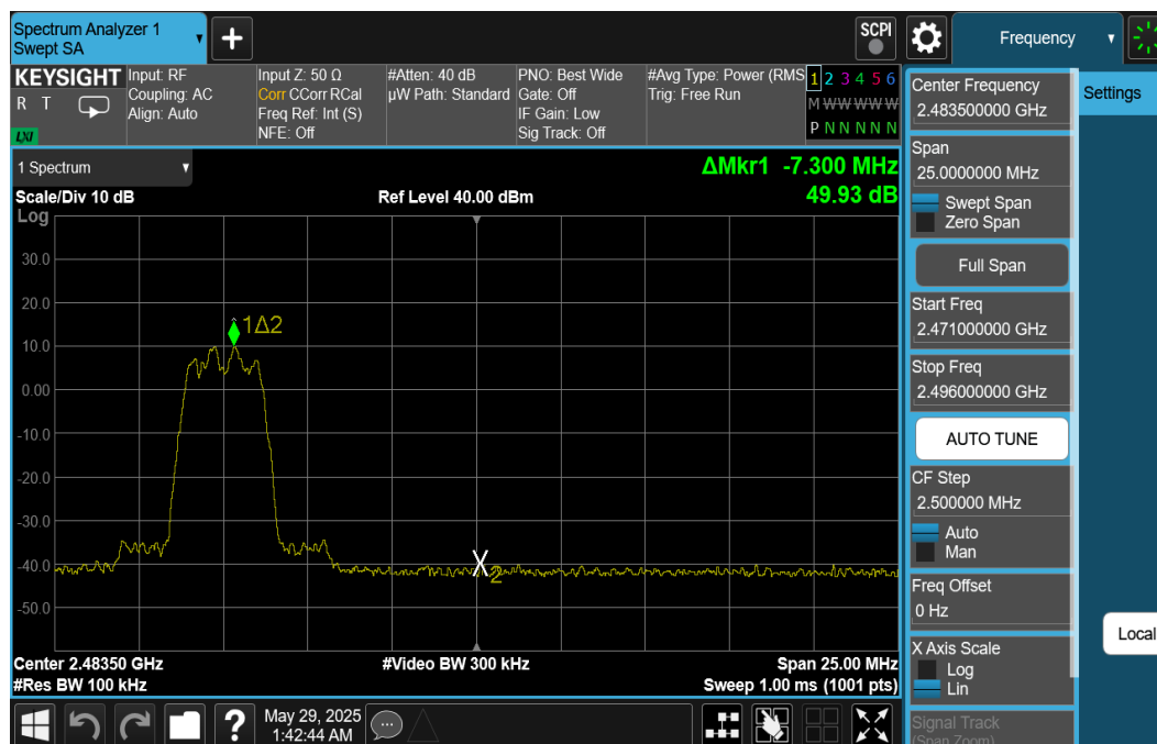
Plot 7-78. Band Edge Plot Ant2 (Bluetooth (HDR4), ePA – Ch. 73)
