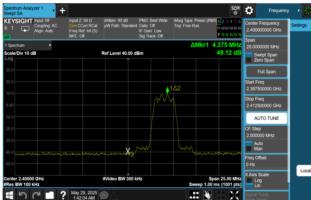
Plot 7-77. Band Edge Plot Ant2 (Bluetooth (HDR4), ePA – Ch. 1)
