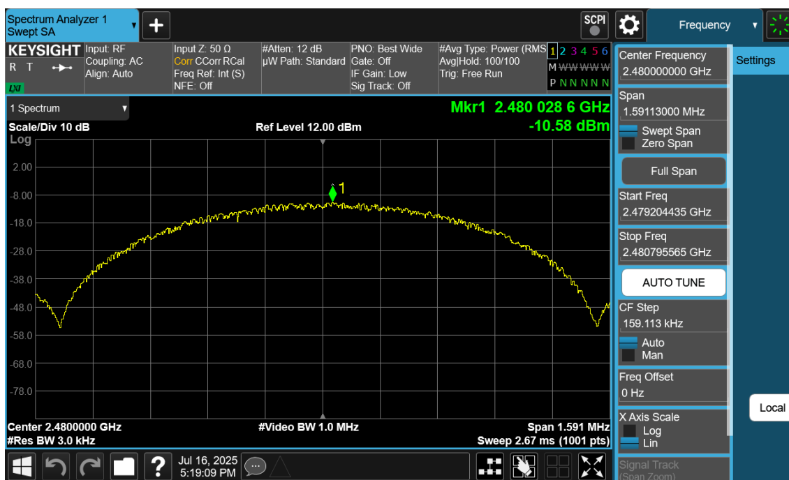
Plot 7-36. Power Spectral Density Plot Ant2 (Bluetooth (LE), 1Mbps, iPA – Ch. 39)
