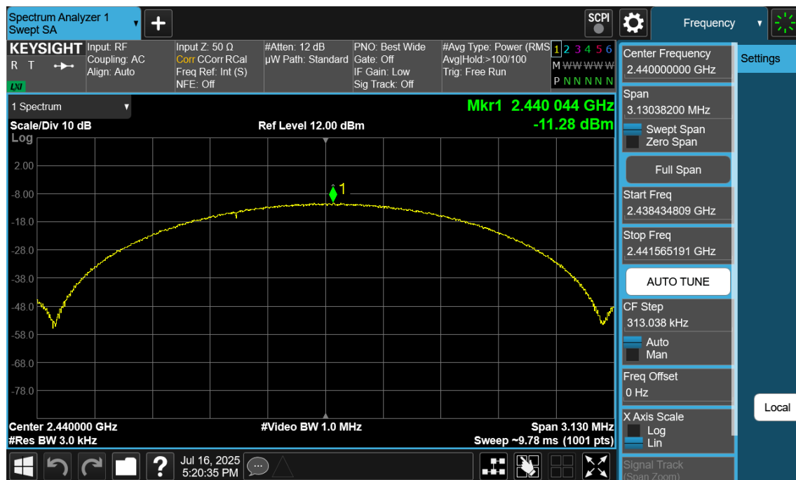
Plot 7-38. Power Spectral Density Plot Ant2 (Bluetooth (LE), 2Mbps, ePA – Ch. 19)
