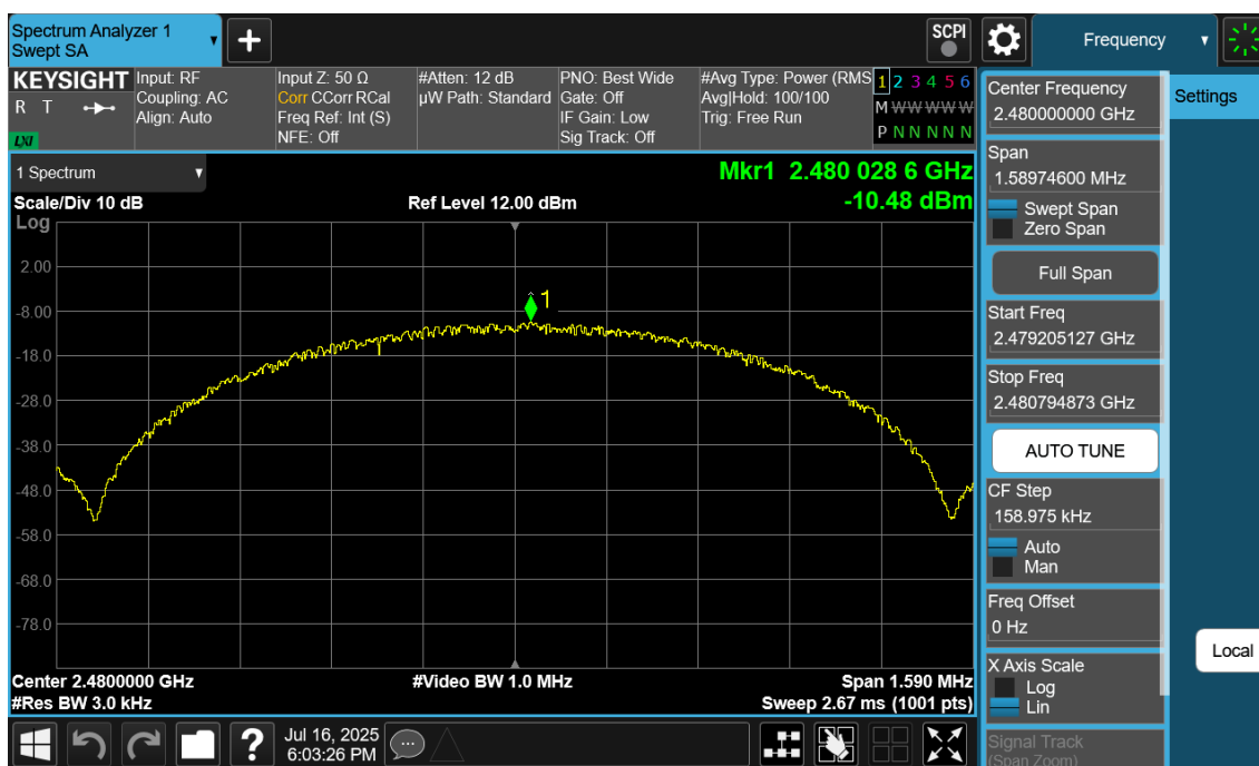
Plot 7-24. Power Spectral Density Plot Ant1 (Bluetooth (LE), 1Mbps, iPA – Ch. 39)
