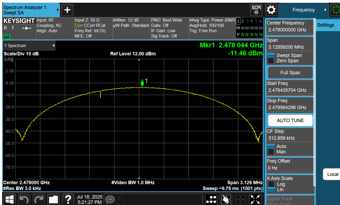
Plot 7-39. Power Spectral Density Plot Ant2 (Bluetooth (LE), 2Mbps, ePA – Ch. 38)
