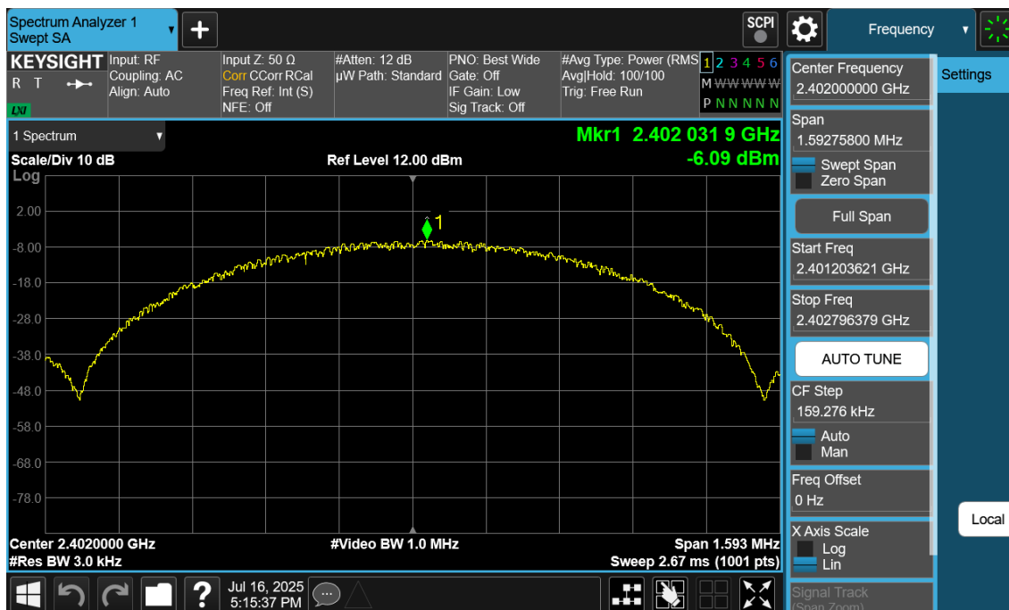
Plot 7-31. Power Spectral Density Plot Ant2 (Bluetooth (LE), 1Mbps, ePA – Ch. 0)
