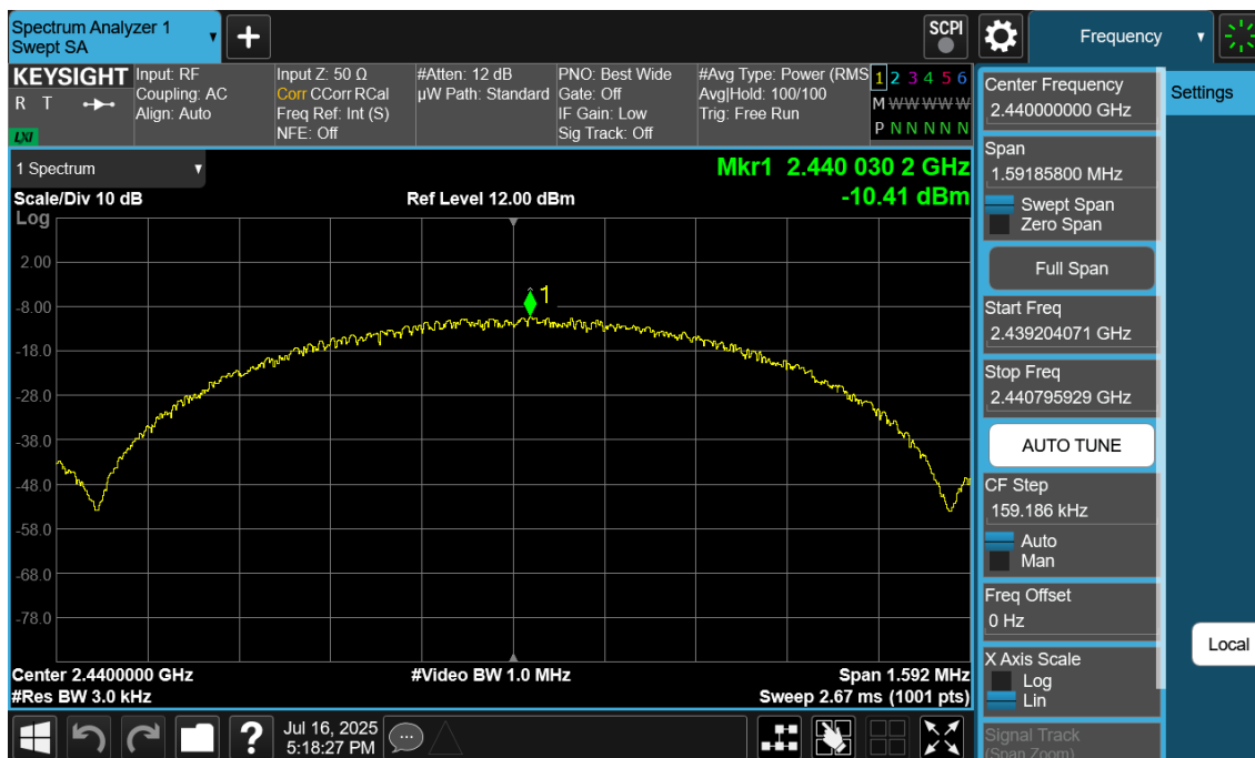
Plot 7-35. Power Spectral Density Plot Ant2 (Bluetooth (LE), 1Mbps, iPA – Ch. 19)
