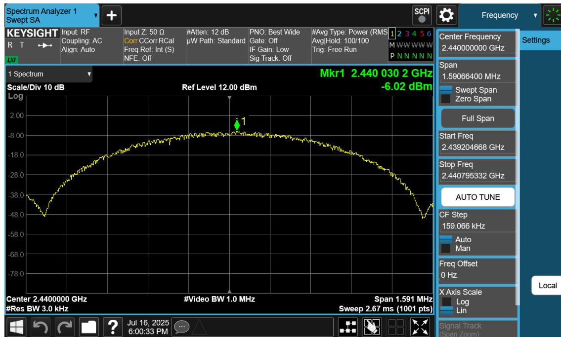
Plot 7-20. Power Spectral Density Plot Ant1 (Bluetooth (LE), 1Mbps, ePA – Ch. 19)
