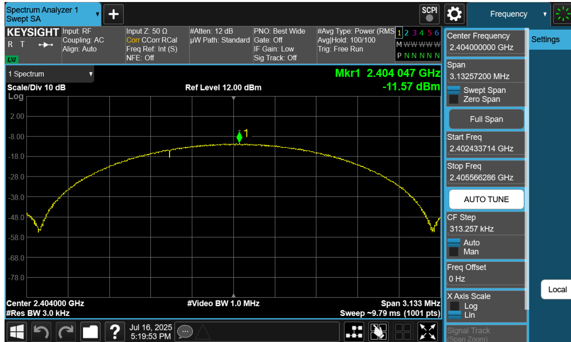
Plot 7-37. Power Spectral Density Plot Ant2 (Bluetooth (LE), 2Mbps, ePA – Ch. 1)
