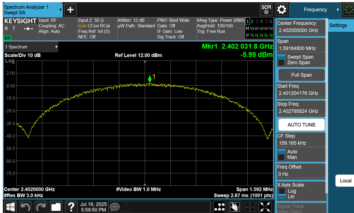
Plot 7-19. Power Spectral Density Plot Ant1 (Bluetooth (LE), 1Mbps, ePA – Ch. 0)
