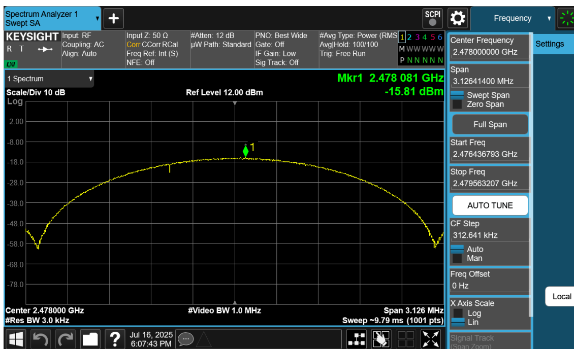
Plot 7-30. Power Spectral Density Plot Ant1 (Bluetooth (LE), 2Mbps, iPA – Ch. 38)
