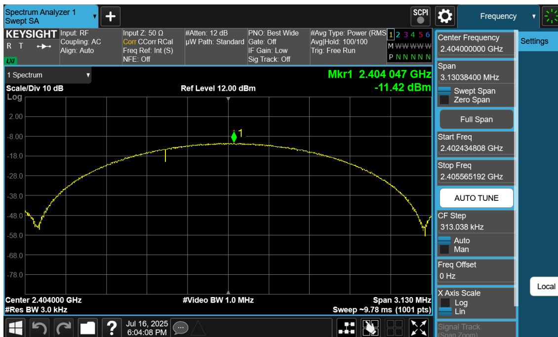
Plot 7-25. Power Spectral Density Plot Ant1 (Bluetooth (LE), 2Mbps, ePA – Ch. 1)
