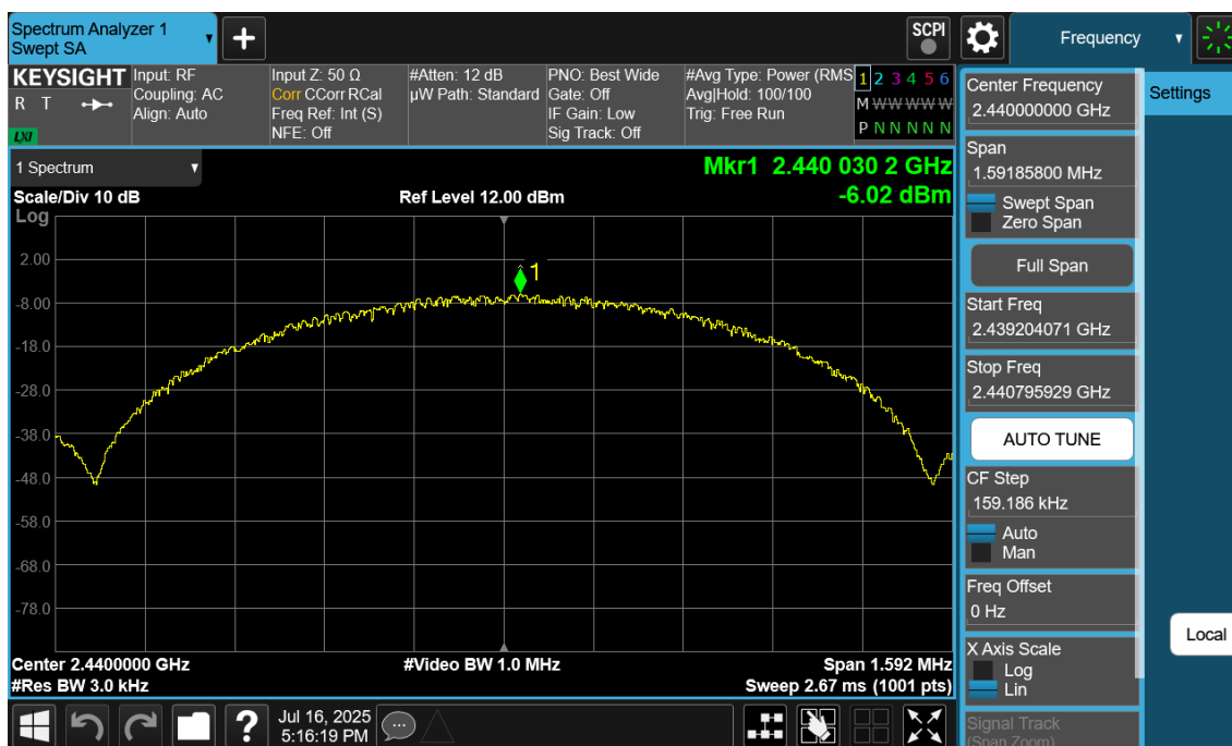
Plot 7-32. Power Spectral Density Plot Ant2 (Bluetooth (LE), 1Mbps, ePA – Ch. 19)
