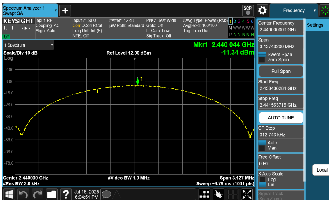
Plot 7-26. Power Spectral Density Plot Ant1 (Bluetooth (LE), 2Mbps, ePA – Ch. 19)
