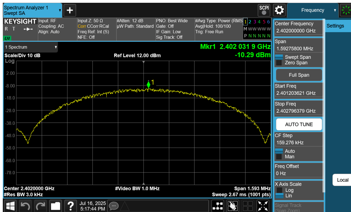
Plot 7-34. Power Spectral Density Plot Ant2 (Bluetooth (LE), 1Mbps, iPA – Ch. 0)
