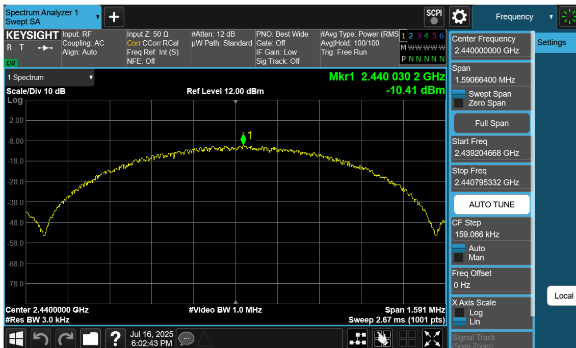
Plot 7-23. Power Spectral Density Plot Ant1 (Bluetooth (LE), 1Mbps, iPA – Ch. 19)
