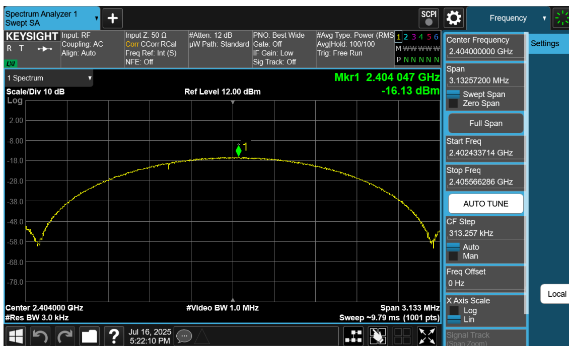
Plot 7-40. Power Spectral Density Plot Ant2 (Bluetooth (LE), 2Mbps, iPA – Ch. 1)
