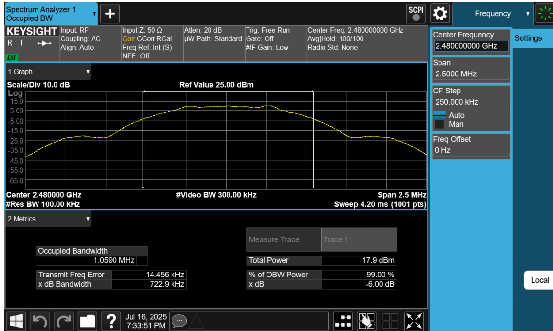
Plot 7-15. 6dB BW & 99% OBW Plot NB UNII_L (Bluetooth (LE), 1Mbps, iPA – Ch. 39)
