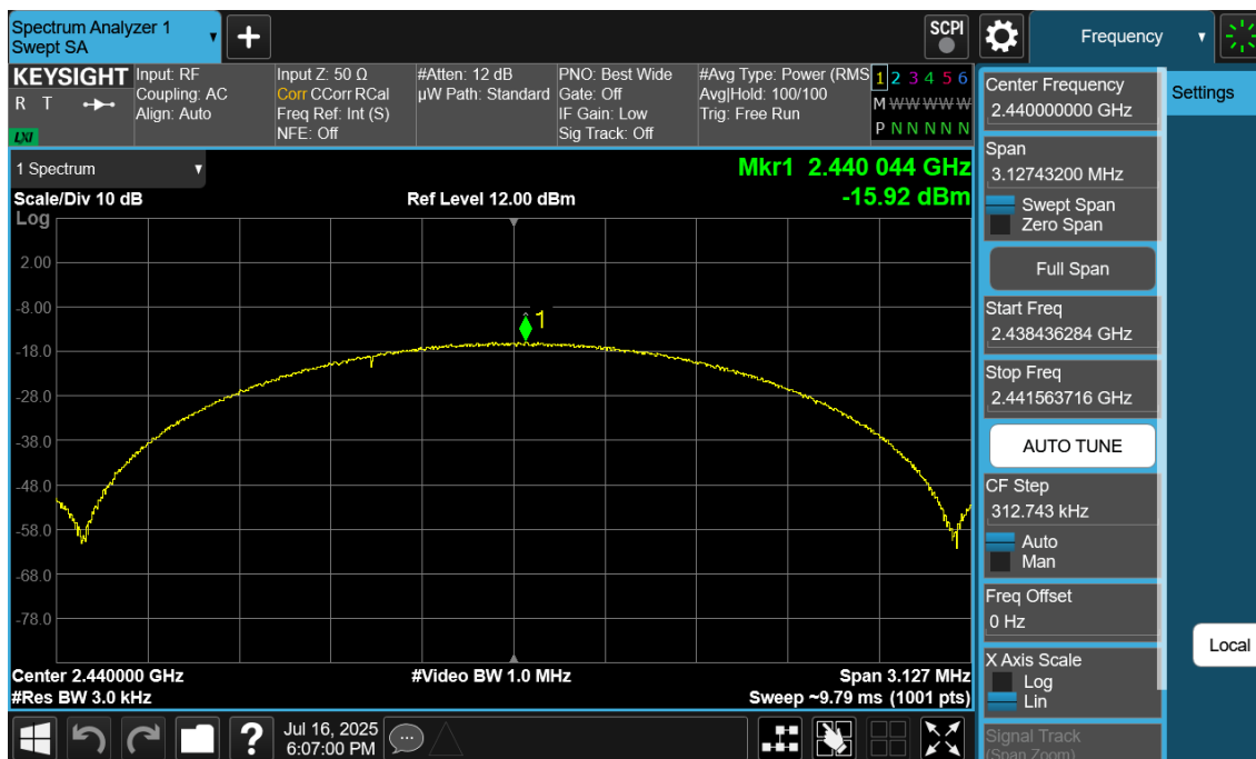
Plot 7-29. Power Spectral Density Plot Ant1 (Bluetooth (LE), 2Mbps, iPA – Ch. 19)
