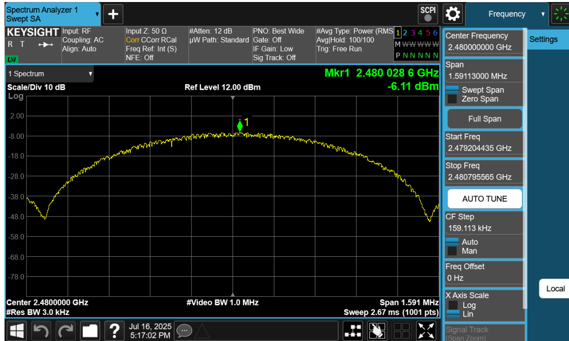
Plot 7-33. Power Spectral Density Plot Ant2 (Bluetooth (LE), 1Mbps, ePA – Ch. 39)
