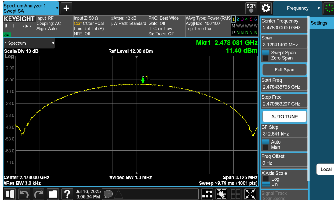
Plot 7-27. Power Spectral Density Plot Ant1 (Bluetooth (LE), 2Mbps, ePA – Ch. 38)
