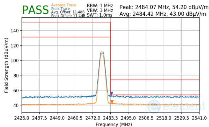
Plot 7-126. Radiated Restricted Upper Band Edge Measurement TxBF (Average & Peak)
