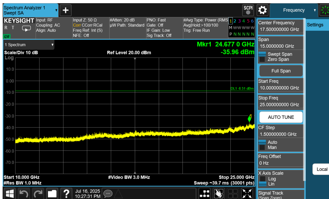
Plot 7-100. Conducted Spurious Plot NB UNII_L (Bluetooth (LE), 1Mbps, iPA – Ch. 19)
