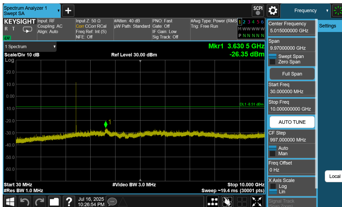
Plot 7-99. Conducted Spurious Plot NB UNII_L (Bluetooth (LE), 1Mbps, iPA – Ch. 19)
