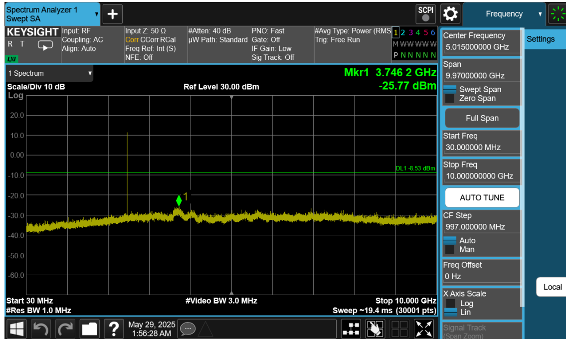
Plot 7-95. Conducted Spurious Plot Ant2 (Bluetooth (LE), 1Mbps, ePA – Ch. 39)
