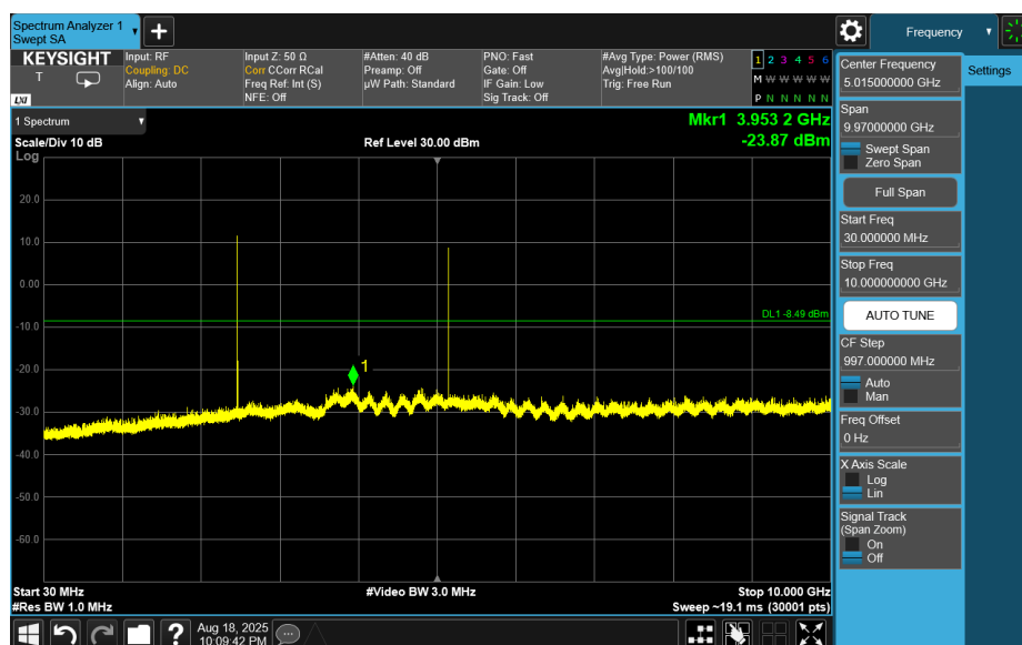
Plot 7-103. Conducted Spurious Plot Simultaneous Transmission
