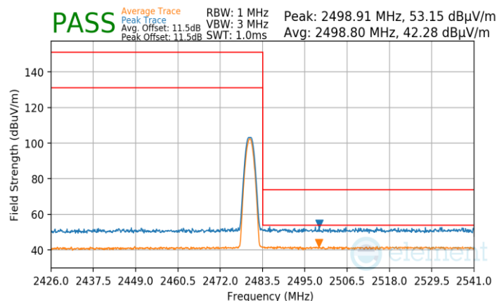
Plot 7-112. Radiated Restricted Upper Band Edge Measurement Ant1 (Average & Peak)
