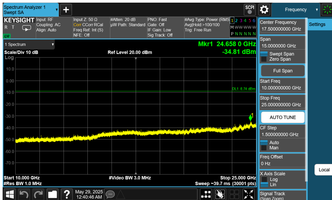
Plot 7-90. Conducted Spurious Plot Ant1 (Bluetooth (LE), 1Mbps, ePA – Ch. 39)
