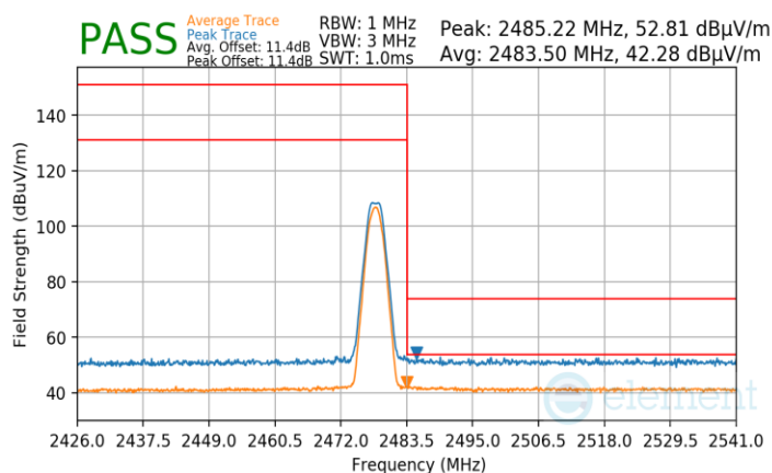
Plot 7-118. Radiated Restricted Upper Band Edge Measurement Ant2 (Average & Peak)
