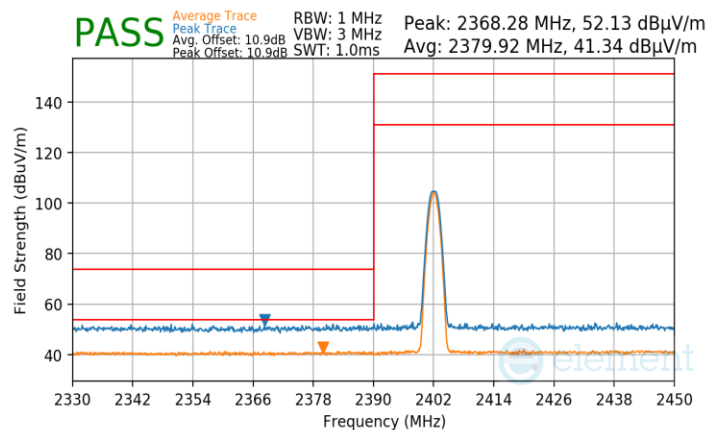
Plot 7-111. Radiated Restricted Lower Band Edge Measurement Ant1 (Average & Peak)
