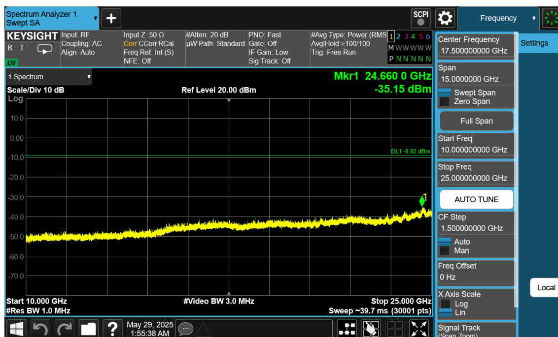
Plot 7-94. Conducted Spurious Plot Ant2 (Bluetooth (LE), 1Mbps, ePA – Ch. 19)
