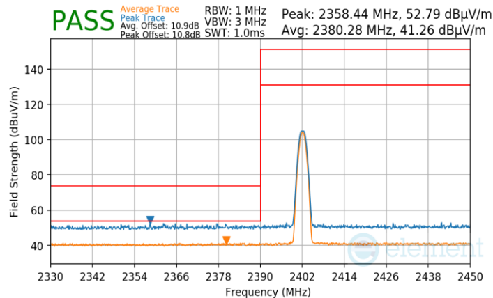
Plot 7-115. Radiated Restricted Lower Band Edge Measurement Ant2 (Average & Peak)
