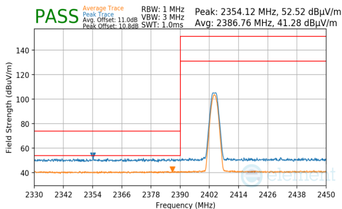
Plot 7-117. Radiated Restricted Lower Band Edge Measurement Ant2 (Average & Peak)
