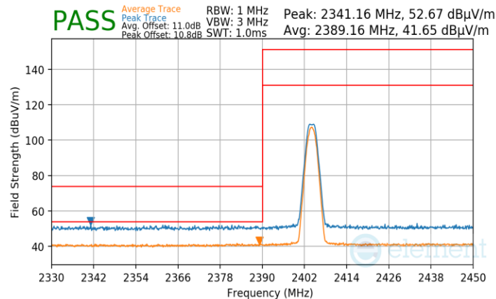
Plot 7-125. Radiated Restricted Lower Band Edge Measurement TxBF (Average & Peak)
