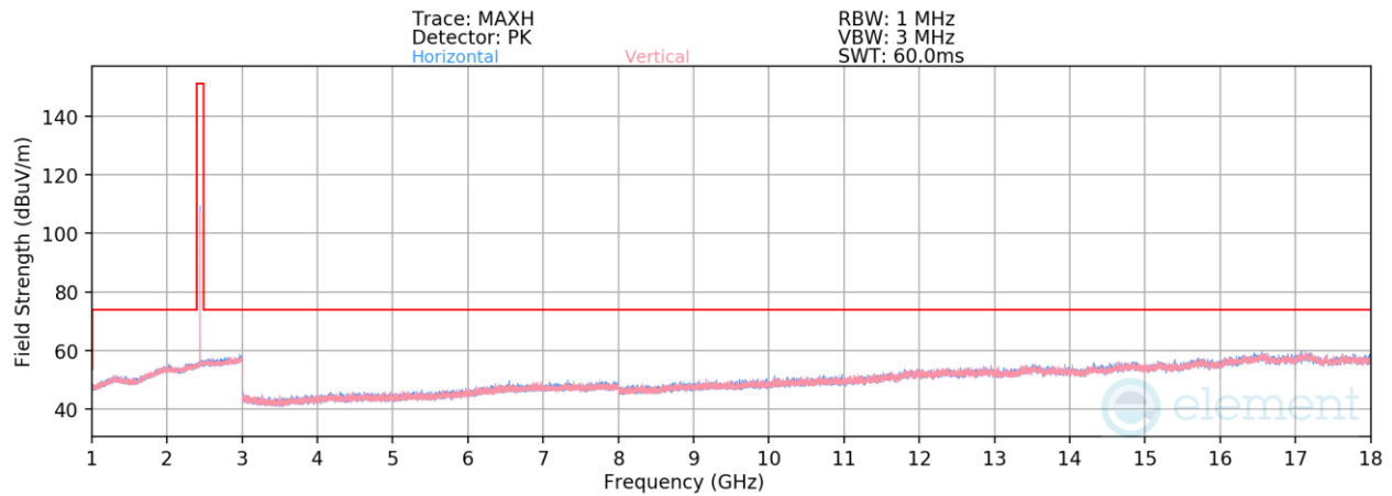
Plot 7-106. Radiated Spurious Emissions 1-18GHz TxBF (1Mbps, ePA – Ch. 19)
