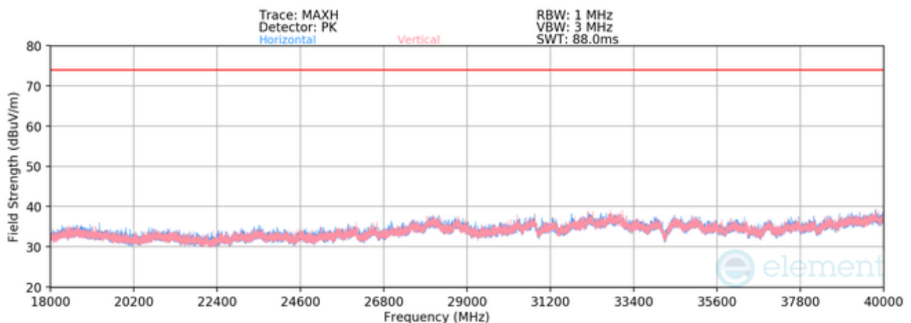
Plot 7-110. Radiated Spurious Emissions Simultaneous Transmission (Above 18GHz)
