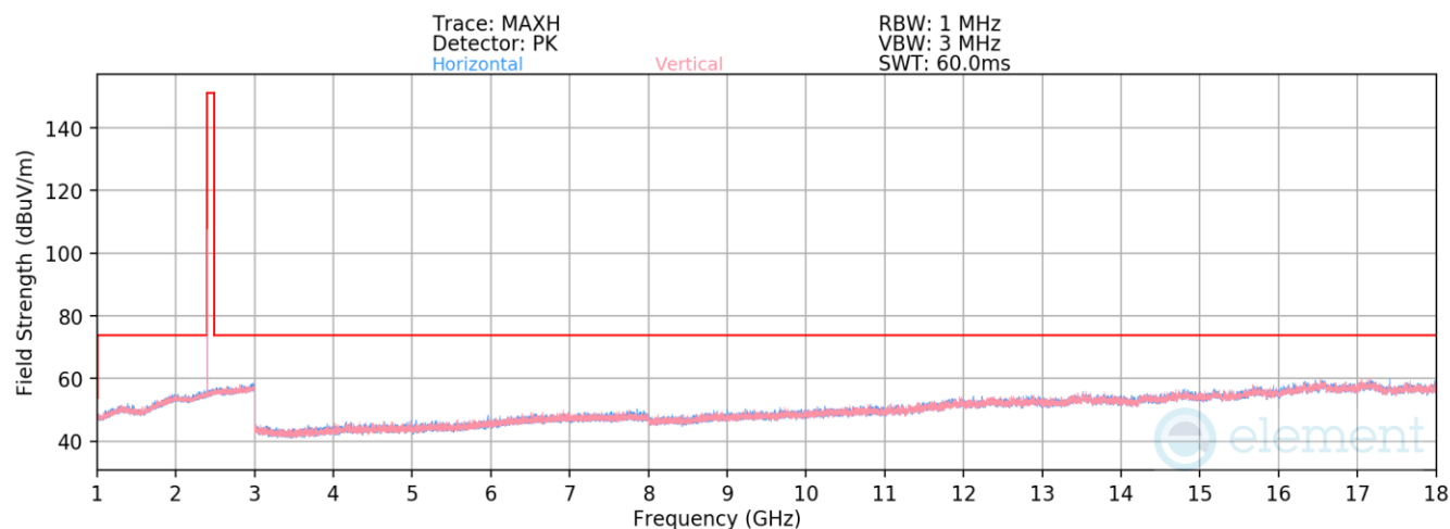
Plot 7-105. Radiated Spurious Emissions 1-18GHz TxBF (1Mbps, ePA – Ch. 0)
