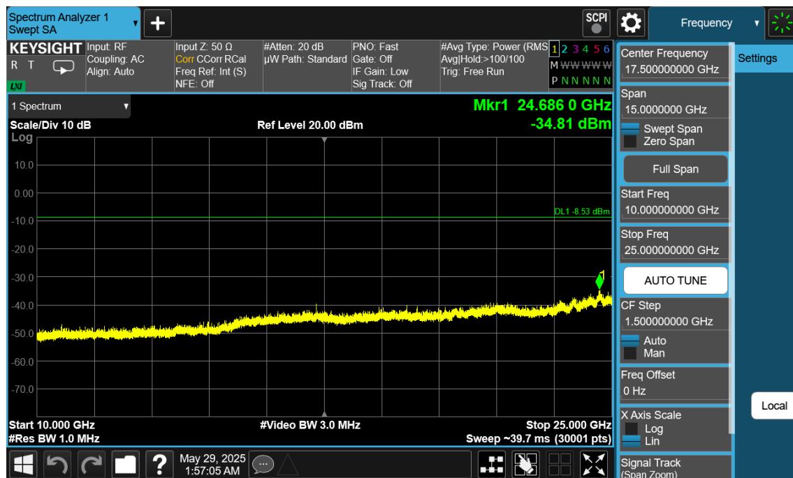
Plot 7-96. Conducted Spurious Plot Ant2 (Bluetooth (LE), 1Mbps, ePA – Ch. 39)
