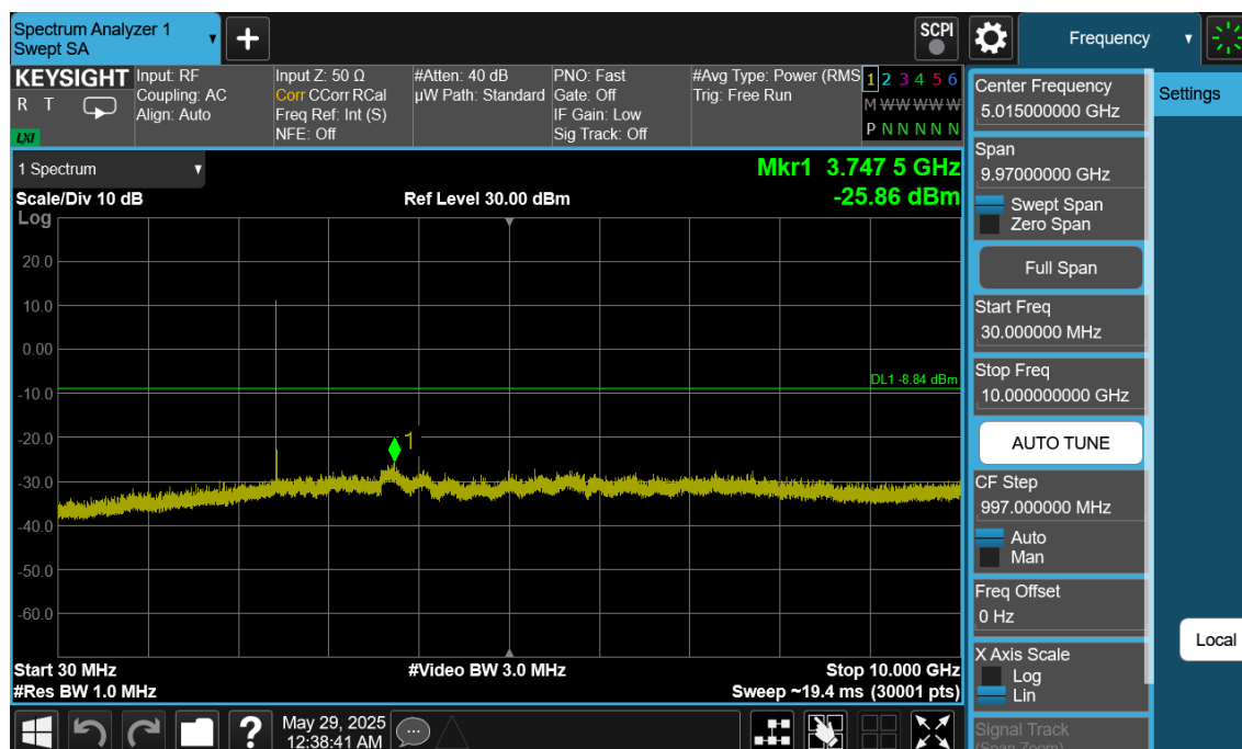
Plot 7-87. Conducted Spurious Plot Ant1 (Bluetooth (LE), 1Mbps, ePA – Ch. 19)
