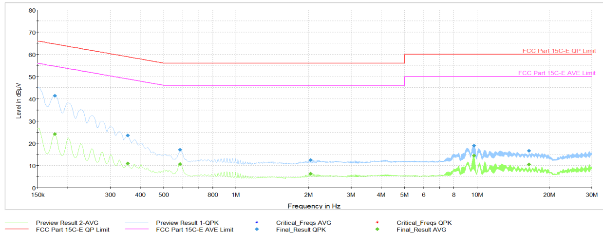
Plot 7-129. AC Line Conducted Plot with Bluetooth LE Tx BF (L1, 1Mbps ePA – Ch.19 with AC/DC Adapter)
