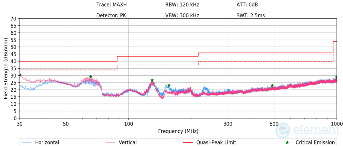
Plot 7-127. Radiated Spurious Emissions Below 1GHz TxBF (1Mbps, ePA – Ch.19, Pol. H & V, with AC/DC Adapter)
