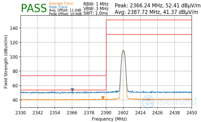
Plot 7-123. Radiated Restricted Lower Band Edge Measurement TxBF (Average & Peak)
