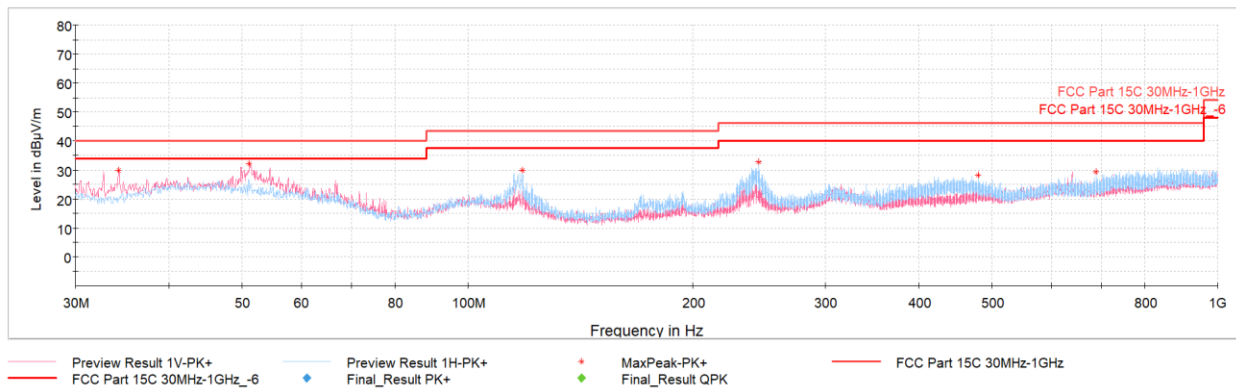
Plot 7-128. Radiated Spurious Emissions Simultaneous Transmission Below 1GHz (NB UNII & BLE 1M, with AC/DC Adapter)
