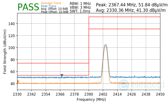
Plot 7-113. Radiated Restricted Lower Band Edge Measurement Ant1 (Average & Peak)
