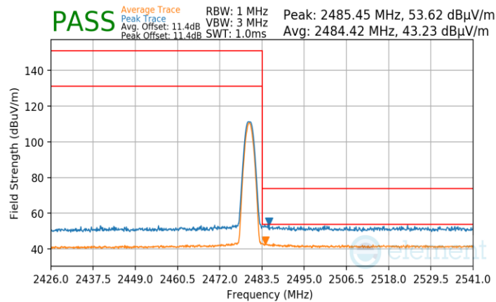
Plot 7-124. Radiated Restricted Upper Band Edge Measurement TxBF (Average & Peak)
