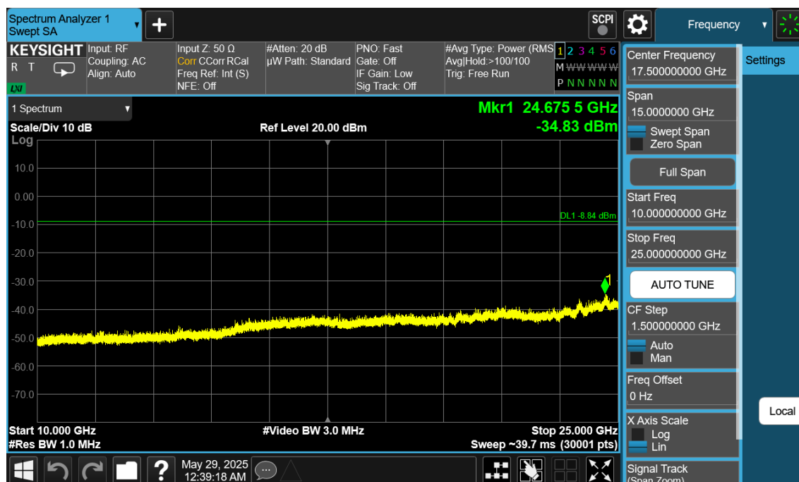
Plot 7-88. Conducted Spurious Plot Ant1 (Bluetooth (LE), 1Mbps, ePA – Ch. 19)
