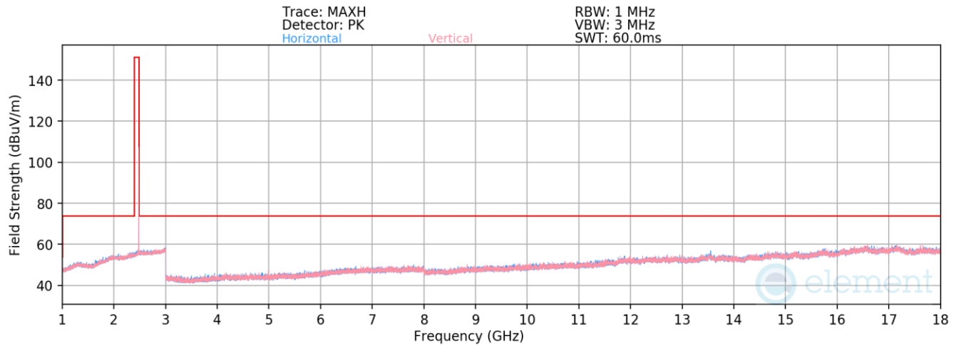
Plot 7-108. Radiated Spurious Emissions 1-18GHz TxBF (1Mbps ePA – Ch. 39)
