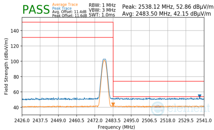
Plot 7-114. Radiated Restricted Upper Band Edge Measurement Ant1 (Average & Peak)
