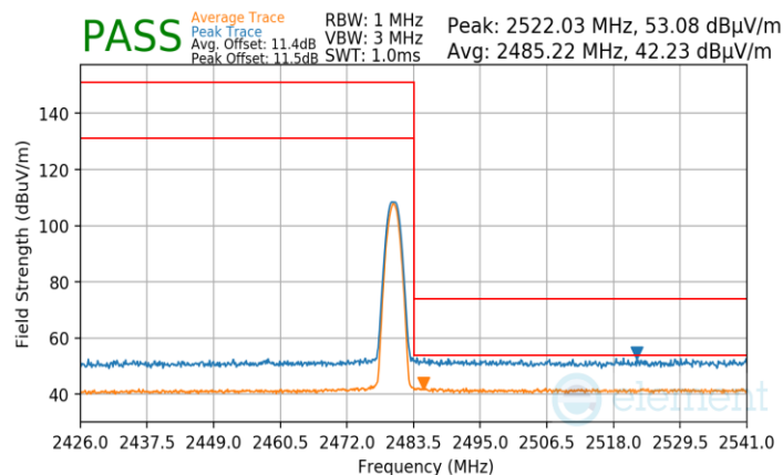
Plot 7-116. Radiated Restricted Upper Band Edge Measurement Ant2 (Average & Peak)
