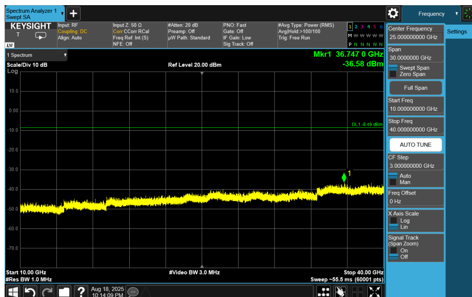
Plot 7-104. Conducted Spurious Plot Simultaneous Transmission
