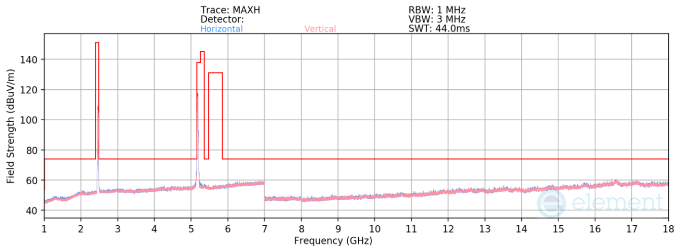
Plot 7-109. Radiated Spurious Emissions Simultaneous Transmission (1-18GHz)
