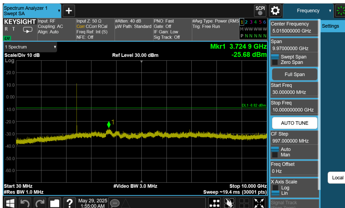
Plot 7-93. Conducted Spurious Plot Ant2 (Bluetooth (LE), 1Mbps, ePA – Ch. 19)
