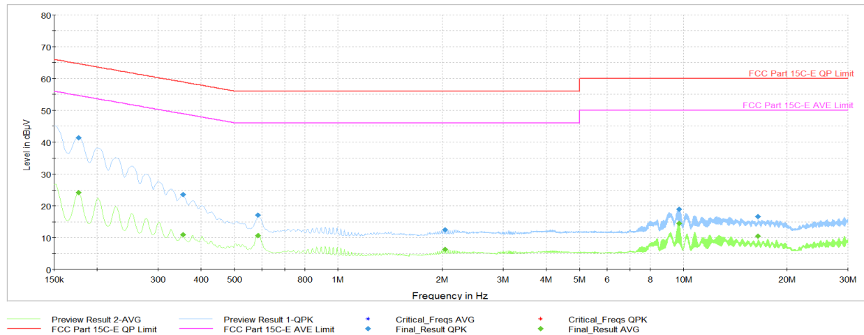
Plot 7-130. AC Line Conducted Plot with Bluetooth LE Tx BF (N, 1Mbps ePA – Ch.19, with AC/DC Adapter)
