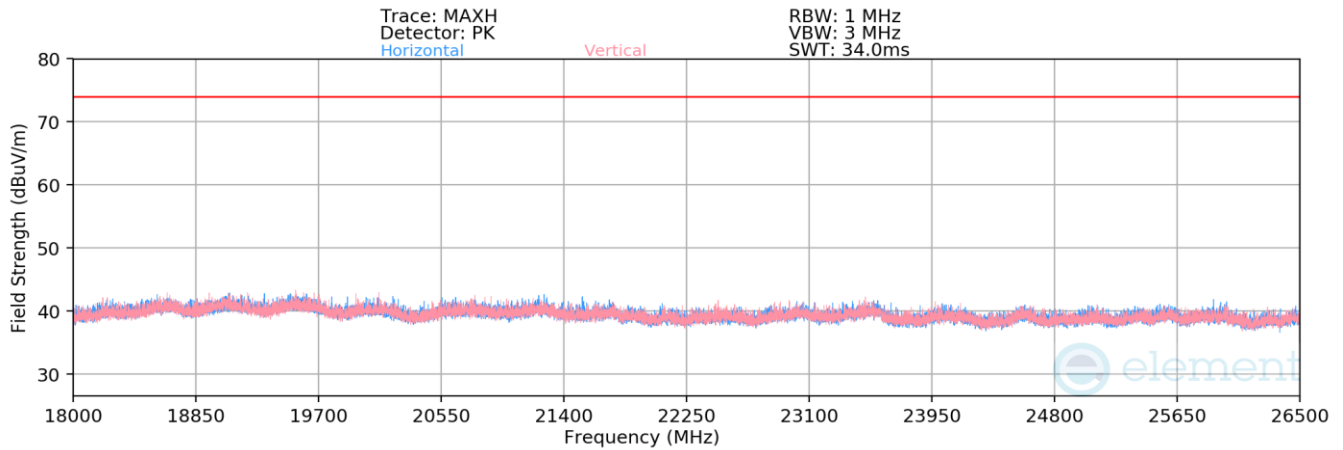
Plot 7-107. Radiated Spurious Emissions Above 18GHz TxBF (1Mbps ePA – Ch. 19)
