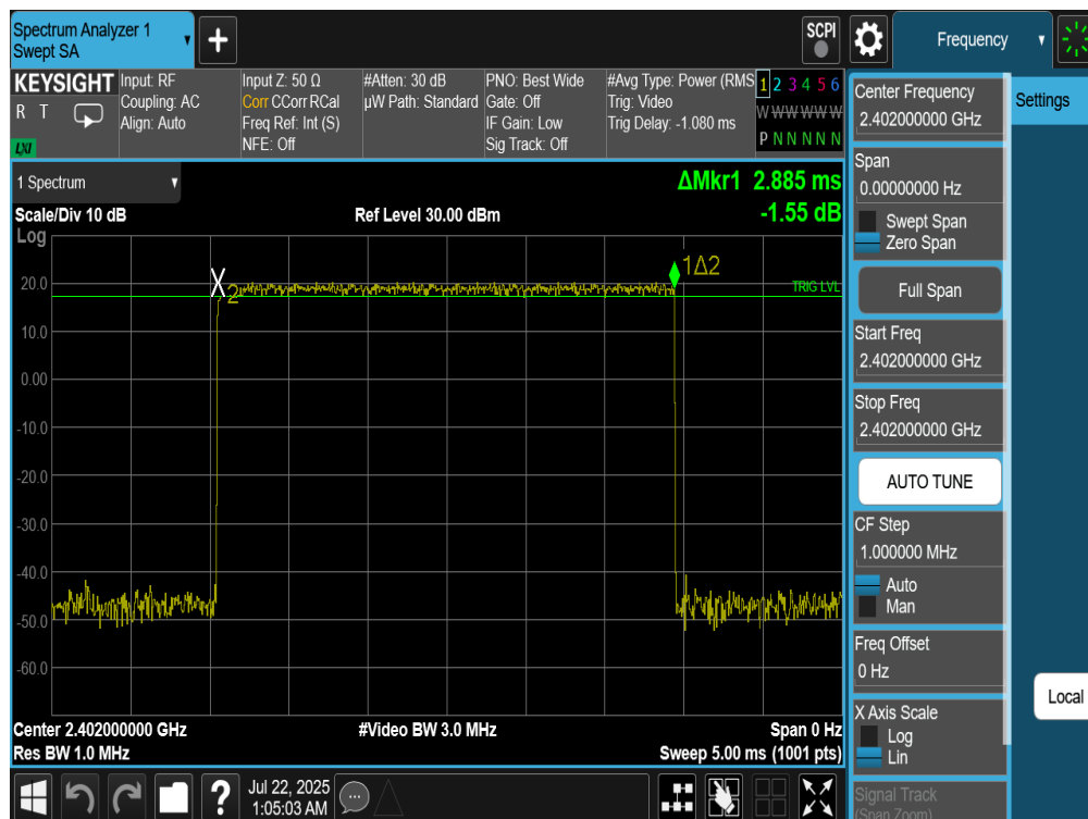
Plot 7-52. Time of Occupancy Plot Ant2 (Bluetooth, 8DPSK, ePA)
