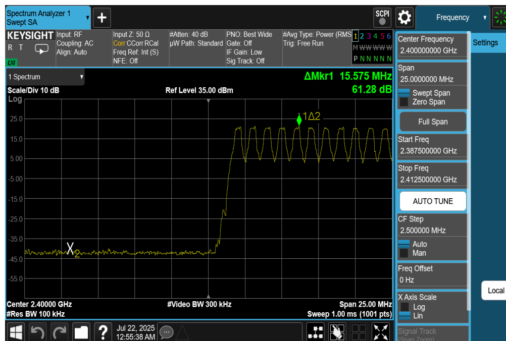
Plot 7-29. Band Edge Plot Ant2 (Bluetooth with Hopping Enabled, GFSK, ePA – Ch. 0)
