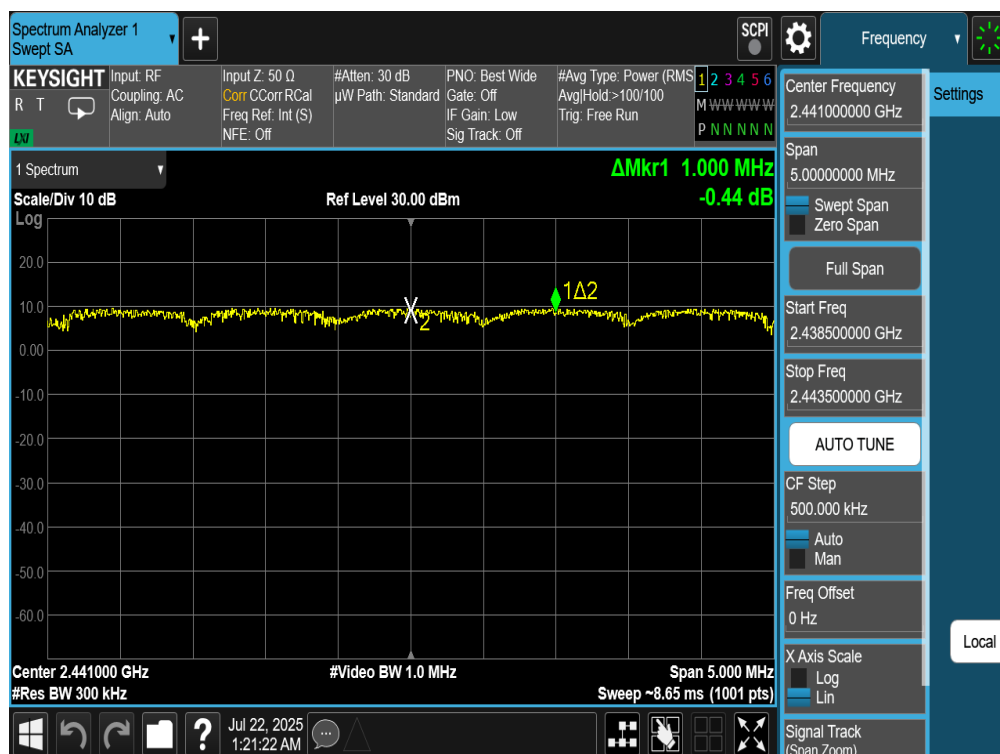
Plot 7-48. Channel Spacing Plot Antenna NB UNII_L (Bluetooth, 8DPSK, iPA)
