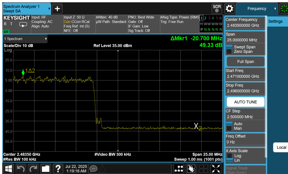
Plot 7-42. Band Edge Plot NB UNII_L (Bluetooth with Hopping Enabled, 8DPSK, iPA – Ch. 78)
