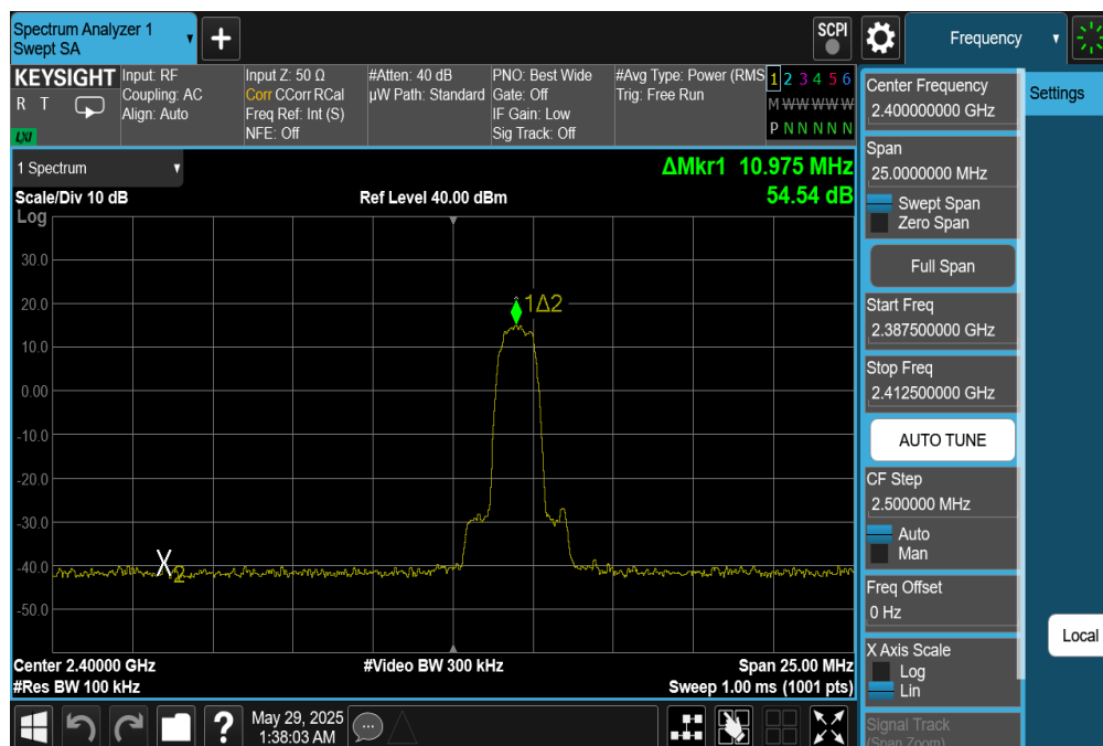
Plot 7-31. Band Edge Plot Ant2 (Bluetooth with Hopping Disabled, 8DPSK, ePA – Ch. 0)
