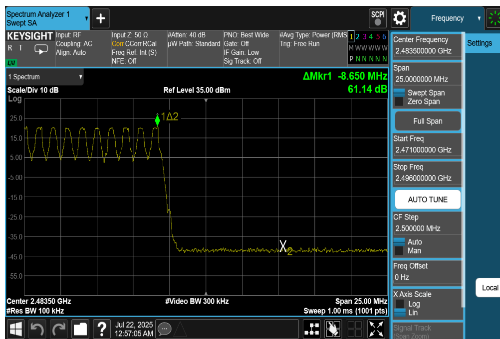
Plot 7-30. Band Edge Plot Ant2 (Bluetooth with Hopping Enabled, GFSK, ePA – Ch. 78)
