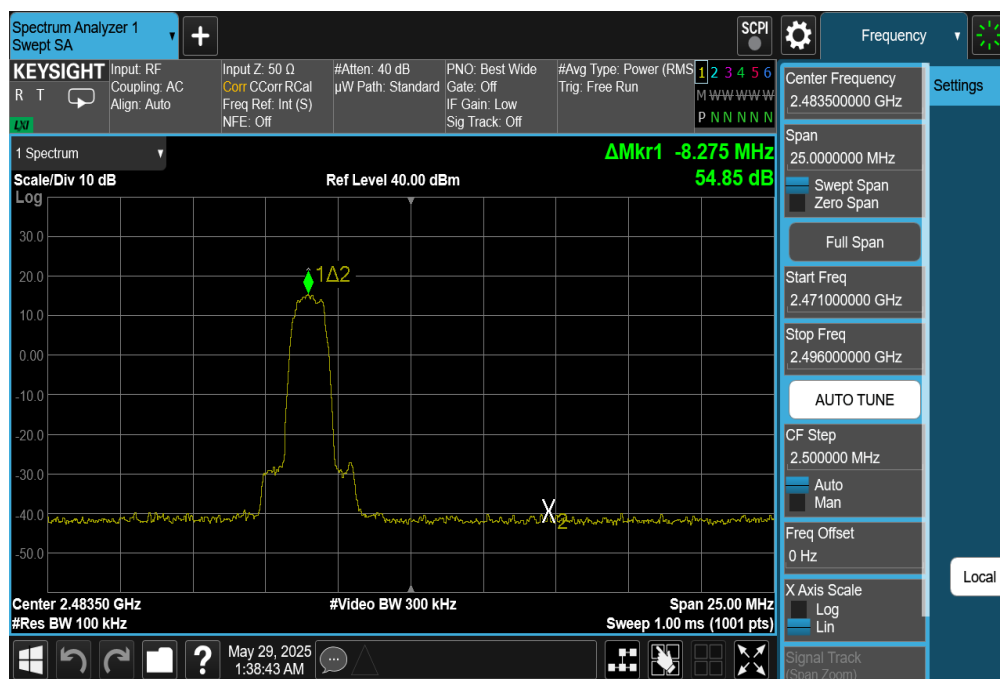
Plot 7-32. Band Edge Plot Ant2 (Bluetooth with Hopping Disabled, 8DPSK, ePA – Ch. 78)
