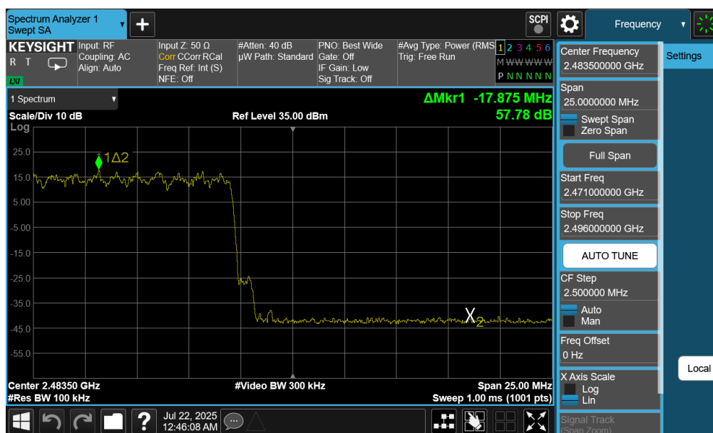
Plot 7-26. Band Edge Plot Ant1 (Bluetooth with Hopping Enabled, 8DPSK, ePA – Ch. 78)
