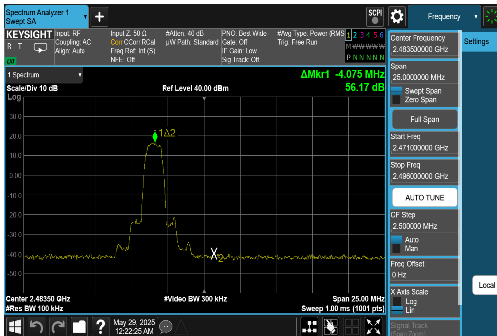
Plot 7-24. Band Edge Plot Ant1 (Bluetooth with Hopping Disabled, 8DPSK, ePA – Ch. 78)
