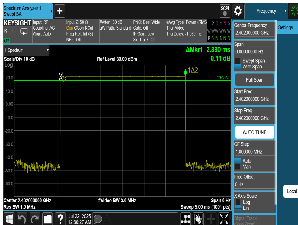
Plot 7-49. Time of Occupancy Plot Ant1 (Bluetooth, GFSK, ePA)
