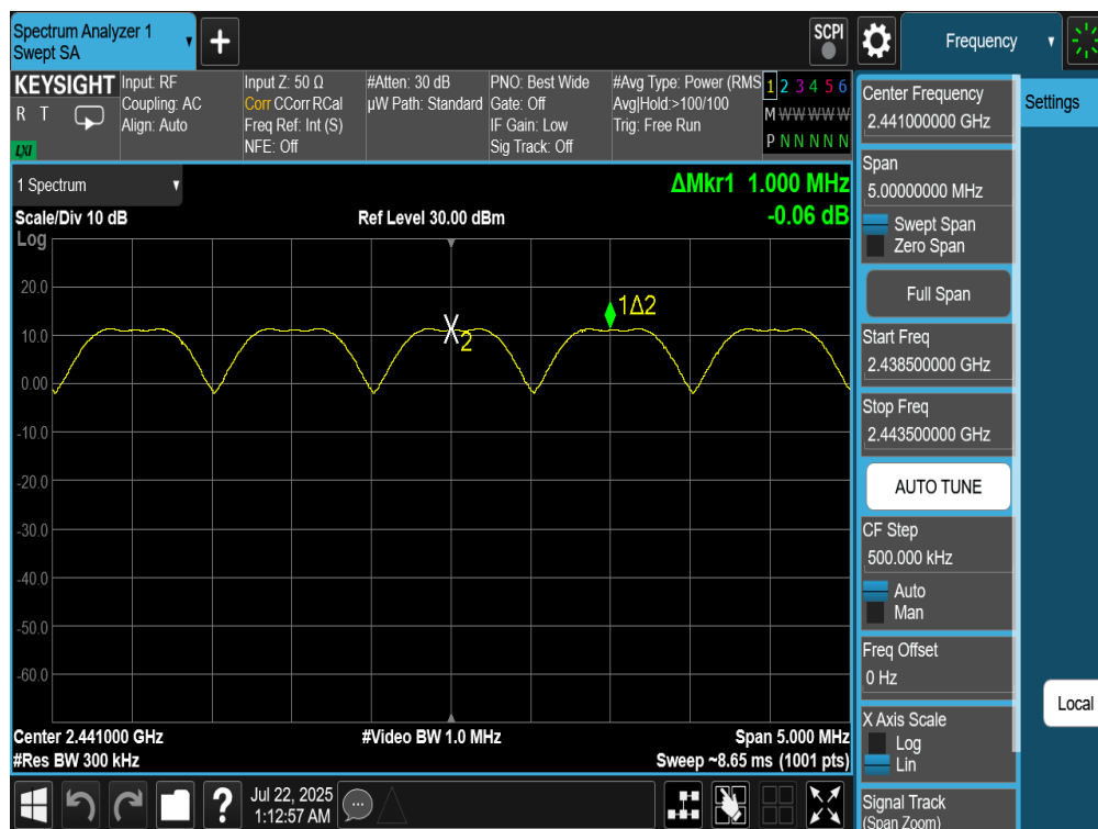
Plot 7-47. Channel Spacing Plot Antenna NB UNII_L (Bluetooth, GFSK, iPA)
