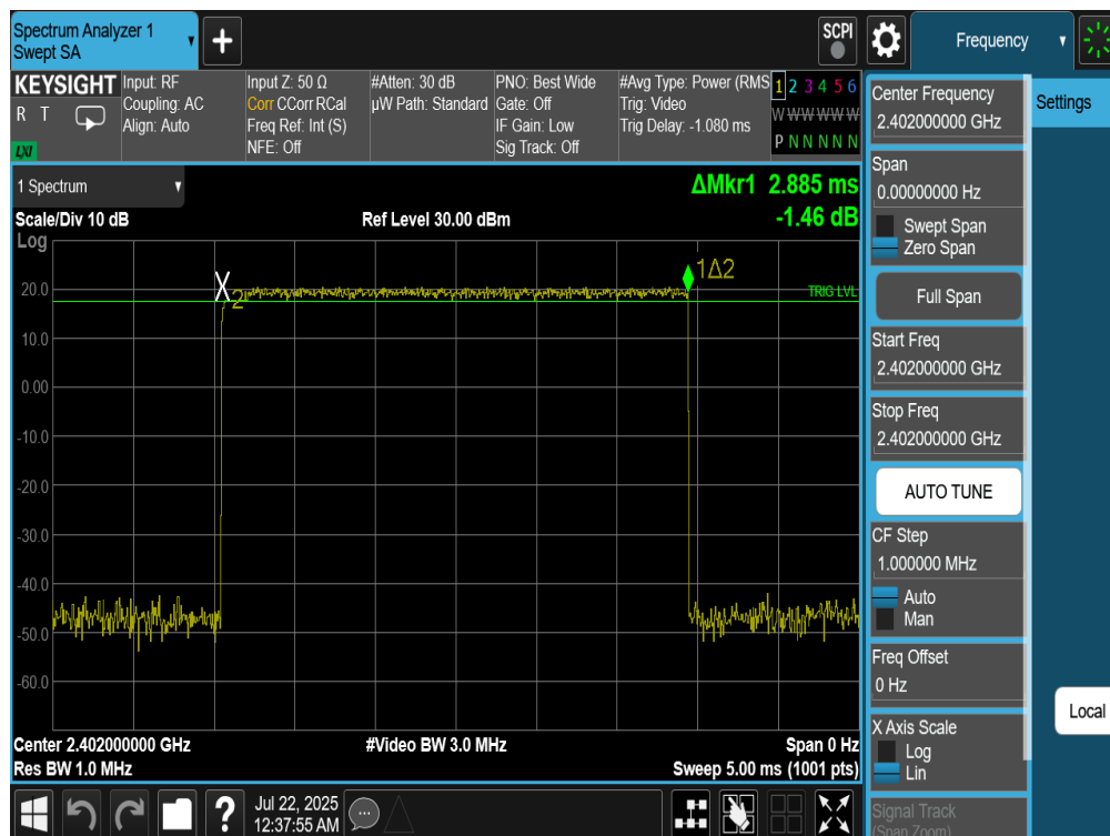
Plot 7-50. Time of Occupancy Plot Ant1 (Bluetooth, 8DPSK, ePA)
