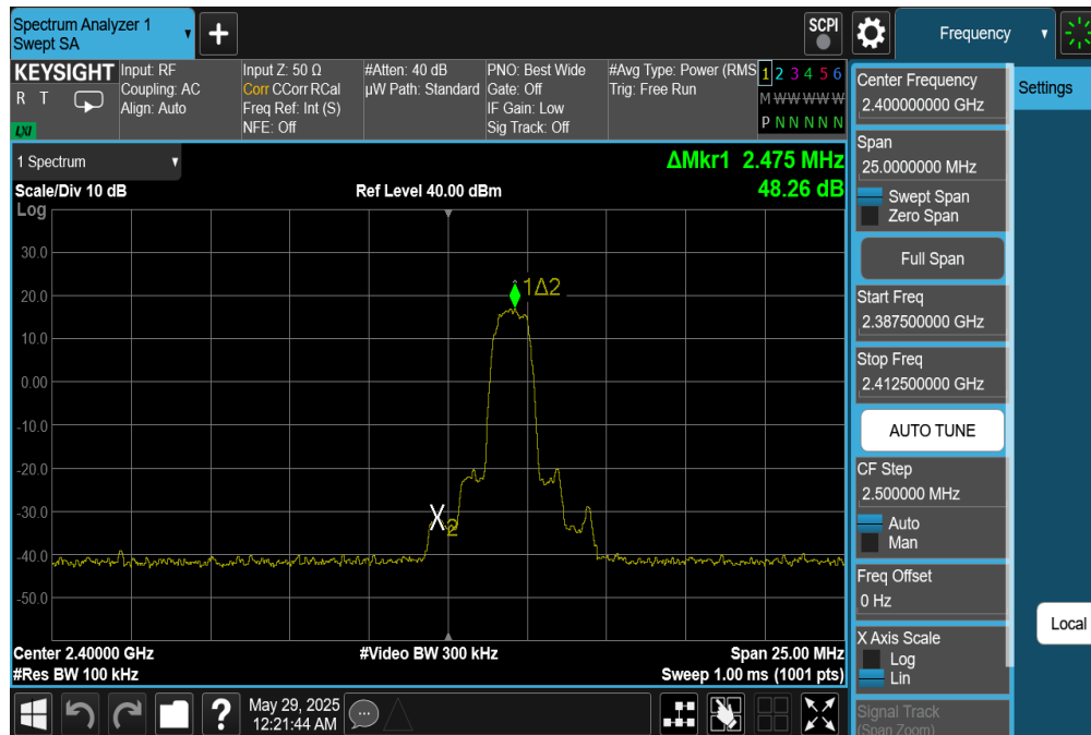
Plot 7-23. Band Edge Plot Ant1 (Bluetooth with Hopping Disabled, 8DPSK, ePA – Ch. 0)
