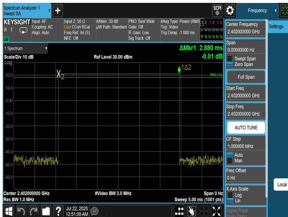
Plot 7-51. Time of Occupancy Plot Ant2 (Bluetooth, GFSK, ePA)
