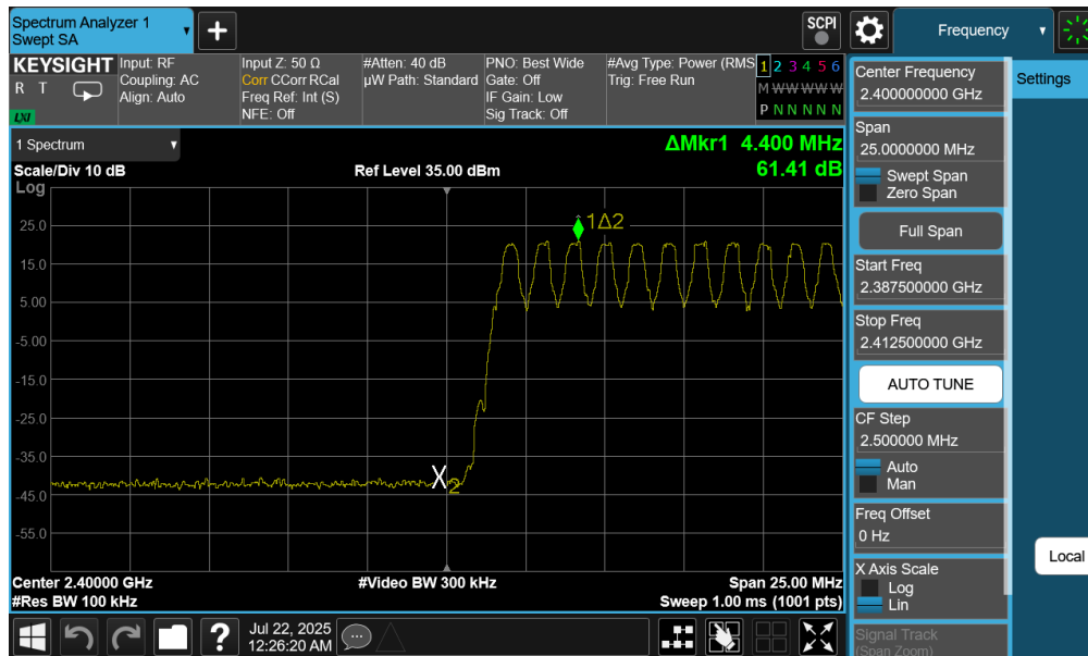
Plot 7-21. Band Edge Plot Ant1 (Bluetooth with Hopping Enabled, GFSK, ePA – Ch. 0)
