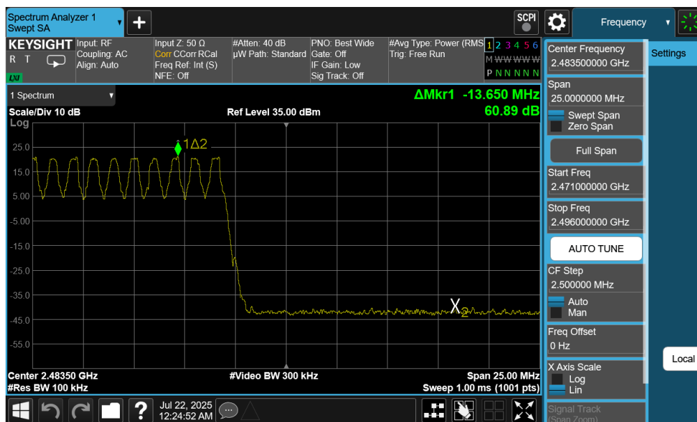
Plot 7-22. Band Edge Plot Ant1 (Bluetooth with Hopping Enabled, GFSK, ePA – Ch. 78)
