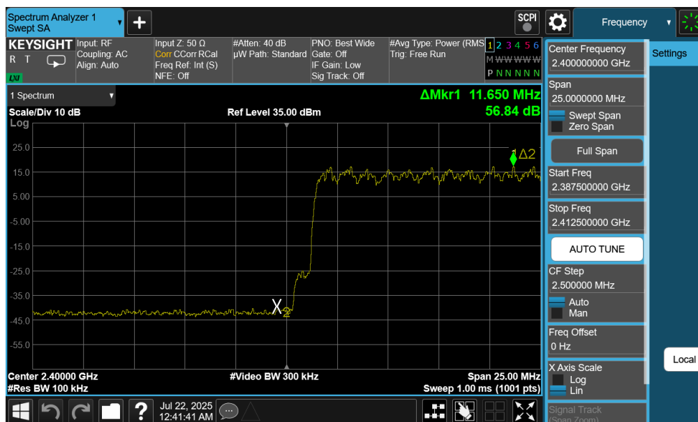
Plot 7-25. Band Edge Plot Ant1 (Bluetooth with Hopping Enabled, 8DPSK, ePA – Ch. 0)
