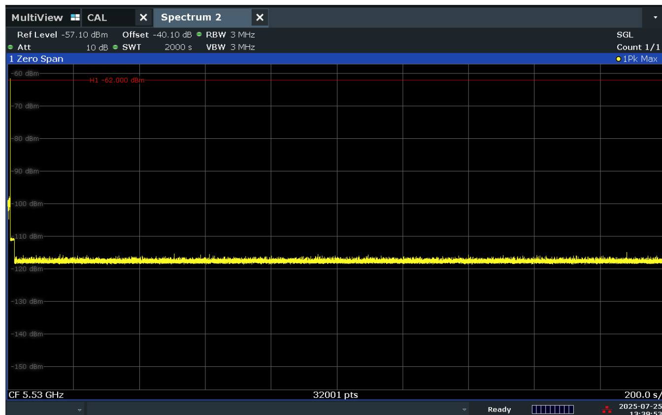
Figure 9-16. 5530MHz - Non-Occupancy Period (30 Minutes) - Mode 4 (80MHz)
