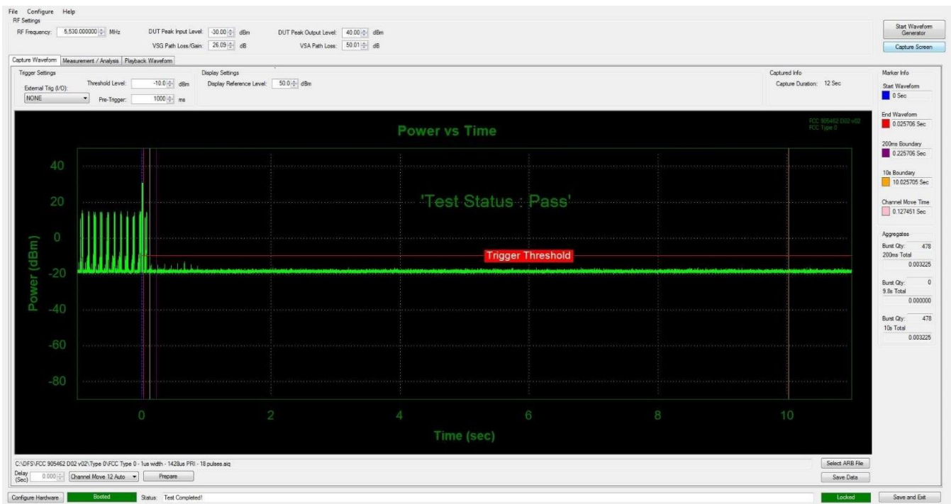
Figure 9-9. 5530MHz - Channel Move/ Closing Transmission Time - Mode 1 (80 MHz)
