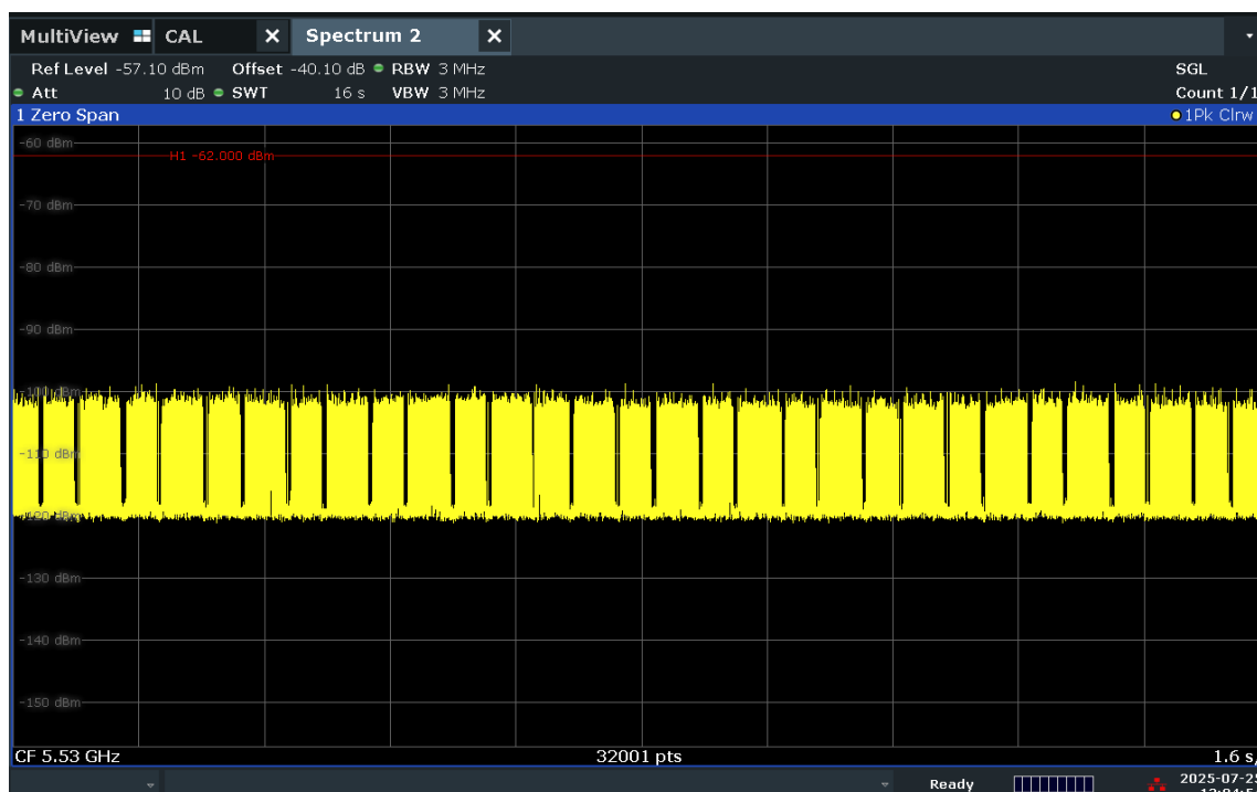
Figure 9-7. 5530 MHz - Channel Loading - Mode 4 (80MHz)
