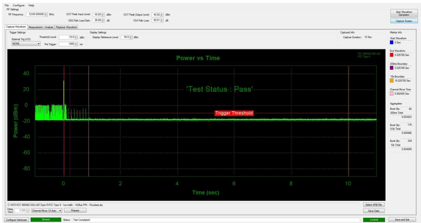
Figure 9-11. 5530MHz - Channel Move/ Closing Transmission Time - Mode 3 (80 MHz)
