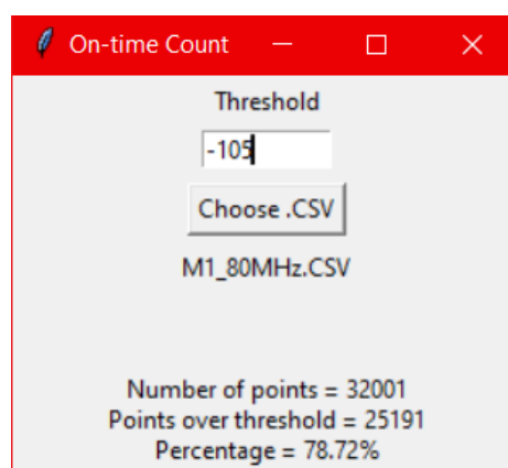
Figure 9-2. 5530MHz - Channel Loading Calculation - Mode 1 (80MHz)
