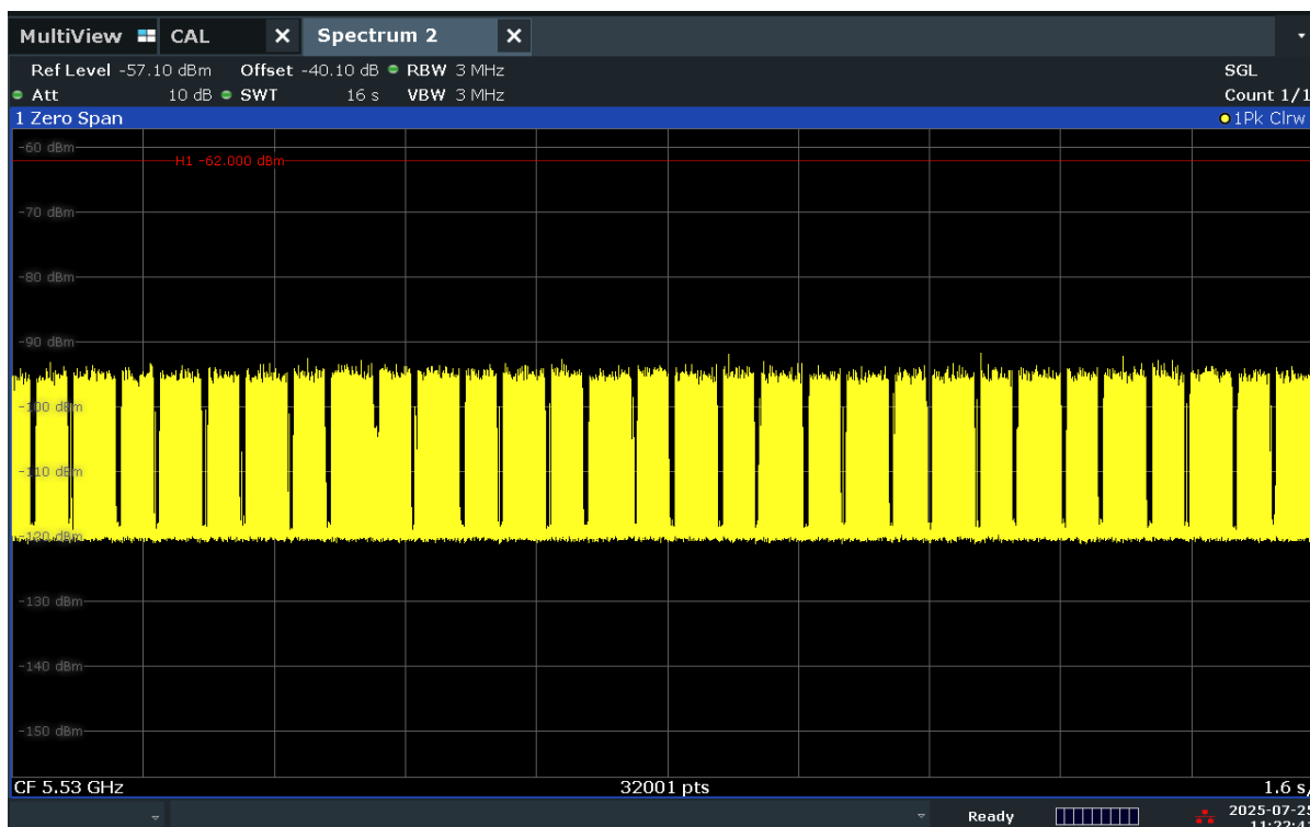
Figure 9-5. 5530MHz - Channel Loading - Mode 3 (80MHz)
