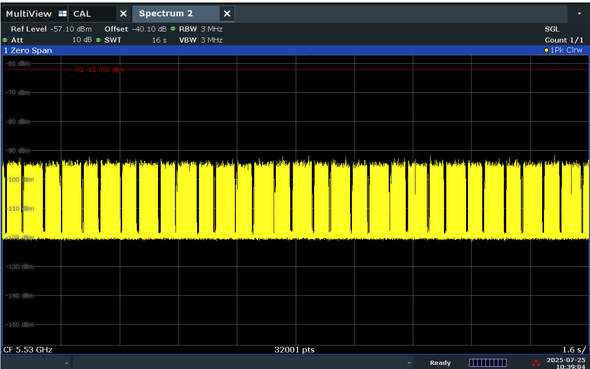
Figure 9-3. 5530MHz - Channel Loading - Mode 2 (80MHz)
