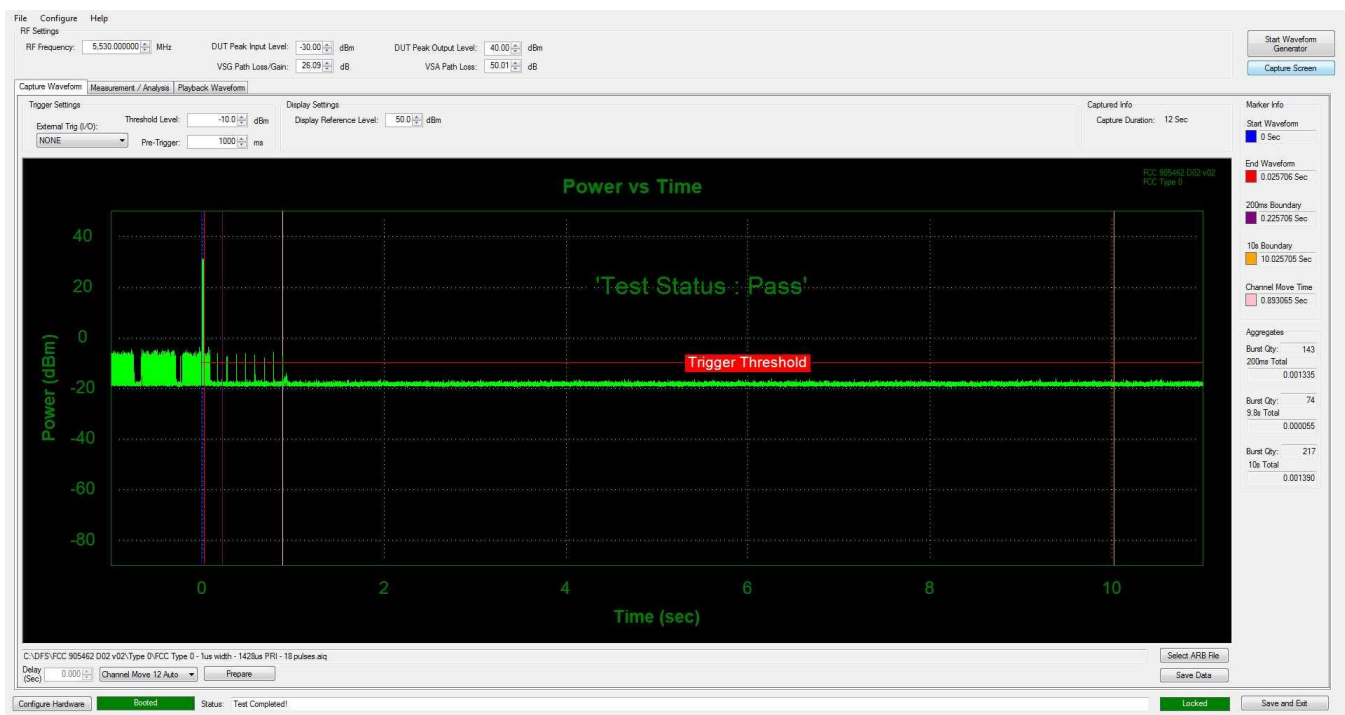
Figure 9-12. 5530MHz - Channel Move/ Closing Transmission Time - Mode 4 (80 MHz)
