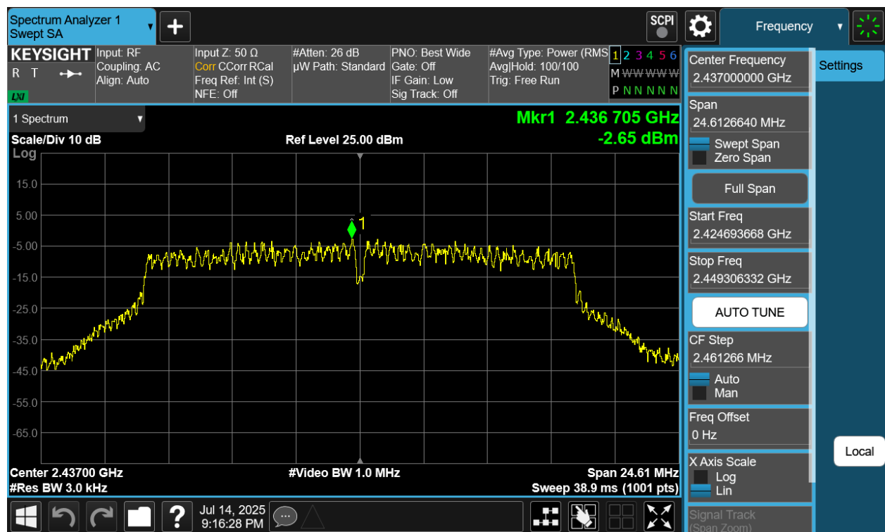
Plot 7-10. Power Spectral Density Plot Ant1 (802.11g – Ch. 6)
