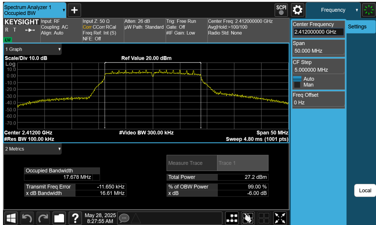
Plot 7-7. 6 dB BW and 99% OBW Plot Ant2 (802.11n – Ch. 1)
