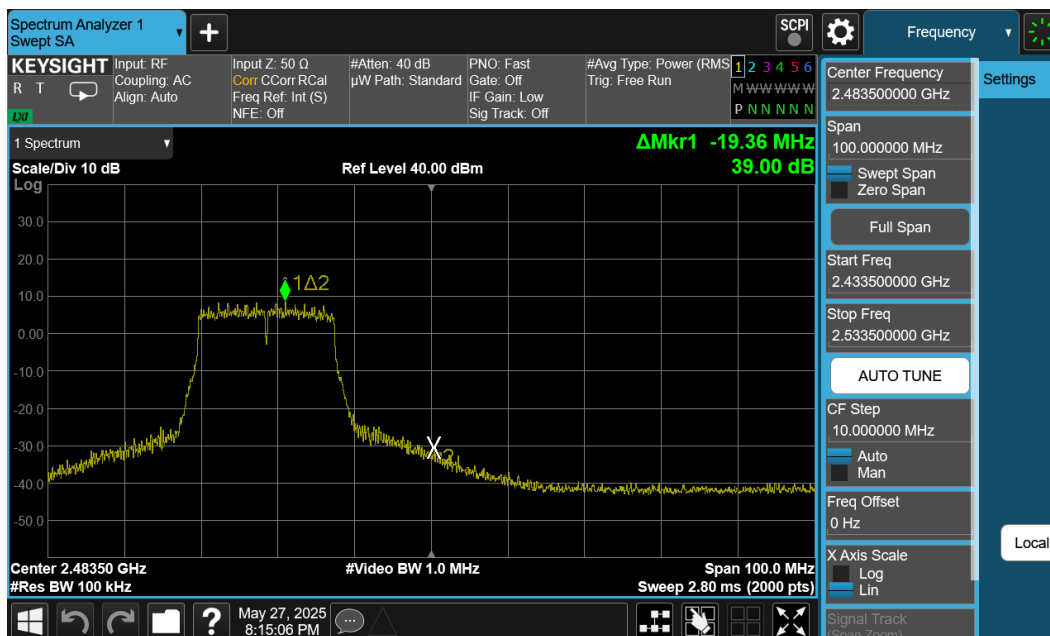
Plot 7-49. Band Edge Plot Ant1 (802.11n (2.4GHz) – Ch. 11)
