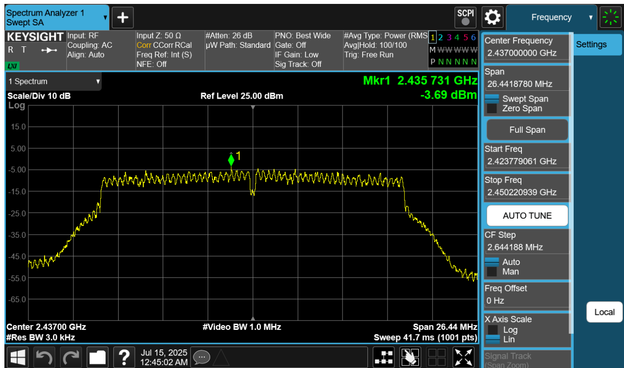
Plot 7-20. Power Spectral Density Plot CDD Ant2 (802.11n – Ch. 6)
