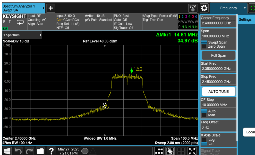
Plot 7-28. Band Edge Plot Ant1 (802.11g – Ch. 1)
