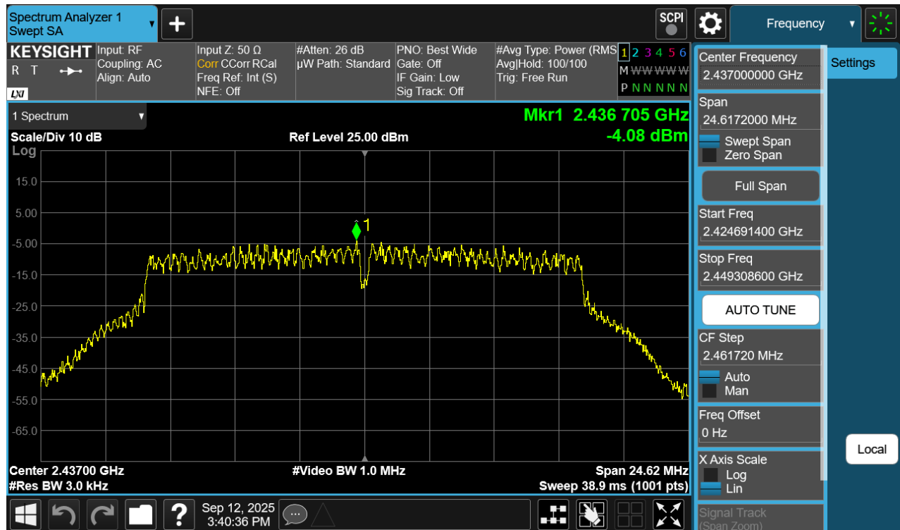
Plot 7-18. Power Spectral Density Plot CDD Ant2 (802.11g – Ch. 6)
