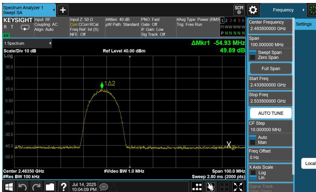
Plot 7-27. Band Edge Plot Ant1 (802.11b – Ch. 13)
