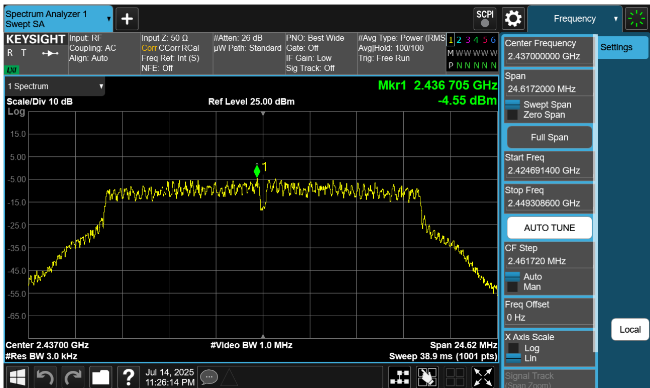
Plot 7-14. Power Spectral Density Plot Ant2 (802.11g – Ch. 6)
