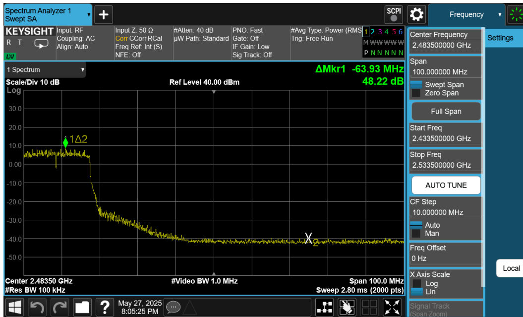
Plot 7-45. Band Edge Plot Ant1 (802.11n (2.4GHz) – Ch. 7)
