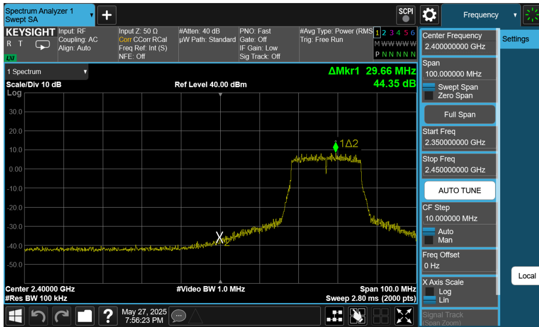
Plot 7-43. Band Edge Plot Ant1 (802.11n (2.4GHz) – Ch. 4)
