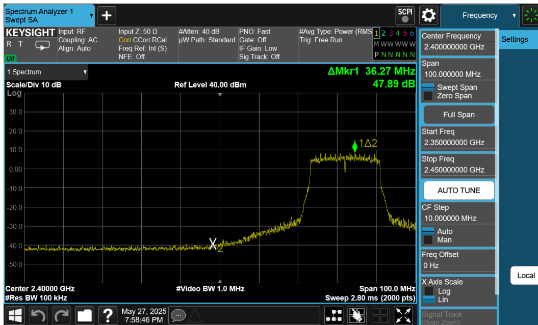
Plot 7-44. Band Edge Plot Ant1 (802.11n (2.4GHz) – Ch. 5)
