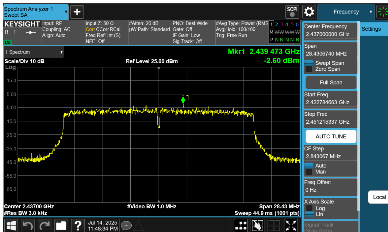
Plot 7-16. Power Spectral Density Plot Ant2 (802.11ax SU – Ch. 6)
