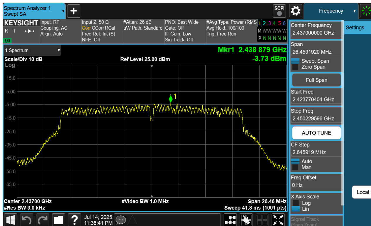
Plot 7-15. Power Spectral Density Plot Ant2 (802.11n – Ch. 6)
