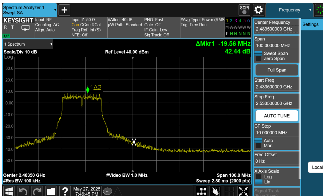
Plot 7-37. Band Edge Plot Ant1 (802.11g – Ch. 11)
