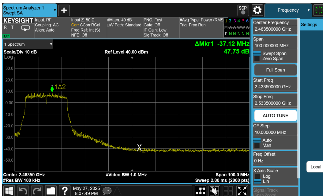
Plot 7-46. Band Edge Plot Ant1 (802.11n (2.4GHz) – Ch. 7)
