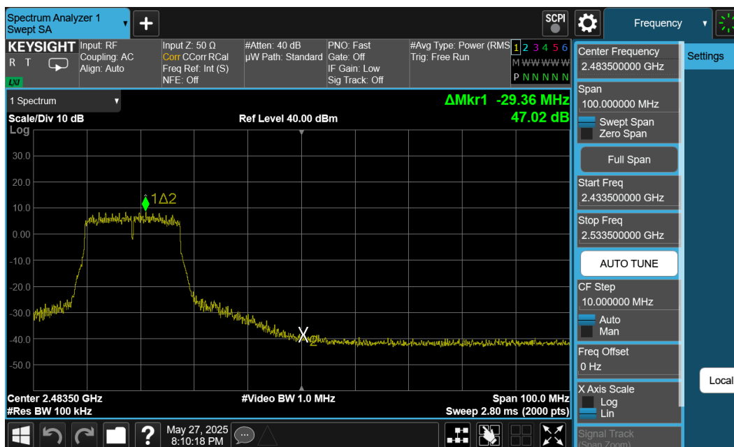
Plot 7-47. Band Edge Plot Ant1 (802.11n (2.4GHz) – Ch. 9)
