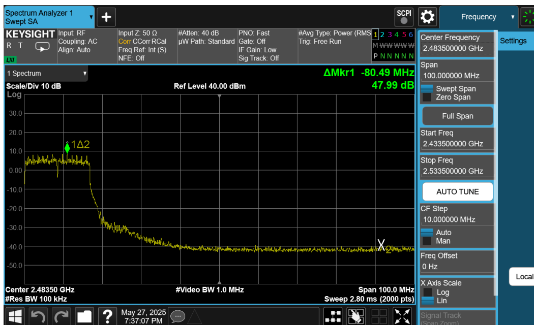
Plot 7-33. Band Edge Plot Ant1 (802.11g – Ch. 7)
