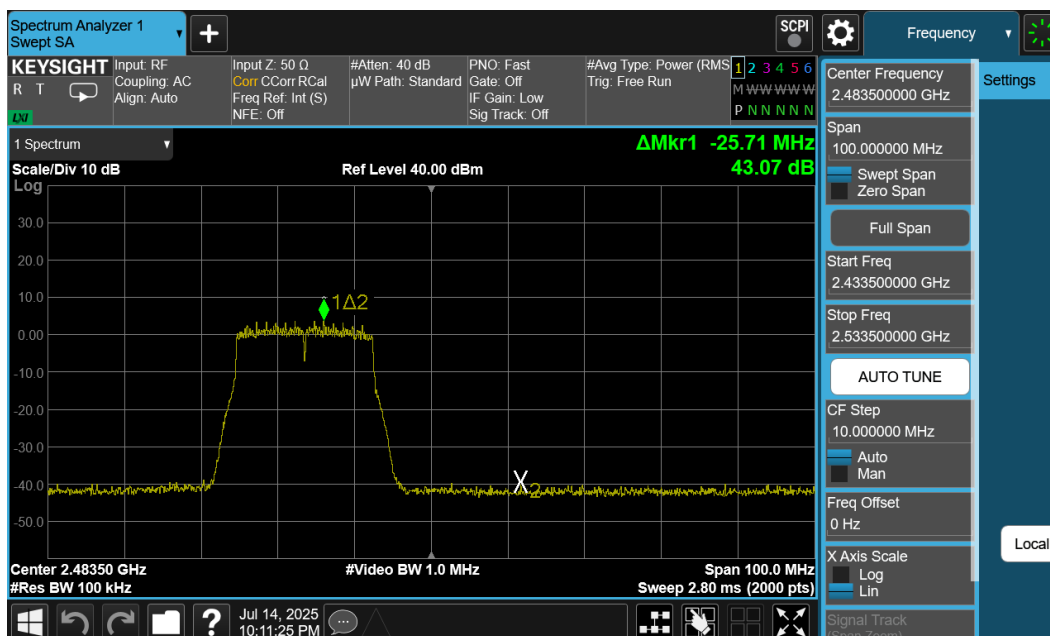
Plot 7-50. Band Edge Plot Ant1 (802.11n (2.4GHz) – Ch. 12)
