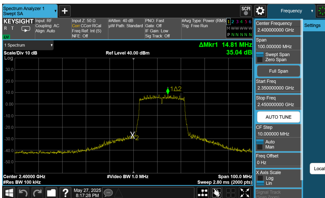
Plot 7-52. Band Edge Plot Ant1 (802.11ax (SU - 2.4GHz) – Ch. 1)
