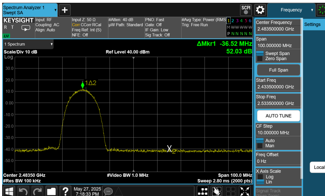
Plot 7-25. Band Edge Plot Ant1 (802.11b – Ch. 11)
