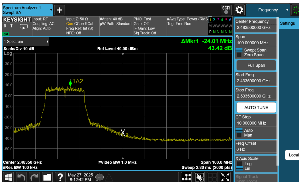
Plot 7-48. Band Edge Plot Ant1 (802.11n (2.4GHz) – Ch. 10)
