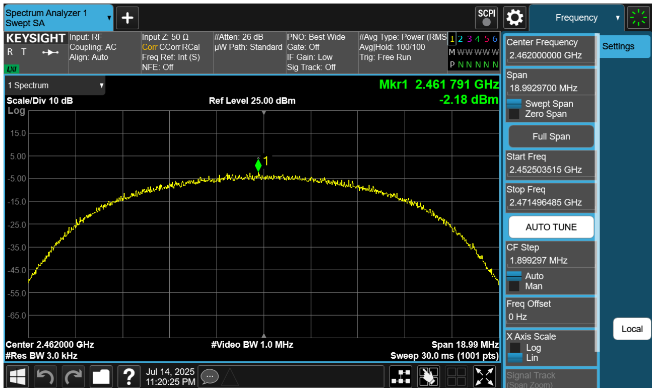
Plot 7-13. Power Spectral Density Plot Ant2 (802.11b – Ch. 11)
