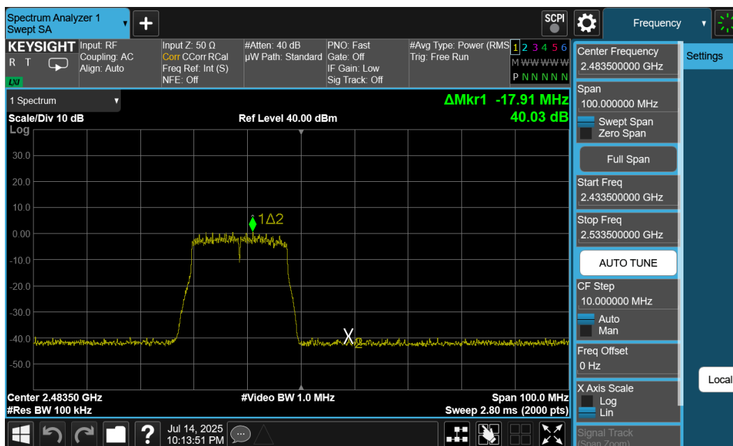
Plot 7-51. Band Edge Plot Ant1 (802.11n (2.4GHz) – Ch. 13)
