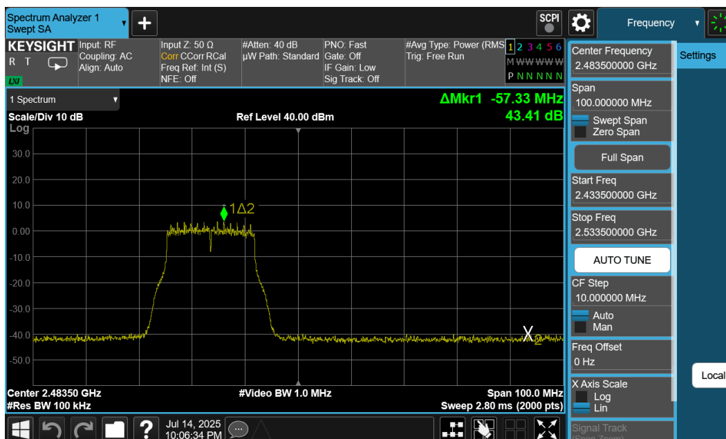
Plot 7-38. Band Edge Plot Ant1 (802.11g – Ch. 12)
