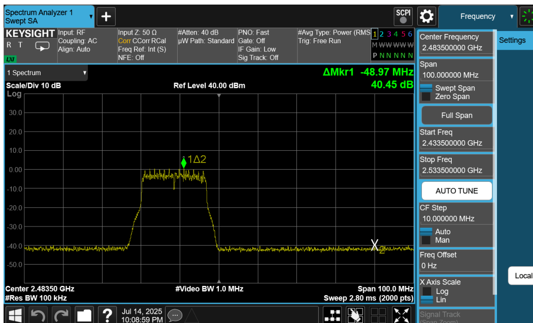
Plot 7-39. Band Edge Plot Ant1 (802.11g – Ch. 13)
