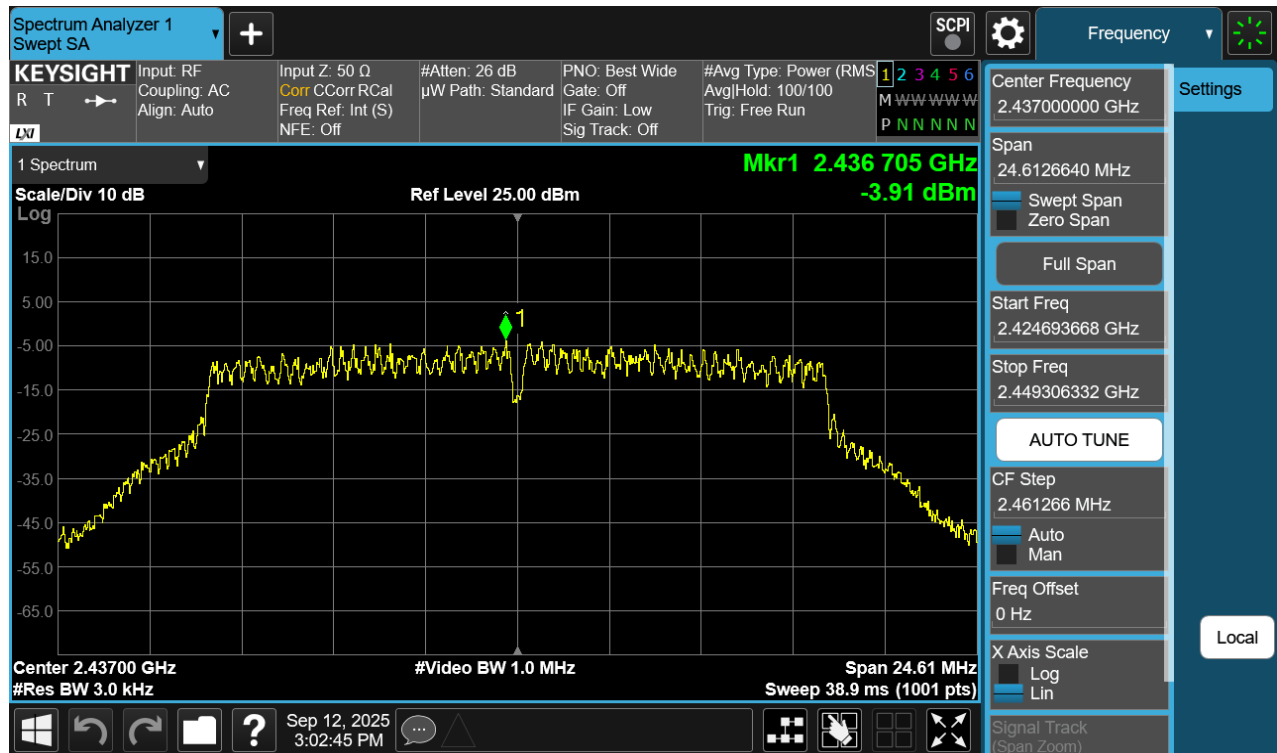
Plot 7-17. Power Spectral Density Plot CDD Ant1 (802.11g – Ch. 6)
