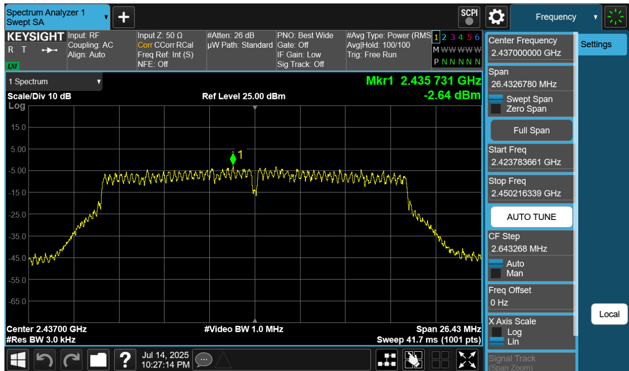
Plot 7-19. Power Spectral Density Plot CDD Ant1 (802.11n – Ch. 6)
