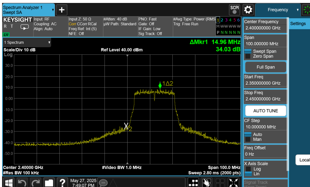
Plot 7-40. Band Edge Plot Ant1 (802.11n (2.4GHz) – Ch. 1)
