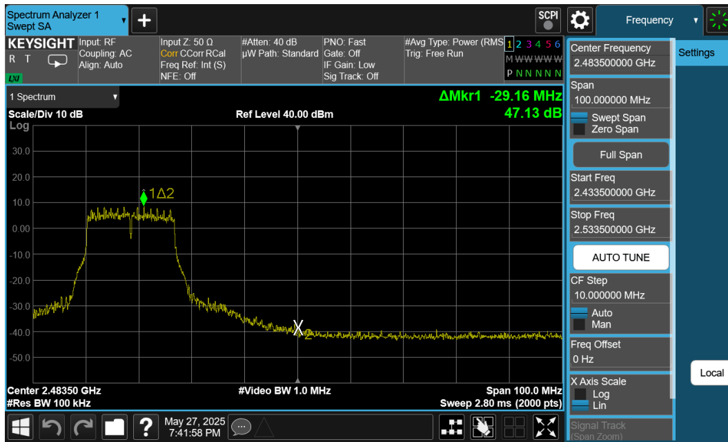
Plot 7-35. Band Edge Plot Ant1 (802.11g – Ch. 9)
