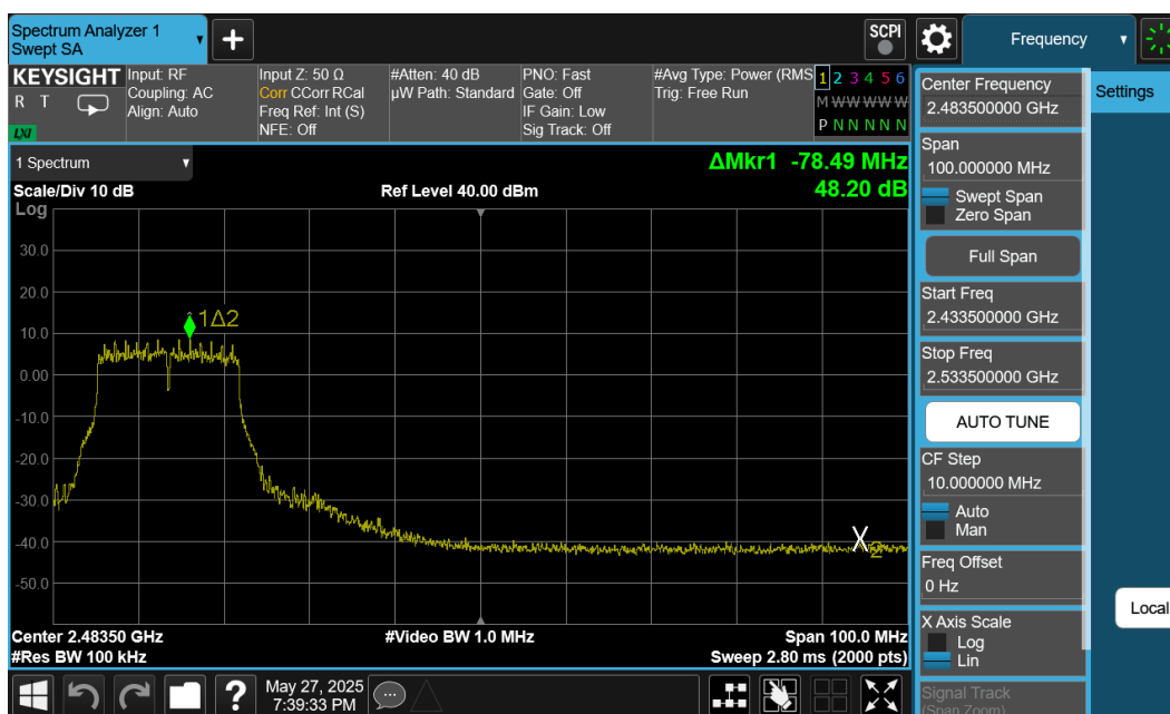
Plot 7-34. Band Edge Plot Ant1 (802.11g – Ch. 8)
