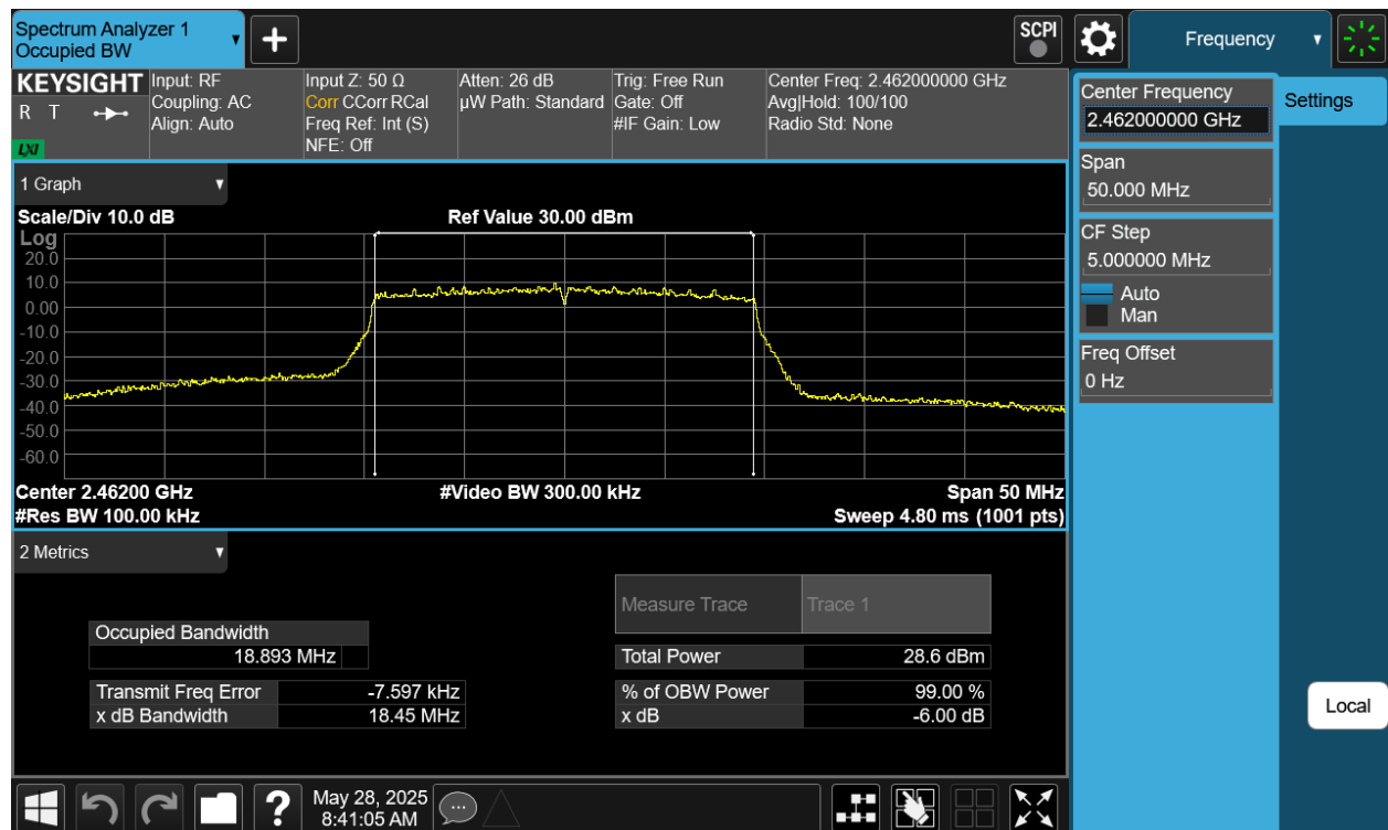
Plot 7-8. 6 dB BW and 99% OBW Plot Ant2 (802.11ax SU – Ch. 11)
