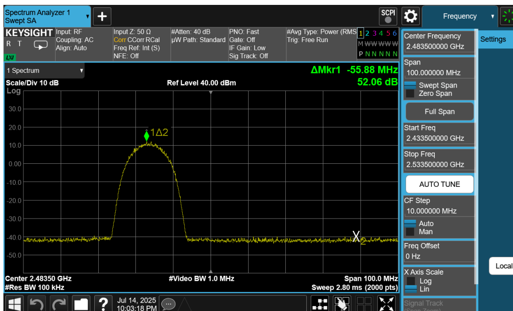
Plot 7-26. Band Edge Plot Ant1 (802.11b – Ch. 12)
