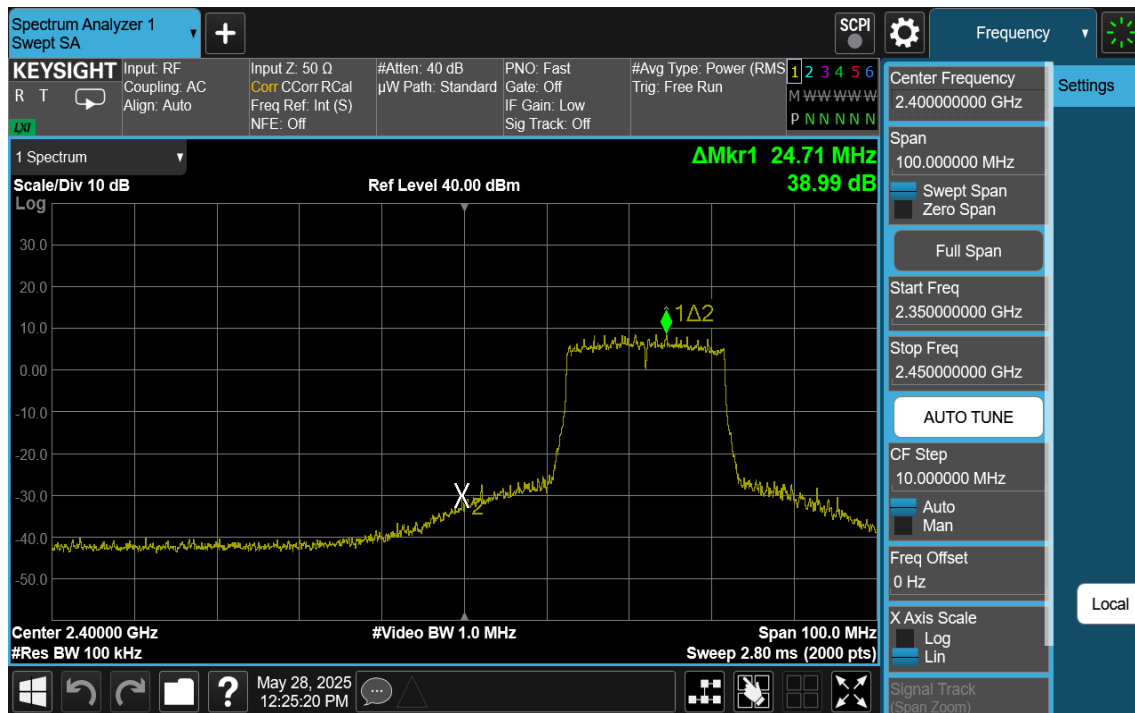
Plot 7-31. Band Edge Ant2 (802.11ax OFDMA – RU242 – Ch. 3)
