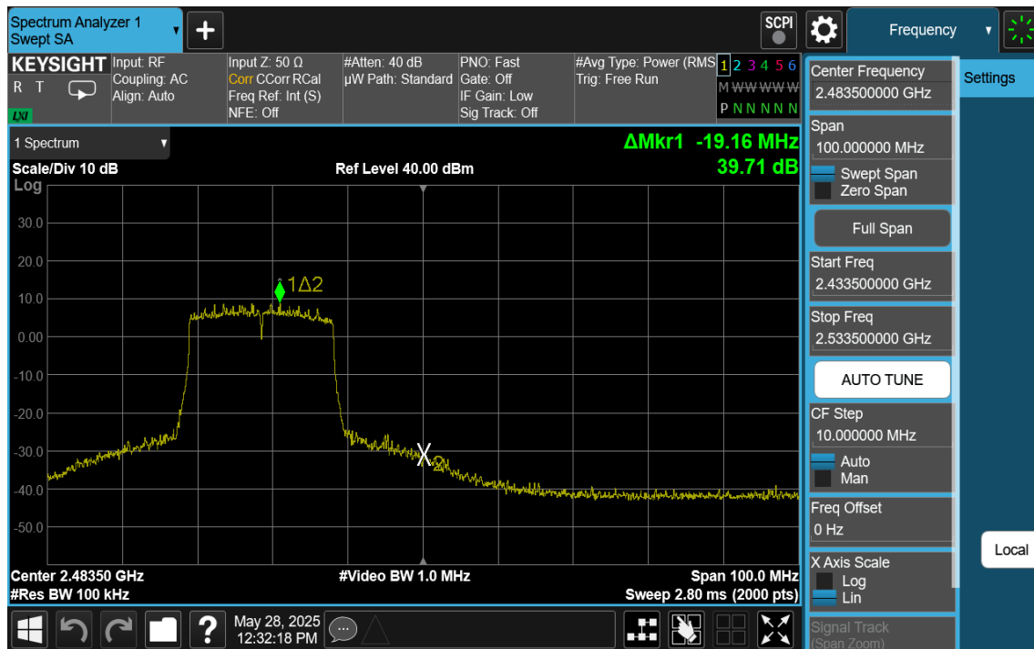
Plot 7-39. Band Edge Ant2 (802.11ax OFDMA – RU242 – Ch. 11)
