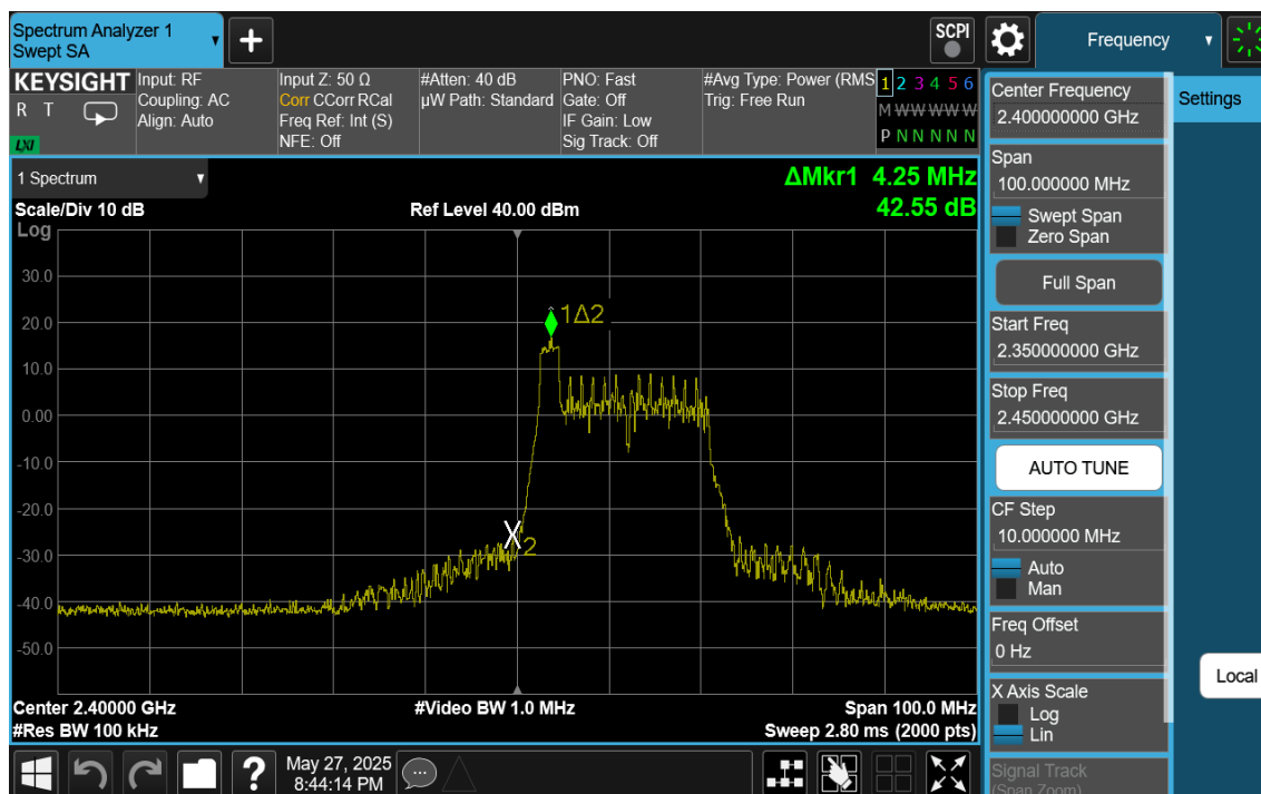
Plot 7-13. Band Edge Ant1 (802.11ax OFDMA – RU26 Index 0 – Ch. 1)
