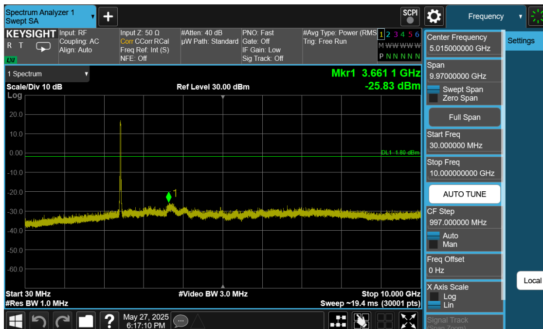
Plot 7-49. Conducted Spurious Plot Ant1 (802.11ax OFDMA – RU242 – Ch. 6)
