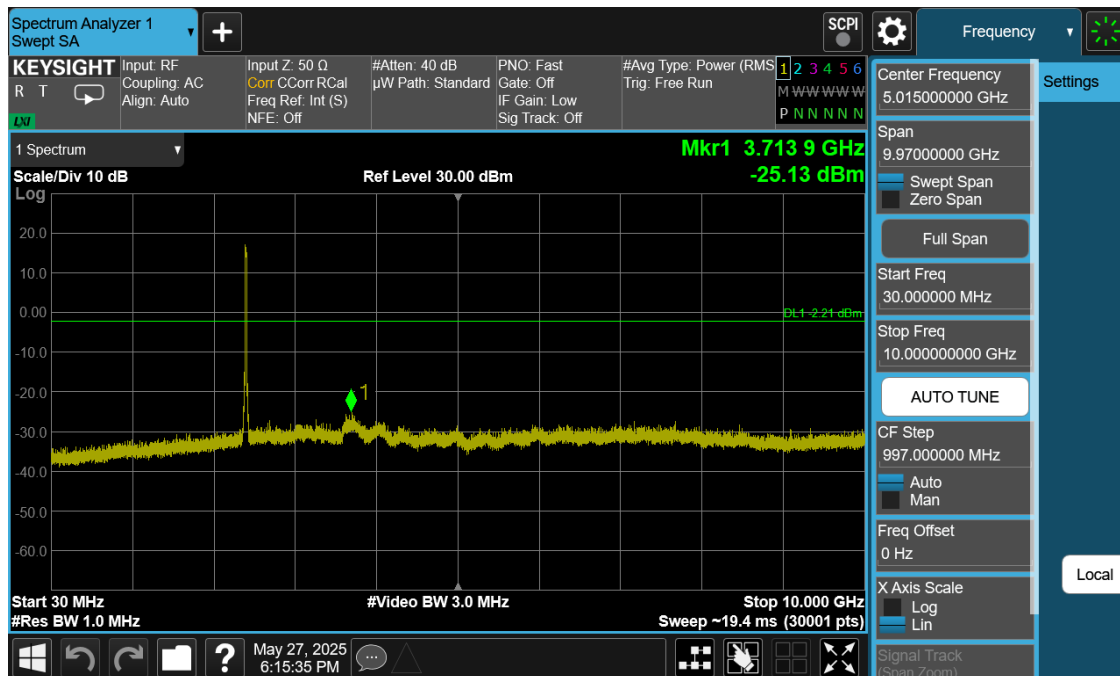
Plot 7-47. Conducted Spurious Plot Ant1 (802.11ax OFDMA – RU242 – Ch. 1)
