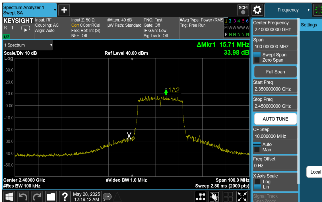
Plot 7-15. Band Edge Ant1 (802.11ax OFDMA – RU242 – Ch. 1)
