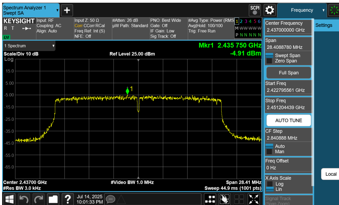
Plot 7-6. Power Spectral Density Plot Ant1 (802.11ax OFDMA – RU242 – Ch. 6)
