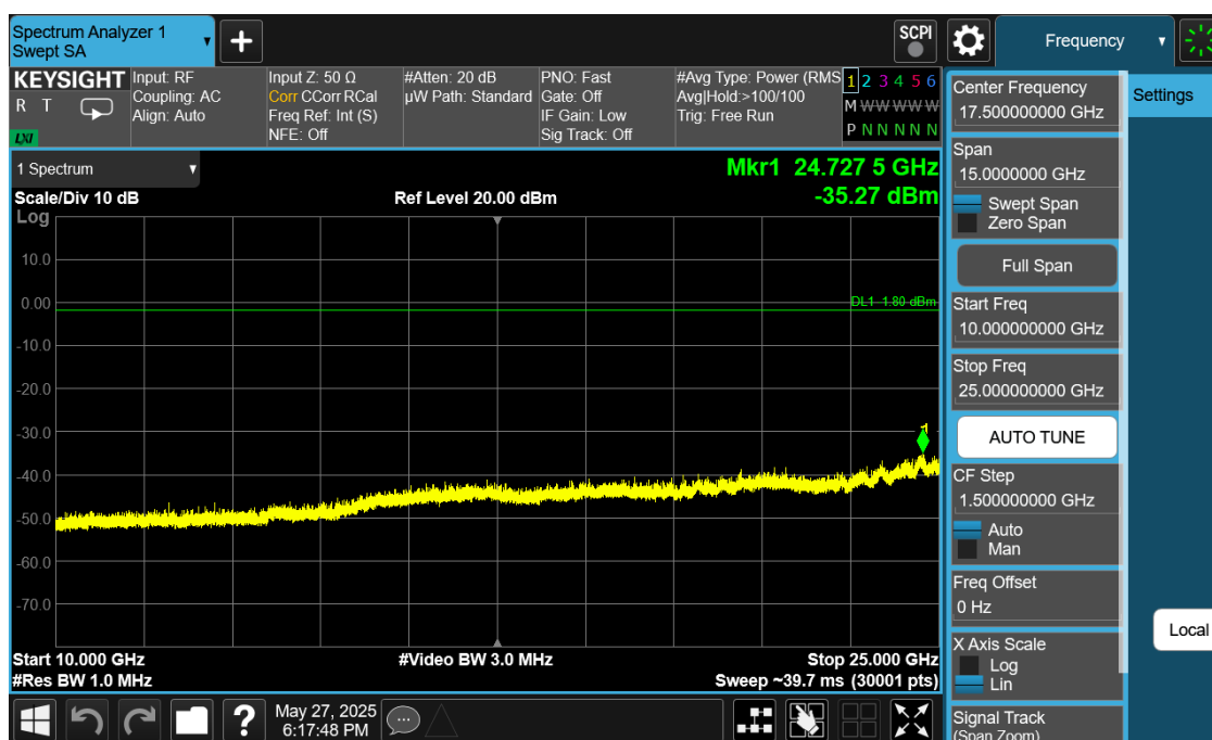
Plot 7-50. Conducted Spurious Plot Ant1 (802.11ax OFDMA – RU242 – Ch. 6)
