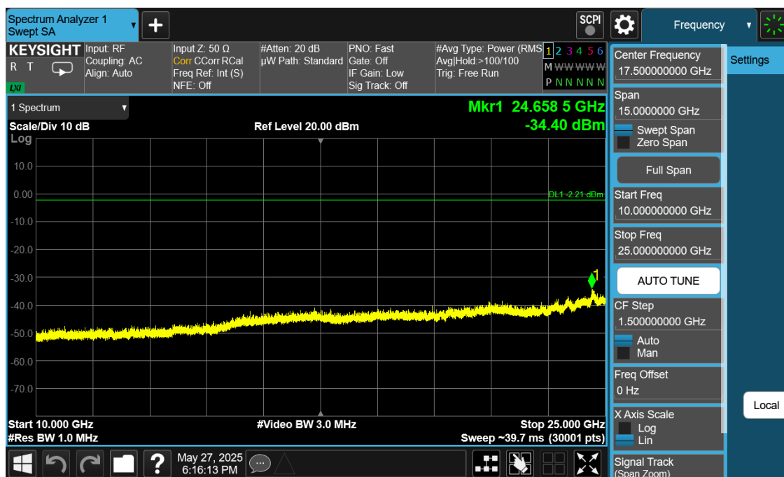
Plot 7-48. Conducted Spurious Plot Ant1 (802.11ax OFDMA – RU242 – Ch. 1)
