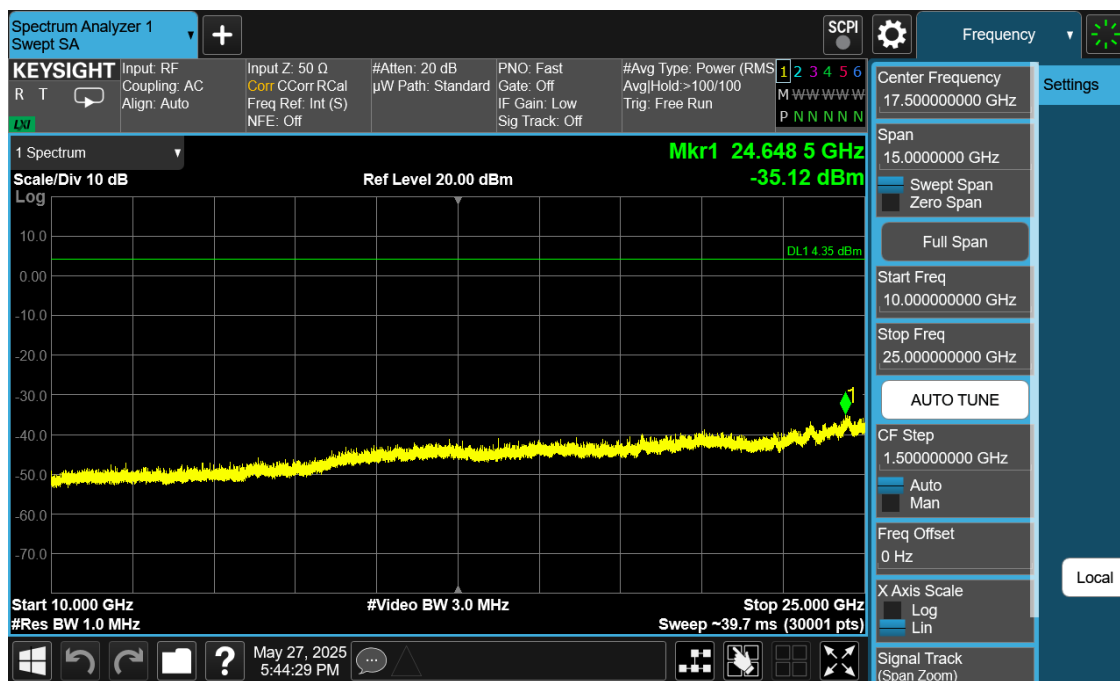
Plot 7-44. Conducted Spurious Plot Ant1 (802.11ax OFDMA – RU26 – Ch. 6)
