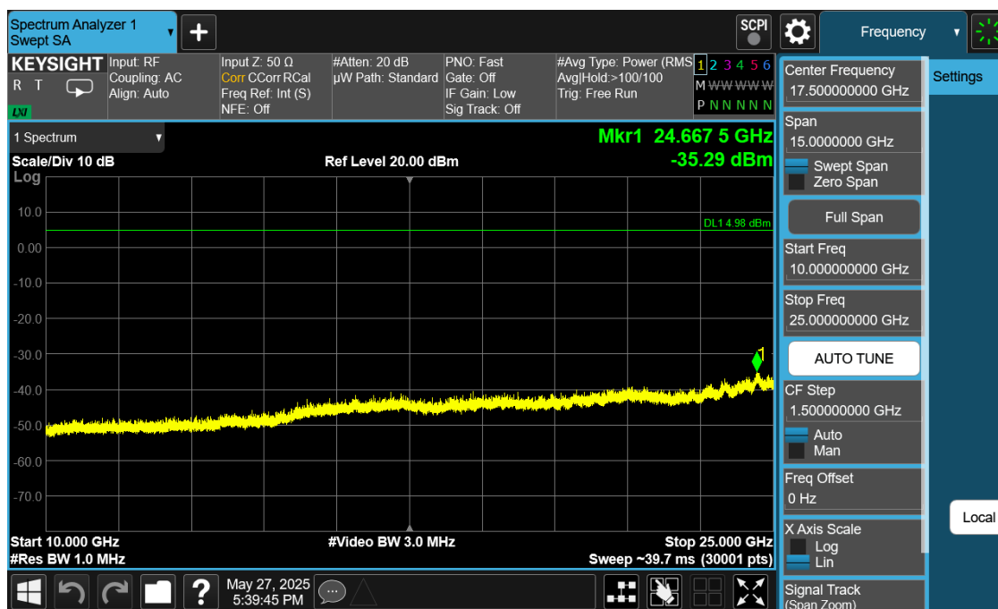
Plot 7-42. Conducted Spurious Plot Ant1 (802.11ax OFDMA – RU26 – Ch. 1)
