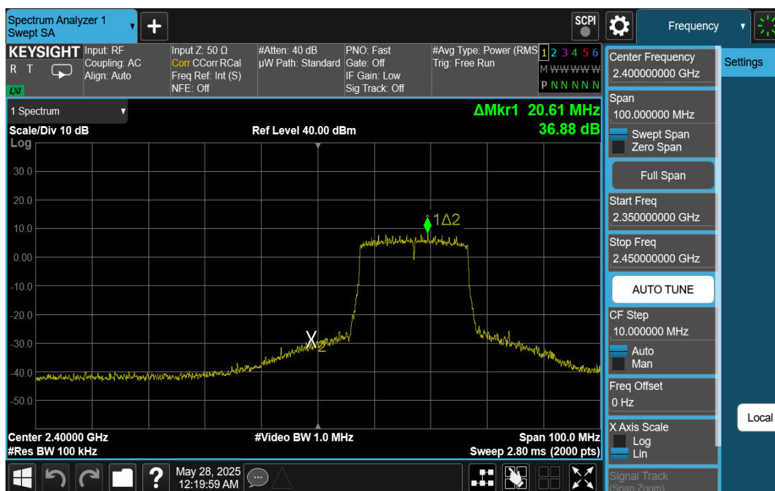
Plot 7-16. Band Edge Ant1 (802.11ax OFDMA – RU242 – Ch. 2)
