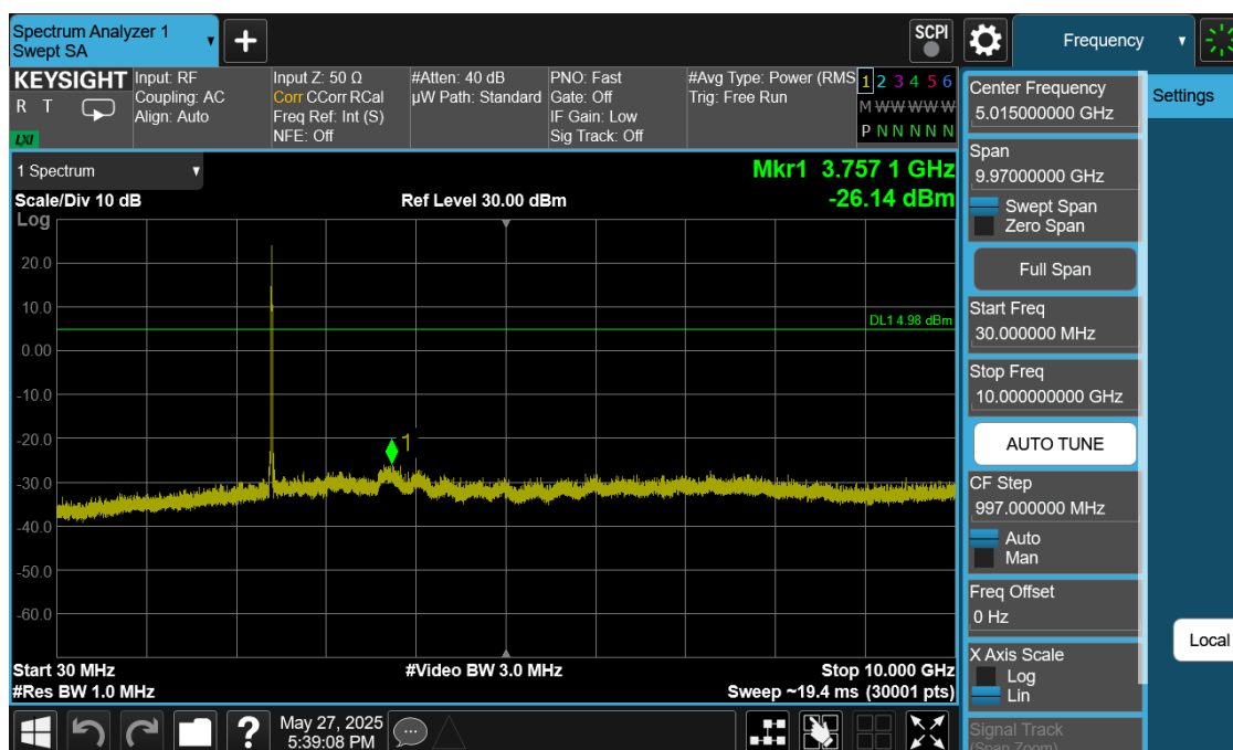
Plot 7-41. Conducted Spurious Plot Ant1 (802.11ax OFDMA – RU26 – Ch. 1)
