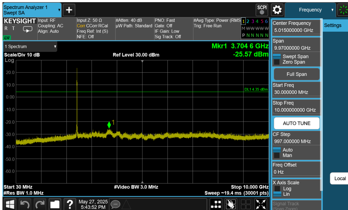
Plot 7-43. Conducted Spurious Plot Ant1 (802.11ax OFDMA – RU26 – Ch. 6)
