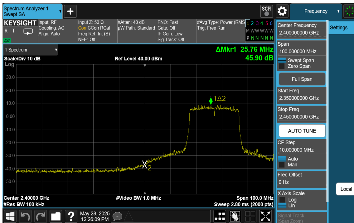
Plot 7-32. Band Edge Ant2 (802.11ax OFDMA – RU242 – Ch. 4)
