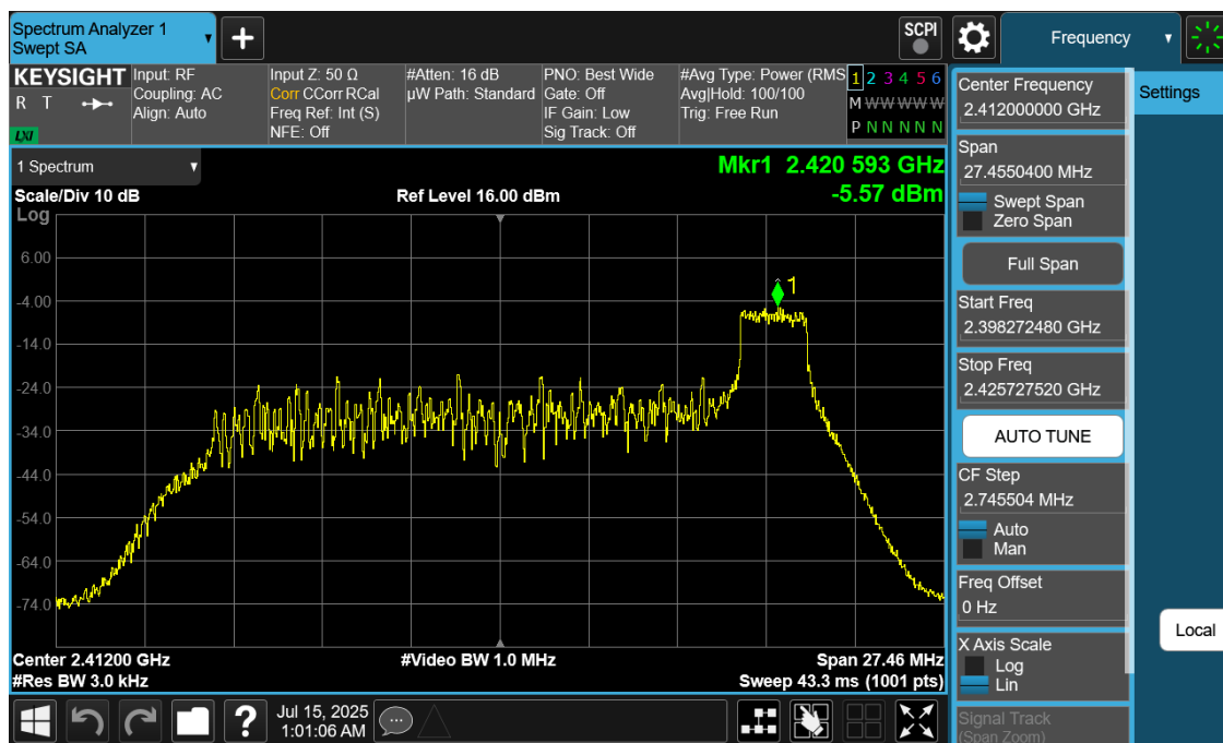
Plot 7-10. Power Spectral Density Plot Ant2 (802.11ax OFDMA – RU26 Index 8 – Ch. 1)
