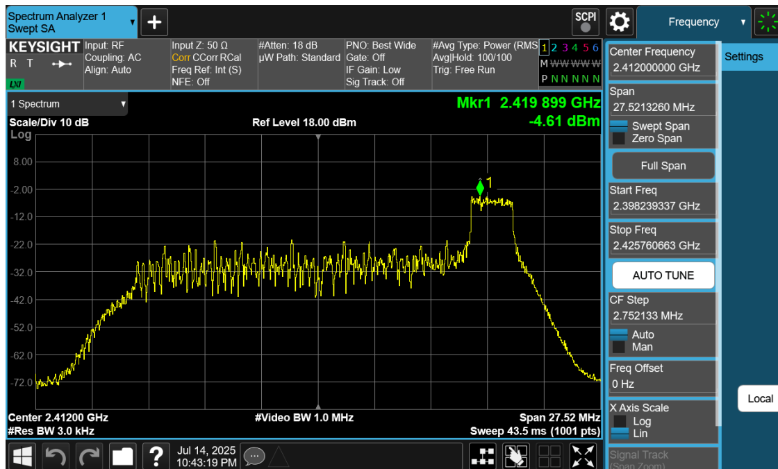
Plot 7-9. Power Spectral Density Plot Ant1 (802.11ax OFDMA – RU26 Index 8 – Ch. 1)
