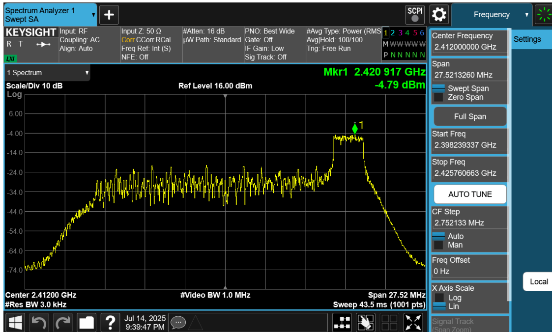
Plot 7-5. Power Spectral Density Plot Ant1 (802.11ax OFDMA – RU26 Index 8 – Ch. 1)
