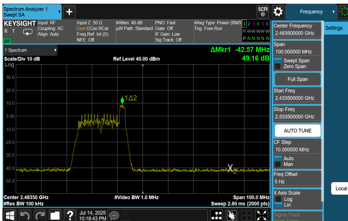
Plot 7-14. Band Edge Ant1 (802.11ax OFDMA – RU26 Index 8 – Ch. 12)
