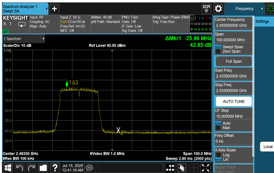
Plot 7-40. Band Edge Ant2 (802.11ax OFDMA – RU242 – Ch. 12)
