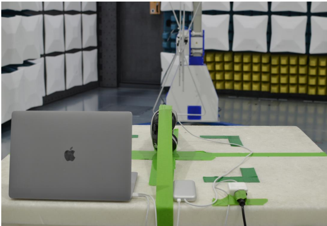
Figure 16: 30MHz-1GHz Test Setup (Rear View)
