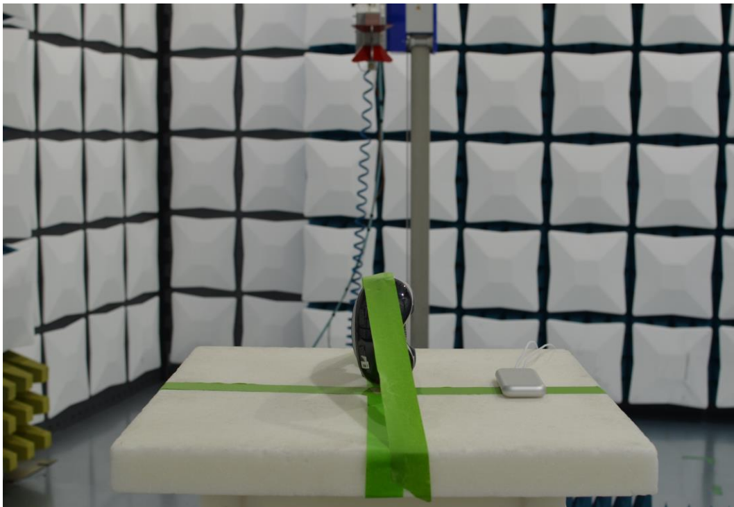
Figure 8: Above 1GHz Test Setup (Rear View)
