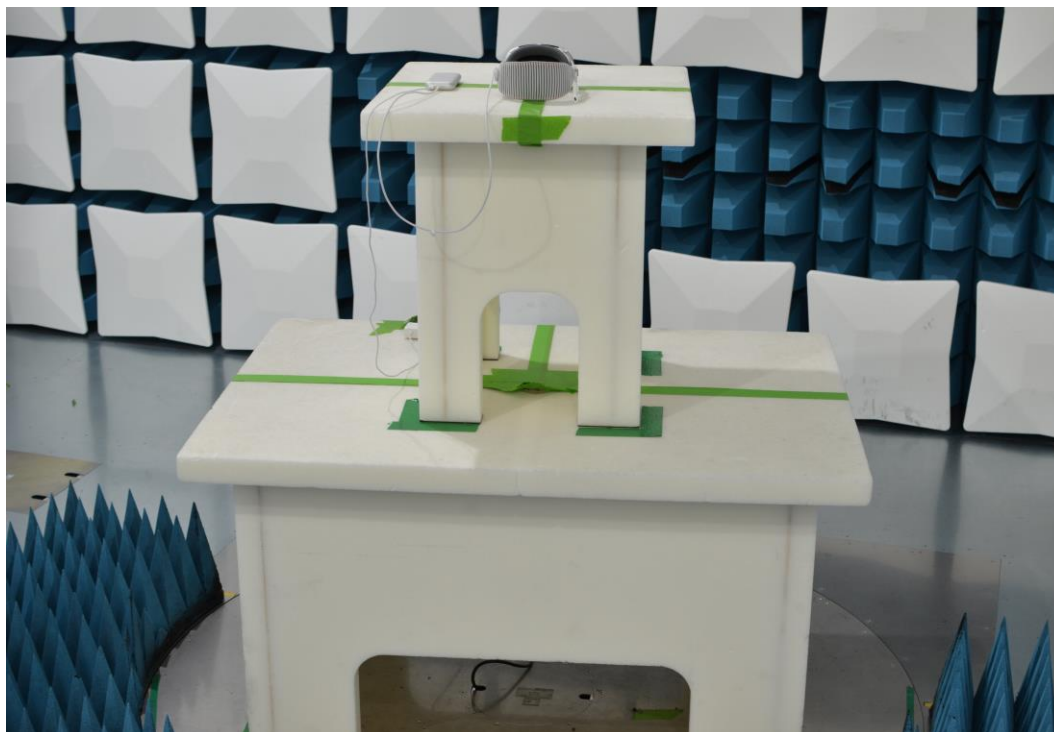
Figure 5: Above 1GHz Test Setup (Front View)
