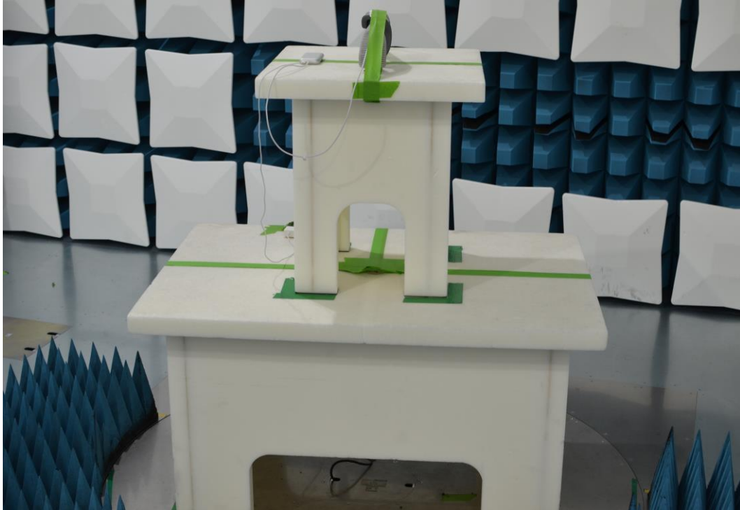
Figure 7: Above 1GHz Test Setup (Front View)
