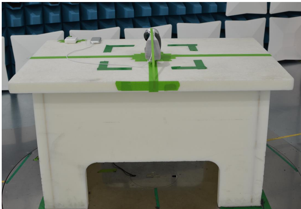
Figure 11: 30MHz-1GHz Test Setup (Front View)
