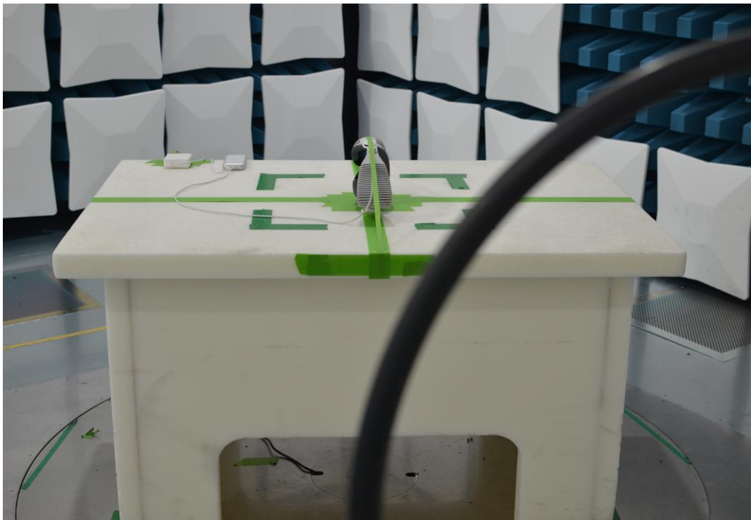
Figure 18: 9kHz-30MHz Test Setup (Front View)
