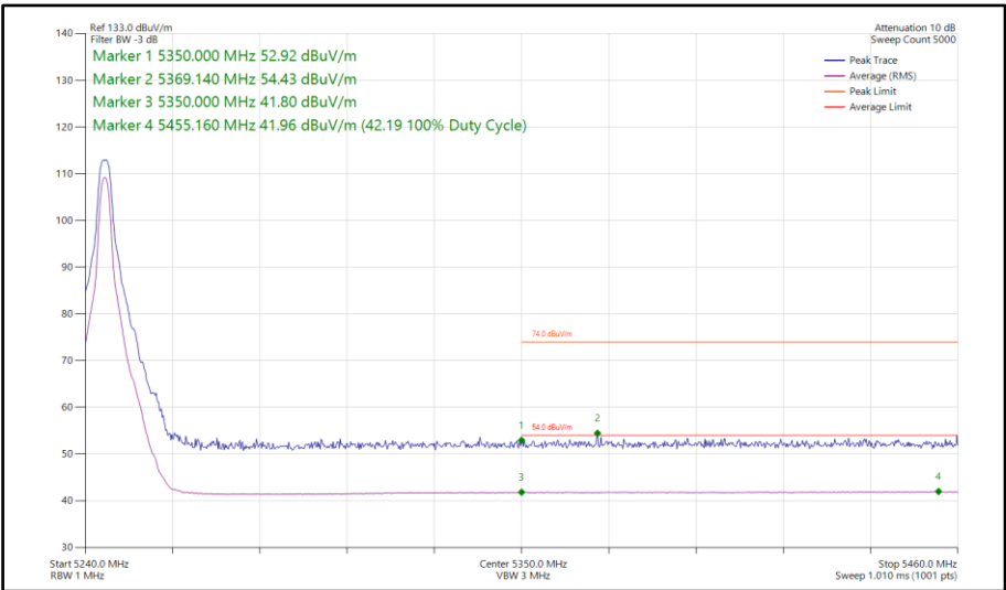
Figure 76 - HDT3, MIMO, Core 0-1 - 5245 MHz Band Edge Frequency 5350 MHz
