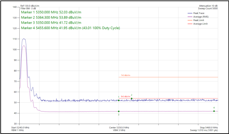
Figure 73 - HDR8, MIMO, Core 0-1 - 5245 MHz Band Edge Frequency 5350 MHz
