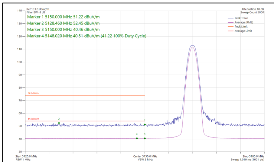
Figure 60 - LE1M, MIMO, Core 0-1 - 5162 MHz Band Edge Frequency 5150 MHz
