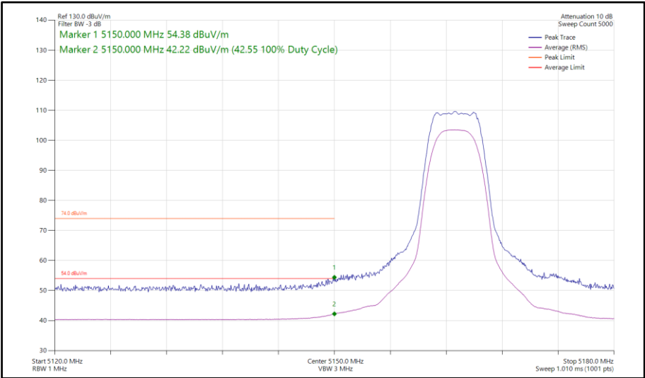
Figure 69 - XHDRPM8, MIMO, Core 0-1 - 5163 MHz Band Edge Frequency 5150 MHz
