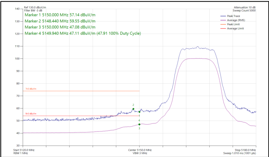
Figure 70 - XHDRPL24, MIMO, Core 0-1 - 5165 MHz Band Edge Frequency 5150 MHz
