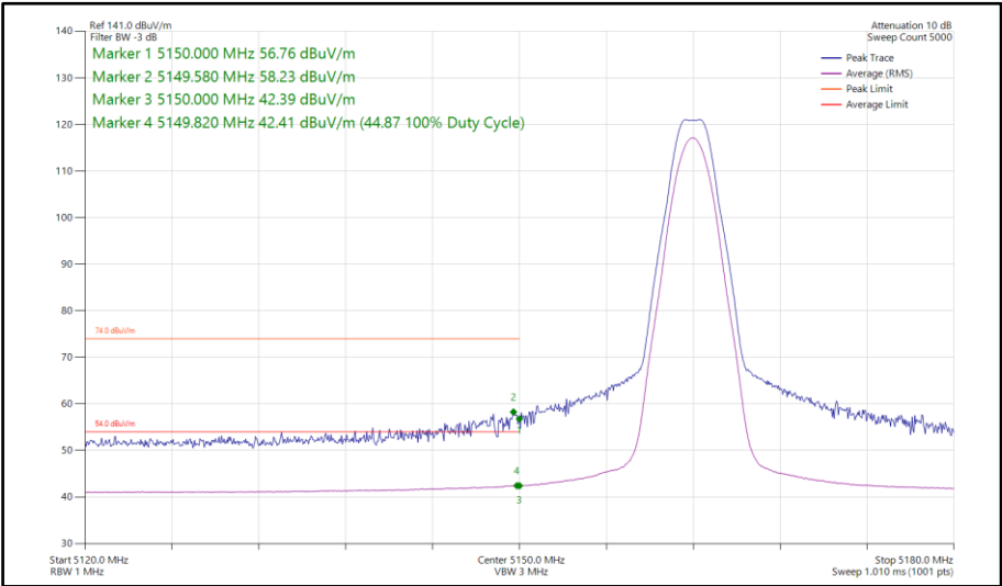
Figure 117 - LE2M, SISO, Core 1 - 5162 MHz Band Edge Frequency 5150 MHz
