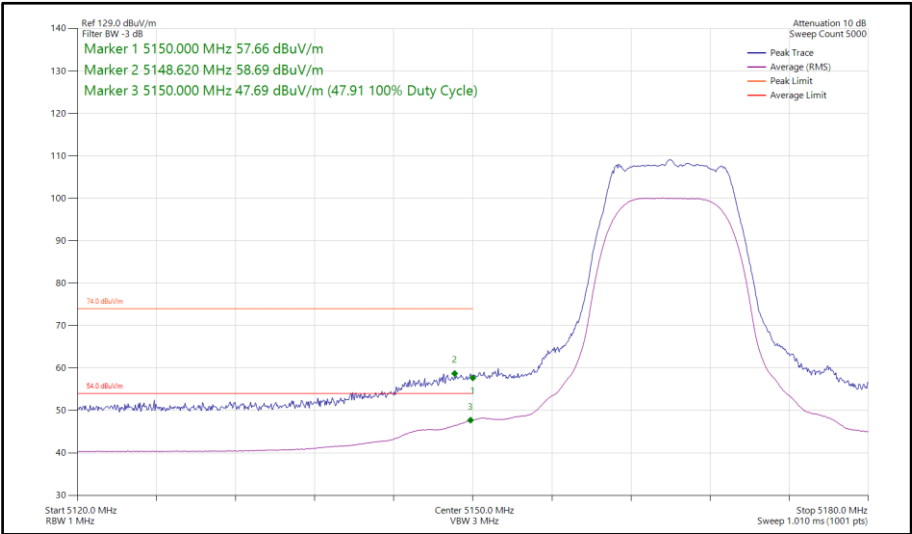
Figure 67 - HDRPL8, MIMO, Core 0-1 - 5165 MHz Band Edge Frequency 5150 MHz
