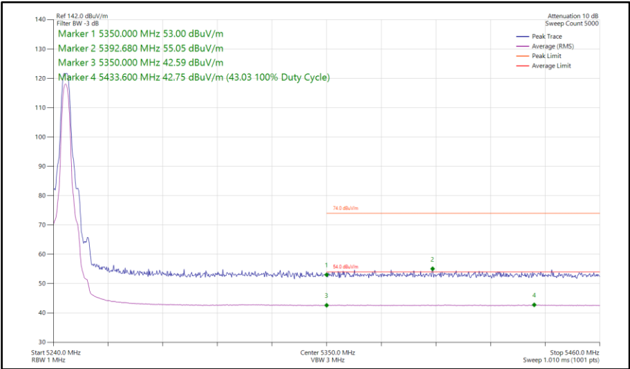
Figure 105 - HDT4, SISO, Core 0 - 5245 MHz Band Edge Frequency 5350 MHz
