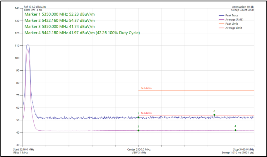
Figure 79 - HDRPS2, MIMO, Core 0-1 - 5245 MHz Band Edge Frequency 5350 MHz
