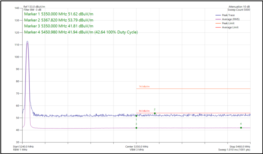
Figure 74 - LE1M, MIMO, Core 0-1 - 5245 MHz Band Edge Frequency 5350 MHz
