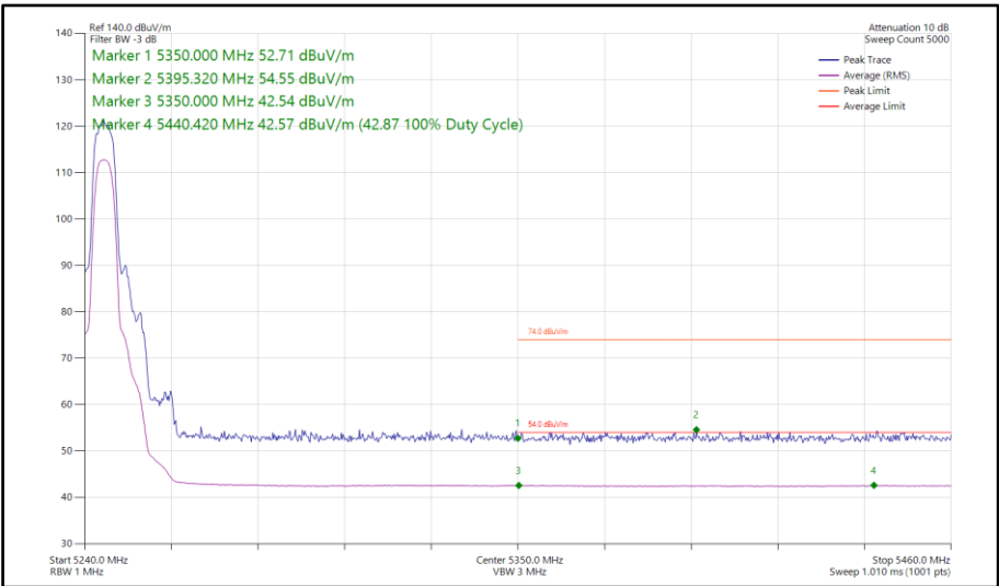
Figure 108 - HDRPM12, SISO, Core 0 - 5245 MHz Band Edge Frequency 5350 MHz
