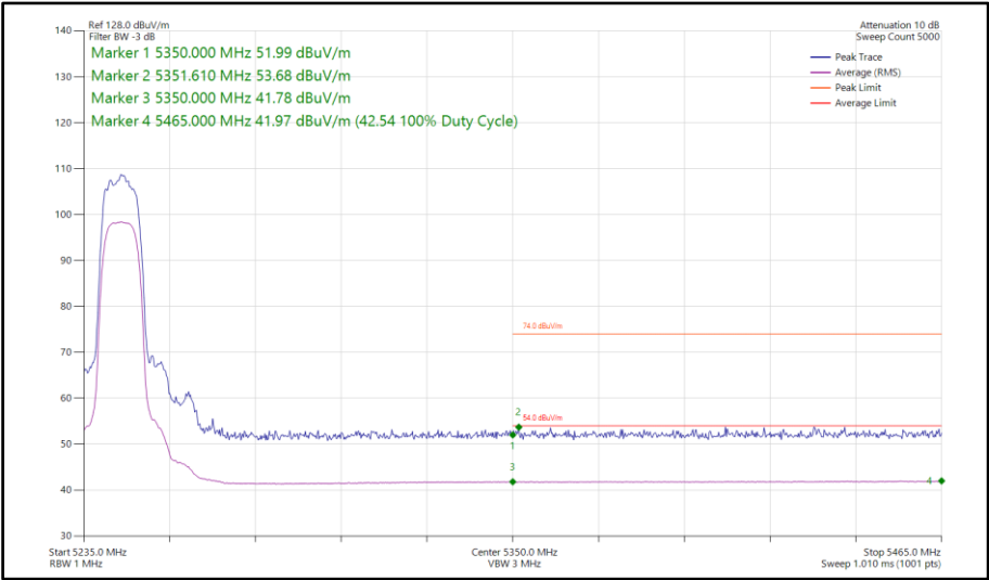
Figure 82 - HDRPL24, MIMO, Core 0-1 - 5245 MHz Band Edge Frequency 5350 MHz
