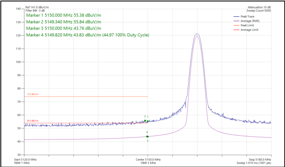
Figure 85 - DH5, SISO, Core 0 - 5162 MHz Band Edge Frequency 5150 MHz
