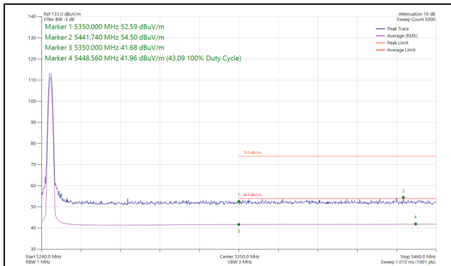
Figure 71 - DH5, MIMO, Core 0-1 - 5245 MHz Band Edge Frequency 5350 MHz
