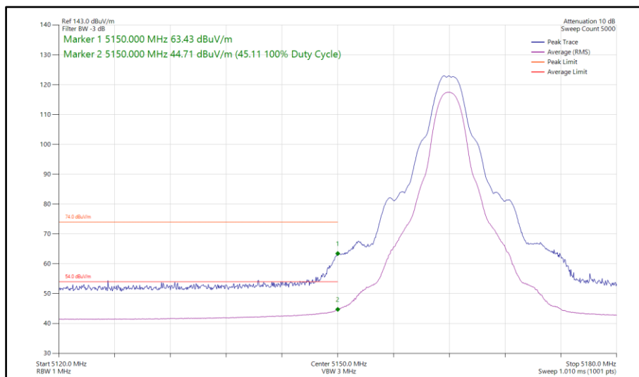
Figure 92 - HDT6, SISO, Core 0 - 5162 MHz Band Edge Frequency 5150 MHz
