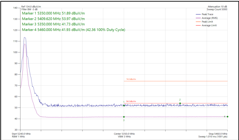
Figure 78 - HDT6, MIMO, Core 0-1 - 5245 MHz Band Edge Frequency 5350 MHz
