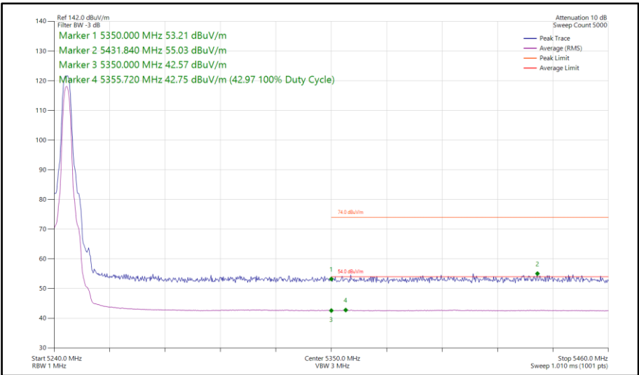
Figure 104 - HDT3, SISO, Core 0 - 5245 MHz Band Edge Frequency 5350 MHz
