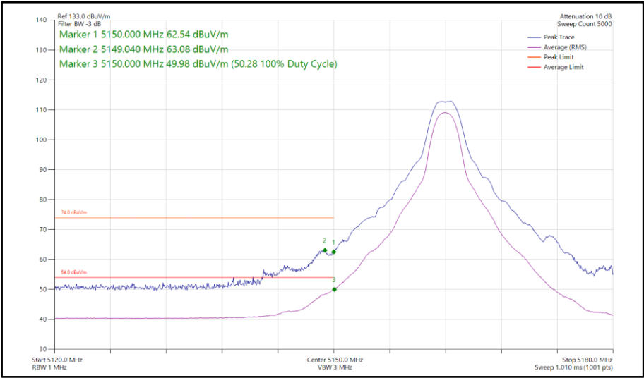
Figure 63 - HDT4, MIMO, Core 0-1 - 5162 MHz Band Edge Frequency 5150 MHz
