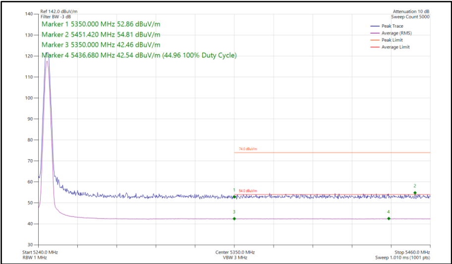
Figure 103 - LE2M, SISO, Core 0 - 5245 MHz Band Edge Frequency 5350 MHz
