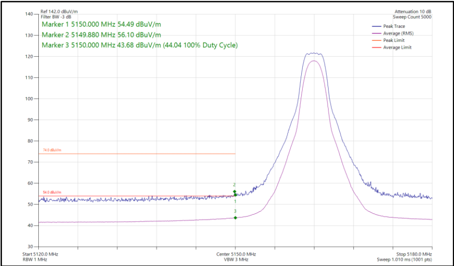
Figure 93 - HDRPS2, SISO, Core 0 - 5162 MHz Band Edge Frequency 5150 MHz
