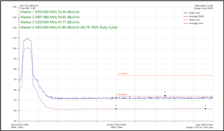
Figure 84 - XHDRPL24, MIMO, Core 0-1 - 5245 MHz Band Edge Frequency 5350 MHz
