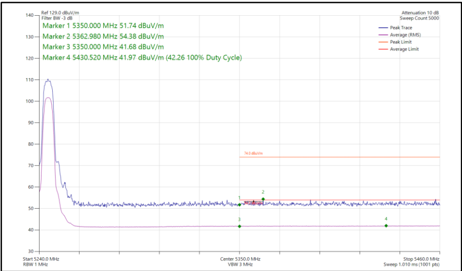
Figure 80 - HDRPM12, MIMO, Core 0-1 - 5245 MHz Band Edge Frequency 5350 MHz
