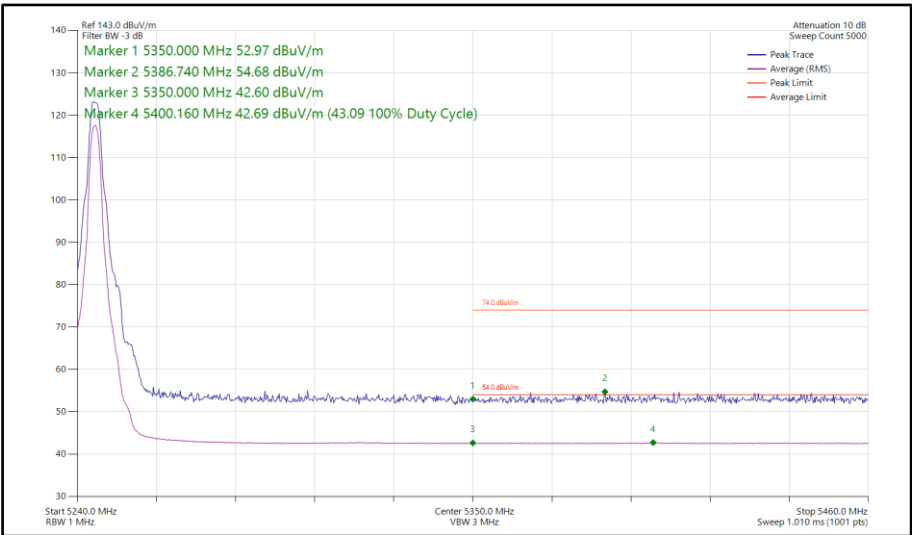
Figure 106 - HDT6, SISO, Core 0 - 5245 MHz Band Edge Frequency 5350 MHz
