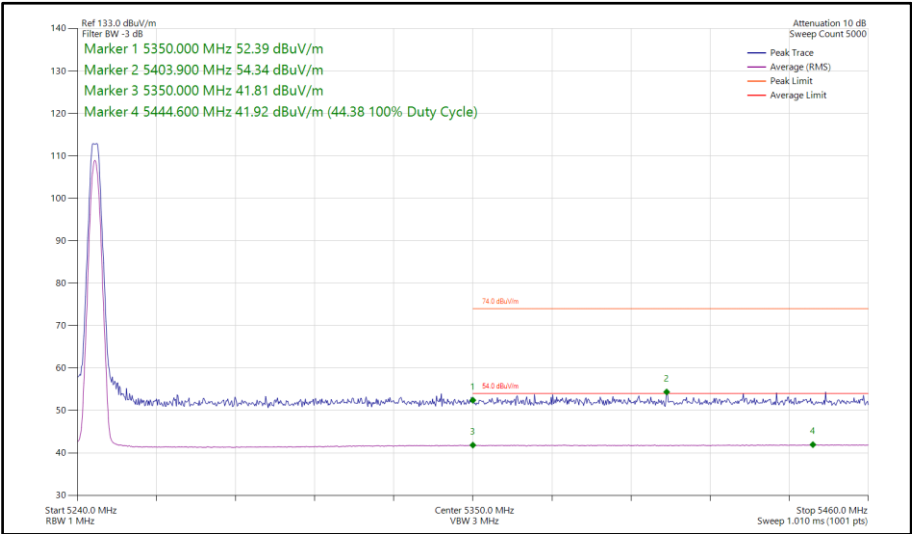
Figure 75 - LE2M, MIMO, Core 0-1 - 5245 MHz Band Edge Frequency 5350 MHz
