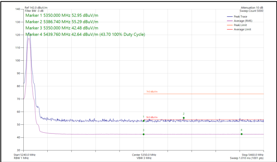
Figure 100 - HDR4, SISO, Core 0 - 5245 MHz Band Edge Frequency 5350 MHz
