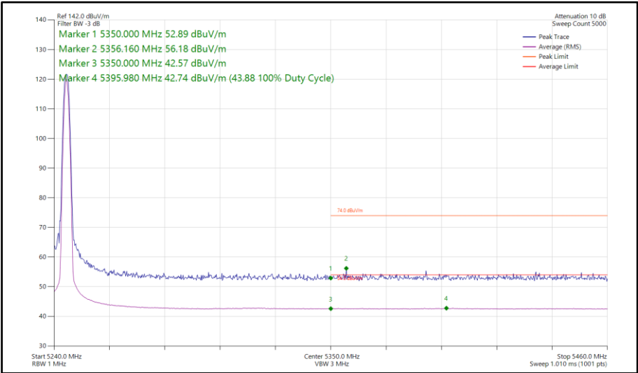
Figure 99 - DH5, SISO, Core 0 - 5245 MHz Band Edge Frequency 5350 MHz
