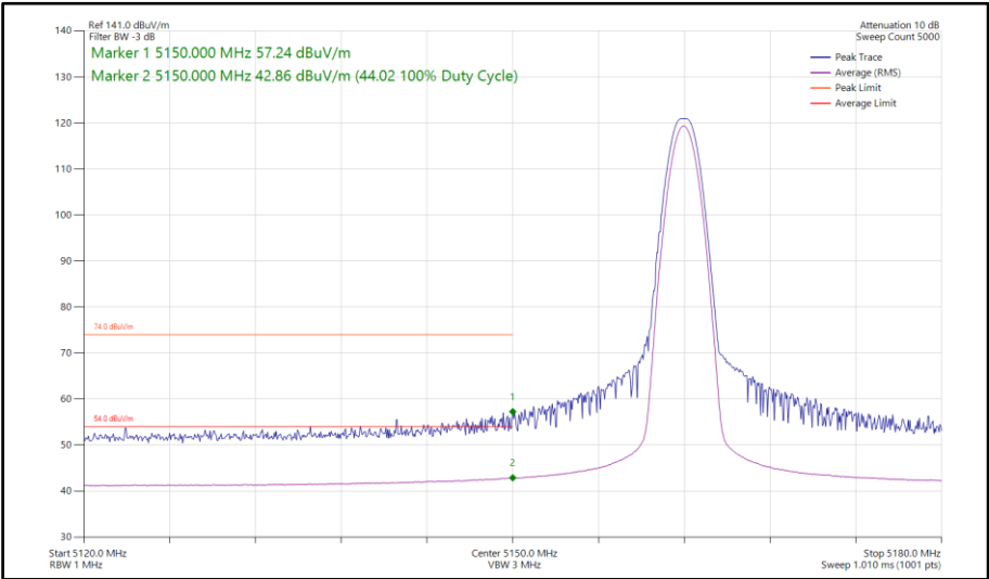
Figure 113 - DH5, SISO, Core 1 - 5162 MHz Band Edge Frequency 5150 MHz
