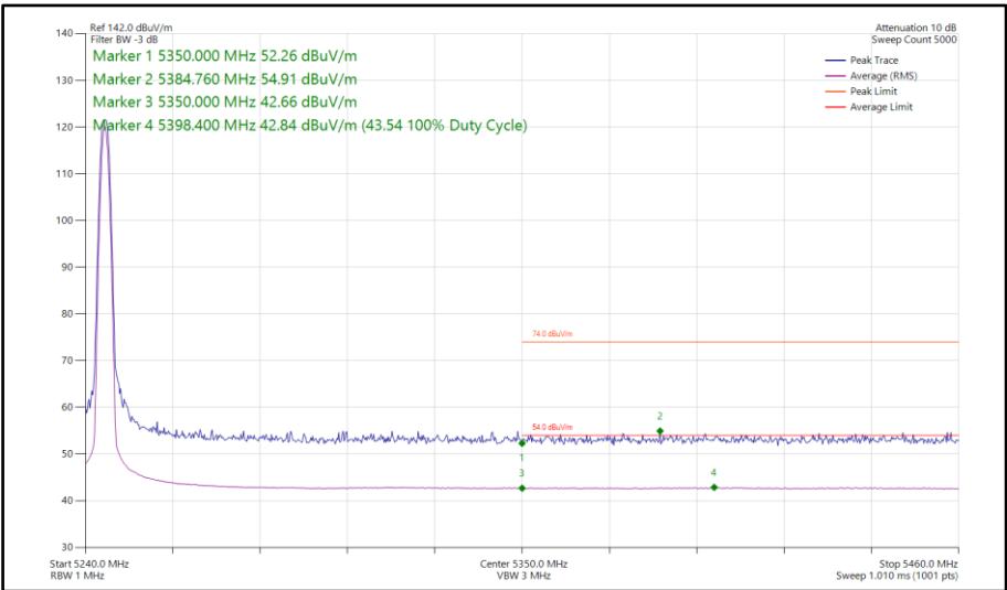
Figure 102 - LE1M, SISO, Core 0 - 5245 MHz Band Edge Frequency 5350 MHz
