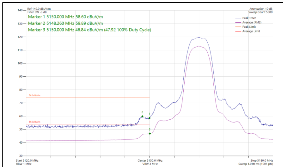
Figure 87 - HDR8, SISO, Core 0 - 5162 MHz Band Edge Frequency 5150 MHz
