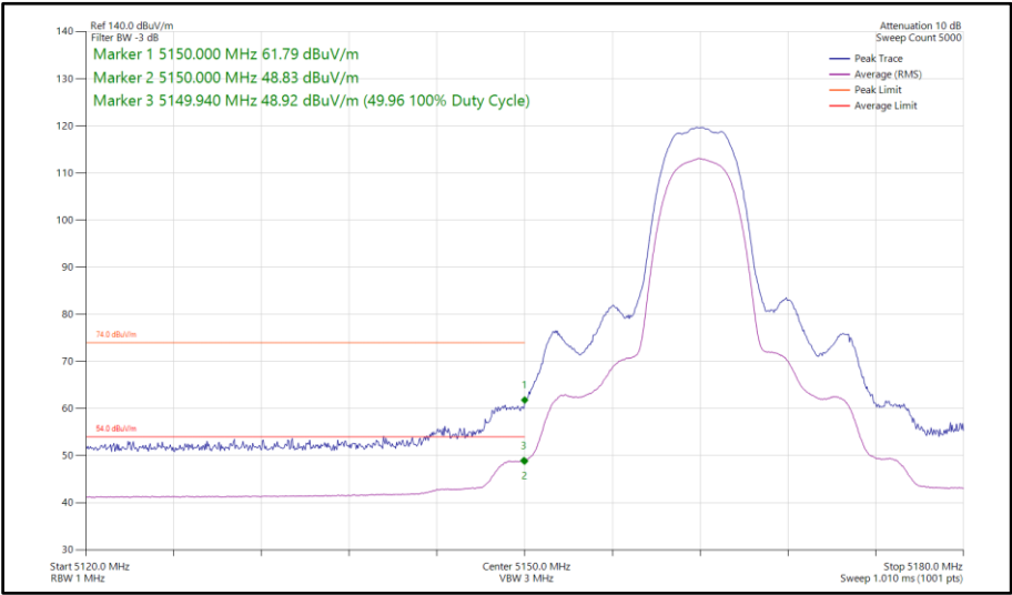
Figure 115 - HDR8, SISO, Core 1 - 5162 MHz Band Edge Frequency 5150 MHz
