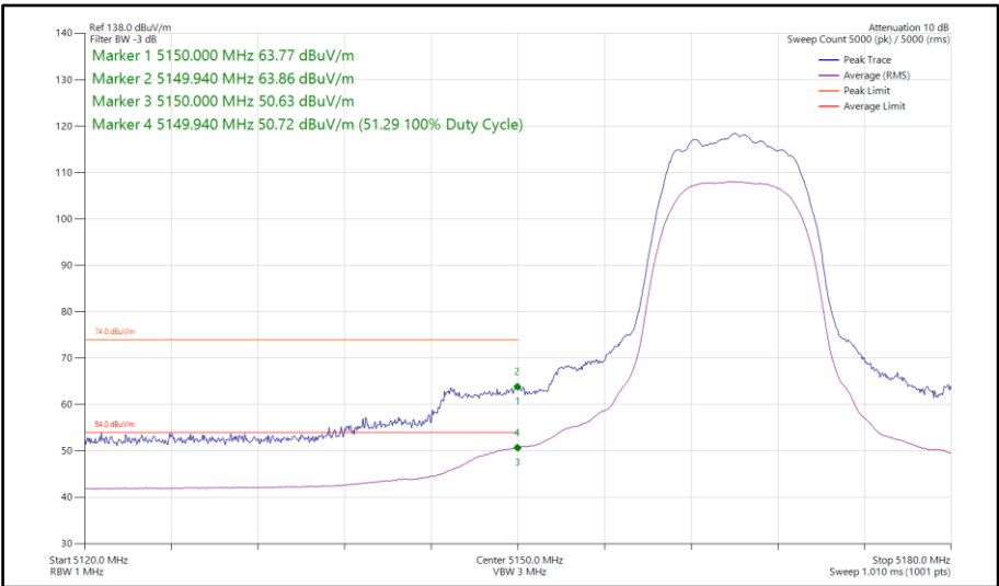
Figure 96 - HDRPL24, SISO, Core 0 - 5165 MHz Band Edge Frequency 5150 MHz
