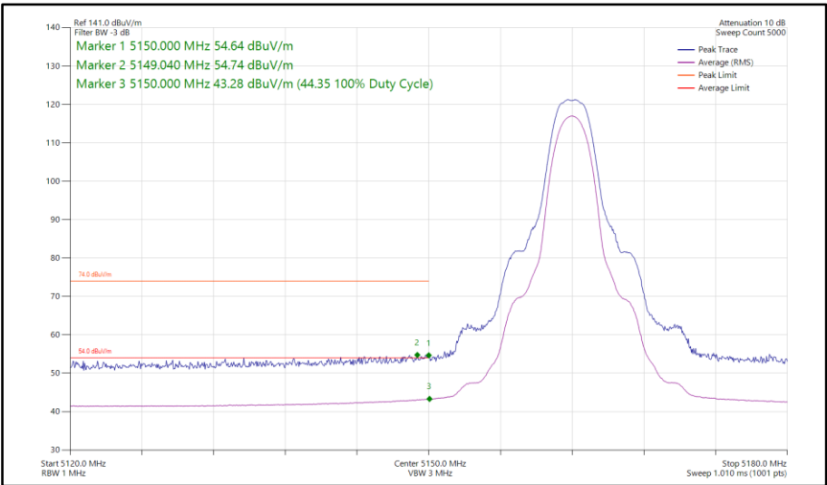
Figure 86 - HDR4, SISO, Core 0 - 5162 MHz Band Edge Frequency 5150 MHz
