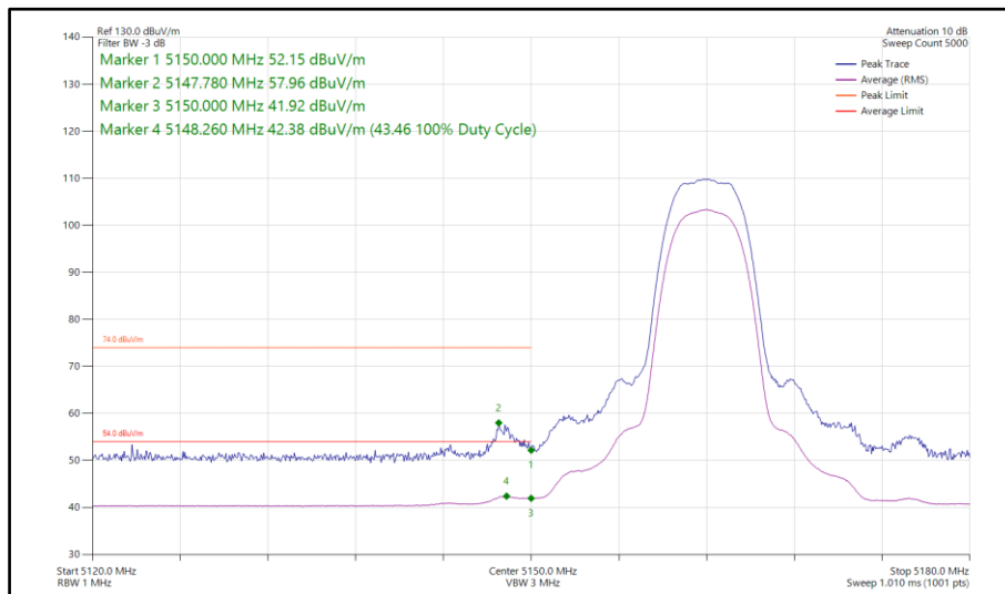
Figure 59 - HDR8, MIMO, Core 0-1 - 5162 MHz Band Edge Frequency 5150 MHz
