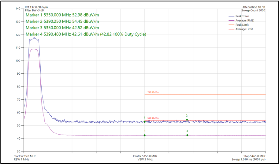
Figure 109 - HDRPL8, SISO, Core 0 - 5245 MHz Band Edge Frequency 5350 MHz
