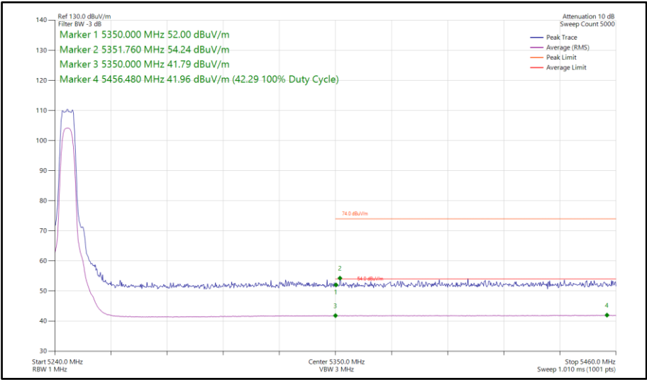
Figure 83 - XHDRPM8, MIMO, Core 0-1 - 5245 MHz Band Edge Frequency 5350 MHz
