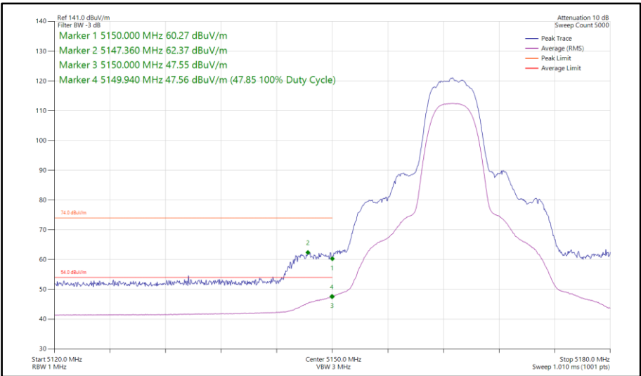
Figure 94 - HDRPM12, SISO, Core 0 - 5163 MHz Band Edge Frequency 5150 MHz
