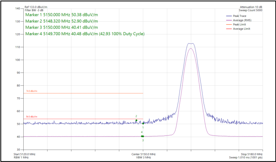
Figure 61 - LE2M, MIMO, Core 0-1 - 5162 MHz Band Edge Frequency 5150 MHz
