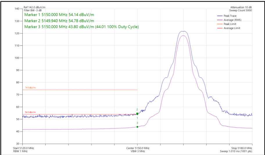
Figure 90 - HDT3, SISO, Core 0 - 5162 MHz Band Edge Frequency 5150 MHz
