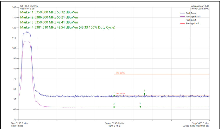
Figure 112 - XHDRPL24, SISO, Core 0 - 5245 MHz Band Edge Frequency 5350 MHz
