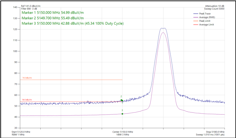
Figure 89 - LE2M, SISO, Core 0 - 5162 MHz Band Edge Frequency 5150 MHz
