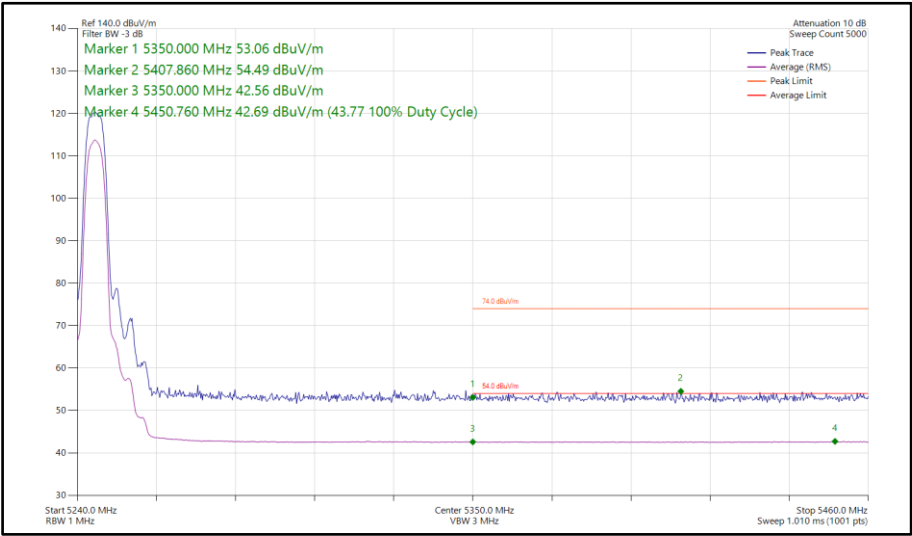
Figure 101 - HDR8, SISO, Core 0 - 5245 MHz Band Edge Frequency 5350 MHz
