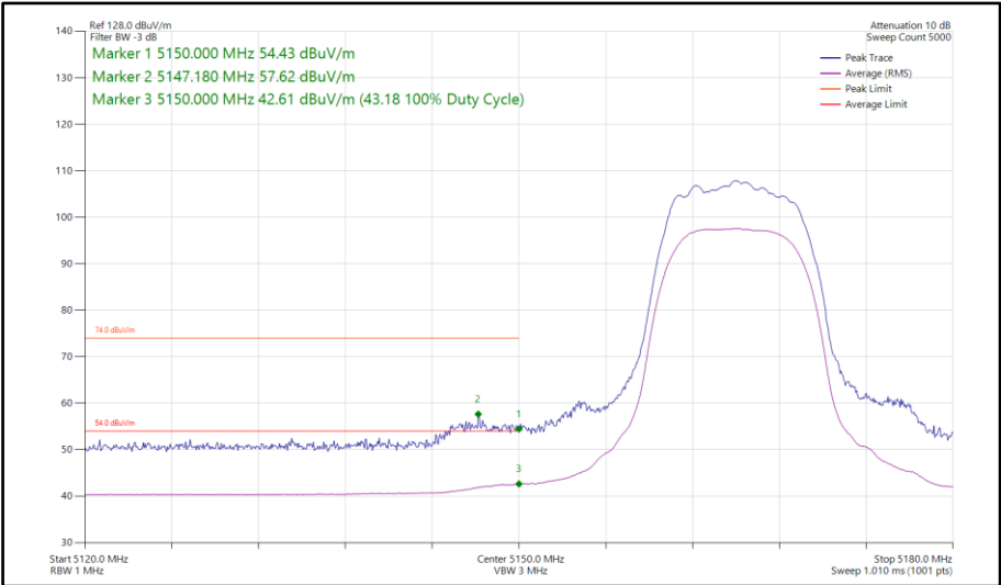
Figure 68 - HDRPL24, MIMO, Core 0-1 - 5165 MHz Band Edge Frequency 5150 MHz
