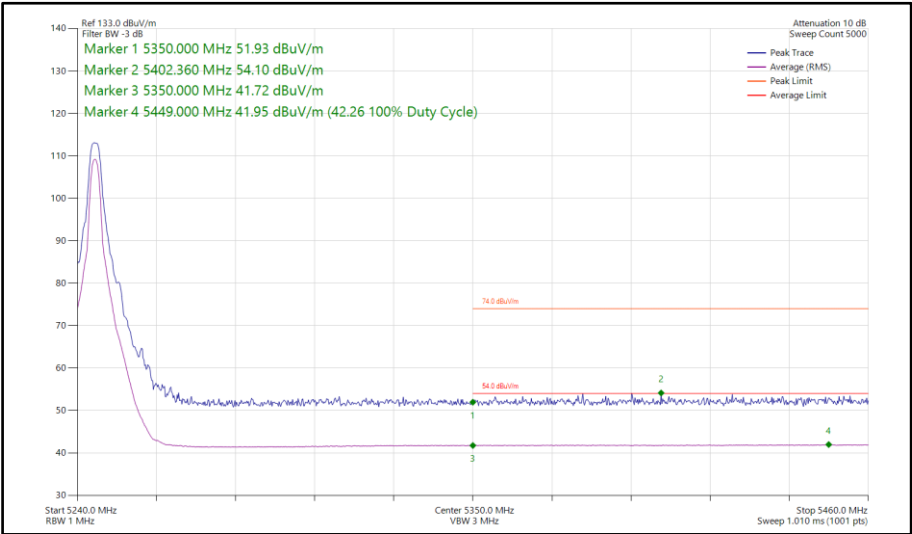
Figure 77 - HDT4, MIMO, Core 0-1 - 5245 MHz Band Edge Frequency 5350 MHz
