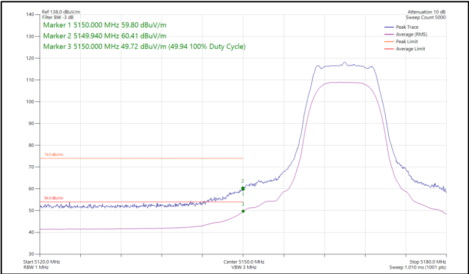
Figure 95 - HDRPL8, SISO, Core 0 - 5165 MHz Band Edge Frequency 5150 MHz
