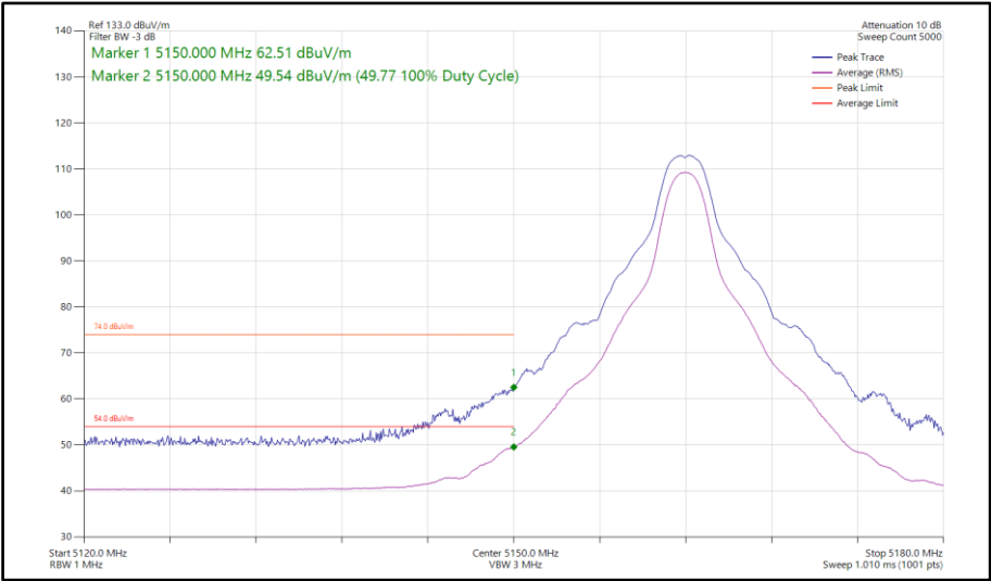
Figure 62 - HDT3, MIMO, Core 0-1 - 5162 MHz Band Edge Frequency 5150 MHz
