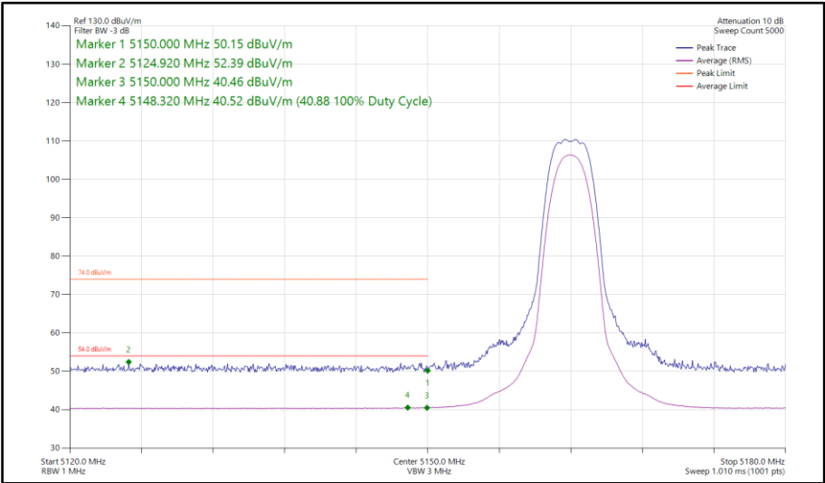
Figure 65 - HDRPS2, MIMO, Core 0-1 - 5162 MHz Band Edge Frequency 5150 MHz
