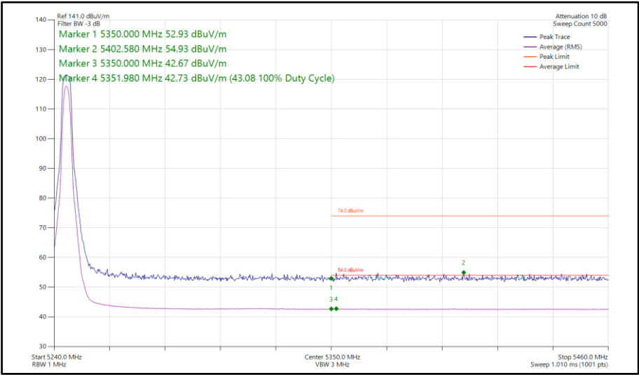
Figure 107 - HDRPS2, SISO, Core 0 - 5245 MHz Band Edge Frequency 5350 MHz
