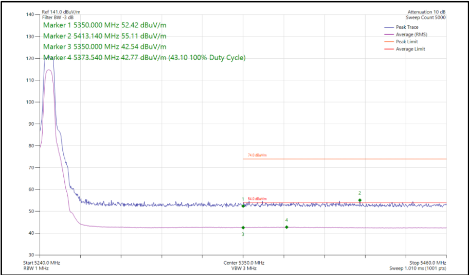
Figure 111 - XHDRPM8, SISO, Core 0 - 5245 MHz Band Edge Frequency 5350 MHz
