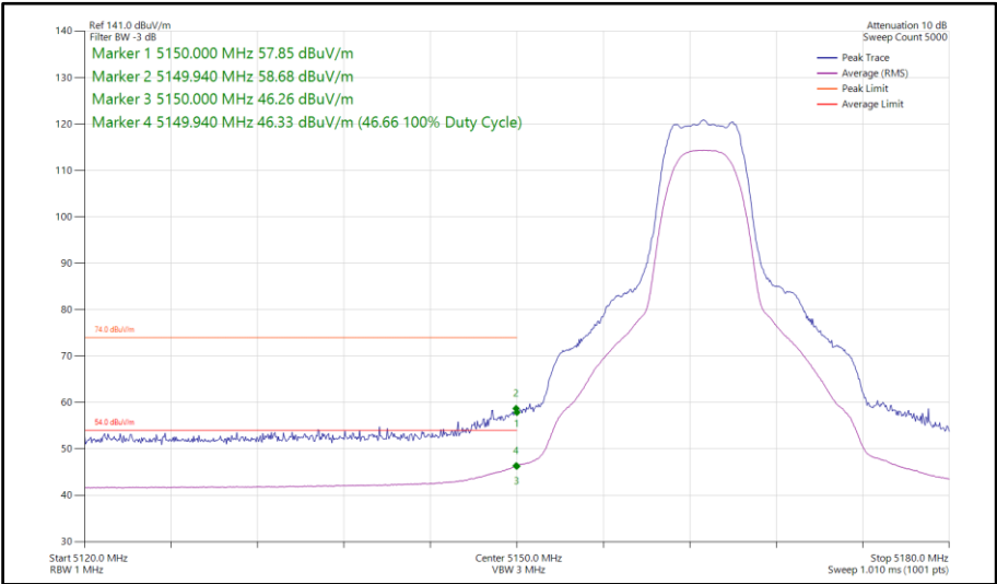
Figure 97 - XHDRPM8, SISO, Core 0 - 5163 MHz Band Edge Frequency 5150 MHz
