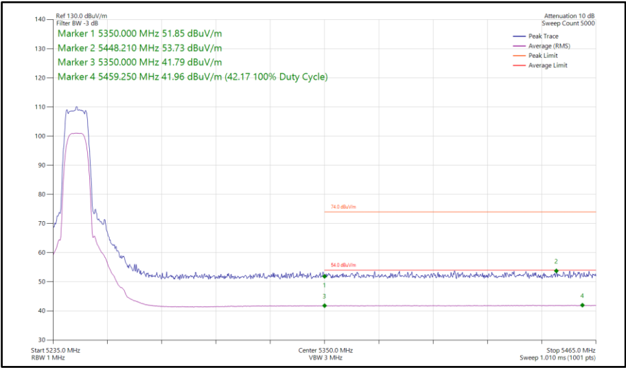
Figure 81 - HDRPL8, MIMO, Core 0-1 - 5245 MHz Band Edge Frequency 5350 MHz
