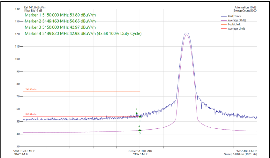
Figure 116 - LE1M, SISO, Core 1 - 5162 MHz Band Edge Frequency 5150 MHz
