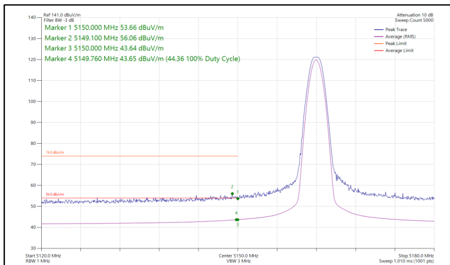
Figure 88 - LE1M, SISO, Core 0 - 5162 MHz Band Edge Frequency 5150 MHz
