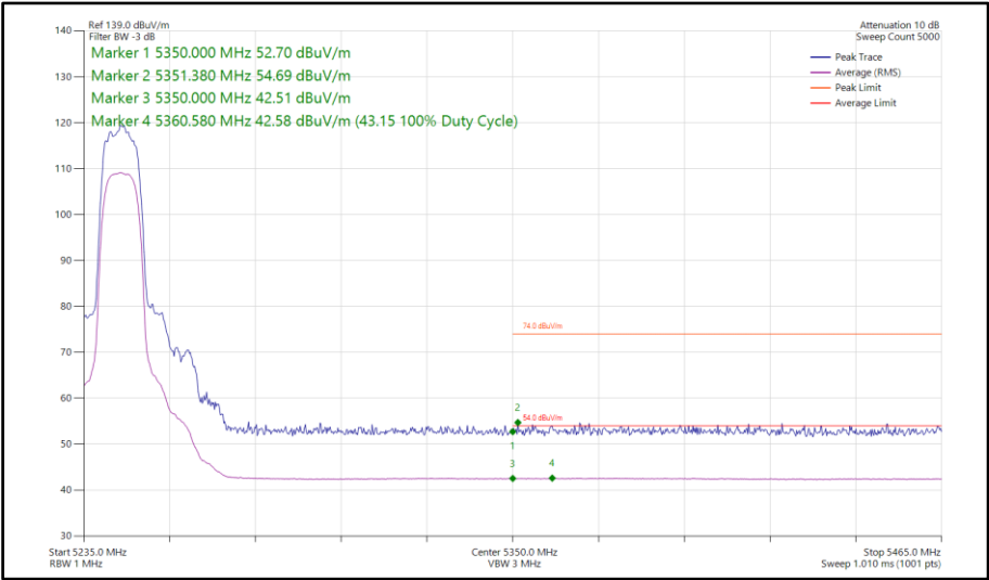
Figure 110 - HDRPL24, SISO, Core 0 - 5245 MHz Band Edge Frequency 5350 MHz
