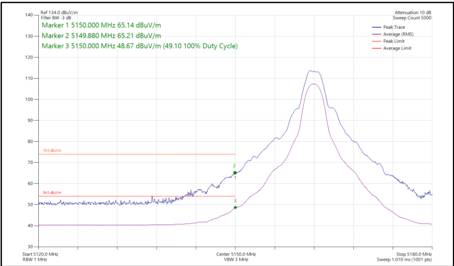
Figure 64 - HDT6, MIMO, Core 0-1 - 5162 MHz Band Edge Frequency 5150 MHz
