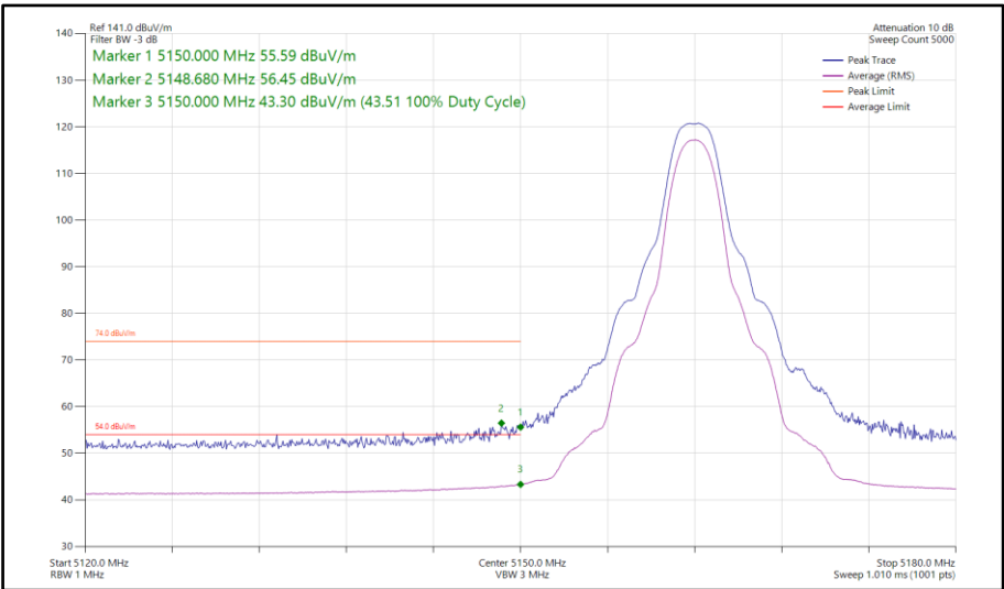
Figure 118 - HDT3, SISO, Core 1 - 5162 MHz Band Edge Frequency 5150 MHz
