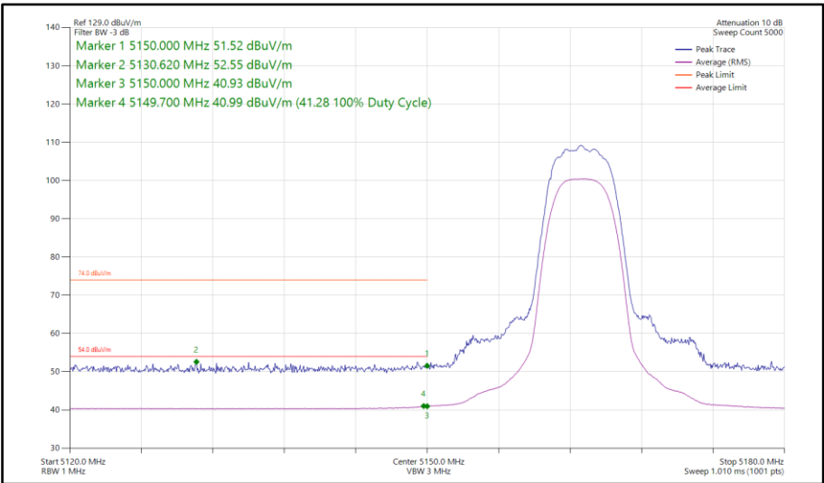
Figure 66 - HDRPM12, MIMO, Core 0-1 - 5163 MHz Band Edge Frequency 5150 MHz
