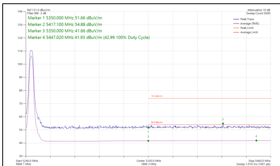
Figure 72 - HDR4, MIMO, Core 0-1 - 5245 MHz Band Edge Frequency 5350 MHz
