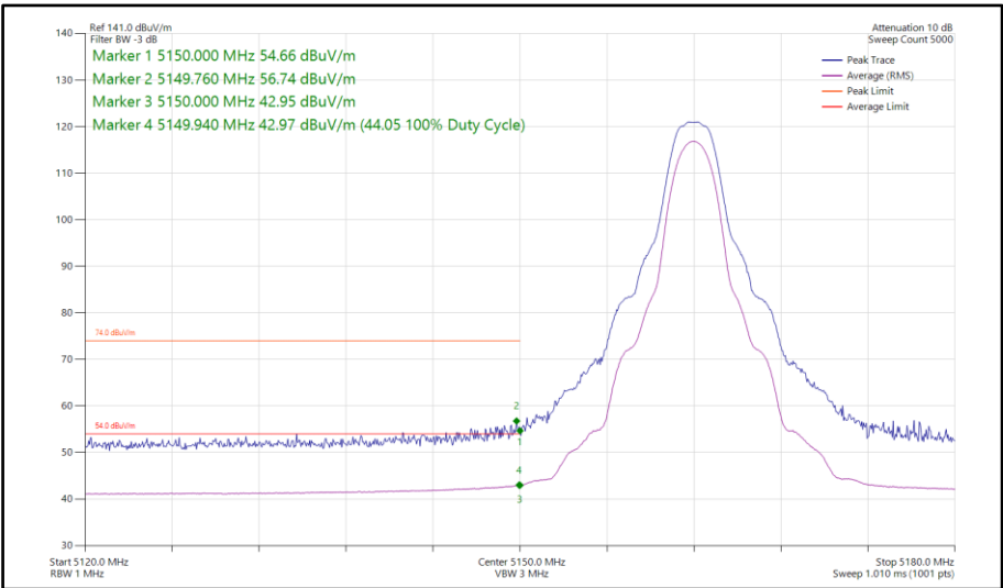
Figure 114 - HDR4, SISO, Core 1 - 5162 MHz Band Edge Frequency 5150 MHz
