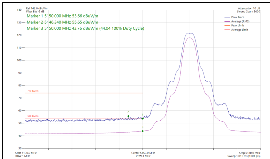
Figure 91 - HDT4, SISO, Core 0 - 5162 MHz Band Edge Frequency 5150 MHz
