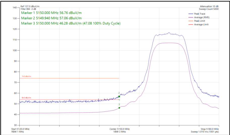
Figure 98 - XHDRPL24, SISO, Core 0 - 5165 MHz Band Edge Frequency 5150 MHz
