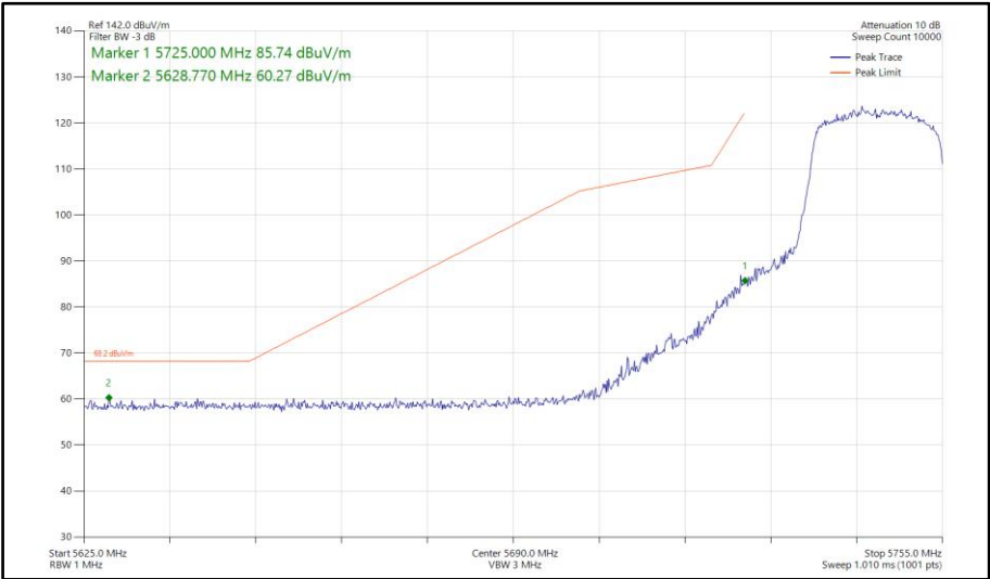
Figure 620 - 802.11ax HE20, SU, SDM, Core 0-1 - 5745 MHz Band Edge Frequency 5725 MHz
