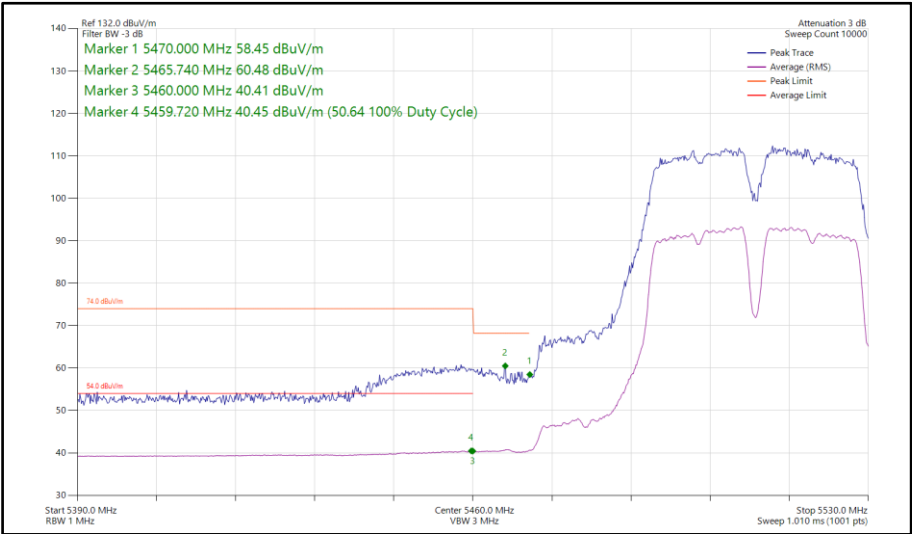
Figure 644 - 802.11a a40, SISO, Core 0 - 5510 MHz Band Edge Frequency 5470 MHz
