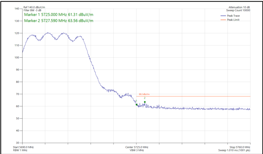
Figure 601 - 802.11n HT20, CDD, Core 0-1 - 5700 MHz Band Edge Frequency 5725 MHz
