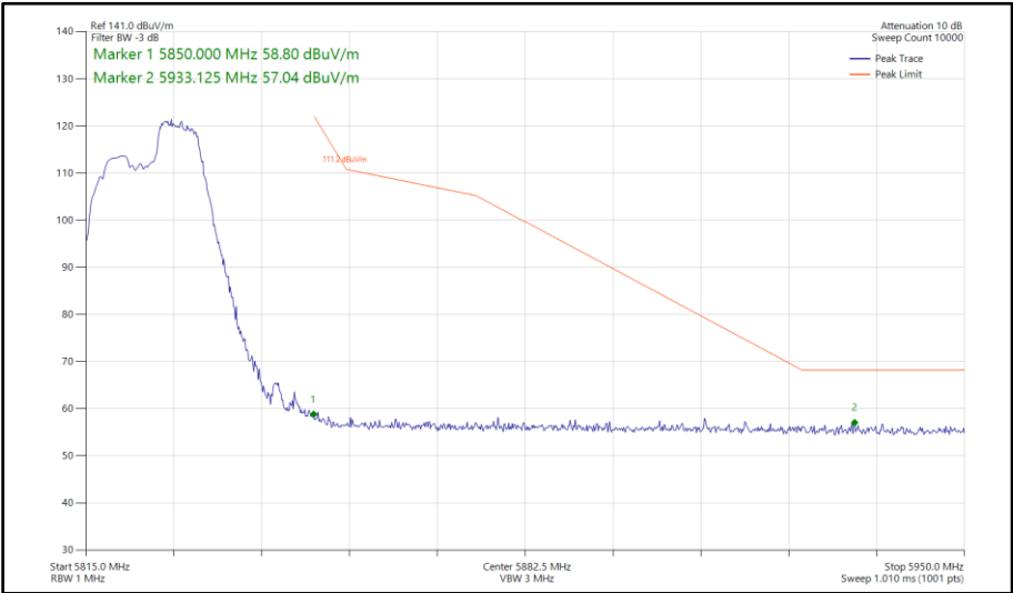
Figure 589 - 802.11be EHT20, RU 52+26-72, SISO, Core 1 - 5825 MHz Band Edge Frequency 5850 MHz
