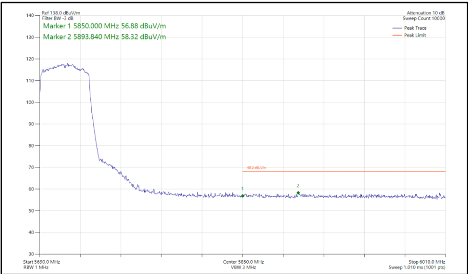
Figure 663 - 802.11ax HE40, SU, SISO, Core 0 - 5710 MHz Band Edge Frequency 5850 MHz
