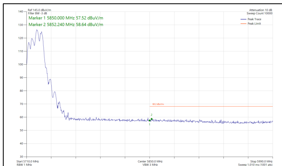
Figure 613 - 802.11be EHT20, RU 106+26-83, CDD, Core 0-1 - 5720 MHz Band Edge Frequency 5850 MHz
