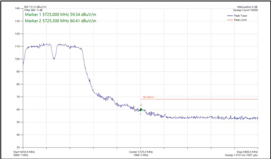
Figure 654 - 802.11a a40, SISO, Core 0 - 5670 MHz Band Edge Frequency 5725 MHz
