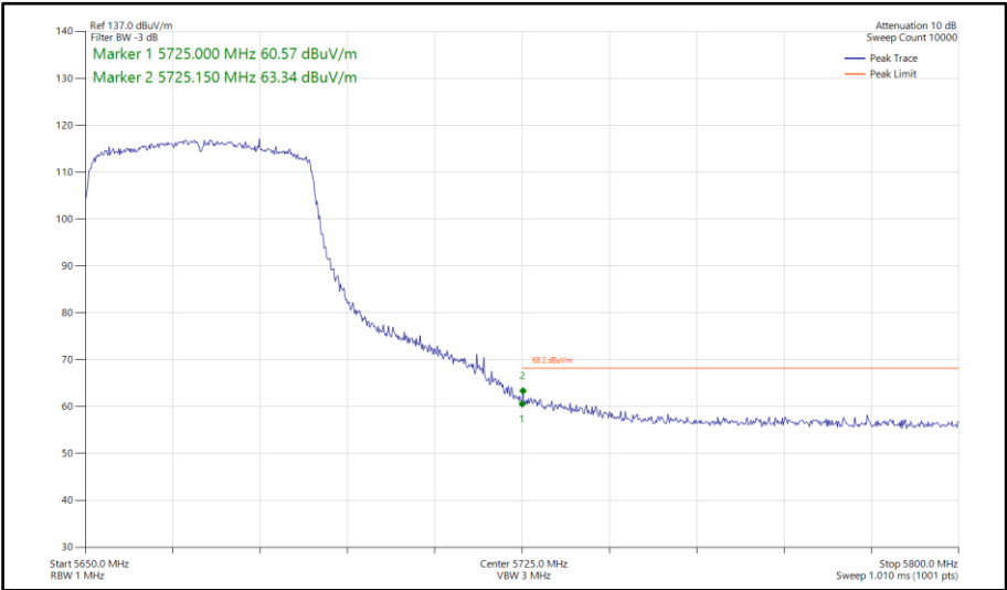
Figure 656 - 802.11ax HE40, SU, SISO, Core 0 - 5670 MHz Band Edge Frequency 5725 MHz
