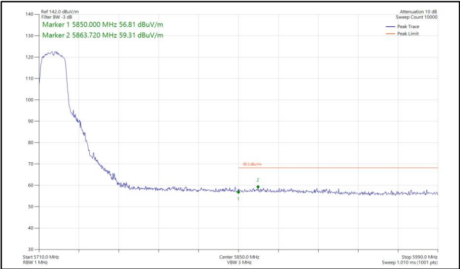
Figure 626 - 802.11n HT20, SDM, Core 0-1 - 5720 MHz Band Edge Frequency 5850 MHz
