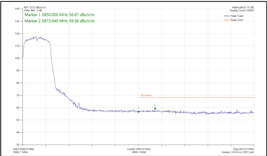
Figure 661 - 802.11n HT40, SISO, Core 0 - 5710 MHz Band Edge Frequency 5850 MHz
