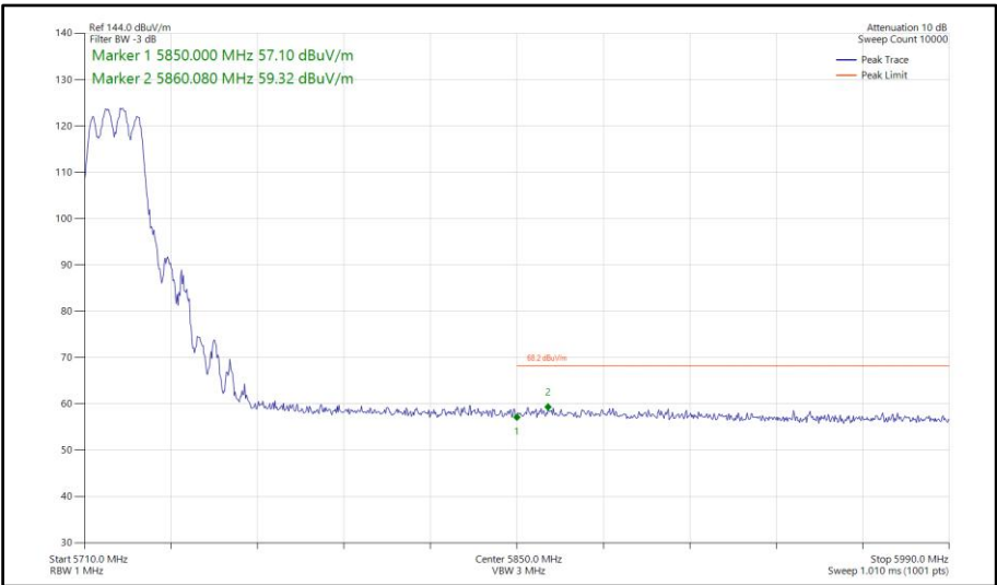
Figure 605 - 802.11a, CDD, Core 0-1 - 5720 MHz Band Edge Frequency 5850 MHz
