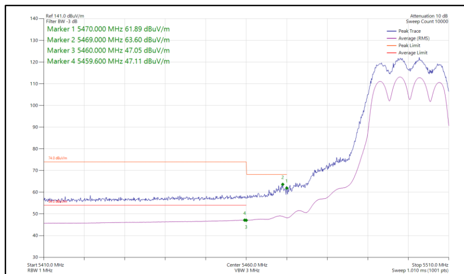
Figure 634 - 802.11ac VHT20, TxBF, Core 0-1 - 5500 MHz Band Edge Frequency 5470 MHz
