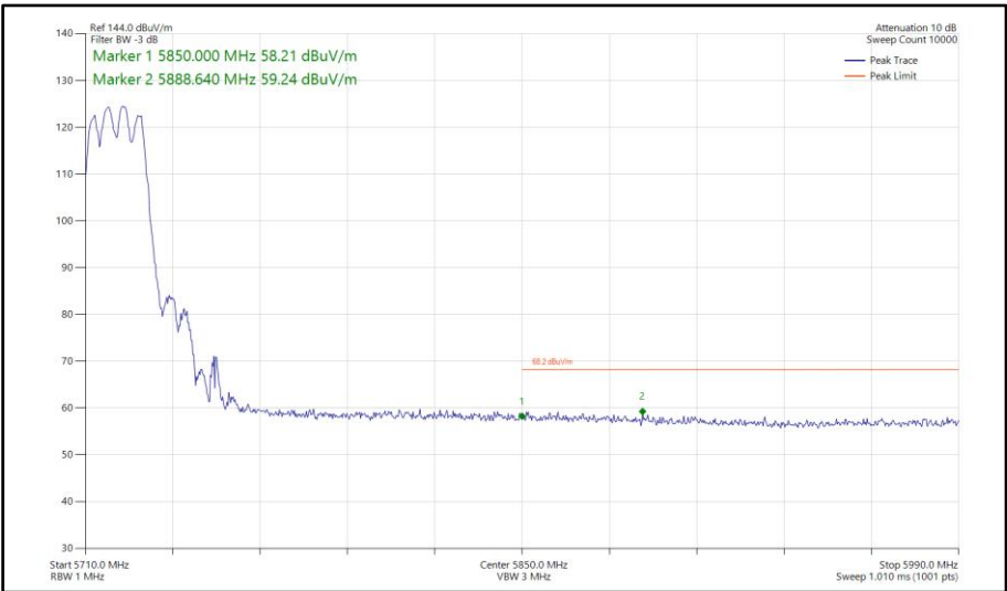
Figure 642 - 802.11ax HE20, SU, TxBF, Core 0-1 - 5720 MHz Band Edge Frequency 5850 MHz
