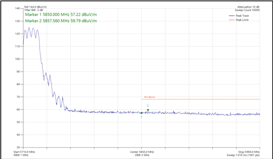
Figure 609 - 802.11ax HE20, SU, CDD, Core 0-1 - 5720 MHz Band Edge Frequency 5850 MHz
