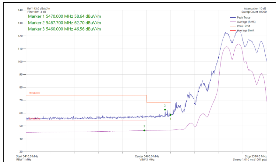
Figure 618 - 802.11be EHT20, RU 106+26-82, SDM, Core 0-1 - 5500 MHz Band Edge Frequency 5470 MHz
