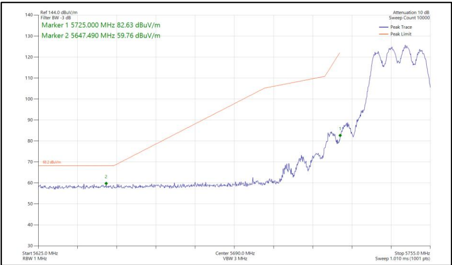
Figure 597 - 802.11ax HE20, SU, CDD, Core 0-1 - 5745 MHz Band Edge Frequency 5725 MHz
