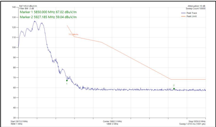
Figure 633 - 802.11be EHT20, RU 106+26-83, SDM, Core 0-1 - 5825 MHz Band Edge Frequency 5850 MHz
