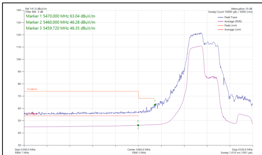
Figure 647 - 802.11ax HE40, RU 106-53, SISO, Core 0 - 5510 MHz Band Edge Frequency 5470 MHz
