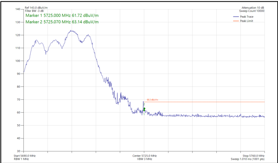
Figure 625 - 802.11ax HE20, RU 106-54, SDM, Core 0-1 - 5700 MHz Band Edge Frequency 5725 MHz
