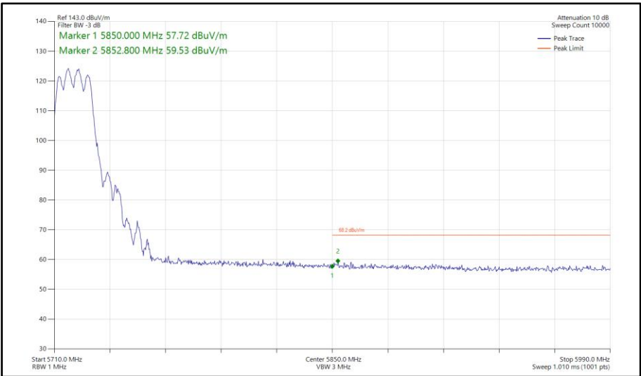
Figure 640 - 802.11ac VHT20, TxBF, Core 0-1 - 5720 MHz Band Edge Frequency 5850 MHz
