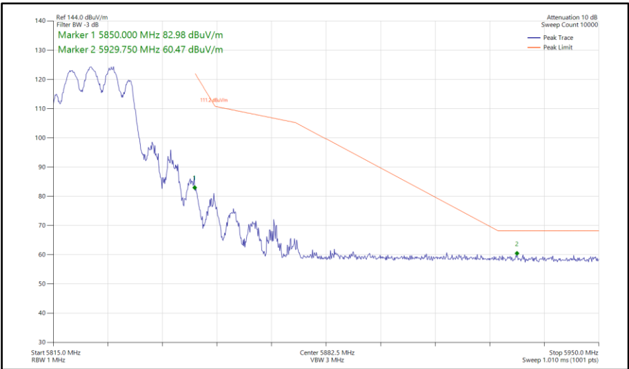
Figure 611 - 802.11ax HE20, SU, CDD, Core 0-1 - 5825 MHz Band Edge Frequency 5850 MHz
