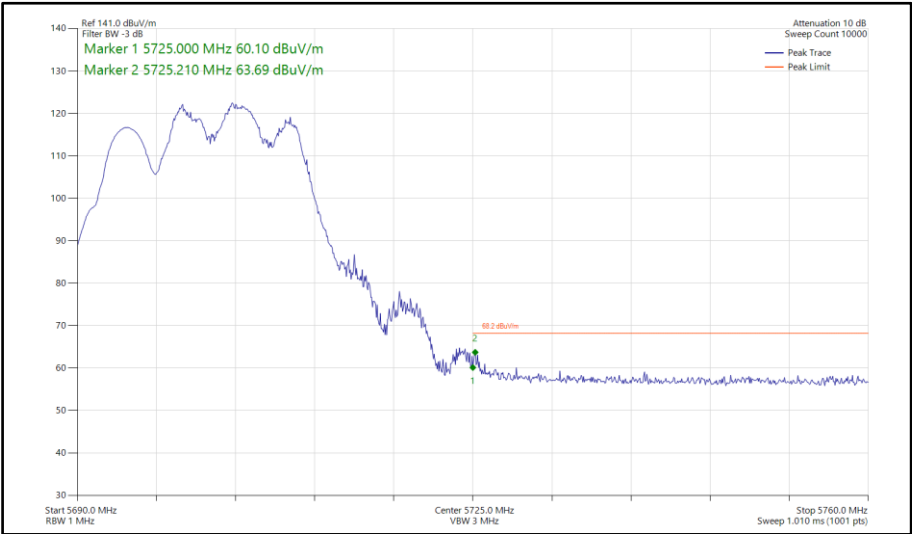
Figure 604 - 802.11be EHT20, RU 106+26-83, CDD, Core 0-1 - 5700 MHz Band Edge Frequency 5725 MHz
