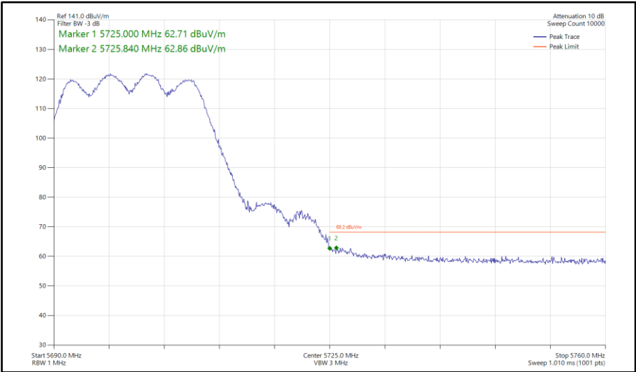
Figure 600 - 802.11a, CDD, Core 0-1 - 5700 MHz Band Edge Frequency 5725 MHz
