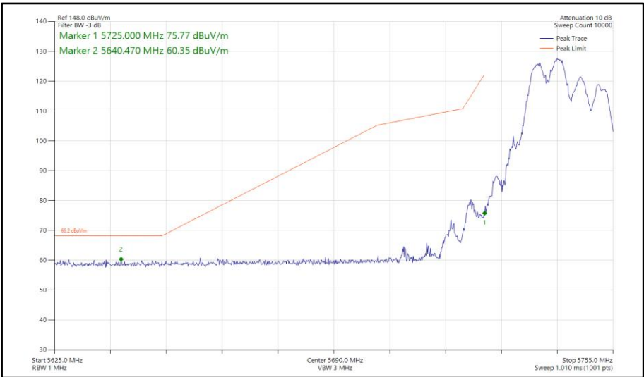
Figure 621 - 802.11ax HE20, RU 106-53, SDM, Core 0-1 - 5745 MHz Band Edge Frequency 5725 MHz
