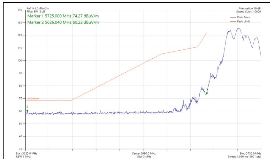
Figure 622 - 802.11be EHT20, RU 106+26-82, SDM, Core 0-1 - 5745 MHz Band Edge Frequency 5725 MHz
