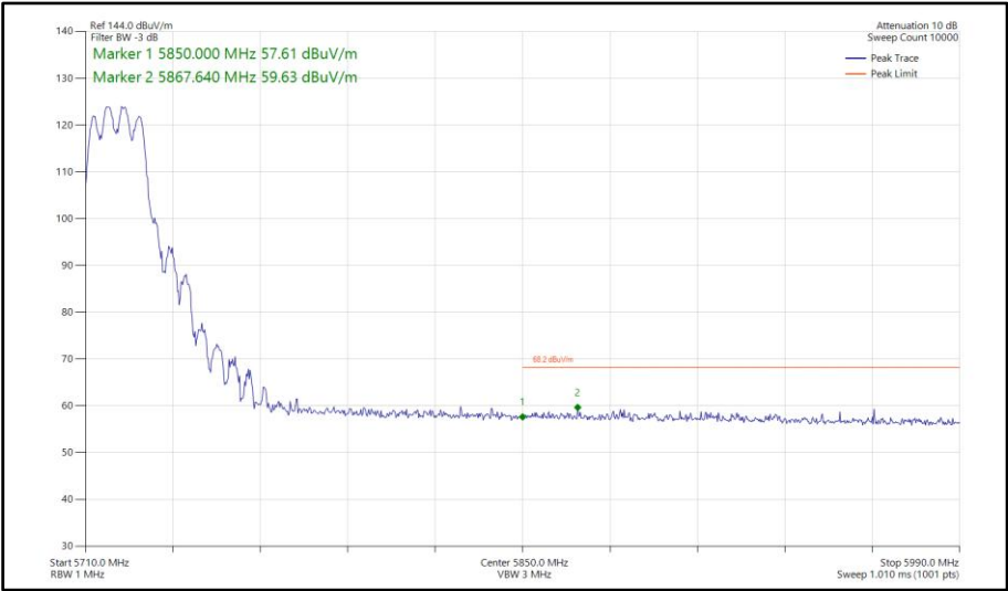
Figure 607 - 802.11n HT20, CDD, Core 0-1 - 5720 MHz Band Edge Frequency 5850 MHz
