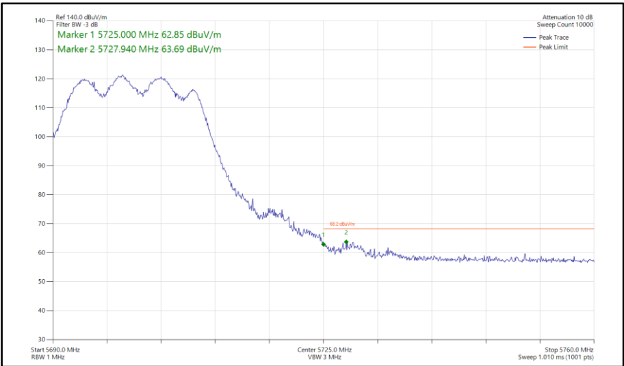
Figure 638 - 802.11ac VHT20, TxBF, Core 0-1 - 5700 MHz Band Edge Frequency 5725 MHz
