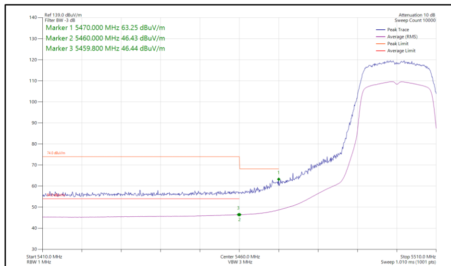
Figure 615 - 802.11n HT20, SDM, Core 0-1 - 5500 MHz Band Edge Frequency 5470 MHz
