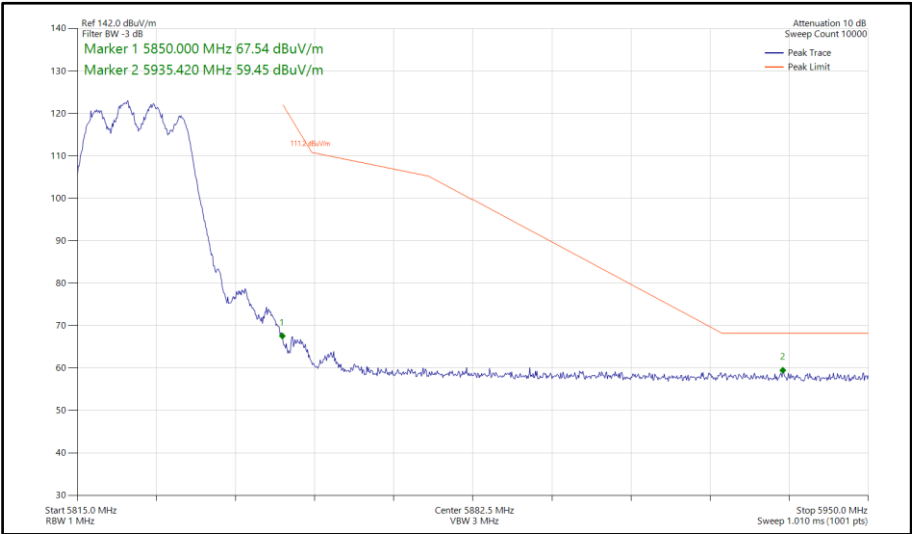
Figure 608 - 802.11n HT20, CDD, Core 0-1 - 5825 MHz Band Edge Frequency 5850 MHz
