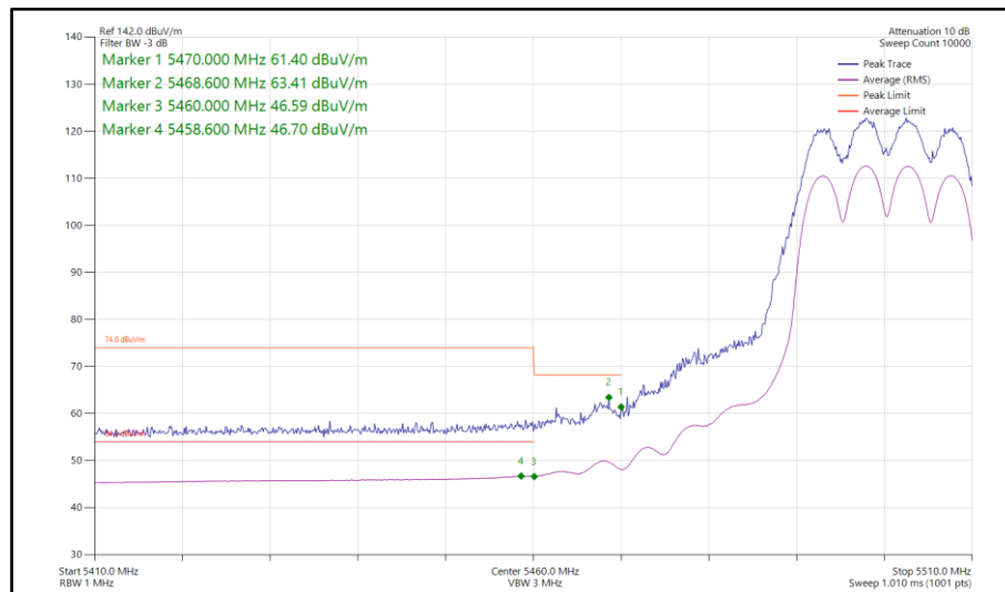
Figure 592 - 802.11ax HE20, SU, CDD, Core 0-1 - 5500 MHz Band Edge Frequency 5470 MHz
