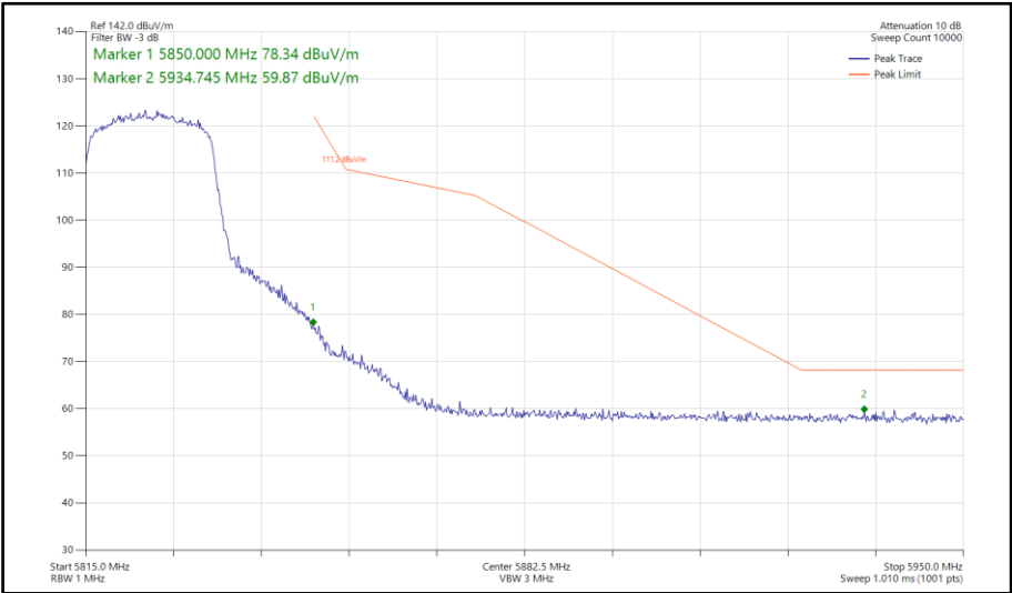
Figure 630 - 802.11ax HE20, SU, SDM, Core 0-1 - 5825 MHz Band Edge Frequency 5850 MHz
