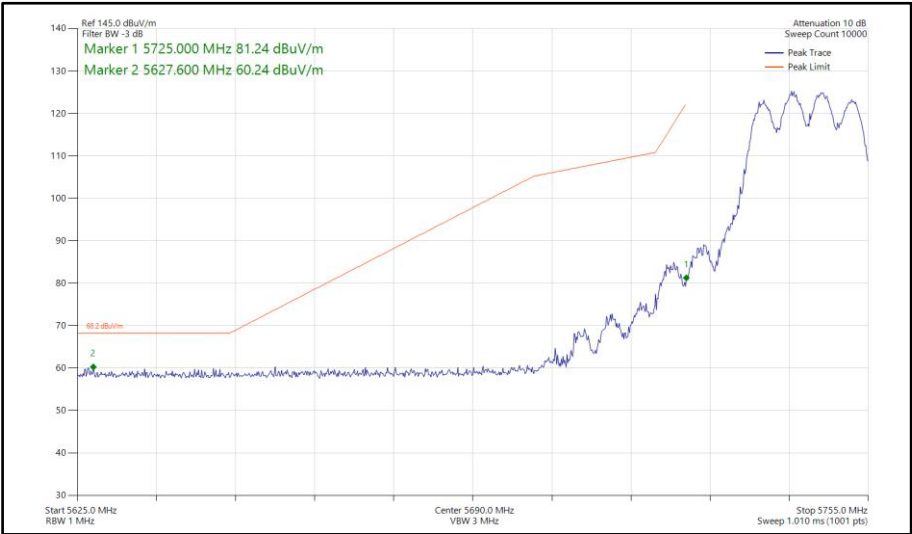
Figure 637 - 802.11ax HE20, SU, TxBF, Core 0-1 - 5745 MHz Band Edge Frequency 5725 MHz
