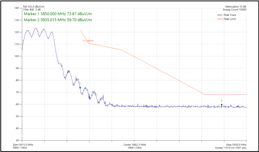
Figure 606 - 802.11a, CDD, Core 0-1 - 5825 MHz Band Edge Frequency 5850 MHz
