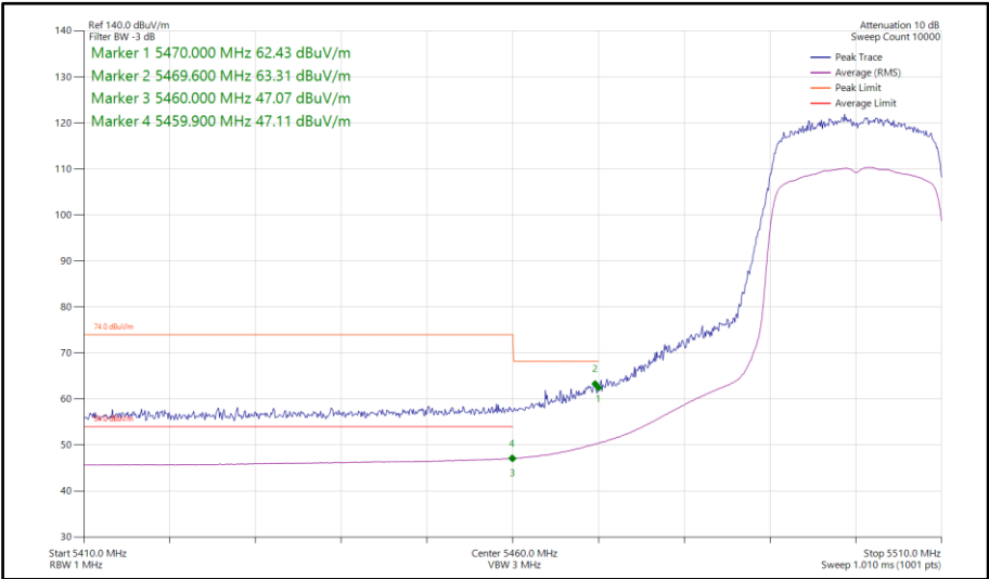
Figure 616 - 802.11ax HE20, SU, SDM, Core 0-1 - 5500 MHz Band Edge Frequency 5470 MHz
