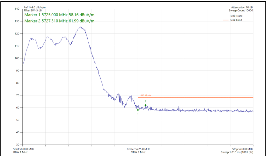
Figure 603 - 802.11ax HE20, RU 52-40, CDD, Core 0-1 - 5700 MHz Band Edge Frequency 5725 MHz
