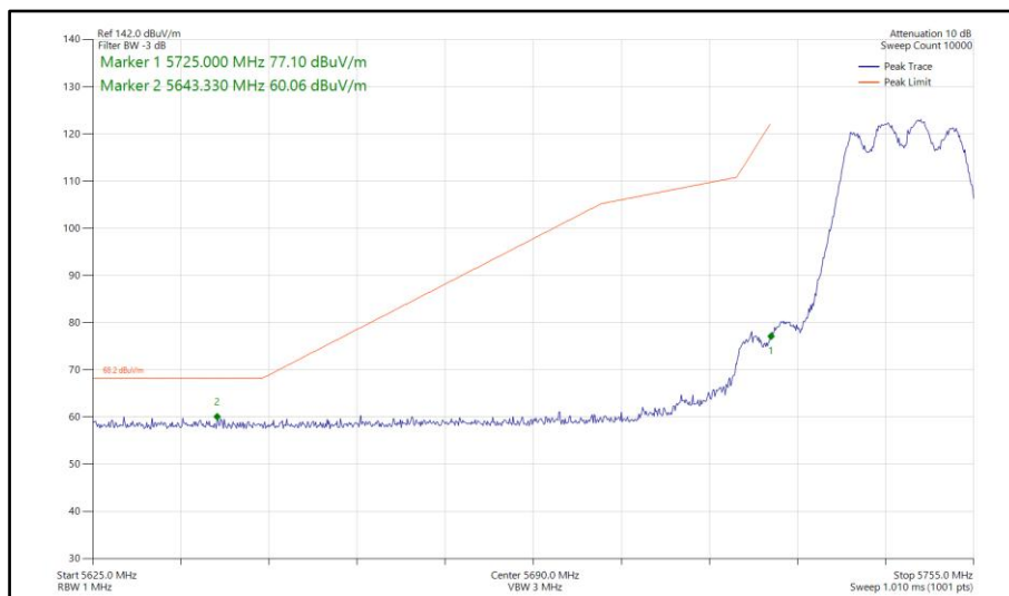
Figure 595 - 802.11a, CDD, Core 0-1 - 5745 MHz Band Edge Frequency 5725 MHz
