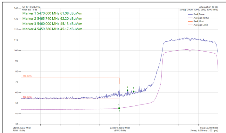
Figure 646 - 802.11ax HE40, SU, SISO, Core 0 - 5510 MHz Band Edge Frequency 5470 MHz
