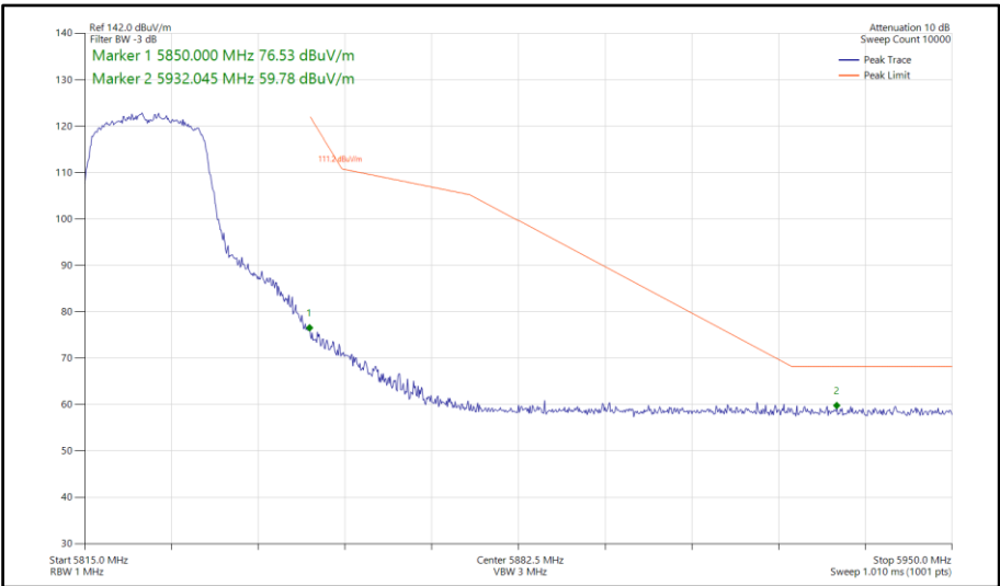
Figure 627 - 802.11n HT20, SDM, Core 0-1 - 5825 MHz Band Edge Frequency 5850 MHz
