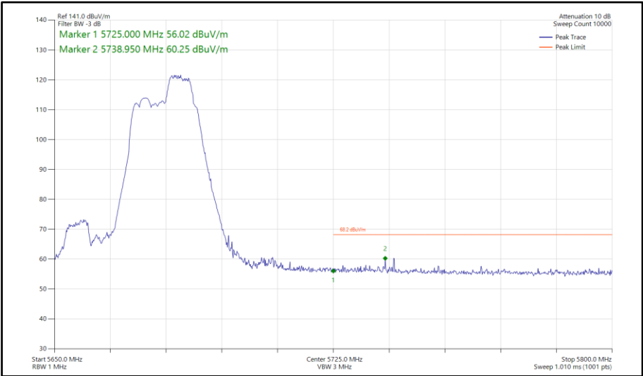
Figure 658 - 802.11be EHT40, RU 52+26-75, SISO, Core 0 - 5670 MHz Band Edge Frequency 5725 MHz
