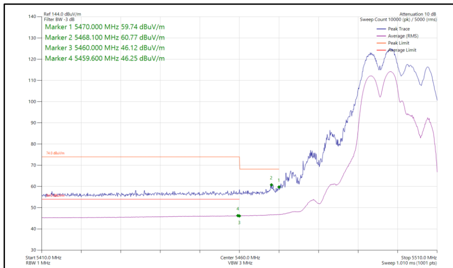
Figure 594 - 802.11be EHT20, RU 106+26-82, CDD, Core 0-1 - 5500 MHz Band Edge Frequency 5470 MHz
