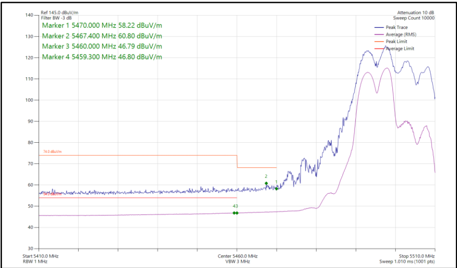
Figure 617 - 802.11ax HE20, RU 106-53, SDM, Core 0-1 - 5500 MHz Band Edge Frequency 5470 MHz
