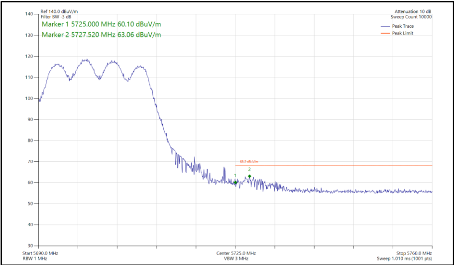
Figure 639 - 802.11ax HE20, SU, TxBF, Core 0-1 - 5700 MHz Band Edge Frequency 5725 MHz
