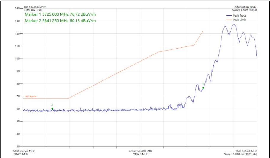
Figure 598 - 802.11ax HE20, RU 106-53, CDD, Core 0-1 - 5745 MHz Band Edge Frequency 5725 MHz
