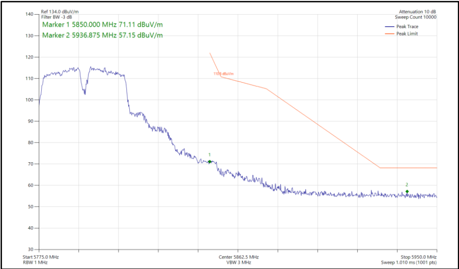
Figure 660 - 802.11a a40, SISO, Core 0 - 5795 MHz Band Edge Frequency 5850 MHz
