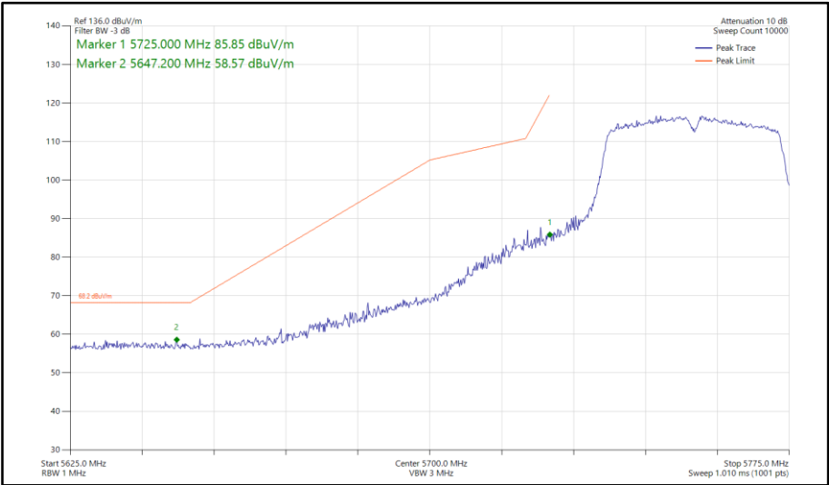
Figure 650 - 802.11n HT40, SISO, Core 0 - 5755 MHz Band Edge Frequency 5725 MHz
