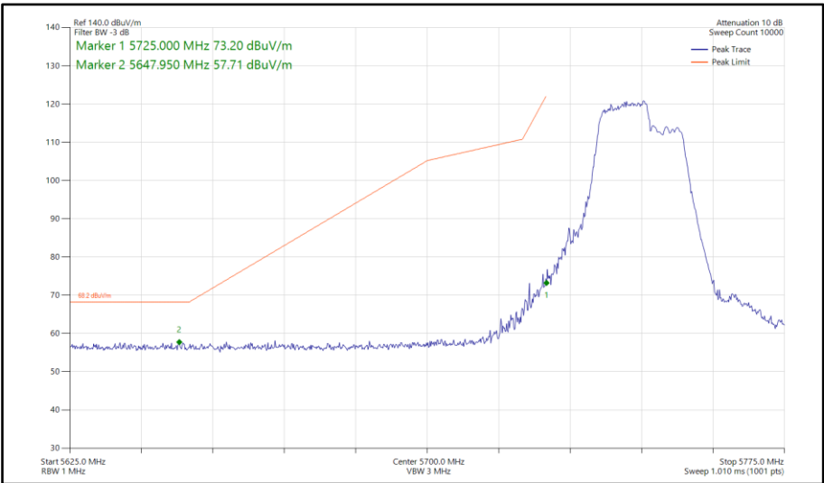
Figure 653 - 802.11be EHT40, RU 106+26-82, SISO, Core 0 - 5755 MHz Band Edge Frequency 5725 MHz
