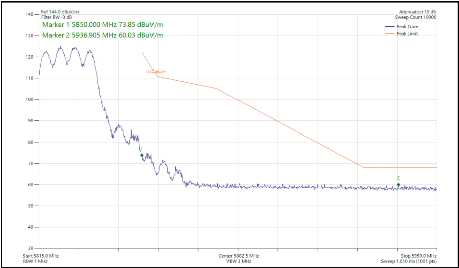
Figure 643 - 802.11ax HE20, SU, TxBF, Core 0-1 - 5825 MHz Band Edge Frequency 5850 MHz
