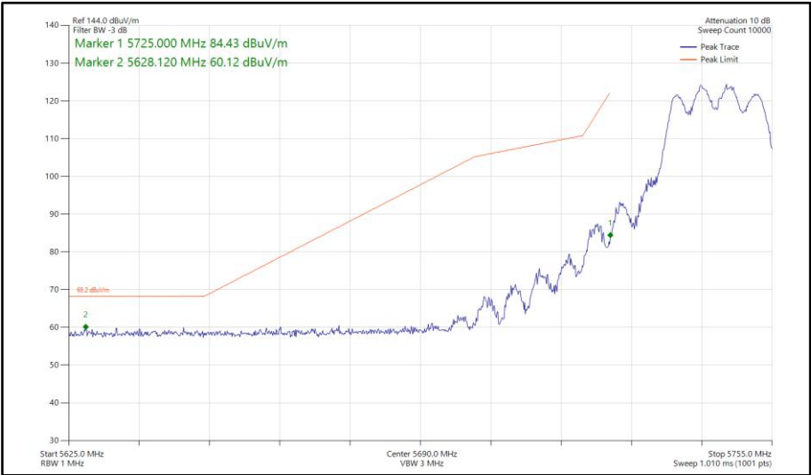
Figure 596 - 802.11n HT20, CDD, Core 0-1 - 5745 MHz Band Edge Frequency 5725 MHz
