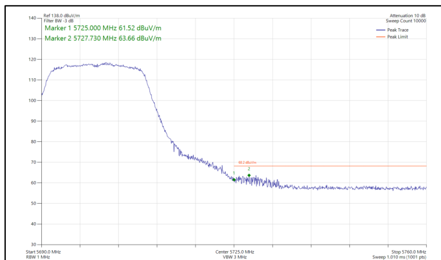
Figure 623 - 802.11n HT20, SDM, Core 0-1 - 5700 MHz Band Edge Frequency 5725 MHz
