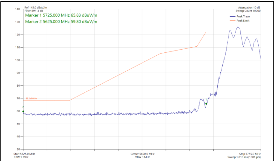
Figure 599 - 802.11be EHT20, RU 52+26-70, CDD, Core 0-1 - 5745 MHz Band Edge Frequency 5725 MHz
