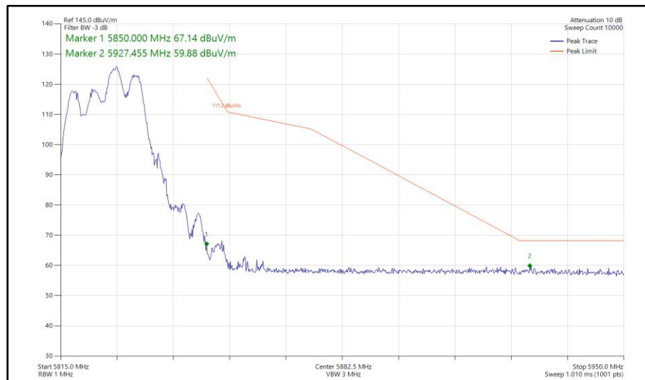
Figure 612 - 802.11ax HE20, RU 106-54, CDD, Core 0-1 - 5825 MHz Band Edge Frequency 5850 MHz
