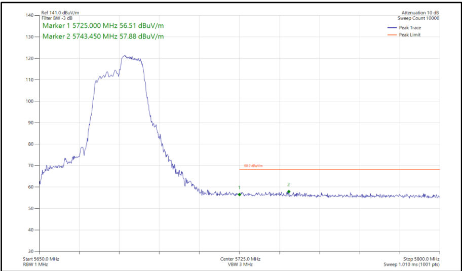
Figure 657 - 802.11ax HE40, RU 106-56, SISO, Core 0 - 5670 MHz Band Edge Frequency 5725 MHz
