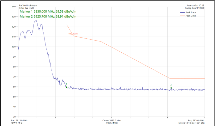
Figure 614 - 802.11be EHT20, RU 52+26-72, CDD, Core 0-1 - 5825 MHz Band Edge Frequency 5850 MHz
