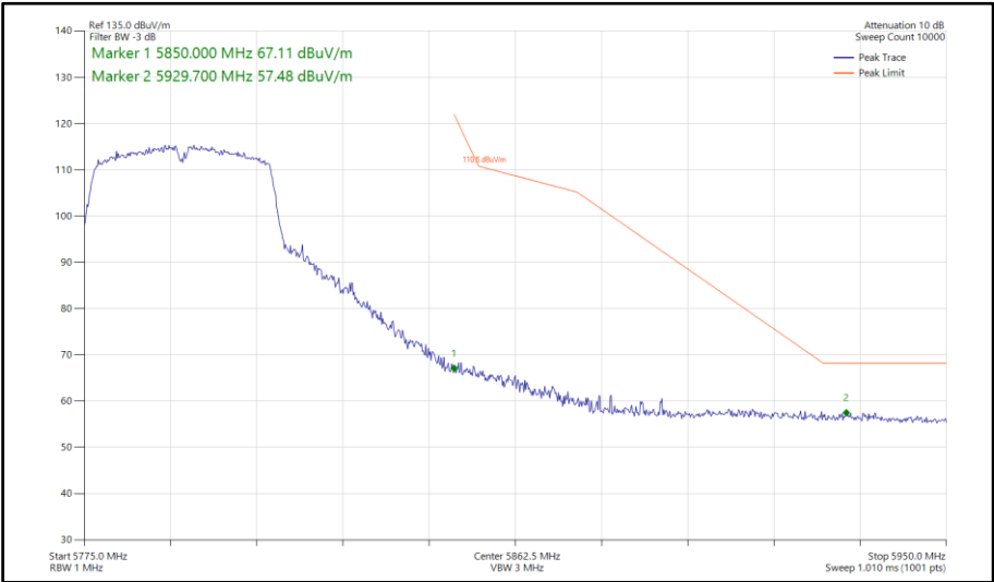
Figure 662 - 802.11n HT40, SISO, Core 0 - 5795 MHz Band Edge Frequency 5850 MHz
