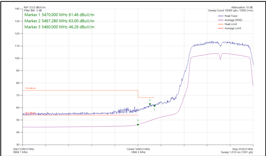
Figure 645 - 802.11n HT40, SISO, Core 0 - 5510 MHz Band Edge Frequency 5470 MHz
