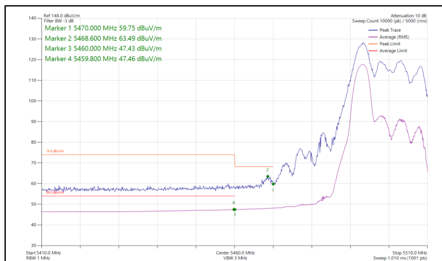
Figure 593 - 802.11ax HE20, RU 52-37, CDD, Core 0-1 - 5500 MHz Band Edge Frequency 5470 MHz
