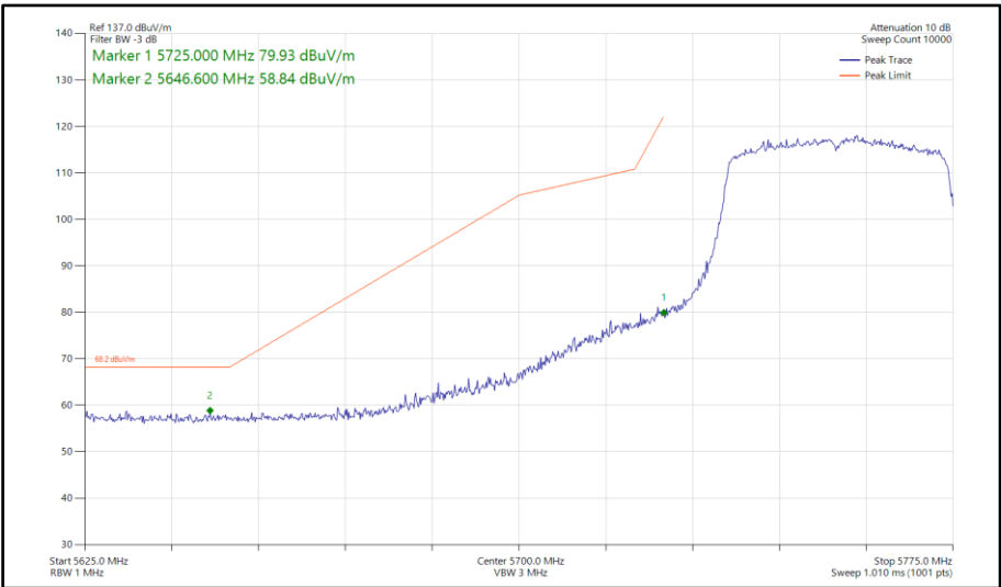
Figure 651 - 802.11ax HE40, SU, SISO, Core 0 - 5755 MHz Band Edge Frequency 5725 MHz
