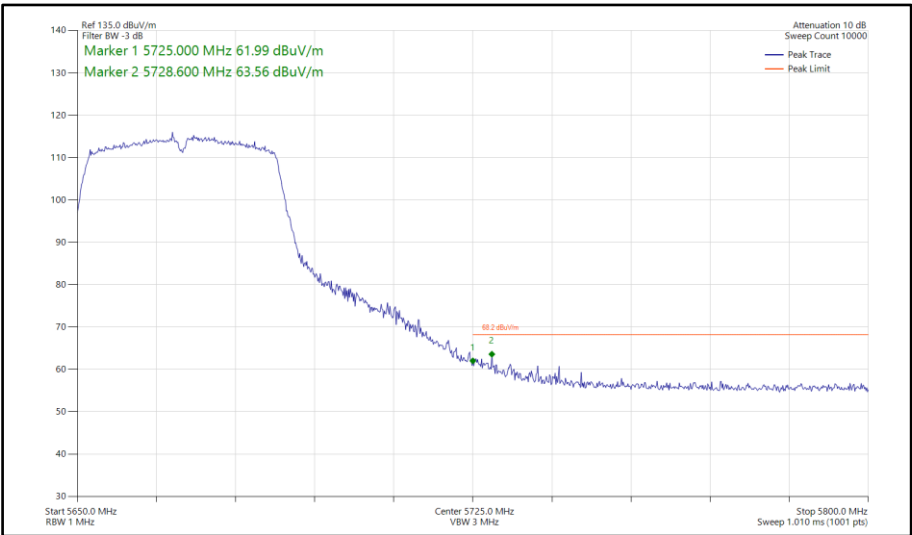
Figure 655 - 802.11n HT40, SISO, Core 0 - 5670 MHz Band Edge Frequency 5725 MHz
