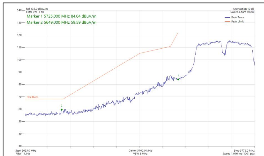
Figure 649 - 802.11a a40, SISO, Core 0 - 5755 MHz Band Edge Frequency 5725 MHz
