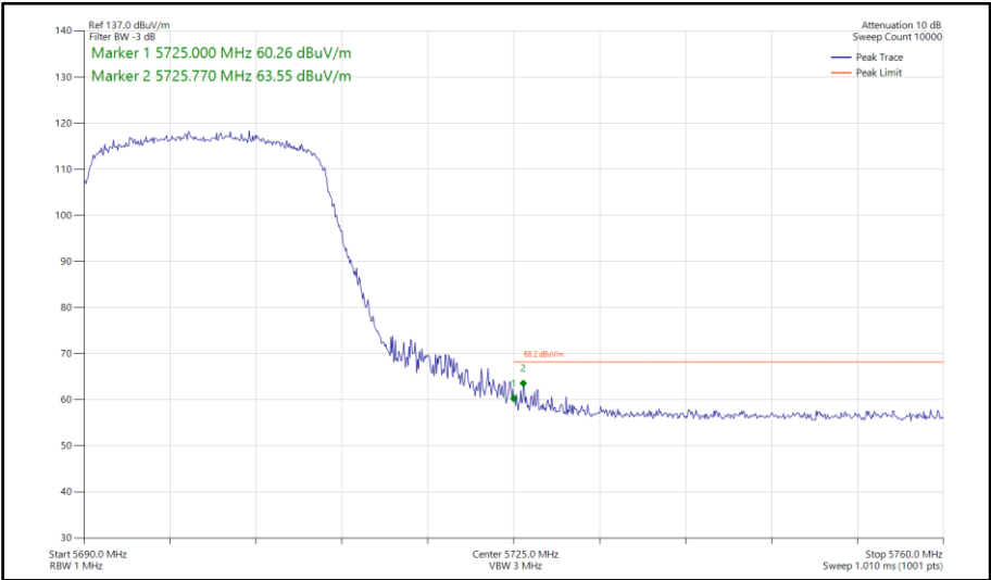
Figure 624 - 802.11ax HE20, SU, SDM, Core 0-1 - 5700 MHz Band Edge Frequency 5725 MHz
