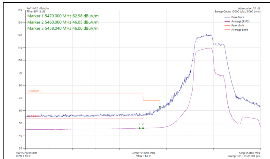
Figure 648 - 802.11be EHT40, RU 106+26-82, SISO, Core 0 - 5510 MHz Band Edge Frequency 5470 MHz
