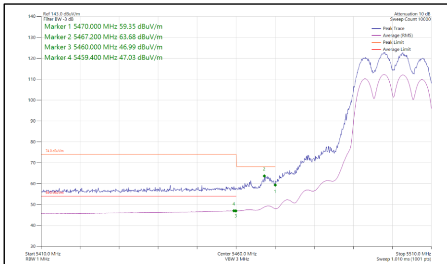
Figure 635 - 802.11ax HE20, SU, TxBF, Core 0-1 - 5500 MHz Band Edge Frequency 5470 MHz
