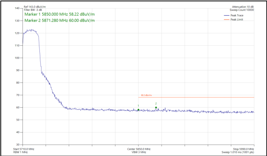
Figure 628 - 802.11ax HE20, SU, SDM, Core 0-1 - 5720 MHz Band Edge Frequency 5850 MHz
