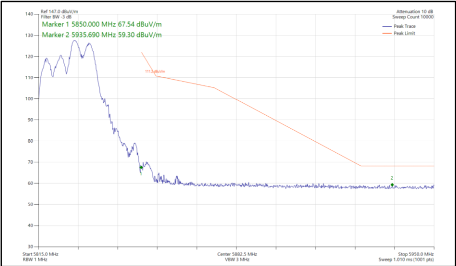
Figure 631 - 802.11ax HE20, RU 106-54, SDM, Core 0-1 - 5825 MHz Band Edge Frequency 5850 MHz
