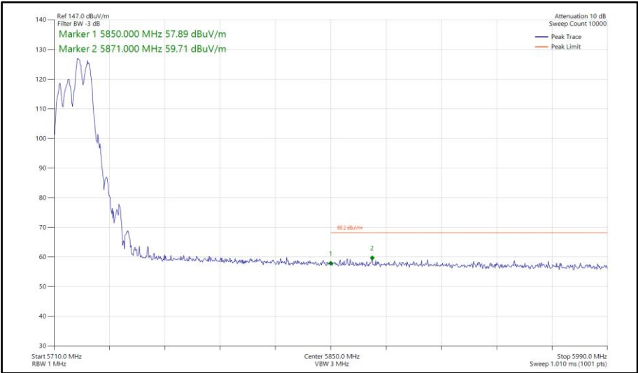
Figure 610 - 802.11ax HE20, RU 106-54, CDD, Core 0-1 - 5720 MHz Band Edge Frequency 5850 MHz
