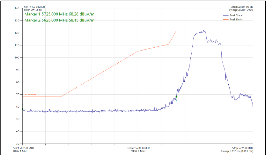
Figure 652 - 802.11ax HE40, RU 106-53, SISO, Core 0 - 5755 MHz Band Edge Frequency 5725 MHz
