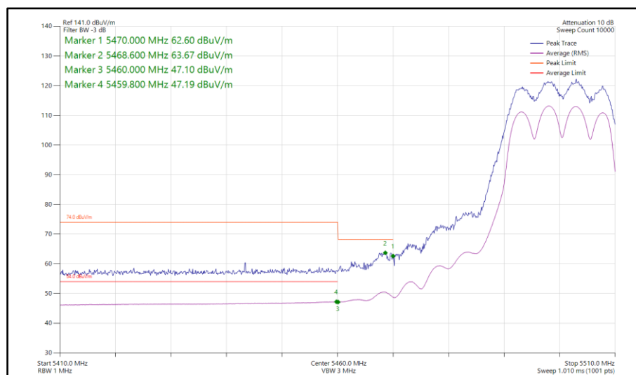
Figure 591 - 802.11n HT20, CDD, Core 0-1 - 5500 MHz Band Edge Frequency 5470 MHz
