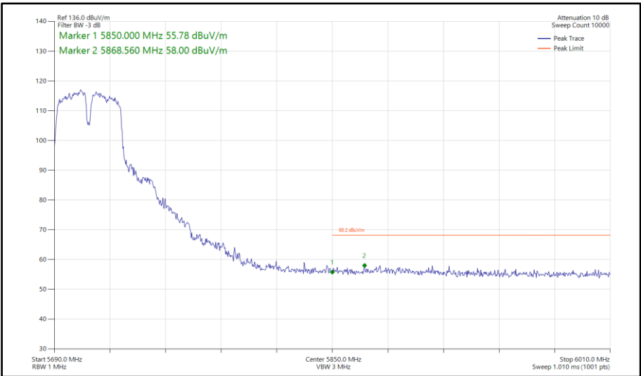
Figure 659 - 802.11a a40, SISO, Core 0 - 5710 MHz Band Edge Frequency 5850 MHz
