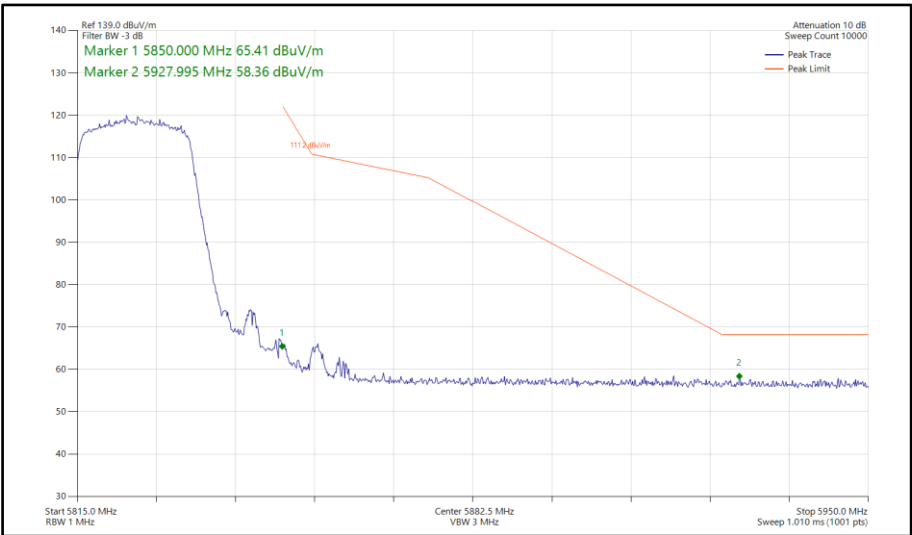
Figure 586 - 802.11ax HE20, SU, SISO, Core 1 - 5825 MHz Band Edge Frequency 5850 MHz
