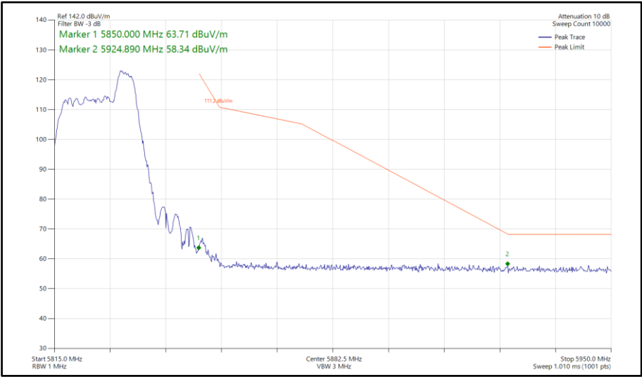
Figure 587 - 802.11ax HE20, RU 52-40, SISO, Core 1 - 5825 MHz Band Edge Frequency 5850 MHz
