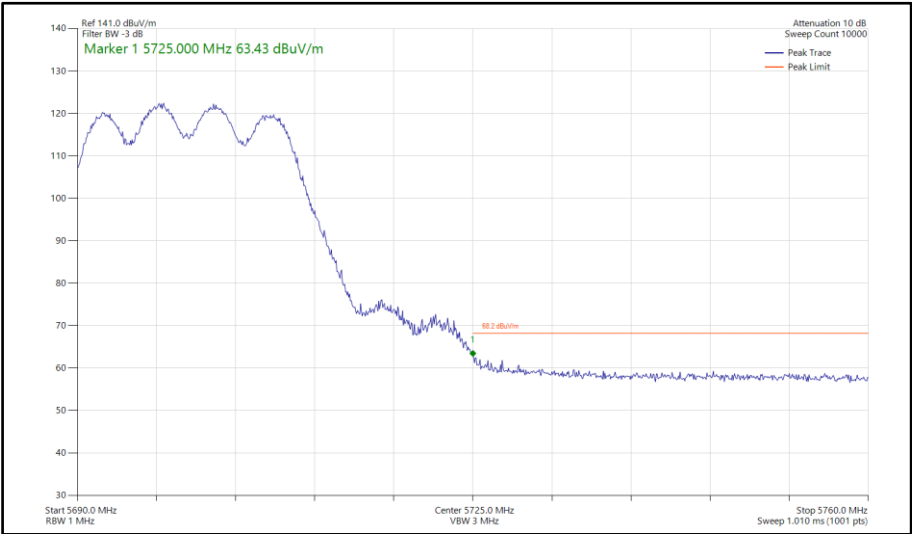
Figure 602 - 802.11ax HE20, SU, CDD, Core 0-1 - 5700 MHz Band Edge Frequency 5725 MHz
