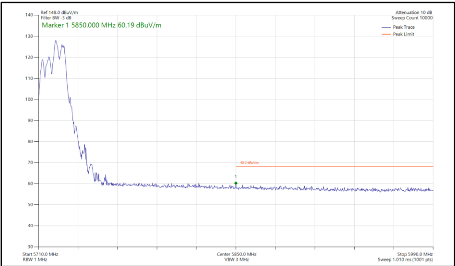
Figure 629 - 802.11ax HE20, RU 106-54, SDM, Core 0-1 - 5720 MHz Band Edge Frequency 5850 MHz
