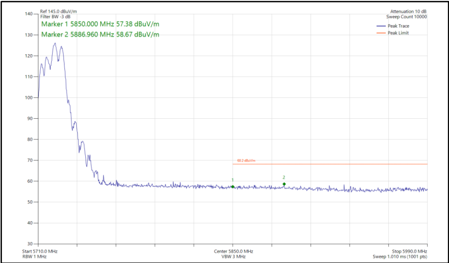
Figure 632 - 802.11be EHT20, RU 106+26-83, SDM, Core 0-1 - 5720 MHz Band Edge Frequency 5850 MHz
