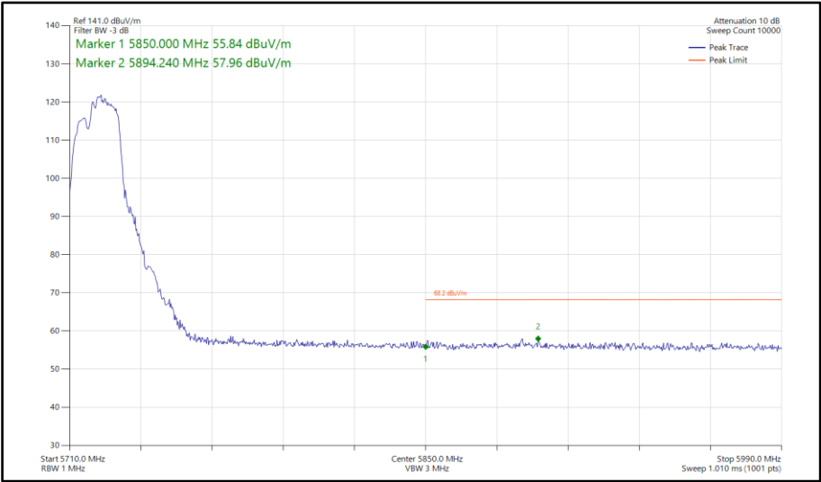
Figure 588 - 802.11be EHT20, RU 106+26-83, SISO, Core 1 - 5720 MHz Band Edge Frequency 5850 MHz
