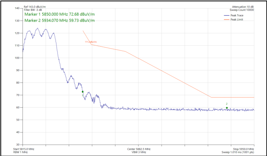
Figure 641 - 802.11ac VHT20, TxBF, Core 0-1 - 5825 MHz Band Edge Frequency 5850 MHz
