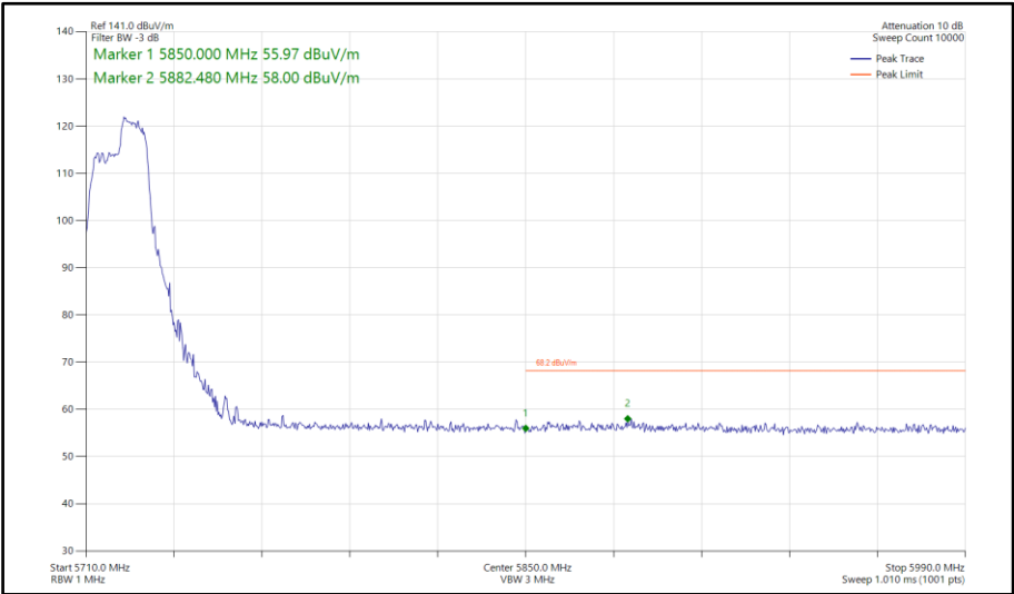
Figure 585 - 802.11ax HE20, RU 106-54, SISO, Core 1 - 5720 MHz Band Edge Frequency 5850 MHz
