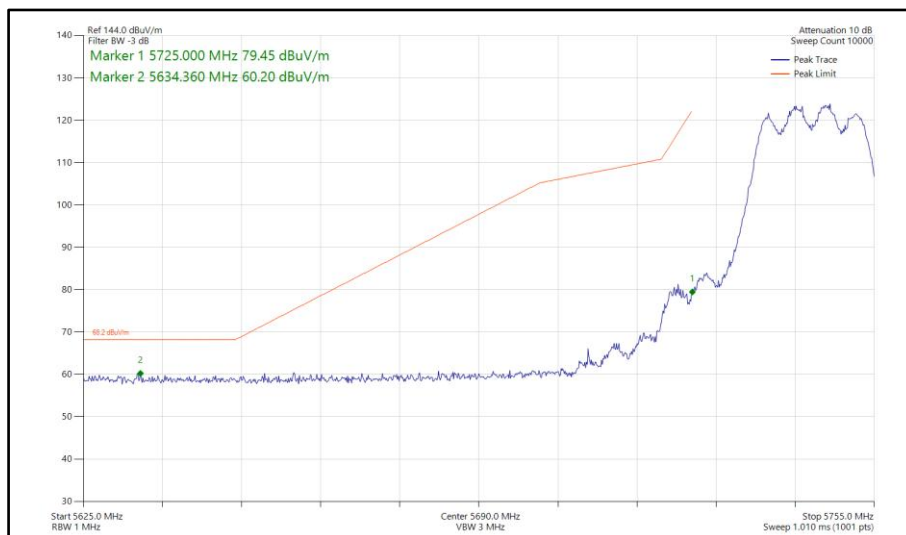
Figure 636 - 802.11ac VHT20, TxBF, Core 0-1 - 5745 MHz Band Edge Frequency 5725 MHz
