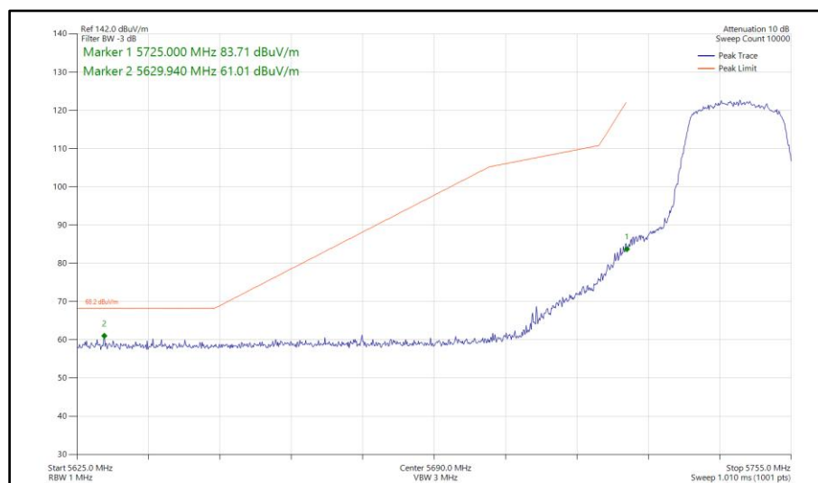
Figure 619 - 802.11n HT20, SDM, Core 0-1 - 5745 MHz Band Edge Frequency 5725 MHz
