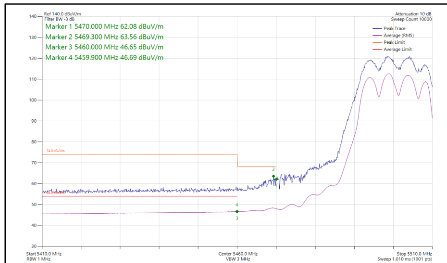
Figure 590 - 802.11a, CDD, Core 0-1 - 5500 MHz Band Edge Frequency 5470 MHz
