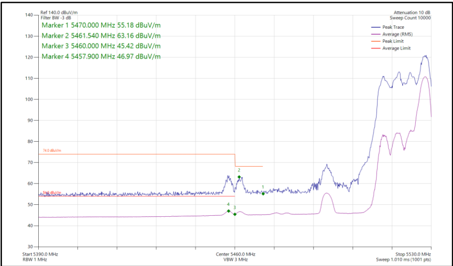
Figure 697 - 802.11ax HE40, RU 52-44, CDD, Core 0-1 - 5510 MHz Band Edge Frequency 5470 MHz
