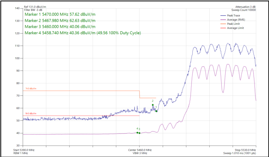
Figure 694 - 802.11a a40, CDD, Core 0-1 - 5510 MHz Band Edge Frequency 5470 MHz
