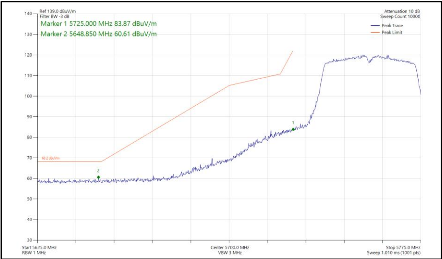
Figure 724 - 802.11n HT40, SDM, Core 0-1 - 5755 MHz Band Edge Frequency 5725 MHz
