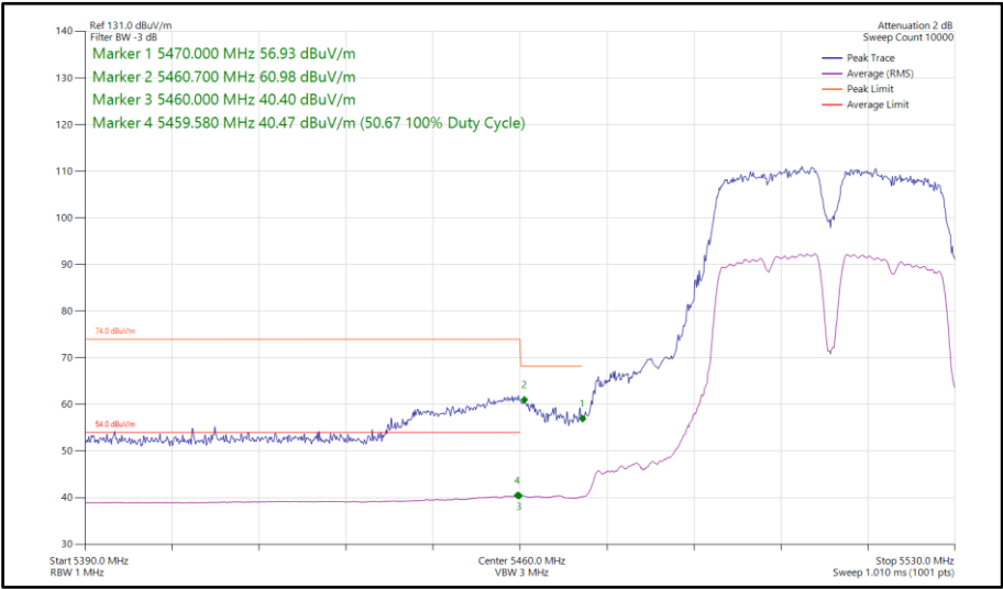
Figure 669 - 802.11a a40, SISO, Core 1 - 5510 MHz Band Edge Frequency 5470 MHz
