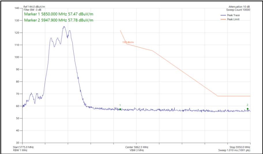
Figure 718 - 802.11be EHT40, RU 52+26-75, CDD, Core 0-1 - 5795 MHz Band Edge Frequency 5850 MHz
