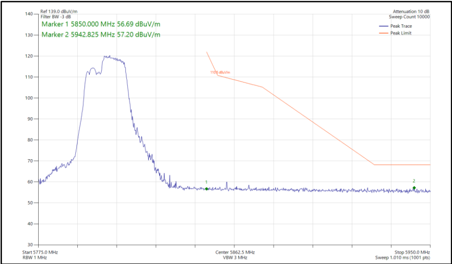
Figure 693 - 802.11be EHT40, RU 106+26-85, SISO, Core 1 - 5795 MHz Band Edge Frequency 5850 MHz
