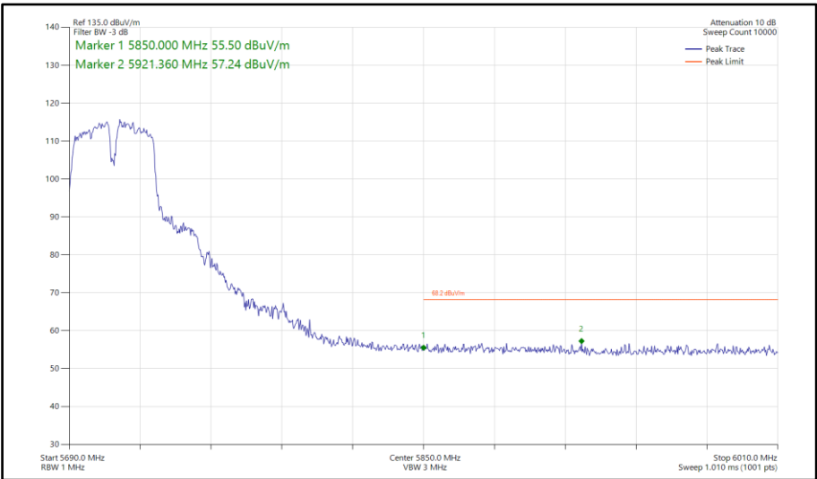
Figure 684 - 802.11a a40, SISO, Core 1 - 5710 MHz Band Edge Frequency 5850 MHz
