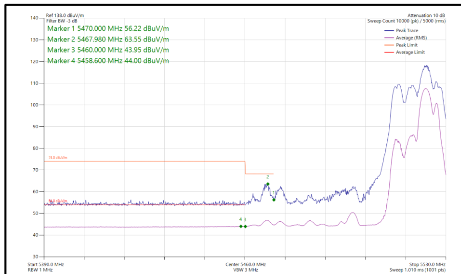
Figure 722 - 802.11be EHT40, RU 52+26-75, SDM, Core 0-1 - 5510 MHz Band Edge Frequency 5470 MHz
