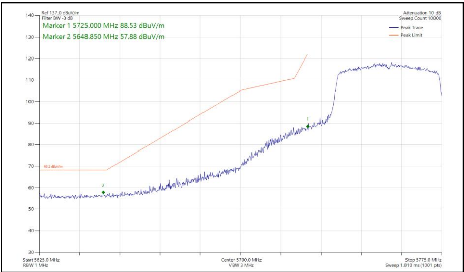
Figure 676 - 802.11ax HE40, SU, SISO, Core 1 - 5755 MHz Band Edge Frequency 5725 MHz
