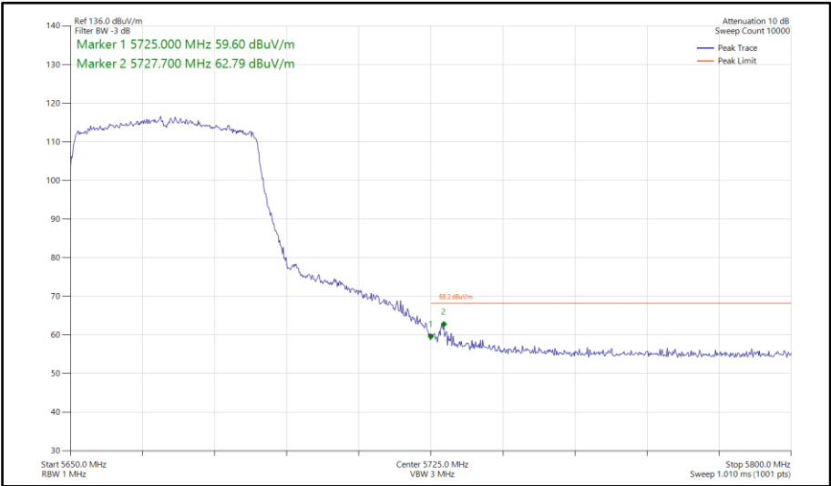
Figure 681 - 802.11ax HE40, SU, SISO, Core 1 - 5670 MHz Band Edge Frequency 5725 MHz
