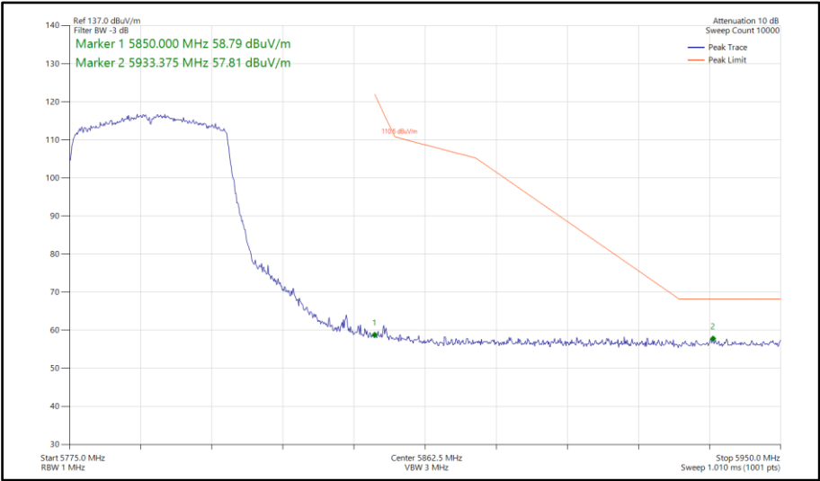
Figure 665 - 802.11ax HE40, SU, SISO, Core 0 - 5795 MHz Band Edge Frequency 5850 MHz
