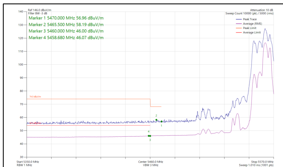
Figure 723 - 802.11be EHT40, RU 52+26-75, SDM, Core 0-1 - 5550 MHz Band Edge Frequency 5470 MHz
