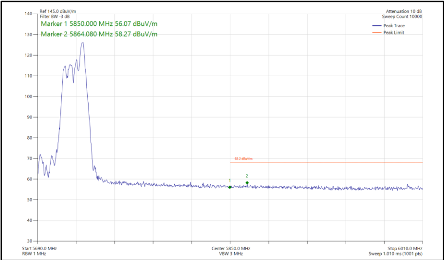
Figure 735 - 802.11ax HE40, RU 52-44, SDM, Core 0-1 - 5710 MHz Band Edge Frequency 5850 MHz
