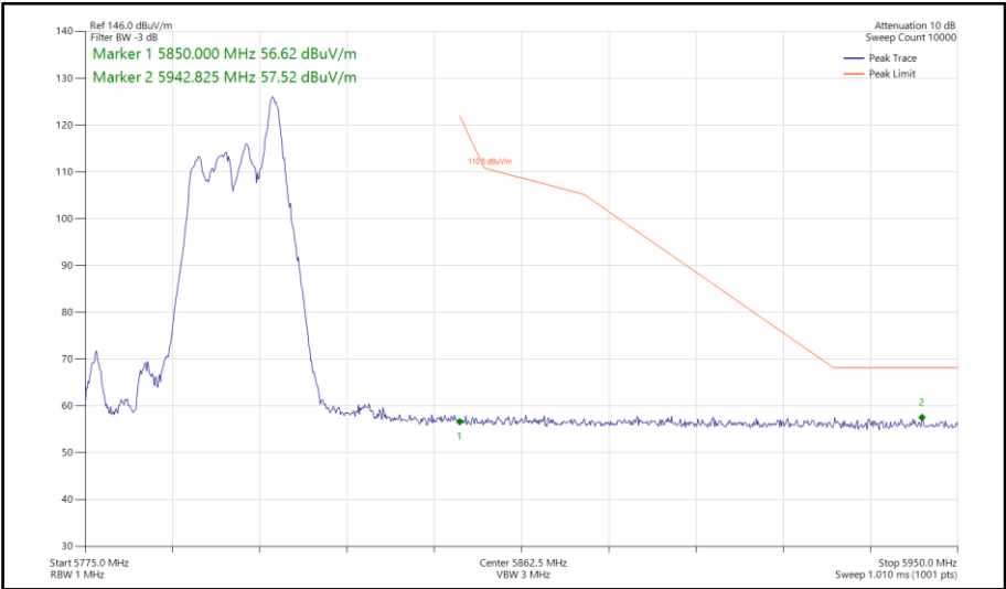
Figure 716 - 802.11ax HE40, RU 26-17, CDD, Core 0-1 - 5795 MHz Band Edge Frequency 5850 MHz
