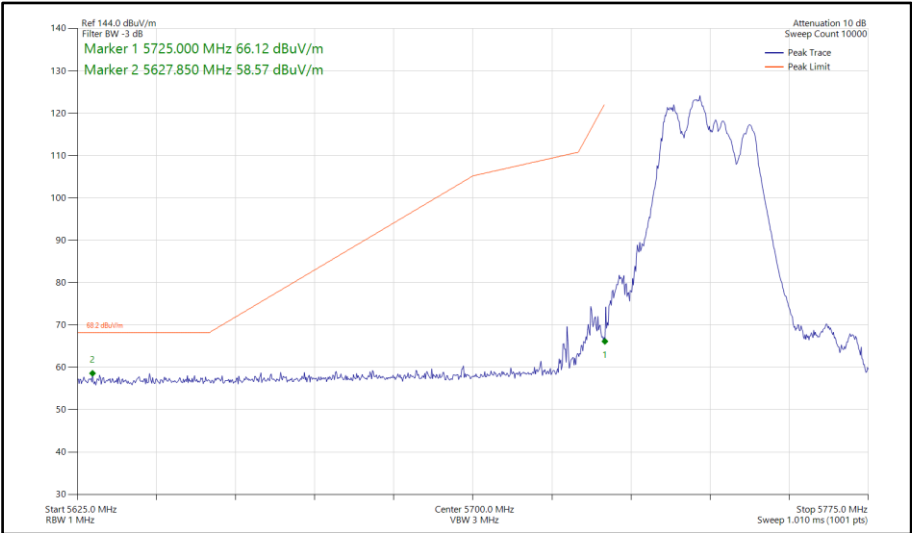
Figure 727 - 802.11be EHT40, RU 106+26-82, SDM, Core 0-1 - 5755 MHz Band Edge Frequency 5725 MHz
