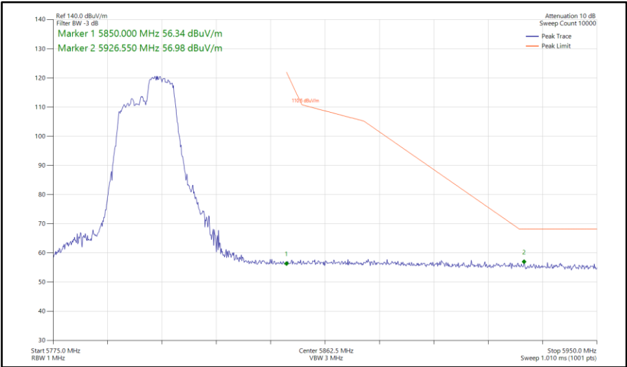
Figure 666 - 802.11ax HE40, RU 106-56, SISO, Core 0 - 5795 MHz Band Edge Frequency 5850 MHz
