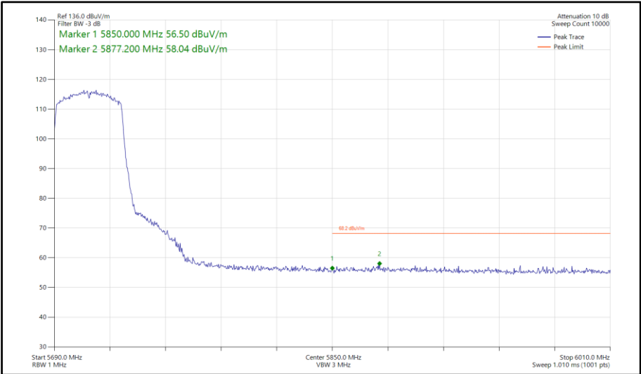
Figure 688 - 802.11ax HE40, SU, SISO, Core 1 - 5710 MHz Band Edge Frequency 5850 MHz
