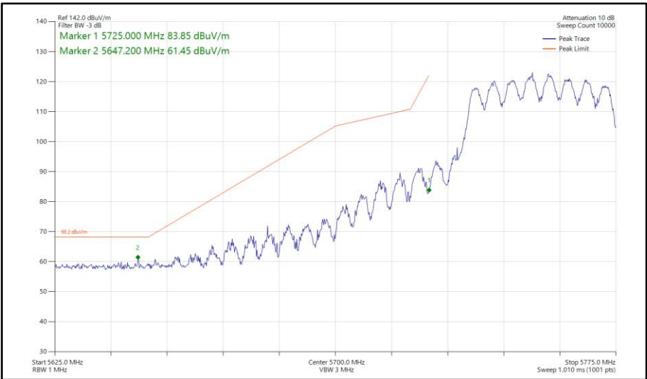
Figure 701 - 802.11ax HE40, SU, CDD, Core 0-1 - 5755 MHz Band Edge Frequency 5725 MHz
