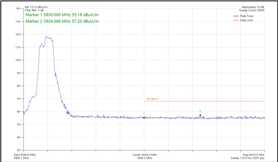
Figure 692 - 802.11be EHT40, RU 106+26-85, SISO, Core 1 - 5710 MHz Band Edge Frequency 5850 MHz
