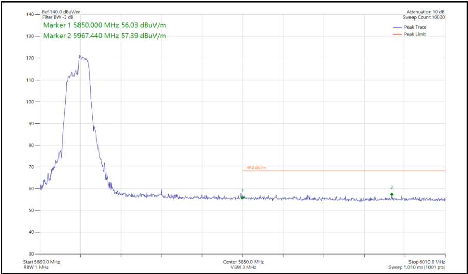
Figure 689 - 802.11ax HE40, RU 106-56, SISO, Core 1 - 5710 MHz Band Edge Frequency 5850 MHz
