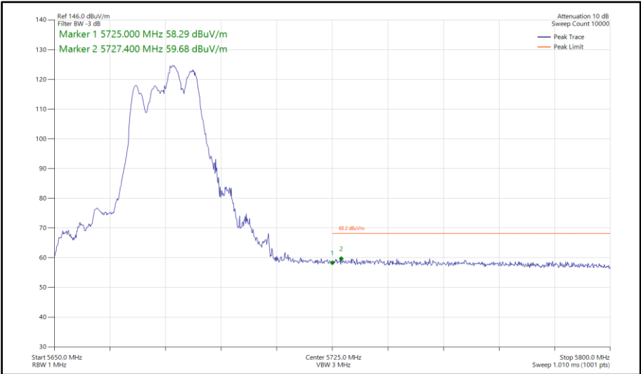
Figure 731 - 802.11be EHT40, RU 106+26-85, SDM, Core 0-1 - 5670 MHz Band Edge Frequency 5725 MHz
