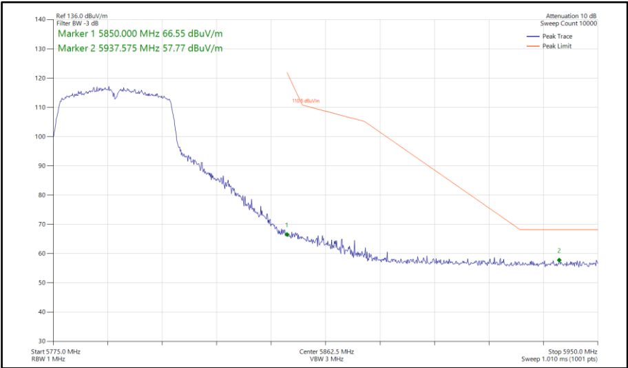
Figure 687 - 802.11n HT40, SISO, Core 1 - 5795 MHz Band Edge Frequency 5850 MHz
