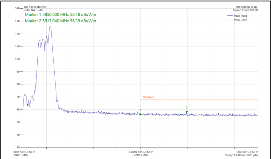
Figure 714 - 802.11ax HE40, RU 52-44, CDD, Core 0-1 - 5710 MHz Band Edge Frequency 5850 MHz
