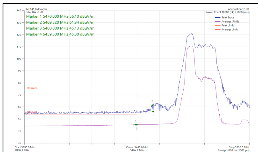
Figure 672 - 802.11ax HE40, RU 52-37, SISO, Core 1 - 5510 MHz Band Edge Frequency 5470 MHz
