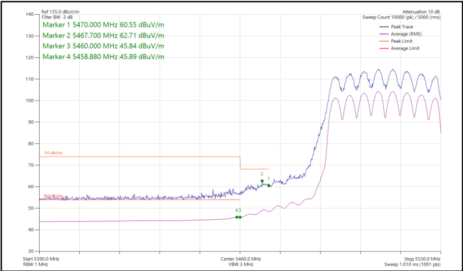
Figure 696 - 802.11ax HE40, SU, CDD, Core 0-1 - 5510 MHz Band Edge Frequency 5470 MHz
