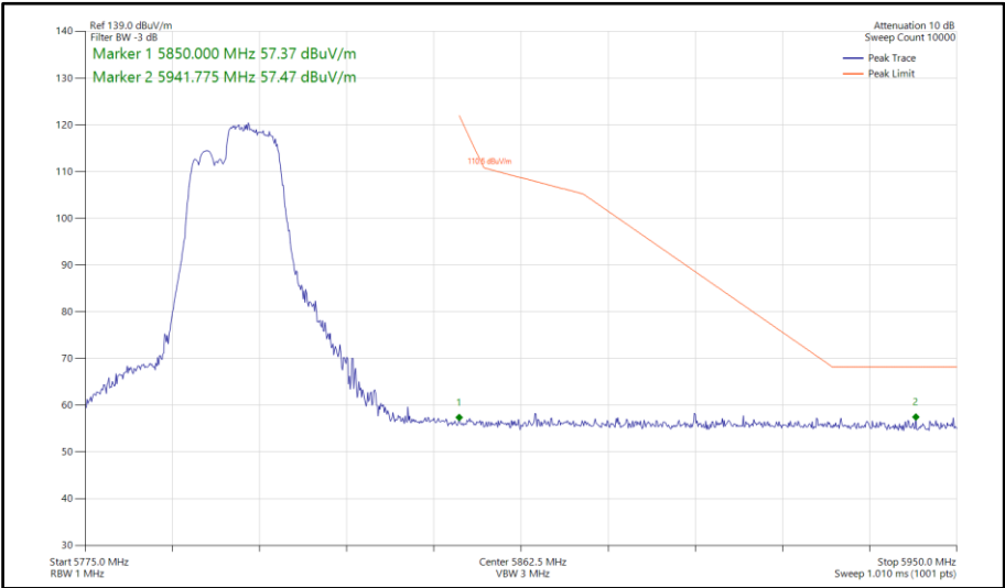
Figure 668 - 802.11be EHT40, RU 106+26-85, SISO, Core 0 - 5795 MHz Band Edge Frequency 5850 MHz
