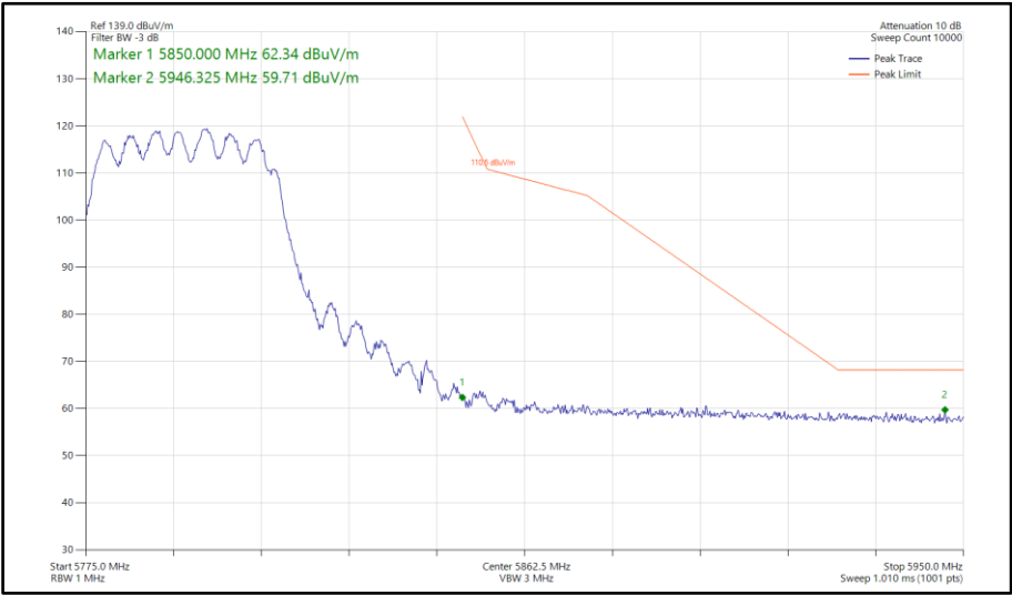
Figure 712 - 802.11n HT40, CDD, Core 0-1 - 5795 MHz Band Edge Frequency 5850 MHz
