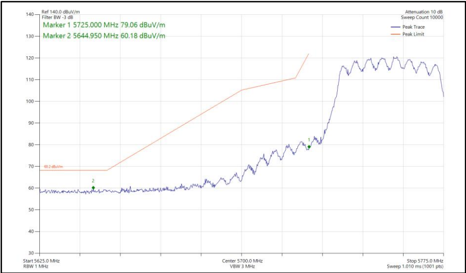
Figure 700 - 802.11n HT40, CDD, Core 0-1 - 5755 MHz Band Edge Frequency 5725 MHz
