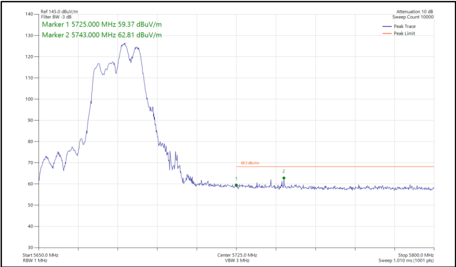
Figure 730 - 802.11ax HE40, RU 106-56, SDM, Core 0-1 - 5670 MHz Band Edge Frequency 5725 MHz
