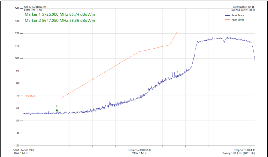
Figure 675 - 802.11n HT40, SISO, Core 1 - 5755 MHz Band Edge Frequency 5725 MHz
