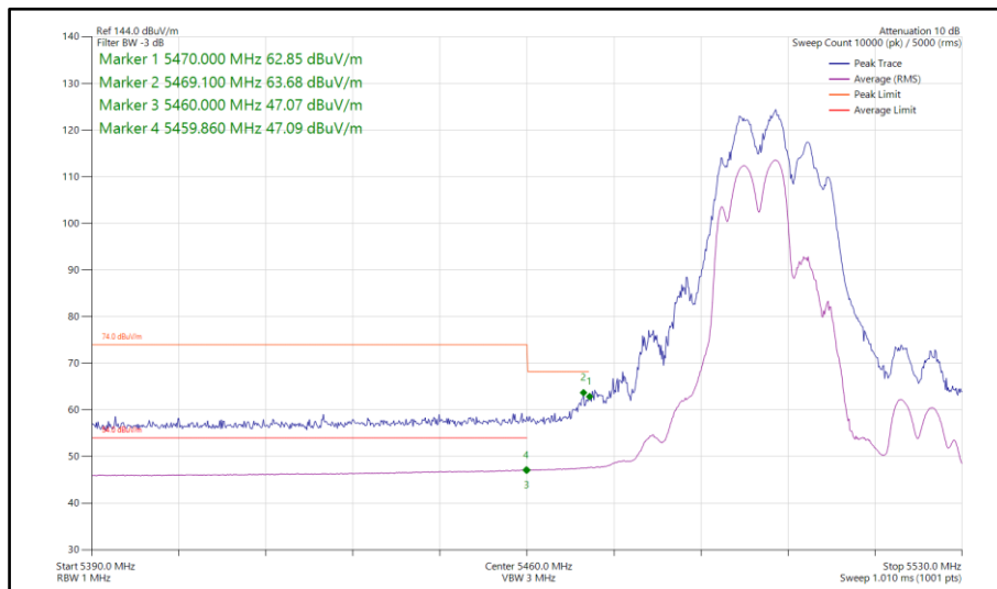
Figure 698 - 802.11be EHT40, RU 106+26-82, CDD, Core 0-1 - 5510 MHz Band Edge Frequency 5470 MHz
