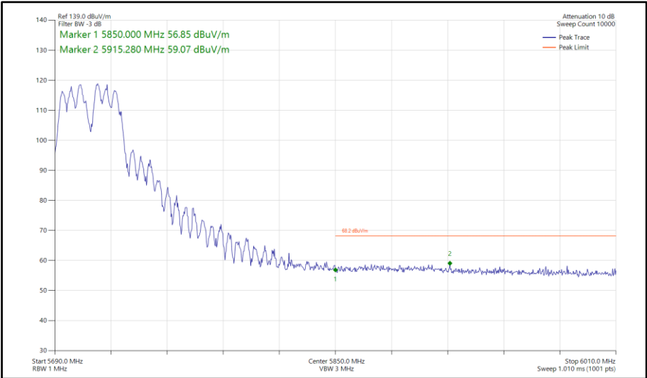
Figure 709 - 802.11a a40, CDD, Core 0-1 - 5710 MHz Band Edge Frequency 5850 MHz
