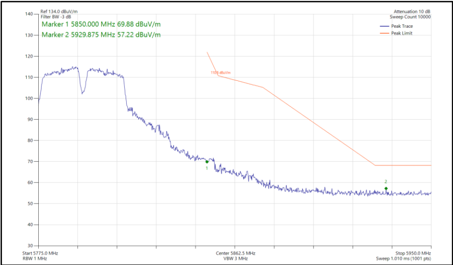
Figure 685 - 802.11a a40, SISO, Core 1 - 5795 MHz Band Edge Frequency 5850 MHz
