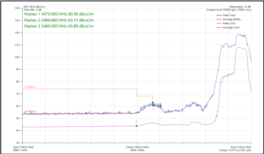
Figure 673 - 802.11be EHT40, RU 52+26-75, SISO, Core 1 - 5510 MHz Band Edge Frequency 5470 MHz
