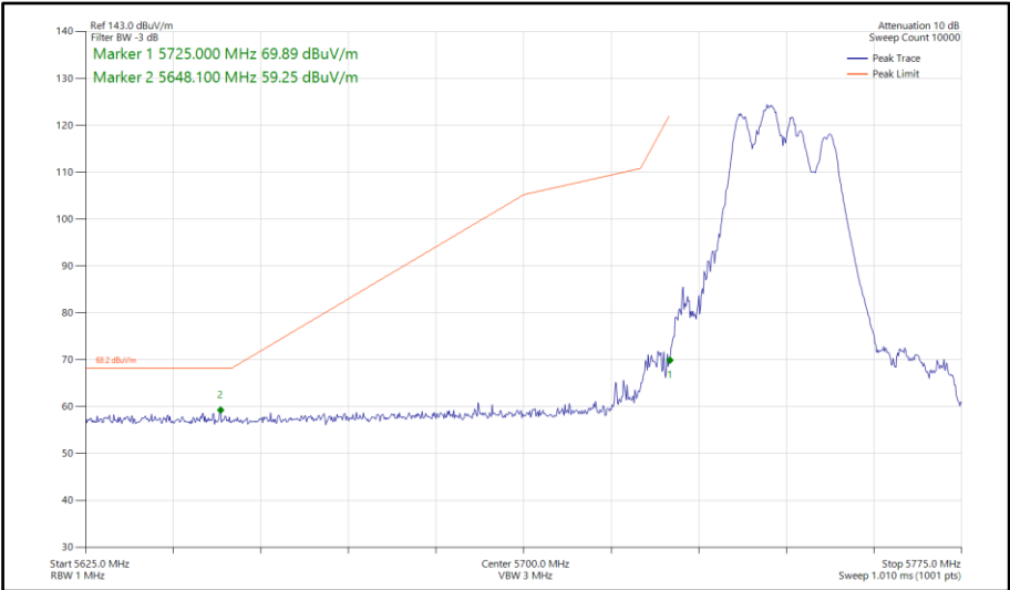
Figure 703 - 802.11be EHT40, RU 106+26-82, CDD, Core 0-1 - 5755 MHz Band Edge Frequency 5725 MHz
