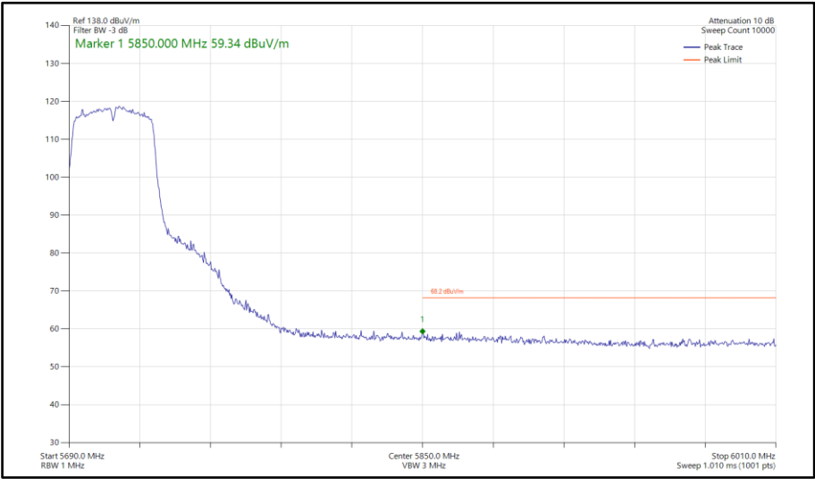
Figure 732 - 802.11n HT40, SDM, Core 0-1 - 5710 MHz Band Edge Frequency 5850 MHz
