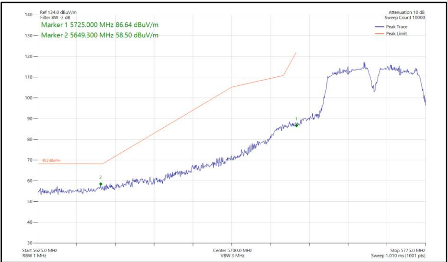
Figure 674 - 802.11a a40, SISO, Core 1 - 5755 MHz Band Edge Frequency 5725 MHz
