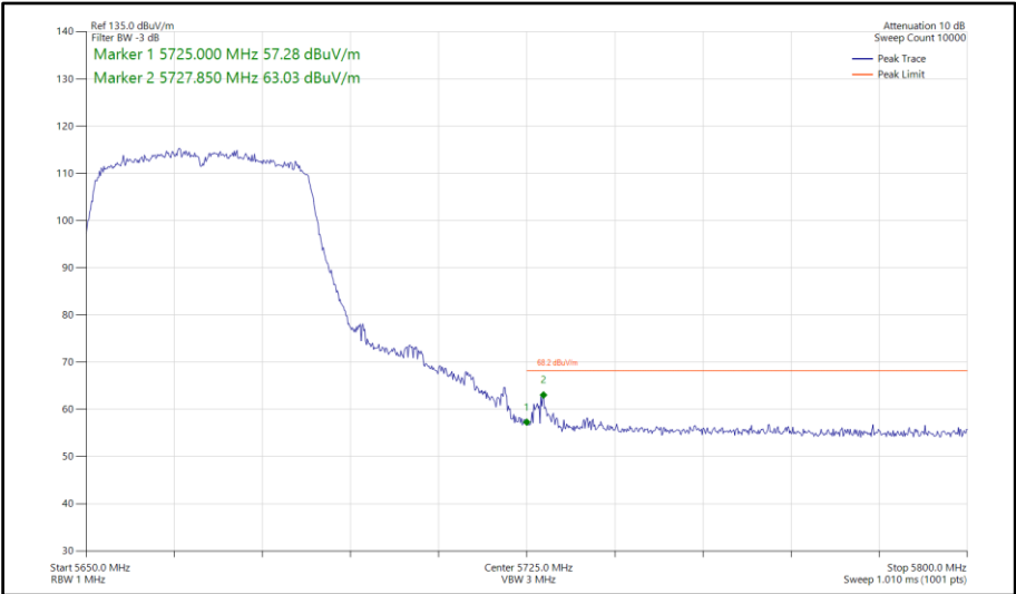
Figure 680 - 802.11n HT40, SISO, Core 1 - 5670 MHz Band Edge Frequency 5725 MHz
