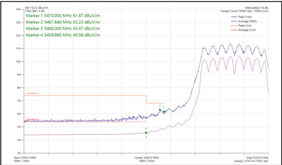
Figure 695 - 802.11n HT40, CDD, Core 0-1 - 5510 MHz Band Edge Frequency 5470 MHz
