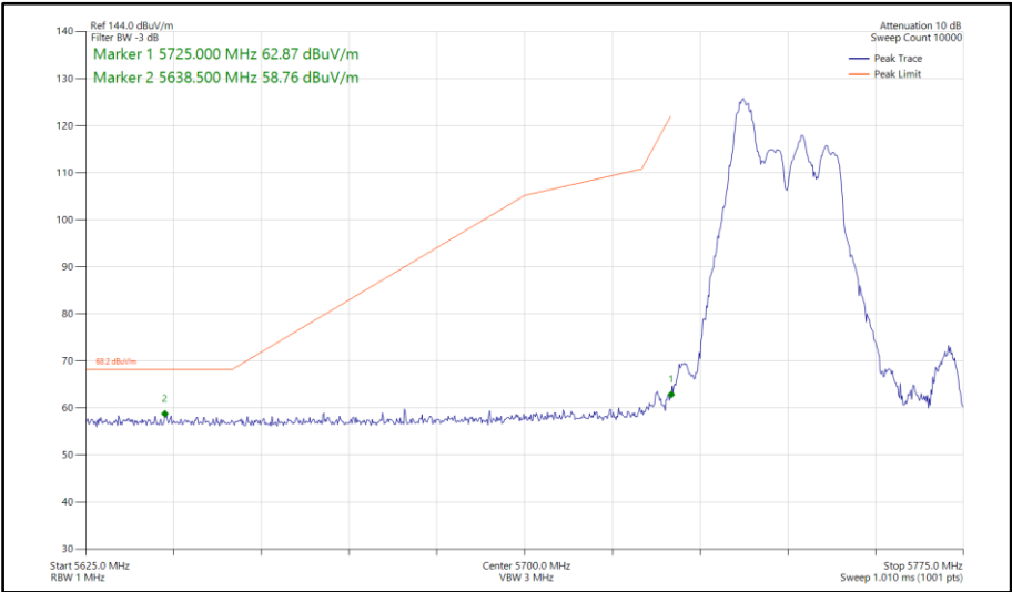
Figure 702 - 802.11ax HE40, RU 52-37, CDD, Core 0-1 - 5755 MHz Band Edge Frequency 5725 MHz
