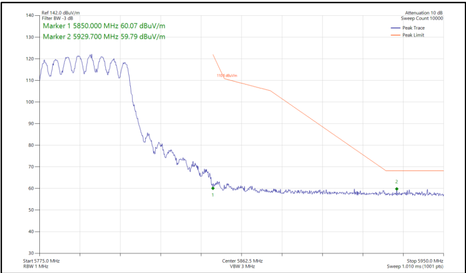
Figure 715 - 802.11ax HE40, SU, CDD, Core 0-1 - 5795 MHz Band Edge Frequency 5850 MHz
