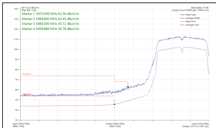
Figure 719 - 802.11n HT40, SDM, Core 0-1 - 5510 MHz Band Edge Frequency 5470 MHz
