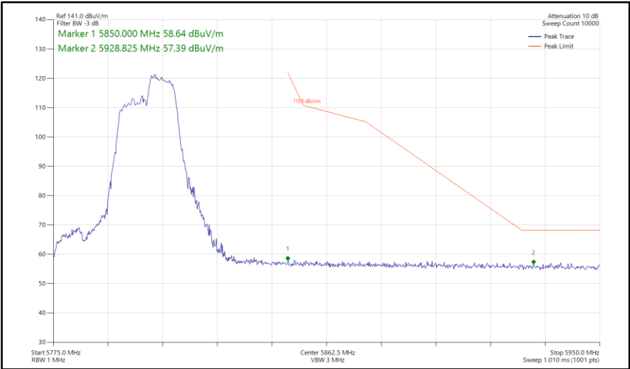
Figure 691 - 802.11ax HE40, RU 106-56, SISO, Core 1 - 5795 MHz Band Edge Frequency 5850 MHz
