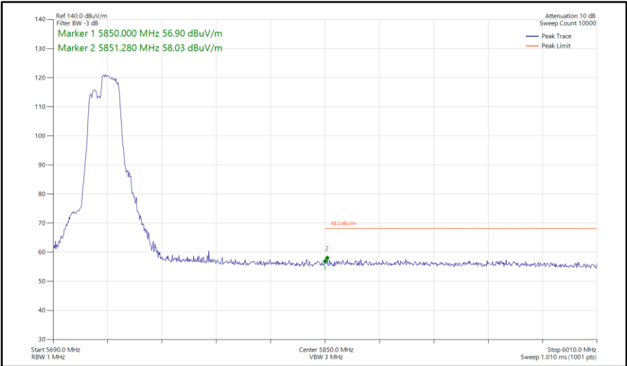
Figure 667 - 802.11be EHT40, RU 106+26-85, SISO, Core 0 - 5710 MHz Band Edge Frequency 5850 MHz
