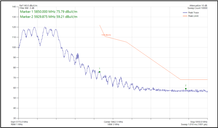
Figure 710 - 802.11a a40, CDD, Core 0-1 - 5795 MHz Band Edge Frequency 5850 MHz
