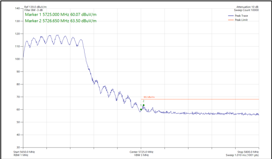
Figure 705 - 802.11n HT40, CDD, Core 0-1 - 5670 MHz Band Edge Frequency 5725 MHz
