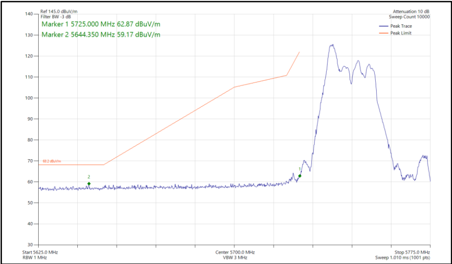
Figure 726 - 802.11ax HE40, RU 52-37, SDM, Core 0-1 - 5755 MHz Band Edge Frequency 5725 MHz
