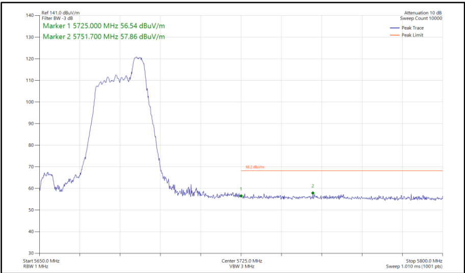
Figure 682 - 802.11ax HE40, RU 52-44, SISO, Core 1 - 5670 MHz Band Edge Frequency 5725 MHz
