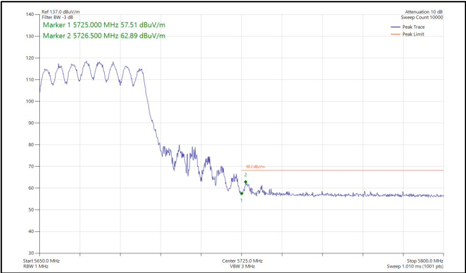
Figure 706 - 802.11ax HE40, SU, CDD, Core 0-1 - 5670 MHz Band Edge Frequency 5725 MHz
