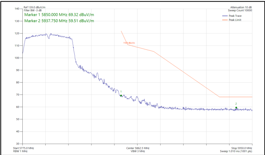
Figure 733 - 802.11n HT40, SDM, Core 0-1 - 5795 MHz Band Edge Frequency 5850 MHz
