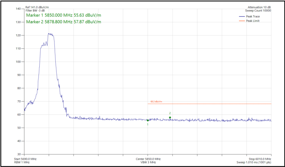
Figure 664 - 802.11ax HE40, RU 106-56, SISO, Core 0 - 5710 MHz Band Edge Frequency 5850 MHz
