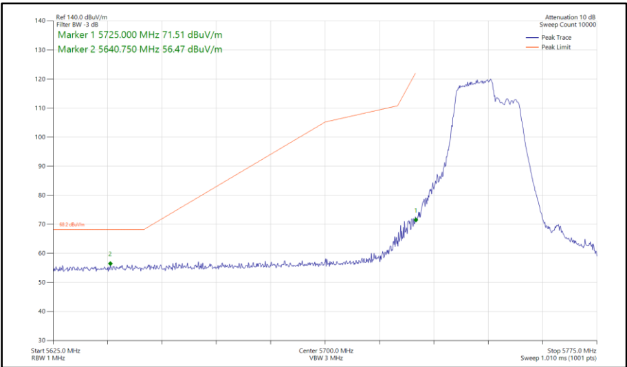
Figure 678 - 802.11be EHT40, RU 106+26-82, SISO, Core 1 - 5755 MHz Band Edge Frequency 5725 MHz
