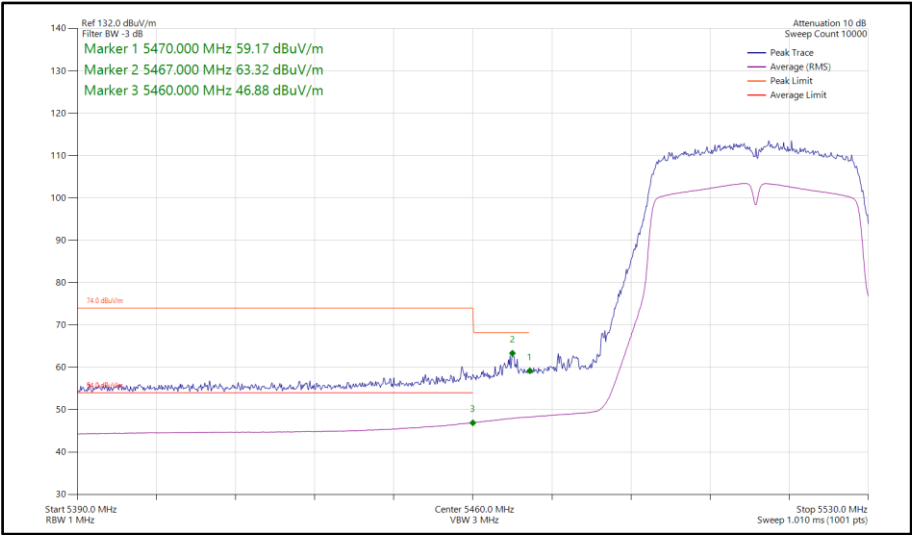
Figure 670 - 802.11n HT40, SISO, Core 1 - 5510 MHz Band Edge Frequency 5470 MHz
