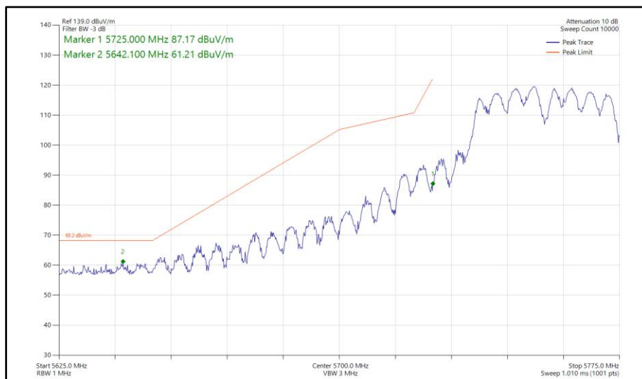
Figure 699 - 802.11a a40, CDD, Core 0-1 - 5755 MHz Band Edge Frequency 5725 MHz
