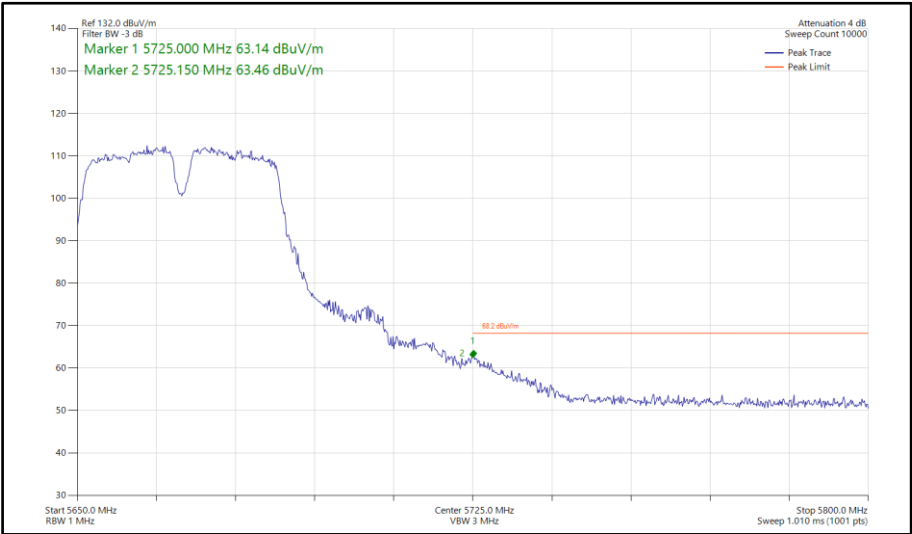
Figure 679 - 802.11a a40, SISO, Core 1 - 5670 MHz Band Edge Frequency 5725 MHz
