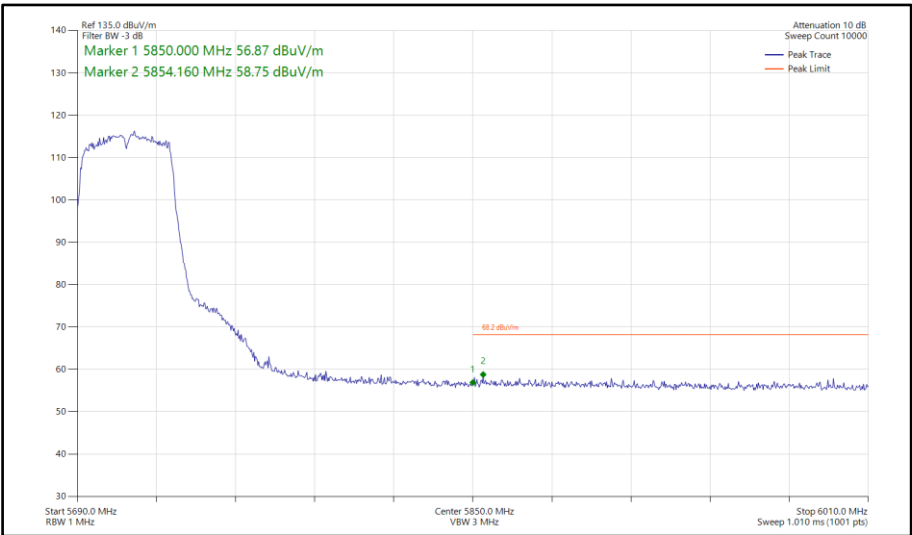
Figure 686 - 802.11n HT40, SISO, Core 1 - 5710 MHz Band Edge Frequency 5850 MHz
