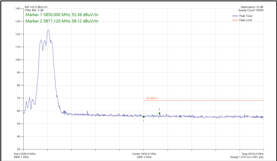
Figure 717 - 802.11be EHT40, RU 52+26-75, CDD, Core 0-1 - 5710 MHz Band Edge Frequency 5850 MHz
