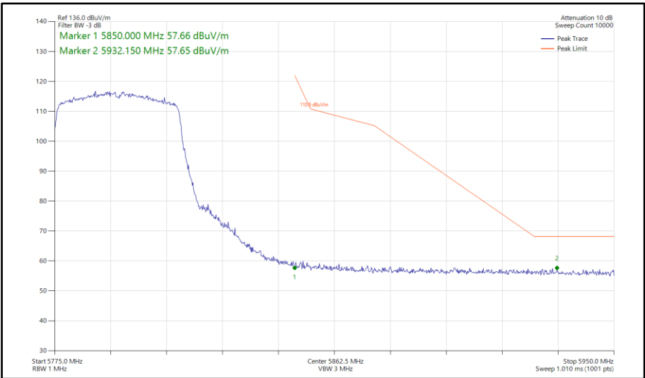
Figure 690 - 802.11ax HE40, SU, SISO, Core 1 - 5795 MHz Band Edge Frequency 5850 MHz
