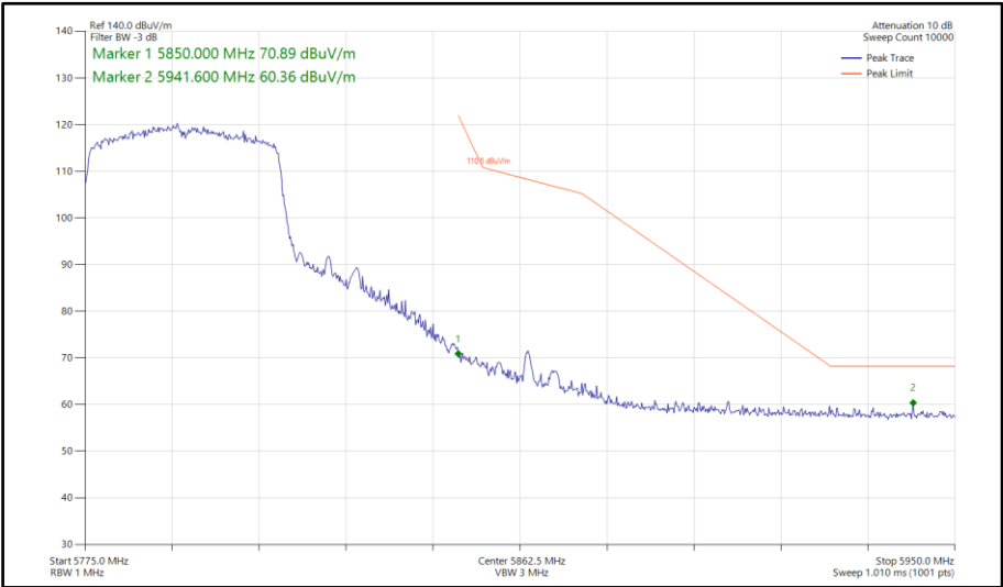
Figure 736 - 802.11ax HE40, SU, SDM, Core 0-1 - 5795 MHz Band Edge Frequency 5850 MHz
