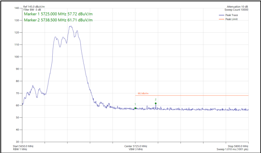
Figure 708 - 802.11be EHT40, RU52+26-75, CDD, Core 0-1 - 5670 MHz Band Edge Frequency 5725 MHz
