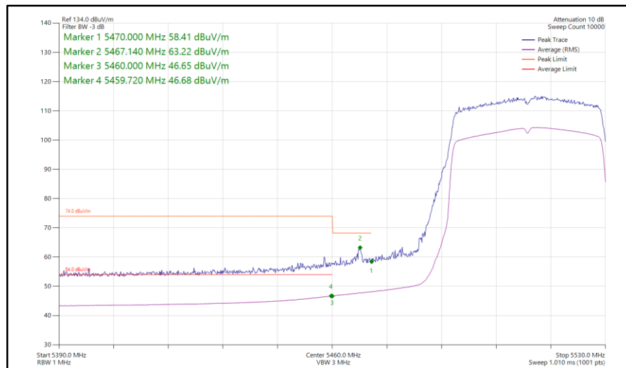
Figure 671 - 802.11ax HE40, SU, SISO, Core 1 - 5510 MHz Band Edge Frequency 5470 MHz
