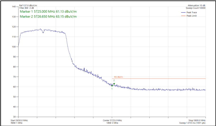
Figure 728 - 802.11n HT40, SDM, Core 0-1 - 5670 MHz Band Edge Frequency 5725 MHz
