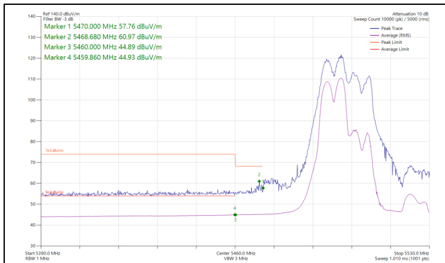
Figure 721 - 802.11ax HE40, RU 106-53, SDM, Core 0-1 - 5510 MHz Band Edge Frequency 5470 MHz
