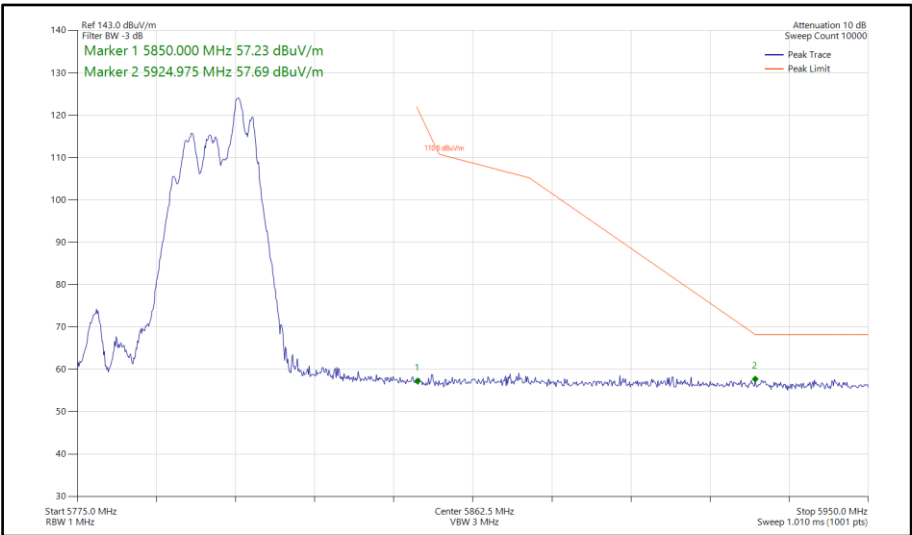
Figure 737 - 802.11ax HE40, RU 52-44, SDM, Core 0-1 - 5795 MHz Band Edge Frequency 5850 MHz
