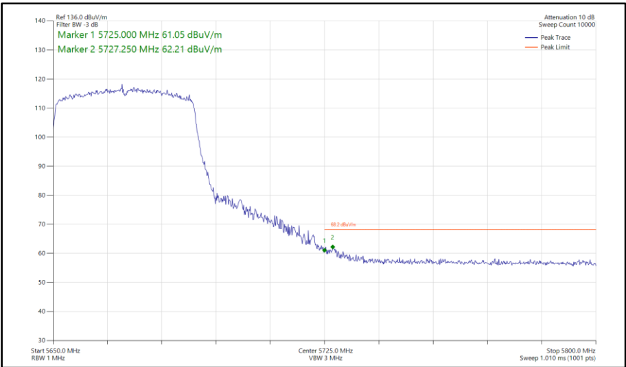
Figure 729 - 802.11ax HE40, SU, SDM, Core 0-1 - 5670 MHz Band Edge Frequency 5725 MHz
