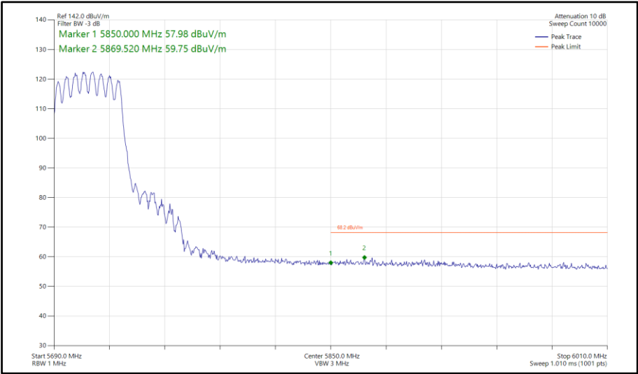
Figure 713 - 802.11ax HE40, SU, CDD, Core 0-1 - 5710 MHz Band Edge Frequency 5850 MHz
