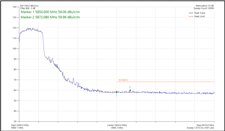
Figure 734 - 802.11ax HE40, SU, SDM, Core 0-1 - 5710 MHz Band Edge Frequency 5850 MHz
