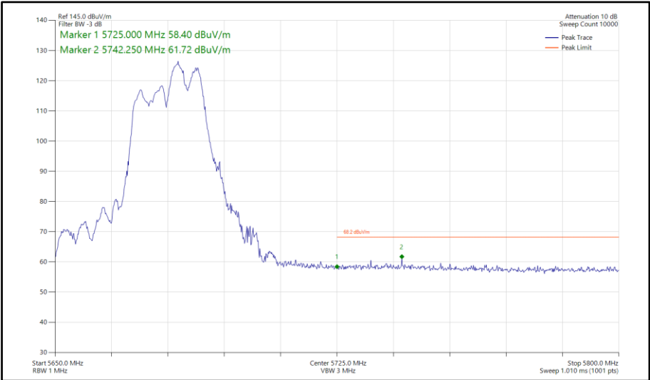
Figure 707 - 802.11ax HE40, RU 106-56, CDD, Core 0-1 - 5670 MHz Band Edge Frequency 5725 MHz
