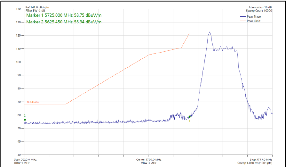
Figure 677 - 802.11ax HE40, RU 26-0, SISO, Core 1 - 5755 MHz Band Edge Frequency 5725 MHz
