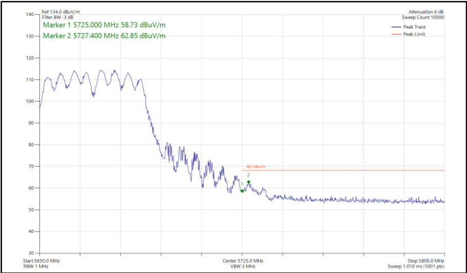
Figure 704 - 802.11a a40, CDD, Core 0-1 - 5670 MHz Band Edge Frequency 5725 MHz
