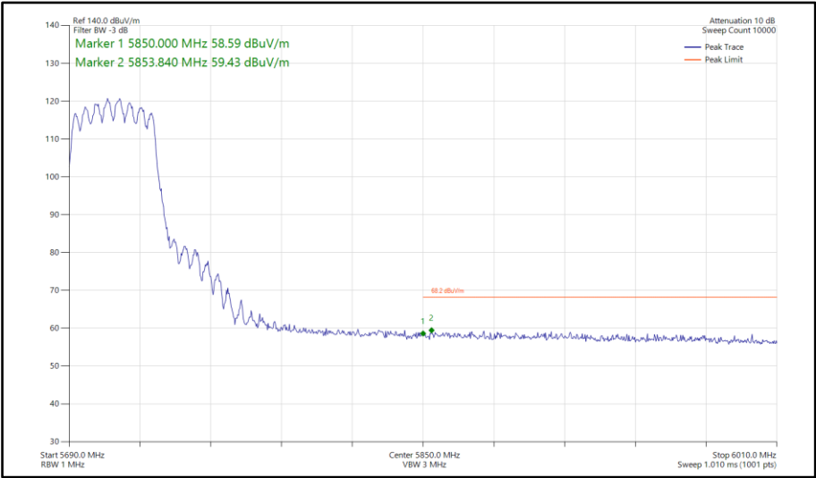
Figure 711 - 802.11n HT40, CDD, Core 0-1 - 5710 MHz Band Edge Frequency 5850 MHz
