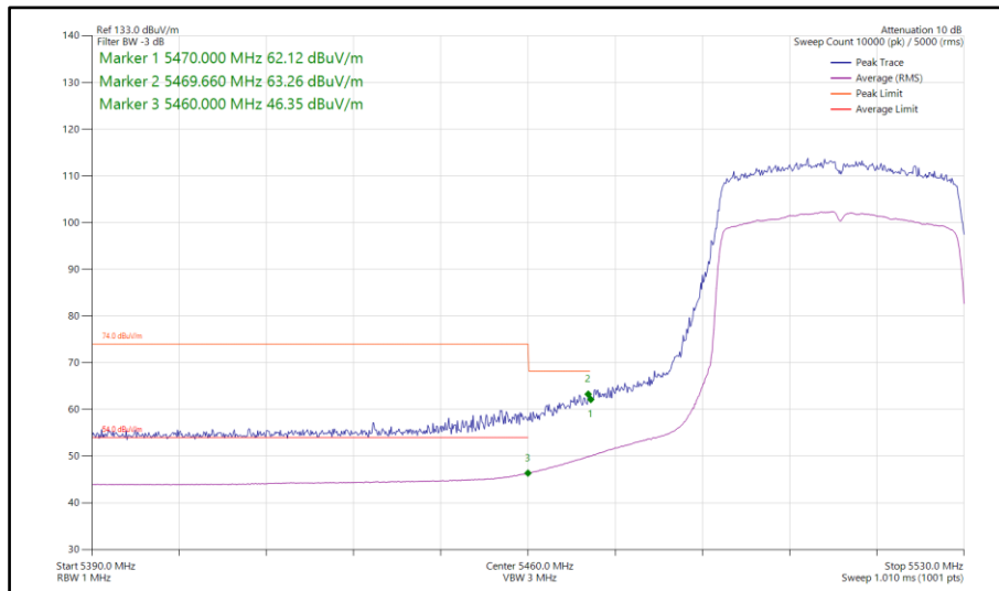
Figure 720 - 802.11ax HE40, SU, SDM, Core 0-1 - 5510 MHz Band Edge Frequency 5470 MHz
