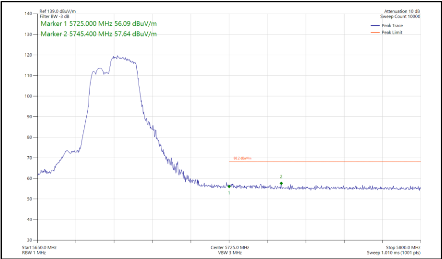
Figure 683 - 802.11be EHT40, RU 106+26-85, SISO, Core 1 - 5670 MHz Band Edge Frequency 5725 MHz
