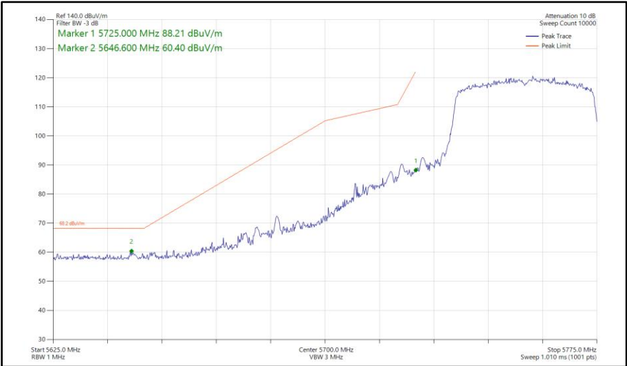
Figure 725 - 802.11ax HE40, SU, SDM, Core 0-1 - 5755 MHz Band Edge Frequency 5725 MHz
