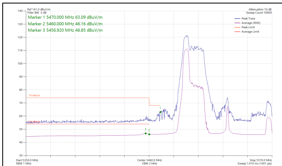
Figure 753 - 802.11ax HE80, RU 52-37, SISO, Core 0 - 5530 MHz Band Edge Frequency 5470 MHz
