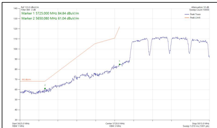
Figure 780 - 802.11a a80, SISO, Core 1 - 5775 MHz Band Edge Frequency 5725 MHz
