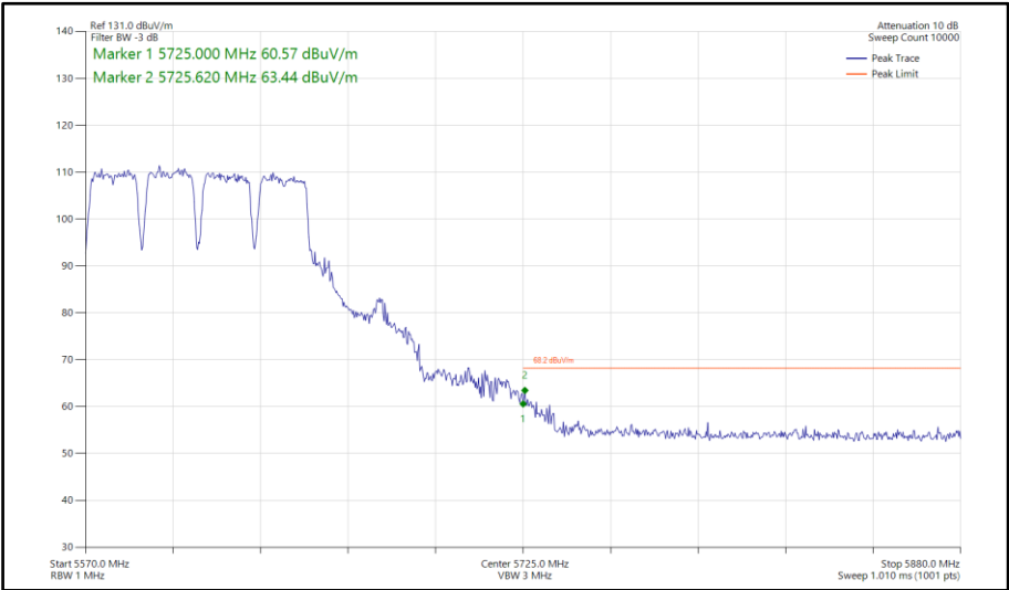
Figure 760 - 802.11a a80, SISO, Core 0 - 5610 MHz Band Edge Frequency 5725 MHz
