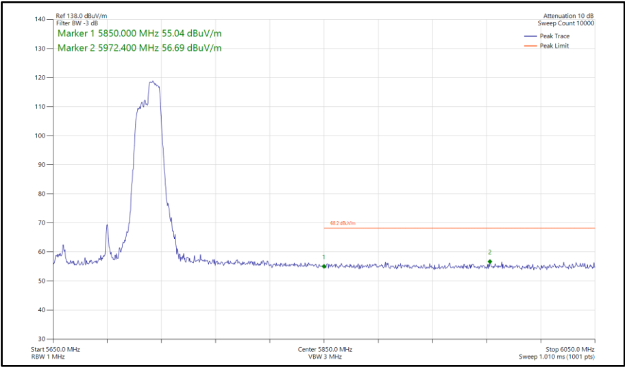
Figure 795 - 802.11ax HE80, RU 106-60, SISO, Core 1 - 5690 MHz Band Edge Frequency 5850 MHz
