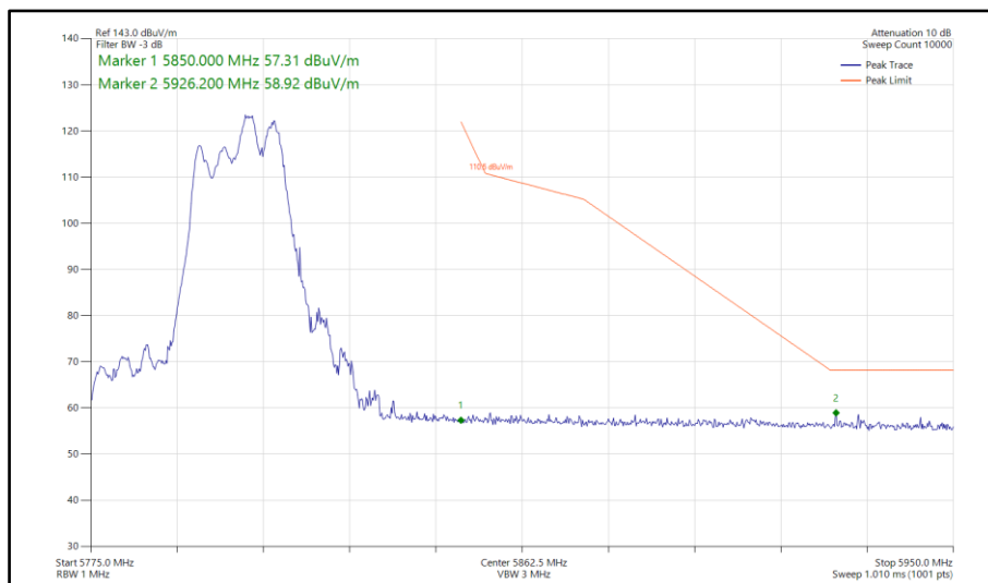
Figure 739 - 802.11be EHT40, RU 106+26-85, SDM, Core 0-1 - 5795 MHz Band Edge Frequency 5850 MHz
