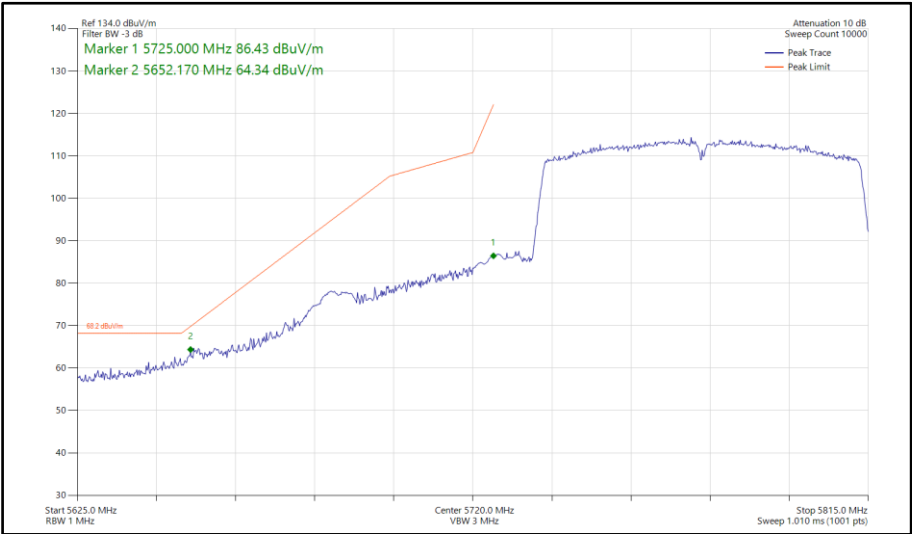
Figure 781 - 802.11ac VHT80, SISO, Core 1 - 5775 MHz Band Edge Frequency 5725 MHz
