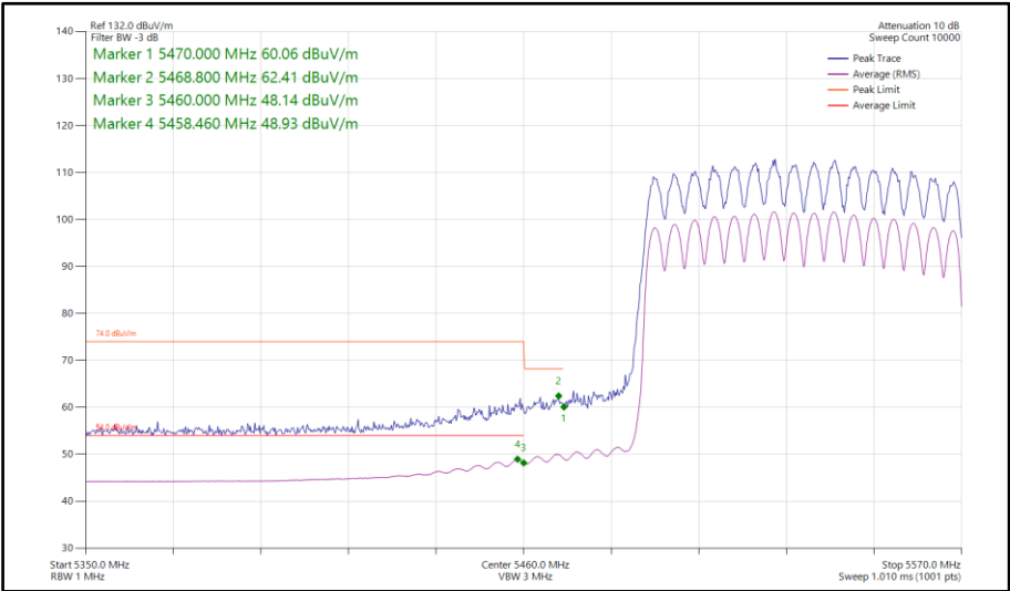
Figure 802 - 802.11ax HE80, SU, CDD, Core 0-1 - 5530 MHz Band Edge Frequency 5470 MHz
