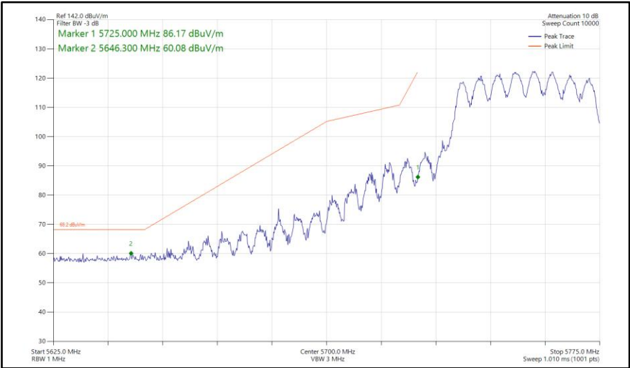
Figure 743 - 802.11ax HE40, SU, TxBF, Core 0-1 - 5755 MHz Band Edge Frequency 5725 MHz
