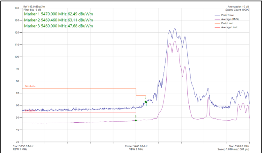
Figure 804 - 802.11be EHT80, RU 106+26-82, CDD, Core 0-1 - 5530 MHz Band Edge Frequency 5470 MHz
