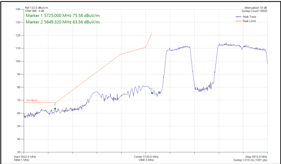
Figure 759 - 802.11be EHT80, RU 484+242-91, SISO, Core 0 - 5775 MHz Band Edge Frequency 5725 MHz
