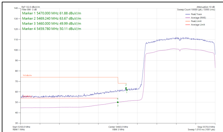
Figure 752 - 802.11ax HE80, SU, SISO, Core 0 - 5530 MHz Band Edge Frequency 5470 MHz
