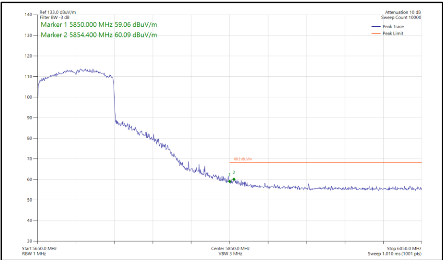
Figure 794 - 802.11ax HE80, SU, SISO, Core 1 - 5690 MHz Band Edge Frequency 5850 MHz
