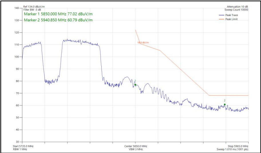
Figure 774 - 802.11be EHT80, RU 484+242-91, SISO, Core 0 - 5775 MHz Band Edge Frequency 5850 MHz
