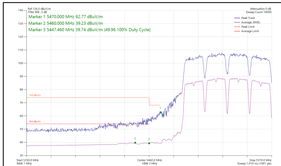
Figure 775 - 802.11a a80, SISO, Core 1 - 5530 MHz Band Edge Frequency 5470 MHz
