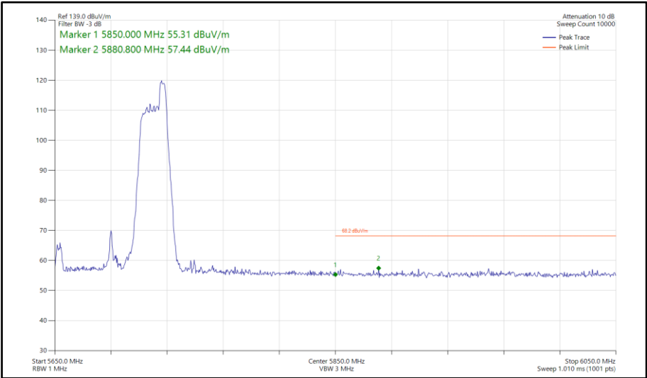
Figure 770 - 802.11ax HE80, RU 52-52, SISO, Core 0 - 5690 MHz Band Edge Frequency 5850 MHz
