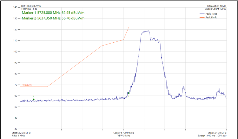
Figure 783 - 802.11ax HE80, RU 106-53, SISO, Core 1 - 5775 MHz Band Edge Frequency 5725 MHz
