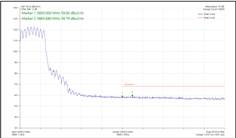
Figure 748 - 802.11ax HE40, SU, TxBF, Core 0-1 - 5710 MHz Band Edge Frequency 5850 MHz
