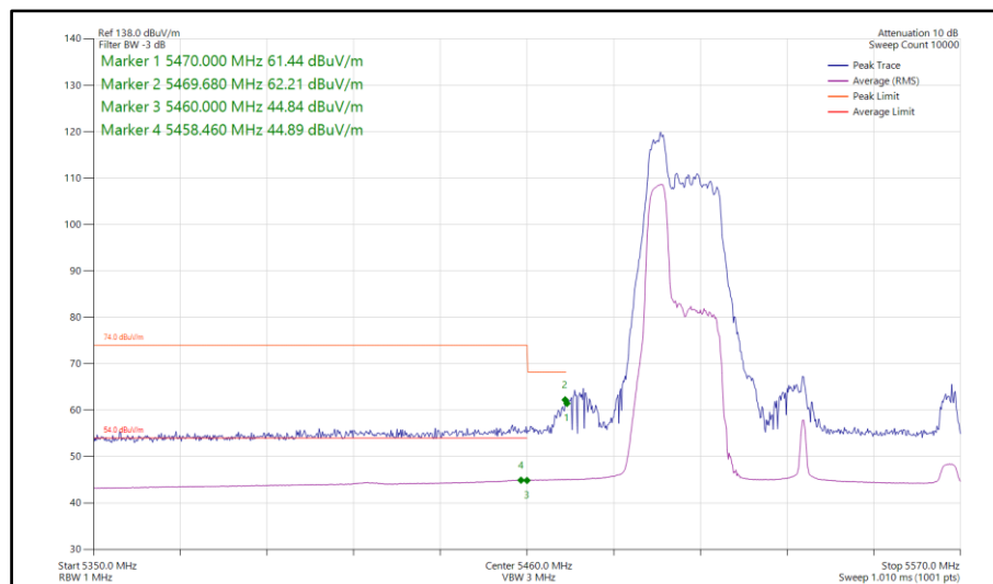
Figure 778 - 802.11ax HE80, RU 52-37, SISO, Core 1 - 5530 MHz Band Edge Frequency 5470 MHz
