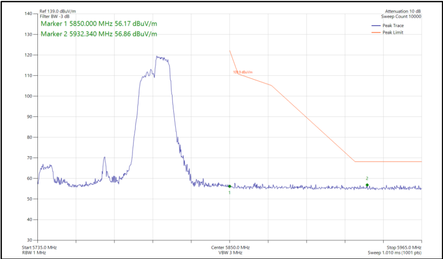
Figure 772 - 802.11ax HE80, RU 106-60, SISO, Core 0 - 5775 MHz Band Edge Frequency 5850 MHz
