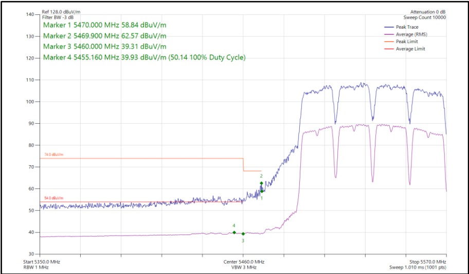
Figure 750 - 802.11a a80, SISO, Core 0 - 5530 MHz Band Edge Frequency 5470 MHz
