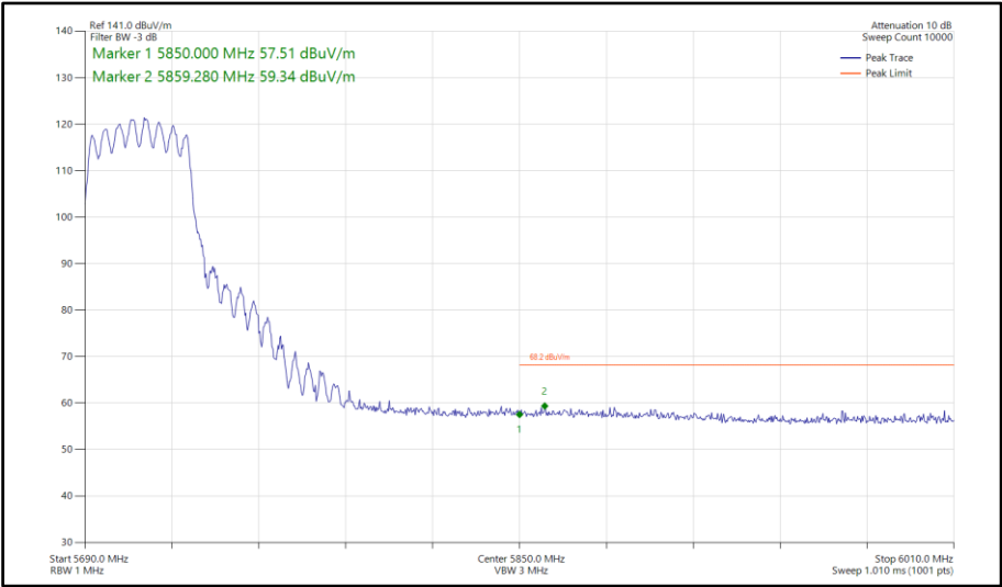
Figure 746 - 802.11ac VHT40, TxBF, Core 0-1 - 5710 MHz Band Edge Frequency 5850 MHz
