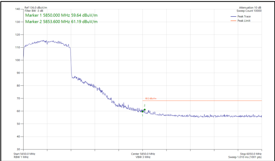
Figure 769 - 802.11ax HE80, SU, SISO, Core 0 - 5690 MHz Band Edge Frequency 5850 MHz
