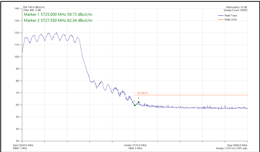
Figure 744 - 802.11ac VHT40, TxBF, Core 0-1 - 5670 MHz Band Edge Frequency 5725 MHz
