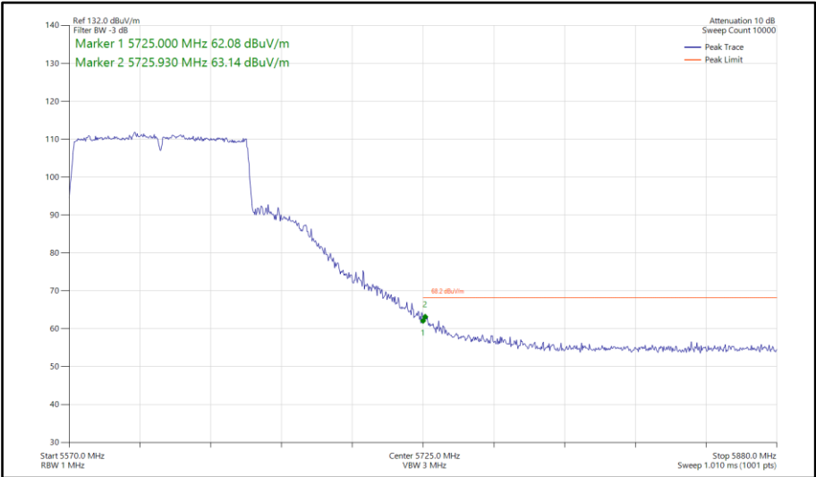
Figure 786 - 802.11ac VHT80, SISO, Core 1 - 5610 MHz Band Edge Frequency 5725 MHz
