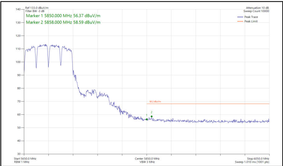
Figure 765 - 802.11a a80, SISO, Core 0 - 5690 MHz Band Edge Frequency 5850 MHz
