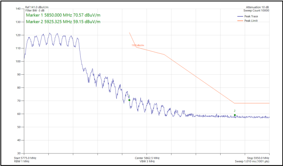
Figure 749 - 802.11ax HE40, SU, TxBF, Core 0-1 - 5795 MHz Band Edge Frequency 5850 MHz
