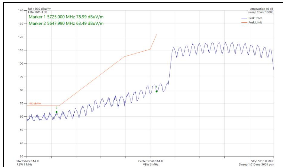
Figure 806 - 802.11ac VHT80, CDD, Core 0-1 - 5775 MHz Band Edge Frequency 5725 MHz
