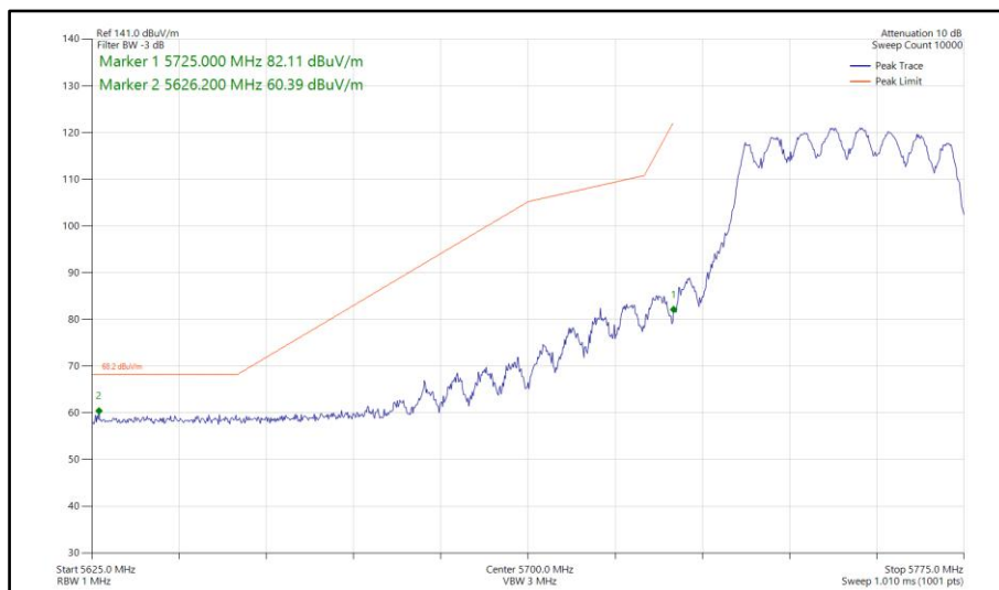
Figure 742 - 802.11ac VHT40, TxBF, Core 0-1 - 5755 MHz Band Edge Frequency 5725 MHz
