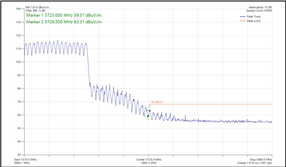
Figure 812 - 802.11ax HE80, SU, CDD, Core 0-1 - 5610 MHz Band Edge Frequency 5725 MHz
