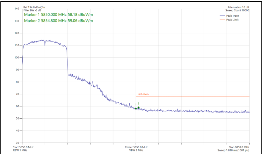
Figure 767 - 802.11ac VHT80, SISO, Core 0 - 5690 MHz Band Edge Frequency 5850 MHz
