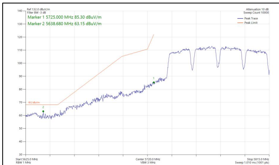
Figure 755 - 802.11a a80, SISO, Core 0 - 5775 MHz Band Edge Frequency 5725 MHz
