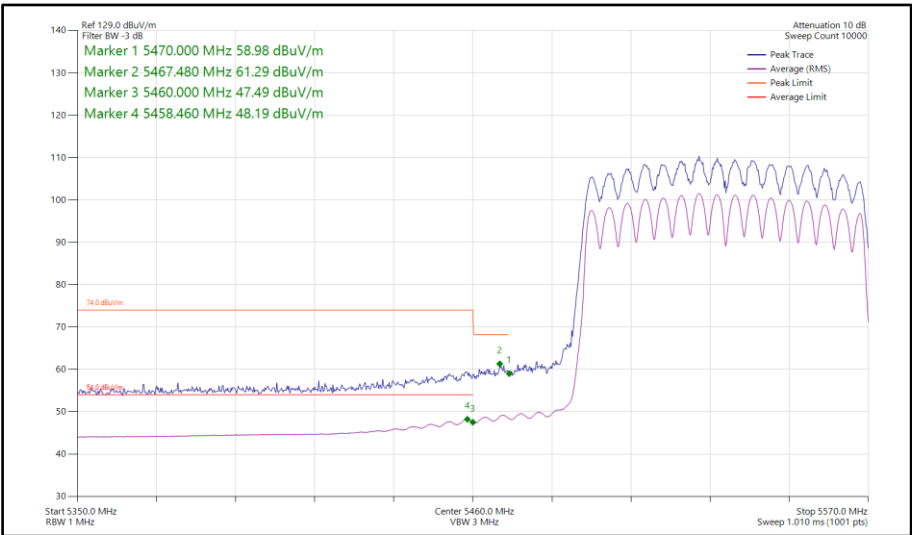
Figure 801 - 802.11ac VHT80, CDD, Core 0-1 - 5530 MHz Band Edge Frequency 5470 MHz
