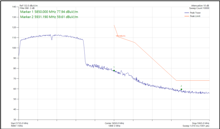
Figure 768 - 802.11ac VHT80, SISO, Core 0 - 5775 MHz Band Edge Frequency 5850 MHz
