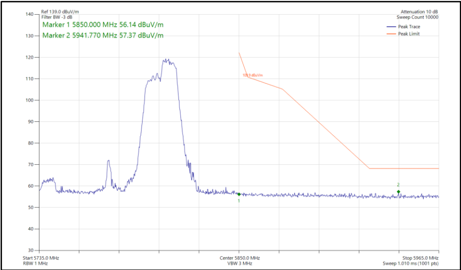
Figure 797 - 802.11ax HE80, RU 106-60, SISO, Core 1 - 5775 MHz Band Edge Frequency 5850 MHz
