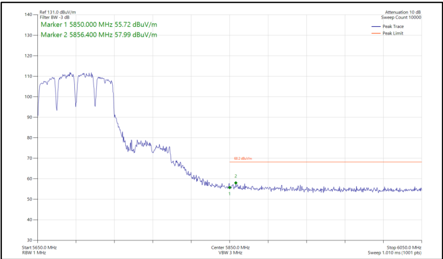
Figure 790 - 802.11a a80, SISO, Core 1 - 5690 MHz Band Edge Frequency 5850 MHz
