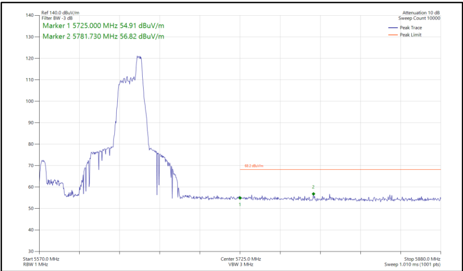
Figure 763 - 802.11ax HE80, RU 52-52, SISO, Core 0 - 5610 MHz Band Edge Frequency 5725 MHz
