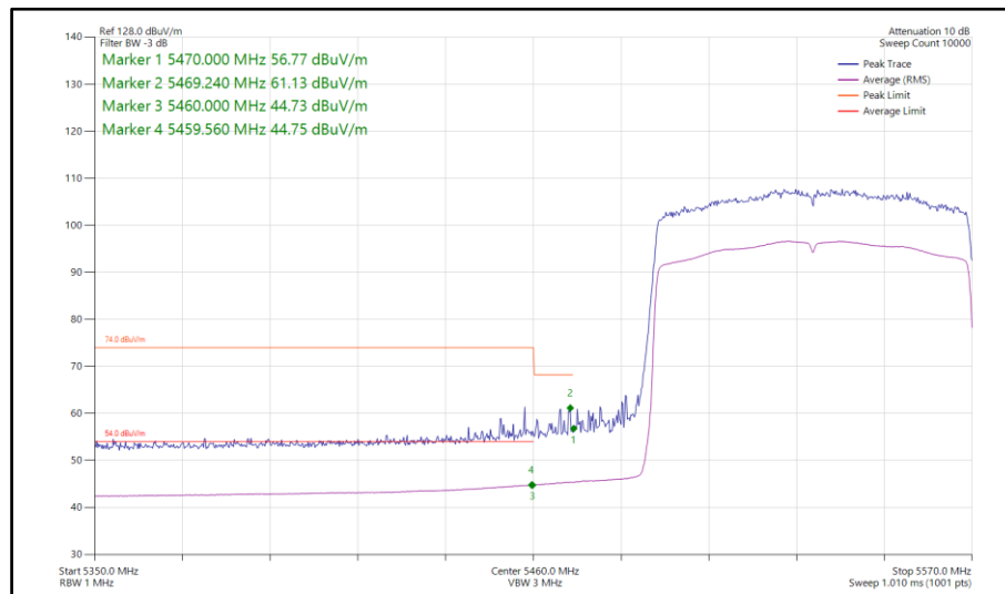
Figure 777 - 802.11ax HE80, SU, SISO, Core 1 - 5530 MHz Band Edge Frequency 5470 MHz
