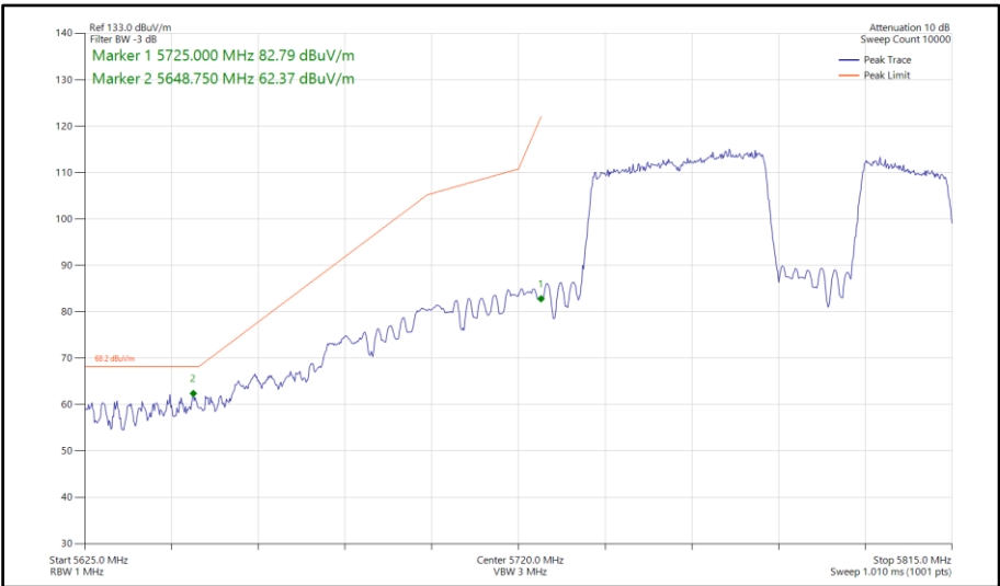
Figure 784 - 802.11be EHT80, RU 484+242-92, SISO, Core 1 - 5775 MHz Band Edge Frequency 5725 MHz
