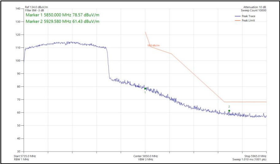
Figure 796 - 802.11ax HE80, SU, SISO, Core 1 - 5775 MHz Band Edge Frequency 5850 MHz
