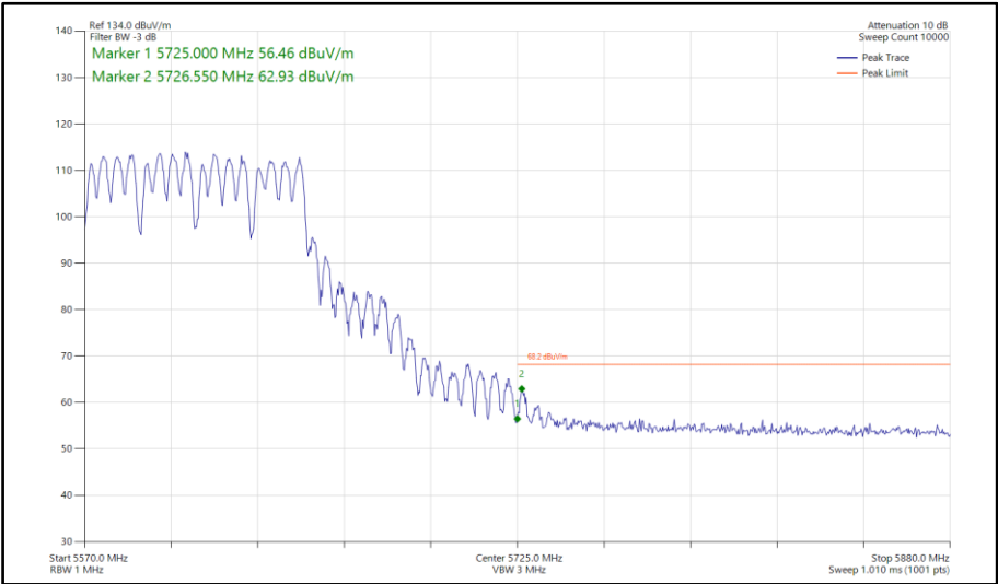
Figure 810 - 802.11a a80, CDD, Core 0-1 - 5610 MHz Band Edge Frequency 5725 MHz
