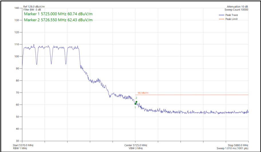
Figure 785 - 802.11a a80, SISO, Core 1 - 5610 MHz Band Edge Frequency 5725 MHz
