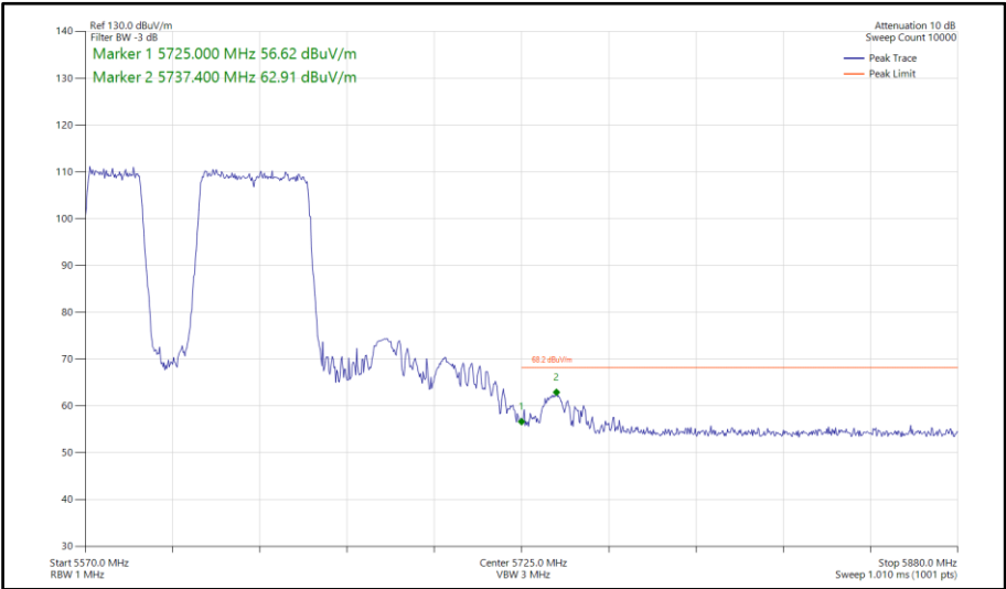
Figure 764 - 802.11be EHT80, RU 484+242-91, SISO, Core 0 - 5610 MHz Band Edge Frequency 5725 MHz
