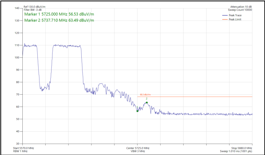
Figure 789 - 802.11be EHT80, RU 484+242-91, SISO, Core 1 - 5610 MHz Band Edge Frequency 5725 MHz
