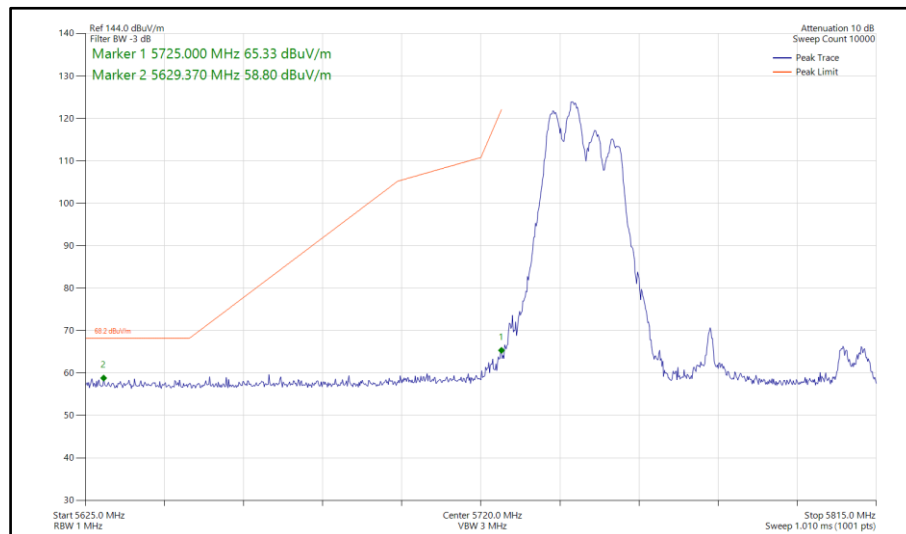
Figure 808 - 802.11ax HE80, RU 106-53, CDD, Core 0-1 - 5775 MHz Band Edge Frequency 5725 MHz
