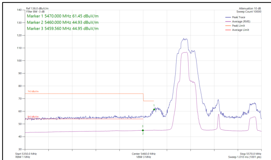
Figure 779 - 802.11be EHT80, RU 52+26-71, SISO, Core 1 - 5530 MHz Band Edge Frequency 5470 MHz
