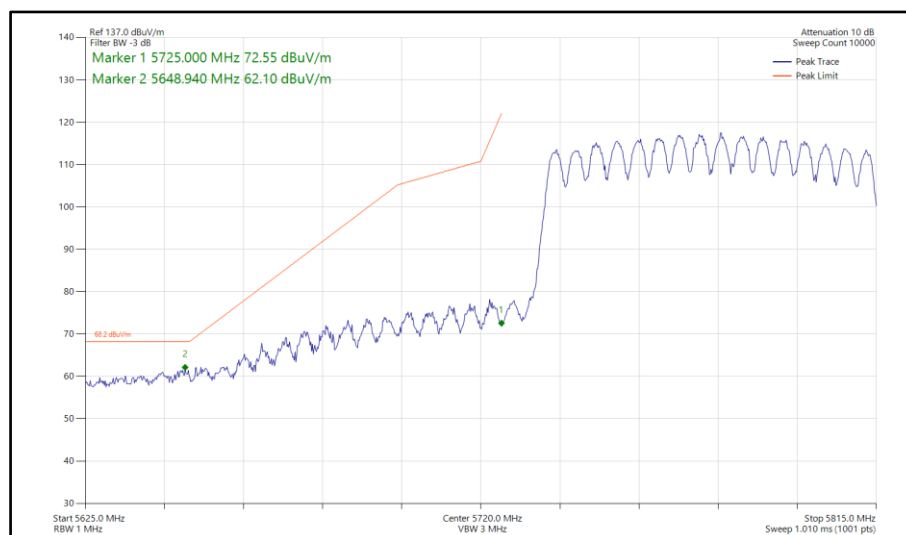
Figure 807 - 802.11ax HE80, SU, CDD, Core 0-1 - 5775 MHz Band Edge Frequency 5725 MHz
