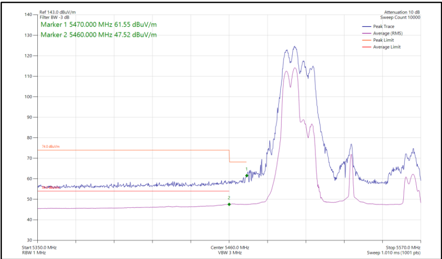
Figure 803 - 802.11ax HE80, RU 106-53, CDD, Core 0-1 - 5530 MHz Band Edge Frequency 5470 MHz
