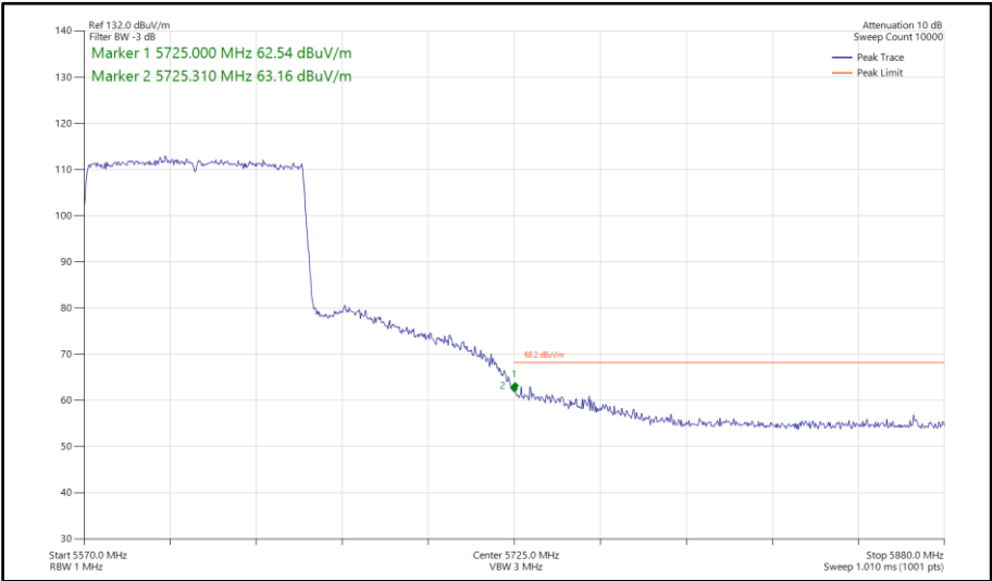
Figure 787 - 802.11ax HE80, SU, SISO, Core 1 - 5610 MHz Band Edge Frequency 5725 MHz
