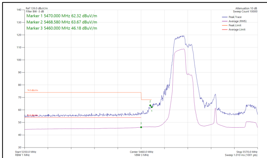
Figure 754 - 802.11be EHT80, RU 106+26-82, SISO, Core 0 - 5530 MHz Band Edge Frequency 5470 MHz
