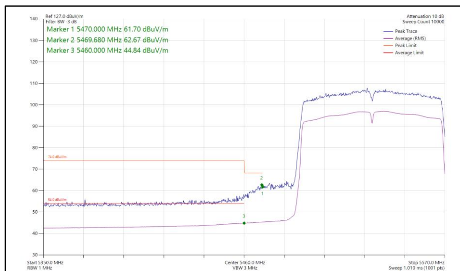
Figure 776 - 802.11ac VHT80, SISO, Core 1 - 5530 MHz Band Edge Frequency 5470 MHz
