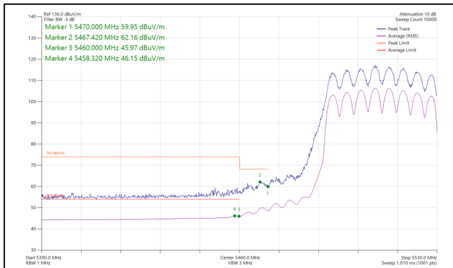
Figure 741 - 802.11ax HE40, SU, TxBF, Core 0-1 - 5510 MHz Band Edge Frequency 5470 MHz
