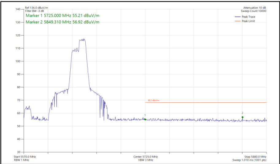
Figure 788 - 802.11ax HE80, RU 106-60, SISO, Core 1 - 5610 MHz Band Edge Frequency 5725 MHz
