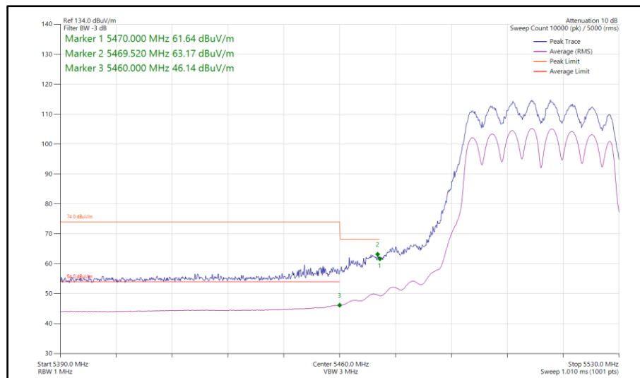
Figure 740 - 802.11ac VHT40, TxBF, Core 0-1 - 5510 MHz Band Edge Frequency 5470 MHz
