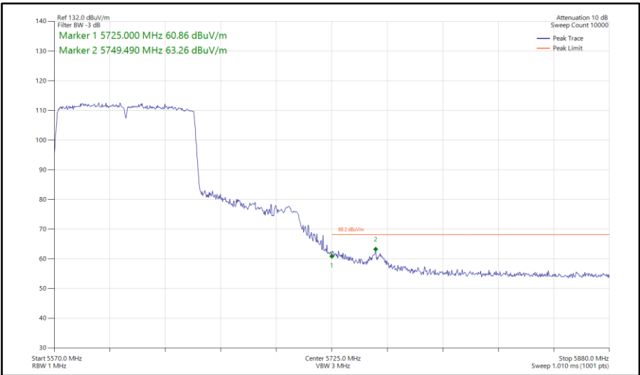
Figure 761 - 802.11ac VHT80, SISO, Core 0 - 5610 MHz Band Edge Frequency 5725 MHz
