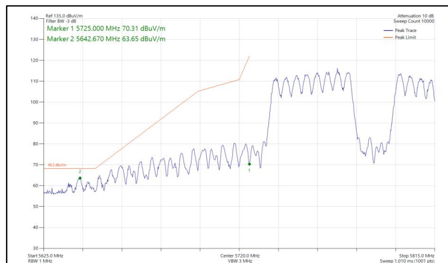
Figure 809 - 802.11be EHT80, RU 484+242-92, CDD, Core 0-1 - 5775 MHz Band Edge Frequency 5725 MHz
