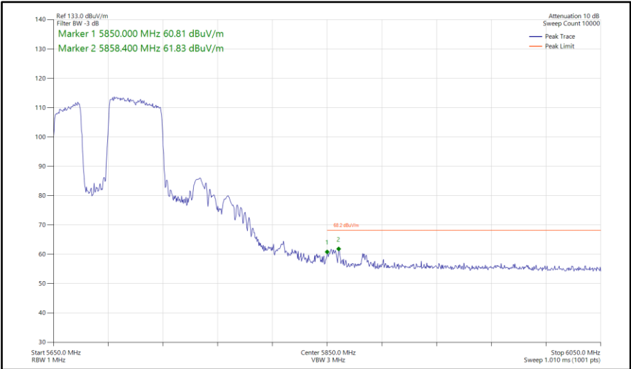
Figure 798 - 802.11be EHT80, RU 484+242-91, SISO, Core 1 - 5690 MHz Band Edge Frequency 5850 MHz
