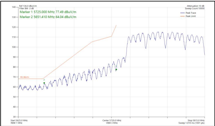
Figure 805 - 802.11a a80, CDD, Core 0-1 - 5775 MHz Band Edge Frequency 5725 MHz
