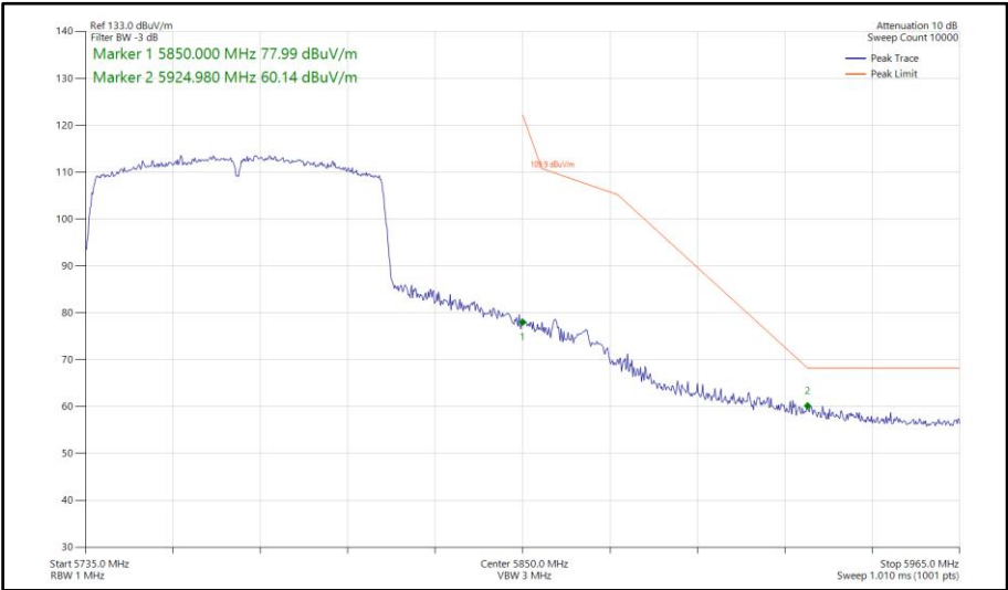
Figure 793 - 802.11ac VHT80, SISO, Core 1 - 5775 MHz Band Edge Frequency 5850 MHz
