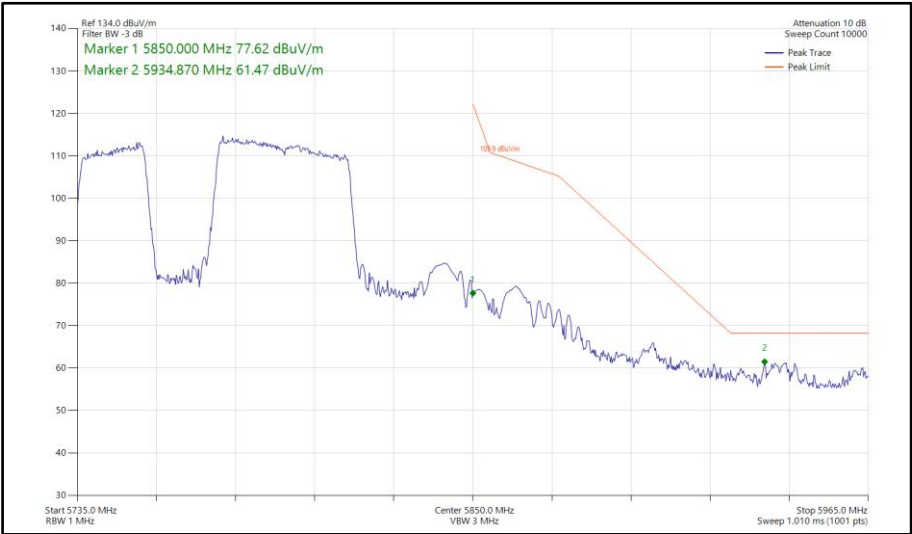
Figure 799 - 802.11be EHT80, RU 484+242-91, SISO, Core 1 - 5775 MHz Band Edge Frequency 5850 MHz
