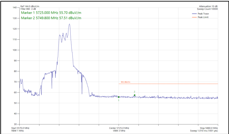
Figure 813 - 802.11ax HE80, RU 52-52, CDD, Core 0-1 - 5610 MHz Band Edge Frequency 5725 MHz
