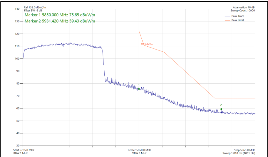
Figure 771 - 802.11ax HE80, SU, SISO, Core 0 - 5775 MHz Band Edge Frequency 5850 MHz
