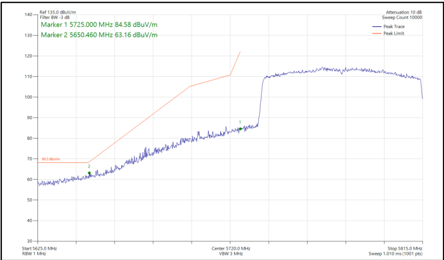
Figure 782 - 802.11ax HE80, SU, SISO, Core 1 - 5775 MHz Band Edge Frequency 5725 MHz
