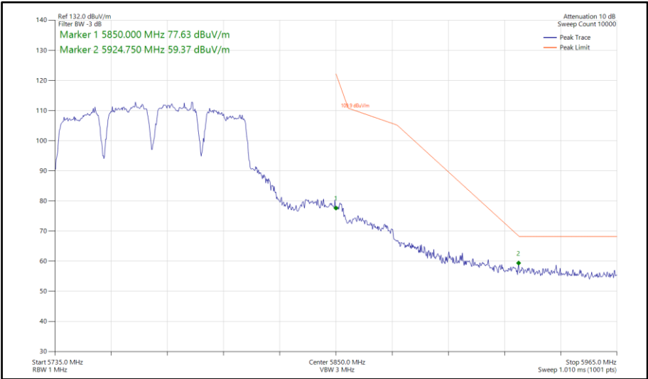
Figure 766 - 802.11a a80, SISO, Core 0 - 5775 MHz Band Edge Frequency 5850 MHz
