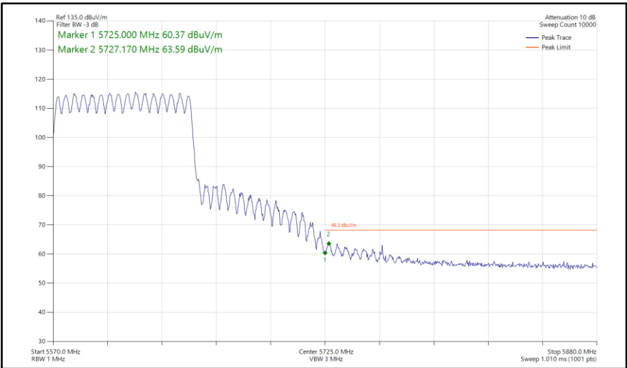
Figure 811 - 802.11ac VHT80, CDD, Core 0-1 - 5610 MHz Band Edge Frequency 5725 MHz
