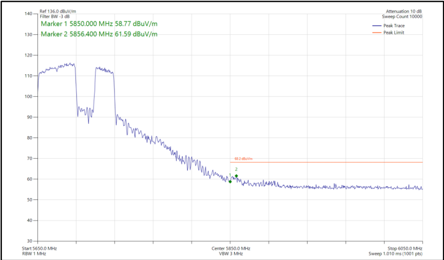
Figure 773 - 802.11be EHT80, RU 484+242-92, SISO, Core 0 - 5690 MHz Band Edge Frequency 5850 MHz
