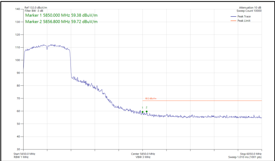
Figure 792 - 802.11ac VHT80, SISO, Core 1 - 5690 MHz Band Edge Frequency 5850 MHz
