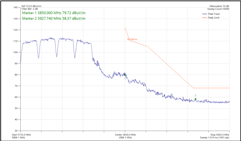
Figure 791 - 802.11a a80, SISO, Core 1 - 5775 MHz Band Edge Frequency 5850 MHz
