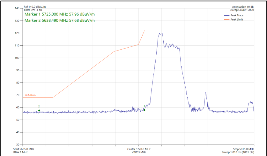
Figure 758 - 802.11ax HE80, RU 52-37, SISO, Core 0 - 5775 MHz Band Edge Frequency 5725 MHz
