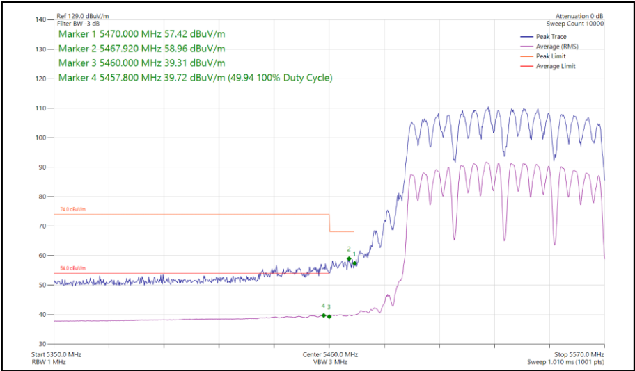
Figure 800 - 802.11a a80, CDD, Core 0-1 - 5530 MHz Band Edge Frequency 5470 MHz
