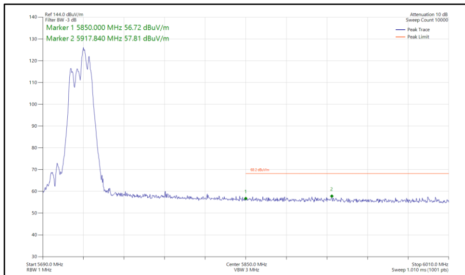
Figure 738 - 802.11be EHT40, RU 52+26-75, SDM, Core 0-1 - 5710 MHz Band Edge Frequency 5850 MHz
