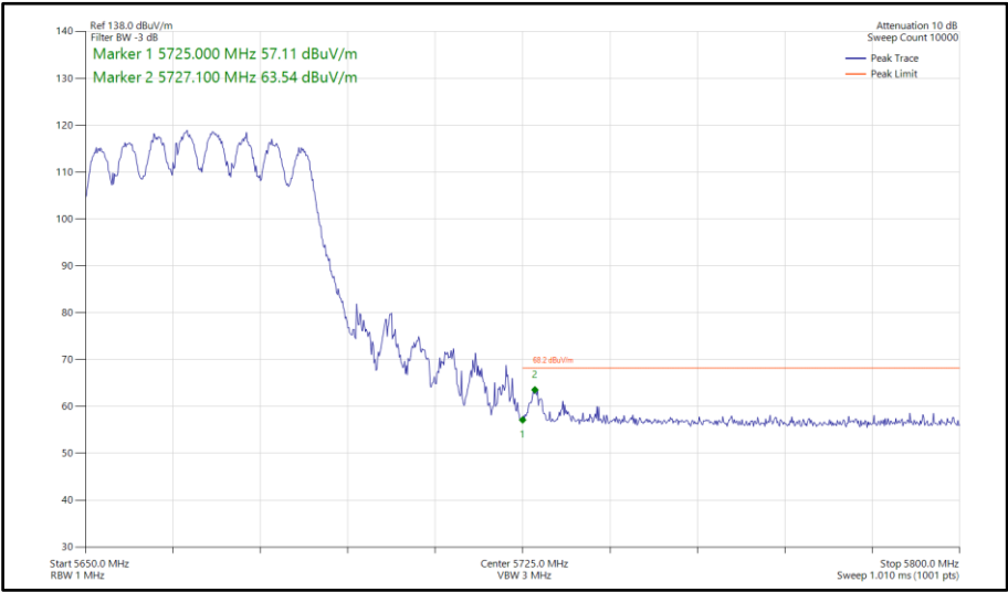
Figure 745 - 802.11ax HE40, SU, TxBF, Core 0-1 - 5670 MHz Band Edge Frequency 5725 MHz
