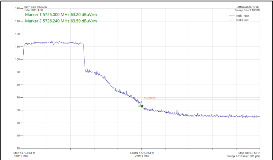
Figure 762 - 802.11ax HE80, SU, SISO, Core 0 - 5610 MHz Band Edge Frequency 5725 MHz
