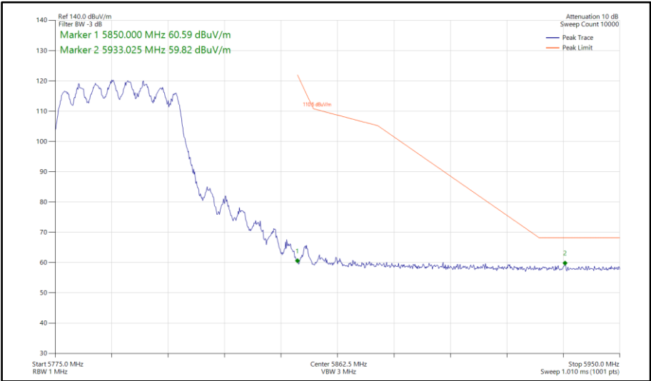
Figure 747 - 802.11ac VHT40, TxBF, Core 0-1 - 5795 MHz Band Edge Frequency 5850 MHz
