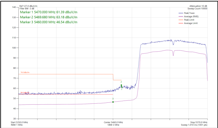
Figure 751 - 802.11ac VHT80, SISO, Core 0 - 5530 MHz Band Edge Frequency 5470 MHz
