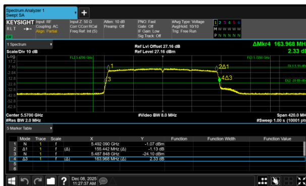
Figure 340 - 802.11ax HE160 SU Minimum 26 dB EBW
