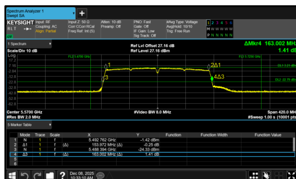
Figure 333 - 802.11ac VHT160 Maximum 26 dB EBW
