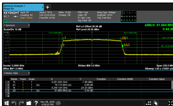
Figure 354 - 802.11ax HE80 SU Minimum 26 dB EBW
