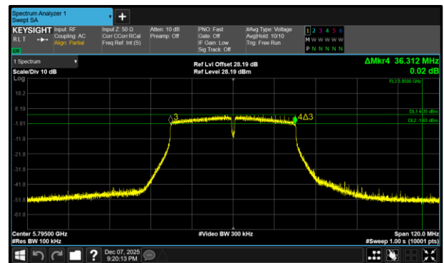
Figure 367 - 802.11n HT40 Maximum 6 dB EBW
