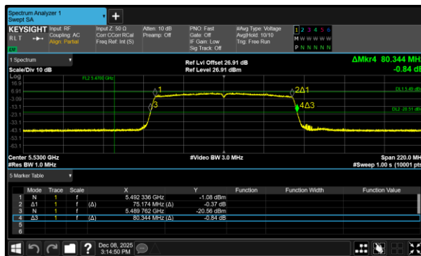
Figure 346 - 802.11ac VHT80 Minimum 26 dB EBW
