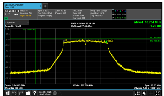
Figure 395 - 802.11a20 Maximum 6 dB EBW
