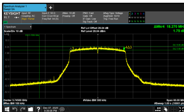
Figure 370 - 802.11ax HE20 SU Minimum 6 dB EBW
