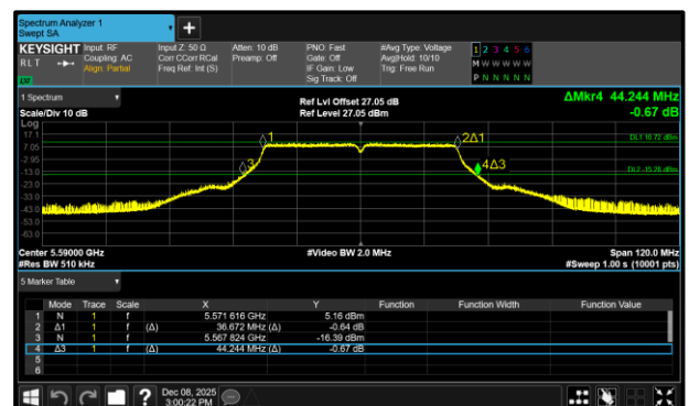
Figure 345 - 802.11ac VHT40 Maximum 26 dB EBW
