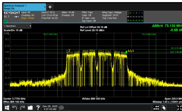
Figure 398 - 802.11a80 Minimum 6 dB EBW
