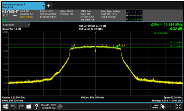
Figure 382 - 802.11n HT20 Minimum 6 dB EBW
