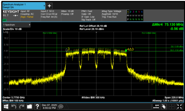
Figure 362 - 802.11a80 Minimum 6 dB EBW
