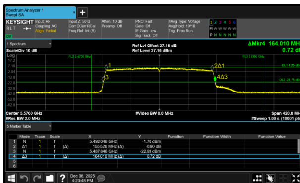
Figure 356 - 802.11ax HE160 SU Minimum 26 dB EBW
