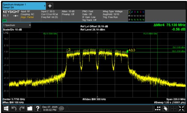
Figure 363 - 802.11a80 Maximum 6 dB EBW
