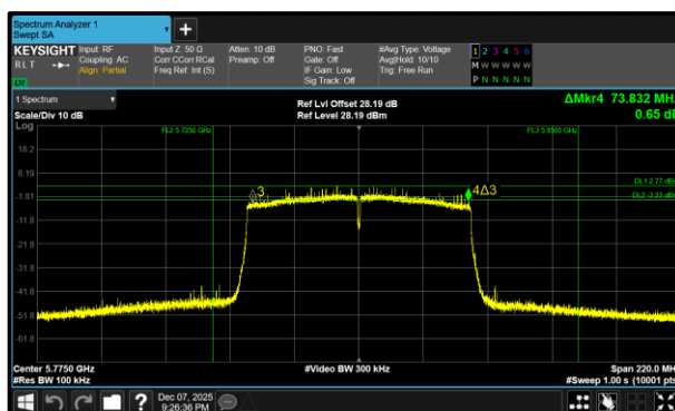
Figure 368 - 802.11ac VHT80 Minimum 6 dB EBW
