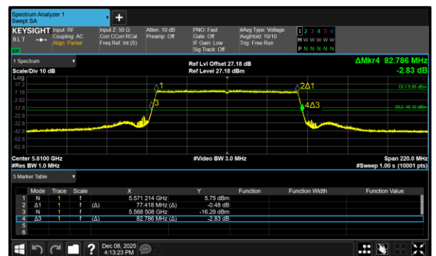
Figure 355 - 802.11ax HE80 SU Maximum 26 dB EBW
