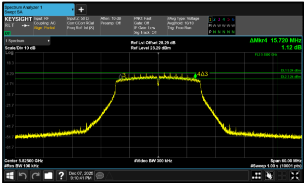
Figure 364 - 802.11n HT20 Minimum 6 dB EBW
