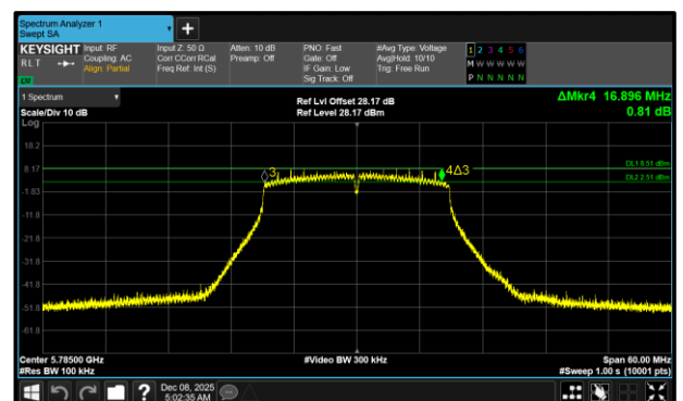
Figure 401 - 802.11n HT20 Maximum 6 dB EBW
