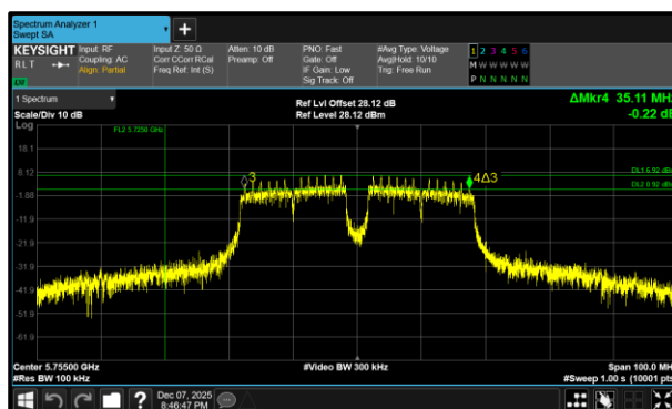
Figure 360 - 802.11a40 Minimum 6 dB EBW
