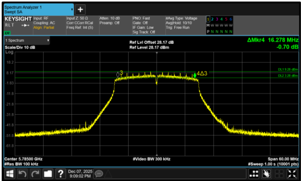
Figure 365 - 802.11n HT20 Maximum 6 dB EBW
