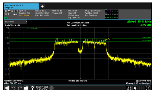
Figure 361 - 802.11a40 Maximum 6 dB EBW
