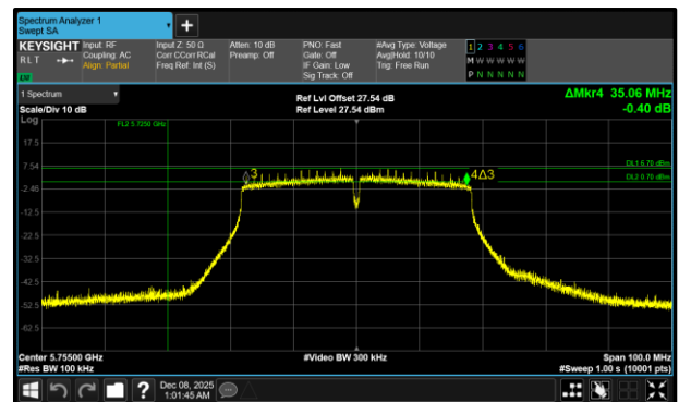
Figure 385 - 802.11n HT40 Maximum 6 dB EBW
