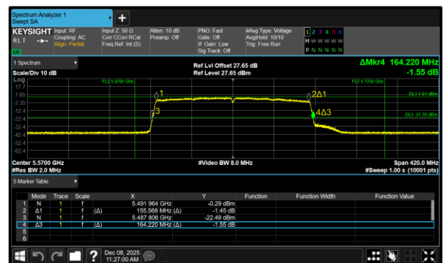
Figure 341 - 802.11ax HE160 SU Maximum 26 dB EBW
