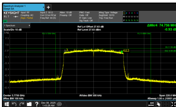
Figure 392 - 802.11ax HE80 SU Minimum 6 dB EBW
