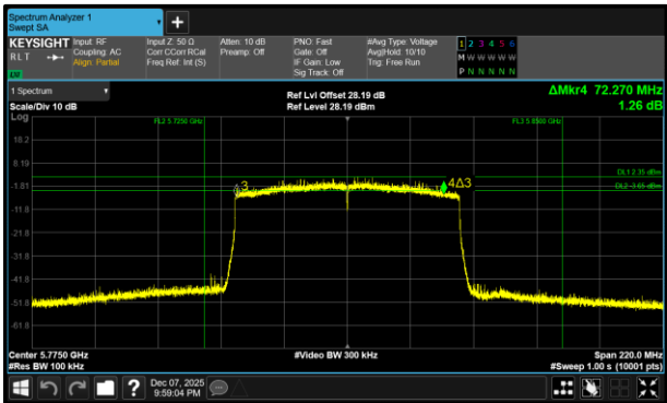
Figure 375 - 802.11ax HE80 SU Maximum 6 dB EBW
