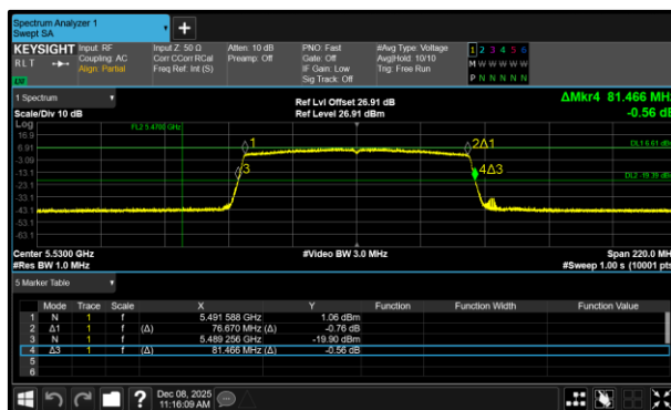
Figure 338 - 802.11ax HE80 SU Minimum 26 dB EBW
