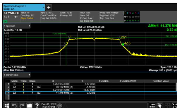
Figure 344 - 802.11ac VHT40 Minimum 26 dB EBW
