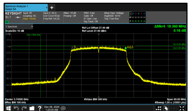
Figure 389 - 802.11ax HE20 SU Maximum 6 dB EBW
