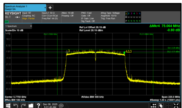
Figure 405 - 802.11ac VHT80 Maximum 6 dB EBW
