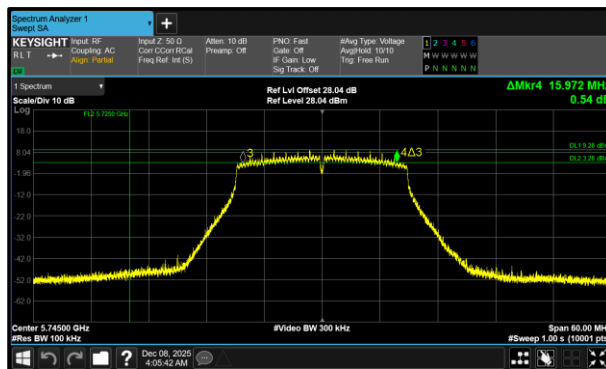
Figure 394 - 802.11a20 Minimum 6 dB EBW
