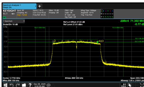
Figure 404 - 802.11ac VHT80 Minimum 6 dB EBW
