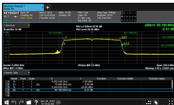
Figure 330 - 802.11ac VHT80 Minimum 26 dB EBW
