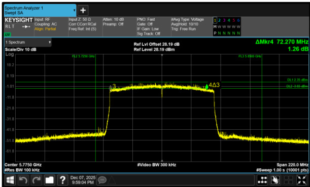
Figure 374 - 802.11ax HE80 SU Minimum 6 dB EBW
