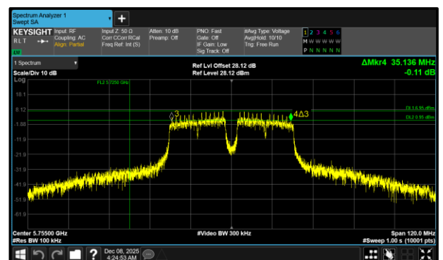
Figure 397 - 802.11a40 Maximum 6 dB EBW
