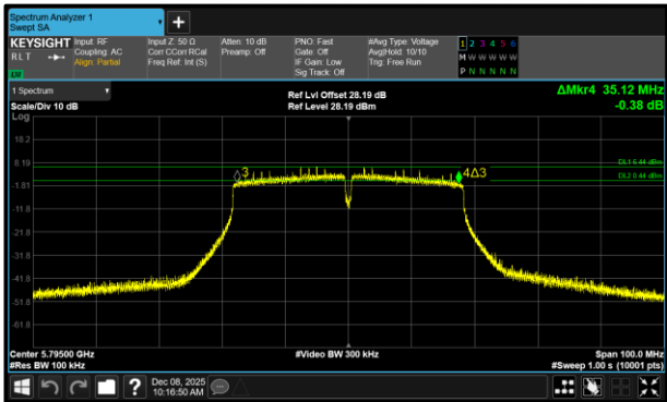
Figure 415 - 802.11n HT40 Maximum 6 dB EBW
