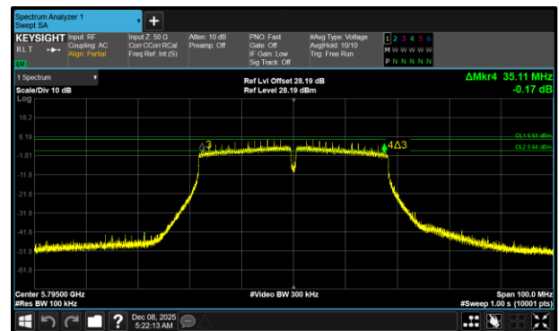
Figure 403 - 802.11n HT40 Maximum 6 dB EBW
