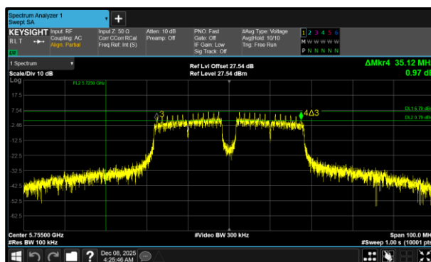
Figure 396 - 802.11a40 Minimum 6 dB EBW
