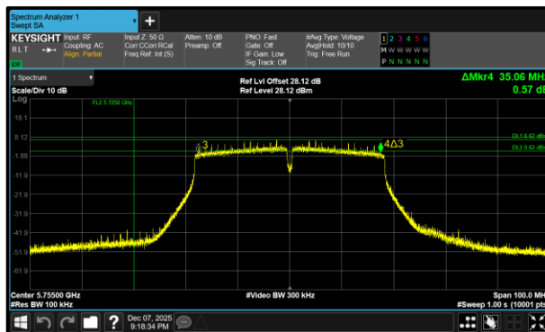
Figure 366 - 802.11n HT40 Minimum 6 dB EBW
