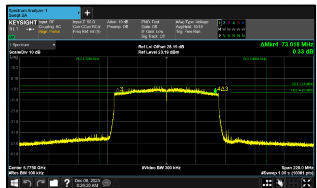
Figure 411 - 802.11ax HE80 SU Maximum 6 dB EBW
