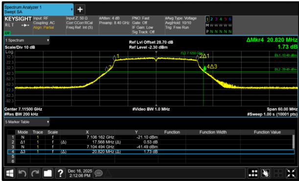
Figure 225 - 802.11a20 VLP Minimum 26 dB EBW
