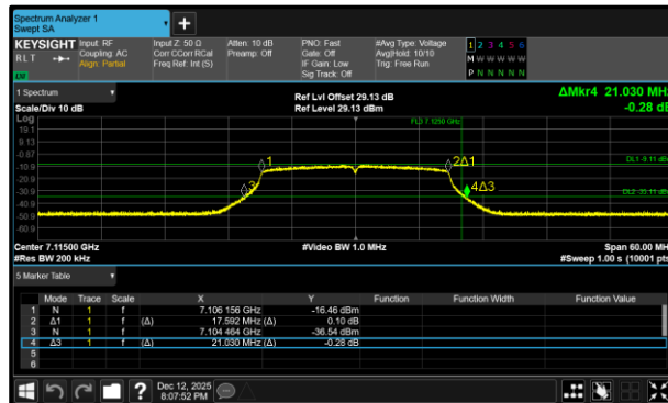
Figure 193 - 802.11a20 LPI Minimum 26 dB EBW
