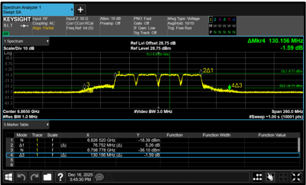
Figure 230 - 802.11a80 VLP Maximum 26 dB EBW
