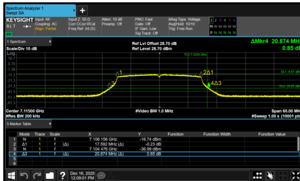
Figure 177 - 802.11a20 VLP Minimum 99% OBW
