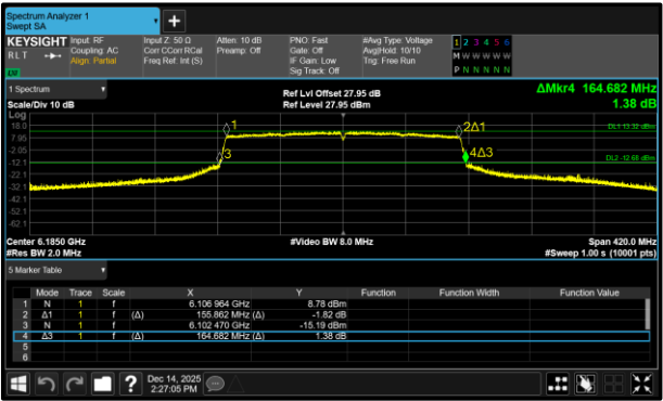
Figure 176 - 802.11ax HE160 SU SP Maximum 99% OBW
