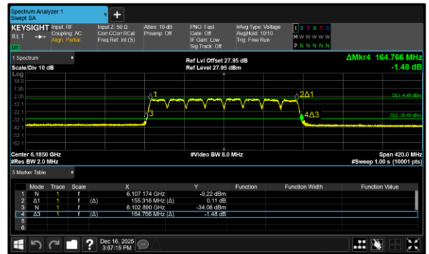
Figure 232 - 802.11a160 VLP Maximum 26 dB EBW
