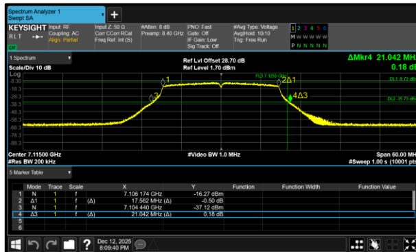
Figure 241 - 802.11a20 LPI Minimum 99% OBW
