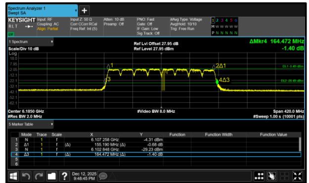
Figure 200 - 802.11a160 LPI Maximum 26 dB EBW
