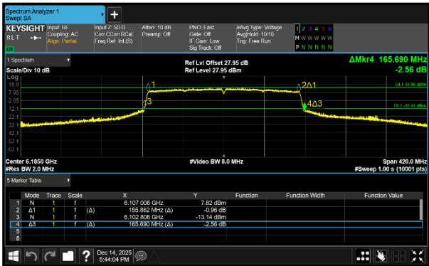
Figure 224 - 802.11ax HE160 SU SP Maximum 26 dB EBW
