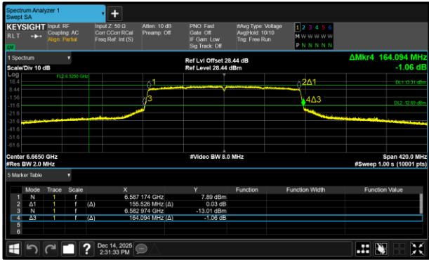
Figure 175 - 802.11ax HE160 SU SP Minimum 99% OBW
