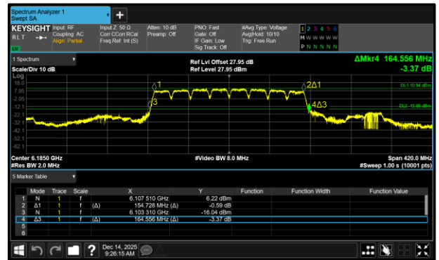
Figure 168 - 802.11a160 SP Maximum 99% OBW
