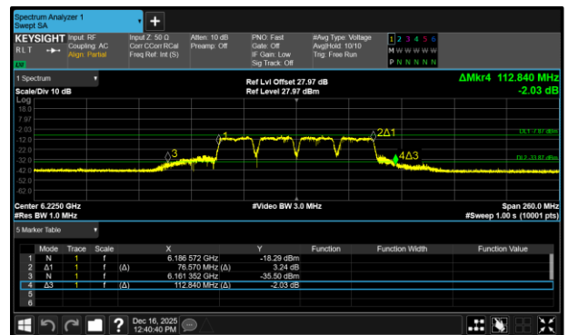
Figure 182 - 802.11a80 VLP Maximum 99% OBW
