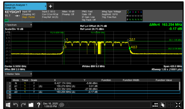
Figure 184 - 802.11a160 VLP Maximum 99% OBW
