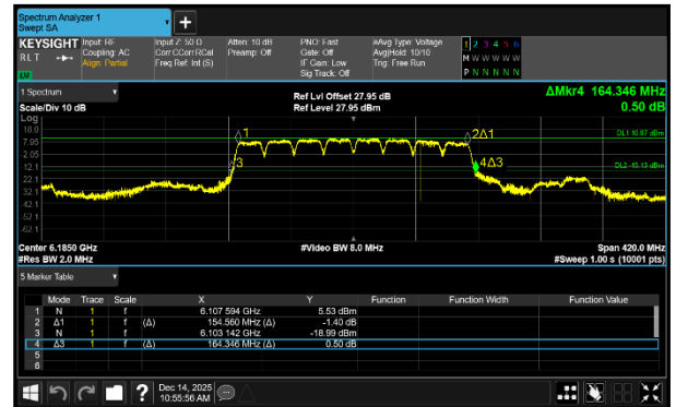
Figure 216 - 802.11a160 SP Maximum 26 dB EBW
