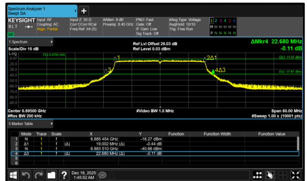
Figure 234 - 802.11ax HE20 SU VLP Maximum 26 dB EBW
