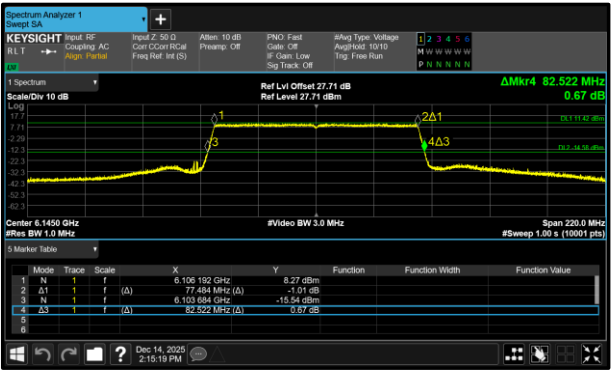
Figure 174 - 802.11ax HE80 SU SP Maximum 99% OBW
