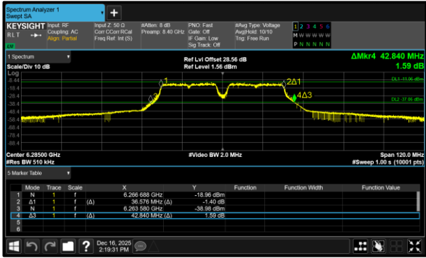
Figure 227 - 802.11a40 VLP Minimum 26 dB EBW
