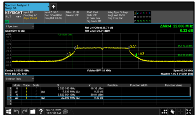
Figure 178 - 802.11a20 VLP Maximum 99% OBW
