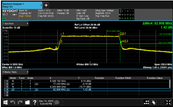
Figure 222 - 802.11ax HE80 SU SP Maximum 26 dB EBW
