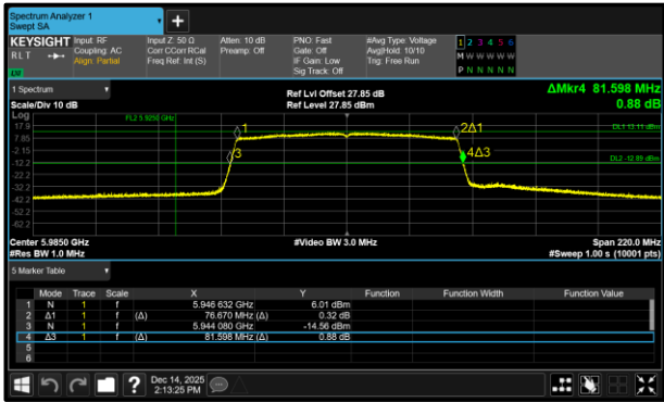
Figure 173 - 802.11ax HE80 SU SP Minimum 99% OBW
