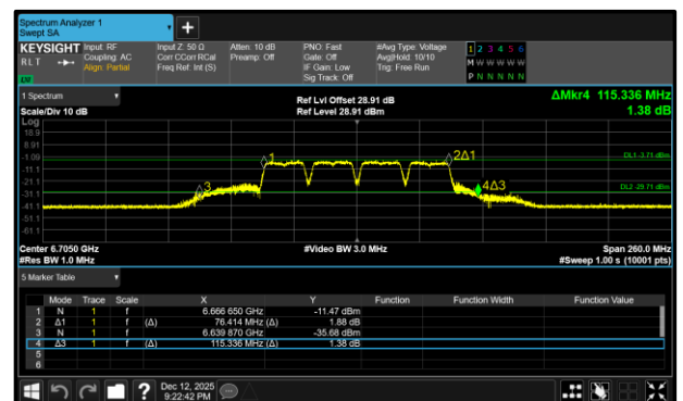
Figure 198 - 802.11a80 LPI Maximum 26 dB EBW
