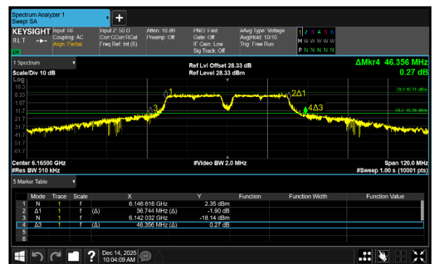
Figure 260 - 802.11a40 SP Maximum 99% OBW
