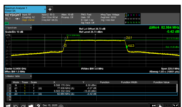
Figure 302 - 802.11ax HE80 SU SP Maximum 26 dB EBW
