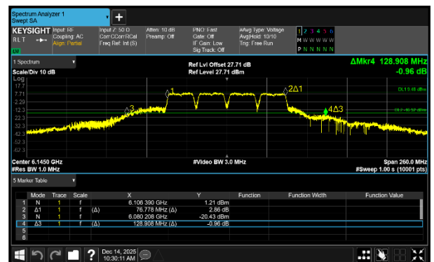
Figure 262 - 802.11a80 SP Maximum 99% OBW
