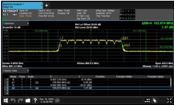
Figure 279 - 802.11a160 VLP Minimum 99% OBW
