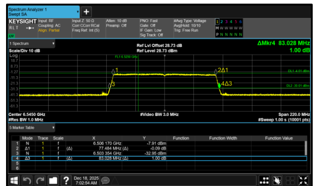
Figure 310 - 802.11ax HE80 SU VLP Maximum 26 dB EBW
