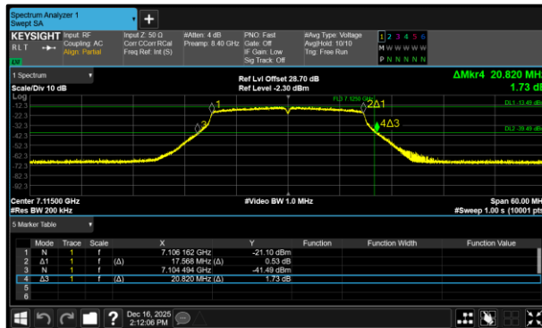
Figure 273 - 802.11a20 VLP Minimum 99% OBW
