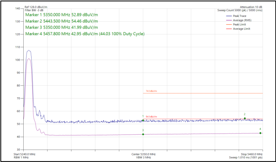
Figure 649 - HDR8, SISO, Core 1 - 5245 MHz Band Edge Frequency 5350 MHz
