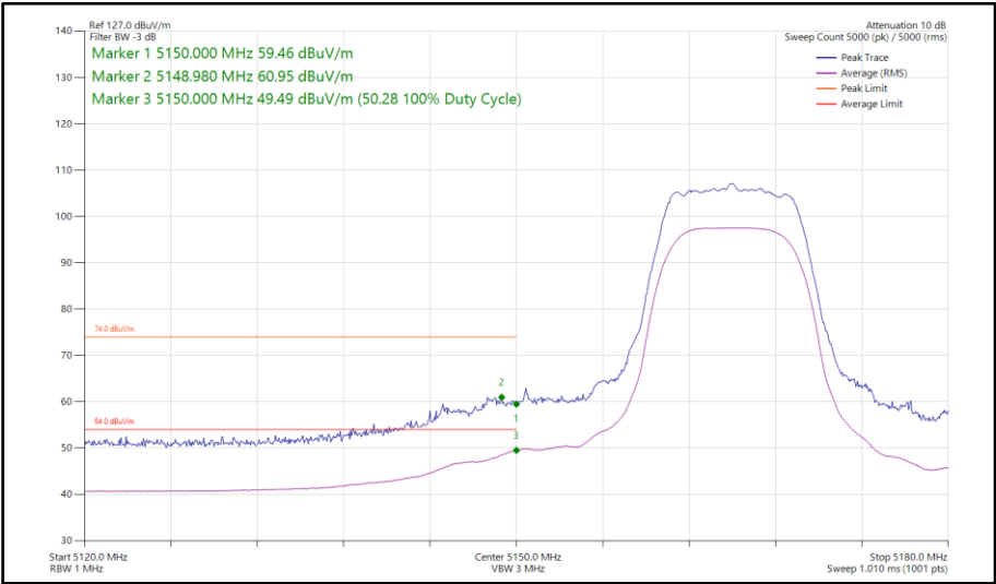
Figure 646 - XHDRPL24, SISO, Core 1 - 5165 MHz Band Edge Frequency 5150 MHz
