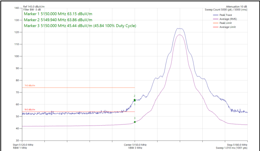
Figure 696 - HDT6, SISO, Core 0 - 5162 MHz Band Edge Frequency 5150 MHz
