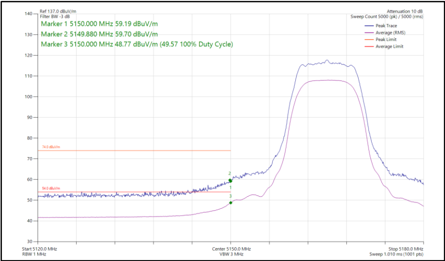
Figure 702 - XHDRPL24, SISO, Core 0 - 5165 MHz Band Edge Frequency 5150 MHz
