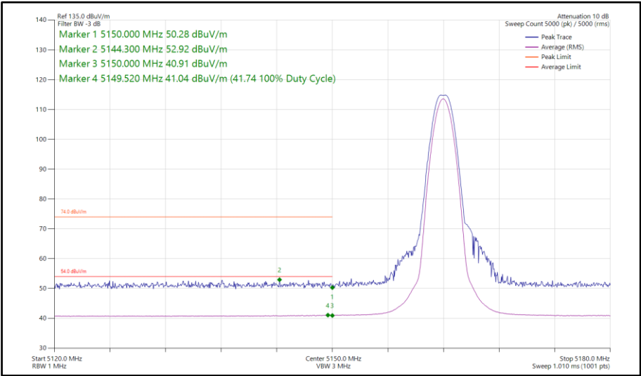
Figure 664 - LE1M, MIMO, Core 0-1 - 5162 MHz Band Edge Frequency 5150 MHz
