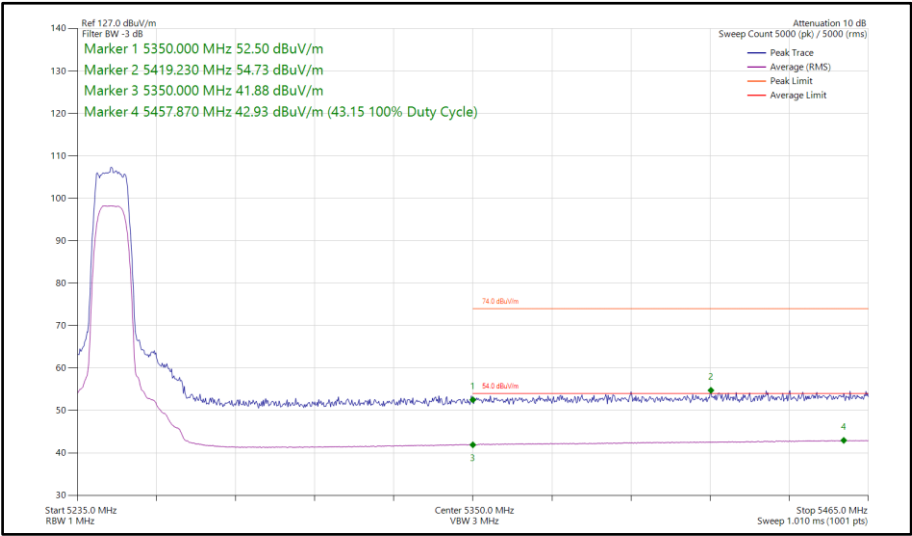
Figure 657 - HDRPL8, SISO, Core 1 - 5245 MHzBand Edge Frequency 5350 MHz
