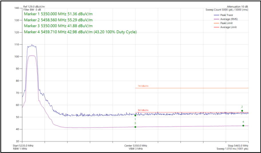
Figure 685 - HDRPL8, MIMO, Core 0-1 - 5245 MHzBand Edge Frequency 5350 MHz
