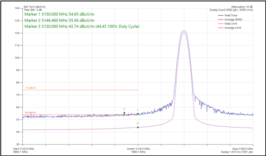
Figure 692 - LE1M, SISO, Core 0 - 5162 MHz Band Edge Frequency 5150 MHz
