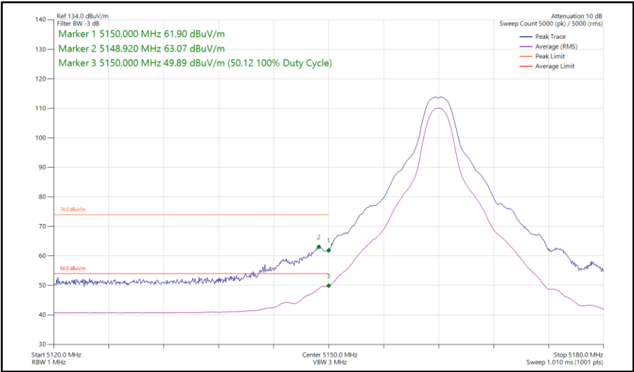
Figure 666 - HDT3, MIMO, Core 0-1 - 5162 MHzBand Edge Frequency 5150 MHz
