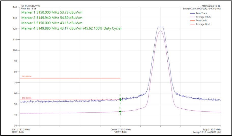
Figure 693 - LE2M, SISO, Core 0 - 5162 MHzBand Edge Frequency 5150 MHz
