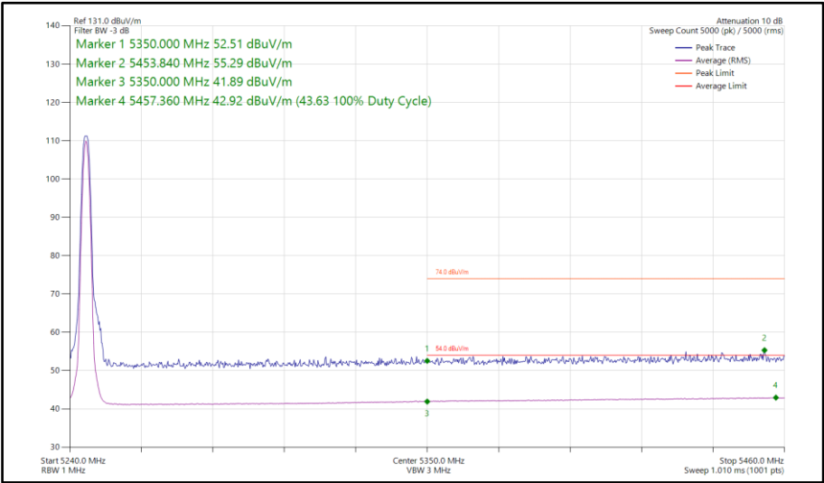
Figure 650 - LE1M, SISO, Core 1 - 5245 MHz Band Edge Frequency 5350 MHz
