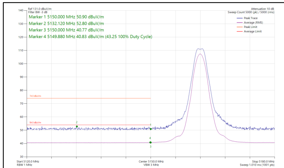
Figure 637 - LE2M, SISO, Core 1 - 5162 MHz Band Edge Frequency 5150 MHz
