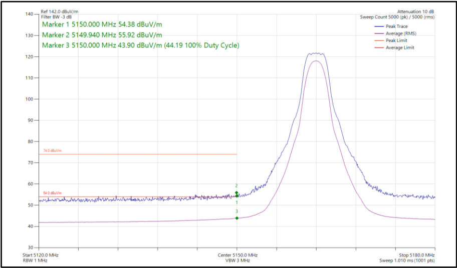
Figure 697 - HDRPS2, SISO, Core 0 - 5162 MHz Band Edge Frequency 5150 MHz
