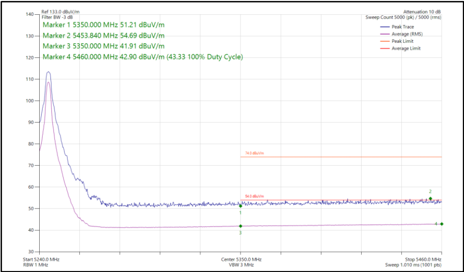
Figure 682 - HDT6, MIMO, Core 0-1 - 5245 MHz Band Edge Frequency 5350 MHz
