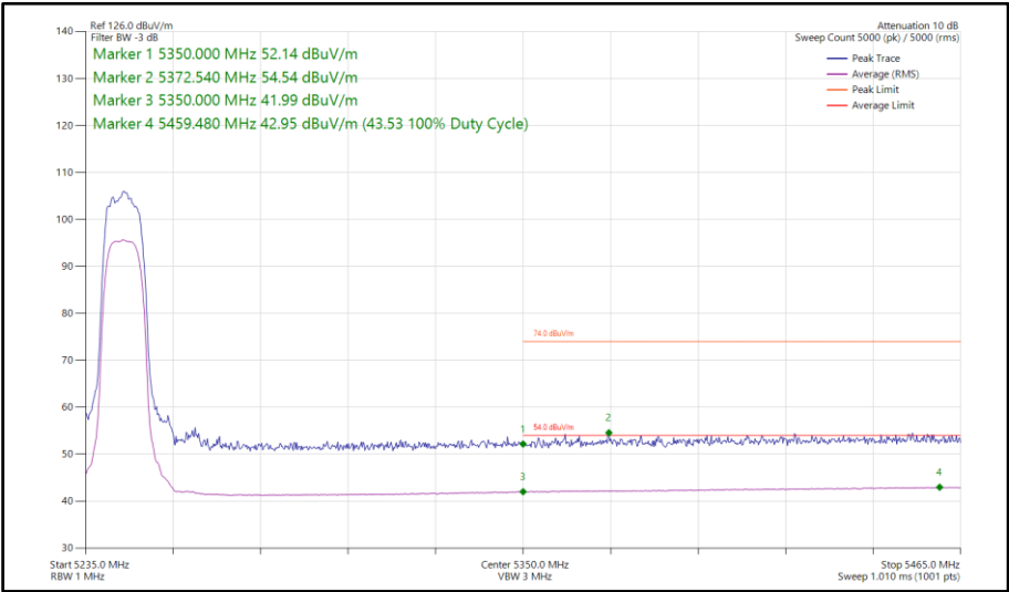
Figure 658 - HDRPL24, SISO, Core 1 - 5245 MHzBand Edge Frequency 5350 MHz
