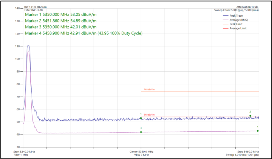
Figure 676 - HDR4, MIMO, Core 0-1 - 5245 MHzBand Edge Frequency 5350 MHz
