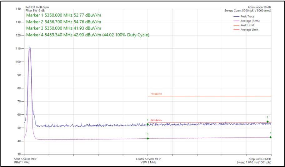
Figure 647 - DH5, SISO, Core 1 - 5245 MHz Band Edge Frequency 5350 MHz
