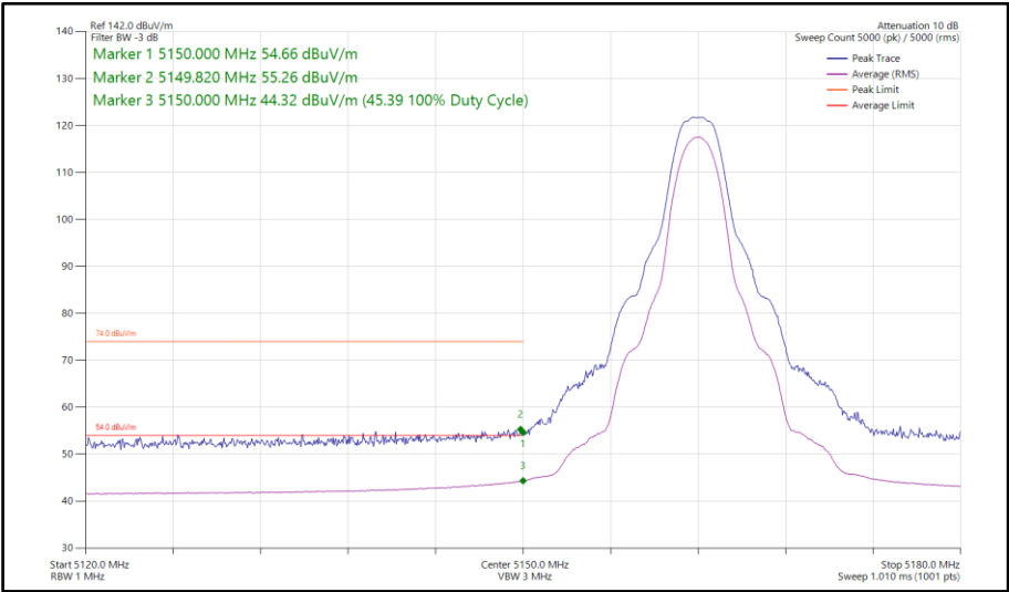
Figure 690 - HDR4, SISO, Core 0 - 5162 MHzBand Edge Frequency 5150 MHz
