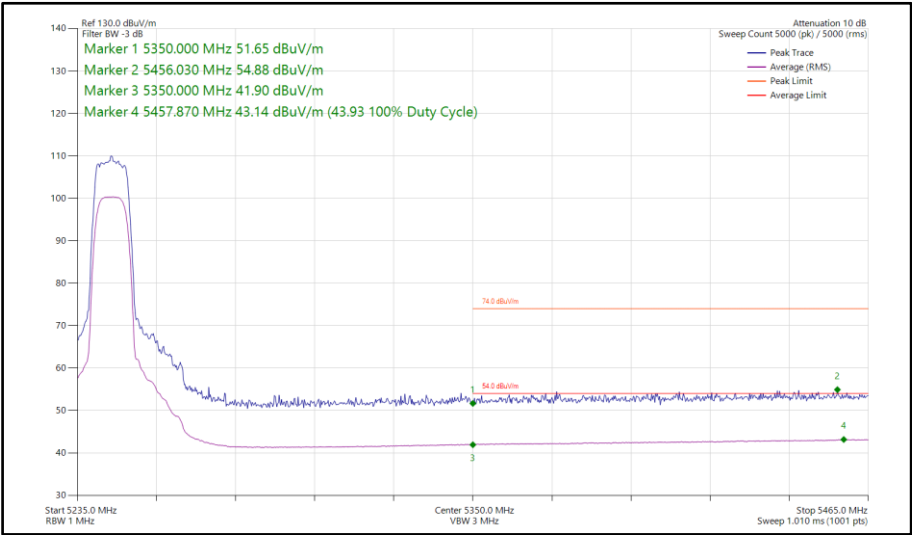
Figure 688 - XHDRPL24, MIMO, Core 0-1 - 5245 MHz Band Edge Frequency 5350 MHz
