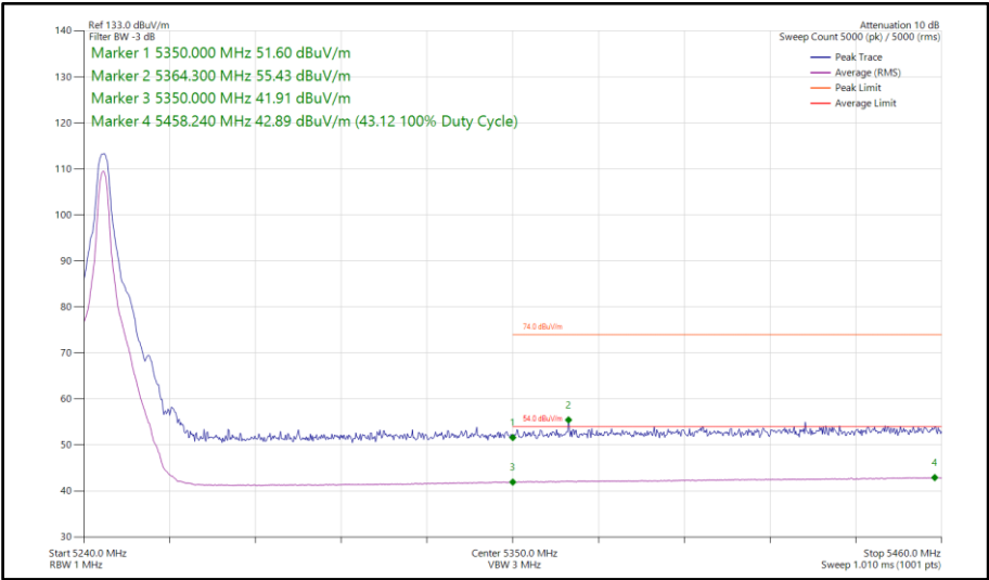
Figure 680 - HDT3, MIMO, Core 0-1 - 5245 MHz Band Edge Frequency 5350 MHz
