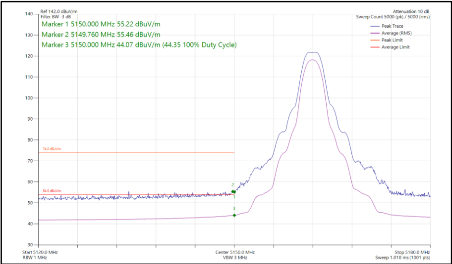
Figure 695 - HDT4, SISO, Core 0 - 5162 MHz Band Edge Frequency 5150 MHz
