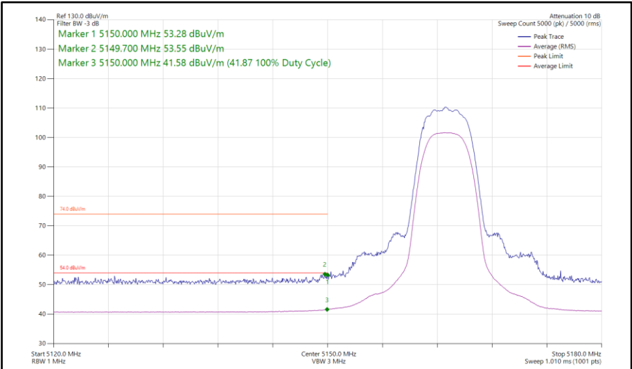
Figure 670 - HDRPM12, MIMO, Core 0-1 - 5163 MHzBand Edge Frequency 5150 MHz
