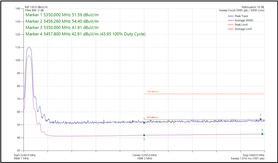
Figure 677 - HDR8, MIMO, Core 0-1 - 5245 MHz Band Edge Frequency 5350 MHz
