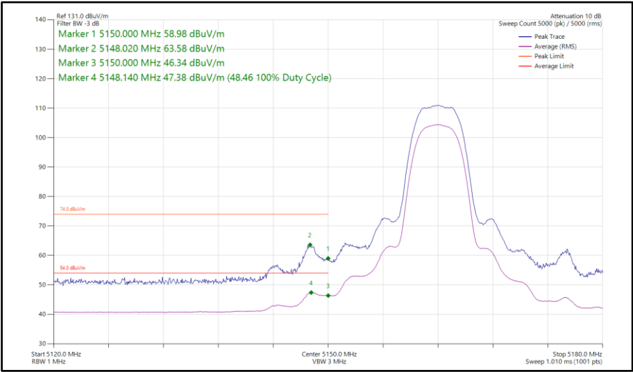
Figure 663 - HDR8, MIMO, Core 0-1 - 5162 MHz Band Edge Frequency 5150 MHz
