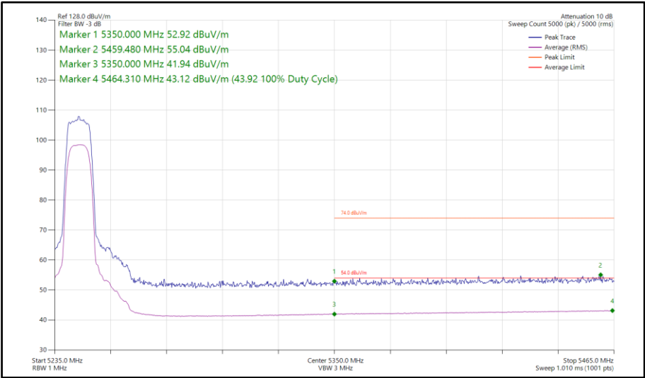
Figure 660 - XHDRPL24, SISO, Core 1 - 5245 MHz Band Edge Frequency 5350 MHz
