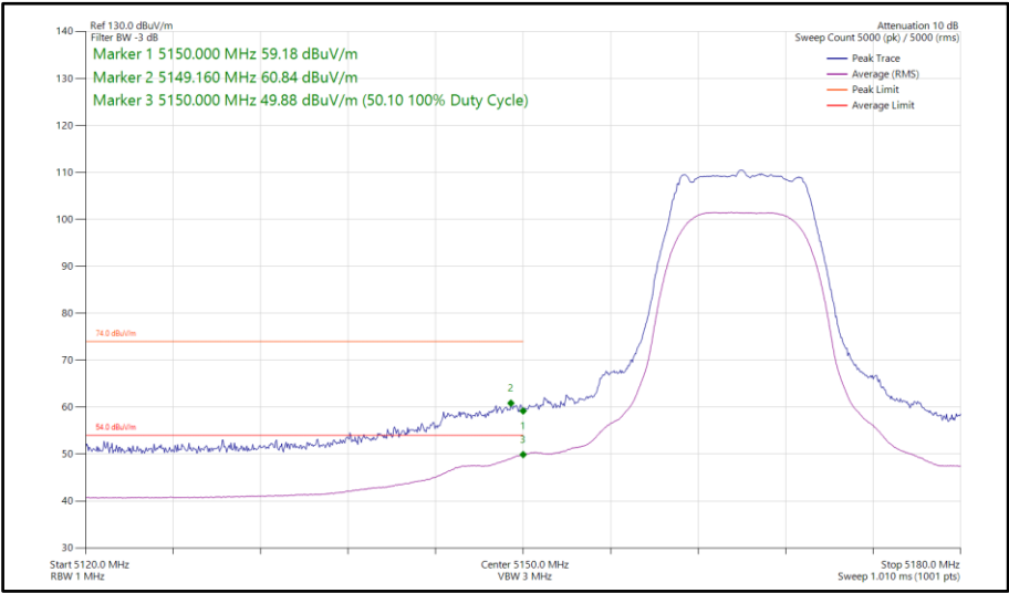
Figure 671 - HDRPL8, MIMO, Core 0-1 - 5165 MHzBand Edge Frequency 5150 MHz
