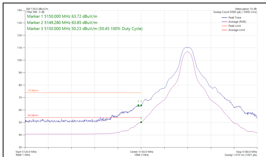
Figure 638 - HDT3, SISO, Core 1 - 5162 MHz Band Edge Frequency 5150 MHz
