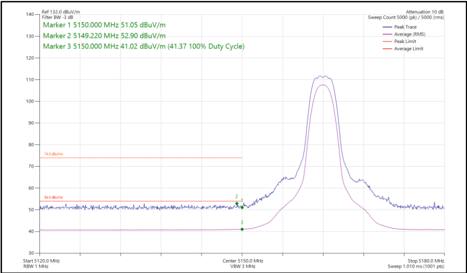
Figure 669 - HDRPS2, MIMO, Core 0-1 - 5162 MHzBand Edge Frequency 5150 MHz
