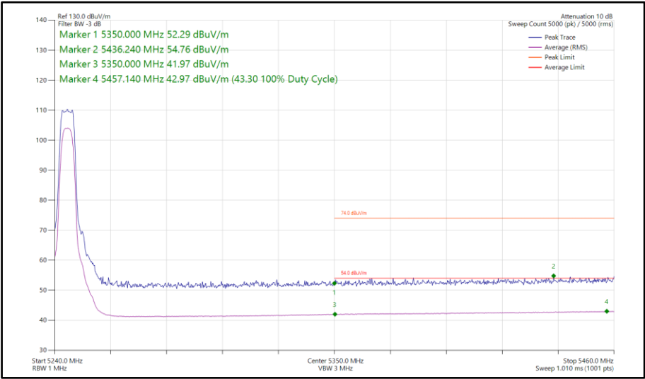
Figure 687 - XHDRPM8, MIMO, Core 0-1 - 5245 MHz Band Edge Frequency 5350 MHz
