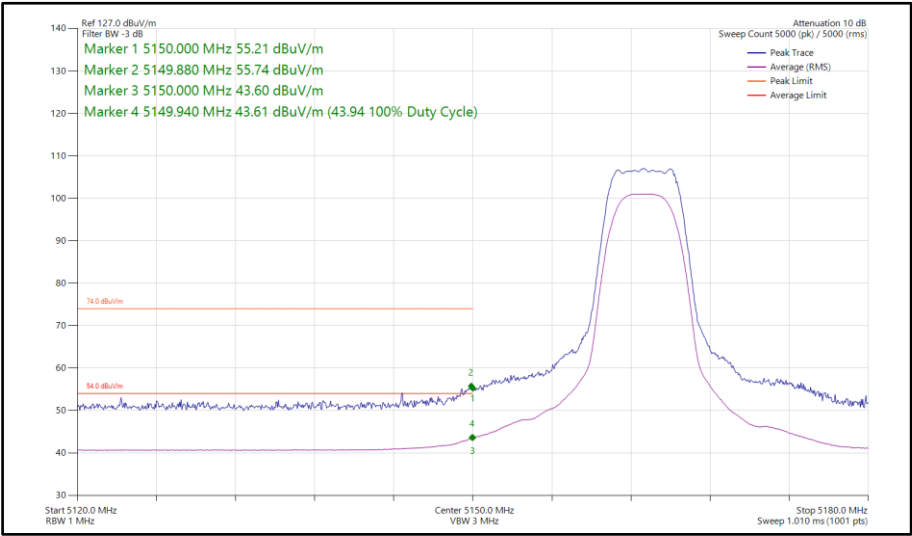
Figure 645 - XHDRPM8, SISO, Core 1 - 5163 MHz Band Edge Frequency 5150 MHz
