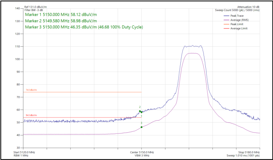
Figure 673 - XHDRPM8, MIMO, Core 0-1 - 5163 MHzBand Edge Frequency 5150 MHz
