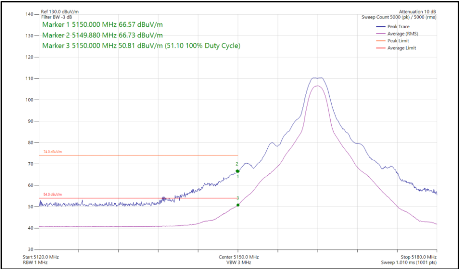
Figure 639 - HDT4, SISO, Core 1 - 5162 MHz Band Edge Frequency 5150 MHz
