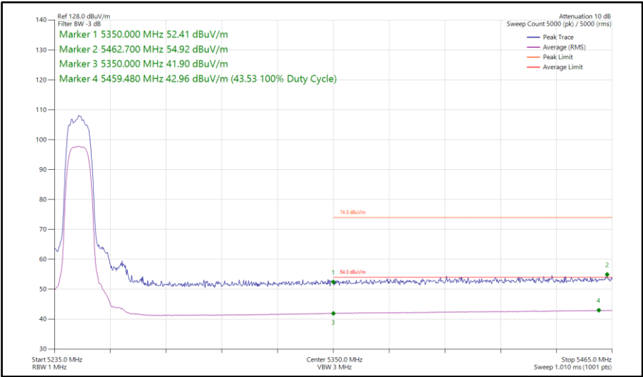
Figure 686 - HDRPL24, MIMO, Core 0-1 - 5245 MHzBand Edge Frequency 5350 MHz
