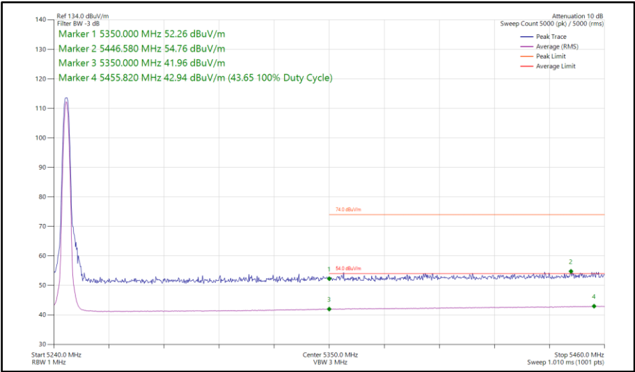
Figure 678 - LE1M, MIMO, Core 0-1 - 5245 MHz Band Edge Frequency 5350 MHz
