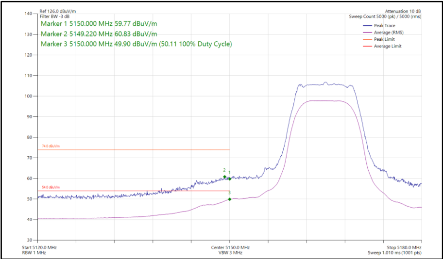
Figure 643 - HDRPL8, SISO, Core 1 - 5165 MHzBand Edge Frequency 5150 MHz
