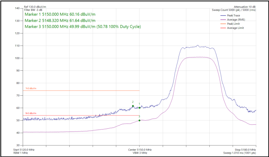
Figure 674 - XHDRPL24, MIMO, Core 0-1 - 5165 MHzBand Edge Frequency 5150 MHz
