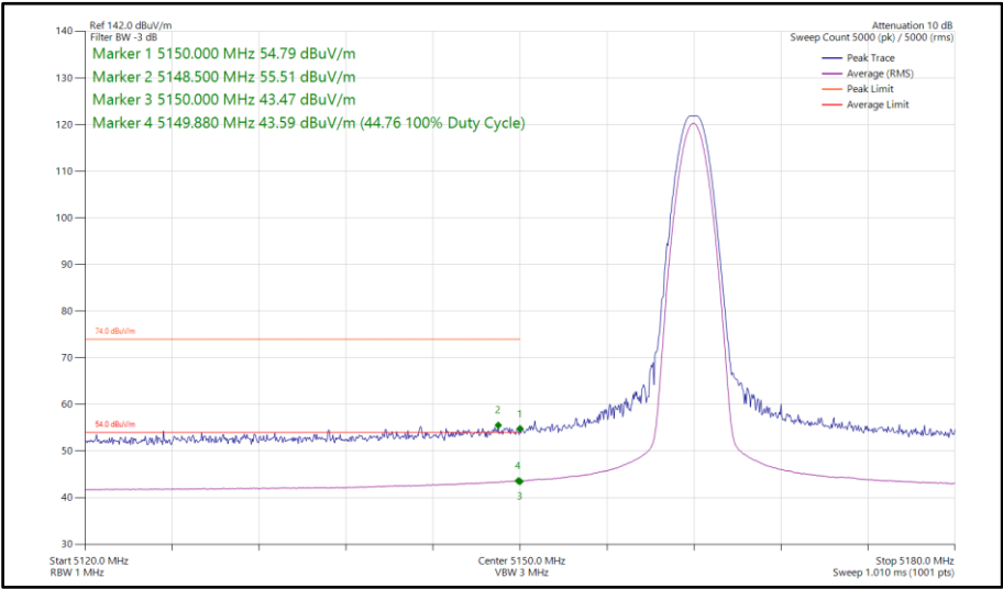
Figure 689 - DH5, SISO, Core 0 - 5162 MHzBand Edge Frequency 5150 MHz
