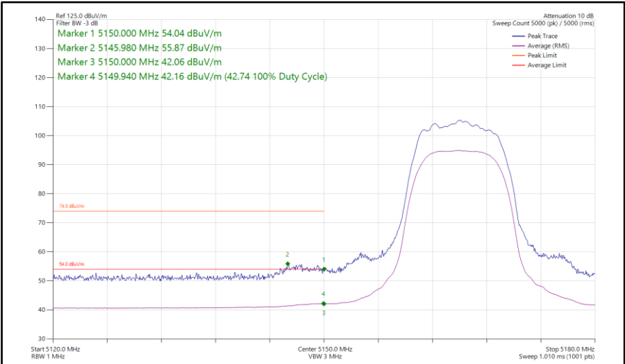
Figure 644 - HDRPL24, SISO, Core 1 - 5165 MHzBand Edge Frequency 5150 MHz
