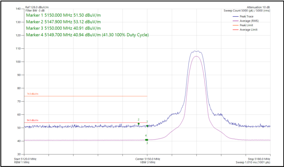
Figure 641 - HDRPS2, SISO, Core 1 - 5162 MHz Band Edge Frequency 5150 MHz
