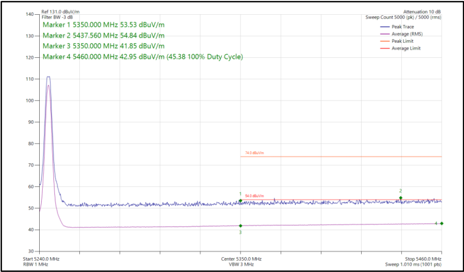
Figure 651 - LE2M, SISO, Core 1 - 5245 MHz Band Edge Frequency 5350 MHz
