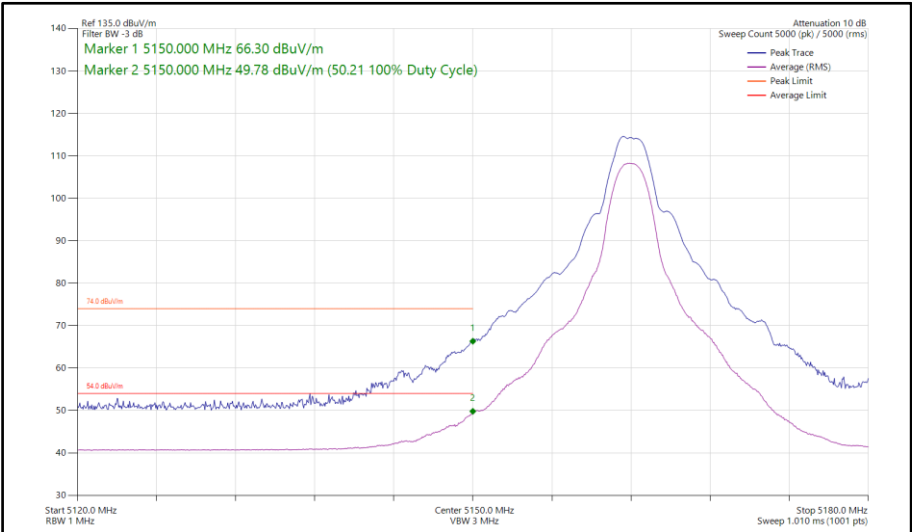
Figure 668 - HDT6, MIMO, Core 0-1 - 5162 MHz Band Edge Frequency 5150 MHz
