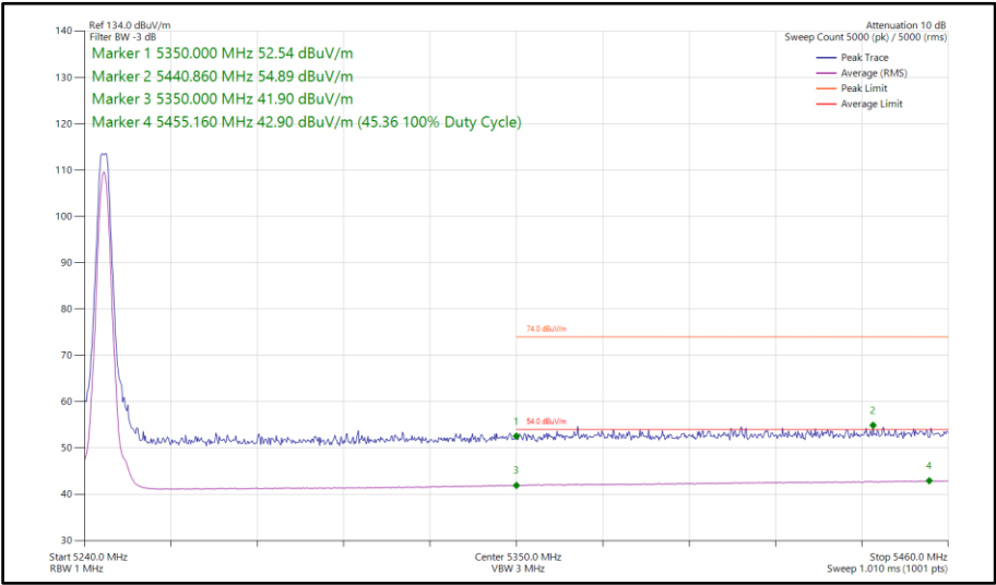
Figure 679 - LE2M, MIMO, Core 0-1 - 5245 MHz Band Edge Frequency 5350 MHz
