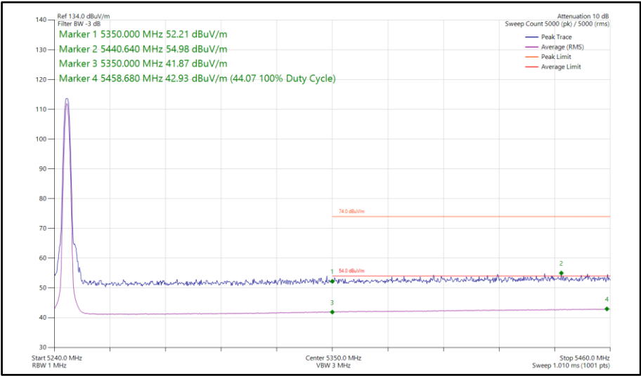
Figure 675 - DH5, MIMO, Core 0-1 - 5245 MHzBand Edge Frequency 5350 MHz
