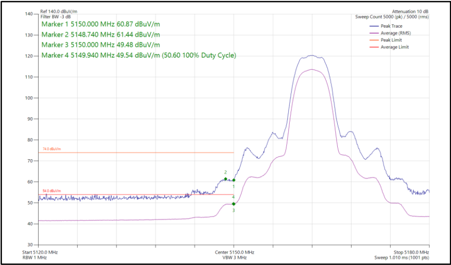
Figure 691 - HDR8, SISO, Core 0 - 5162 MHz Band Edge Frequency 5150 MHz
