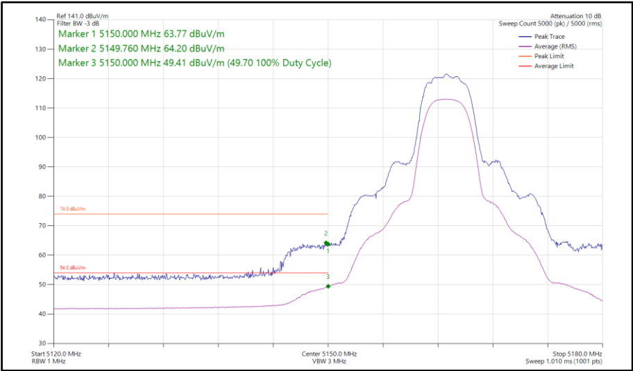
Figure 698 - HDRPM12, SISO, Core 0 - 5163 MHz Band Edge Frequency 5150 MHz
