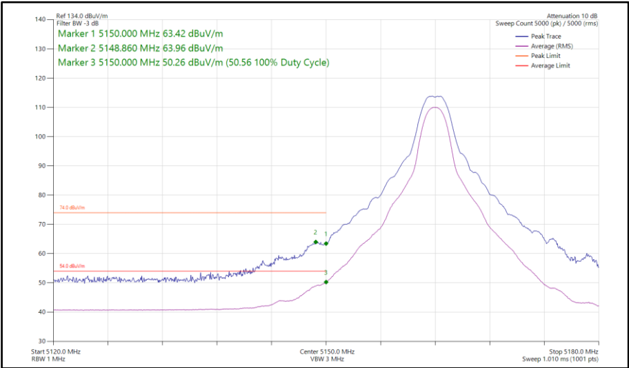
Figure 667 - HDT4, MIMO, Core 0-1 - 5162 MHz Band Edge Frequency 5150 MHz
