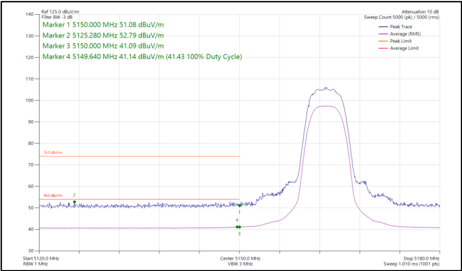
Figure 642 - HDRPM12, SISO, Core 1 - 5163 MHz Band Edge Frequency 5150 MHz
