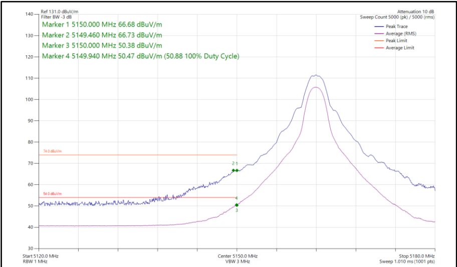
Figure 640 - HDT6, SISO, Core 1 - 5162 MHz Band Edge Frequency 5150 MHz
