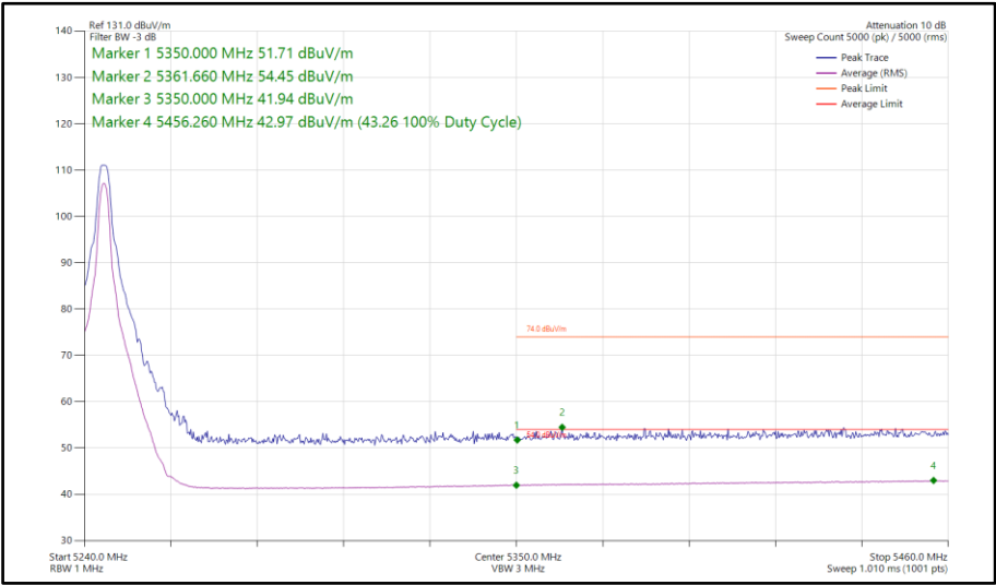
Figure 653 - HDT4, SISO, Core 1 - 5245 MHz Band Edge Frequency 5350 MHz
