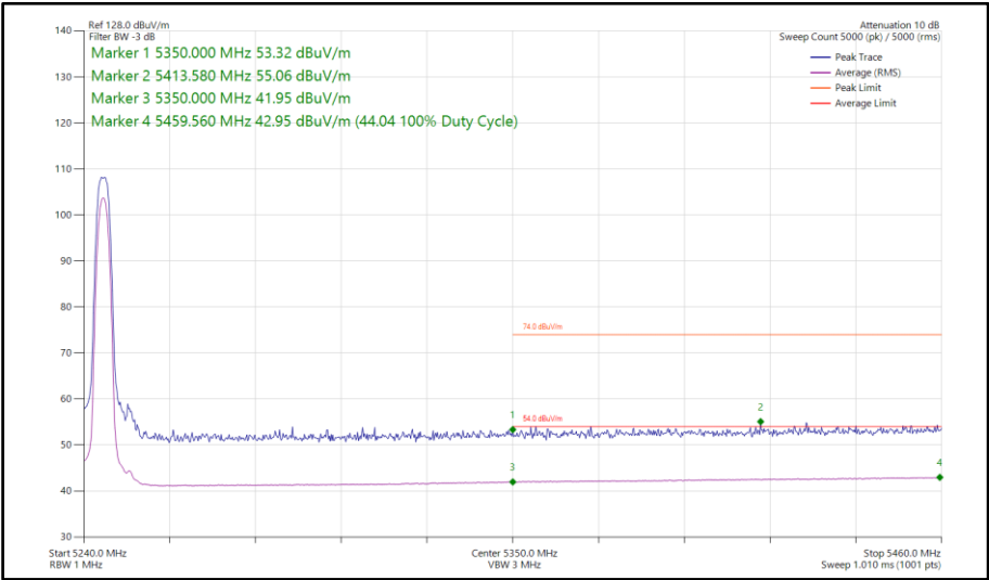
Figure 648 - HDR4, SISO, Core 1 - 5245 MHz Band Edge Frequency 5350 MHz
