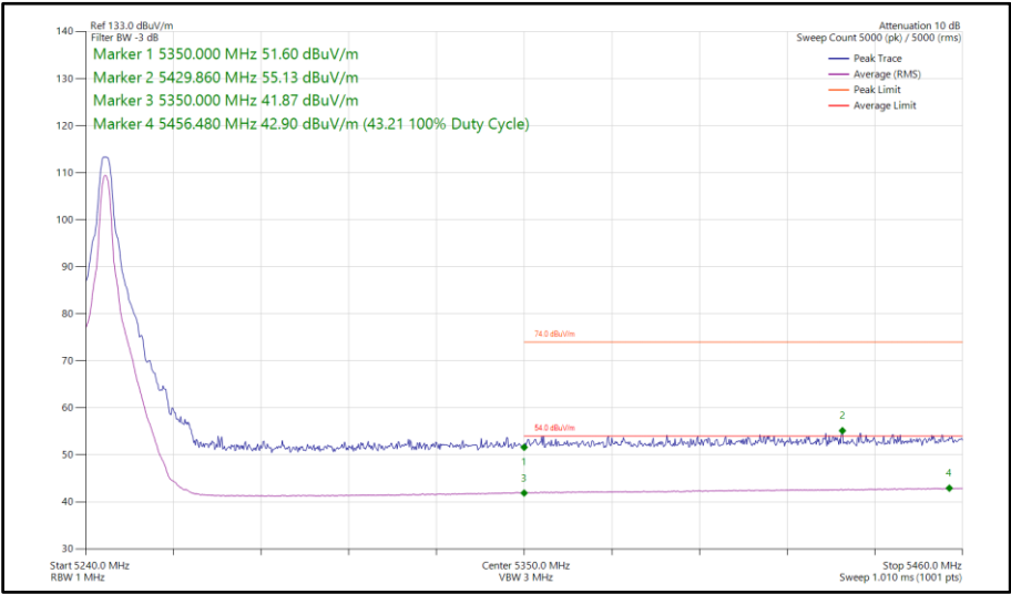
Figure 681 - HDT4, MIMO, Core 0-1 - 5245 MHz Band Edge Frequency 5350 MHz
