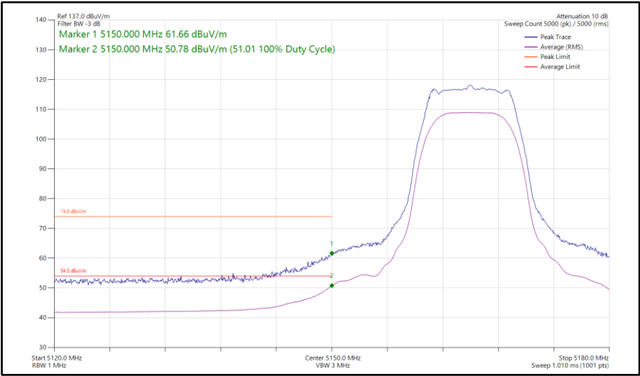
Figure 699 - HDRPL8, SISO, Core 0 - 5165 MHzBand Edge Frequency 5150 MHz
