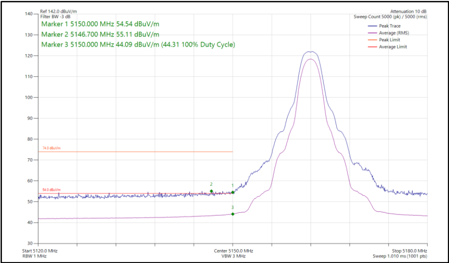
Figure 694 - HDT3, SISO, Core 0 - 5162 MHzBand Edge Frequency 5150 MHz
