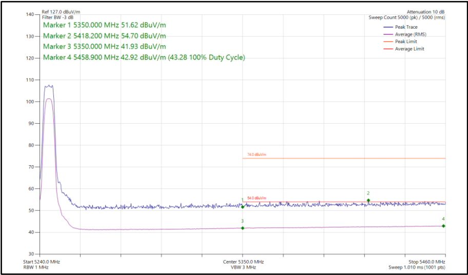
Figure 659 - XHDRPM8, SISO, Core 1 - 5245 MHz Band Edge Frequency 5350 MHz
