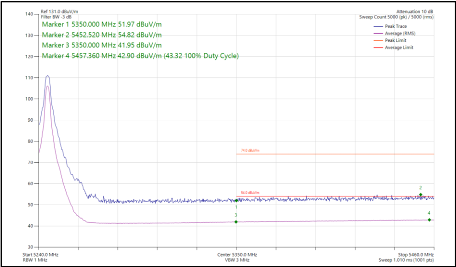
Figure 654 - HDT6, SISO, Core 1 - 5245 MHz Band Edge Frequency 5350 MHz
