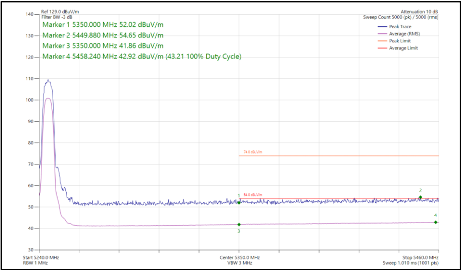
Figure 684 - HDRPM12, MIMO, Core 0-1 - 5245 MHzBand Edge Frequency 5350 MHz
