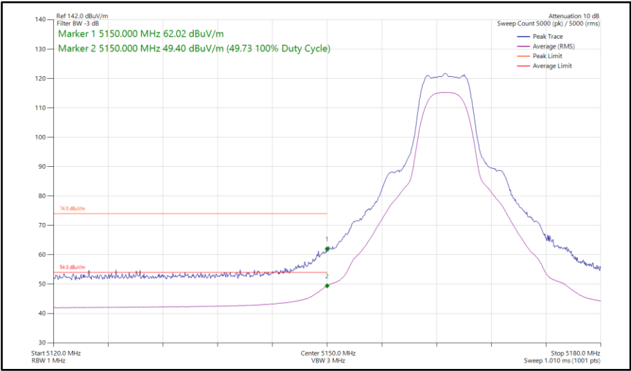
Figure 701 - XHDRPM8, SISO, Core 0 - 5163 MHz Band Edge Frequency 5150 MHz
