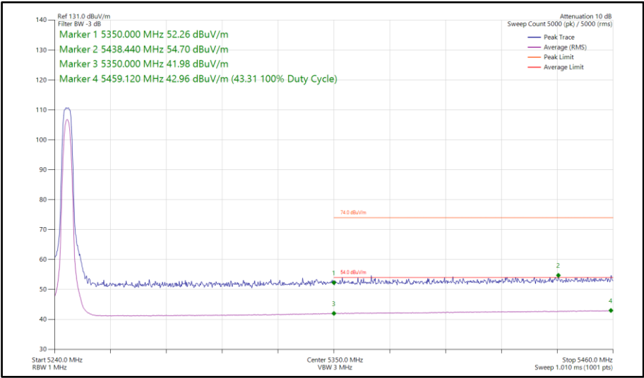
Figure 683 - HDRPS2, MIMO, Core 0-1 - 5245 MHzBand Edge Frequency 5350 MHz
