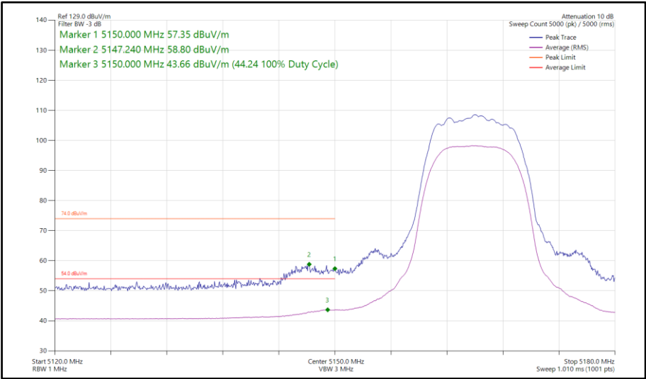
Figure 672 - HDRPL24, MIMO, Core 0-1 - 5165 MHzBand Edge Frequency 5150 MHz
