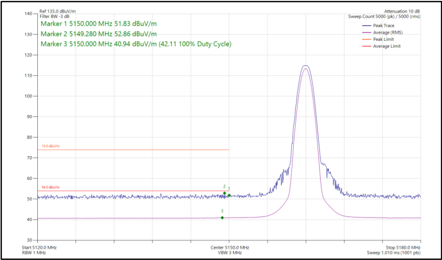
Figure 661 - DH5, MIMO, Core 0-1 - 5162 MHzBand Edge Frequency 5150 MHz
