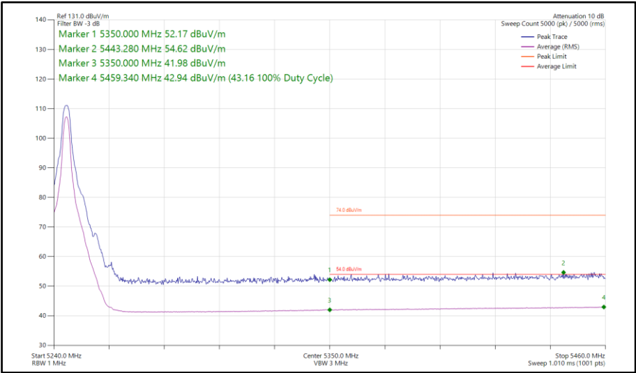
Figure 652 - HDT3, SISO, Core 1 - 5245 MHz Band Edge Frequency 5350 MHz
