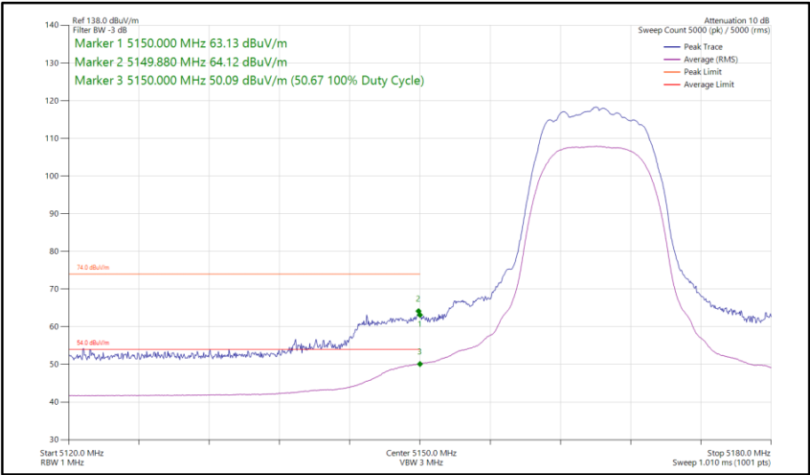
Figure 700 - HDRPL24, SISO, Core 0 - 5165 MHzBand Edge Frequency 5150 MHz
