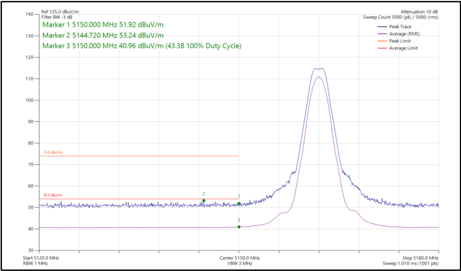
Figure 665 - LE2M, MIMO, Core 0-1 - 5162 MHzBand Edge Frequency 5150 MHz
