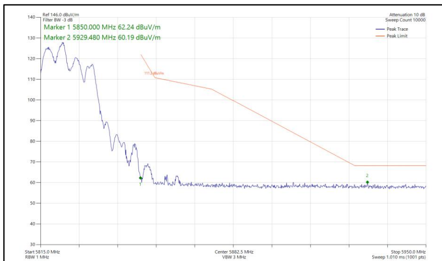
Figure 813 - 802.11ax HE20, RU 106-53, SDM, Core 0-1 - 5825 MHz Band Edge Frequency 5850 MHz
