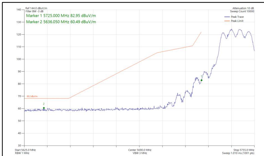
Figure 756 - 802.11n HT20, CDD, Core 0-1 - 5745 MHz Band Edge Frequency 5725 MHz
