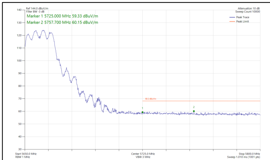
Figure 760 - 802.11a, CDD, Core 0-1 - 5660 MHz Band Edge Frequency 5725 MHz
