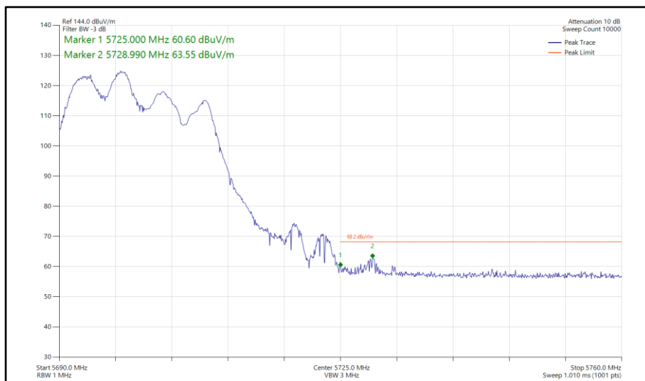
Figure 771 - 802.11ax HE20, RU 106-53, CDD, Core 0-1 - 5700 MHz Band Edge Frequency 5725 MHz
