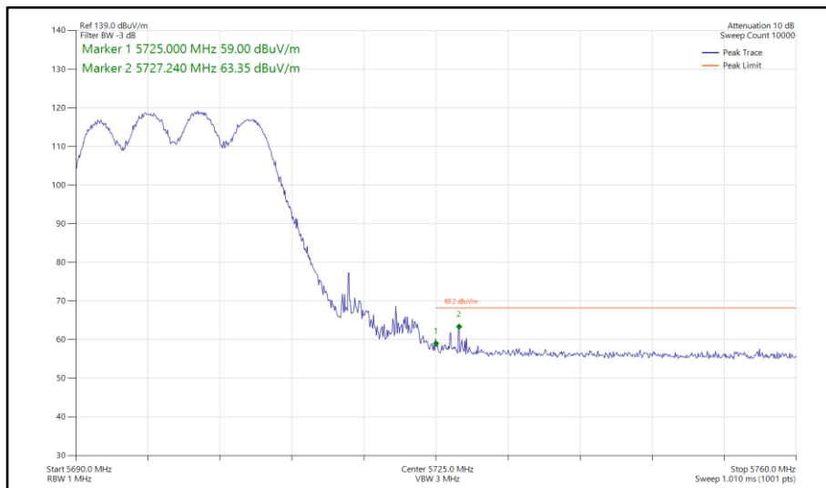
Figure 829 - 802.11ax HE20, SU, TxBF, Core 0-1 - 5700 MHz Band Edge Frequency 5725 MHz
