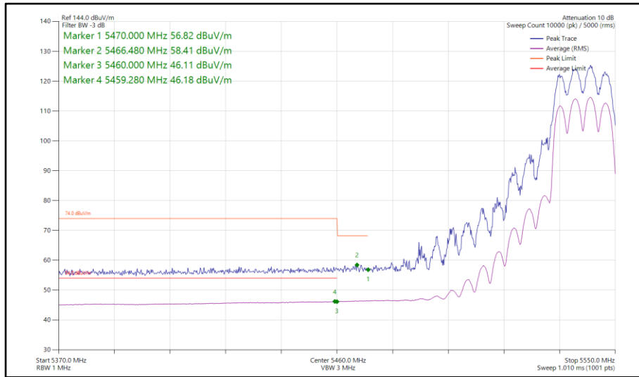
Figure 821 - 802.11ax HE20, SU, TxBF, Core 0-1 - 5540 MHz Band Edge Frequency 5470 MHz
