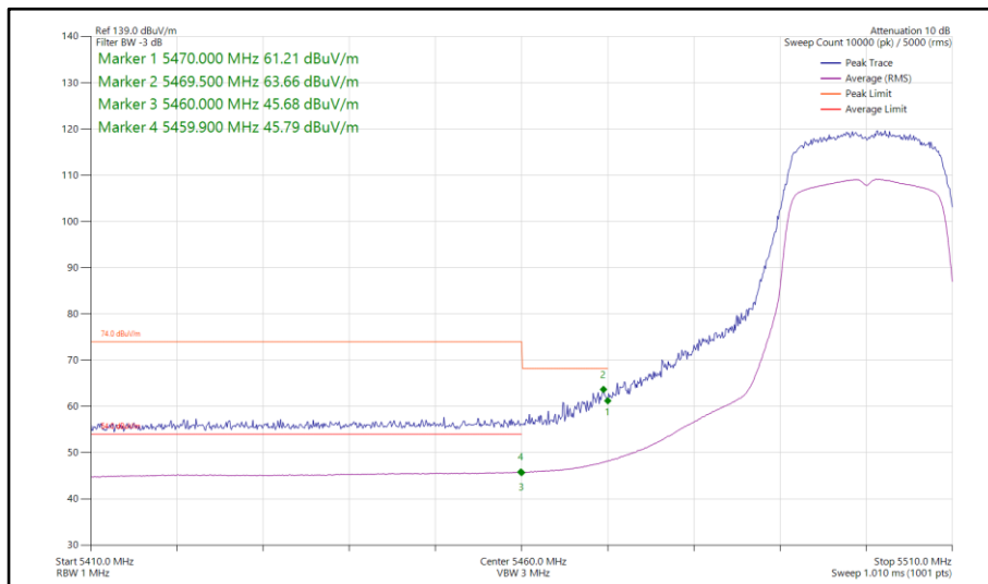
Figure 784 - 802.11n HT20, SDM, Core 0-1 - 5500 MHz Band Edge Frequency 5470 MHz
