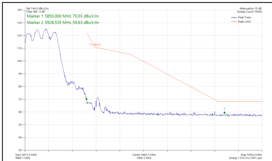
Figure 780 - 802.11ax HE20, SU, CDD, Core 0-1 - 5825 MHz Band Edge Frequency 5850 MHz
