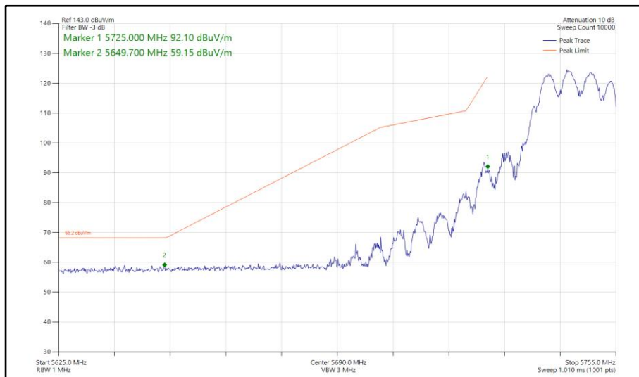
Figure 823 - 802.11ax HE20, SU, TxBF, Core 0-1 - 5745 MHz Band Edge Frequency 5725 MHz
