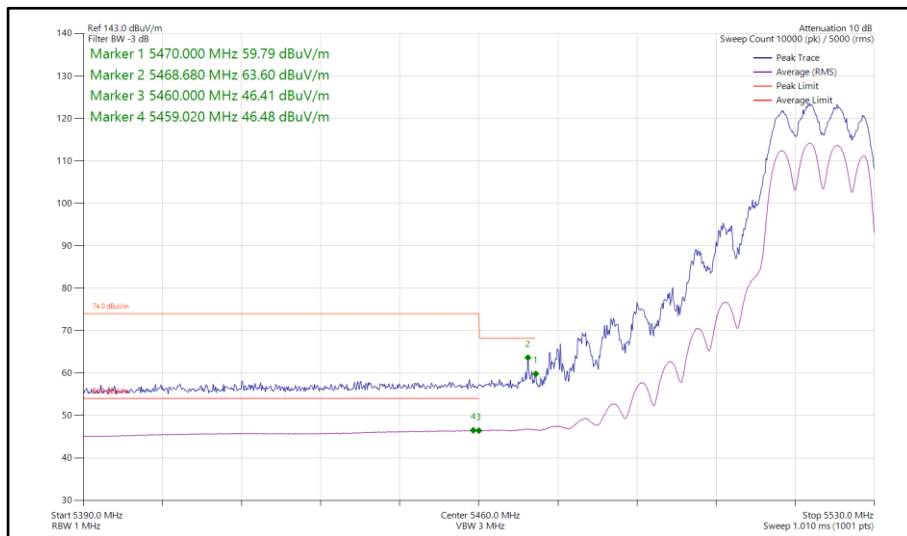
Figure 817 - 802.11ac VHT20, TxBF, Core 0-1 - 5520 MHz Band Edge Frequency 5470 MHz
