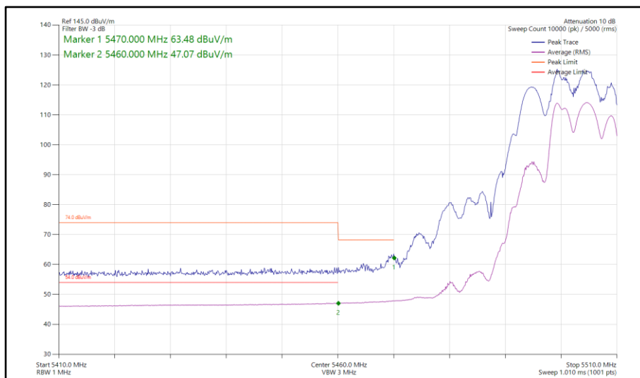
Figure 753 - 802.11be EHT20, RU 106+26-83, CDD, Core 0-1 - 5500 MHz Band Edge Frequency 5470 MHz
