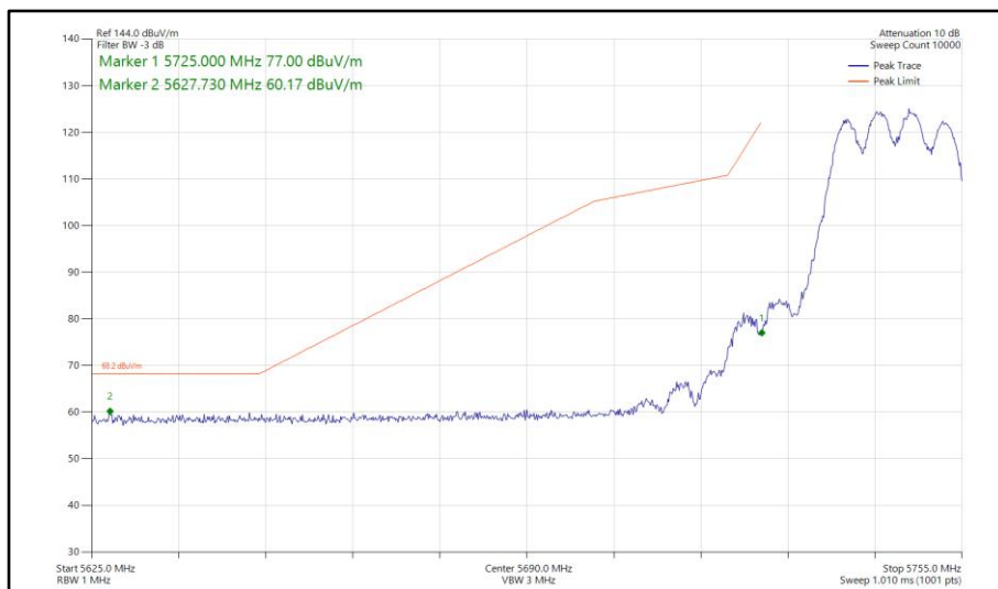
Figure 757 - 802.11ax HE20, SU, CDD, Core 0-1 - 5745 MHz Band Edge Frequency 5725 MHz
