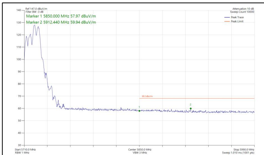
Figure 779 - 802.11ax HE20, RU 106-54, CDD, Core 0-1 - 5720 MHz Band Edge Frequency 5850 MHz
