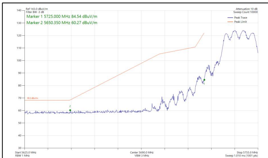
Figure 822 - 802.11ac VHT20, TxBF, Core 0-1 - 5745 MHz Band Edge Frequency 5725 MHz
