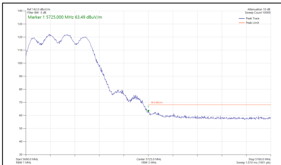
Figure 826 - 802.11ac VHT20, TxBF, Core 0-1 - 5700 MHz Band Edge Frequency 5725 MHz
