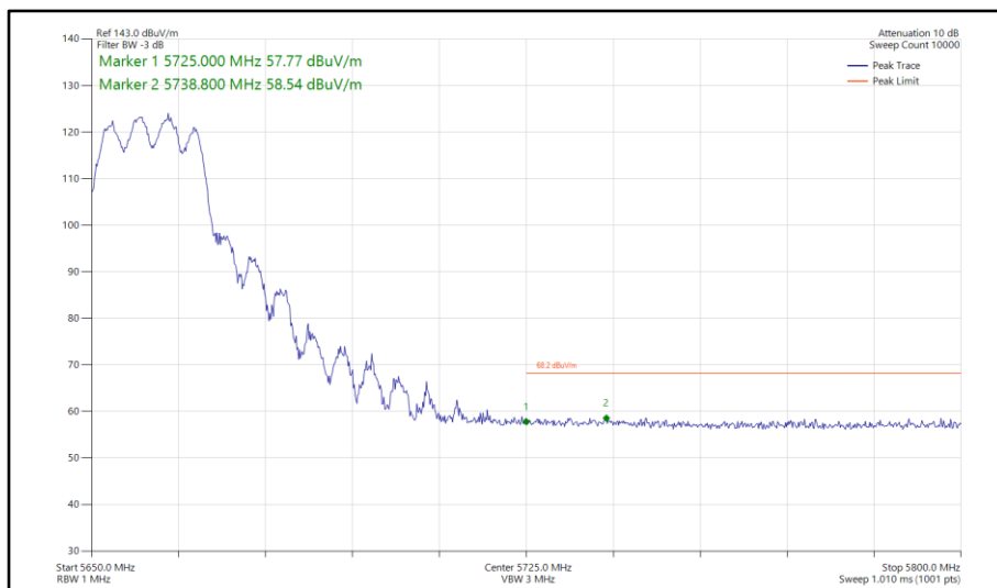
Figure 824 - 802.11ac VHT20, TxBF, Core 0-1 - 5660 MHz Band Edge Frequency 5725 MHz
