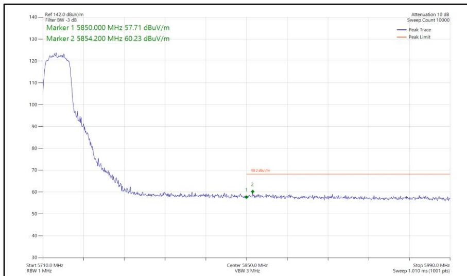
Figure 808 - 802.11n HT20, SDM, Core 0-1 - 5720 MHz Band Edge Frequency 5850 MHz
