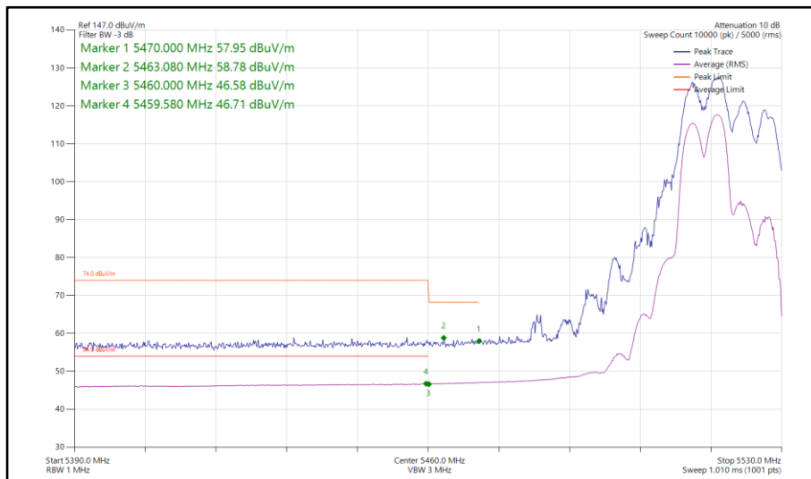
Figure 750 - 802.11ax HE20, RU 106-53, CDD, Core 0-1 - 5520 MHz Band Edge Frequency 5470 MHz
