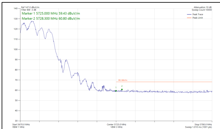
Figure 769 - 802.11ax HE20, RU 106-53, CDD, Core 0-1 - 5680 MHz Band Edge Frequency 5725 MHz
