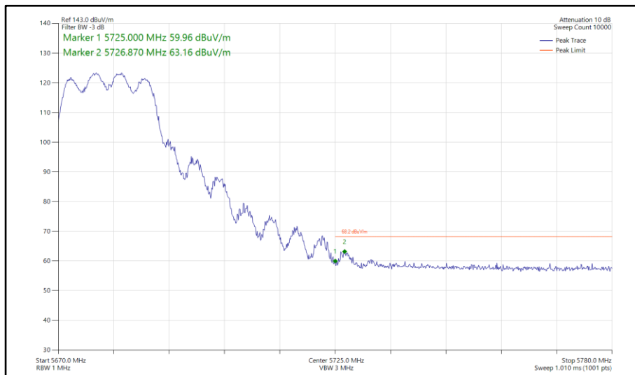
Figure 764 - 802.11n HT20, CDD, Core 0-1 - 5680 MHz Band Edge Frequency 5725 MHz
