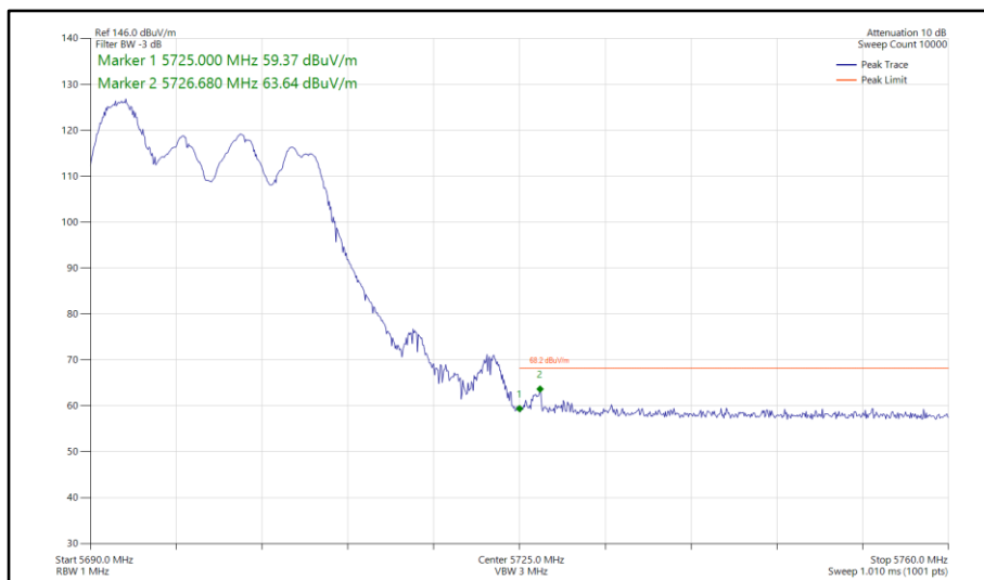
Figure 805 - 802.11ax HE20, RU 52-37, SDM, Core 0-1 - 5700 MHz Band Edge Frequency 5725 MHz
