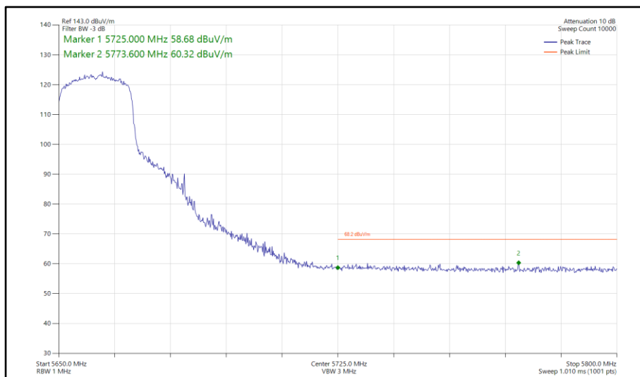
Figure 801 - 802.11ax HE20, SU, SDM, Core 0-1 - 5660 MHz Band Edge Frequency 5725 MHz
