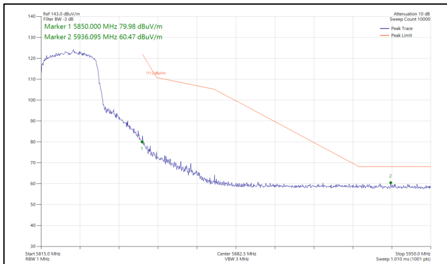
Figure 812 - 802.11ax HE20, SU, SDM, Core 0-1 - 5825 MHz Band Edge Frequency 5850 MHz
