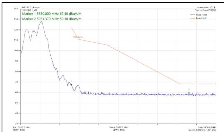
Figure 815 - 802.11be EHT20, RU 52+26-72, SDM, Core 0-1 - 5825 MHz Band Edge Frequency 5850 MHz
