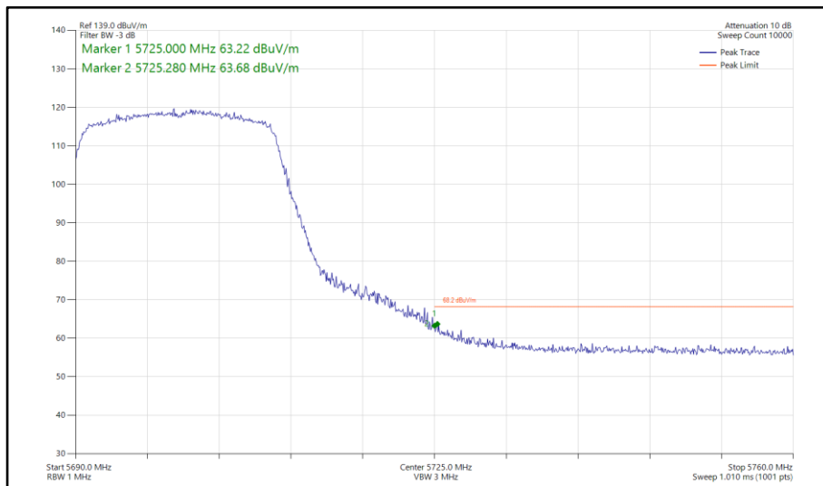
Figure 804 - 802.11ax HE20, SU, SDM, Core 0-1 - 5700 MHz Band Edge Frequency 5725 MHz
