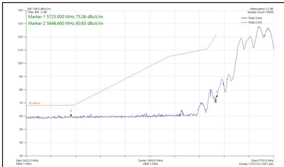
Figure 796 - 802.11ax HE20, RU 106-54, SDM, Core 0-1 - 5745 MHz Band Edge Frequency 5725 MHz
