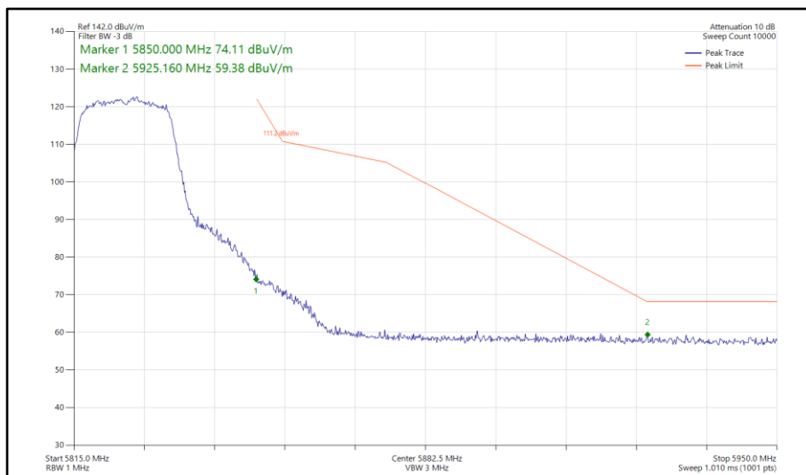
Figure 809 - 802.11n HT20, SDM, Core 0-1 - 5825 MHz Band Edge Frequency 5850 MHz
