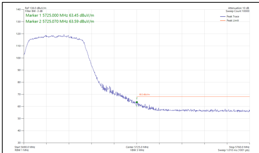
Figure 800 - 802.11n HT20, SDM, Core 0-1 - 5700 MHz Band Edge Frequency 5725 MHz
