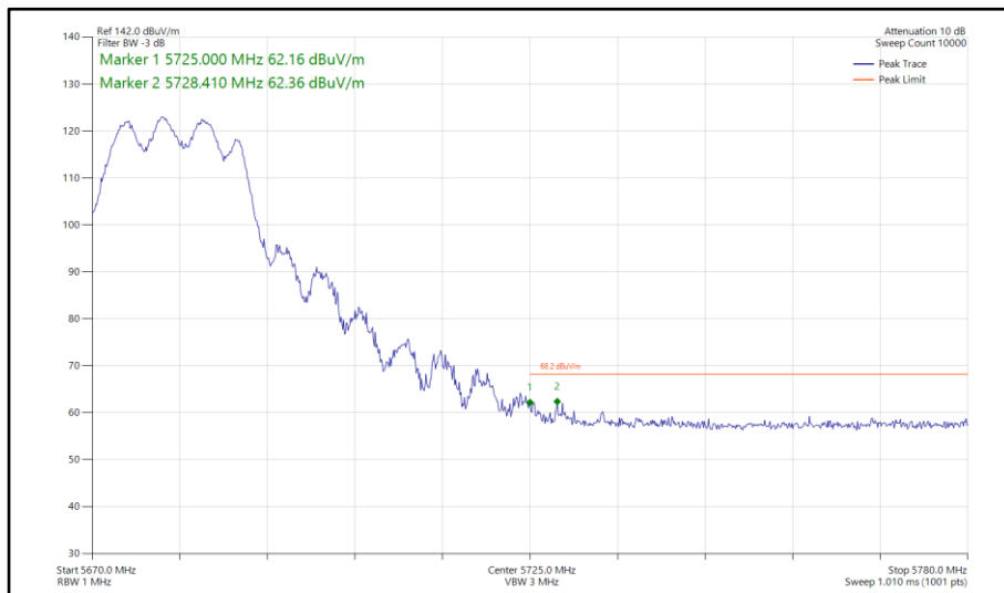
Figure 825 - 802.11ac VHT20, TxBF, Core 0-1 - 5680 MHz Band Edge Frequency 5725 MHz
