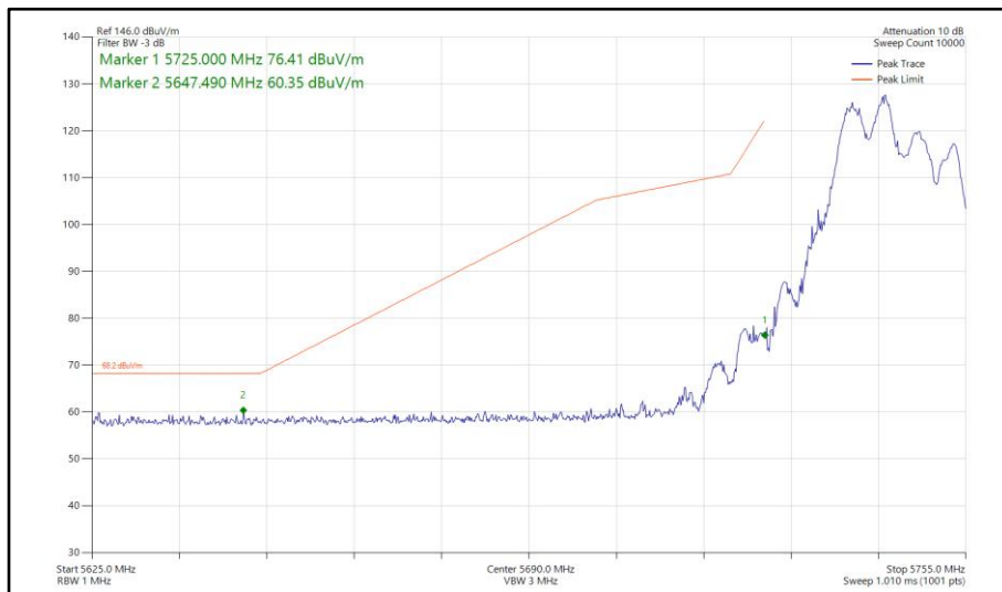
Figure 758 - 802.11ax HE20, RU 106-53, CDD, Core 0-1 - 5745 MHz Band Edge Frequency 5725 MHz
