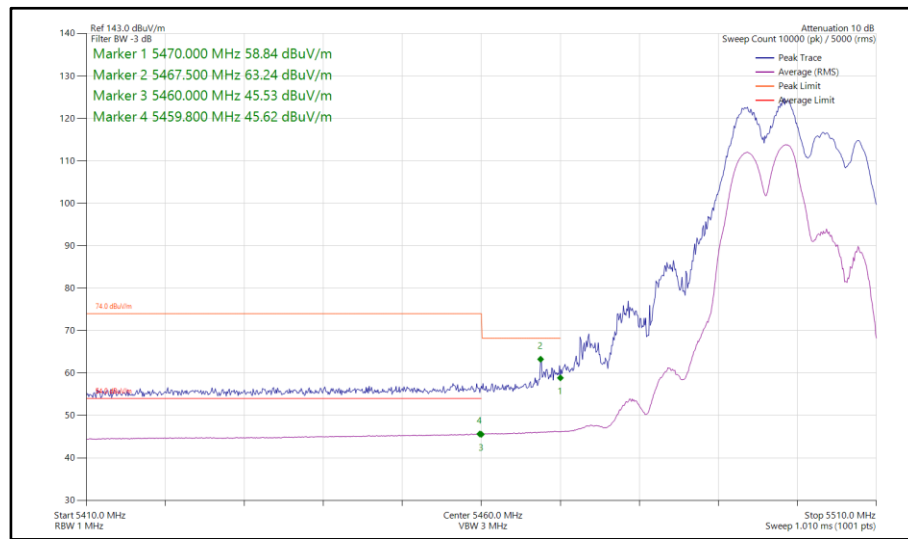
Figure 792 - 802.11be EHT20, RU 106+26-82, SDM, Core 0-1 - 5500 MHz Band Edge Frequency 5470 MHz
