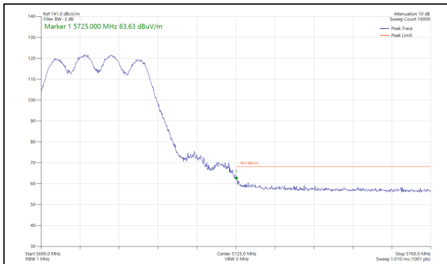
Figure 770 - 802.11ax HE20, SU, CDD, Core 0-1 - 5700 MHz Band Edge Frequency 5725 MHz
