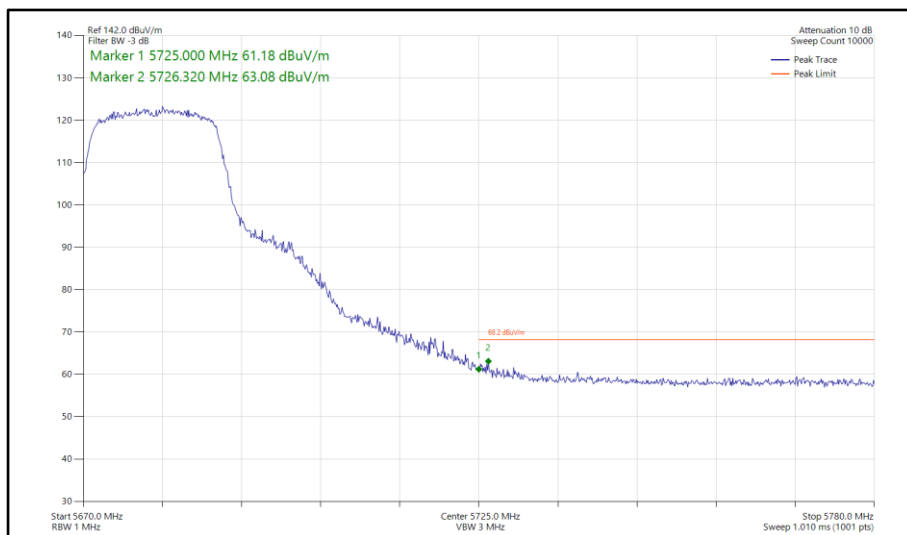
Figure 799 - 802.11n HT20, SDM, Core 0-1 - 5680 MHz Band Edge Frequency 5725 MHz
