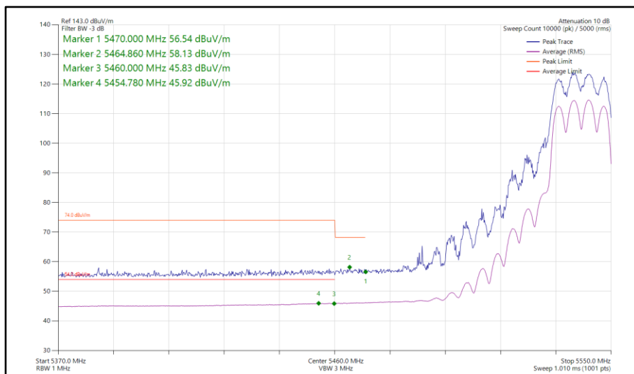
Figure 818 - 802.11ac VHT20, TxBF, Core 0-1 - 5540 MHz Band Edge Frequency 5470 MHz
