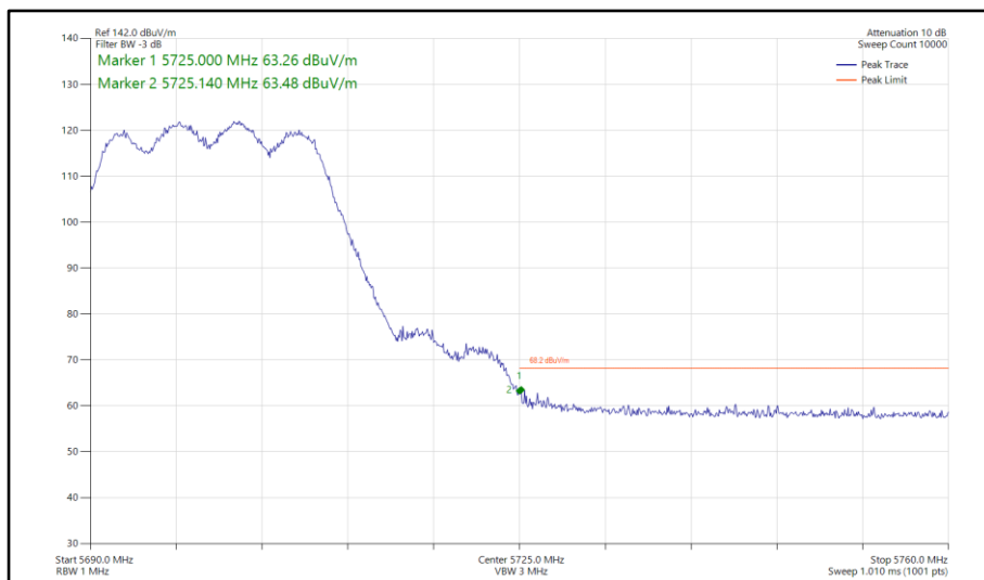
Figure 765 - 802.11n HT20, CDD, Core 0-1 - 5700 MHz Band Edge Frequency 5725 MHz
