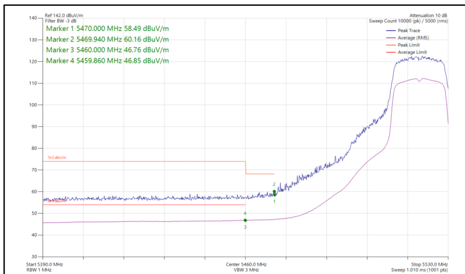
Figure 785 - 802.11n HT20, SDM, Core 0-1 - 5520 MHz Band Edge Frequency 5470 MHz
