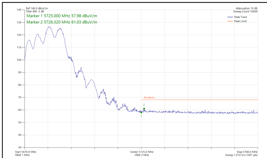
Figure 772 - 802.11be EHT20, RU 106+26-83, CDD, Core 0-1 - 5680 MHz Band Edge Frequency 5725 MHz
