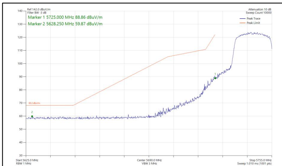
Figure 795 - 802.11ax HE20, SU, SDM, Core 0-1 - 5745 MHz Band Edge Frequency 5725 MHz
