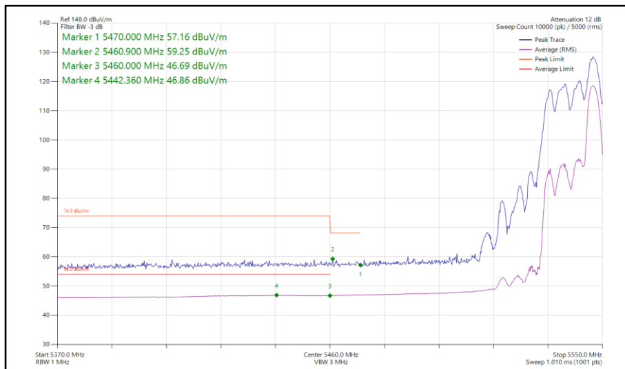
Figure 752 - 802.11ax HE20, RU 52-40, CDD, Core 0-1 - 5540 MHz Band Edge Frequency 5470 MHz
