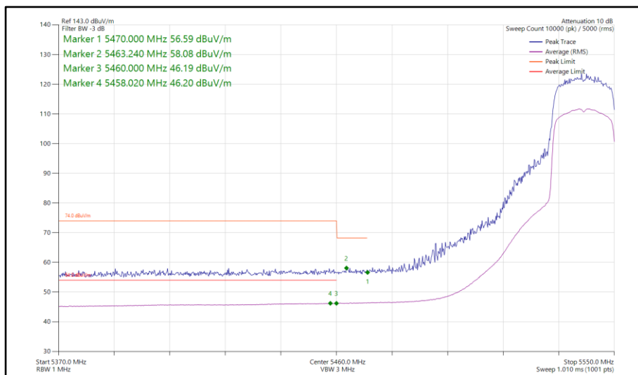
Figure 791 - 802.11ax HE20, SU, SDM, Core 0-1 - 5540 MHz Band Edge Frequency 5470 MHz
