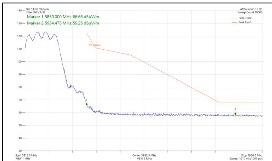
Figure 775 - 802.11a, CDD, Core 0-1 - 5825 MHz Band Edge Frequency 5850 MHz
