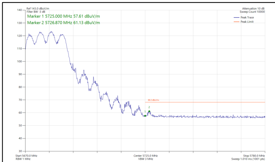
Figure 768 - 802.11ax HE20, SU, CDD, Core 0-1 - 5680 MHz Band Edge Frequency 5725 MHz
