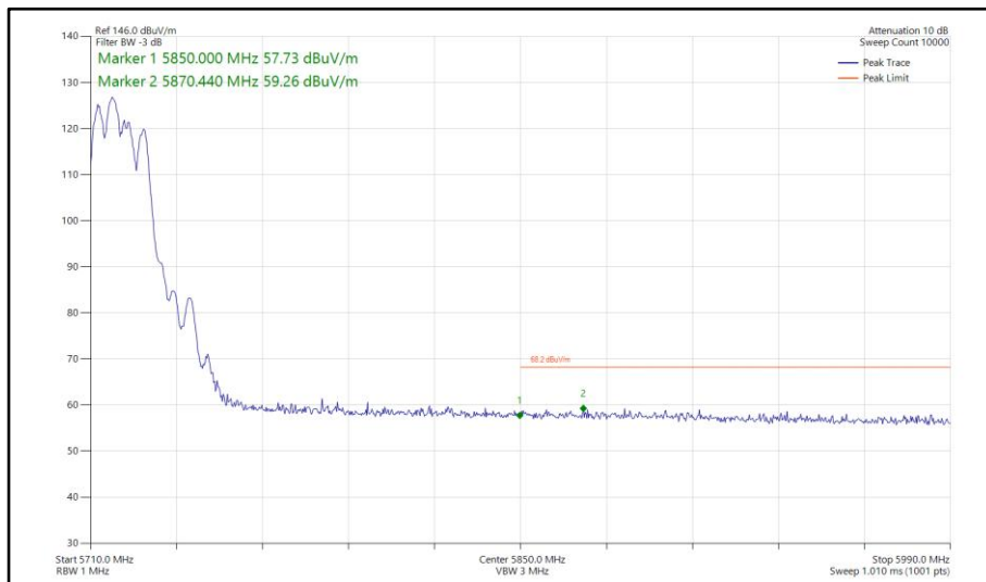
Figure 782 - 802.11be EHT20, RU 106+26-82, CDD, Core 0-1 - 5720 MHz Band Edge Frequency 5850 MHz
