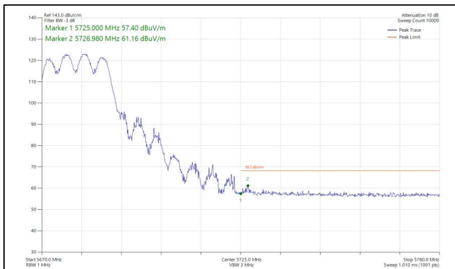
Figure 828 - 802.11ax HE20, SU, TxBF, Core 0-1 - 5680 MHz Band Edge Frequency 5725 MHz
