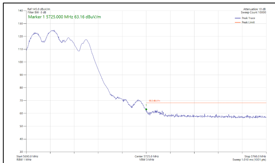
Figure 807 - 802.11be EHT20, RU 106+26-82, SDM, Core 0-1 - 5700 MHz Band Edge Frequency 5725 MHz
