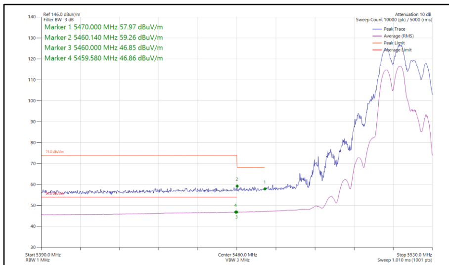
Figure 793 - 802.11be EHT20, RU 106+26-82, SDM, Core 0-1 - 5520 MHz Band Edge Frequency 5470 MHz
