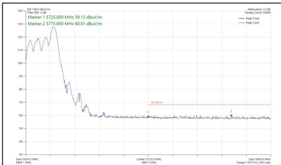
Figure 767 - 802.11ax HE20, RU 52-40, CDD, Core 0-1 - 5660 MHz Band Edge Frequency 5725 MHz
