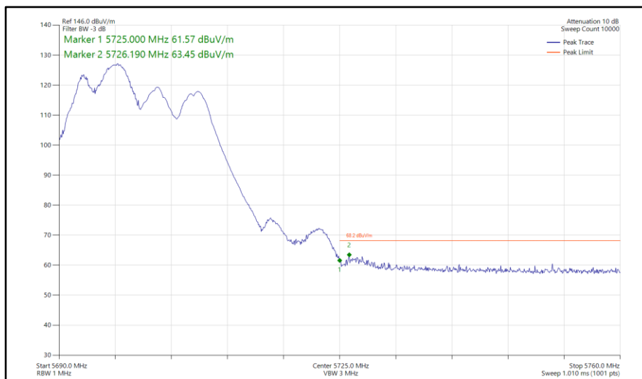
Figure 773 - 802.11be EHT20, RU 52+26-70 CDD, Core 0-1 - 5700 MHz Band Edge Frequency 5725 MHz
