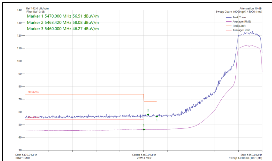
Figure 786 - 802.11n HT20, SDM, Core 0-1 - 5540 MHz Band Edge Frequency 5470 MHz
