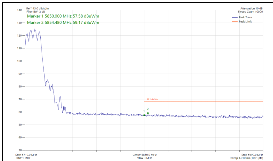
Figure 778 - 802.11ax HE20, SU, CDD, Core 0-1 - 5720 MHz Band Edge Frequency 5850 MHz
