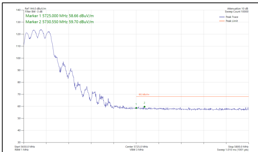
Figure 763 - 802.11n HT20, CDD, Core 0-1 - 5660 MHz Band Edge Frequency 5725 MHz
