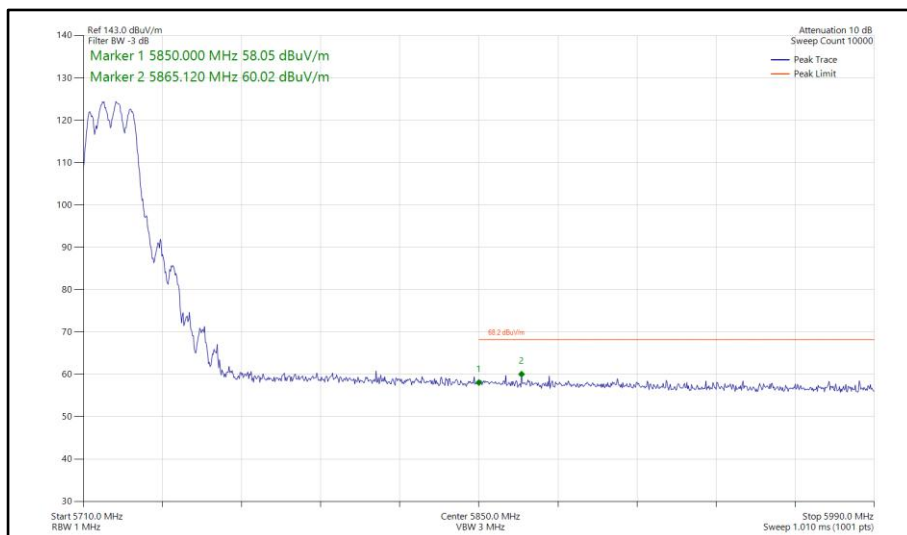
Figure 830 - 802.11ac VHT20, TxBF, Core 0-1 - 5720 MHz Band Edge Frequency 5850 MHz
