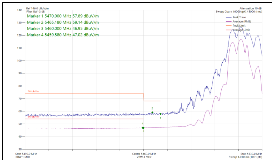
Figure 754 - 802.11be EHT20, RU 106+26-82, CDD, Core 0-1 - 5520 MHz Band Edge Frequency 5470 MHz
