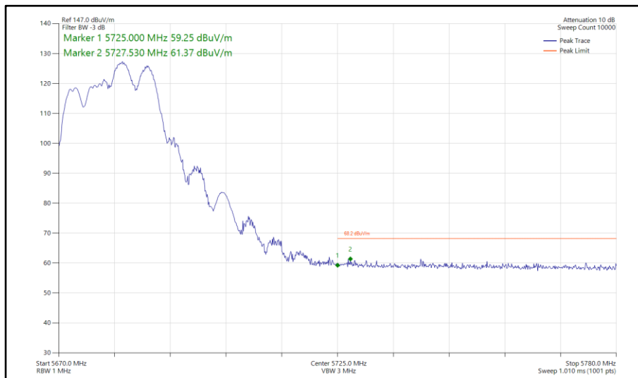
Figure 806 - 802.11be EHT20, RU 106+26-83, SDM, Core 0-1 - 5680 MHz Band Edge Frequency 5725 MHz
