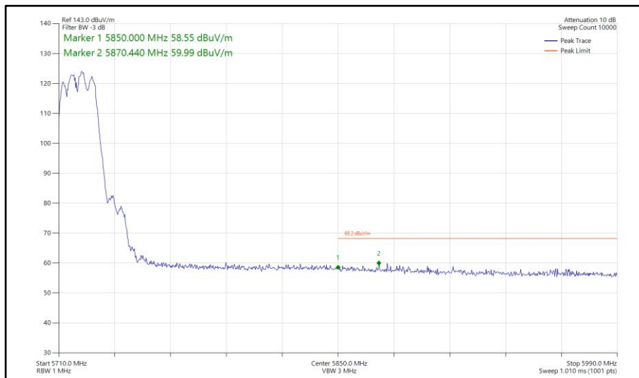
Figure 774 - 802.11a, CDD, Core 0-1 - 5720 MHz Band Edge Frequency 5850 MHz
