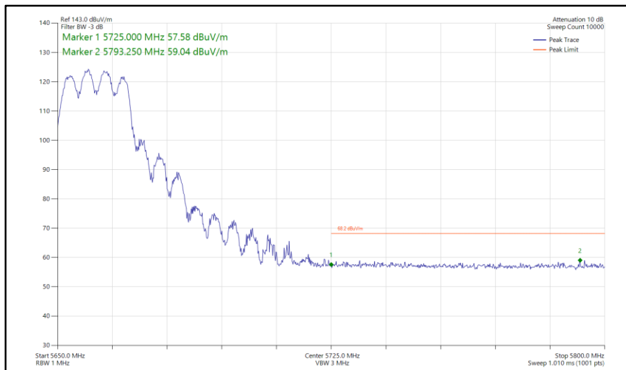
Figure 827 - 802.11ax HE20, SU, TxBF, Core 0-1 - 5660 MHz Band Edge Frequency 5725 MHz
