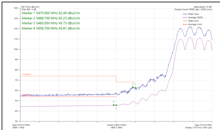
Figure 819 - 802.11ax HE20, SU, TxBF, Core 0-1 - 5500 MHz Band Edge Frequency 5470 MHz
