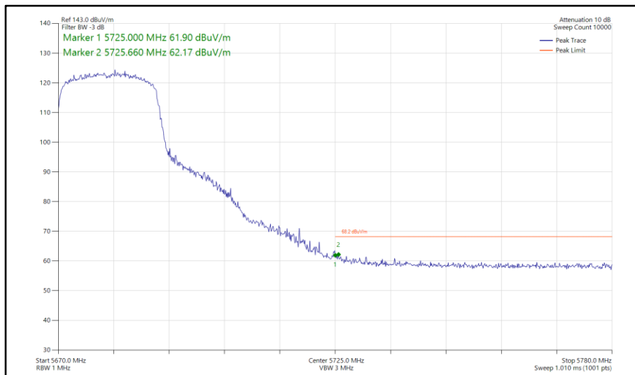
Figure 802 - 802.11ax HE20, SU, SDM, Core 0-1 - 5680 MHz Band Edge Frequency 5725 MHz
