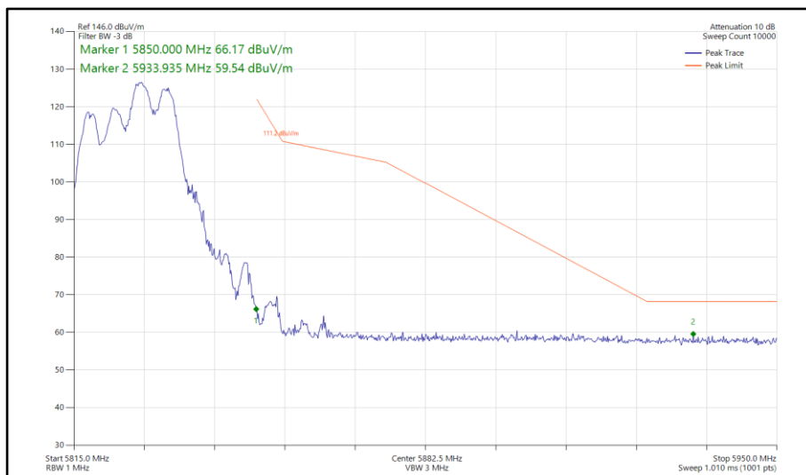
Figure 781 - 802.11ax HE20, RU 106-54, CDD, Core 0-1 - 5825 MHz Band Edge Frequency 5850 MHz
