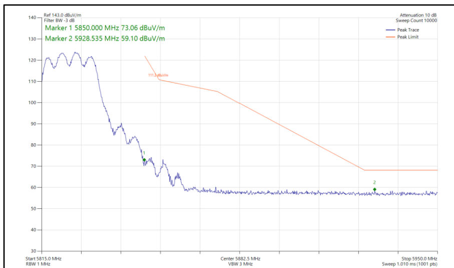
Figure 777 - 802.11n HT20, CDD, Core 0-1 - 5825 MHz Band Edge Frequency 5850 MHz
