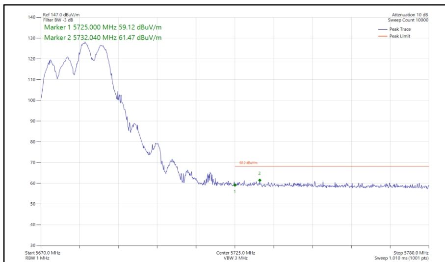
Figure 803 - 802.11ax HE20, RU 106-54, SDM, Core 0-1 - 5680 MHz Band Edge Frequency 5725 MHz
