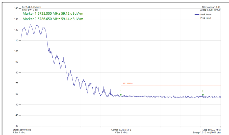
Figure 766 - 802.11ax HE20, SU, CDD, Core 0-1 - 5660 MHz Band Edge Frequency 5725 MHz
