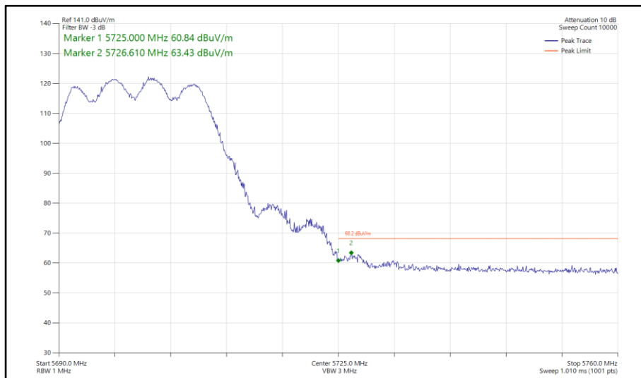
Figure 762 - 802.11a, CDD, Core 0-1 - 5700 MHz Band Edge Frequency 5725 MHz
