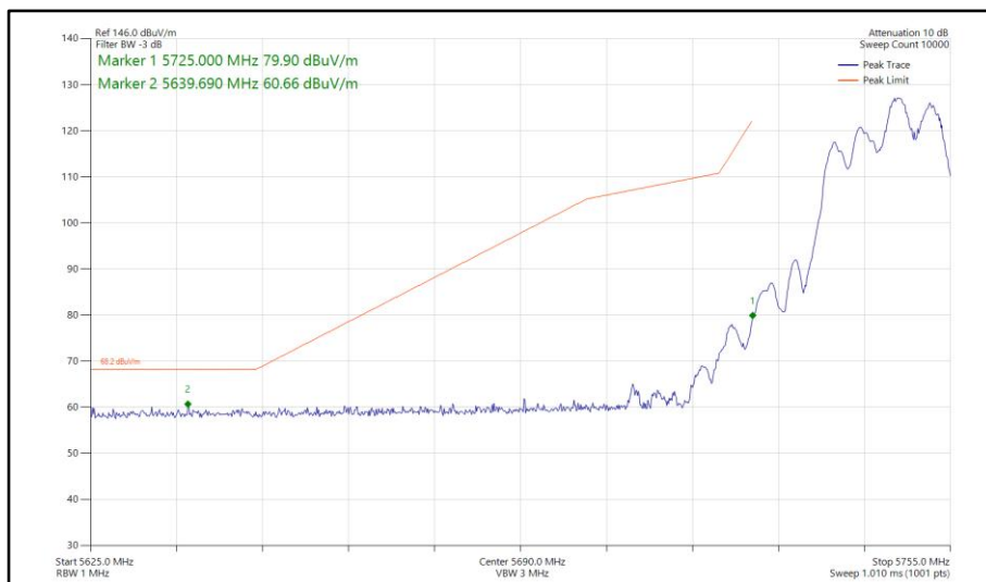
Figure 759 - 802.11be EHT20, RU 106+26-83, CDD, Core 0-1 - 5745 MHz Band Edge Frequency 5725 MHz
