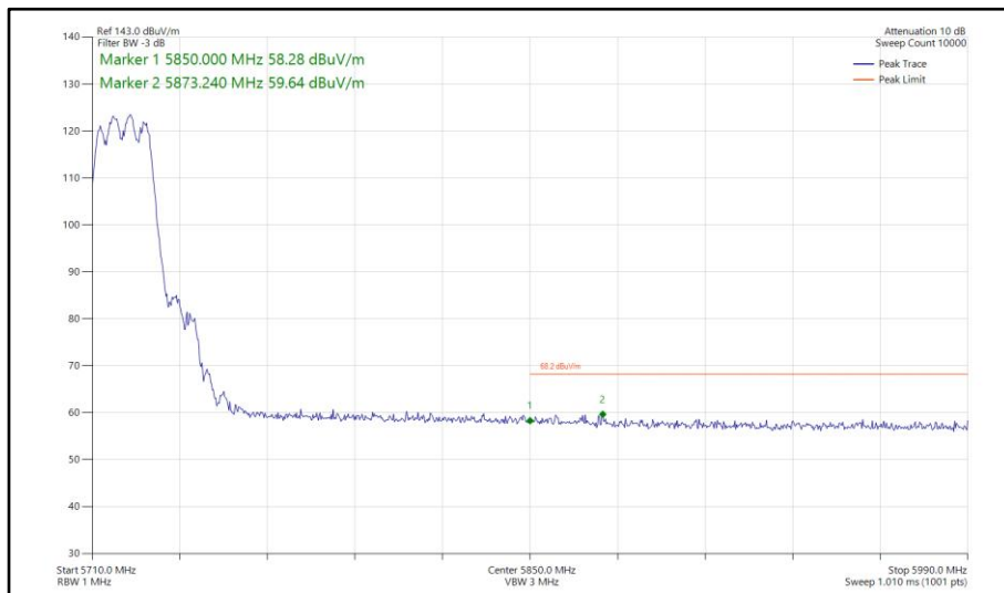
Figure 776 - 802.11n HT20, CDD, Core 0-1 - 5720 MHz Band Edge Frequency 5850 MHz
