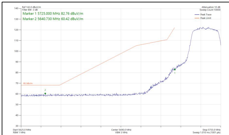
Figure 794 - 802.11n HT20, SDM, Core 0-1 - 5745 MHz Band Edge Frequency 5725 MHz
