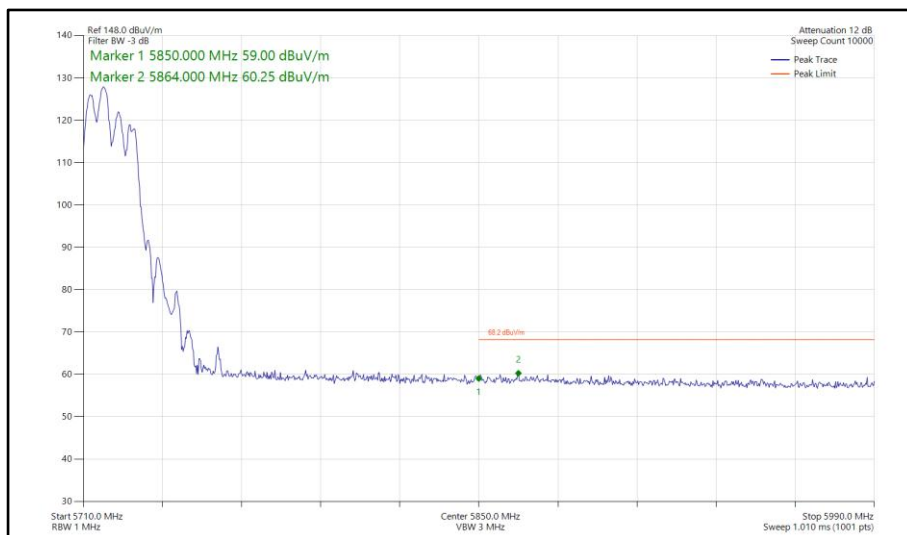
Figure 811 - 802.11ax HE20, RU 106-53, SDM, Core 0-1 - 5720 MHz Band Edge Frequency 5850 MHz
