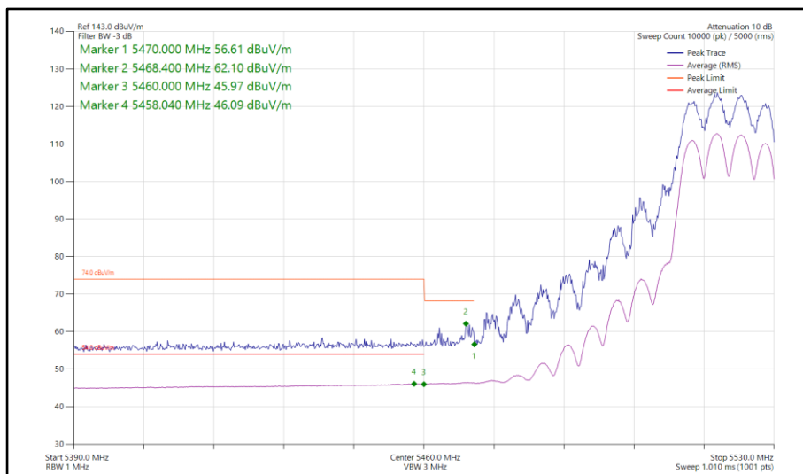
Figure 820 - 802.11ax HE20, SU, TxBF, Core 0-1 - 5520 MHz Band Edge Frequency 5470 MHz
