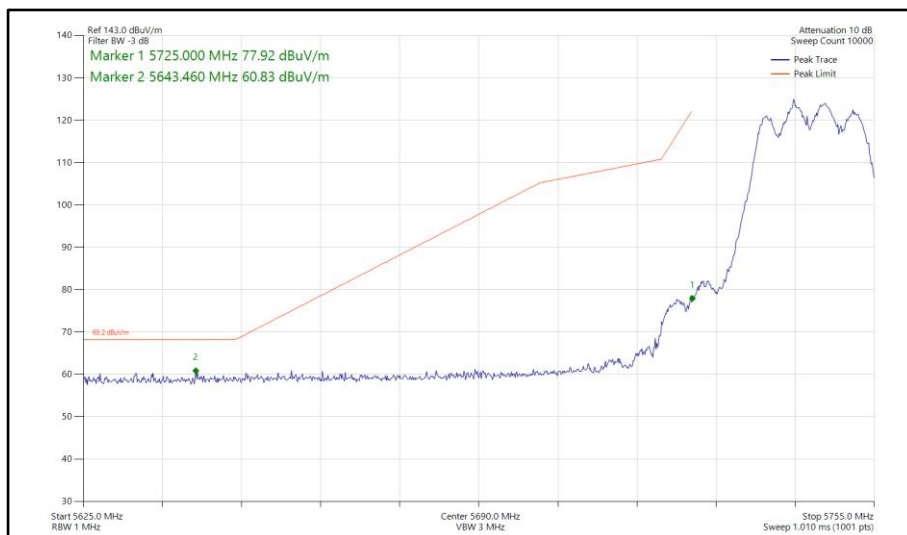
Figure 755 - 802.11a, CDD, Core 0-1 - 5745 MHz Band Edge Frequency 5725 MHz
