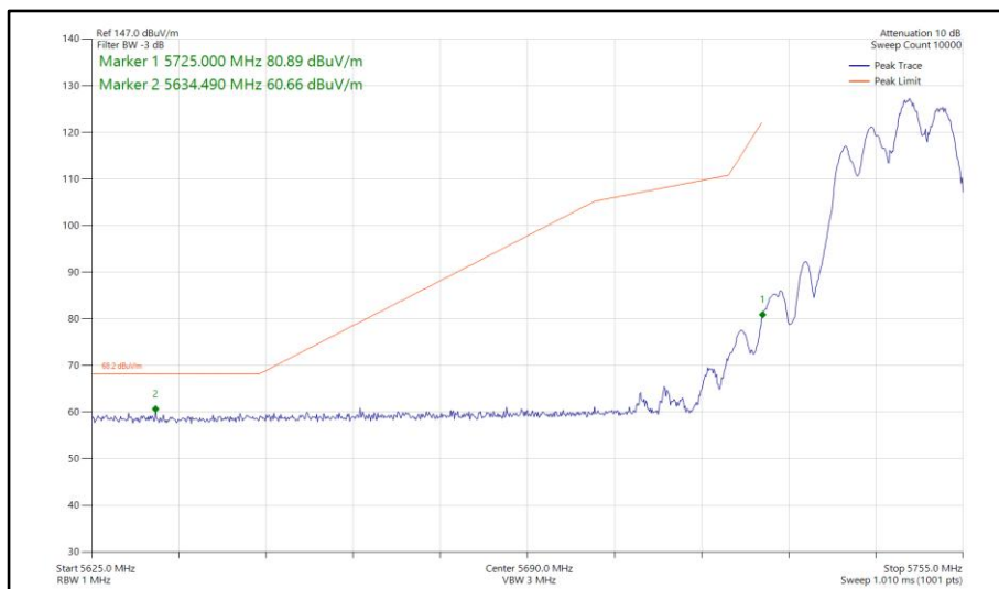
Figure 797 - 802.11be EHT20, RU 106+26-83, SDM, Core 0-1 - 5745 MHz Band Edge Frequency 5725 MHz
