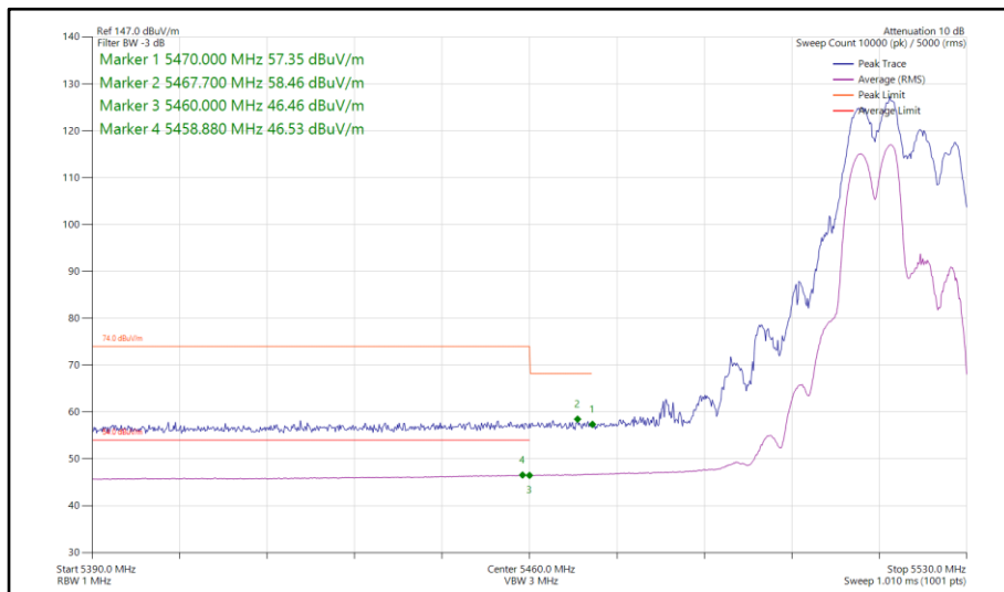
Figure 790 - 802.11ax HE20, RU 106-53, SDM, Core 0-1 - 5520 MHz Band Edge Frequency 5470 MHz
