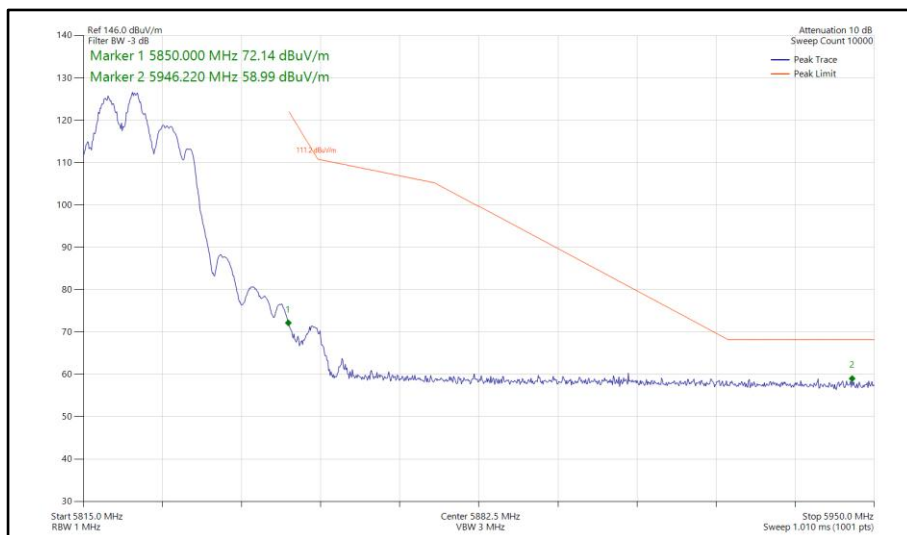
Figure 783 - 802.11be EHT20, RU 106+26-82, CDD, Core 0-1 - 5825 MHz Band Edge Frequency 5850 MHz
