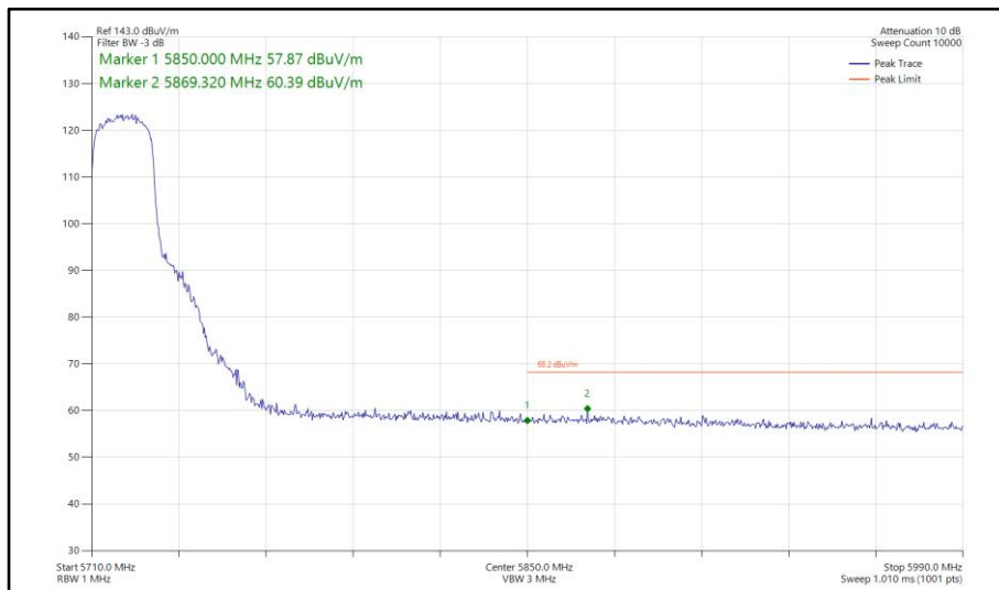
Figure 810 - 802.11ax HE20, SU, SDM, Core 0-1 - 5720 MHz Band Edge Frequency 5850 MHz
