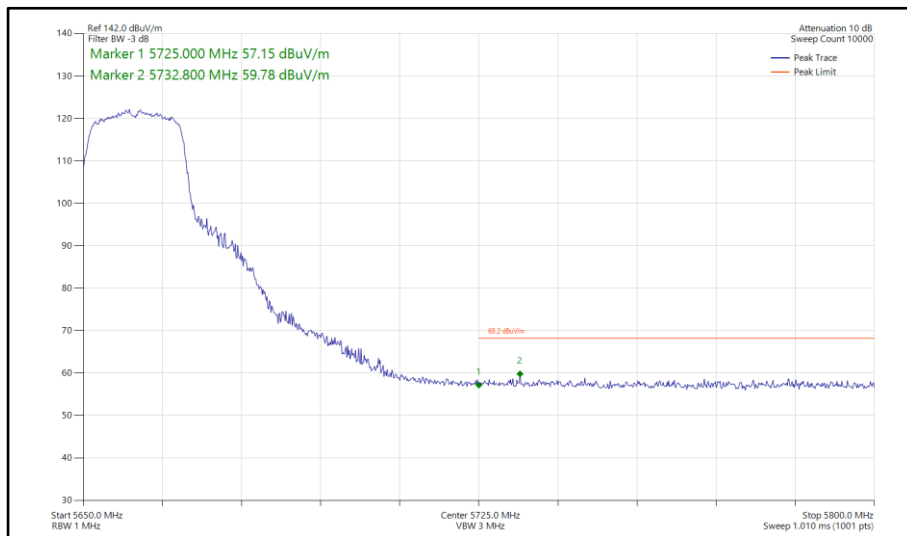
Figure 798 - 802.11n HT20, SDM, Core 0-1 - 5660 MHz Band Edge Frequency 5725 MHz
