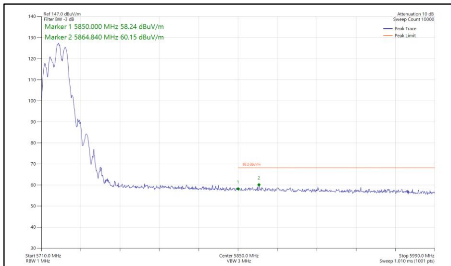
Figure 814 - 802.11be EHT20, RU 106+26-83, SDM, Core 0-1 - 5720 MHz Band Edge Frequency 5850 MHz
