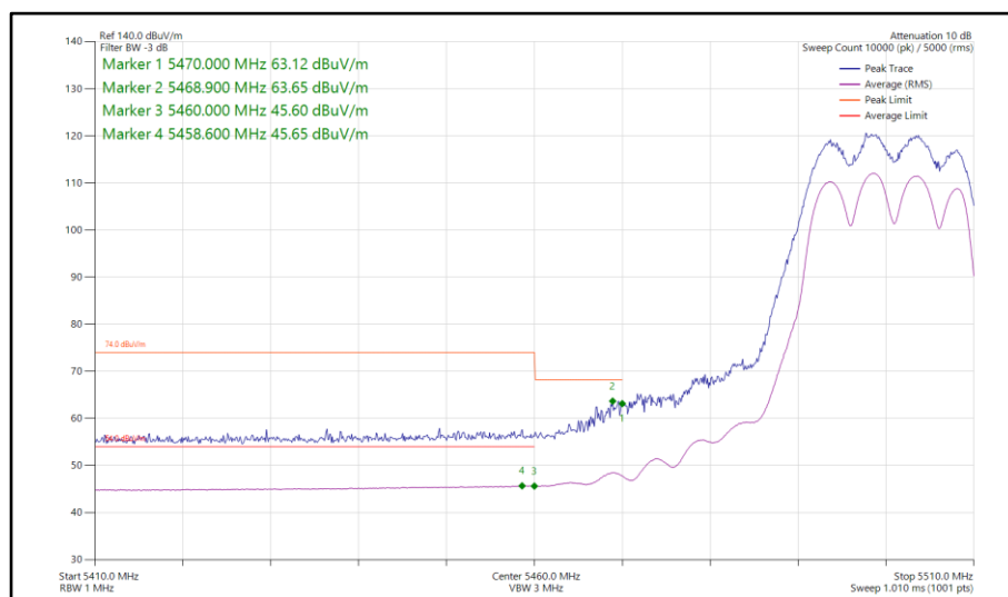
Figure 816 - 802.11ac VHT20, TxBF, Core 0-1 - 5500 MHz Band Edge Frequency 5470 MHz
