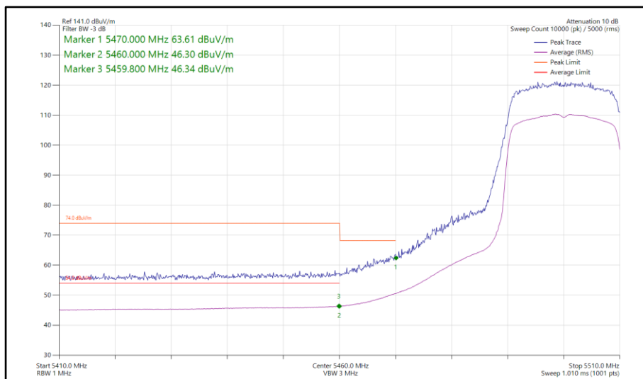
Figure 787 - 802.11ax HE20, SU, SDM, Core 0-1 - 5500 MHz Band Edge Frequency 5470 MHz
