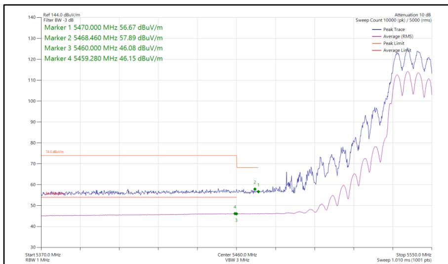
Figure 751 - 802.11ax HE20, SU, CDD, Core 0-1 - 5540 MHz Band Edge Frequency 5470 MHz
