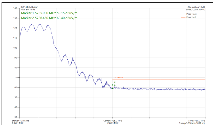
Figure 761 - 802.11a, CDD, Core 0-1 - 5680 MHz Band Edge Frequency 5725 MHz
