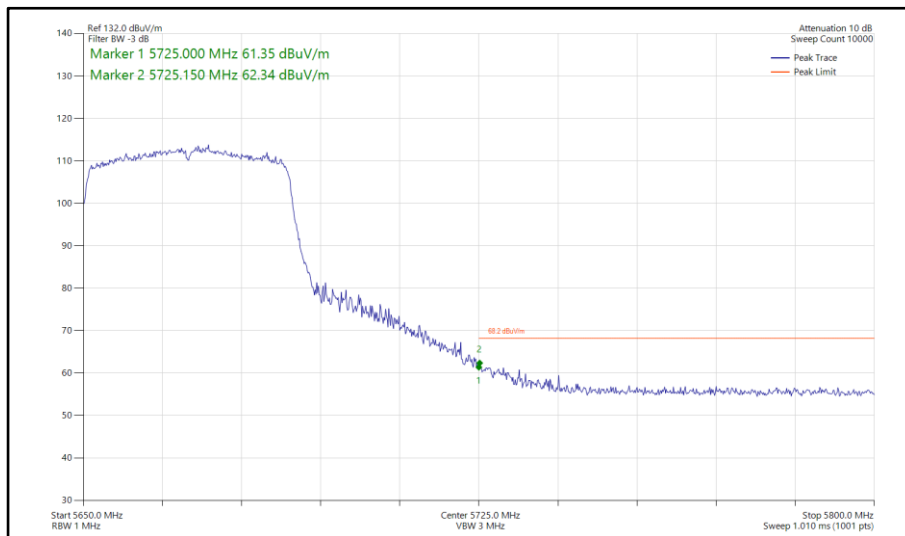
Figure 892 - 802.11ax HE40, SU, SISO, Core 1 - 5670 MHz Band Edge Frequency 5725 MHz
