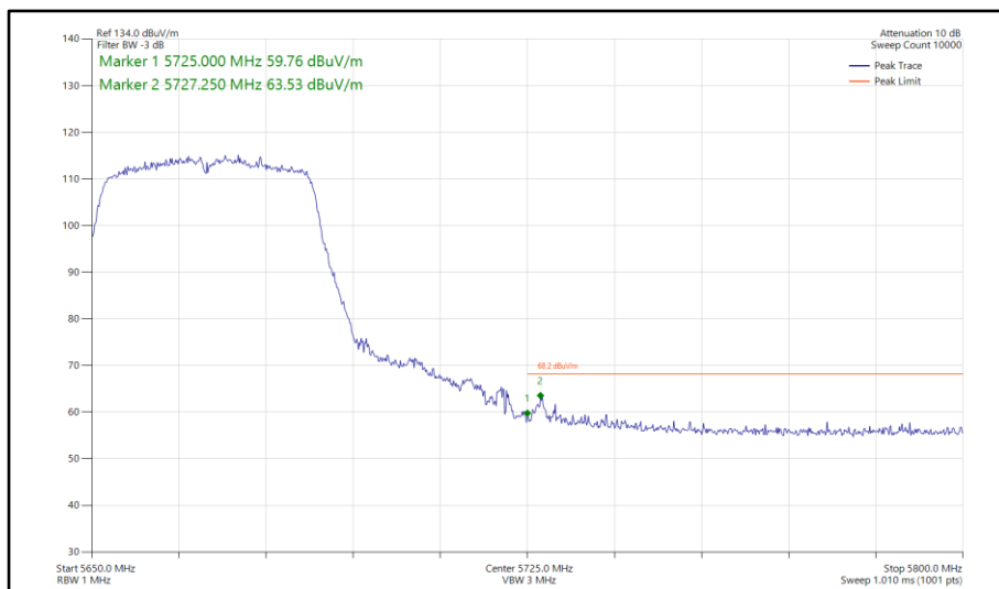
Figure 889 - 802.11n HT40, SISO, Core 1 - 5670 MHz Band Edge Frequency 5725 MHz
