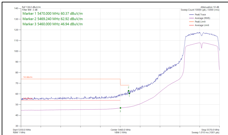
Figure 838 - 802.11n HT40, SISO, Core 0 - 5550 MHz Band Edge Frequency 5470 MHz
