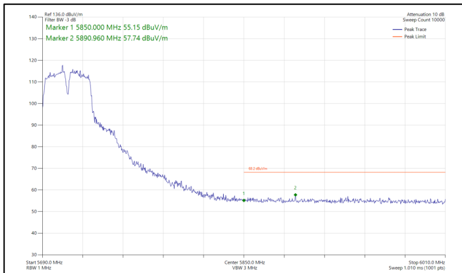
Figure 860 - 802.11a a40, SISO, Core 0 - 5710 MHz Band Edge Frequency 5850 MHz
