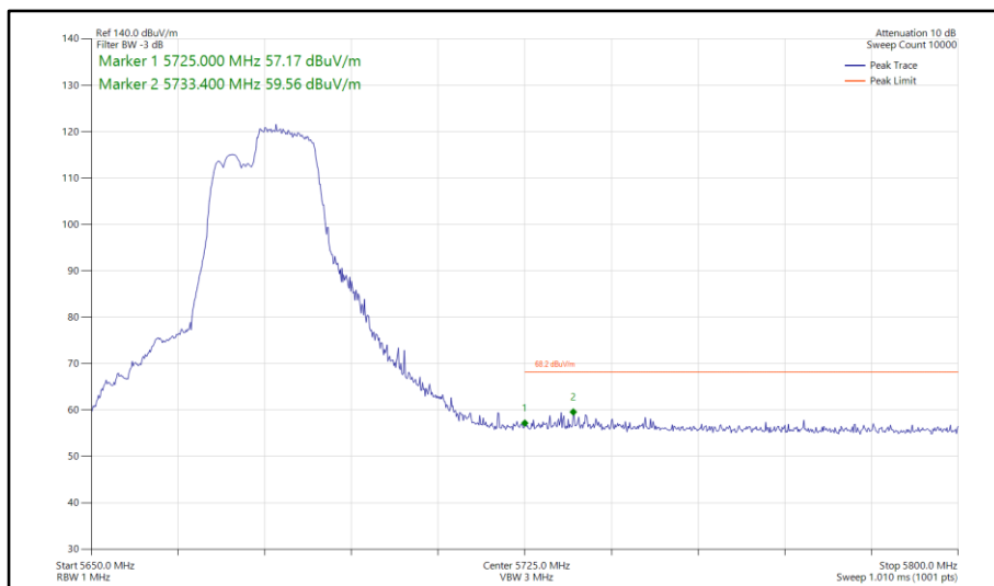
Figure 859 - 802.11be EHT40, RU 106+26-85, SISO, Core 0 - 5670 MHz Band Edge Frequency 5725 MHz
