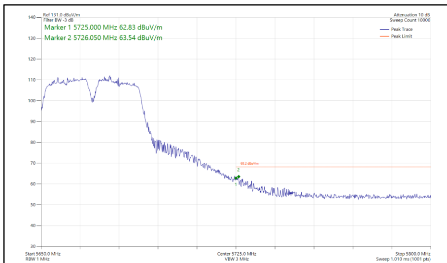
Figure 851 - 802.11a a40, SISO, Core 0 - 5670 MHz Band Edge Frequency 5725 MHz
