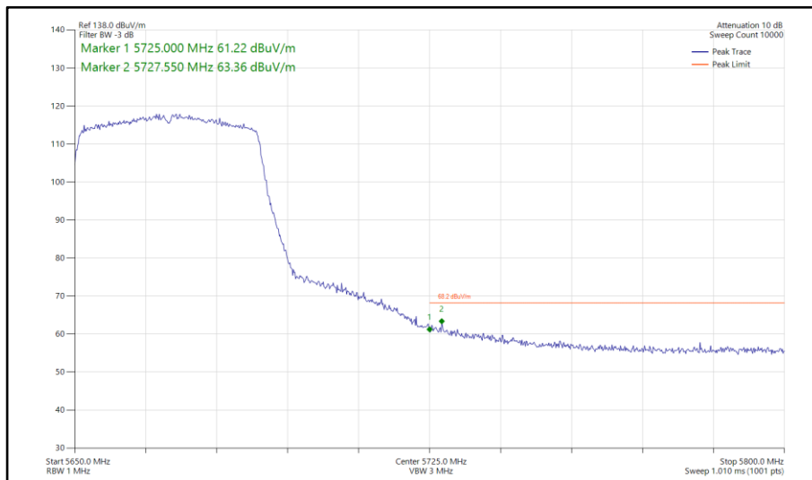
Figure 856 - 802.11ax HE40, SU, SISO, Core 0 - 5670 MHz Band Edge Frequency 5725 MHz
