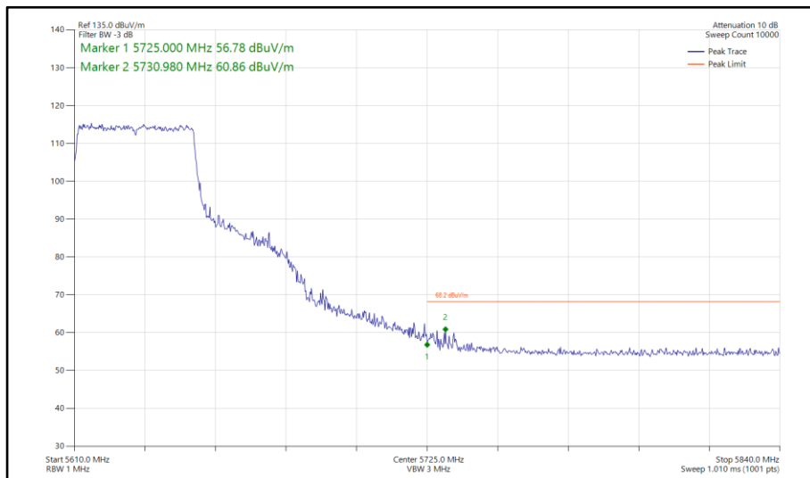
Figure 890 - 802.11ax HE40, SU, SISO, Core 1 - 5630 MHz Band Edge Frequency 5725 MHz
