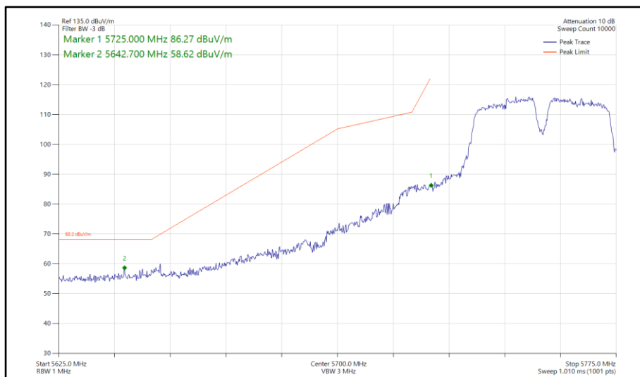
Figure 881 - 802.11a a40, SISO, Core 1 - 5755 MHz Band Edge Frequency 5725 MHz
