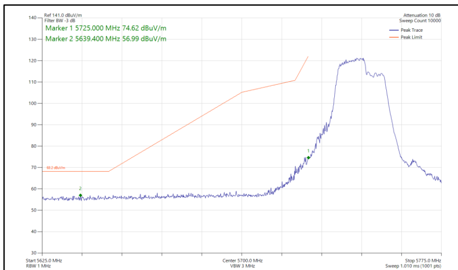
Figure 885 - 802.11be EHT40, RU 106+26-82, SISO, Core 1 - 5755 MHz Band Edge Frequency 5725 MHz
