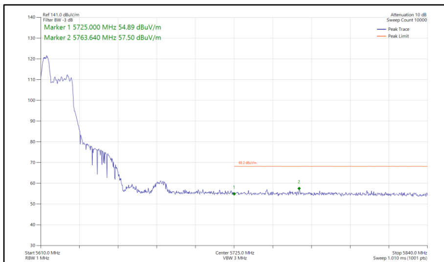
Figure 891 - 802.11ax HE40, RU 52-37, SISO, Core 1 - 5630 MHz Band Edge Frequency 5725 MHz
