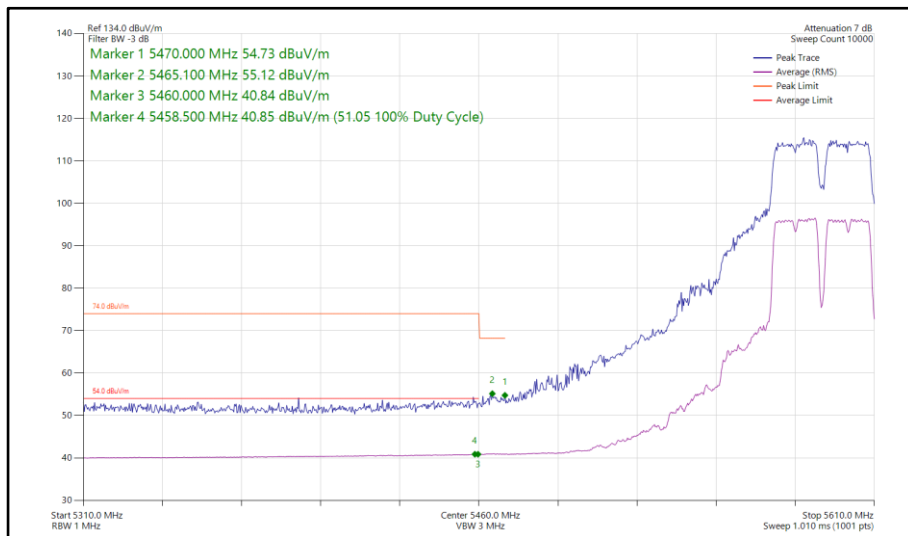
Figure 872 - 802.11a a40, SISO, Core 1 - 5590 MHz Band Edge Frequency 5470 MHz
