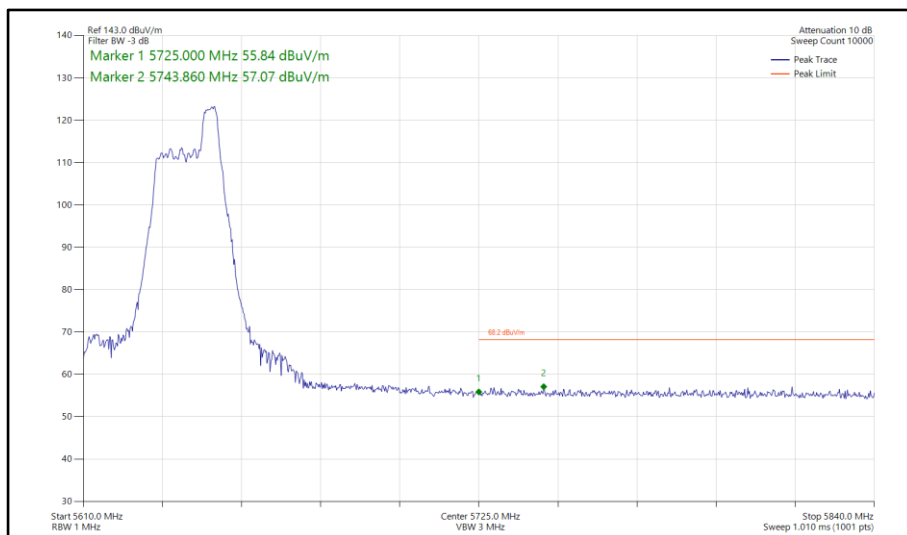
Figure 855 - 802.11ax HE40, RU 52-44, SISO, Core 0 - 5630 MHz Band Edge Frequency 5725 MHz
