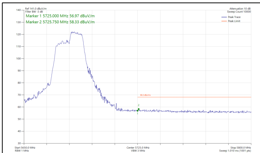
Figure 857 - 802.11ax HE40, RU 106-56, SISO, Core 0 - 5670 MHz Band Edge Frequency 5725 MHz
