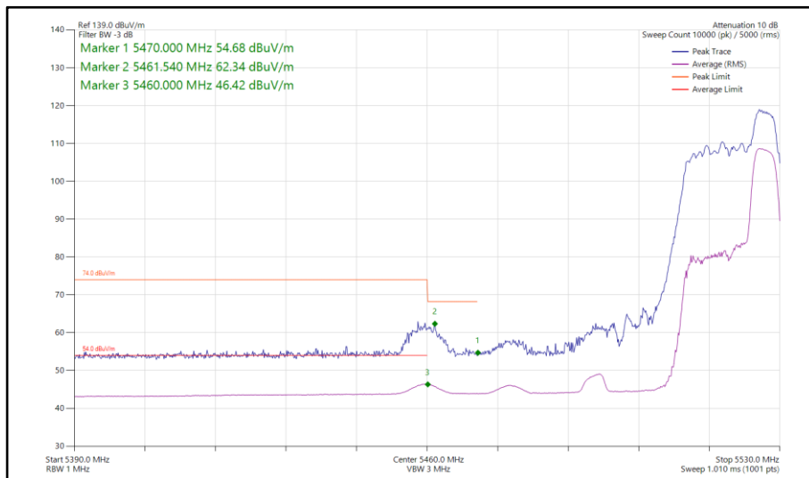
Figure 840 - 802.11ax HE40, RU 52-44, SISO, Core 0 - 5510 MHz Band Edge Frequency 5470 MHz
