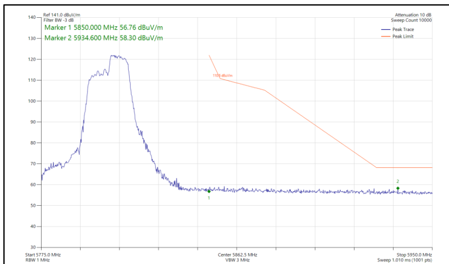
Figure 903 - 802.11ax HE40, RU 106-56, SISO, Core 1 - 5795 MHz Band Edge Frequency 5850 MHz
