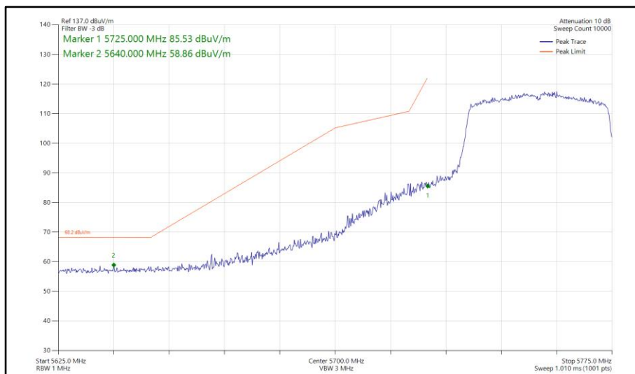
Figure 847 - 802.11ax HE40, SU, SISO, Core 0 - 5755 MHz Band Edge Frequency 5725 MHz
