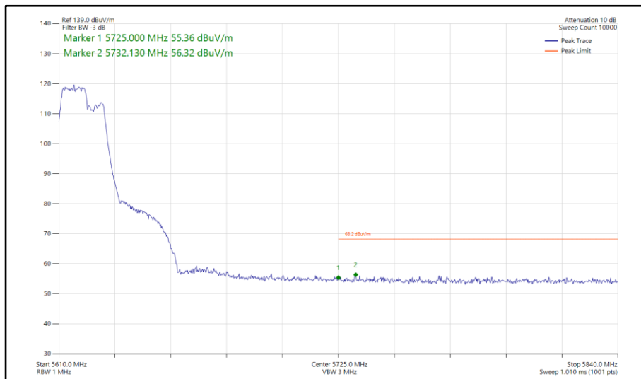
Figure 894 - 802.11be EHT40, RU 106+26-82, SISO, Core 1 - 5630 MHz Band Edge Frequency 5725 MHz
