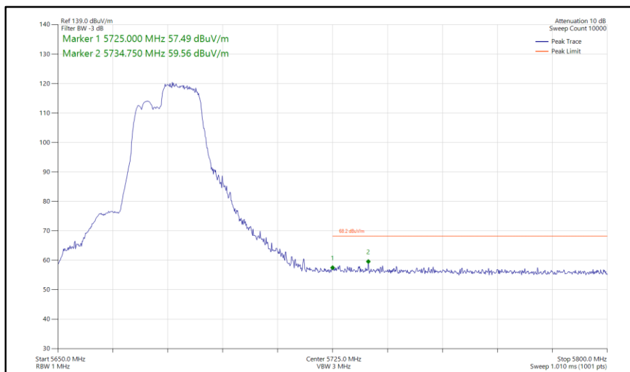
Figure 895 - 802.11be EHT40, RU 106+26-85, SISO, Core 1 - 5670 MHz Band Edge Frequency 5725 MHz
