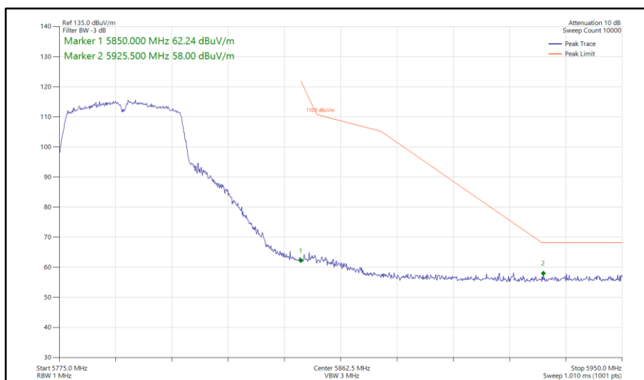
Figure 863 - 802.11n HT40, SISO, Core 0 - 5795 MHz Band Edge Frequency 5850 MHz
