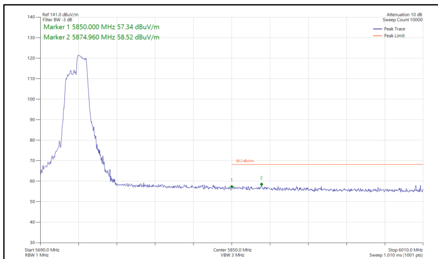
Figure 901 - 802.11ax HE40, RU 106-56, SISO, Core 1 - 5710 MHz Band Edge Frequency 5850 MHz
