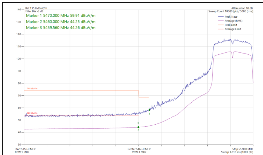
Figure 874 - 802.11n HT40, SISO, Core 1 - 5550 MHz Band Edge Frequency 5470 MHz
