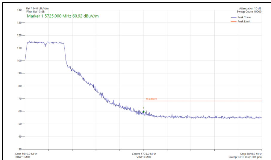
Figure 852 - 802.11n HT40, SISO, Core 0 - 5630 MHz Band Edge Frequency 5725 MHz
