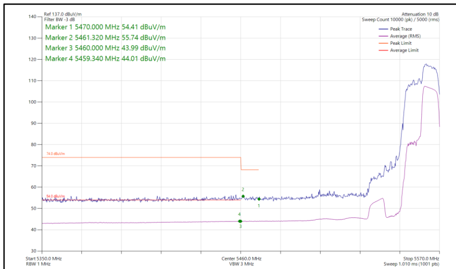
Figure 842 - 802.11ax HE40, RU 106-56, SISO, Core 0 - 5550 MHz Band Edge Frequency 5470 MHz
