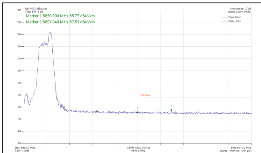
Figure 865 - 802.11ax HE40, RU 52-44, SISO, Core 0 - 5710 MHz Band Edge Frequency 5850 MHz
