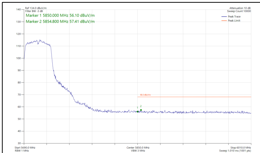
Figure 862 - 802.11n HT40, SISO, Core 0 - 5710 MHz Band Edge Frequency 5850 MHz
