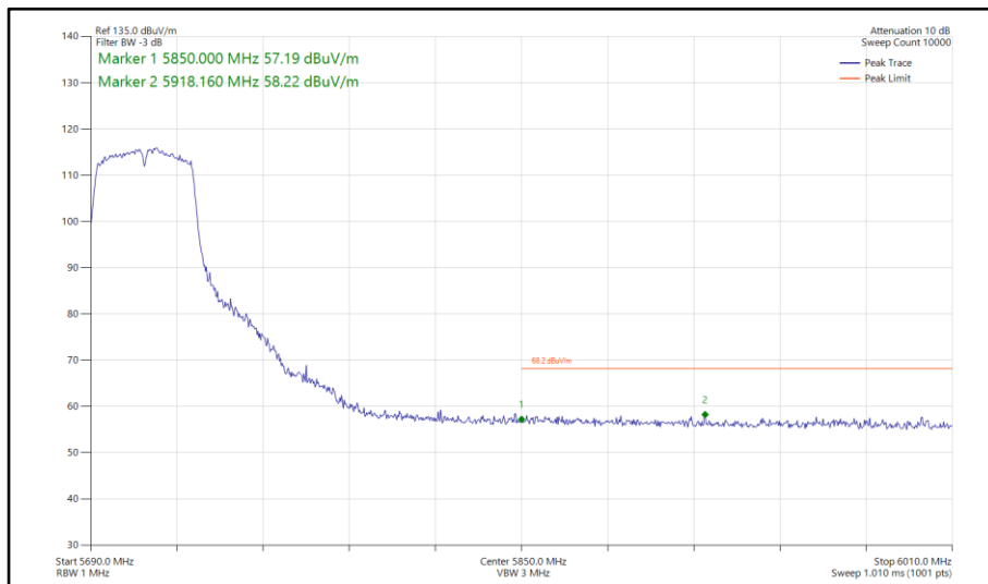
Figure 898 - 802.11n HT40, SISO, Core 1 - 5710 MHz Band Edge Frequency 5850 MHz
