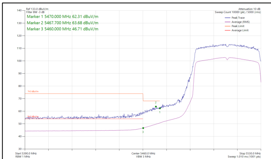
Figure 839 - 802.11ax HE40, SU, SISO, Core 0 - 5510 MHz Band Edge Frequency 5470 MHz
