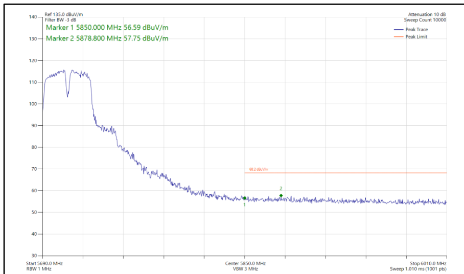
Figure 896 - 802.11a a40, SISO, Core 1 - 5710 MHz Band Edge Frequency 5850 MHz
