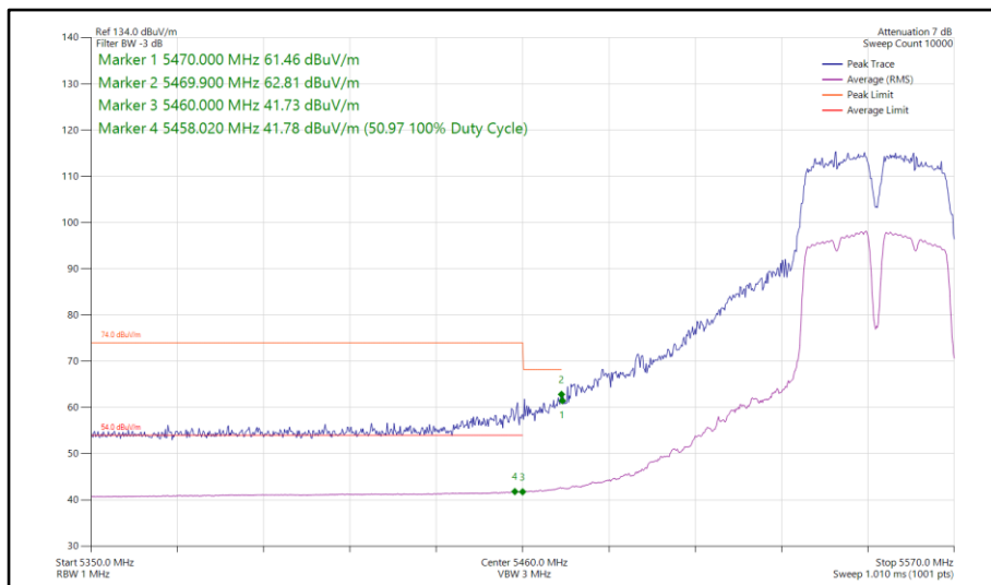
Figure 835 - 802.11a a40, SISO, Core 0 - 5550 MHz Band Edge Frequency 5470 MHz
