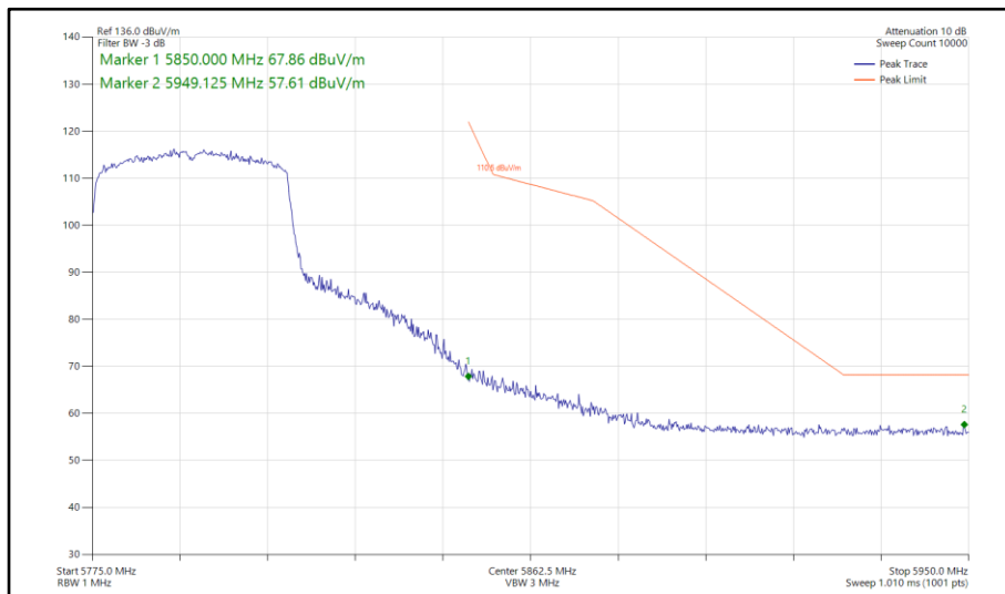
Figure 866 - 802.11ax HE40, SU, SISO, Core 0 - 5795 MHz Band Edge Frequency 5850 MHz
