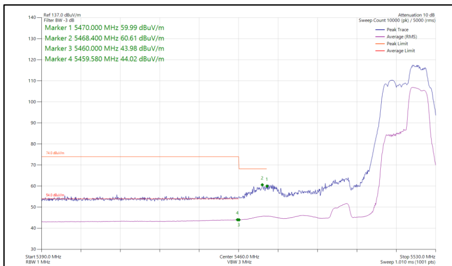
Figure 843 - 802.11be EHT40, RU 52+26-75, SISO, Core 0 - 5510 MHz Band Edge Frequency 5470 MHz
