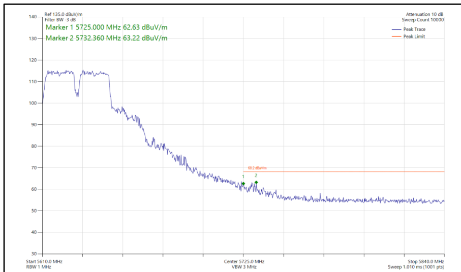
Figure 850 - 802.11a a40, SISO, Core 0 - 5630 MHz Band Edge Frequency 5725 MHz
