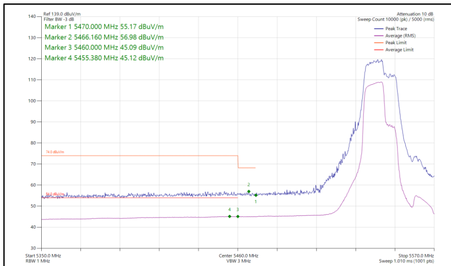
Figure 880 - 802.11be EHT40, RU 106+26-82, SISO, Core 1 - 5550 MHz Band Edge Frequency 5470 MHz
