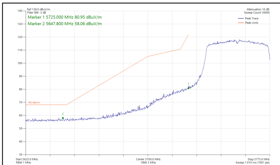
Figure 883 - 802.11ax HE40, SU, SISO, Core 1 - 5755 MHz Band Edge Frequency 5725 MHz
