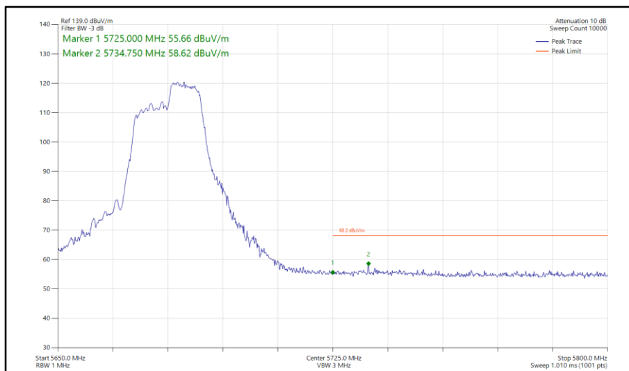
Figure 893 - 802.11ax HE40, RU 106-56, SISO, Core 1 - 5670 MHz Band Edge Frequency 5725 MHz
