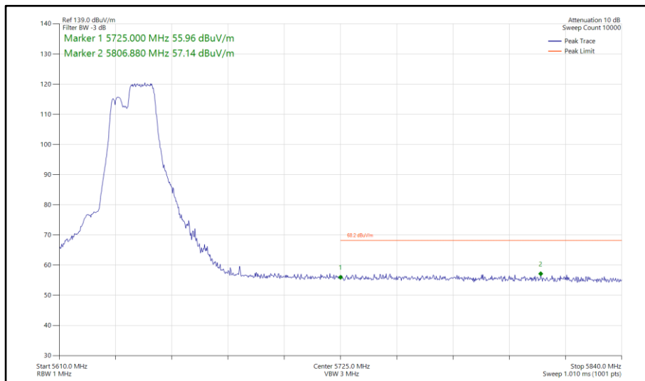
Figure 858 - 802.11be EHT40, RU 106+26-85, SISO, Core 0 - 5630 MHz Band Edge Frequency 5725 MHz
