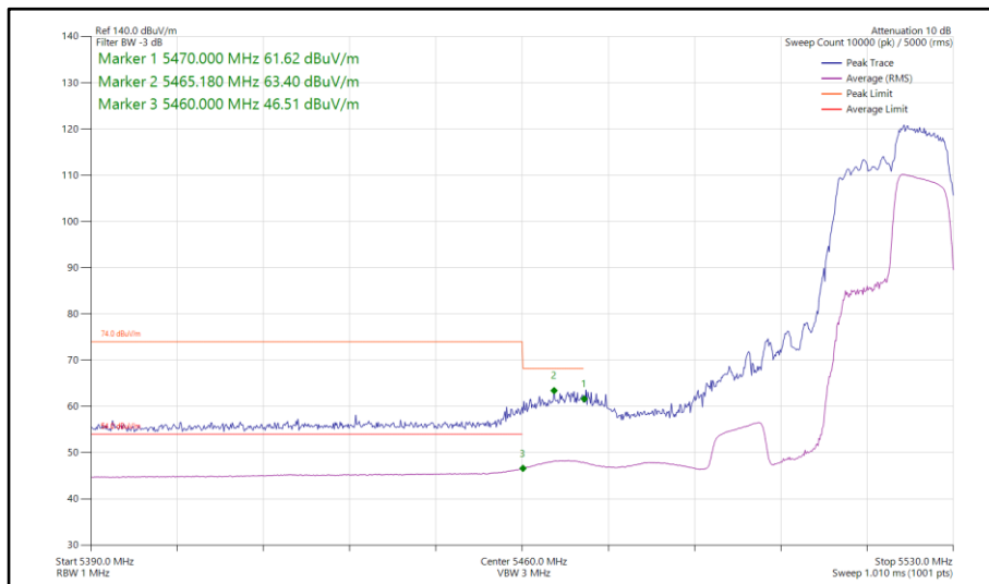
Figure 876 - 802.11ax HE40, RU 106-56, SISO, Core 1 - 5510 MHz Band Edge Frequency 5470 MHz
