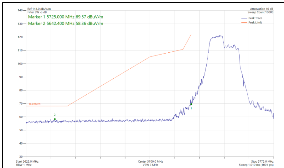
Figure 848 - 802.11ax HE40, RU 106-53, SISO, Core 0 - 5755 MHz Band Edge Frequency 5725 MHz
