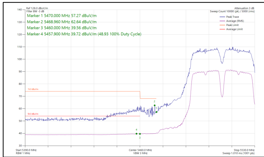
Figure 834 - 802.11a a40, SISO, Core 0 - 5510 MHz Band Edge Frequency 5470 MHz
