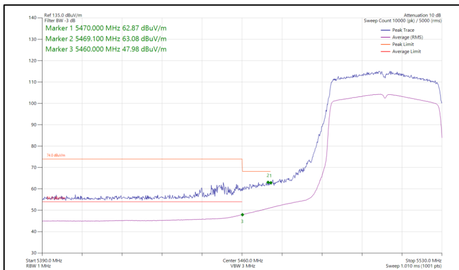
Figure 875 - 802.11ax HE40, SU, SISO, Core 1 - 5510 MHz Band Edge Frequency 5470 MHz
