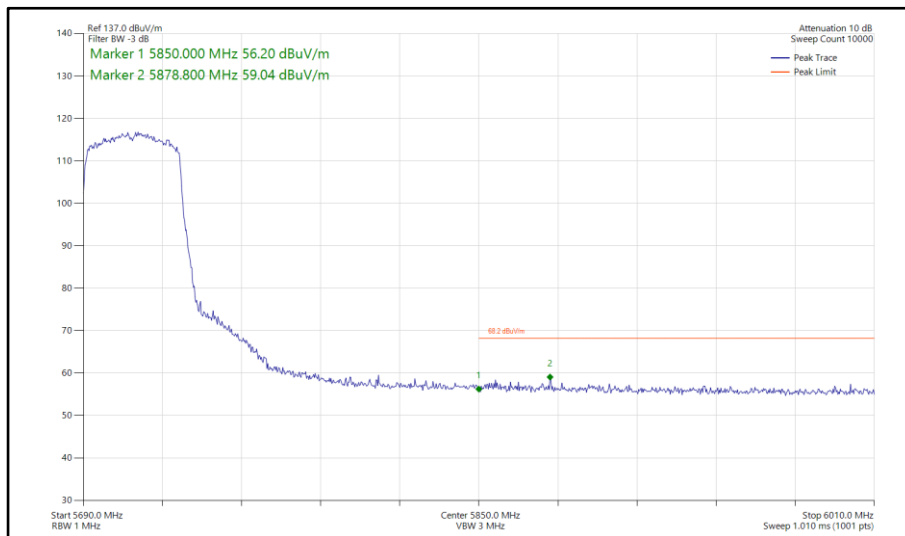
Figure 900 - 802.11ax HE40, SU, SISO, Core 1 - 5710 MHz Band Edge Frequency 5850 MHz
