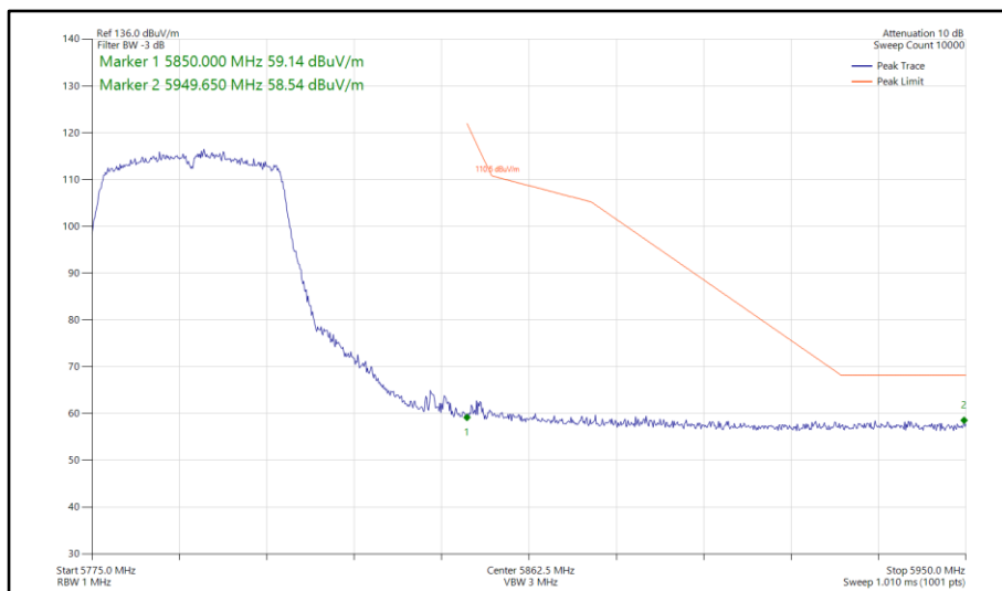
Figure 899 - 802.11n HT40, SISO, Core 1 - 5795 MHz Band Edge Frequency 5850 MHz
