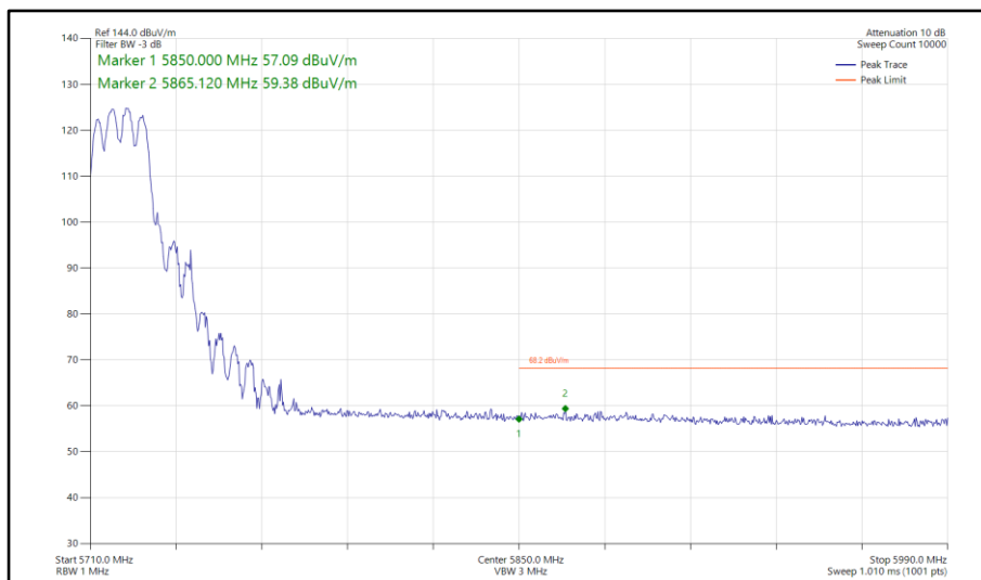
Figure 832 - 802.11ax HE20, SU, TxBF, Core 0-1 - 5720 MHz Band Edge Frequency 5850 MHz
