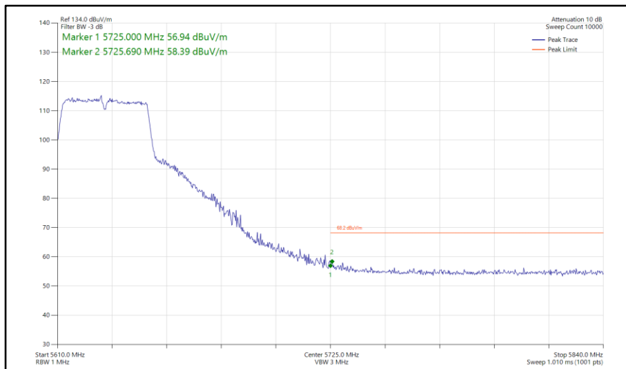
Figure 888 - 802.11n HT40, SISO, Core 1 - 5630 MHz Band Edge Frequency 5725 MHz
