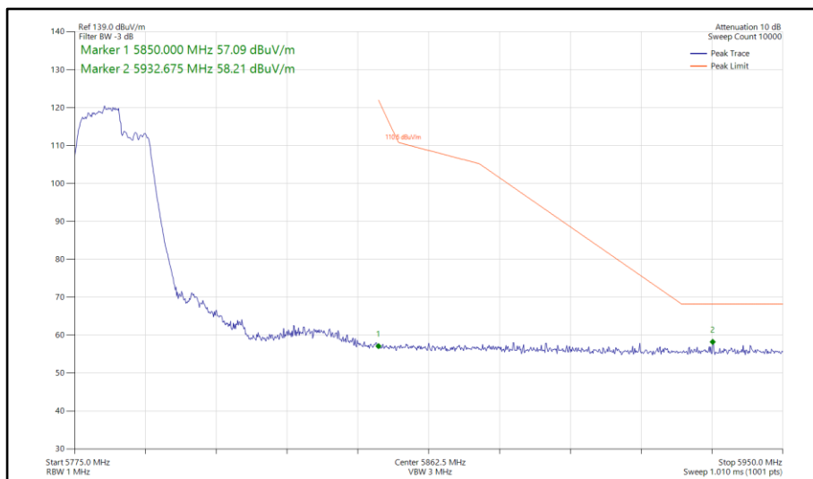
Figure 869 - 802.11be EHT40, RU 106+26-82, SISO, Core 0 - 5795 MHz Band Edge Frequency 5850 MHz
