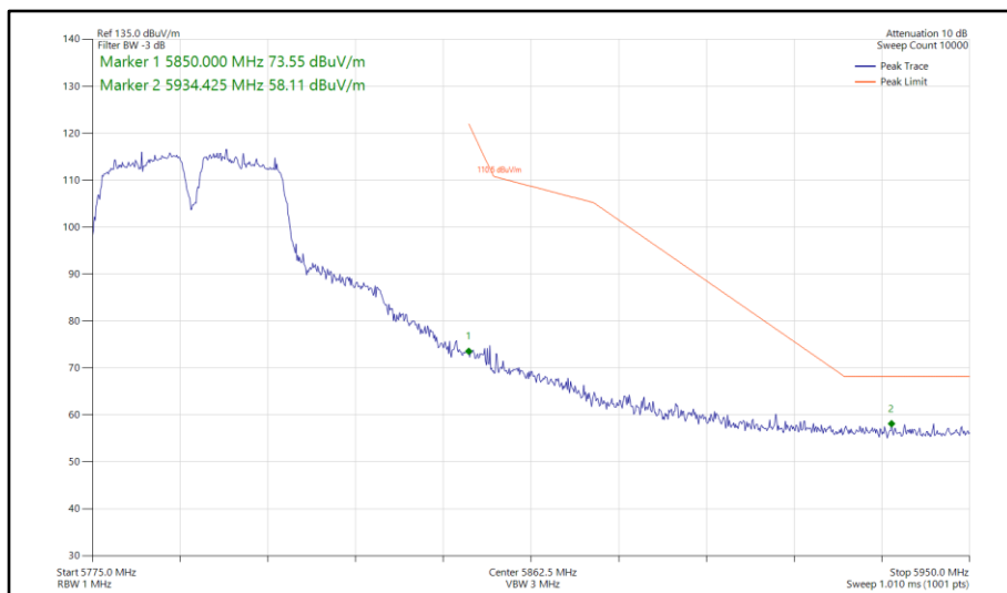
Figure 897 - 802.11a a40, SISO, Core 1 - 5795 MHz Band Edge Frequency 5850 MHz
