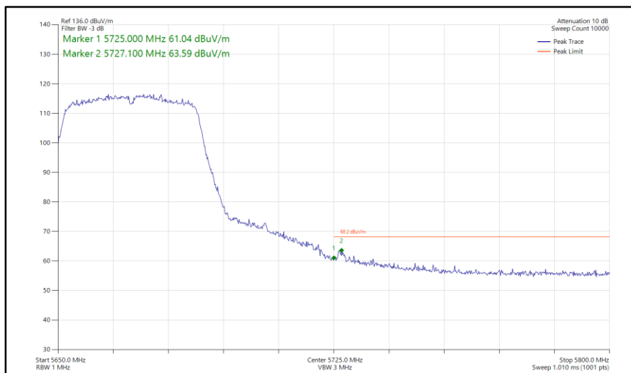
Figure 853 - 802.11n HT40, SISO, Core 0 - 5670 MHz Band Edge Frequency 5725 MHz
