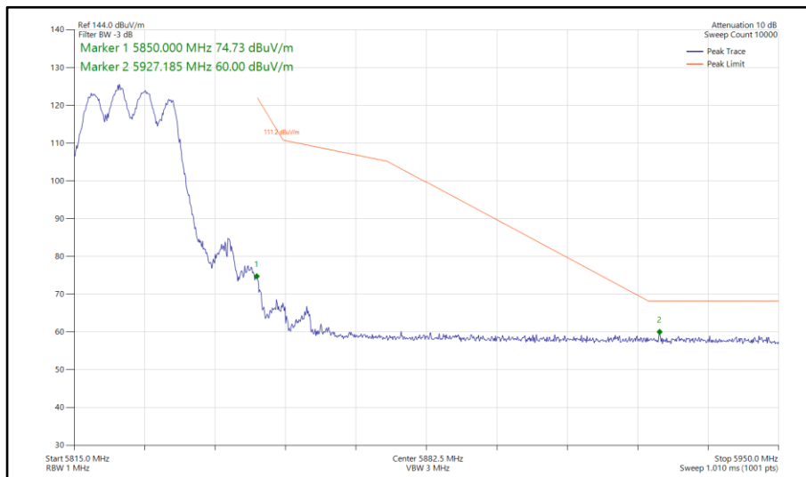
Figure 833 - 802.11ax HE20, SU, TxBF, Core 0-1 - 5825 MHz Band Edge Frequency 5850 MHz
