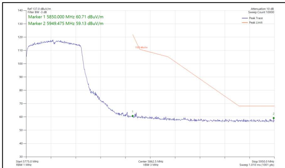
Figure 902 - 802.11ax HE40, SU, SISO, Core 1 - 5795 MHz Band Edge Frequency 5850 MHz
