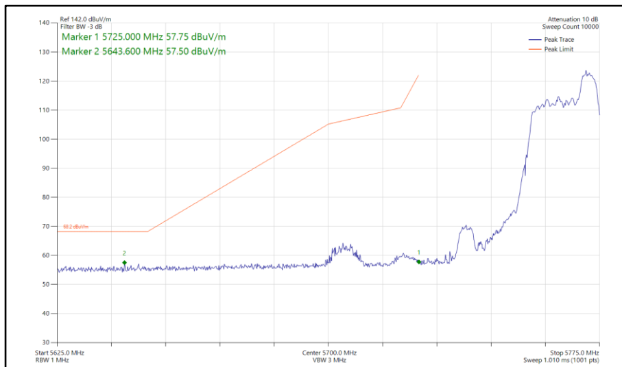
Figure 884 - 802.11ax HE40, RU 52-44, SISO, Core 1 - 5755 MHz Band Edge Frequency 5725 MHz
