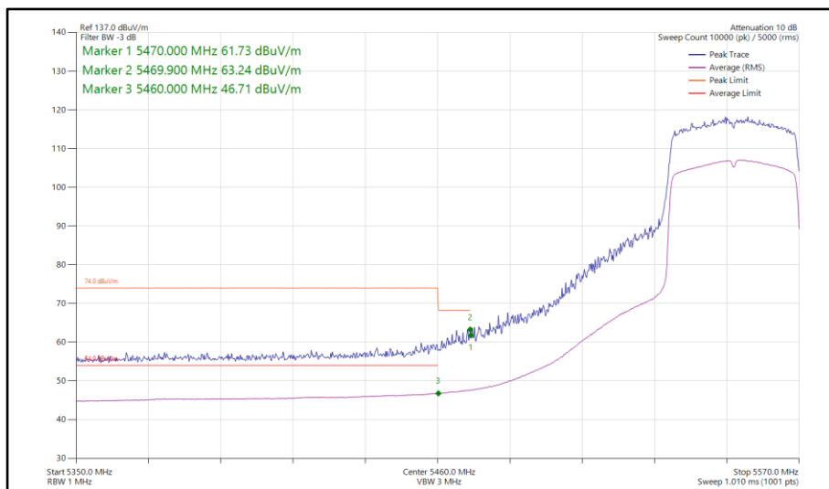
Figure 841 - 802.11ax HE40, SU, SISO, Core 0 - 5550 MHz Band Edge Frequency 5470 MHz
