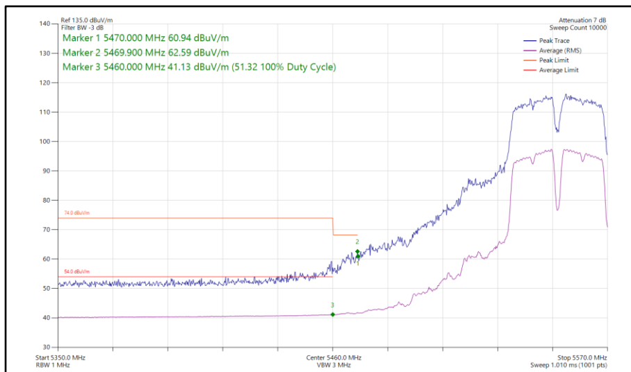
Figure 871 - 802.11a a40, SISO, Core 1 - 5550 MHz Band Edge Frequency 5470 MHz
