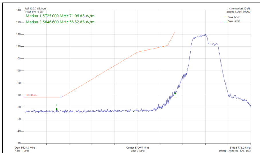
Figure 849 - 802.11be EHT40, RU 106+26-82, SISO, Core 0 - 5755 MHz Band Edge Frequency 5725 MHz
