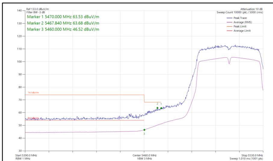
Figure 837 - 802.11n HT40, SISO, Core 0 - 5510 MHz Band Edge Frequency 5470 MHz
