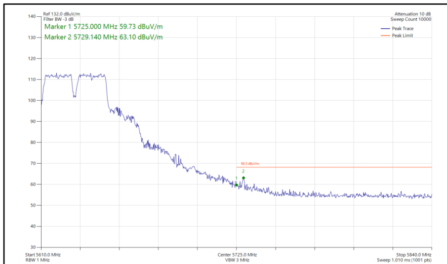
Figure 886 - 802.11a a40, SISO, Core 1 - 5630 MHz Band Edge Frequency 5725 MHz
