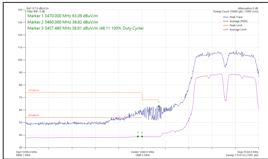
Figure 870 - 802.11a a40, SISO, Core 1 - 5510 MHz Band Edge Frequency 5470 MHz
