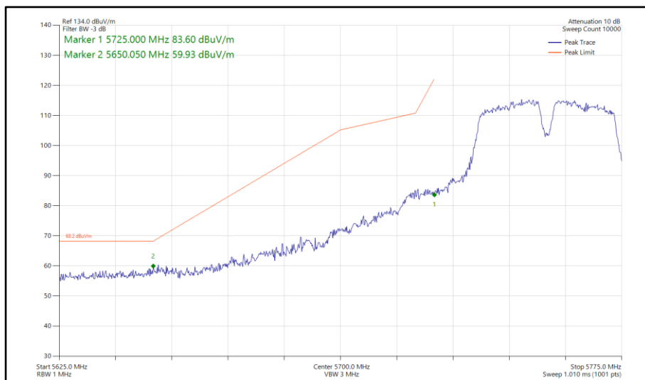
Figure 845 - 802.11a a40, SISO, Core 0 - 5755 MHz Band Edge Frequency 5725 MHz
