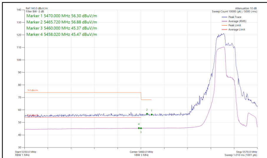
Figure 878 - 802.11ax HE40, RU 106-53, SISO, Core 1 - 5550 MHz Band Edge Frequency 5470 MHz
