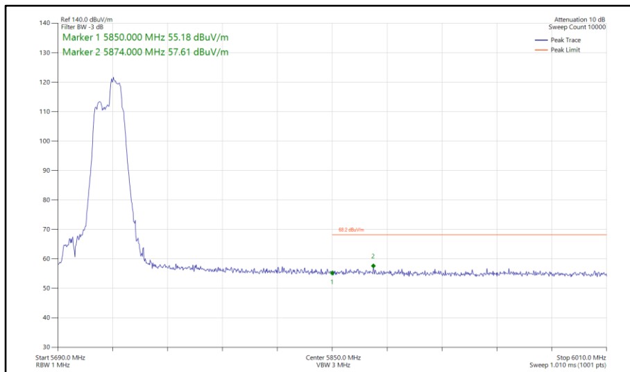
Figure 868 - 802.11be EHT40, RU 52+26-75, SISO, Core 0 - 5710 MHz Band Edge Frequency 5850 MHz
