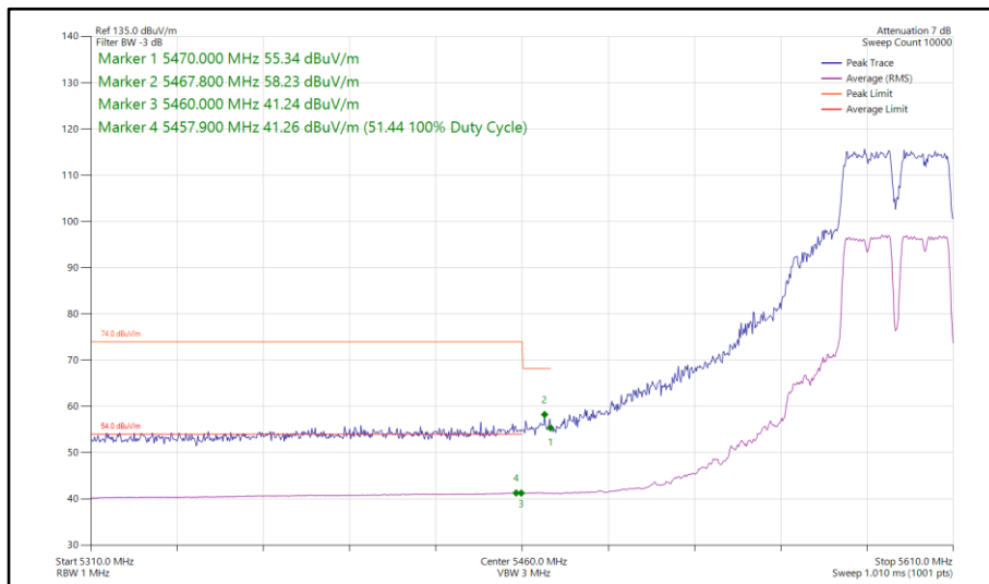
Figure 836 - 802.11a a40, SISO, Core 0 - 5590 MHz Band Edge Frequency 5470 MHz
