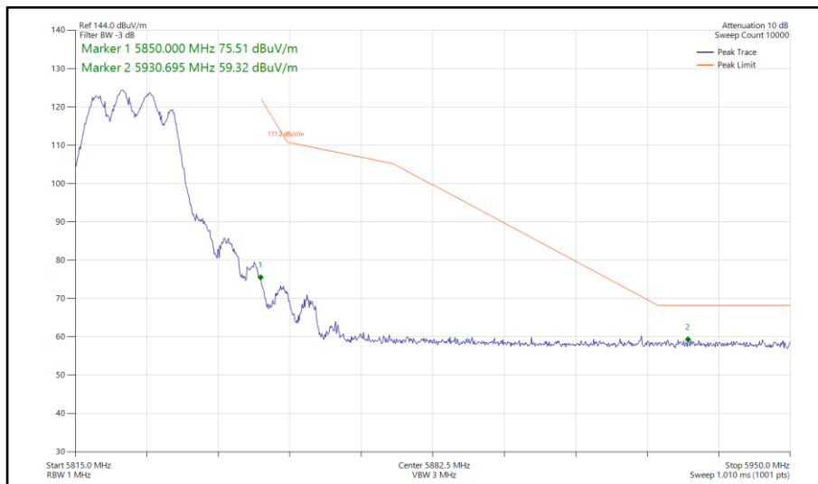
Figure 831 - 802.11ac VHT20, TxBF, Core 0-1 - 5825 MHz Band Edge Frequency 5850 MHz
