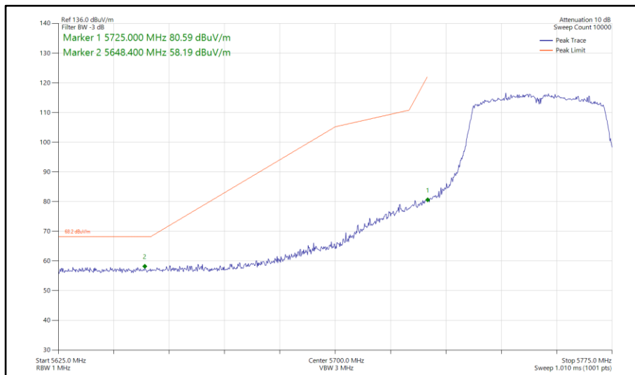
Figure 846 - 802.11n HT40, SISO, Core 0 - 5755 MHz Band Edge Frequency 5725 MHz
