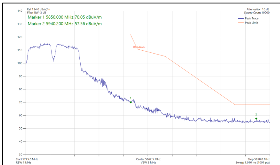
Figure 861 - 802.11a a40, SISO, Core 0 - 5795 MHz Band Edge Frequency 5850 MHz
