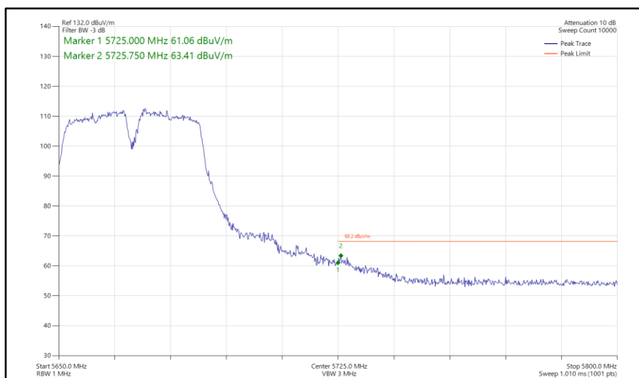
Figure 887 - 802.11a a40, SISO, Core 1 - 5670 MHz Band Edge Frequency 5725 MHz
