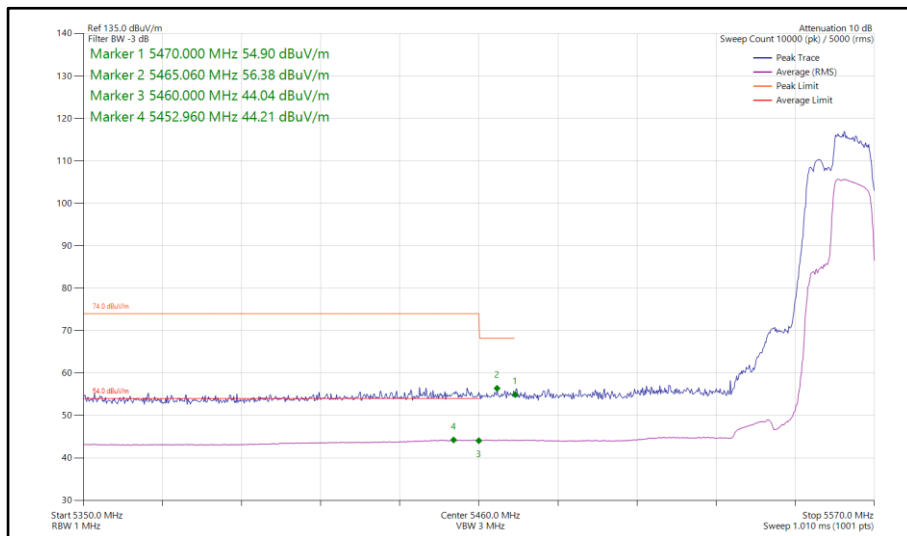
Figure 844 - 802.11be EHT40, RU 106+26-85, SISO, Core 0 - 5550 MHz Band Edge Frequency 5470 MHz
