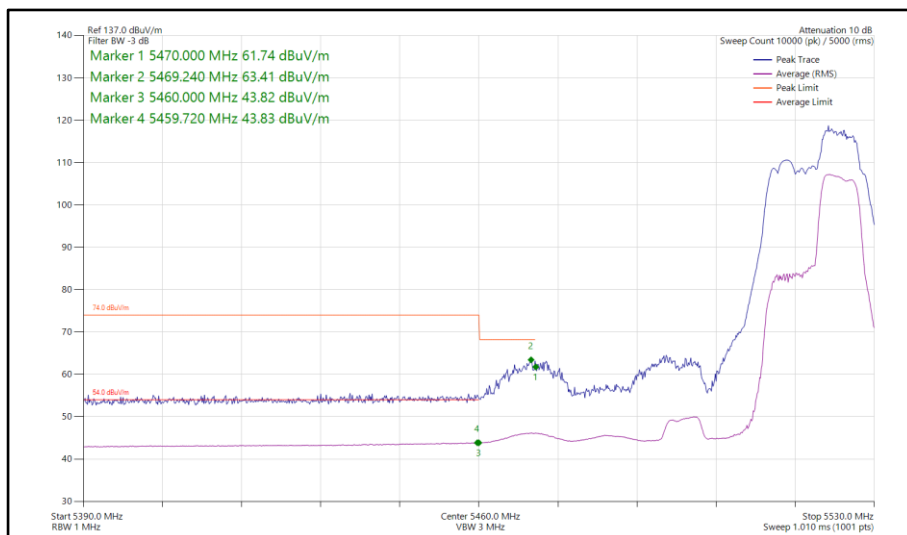
Figure 879 - 802.11be EHT40, RU 52+26-75, SISO, Core 1 - 5510 MHz Band Edge Frequency 5470 MHz
