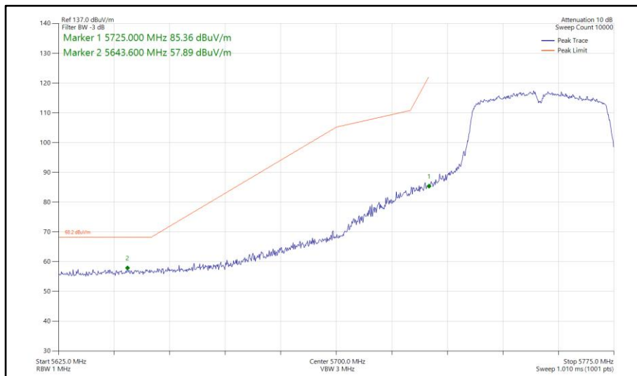
Figure 882 - 802.11n HT40, SISO, Core 1 - 5755 MHz Band Edge Frequency 5725 MHz
