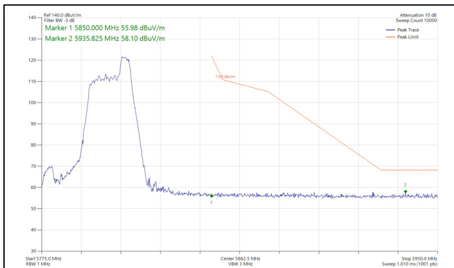
Figure 867 - 802.11ax HE40, RU 52-44, SISO, Core 0 - 5795 MHz Band Edge Frequency 5850 MHz
