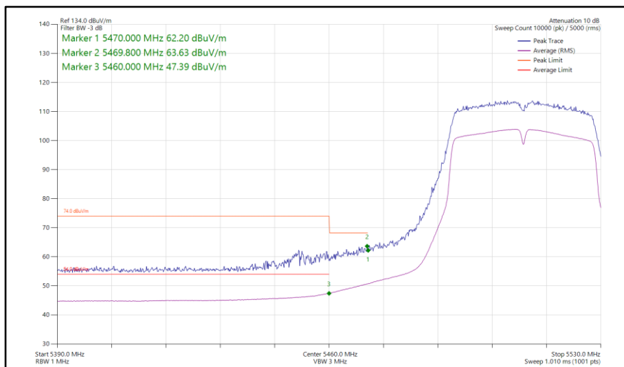
Figure 873 - 802.11n HT40, SISO, Core 1 - 5510 MHz Band Edge Frequency 5470 MHz
