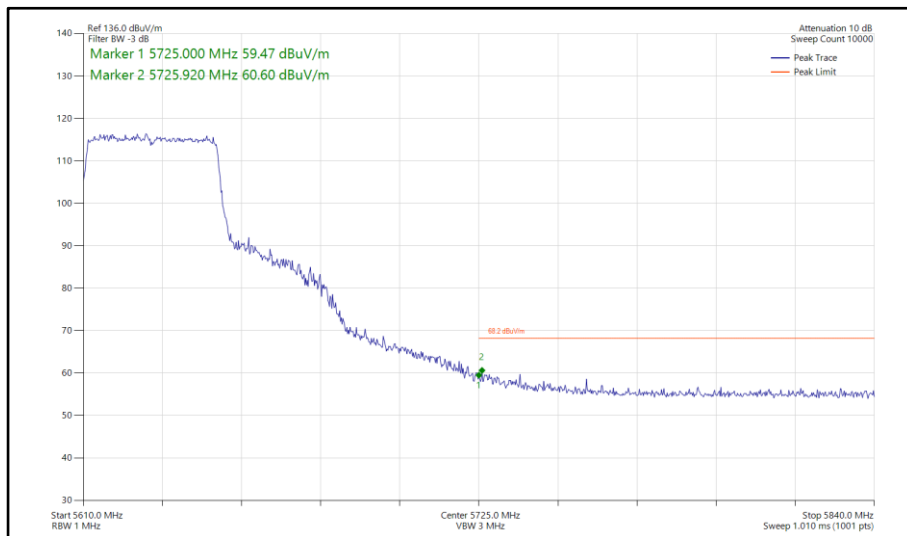
Figure 854 - 802.11ax HE40, SU, SISO, Core 0 - 5630 MHz Band Edge Frequency 5725 MHz
