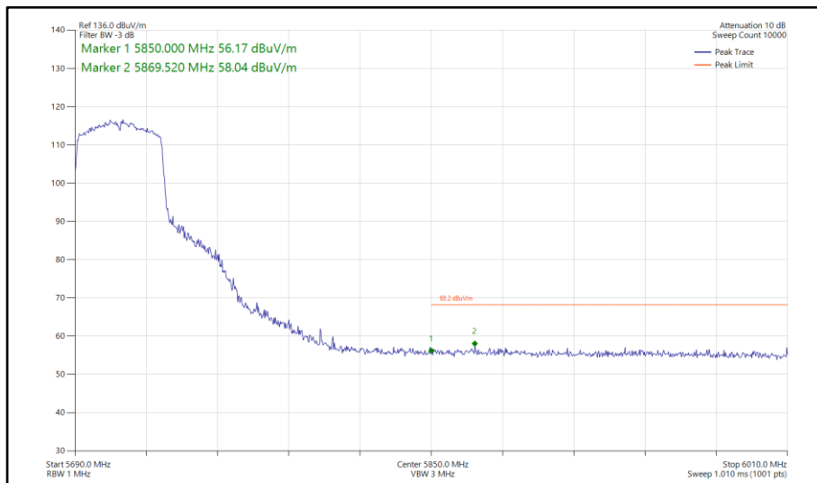
Figure 864 - 802.11ax HE40, SU, SISO, Core 0 - 5710 MHz Band Edge Frequency 5850 MHz
