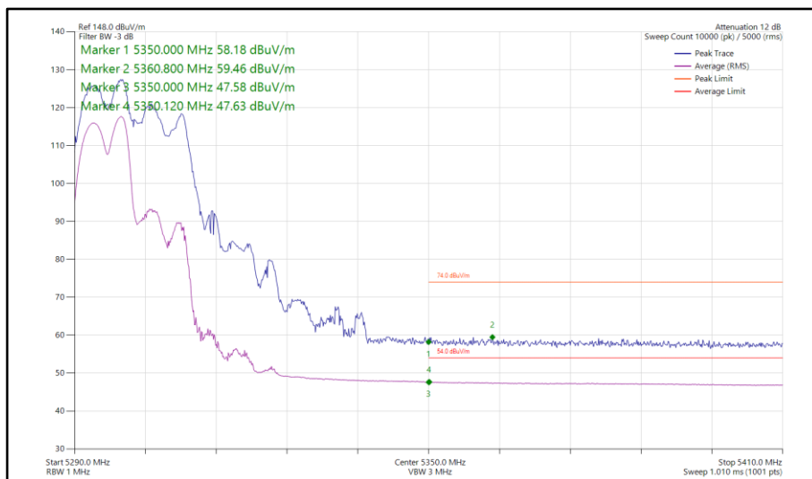
Figure 70 - 802.11ax HE20, RU 106-53, CDD, Core 0-1 - 5300 MHz Band Edge Frequency 5350 MHz
