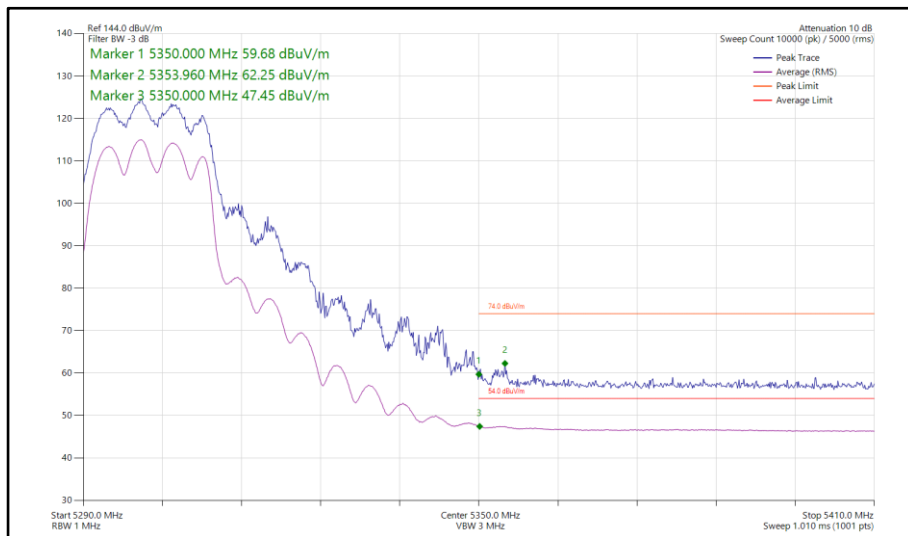
Figure 67 - 802.11n HT20, CDD, Core 0-1 - 5300 MHz Band Edge Frequency 5350 MHz
