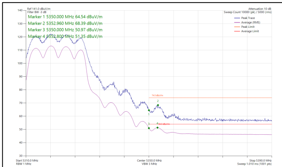
Figure 116 - 802.11ac VHT20, TxBF, Core 0-1 - 5320 MHz Band Edge Frequency 5350 MHz
