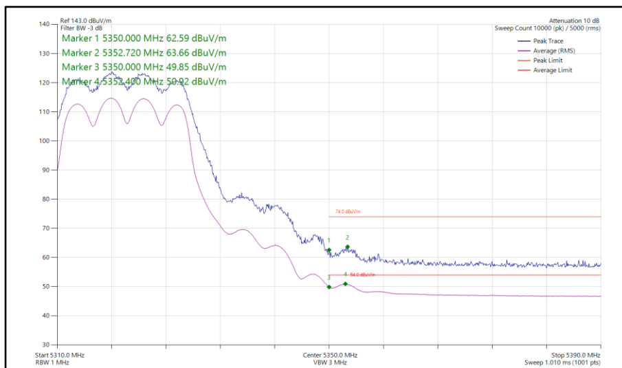
Figure 66 - 802.11a, CDD, Core 0-1 - 5320 MHz Band Edge Frequency 5350 MHz
