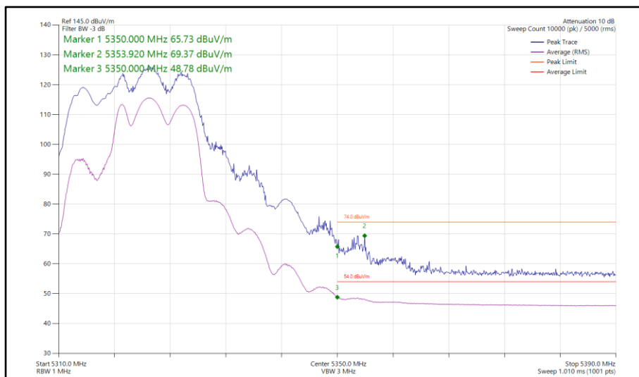
Figure 100 - 802.11be EHT20, RU 106+26-83, SDM, Core 0-1 - 5320 MHz Band Edge Frequency 5350 MHz
