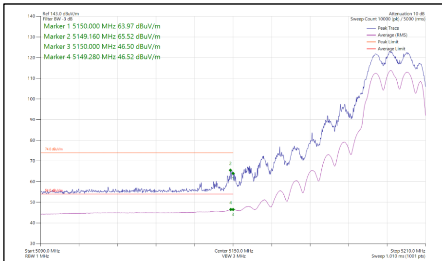
Figure 112 - 802.11ac VHT20, TxBF, Core 0-1 - 5200 MHz Band Edge Frequency 5150 MHz
