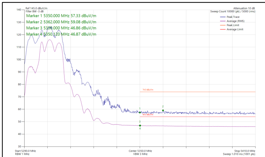
Figure 99 - 802.11be EHT20, RU 106+26-83, SDM, Core 0-1 - 5300 MHz Band Edge Frequency 5350 MHz
