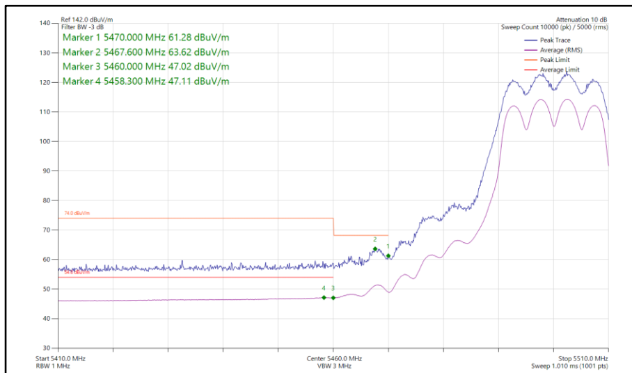
Figure 75 - 802.11a, CDD, Core 0-1 - 5500 MHz Band Edge Frequency 5460 MHz
