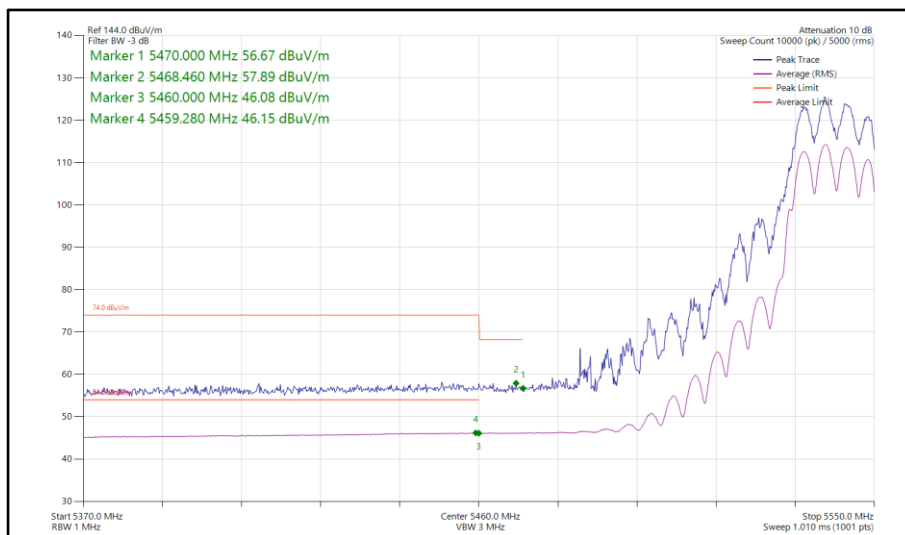
Figure 84 - 802.11ax HE20, SU, CDD, Core 0-1 - 5540 MHz Band Edge Frequency 5460 MHz
