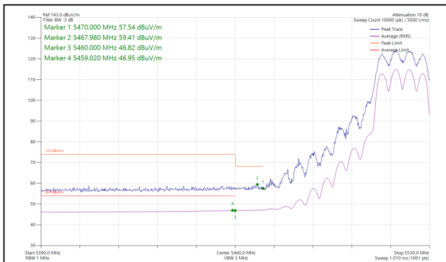
Figure 76 - 802.11a, CDD, Core 0-1 - 5520 MHz Band Edge Frequency 5460 MHz
