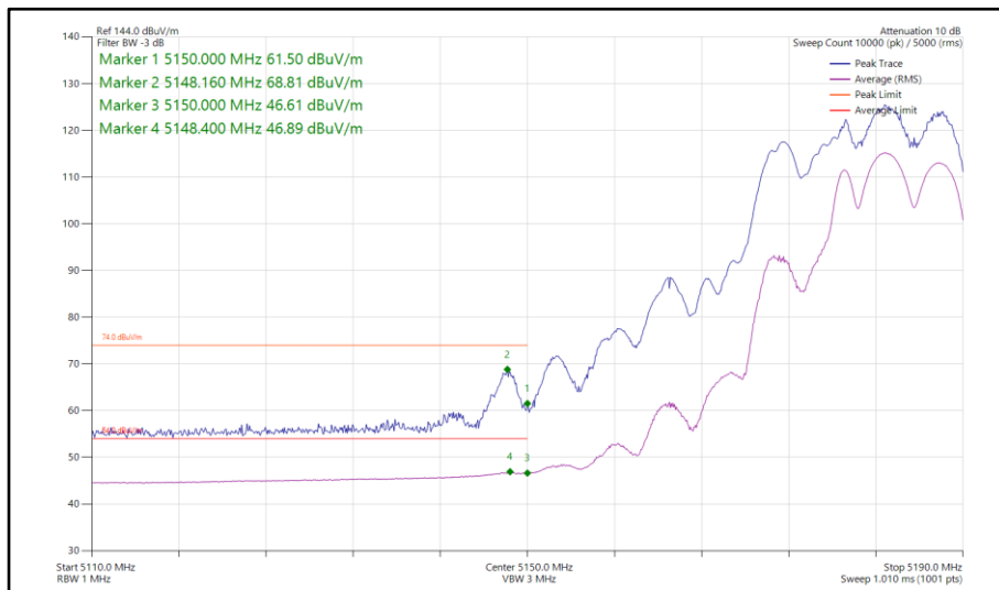
Figure 93 - 802.11be EHT20, RU 106+26-83, SDM, Core 0-1 - 5180 MHz Band Edge Frequency 5150 MHz
