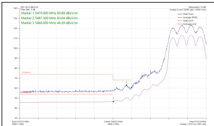
Figure 80 - 802.11ax HE20, SU, CDD, Core 0-1 - 5500 MHz Band Edge Frequency 5460 MHz
