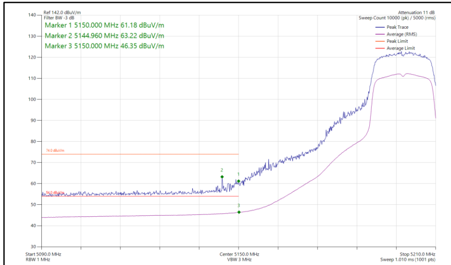
Figure 89 - 802.11n HT20, SDM, Core 0-1 - 5200 MHz Band Edge Frequency 5150 MHz
