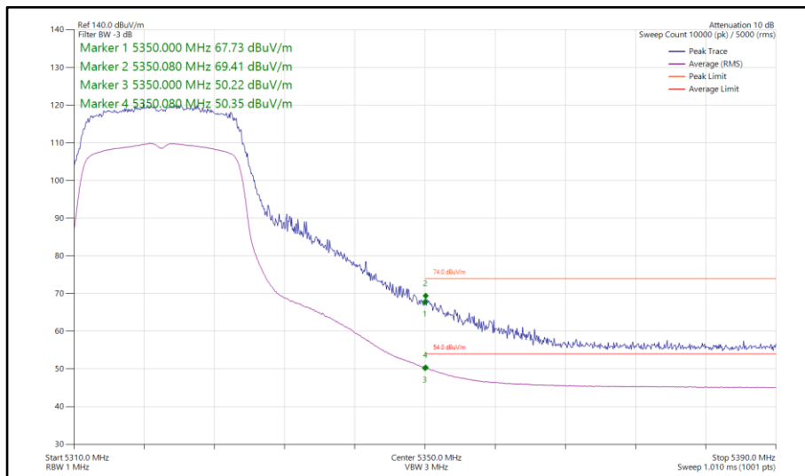
Figure 95 - 802.11n HT20, SDM, Core 0-1 - 5320 MHz Band Edge Frequency 5350 MHz
