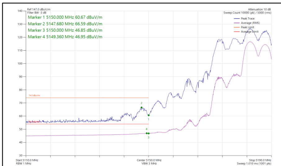
Figure 60 - 802.11ax HE20, RU 106-54, CDD, Core 0-1 - 5180 MHz Band Edge Frequency 5150 MHz
