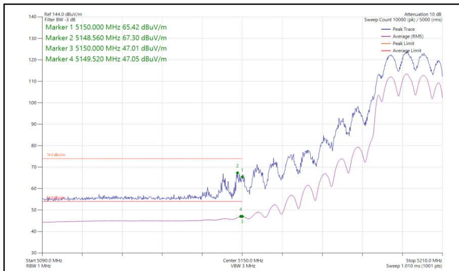
Figure 114 - 802.11ax HE20, SU, TxBF, Core 0-1 - 5200 MHz Band Edge Frequency 5150 MHz
