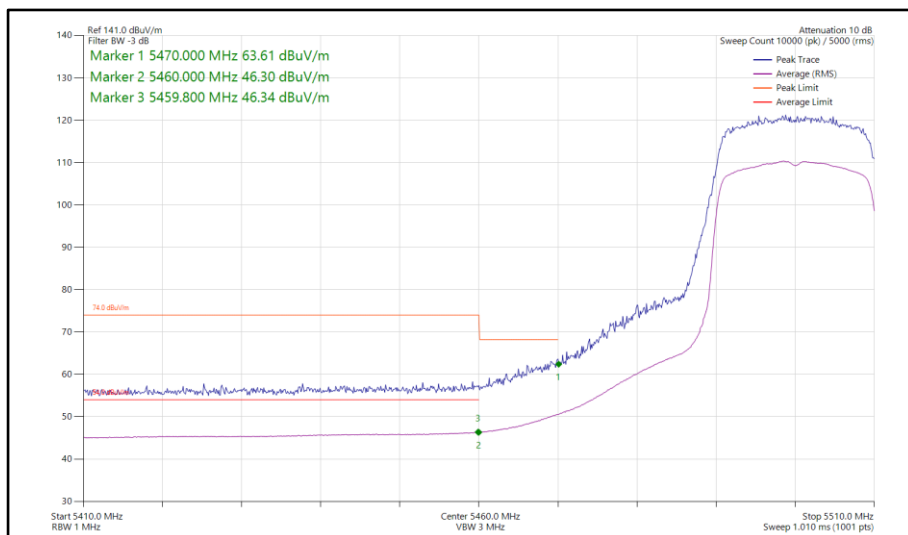
Figure 104 - 802.11ax HE20, SU, SDM, Core 0-1 - 5500 MHz Band Edge Frequency 5460 MHz
