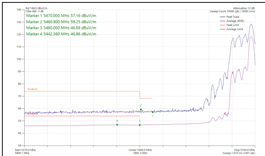
Figure 85 - 802.11ax HE20, RU 52-40, CDD, Core 0-1 - 5540 MHz Band Edge Frequency 5460 MHz
