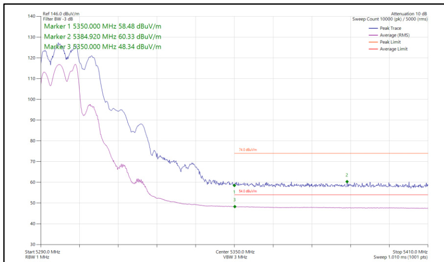
Figure 73 - 802.11be EHT20, RU 106+26-82, CDD, Core 0-1 - 5300 MHz Band Edge Frequency 5350 MHz
