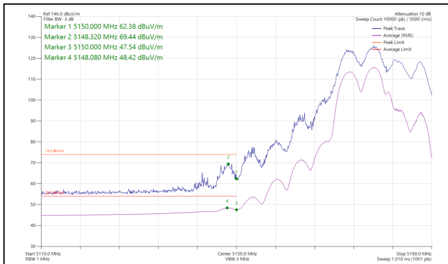
Figure 63 - 802.11be EHT20, RU 106+26-82, CDD, Core 0-1 - 5180 MHz Band Edge Frequency 5150 MHz
