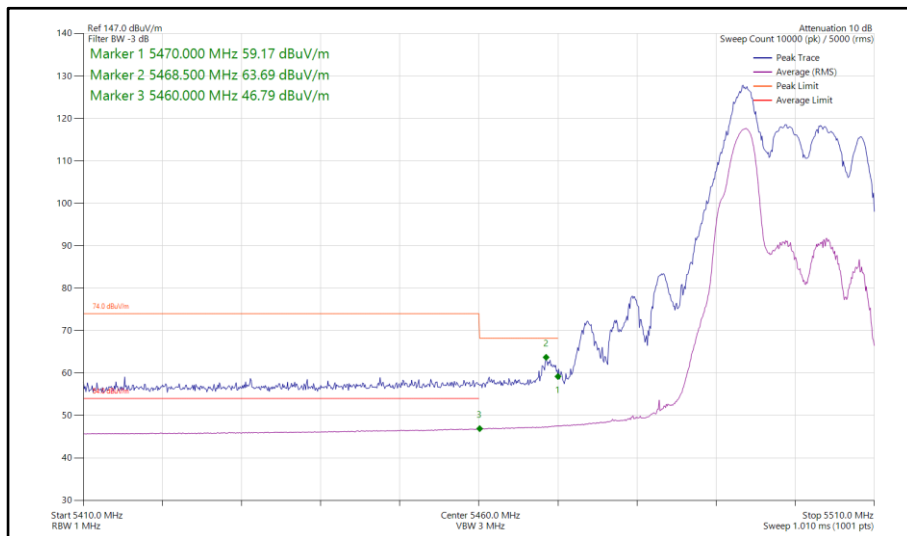
Figure 81 - 802.11ax HE20, RU 52-37, CDD, Core 0-1 - 5500 MHz Band Edge Frequency 5460 MHz
