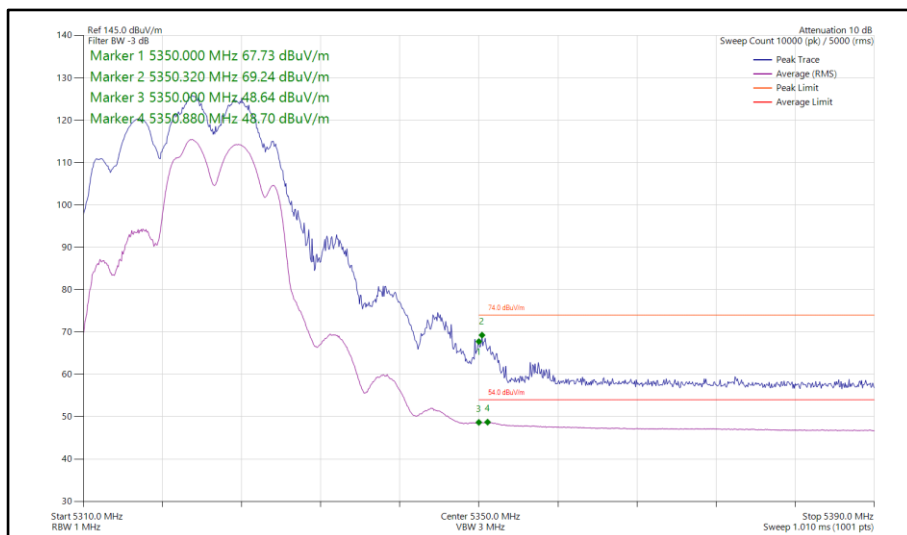
Figure 74 - 802.11be EHT20, RU 106+26-83, CDD, Core 0-1 - 5320 MHz Band Edge Frequency 5350 MHz
