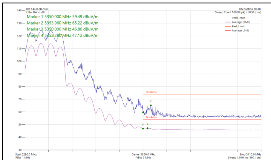
Figure 117 - 802.11ax HE20, SU, TxBF, Core 0-1 - 5300 MHz Band Edge Frequency 5350 MHz
