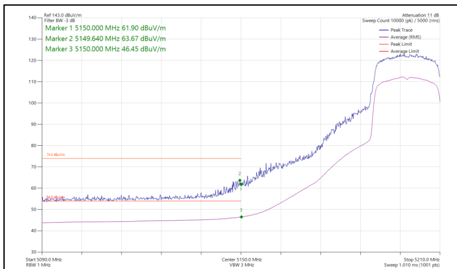
Figure 92 - 802.11ax HE20, SU, SDM, Core 0-1 - 5200 MHz Band Edge Frequency 5150 MHz
