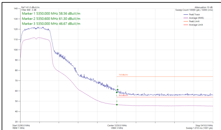
Figure 94 - 802.11n HT20, SDM, Core 0-1 - 5300 MHz Band Edge Frequency 5350 MHz
