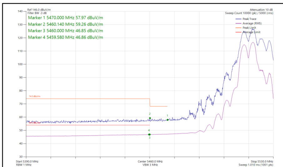
Figure 110 - 802.11be EHT20, RU 106+26-82, SDM, Core 0-1 - 5520 MHz Band Edge Frequency 5460 MHz
