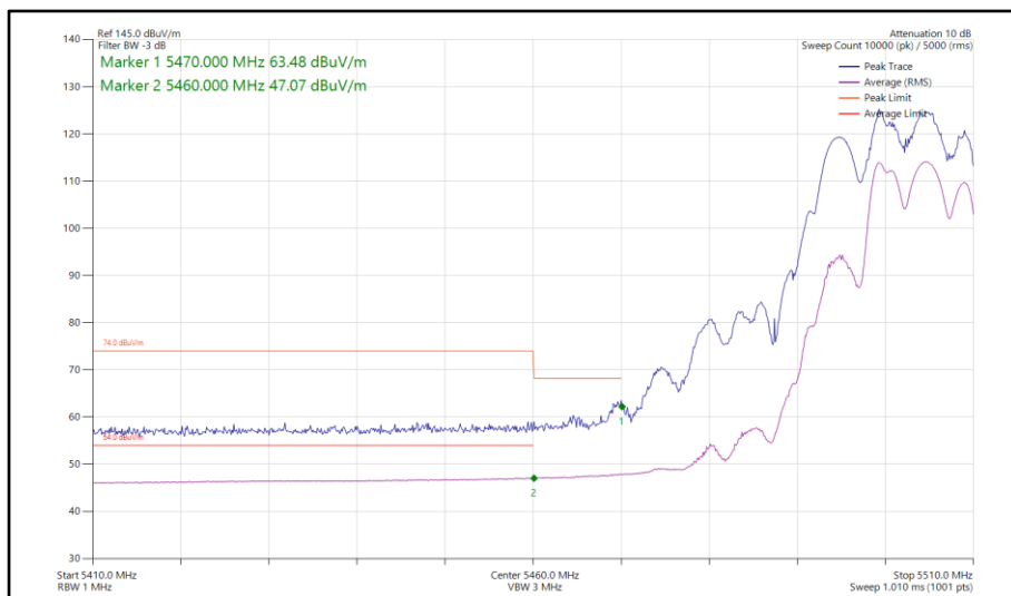
Figure 86 - 802.11be EHT20, RU 106+26-83, CDD, Core 0-1 - 5500 MHz Band Edge Frequency 5460 MHz
