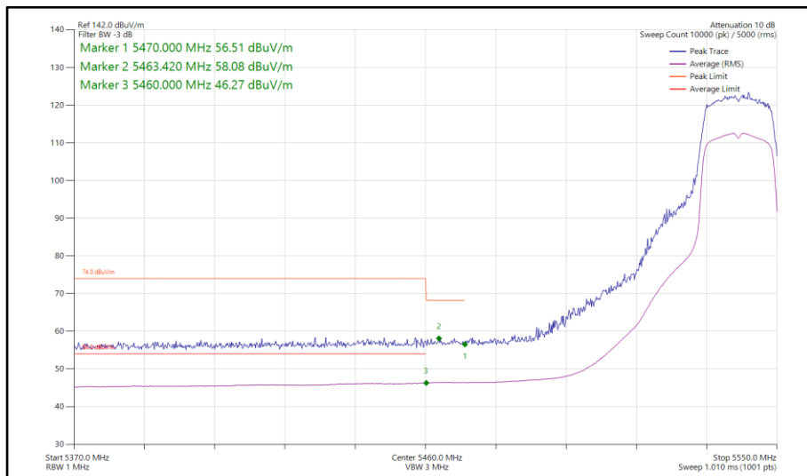
Figure 103 - 802.11n HT20, SDM, Core 0-1 - 5540 MHz Band Edge Frequency 5460 MHz
