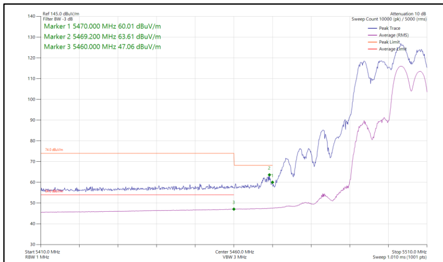
Figure 105 - 802.11ax HE20, RU 106-54, SDM, Core 0-1 - 5500 MHz Band Edge Frequency 5460 MHz
