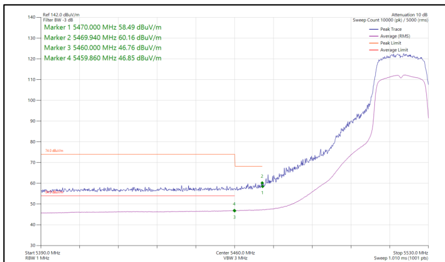
Figure 102 - 802.11n HT20, SDM, Core 0-1 - 5520 MHz Band Edge Frequency 5460 MHz
