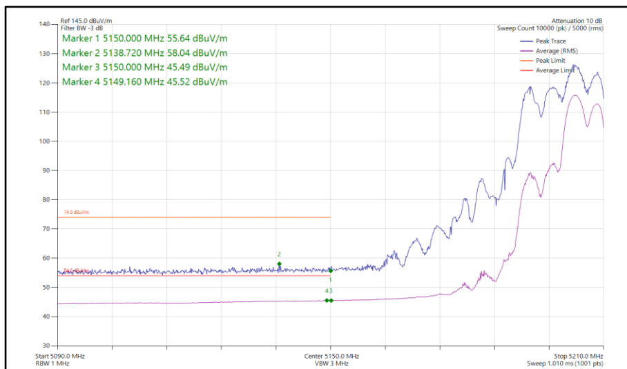
Figure 62 - 802.11ax HE20, RU 106-54, CDD, Core 0-1 - 5200 MHz Band Edge Frequency 5150 MHz
