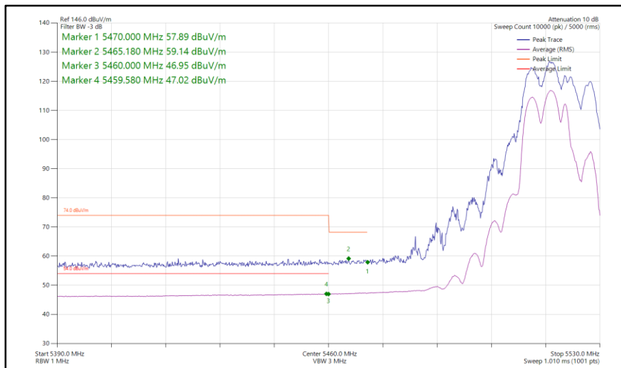
Figure 87 - 802.11be EHT20, RU 106+26-82, CDD, Core 0-1 - 5520 MHz Band Edge Frequency 5460 MHz
