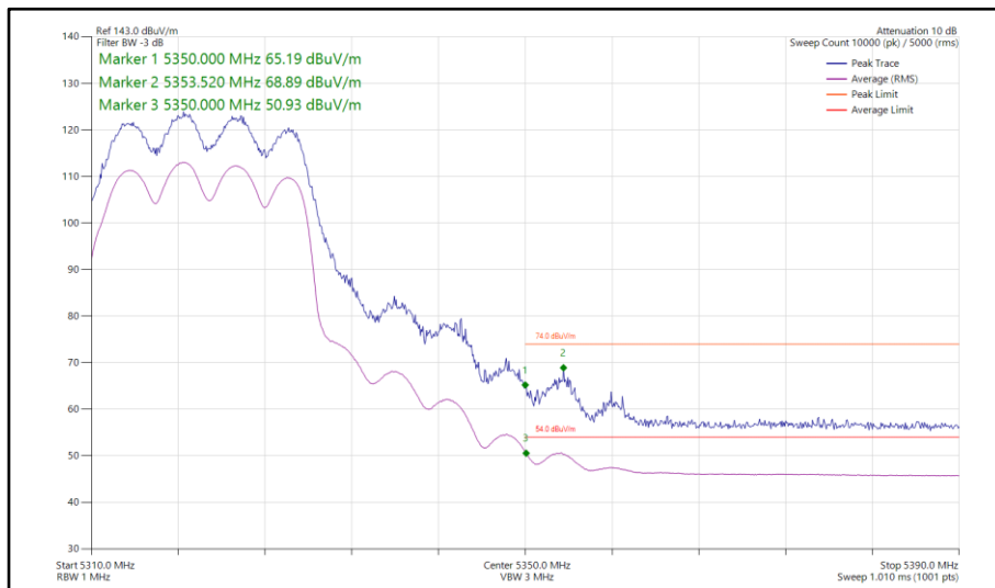
Figure 71 - 802.11ax HE20, SU, CDD, Core 0-1 - 5320 MHz Band Edge Frequency 5350 MHz
