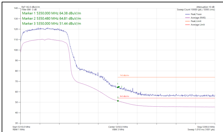
Figure 97 - 802.11ax HE20, SU, SDM, Core 0-1 - 5320 MHz Band Edge Frequency 5350 MHz
