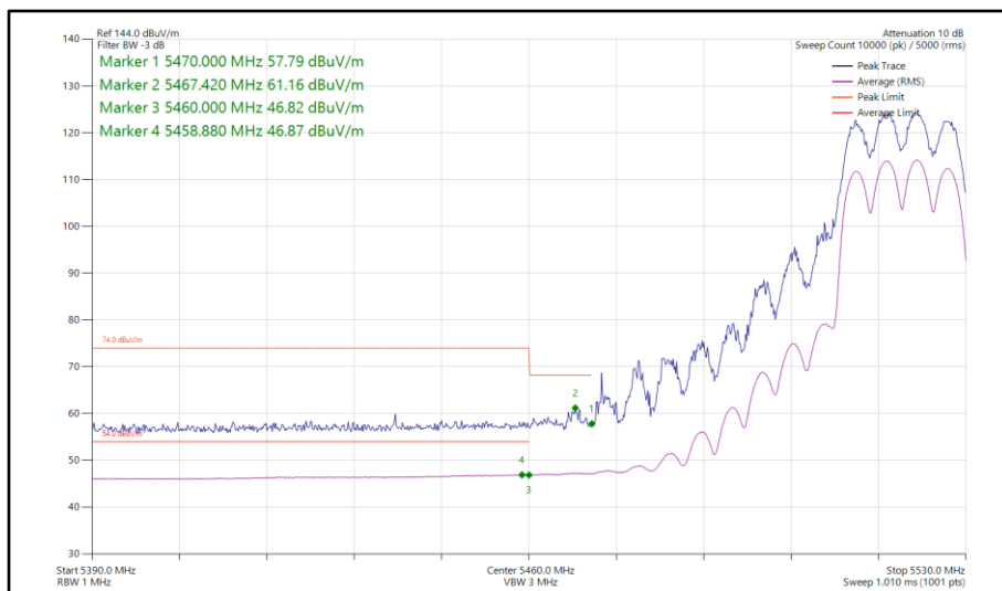
Figure 82 - 802.11ax HE20, SU, CDD, Core 0-1 - 5520 MHz Band Edge Frequency 5460 MHz
