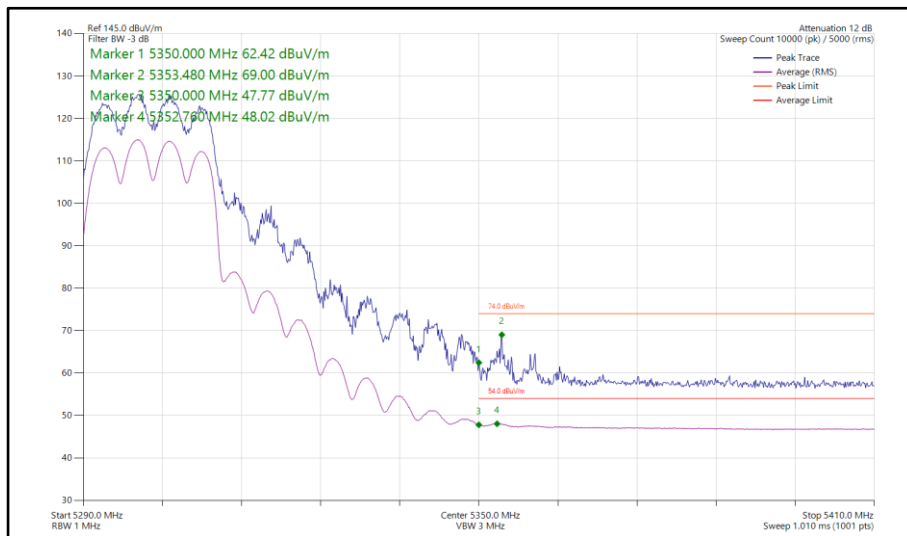
Figure 69 - 802.11ax HE20, SU, CDD, Core 0-1 - 5300 MHz Band Edge Frequency 5350 MHz
