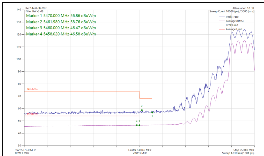
Figure 79 - 802.11n HT20, CDD, Core 0-1 - 5540 MHz Band Edge Frequency 5460 MHz
