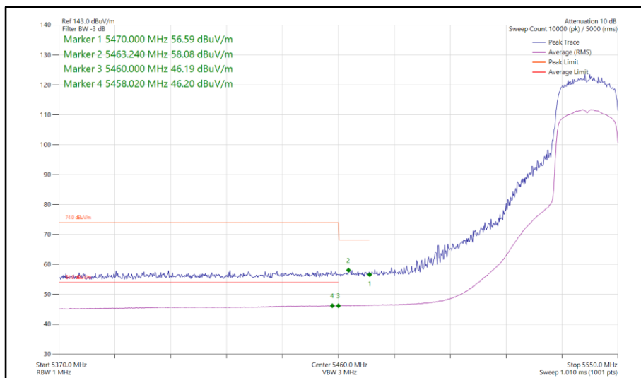
Figure 108 - 802.11ax HE20, SU, SDM, Core 0-1 - 5540 MHz Band Edge Frequency 5460 MHz
