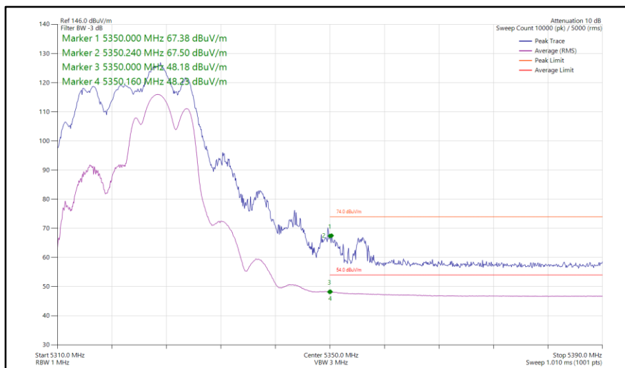
Figure 72 - 802.11ax HE20, RU 106-54, CDD, Core 0-1 - 5320 MHz Band Edge Frequency 5350 MHz
