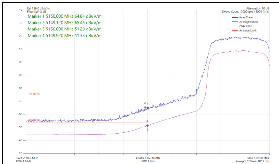
Figure 90 - 802.11ax HE20, SU, SDM, Core 0-1 - 5180 MHz Band Edge Frequency 5150 MHz
