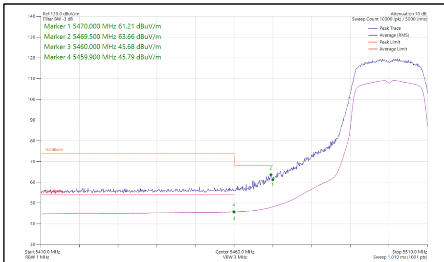
Figure 101 - 802.11n HT20, SDM, Core 0-1 - 5500 MHz Band Edge Frequency 5460 MHz
