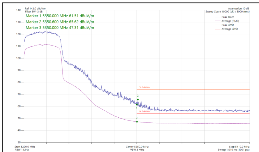
Figure 96 - 802.11ax HE20, SU, SDM, Core 0-1 - 5300 MHz Band Edge Frequency 5350 MHz
