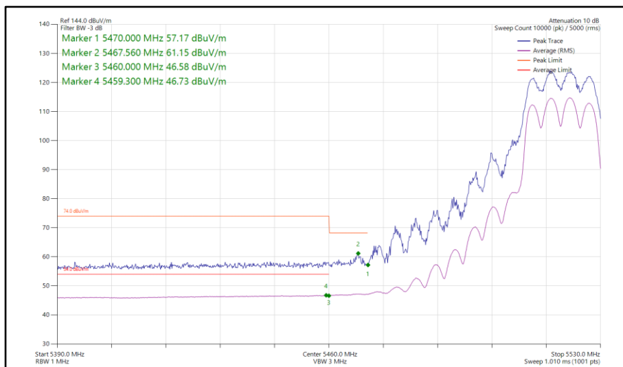
Figure 78 - 802.11n HT20, CDD, Core 0-1 - 5520 MHz Band Edge Frequency 5460 MHz
