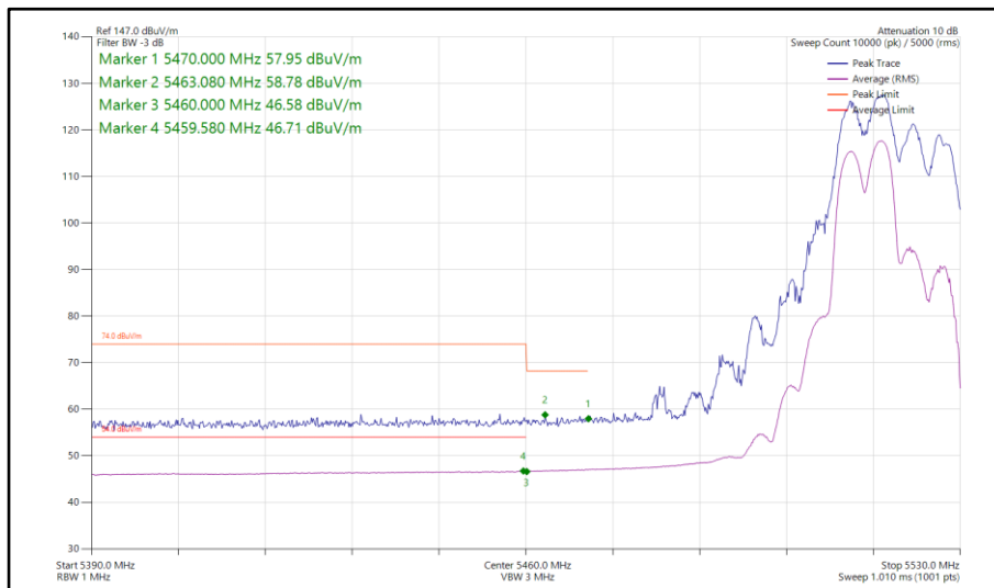
Figure 83 - 802.11ax HE20, RU 106-53, CDD, Core 0-1 - 5520 MHz Band Edge Frequency 5460 MHz
