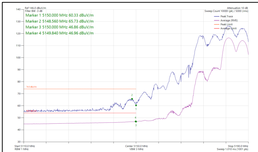
Figure 91 - 802.11ax HE20, RU 106-54, SDM, Core 0-1 - 5180 MHz Band Edge Frequency 5150 MHz
