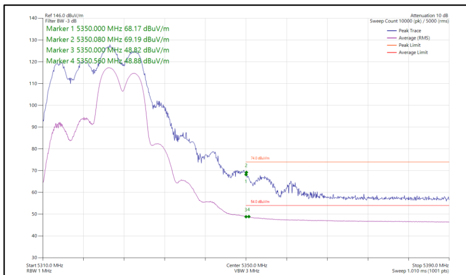
Figure 98 - 802.11ax HE20, RU 106-54, SDM, Core 0-1 - 5320 MHz Band Edge Frequency 5350 MHz
