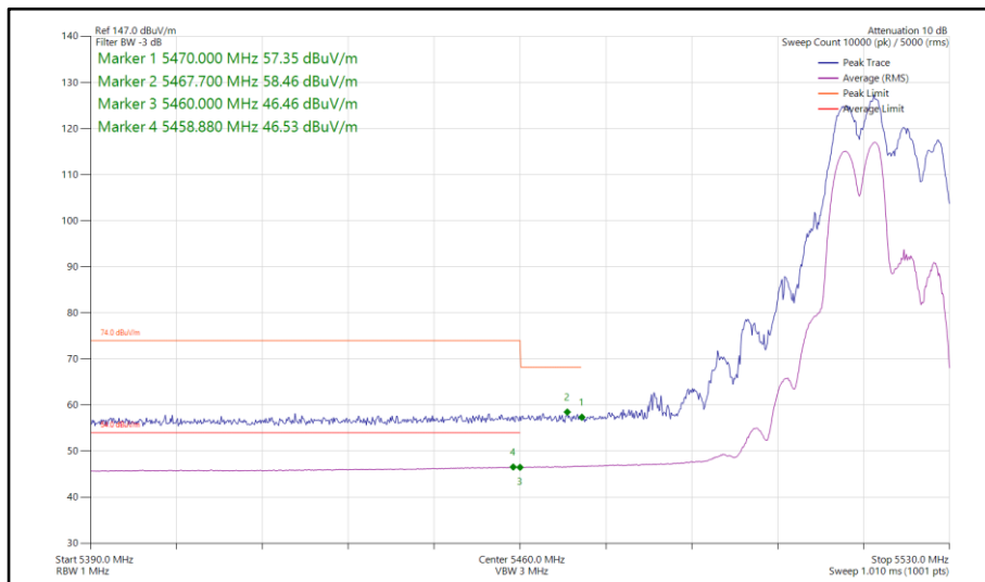
Figure 107 - 802.11ax HE20, RU 106-53, SDM, Core 0-1 - 5520 MHz Band Edge Frequency 5460 MHz
