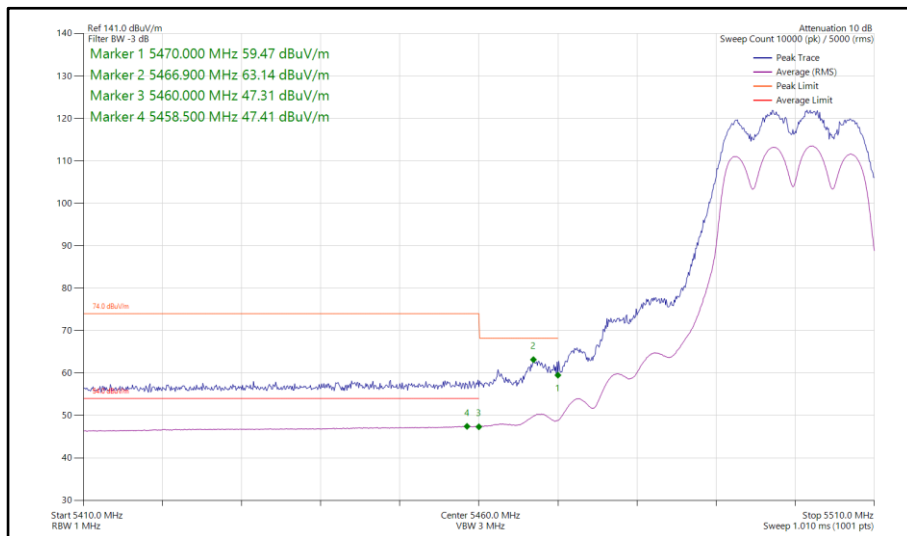
Figure 77 - 802.11n HT20, CDD, Core 0-1 - 5500 MHz Band Edge Frequency 5460 MHz
