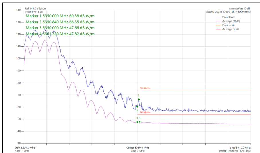
Figure 115 - 802.11ac VHT20, TxBF, Core 0-1 - 5300 MHz Band Edge Frequency 5350 MHz
