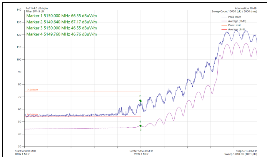
Figure 61 - 802.11ax HE20, SU, CDD, Core 0-1 - 5200 MHz Band Edge Frequency 5150 MHz
