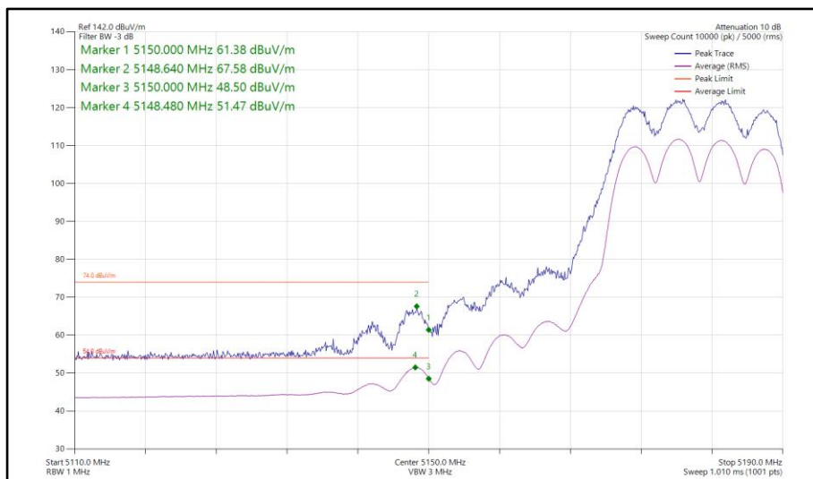
Figure 113 - 802.11ax HE20, SU, TxBF, Core 0-1 - 5180 MHz Band Edge Frequency 5150 MHz
