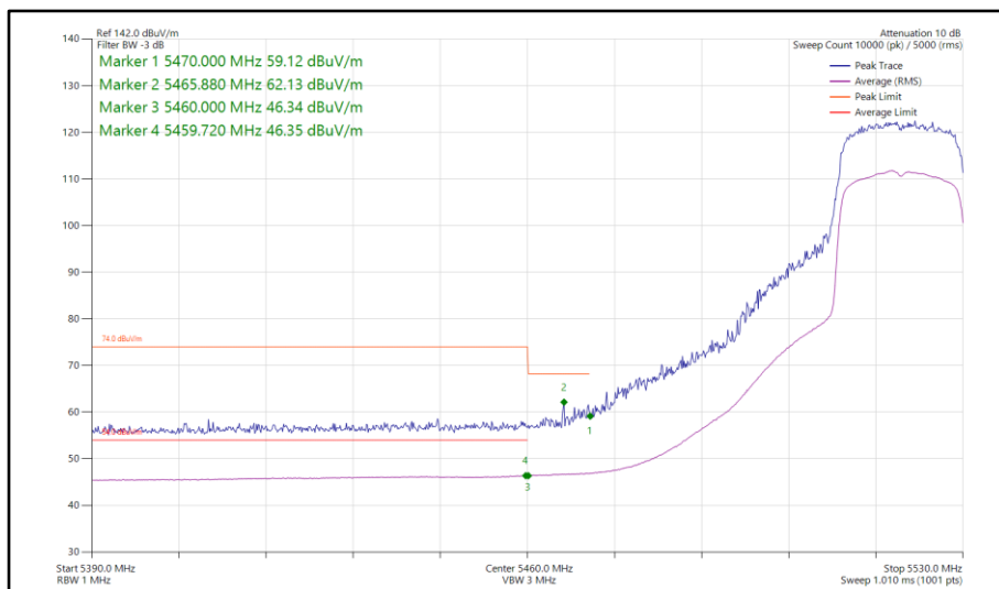
Figure 106 - 802.11ax HE20, SU, SDM, Core 0-1 - 5520 MHz Band Edge Frequency 5460 MHz
