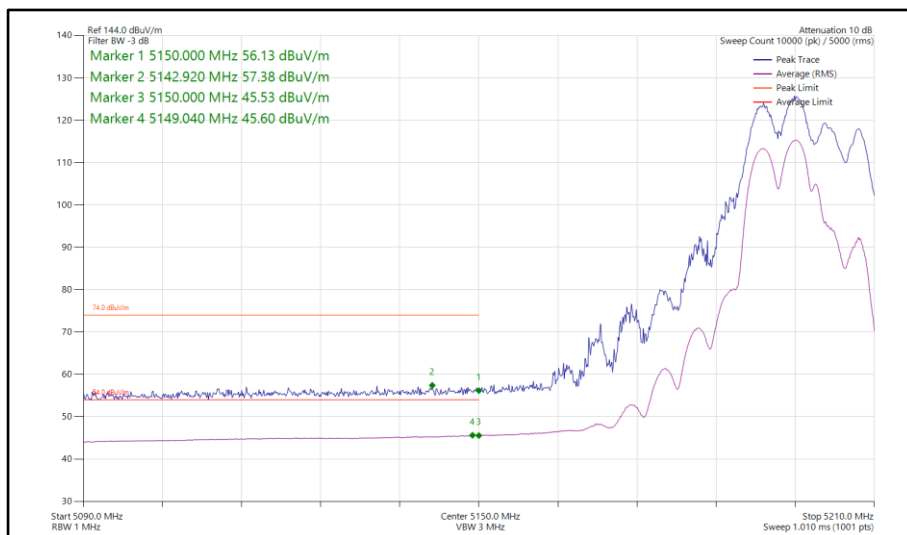
Figure 64 - 802.11be EHT20, RU 106+26-82, CDD, Core 0-1 - 5200 MHz Band Edge Frequency 5150 MHz
