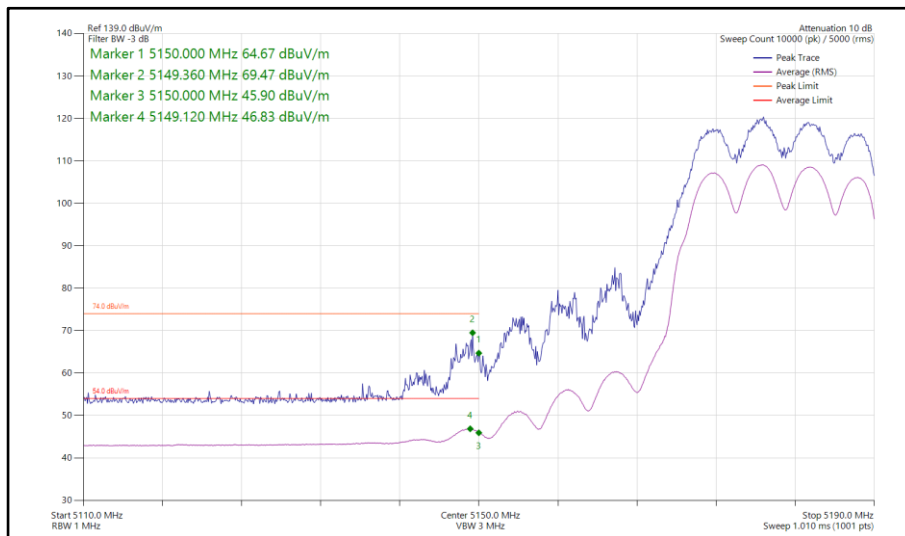
Figure 59 - 802.11ax HE20, SU, CDD, Core 0-1 - 5180 MHz Band Edge Frequency 5150 MHz
