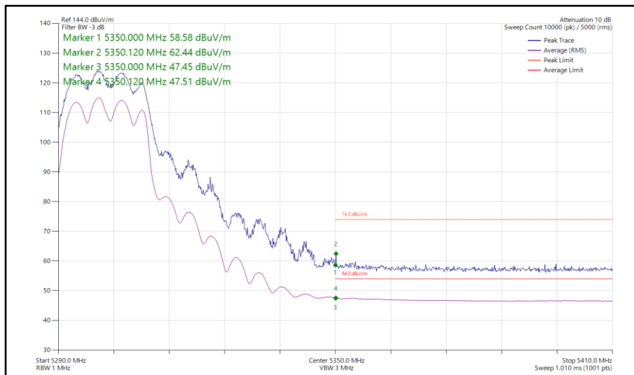
Figure 65 - 802.11a, CDD, Core 0-1 - 5300 MHz Band Edge Frequency 5350 MHz
