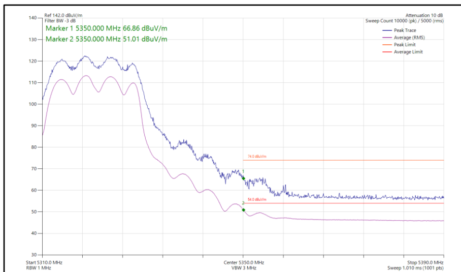
Figure 68 - 802.11n HT20, CDD, Core 0-1 - 5320 MHz Band Edge Frequency 5350 MHz
