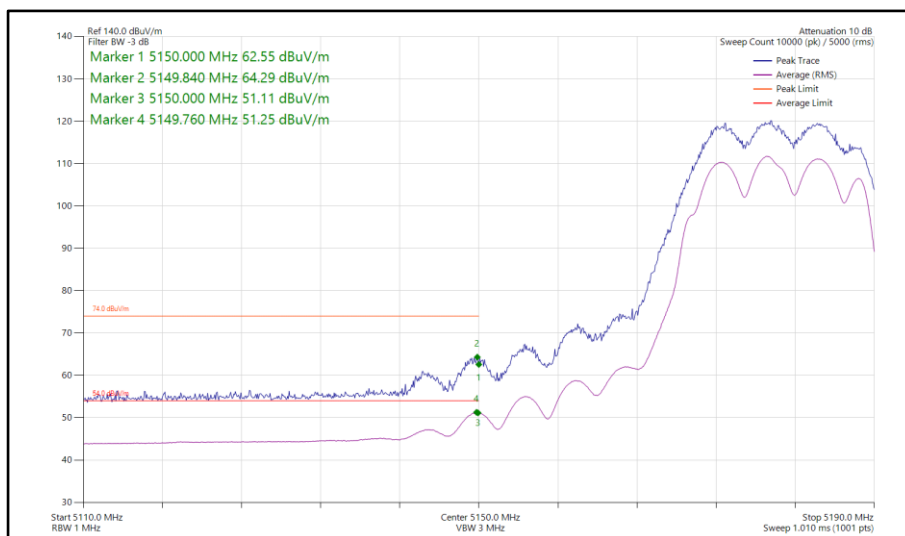
Figure 111 - 802.11ac VHT20, TxBF, Core 0-1 - 5180 MHz Band Edge Frequency 5150 MHz
