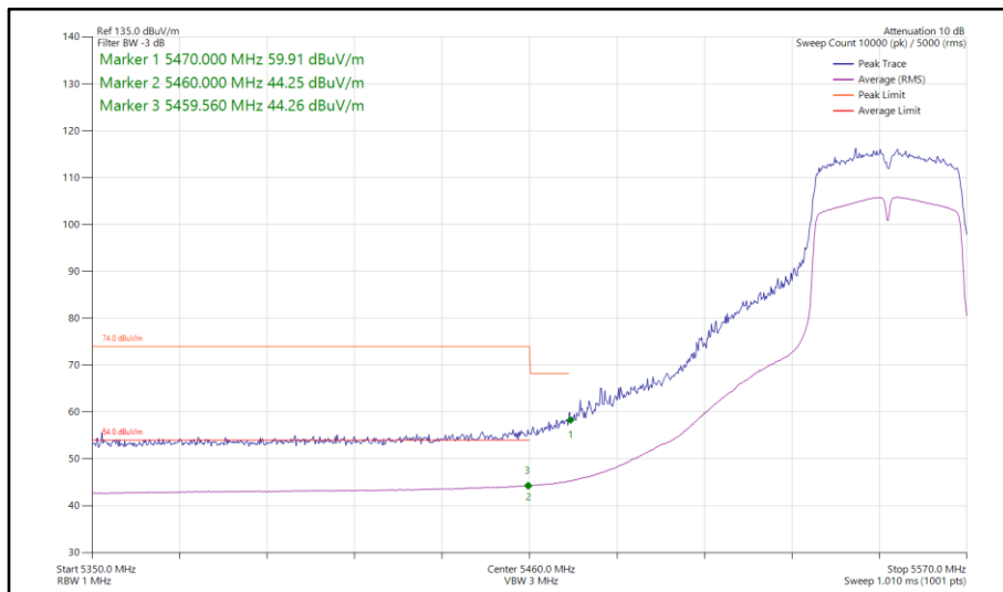
Figure 180 - 802.11n HT40, SISO, Core 1 - 5550 MHz Band Edge Frequency 5460 MHz
