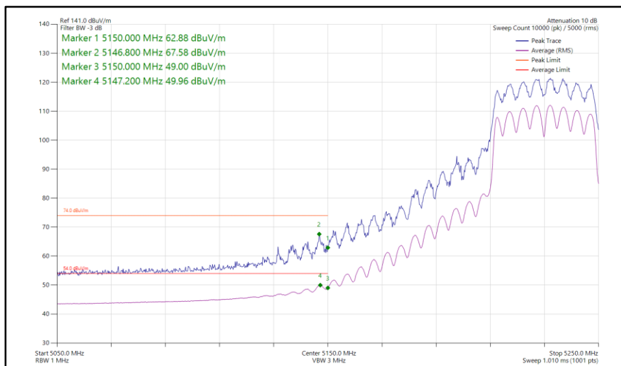
Figure 190 - 802.11n HT40, CDD, Core 0-1 - 5230 MHz Band Edge Frequency 5150 MHz
