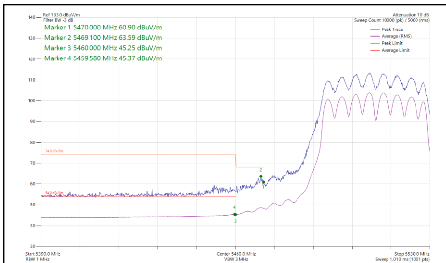
Figure 210 - 802.11n HT40, CDD, Core 0-1 - 5510 MHz Band Edge Frequency 5460 MHz
