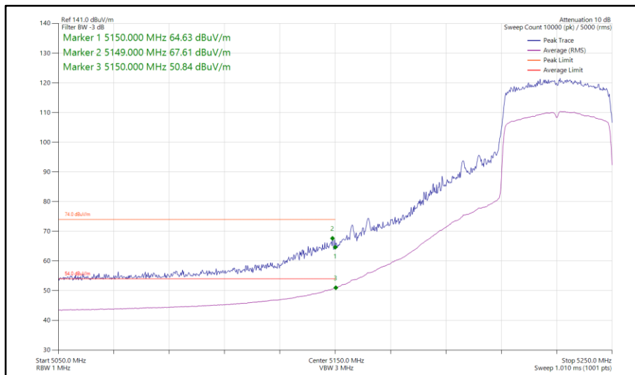
Figure 222 - 802.11ax HE40, SU, SDM, Core 0-1 - 5230 MHz Band Edge Frequency 5150 MHz
