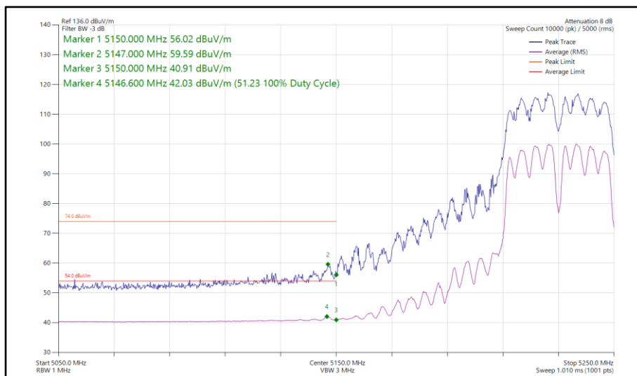
Figure 188 - 802.11a a40, CDD, Core 0-1 - 5230 MHz Band Edge Frequency 5150 MHz
