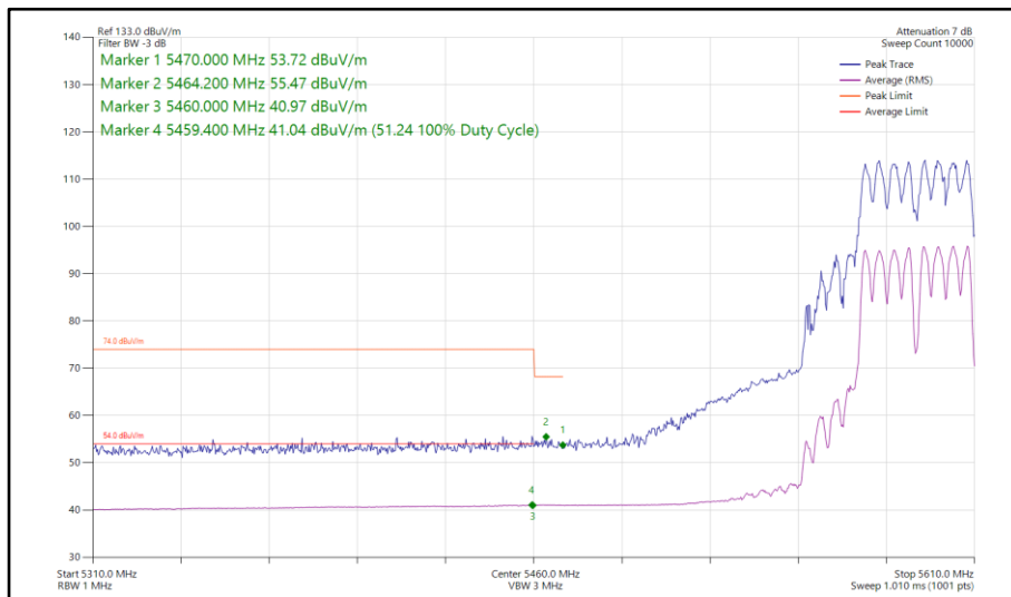
Figure 209 - 802.11a a40, CDD, Core 0-1 - 5590 MHz Band Edge Frequency 5460 MHz
