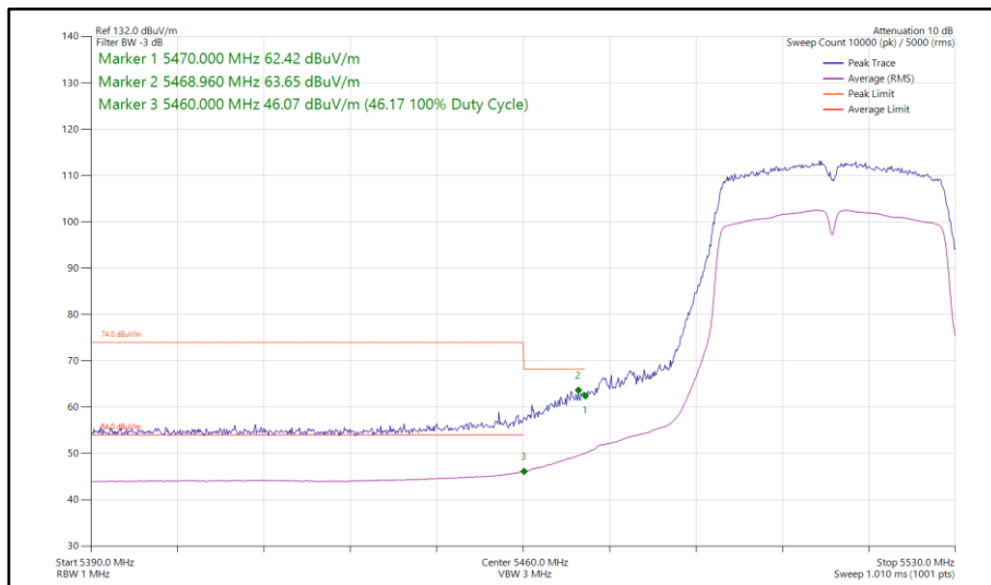
Figure 234 - 802.11n HT40, SDM, Core 0-1 - 5510 MHz Band Edge Frequency 5460 MHz
