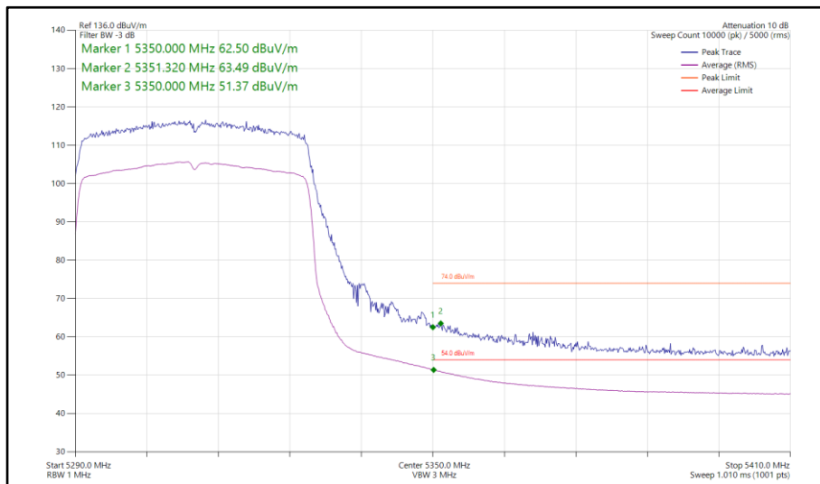
Figure 230 - 802.11ax HE40, SU, SDM, Core 0-1 - 5310 MHz Band Edge Frequency 5350 MHz
