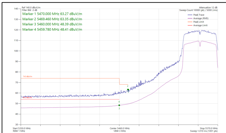
Figure 235 - 802.11n HT40, SDM, Core 0-1 - 5550 MHz Band Edge Frequency 5460 MHz
