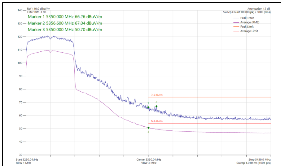
Figure 228 - 802.11ax HE40, SU, SDM, Core 0-1 - 5270 MHz Band Edge Frequency 5350 MHz
