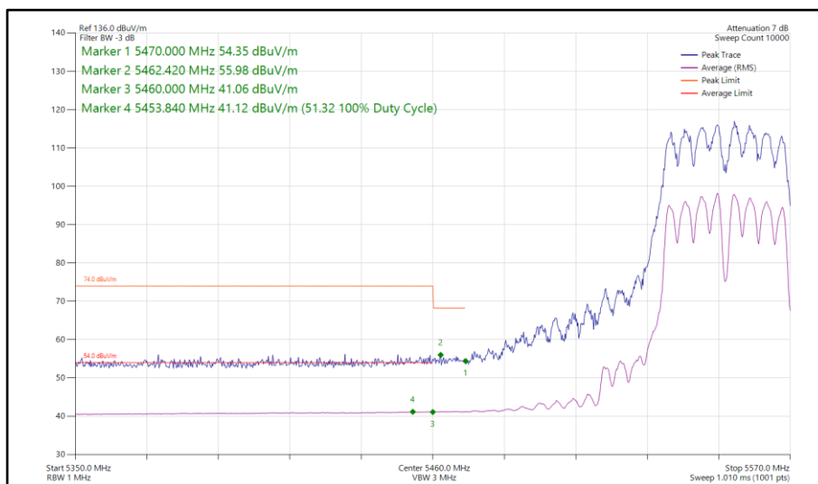
Figure 208 - 802.11a a40, CDD, Core 0-1 - 5550 MHz Band Edge Frequency 5460 MHz
