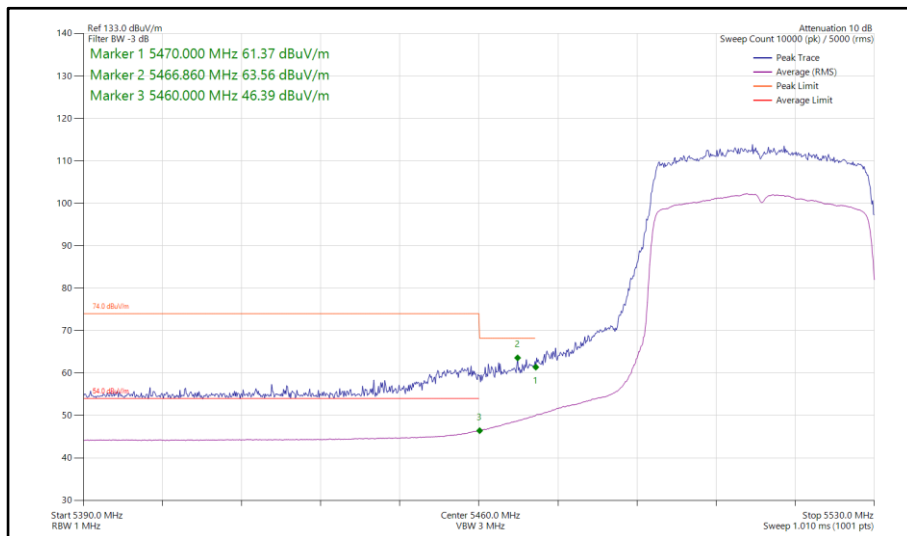
Figure 236 - 802.11ax HE40, SU, SDM, Core 0-1 - 5510 MHz Band Edge Frequency 5460 MHz
