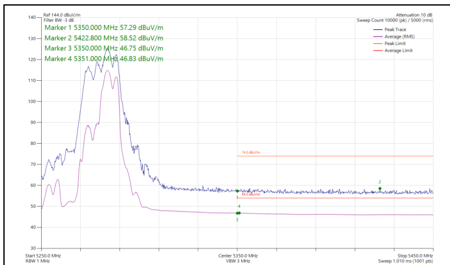
Figure 202 - 802.11ax HE40, RU 106-56, CDD, Core 0-1 - 5270 MHz Band Edge Frequency 5350 MHz
