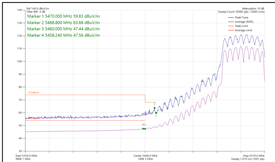
Figure 211 - 802.11n HT40, CDD, Core 0-1 - 5550 MHz Band Edge Frequency 5460 MHz
