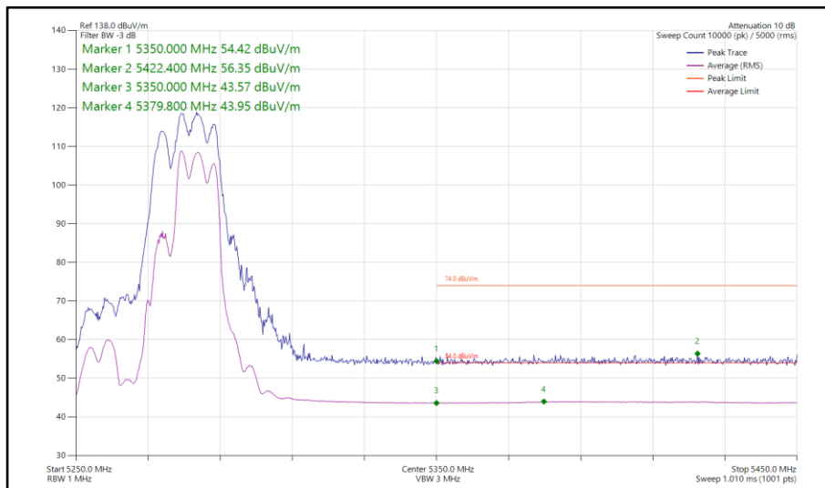
Figure 232 - 802.11be EHT40, RU 106+26-85, SDM, Core 0-1 - 5270 MHz Band Edge Frequency 5350 MHz
