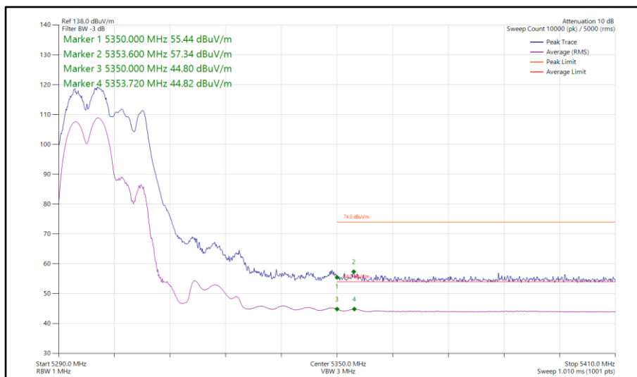
Figure 233 - 802.11be EHT40, RU 106+26-82, SDM, Core 0-1 - 5310 MHz Band Edge Frequency 5350 MHz
