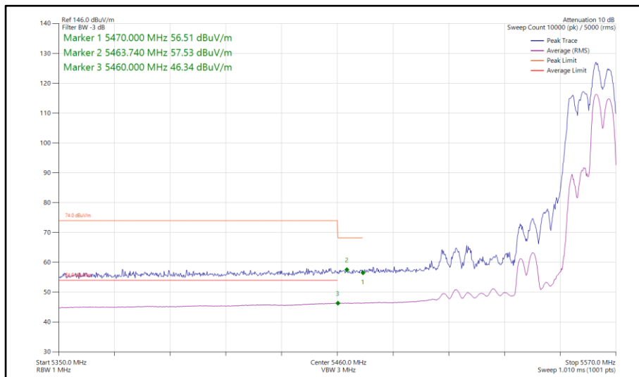
Figure 215 - 802.11ax HE40, RU 106-56, CDD, Core 0-1 - 5550 MHz Band Edge Frequency 5460 MHz
