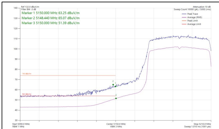
Figure 220 - 802.11ax HE40, SU, SDM, Core 0-1 - 5190 MHz Band Edge Frequency 5150 MHz
