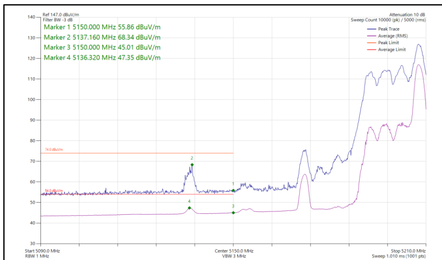
Figure 192 - 802.11ax HE40, RU 26-17, CDD, Core 0-1 - 5190 MHz Band Edge Frequency 5150 MHz
