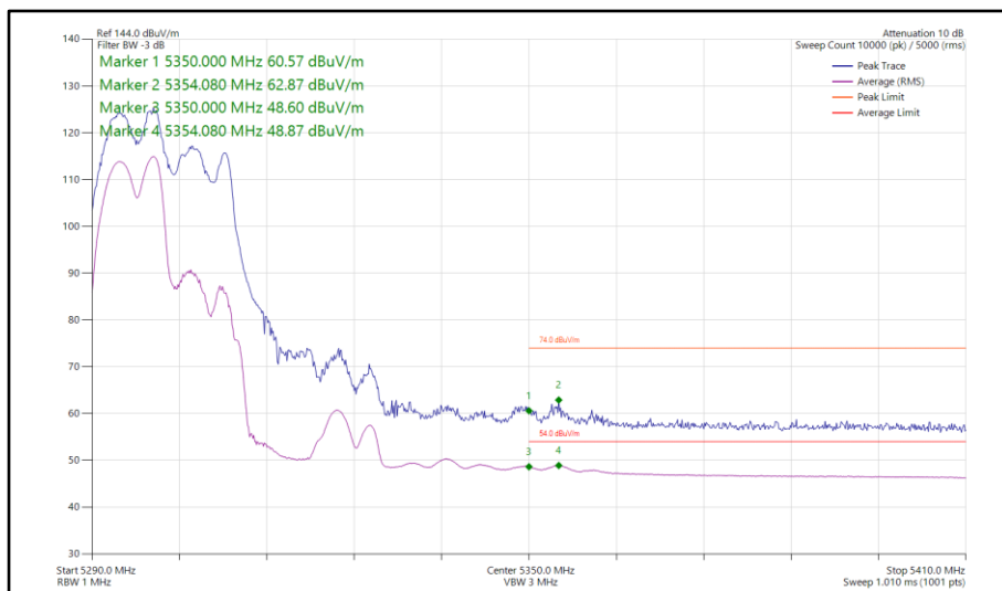
Figure 204 - 802.11ax HE40, RU 106-53, CDD, Core 0-1 - 5310 MHz Band Edge Frequency 5350 MHz
