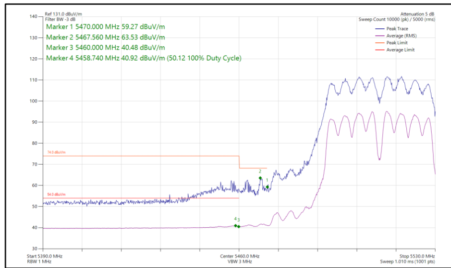
Figure 207 - 802.11a a40, CDD, Core 0-1 - 5510 MHz Band Edge Frequency 5460 MHz
