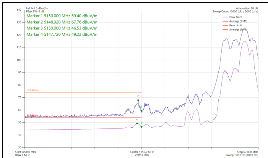
Figure 224 - 802.11be EHT40, RU 52+26-75, SDM, Core 0-1 - 5190 MHz Band Edge Frequency 5150 MHz
