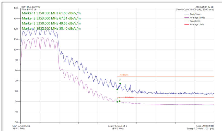
Figure 199 - 802.11n HT40, CDD, Core 0-1 - 5270 MHz Band Edge Frequency 5350 MHz
