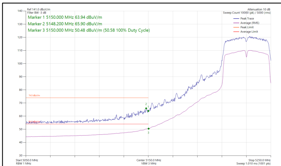
Figure 219 - 802.11n HT40, SDM, Core 0-1 - 5230 MHz Band Edge Frequency 5150 MHz
