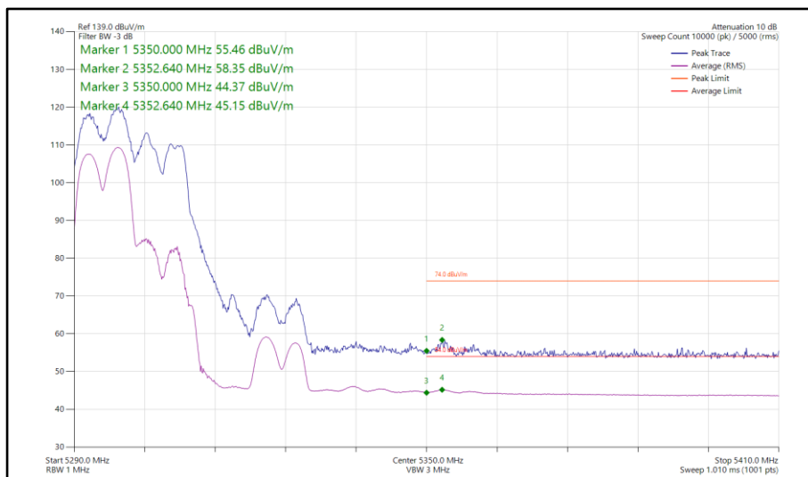
Figure 231 - 802.11ax HE40, RU 106-53, SDM, Core 0-1 - 5310 MHz Band Edge Frequency 5350 MHz
