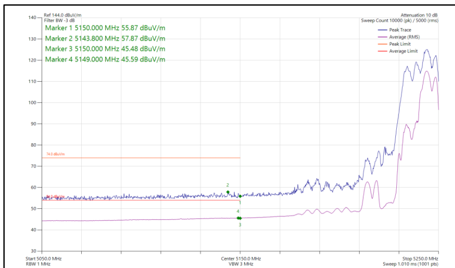
Figure 223 - 802.11ax HE40, RU 106-56, SDM, Core 0-1 - 5230 MHz Band Edge Frequency 5150 MHz
