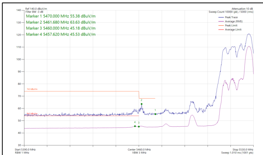
Figure 237 - 802.11ax HE40, RU 52-44, SDM, Core 0-1 - 5510 MHz Band Edge Frequency 5460 MHz
