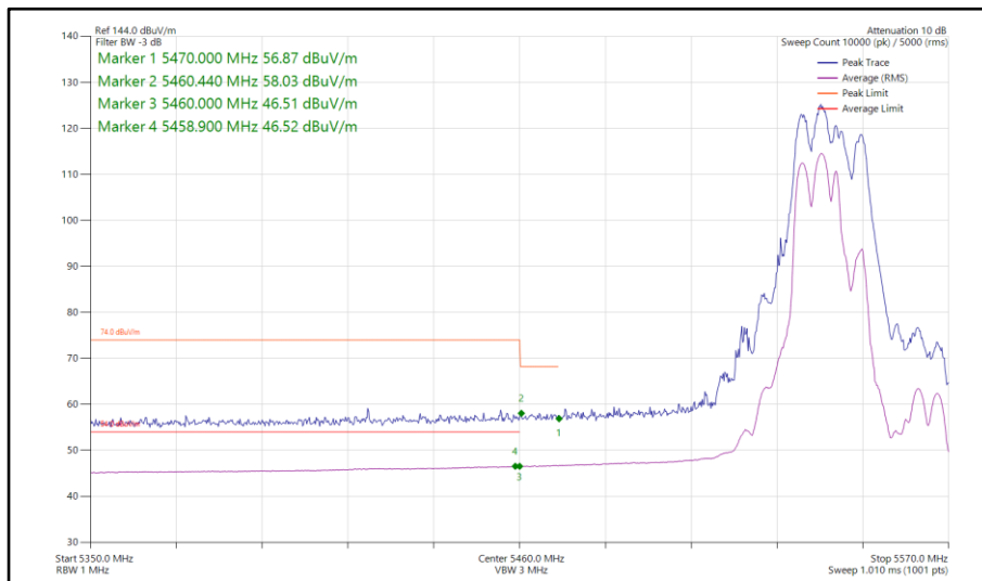
Figure 217 - 802.11be EHT40, RU 106+26-82, CDD, Core 0-1 - 5550 MHz Band Edge Frequency 5460 MHz
