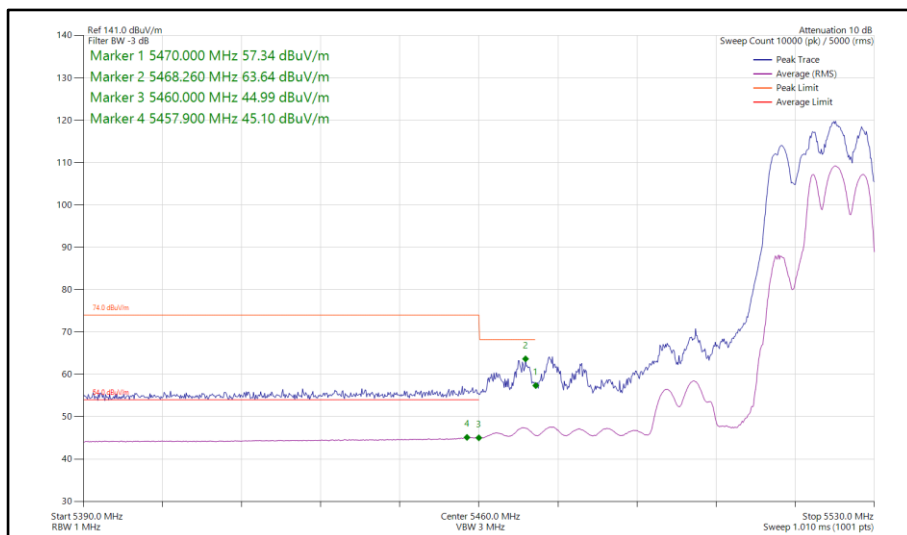
Figure 216 - 802.11be EHT40, RU 106+26-85, CDD, Core 0-1 - 5510 MHz Band Edge Frequency 5460 MHz
