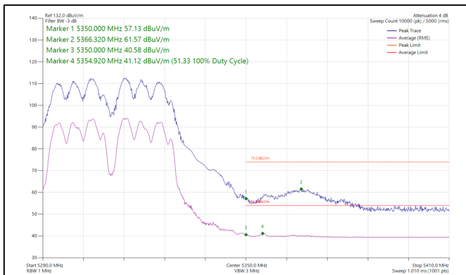
Figure 198 - 802.11a a40, CDD, Core 0-1 - 5310 MHz Band Edge Frequency 5350 MHz
