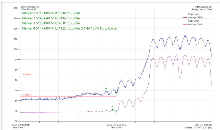
Figure 187 - 802.11a a40, CDD, Core 0-1 - 5190 MHz Band Edge Frequency 5150 MHz
