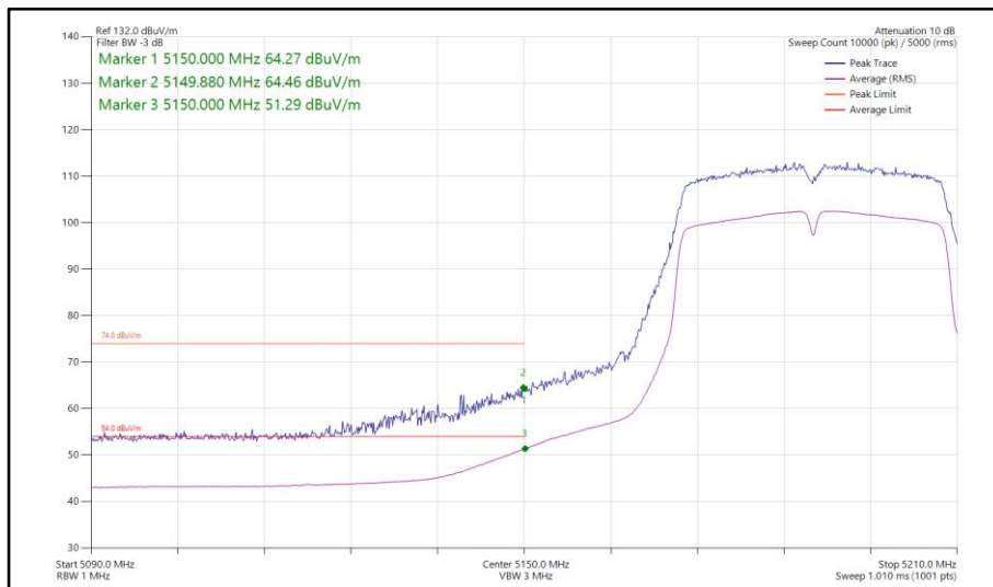
Figure 218 - 802.11n HT40, SDM, Core 0-1 - 5190 MHz Band Edge Frequency 5150 MHz
