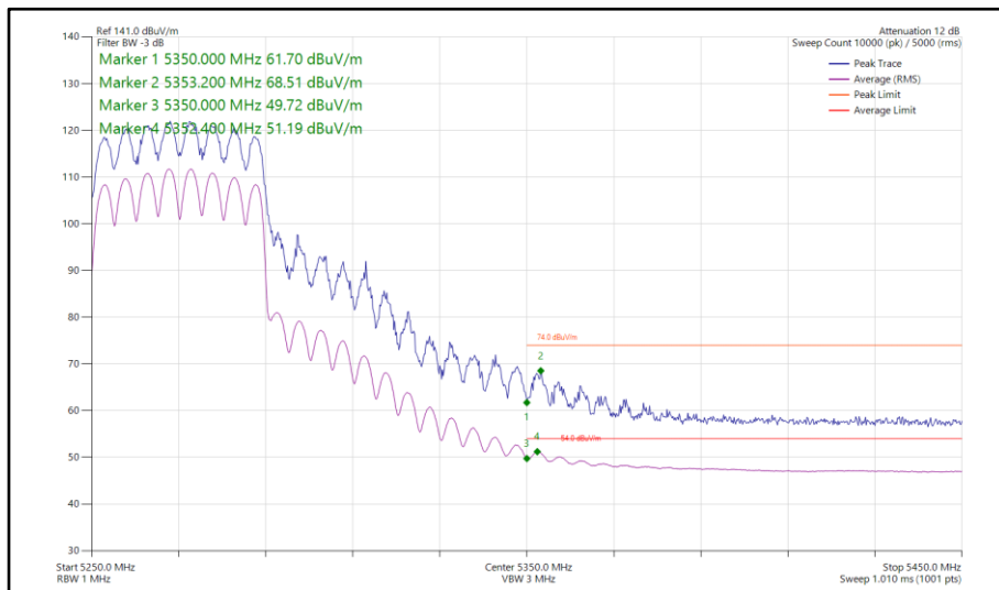
Figure 201 - 802.11ax HE40, SU, CDD, Core 0-1 - 5270 MHz Band Edge Frequency 5350 MHz
