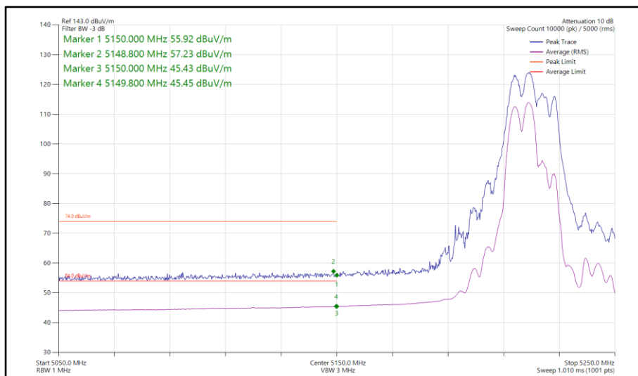
Figure 225 - 802.11be EHT40, RU 106+26-82, SDM, Core 0-1 - 5230 MHz Band Edge Frequency 5150 MHz
