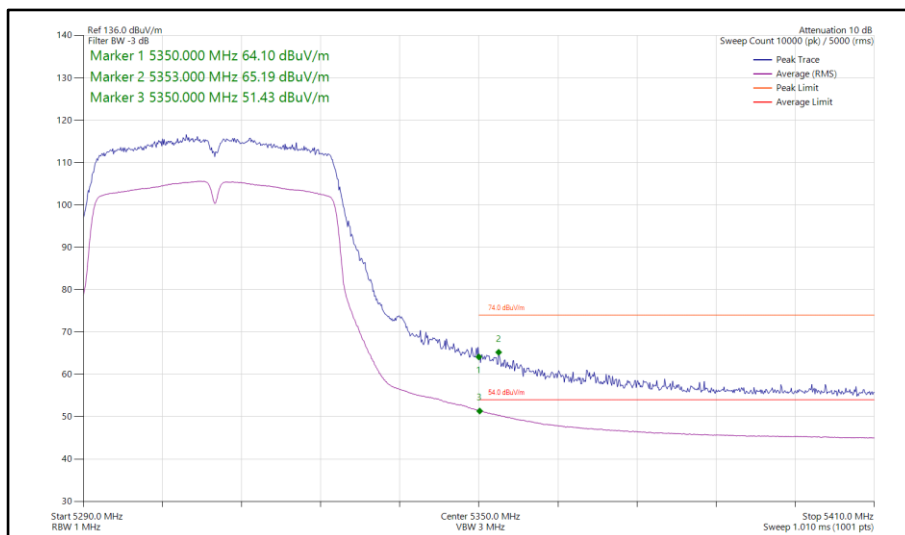
Figure 227 - 802.11n HT40, SDM, Core 0-1 - 5310 MHz Band Edge Frequency 5350 MHz
