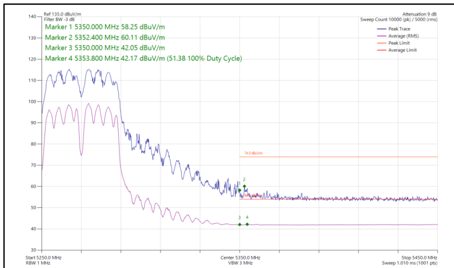
Figure 197 - 802.11a a40, CDD, Core 0-1 - 5270 MHz Band Edge Frequency 5350 MHz
