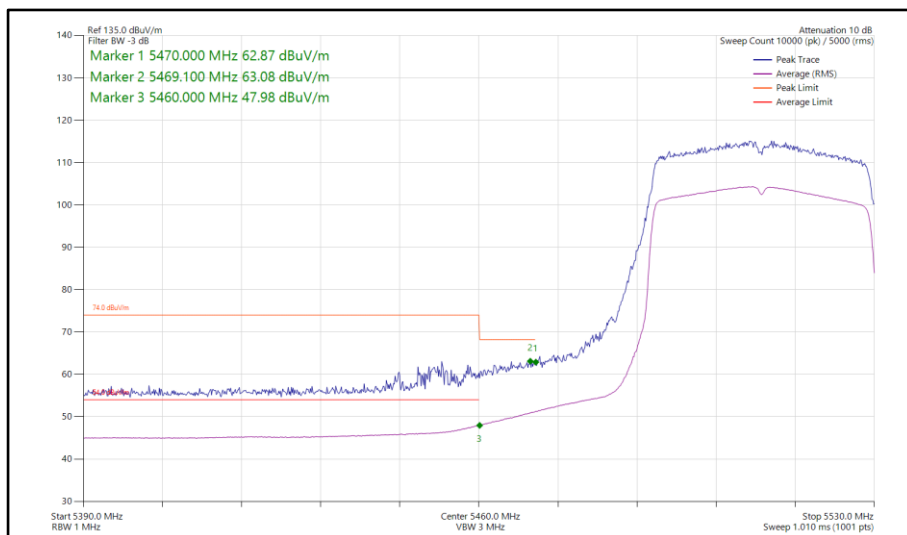
Figure 181 - 802.11ax HE40, SU, SISO, Core 1 - 5510 MHz Band Edge Frequency 5460 MHz
