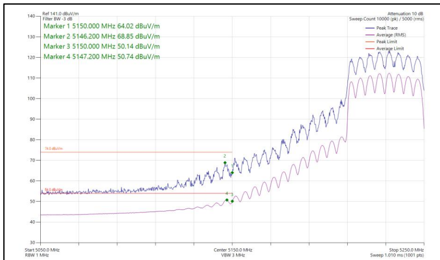
Figure 193 - 802.11ax HE40, SU, CDD, Core 0-1 - 5230 MHz Band Edge Frequency 5150 MHz
