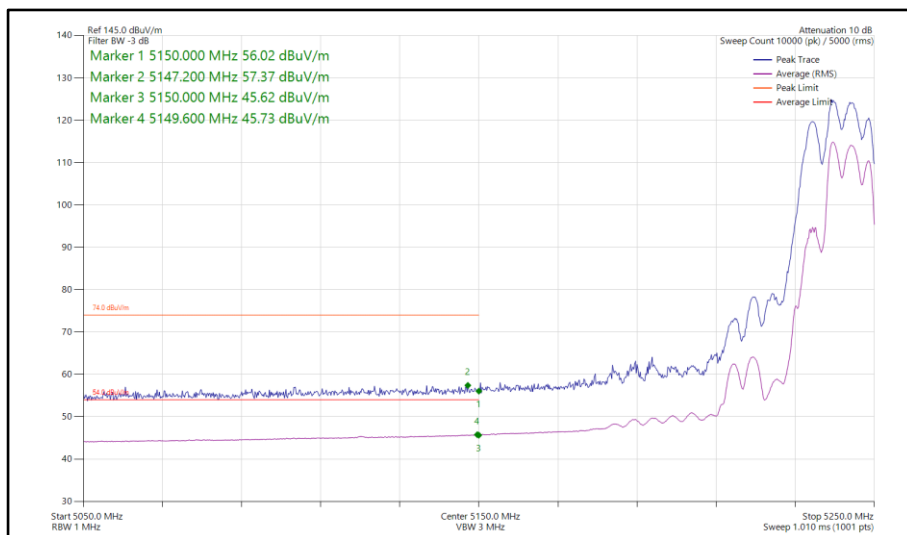
Figure 196 - 802.11be EHT40, RU 106+26-85, CDD, Core 0-1 - 5230 MHz Band Edge Frequency 5150 MHz
