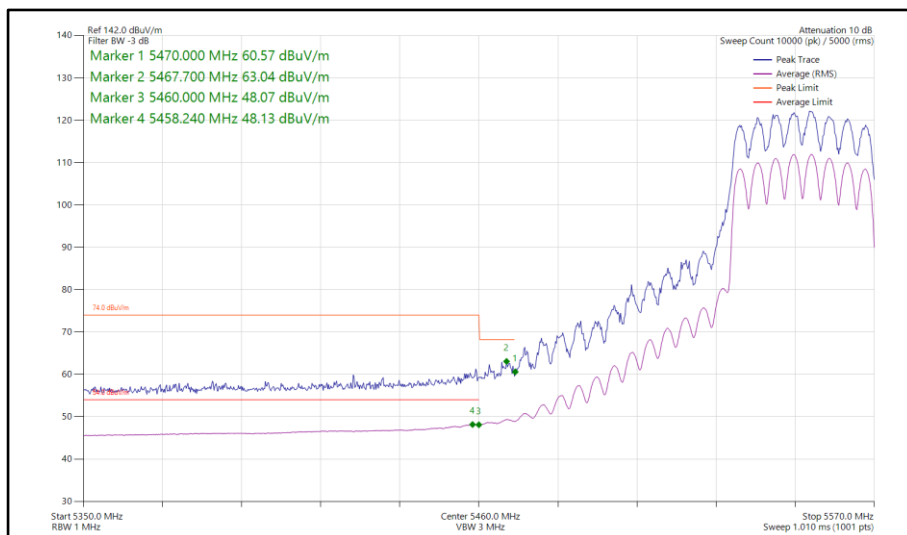
Figure 214 - 802.11ax HE40, SU, CDD, Core 0-1 - 5550 MHz Band Edge Frequency 5460 MHz
