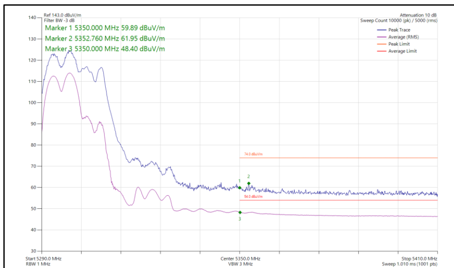
Figure 206 - 802.11be EHT40, RU 106+26-82, CDD, Core 0-1 - 5310 MHz Band Edge Frequency 5350 MHz
