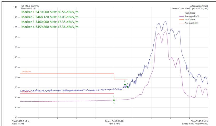
Figure 213 - 802.11ax HE40, RU 106-53, CDD, Core 0-1 - 5510 MHz Band Edge Frequency 5460 MHz
