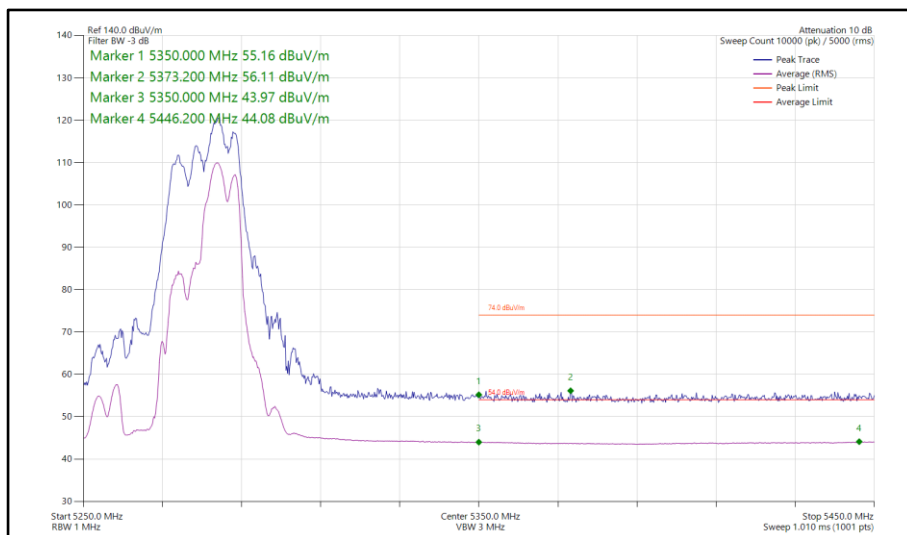
Figure 229 - 802.11ax HE40, RU 106-56, SDM, Core 0-1 - 5270 MHz Band Edge Frequency 5350 MHz
