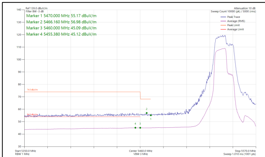
Figure 186 - 802.11be EHT40, RU 106+26-82, SISO, Core 1 - 5550 MHz Band Edge Frequency 5460 MHz
