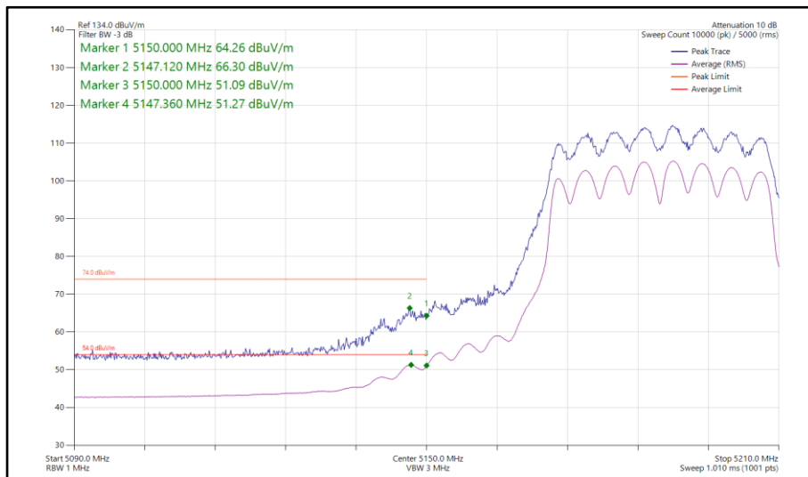
Figure 189 - 802.11n HT40, CDD, Core 0-1 - 5190 MHz Band Edge Frequency 5150 MHz
