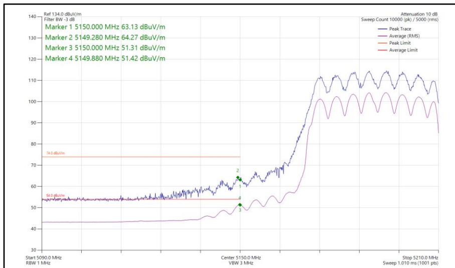
Figure 191 - 802.11ax HE40, SU, CDD, Core 0-1 - 5190 MHz Band Edge Frequency 5150 MHz
