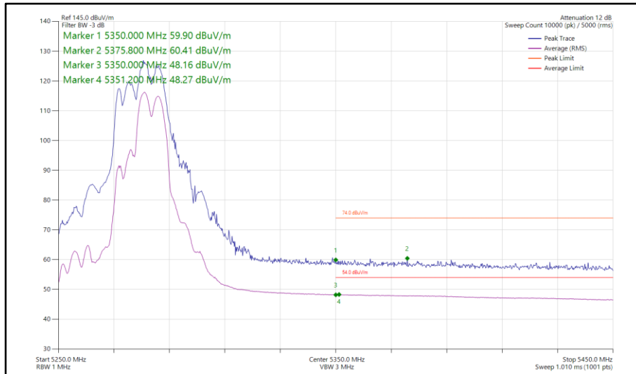
Figure 205 - 802.11be EHT40, RU 106+26-85, CDD, Core 0-1 - 5270 MHz Band Edge Frequency 5350 MHz
