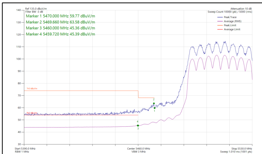
Figure 212 - 802.11ax HE40, SU, CDD, Core 0-1 - 5510 MHz Band Edge Frequency 5460 MHz
