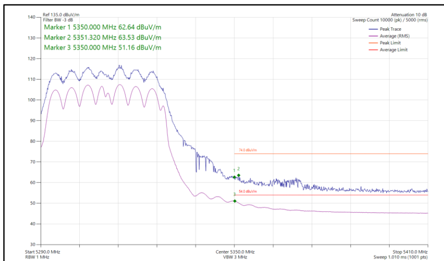
Figure 200 - 802.11n HT40, CDD, Core 0-1 - 5310 MHz Band Edge Frequency 5350 MHz
