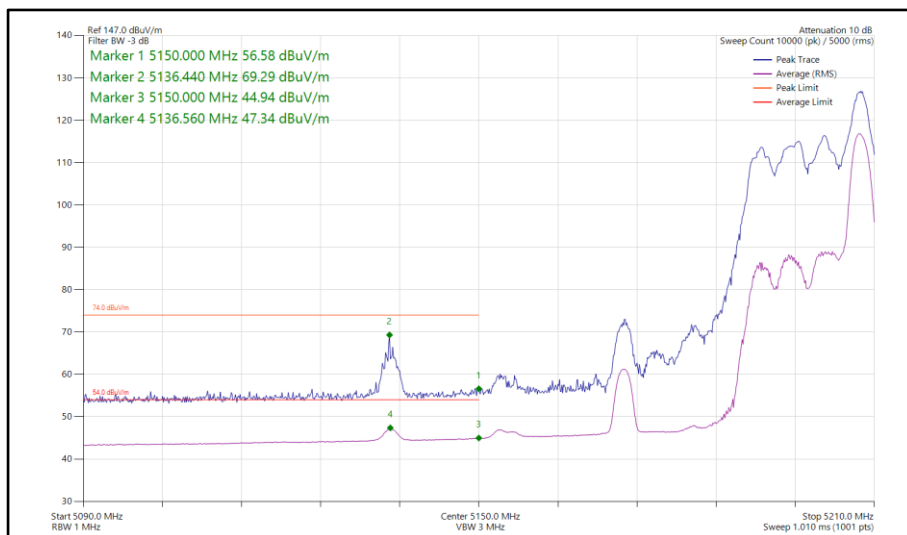
Figure 221 - 802.11ax HE40, RU 26-17, SDM, Core 0-1 - 5190 MHz Band Edge Frequency 5150 MHz
