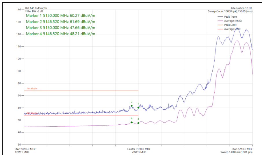
Figure 195 - 802.11be EHT40, RU 106+26-85, CDD, Core 0-1 - 5190 MHz Band Edge Frequency 5150 MHz
