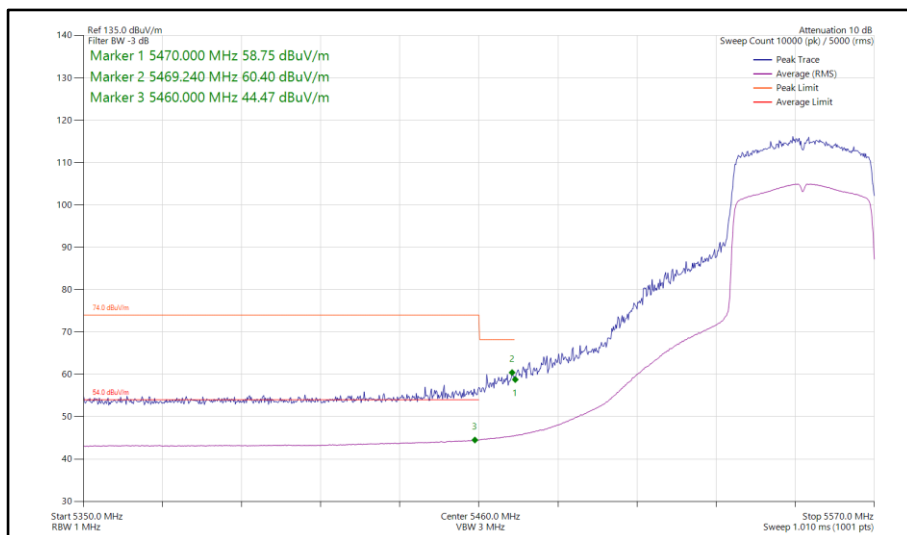
Figure 183 - 802.11ax HE40, SU, SISO, Core 1 - 5550 MHz Band Edge Frequency 5460 MHz
