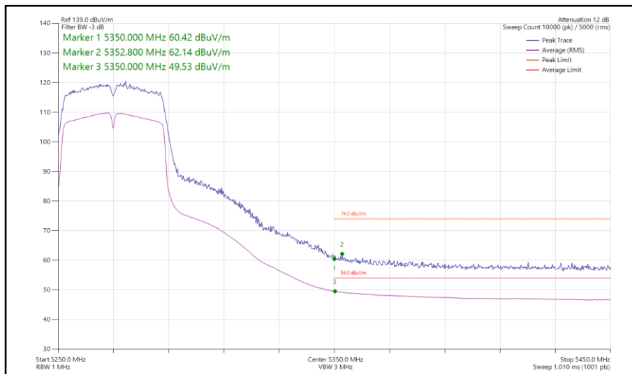
Figure 226 - 802.11n HT40, SDM, Core 0-1 - 5270 MHz Band Edge Frequency 5350 MHz
