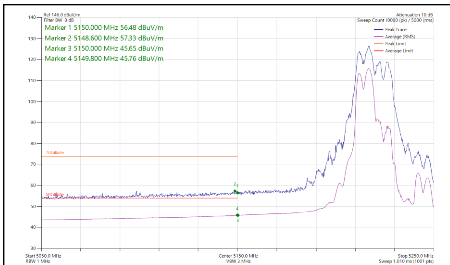
Figure 194 - 802.11ax HE40, RU 106-53, CDD, Core 0-1 - 5230 MHz Band Edge Frequency 5150 MHz
