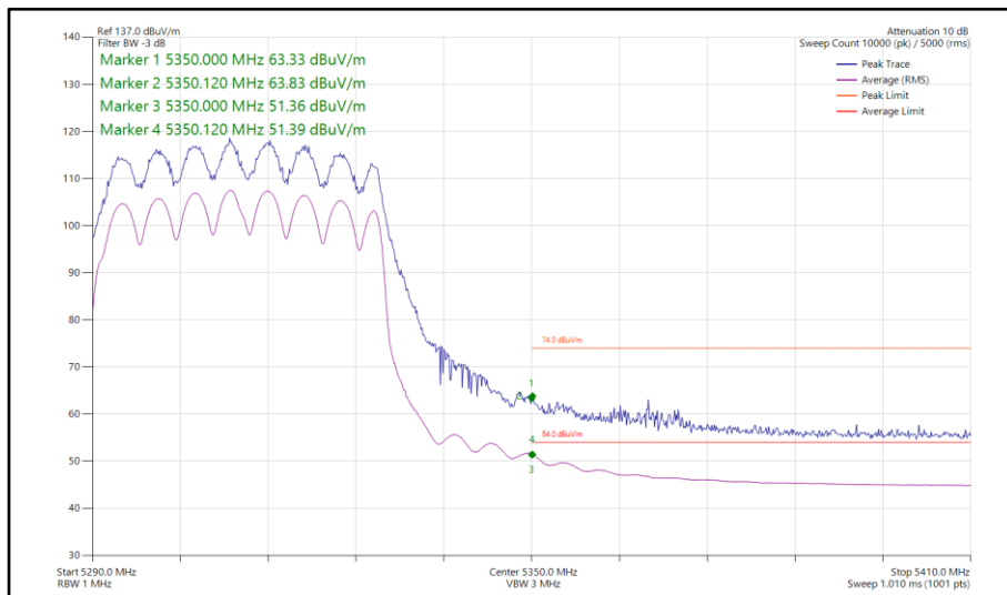
Figure 203 - 802.11ax HE40, SU, CDD, Core 0-1 - 5310 MHz Band Edge Frequency 5350 MHz
