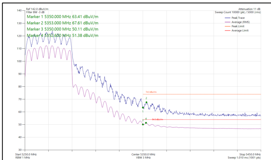
Figure 248 - 802.11ax HE40, SU, TxBF, Core 0-1 - 5270 MHz Band Edge Frequency 5350 MHz
