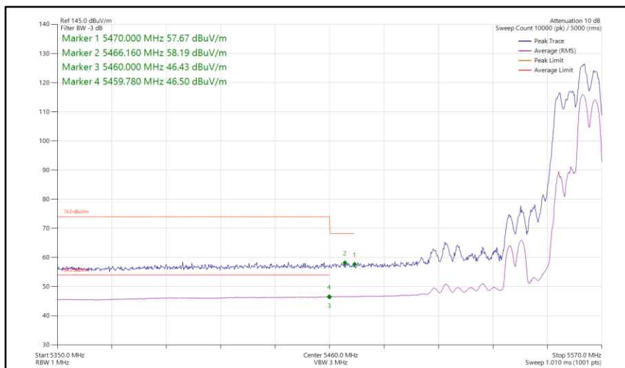
Figure 239 - 802.11ax HE40, RU 106-56, SDM, Core 0-1 - 5550 MHz Band Edge Frequency 5460 MHz
