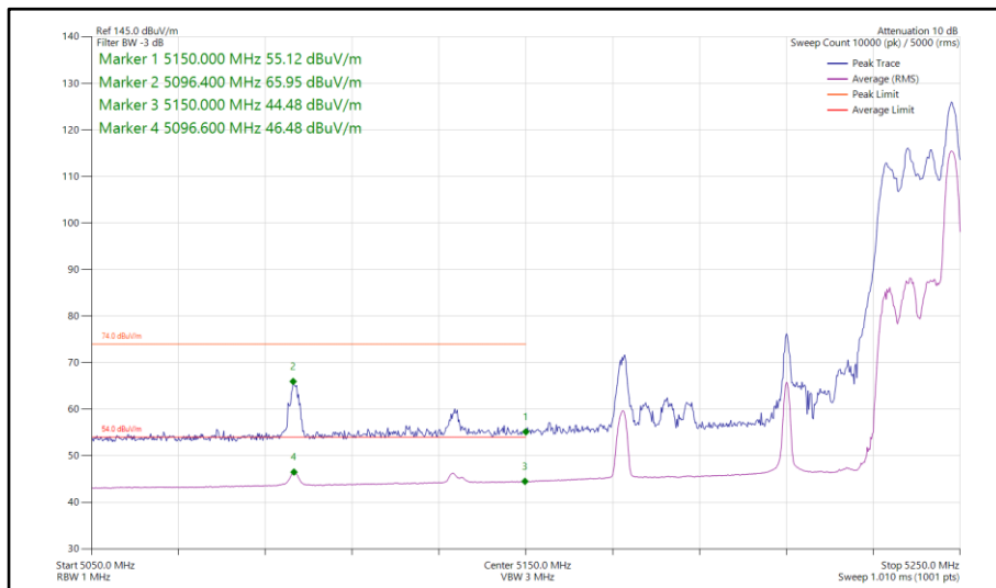
Figure 287 - 802.11ax HE80, RU 26-36, CDD, Core 0-1 - 5210 MHz Band Edge Frequency 5150 MHz
