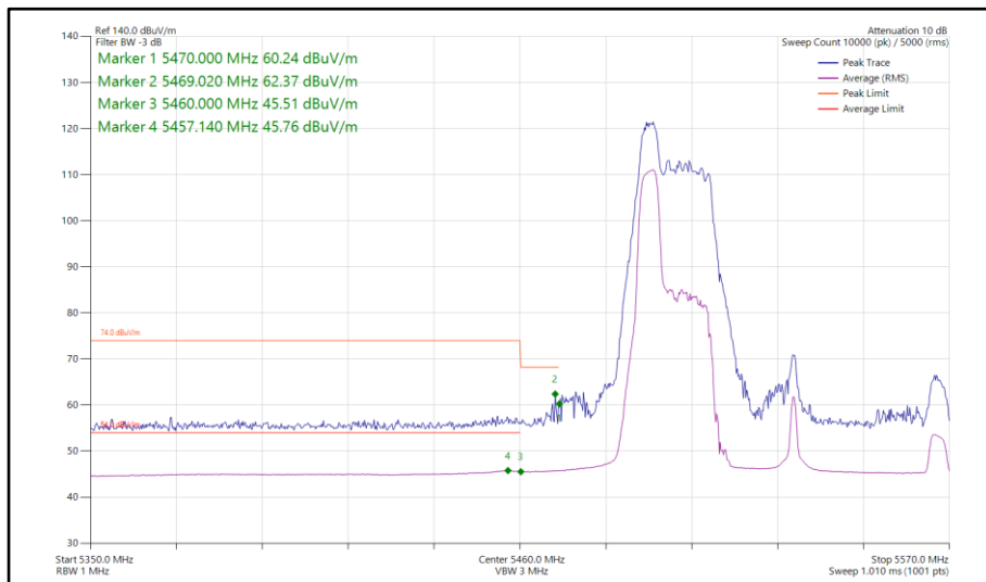
Figure 267 - 802.11ax HE80, RU 52-37, SISO, Core 0 - 5530 MHz Band Edge Frequency 5460 MHz
