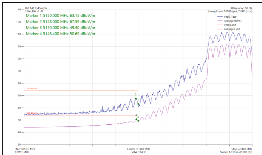
Figure 243 - 802.11ac VHT40, TxBF, Core 0-1 - 5230 MHz Band Edge Frequency 5150 MHz
