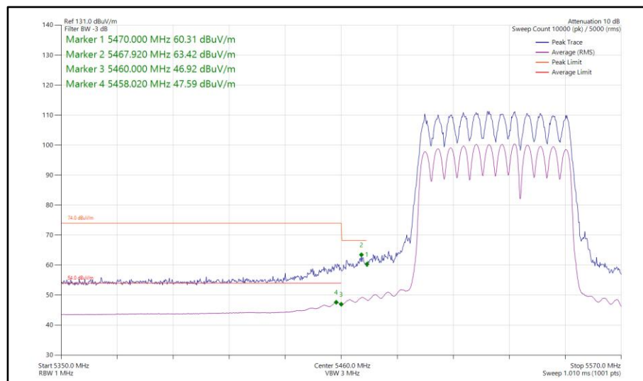
Figure 298 - 802.11be EHT80, RU484+242-93, CDD, Core 0-1 - 5530 MHz Band Edge Frequency 5460 MHz
