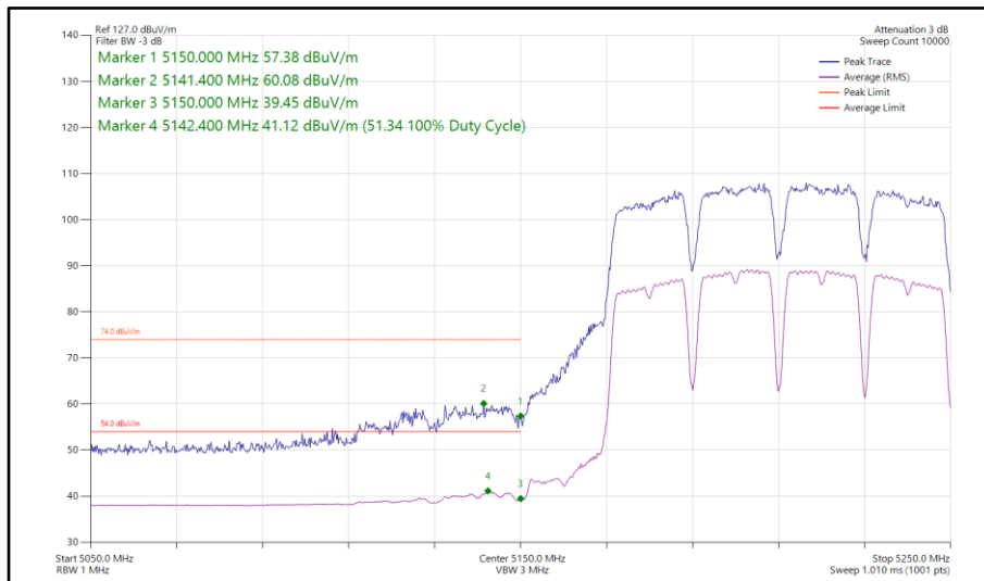
Figure 254 - 802.11a a80, SISO, Core 0 - 5210 MHz Band Edge Frequency 5150 MHz
