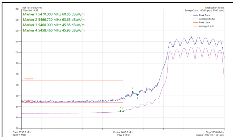
Figure 250 - 802.11ac VHT40, TxBF, Core 0-1 - 5510 MHz Band Edge Frequency 5460 MHz
