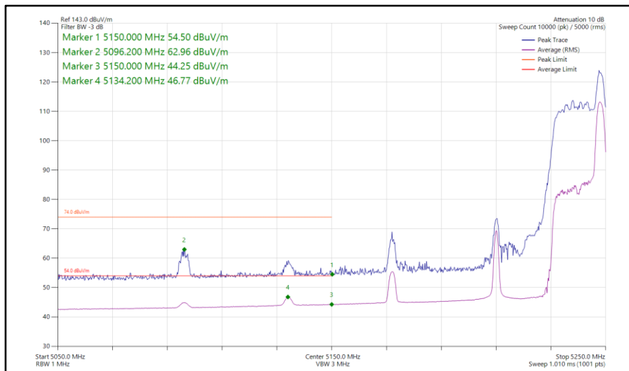
Figure 272 - 802.11ax HE80, RU 26-36, SISO, Core 1 - 5210 MHz Band Edge Frequency 5150 MHz
