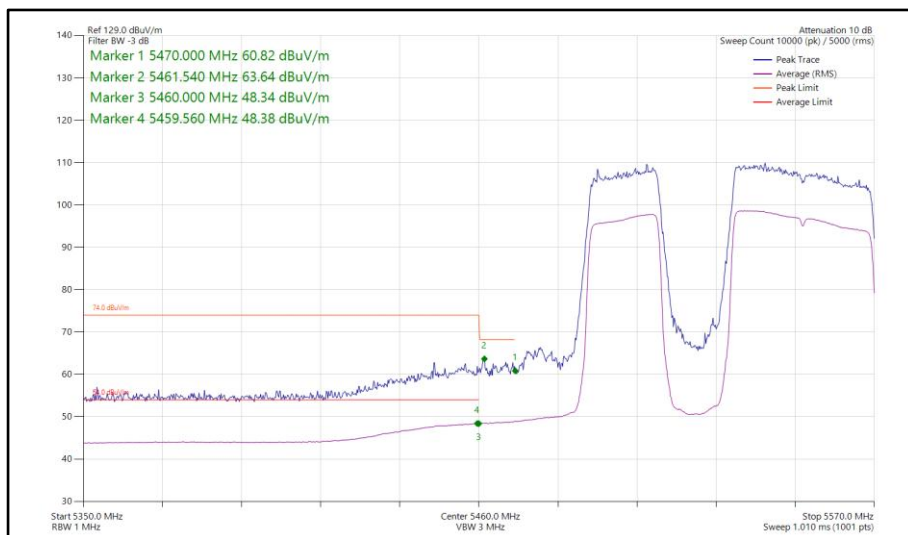
Figure 268 - 802.11be EHT80, RU 484+242-91, SISO, Core 0 - 5530 MHz Band Edge Frequency 5460 MHz
