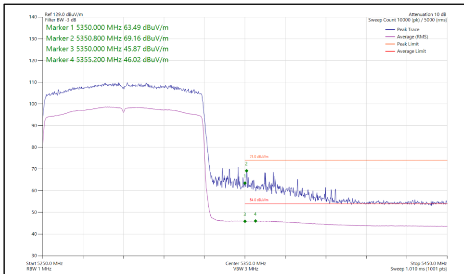
Figure 261 - 802.11ax HE80, SU, SISO, Core 0 - 5290 MHz Band Edge Frequency 5350 MHz
