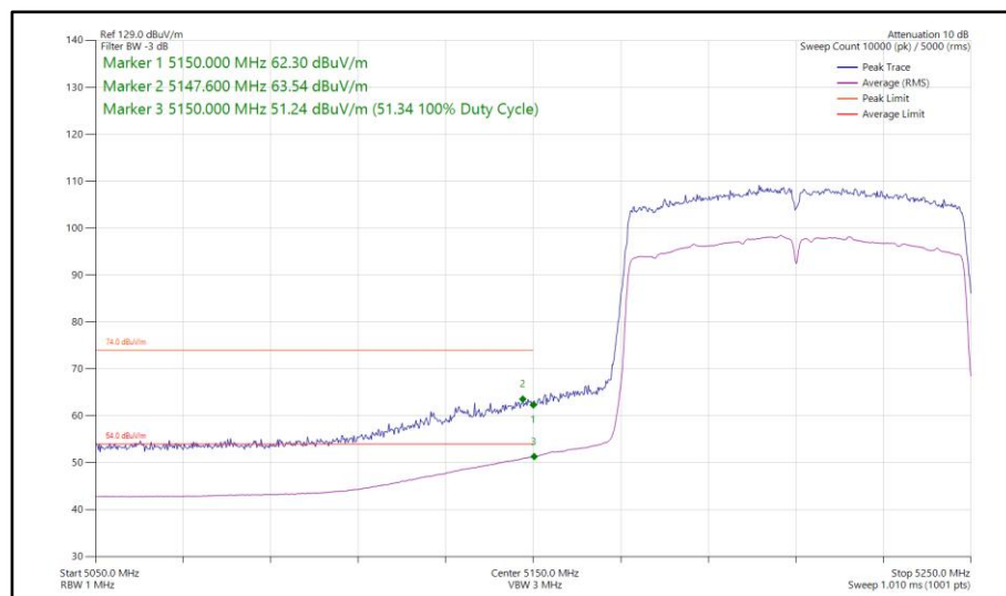
Figure 299 - 802.11ac VHT80, SDM, Core 0-1 - 5210 MHz Band Edge Frequency 5150 MHz
