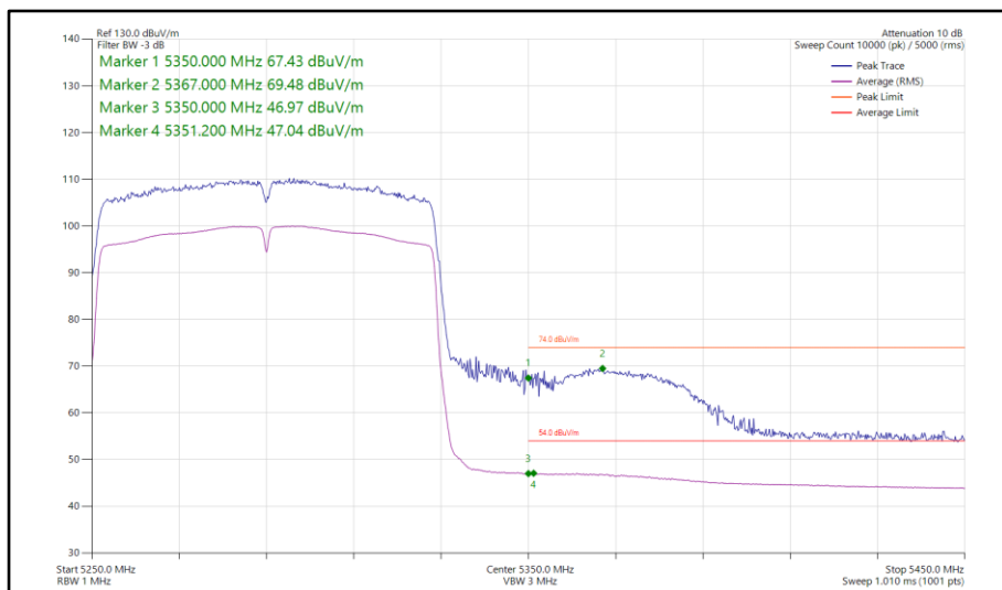
Figure 260 - 802.11ac VHT80, SISO, Core 0 - 5290 MHz Band Edge Frequency 5350 MHz
