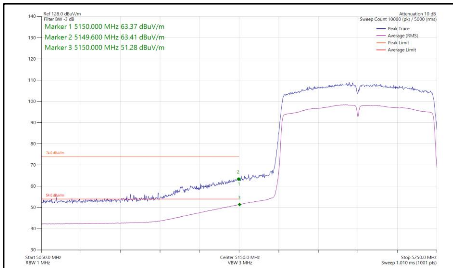
Figure 255 - 802.11ac VHT80, SISO, Core 0 - 5210 MHz Band Edge Frequency 5150 MHz
