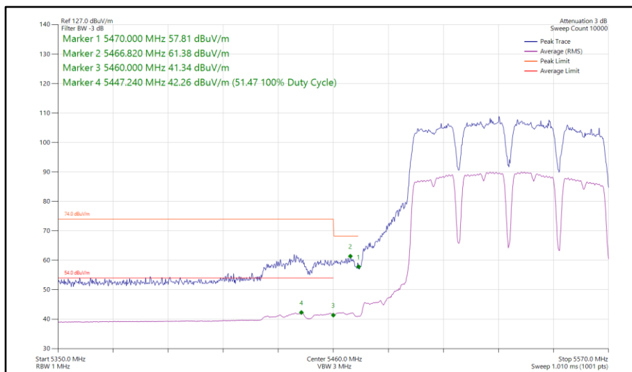
Figure 264 - 802.11a a80, SISO, Core 0 - 5530 MHz Band Edge Frequency 5460 MHz
