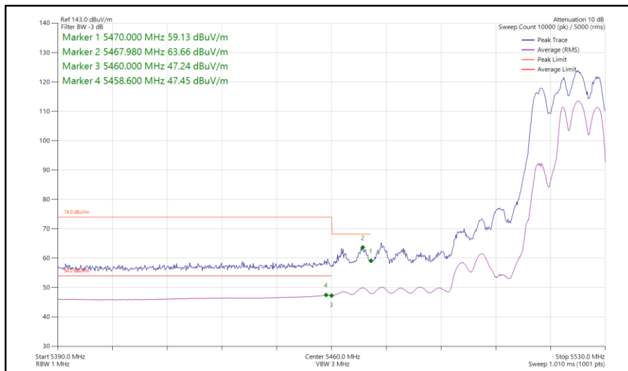
Figure 240 - 802.11be EHT40, RU 106+26-85, SDM, Core 0-1 - 5510 MHz Band Edge Frequency 5460 MHz
