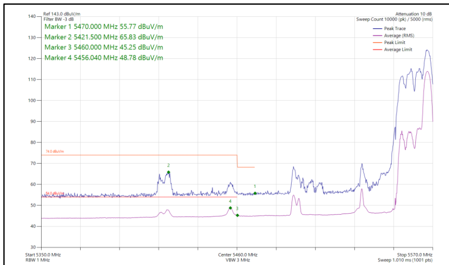
Figure 297 - 802.11ax HE80, RU 52-52, CDD, Core 0-1 - 5530 MHz Band Edge Frequency 5460 MHz
