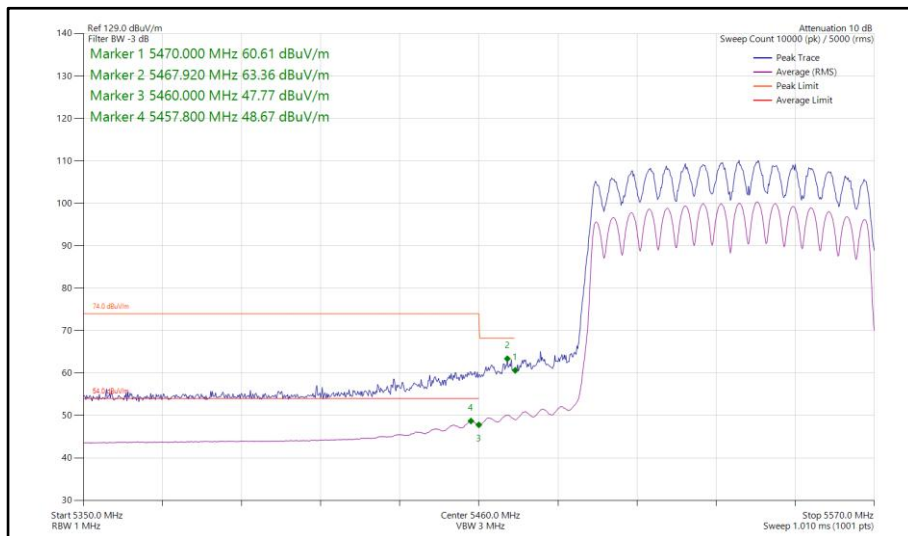
Figure 295 - 802.11ac VHT80, CDD, Core 0-1 - 5530 MHz Band Edge Frequency 5460 MHz
