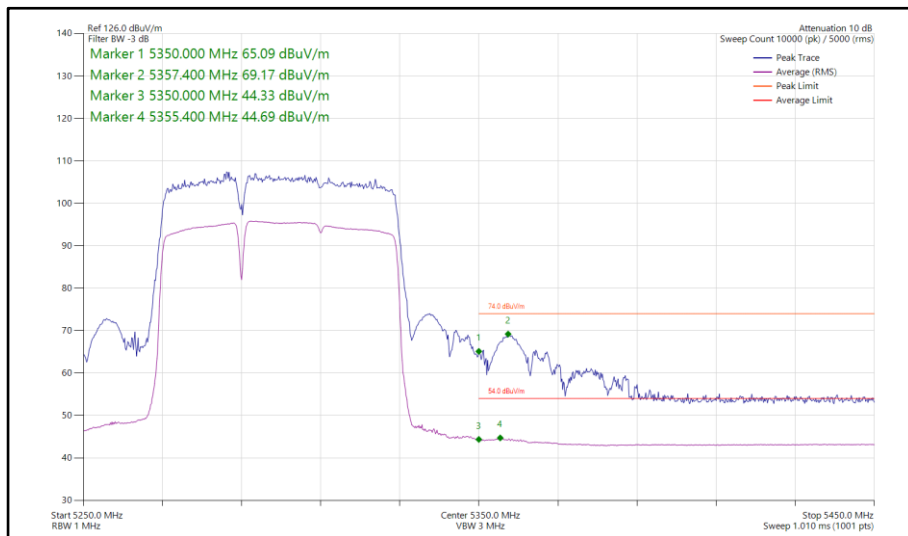
Figure 263 - 802.11be EHT80, RU 484+242-90, SISO, Core 0 - 5290 MHz Band Edge Frequency 5350 MHz
