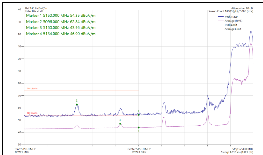
Figure 257 - 802.11ax HE80, RU 26-36, SISO, Core 0 - 5210 MHz Band Edge Frequency 5150 MHz
