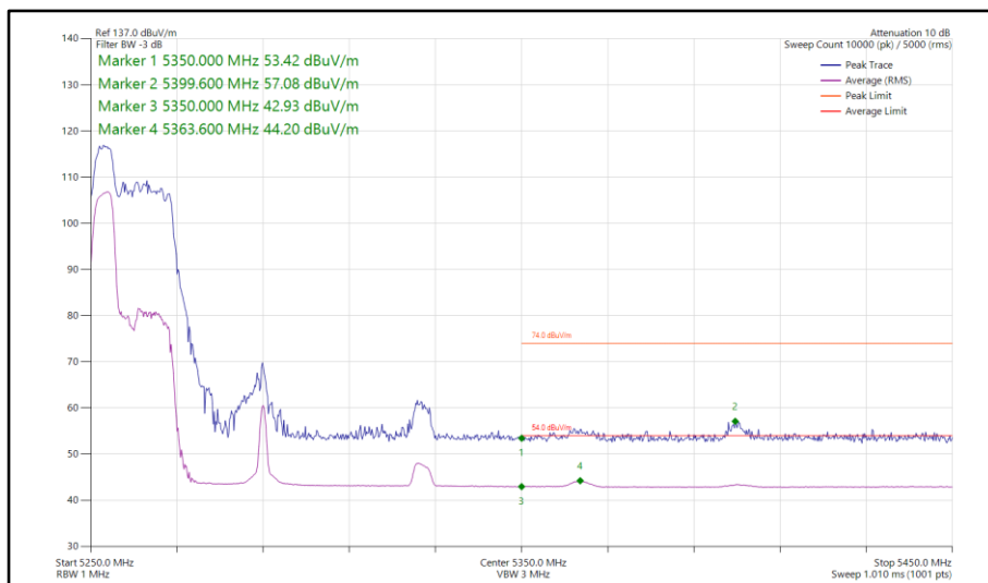
Figure 277 - 802.11ax HE80, RU 52-37, SISO, Core 1 - 5290 MHz Band Edge Frequency 5350 MHz
