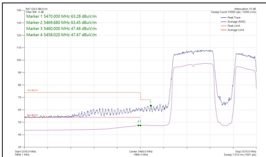
Figure 283 - 802.11be EHT80, RU 484+242-92, SISO, Core 1 - 5530 MHz Band Edge Frequency 5460 MHz
