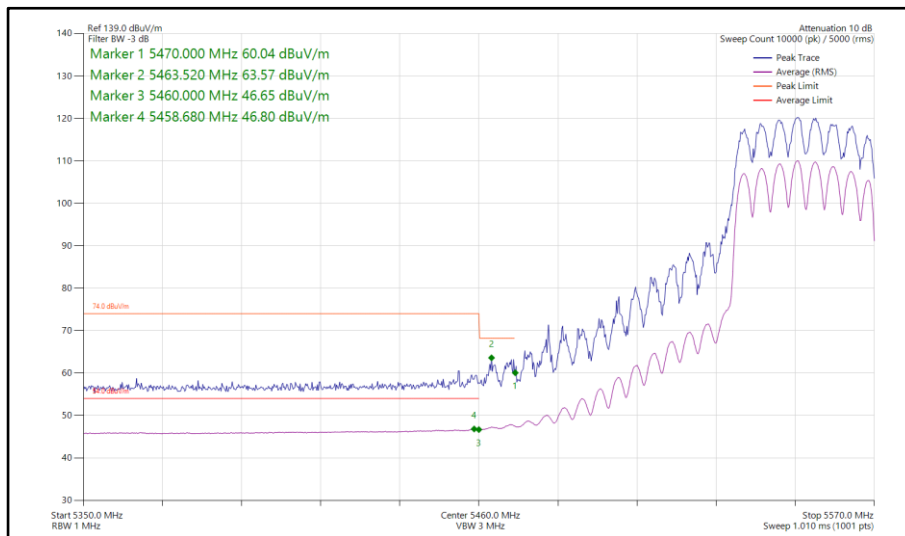
Figure 253 - 802.11ax HE40, SU, TxBF, Core 0-1 - 5550 MHz Band Edge Frequency 5460 MHz
