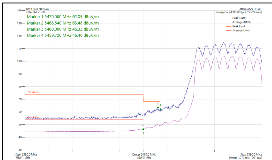
Figure 252 - 802.11ax HE40, SU, TxBF, Core 0-1 - 5510 MHz Band Edge Frequency 5460 MHz
