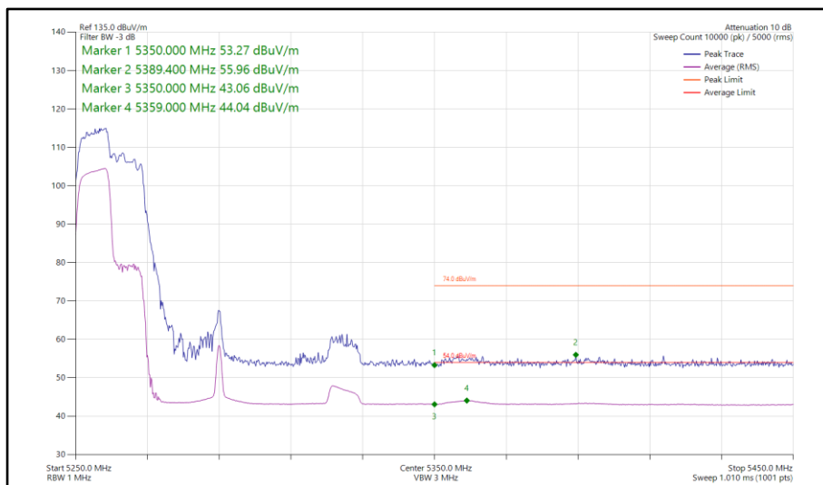
Figure 262 - 802.11ax HE80, RU 106-53, SISO, Core 0 - 5290 MHz Band Edge Frequency 5350 MHz
