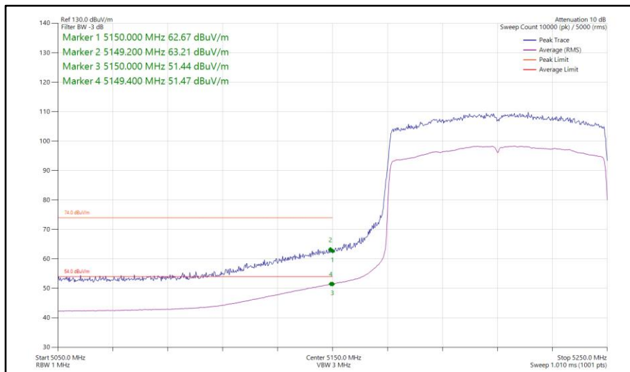
Figure 300 - 802.11ax HE80, SU, SDM, Core 0-1 - 5210 MHz Band Edge Frequency 5150 MHz
