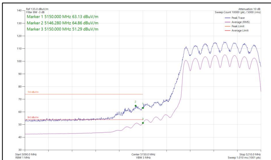
Figure 244 - 802.11ax HE40, SU, TxBF, Core 0-1 - 5190 MHz Band Edge Frequency 5150 MHz
