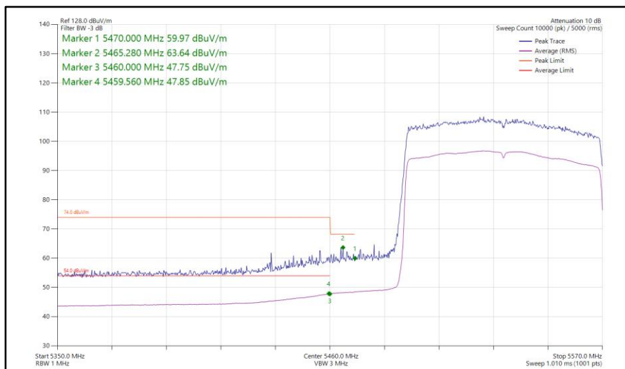
Figure 281 - 802.11ax HE80, SU, SISO, Core 1 - 5530 MHz Band Edge Frequency 5460 MHz
