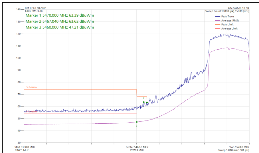
Figure 238 - 802.11ax HE40, SU, SDM, Core 0-1 - 5550 MHz Band Edge Frequency 5460 MHz
