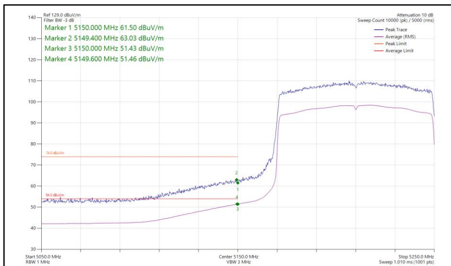
Figure 271 - 802.11ax HE80, SU, SISO, Core 1 - 5210 MHz Band Edge Frequency 5150 MHz
