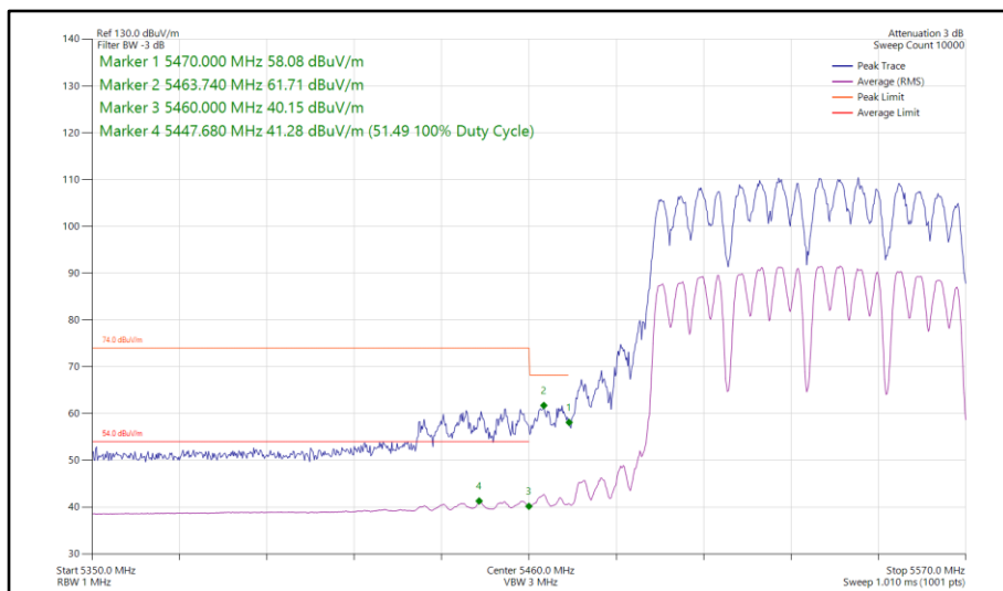
Figure 294 - 802.11a a80, CDD, Core 0-1 - 5530 MHz Band Edge Frequency 5460 MHz
