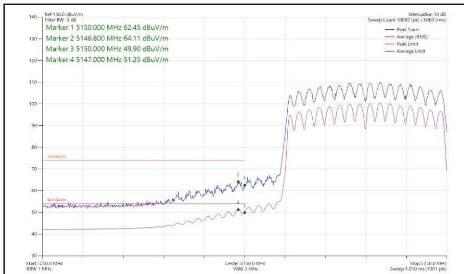
Figure 285 - 802.11ac VHT80, CDD, Core 0-1 - 5210 MHz Band Edge Frequency 5150 MHz
