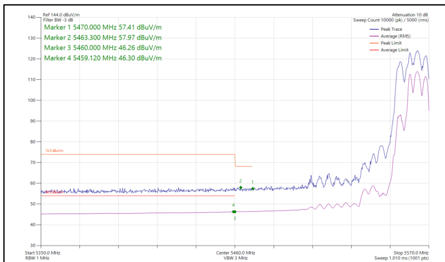
Figure 241 - 802.11be EHT40, RU 106+26-85, SDM, Core 0-1 - 5550 MHz Band Edge Frequency 5460 MHz
