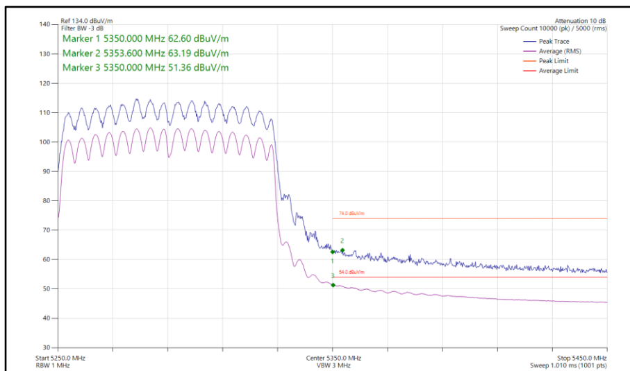
Figure 290 - 802.11ac VHT80, CDD, Core 0-1 - 5290 MHz Band Edge Frequency 5350 MHz
