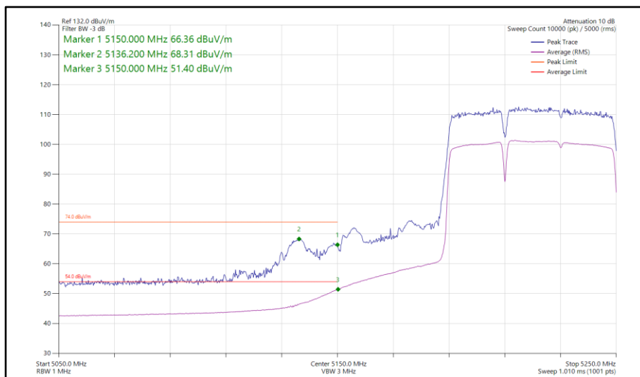
Figure 273 - 802.11be EHT80, RU 484+242-90, SISO, Core 1 - 5210 MHz Band Edge Frequency 5150 MHz
