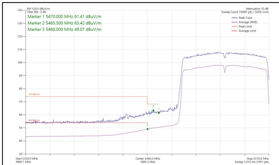
Figure 265 - 802.11ac VHT80, SISO, Core 0 - 5530 MHz Band Edge Frequency 5460 MHz
