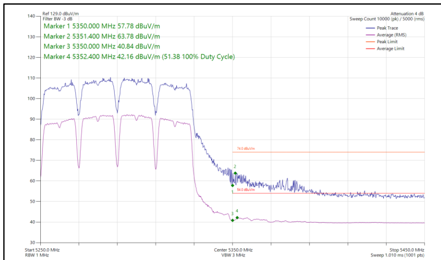
Figure 259 - 802.11a a80, SISO, Core 0 - 5290 MHz Band Edge Frequency 5350 MHz
