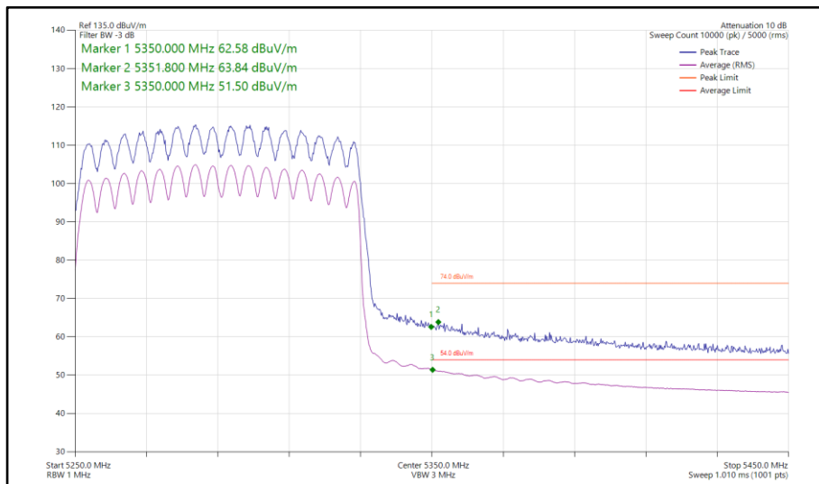
Figure 291 - 802.11ax HE80, SU, CDD, Core 0-1 - 5290 MHz Band Edge Frequency 5350 MHz
