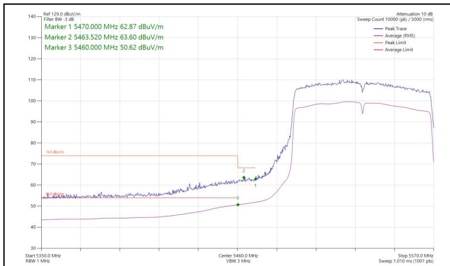
Figure 280 - 802.11ac VHT80, SISO, Core 1 - 5530 MHz Band Edge Frequency 5460 MHz
