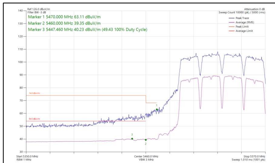
Figure 279 - 802.11a a80, SISO, Core 1 - 5530 MHz Band Edge Frequency 5460 MHz
