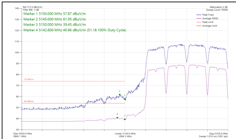
Figure 269 - 802.11a a80, SISO, Core 1 - 5210 MHz Band Edge Frequency 5150 MHz
