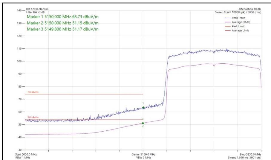
Figure 256 - 802.11ax HE80, SU, SISO, Core 0 - 5210 MHz Band Edge Frequency 5150 MHz
