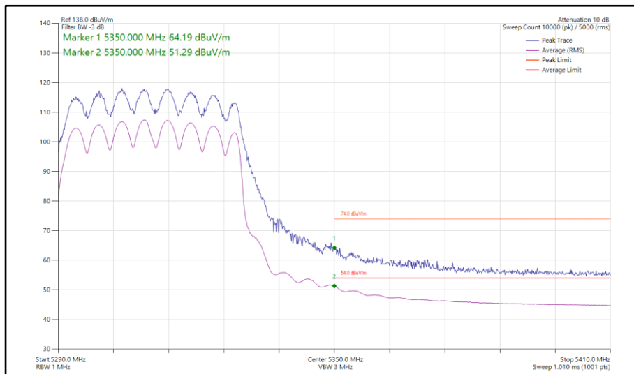
Figure 249 - 802.11ax HE40, SU, TxBF, Core 0-1 - 5310 MHz Band Edge Frequency 5350 MHz
