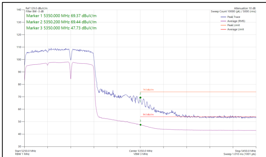
Figure 278 - 802.11be EHT80, RU 484+242-93, SISO, Core 1 - 5290 MHz Band Edge Frequency 5350 MHz
