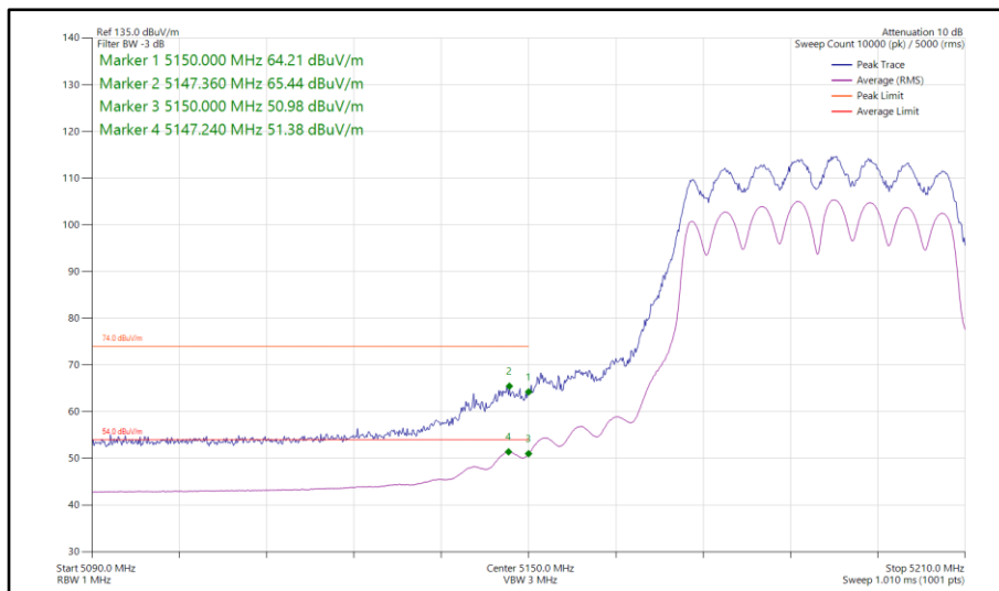
Figure 242 - 802.11ac VHT40, TxBF, Core 0-1 - 5190 MHz Band Edge Frequency 5150 MHz
