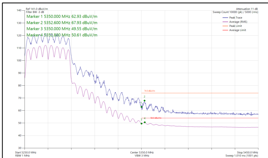
Figure 246 - 802.11ac VHT40, TxBF, Core 0-1 - 5270 MHz Band Edge Frequency 5350 MHz
