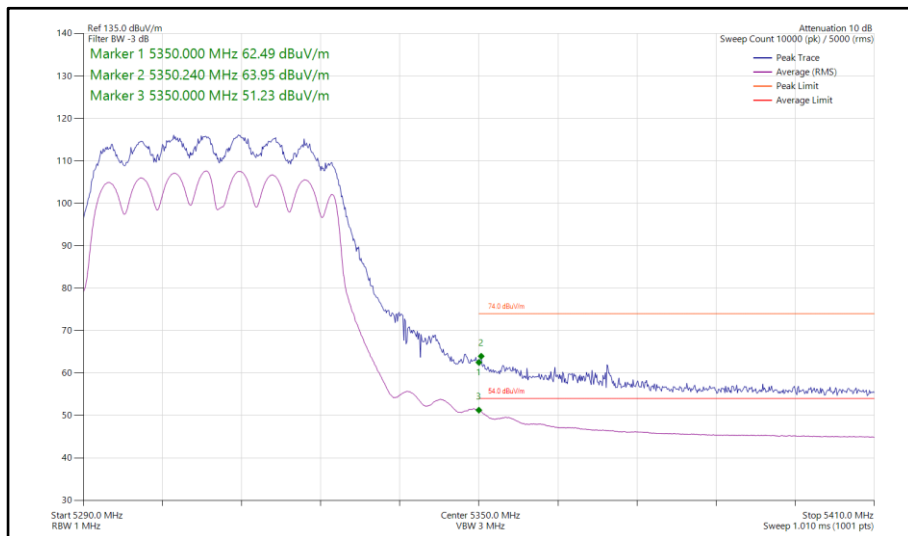
Figure 247 - 802.11ac VHT40, TxBF, Core 0-1 - 5310 MHz Band Edge Frequency 5350 MHz
