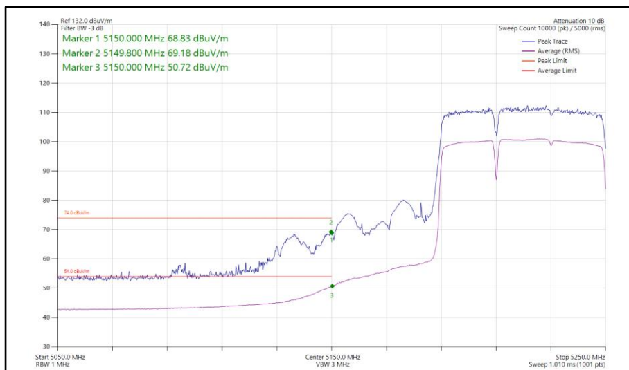
Figure 258 - 802.11be EHT80, RU 484+242-90, SISO, Core 0 - 5210 MHz Band Edge Frequency 5150 MHz
