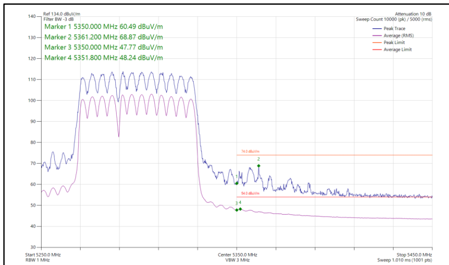
Figure 293 - 802.11be EHT80, RU 484+242-90, CDD, Core 0-1 - 5290 MHz Band Edge Frequency 5350 MHz
