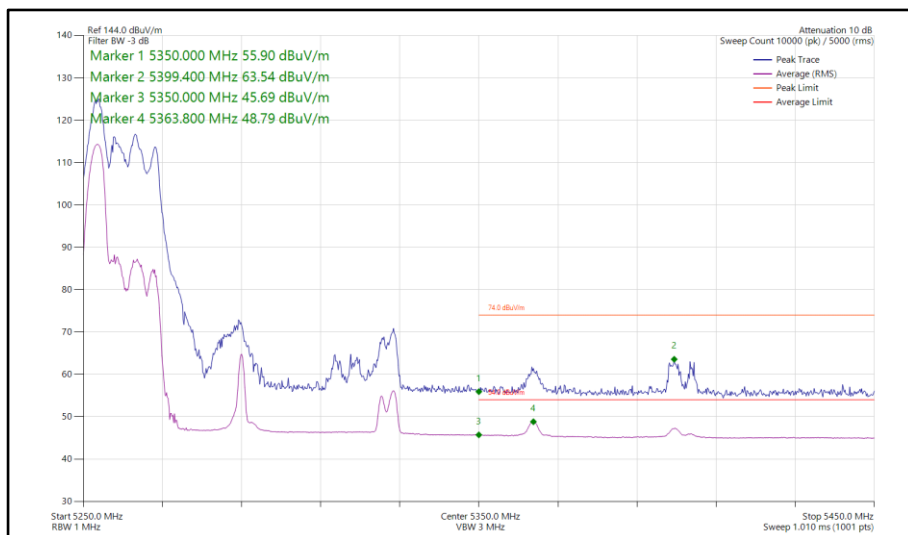
Figure 292 - 802.11ax HE80, RU 52-37, CDD, Core 0-1 - 5290 MHz Band Edge Frequency 5350 MHz
