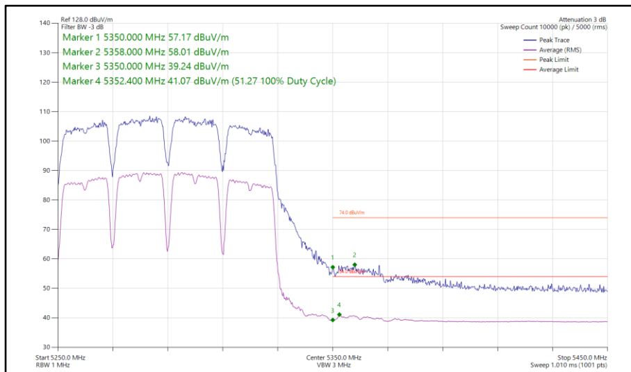
Figure 274 - 802.11a a80, SISO, Core 1 - 5290 MHz Band Edge Frequency 5350 MHz
