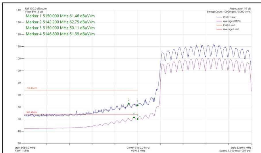
Figure 286 - 802.11ax HE80, SU, CDD, Core 0-1 - 5210 MHz Band Edge Frequency 5150 MHz
