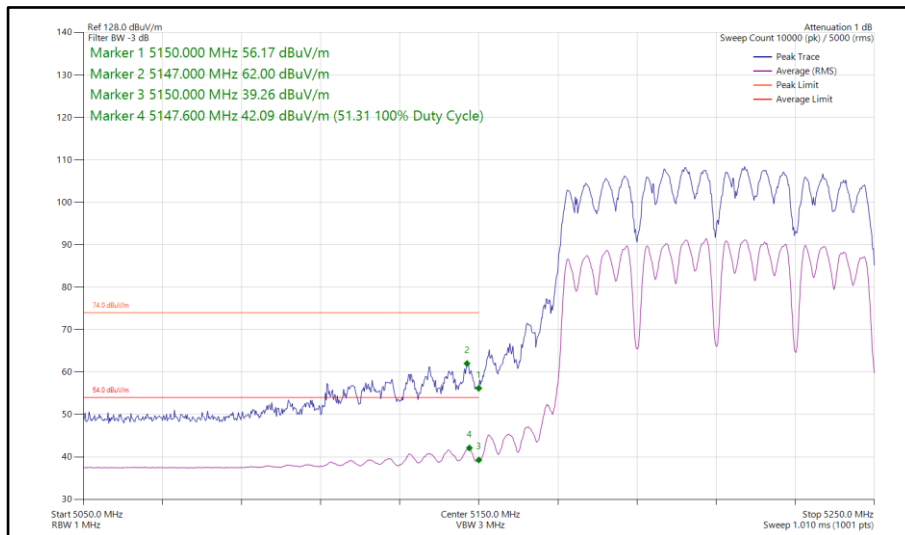
Figure 284 - 802.11a a80, CDD, Core 0-1 - 5210 MHz Band Edge Frequency 5150 MHz
