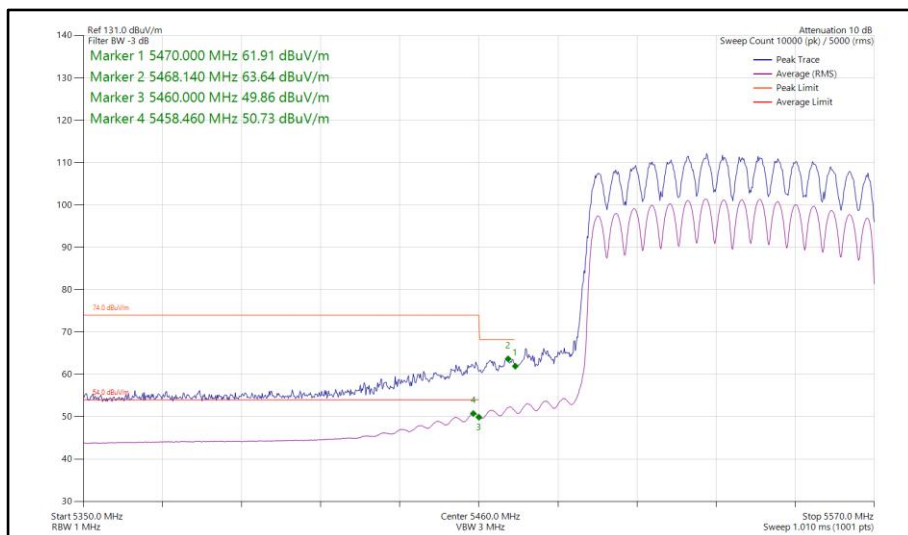
Figure 296 - 802.11ax HE80, SU, CDD, Core 0-1 - 5530 MHz Band Edge Frequency 5460 MHz
