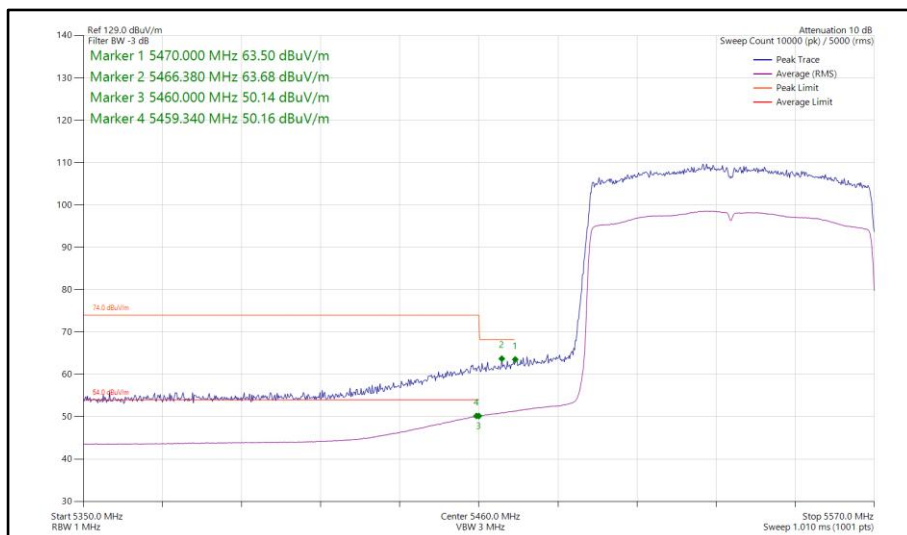
Figure 266 - 802.11ax HE80, SU, SISO, Core 0 - 5530 MHz Band Edge Frequency 5460 MHz
