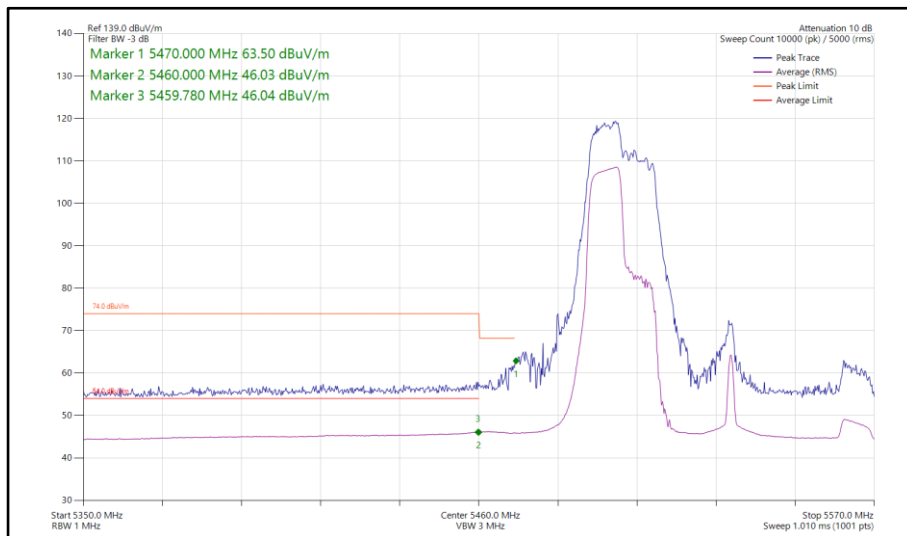
Figure 282 - 802.11ax HE80, RU 106-53, SISO, Core 1 - 5530 MHz Band Edge Frequency 5460 MHz
