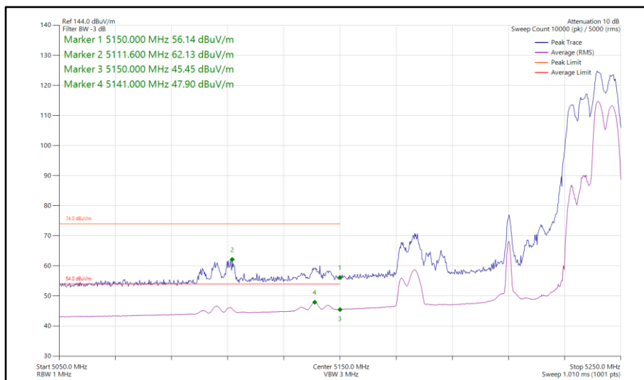
Figure 301 - 802.11ax HE80, RU 106-60, SDM, Core 0-1 - 5210 MHz Band Edge Frequency 5150 MHz
