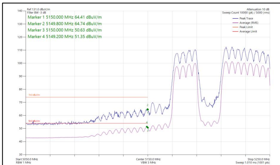
Figure 288 - 802.11be EHT80, RU 484+242-91, CDD, Core 0-1 - 5210 MHz Band Edge Frequency 5150 MHz
