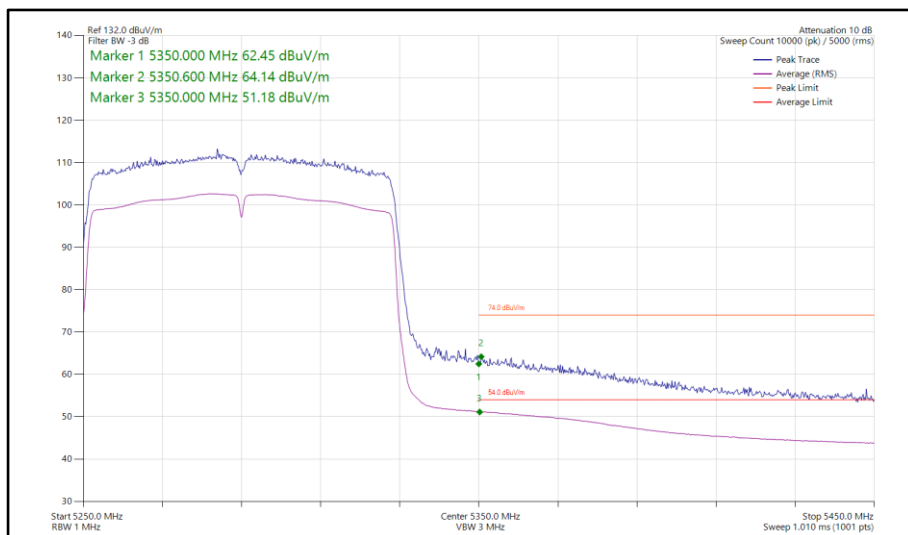
Figure 275 - 802.11ac VHT80, SISO, Core 1 - 5290 MHz Band Edge Frequency 5350 MHz
