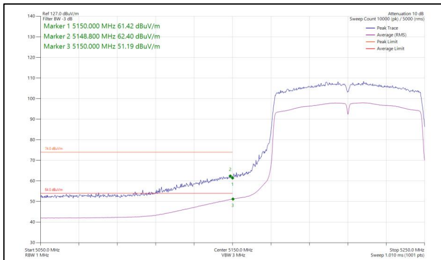
Figure 270 - 802.11ac VHT80, SISO, Core 1 - 5210 MHz Band Edge Frequency 5150 MHz
