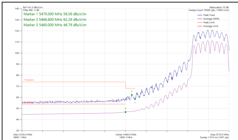
Figure 251 - 802.11ac VHT40, TxBF, Core 0-1 - 5550 MHz Band Edge Frequency 5460 MHz
