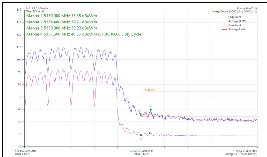
Figure 289 - 802.11a a80, CDD, Core 0-1 - 5290 MHz Band Edge Frequency 5350 MHz
