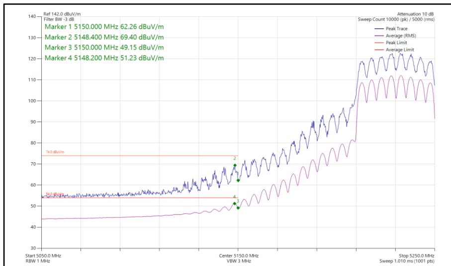
Figure 245 - 802.11ax HE40, SU, TxBF, Core 0-1 - 5230 MHz Band Edge Frequency 5150 MHz
