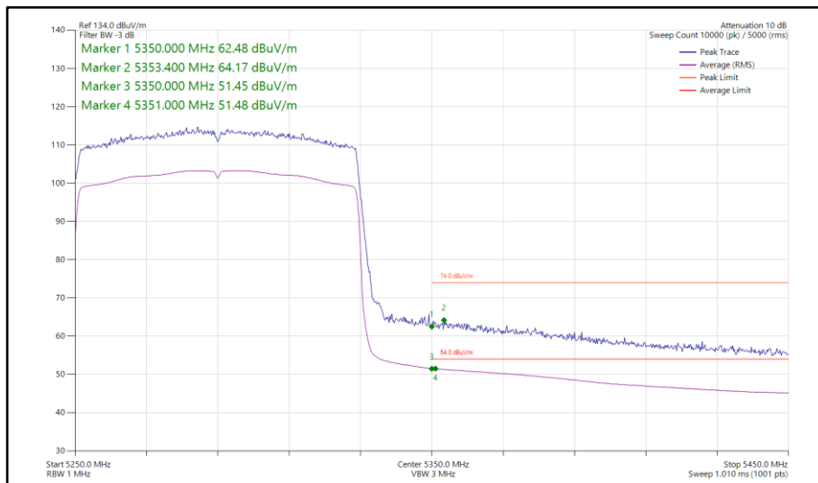
Figure 276 - 802.11ax HE80, SU, SISO, Core 1 - 5290 MHz Band Edge Frequency 5350 MHz
