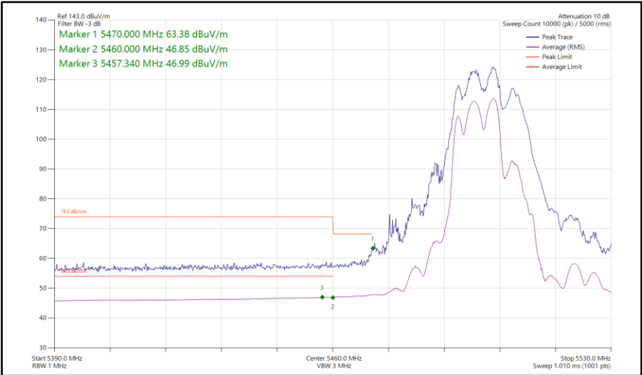
Figure 802 - 802.11be EHT40, RU 106+26-82, CDD, Core 0-1 - 5510 MHz Band Edge Frequency 5460 MHz
