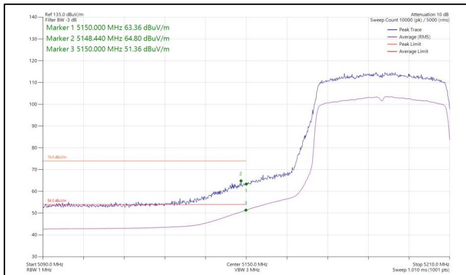
Figure 804 - 802.11ax HE40, SU, SDM, Core 0-1 - 5190 MHz Band Edge Frequency 5150 MHz
