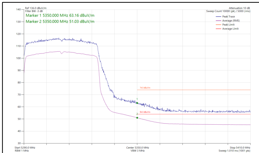
Figure 808 - 802.11ax HE40, SU, SDM, Core 0-1 - 5310 MHz Band Edge Frequency 5350 MHz
