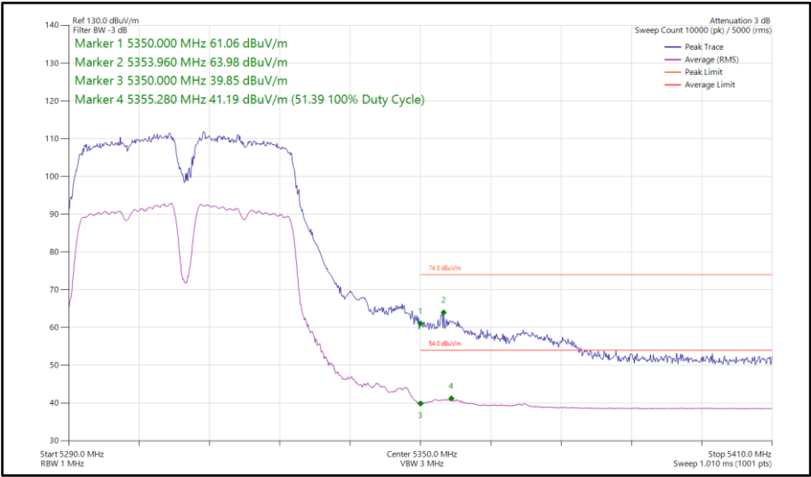
Figure 763 - 802.11a a40, SISO, Core 0 - 5310 MHz Band Edge Frequency 5350 MHz
