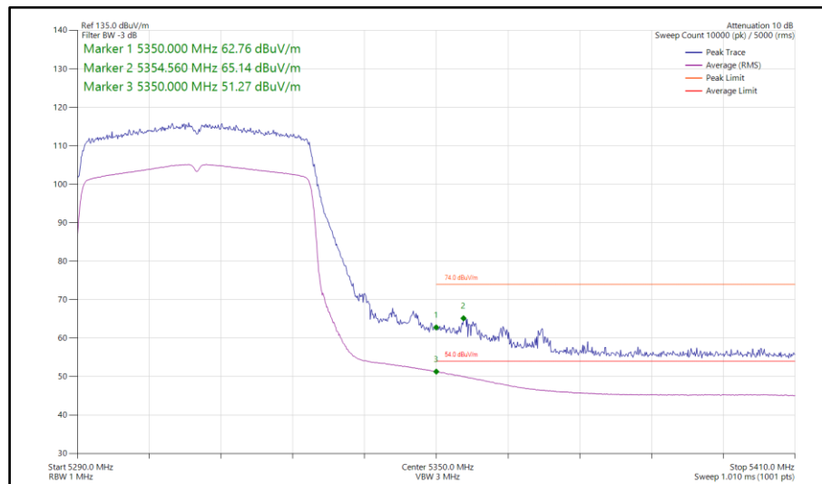
Figure 780 - 802.11ax HE40, SU, SISO, Core 1 - 5310 MHz Band Edge Frequency 5350 MHz
