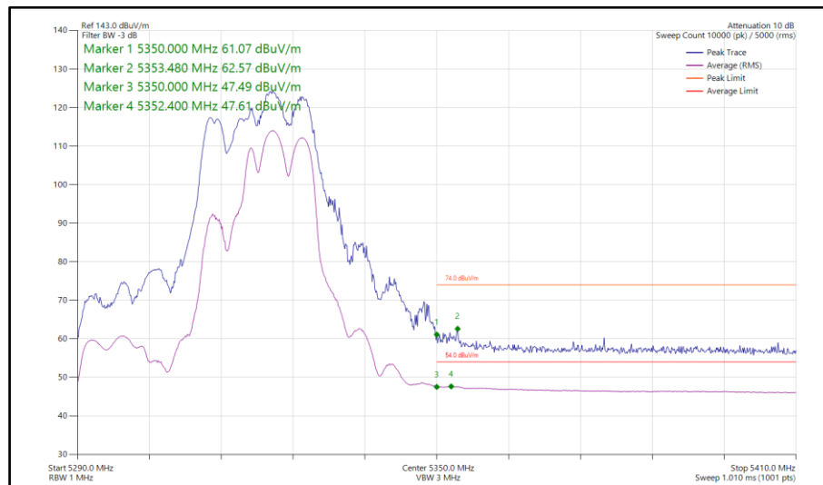
Figure 797 - 802.11be EHT40, RU 106+26-85, CDD, Core 0-1 - 5310 MHz Band Edge Frequency 5350 MHz
