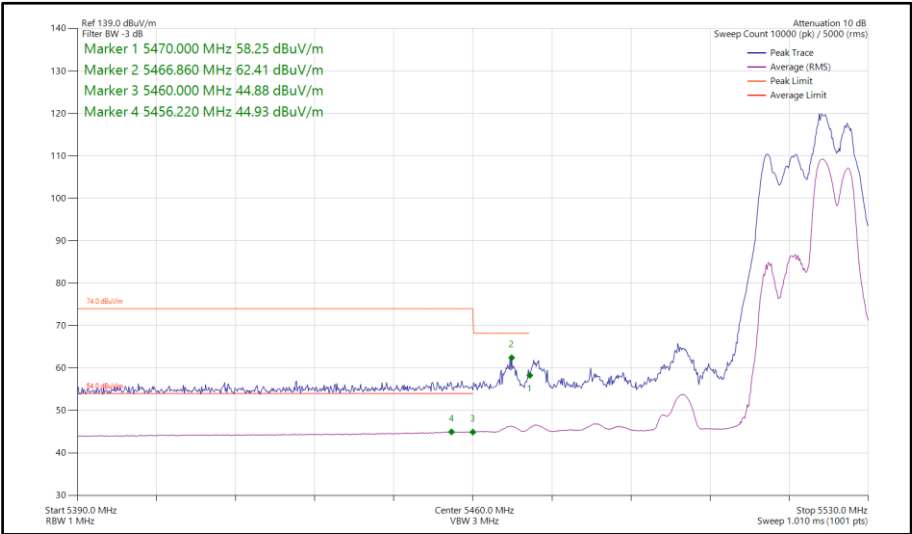
Figure 814 - 802.11be EHT40, RU 52+26-75, SDM, Core 0-1 - 5510 MHz Band Edge Frequency 5460 MHz
