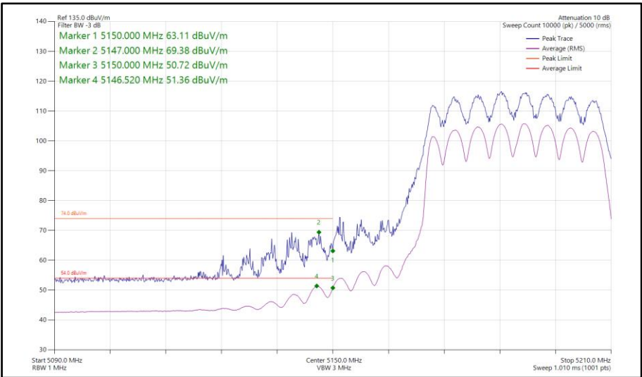
Figure 790 - 802.11ax HE40, SU, CDD, Core 0-1 - 5190 MHz Band Edge Frequency 5150 MHz
