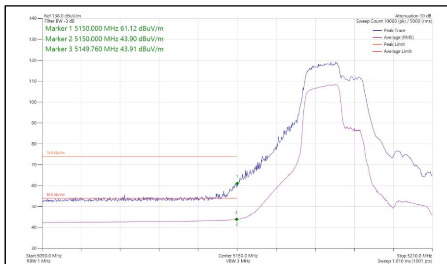
Figure 777 - 802.11be EHT40, RU 106+26-82, SISO, Core 1 - 5190 MHz Band Edge Frequency 5150 MHz
