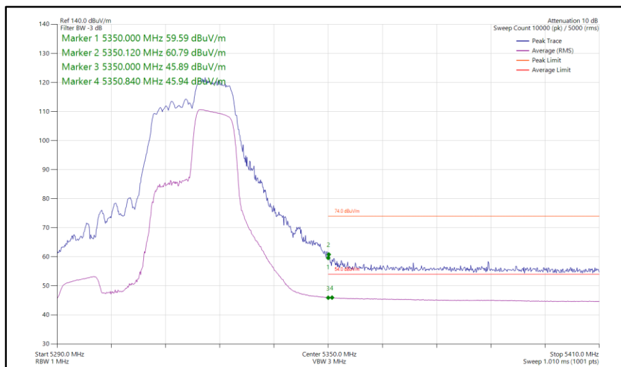
Figure 766 - 802.11ax HE40, RU 106-56, SISO, Core 0 - 5310 MHz Band Edge Frequency 5350 MHz
