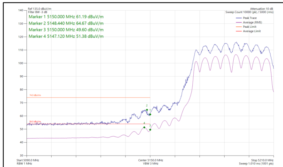
Figure 815 - 802.11ac VHT40, TxBF, Core 0-1 - 5190 MHz Band Edge Frequency 5150 MHz
