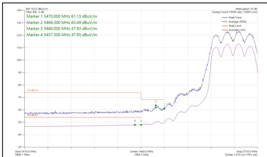
Figure 757 - 802.11ax HE20, SU, TxBF, Core 0-1 - 5500 MHz Band Edge Frequency 5460 MHz
