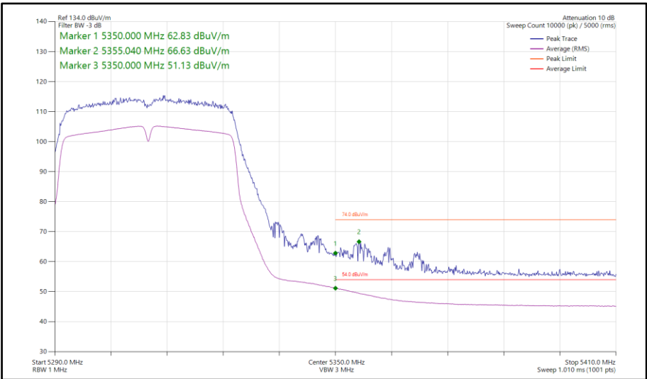
Figure 779 - 802.11n HT40, SISO, Core 1 - 5310 MHz Band Edge Frequency 5350 MHz
