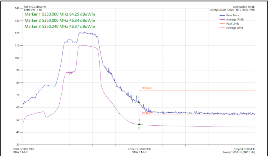
Figure 767 - 802.11be EHT40, RU 106+26-85, SISO, Core 0 - 5310 MHz Band Edge Frequency 5350 MHz
