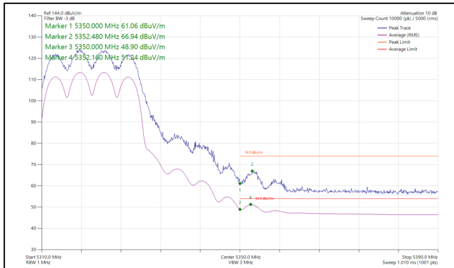
Figure 755 - 802.11ax HE20, SU, TxBF, Core 0-1 - 5320 MHz Band Edge Frequency 5350 MHz
