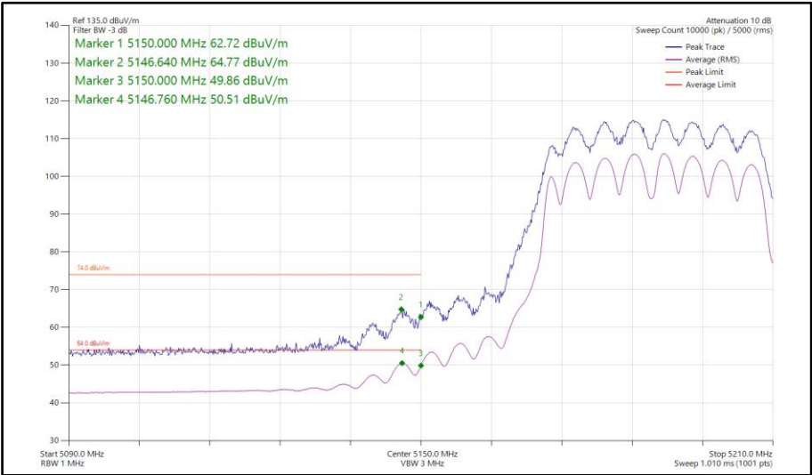
Figure 789 - 802.11n HT40, CDD, Core 0-1 - 5190 MHz Band Edge Frequency 5150 MHz
