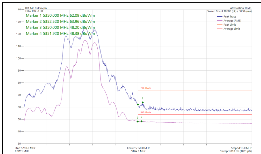
Figure 810 - 802.11be EHT40, RU 106+26-85, SDM, Core 0-1 - 5310 MHz Band Edge Frequency 5350 MHz
