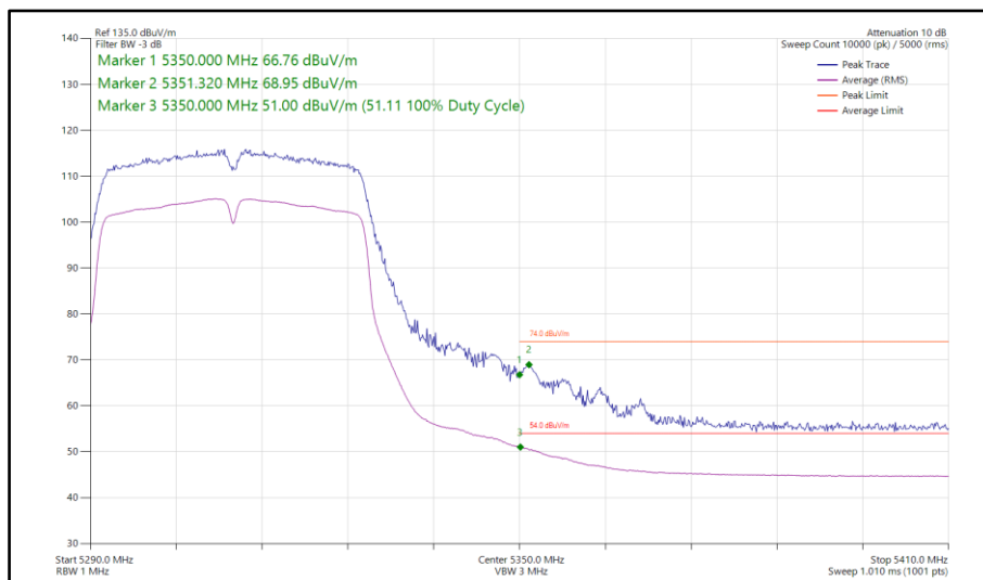
Figure 807 - 802.11n HT40, SDM, Core 0-1 - 5310 MHz Band Edge Frequency 5350 MHz
