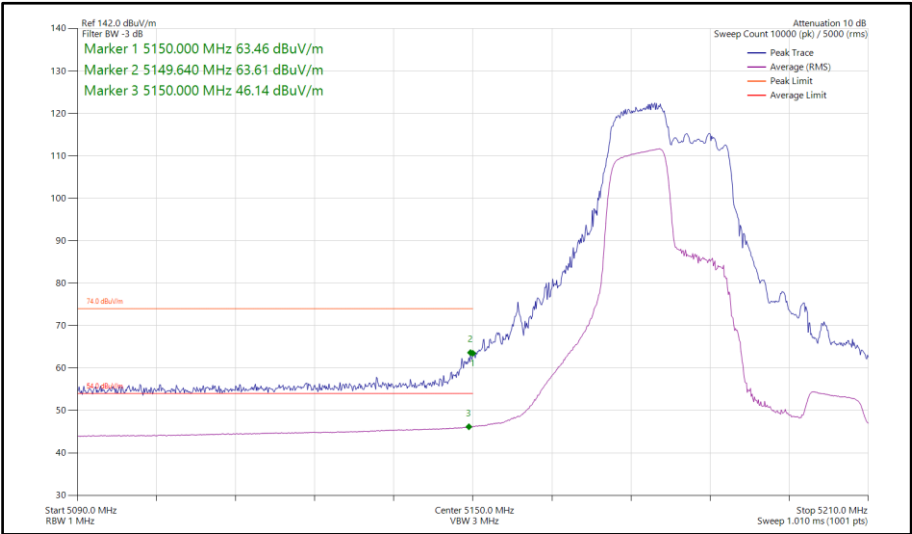
Figure 761 - 802.11ax HE40, RU 106-53, SISO, Core 0 - 5190 MHz Band Edge Frequency 5150 MHz
