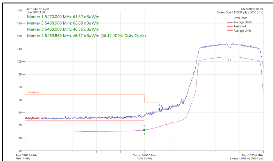
Figure 811 - 802.11n HT40, SDM, Core 0-1 - 5510 MHz Band Edge Frequency 5460 MHz
