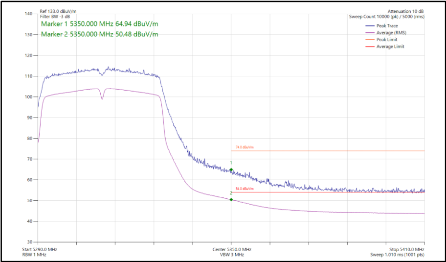
Figure 764 - 802.11n HT40, SISO, Core 0 - 5310 MHz Band Edge Frequency 5350 MHz
