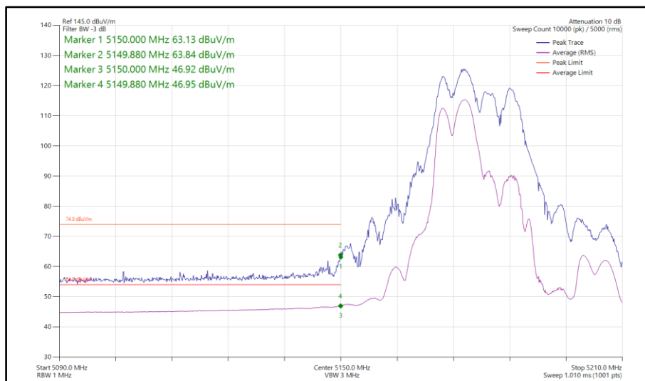
Figure 805 - 802.11ax HE40, RU 106-53, SDM, Core 0-1 - 5190 MHz Band Edge Frequency 5150 MHz
