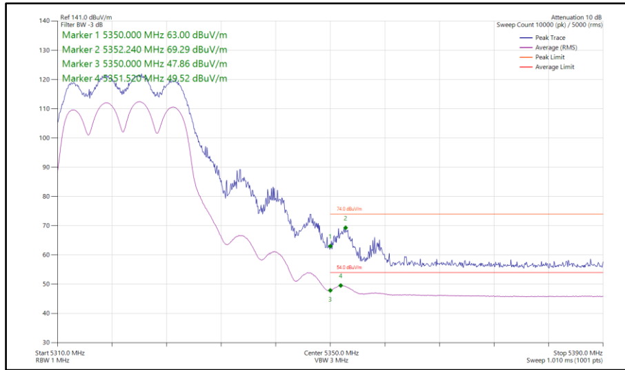
Figure 754 - 802.11ac VHT20, TxBF, Core 0-1 - 5320 MHz Band Edge Frequency 5350 MHz
