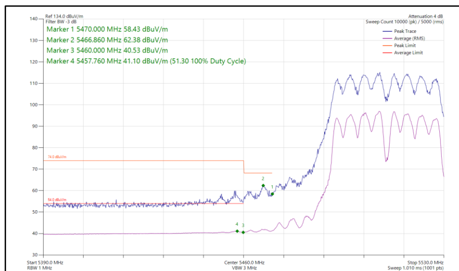
Figure 798 - 802.11a a40, CDD, Core 0-1 - 5510 MHz Band Edge Frequency 5460 MHz
