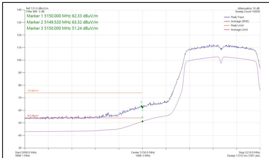
Figure 759 - 802.11n HT40, SISO, Core 0 - 5190 MHz Band Edge Frequency 5150 MHz
