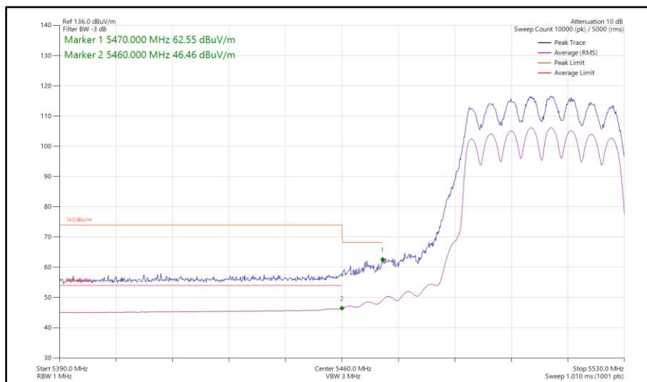
Figure 800 - 802.11ax HE40, SU, CDD, Core 0-1 - 5510 MHz Band Edge Frequency 5460 MHz
