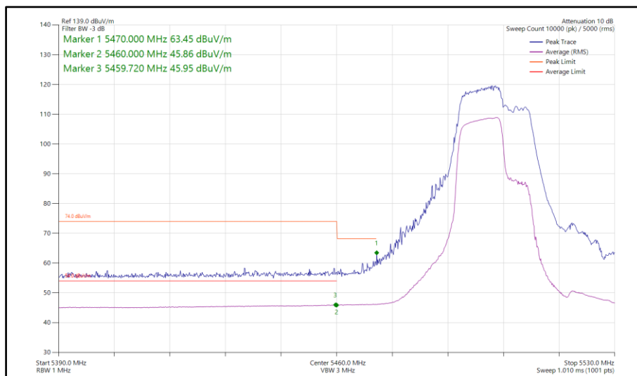
Figure 772 - 802.11be EHT40, RU 106+26-82, SISO, Core 0 - 5510 MHz Band Edge Frequency 5460 MHz
