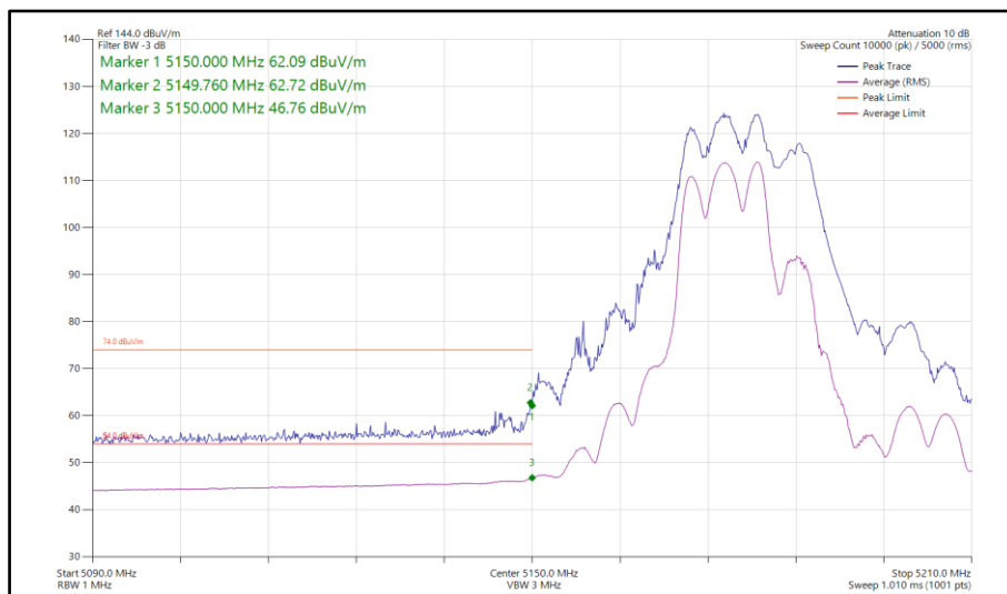
Figure 792 - 802.11be EHT40, RU 106+26-82, CDD, Core 0-1 - 5190 MHz Band Edge Frequency 5150 MHz
