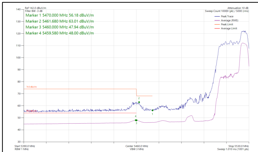
Figure 771 - 802.11ax HE40, RU 52-44, SISO, Core 0 - 5510 MHz Band Edge Frequency 5460 MHz
