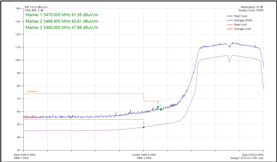
Figure 769 - 802.11n HT40, SISO, Core 0 - 5510 MHz Band Edge Frequency 5460 MHz
