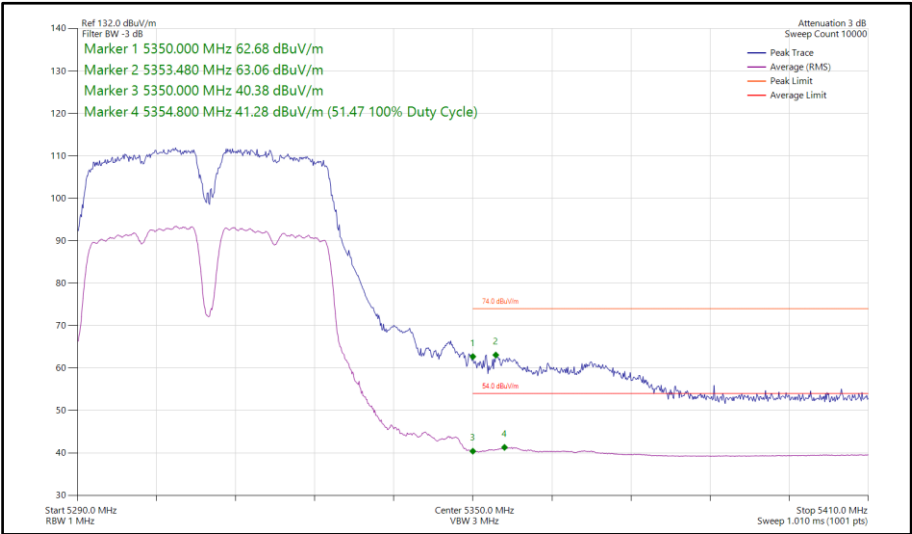
Figure 778 - 802.11a a40, SISO, Core 1 - 5310 MHz Band Edge Frequency 5350 MHz
