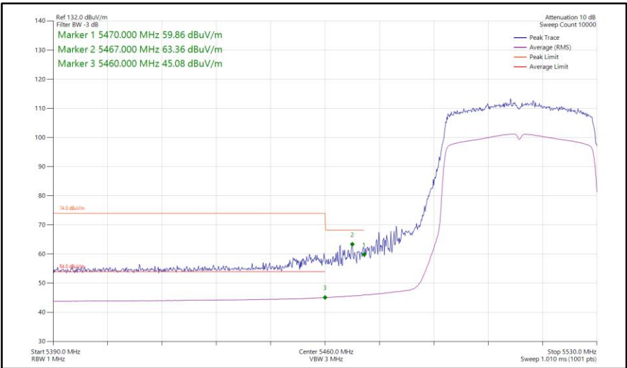
Figure 785 - 802.11ax HE40, SU, SISO, Core 1 - 5510 MHz Band Edge Frequency 5460 MHz
