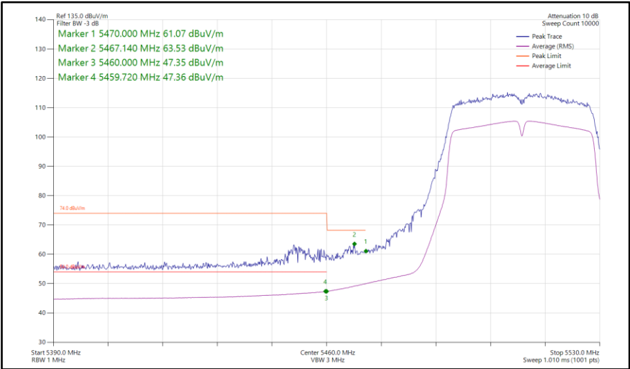
Figure 784 - 802.11n HT40, SISO, Core 1 - 5510 MHz Band Edge Frequency 5460 MHz
