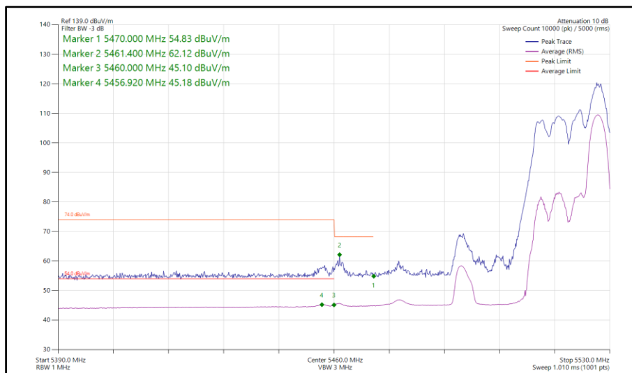
Figure 813 - 802.11ax HE40, RU 52-44, SDM, Core 0-1 - 5510 MHz Band Edge Frequency 5460 MHz
