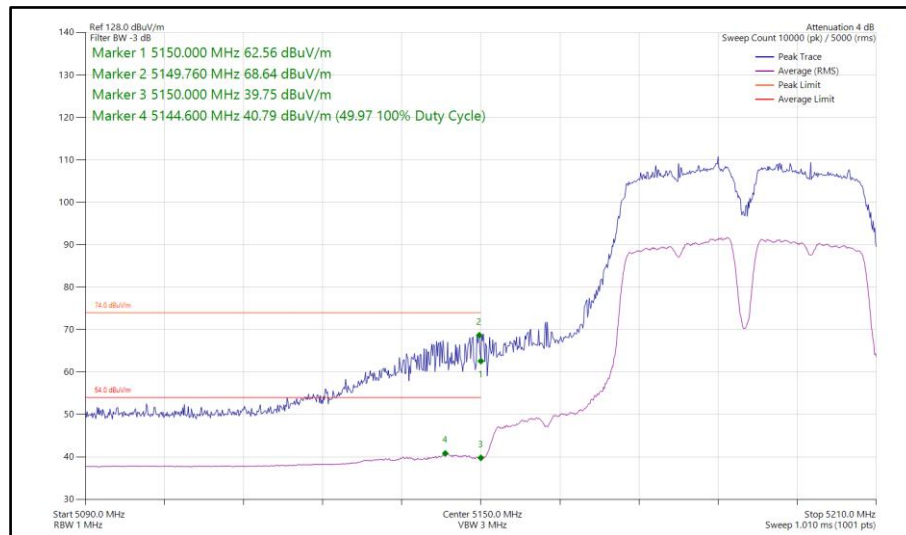
Figure 758 - 802.11a a40, SISO, Core 0 - 5190 MHz Band Edge Frequency 5150 MHz
