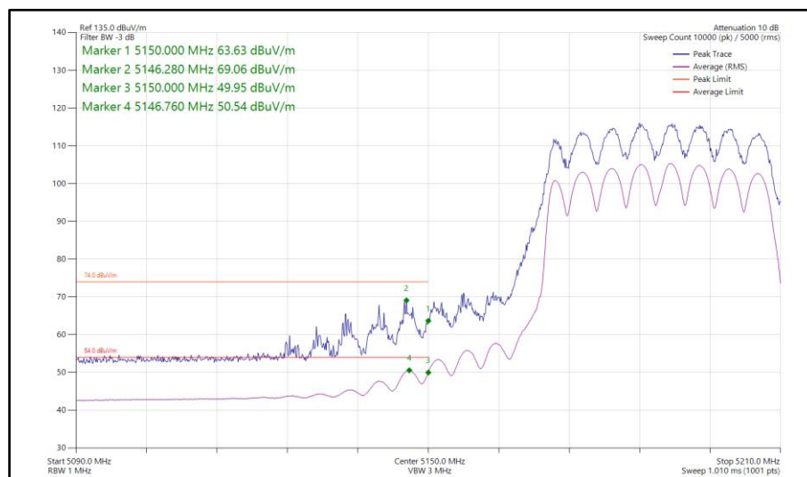
Figure 816 - 802.11ax HE40, SU, TxBF, Core 0-1 - 5190 MHz Band Edge Frequency 5150 MHz
