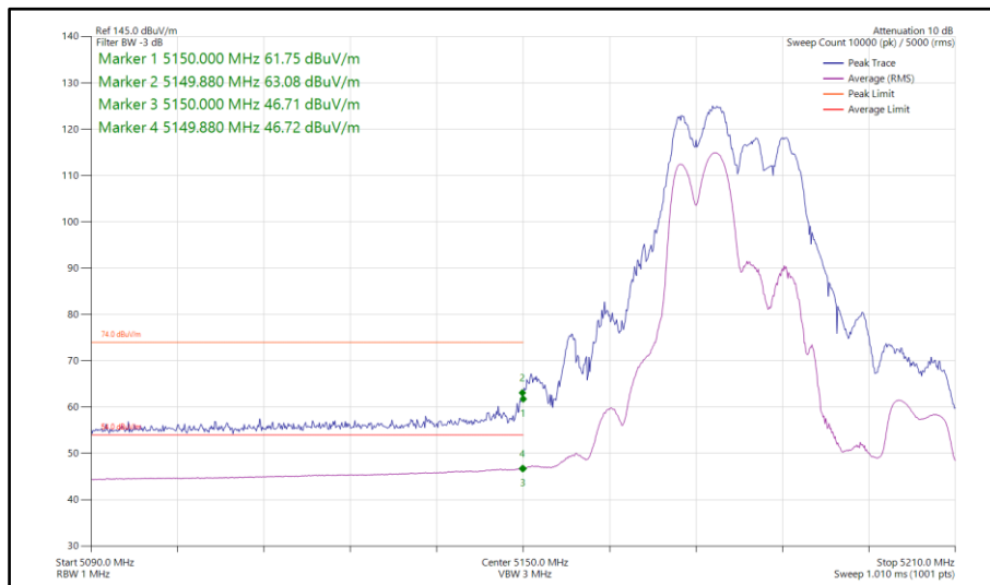
Figure 791 - 802.11ax HE40, RU 106-53, CDD, Core 0-1 - 5190 MHz Band Edge Frequency 5150 MHz
