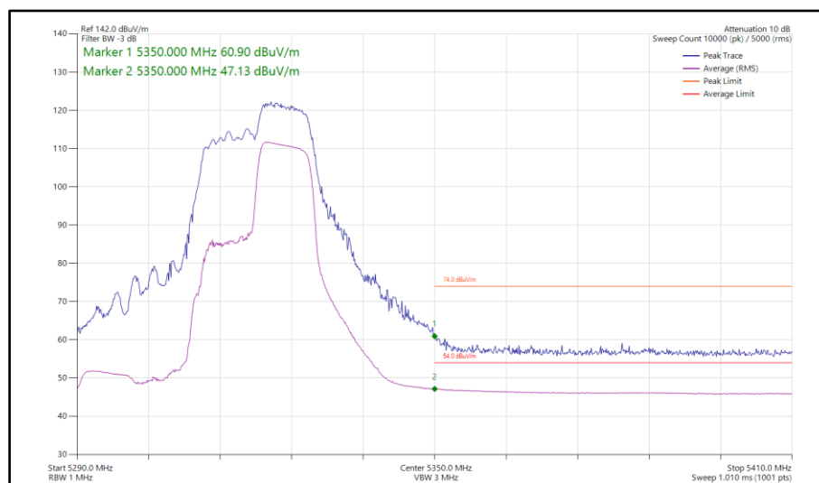
Figure 781 - 802.11ax HE40, RU 106-56, SISO, Core 1 - 5310 MHz Band Edge Frequency 5350 MHz
