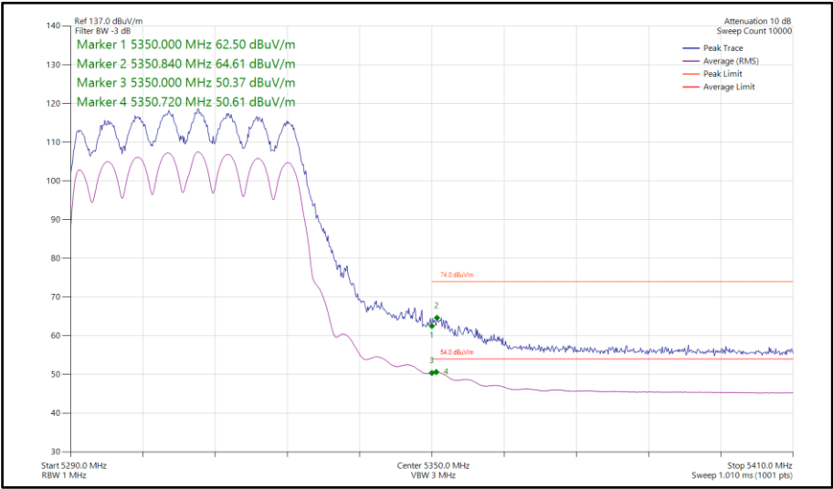
Figure 795 - 802.11ax HE40, SU, CDD, Core 0-1 - 5310 MHz Band Edge Frequency 5350 MHz
