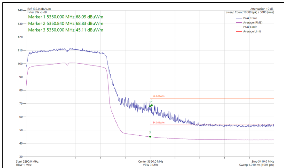
Figure 765 - 802.11ax HE40, SU, SISO, Core 0 - 5310 MHz Band Edge Frequency 5350 MHz
