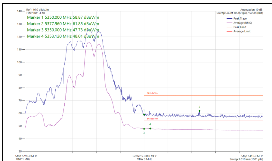
Figure 809 - 802.11ax HE40, RU 106-56, SDM, Core 0-1 - 5310 MHz Band Edge Frequency 5350 MHz
