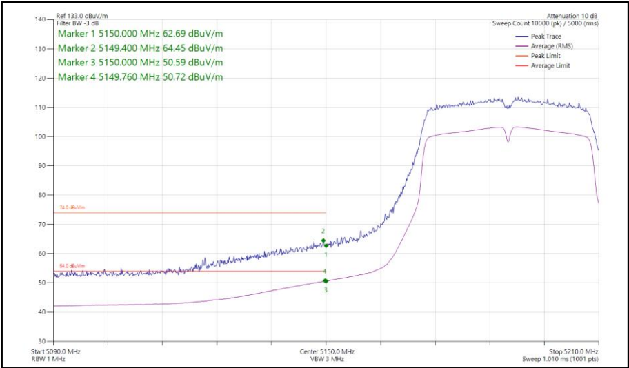
Figure 774 - 802.11n HT40, SISO, Core 1 - 5190 MHz Band Edge Frequency 5150 MHz
