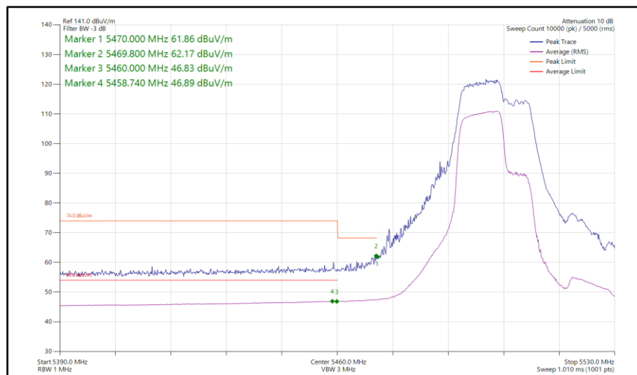
Figure 787 - 802.11be EHT40, RU 106+26-82, SISO, Core 1 - 5510 MHz Band Edge Frequency 5460 MHz
