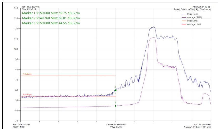
Figure 776 - 802.11ax HE40, RU 52-37, SISO, Core 1 - 5190 MHz Band Edge Frequency 5150 MHz
