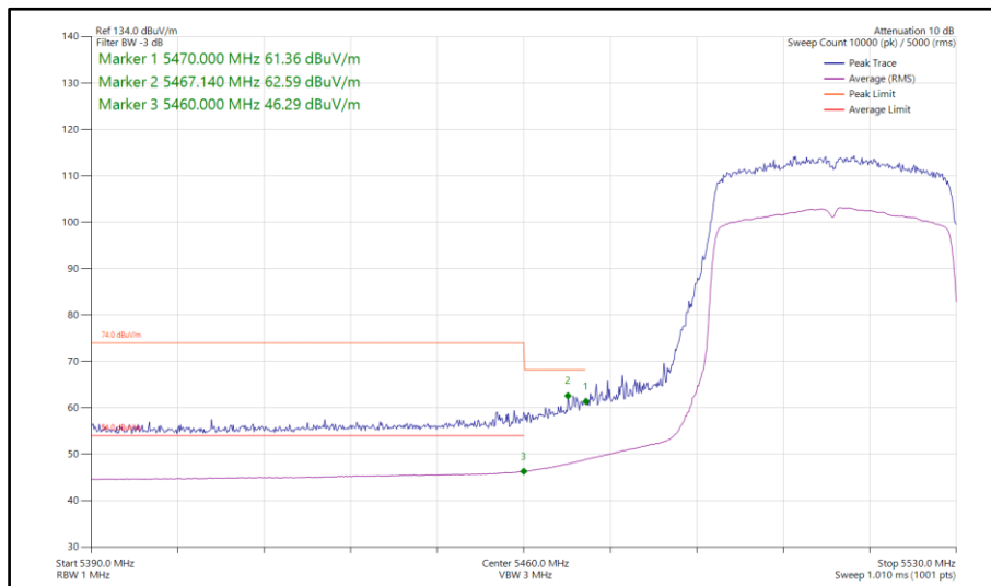
Figure 812 - 802.11ax HE40, SU, SDM, Core 0-1 - 5510 MHz Band Edge Frequency 5460 MHz
