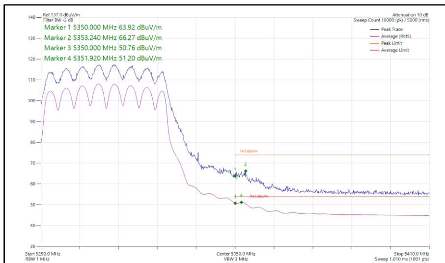
Figure 794 - 802.11n HT40, CDD, Core 0-1 - 5310 MHz Band Edge Frequency 5350 MHz
