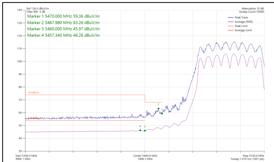
Figure 799 - 802.11n HT40, CDD, Core 0-1 - 5510 MHz Band Edge Frequency 5460 MHz
