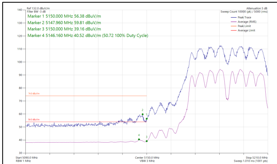
Figure 788 - 802.11a a40, CDD, Core 0-1 - 5190 MHz Band Edge Frequency 5150 MHz
