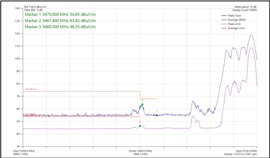
Figure 801 - 802.11ax HE40, RU 52-44, CDD, Core 0-1 - 5510 MHz Band Edge Frequency 5460 MHz
