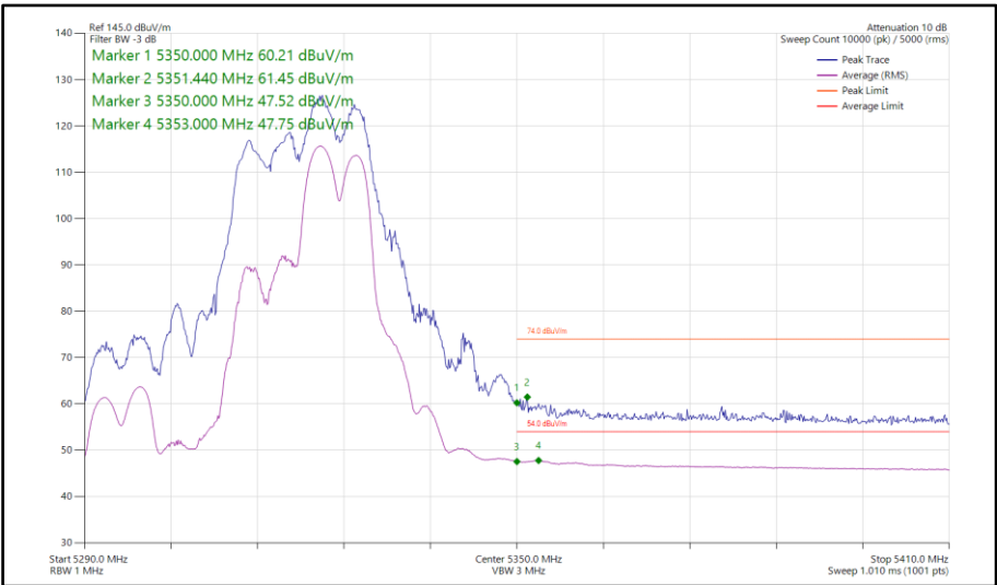
Figure 796 - 802.11ax HE40, RU 106-56, CDD, Core 0-1 - 5310 MHz Band Edge Frequency 5350 MHz
