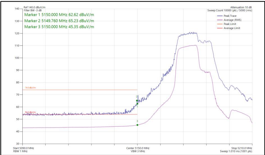
Figure 762 - 802.11be EHT40, RU 106+26-82, SISO, Core 0 - 5190 MHz Band Edge Frequency 5150 MHz
