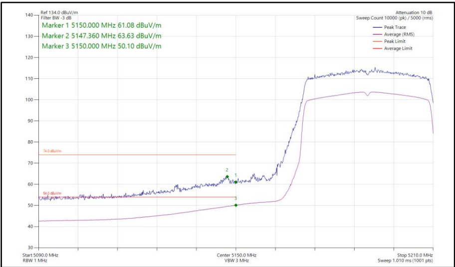
Figure 775 - 802.11ax HE40, SU, SISO, Core 1 - 5190 MHz Band Edge Frequency 5150 MHz
