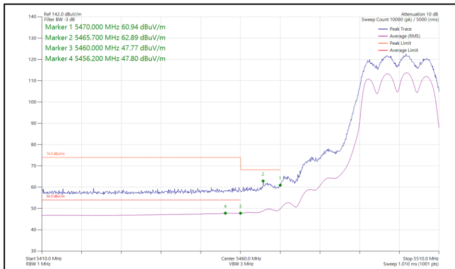
Figure 756 - 802.11ac VHT20, TxBF, Core 0-1 - 5500 MHz Band Edge Frequency 5460 MHz
