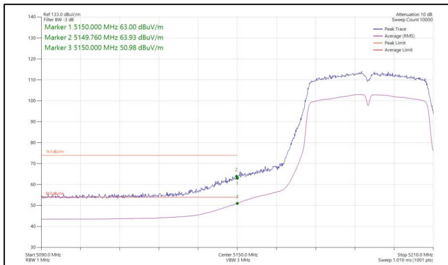
Figure 803 - 802.11n HT40, SDM, Core 0-1 - 5190 MHz Band Edge Frequency 5150 MHz
