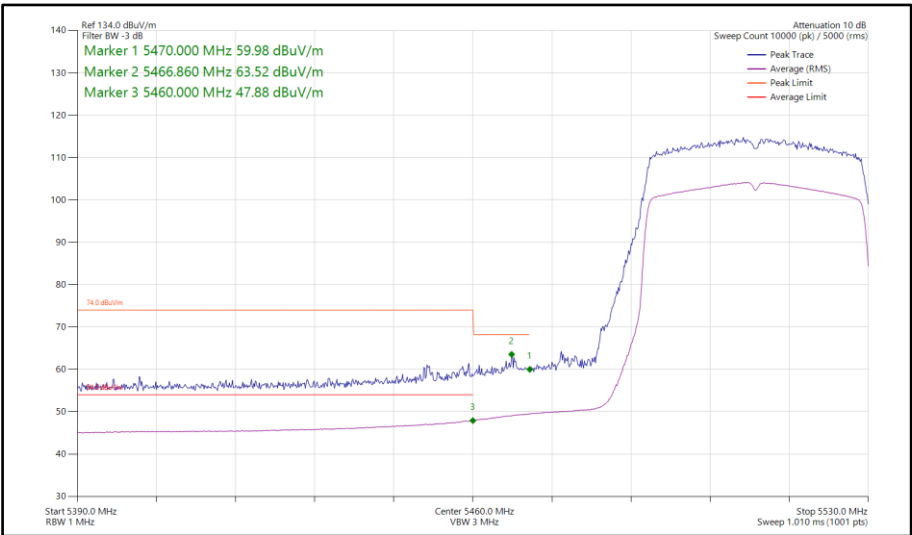
Figure 770 - 802.11ax HE40, SU, SISO, Core 0 - 5510 MHz Band Edge Frequency 5460 MHz
