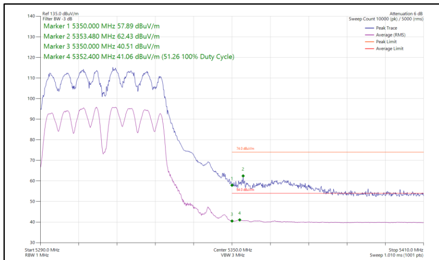
Figure 793 - 802.11a a40, CDD, Core 0-1 - 5310 MHz Band Edge Frequency 5350 MHz
