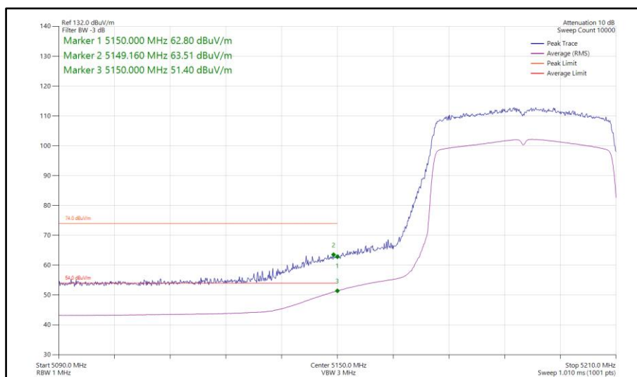
Figure 760 - 802.11ax HE40, SU, SISO, Core 0 - 5190 MHz Band Edge Frequency 5150 MHz
