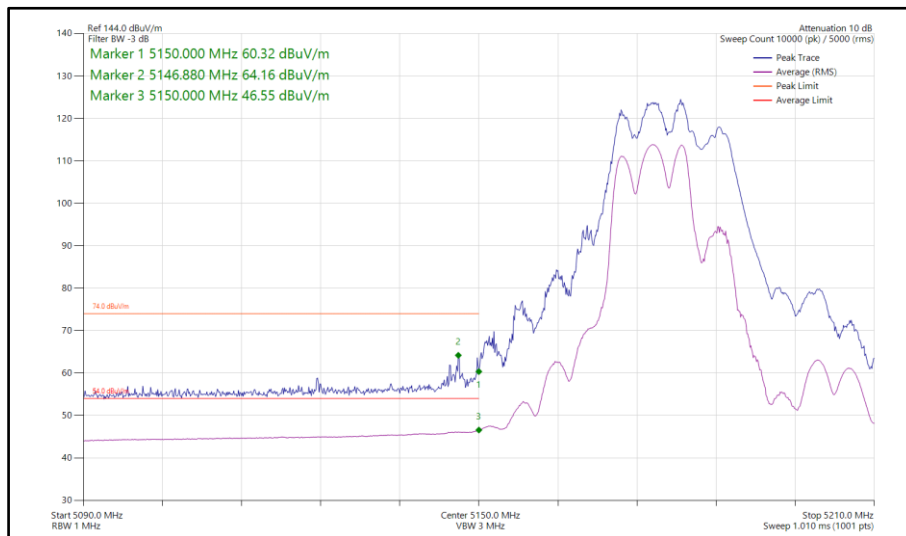
Figure 806 - 802.11be EHT40, RU 106+26-82, SDM, Core 0-1 - 5190 MHz Band Edge Frequency 5150 MHz
