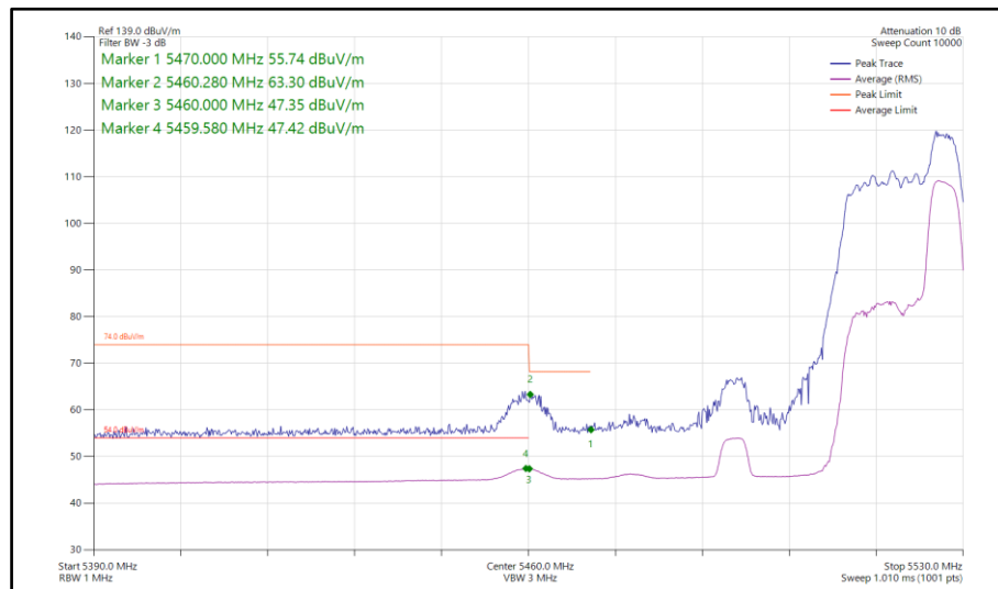
Figure 786 - 802.11ax HE40, RU 52-44, SISO, Core 1 - 5510 MHz Band Edge Frequency 5460 MHz
