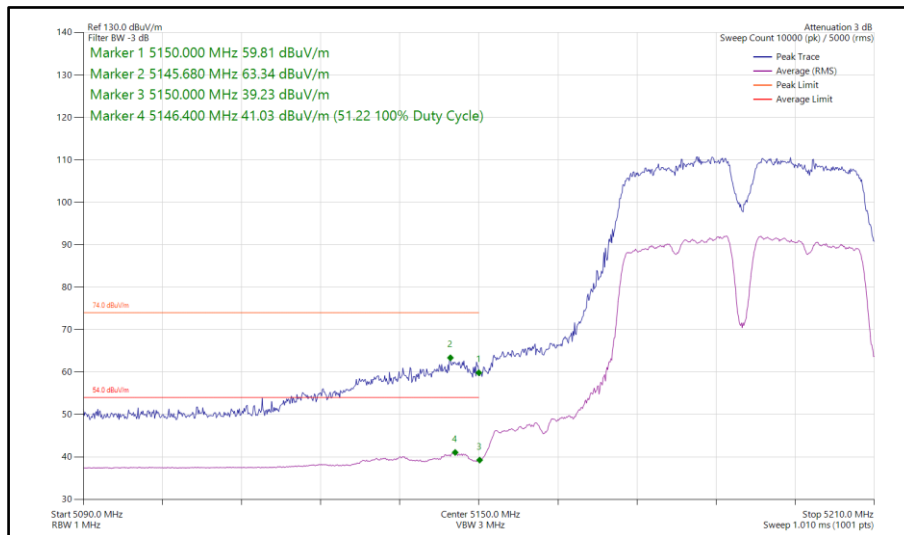
Figure 773 - 802.11a a40, SISO, Core 1 - 5190 MHz Band Edge Frequency 5150 MHz
