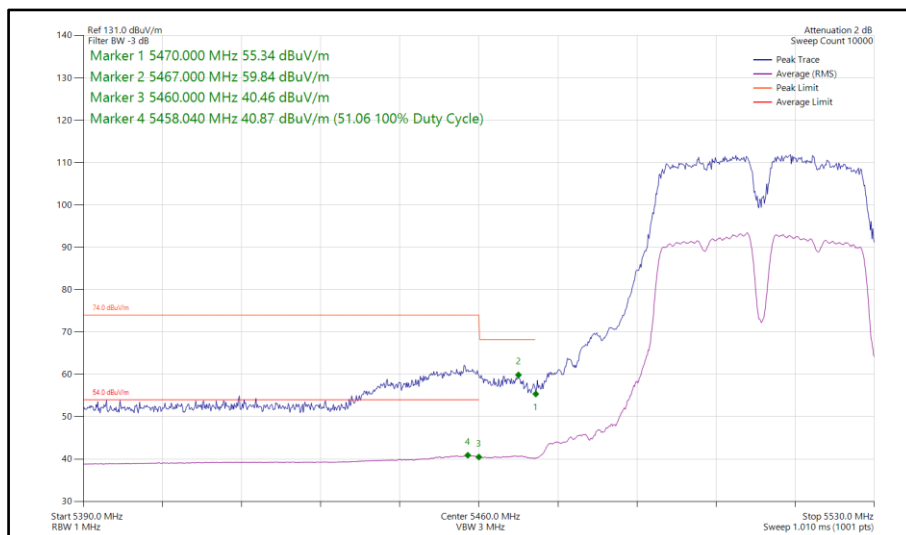
Figure 783 - 802.11a a40, SISO, Core 1 - 5510 MHz Band Edge Frequency 5460 MHz
