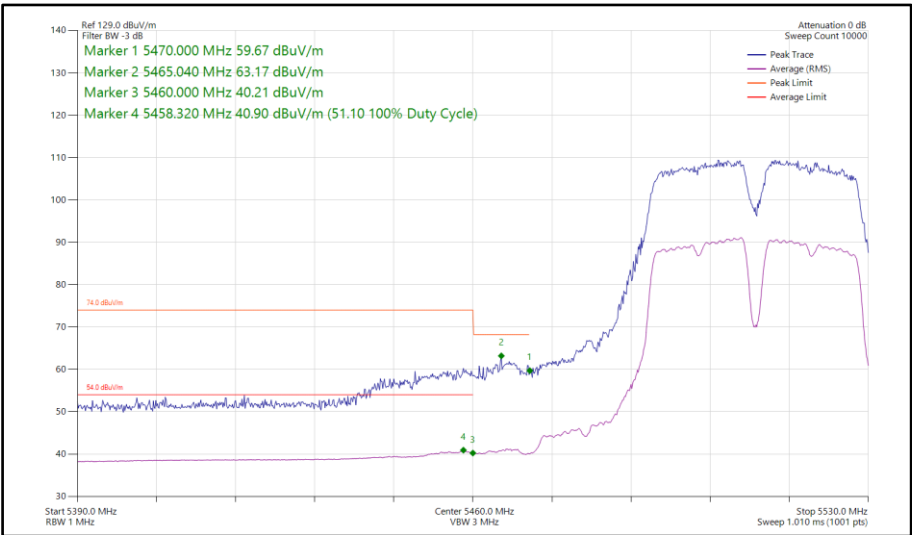
Figure 768 - 802.11a a40, SISO, Core 0 - 5510 MHz Band Edge Frequency 5460 MHz
