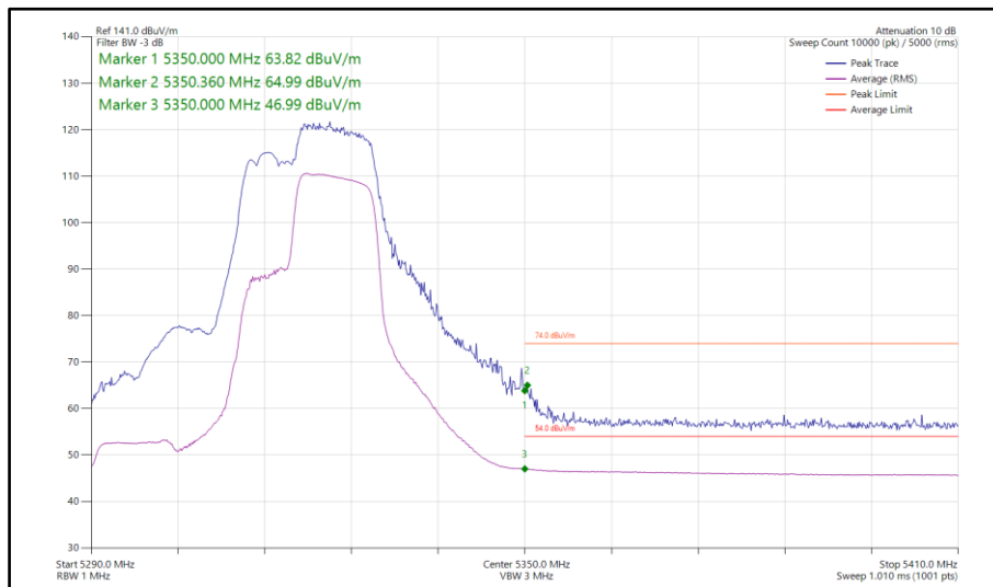
Figure 782 - 802.11be EHT40, RU 106+26-85, SISO, Core 1 - 5310 MHz Band Edge Frequency 5350 MHz
