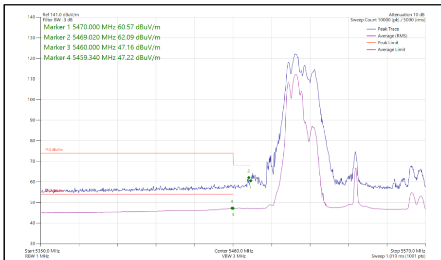
Figure 876 - 802.11ax HE80, RU 106-53, SDM, Core 0-1 - 5530 MHz Band Edge Frequency 5460 MHz
