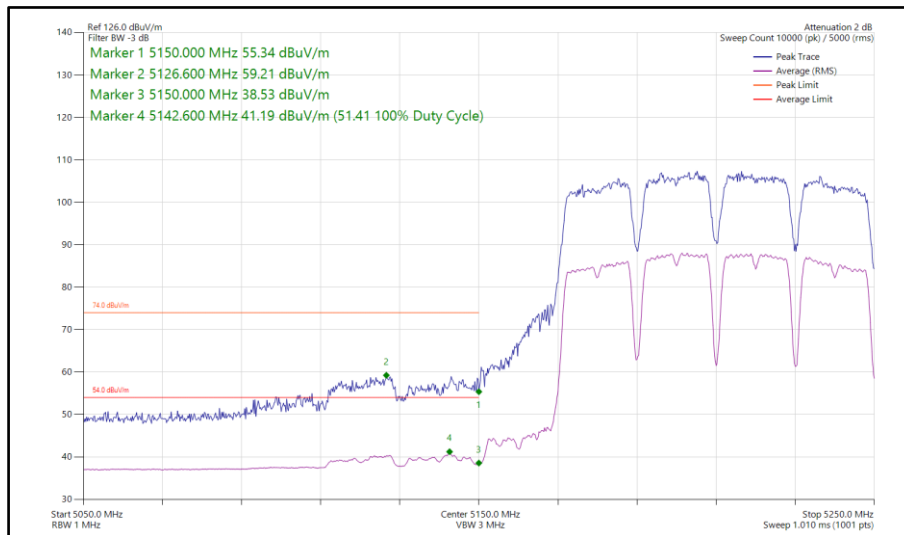
Figure 836 - 802.11a a80, SISO, Core 1 - 5210 MHz Band Edge Frequency 5150 MHz
