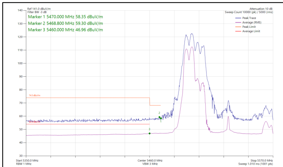
Figure 864 - 802.11ax HE80, RU 106-53, CDD, Core 0-1 - 5530 MHz Band Edge Frequency 5460 MHz
