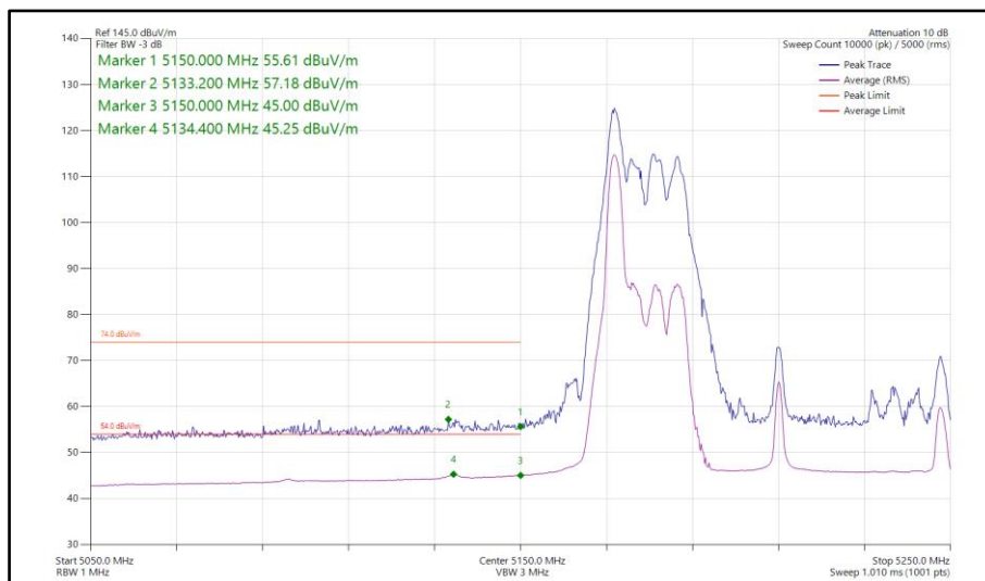
Figure 868 - 802.11ax HE80, RU 26-0, SDM, Core 0-1 - 5210 MHz Band Edge Frequency 5150 MHz
