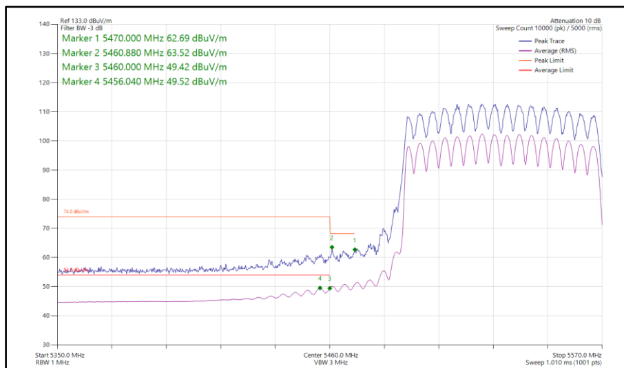
Figure 863 - 802.11ax HE80, SU, CDD, Core 0-1 - 5530 MHz Band Edge Frequency 5460 MHz
