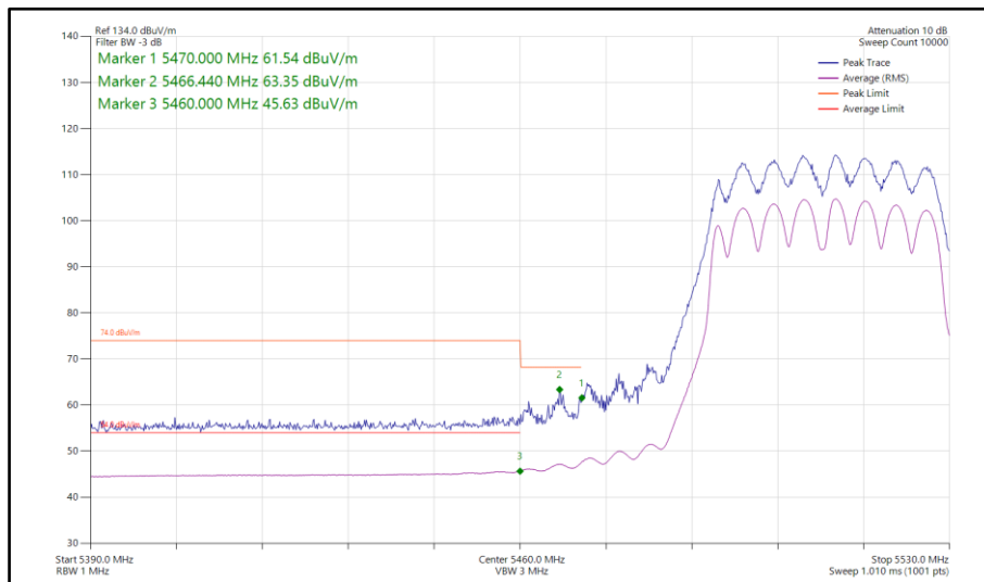
Figure 819 - 802.11ac VHT40, TxBF, Core 0-1 - 5510 MHz Band Edge Frequency 5460 MHz
