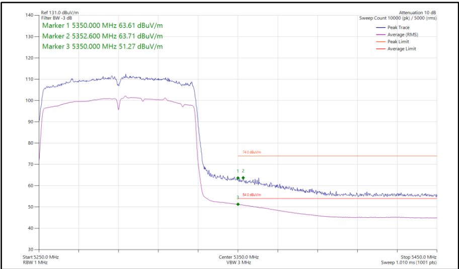
Figure 870 - 802.11ac VHT80, SDM, Core 0-1 - 5290 MHz Band Edge Frequency 5350 MHz
