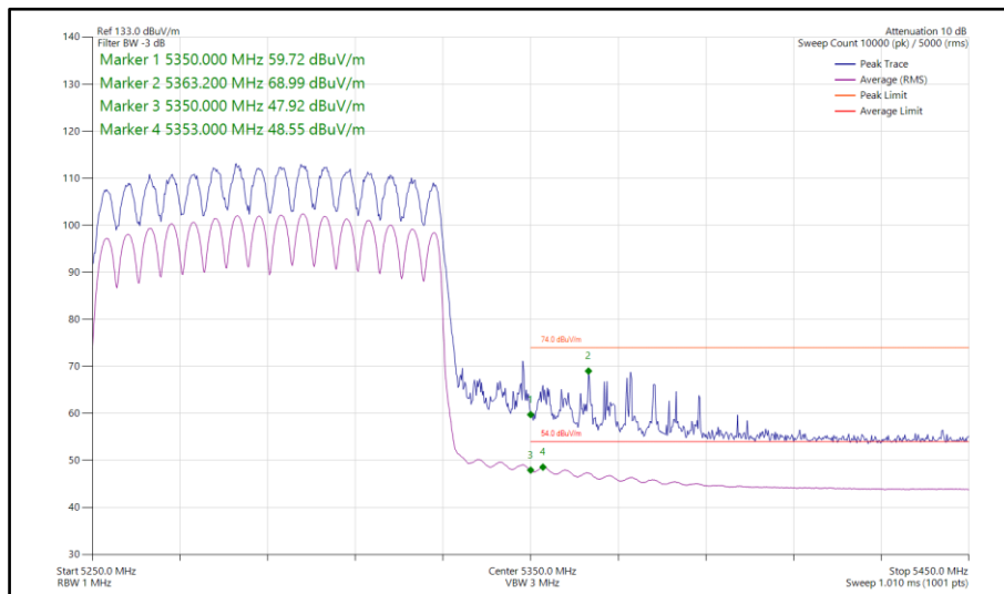
Figure 858 - 802.11ax HE80, SU, CDD, Core 0-1 - 5290 MHz Band Edge Frequency 5350 MHz
