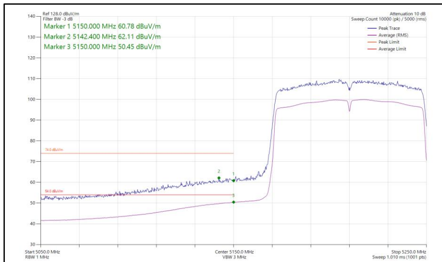
Figure 837 - 802.11ac VHT80, SISO, Core 1 - 5210 MHz Band Edge Frequency 5150 MHz
