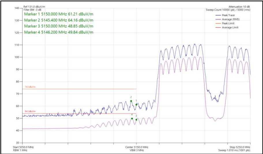
Figure 869 - 802.11be EHT80, RU 484+242-92, SDM, Core 0-1 - 5210 MHz Band Edge Frequency 5150 MHz
