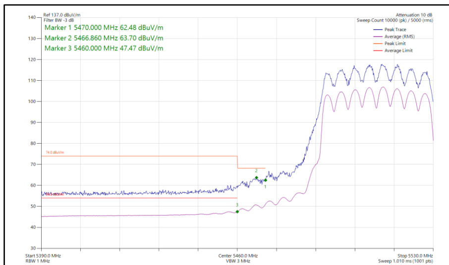
Figure 820 - 802.11ax HE40, SU, TxBF, Core 0-1 - 5510 MHz Band Edge Frequency 5460 MHz
