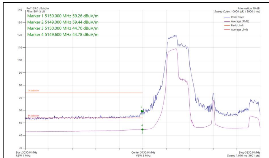
Figure 824 - 802.11ax HE80, RU 106-53, SISO, Core 0 - 5210 MHz Band Edge Frequency 5150 MHz
