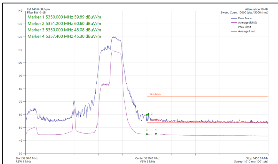
Figure 829 - 802.11ax HE80, RU 106-60, SISO, Core 0 - 5290 MHz Band Edge Frequency 5350 MHz
