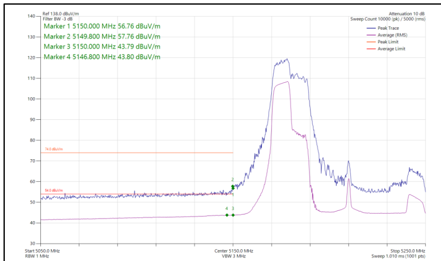
Figure 839 - 802.11ax HE80, RU 106-53, SISO, Core 1 - 5210 MHz Band Edge Frequency 5150 MHz
