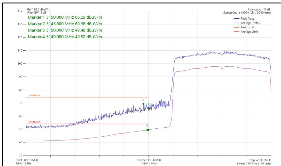
Figure 838 - 802.11ax HE80, SU, SISO, Core 1 - 5210 MHz Band Edge Frequency 5150 MHz
