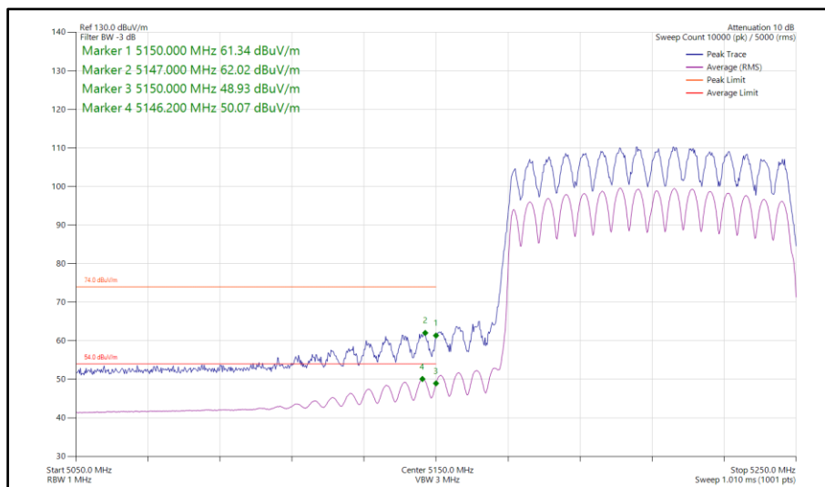
Figure 853 - 802.11ax HE80, SU, CDD, Core 0-1 - 5210 MHz Band Edge Frequency 5150 MHz
