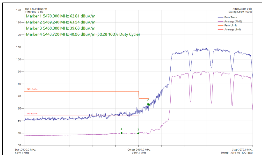
Figure 846 - 802.11a a80, SISO, Core 1 - 5530 MHz Band Edge Frequency 5460 MHz
