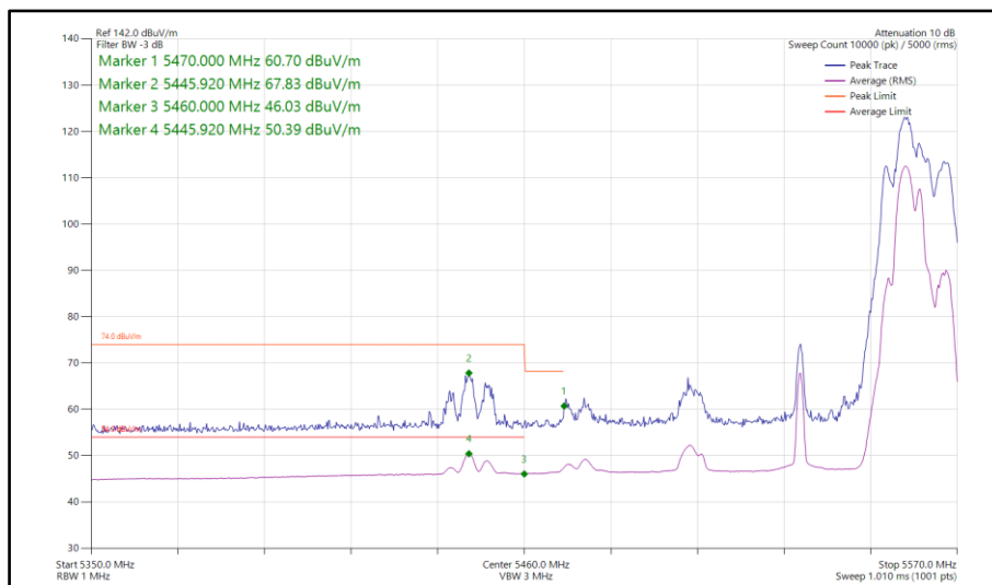
Figure 865 - 802.11be EHT80, RU 52+26-80, CDD, Core 0-1 - 5530 MHz Band Edge Frequency 5460 MHz
