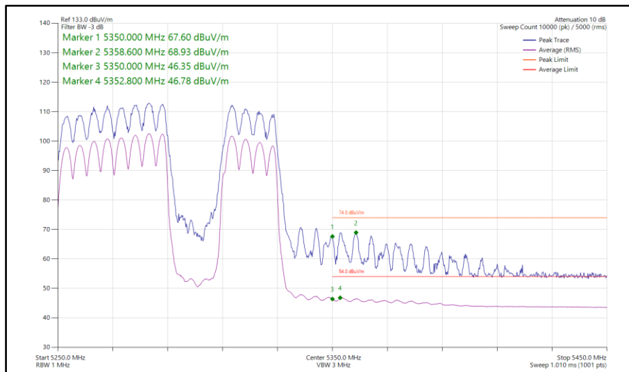
Figure 860 - 802.11be EHT80, RU 484+242-92, CDD, Core 0-1 - 5290 MHz Band Edge Frequency 5350 MHz
