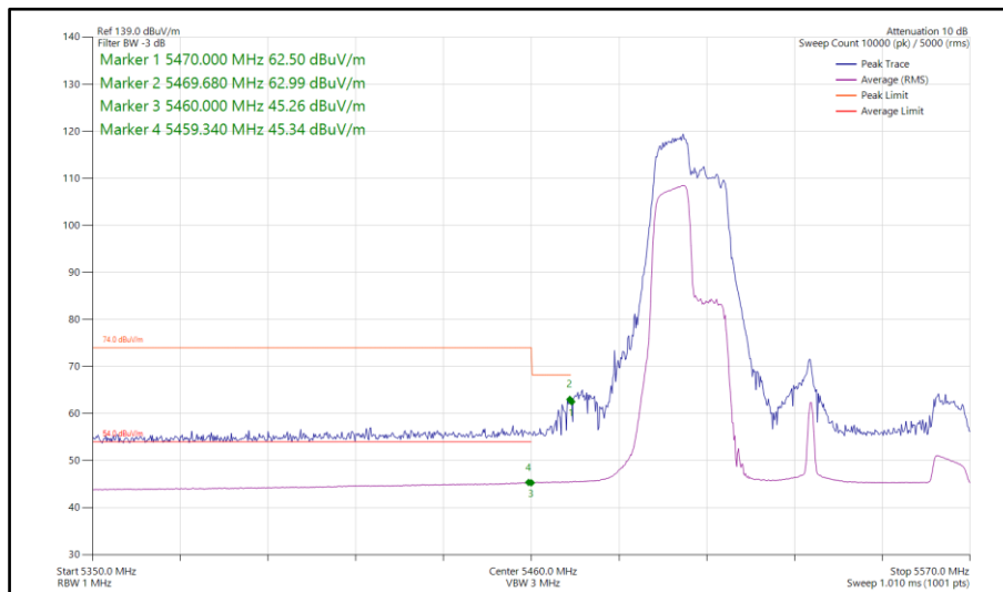
Figure 834 - 802.11ax HE80, RU 106-53, SISO, Core 0 - 5530 MHz Band Edge Frequency 5460 MHz
