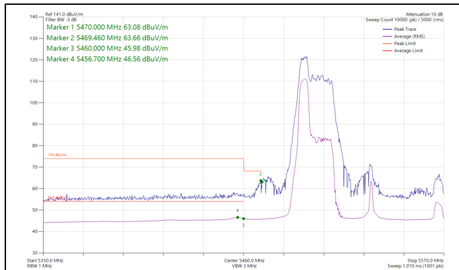
Figure 849 - 802.11ax HE80, RU 52-37, SISO, Core 1 - 5530 MHz Band Edge Frequency 5460 MHz
