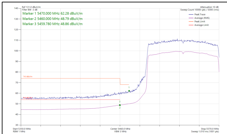
Figure 875 - 802.11ax HE80, SU, SDM, Core 0-1 - 5530 MHz Band Edge Frequency 5460 MHz
