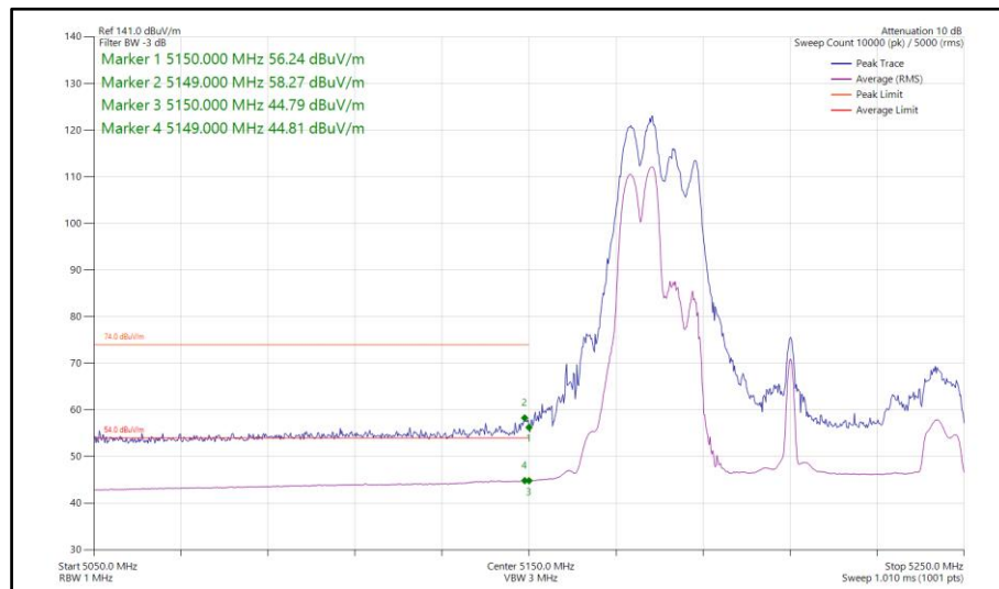
Figure 854 - 802.11ax HE80, RU 106-53, CDD, Core 0-1 - 5210 MHz Band Edge Frequency 5150 MHz
