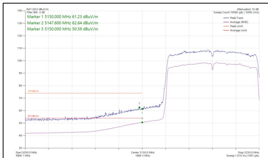
Figure 866 - 802.11ac VHT80, SDM, Core 0-1 - 5210 MHz Band Edge Frequency 5150 MHz
