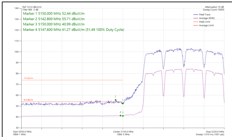
Figure 821 - 802.11a a80, SISO, Core 0 - 5210 MHz Band Edge Frequency 5150 MHz
