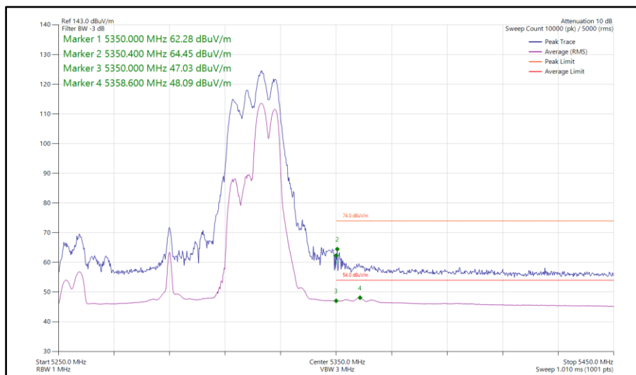
Figure 872 - 802.11ax HE80, RU 106-60, SDM, Core 0-1 - 5290 MHz Band Edge Frequency 5350 MHz
