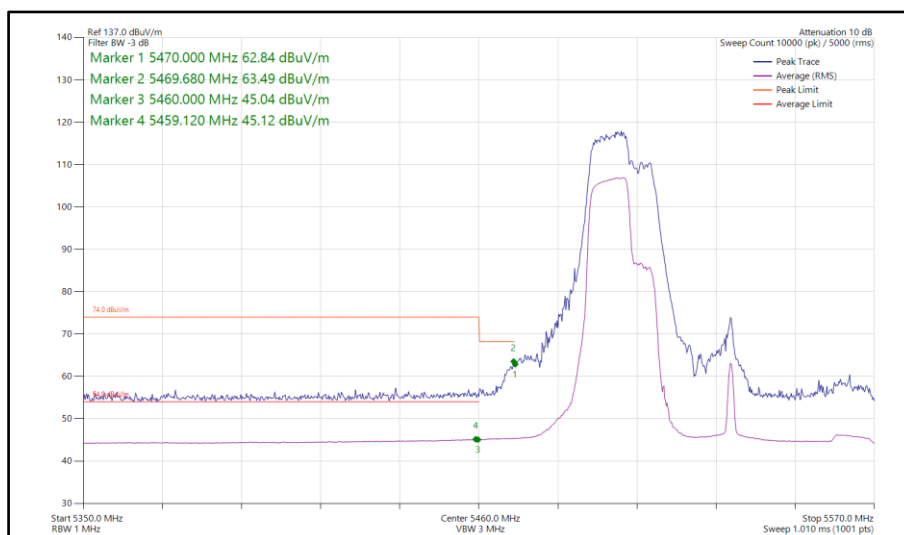
Figure 835 - 802.11be EHT80, RU 106+26-82, SISO, Core 0 - 5530 MHz Band Edge Frequency 5460 MHz
