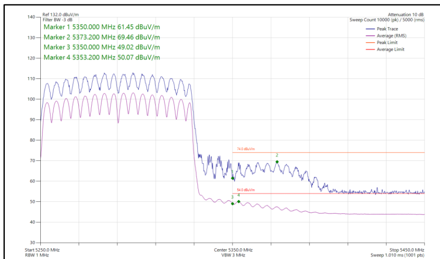
Figure 857 - 802.11ac VHT80, CDD, Core 0-1 - 5290 MHz Band Edge Frequency 5350 MHz
