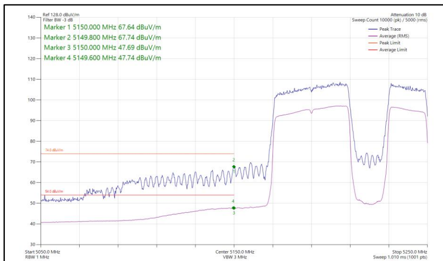
Figure 840 - 802.11be EHT80, RU 484+242-92, SISO, Core 1 - 5210 MHz Band Edge Frequency 5150 MHz
