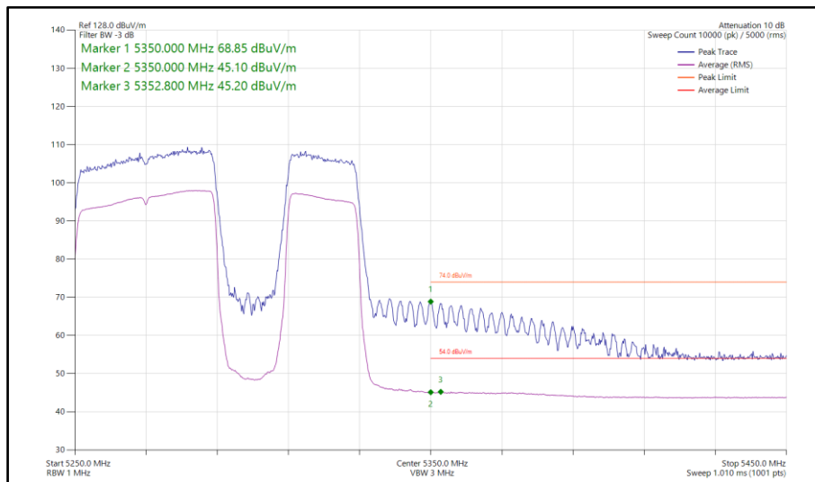
Figure 845 - 802.11be EHT80, RU 484+242-92, SISO, Core 1 - 5290 MHz Band Edge Frequency 5350 MHz
