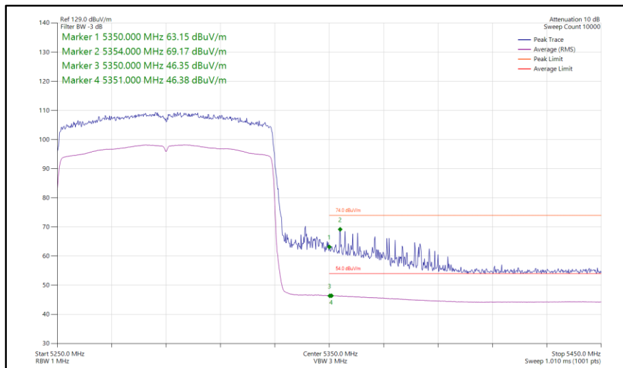
Figure 828 - 802.11ax HE80, SU, SISO, Core 0 - 5290 MHz Band Edge Frequency 5350 MHz
