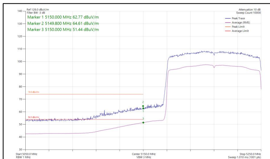
Figure 823 - 802.11ax HE80, SU, SISO, Core 0 - 5210 MHz Band Edge Frequency 5150 MHz
