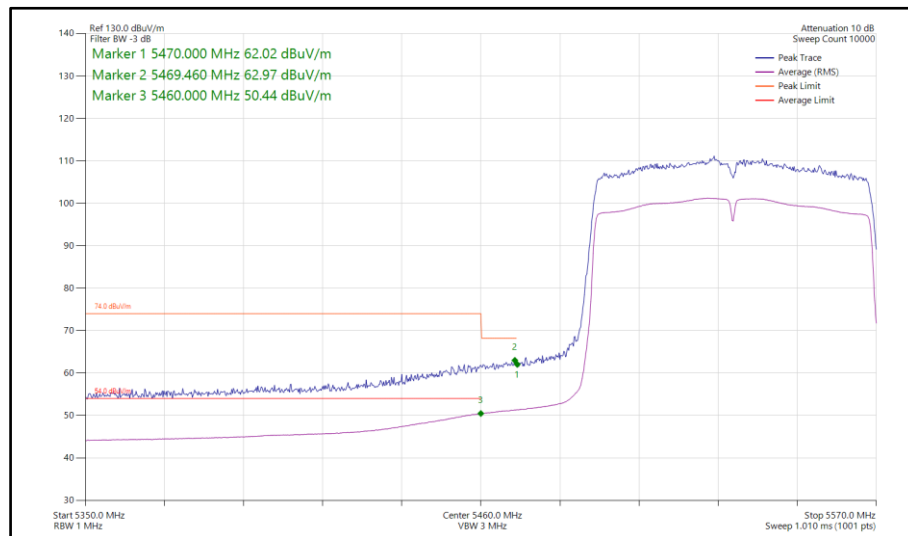
Figure 847 - 802.11ac VHT80, SISO, Core 1 - 5530 MHz Band Edge Frequency 5460 MHz
