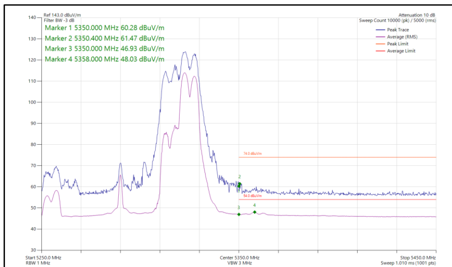
Figure 859 - 802.11ax HE80, RU 106-60, CDD, Core 0-1 - 5290 MHz Band Edge Frequency 5350 MHz
