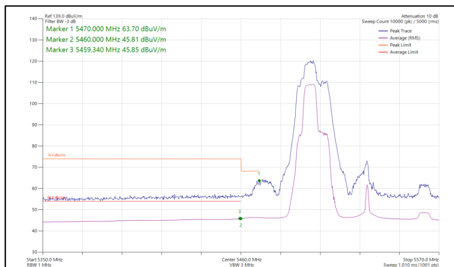
Figure 850 - 802.11be EHT80, RU 52+26-71, SISO, Core 1 - 5530 MHz Band Edge Frequency 5460 MHz
