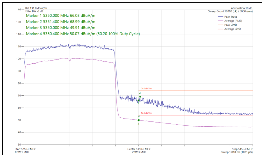
Figure 871 - 802.11ax HE80, SU, SDM, Core 0-1 - 5290 MHz Band Edge Frequency 5350 MHz
