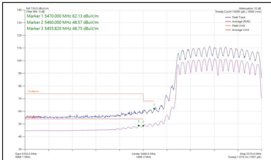
Figure 862 - 802.11ac VHT80, CDD, Core 0-1 - 5530 MHz Band Edge Frequency 5460 MHz
