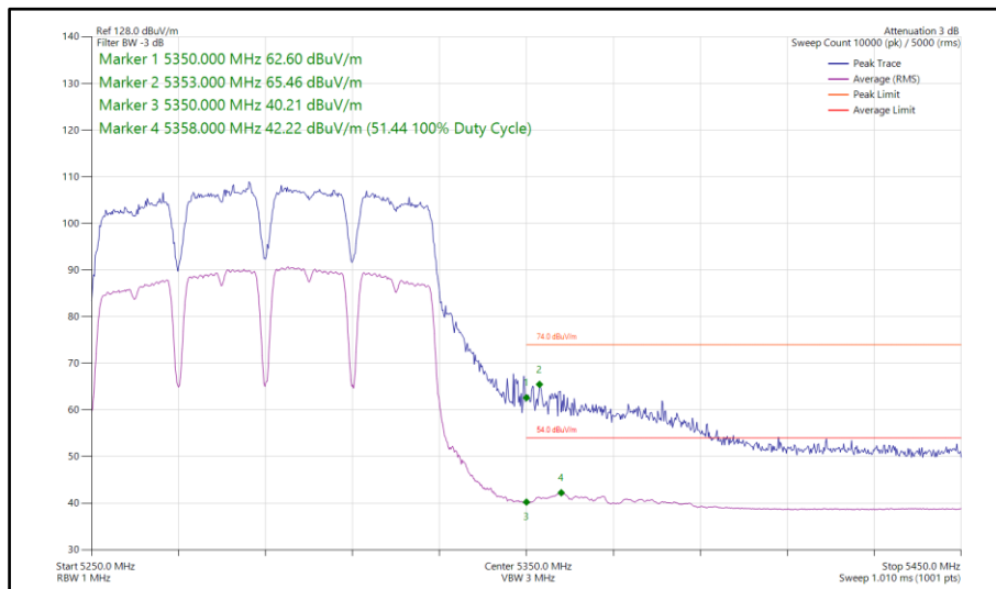
Figure 826 - 802.11a a80, SISO, Core 0 - 5290 MHz Band Edge Frequency 5350 MHz
