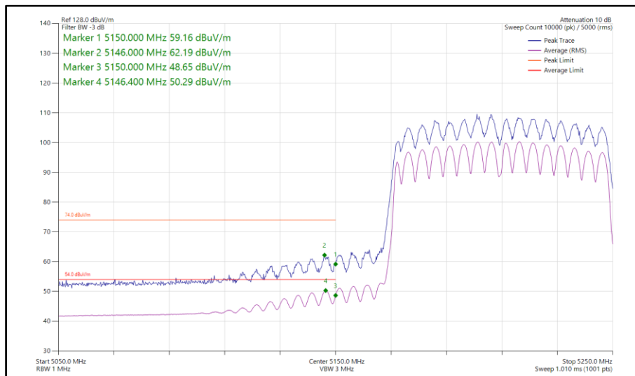
Figure 852 - 802.11ac VHT80, CDD, Core 0-1 - 5210 MHz Band Edge Frequency 5150 MHz
