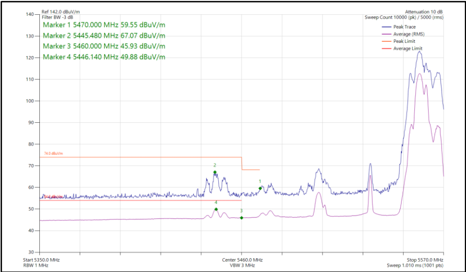
Figure 877 - 802.11be EHT80, RU 52+26-80, SDM, Core 0-1 - 5530 MHz Band Edge Frequency 5460 MHz
