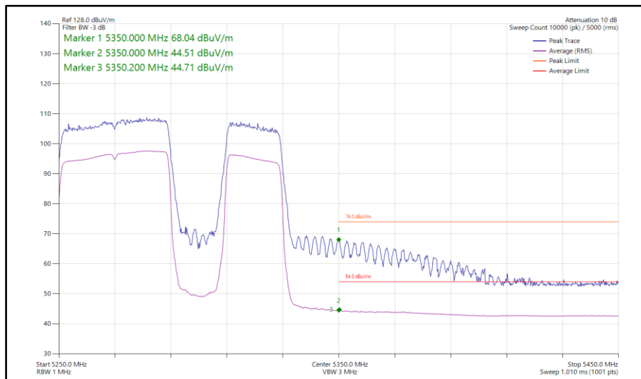
Figure 830 - 802.11be EHT80, RU 484+242-92, SISO, Core 0 - 5290 MHz Band Edge Frequency 5350 MHz
