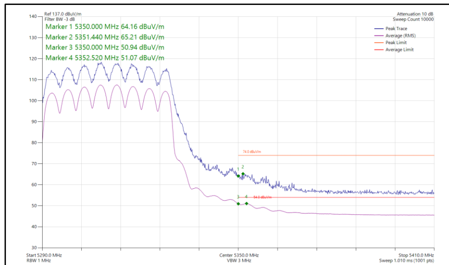
Figure 818 - 802.11ax HE40, SU, TxBF, Core 0-1 - 5310 MHz Band Edge Frequency 5350 MHz
