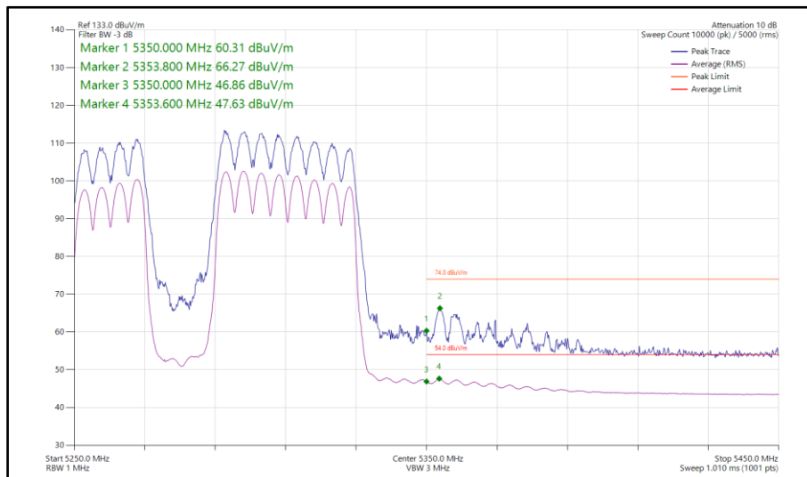
Figure 873 - 802.11be EHT80, RU 484+242-91, SDM, Core 0-1 - 5290 MHz Band Edge Frequency 5350 MHz
