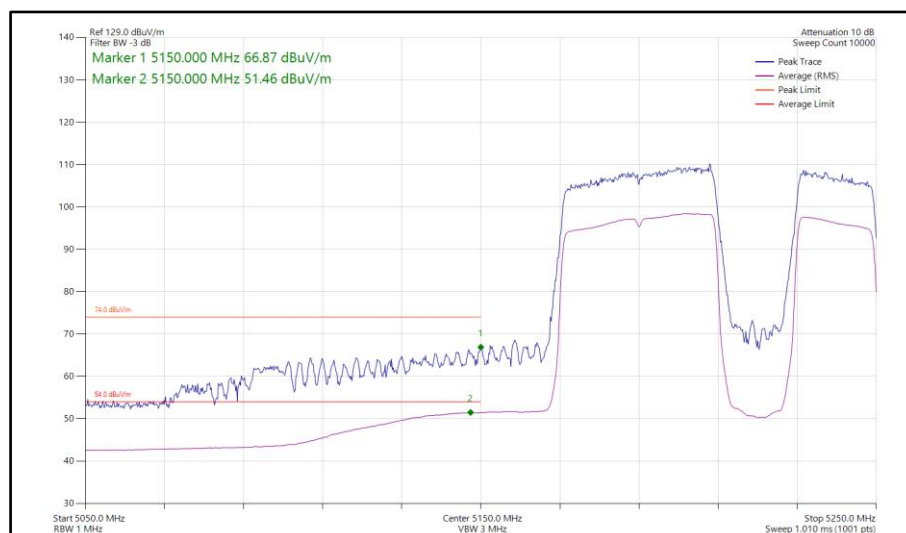
Figure 825 - 802.11be EHT80, RU 484+242-92, SISO, Core 0 - 5210 MHz Band Edge Frequency 5150 MHz
