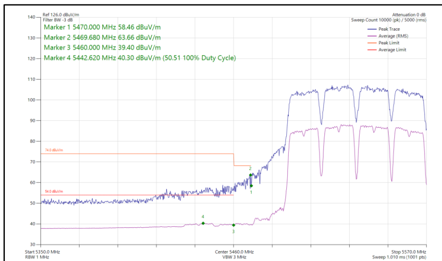
Figure 831 - 802.11a a80, SISO, Core 0 - 5530 MHz Band Edge Frequency 5460 MHz
