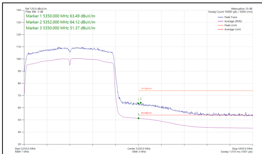
Figure 827 - 802.11ac VHT80, SISO, Core 0 - 5290 MHz Band Edge Frequency 5350 MHz
