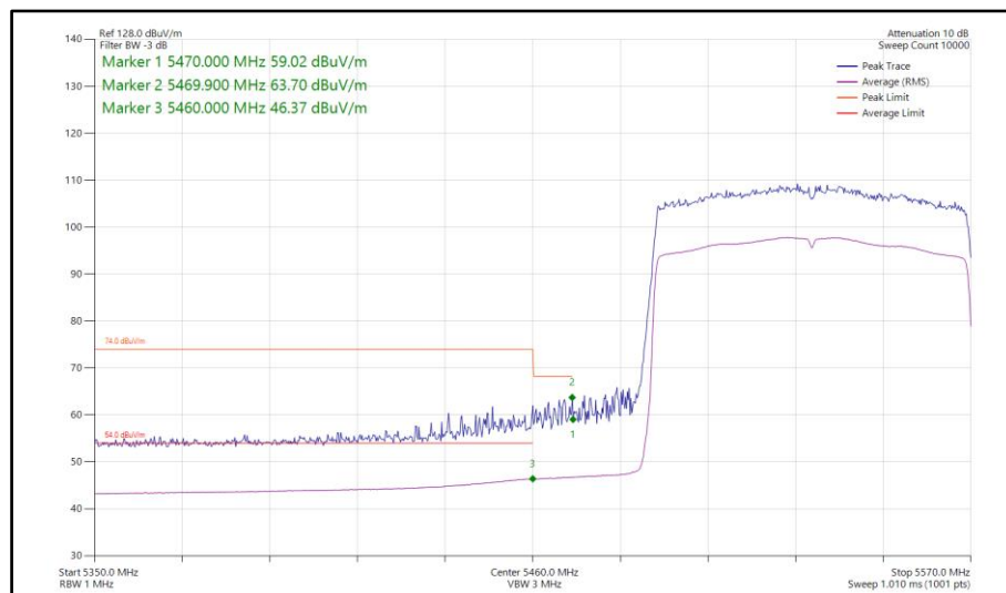
Figure 848 - 802.11ax HE80, SU, SISO, Core 1 - 5530 MHz Band Edge Frequency 5460 MHz
