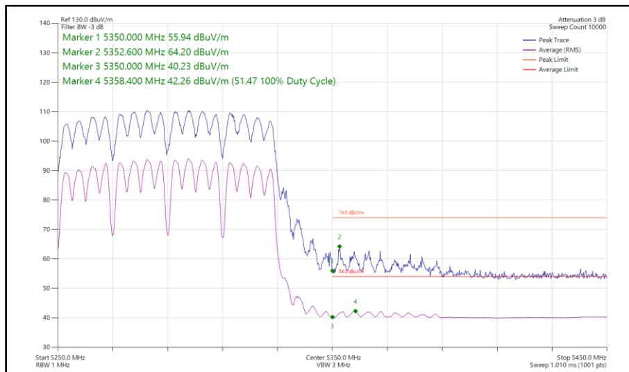
Figure 856 - 802.11a a80, CDD, Core 0-1 - 5290 MHz Band Edge Frequency 5350 MHz
