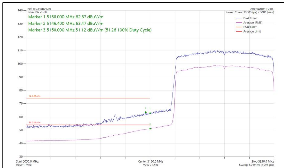
Figure 867 - 802.11ax HE80, SU, SDM, Core 0-1 - 5210 MHz Band Edge Frequency 5150 MHz
