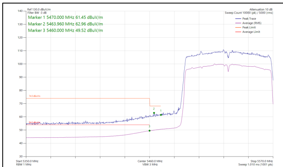
Figure 874 - 802.11ac VHT80, SDM, Core 0-1 - 5530 MHz Band Edge Frequency 5460 MHz
