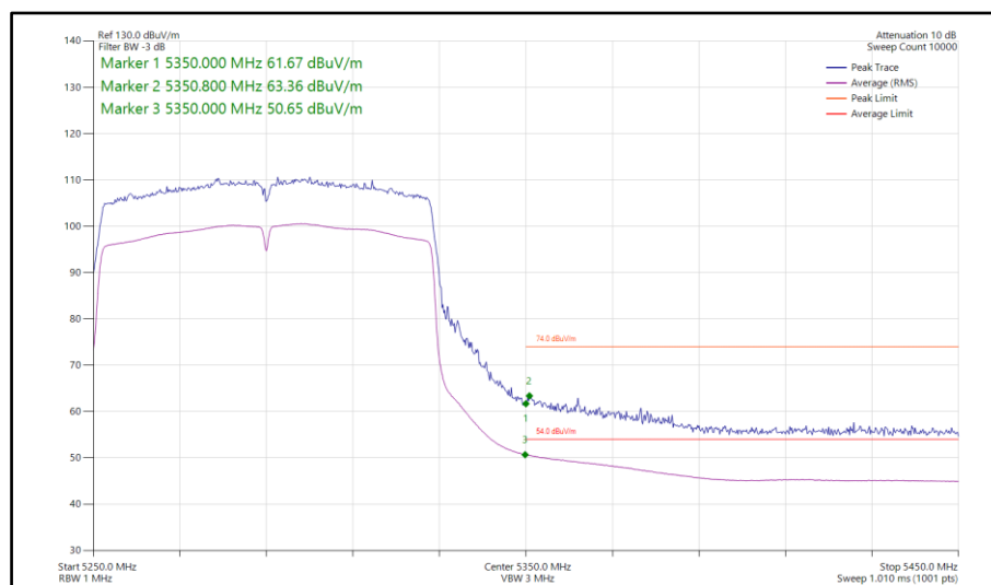
Figure 842 - 802.11ac VHT80, SISO, Core 1 - 5290 MHz Band Edge Frequency 5350 MHz
