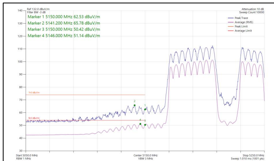
Figure 855 - 802.11be EHT80, RU 484+242-92, CDD, Core 0-1 - 5210 MHz Band Edge Frequency 5150 MHz
