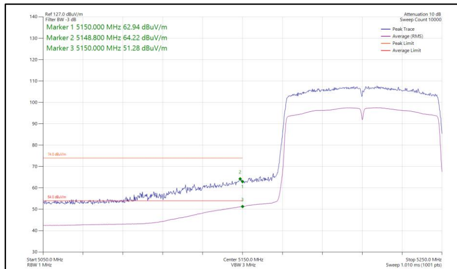
Figure 822 - 802.11ac VHT80, SISO, Core 0 - 5210 MHz Band Edge Frequency 5150 MHz
