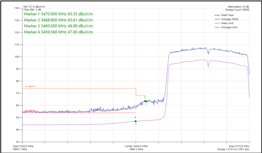
Figure 832 - 802.11ac VHT80, SISO, Core 0 - 5530 MHz Band Edge Frequency 5460 MHz
