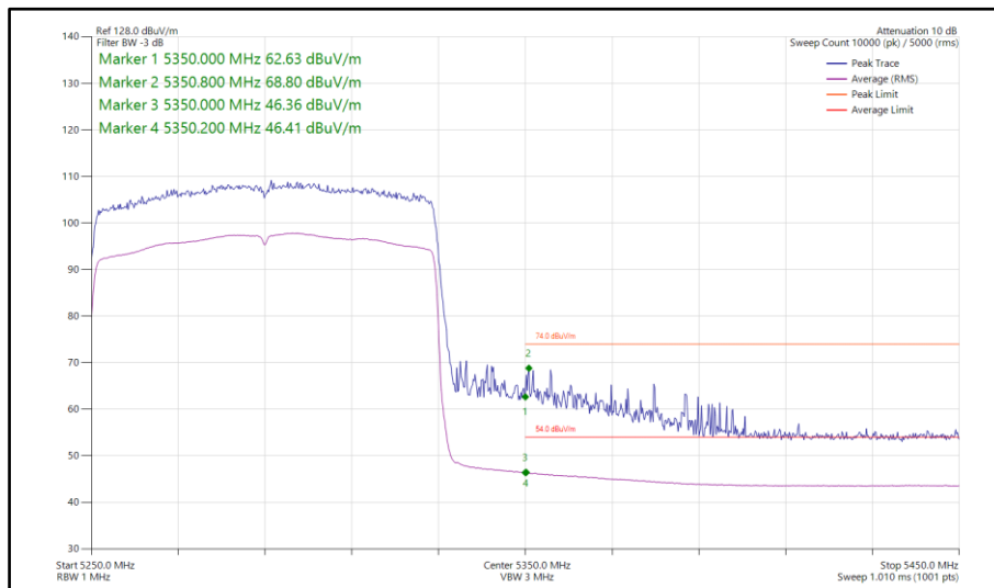
Figure 843 - 802.11ax HE80, SU, SISO, Core 1 - 5290 MHz Band Edge Frequency 5350 MHz
