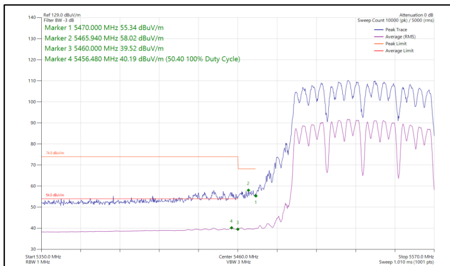
Figure 861 - 802.11a a80, CDD, Core 0-1 - 5530 MHz Band Edge Frequency 5460 MHz
