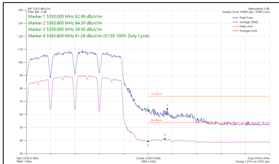
Figure 841 - 802.11a a80, SISO, Core 1 - 5290 MHz Band Edge Frequency 5350 MHz
