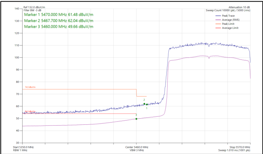
Figure 833 - 802.11ax HE80, SU, SISO, Core 0 - 5530 MHz Band Edge Frequency 5460 MHz
