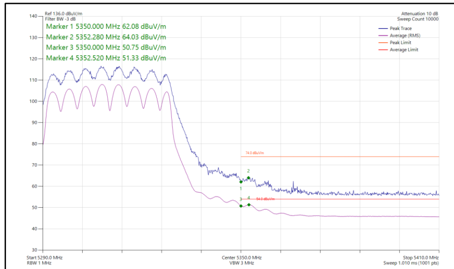
Figure 817 - 802.11ac VHT40, TxBF, Core 0-1 - 5310 MHz Band Edge Frequency 5350 MHz
