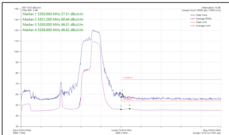
Figure 844 - 802.11ax HE80, RU 106-60, SISO, Core 1 - 5290 MHz Band Edge Frequency 5350 MHz
