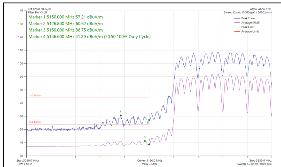
Figure 851 - 802.11a a80, CDD, Core 0-1 - 5210 MHz Band Edge Frequency 5150 MHz
