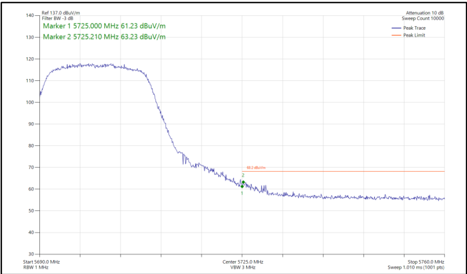
Figure 88 - 802.11n HT20, SISO, Core 1 - 5700 MHz Band Edge Frequency 5725 MHz
