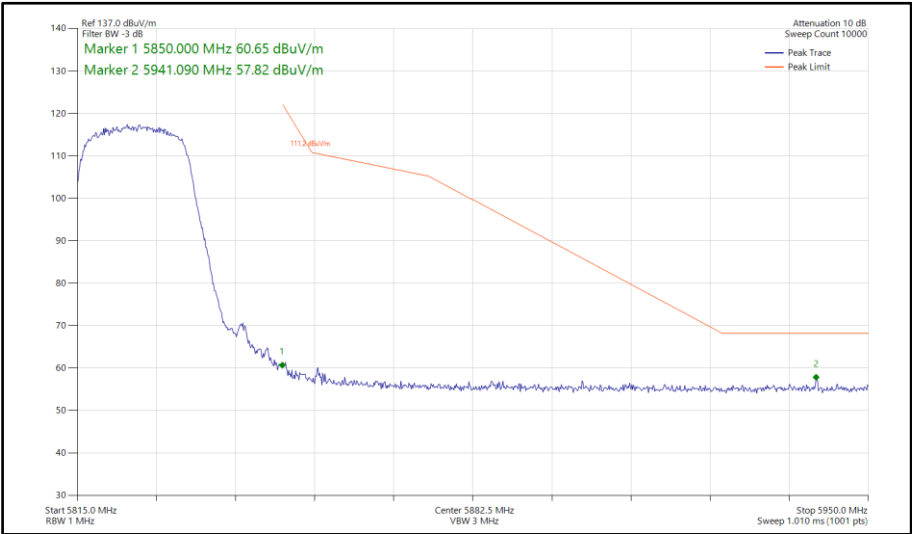
Figure 68 - 802.11a, SISO, Core 0 - 5825 MHz Band Edge Frequency 5850 MHz
