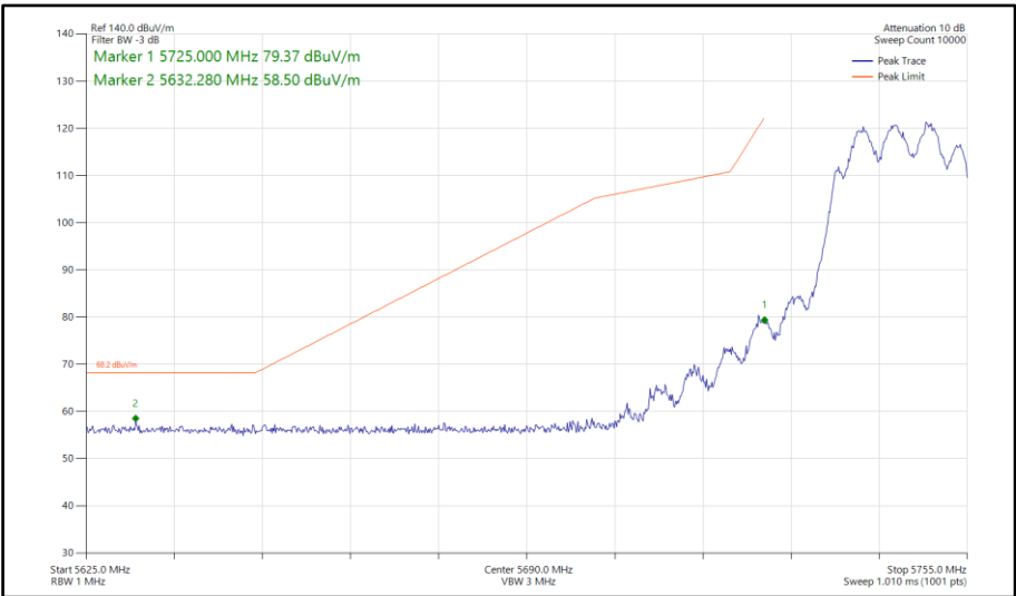
Figure 109 - 802.11ax HE20, SU, CDD, Core 0-1 - 5745 MHz Band Edge Frequency 5725 MHz
