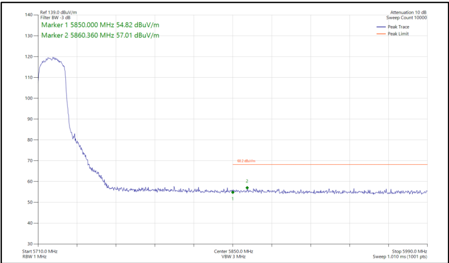
Figure 96 - 802.11ax HE20, SU, SISO, Core 1 - 5720 MHz Band Edge Frequency 5850 MHz
