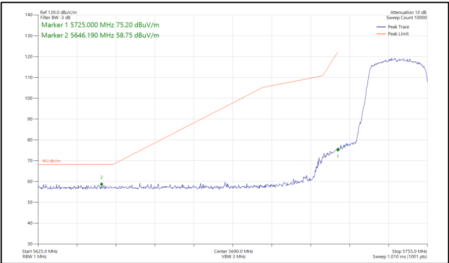
Figure 84 - 802.11ax HE20, SU, SISO, Core 1 - 5745 MHz Band Edge Frequency 5725 MHz
