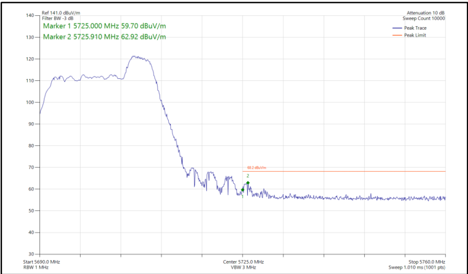
Figure 65 - 802.11ax HE20, RU 52-40, SISO, Core 0 - 5700 MHz Band Edge Frequency 5725 MHz
