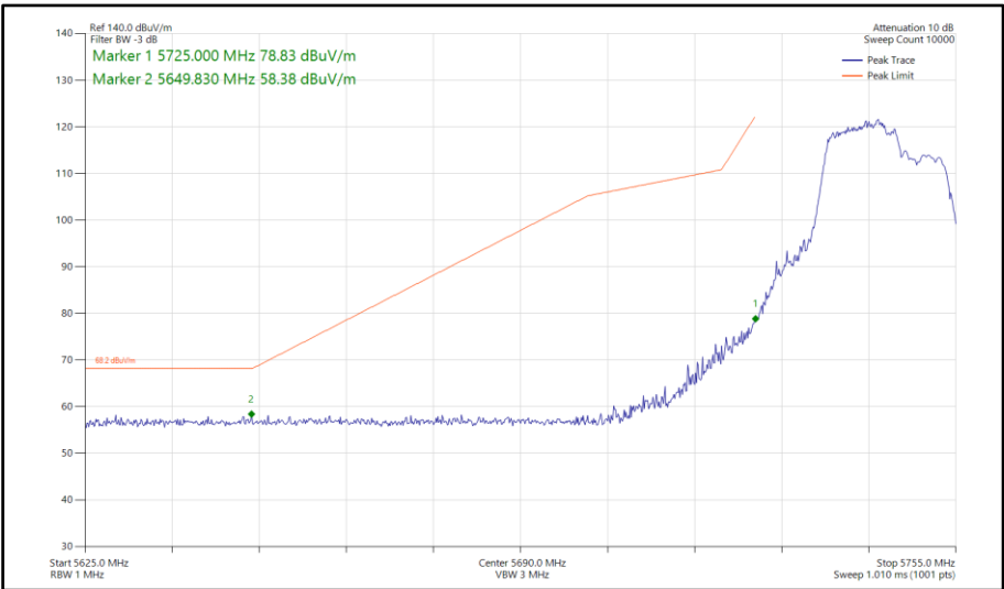
Figure 86 - 802.11be EHT20, RU 106+26-82, SISO, Core 1 - 5745 MHz Band Edge Frequency 5725 MHz
