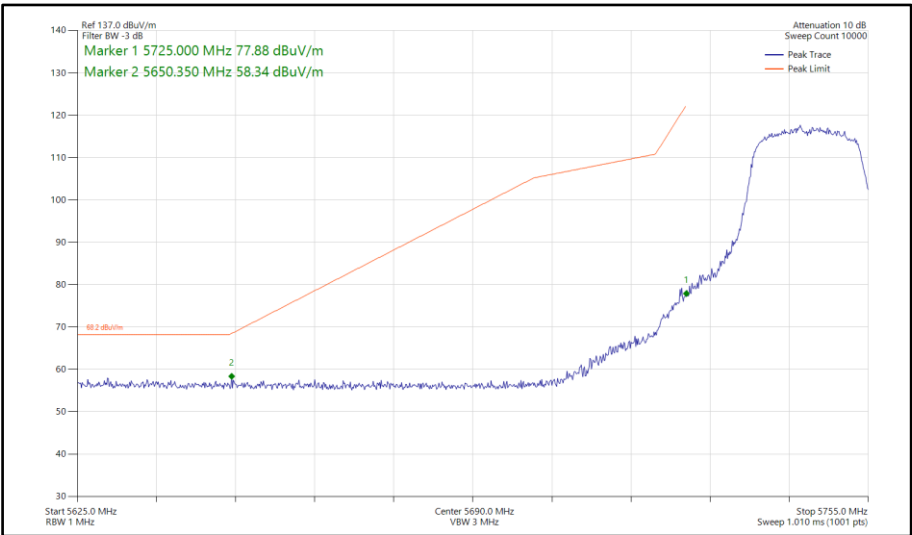
Figure 57 - 802.11a, SISO, Core 0 - 5745 MHz Band Edge Frequency 5725 MHz
