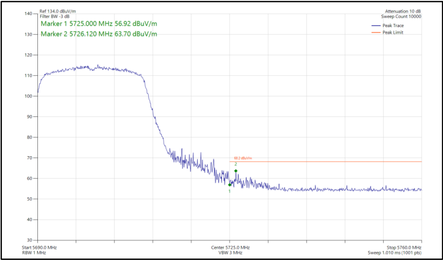
Figure 89 - 802.11ax HE20, SU, SISO, Core 1 - 5700 MHz Band Edge Frequency 5725 MHz
