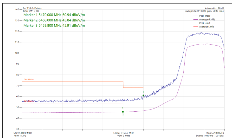
Figure 127 - 802.11n HT20, SDM, Core 0-1 - 5500 MHz Band Edge Frequency 5470 MHz
