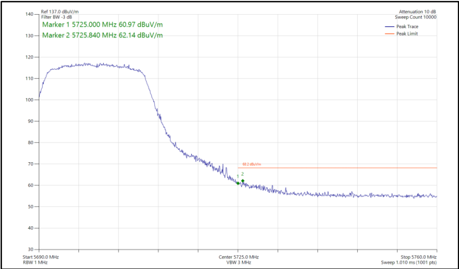
Figure 87 - 802.11a, SISO, Core 1 - 5700 MHz Band Edge Frequency 5725 MHz
