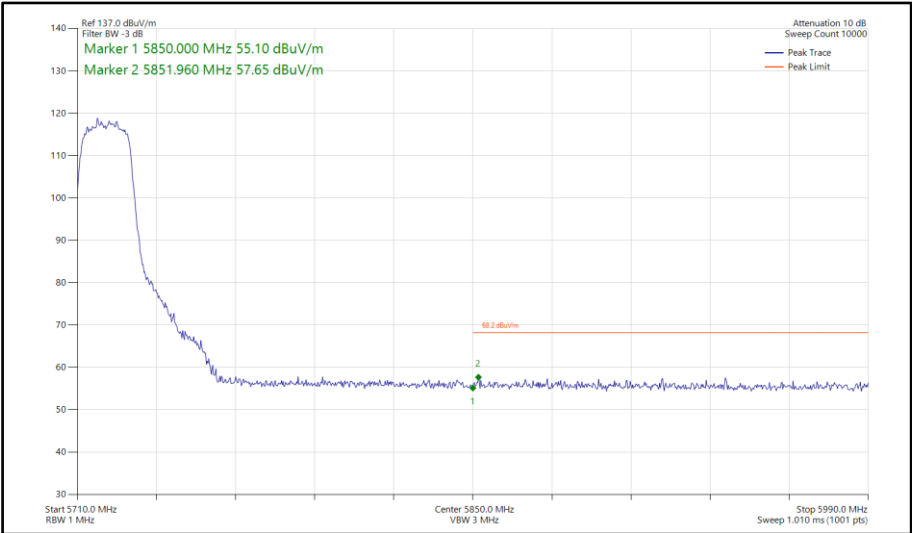
Figure 69 - 802.11n HT20, SISO, Core 0 - 5720 MHz Band Edge Frequency 5850 MHz
