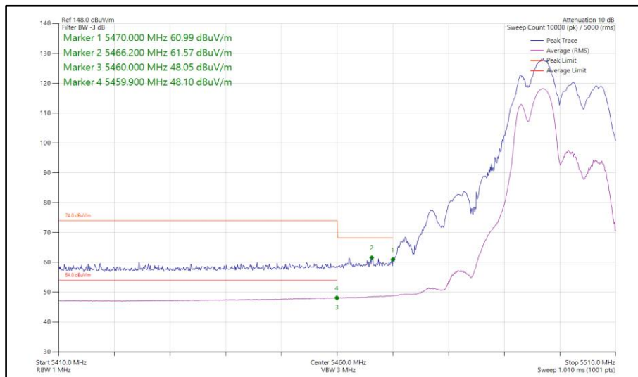
Figure 106 - 802.11be EHT20, RU 52+26-70, CDD, Core 0-1 - 5500 MHz Band Edge Frequency 5470 MHz
