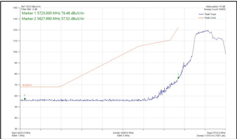
Figure 61 - 802.11be EHT20, RU 106+26-82, SISO, Core 0 - 5745 MHz Band Edge Frequency 5725 MHz
