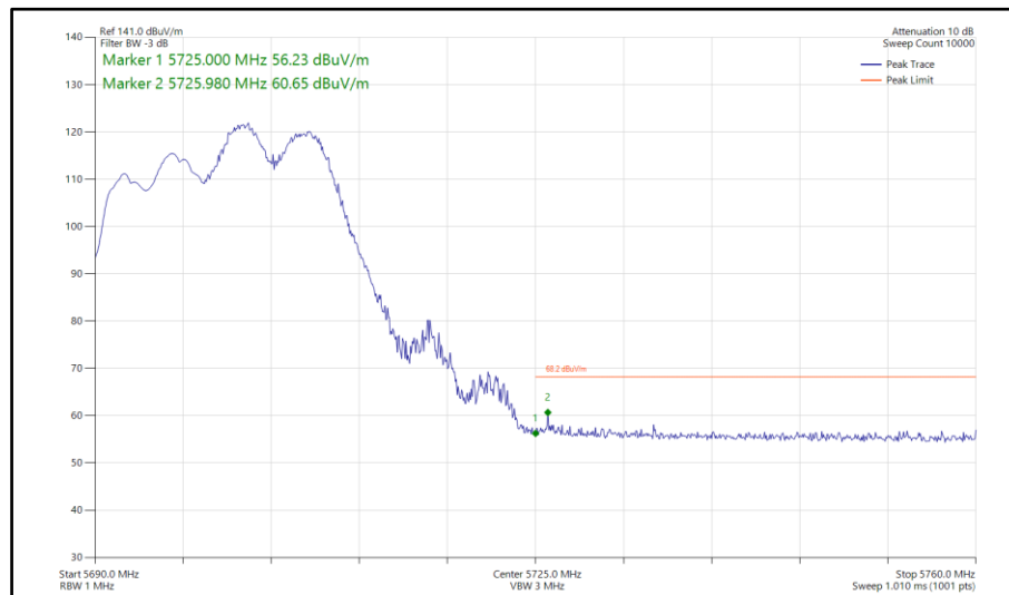
Figure 116 - 802.11be EHT20, RU 106+26-83, CDD, Core 0-1 - 5700 MHz Band Edge Frequency 5725 MHz
