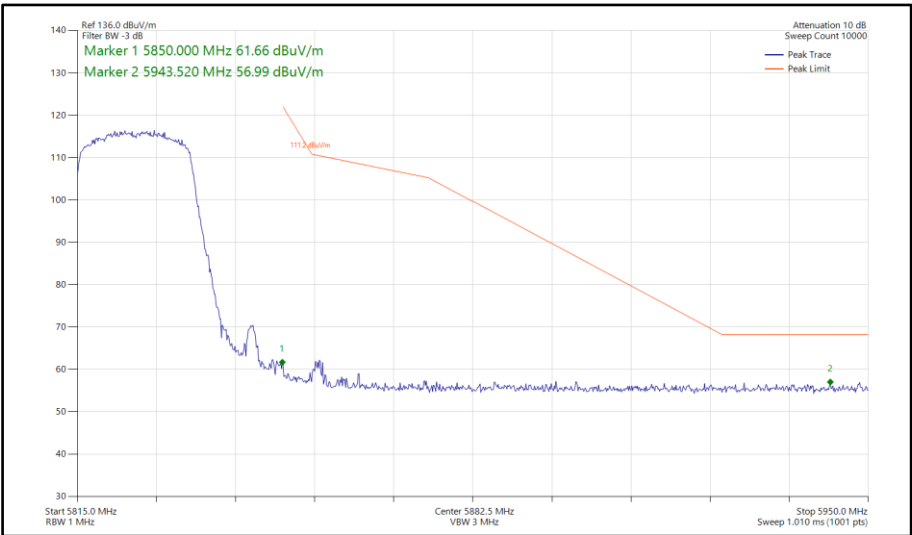
Figure 98 - 802.11ax HE20, SU, SISO, Core 1 - 5825 MHz Band Edge Frequency 5850 MHz
