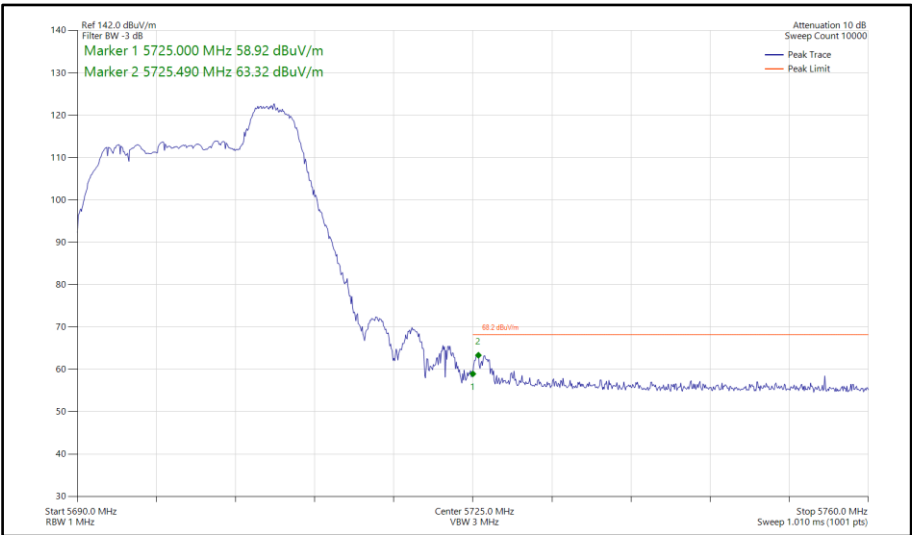
Figure 90 - 802.11ax HE20, RU 52-40, SISO, Core 1 - 5700 MHz Band Edge Frequency 5725 MHz
