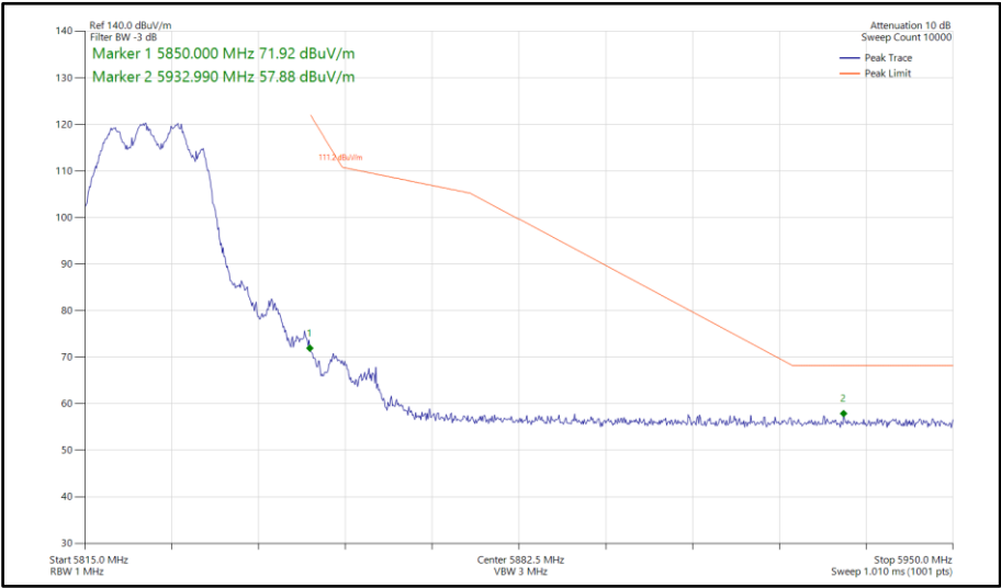
Figure 120 - 802.11n HT20, CDD, Core 0-1 - 5825 MHz Band Edge Frequency 5850 MHz
