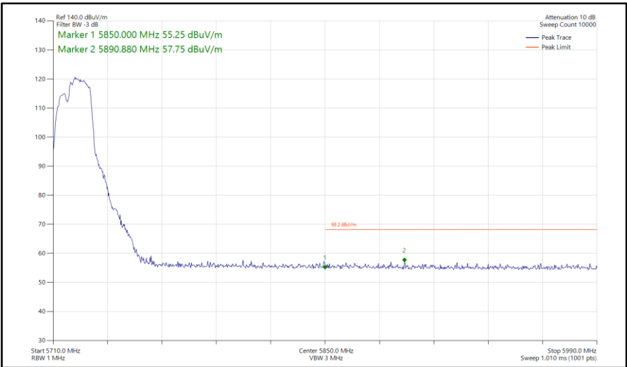
Figure 75 - 802.11be EHT20, RU 106+26-83, SISO, Core 0 - 5720 MHz Band Edge Frequency 5850 MHz
