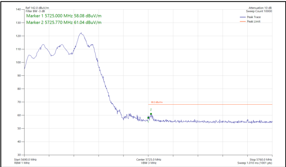
Figure 115 - 802.11ax HE20, RU 52-40, CDD, Core 0-1 - 5700 MHz Band Edge Frequency 5725 MHz
