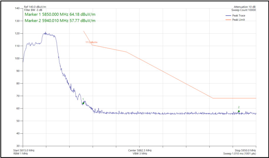
Figure 99 - 802.11ax HE20, RU 106-54, SISO, Core 1 - 5825 MHz Band Edge Frequency 5850 MHz
