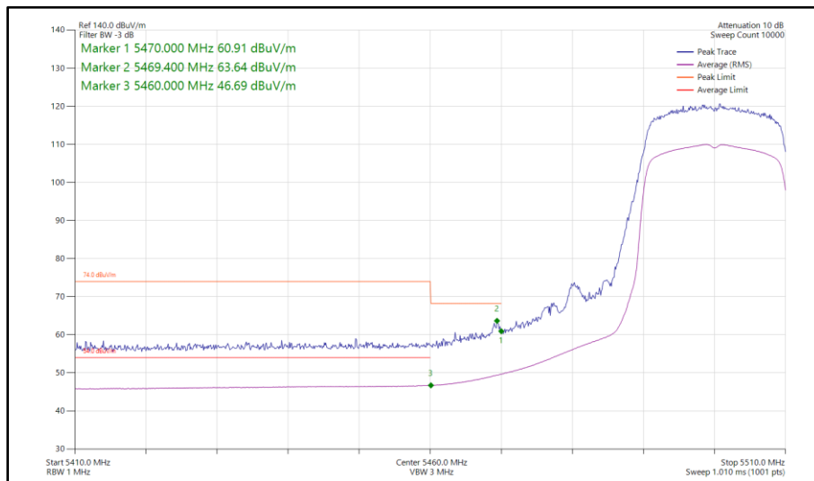
Figure 79 - 802.11ax HE20, SU, SISO, Core 1 - 5500 MHz Band Edge Frequency 5470 MHz
