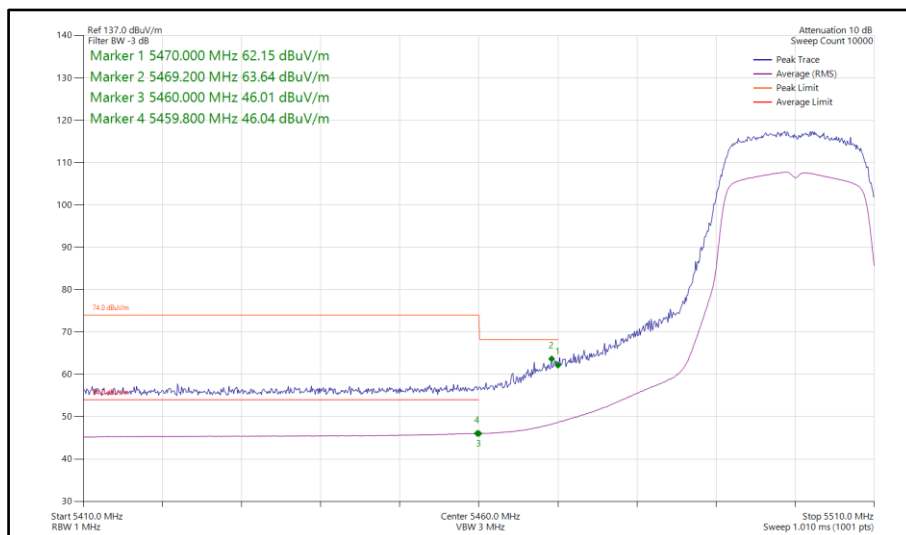
Figure 53 - 802.11n HT20, SISO, Core 0 - 5500 MHz Band Edge Frequency 5470 MHz
