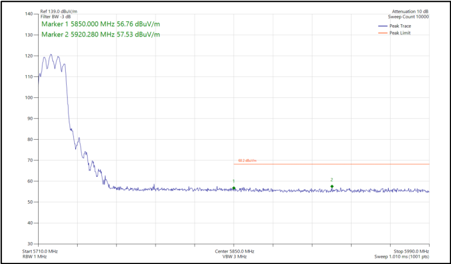
Figure 121 - 802.11ax HE20, SU, CDD, Core 0-1 - 5720 MHz Band Edge Frequency 5850 MHz
