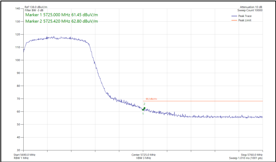
Figure 64 - 802.11ax HE20, SU, SISO, Core 0 - 5700 MHz Band Edge Frequency 5725 MHz
