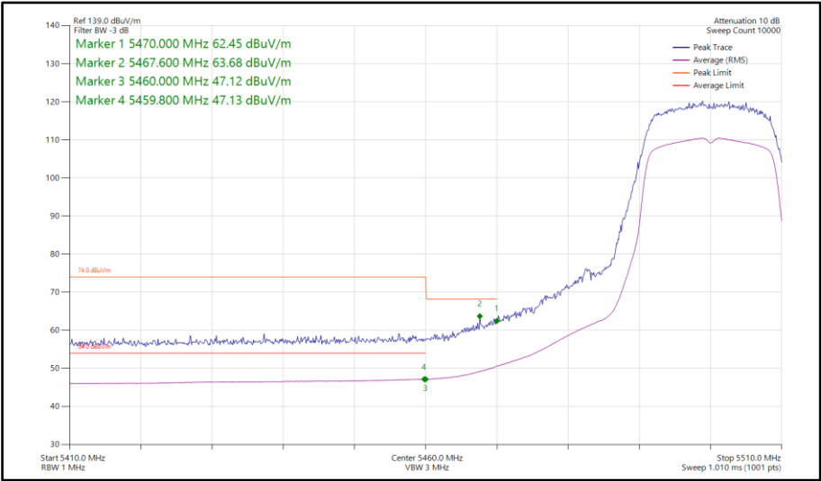
Figure 78 - 802.11n HT20, SISO, Core 1 - 5500 MHz Band Edge Frequency 5470 MHz
