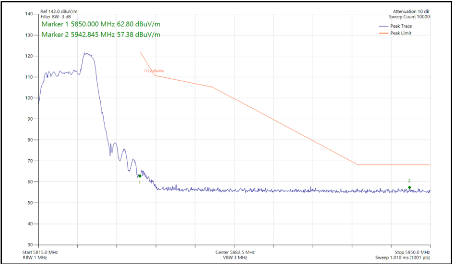
Figure 74 - 802.11ax HE20, RU 52-40, SISO, Core 0 - 5825 MHz Band Edge Frequency 5850 MHz
