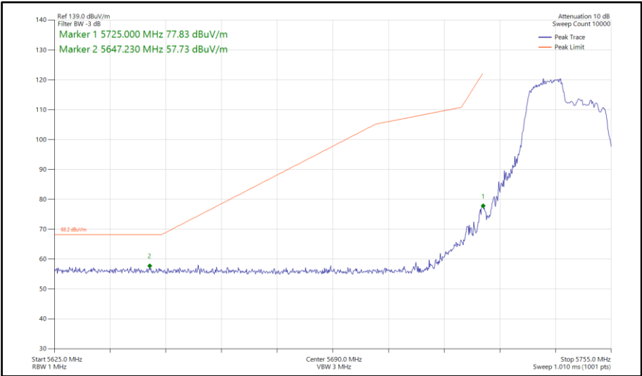
Figure 60 - 802.11ax HE20, RU 106-53, SISO, Core 0 - 5745 MHz Band Edge Frequency 5725 MHz
