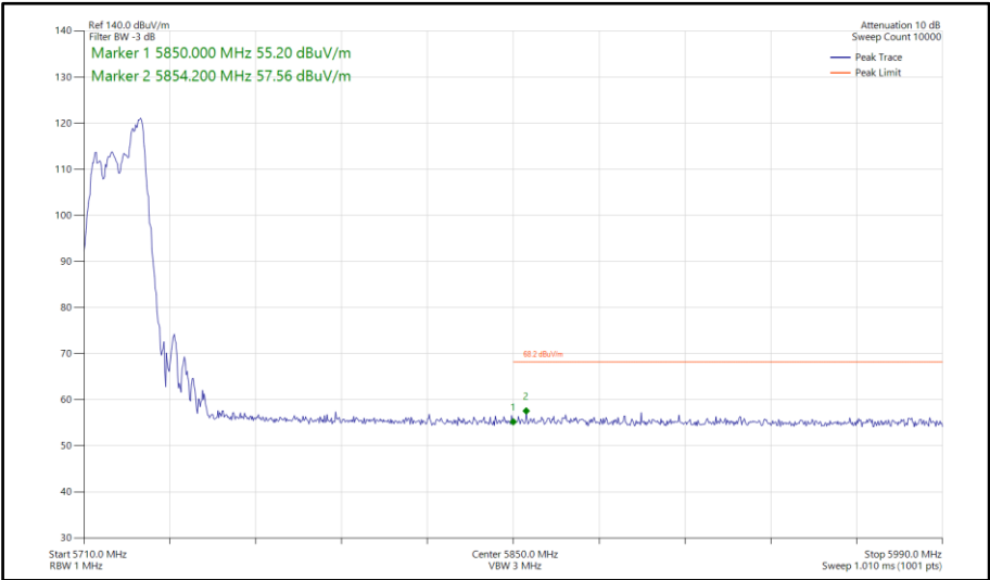
Figure 122 - 802.11ax HE20, RU 52-40, CDD, Core 0-1 - 5720 MHz Band Edge Frequency 5850 MHz
