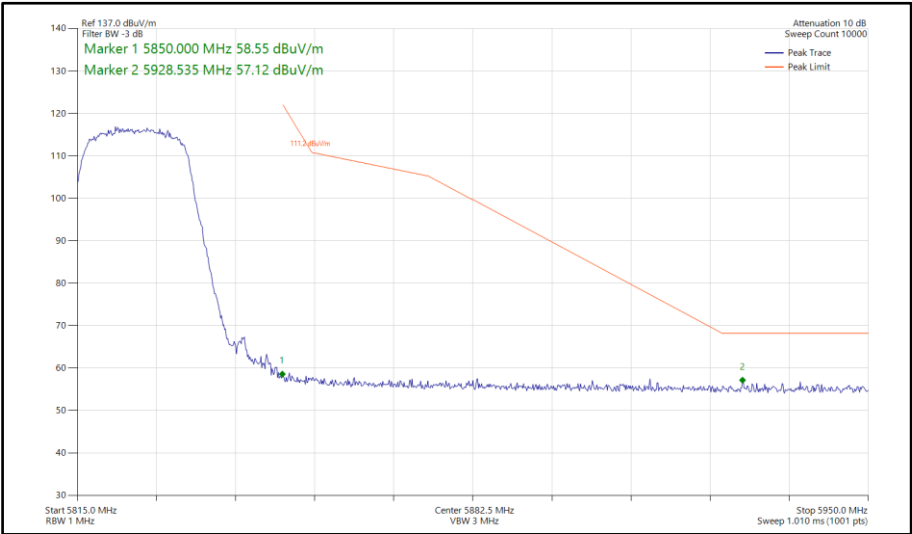
Figure 93 - 802.11a, SISO, Core 1 - 5825 MHz Band Edge Frequency 5850 MHz
