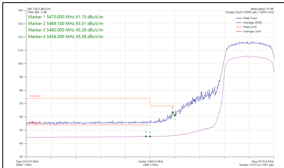
Figure 54 - 802.11ax HE20, SU, SISO, Core 0 - 5500 MHz Band Edge Frequency 5470 MHz
