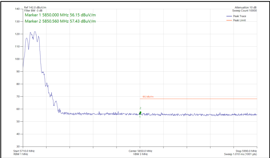
Figure 125 - 802.11be EHT20, RU 106+26-83, CDD, Core 0-1 - 5720 MHz Band Edge Frequency 5850 MHz
