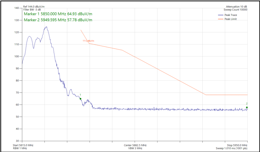
Figure 126 - 802.11be EHT20, RU 52+26-72, CDD, Core 0-1 - 5825 MHz Band Edge Frequency 5850 MHz
