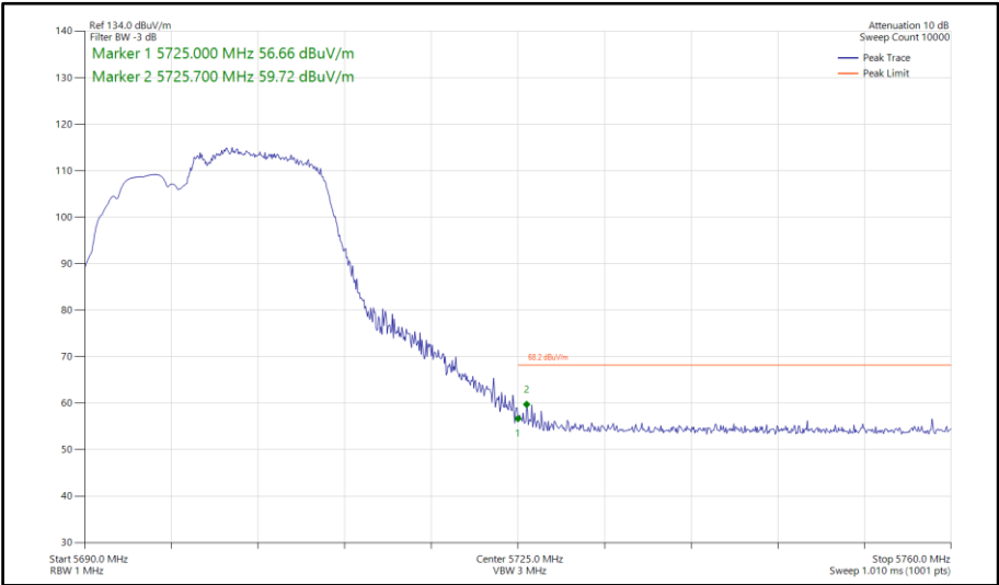
Figure 66 - 802.11be EHT20, RU 106+26-83, SISO, Core 0 - 5700 MHz Band Edge Frequency 5725 MHz
