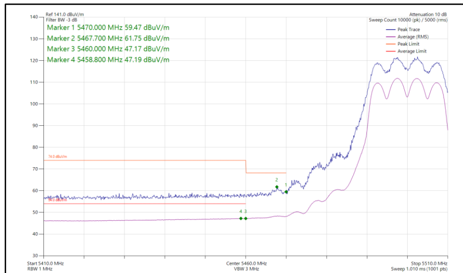
Figure 102 - 802.11a, CDD, Core 0-1 - 5500 MHz Band Edge Frequency 5470 MHz
