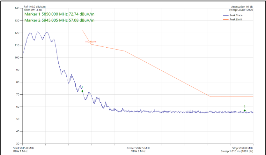
Figure 118 - 802.11a, CDD, Core 0-1 - 5825 MHz Band Edge Frequency 5850 MHz
