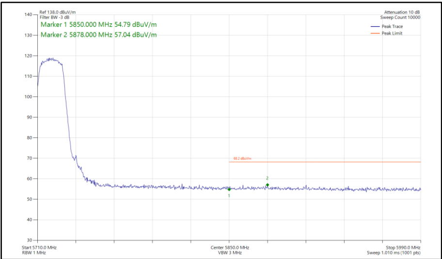
Figure 92 - 802.11a, SISO, Core 1 - 5720 MHz Band Edge Frequency 5850 MHz
