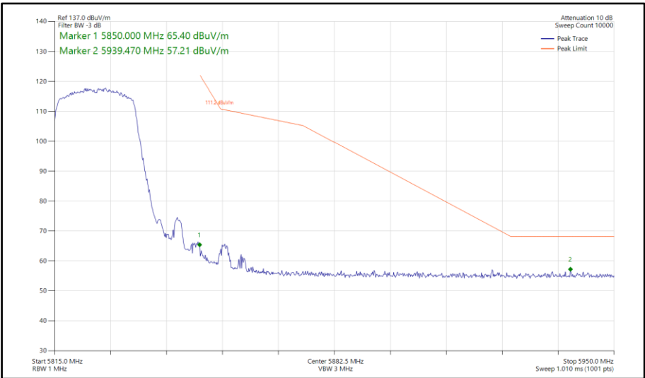
Figure 73 - 802.11ax HE20, SU, SISO, Core 0 - 5825 MHz Band Edge Frequency 5850 MHz
