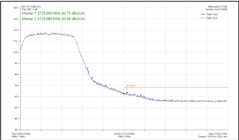
Figure 63 - 802.11n HT20, SISO, Core 0 - 5700 MHz Band Edge Frequency 5725 MHz
