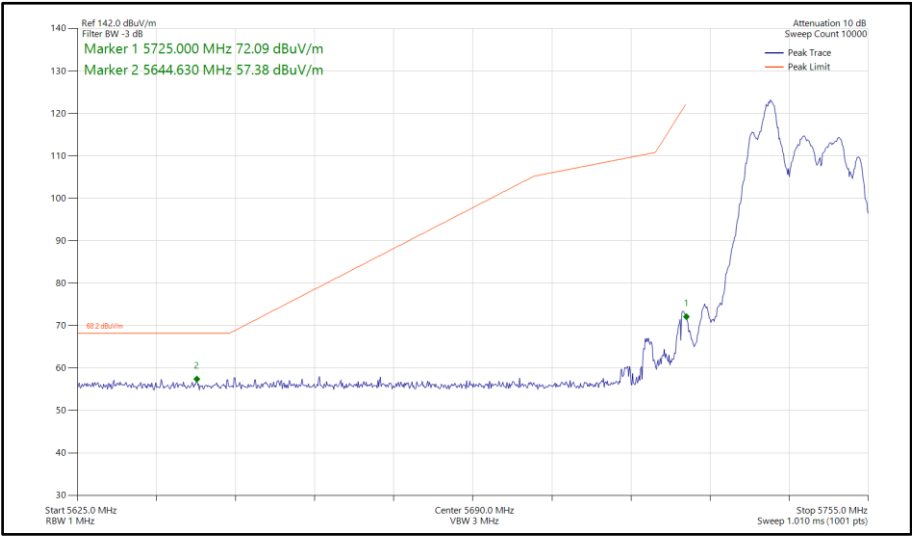
Figure 110 - 802.11ax HE20, RU 52-37, CDD, Core 0-1 - 5745 MHz Band Edge Frequency 5725 MHz
