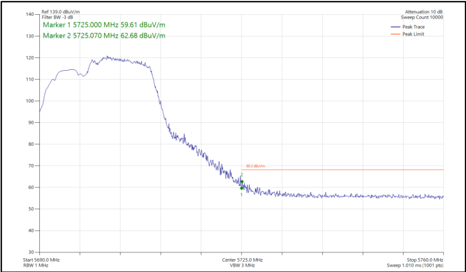
Figure 91 - 802.11be EHT20, RU 106+26-83, SISO, Core 1 - 5700 MHz Band Edge Frequency 5725 MHz
