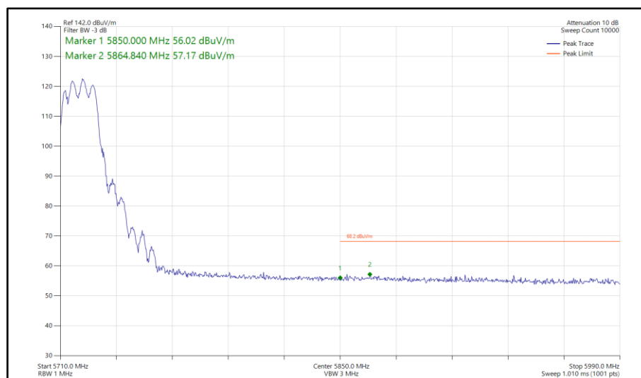
Figure 117 - 802.11a, CDD, Core 0-1 - 5720 MHz Band Edge Frequency 5850 MHz
