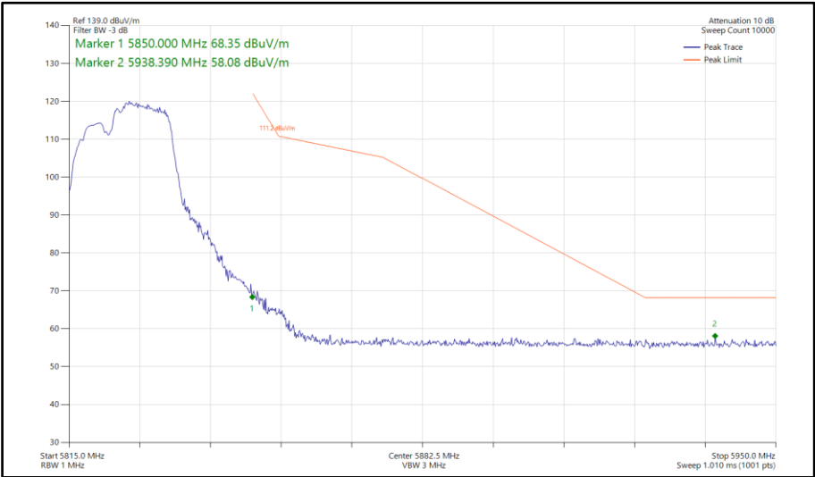
Figure 101 - 802.11be EHT20, RU 106+26-83, SISO, Core 1 - 5825 MHz Band Edge Frequency 5850 MHz
