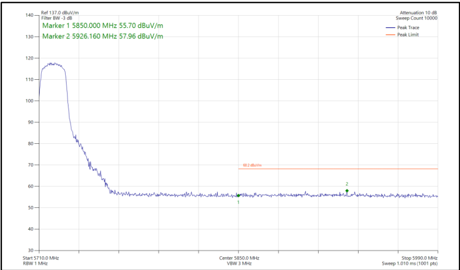
Figure 67 - 802.11a, SISO, Core 0 - 5720 MHz Band Edge Frequency 5850 MHz
