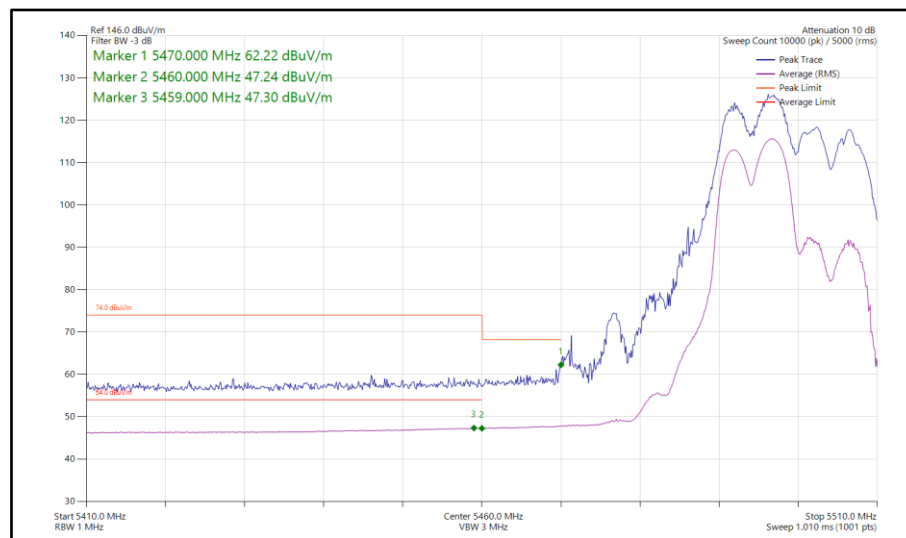
Figure 105 - 802.11ax HE20, RU 106-53, CDD, Core 0-1 - 5500 MHz Band Edge Frequency 5470 MHz
