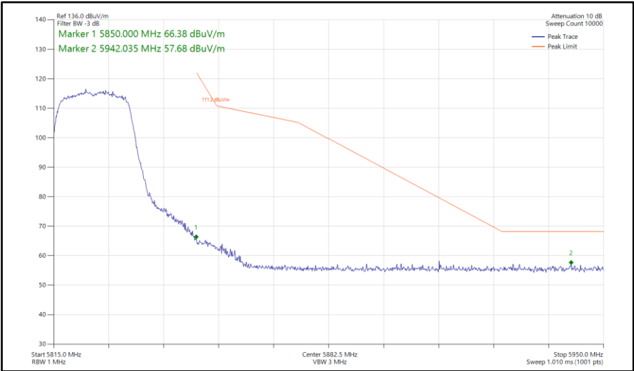
Figure 95 - 802.11n HT20, SISO, Core 1 - 5825 MHz Band Edge Frequency 5850 MHz
