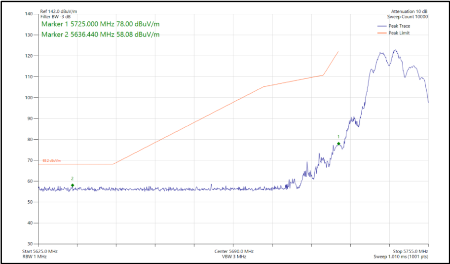
Figure 111 - 802.11be EHT20, RU 106+26-82, CDD, Core 0-1 - 5745 MHz Band Edge Frequency 5725 MHz
