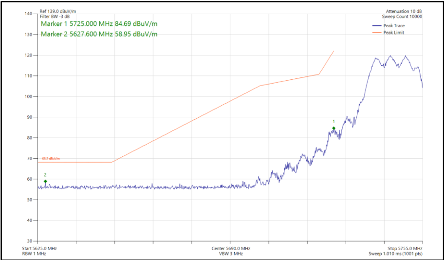
Figure 108 - 802.11n HT20, CDD, Core 0-1 - 5745 MHz Band Edge Frequency 5725 MHz
