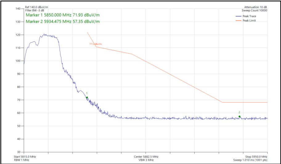
Figure 76 - 802.11be EHT20, RU 106+26-83, SISO, Core 0 - 5825 MHz Band Edge Frequency 5850 MHz
