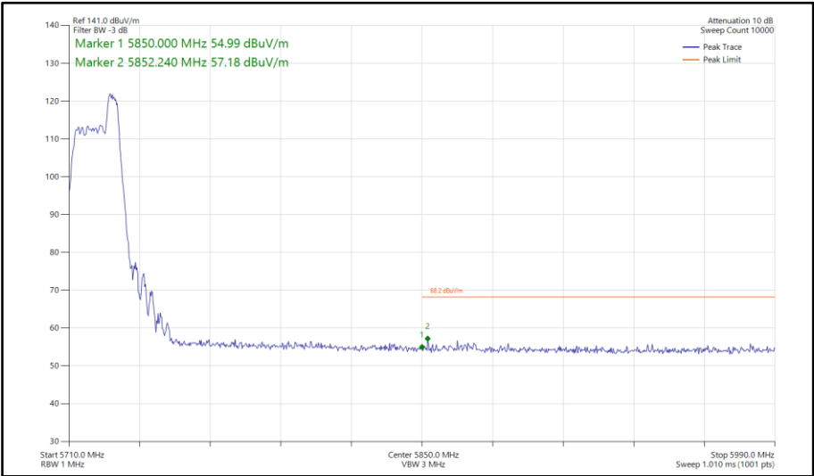
Figure 97 - 802.11ax HE20, RU 52-40, SISO, Core 1 - 5720 MHz Band Edge Frequency 5850 MHz
