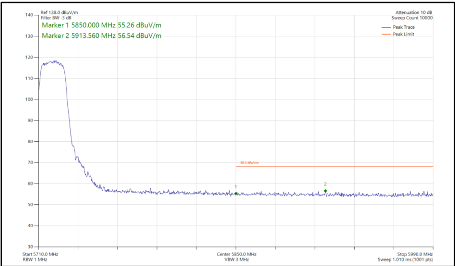
Figure 94 - 802.11n HT20, SISO, Core 1 - 5720 MHz Band Edge Frequency 5850 MHz
