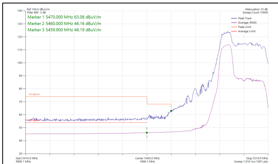
Figure 80 - 802.11ax HE20, RU 52-37, SISO, Core 1 - 5500 MHz Band Edge Frequency 5470 MHz
