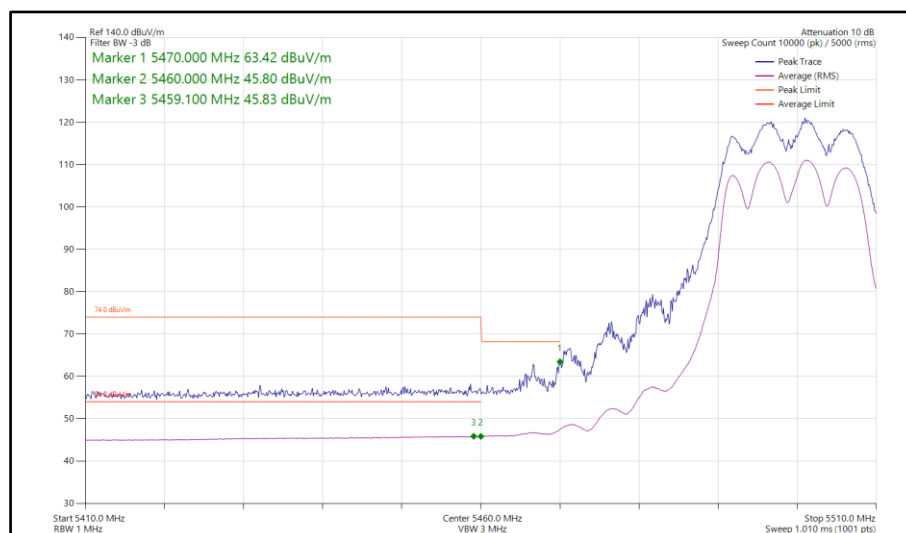
Figure 103 - 802.11n HT20, CDD, Core 0-1 - 5500 MHz Band Edge Frequency 5470 MHz
