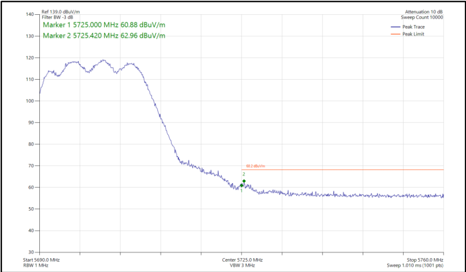
Figure 113 - 802.11n HT20, CDD, Core 0-1 - 5700 MHz Band Edge Frequency 5725 MHz
