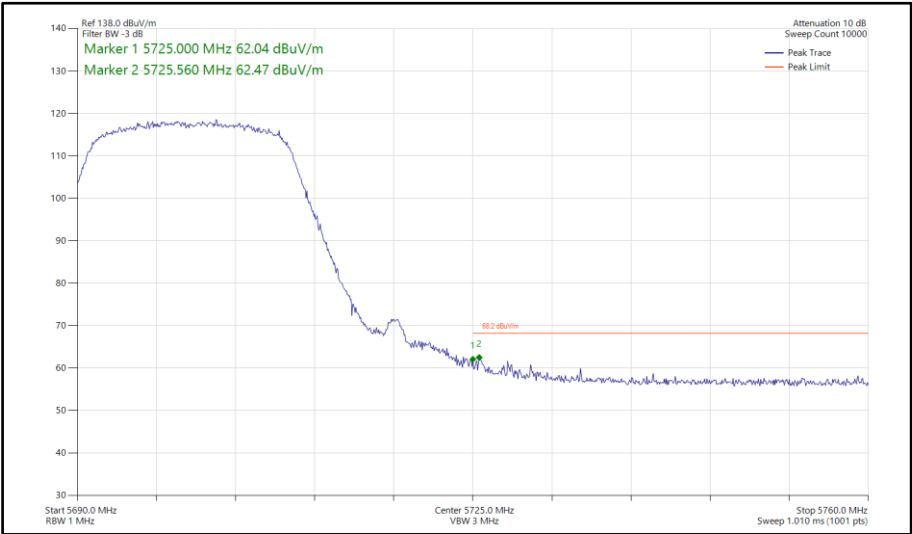
Figure 62 - 802.11a, SISO, Core 0 - 5700 MHz Band Edge Frequency 5725 MHz
