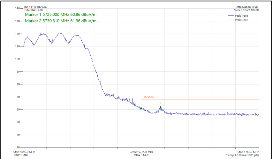
Figure 114 - 802.11ax HE20, SU, CDD, Core 0-1 - 5700 MHz Band Edge Frequency 5725 MHz
