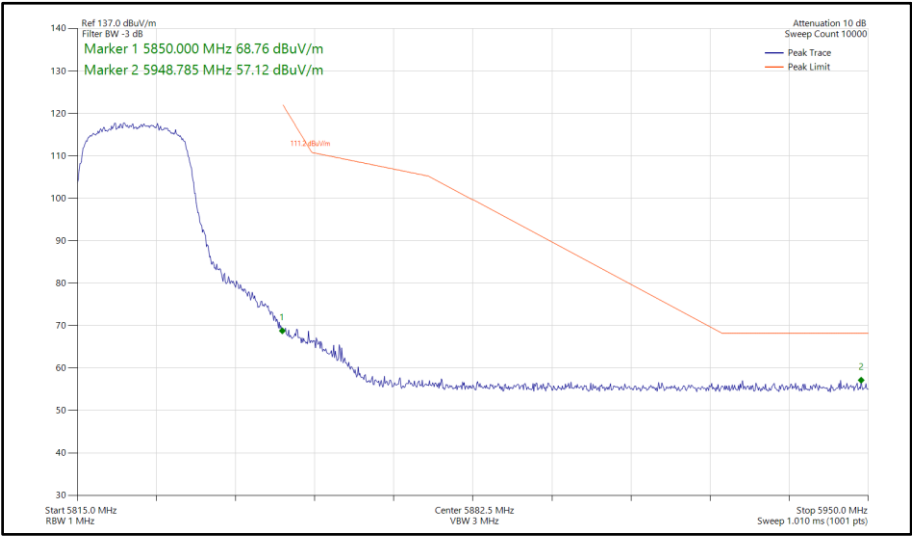
Figure 70 - 802.11n HT20, SISO, Core 0 - 5825 MHz Band Edge Frequency 5850 MHz
