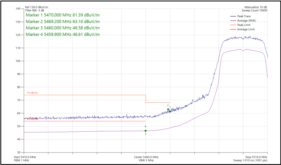
Figure 77 - 802.11a, SISO, Core 1 - 5500 MHz Band Edge Frequency 5470 MHz
