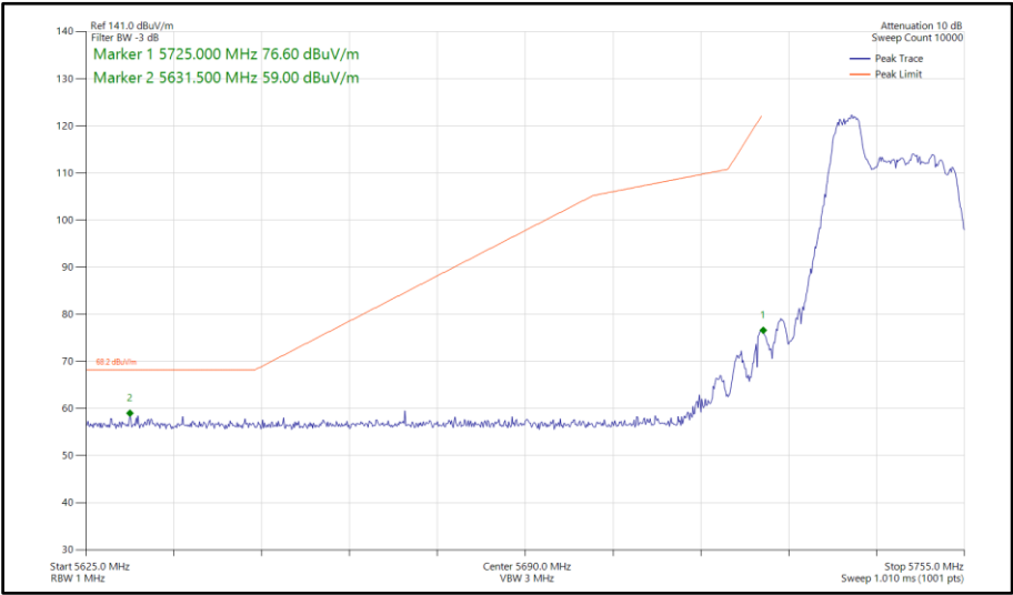
Figure 85 - 802.11ax HE20, RU 52-37, SISO, Core 1 - 5745 MHz Band Edge Frequency 5725 MHz
