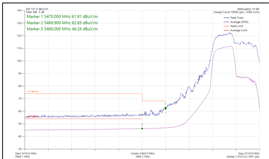
Figure 55 - 802.11ax HE20, RU 106-53, SISO, Core 0 - 5500 MHz Band Edge Frequency 5470 MHz
