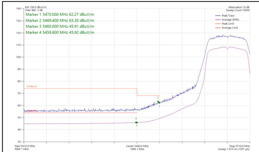
Figure 52 - 802.11a, SISO, Core 0 - 5500 MHz Band Edge Frequency 5470 MHz
