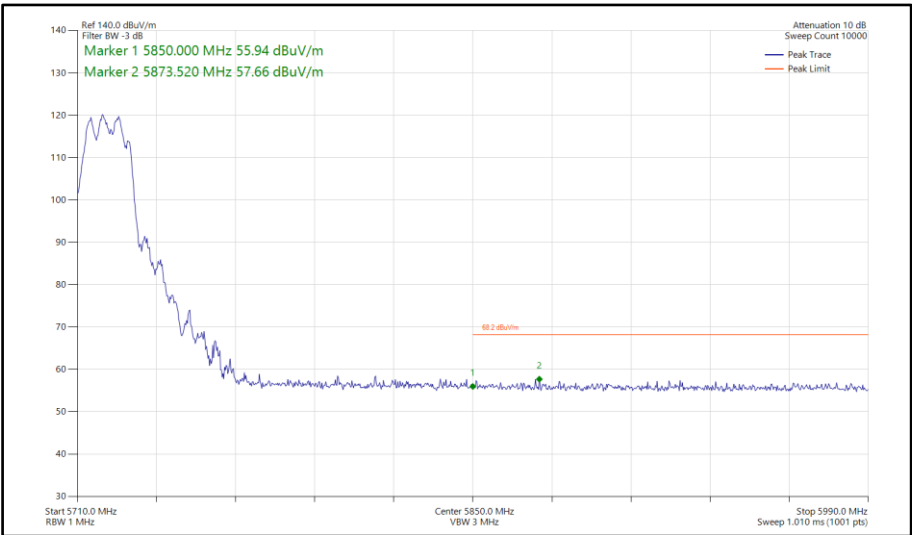
Figure 119 - 802.11n HT20, CDD, Core 0-1 - 5720 MHz Band Edge Frequency 5850 MHz
