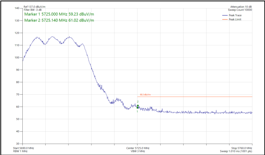
Figure 112 - 802.11a, CDD, Core 0-1 - 5700 MHz Band Edge Frequency 5725 MHz
