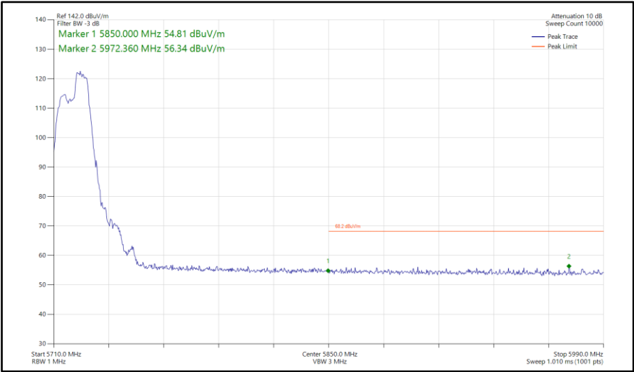
Figure 100 - 802.11be EHT20, RU 52+26-72, SISO, Core 1 - 5720 MHz Band Edge Frequency 5850 MHz
