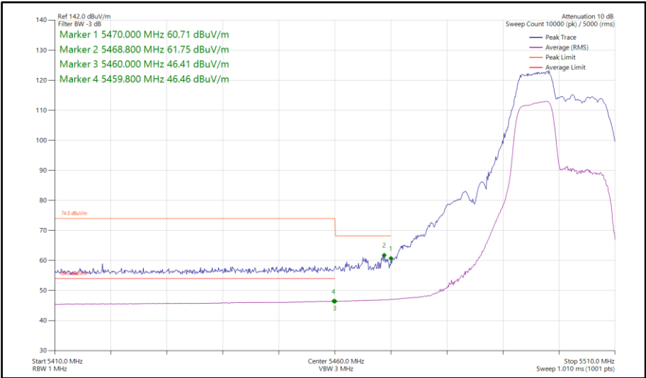
Figure 56 - 802.11be EHT20, RU 52+26-70, SISO, Core 0 - 5500 MHz Band Edge Frequency 5470 MHz
