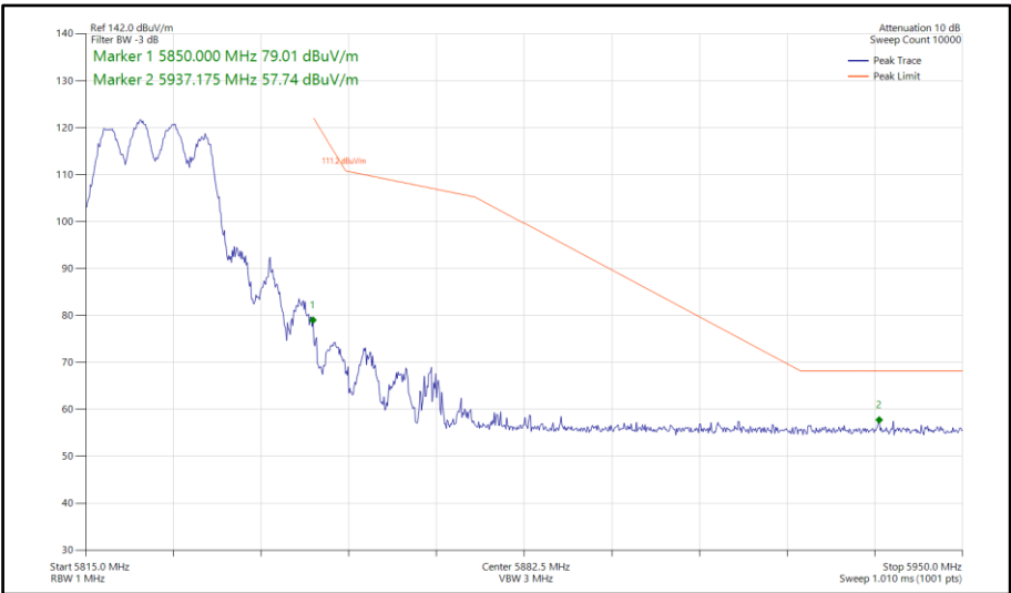
Figure 123 - 802.11ax HE20, SU, CDD, Core 0-1 - 5825 MHz Band Edge Frequency 5850 MHz
