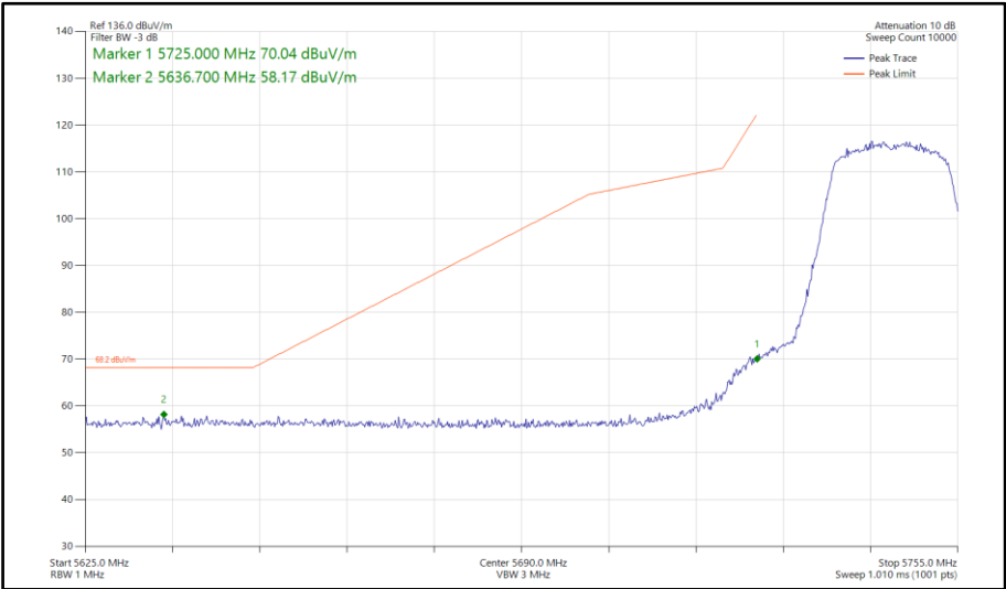
Figure 58 - 802.11n HT20, SISO, Core 0 - 5745 MHz Band Edge Frequency 5725 MHz
