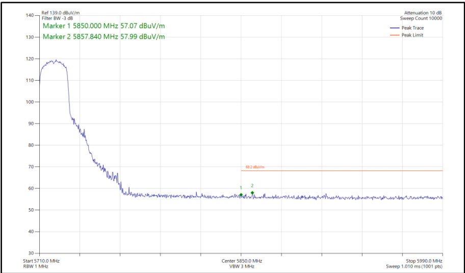
Figure 71 - 802.11ax HE20, SU, SISO, Core 0 - 5720 MHz Band Edge Frequency 5850 MHz
