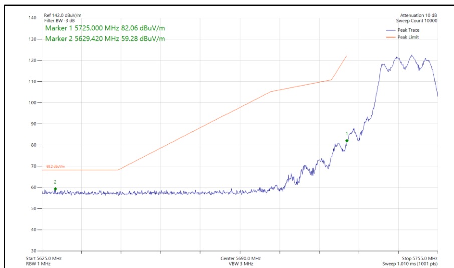
Figure 107 - 802.11a, CDD, Core 0-1 - 5745 MHz Band Edge Frequency 5725 MHz
