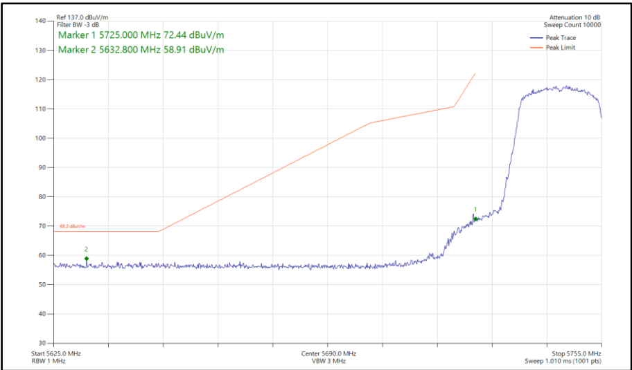
Figure 59 - 802.11ax HE20, SU, SISO, Core 0 - 5745 MHz Band Edge Frequency 5725 MHz
