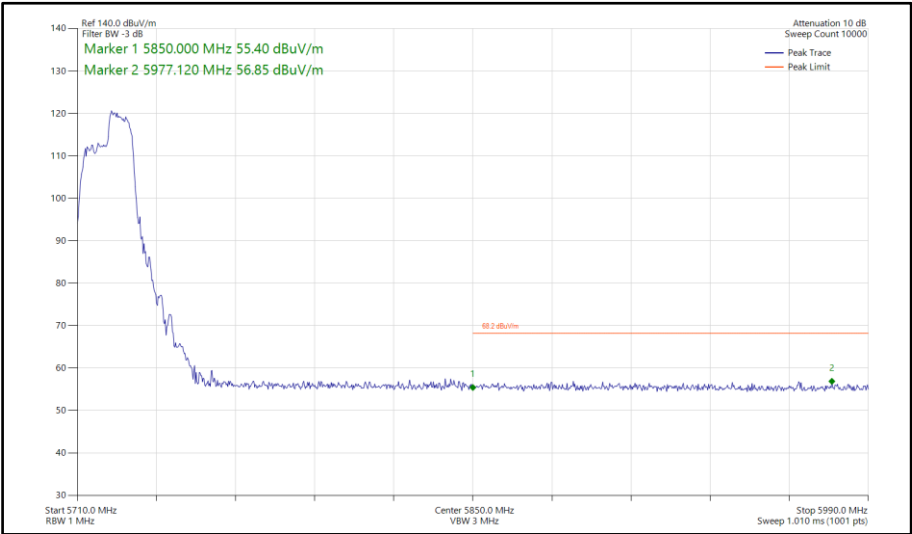
Figure 72 - 802.11ax HE20, RU 106-54, SISO, Core 0 - 5720 MHz Band Edge Frequency 5850 MHz
