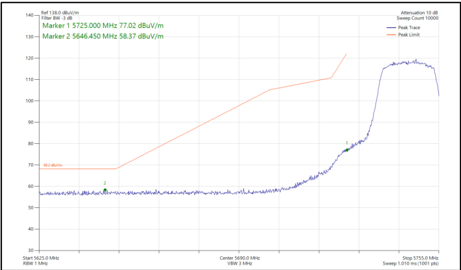
Figure 82 - 802.11a, SISO, Core 1 - 5745 MHz Band Edge Frequency 5725 MHz
