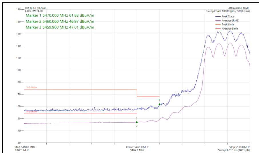
Figure 104 - 802.11ax HE20, SU, CDD, Core 0-1 - 5500 MHz Band Edge Frequency 5470 MHz
