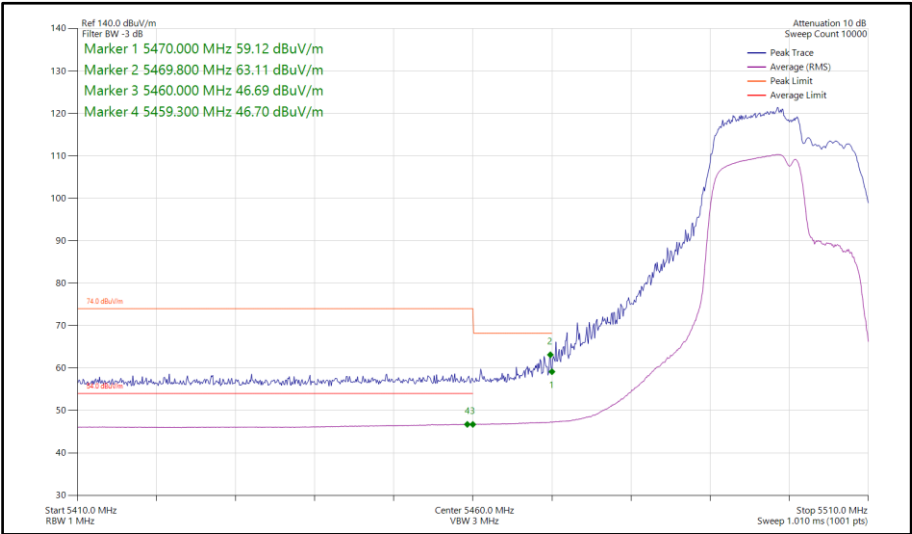
Figure 81 - 802.11be EHT20, RU 106+26-82, SISO, Core 1 - 5500 MHz Band Edge Frequency 5470 MHz
