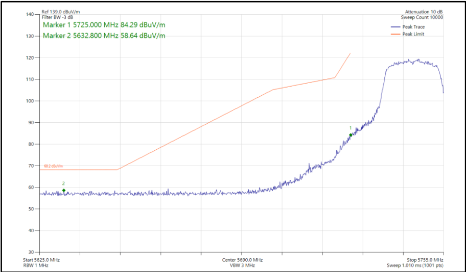
Figure 83 - 802.11n HT20, SISO, Core 1 - 5745 MHz Band Edge Frequency 5725 MHz
