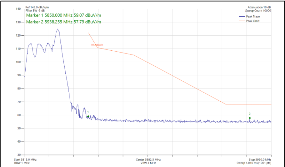
Figure 124 - 802.11ax HE20, RU 26-8, CDD, Core 0-1 - 5825 MHz Band Edge Frequency 5850 MHz
