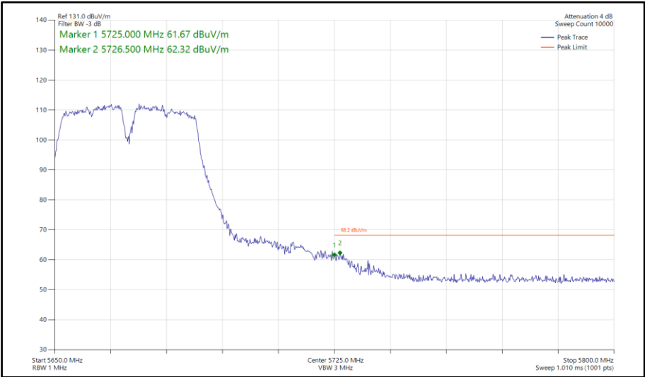
Figure 167 - 802.11a a40, SISO, Core 0 - 5670 MHz Band Edge Frequency 5725 MHz
