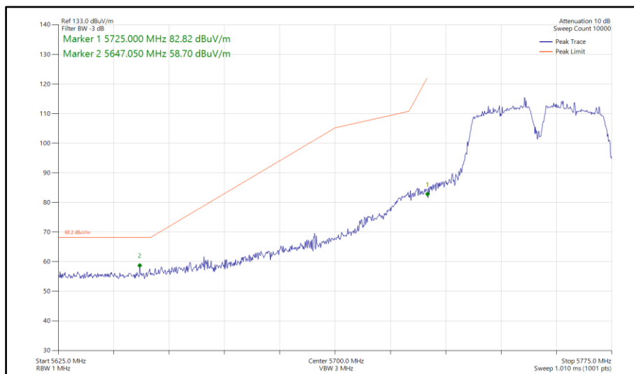
Figure 162 - 802.11a a40, SISO, Core 0 - 5755 MHz Band Edge Frequency 5725 MHz
