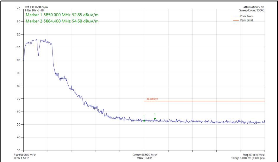
Figure 197 - 802.11a a40, SISO, Core 1 - 5710 MHz Band Edge Frequency 5850 MHz
