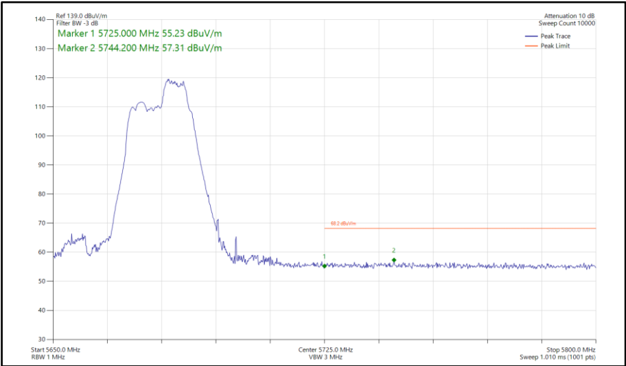
Figure 171 - 802.11be EHT40, RU 52+26-75, SISO, Core 0 - 5670 MHz Band Edge Frequency 5725 MHz
