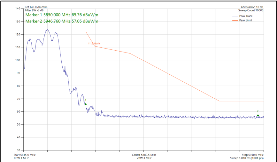
Figure 144 - 802.11ax HE20, RU 106-54, SDM, Core 0-1 - 5825 MHz Band Edge Frequency 5850 MHz
