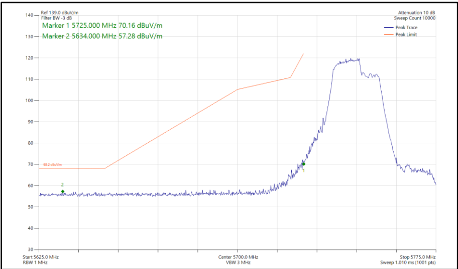
Figure 191 - 802.11be EHT40, RU 106+26-82, SISO, Core 1 - 5755 MHz Band Edge Frequency 5725 MHz
