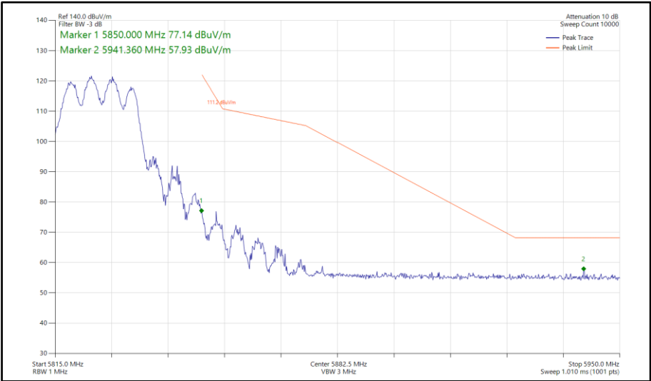
Figure 156 - 802.11ax HE20, SU, TxBF, Core 0-1 - 5825 MHz Band Edge Frequency 5850 MHz
