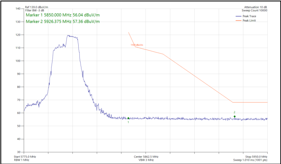
Figure 179 - 802.11ax HE40, RU 106-56, SISO, Core 0 - 5795 MHz Band Edge Frequency 5850 MHz
