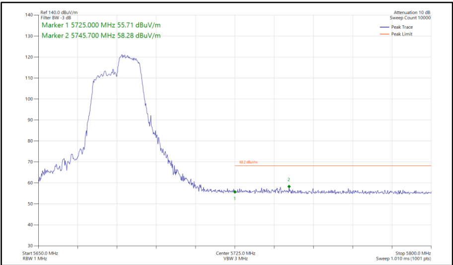
Figure 170 - 802.11ax HE40, RU 106-56, SISO, Core 0 - 5670 MHz Band Edge Frequency 5725 MHz
