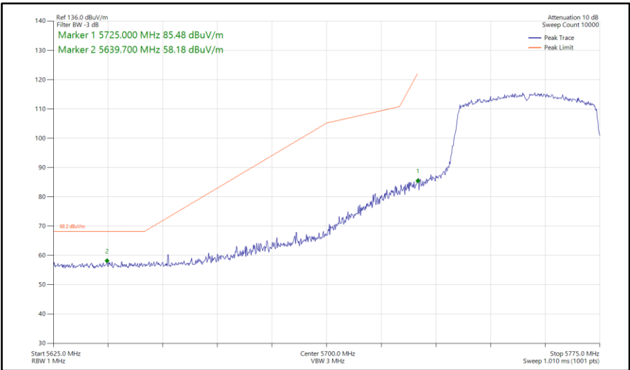
Figure 164 - 802.11ax HE40, SU, SISO, Core 0 - 5755 MHz Band Edge Frequency 5725 MHz
