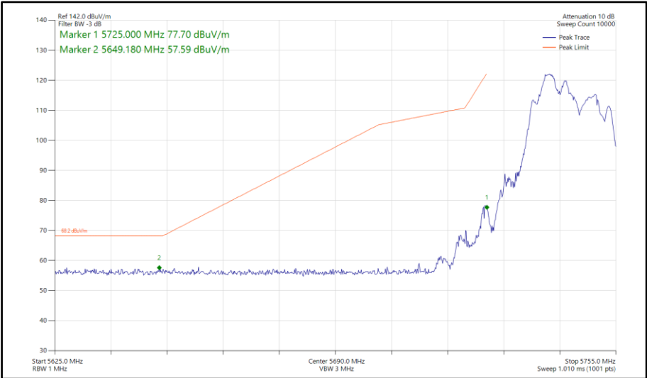
Figure 133 - 802.11ax HE20, RU 106-53, SDM, Core 0-1 - 5745 MHz Band Edge Frequency 5725 MHz
