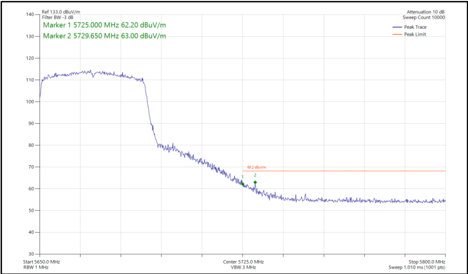
Figure 194 - 802.11ax HE40, SU, SISO, Core 1 - 5670 MHz Band Edge Frequency 5725 MHz
