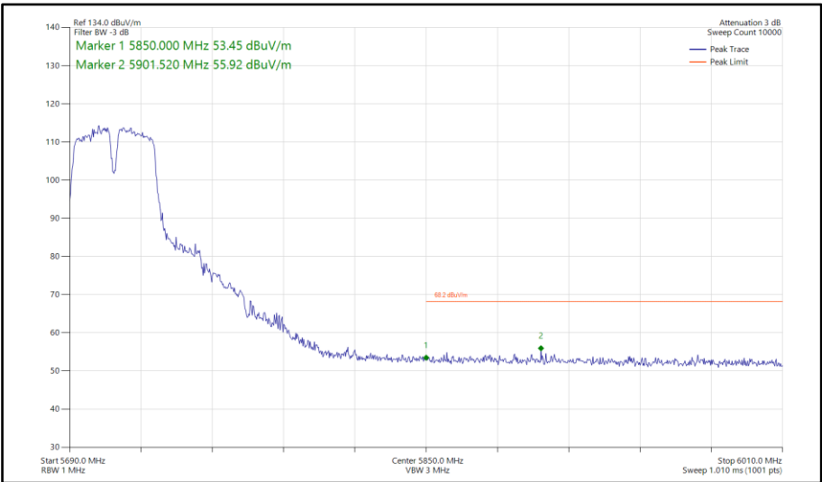
Figure 172 - 802.11a a40, SISO, Core 0 - 5710 MHz Band Edge Frequency 5850 MHz
