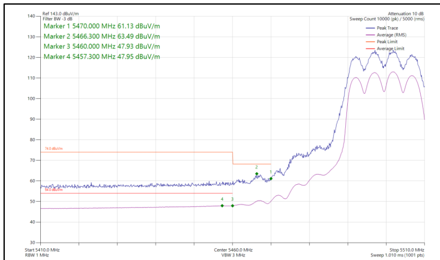
Figure 148 - 802.11ax HE20, SU, TxBF, Core 0-1 - 5500 MHz Band Edge Frequency 5470 MHz
