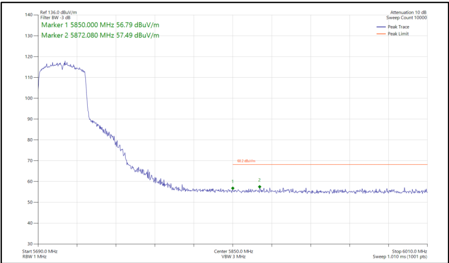
Figure 201 - 802.11ax HE40, SU, SISO, Core 1 - 5710 MHz Band Edge Frequency 5850 MHz
