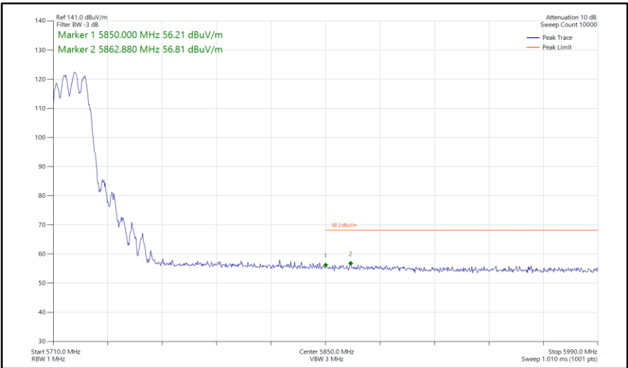
Figure 155 - 802.11ax HE20, SU, TxBF, Core 0-1 - 5720 MHz Band Edge Frequency 5850 MHz
