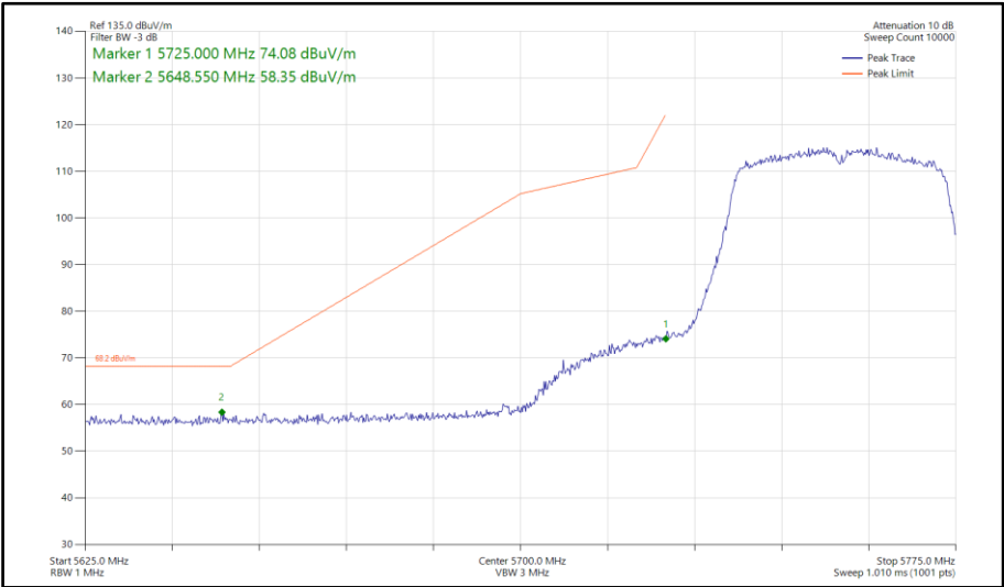
Figure 188 - 802.11n HT40, SISO, Core 1 - 5755 MHz Band Edge Frequency 5725 MHz
