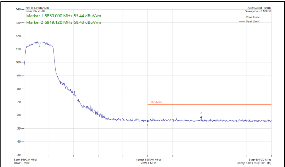
Figure 174 - 802.11n HT40, SISO, Core 0 - 5710 MHz Band Edge Frequency 5850 MHz
