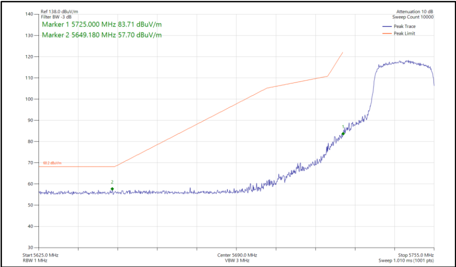
Figure 132 - 802.11ax HE20, SU, SDM, Core 0-1 - 5745 MHz Band Edge Frequency 5725 MHz
