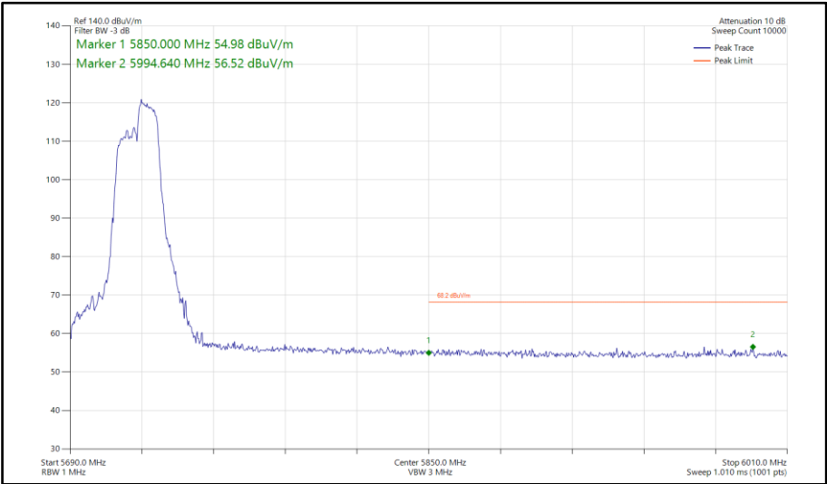
Figure 202 - 802.11ax HE40, RU 106-56, SISO, Core 1 - 5710 MHz Band Edge Frequency 5850 MHz
