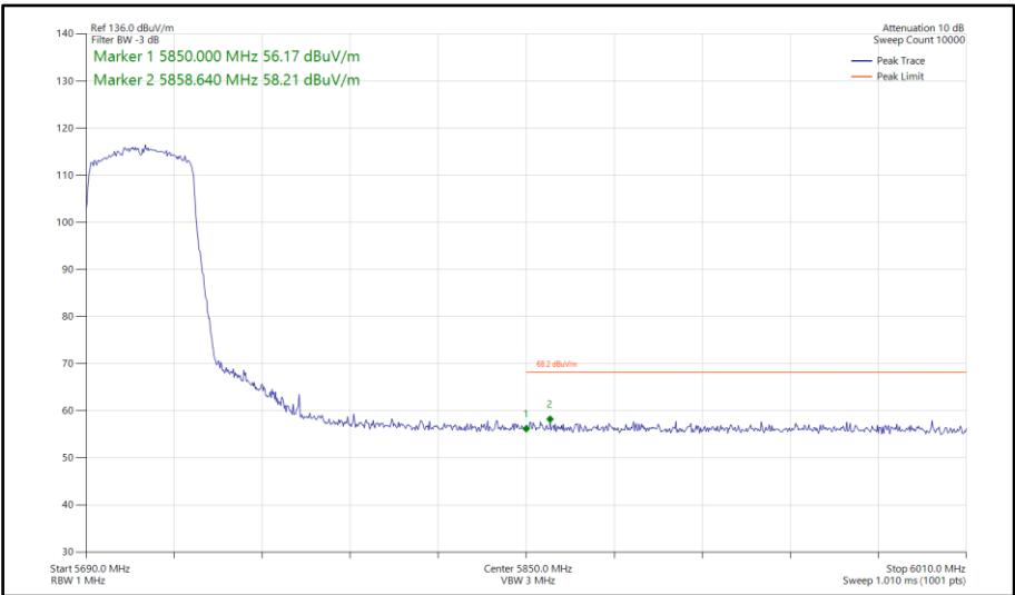
Figure 176 - 802.11ax HE40, SU, SISO, Core 0 - 5710 MHz Band Edge Frequency 5850 MHz
