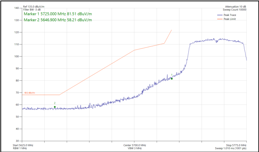
Figure 163 - 802.11n HT40, SISO, Core 0 - 5755 MHz Band Edge Frequency 5725 MHz
