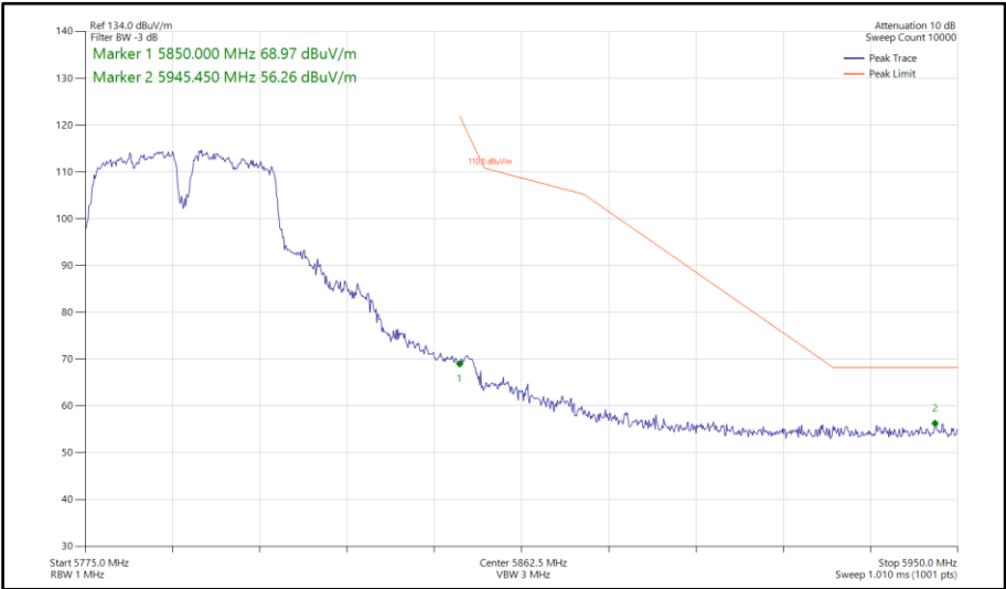
Figure 198 - 802.11a a40, SISO, Core 1 - 5795 MHz Band Edge Frequency 5850 MHz
