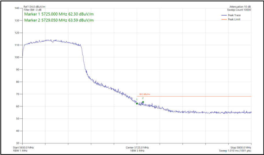
Figure 169 - 802.11ax HE40, SU, SISO, Core 0 - 5670 MHz Band Edge Frequency 5725 MHz
