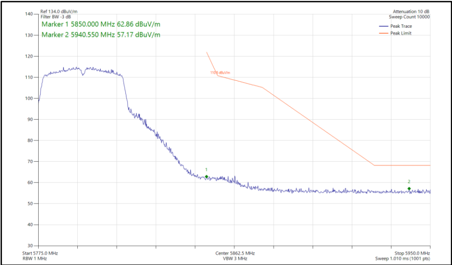
Figure 175 - 802.11n HT40, SISO, Core 0 - 5795 MHz Band Edge Frequency 5850 MHz
