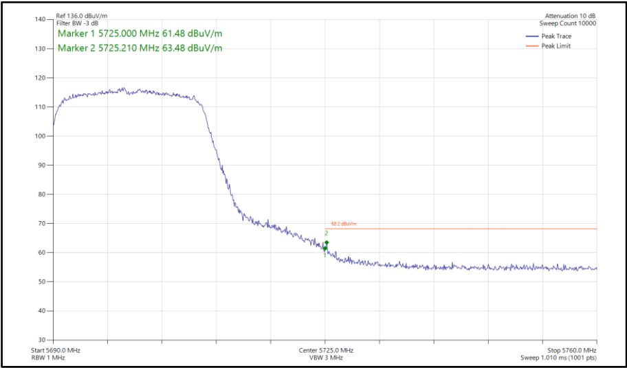
Figure 136 - 802.11ax HE20, SU, SDM, Core 0-1 - 5700 MHz Band Edge Frequency 5725 MHz
