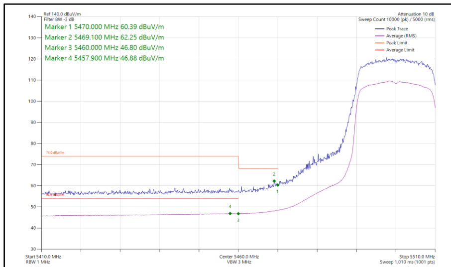
Figure 128 - 802.11ax HE20, SU, SDM, Core 0-1 - 5500 MHz Band Edge Frequency 5470 MHz
