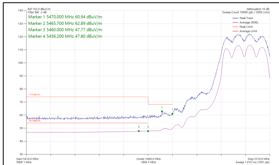
Figure 147 - 802.11ac VHT20, TxBF, Core 0-1 - 5500 MHz Band Edge Frequency 5470 MHz
