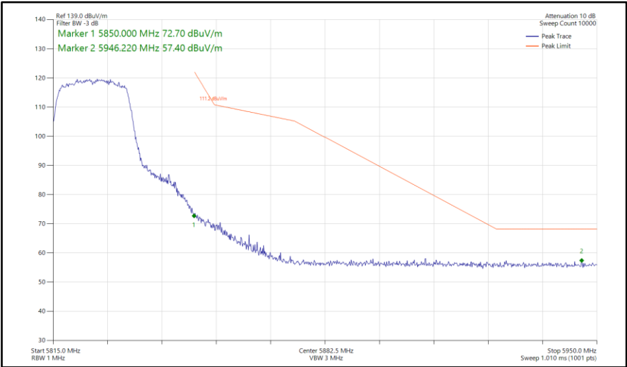
Figure 140 - 802.11n HT20, SDM, Core 0-1 - 5825 MHz Band Edge Frequency 5850 MHz
