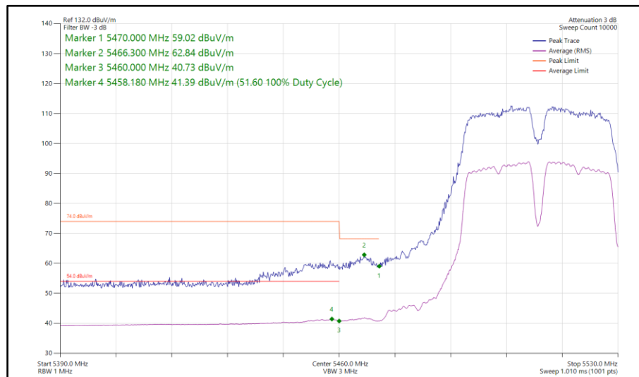
Figure 182 - 802.11a a40, SISO, Core 1 - 5510 MHz Band Edge Frequency 5470 MHz
