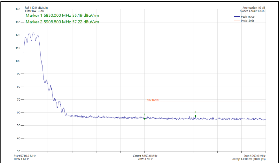
Figure 153 - 802.11ac VHT20, TxBF, Core 0-1 - 5720 MHz Band Edge Frequency 5850 MHz
