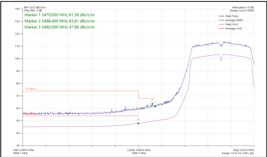
Figure 158 - 802.11n HT40, SISO, Core 0 - 5510 MHz Band Edge Frequency 5470 MHz
