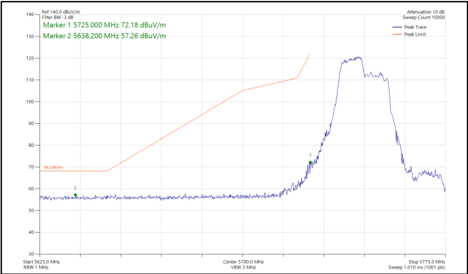
Figure 190 - 802.11ax HE40, RU 106-53, SISO, Core 1 - 5755 MHz Band Edge Frequency 5725 MHz
