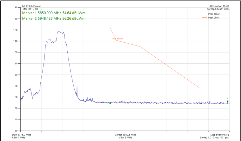
Figure 181 - 802.11be EHT40, RU 52+26-75, SISO, Core 0 - 5795 MHz Band Edge Frequency 5850 MHz
