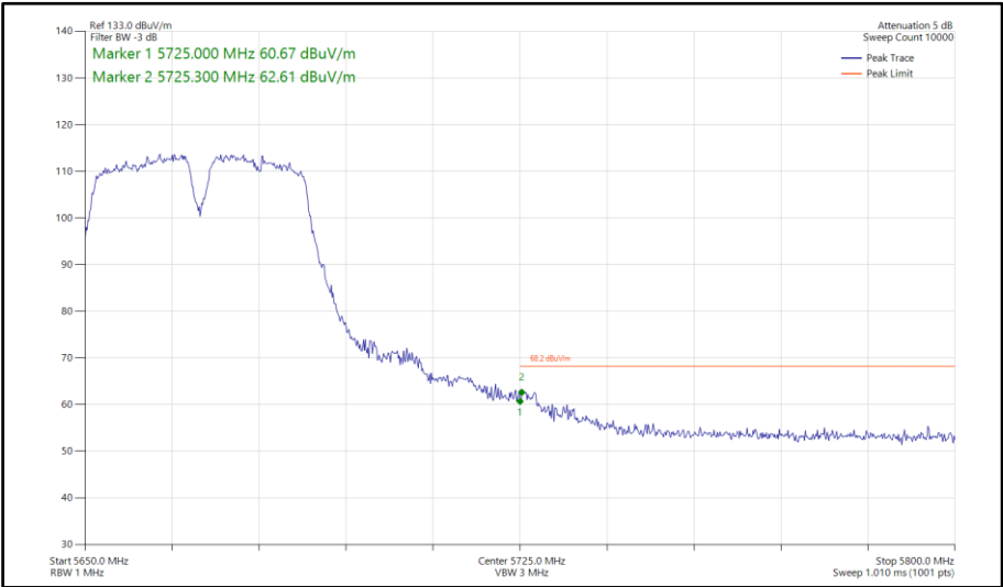
Figure 192 - 802.11a a40, SISO, Core 1 - 5670 MHz Band Edge Frequency 5725 MHz
