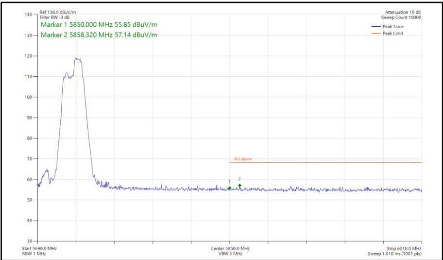
Figure 180 - 802.11be EHT40, RU 52+26-75, SISO, Core 0 - 5710 MHz Band Edge Frequency 5850 MHz
