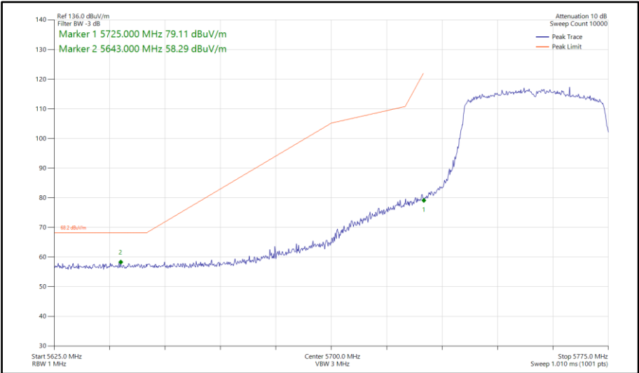
Figure 189 - 802.11ax HE40, SU, SISO, Core 1 - 5755 MHz Band Edge Frequency 5725 MHz
