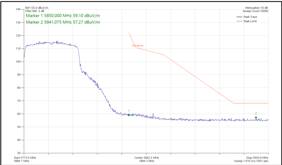
Figure 203 - 802.11ax HE40, SU, SISO, Core 1 - 5795 MHz Band Edge Frequency 5850 MHz
