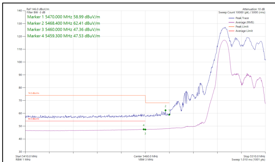
Figure 129 - 802.11ax HE20, RU 52-37, SDM, Core 0-1 - 5500 MHz Band Edge Frequency 5470 MHz
