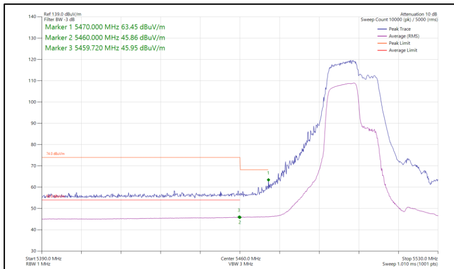
Figure 161 - 802.11be EHT40, RU 106+26-82, SISO, Core 0 - 5510 MHz Band Edge Frequency 5470 MHz
