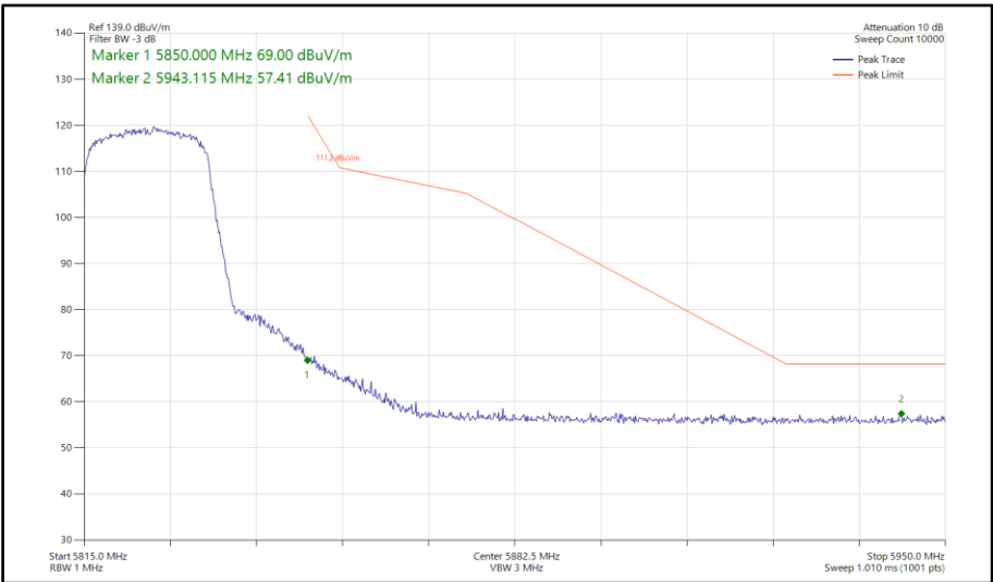
Figure 143 - 802.11ax HE20, SU, SDM, Core 0-1 - 5825 MHz Band Edge Frequency 5850 MHz
