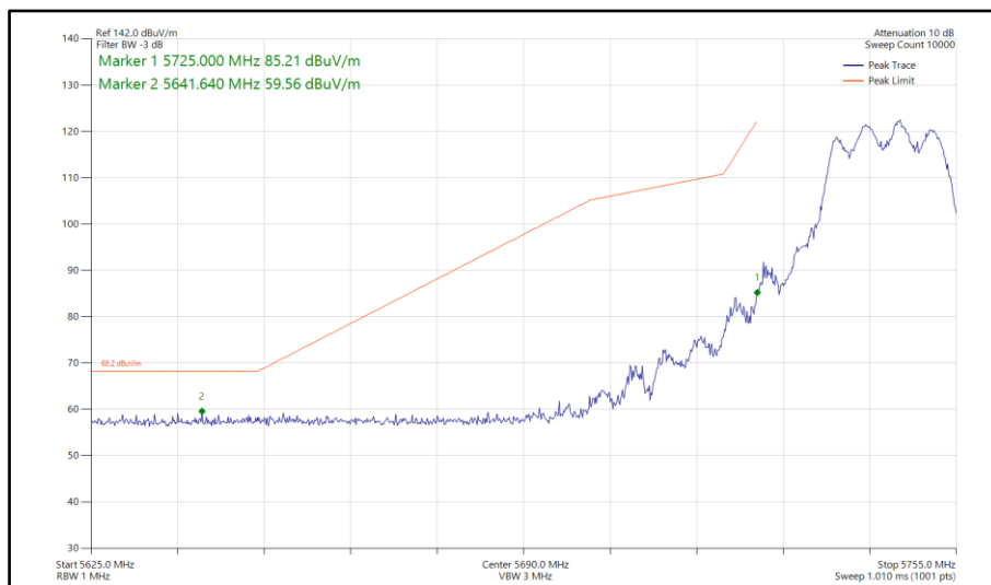
Figure 149 - 802.11ac VHT20, TxBF, Core 0-1 - 5745 MHz Band Edge Frequency 5725 MHz
