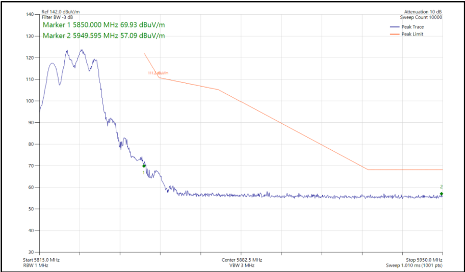
Figure 146 - 802.11be EHT20, RU 106+26-83, SDM, Core 0-1 - 5825 MHz Band Edge Frequency 5850 MHz
