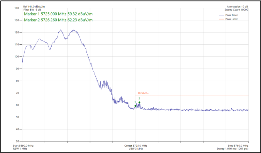
Figure 137 - 802.11ax HE20, RU 106-54, SDM, Core 0-1 - 5700 MHz Band Edge Frequency 5725 MHz
