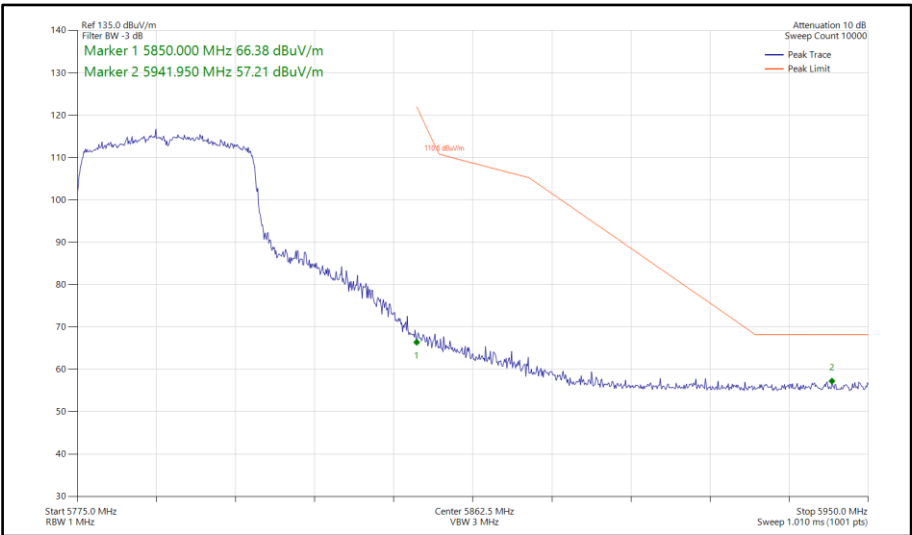
Figure 178 - 802.11ax HE40, SU, SISO, Core 0 - 5795 MHz Band Edge Frequency 5850 MHz
