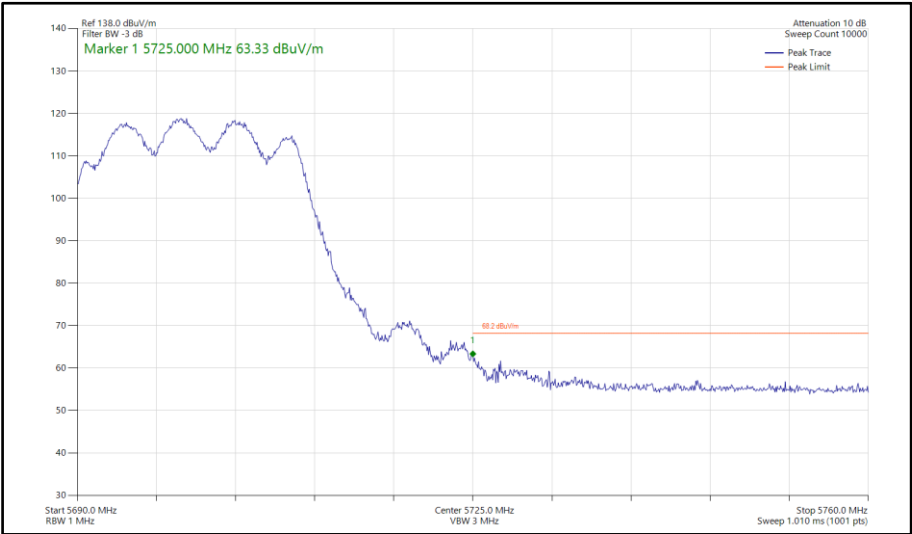
Figure 152 - 802.11ax HE20, SU, TxBF, Core 0-1 - 5700 MHz Band Edge Frequency 5725 MHz
