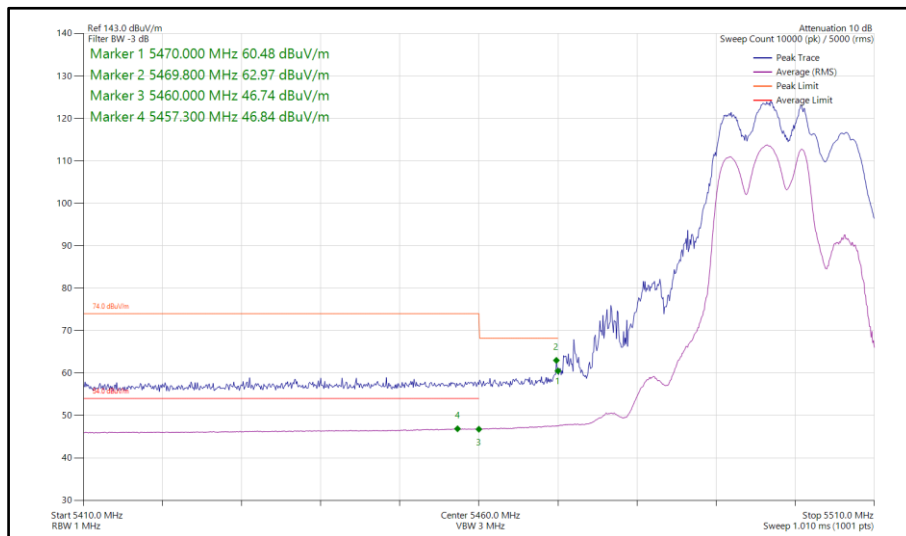
Figure 130 - 802.11be EHT20, RU 106+26-82, SDM, Core 0-1 - 5500 MHz Band Edge Frequency 5470 MHz
