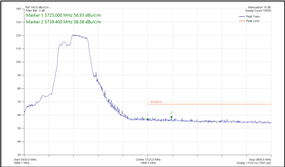
Figure 196 - 802.11be EHT40, RU 106+26-85, SISO, Core 1 - 5670 MHz Band Edge Frequency 5725 MHz
