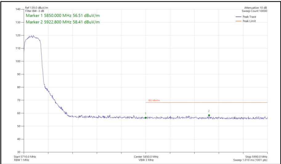
Figure 141 - 802.11ax HE20, SU, SDM, Core 0-1 - 5720 MHz Band Edge Frequency 5850 MHz
