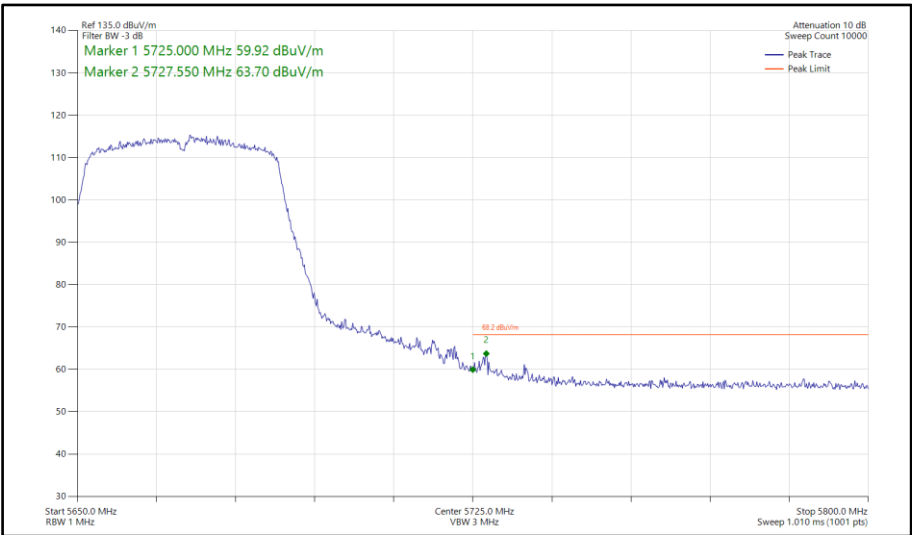
Figure 168 - 802.11n HT40, SISO, Core 0 - 5670 MHz Band Edge Frequency 5725 MHz
