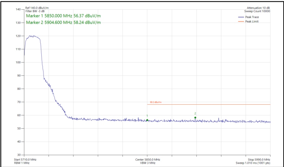
Figure 139 - 802.11n HT20, SDM, Core 0-1 - 5720 MHz Band Edge Frequency 5850 MHz
