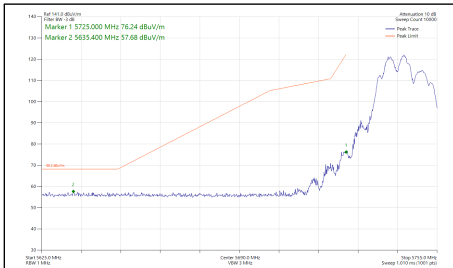
Figure 134 - 802.11be EHT20, RU 106+26-82, SDM, Core 0-1 - 5745 MHz Band Edge Frequency 5725 MHz
