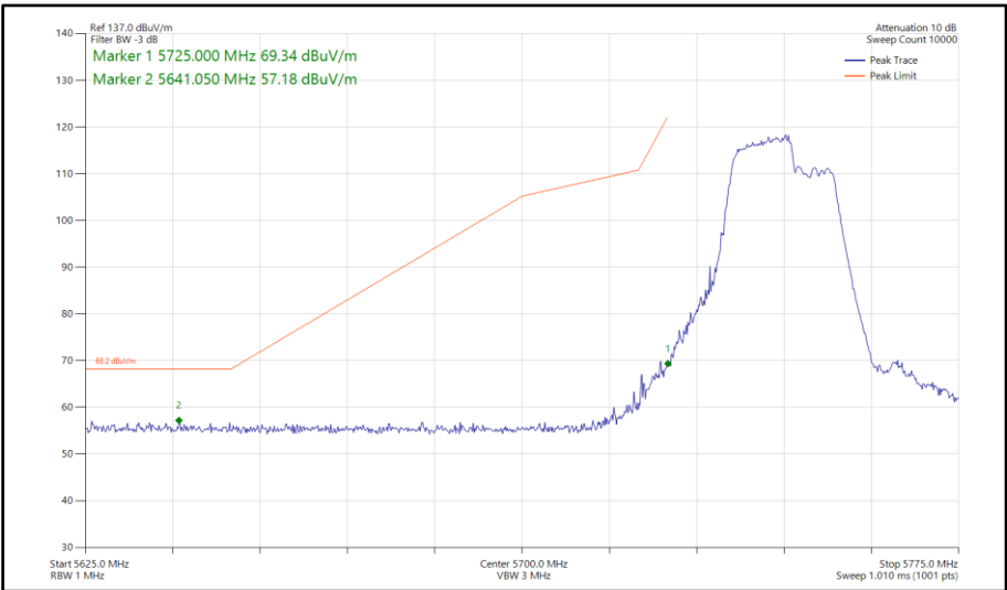
Figure 166 - 802.11be EHT40, RU 106+26-82, SISO, Core 0 - 5755 MHz Band Edge Frequency 5725 MHz
