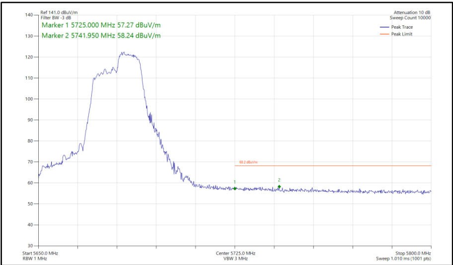
Figure 195 - 802.11ax HE40, RU 106-56, SISO, Core 1 - 5670 MHz Band Edge Frequency 5725 MHz
