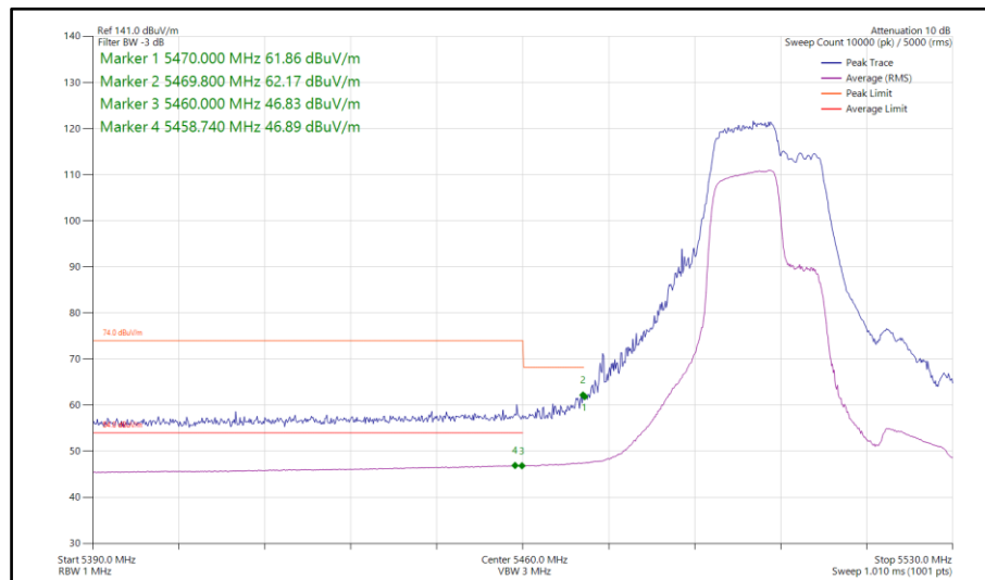
Figure 186 - 802.11be EHT40, RU 106+26-82, SISO, Core 1 - 5510 MHz Band Edge Frequency 5470 MHz
