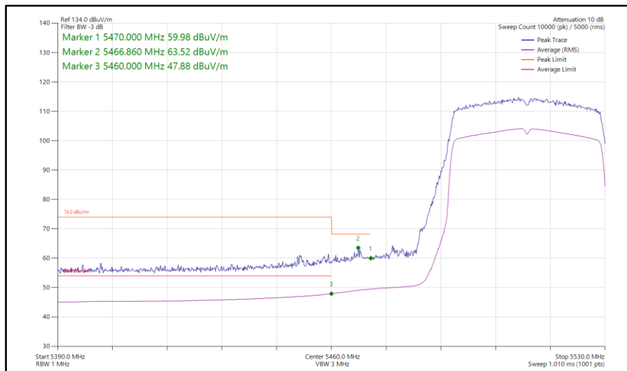
Figure 159 - 802.11ax HE40, SU, SISO, Core 0 - 5510 MHz Band Edge Frequency 5470 MHz
