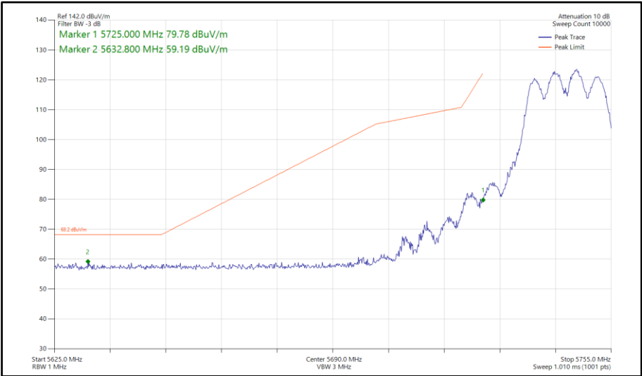
Figure 150 - 802.11ax HE20, SU, TxBF, Core 0-1 - 5745 MHz Band Edge Frequency 5725 MHz
