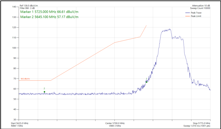
Figure 165 - 802.11ax HE40, RU 106-53, SISO, Core 0 - 5755 MHz Band Edge Frequency 5725 MHz
