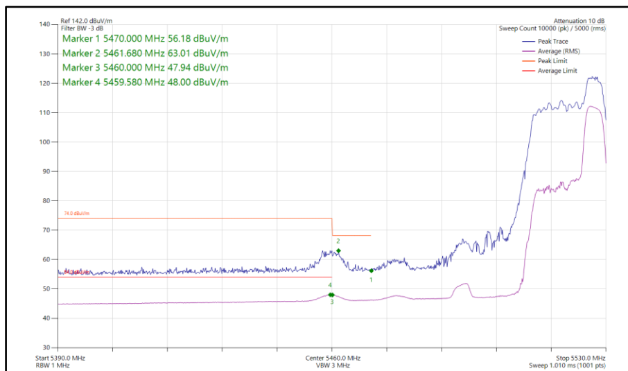
Figure 160 - 802.11ax HE40, RU 52-44, SISO, Core 0 - 5510 MHz Band Edge Frequency 5470 MHz
