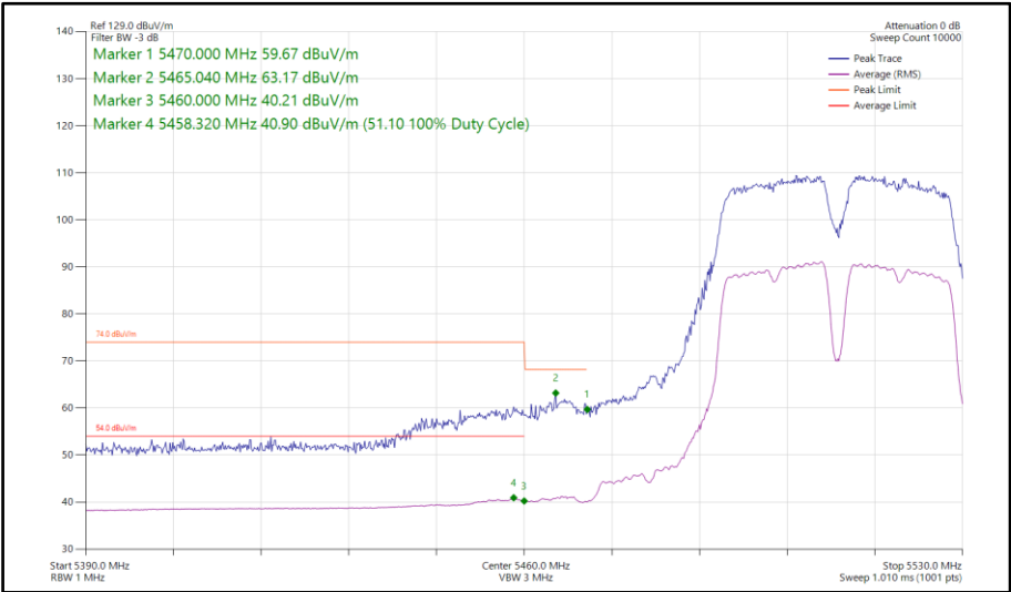
Figure 157 - 802.11a a40, SISO, Core 0 - 5510 MHz Band Edge Frequency 5470 MHz
