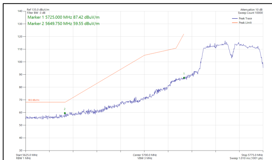
Figure 187 - 802.11a a40, SISO, Core 1 - 5755 MHz Band Edge Frequency 5725 MHz
