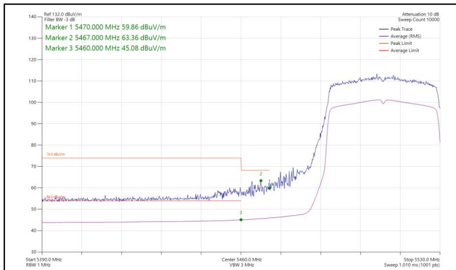
Figure 184 - 802.11ax HE40, SU, SISO, Core 1 - 5510 MHz Band Edge Frequency 5470 MHz
