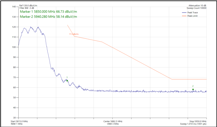
Figure 154 - 802.11ac VHT20, TxBF, Core 0-1 - 5825 MHz Band Edge Frequency 5850 MHz
