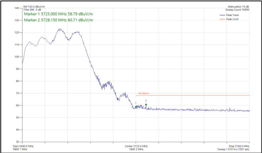
Figure 138 - 802.11be EHT20, RU 106+26-83, SDM, Core 0-1 - 5700 MHz Band Edge Frequency 5725 MHz
