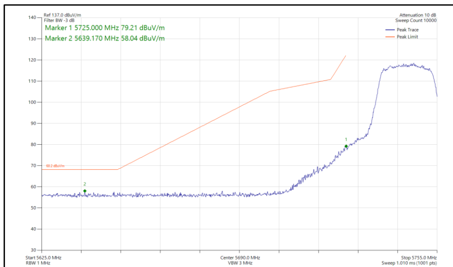
Figure 131 - 802.11n HT20, SDM, Core 0-1 - 5745 MHz Band Edge Frequency 5725 MHz
