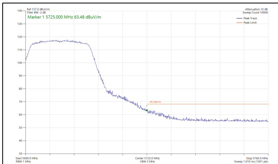
Figure 135 - 802.11n HT20, SDM, Core 0-1 - 5700 MHz Band Edge Frequency 5725 MHz
