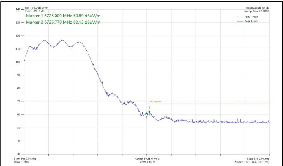
Figure 151 - 802.11ac VHT20, TxBF, Core 0-1 - 5700 MHz Band Edge Frequency 5725 MHz
