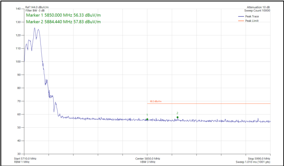
Figure 142 - 802.11ax HE20, RU 106-54, SDM, Core 0-1 - 5720 MHz Band Edge Frequency 5850 MHz
