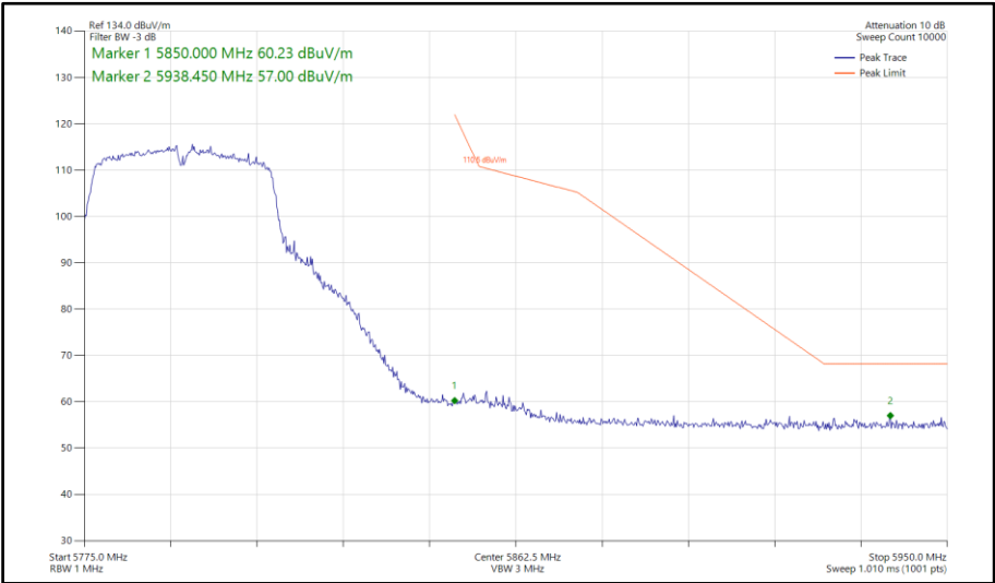
Figure 200 - 802.11n HT40, SISO, Core 1 - 5795 MHz Band Edge Frequency 5850 MHz
