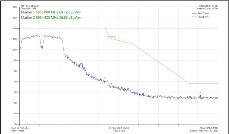
Figure 173 - 802.11a a40, SISO, Core 0 - 5795 MHz Band Edge Frequency 5850 MHz
