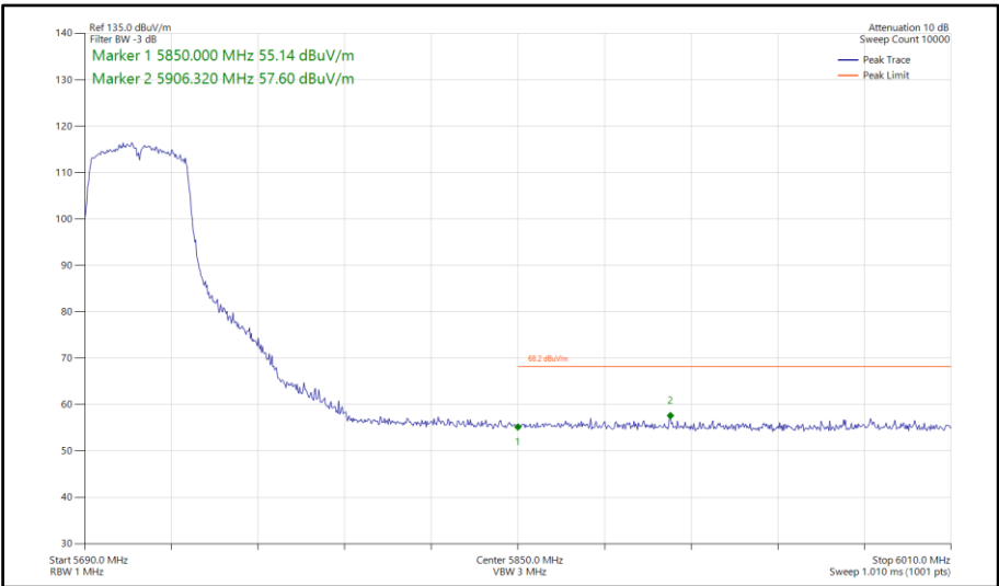
Figure 199 - 802.11n HT40, SISO, Core 1 - 5710 MHz Band Edge Frequency 5850 MHz
