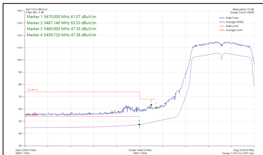
Figure 183 - 802.11n HT40, SISO, Core 1 - 5510 MHz Band Edge Frequency 5470 MHz
