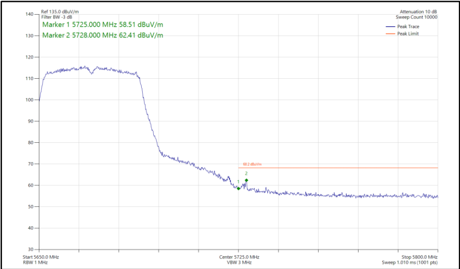
Figure 193 - 802.11n HT40, SISO, Core 1 - 5670 MHz Band Edge Frequency 5725 MHz
