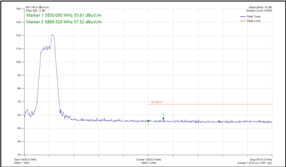
Figure 177 - 802.11ax HE40, RU 52-44, SISO, Core 0 - 5710 MHz Band Edge Frequency 5850 MHz
