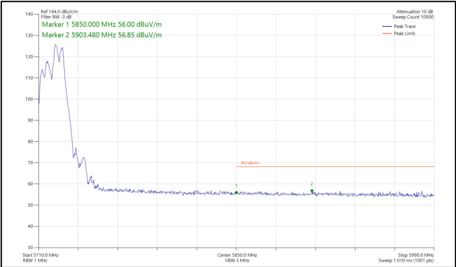
Figure 145 - 802.11be EHT20, RU 52+26-72, SDM, Core 0-1 - 5720 MHz Band Edge Frequency 5850 MHz
