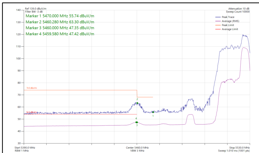
Figure 185 - 802.11ax HE40, RU 52-44, SISO, Core 1 - 5510 MHz Band Edge Frequency 5470 MHz
