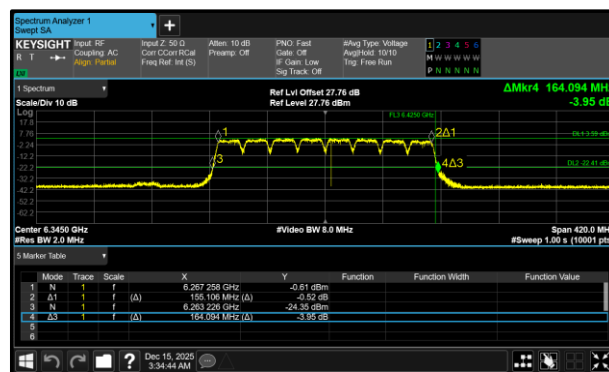
Figure 152 - 802.11a160 LPI Maximum 99% OBW
