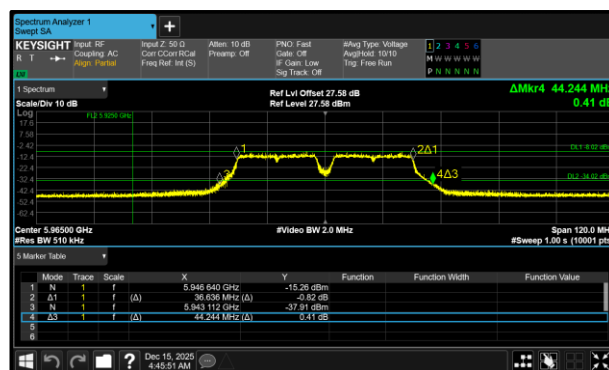
Figure 196 - 802.11a40 LPI Maximum 26 dB EBW
