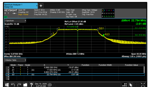
Figure 194 - 802.11a20 LPI Maximum 26 dB EBW
