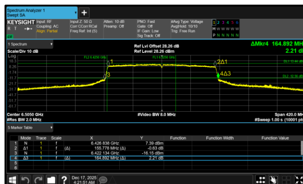
Figure 176 - 802.11ax HE160 SU SP Maximum 99% OBW
