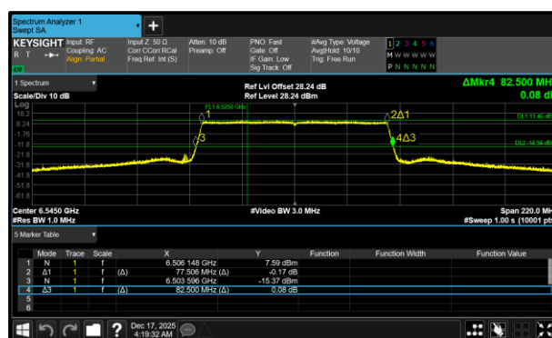
Figure 174 - 802.11ax HE80 SU SP Maximum 99% OBW
