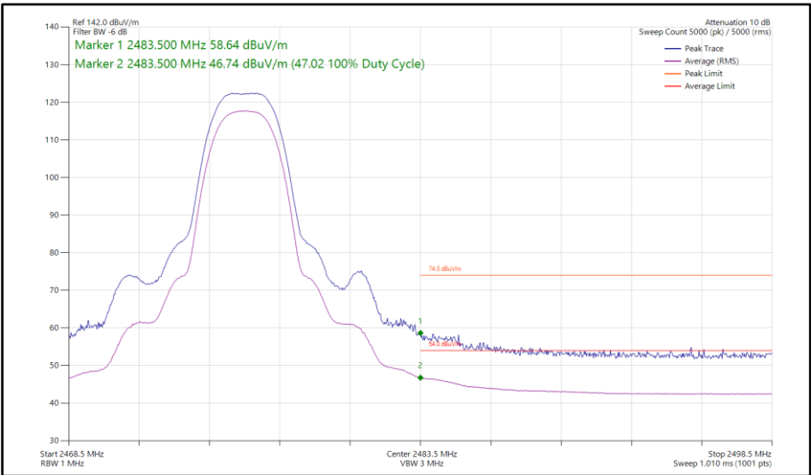
Figure 116 - Bluetooth HDT4, SISO, Core 0 - 2476 MHz Band Edge Frequency 2483.5 MHz
