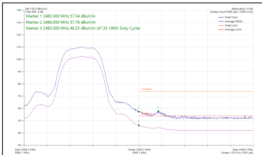
Figure 64 - Bluetooth HDR8, SISO, Core 2 - 2476 MHz Band Edge Frequency 2483.5 MHz
