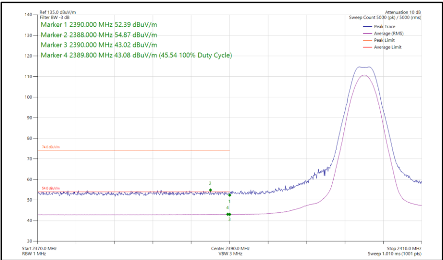
Figure 78 - Bluetooth LE2M, MIMO, Core 0-1 - 2404 MHz Band Edge Frequency 2390 MHz
