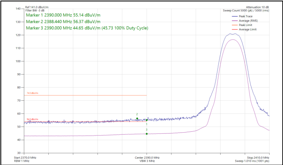
Figure 99 - Bluetooth HDR4, SISO, Core 0 - 2404 MHz Band Edge Frequency 2390 MHz
