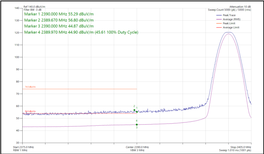
Figure 101 - Bluetooth LE1M, SISO, Core 0 - 2402 MHz Band Edge Frequency 2390 MHz
