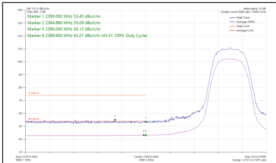
Figure 83 - Bluetooth HDRPM12, MIMO, Core 0-1 - 2404 MHz Band Edge Frequency 2390 MHz
