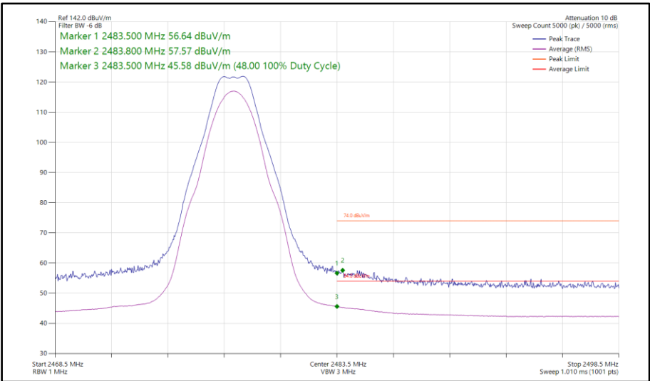
Figure 114 - Bluetooth LE2M, SISO, Core 0 - 2478 MHz Band Edge Frequency 2483.5 MHz
