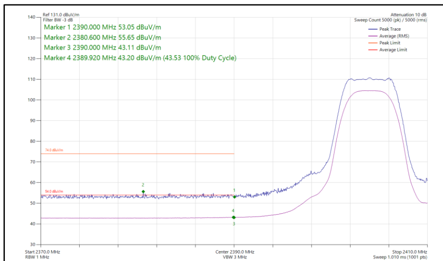
Figure 84 - Bluetooth XHDRPM8, MIMO, Core 0-1 - 2404 MHz Band Edge Frequency 2390 MHz
