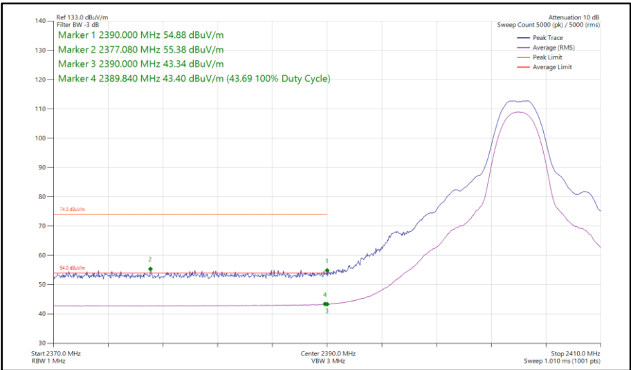
Figure 80 - Bluetooth HDT4, MIMO, Core 0-1 - 2404 MHz Band Edge Frequency 2390 MHz
