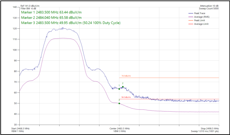
Figure 119 - Bluetooth HDRPM12, SISO, Core 0 - 2475 MHz Band Edge Frequency 2483.5 MHz
