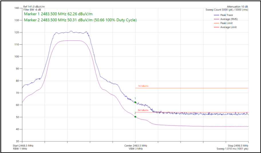
Figure 120 - Bluetooth XHDRPM8, SISO, Core 0 - 2475 MHz Band Edge Frequency 2483.5 MHz
