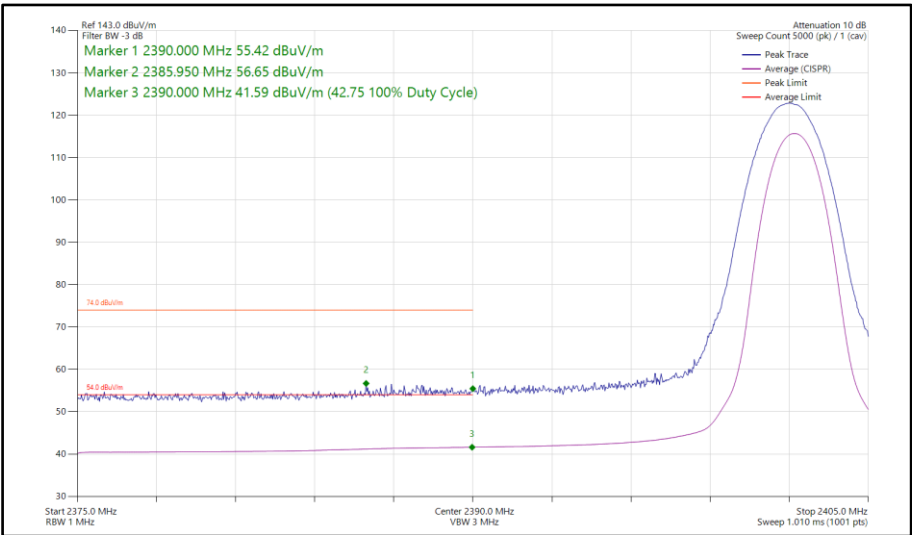
Figure 122 - Bluetooth 3DH5, SISO, Core 1 - 2402 MHz Band Edge Frequency 2390 MHz
