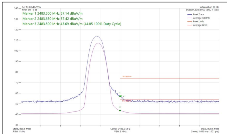
Figure 85 - Bluetooth 2DH5, MIMO, Core 0-1 - 2480 MHz Band Edge Frequency 2483.5 MHz
