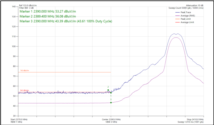
Figure 79 - Bluetooth HDT3, MIMO, Core 0-1 - 2404 MHz Band Edge Frequency 2390 MHz
