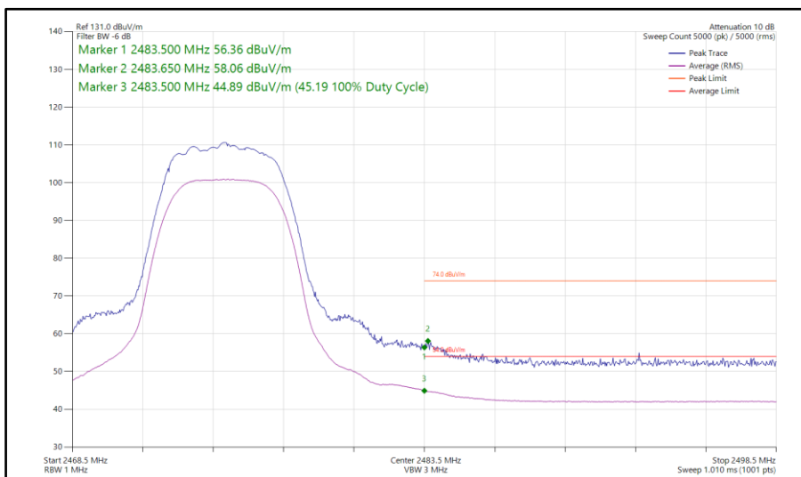
Figure 95 - Bluetooth HDRPM12, MIMO, Core 0-1 - 2475 MHz Band Edge Frequency 2483.5 MHz
