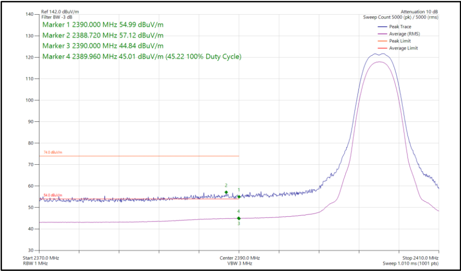
Figure 103 - Bluetooth HDT3, SISO, Core 0 - 2404 MHz Band Edge Frequency 2390 MHz
