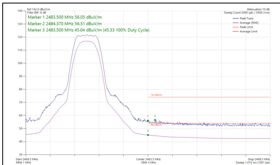
Figure 118 - Bluetooth HDRPS2, SISO, Core 0 - 2476 MHz Band Edge Frequency 2483.5 MHz
