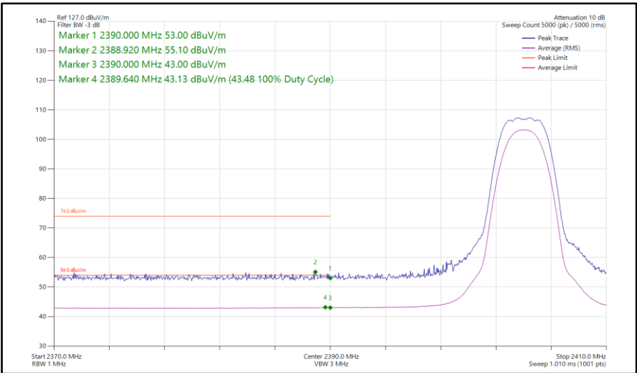
Figure 82 - Bluetooth HDRPS2, MIMO, Core 0-1 - 2404 MHz Band Edge Frequency 2390 MHz
