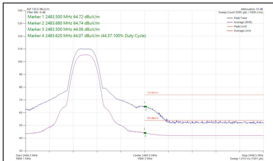
Figure 92 - Bluetooth HDT4, MIMO, Core 0-1 - 2476 MHz Band Edge Frequency 2483.5 MHz
