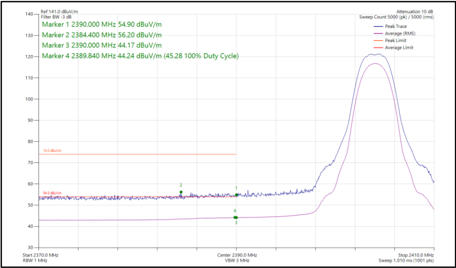
Figure 123 - Bluetooth HDR4, SISO, Core 1 - 2404 MHz Band Edge Frequency 2390 MHz
