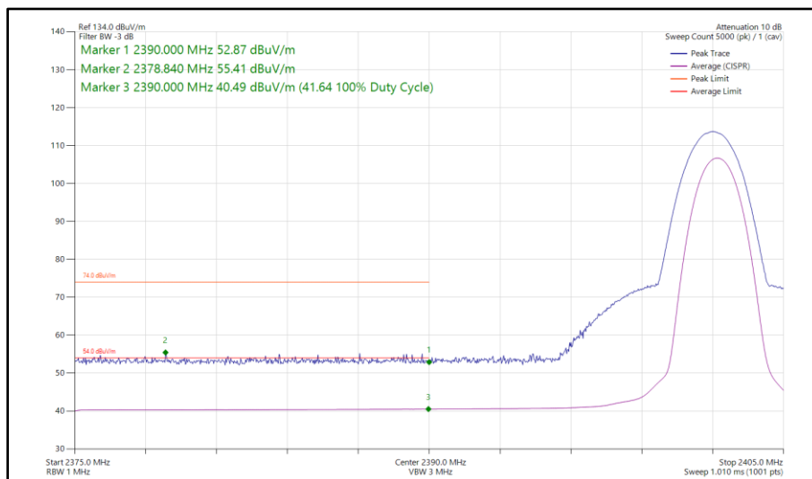
Figure 74 - Bluetooth 3DH5, MIMO, Core 0-1 - 2402 MHz Band Edge Frequency 2390 MHz
