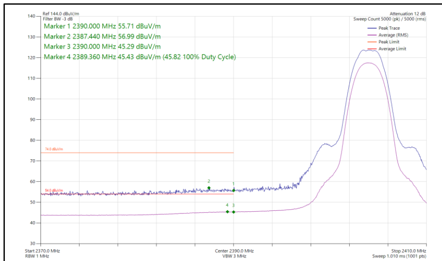
Figure 105 - Bluetooth HDT6, SISO, Core 0 - 2404 MHz Band Edge Frequency 2390 MHz
