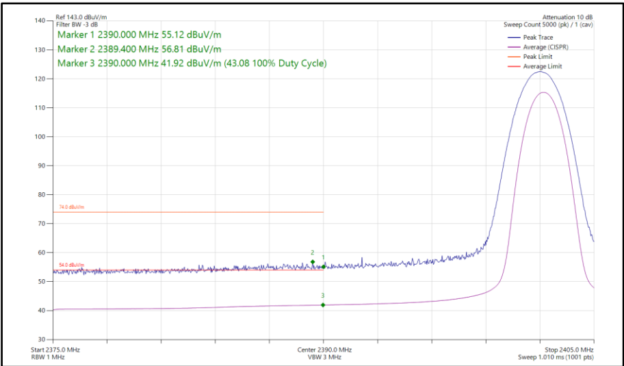
Figure 98 - Bluetooth 3DH5, SISO, Core 0 - 2402 MHz Band Edge Frequency 2390 MHz
