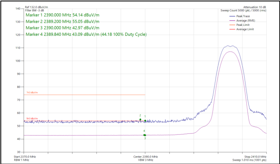
Figure 75 - Bluetooth HDR4, MIMO, Core 0-1 - 2404 MHz Band Edge Frequency 2390 MHz
