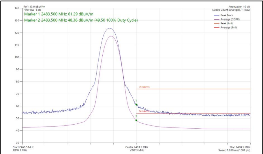
Figure 109 - Bluetooth 2DH5, SISO, Core 0 - 2480 MHz Band Edge Frequency 2483.5 MHz
