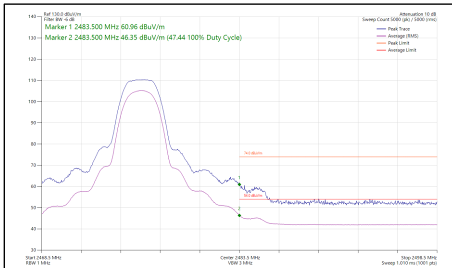
Figure 63 - Bluetooth HDR4, SISO, Core 2 - 2476 MHz Band Edge Frequency 2483.5 MHz
