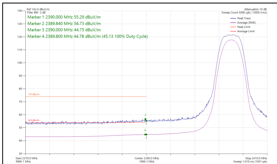
Figure 106 - Bluetooth HDRPS2, SISO, Core 0 - 2404 MHz Band Edge Frequency 2390 MHz
