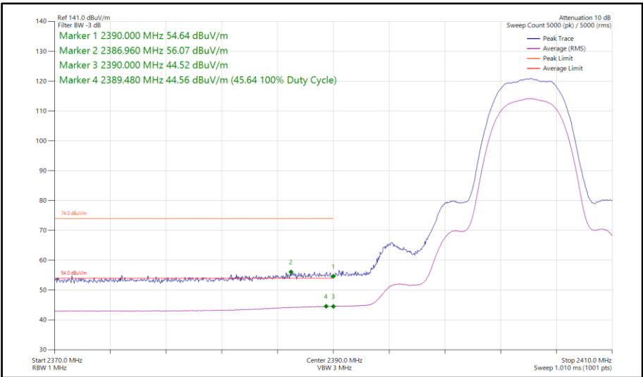
Figure 124 - Bluetooth HDR8, SISO, Core 1 - 2404 MHz Band Edge Frequency 2390 MHz
