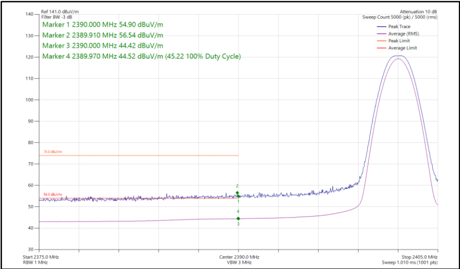
Figure 125 - Bluetooth LE1M, SISO, Core 1 - 2402 MHz Band Edge Frequency 2390 MHz
