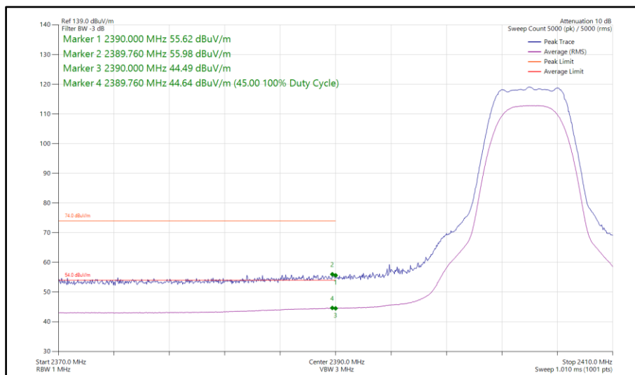
Figure 108 - Bluetooth XHDRPM8, SISO, Core 0 - 2404 MHz Band Edge Frequency 2390 MHz
