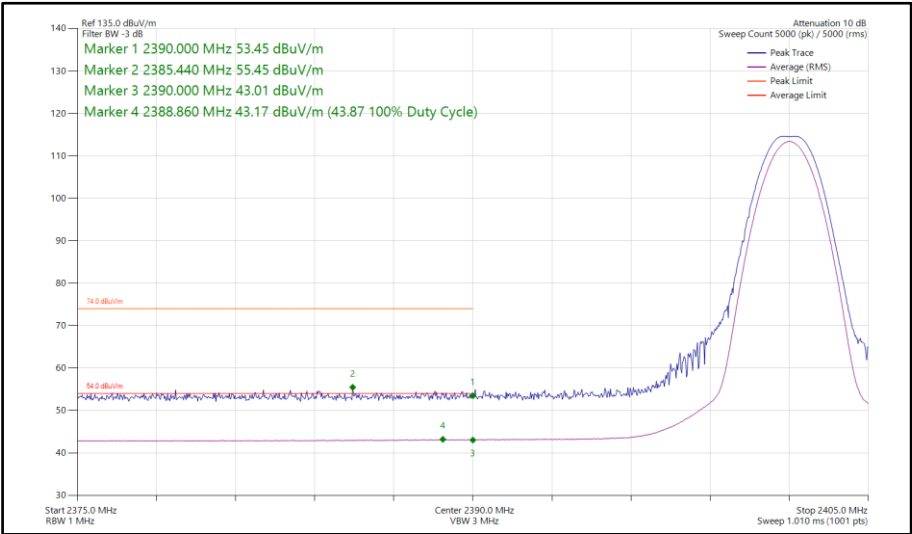
Figure 77 - Bluetooth LE1M, MIMO, Core 0-1 - 2402 MHz Band Edge Frequency 2390 MHz
