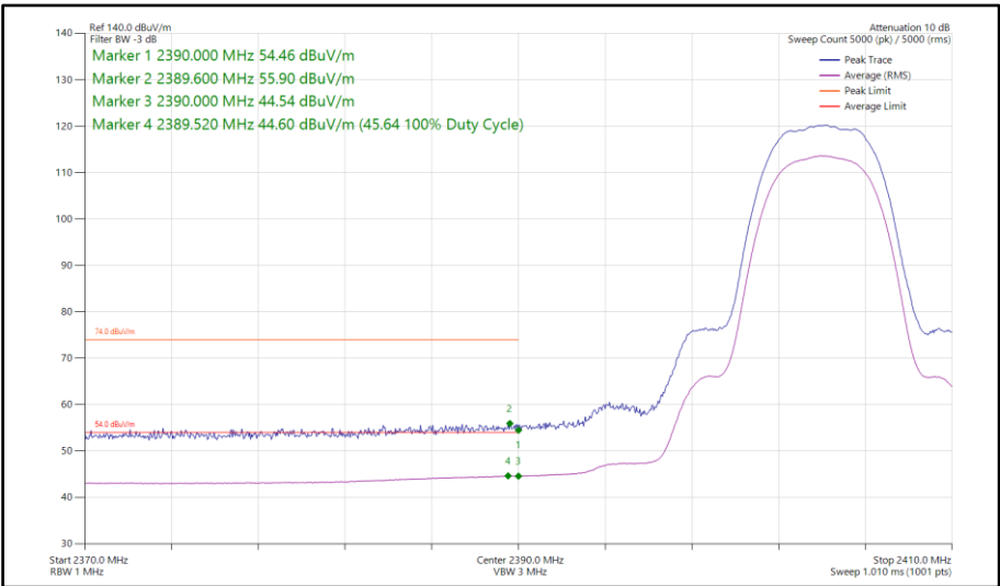
Figure 100 - Bluetooth HDR8, SISO, Core 0 - 2404 MHz Band Edge Frequency 2390 MHz
