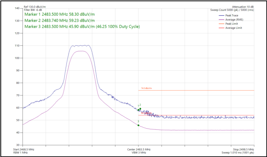
Figure 70 - Bluetooth HDRPS2, SISO, Core 2 - 2476 MHz Band Edge Frequency 2483.5 MHz
