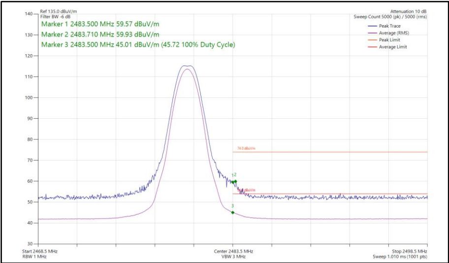
Figure 89 - Bluetooth LE1M, MIMO, Core 0-1 - 2480 MHz Band Edge Frequency 2483.5 MHz
