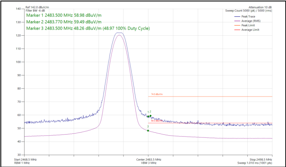
Figure 113 - Bluetooth LE1M, SISO, Core 0 - 2480 MHz Band Edge Frequency 2483.5 MHz
