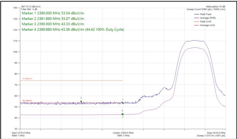
Figure 76 - Bluetooth HDR8, MIMO, Core 0-1 - 2404 MHz Band Edge Frequency 2390 MHz
