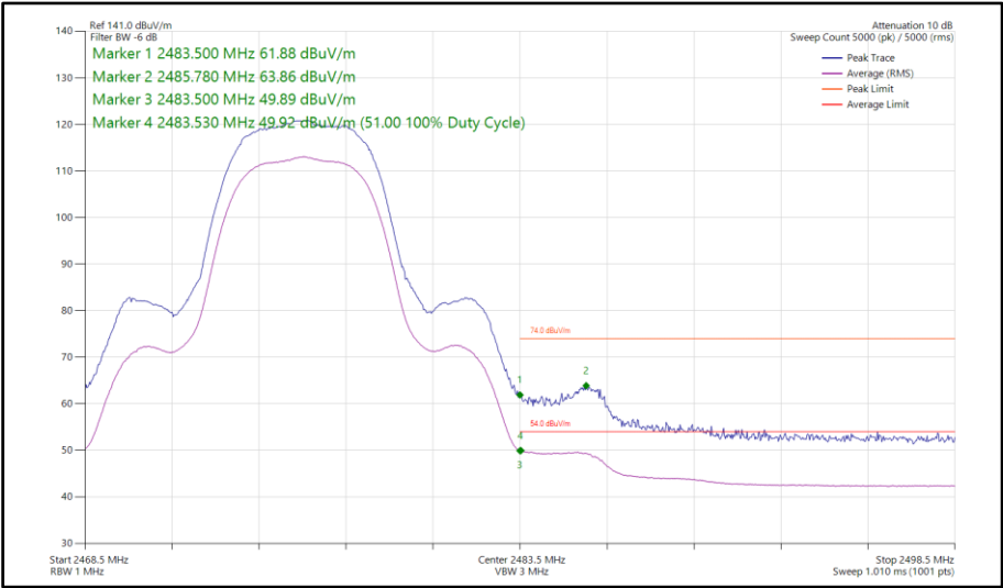
Figure 112 - Bluetooth HDR8, SISO, Core 0 - 2476 MHz Band Edge Frequency 2483.5 MHz
