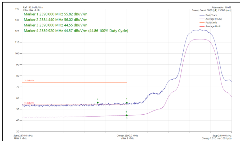
Figure 107 - Bluetooth HDRPM12, SISO, Core 0 - 2404 MHz Band Edge Frequency 2390 MHz
