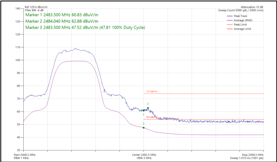
Figure 71 - Bluetooth HDRPM12, SISO, Core 2 - 2475 MHz Band Edge Frequency 2483.5 MHz
