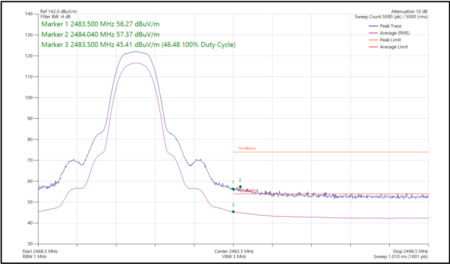
Figure 111 - Bluetooth HDR4, SISO, Core 0 - 2476 MHz Band Edge Frequency 2483.5 MHz
