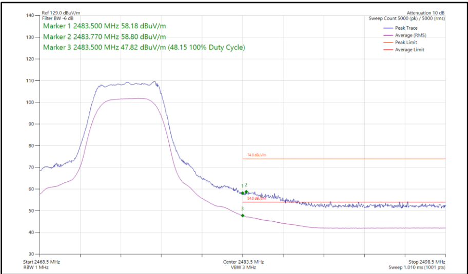
Figure 72 - Bluetooth XHDRPM8, SISO, Core 2 - 2475 MHz Band Edge Frequency 2483.5 MHz
