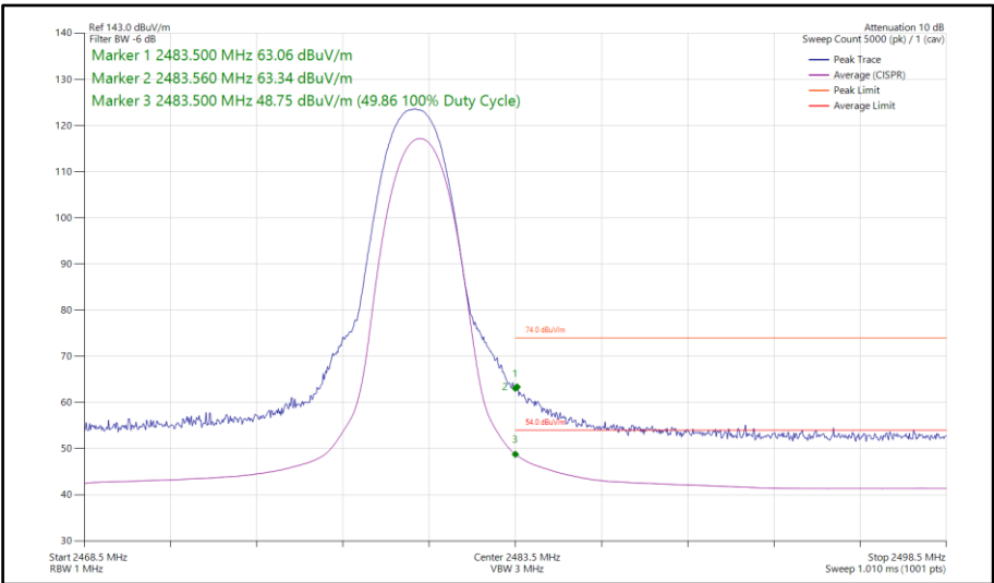
Figure 110 - Bluetooth 3DH5, SISO, Core 0 - 2480 MHz Band Edge Frequency 2483.5 MHz
