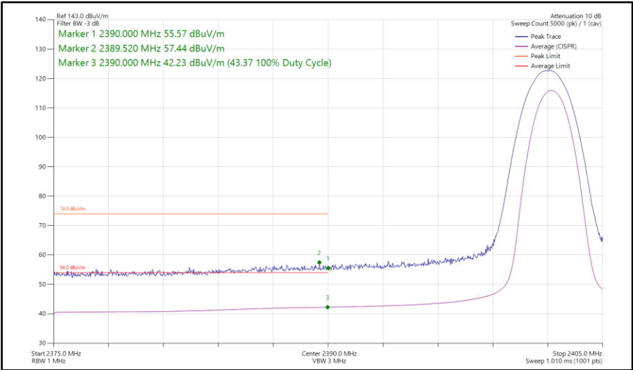
Figure 97 - Bluetooth 2DH5, SISO, Core 0 - 2402 MHz Band Edge Frequency 2390 MHz
