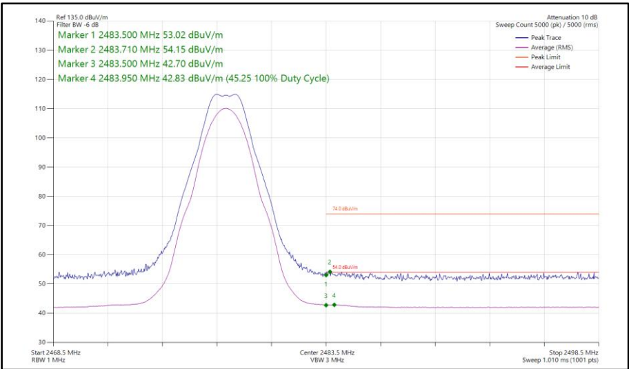
Figure 90 - Bluetooth LE2M, MIMO, Core 0-1 - 2478 MHz Band Edge Frequency 2483.5 MHz
