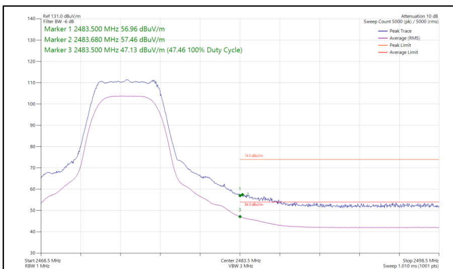
Figure 96 - Bluetooth XHDRPM8, MIMO, Core 0-1 - 2475 MHz Band Edge Frequency 2483.5 MHz
