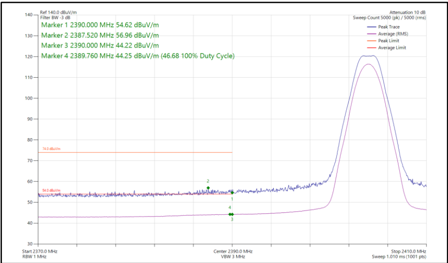
Figure 102 - Bluetooth LE2M, SISO, Core 0 - 2404 MHz Band Edge Frequency 2390 MHz
