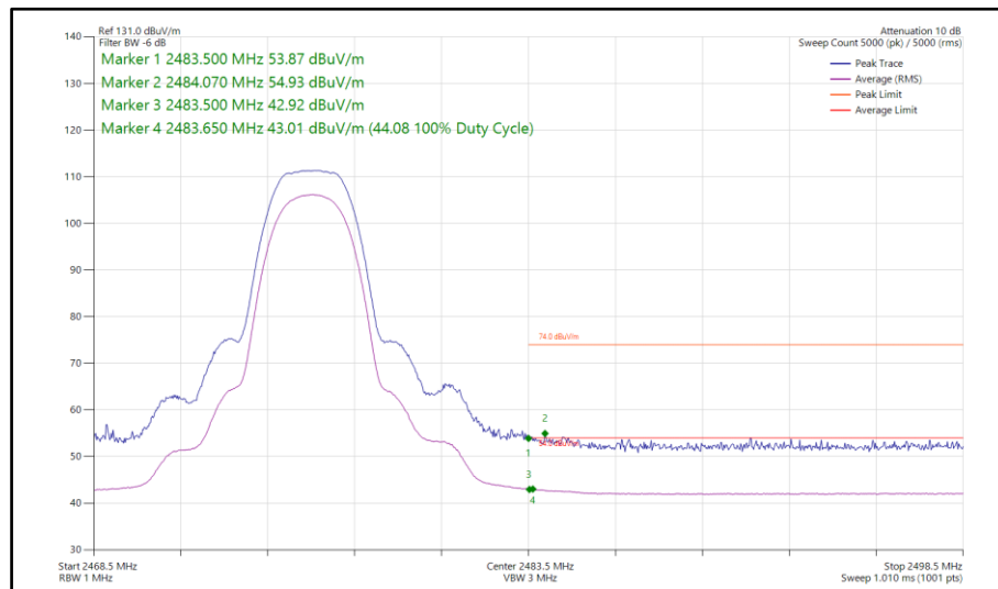
Figure 87 - Bluetooth HDR4, MIMO, Core 0-1 - 2476 MHz Band Edge Frequency 2483.5 MHz
