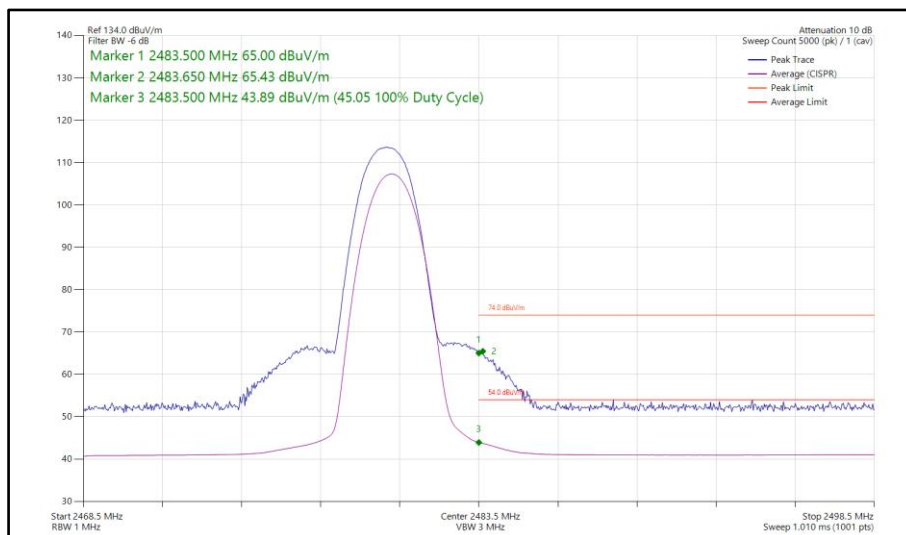
Figure 86 - Bluetooth 3DH5, MIMO, Core 0-1 - 2480 MHz Band Edge Frequency 2483.5 MHz
