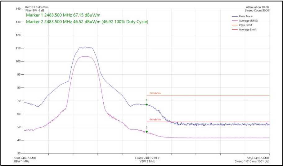
Figure 69 - Bluetooth HDT6, SISO, Core 2 - 2476 MHz Band Edge Frequency 2483.5 MHz
