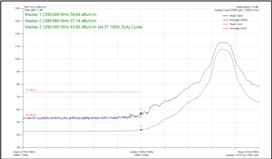
Figure 81 - Bluetooth HDT6, MIMO, Core 0-1 - 2404 MHz Band Edge Frequency 2390 MHz
