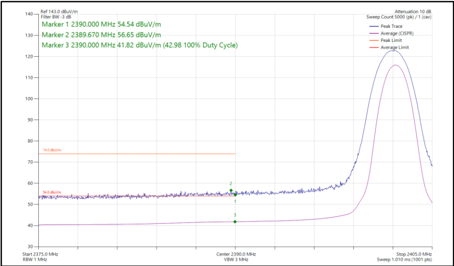
Figure 121 - Bluetooth 2DH5, SISO, Core 1 - 2402 MHz Band Edge Frequency 2390 MHz
