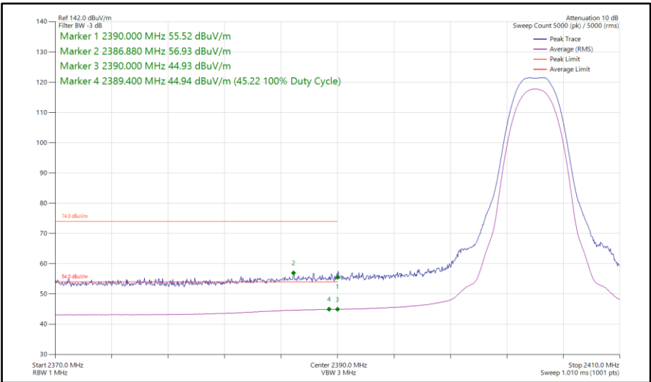
Figure 104 - Bluetooth HDT4, SISO, Core 0 - 2404 MHz Band Edge Frequency 2390 MHz
