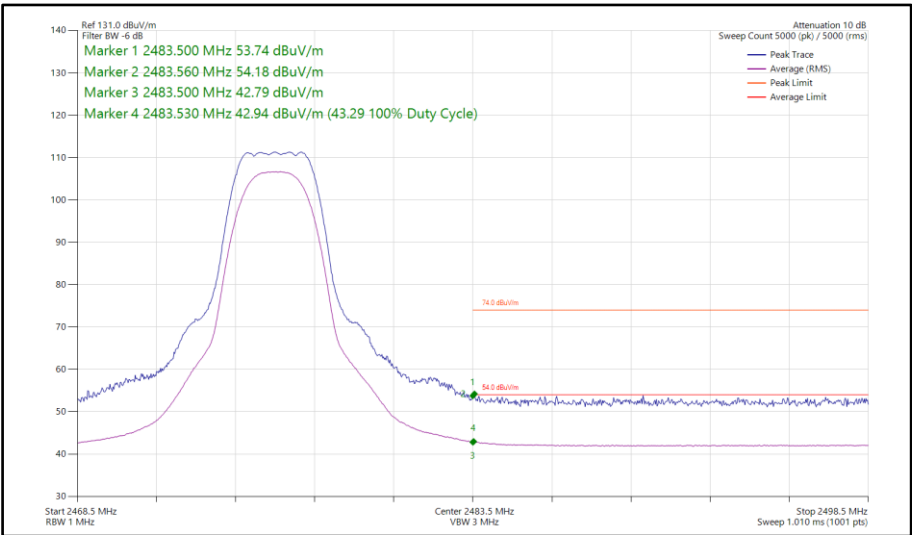
Figure 94 - Bluetooth HDRPS2, MIMO, Core 0-1 - 2476 MHz Band Edge Frequency 2483.5 MHz
