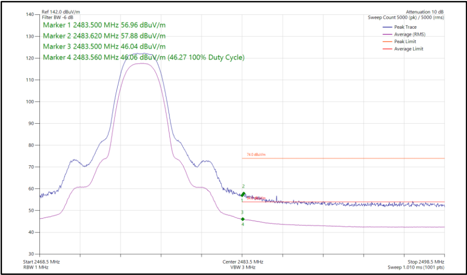
Figure 115 - Bluetooth HDT3, SISO, Core 0 - 2476 MHz Band Edge Frequency 2483.5 MHz
