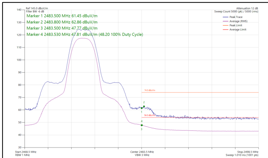
Figure 117 - Bluetooth HDT6, SISO, Core 0 - 2476 MHz Band Edge Frequency 2483.5 MHz
