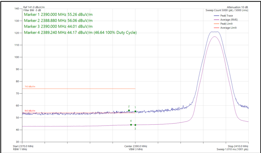
Figure 126 - Bluetooth LE2M, SISO, Core 1 - 2404 MHz Band Edge Frequency 2390 MHz
