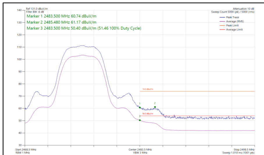
Figure 88 - Bluetooth HDR8, MIMO, Core 0-1 - 2476 MHz Band Edge Frequency 2483.5 MHz
