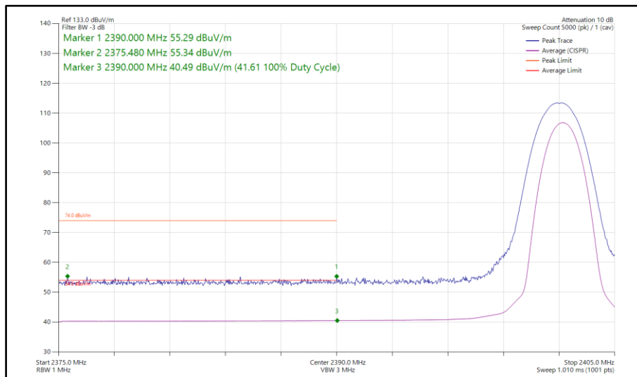
Figure 73 - Bluetooth 2DH5, MIMO, Core 0-1 - 2402 MHz Band Edge Frequency 2390 MHz
