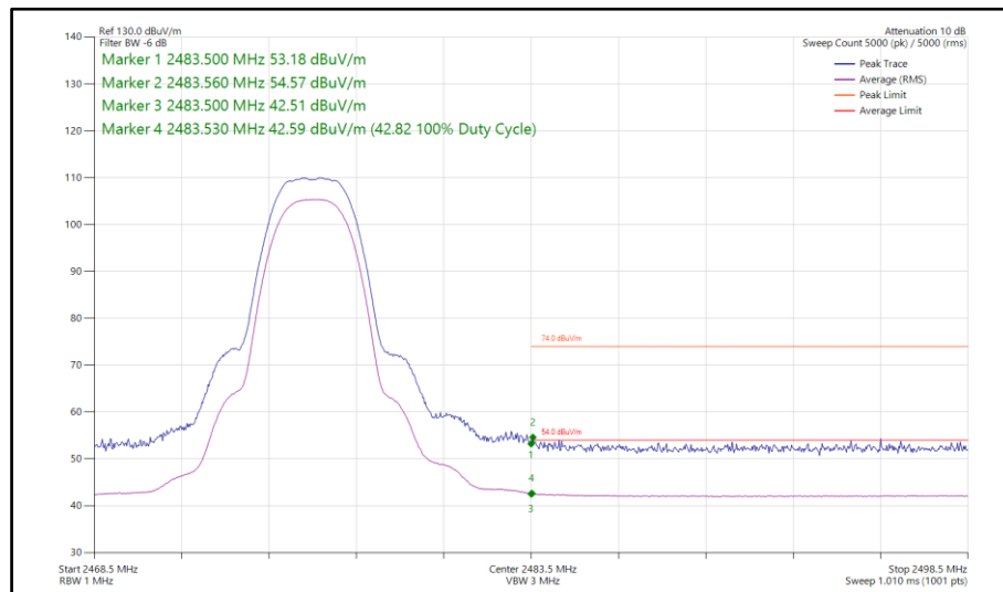
Figure 91 - Bluetooth HDT3, MIMO, Core 0-1 - 2476 MHz Band Edge Frequency 2483.5 MHz
