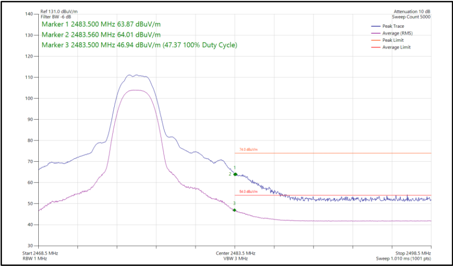
Figure 93 - Bluetooth HDT6, MIMO, Core 0-1 - 2476 MHz Band Edge Frequency 2483.5 MHz
