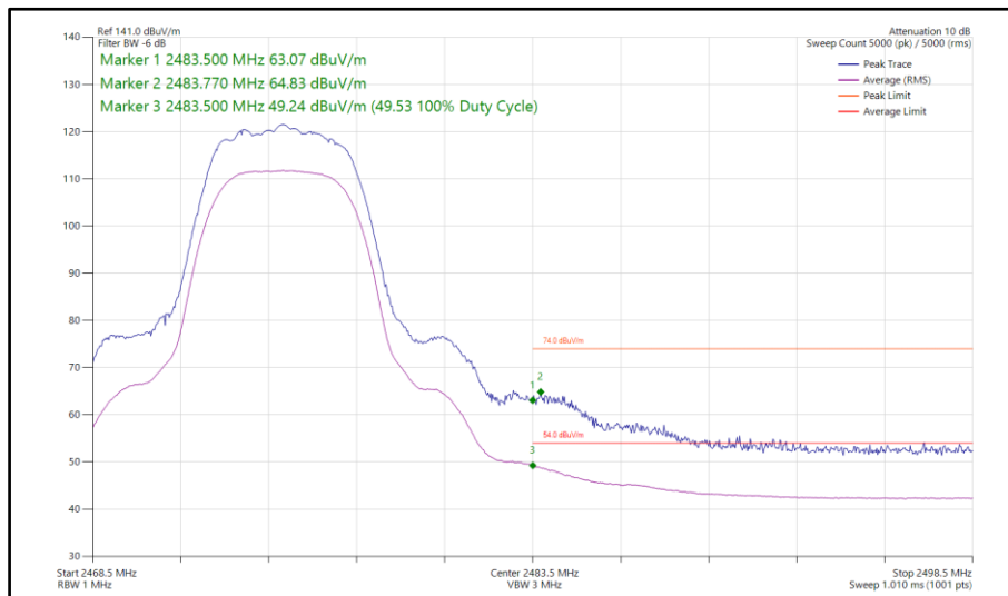
Figure 143 - Bluetooth HDRPM12, SISO, Core 1 - 2475 MHz Band Edge Frequency 2483.5 MHz
