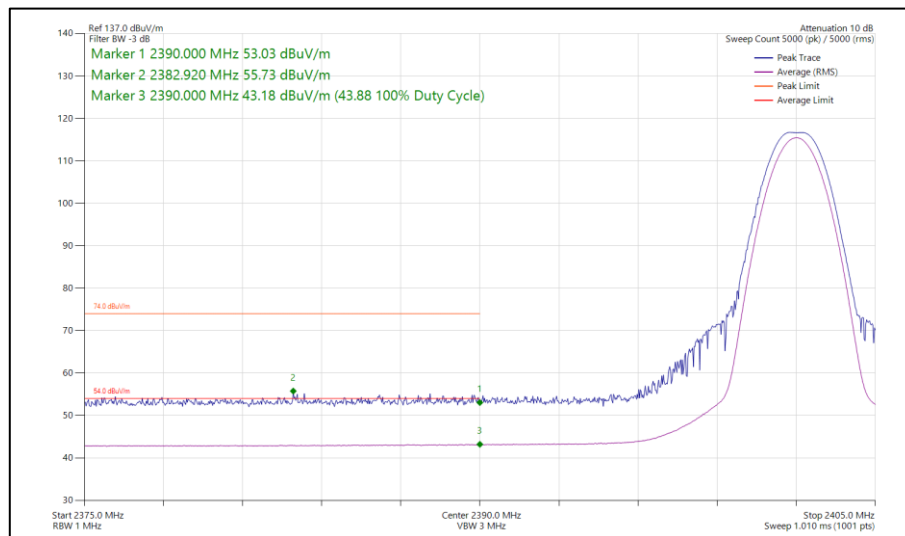
Figure 173 - Bluetooth LE1M, MIMO, Core 0-2 - 2402 MHz Band Edge Frequency 2390 MHz
