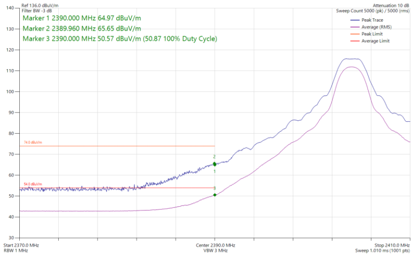
Figure 176 - Bluetooth HDT4, MIMO, Core 0-2 - 2404 MHz Band Edge Frequency 2390 MHz
