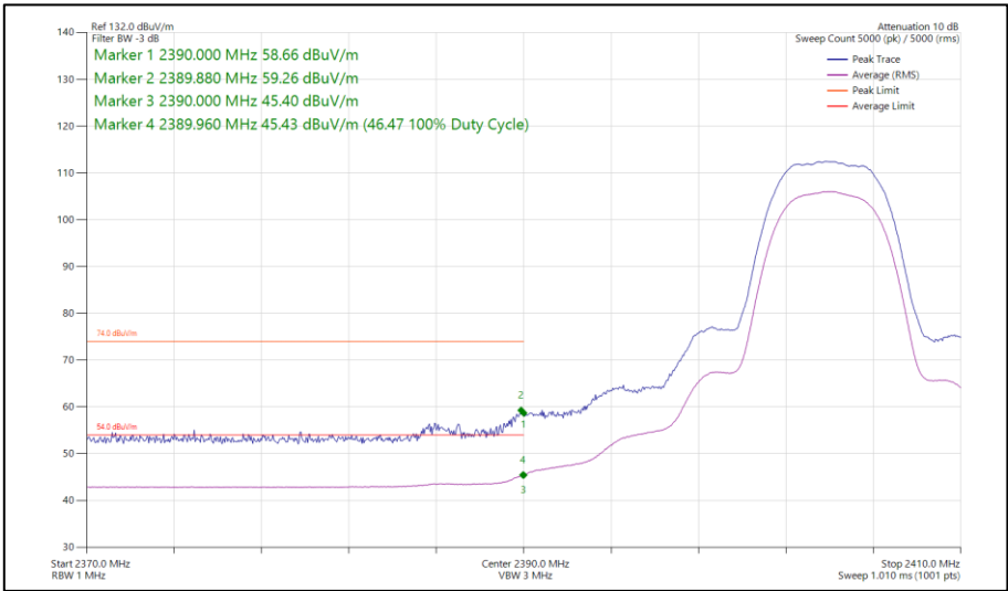
Figure 172 - Bluetooth HDR8, MIMO, Core 0-2 - 2404 MHz Band Edge Frequency 2390 MHz
