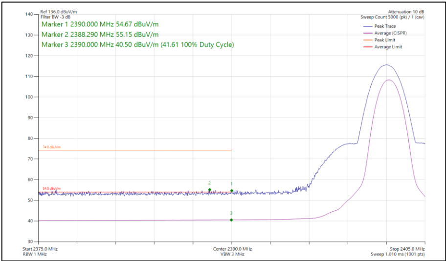
Figure 170 - Bluetooth 3DH5, MIMO, Core 0-2 - 2402 MHz Band Edge Frequency 2390 MHz
