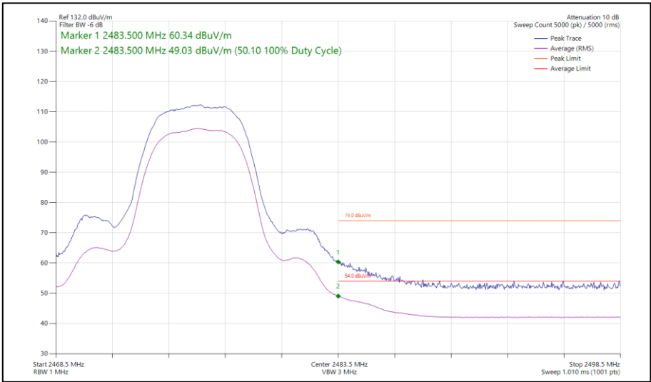
Figure 184 - Bluetooth HDR8, MIMO, Core 0-2 - 2476 MHz Band Edge Frequency 2483.5 MHz
