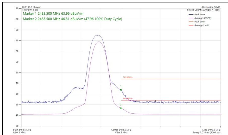
Figure 181 - Bluetooth 2DH5, MIMO, Core 0-2 - 2480 MHz Band Edge Frequency 2483.5 MHz
