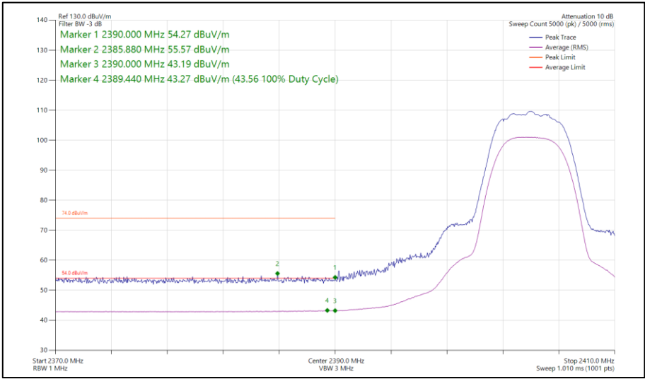
Figure 179 - Bluetooth HDRPM12, MIMO, Core 0-2 - 2404 MHz Band Edge Frequency 2390 MHz
