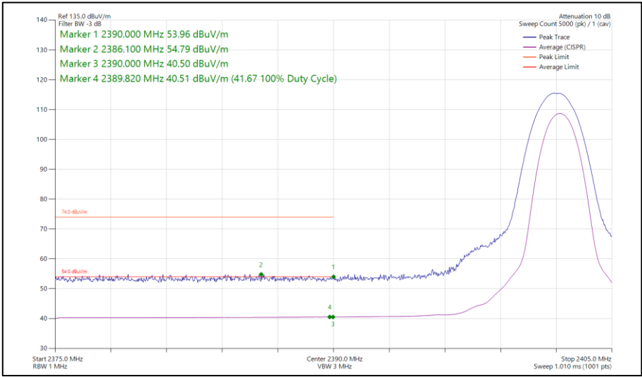
Figure 169 - Bluetooth 2DH5, MIMO, Core 0-2 - 2402 MHz Band Edge Frequency 2390 MHz
