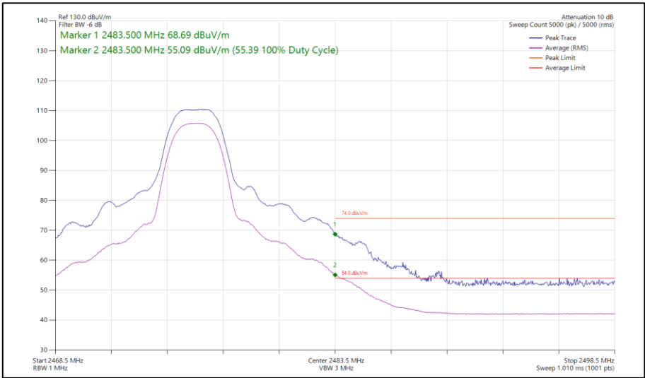
Figure 188 - Bluetooth HDT4, MIMO, Core 0-2 - 2476 MHz Band Edge Frequency 2483.5 MHz
