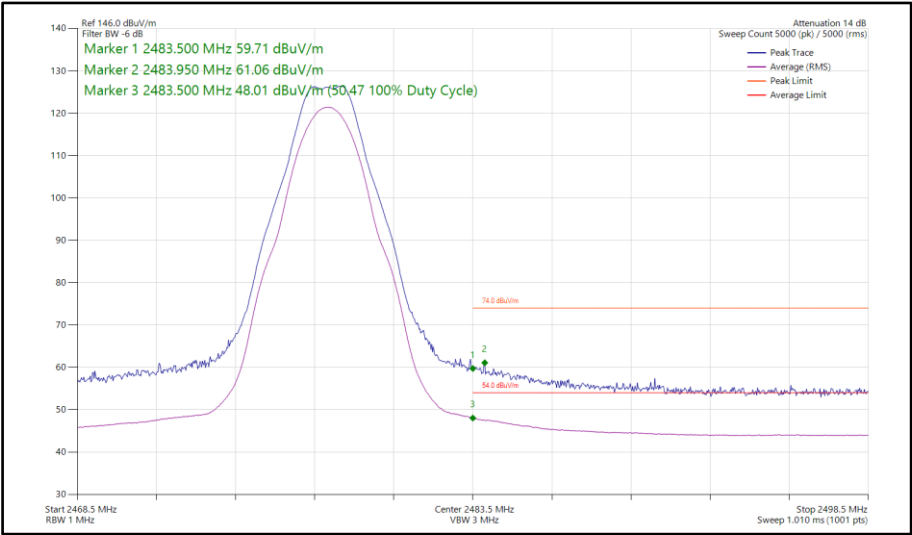
Figure 162 - Bluetooth LE2M, MIMO, Core 0-1 - 2478 MHz Band Edge Frequency 2483.5 MHz
