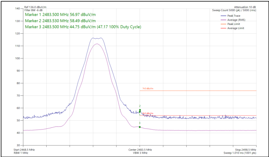
Figure 186 - Bluetooth LE2M, MIMO, Core 0-2 - 2478 MHz Band Edge Frequency 2483.5 MHz
