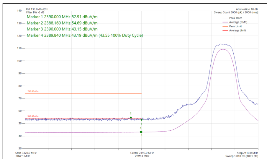
Figure 178 - Bluetooth HDRPS2, MIMO, Core 0-2 - 2404 MHz Band Edge Frequency 2390 MHz
