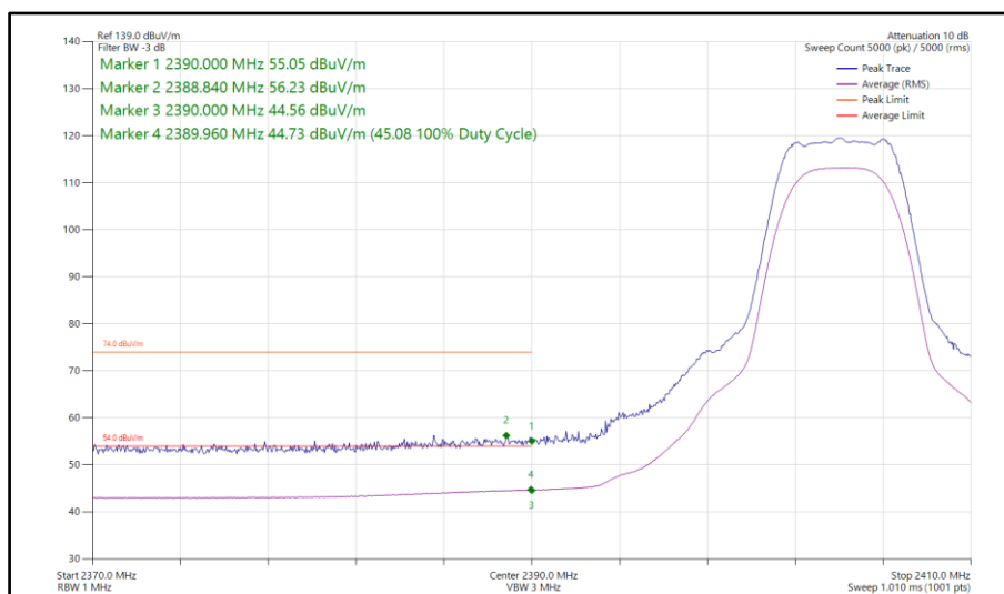
Figure 132 - Bluetooth XHDRPM8, SISO, Core 1 - 2404 MHz Band Edge Frequency 2390 MHz
