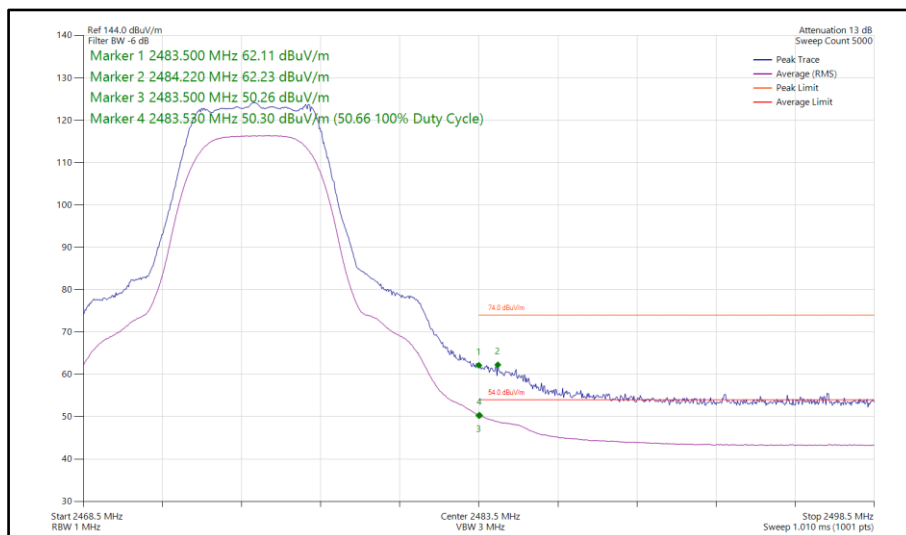
Figure 168 - Bluetooth XHDRPM8, MIMO, Core 0-1 - 2475 MHz Band Edge Frequency 2483.5 MHz
