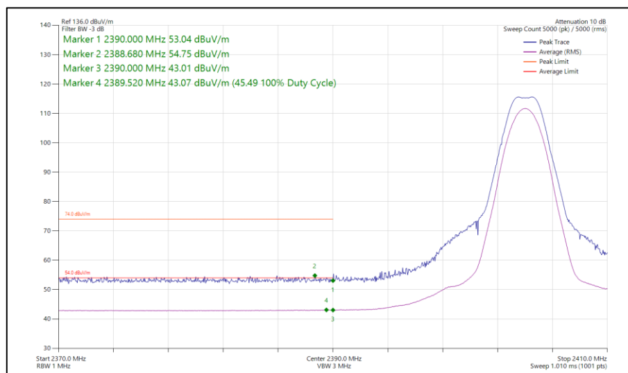
Figure 174 - Bluetooth LE2M, MIMO, Core 0-2 - 2404 MHz Band Edge Frequency 2390 MHz
