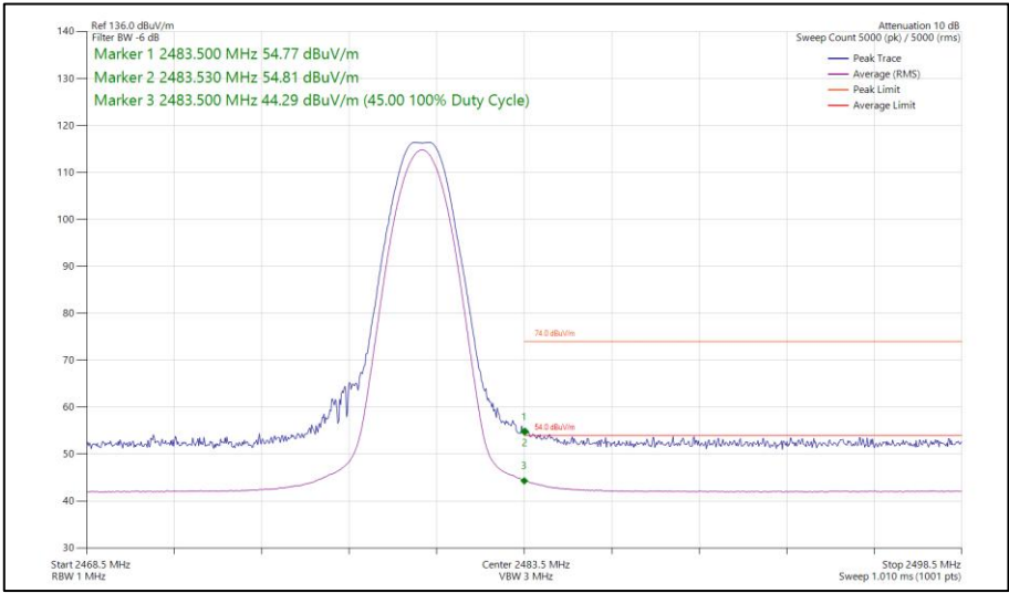
Figure 185 - Bluetooth LE1M, MIMO, Core 0-2 - 2480 MHz Band Edge Frequency 2483.5 MHz
