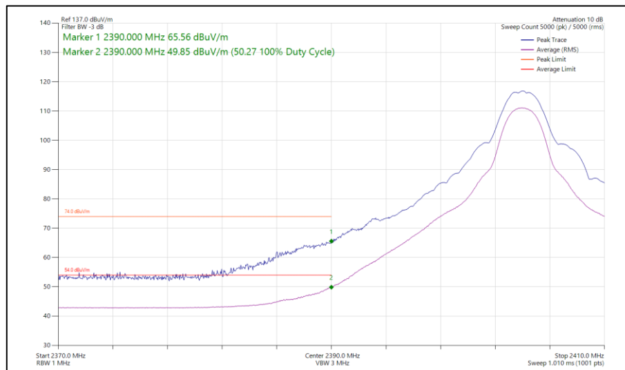
Figure 177 - Bluetooth HDT6, MIMO, Core 0-2 - 2404 MHz Band Edge Frequency 2390 MHz
