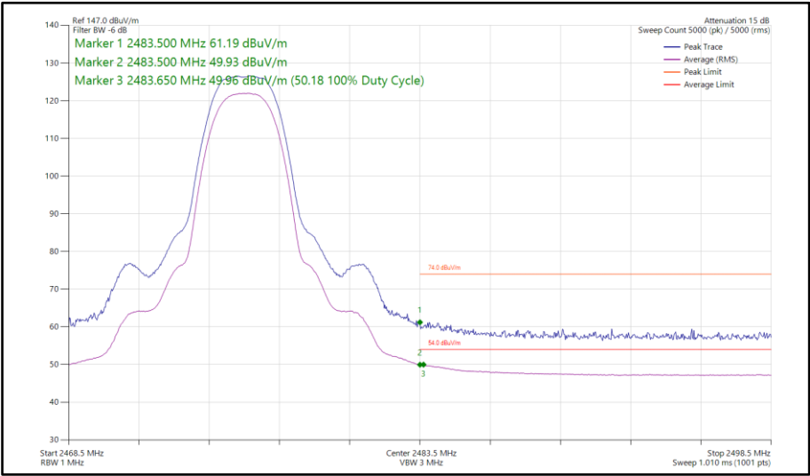
Figure 163 - Bluetooth HDT3, MIMO, Core 0-1 - 2476 MHz Band Edge Frequency 2483.5 MHz
