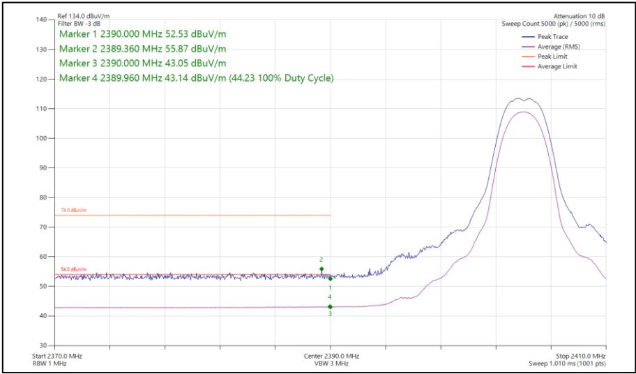
Figure 171 - Bluetooth HDR4, MIMO, Core 0-2 - 2404 MHz Band Edge Frequency 2390 MHz
