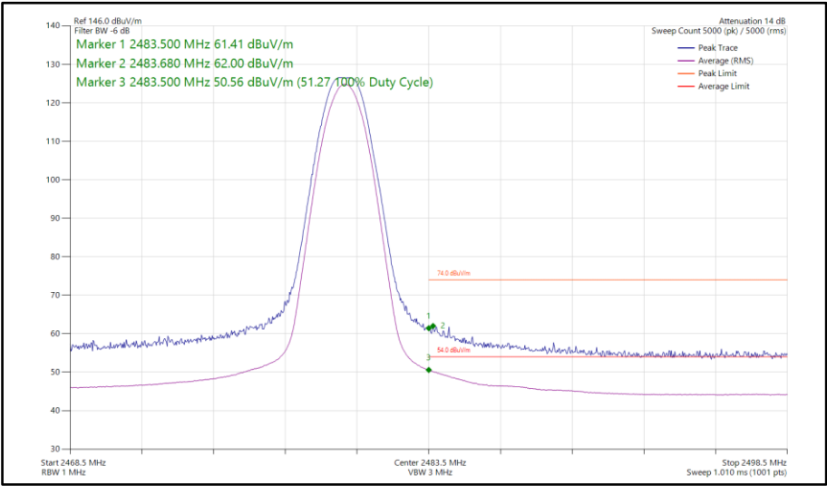
Figure 161 - Bluetooth LE1M, MIMO, Core 0-1 - 2480 MHz Band Edge Frequency 2483.5 MHz
