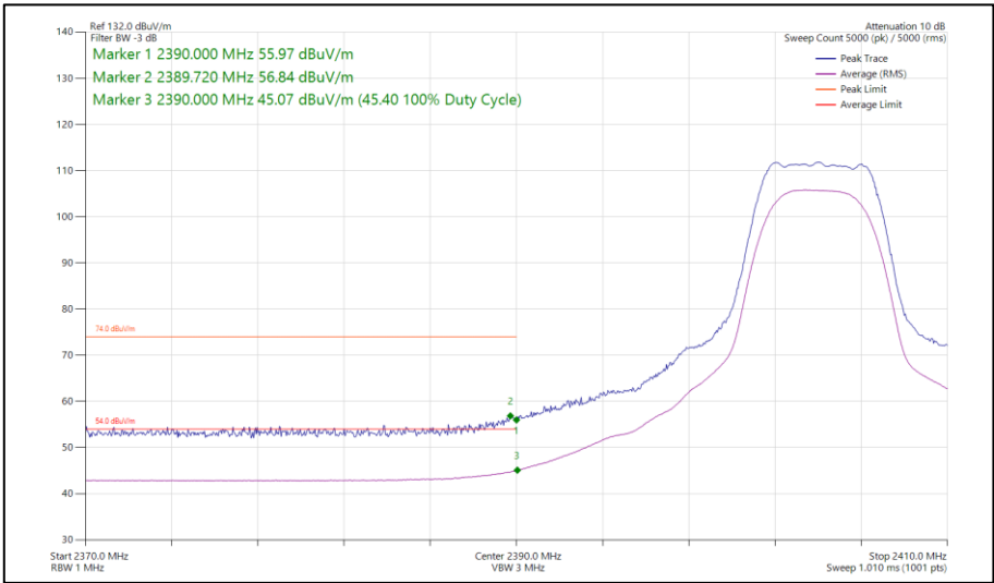
Figure 180 - Bluetooth XHDRPM8, MIMO, Core 0-2 - 2404 MHz Band Edge Frequency 2390 MHz
