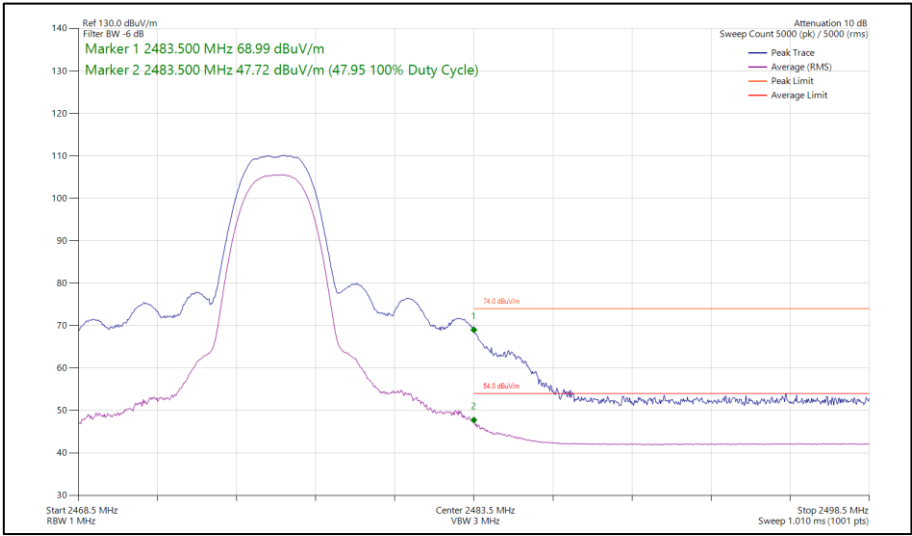
Figure 187 - Bluetooth HDT3, MIMO, Core 0-2 - 2476 MHz Band Edge Frequency 2483.5 MHz
