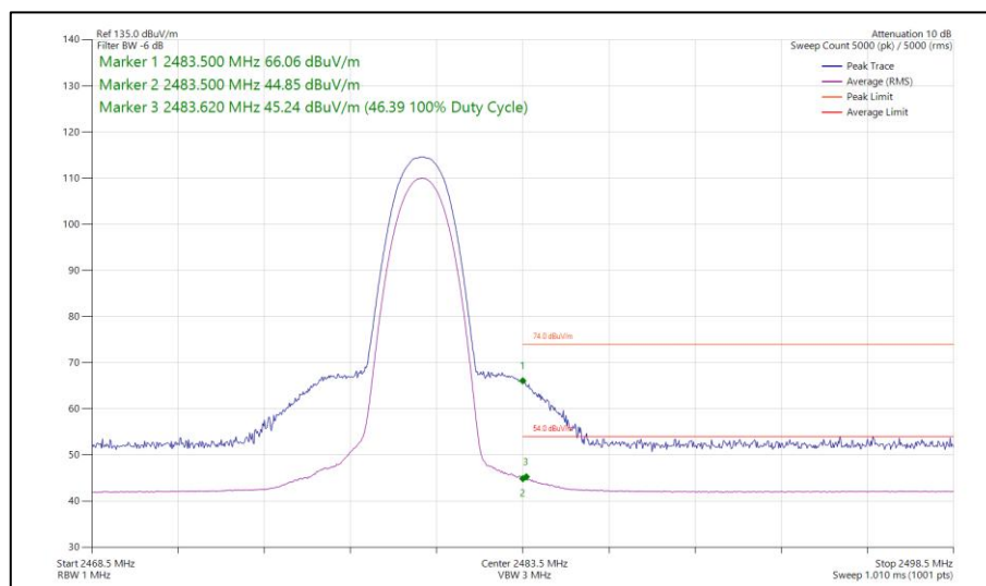
Figure 182 - Bluetooth 3DH5, MIMO, Core 0-2 - 2480 MHz Band Edge Frequency 2483.5 MHz
