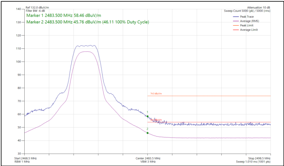
Figure 190 - Bluetooth HDRPS2, MIMO, Core 0-2 - 2476 MHz Band Edge Frequency 2483.5 MHz
