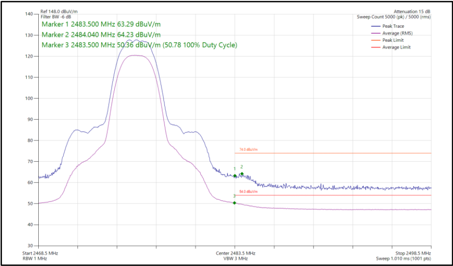
Figure 165 - Bluetooth HDT6, MIMO, Core 0-1 - 2476 MHz Band Edge Frequency 2483.5 MHz
