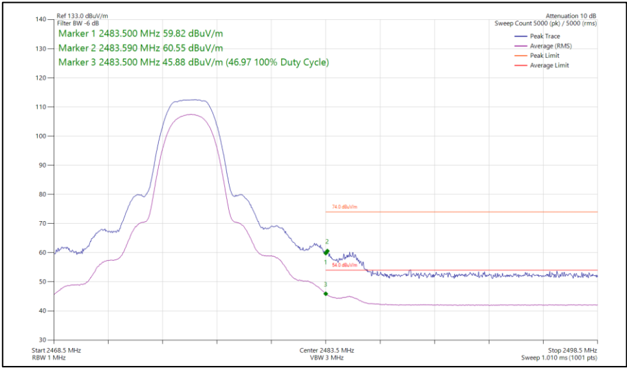
Figure 183 - Bluetooth HDR4, MIMO, Core 0-2 - 2476 MHz Band Edge Frequency 2483.5 MHz
