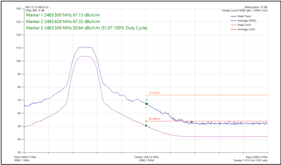
Figure 189 - Bluetooth HDT6, MIMO, Core 0-2 - 2476 MHz Band Edge Frequency 2483.5 MHz
