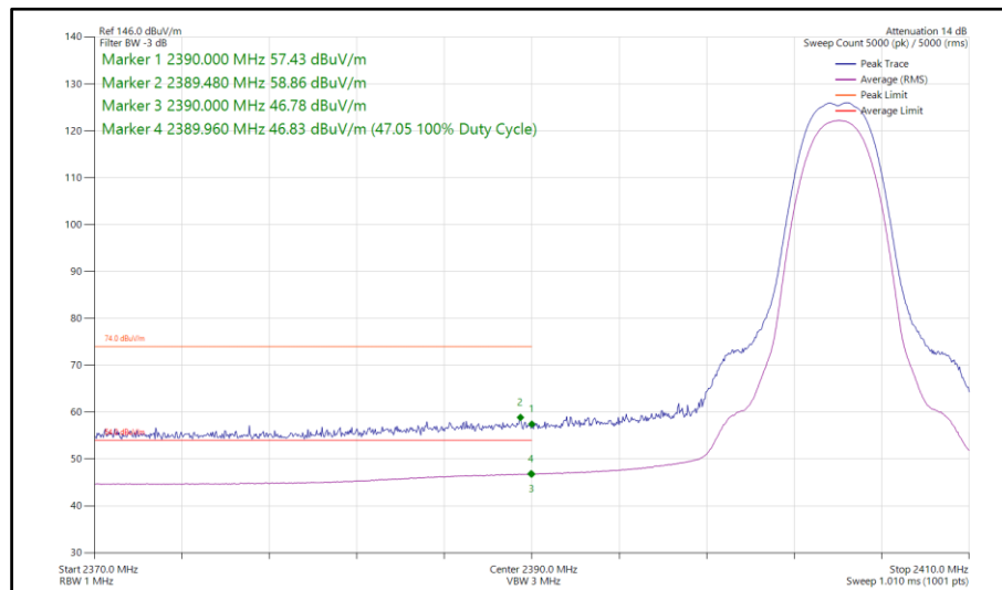
Figure 151 - Bluetooth HDT3, MIMO, Core 0-1 - 2404 MHz Band Edge Frequency 2390 MHz
