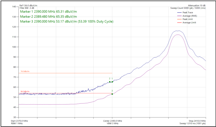
Figure 175 - Bluetooth HDT3, MIMO, Core 0-2 - 2404 MHz Band Edge Frequency 2390 MHz
