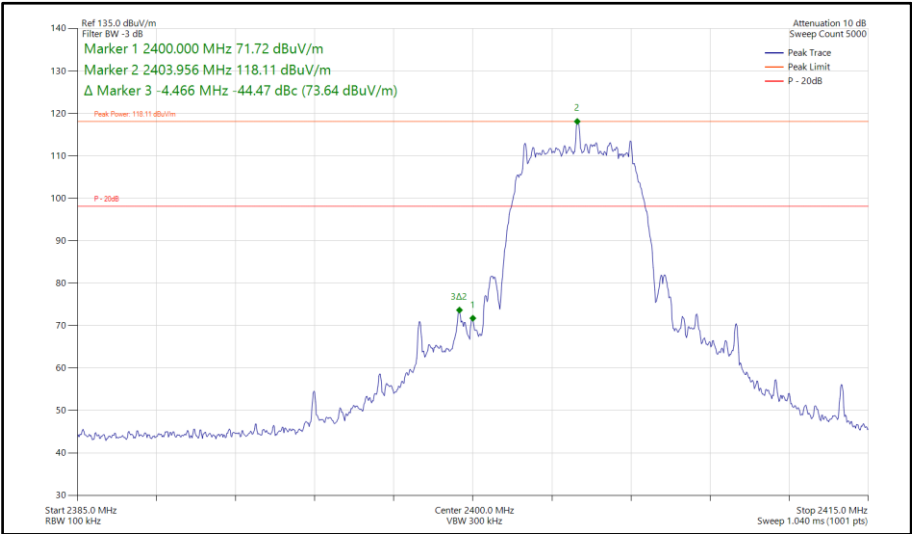
Figure 558 - Bluetooth XDRPM8, SISO, Core 1 - 2404 MHz Band Edge Frequency 2400 MHz
