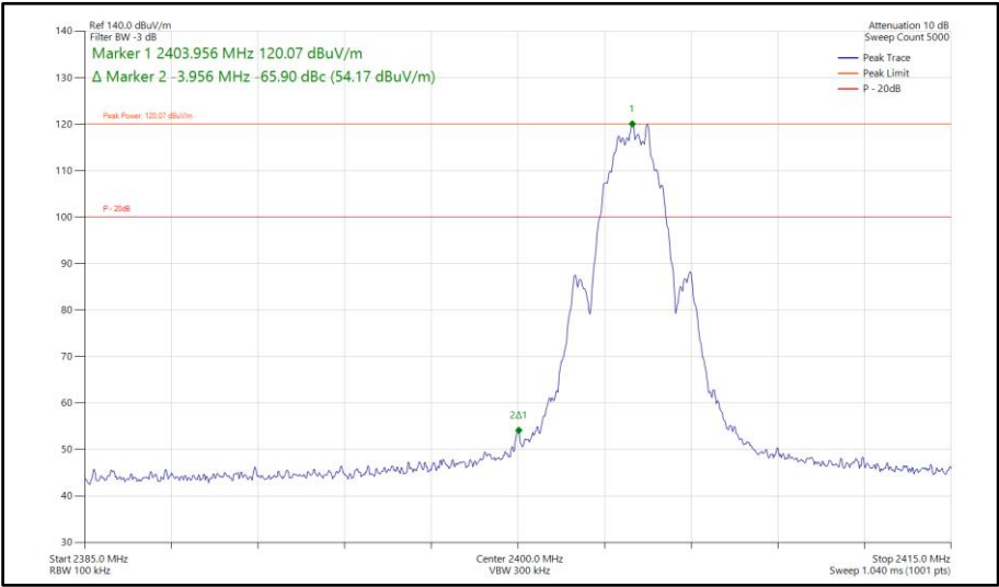
Figure 552 - Bluetooth LE2M, SISO, Core 1 - 2404 MHz Band Edge Frequency 2400 MHz
