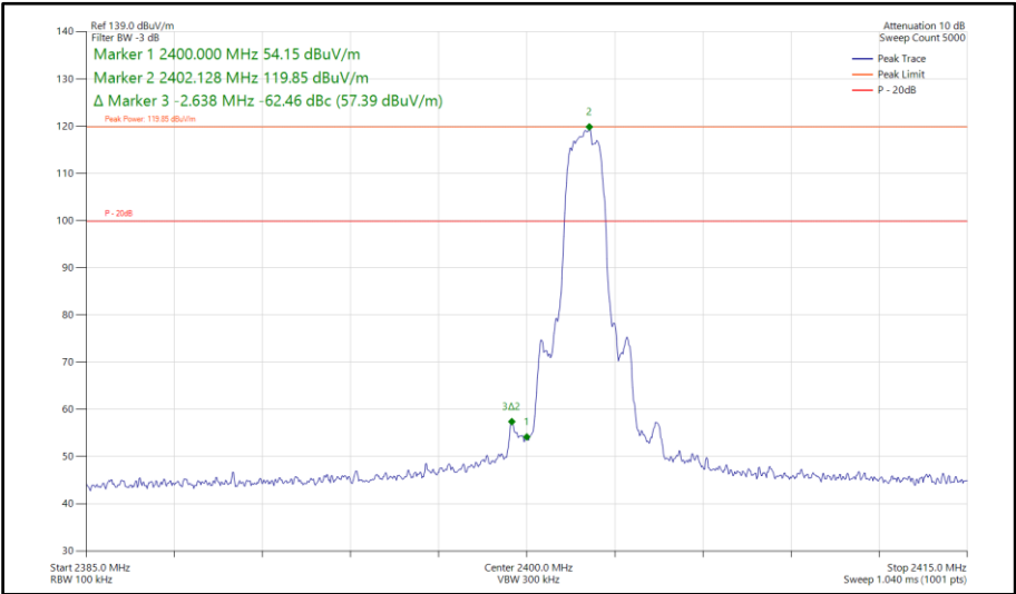
Figure 536 - Bluetooth 3DH5, SISO, Core 0 - 2402 MHz Band Edge Frequency 2400 MHz
