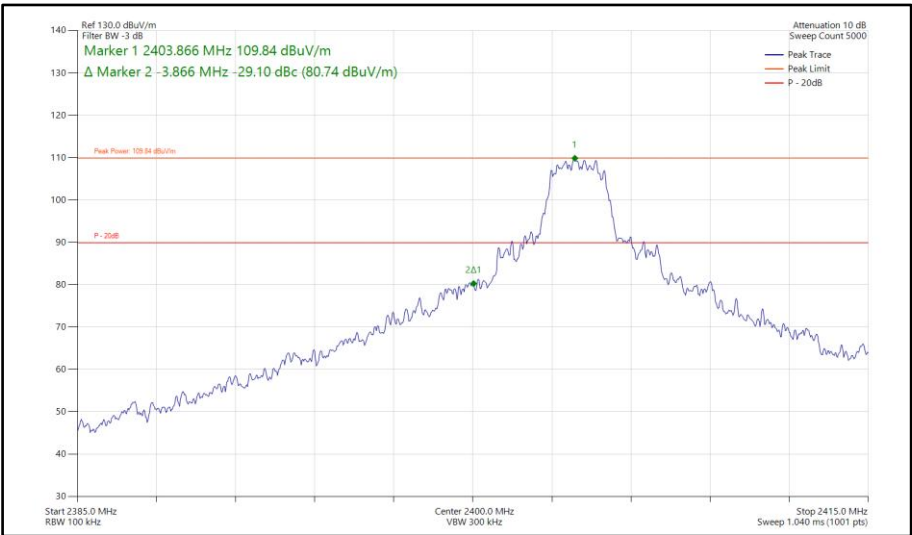
Figure 517 - Bluetooth HDT3, SISO, Core 2 - 2404 MHz Band Edge Frequency 2400 MHz
