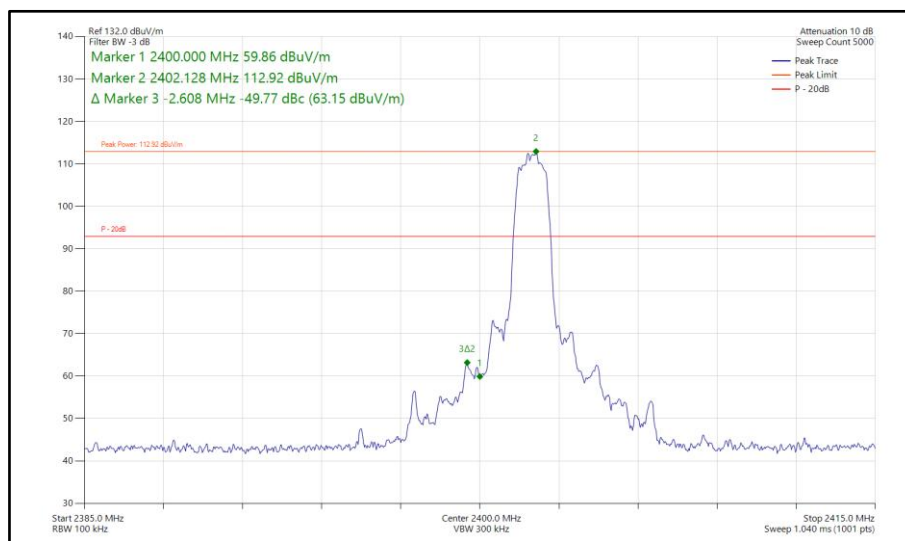
Figure 571 - Bluetooth 2DH5, MIMO, Core 0-2 - 2402 MHz Band Edge Frequency 2400 MHz
