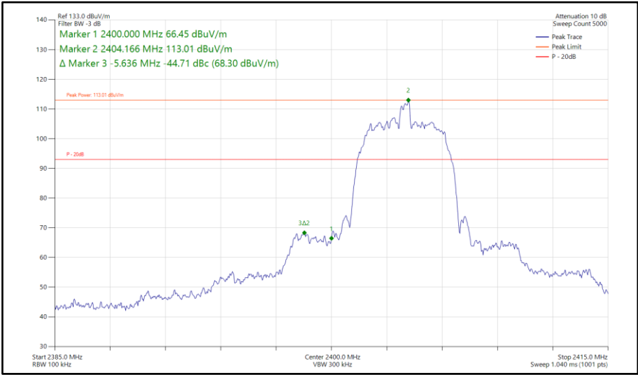
Figure 586 - Bluetooth HDR8, MIMO, Core 1-2 - 2404 MHz Band Edge Frequency 2400 MHz
