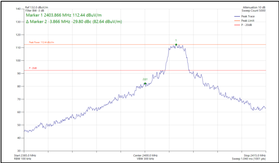
Figure 577 - Bluetooth HDT3, MIMO, Core 0-2 - 2404 MHz Band Edge Frequency 2400 MHz
