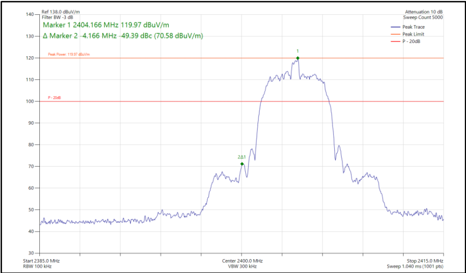
Figure 538 - Bluetooth HDR8, SISO, Core 0 - 2404 MHz Band Edge Frequency 2400 MHz
