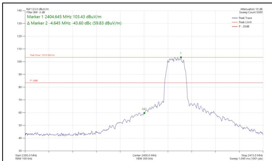
Figure 505 - Bluetooth HDT3, SISO, Core 1 - 2404 MHz Band Edge Frequency 2400 MHz
