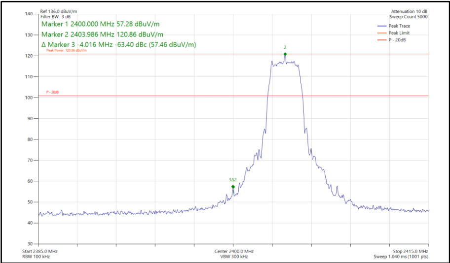
Figure 544 - Bluetooth HDRPS2, SISO, Core 0 - 2404 MHz Band Edge Frequency 2400 MHz
