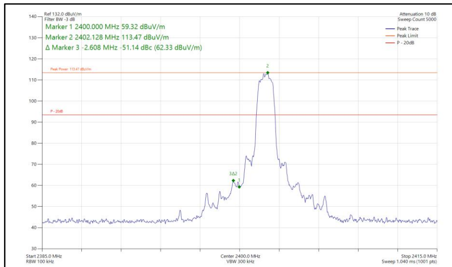
Figure 583 - Bluetooth 2DH5, MIMO, Core 1-2 - 2402 MHz Band Edge Frequency 2400 MHz
