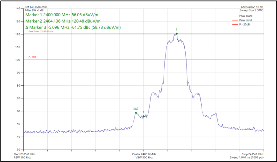
Figure 549 - Bluetooth HDR4, SISO, Core 1 - 2404 MHz Band Edge Frequency 2400 MHz
