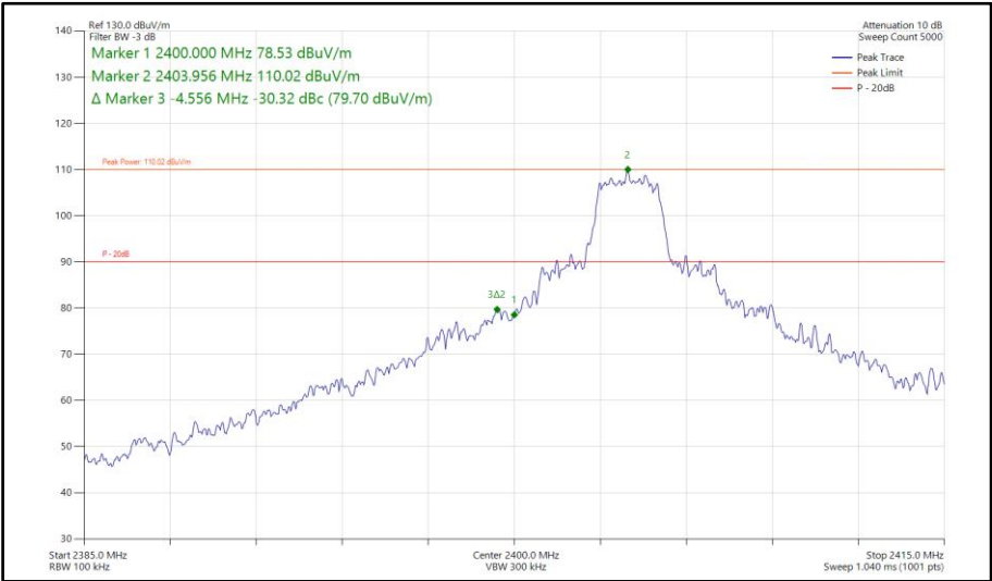
Figure 518 - Bluetooth HDT4, SISO, Core 2 - 2404 MHz Band Edge Frequency 2400 MHz
