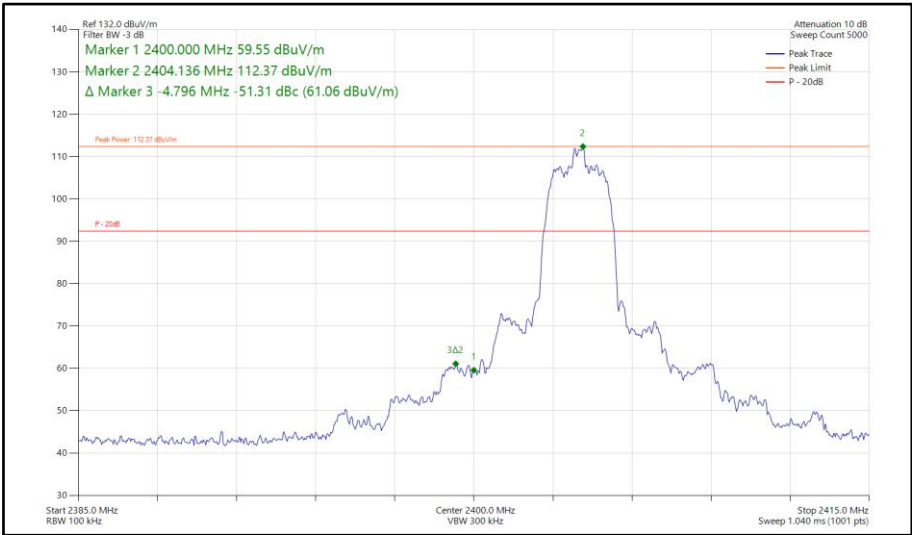
Figure 573 - Bluetooth HDR4, MIMO, Core 0-2 - 2404 MHz Band Edge Frequency 2400 MHz
