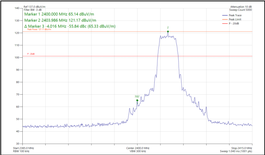
Figure 556 - Bluetooth HDRPS2, SISO, Core 1 - 2404 MHz Band Edge Frequency 2400 MHz
