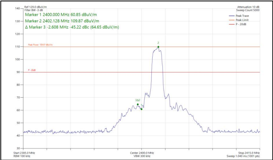
Figure 512 - Bluetooth 3DH5, SISO, Core 2 - 2402 MHz Band Edge Frequency 2400 MHz
