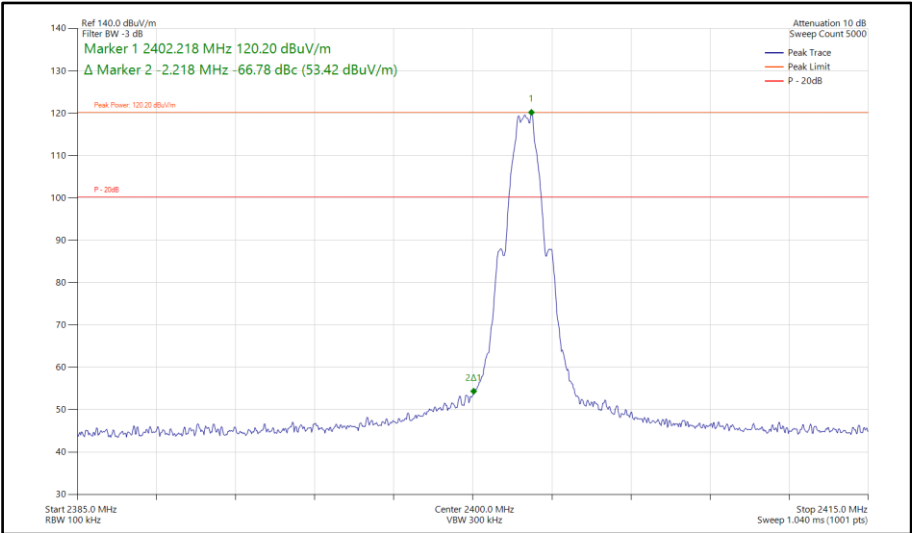
Figure 539 - Bluetooth LE1M, SISO, Core 0 - 2402 MHz Band Edge Frequency 2400 MHz
