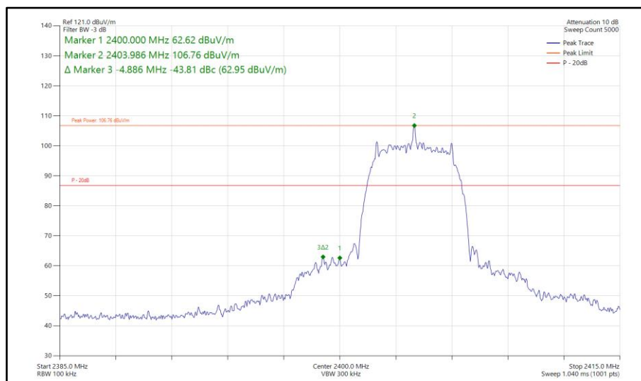
Figure 581 - Bluetooth HDRPM12, MIMO, Core 0-2 - 2404 MHz Band Edge Frequency 2400 MHz
