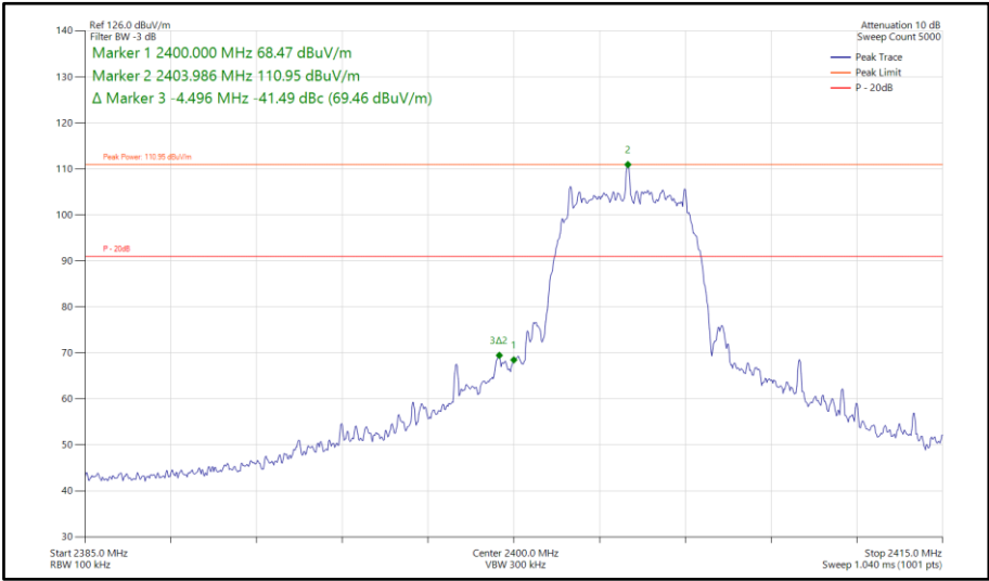
Figure 582 - Bluetooth XHDRPM8, MIMO, Core 0-2 - 2404 MHz Band Edge Frequency 2400 MHz
