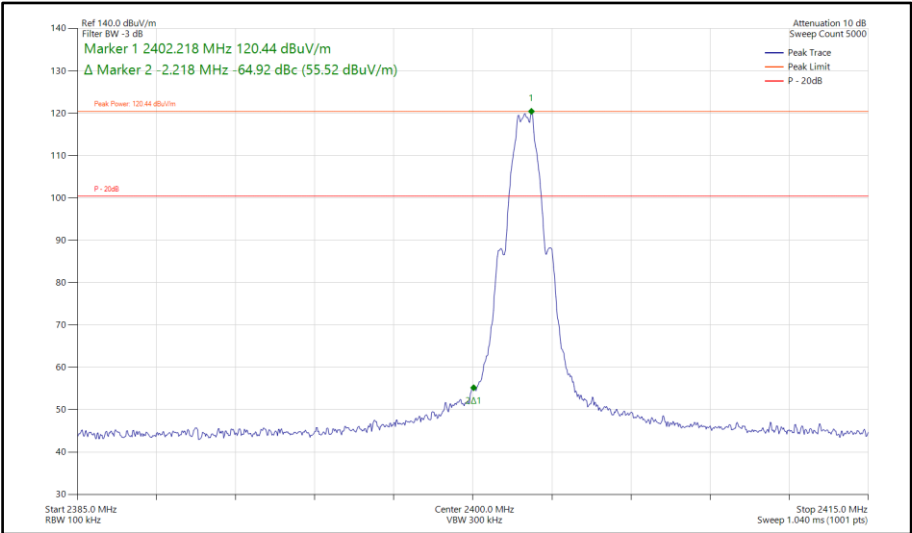
Figure 551 - Bluetooth LE1M, SISO, Core 1 - 2402 MHz Band Edge Frequency 2400 MHz
