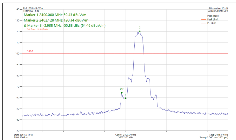
Figure 547 - Bluetooth 2DH5, SISO, Core 1 - 2402 MHz Band Edge Frequency 2400 MHz
