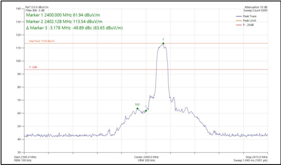
Figure 584 - Bluetooth 3DH5, MIMO, Core 1-2 - 2402 MHz Band Edge Frequency 2400 MHz
