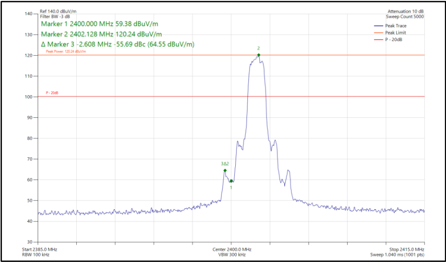
Figure 548 - Bluetooth 3DH5, SISO, Core 1 - 2402 MHz Band Edge Frequency 2400 MHz
