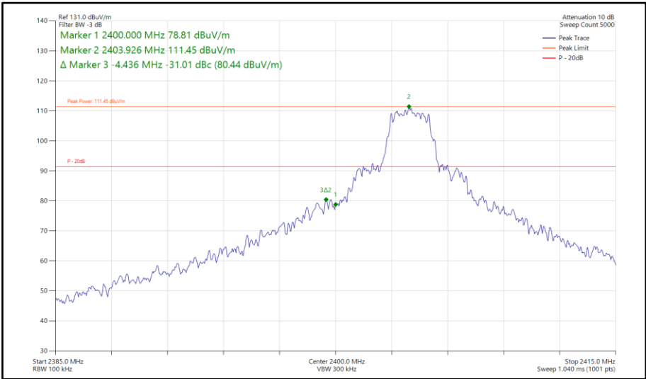
Figure 579 - Bluetooth HDT6, MIMO, Core 0-2 - 2404 MHz Band Edge Frequency 2400 MHz
