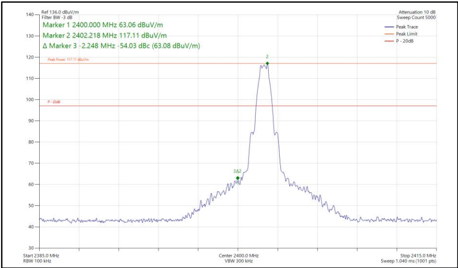
Figure 587 - Bluetooth LE1M, MIMO, Core 1-2 - 2402 MHz Band Edge Frequency 2400 MHz
