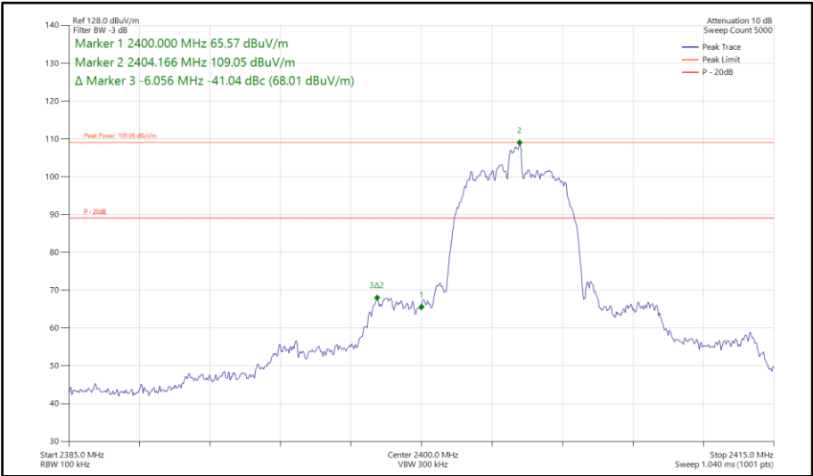
Figure 514 - Bluetooth HDR8, SISO, Core 2 - 2404 MHz Band Edge Frequency 2400 MHz
