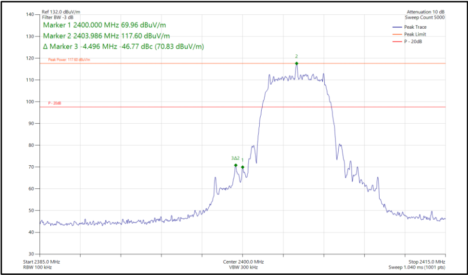
Figure 546 - Bluetooth XHDRPM8, SISO, Core 0 - 2404 MHz Band Edge Frequency 2400 MHz
