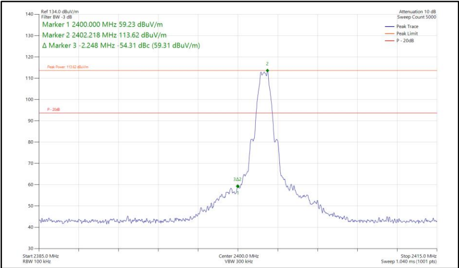
Figure 515 - Bluetooth LE1M, SISO, Core 2 - 2402 MHz Band Edge Frequency 2400 MHz
