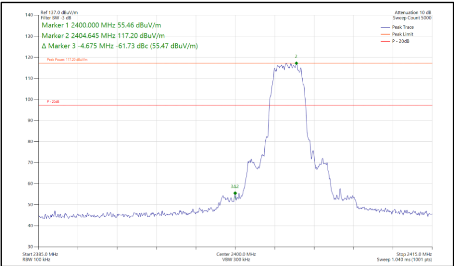
Figure 541 - Bluetooth HDT3, SISO, Core 0 - 2404 MHz Band Edge Frequency 2400 MHz
