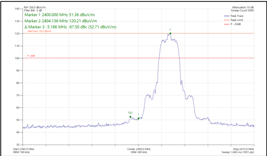
Figure 537 - Bluetooth HDR4, SISO, Core 0 - 2404 MHz Band Edge Frequency 2400 MHz
