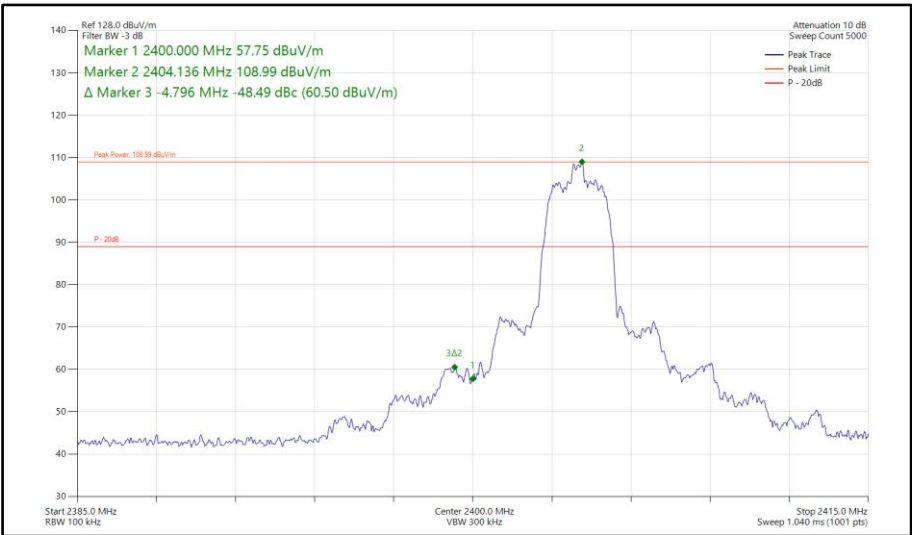
Figure 513 - Bluetooth HDR4, SISO, Core 2 - 2404 MHz Band Edge Frequency 2400 MHz
