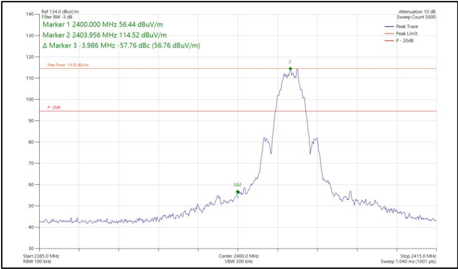
Figure 576 - Bluetooth LE2M, MIMO, Core 0-2 - 2404 MHz Band Edge Frequency 2400 MHz
