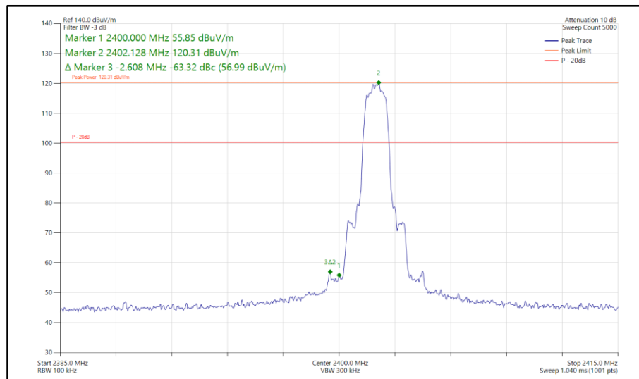
Figure 535 - Bluetooth 2DH5, SISO, Core 0 - 2402 MHz Band Edge Frequency 2400 MHz
