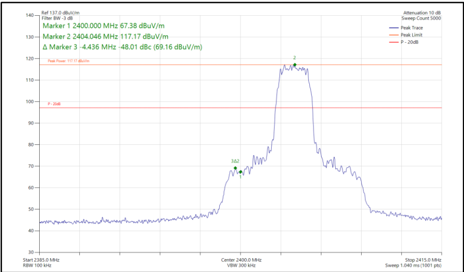
Figure 555 - Bluetooth HDT6, SISO, Core 1 - 2404 MHz Band Edge Frequency 2400 MHz
