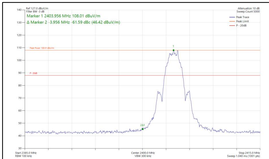
Figure 504 - Bluetooth LE2M, SISO, Core 1 - 2404 MHz Band Edge Frequency 2400 MHz
