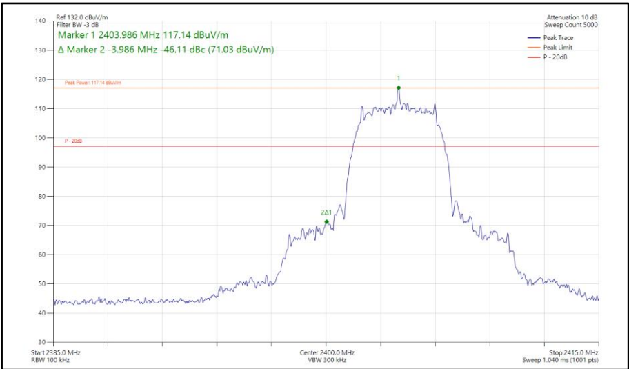
Figure 557 - Bluetooth HDRPM12, SISO, Core 1 - 2404 MHz Band Edge Frequency 2400 MHz
