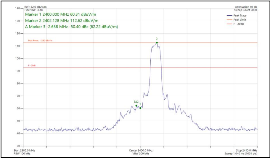
Figure 572 - Bluetooth 3DH5, MIMO, Core 0-2 - 2402 MHz Band Edge Frequency 2400 MHz
