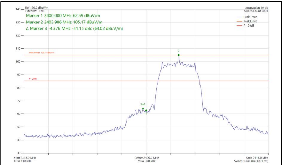
Figure 521 - Bluetooth HDRPM12, SISO, Core 2 - 2404 MHz Band Edge Frequency 2400 MHz
