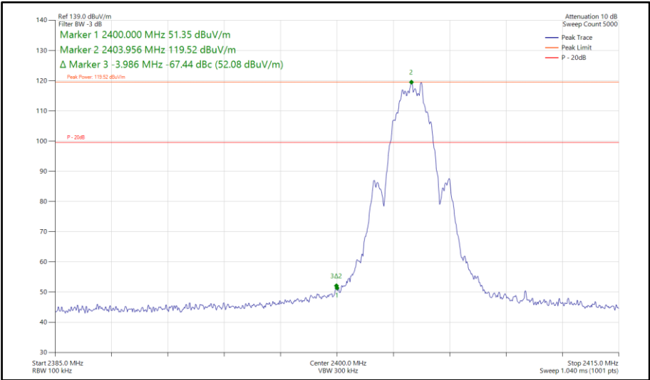
Figure 540 - Bluetooth LE2M, SISO, Core 0 - 2404 MHz Band Edge Frequency 2400 MHz
