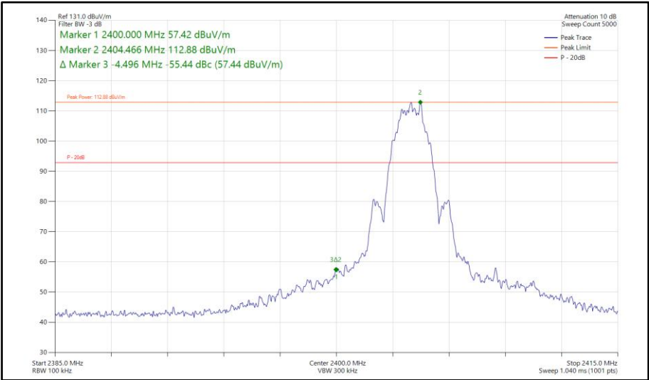
Figure 516 - Bluetooth LE2M, SISO, Core 2 - 2404 MHz Band Edge Frequency 2400 MHz
