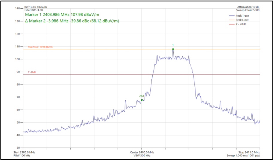
Figure 522 - Bluetooth XHDRPM8, SISO, Core 2 - 2404 MHz Band Edge Frequency 2400 MHz
