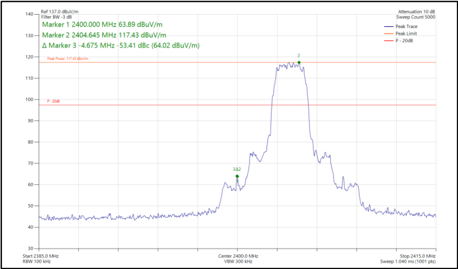
Figure 553 - Bluetooth HDT3, SISO, Core 1 - 2404 MHz Band Edge Frequency 2400 MHz
