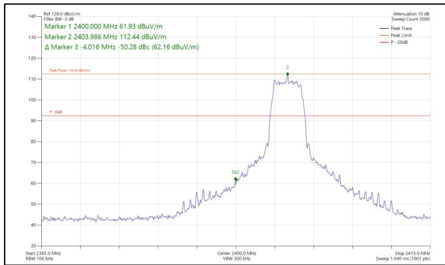
Figure 580 - Bluetooth HDRPS2, MIMO, Core 0-2 - 2404 MHz Band Edge Frequency 2400 MHz
