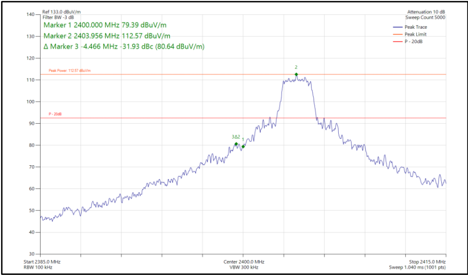
Figure 578 - Bluetooth HDT4, MIMO, Core 0-2 - 2404 MHz Band Edge Frequency 2400 MHz
