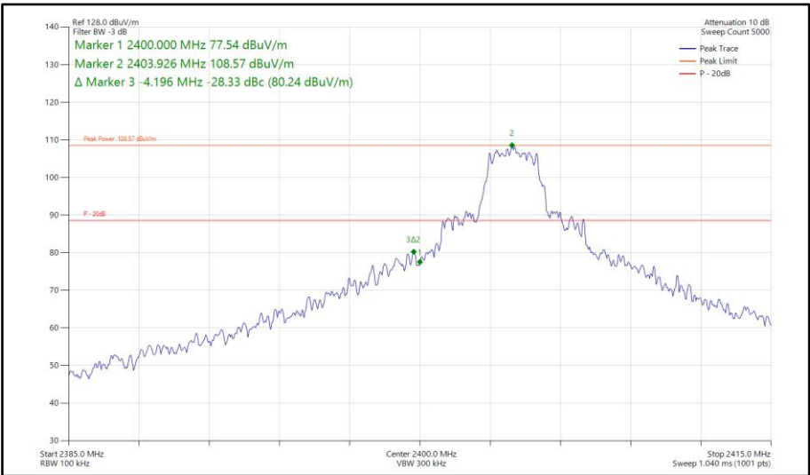
Figure 519 - Bluetooth HDT6, SISO, Core 2 - 2404 MHz Band Edge Frequency 2400 MHz
