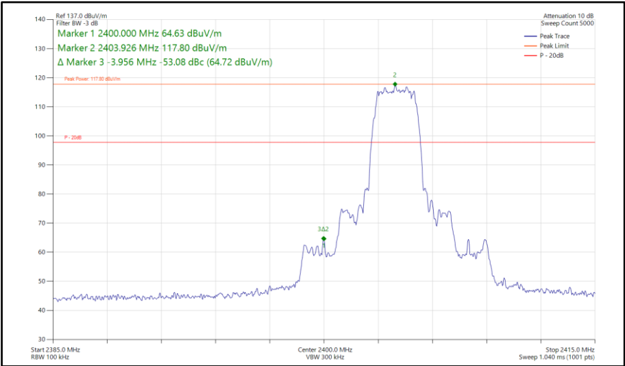
Figure 554 - Bluetooth HDT4, SISO, Core 1 - 2404 MHz Band Edge Frequency 2400 MHz
