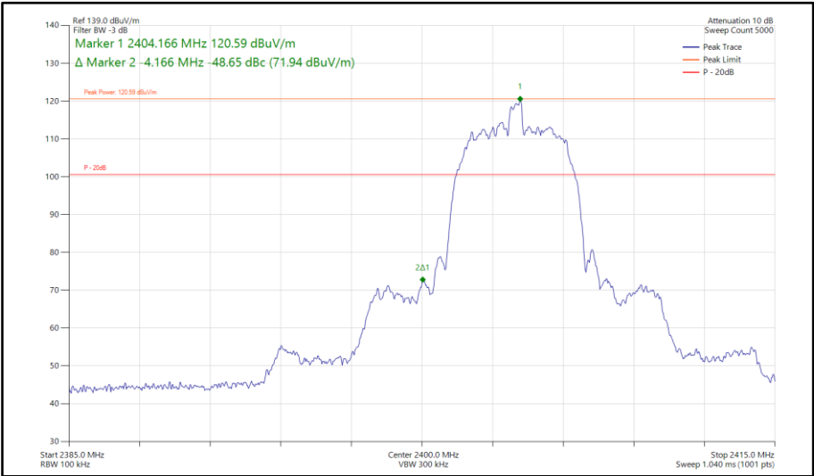
Figure 550 - Bluetooth HDR8, SISO, Core 1 - 2404 MHz Band Edge Frequency 2400 MHz
