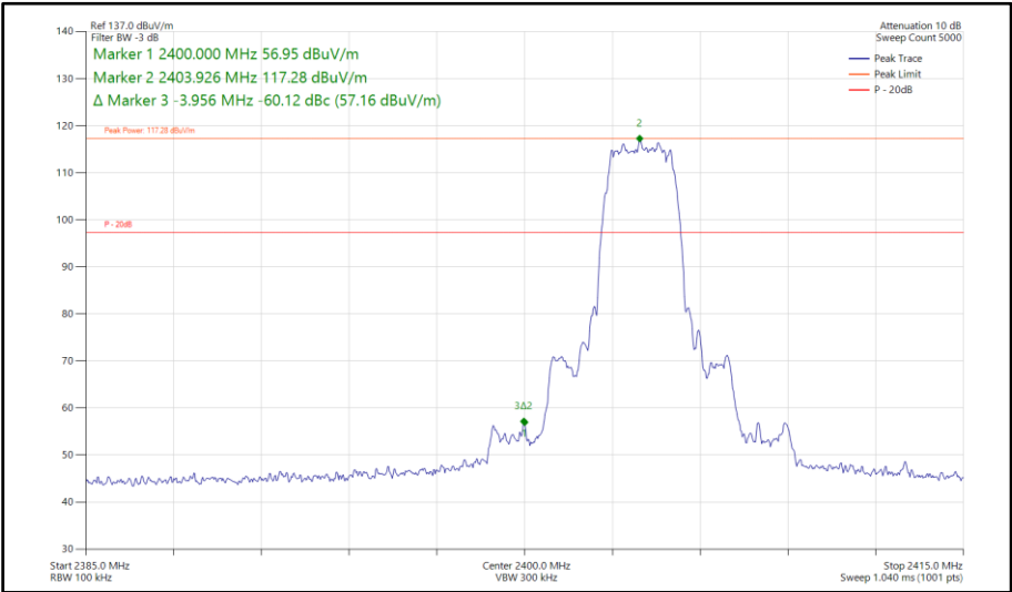
Figure 542 - Bluetooth HDT4, SISO, Core 0 - 2404 MHz Band Edge Frequency 2400 MHz
