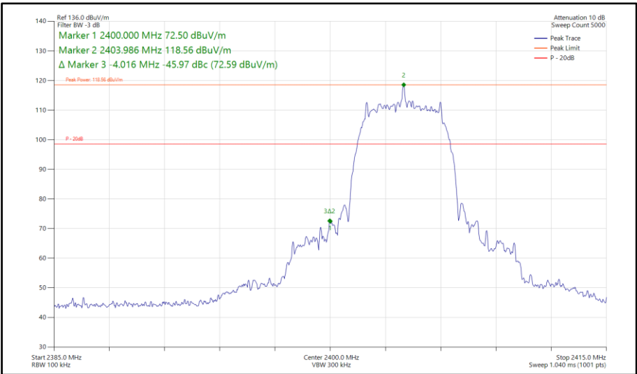
Figure 545 - Bluetooth HDRPM12, SISO, Core 0 - 2404 MHz Band Edge Frequency 2400 MHz
