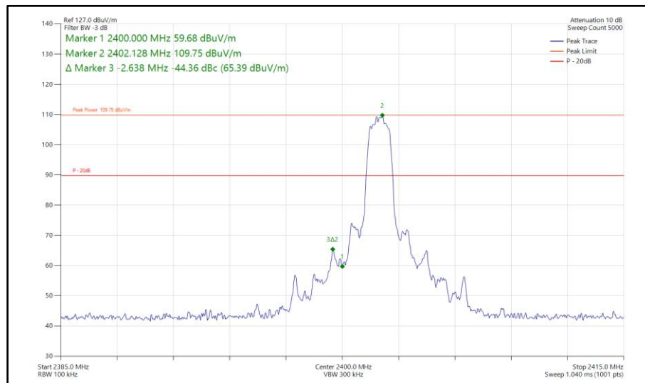
Figure 511 - Bluetooth 2DH5, SISO, Core 2 - 2402 MHz Band Edge Frequency 2400 MHz
