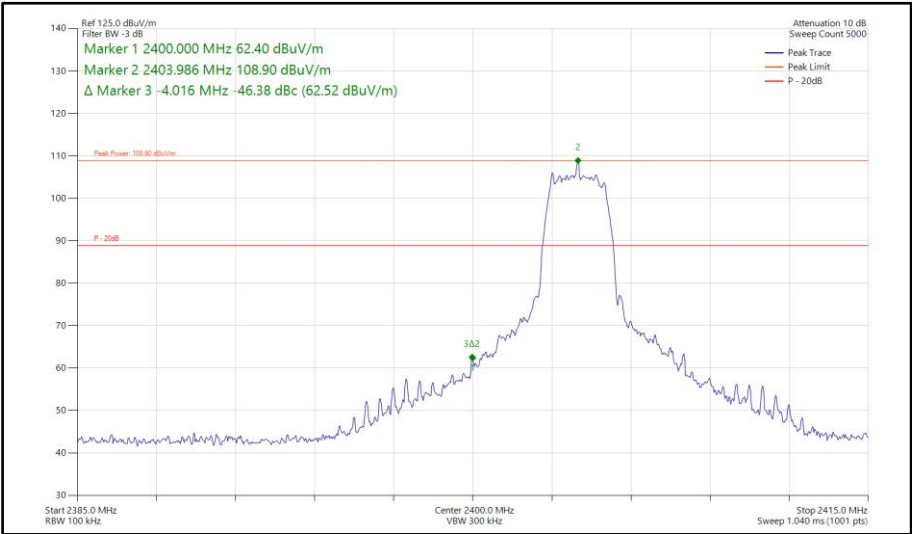
Figure 520 - Bluetooth HDRPS2, SISO, Core 2 - 2404 MHz Band Edge Frequency 2400 MHz
