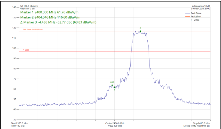
Figure 543 - Bluetooth HDT6, SISO, Core 0 - 2404 MHz Band Edge Frequency 2400 MHz
