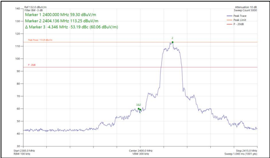
Figure 585 - Bluetooth HDR4, MIMO, Core 1-2 - 2404 MHz Band Edge Frequency 2400 MHz
