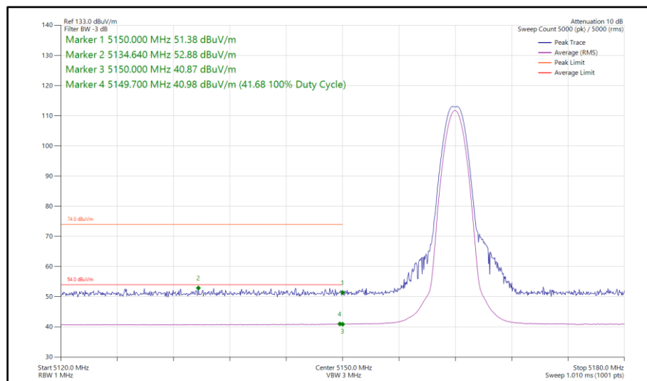
Figure 66 - LE1M, MIMO, Core 0-1 - 5162 MHz Band Edge Frequency 5150 MHz
