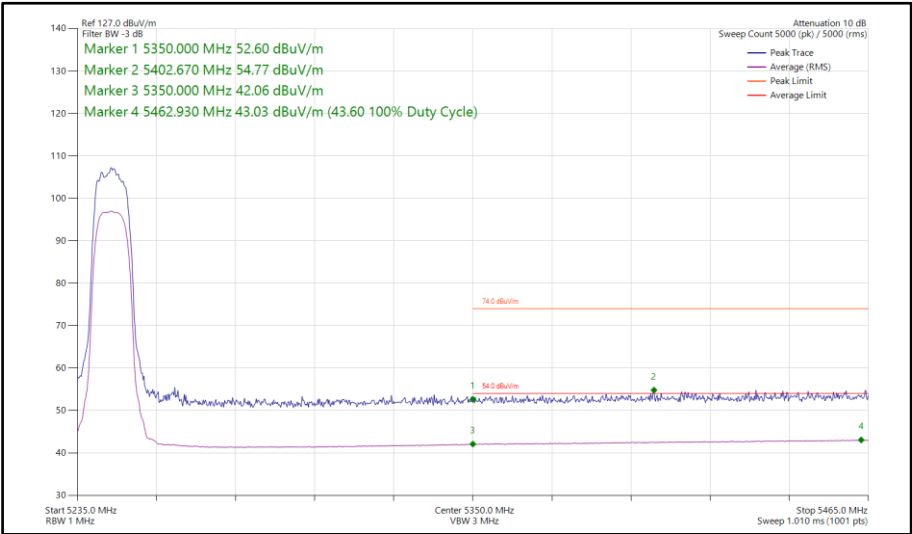
Figure 91 - HDRPL24, MIMO, Core 0-1 - 5245 MHz Band Edge Frequency 5350 MHz
