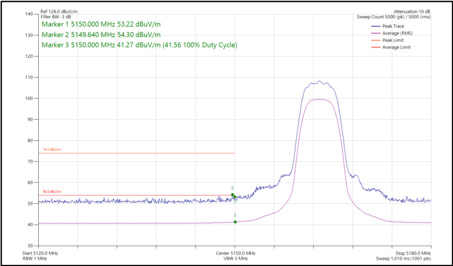
Figure 72 - HDRPM12, MIMO, Core 0-1 - 5163 MHz Band Edge Frequency 5150 MHz
