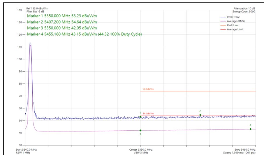
Figure 80 - DH5, MIMO, Core 0-1 - 5245 MHz Band Edge Frequency 5350 MHz
