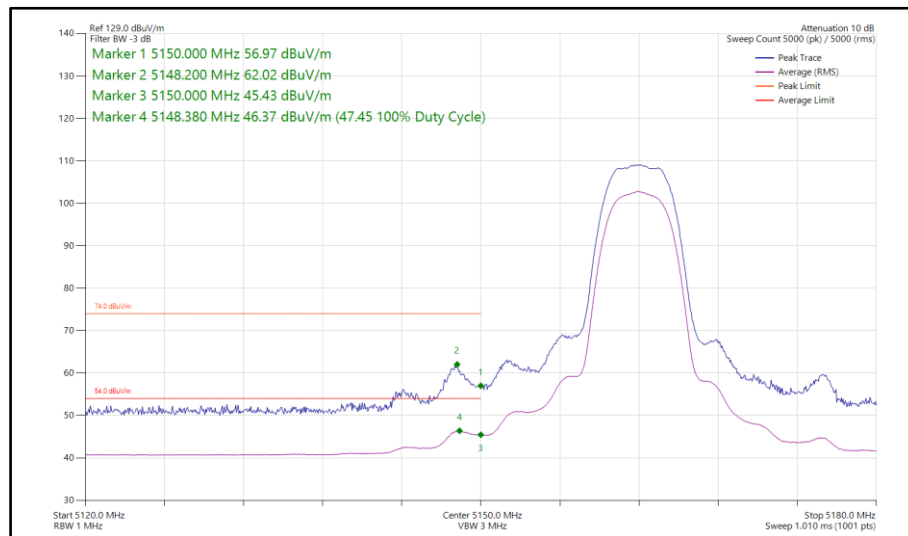
Figure 65 - HDR8, MIMO, Core 0-1 - 5162 MHz Band Edge Frequency 5150 MHz
