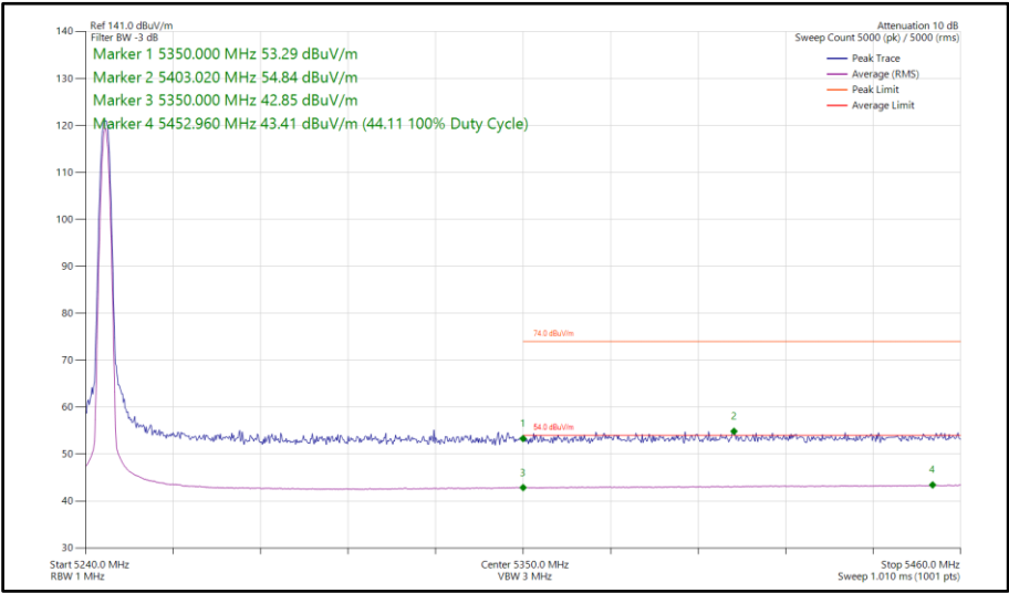
Figure 114 - LE1M, SISO, Core 0 - 5245 MHz Band Edge Frequency 5350 MHz
