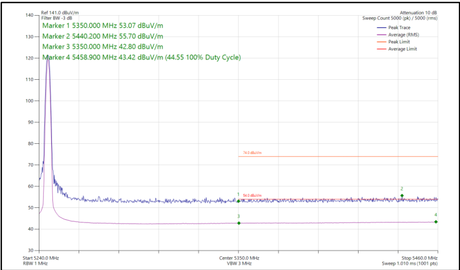
Figure 111 - DH5, SISO, Core 0 - 5245 MHz Band Edge Frequency 5350 MHz
