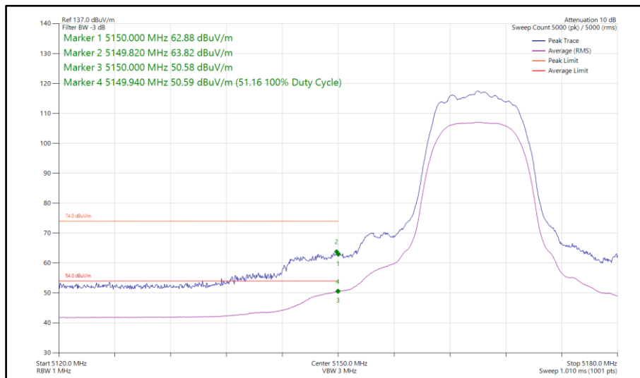
Figure 106 - HDRPL24, SISO, Core 0 - 5165 MHz Band Edge Frequency 5150 MHz
