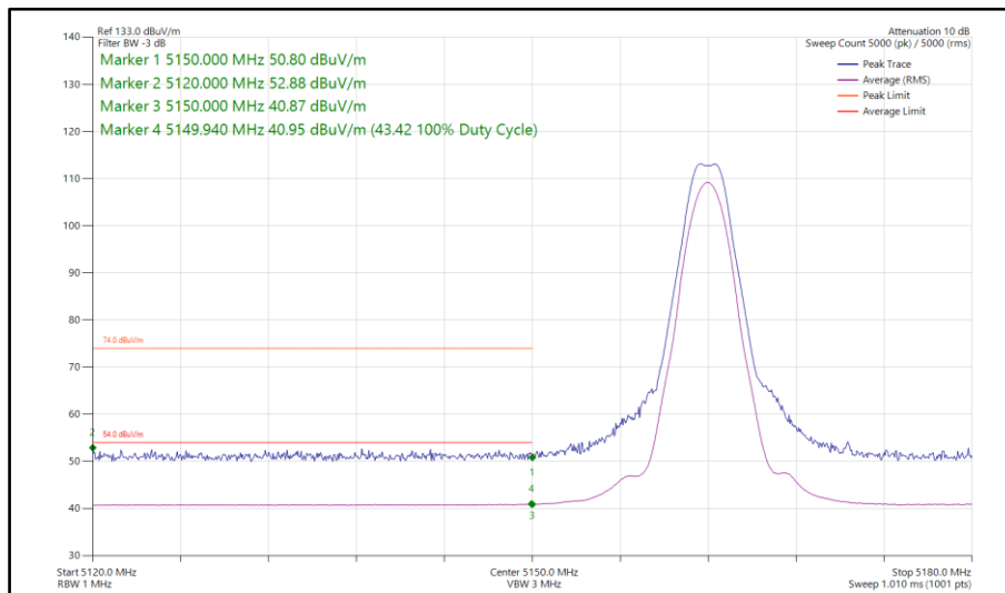
Figure 67 - LE2M, MIMO, Core 0-1 - 5162 MHz Band Edge Frequency 5150 MHz
