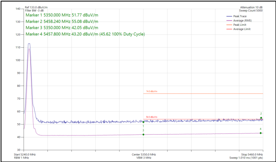
Figure 84 - LE2M, MIMO, Core 0-1 - 5245 MHz Band Edge Frequency 5350 MHz
