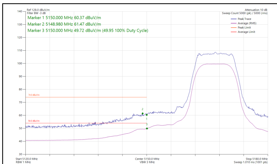
Figure 74 - HDRPL8, MIMO, Core 0-1 - 5167 MHz Band Edge Frequency 5150 MHz
