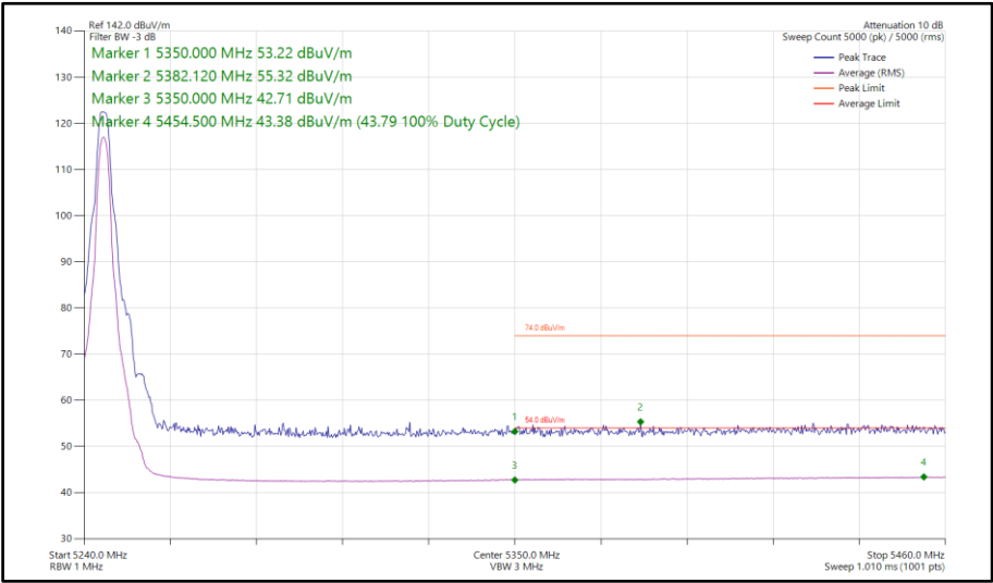
Figure 118 - HDT6, SISO, Core 0 - 5245 MHz Band Edge Frequency 5350 MHz
