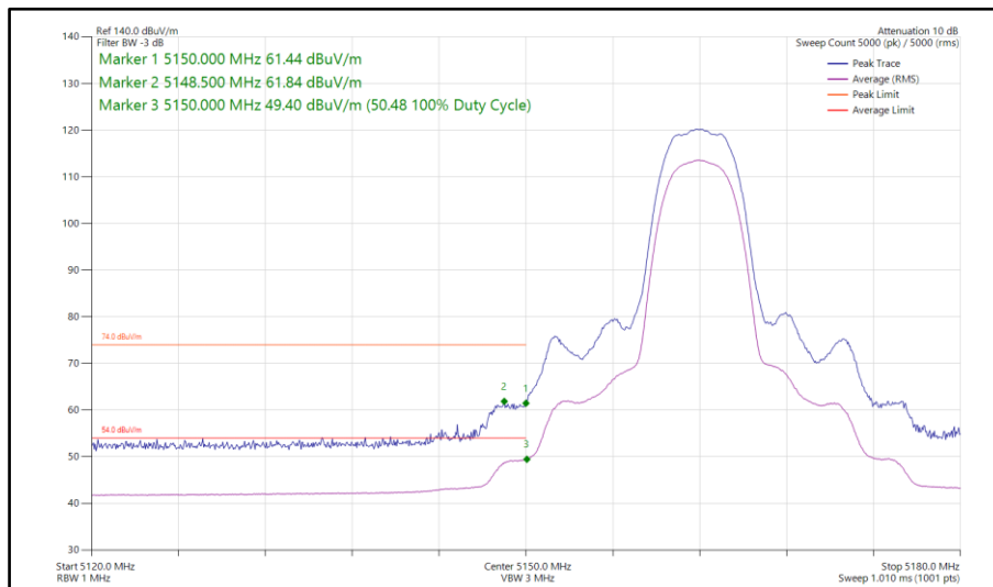
Figure 96 - HDR8, SISO, Core 0 - 5162 MHz Band Edge Frequency 5150 MHz
