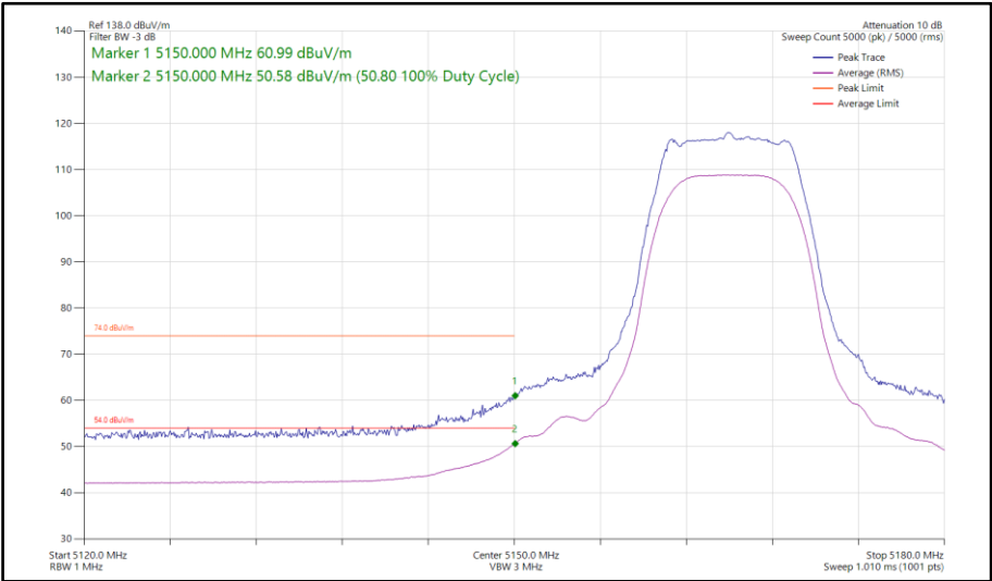
Figure 104 - HDRPL8, SISO, Core 0 - 5165 MHz Band Edge Frequency 5150 MHz
