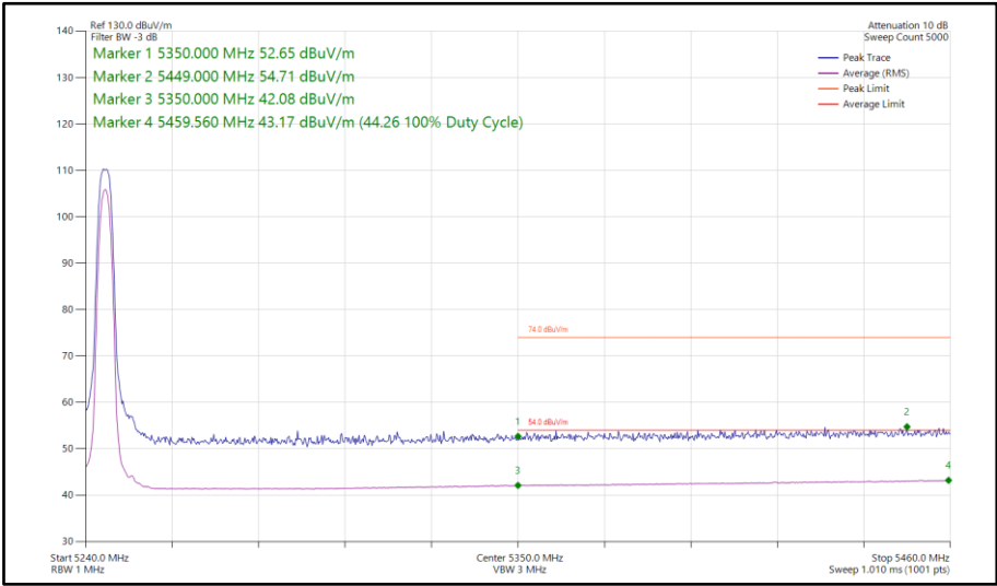
Figure 81 - HDR4, MIMO, Core 0-1 - 5245 MHz Band Edge Frequency 5350 MHz
