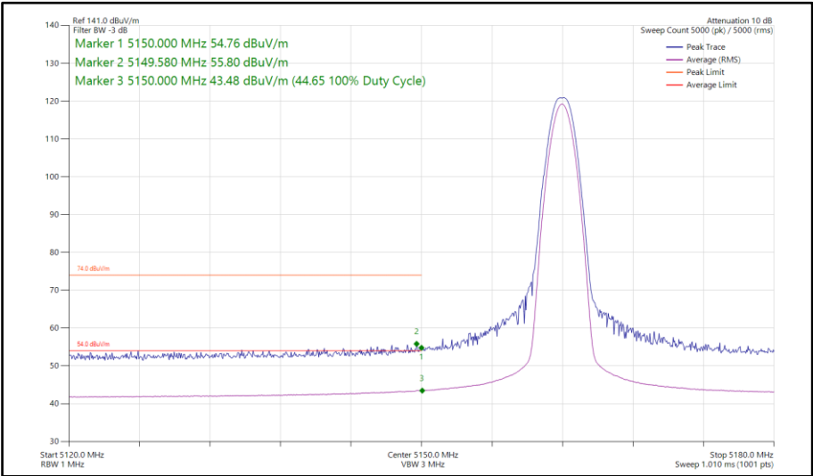
Figure 94 - DH5, SISO, Core 0 - 5162 MHz Band Edge Frequency 5150 MHz
