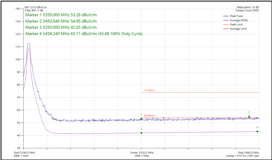
Figure 86 - HDT4, MIMO, Core 0-1 - 5245 MHz Band Edge Frequency 5350 MHz
