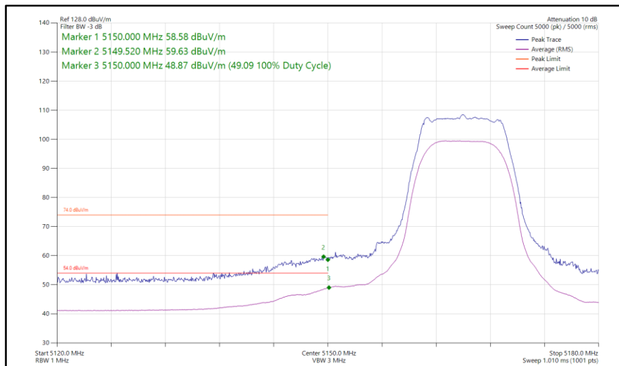
Figure 73 - HDRPL8, MIMO, Core 0-1 - 5165 MHz Band Edge Frequency 5150 MHz
