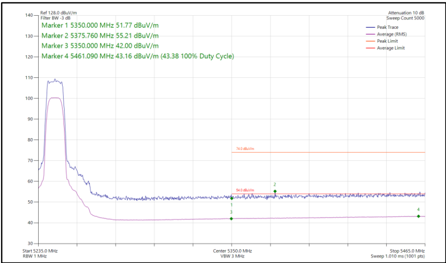
Figure 90 - HDRPL8, MIMO, Core 0-1 - 5245 MHz Band Edge Frequency 5350 MHz
