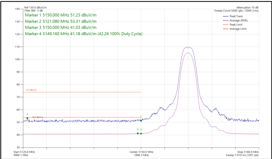
Figure 64 - HDR4, MIMO, Core 0-1 - 5162 MHz Band Edge Frequency 5150 MHz
