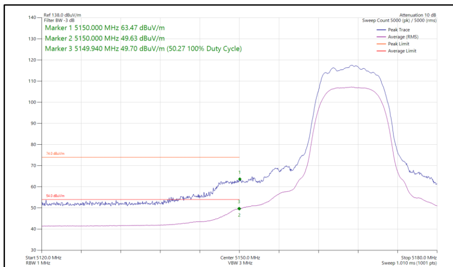
Figure 107 - HDRPL24, SISO, Core 0 - 5167 MHz Band Edge Frequency 5150 MHz
