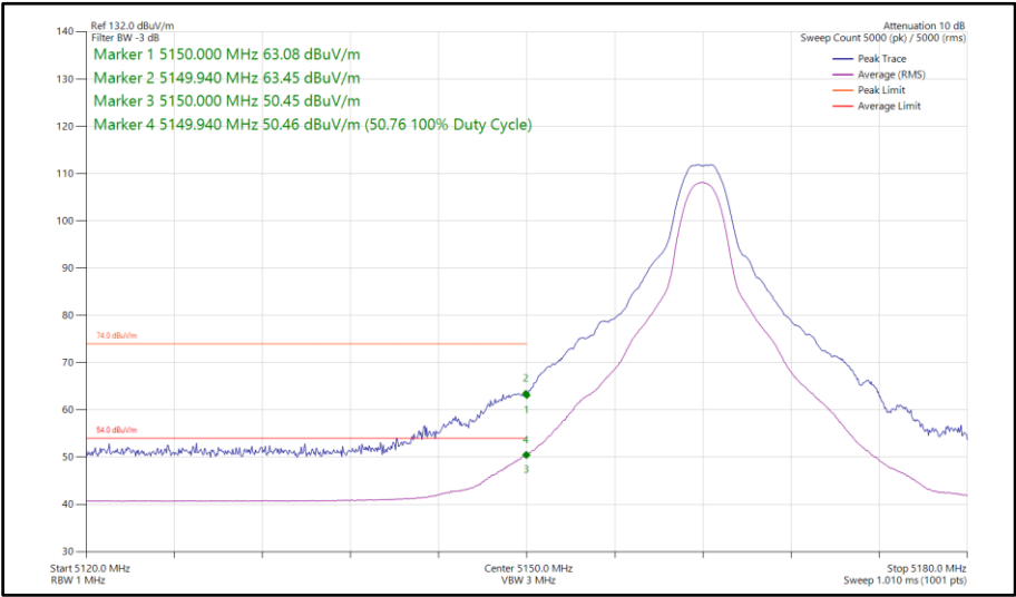
Figure 69 - HDT4, MIMO, Core 0-1 - 5162 MHz Band Edge Frequency 5150 MHz
