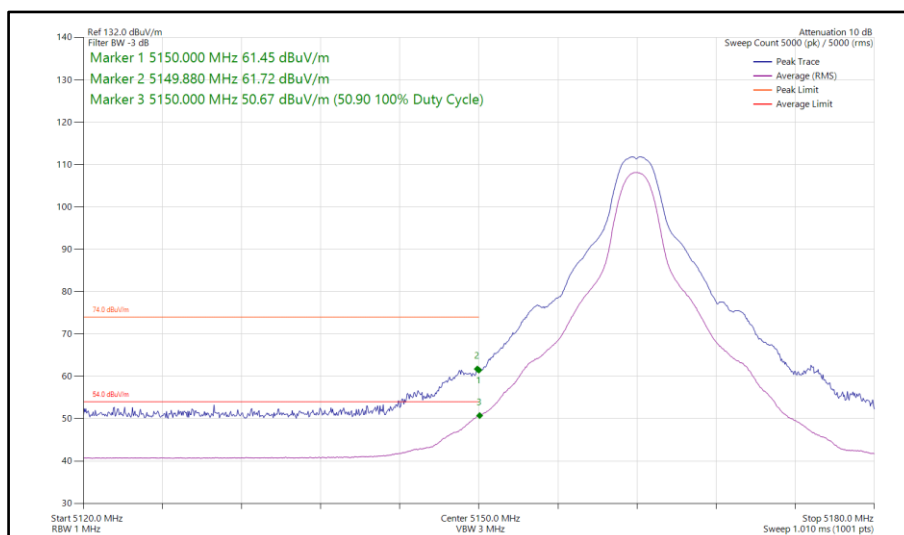
Figure 68 - HDT3, MIMO, Core 0-1 - 5162 MHz Band Edge Frequency 5150 MHz
