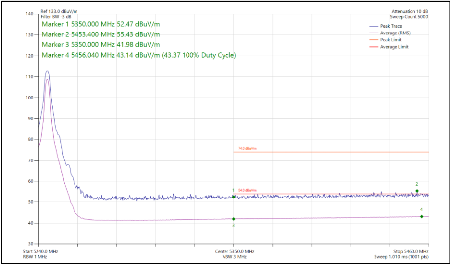
Figure 85 - HDT3, MIMO, Core 0-1 - 5245 MHz Band Edge Frequency 5350 MHz
