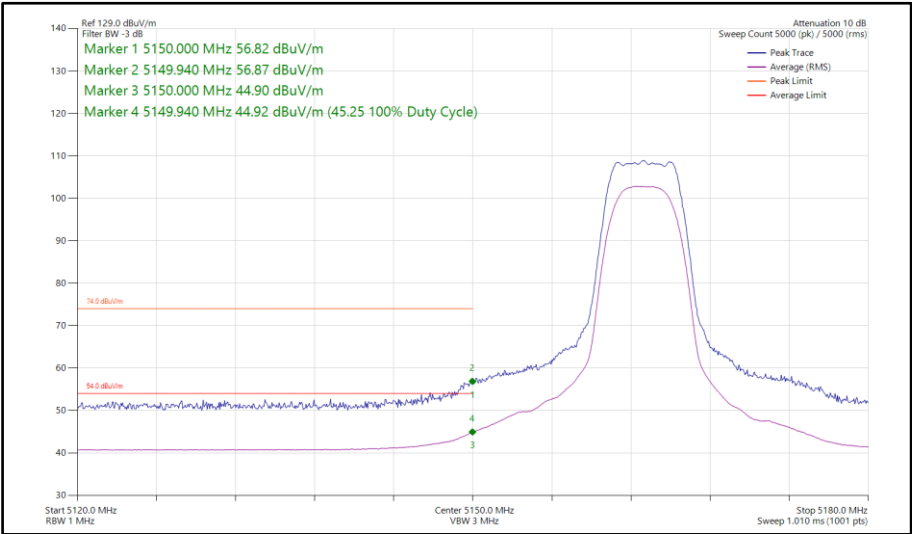
Figure 77 - XHDRPM8, MIMO, Core 0-1 - 5163 MHz Band Edge Frequency 5150 MHz
