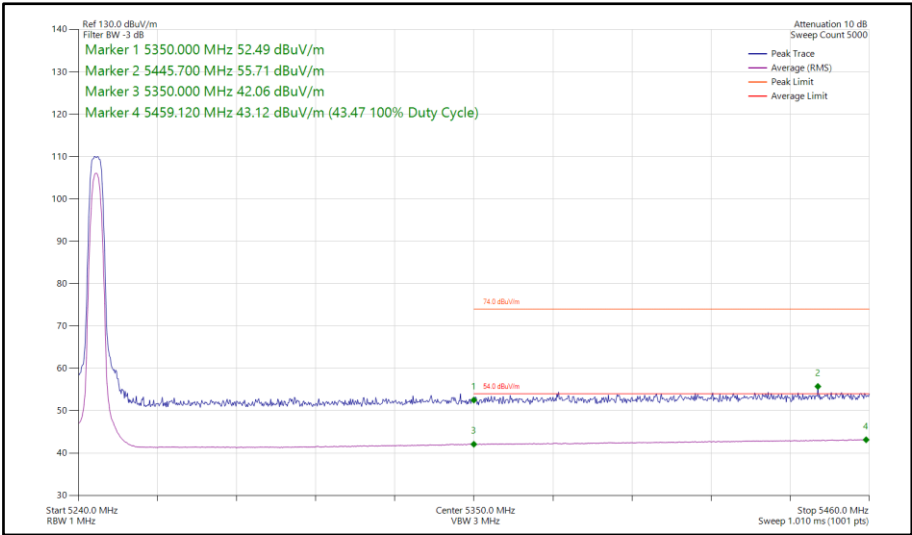
Figure 88 - HDRPS2, MIMO, Core 0-1 - 5245 MHz Band Edge Frequency 5350 MHz
