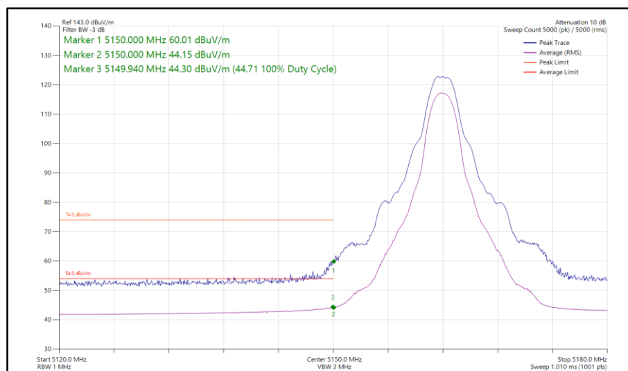
Figure 101 - HDT6, SISO, Core 0 - 5162 MHz Band Edge Frequency 5150 MHz
