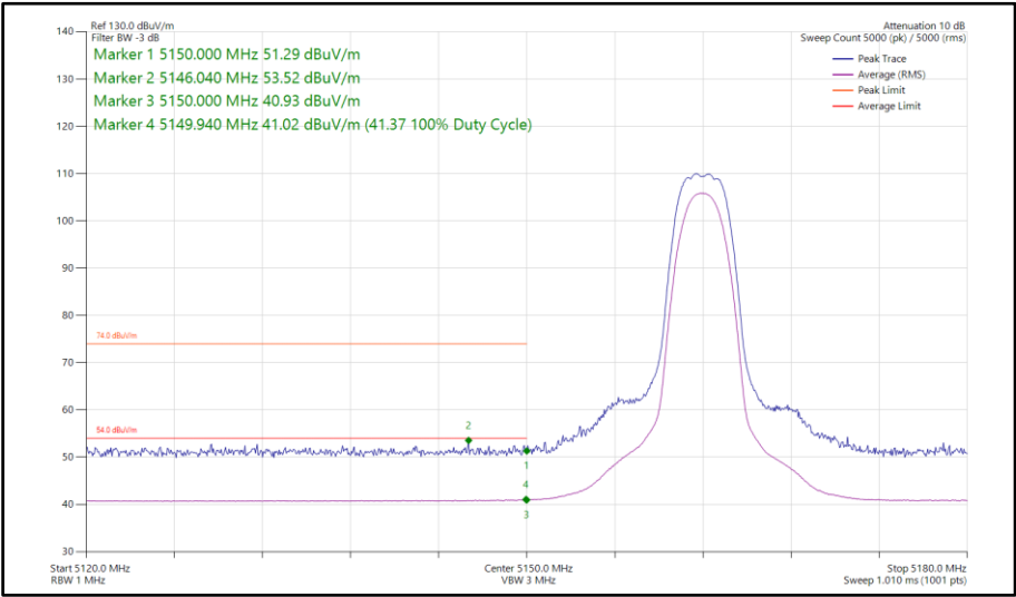
Figure 71 - HDRPS2, MIMO, Core 0-1 - 5162 MHz Band Edge Frequency 5150 MHz
