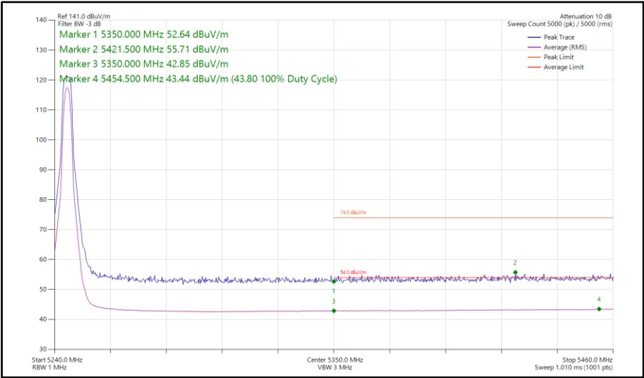
Figure 119 - HDRPS2, SISO, Core 0 - 5245 MHz Band Edge Frequency 5350 MHz
