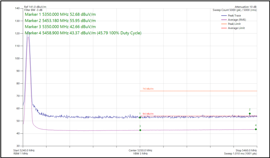
Figure 115 - LE2M, SISO, Core 0 - 5245 MHz Band Edge Frequency 5350 MHz
