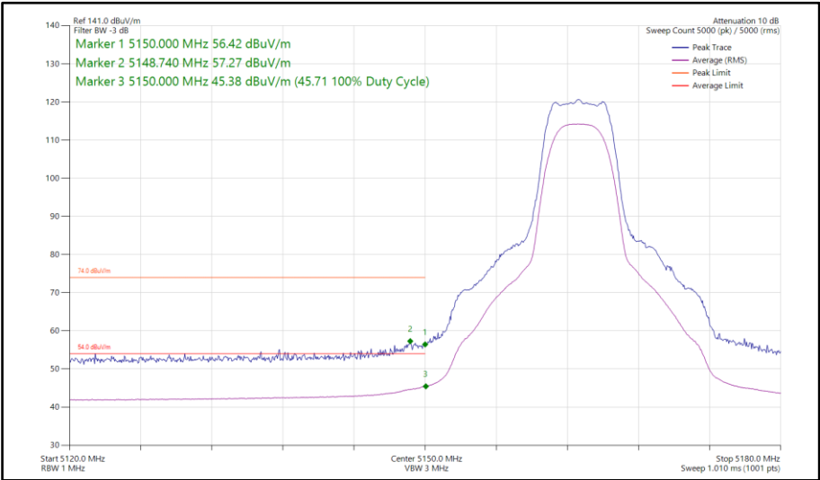
Figure 108 - XHDRPM8, SISO, Core 0 - 5163 MHz Band Edge Frequency 5150 MHz
