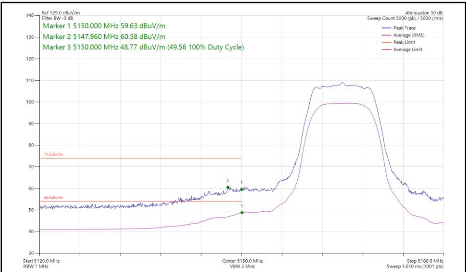
Figure 78 - XHDRPL24, MIMO, Core 0-1 - 5165 MHz Band Edge Frequency 5150 MHz
