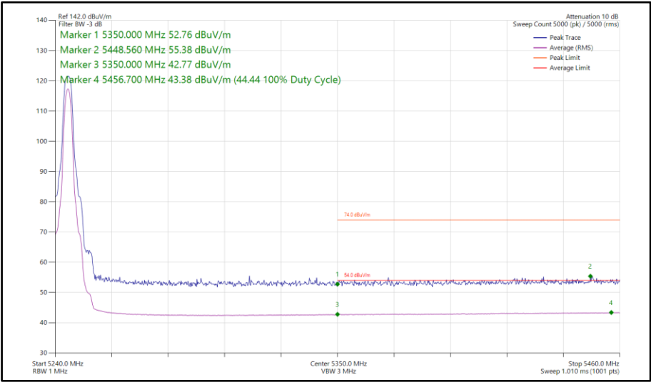
Figure 112 - HDR4, SISO, Core 0 - 5245 MHz Band Edge Frequency 5350 MHz
