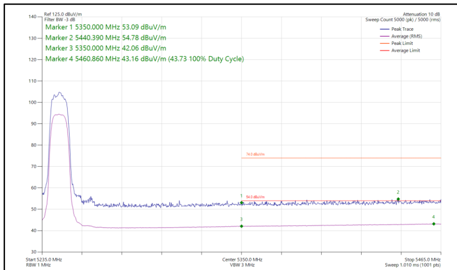
Figure 60 - HDRPL24, SISO, Core 1 - 5245 MHz Band Edge Frequency 5350 MHz
