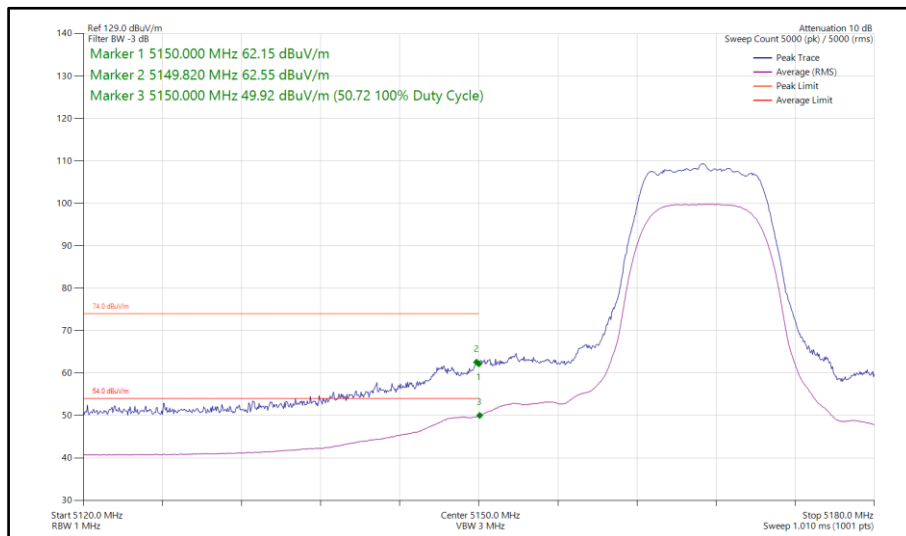
Figure 79 - XHDRPL24, MIMO, Core 0-1 - 5167 MHz Band Edge Frequency 5150 MHz
