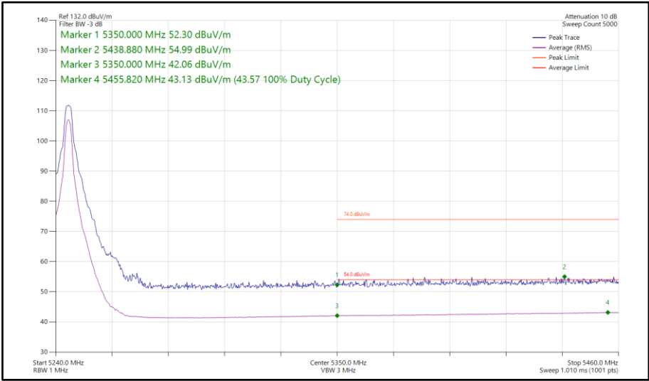
Figure 87 - HDT6, MIMO, Core 0-1 - 5245 MHz Band Edge Frequency 5350 MHz
