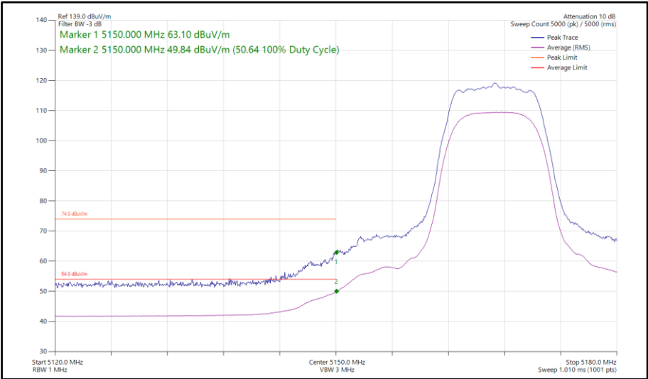
Figure 110 - XHDRPL24, SISO, Core 0 - 5167 MHz Band Edge Frequency 5150 MHz
