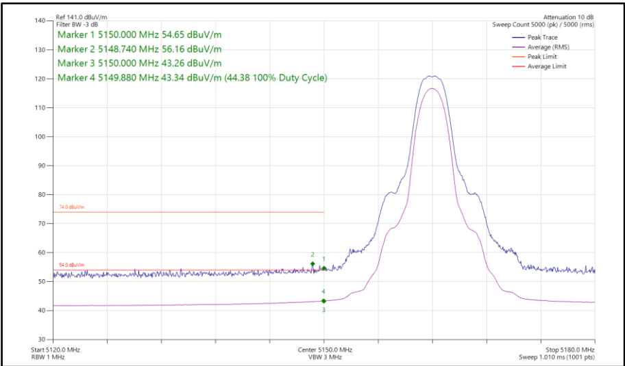
Figure 95 - HDR4, SISO, Core 0 - 5162 MHz Band Edge Frequency 5150 MHz
