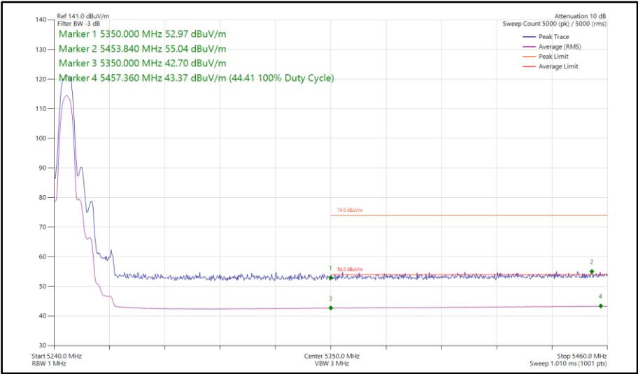
Figure 113 - HDR8, SISO, Core 0 - 5245 MHz Band Edge Frequency 5350 MHz
