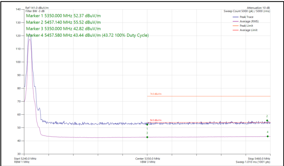
Figure 117 - HDT4, SISO, Core 0 - 5245 MHz Band Edge Frequency 5350 MHz
