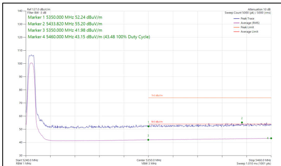
Figure 61 - XHDRPM8, SISO, Core 1 - 5245 MHz Band Edge Frequency 5350 MHz
