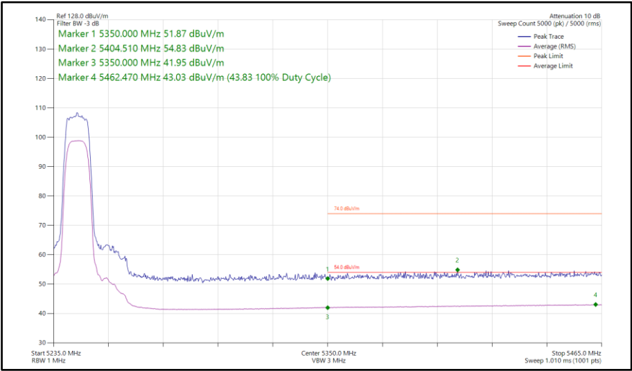
Figure 93 - XHDRPL24, MIMO, Core 0-1 - 5245 MHz Band Edge Frequency 5350 MHz
