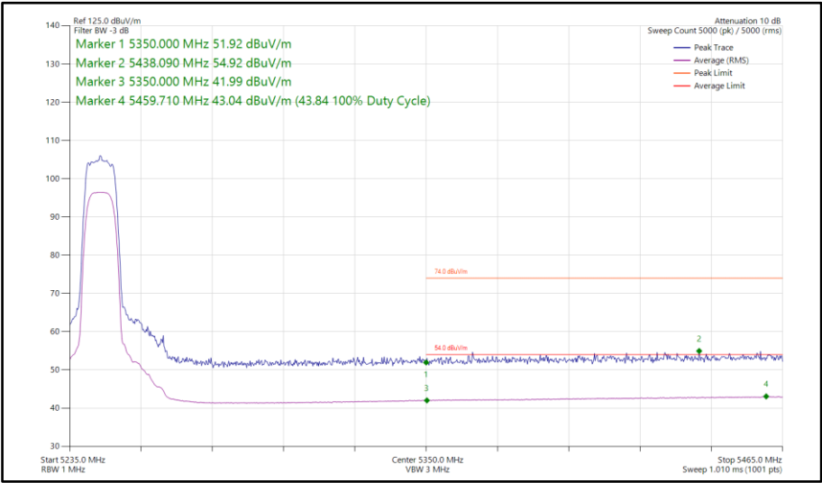
Figure 62 - XHDRPL24, SISO, Core 1 - 5245 MHz Band Edge Frequency 5350 MHz
