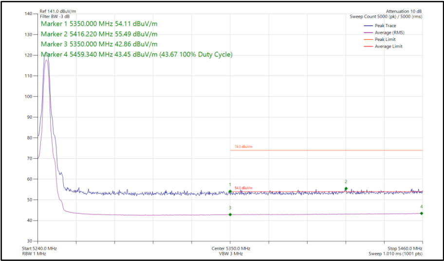
Figure 116 - HDT3, SISO, Core 0 - 5245 MHz Band Edge Frequency 5350 MHz
