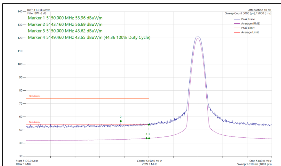
Figure 97 - LE1M, SISO, Core 0 - 5162 MHz Band Edge Frequency 5150 MHz
