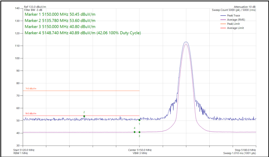
Figure 63 - DH5, MIMO, Core 0-1 - 5162 MHz Band Edge Frequency 5150 MHz
