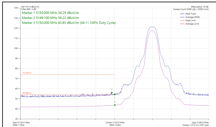
Figure 100 - HDT4, SISO, Core 0 - 5162 MHz Band Edge Frequency 5150 MHz
