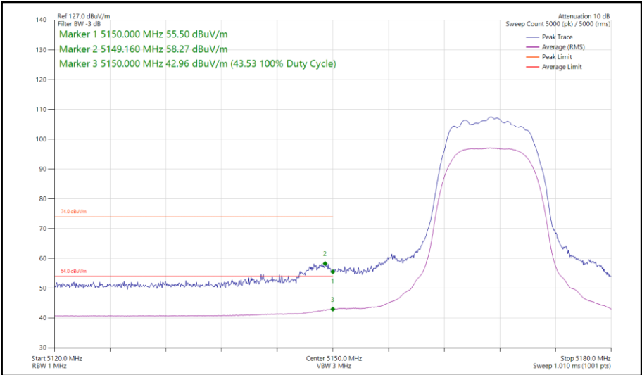
Figure 76 - HDRPL24, MIMO, Core 0-1 - 5167 MHz Band Edge Frequency 5150 MHz
