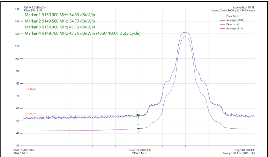
Figure 99 - HDT3, SISO, Core 0 - 5162 MHz Band Edge Frequency 5150 MHz
