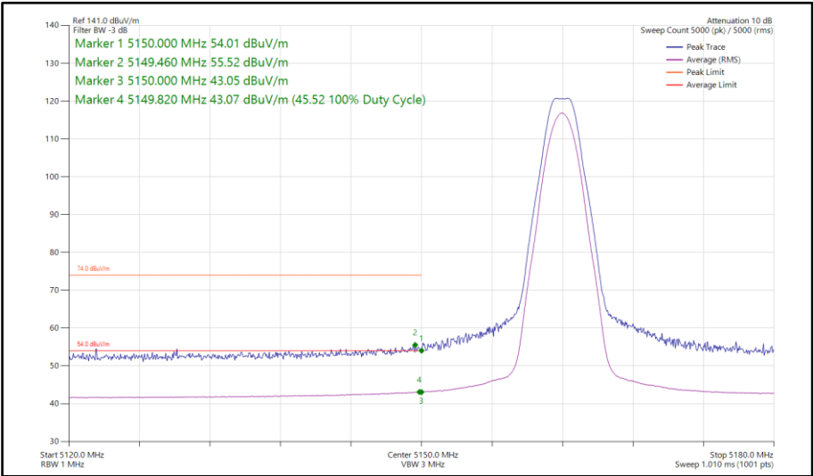
Figure 98 - LE2M, SISO, Core 0 - 5162 MHz Band Edge Frequency 5150 MHz
