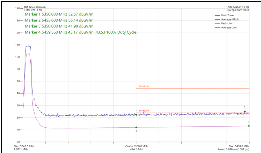
Figure 92 - XHDRPM8, MIMO, Core 0-1 - 5245 MHz Band Edge Frequency 5350 MHz
