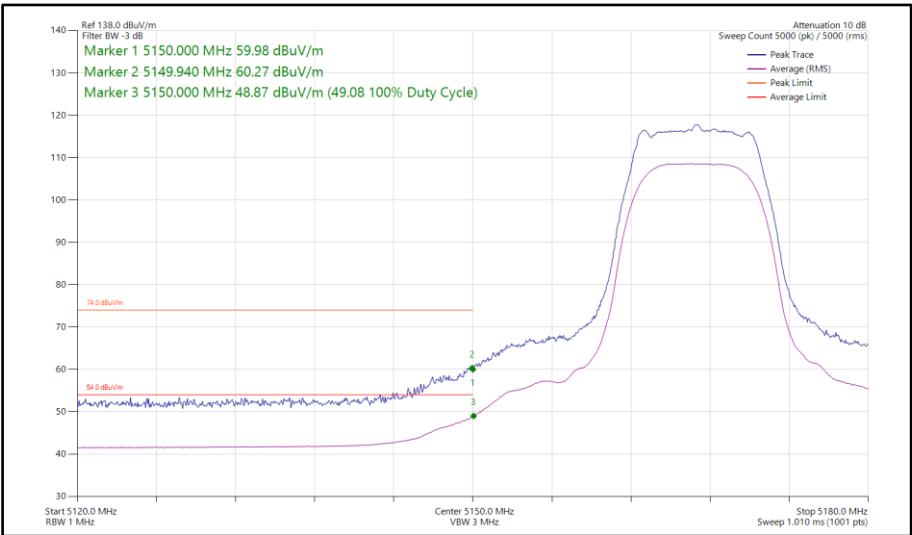
Figure 105 - HDRPL8, SISO, Core 0 - 5167 MHz Band Edge Frequency 5150 MHz
