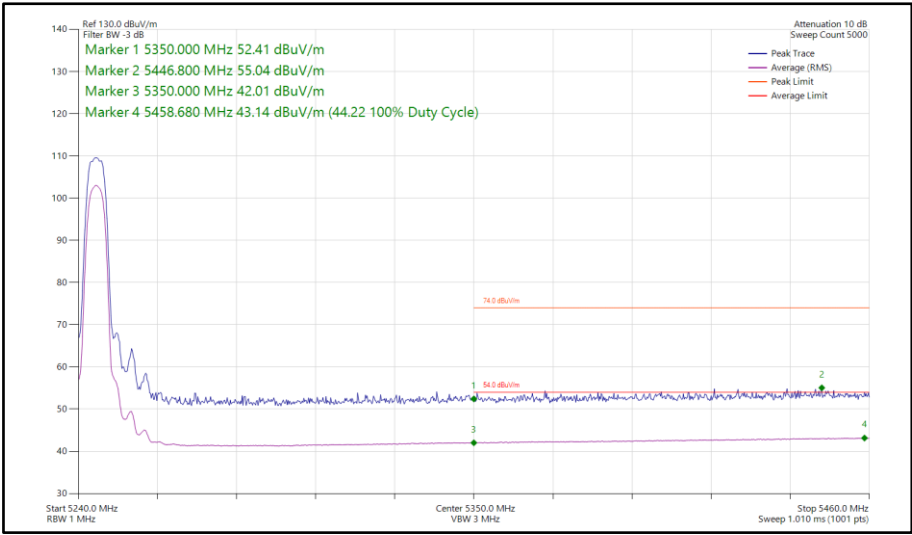
Figure 82 - HDR8, MIMO, Core 0-1 - 5245 MHz Band Edge Frequency 5350 MHz
