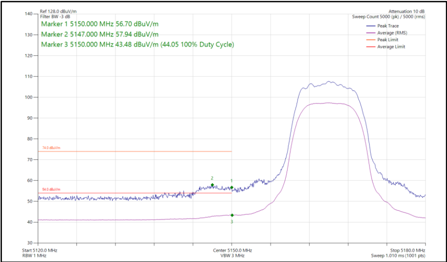
Figure 75 - HDRPL24, MIMO, Core 0-1 - 5165 MHz Band Edge Frequency 5150 MHz
