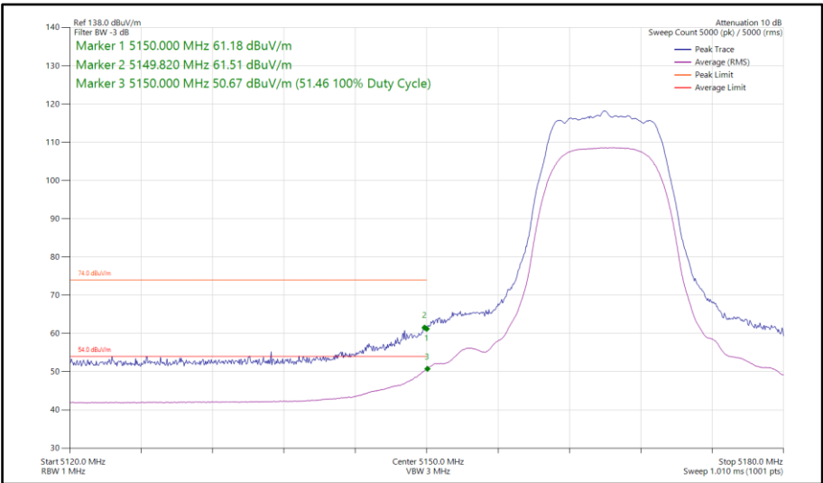
Figure 109 - XHDRPL24, SISO, Core 0 - 5165 MHz Band Edge Frequency 5150 MHz
