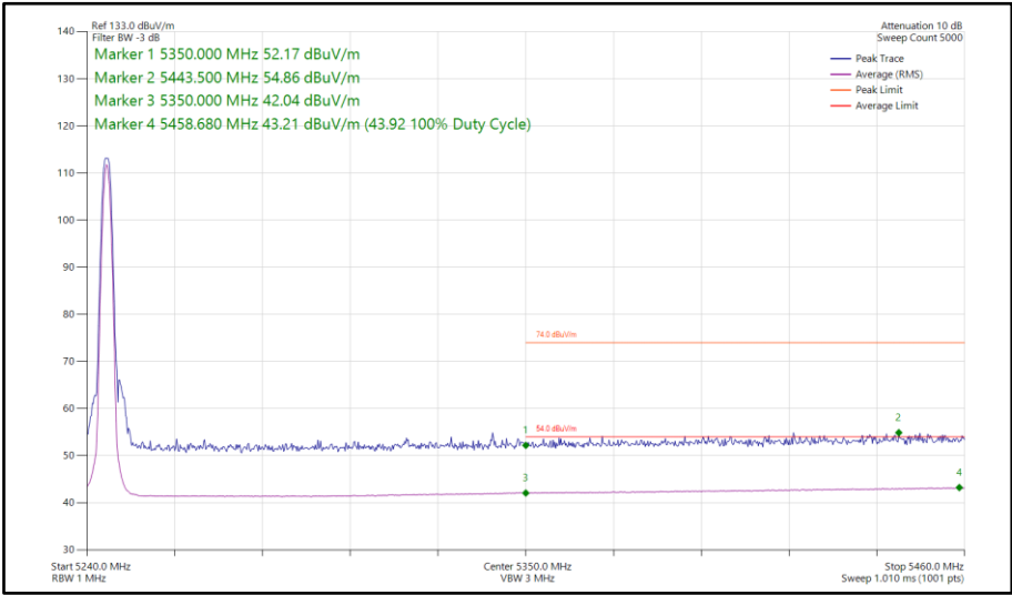
Figure 83 - LE1M, MIMO, Core 0-1 - 5245 MHz Band Edge Frequency 5350 MHz
