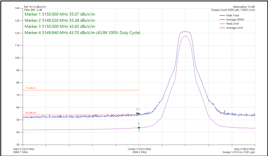
Figure 102 - HDRPS2, SISO, Core 0 - 5162 MHz Band Edge Frequency 5150 MHz
