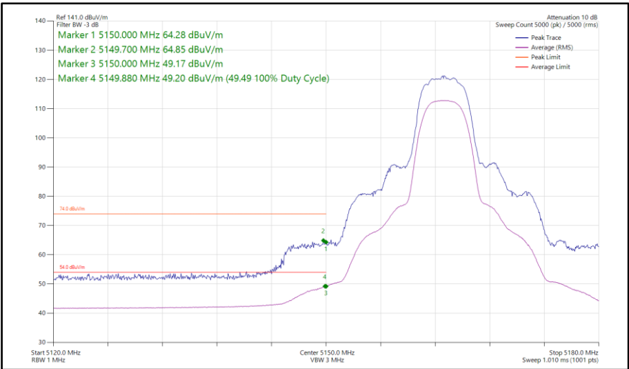
Figure 103 - HDRPM12, SISO, Core 0 - 5163 MHz Band Edge Frequency 5150 MHz
