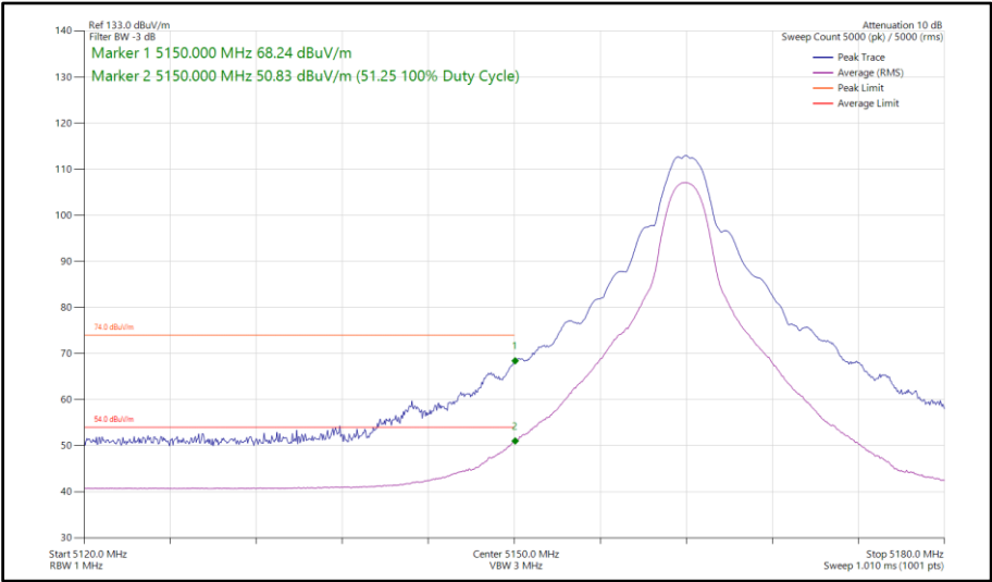
Figure 70 - HDT6, MIMO, Core 0-1 - 5162 MHz Band Edge Frequency 5150 MHz
