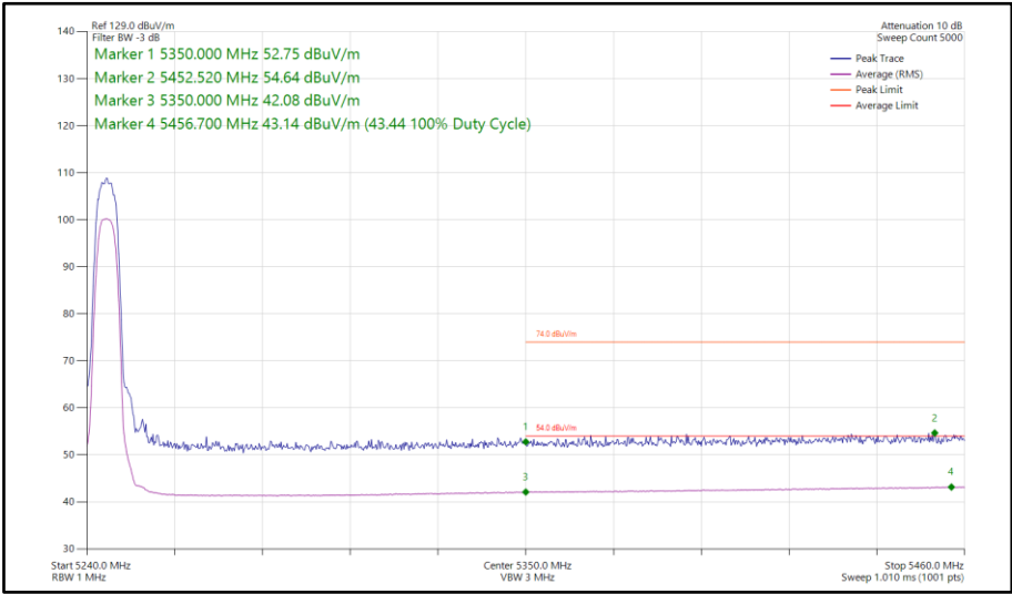
Figure 89 - HDRPM12, MIMO, Core 0-1 - 5245 MHz Band Edge Frequency 5350 MHz
