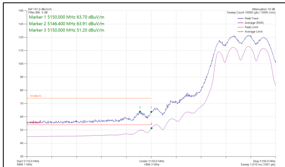
Figure 111 - 802.11ac VHT20, TxBF, Core 0-1 - 5180 MHz Band Edge Frequency 5150 MHz
