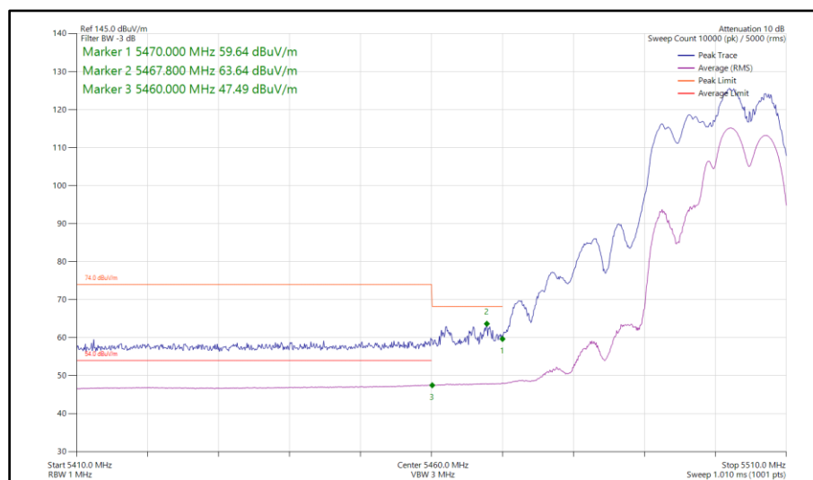
Figure 109 - 802.11be EHT20, SDM, Core 0-1 - 5500 MHz Band Edge Frequency 5460 MHz
