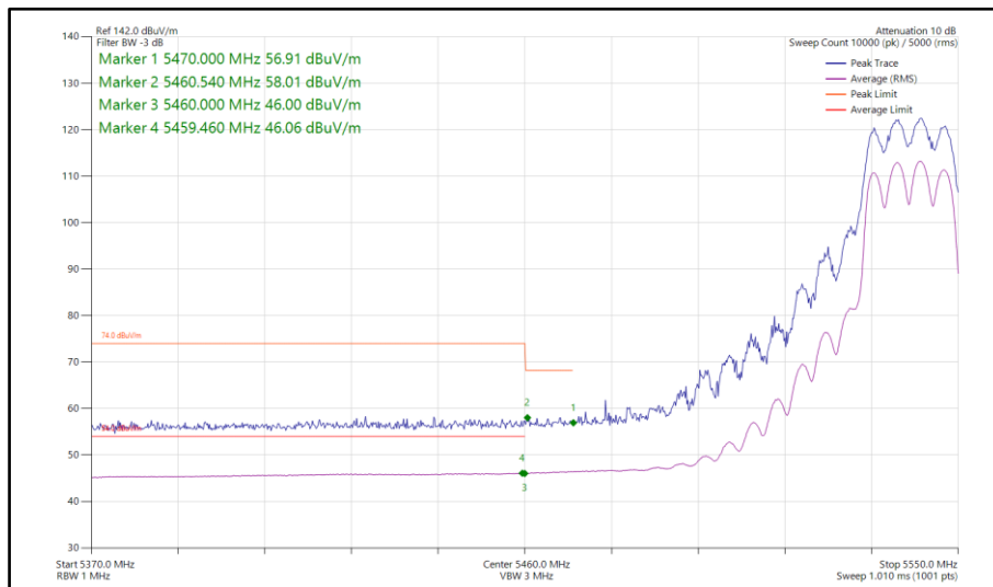
Figure 79 - 802.11n HT20, CDD, Core 0-1 - 5540 MHz Band Edge Frequency 5460 MHz
