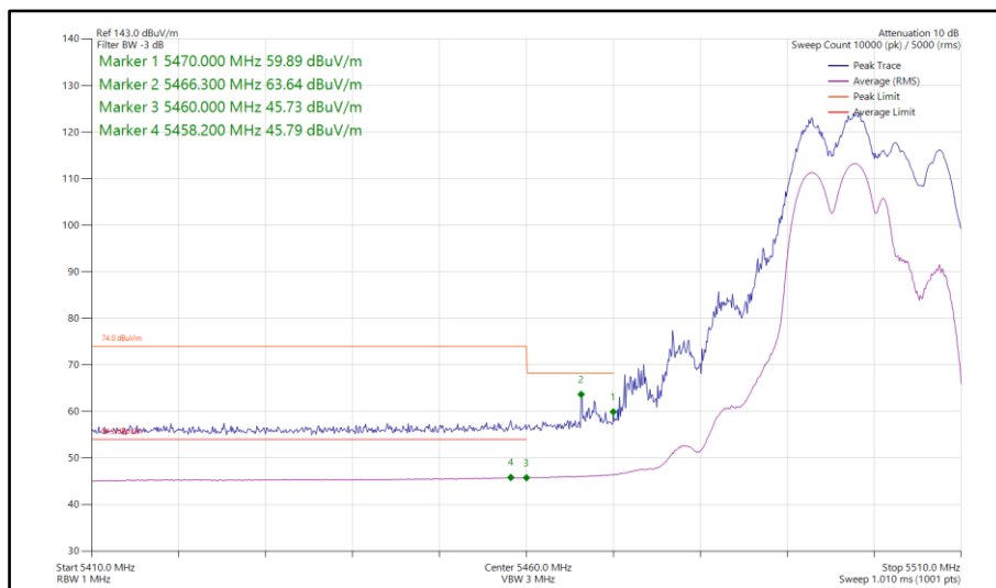
Figure 86 - 802.11be EHT20, CDD, Core 0-1 - 5500 MHz Band Edge Frequency 5460 MHz
