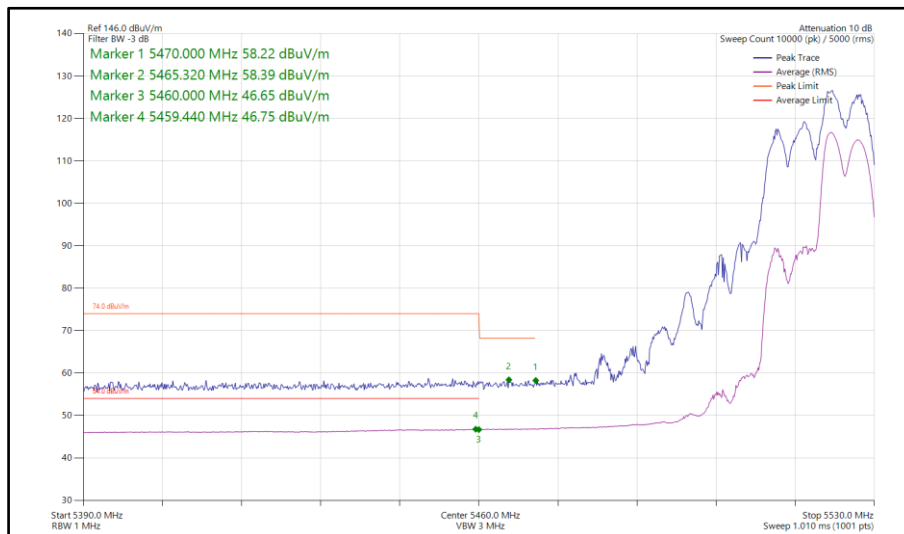
Figure 83 - 802.11ax HE20, RU 106-54, CDD, Core 0-1 - 5520 MHz Band Edge Frequency 5460 MHz
