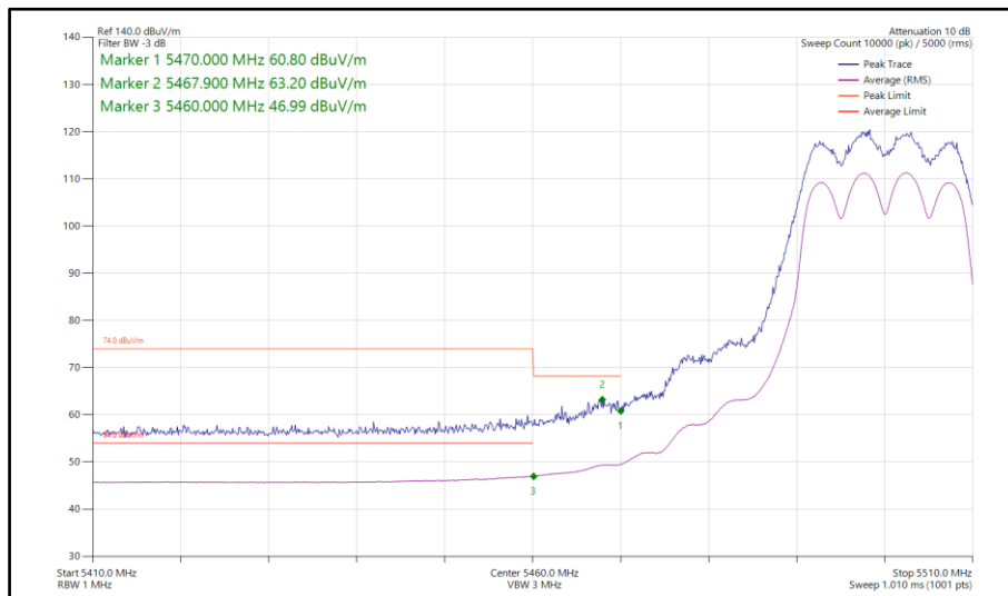
Figure 77 - 802.11n HT20, CDD, Core 0-1 - 5500 MHz Band Edge Frequency 5460 MHz
