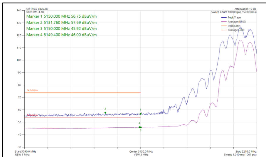
Figure 64 - 802.11be EHT20, CDD, Core 0-1 - 5200 MHz Band Edge Frequency 5150 MHz
