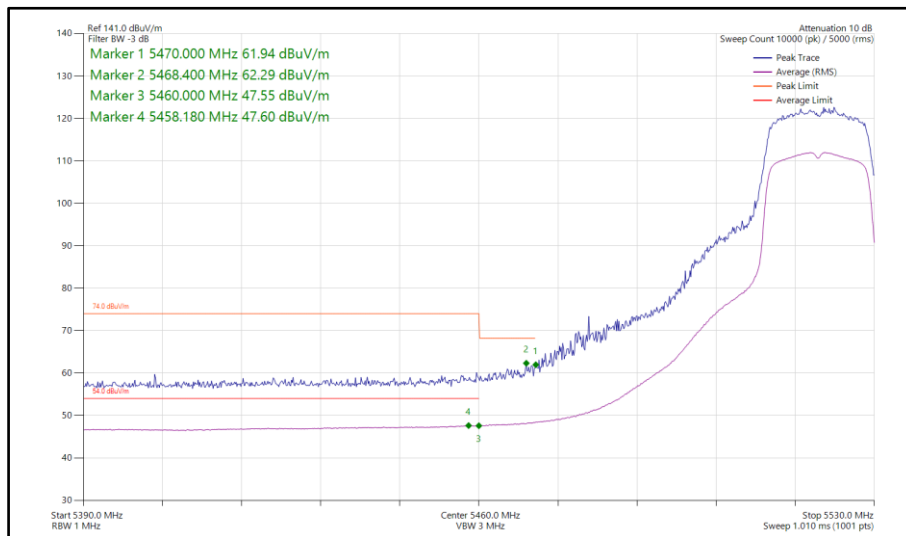
Figure 102 - 802.11n HT20, SDM, Core 0-1 - 5520 MHz Band Edge Frequency 5460 MHz
