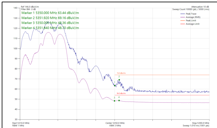
Figure 100 - 802.11be EHT20, SDM, Core 0-1 - 5320 MHz Band Edge Frequency 5350 MHz
