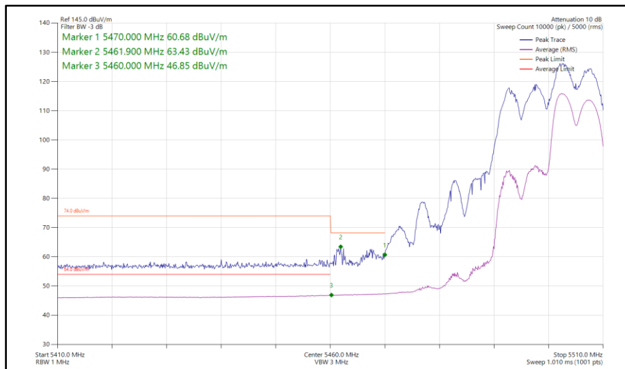
Figure 81 - 802.11ax HE20, RU 106-54, CDD, Core 0-1 - 5500 MHz Band Edge Frequency 5460 MHz
