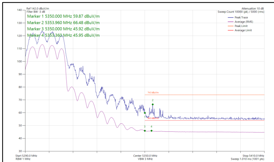
Figure 69 - 802.11ax HE20, SU, CDD, Core 0-1 - 5300 MHz Band Edge Frequency 5350 MHz
