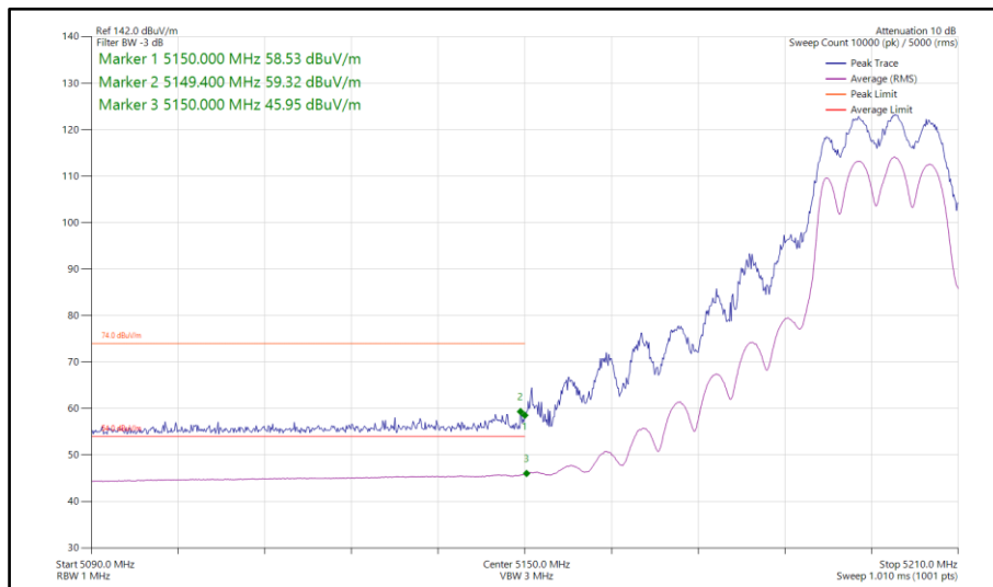
Figure 112 - 802.11ac VHT20, TxBF, Core 0-1 - 5200 MHz Band Edge Frequency 5150 MHz
