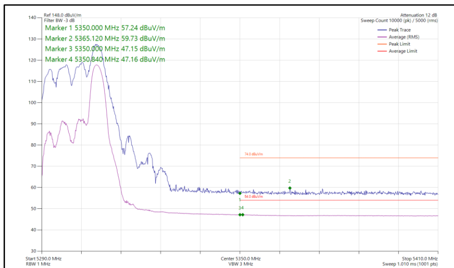
Figure 70 - 802.11ax HE20, RU 52-40, CDD, Core 0-1 - 5300 MHz Band Edge Frequency 5350 MHz
