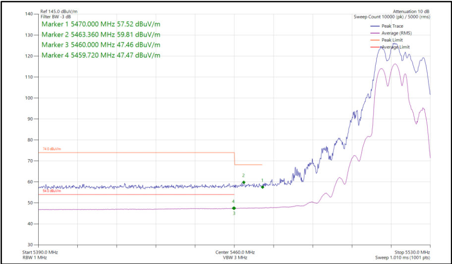
Figure 110 - 802.11be EHT20, SDM, Core 0-1 - 5520 MHz Band Edge Frequency 5460 MHz
