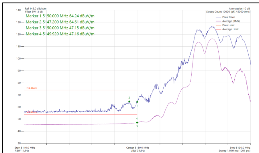
Figure 60 - 802.11ax HE20, RU 106-53, CDD, Core 0-1 - 5180 MHz Band Edge Frequency 5150 MHz
