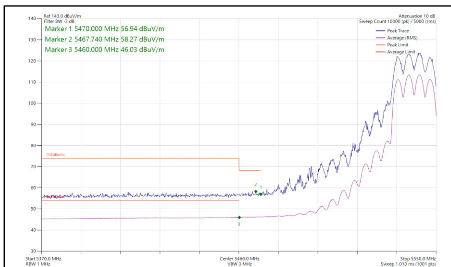
Figure 84 - 802.11ax HE20, SU, CDD, Core 0-1 - 5540 MHz Band Edge Frequency 5460 MHz
