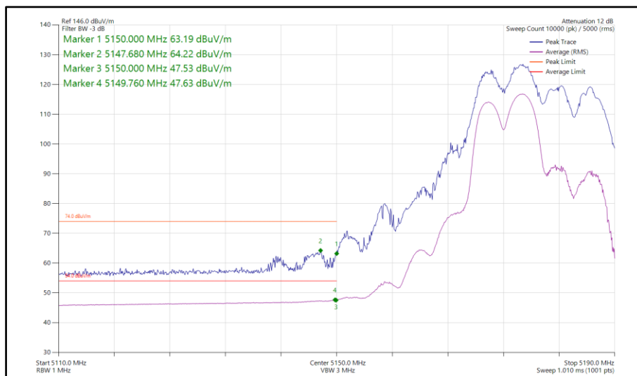
Figure 91 - 802.11ax HE20, RU 106-53, SDM, Core 0-1 - 5180 MHz Band Edge Frequency 5150 MHz
