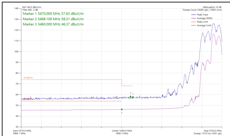
Figure 85 - 802.11ax HE20, RU 106-54, CDD, Core 0-1 - 5540 MHz Band Edge Frequency 5460 MHz
