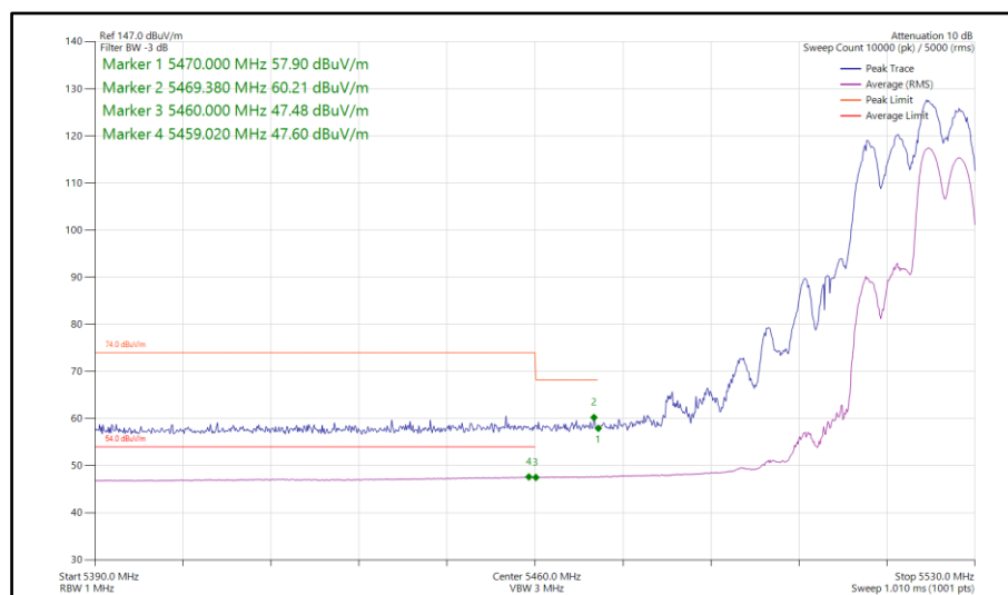
Figure 107 - 802.11ax HE20, RU 106-54, SDM, Core 0-1 - 5520 MHz Band Edge Frequency 5460 MHz
