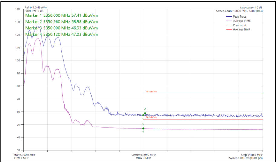
Figure 99 - 802.11be EHT20, SDM, Core 0-1 - 5300 MHz Band Edge Frequency 5350 MHz
