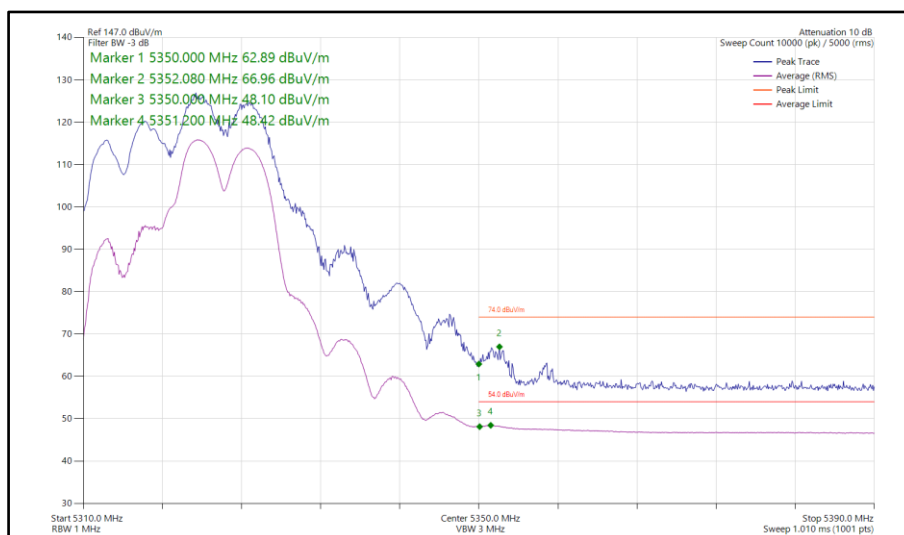
Figure 74 - 802.11be EHT20, CDD, Core 0-1 - 5320 MHz Band Edge Frequency 5350 MHz
