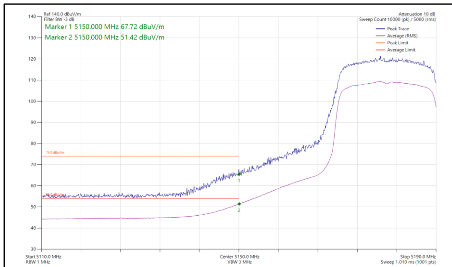
Figure 90 - 802.11ax HE20, SU, SDM, Core 0-1 - 5180 MHz Band Edge Frequency 5150 MHz
