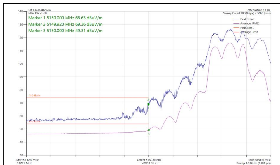
Figure 93 - 802.11be EHT20, SDM, Core 0-1 - 5180 MHz Band Edge Frequency 5150 MHz
