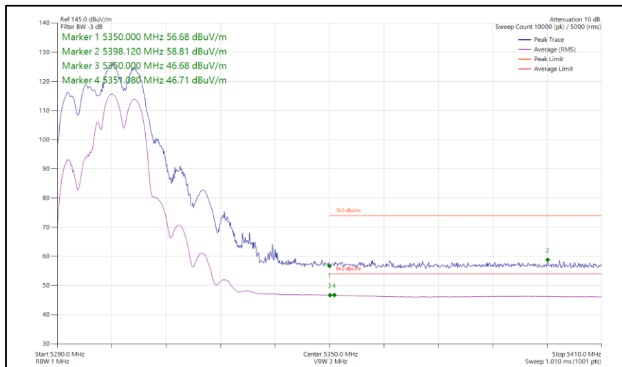
Figure 73 - 802.11be EHT20, CDD, Core 0-1 - 5300 MHz Band Edge Frequency 5350 MHz
