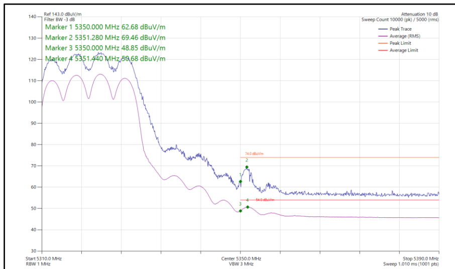
Figure 71 - 802.11ax HE20, SU, CDD, Core 0-1 - 5320 MHz Band Edge Frequency 5350 MHz
