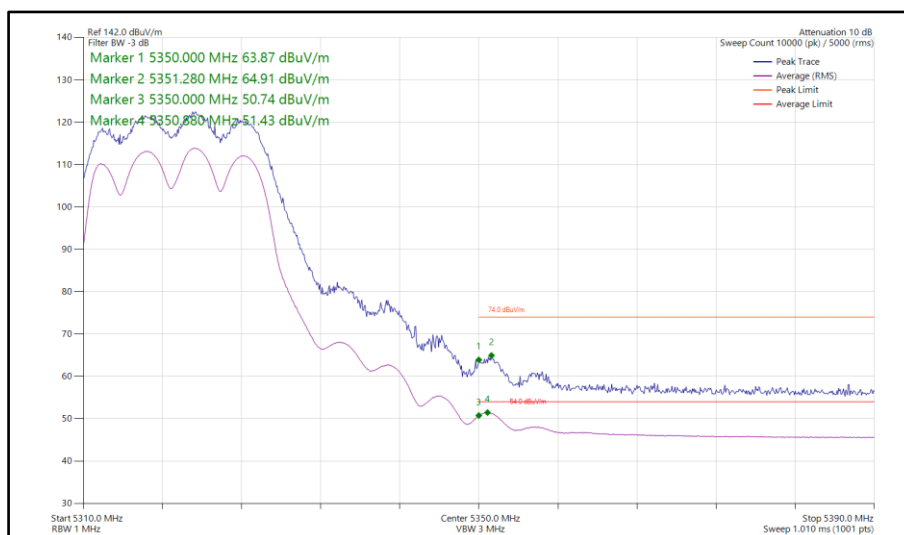
Figure 68 - 802.11n HT20, CDD, Core 0-1 - 5320 MHz Band Edge Frequency 5350 MHz
