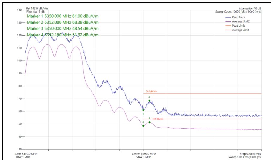
Figure 116 - 802.11ac VHT20, TxBF, Core 0-1 - 5320 MHz Band Edge Frequency 5350 MHz
