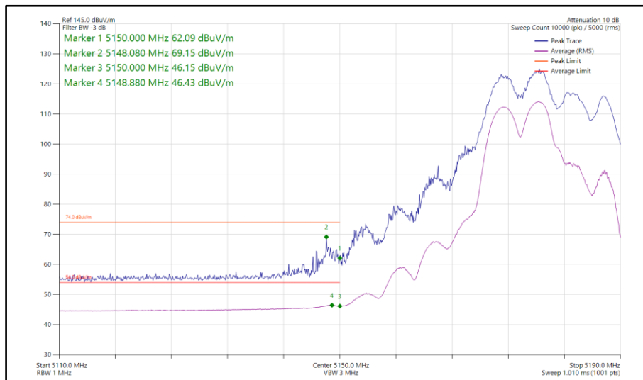
Figure 63 - 802.11be EHT20, CDD, Core 0-1 - 5180 MHz Band Edge Frequency 5150 MHz
