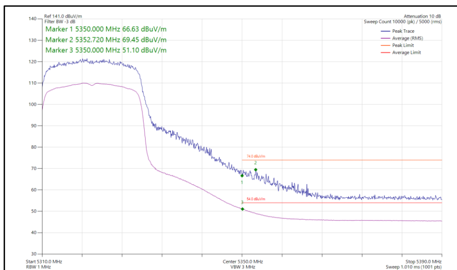
Figure 97 - 802.11ax HE20, SU, SDM, Core 0-1 - 5320 MHz Band Edge Frequency 5350 MHz
