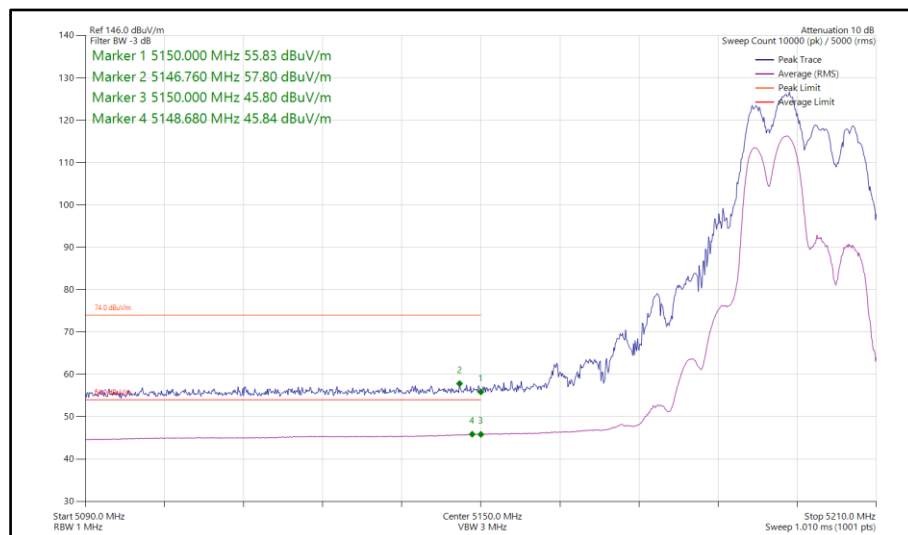
Figure 62 - 802.11ax HE20, RU 106-53, CDD, Core 0-1 - 5200 MHz Band Edge Frequency 5150 MHz
