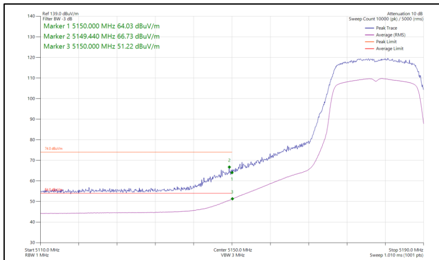
Figure 88 - 802.11n HT20, SDM, Core 0-1 - 5180 MHz Band Edge Frequency 5150 MHz
