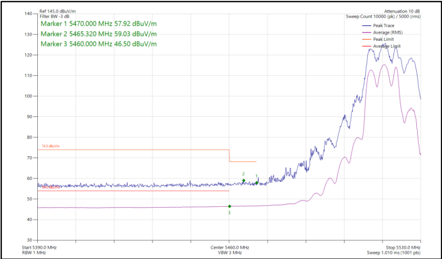
Figure 87 - 802.11be EHT20, CDD, Core 0-1 - 5520 MHz Band Edge Frequency 5460 MHz
