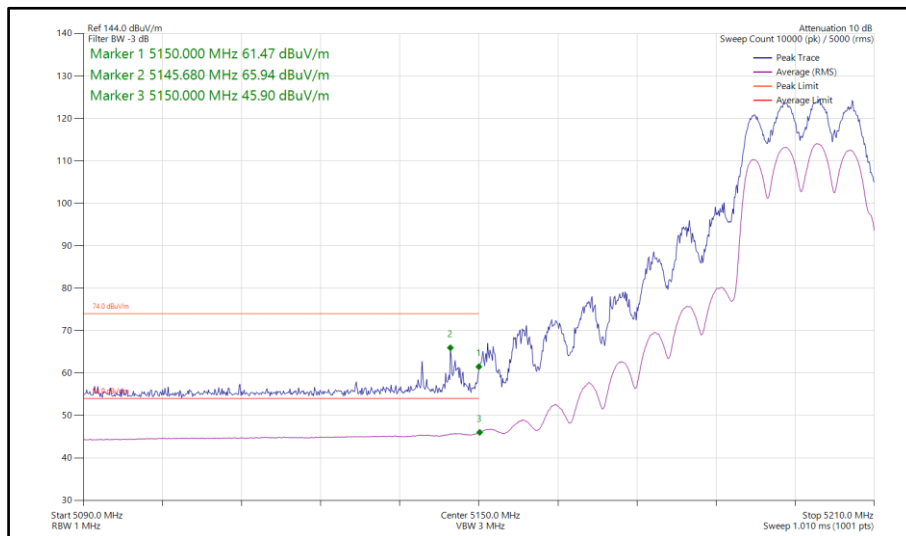
Figure 114 - 802.11ax HE20, SU, TxBF, Core 0-1 - 5200 MHz Band Edge Frequency 5150 MHz
