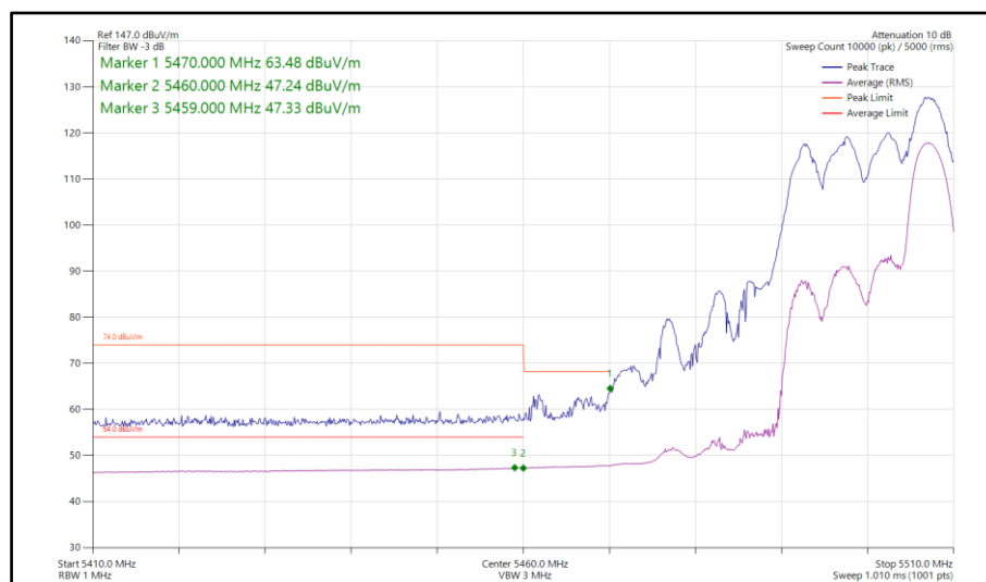
Figure 105 - 802.11ax HE20, RU 52-40, SDM, Core 0-1 - 5500 MHz Band Edge Frequency 5460 MHz
