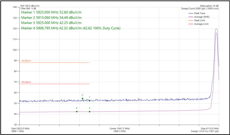
Figure 313 - HDRPS2, SISO, Core 1 - 6106 MHz Band Edge Frequency 5925 MHz
