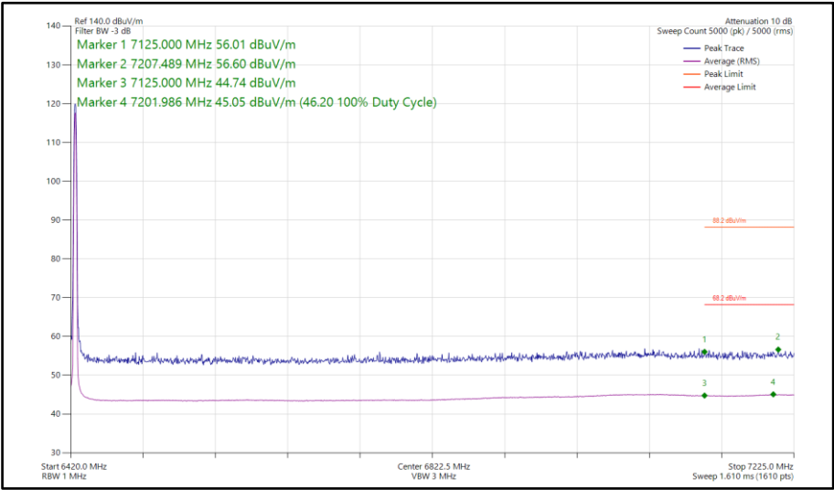
Figure 319 - DH5, SISO, Core 1 - 6425 MHz Band Edge Frequency 7125 MHz
