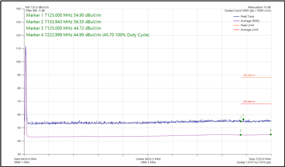
Figure 266 - LE1M, MIMO, Core 0-1 - 6425 MHz Band Edge Frequency 7125 MHz
