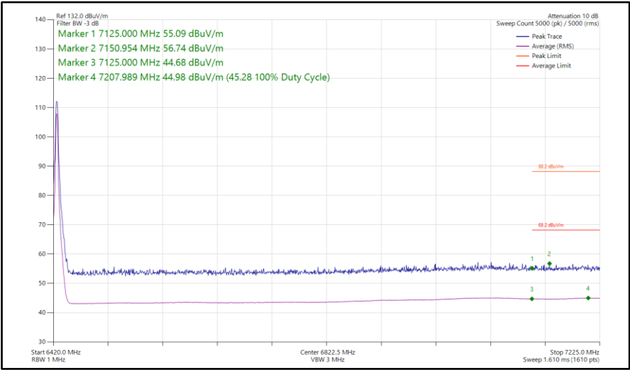
Figure 269 - HDT4, MIMO, Core 0-1 - 6425 MHz Band Edge Frequency 7125 MHz
