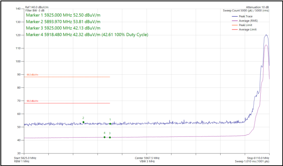
Figure 314 - HDRPM12, SISO, Core 1 - 6106 MHz Band Edge Frequency 5925 MHz
