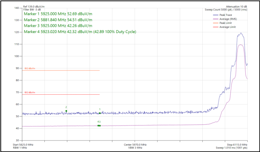
Figure 316 - HDRPL24, SISO, Core 1 - 6106 MHz Band Edge Frequency 5925 MHz
