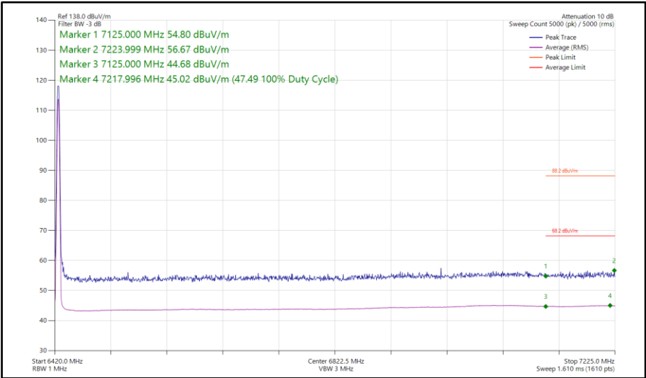
Figure 295 - LE2M, SISO, Core 0 - 6425 MHz Band Edge Frequency 7125 MHz
