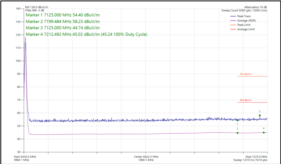
Figure 296 - HDT3, SISO, Core 0 - 6425 MHz Band Edge Frequency 7125 MHz
