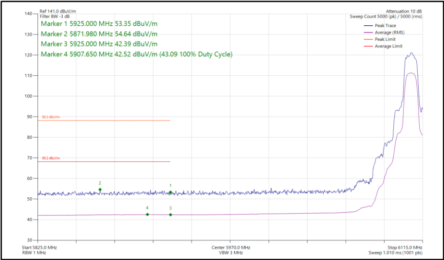
Figure 288 - HDRPL24, SISO, Core 0 - 6106 MHz Band Edge Frequency 5925 MHz
