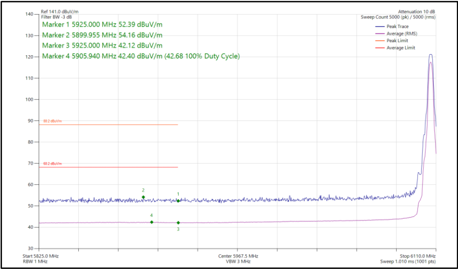
Figure 283 - HDT4, SISO, Core 0 - 6106 MHz Band Edge Frequency 5925 MHz
