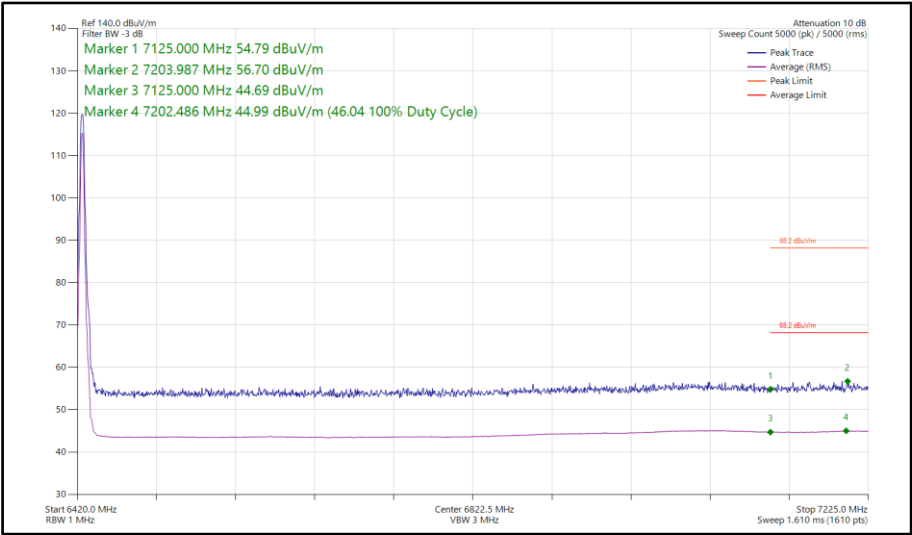
Figure 320 - HDR4, SISO, Core 1 - 6425 MHz Band Edge Frequency 7125 MHz
