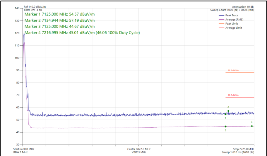
Figure 321 - HDR8, SISO, Core 1 - 6425 MHz Band Edge Frequency 7125 MHz
