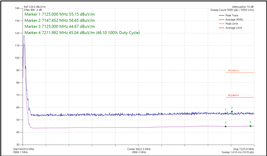
Figure 293 - HDR8, SISO, Core 0 - 6425 MHz Band Edge Frequency 7125 MHz
