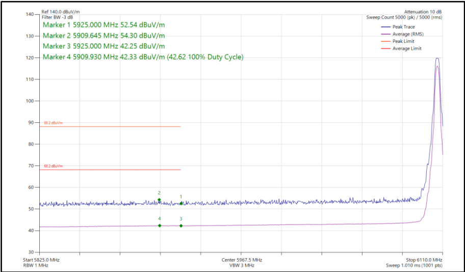
Figure 311 - HDT4, SISO, Core 1 - 6106 MHz Band Edge Frequency 5925 MHz
