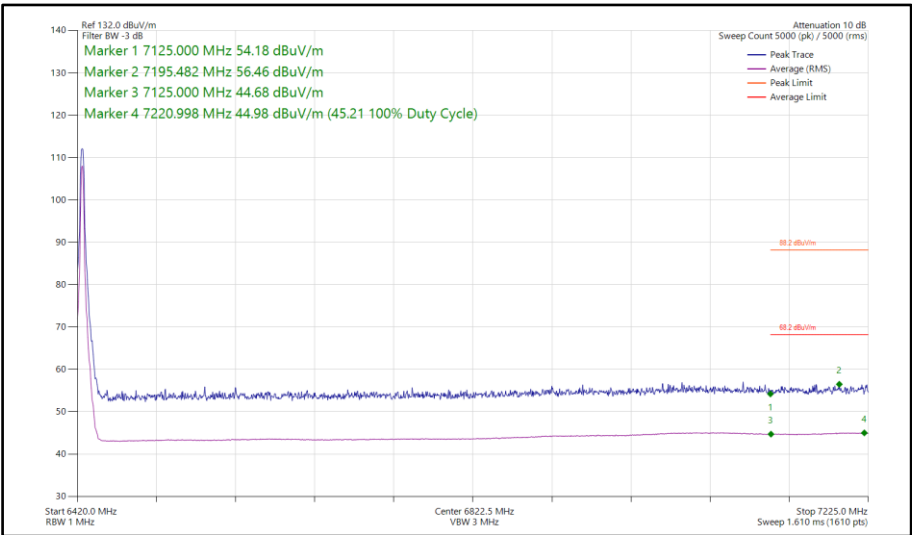
Figure 268 - HDT3, MIMO, Core 0-1 - 6425 MHz Band Edge Frequency 7125 MHz
