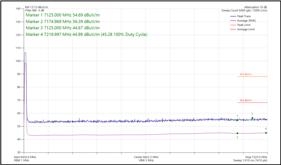
Figure 272 - HDRPM12, MIMO, Core 0-1 - 6425 MHz Band Edge Frequency 7125 MHz
