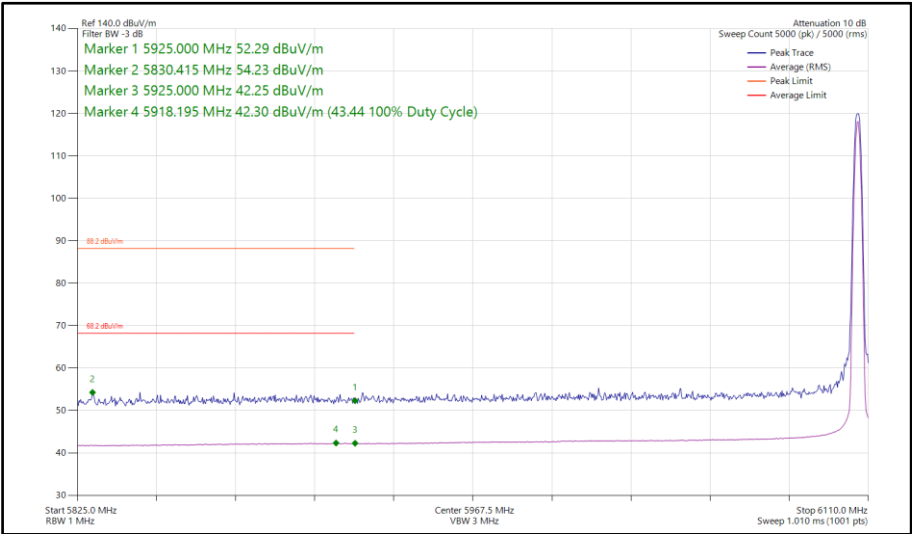
Figure 305 - DH5, SISO, Core 1 - 6106 MHz Band Edge Frequency 5925 MHz
