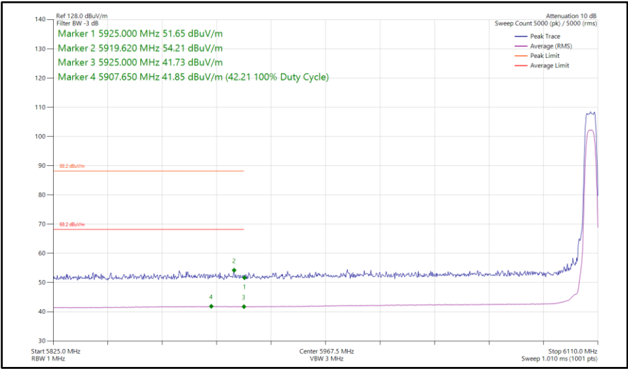
Figure 261 - XHDRPM8, MIMO, Core 0-1 - 6106 MHz Band Edge Frequency 5925 MHz
