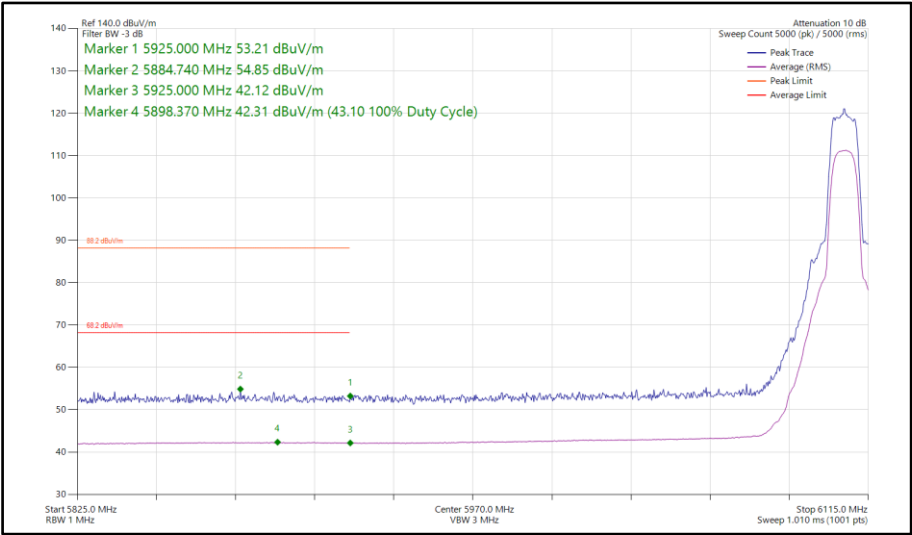
Figure 290 - XHDRPL24, SISO, Core 0 - 6106 MHz Band Edge Frequency 5925 MHz
