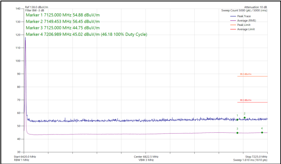
Figure 291 - DH5, SISO, Core 0 - 6425 MHz Band Edge Frequency 7125 MHz
