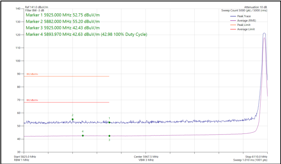
Figure 285 - HDRPS2, SISO, Core 0 - 6106 MHz Band Edge Frequency 5925 MHz
