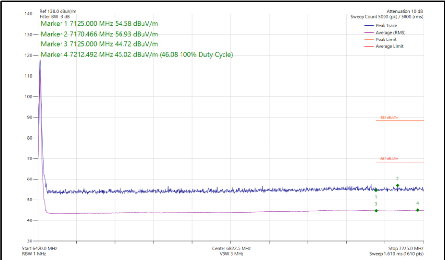
Figure 292 - HDR4, SISO, Core 0 - 6425 MHz Band Edge Frequency 7125 MHz
