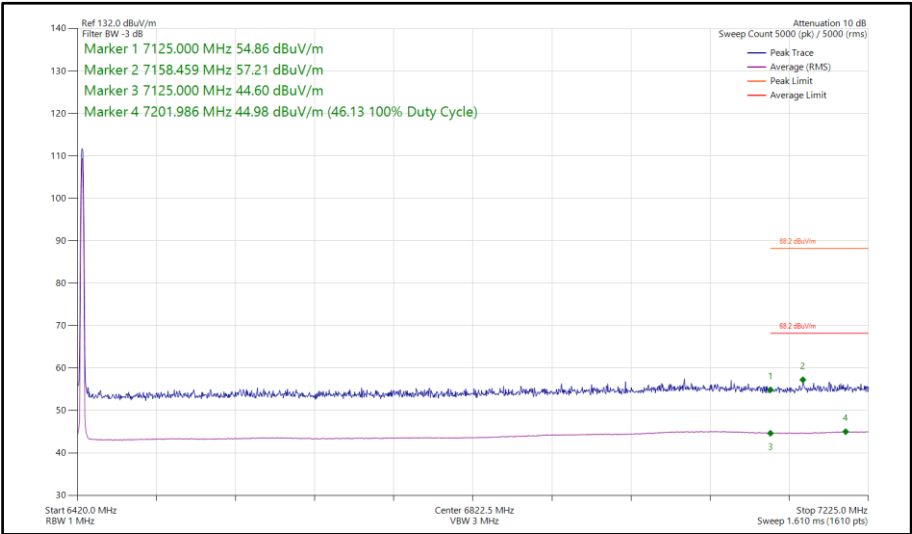
Figure 263 - DH5, MIMO, Core 0-1 - 6425 MHz Band Edge Frequency 7125 MHz
