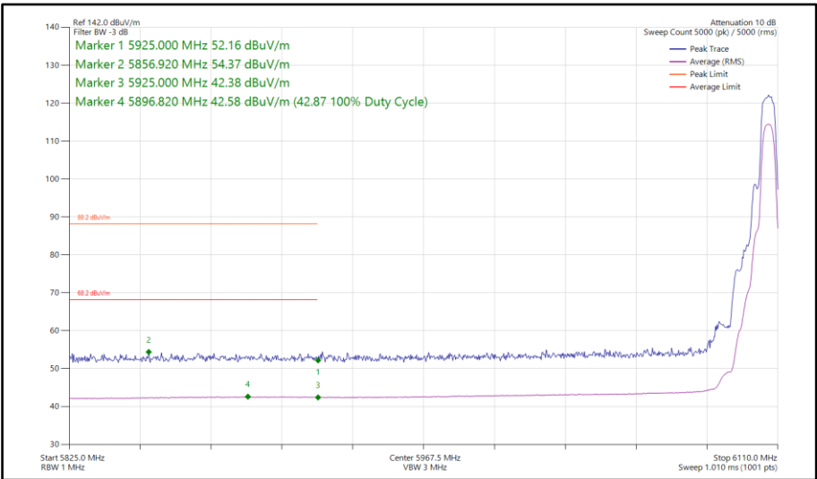
Figure 286 - HDRPM12, SISO, Core 0 - 6106 MHz Band Edge Frequency 5925 MHz
