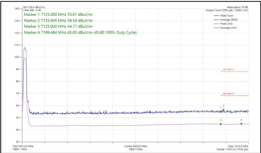
Figure 276 - XHDRPL24, MIMO, Core 0-1 - 6425 MHz Band Edge Frequency 7125 MHz
