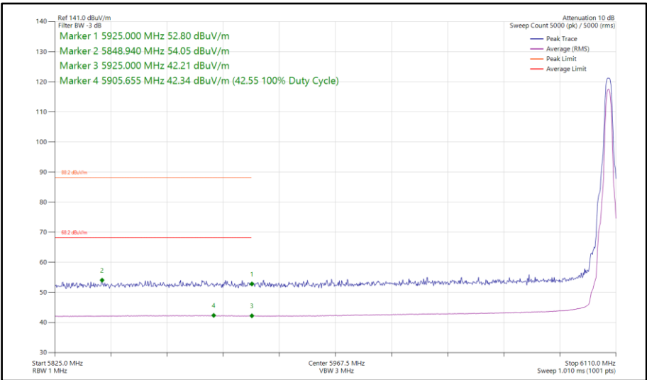
Figure 282 - HDT3, SISO, Core 0 - 6106 MHz Band Edge Frequency 5925 MHz
