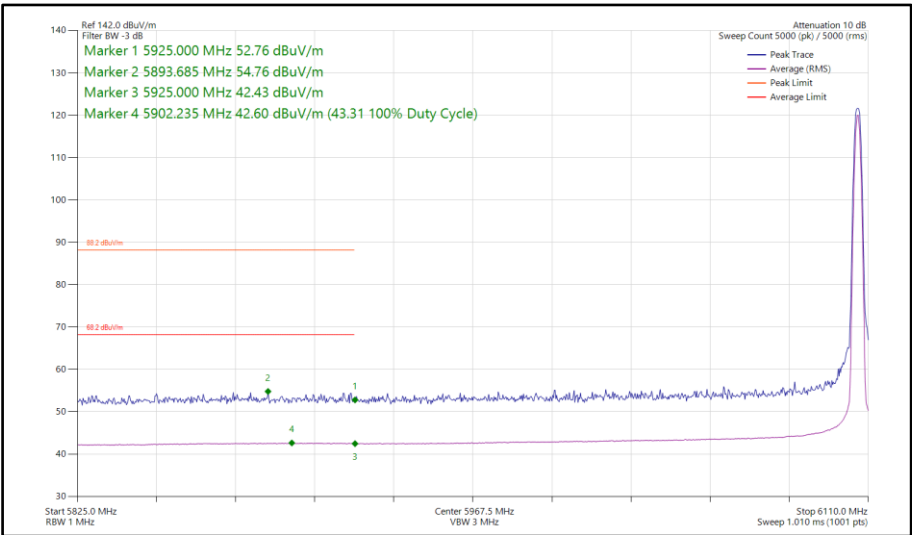
Figure 280 - LE1M, SISO, Core 0 - 6106 MHz Band Edge Frequency 5925 MHz
