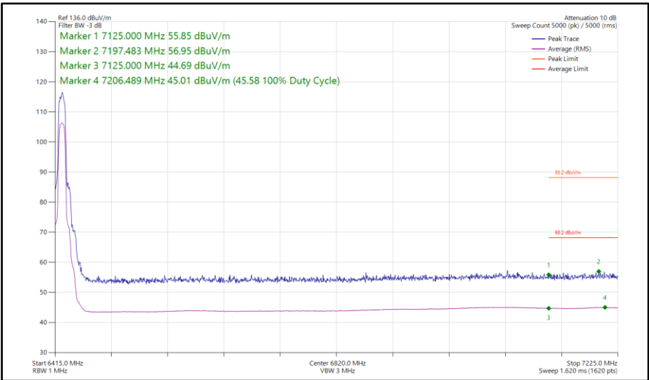
Figure 302 - HDRPL24, SISO, Core 0 - 6425 MHz Band Edge Frequency 7125 MHz
