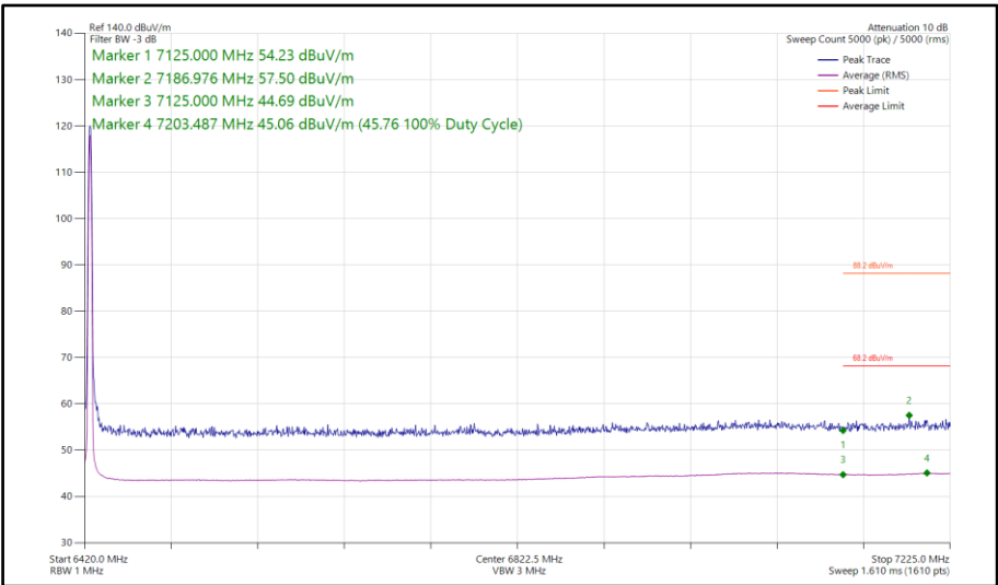
Figure 322 - LE1M, SISO, Core 1 - 6425 MHz Band Edge Frequency 7125 MHz
