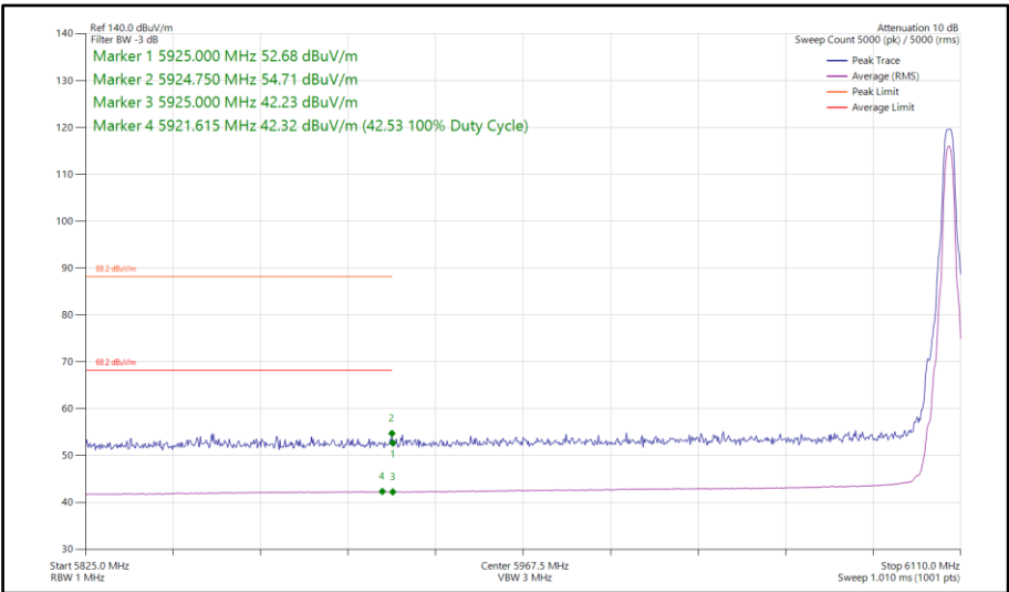
Figure 310 - HDT3, SISO, Core 1 - 6106 MHz Band Edge Frequency 5925 MHz
