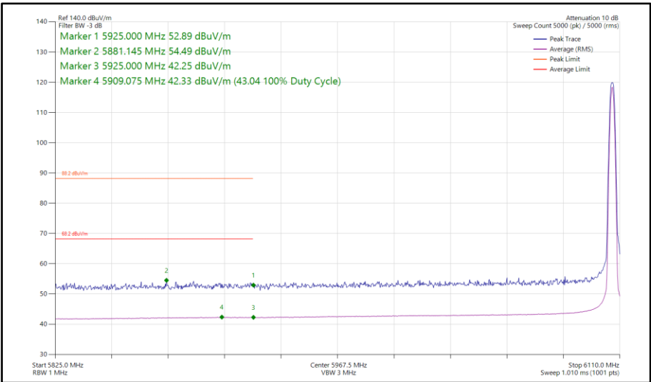
Figure 308 - LE1M, SISO, Core 1 - 6106 MHz Band Edge Frequency 5925 MHz
