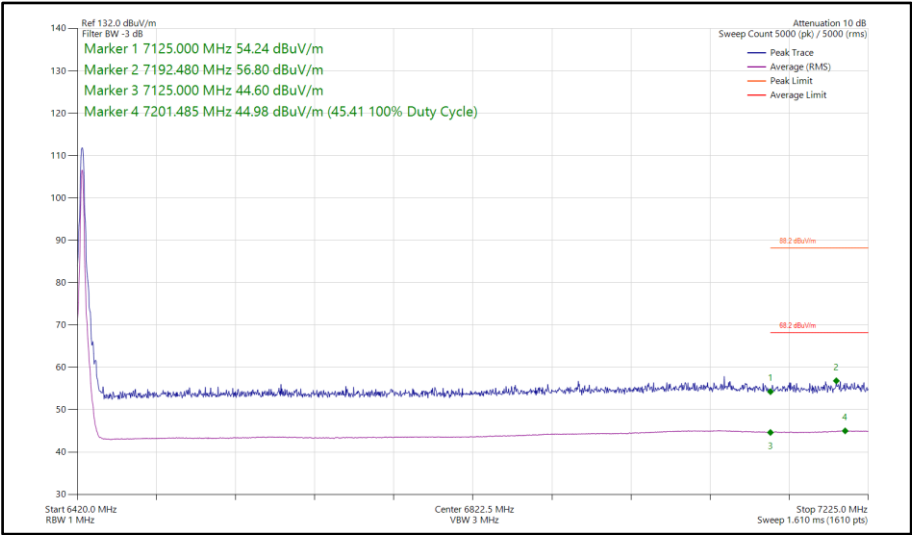
Figure 270 - HDT6, MIMO, Core 0-1 - 6425 MHz Band Edge Frequency 7125 MHz
