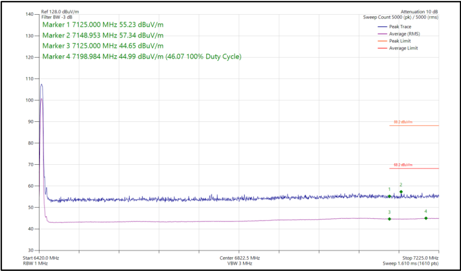
Figure 265 - HDR8, MIMO, Core 0-1 - 6425 MHz Band Edge Frequency 7125 MHz
