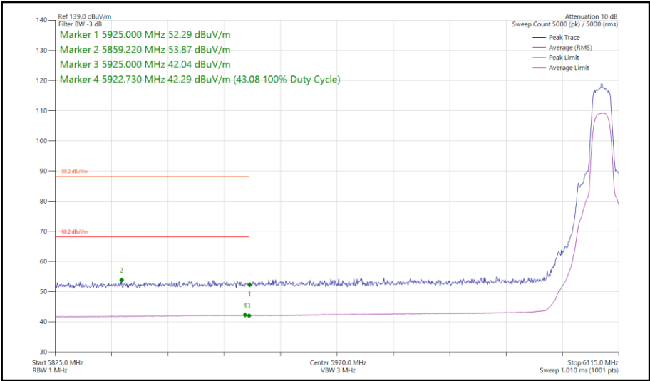
Figure 318 - XHDRPL24, SISO, Core 1 - 6106 MHz Band Edge Frequency 5925 MHz
