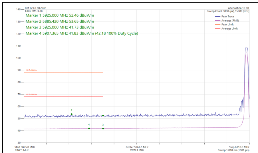
Figure 257 - HDRPS2, MIMO, Core 0-1 - 6106 MHz Band Edge Frequency 5925 MHz
