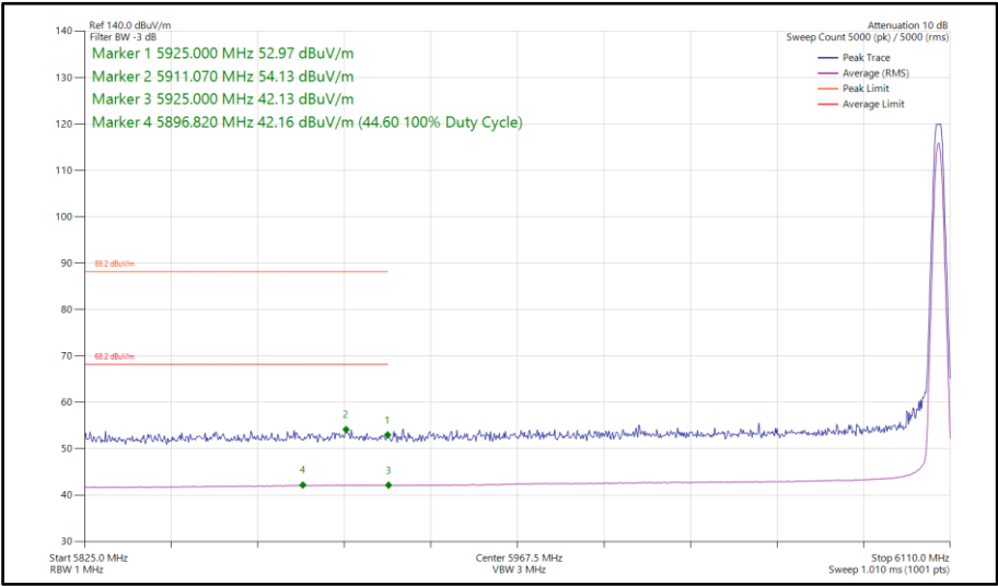
Figure 309 - LE2M, SISO, Core 1 - 6106 MHz Band Edge Frequency 5925 MHz
