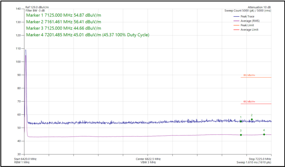
Figure 271 - HDRPS2, MIMO, Core 0-1 - 6425 MHz Band Edge Frequency 7125 MHz
