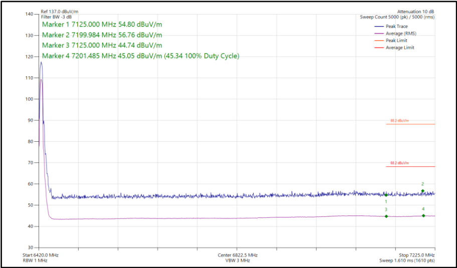
Figure 300 - HDRPM12, SISO, Core 0 - 6425 MHz Band Edge Frequency 7125 MHz
