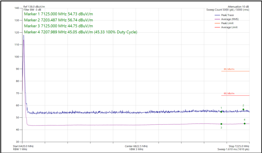
Figure 297 - HDT4, SISO, Core 0 - 6425 MHz Band Edge Frequency 7125 MHz
