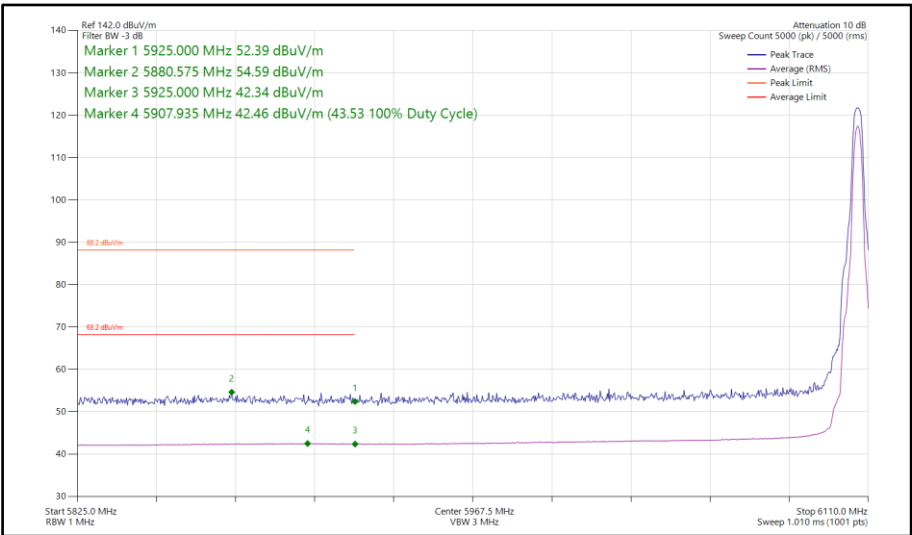
Figure 278 - HDR4, SISO, Core 0 - 6106 MHz Band Edge Frequency 5925 MHz
