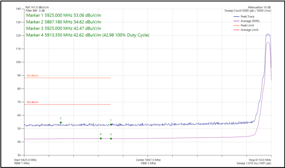
Figure 289 - XHDRPM8, SISO, Core 0 - 6106 MHz Band Edge Frequency 5925 MHz
