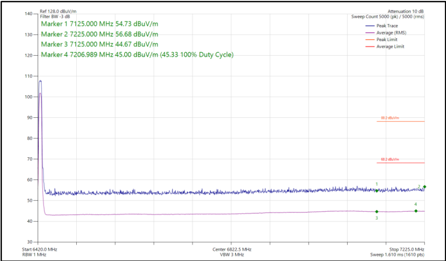
Figure 275 - XHDRPM8, MIMO, Core 0-1 - 6425 MHz Band Edge Frequency 7125 MHz
