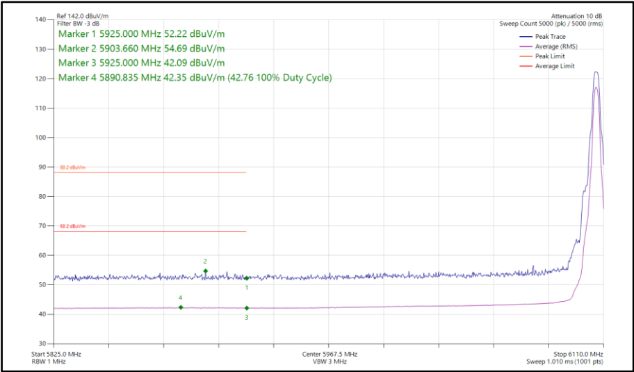
Figure 284 - HDT6, SISO, Core 0 - 6106 MHz Band Edge Frequency 5925 MHz
