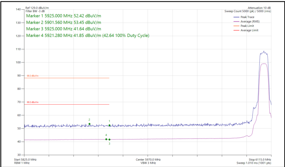
Figure 262 - XHDRPL24, MIMO, Core 0-1 - 6106 MHz Band Edge Frequency 5925 MHz
