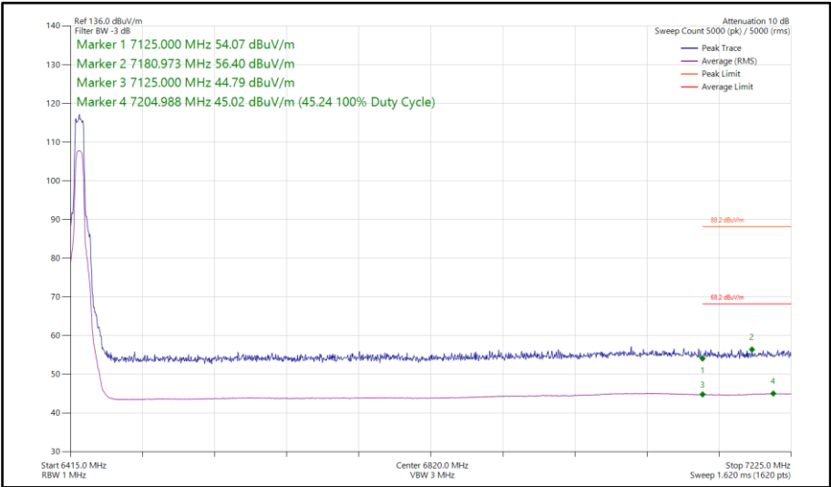
Figure 301 - HDRPL8, SISO, Core 0 - 6425 MHz Band Edge Frequency 7125 MHz
