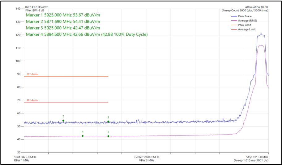
Figure 287 - HDRPL8, SISO, Core 0 - 6106 MHz Band Edge Frequency 5925 MHz
