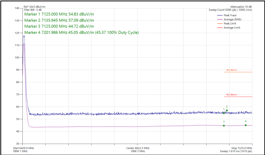
Figure 303 - XHDRPM8, SISO, Core 0 - 6425 MHz Band Edge Frequency 7125 MHz
