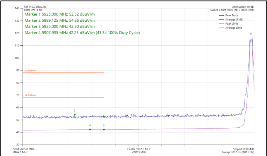
Figure 306 - HDR4, SISO, Core 1 - 6106 MHz Band Edge Frequency 5925 MHz
