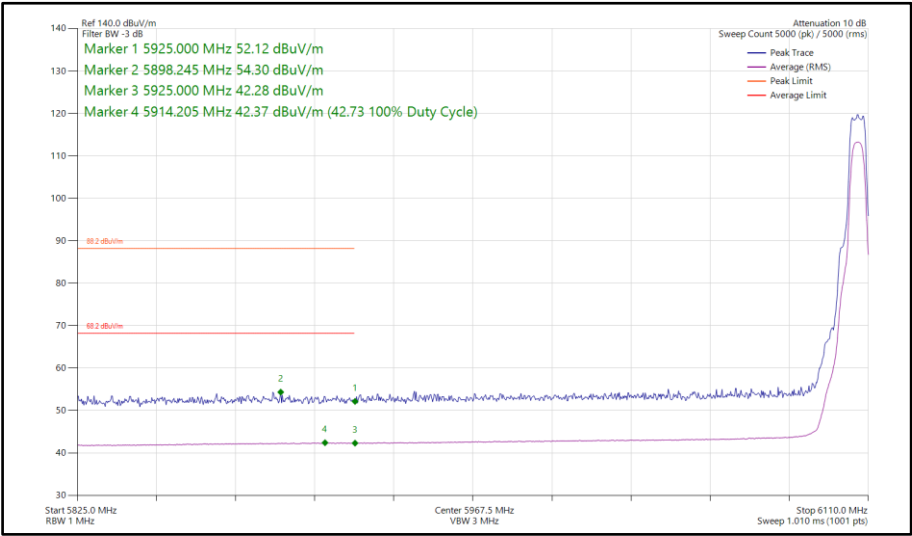
Figure 317 - XHDRPM8, SISO, Core 1 - 6106 MHz Band Edge Frequency 5925 MHz
