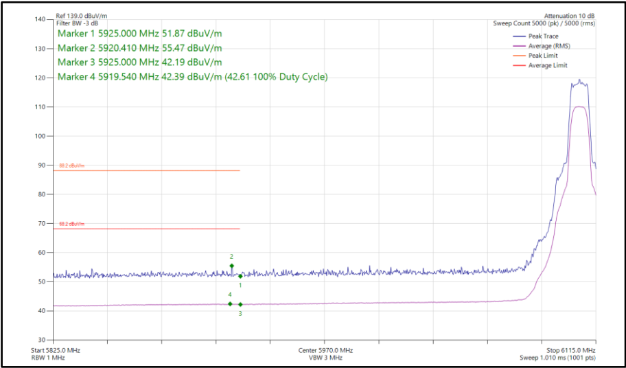
Figure 315 - HDRPL8, SISO, Core 1 - 6106 MHz Band Edge Frequency 5925 MHz
