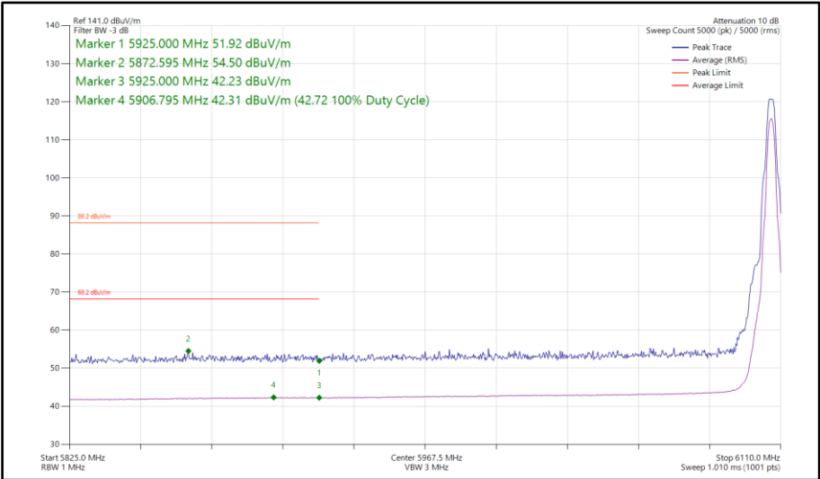
Figure 312 - HDT6, SISO, Core 1 - 6106 MHz Band Edge Frequency 5925 MHz
