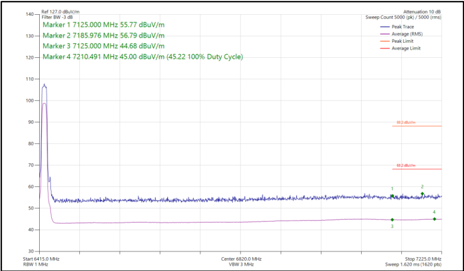
Figure 273 - HDRPL8, MIMO, Core 0-1 - 6425 MHz Band Edge Frequency 7125 MHz
