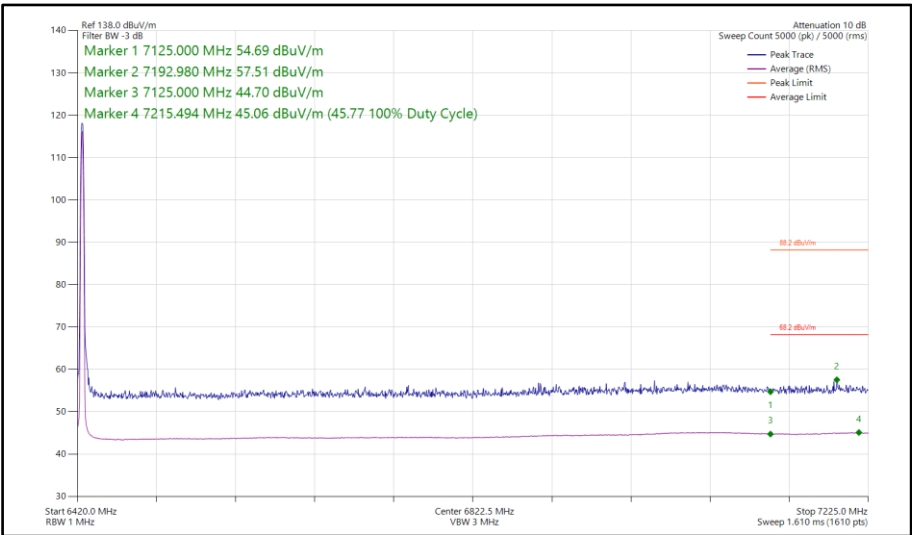
Figure 294 - LE1M, SISO, Core 0 - 6425 MHz Band Edge Frequency 7125 MHz
