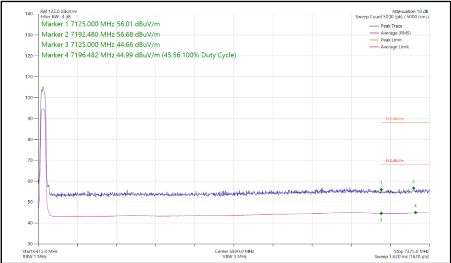
Figure 274 - HDRPL24, MIMO, Core 0-1 - 6425 MHz Band Edge Frequency 7125 MHz
