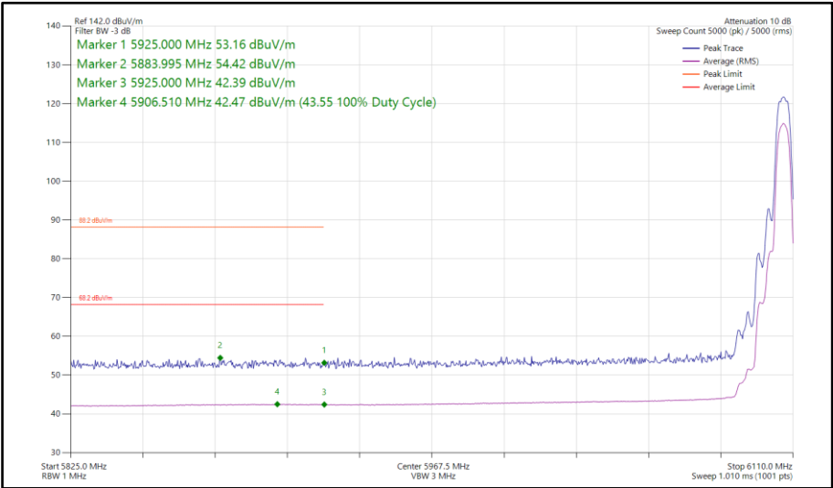
Figure 279 - HDR8, SISO, Core 0 - 6106 MHz Band Edge Frequency 5925 MHz
