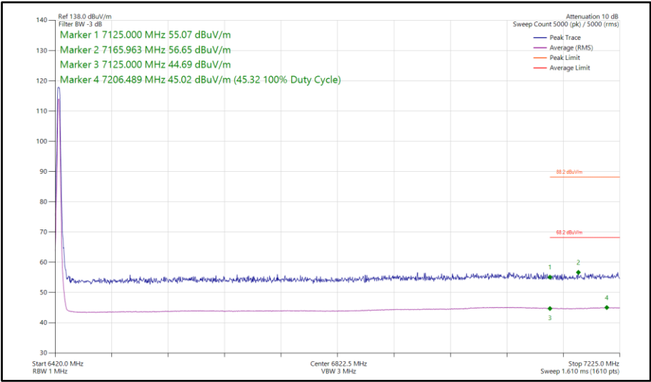
Figure 299 - HDRPS2, SISO, Core 0 - 6425 MHz Band Edge Frequency 7125 MHz
