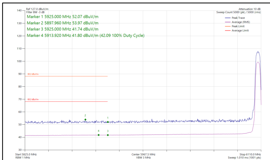
Figure 258 - HDRPM12, MIMO, Core 0-1 - 6106 MHz Band Edge Frequency 5925 MHz
