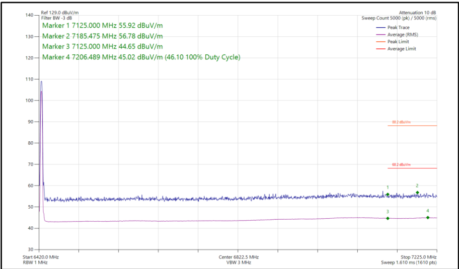
Figure 264 - HDR4, MIMO, Core 0-1 - 6425 MHz Band Edge Frequency 7125 MHz
