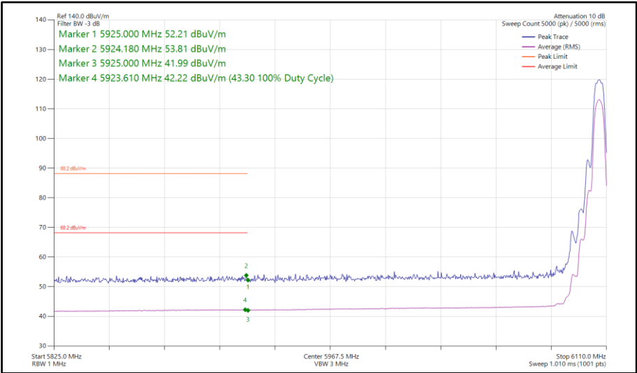
Figure 307 - HDR8, SISO, Core 1 - 6106 MHz Band Edge Frequency 5925 MHz
