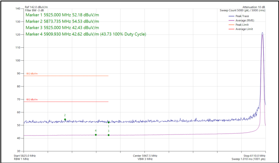
Figure 277 - DH5, SISO, Core 0 - 6106 MHz Band Edge Frequency 5925 MHz
