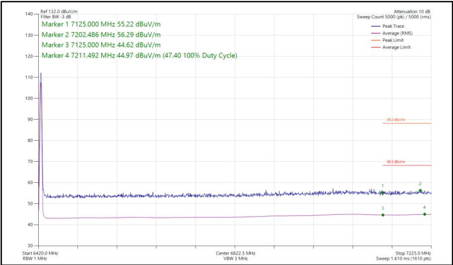
Figure 267 - LE2M, MIMO, Core 0-1 - 6425 MHz Band Edge Frequency 7125 MHz
