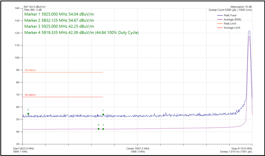
Figure 281 - LE2M, SISO, Core 0 - 6106 MHz Band Edge Frequency 5925 MHz
