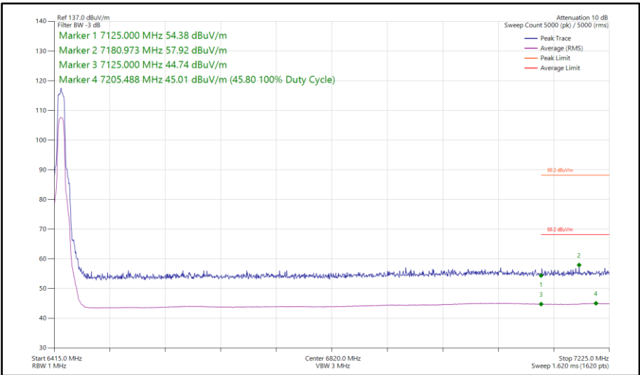
Figure 304 - XHDRPL24, SISO, Core 0 - 6425 MHz Band Edge Frequency 7125 MHz
