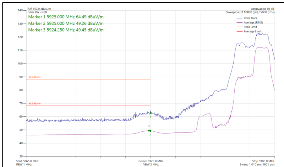
Figure 440 - 802.11be EHT40, RU 52+26-75, SISO, Core 0 - 5965 MHz Band Edge Frequency 5925 MHz
