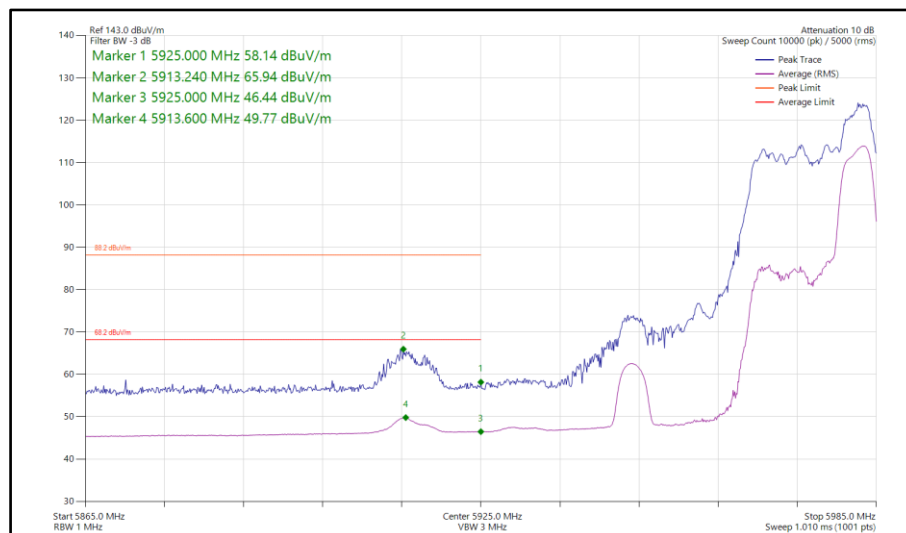
Figure 459 - 802.11ax HE40, RU 52-44, CDD, Core 0-1 - 5965 MHz Band Edge Frequency 5925 MHz
