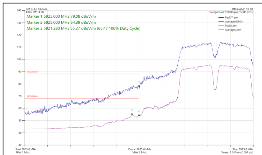
Figure 447 - 802.11a a40, SISO, Core 1 - 5965 MHz Band Edge Frequency 5925 MHz
