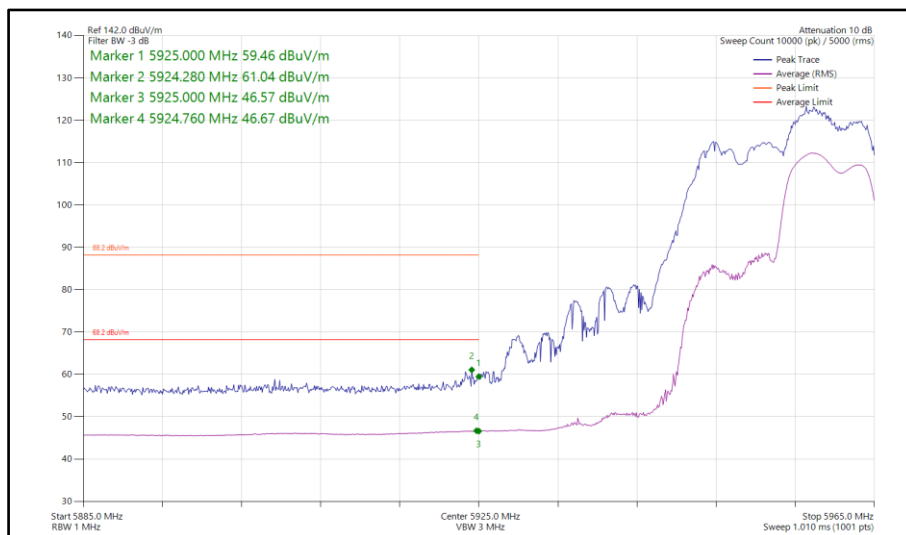
Figure 415 - 802.11ax HE20, RU 106-54, CDD, Core 0-1 - 5955 MHz Band Edge Frequency 5925 MHz
