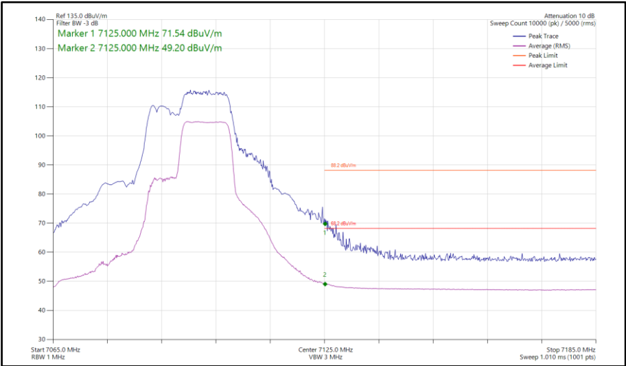
Figure 456 - 802.11be EHT40, RU 106+26-85, SISO, Core 1 - 7085 MHz Band Edge Frequency 7125 MHz
