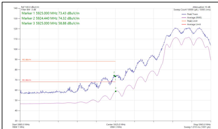
Figure 413 - 802.11a, CDD, Core 0-1 - 5955 MHz Band Edge Frequency 5925 MHz
