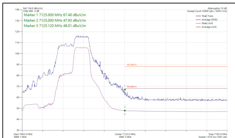
Figure 455 - 802.11ax HE40, RU 106-56, SISO, Core 1 - 7085 MHz Band Edge Frequency 7125 MHz
