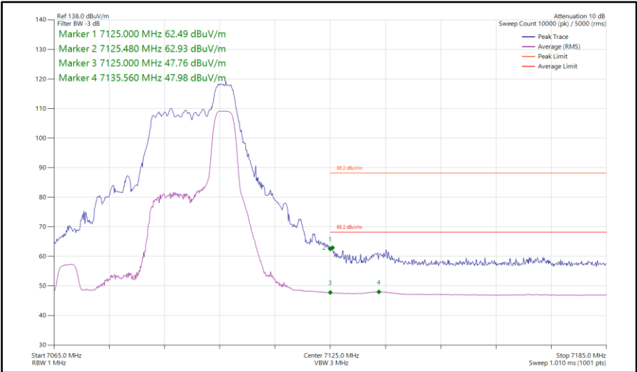
Figure 445 - 802.11ax HE40, RU 52-44, SISO, Core 0 - 7085 MHz Band Edge Frequency 7125 MHz
