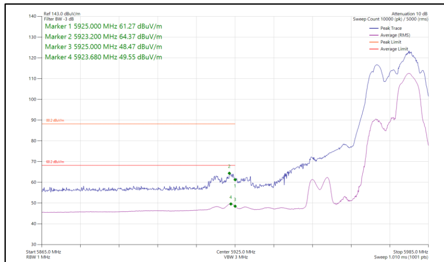
Figure 460 - 802.11be EHT40, RU 52+26-75, CDD, Core 0-1 - 5965 MHz Band Edge Frequency 5925 MHz
