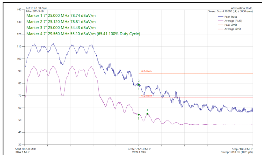
Figure 462 - 802.11a a40, CDD, Core 0-1 - 7085 MHz Band Edge Frequency 7125 MHz
