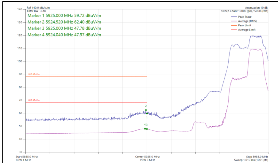
Figure 450 - 802.11be EHT40, RU 52+26-75, SISO, Core 1 - 5965 MHz Band Edge Frequency 5925 MHz
