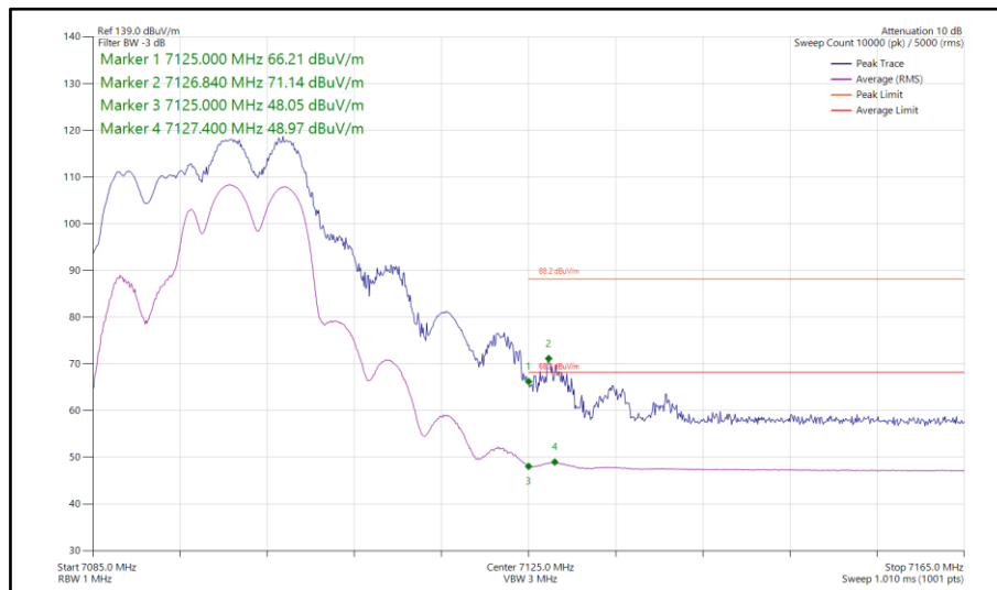
Figure 432 - 802.11be EHT20, RU 106+26-83, SDM, Core 0-1 - 7095 MHz Band Edge Frequency 7125 MHz
