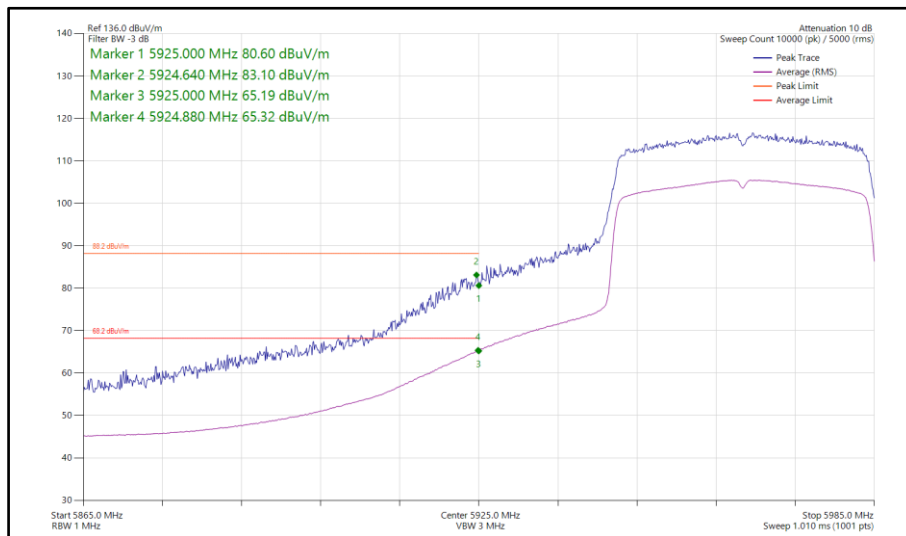
Figure 448 - 802.11ax HE40, SU, SISO, Core 1 - 5965 MHz Band Edge Frequency 5925 MHz
