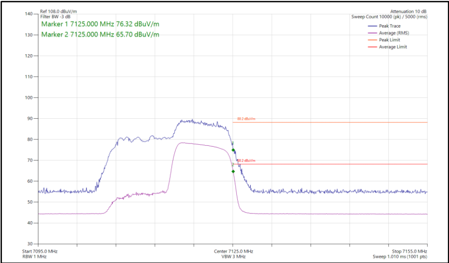
Figure 410 - 802.11ax HE20, RU 106-54, SISO, Core 1 - 7115 MHz Band Edge Frequency 7125 MHz
