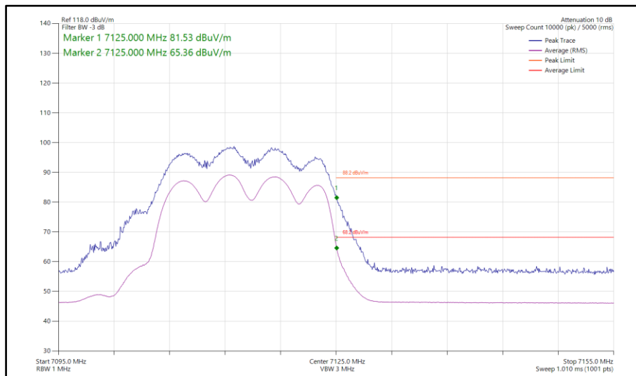
Figure 418 - 802.11a, CDD, Core 0-1 - 7115 MHz Band Edge Frequency 7125 MHz
