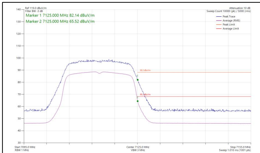
Figure 406 - 802.11a, SISO, Core 1 - 7115 MHz Band Edge Frequency 7125 MHz
