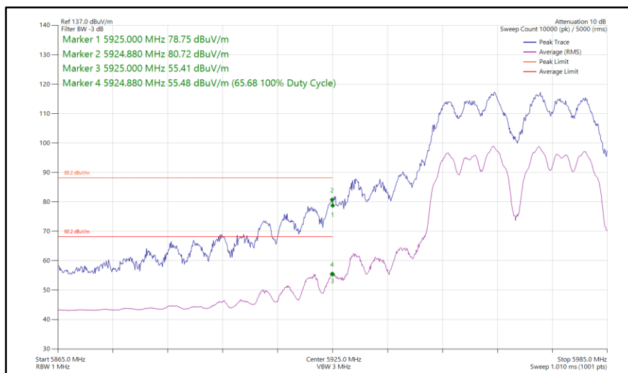
Figure 457 - 802.11a a40, CDD, Core 0-1 - 5965 MHz Band Edge Frequency 5925 MHz
