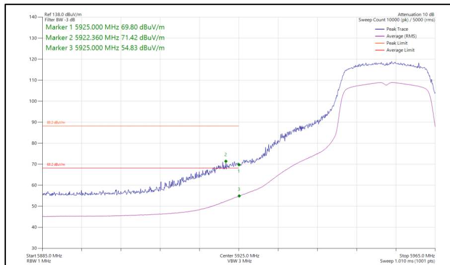
Figure 401 - 802.11a, SISO, Core 1 - 5955 MHz Band Edge Frequency 5925 MHz
