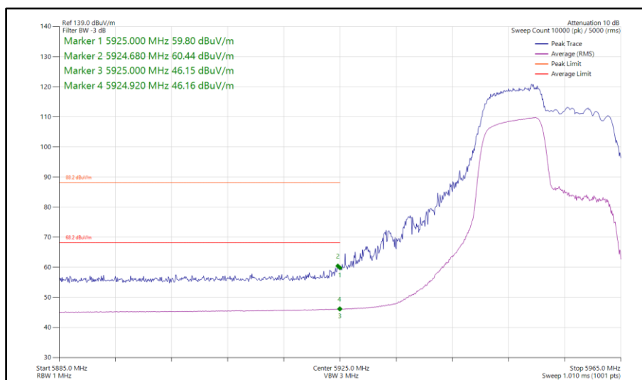
Figure 403 - 802.11ax HE20, RU 106-53, SISO, Core 1 - 5955 MHz Band Edge Frequency 5925 MHz
