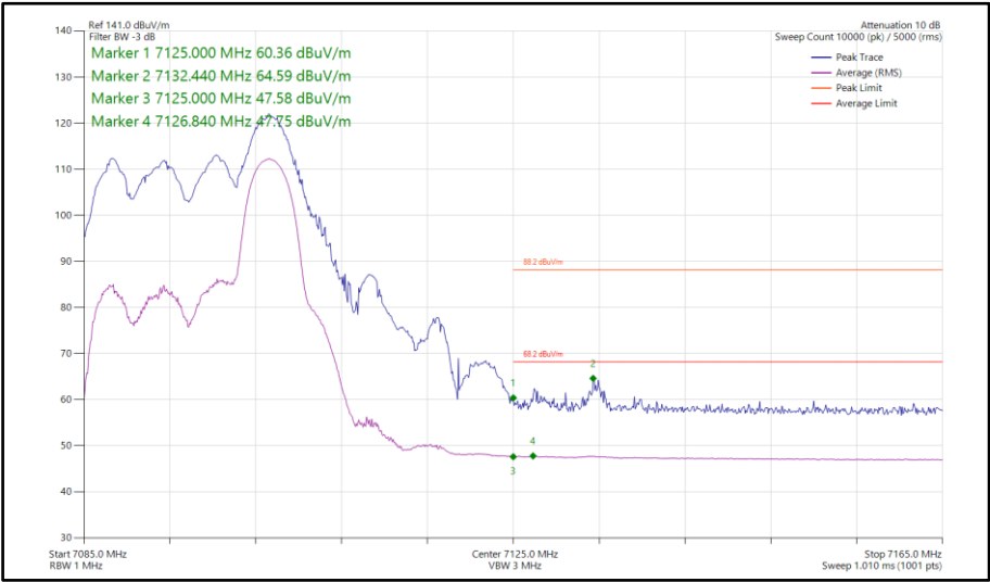
Figure 420 - 802.11ax HE20, RU 52-40, CDD, Core 0-1 - 7095 MHz Band Edge Frequency 7125 MHz
