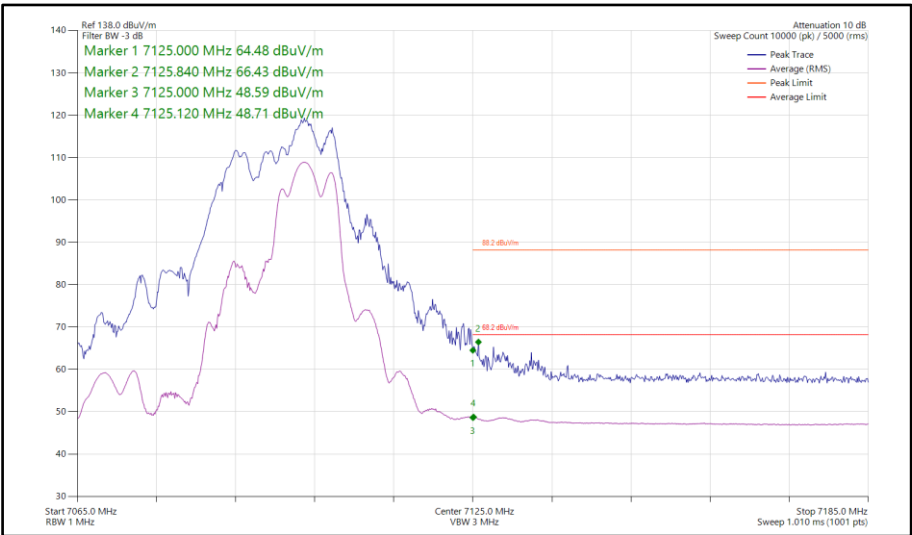
Figure 465 - 802.11ax HE40, RU 106-56, CDD, Core 0-1 - 7085 MHz Band Edge Frequency 7125 MHz
