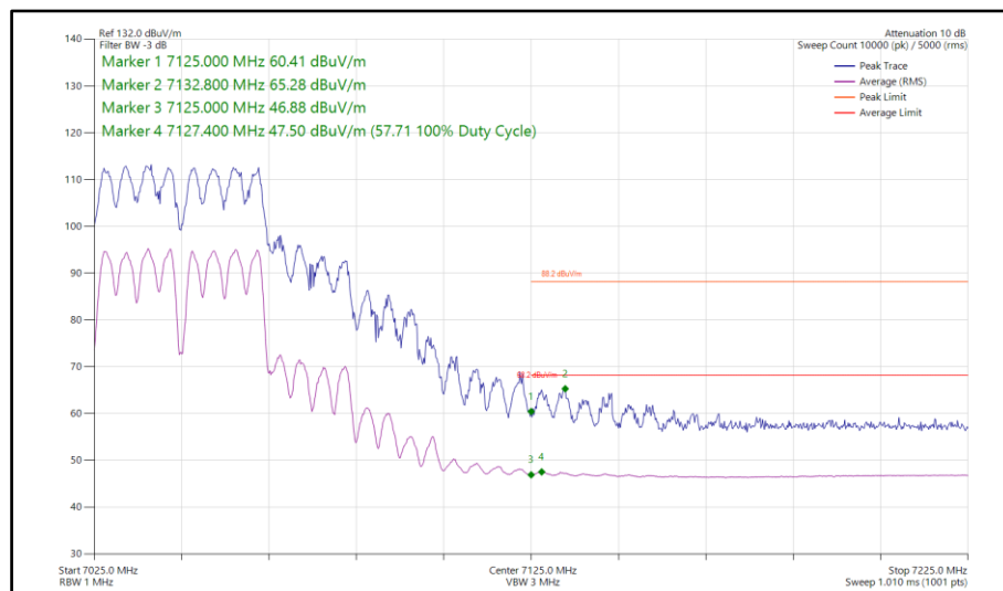
Figure 461 - 802.11a a40, CDD, Core 0-1 - 7045 MHz Band Edge Frequency 7125 MHz
