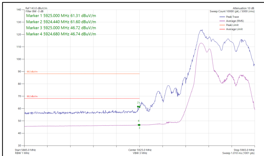
Figure 426 - 802.11ax HE20, RU 52-37, SDM, Core 0-1 - 5955 MHz Band Edge Frequency 5925 MHz
