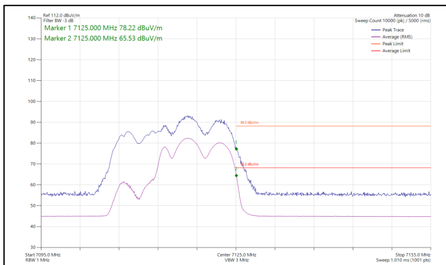
Figure 433 - 802.11be EHT20, RU 106+26-83, SDM, Core 0-1 - 7115 MHz Band Edge Frequency 7125 MHz
