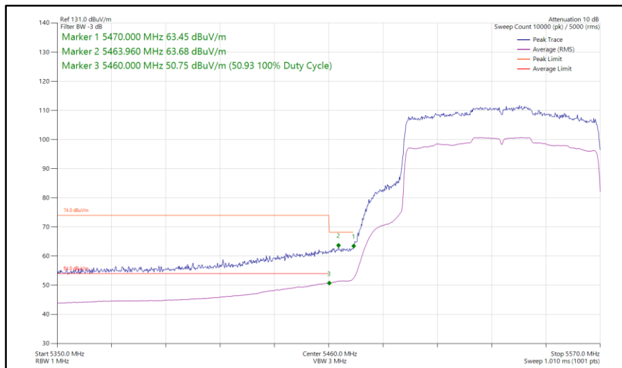
Figure 171 - 802.11ax HE80, SU, SISO, Core 0 - 5530 MHz Band Edge Frequency 5460 MHz
