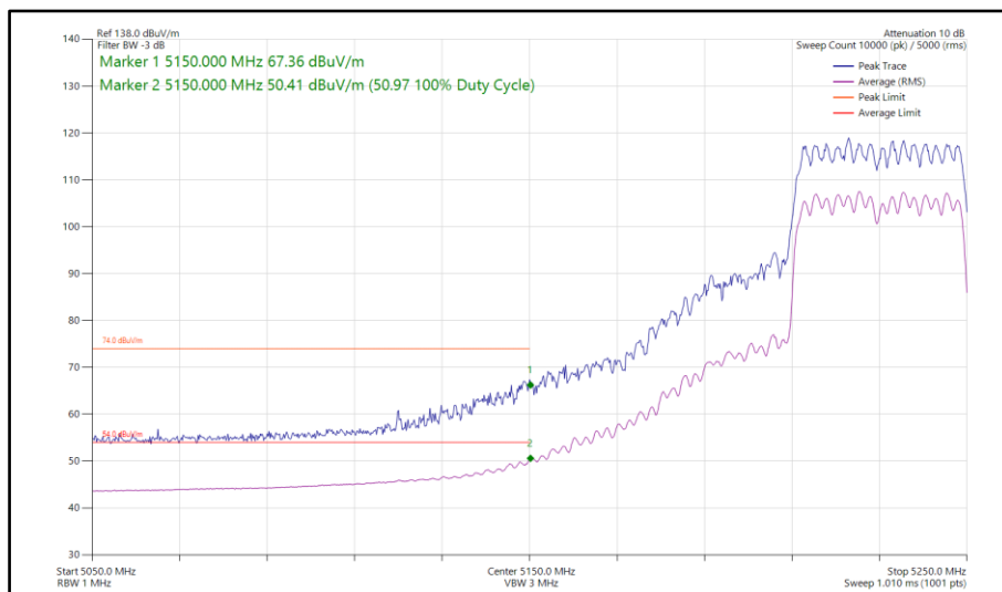
Figure 128 - 802.11ax HE40, SU, CDD, Core 0-1 - 5230 MHz Band Edge Frequency 5150 MHz
