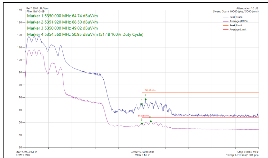
Figure 153 - 802.11ax HE40, RU 106-53, SDM, Core 0-1 - 5310 MHz Band Edge Frequency 5350 MHz
