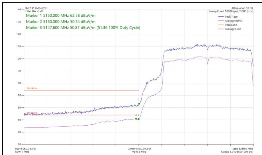
Figure 173 - 802.11ac VHT80, SISO, Core 1 - 5210 MHz Band Edge Frequency 5150 MHz
