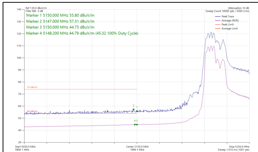
Figure 147 - 802.11ax HE40, RU 106-53, SDM, Core 0-1 - 5230 MHz Band Edge Frequency 5150 MHz
