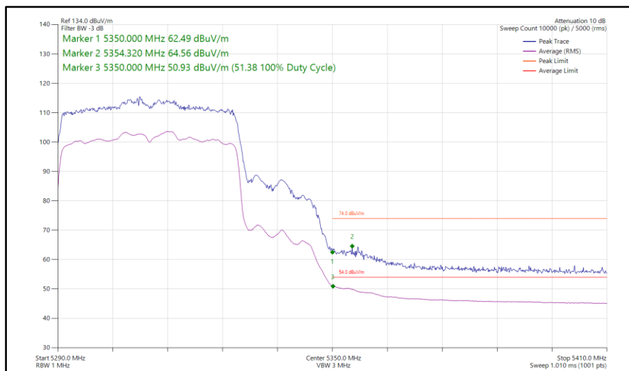
Figure 152 - 802.11ax HE40, SU, SDM, Core 0-1 - 5310 MHz Band Edge Frequency 5350 MHz
