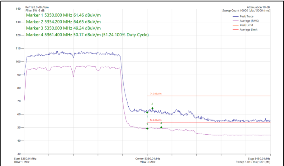
Figure 176 - 802.11ac VHT80, SISO, Core 1 - 5290 MHz Band Edge Frequency 5350 MHz
