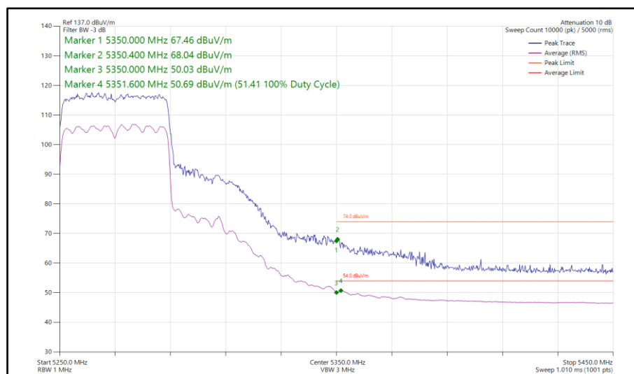
Figure 150 - 802.11ax HE40, SU, SDM, Core 0-1 - 5270 MHz Band Edge Frequency 5350 MHz
