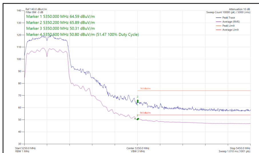
Figure 148 - 802.11n HT40, SDM, Core 0-1 - 5270 MHz Band Edge Frequency 5350 MHz
