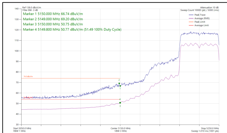
Figure 146 - 802.11ax HE40, SU, SDM, Core 0-1 - 5230 MHz Band Edge Frequency 5150 MHz
