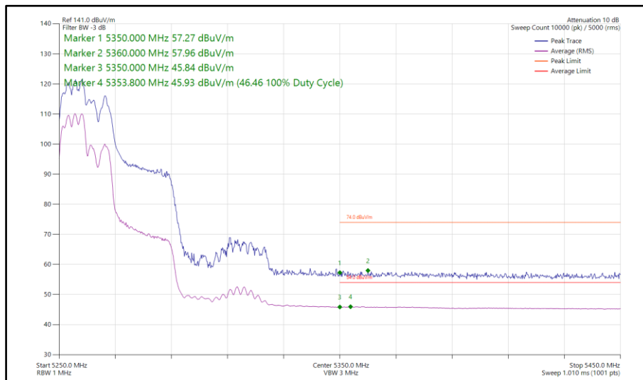
Figure 151 - 802.11ax HE40, RU 106-53, SDM, Core 0-1 - 5270 MHz Band Edge Frequency 5350 MHz
