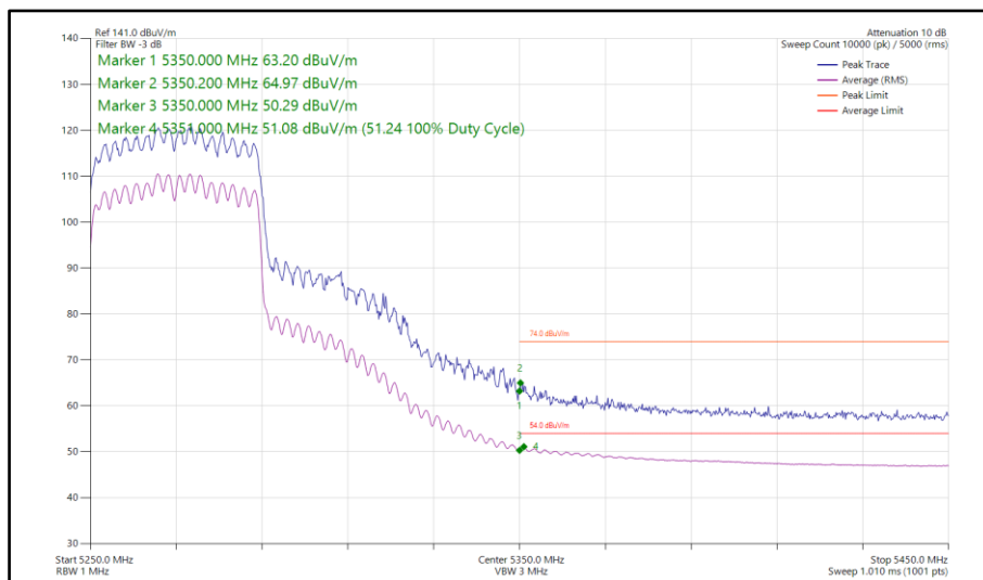
Figure 132 - 802.11ax HE40, SU, CDD, Core 0-1 - 5270 MHz Band Edge Frequency 5350 MHz
