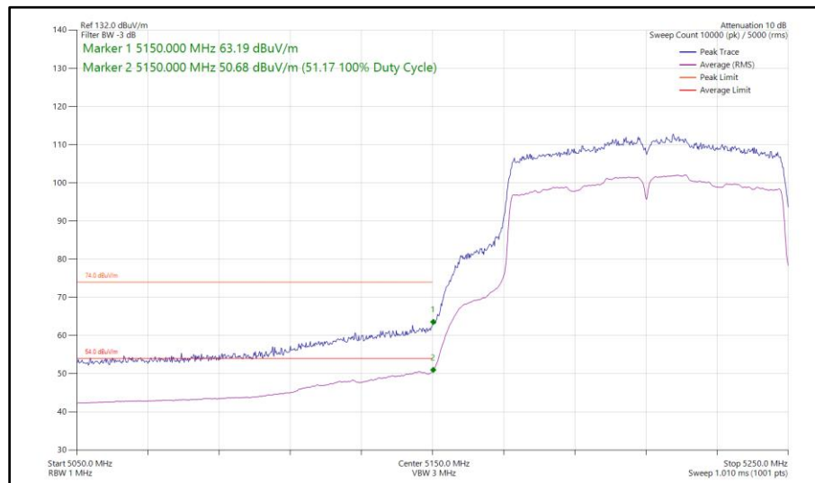
Figure 164 - 802.11ac VHT80, SISO, Core 0 - 5210 MHz Band Edge Frequency 5150 MHz
