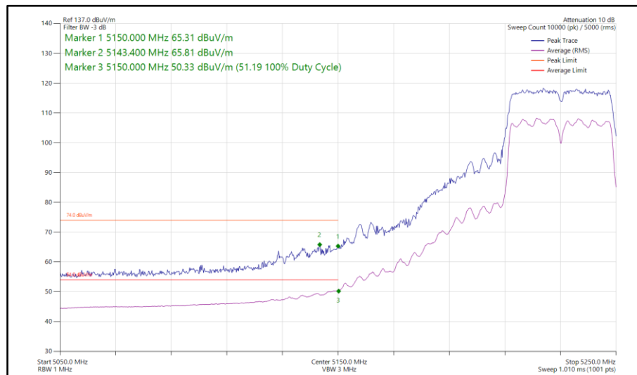
Figure 143 - 802.11n HT40, SDM, Core 0-1 - 5230 MHz Band Edge Frequency 5150 MHz
