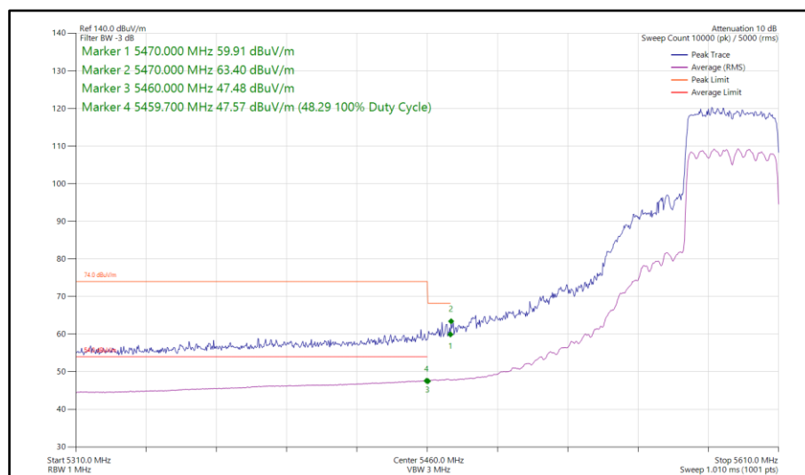
Figure 160 - 802.11ax HE40, SU, SDM, Core 0-1 - 5590 MHz Band Edge Frequency 5460 MHz
