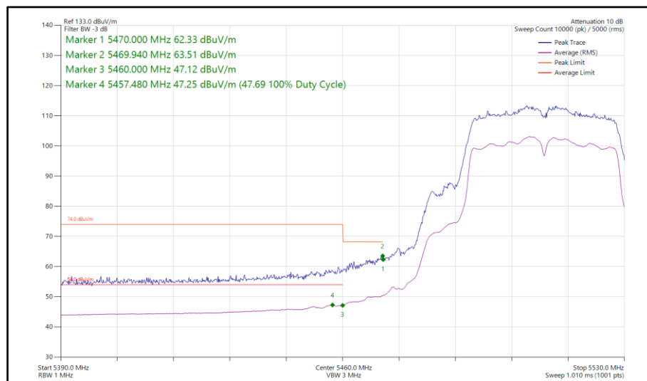
Figure 154 - 802.11n HT40, SDM, Core 0-1 - 5510 MHz Band Edge Frequency 5460 MHz
