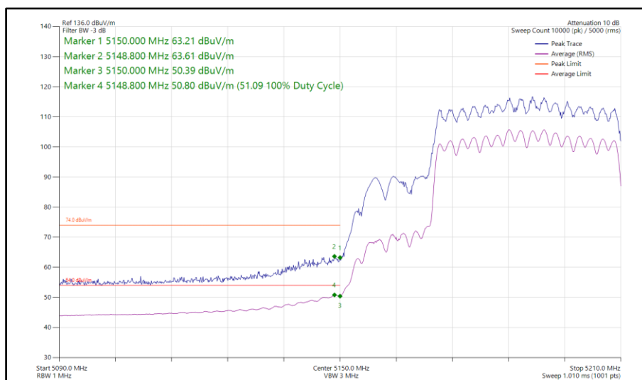
Figure 126 - 802.11ax HE40, SU, CDD, Core 0-1 - 5190 MHz Band Edge Frequency 5150 MHz
