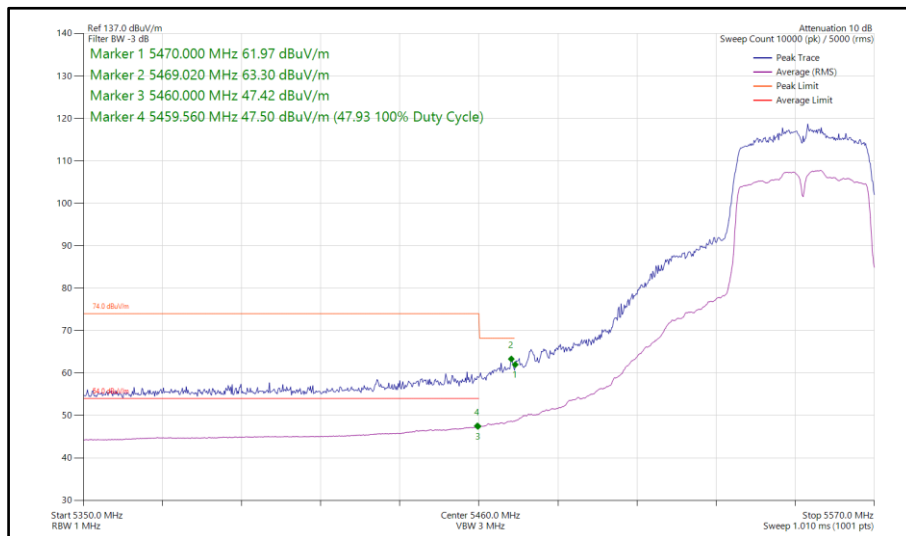
Figure 119 - 802.11n HT40, SISO, Core 1 - 5550 MHz Band Edge Frequency 5460 MHz
