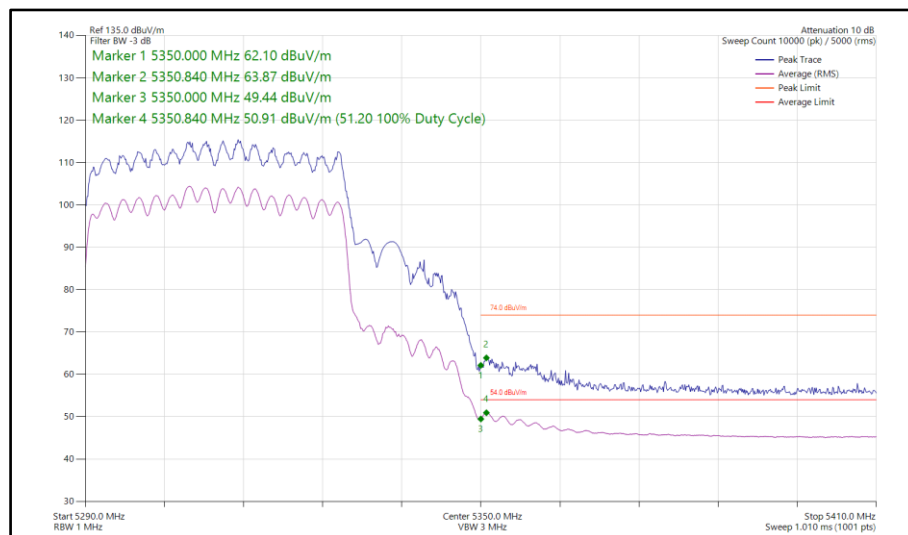
Figure 134 - 802.11ax HE40, SU, CDD, Core 0-1 - 5310 MHz Band Edge Frequency 5350 MHz
