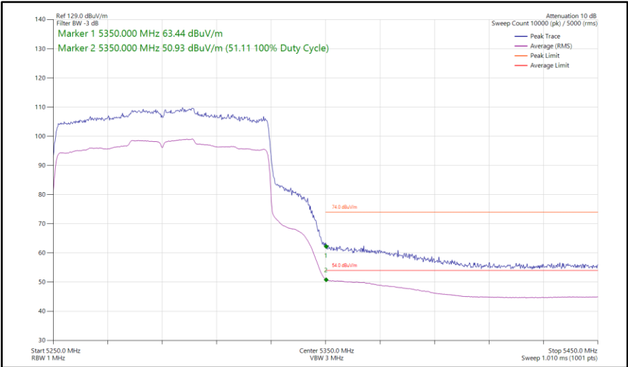
Figure 177 - 802.11ax HE80, SU, SISO, Core 1 - 5290 MHz Band Edge Frequency 5350 MHz
