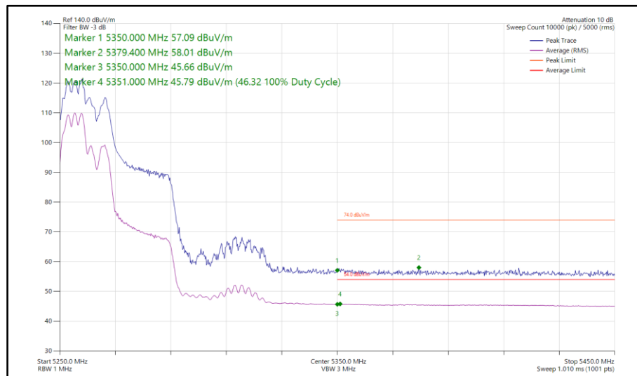
Figure 133 - 802.11ax HE40, RU 106-53, CDD, Core 0-1 - 5270 MHz Band Edge Frequency 5350 MHz
