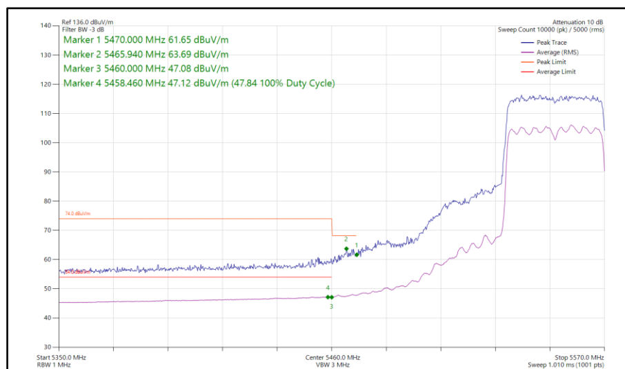
Figure 158 - 802.11ax HE40, SU, SDM, Core 0-1 - 5550 MHz Band Edge Frequency 5460 MHz
