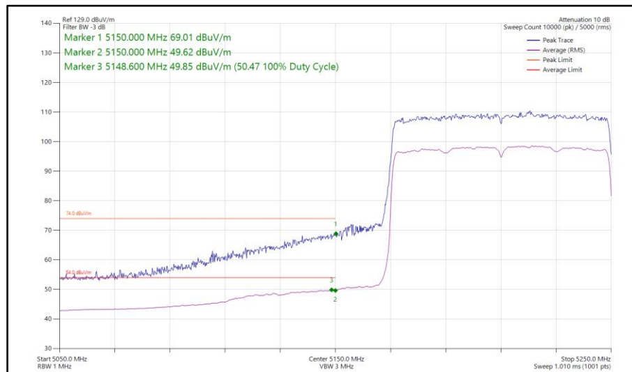
Figure 174 - 802.11ax HE80, SU, SISO, Core 1 - 5210 MHz Band Edge Frequency 5150 MHz
