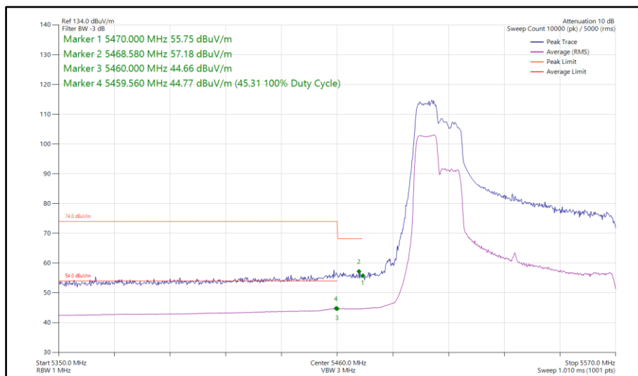
Figure 172 - 802.11ax HE80, RU 106-53, SISO, Core 0 - 5530 MHz Band Edge Frequency 5460 MHz
