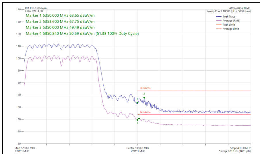
Figure 131 - 802.11n HT40, CDD, Core 0-1 - 5310 MHz Band Edge Frequency 5350 MHz
