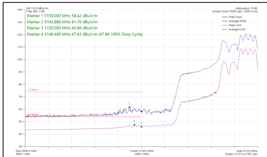
Figure 145 - 802.11ax HE40, RU 106-56, SDM, Core 0-1 - 5190 MHz Band Edge Frequency 5150 MHz
