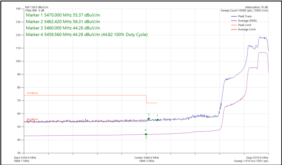
Figure 123 - 802.11ax HE40, RU 106-56, SISO, Core 1 - 5550 MHz Band Edge Frequency 5460 MHz
