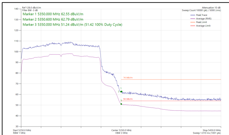
Figure 168 - 802.11ax HE80, SU, SISO, Core 0 - 5290 MHz Band Edge Frequency 5350 MHz
