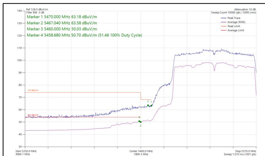
Figure 179 - 802.11ac VHT80, SISO, Core 1 - 5530 MHz Band Edge Frequency 5460 MHz
