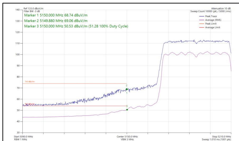
Figure 144 - 802.11ax HE40, SU, SDM, Core 0-1 - 5190 MHz Band Edge Frequency 5150 MHz
