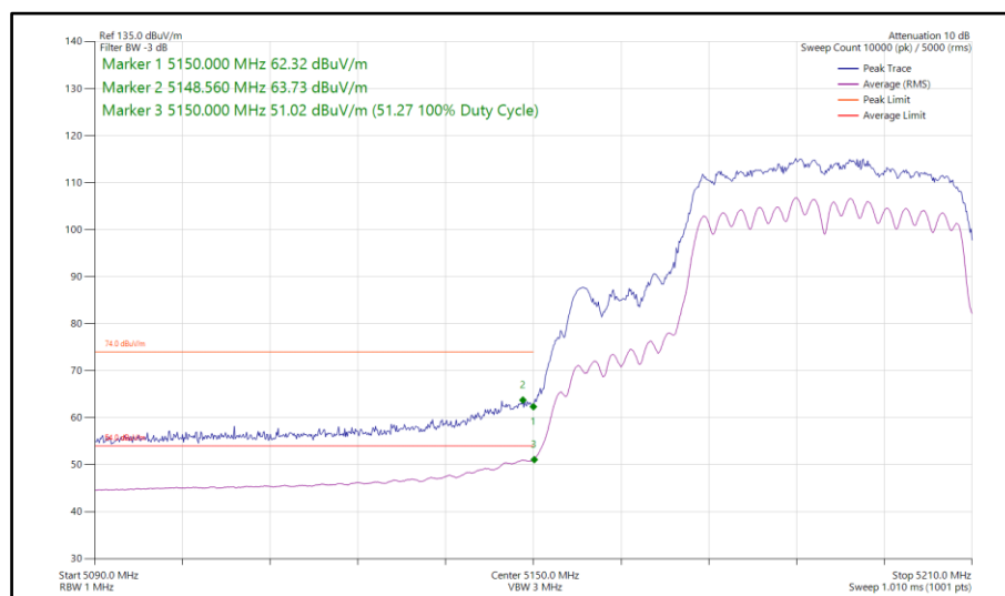
Figure 124 - 802.11n HT40, CDD, Core 0-1 - 5190 MHz Band Edge Frequency 5150 MHz
