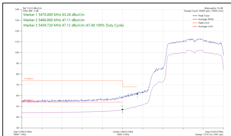
Figure 156 - 802.11ax HE40, SU, SDM, Core 0-1 - 5510 MHz Band Edge Frequency 5460 MHz
