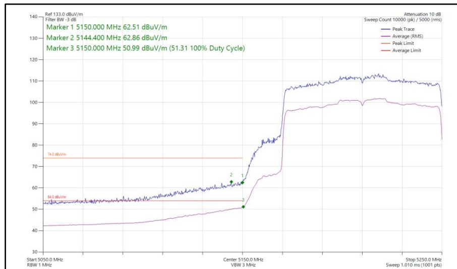
Figure 165 - 802.11ax HE80, SU, SISO, Core 0 - 5210 MHz Band Edge Frequency 5150 MHz
