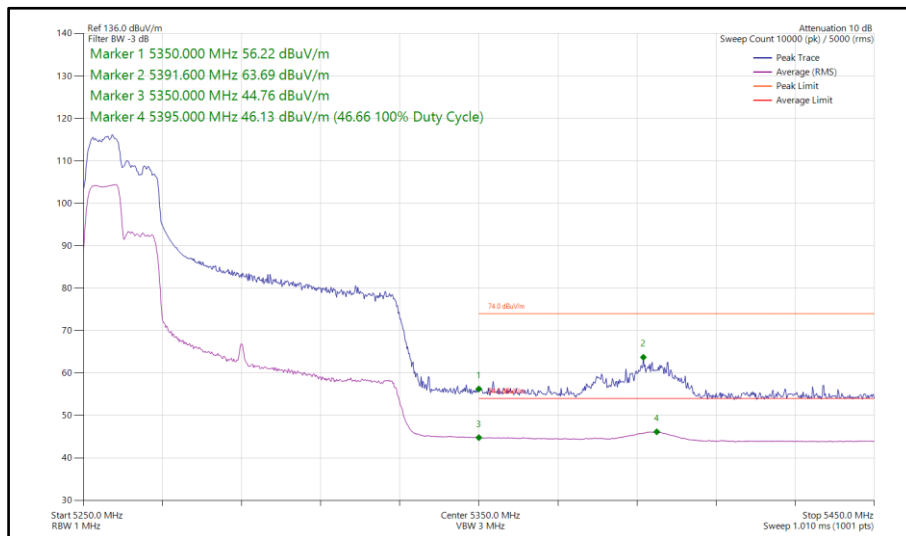
Figure 169 - 802.11ax HE80, RU 106-53, SISO, Core 0 - 5290 MHz Band Edge Frequency 5350 MHz
