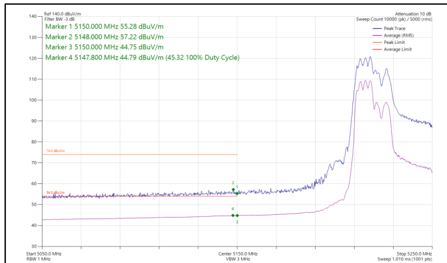
Figure 129 - 802.11ax HE40, RU 106-53, CDD, Core 0-1 - 5230 MHz Band Edge Frequency 5150 MHz
