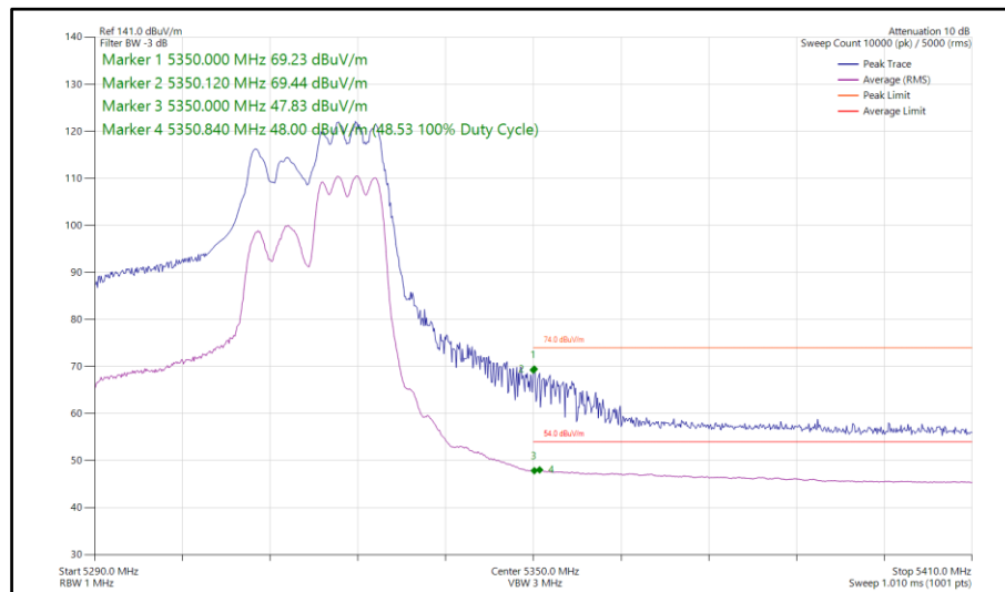
Figure 135 - 802.11ax HE40, RU 106-56, CDD, Core 0-1 - 5310 MHz Band Edge Frequency 5350 MHz
