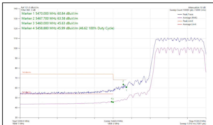
Figure 136 - 802.11n HT40, CDD, Core 0-1 - 5510 MHz Band Edge Frequency 5460 MHz
