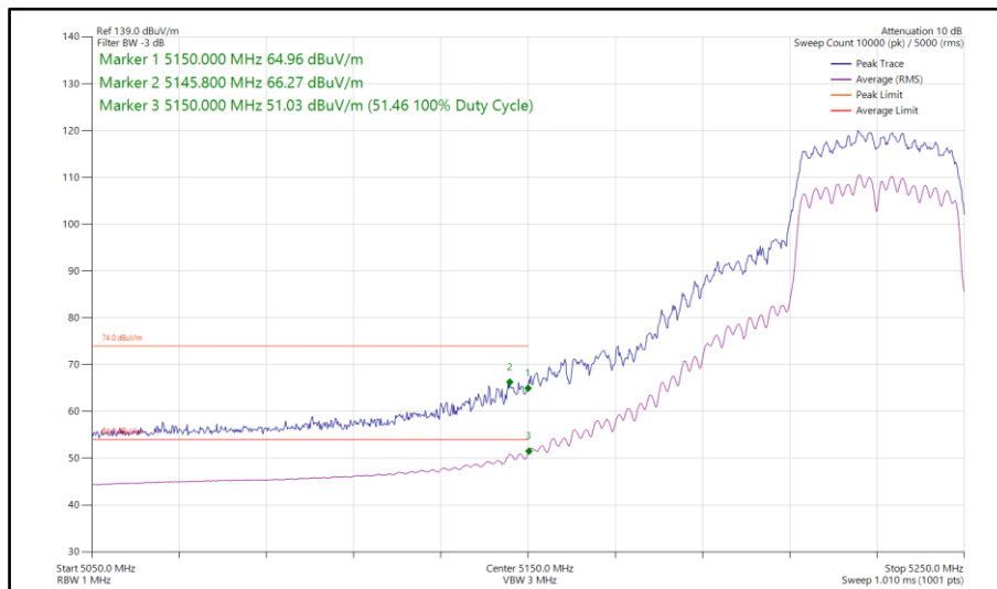
Figure 125 - 802.11n HT40, CDD, Core 0-1 - 5230 MHz Band Edge Frequency 5150 MHz
