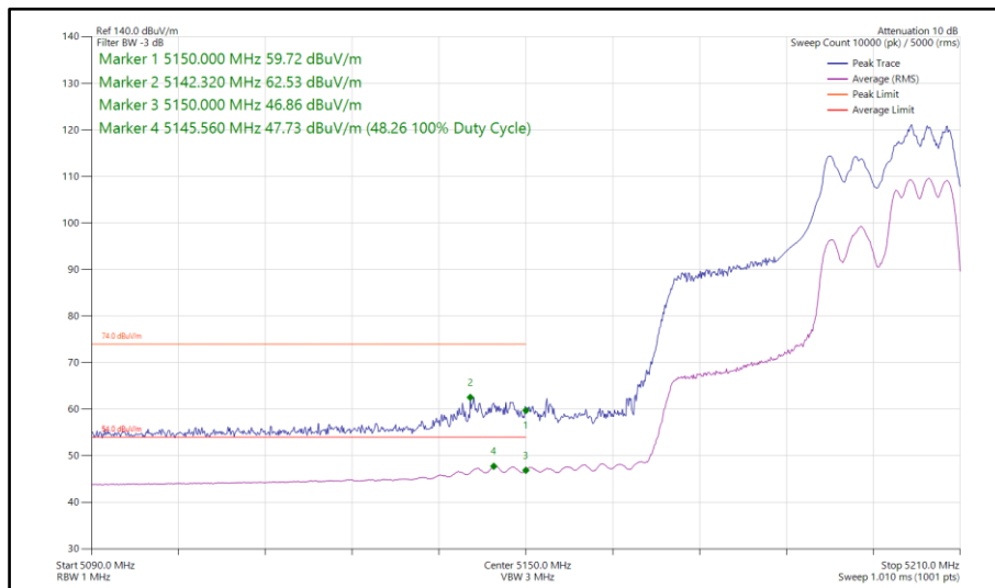
Figure 127 - 802.11ax HE40, RU 106-56, CDD, Core 0-1 - 5190 MHz Band Edge Frequency 5150 MHz
