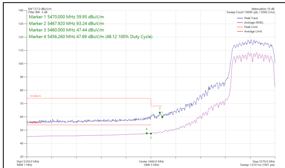
Figure 137 - 802.11n HT40, CDD, Core 0-1 - 5550 MHz Band Edge Frequency 5460 MHz
