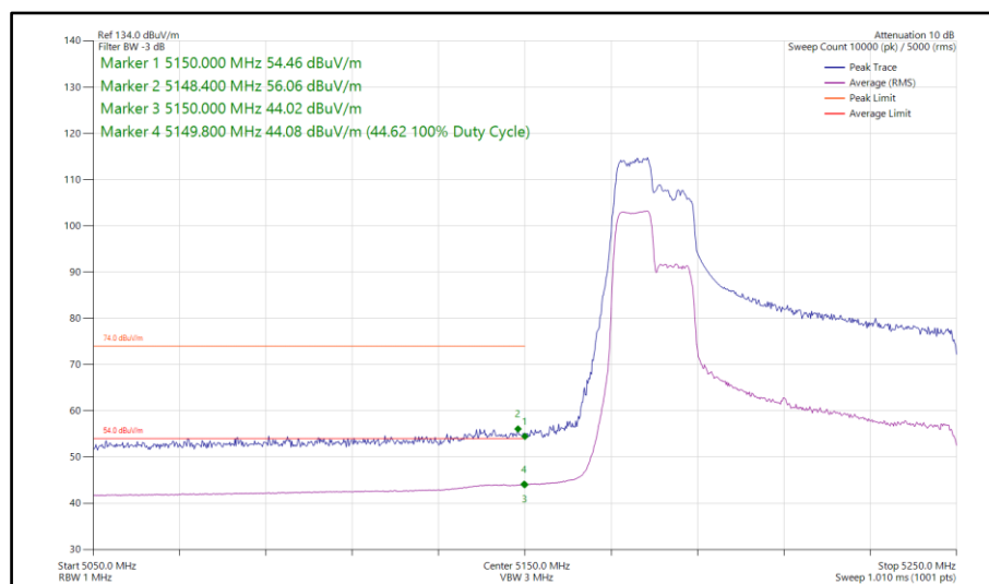
Figure 166 - 802.11ax HE80, RU 106-53, SISO, Core 0 - 5210 MHz Band Edge Frequency 5150 MHz
