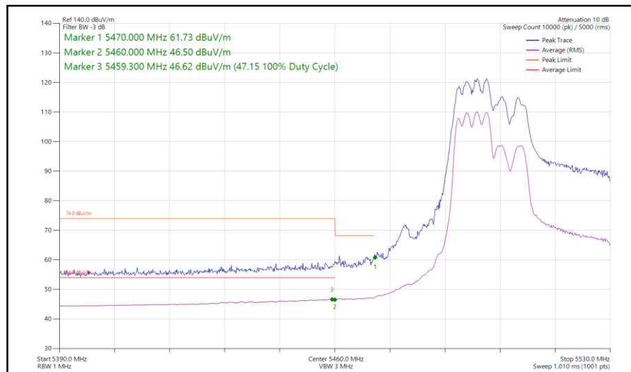
Figure 157 - 802.11ax HE40, RU 106-53, SDM, Core 0-1 - 5510 MHz Band Edge Frequency 5460 MHz
