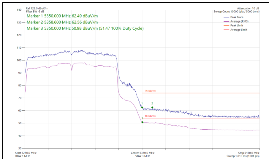
Figure 167 - 802.11ac VHT80, SISO, Core 0 - 5290 MHz Band Edge Frequency 5350 MHz
