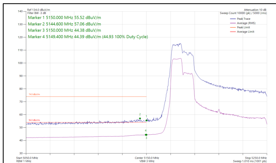
Figure 175 - 802.11ax HE80, RU 106-53, SISO, Core 1 - 5210 MHz Band Edge Frequency 5150 MHz
