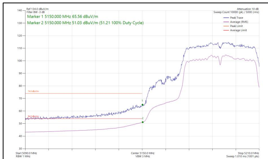
Figure 161 - 802.11ac VHT40, TxBF, Core 0-1 - 5190 MHz Band Edge Frequency 5150 MHz
