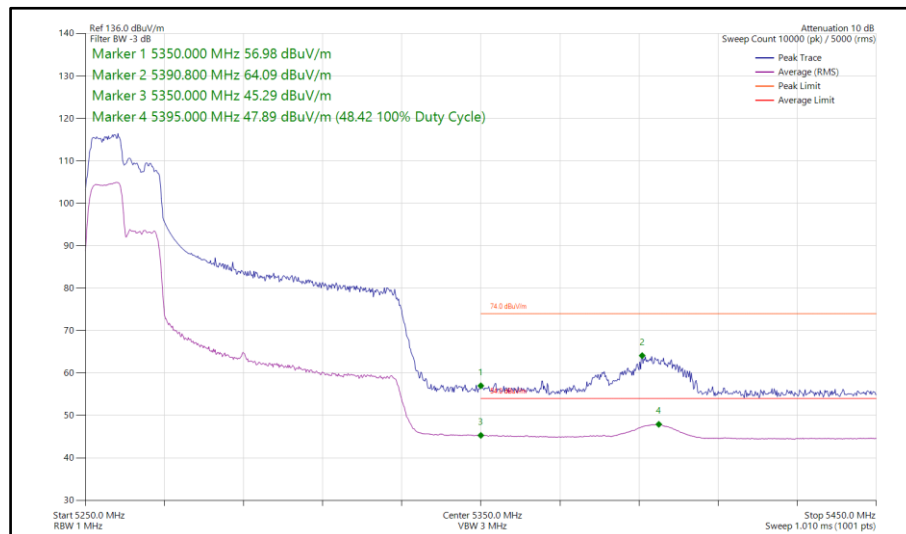
Figure 178 - 802.11ax HE80, RU 106-53, SISO, Core 1 - 5290 MHz Band Edge Frequency 5350 MHz
