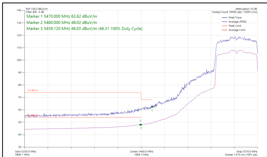
Figure 122 - 802.11ax HE40, SU, SISO, Core 1 - 5550 MHz Band Edge Frequency 5460 MHz
