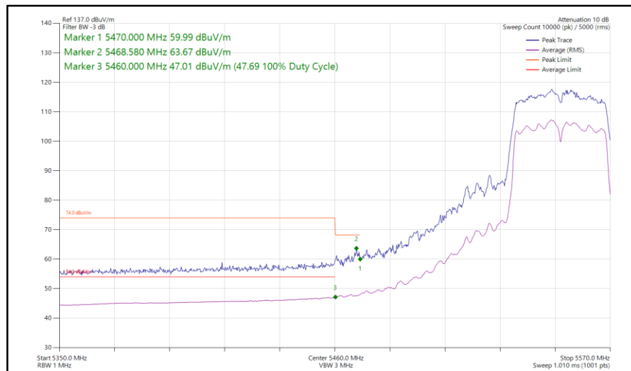
Figure 155 - 802.11n HT40, SDM, Core 0-1 - 5550 MHz Band Edge Frequency 5460 MHz
