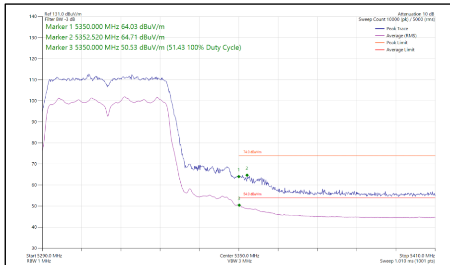
Figure 149 - 802.11n HT40, SDM, Core 0-1 - 5310 MHz Band Edge Frequency 5350 MHz
