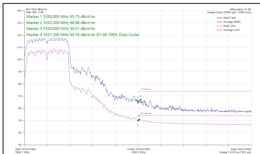
Figure 130 - 802.11n HT40, CDD, Core 0-1 - 5270 MHz Band Edge Frequency 5350 MHz
