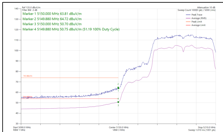
Figure 142 - 802.11n HT40, SDM, Core 0-1 - 5190 MHz Band Edge Frequency 5150 MHz
