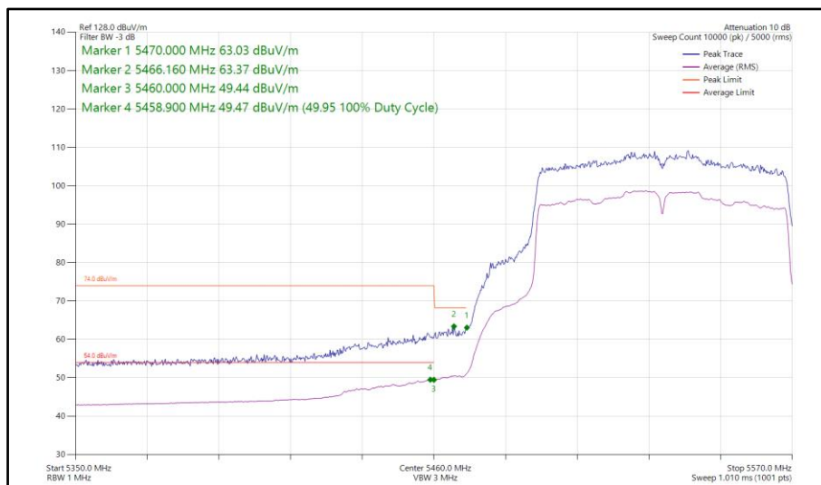
Figure 170 - 802.11ac VHT80, SISO, Core 0 - 5530 MHz Band Edge Frequency 5460 MHz
