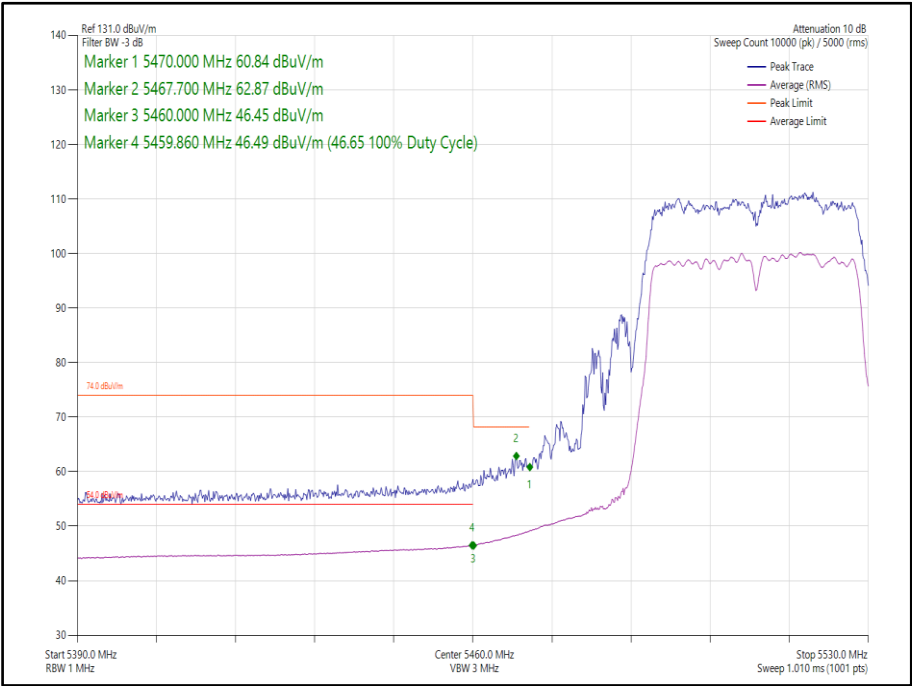
Figure 163 - 802.11ac VHT40, TxBF, Core 0-1 - 5510 MHz Band Edge Frequency 5460 MHz
