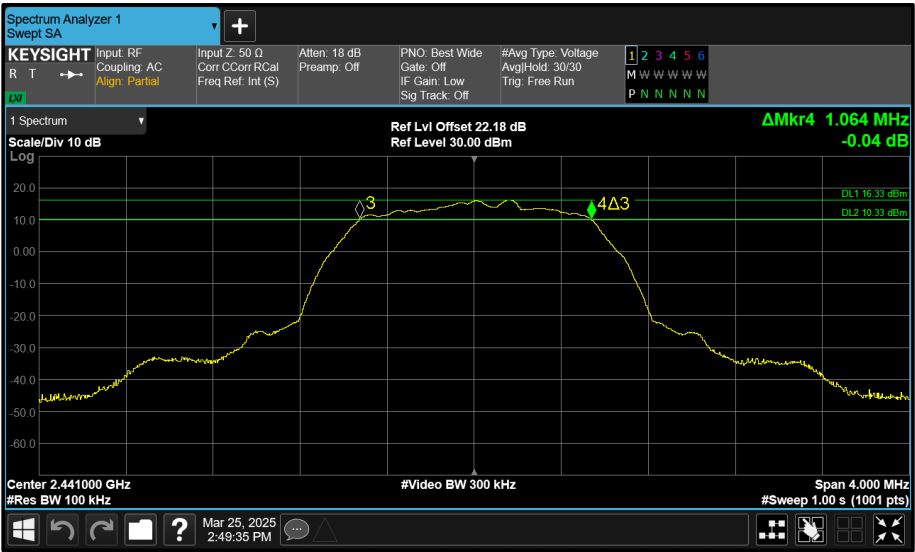
Figure 198 - Core 0 (A) 2441 MHz (CH39) 6 dB Bandwidth
