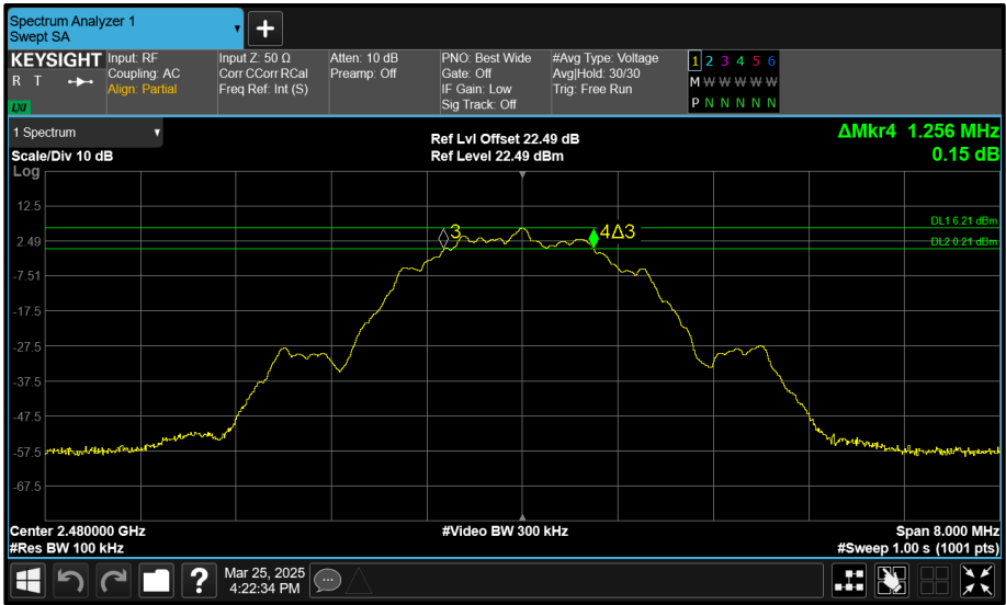
Figure 146 - Core 2 (C) 2480 MHz (CH39) 6 dB Bandwidth
