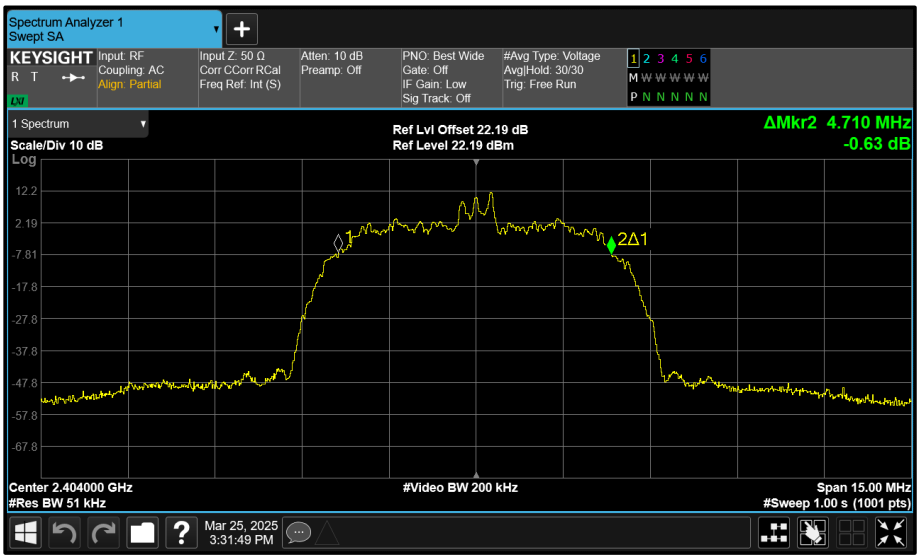
Figure 177 - Core 0 (A) 2404 MHz (CH2) 99% Bandwidth
