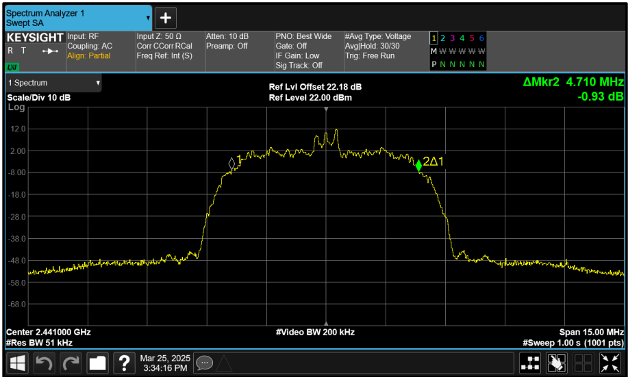
Figure 179 - Core 0 (A) 2441 MHz (CH39) 99% Bandwidth
