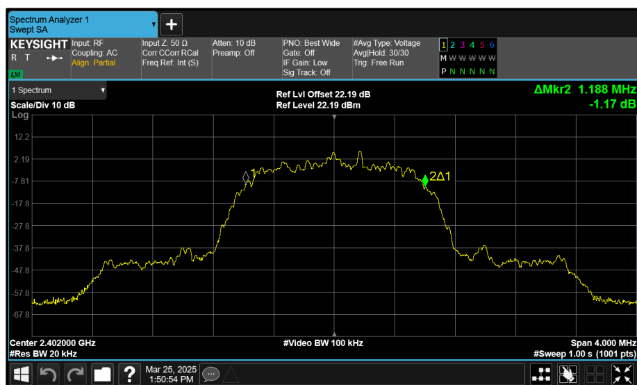
Figure 147 - Core 0 (A) 2402 MHz (CH0) 99% Bandwidth
