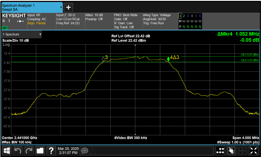
Figure 168 - Core 2 (C) 2441 MHz (CH39) 6 dB Bandwidth
