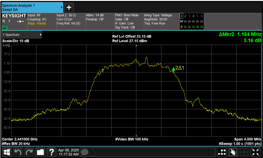
Figure 203 - Core 0 (A) 2441 MHz (CH39) 99% Bandwidth
