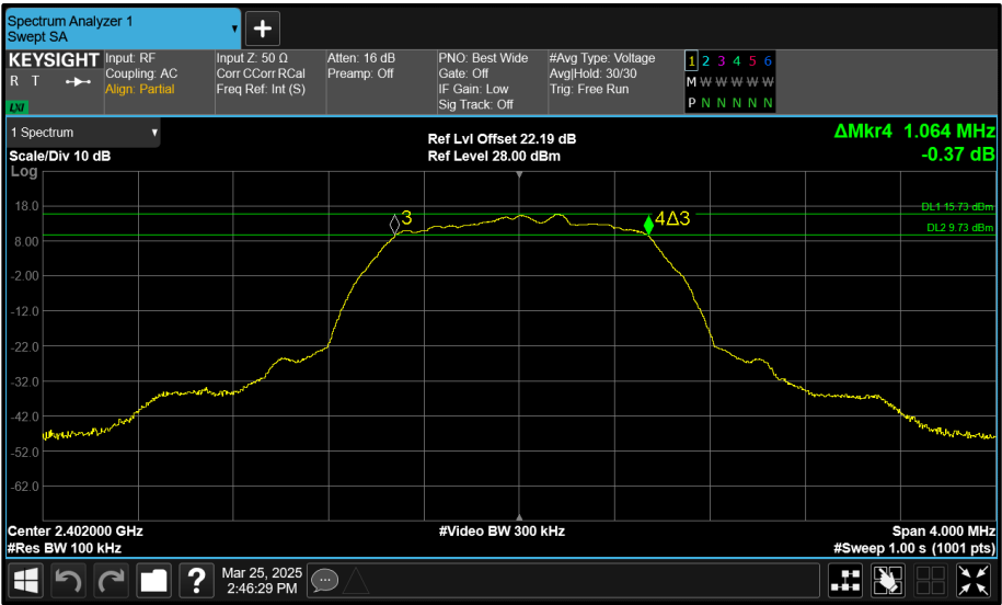
Figure 196 - Core 0 (A) 2402 MHz (CH0) 6 dB Bandwidth
