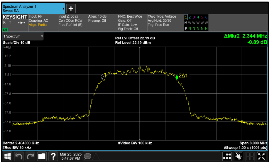
Figure 207 - Core 0 (A) 2404 MHz (CH2) 99% Bandwidth
