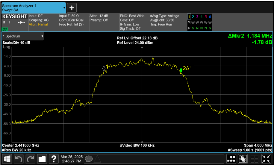
Figure 197 - Core 0 (A) 2441 MHz (CH39) 99% Bandwidth
