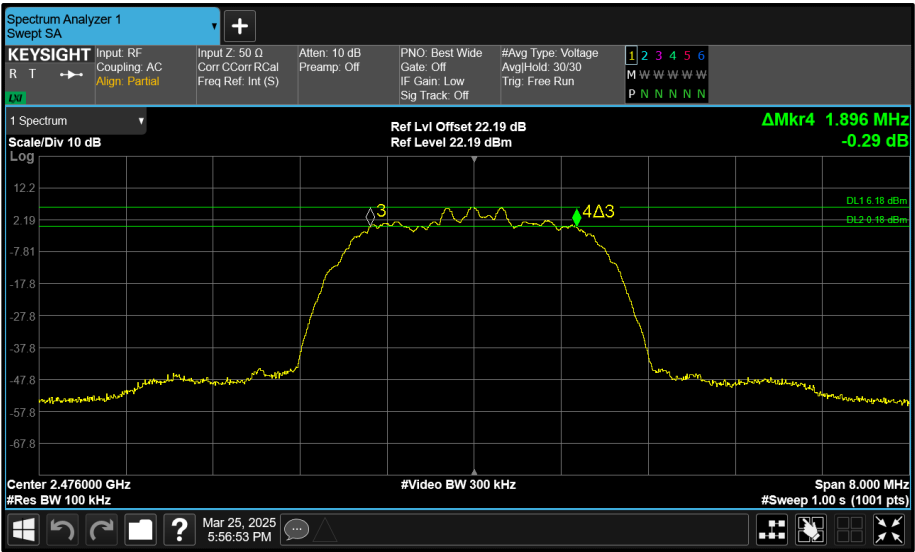
Figure 216 - Core 0 (A) 2476 MHz (CH74) 6 dB Bandwidth
