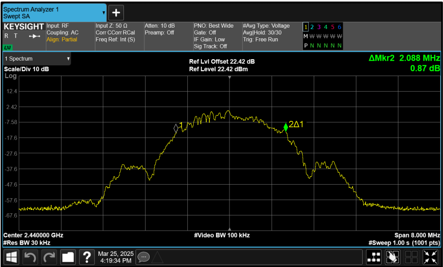
Figure 143 - Core 2 (C) 2440 MHz (CH17) 99% Bandwidth
