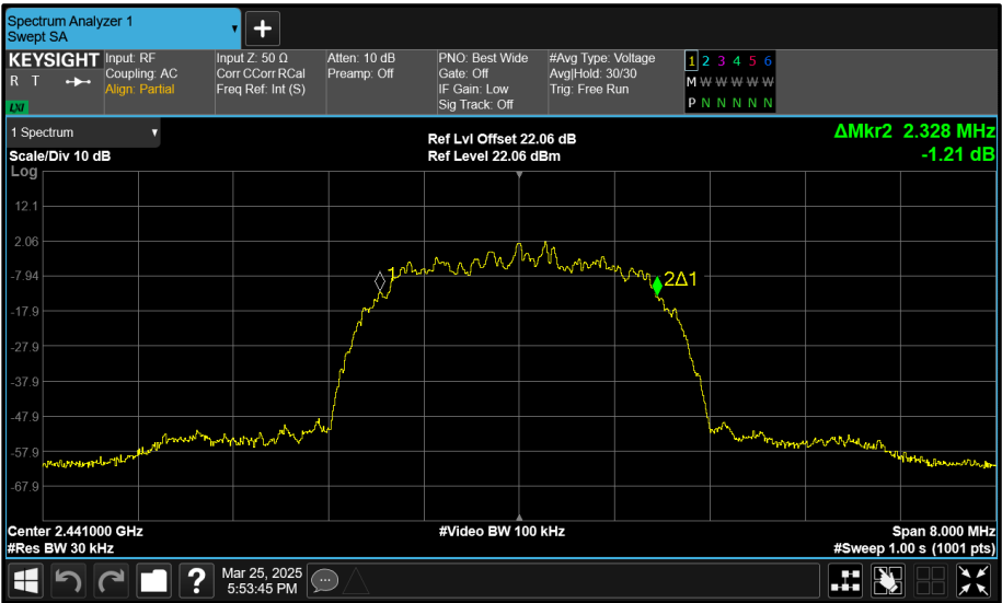
Figure 213 - Core 1 (B) 2441 MHz (CH39) 99% Bandwidth
