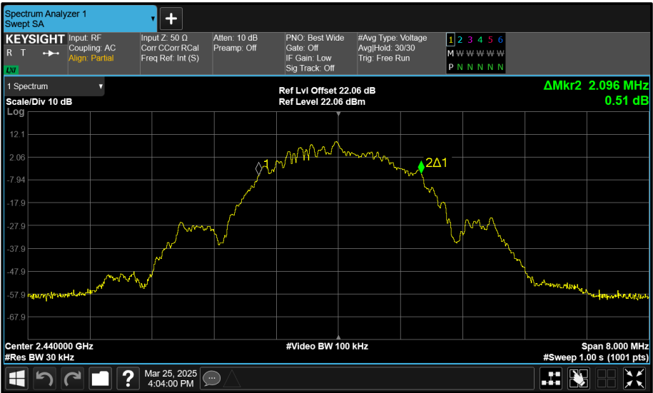
Figure 191 - Core 1 (B) 2440 MHz (CH17) 99% Bandwidth
