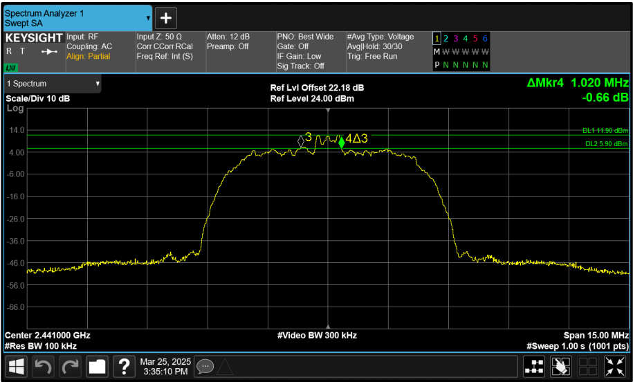
Figure 180 - Core 0 (A) 2441 MHz (CH39) 6 dB Bandwidth
