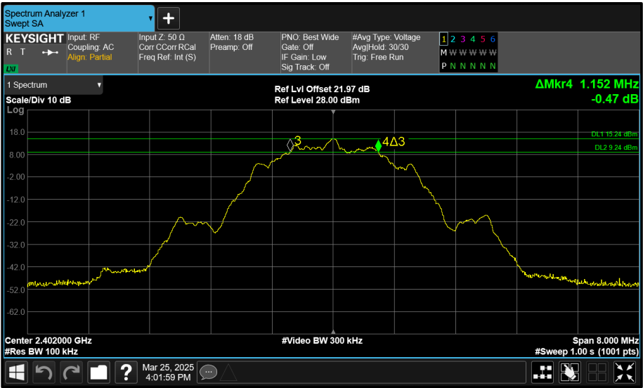
Figure 190 - Core 1 (B) 2402 MHz (CH37) 6 dB Bandwidth
