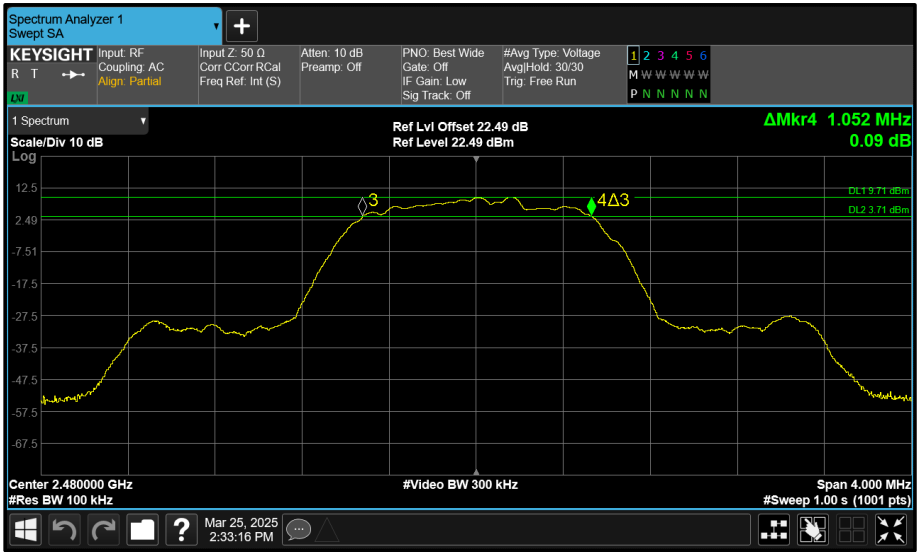
Figure 170 - Core 2 (C) 2480 MHz (CH78) 6 dB Bandwidth
