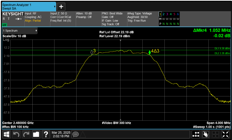
Figure 164 - Core 0 (A) 2480 MHz (CH78) 6 dB Bandwidth
