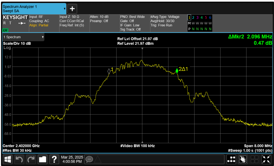
Figure 189 - Core 1 (B) 2402 MHz (CH37) 99% Bandwidth
