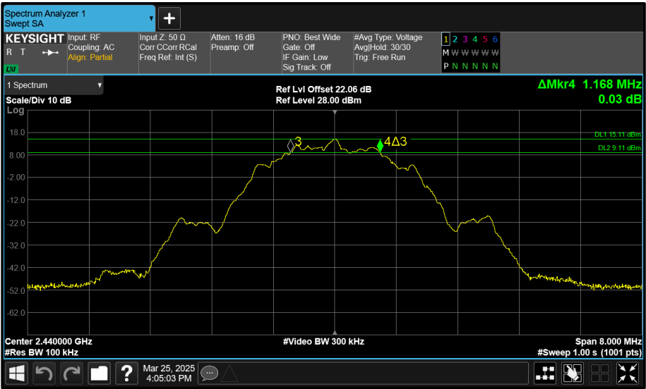
Figure 192 - Core 1 (B) 2440 MHz (CH17) 6 dB Bandwidth
