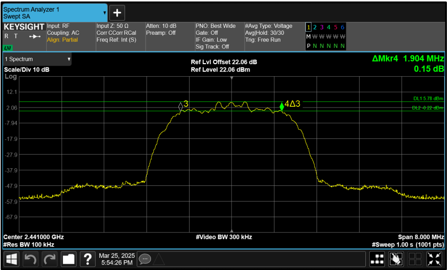
Figure 214 - Core 1 (B) 2441 MHz (CH39) 6 dB Bandwidth
