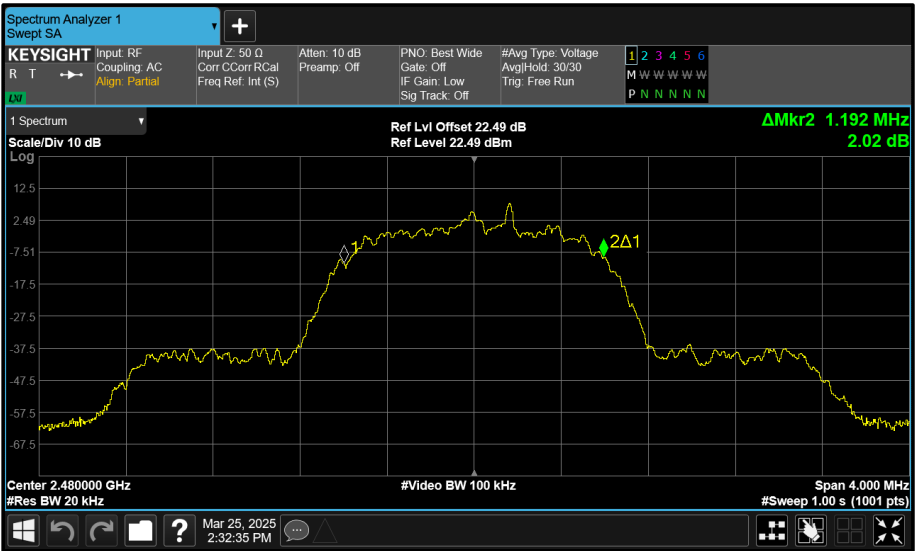
Figure 169 - Core 2 (C) 2480 MHz (CH78) 99% Bandwidth
