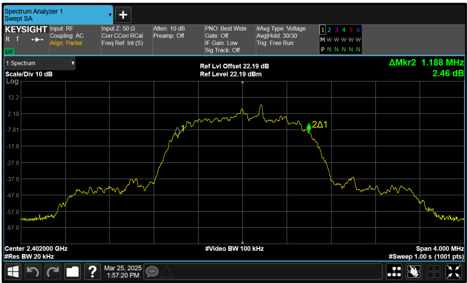
Figure 159 - Core 0 (A) 2402 MHz (CH0) 99% Bandwidth
