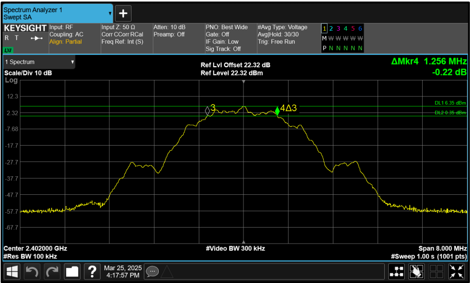
Figure 142 - Core 2 (C) 2402 MHz (CH37) 6 dB Bandwidth
