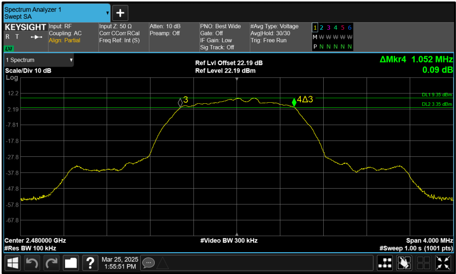
Figure 152 - Core 0 (A) 2480 MHz (CH78) 6 dB Bandwidth
