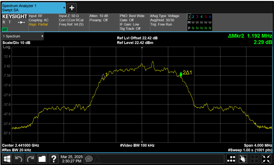
Figure 167 - Core 2 (C) 2441 MHz (CH39) 99% Bandwidth
