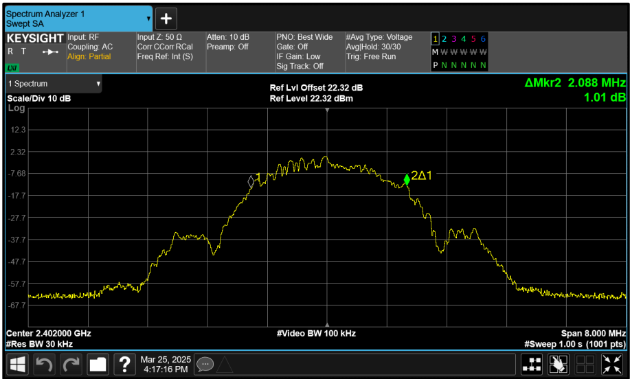
Figure 141 - Core 2 (C) 2402 MHz (CH37) 99% Bandwidth
