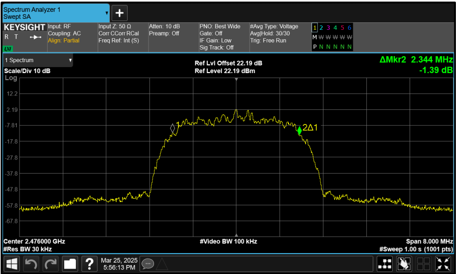
Figure 215 - Core 0 (A) 2476 MHz (CH74) 99% Bandwidth
