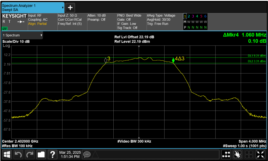
Figure 148 - Core 0 (A) 2402 MHz (CH0) 6 dB Bandwidth
