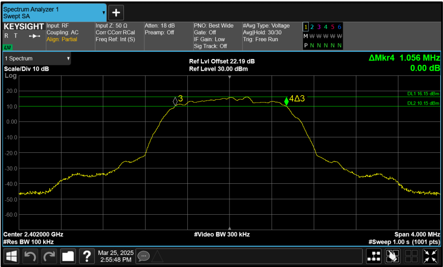
Figure 202 - Core 0 (A) 2402 MHz (CH0) 6 dB Bandwidth
