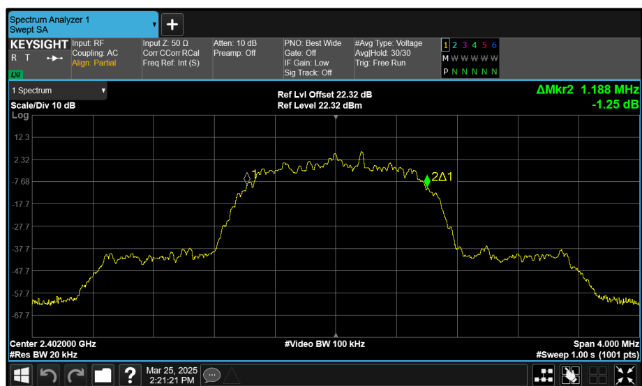
Figure 153 - Core 2 (C) 2402 MHz (CH0) 99% Bandwidth
