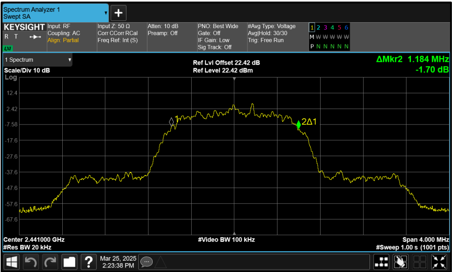
Figure 155 - Core 2 (C) 2441 MHz (CH39) 99% Bandwidth
