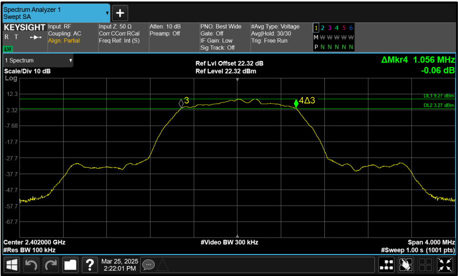
Figure 154 - Core 2 (C) 2402 MHz (CH0) 6 dB Bandwidth
