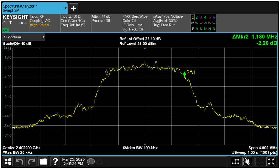
Figure 195 - Core 0 (A) 2402 MHz (CH0) 99% Bandwidth
