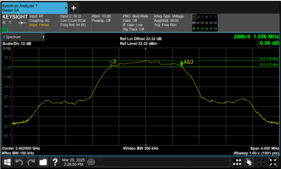
Figure 166 - Core 2 (C) 2402 MHz (CH0) 6 dB Bandwidth
