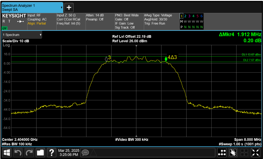
Figure 172 - Core 0 (A) 2404 MHz (CH2) 6 dB Bandwidth
