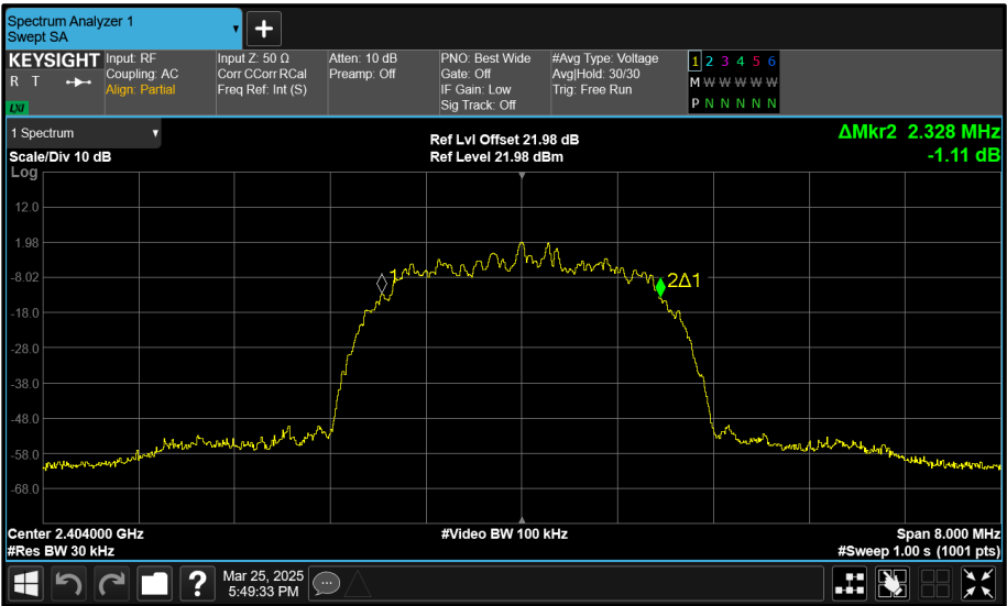
Figure 209 - Core 1 (B) 2404 MHz (CH2) 99% Bandwidth
