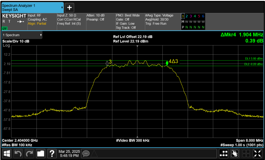
Figure 208 - Core 0 (A) 2404 MHz (CH2) 6 dB Bandwidth
