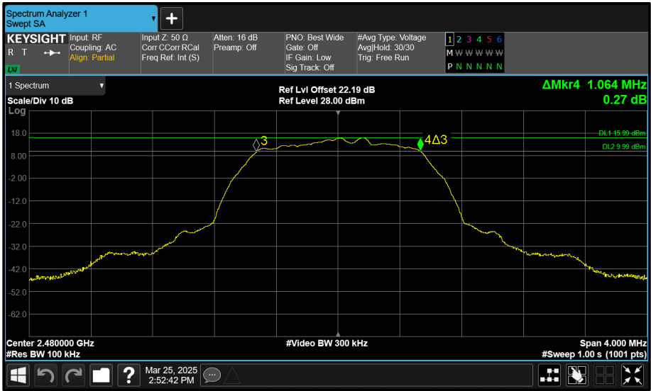
Figure 200 - Core 0 (A) 2480 MHz (CH78) 6 dB Bandwidth
