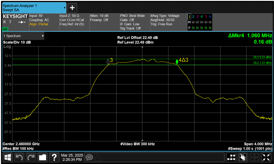
Figure 158 - Core 2 (C) 2480 MHz (CH78) 6 dB Bandwidth
