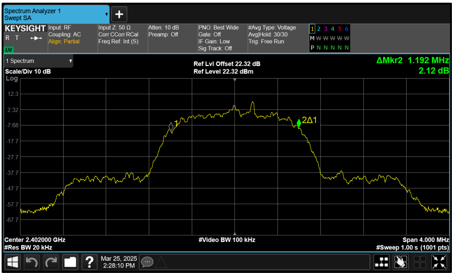
Figure 165 - Core 2 (C) 2402 MHz (CH0) 99% Bandwidth
