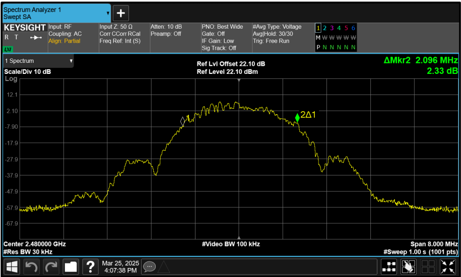
Figure 193 - Core 1 (B) 2480 MHz (CH39) 99% Bandwidth
