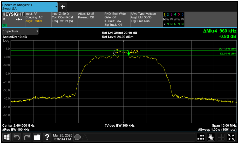
Figure 178 - Core 0 (A) 2404 MHz (CH2) 6 dB Bandwidth
