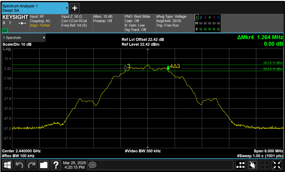
Figure 144 - Core 2 (C) 2440 MHz (CH17) 6 dB Bandwidth
