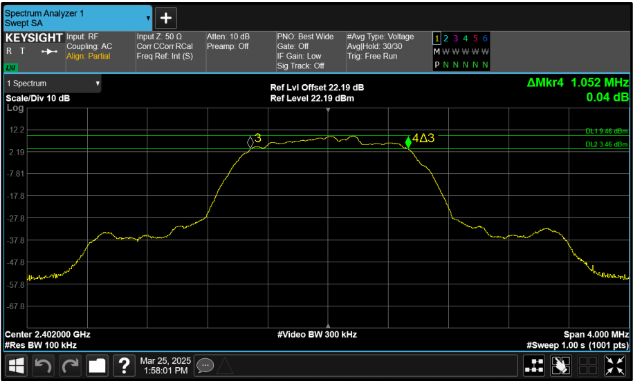
Figure 160 - Core 0 (A) 2402 MHz (CH0) 6 dB Bandwidth
