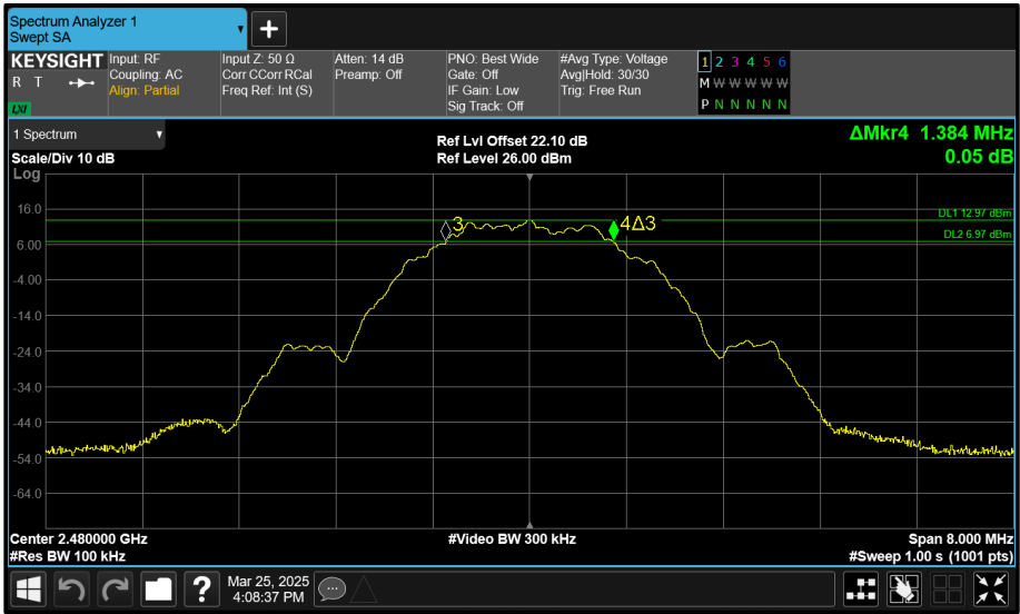
Figure 194 - Core 1 (B) 2480 MHz (CH39) 6 dB Bandwidth
