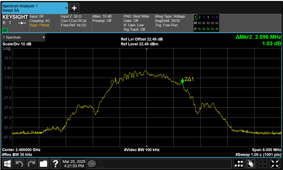
Figure 145 - Core 2 (C) 2480 MHz (CH39) 99% Bandwidth
