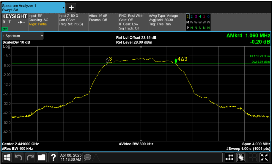
Figure 204 - Core 0 (A) 2441 MHz (CH39) 6 dB Bandwidth
