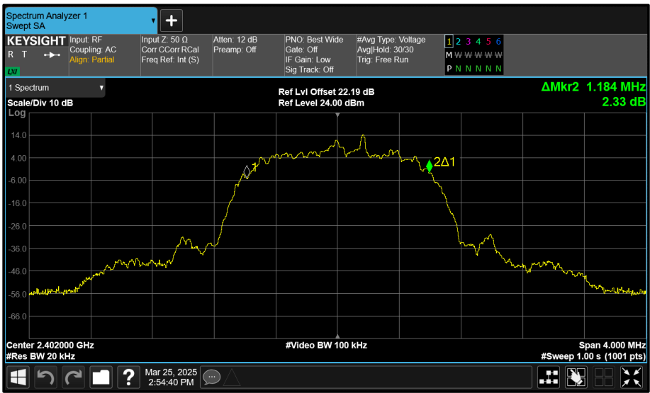
Figure 201 - Core 0 (A) 2402 MHz (CH0) 99% Bandwidth
