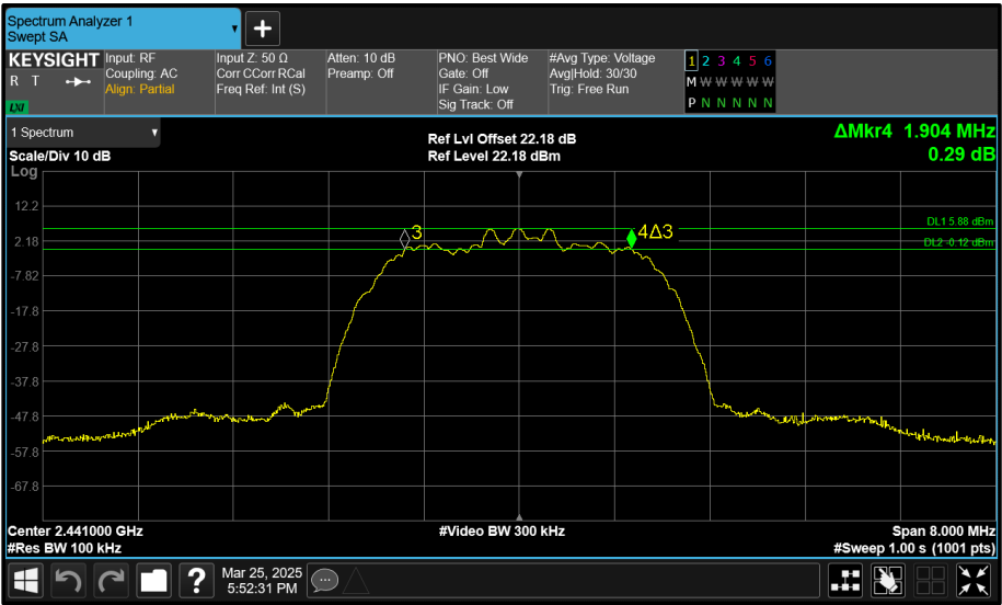
Figure 212 - Core 0 (A) 2441 MHz (CH39) 6 dB Bandwidth
