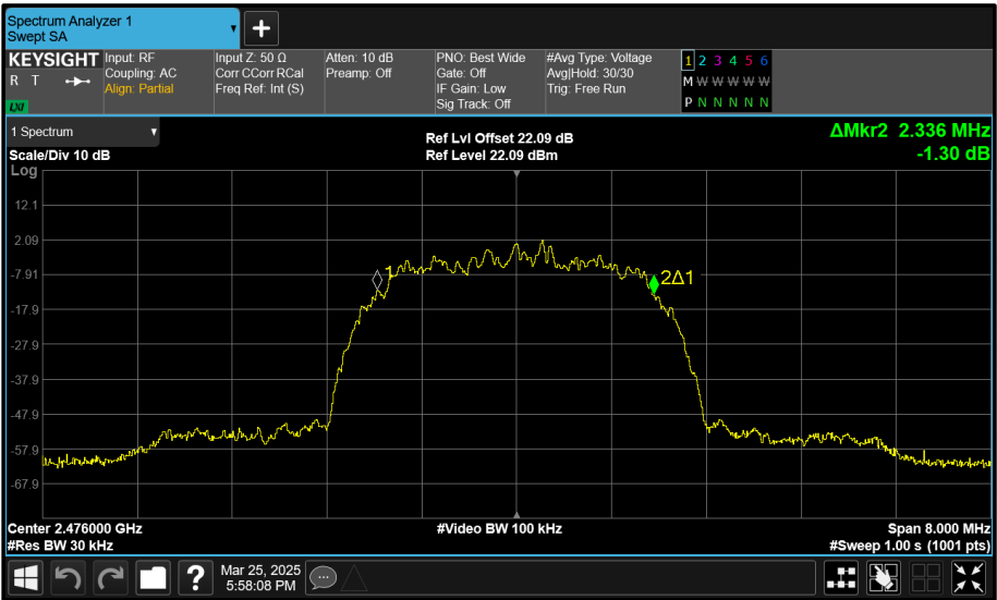
Figure 217 - Core 1 (B) 2476 MHz (CH74) 99% Bandwidth
