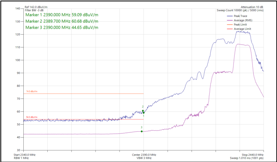
Figure 99 - 802.11be EHT20, RU52+26-72, SISO, Core 1 - 2427 MHz Band Edge Frequency 2390 MHz
