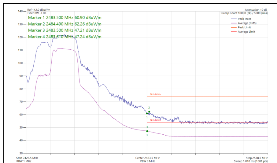
Figure 138 - 802.11be EHT20, RU106+26-83, SISO, Core 1 - 2442 MHz Band Edge Frequency 2483.5 MHz
