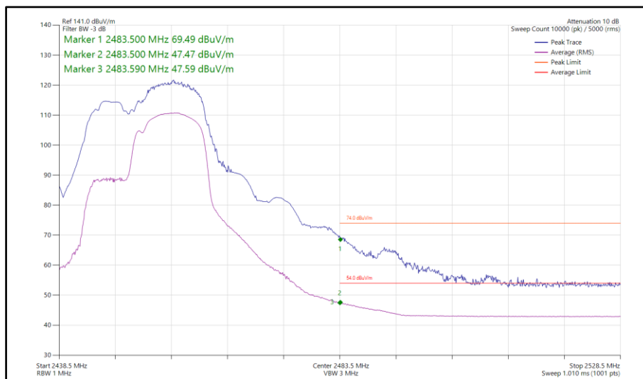
Figure 140 - 802.11be EHT20, RU106+26-83, SISO, Core 1 - 2452 MHz Band Edge Frequency 2483.5 MHz
