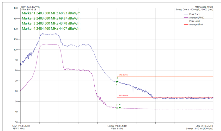
Figure 71 - 802.11be EHT20, RU52+26-70, SISO, Core 0 - 2467 MHz Band Edge Frequency 2483.5 MHz
