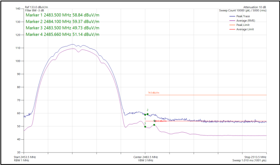
Figure 105 - 802.11b, SISO, Core 1 - 2467 MHz Band Edge Frequency 2483.5 MHz
