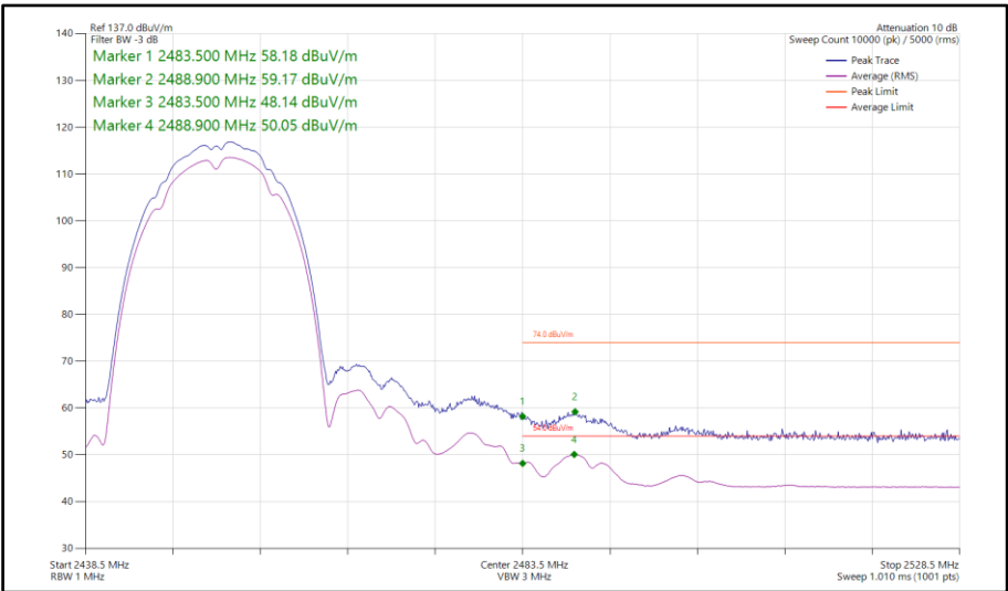
Figure 102 - 802.11b, SISO, Core 1 - 2452 MHz Band Edge Frequency 2483.5 MHz
