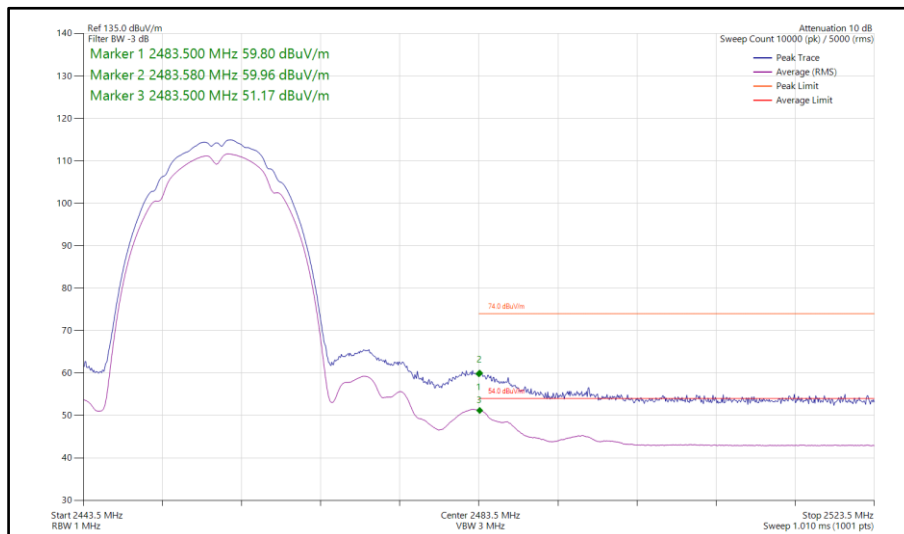
Figure 103 - 802.11b, SISO, Core 1 - 2457 MHz Band Edge Frequency 2483.5 MHz
