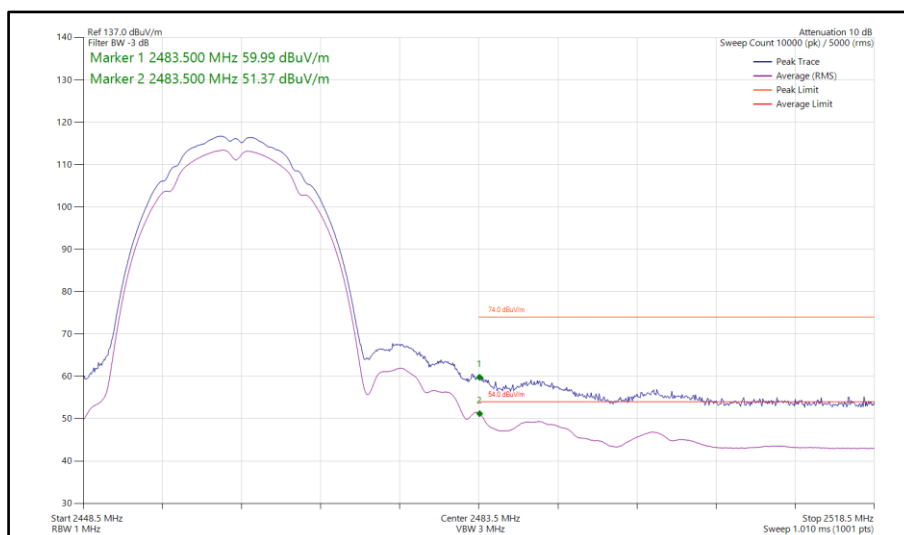
Figure 104 - 802.11b, SISO, Core 1 - 2462 MHz Band Edge Frequency 2483.5 MHz
