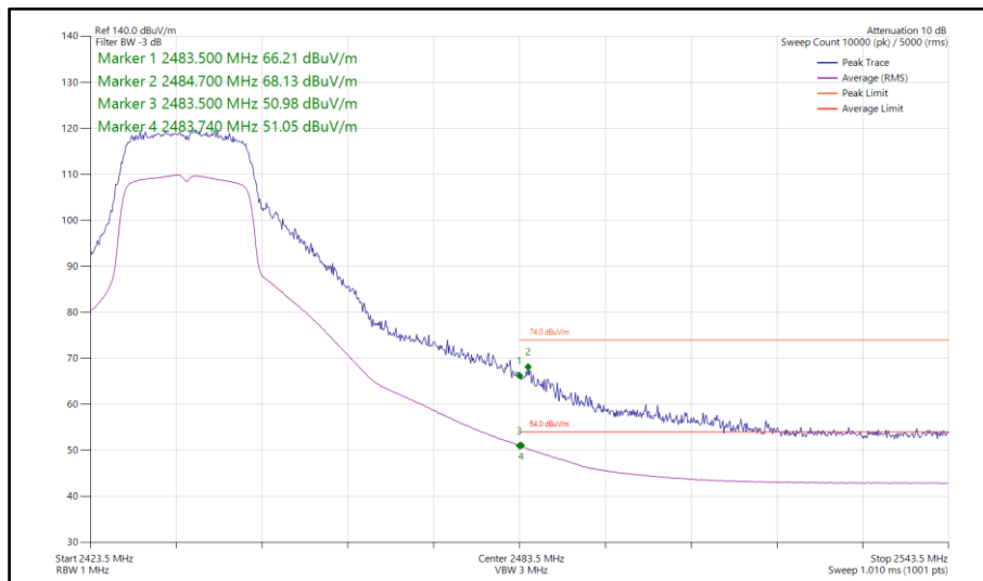
Figure 107 - 802.11g, SISO, Core 1 - 2437 MHz Band Edge Frequency 2483.5 MHz
