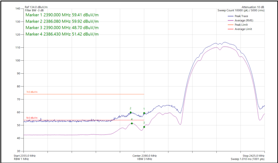
Figure 73 - 802.11b, SISO, Core 1 - 2412 MHz Band Edge Frequency 2390 MHz
