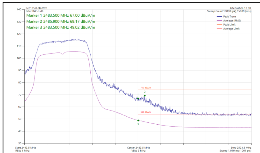
Figure 119 - 802.11n HT20, SISO, Core 1 - 2457 MHz Band Edge Frequency 2483.5 MHz
