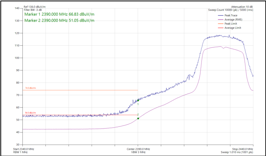
Figure 79 - 802.11g, SISO, Core 1 - 2427 MHz Band Edge Frequency 2390 MHz
