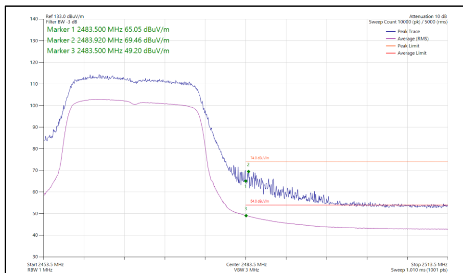
Figure 134 - 802.11ax HE20, SU, SISO, Core 1 - 2467 MHz Band Edge Frequency 2483.5 MHz
