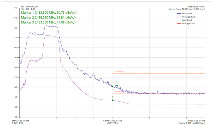
Figure 125 - 802.11ax HE20, RU 106-54, SISO, Core 1 - 2442 MHz Band Edge Frequency 2483.5 MHz
