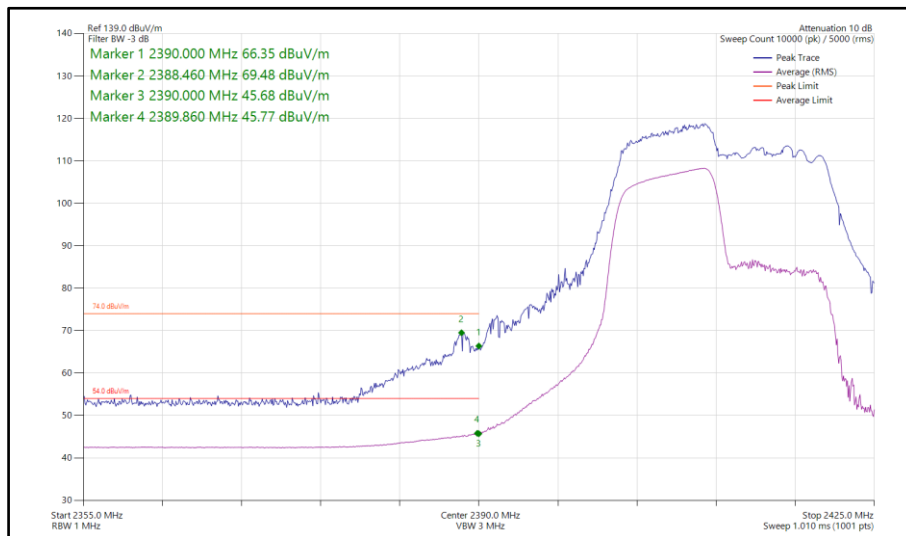
Figure 87 - 802.11ax HE20, RU 106-53, SISO, Core 1 - 2412 MHz Band Edge Frequency 2390 MHz
