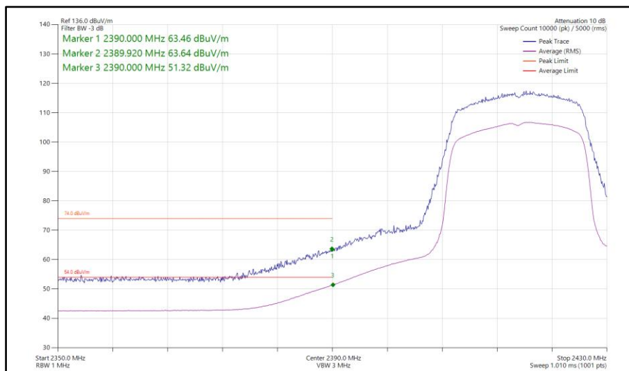
Figure 88 - 802.11ax HE20, SU, SISO, Core 1 - 2417 MHz Band Edge Frequency 2390 MHz
