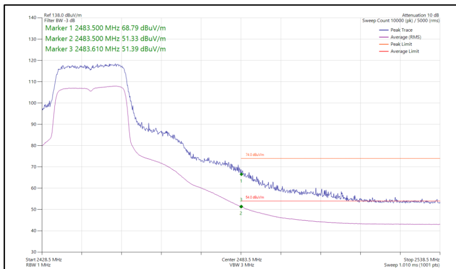
Figure 124 - 802.11ax HE20, SU, SISO, Core 1 - 2442 MHz Band Edge Frequency 2483.5 MHz
