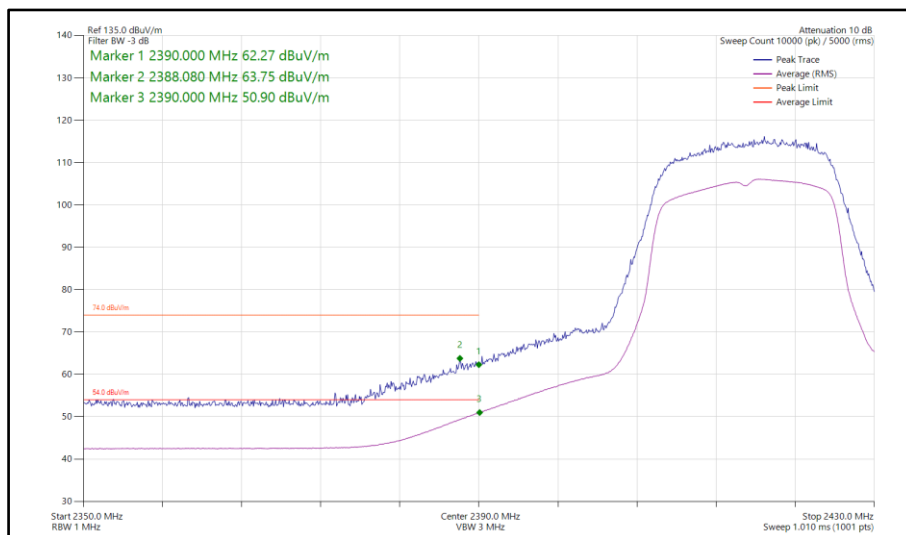
Figure 82 - 802.11n HT20, SISO, Core 1 - 2417 MHz Band Edge Frequency 2390 MHz
