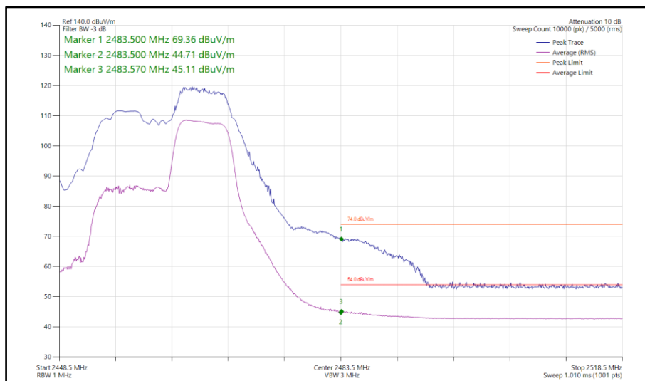
Figure 70 - 802.11be EHT20, RU52+26-72, SISO, Core 0 - 2462 MHz Band Edge Frequency 2483.5 MHz
