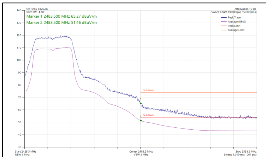
Figure 108 - 802.11g, SISO, Core 1 - 2442 MHz Band Edge Frequency 2483.5 MHz
