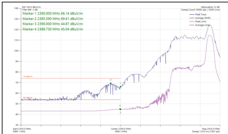
Figure 91 - 802.11ax HE20, RU 26-8, SISO, Core 1 - 2422 MHz Band Edge Frequency 2390 MHz
