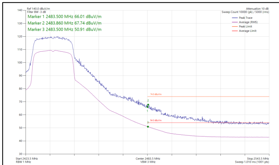
Figure 123 - 802.11ax HE20, SU, SISO, Core 1 - 2437 MHz Band Edge Frequency 2483.5 MHz
