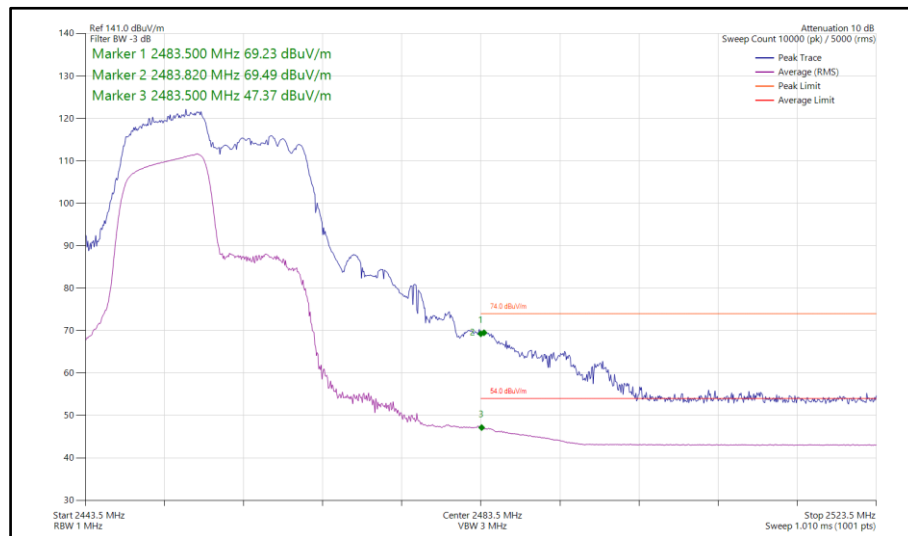
Figure 131 - 802.11ax HE20, RU 106-53, SISO, Core 1 - 2457 MHz Band Edge Frequency 2483.5 MHz
