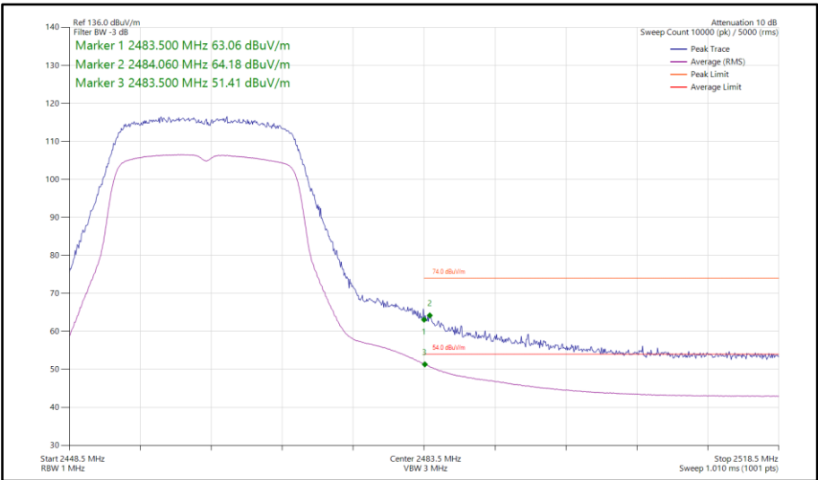
Figure 112 - 802.11g, SISO, Core 1 - 2462 MHz Band Edge Frequency 2483.5 MHz
