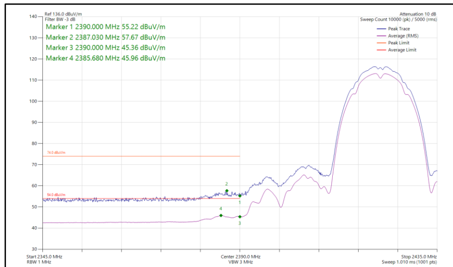
Figure 75 - 802.11b, SISO, Core 1 - 2422 MHz Band Edge Frequency 2390 MHz
