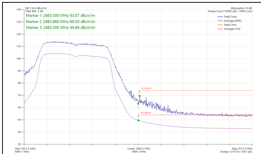
Figure 121 - 802.11n HT20, SISO, Core 1 - 2467 MHz Band Edge Frequency 2483.5 MHz
