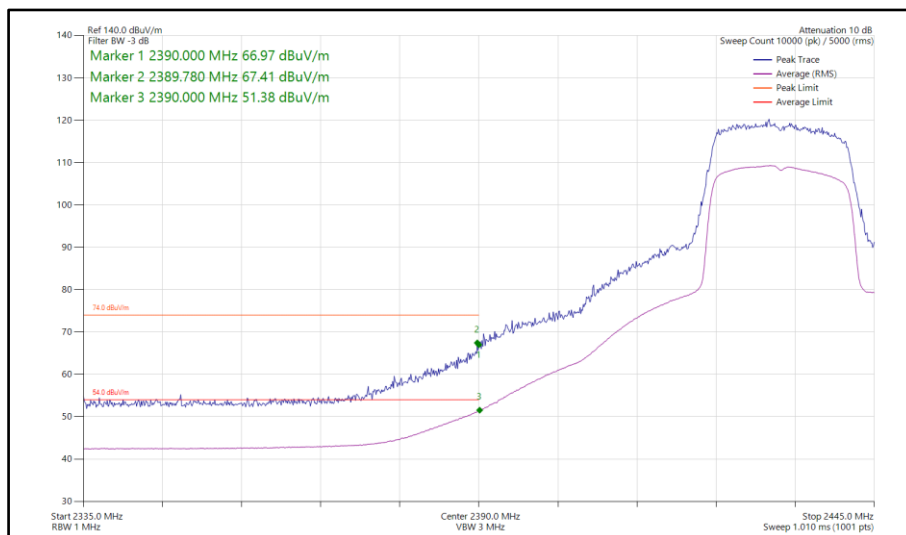
Figure 94 - 802.11ax HE20, SU, SISO, Core 1 - 2432 MHz Band Edge Frequency 2390 MHz
