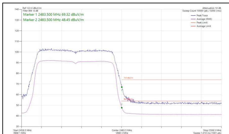
Figure 136 - 802.11ax HE20, SU, SISO, Core 1 - 2472 MHz Band Edge Frequency 2483.5 MHz
