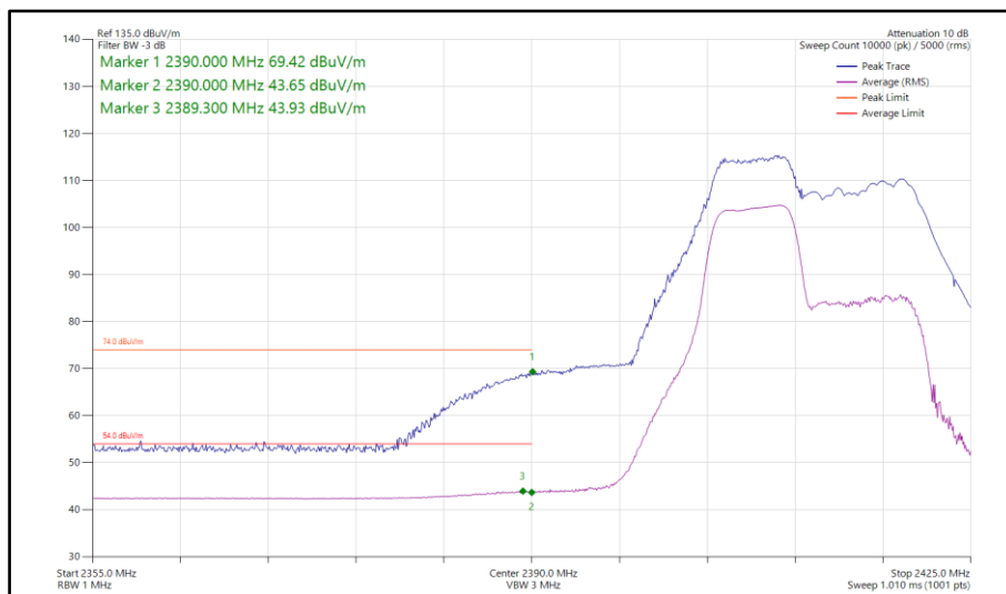
Figure 96 - 802.11be EHT20, RU52+26-70, SISO, Core 1 - 2412 MHz Band Edge Frequency 2390 MHz
