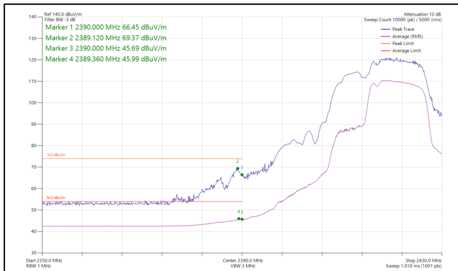
Figure 97 - 802.11be EHT20, RU106+26-83 SISO, Core 1 - 2417 MHz Band Edge Frequency 2390 MHz
