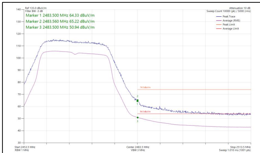
Figure 113 - 802.11g, SISO, Core 1 - 2467 MHz Band Edge Frequency 2483.5 MHz
