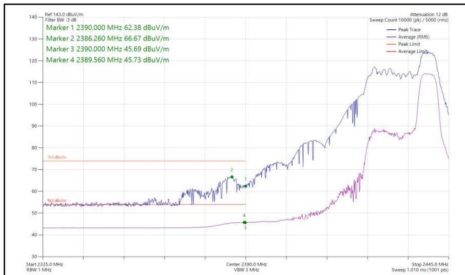
Figure 95 - 802.11ax HE20, RU 52-40, SISO, Core 1 - 2432 MHz Band Edge Frequency 2390 MHz
