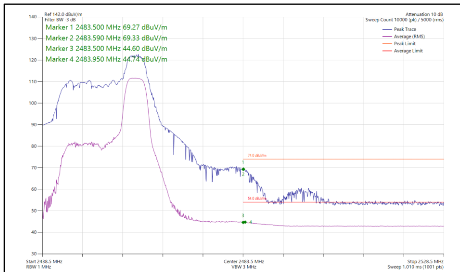
Figure 129 - 802.11ax HE20, RU 52-40, SISO, Core 1 - 2452 MHz Band Edge Frequency 2483.5 MHz
