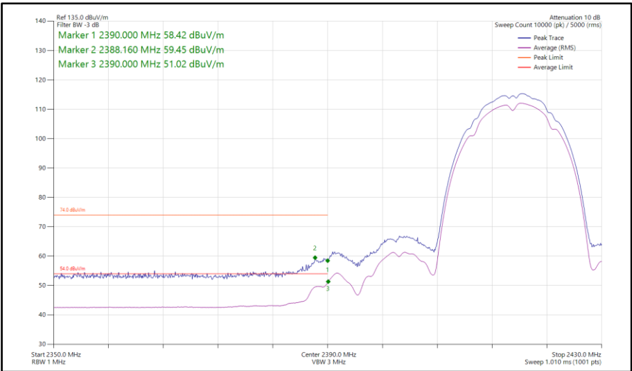
Figure 74 - 802.11b, SISO, Core 1 - 2417 MHz Band Edge Frequency 2390 MHz
