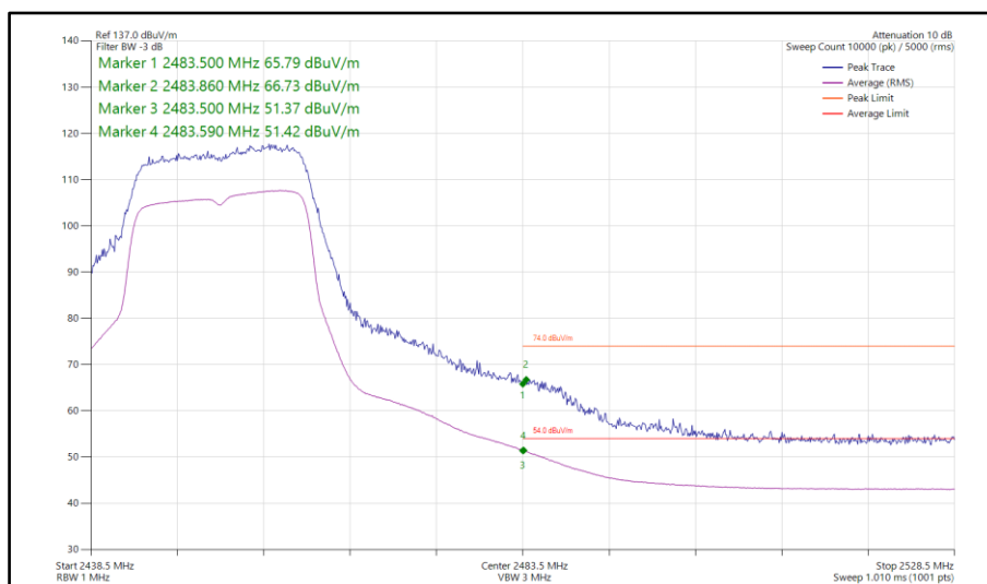
Figure 118 - 802.11n HT20, SISO, Core 1 - 2452 MHz Band Edge Frequency 2483.5 MHz
