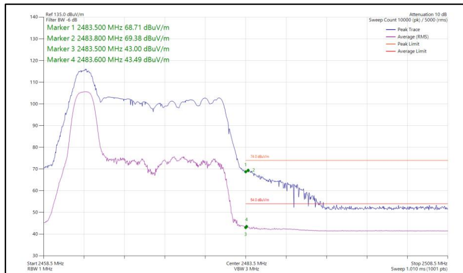
Figure 137 - 802.11ax HE20, RU 26-0, SISO, Core 1 - 2472 MHz Band Edge Frequency 2483.5 MHz
