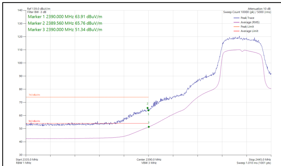
Figure 85 - 802.11n HT20, SISO, Core 1 - 2432 MHz Band Edge Frequency 2390 MHz
