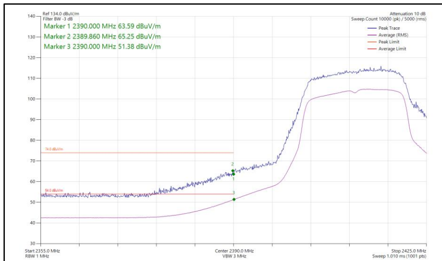
Figure 81 - 802.11n HT20, SISO, Core 1 - 2412 MHz Band Edge Frequency 2390 MHz
