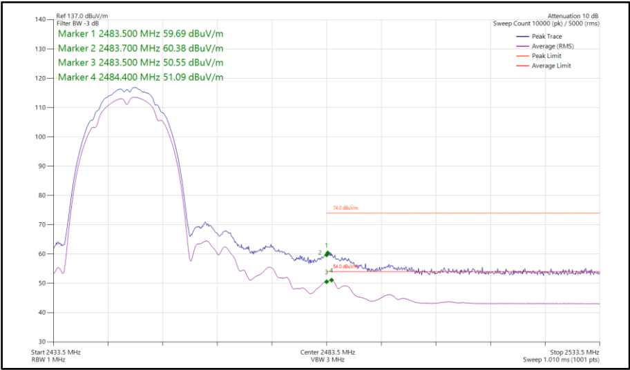
Figure 101 - 802.11b, SISO, Core 1 - 2447 MHz Band Edge Frequency 2483.5 MHz
