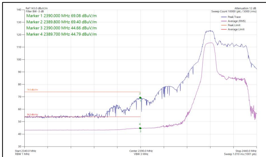
Figure 93 - 802.11ax HE20, RU 52-37, SISO, Core 1 - 2427 MHz Band Edge Frequency 2390 MHz
