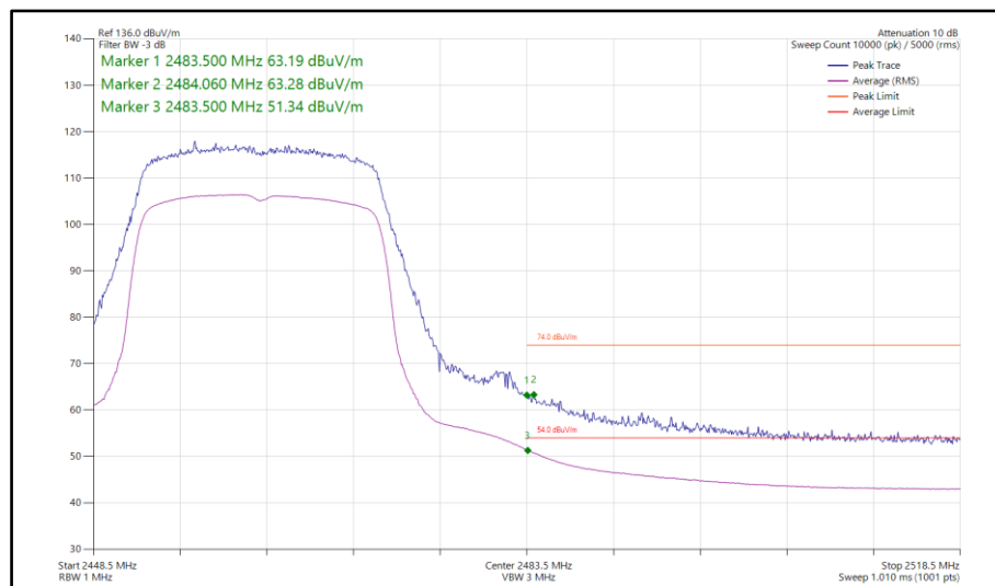
Figure 132 - 802.11ax HE20, SU, SISO, Core 1 - 2462 MHz Band Edge Frequency 2483.5 MHz
