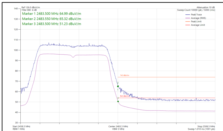
Figure 114 - 802.11g, SISO, Core 1 - 2472 MHz Band Edge Frequency 2483.5 MHz
