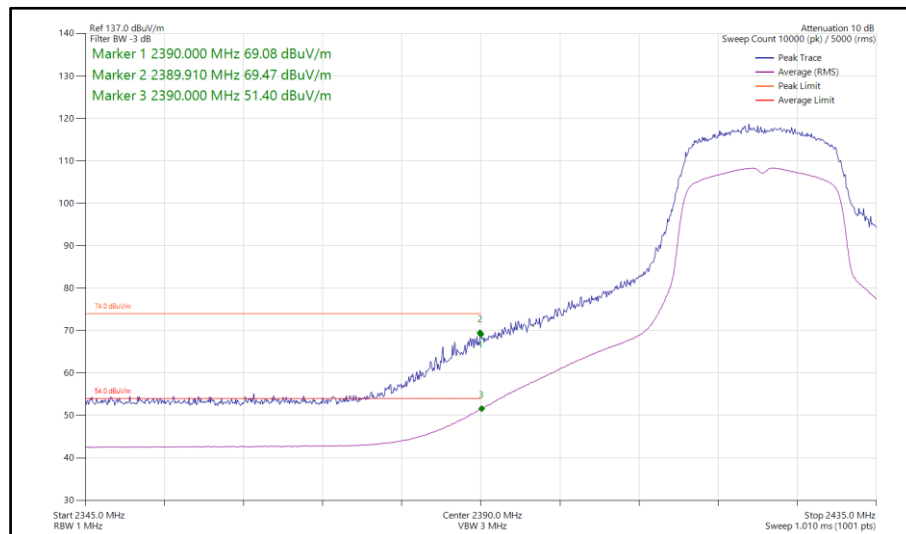
Figure 83 - 802.11n HT20, SISO, Core 1 - 2422 MHz Band Edge Frequency 2390 MHz
