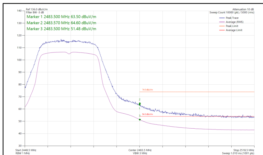
Figure 120 - 802.11n HT20, SISO, Core 1 - 2462 MHz Band Edge Frequency 2483.5 MHz
