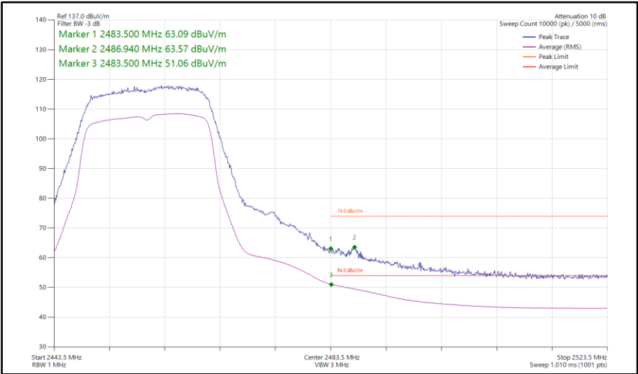
Figure 111 - 802.11g, SISO, Core 1 - 2457 MHz Band Edge Frequency 2483.5 MHz
