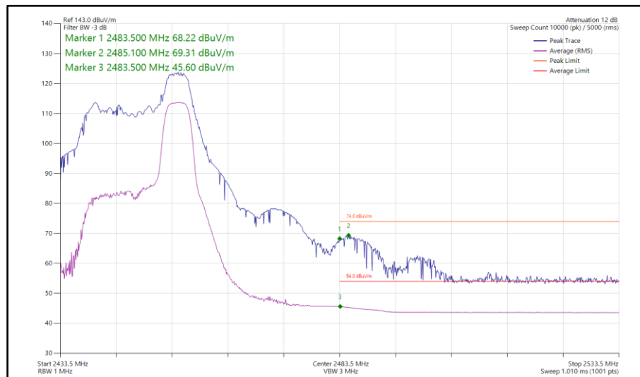
Figure 127 - 802.11ax HE20, RU 52-40, SISO, Core 1 - 2447 MHz Band Edge Frequency 2483.5 MHz
