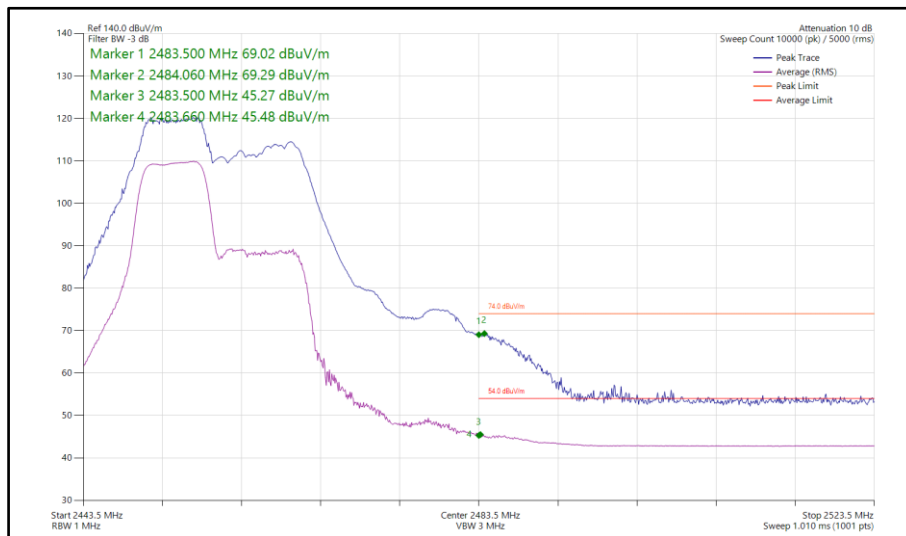
Figure 69 - 802.11be EHT20, RU52+26-70, SISO, Core 0 - 2457 MHz Band Edge Frequency 2483.5 MHz
