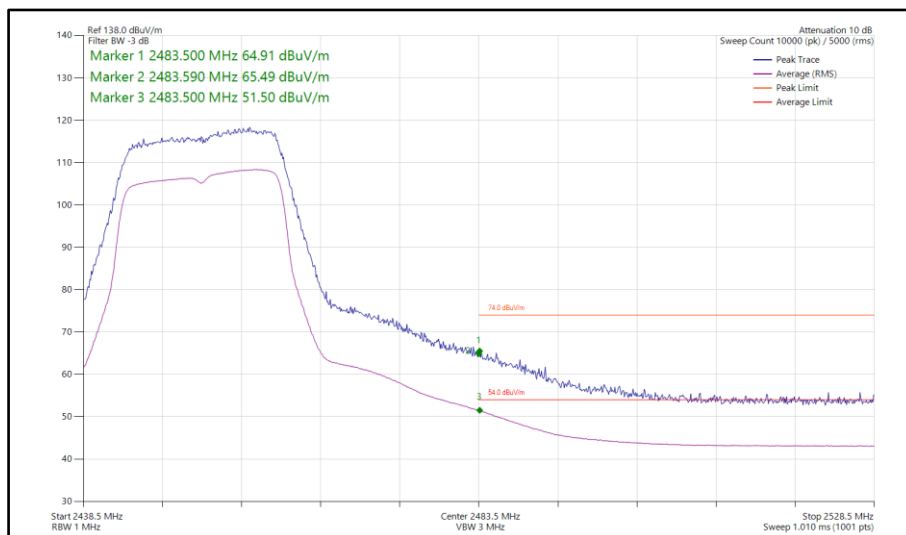
Figure 110 - 802.11g, SISO, Core 1 - 2452 MHz Band Edge Frequency 2483.5 MHz
