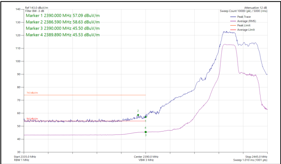
Figure 100 - 802.11be EHT20, RU52+26-70, SISO, Core 1 - 2432 MHz Band Edge Frequency 2390 MHz
