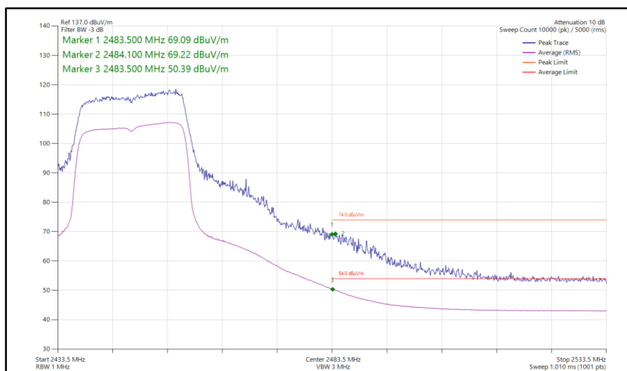
Figure 126 - 802.11ax HE20, SU, SISO, Core 1 - 2447 MHz Band Edge Frequency 2483.5 MHz
