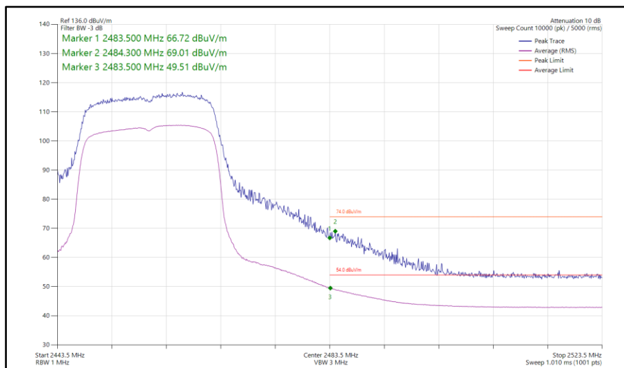
Figure 130 - 802.11ax HE20, SU, SISO, Core 1 - 2457 MHz Band Edge Frequency 2483.5 MHz
