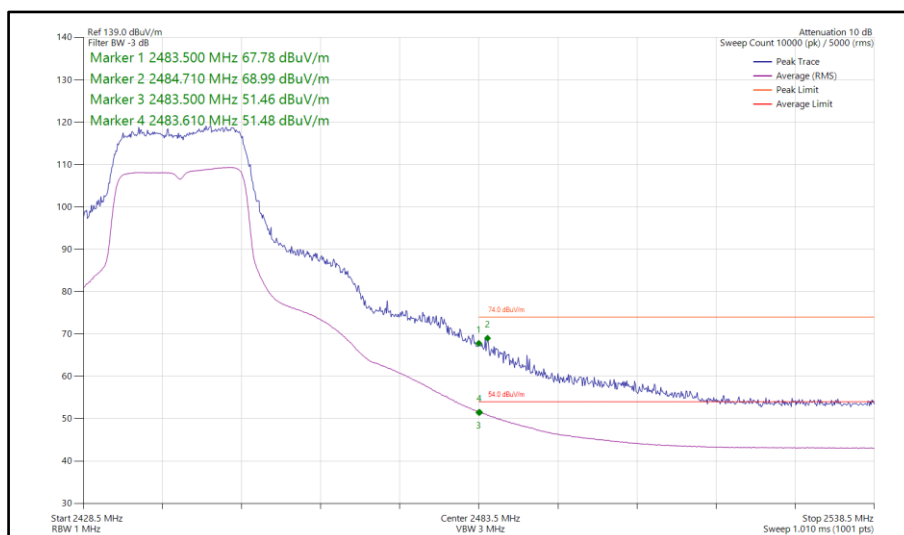
Figure 116 - 802.11n HT20, SISO, Core 1 - 2442 MHz Band Edge Frequency 2483.5 MHz
