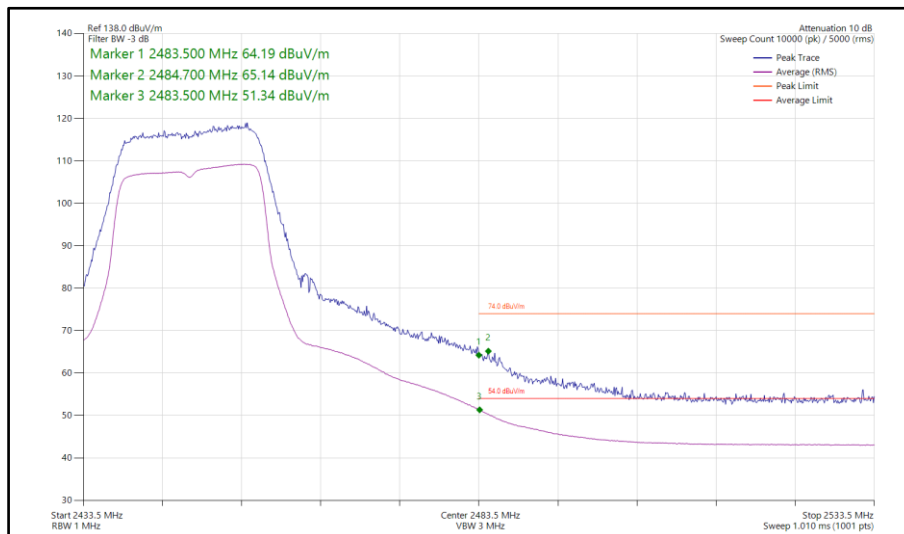
Figure 117 - 802.11n HT20, SISO, Core 1 - 2447 MHz Band Edge Frequency 2483.5 MHz
