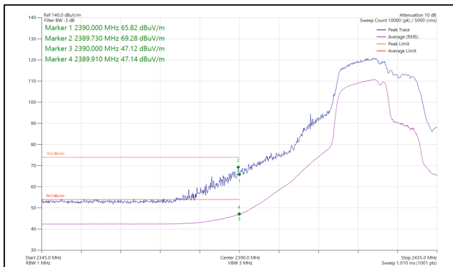
Figure 98 - 802.11be EHT20, RU106+26-82, SISO, Core 1 - 2422 MHz Band Edge Frequency 2390 MHz
