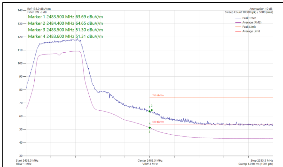
Figure 109 - 802.11g, SISO, Core 1 - 2447 MHz Band Edge Frequency 2483.5 MHz
