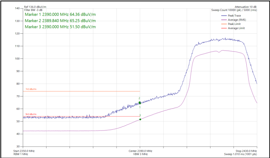
Figure 77 - 802.11g, SISO, Core 1 - 2417 MHz Band Edge Frequency 2390 MHz
