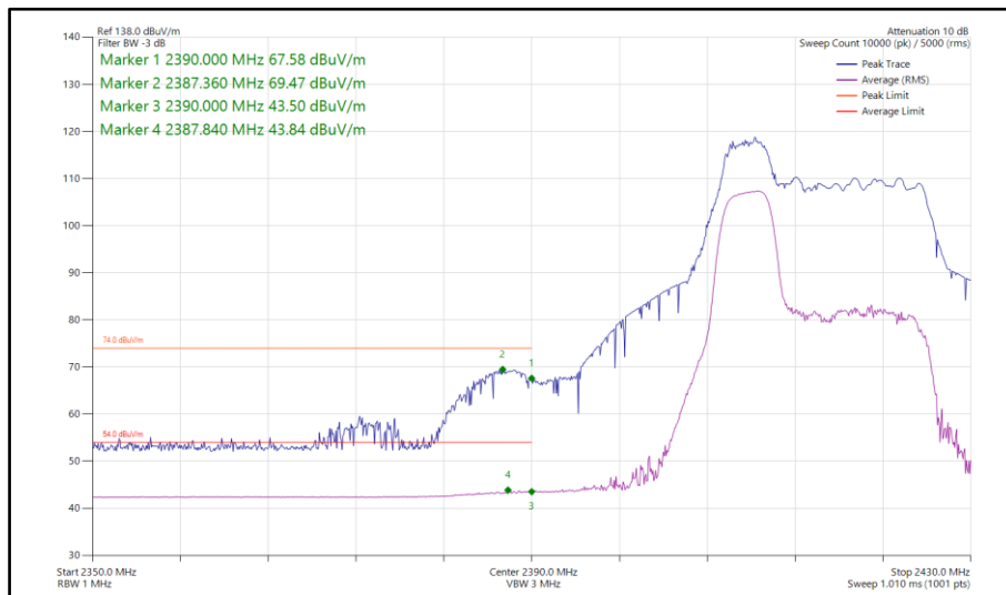
Figure 89 - 802.11ax HE20, RU 52-37, SISO, Core 1 - 2417 MHz Band Edge Frequency 2390 MHz
