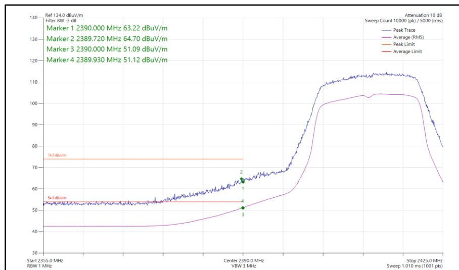
Figure 76 - 802.11g, SISO, Core 1 - 2412 MHz Band Edge Frequency 2390 MHz
