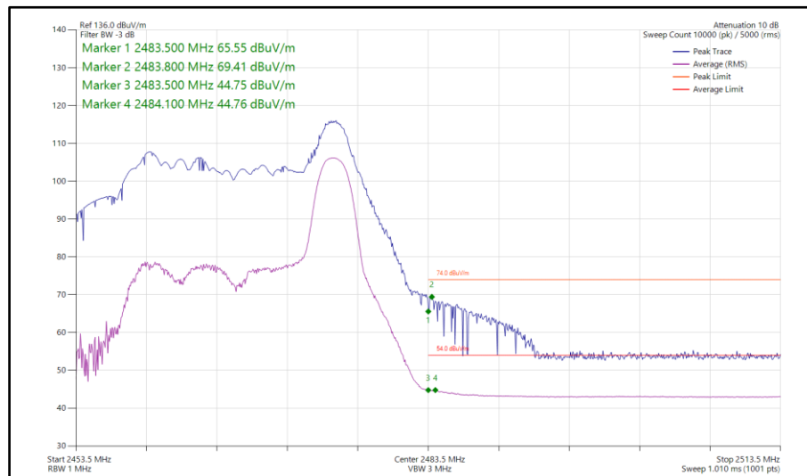
Figure 135 - 802.11ax HE20, RU 26-8, SISO, Core 1 - 2467 MHz Band Edge Frequency 2483.5 MHz
