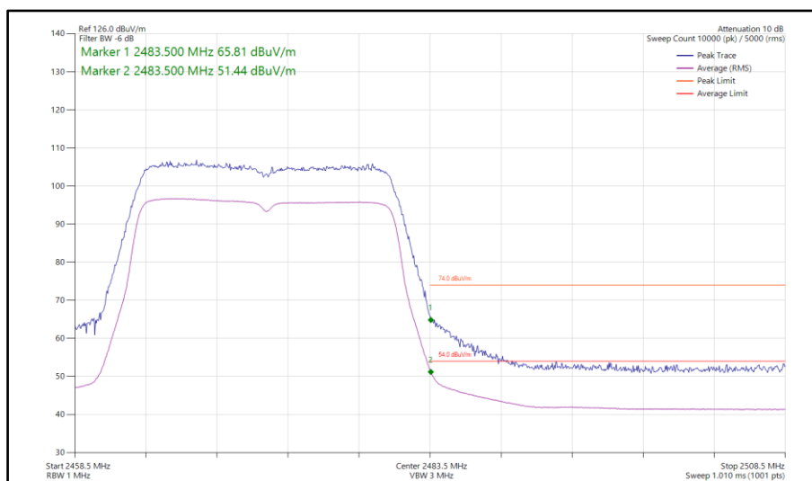
Figure 122 - 802.11n HT20, SISO, Core 1 - 2472 MHz Band Edge Frequency 2483.5 MHz
