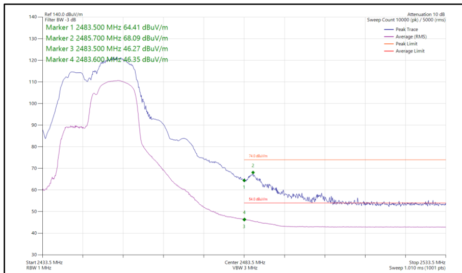
Figure 139 - 802.11be EHT20, RU106+26-83, SISO, Core 1 - 2447 MHz Band Edge Frequency 2483.5 MHz
