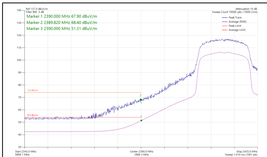
Figure 90 - 802.11ax HE20, SU, SISO, Core 1 - 2422 MHz Band Edge Frequency 2390 MHz
