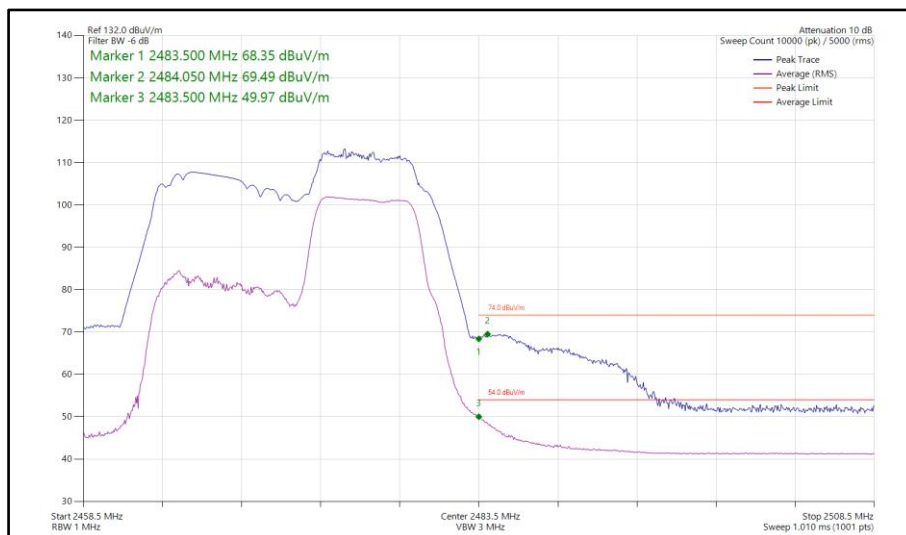
Figure 72 - 802.11be EHT20, RU52+26-72, SISO, Core 0 - 2472 MHz Band Edge Frequency 2483.5 MHz
