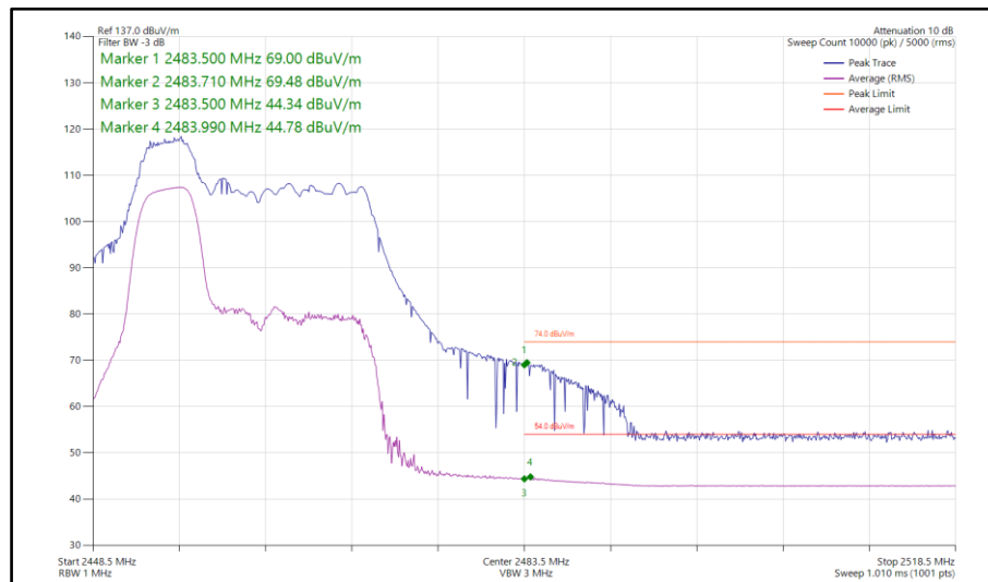
Figure 133 - 802.11ax HE20, RU 52-37, SISO, Core 1 - 2462 MHz Band Edge Frequency 2483.5 MHz
