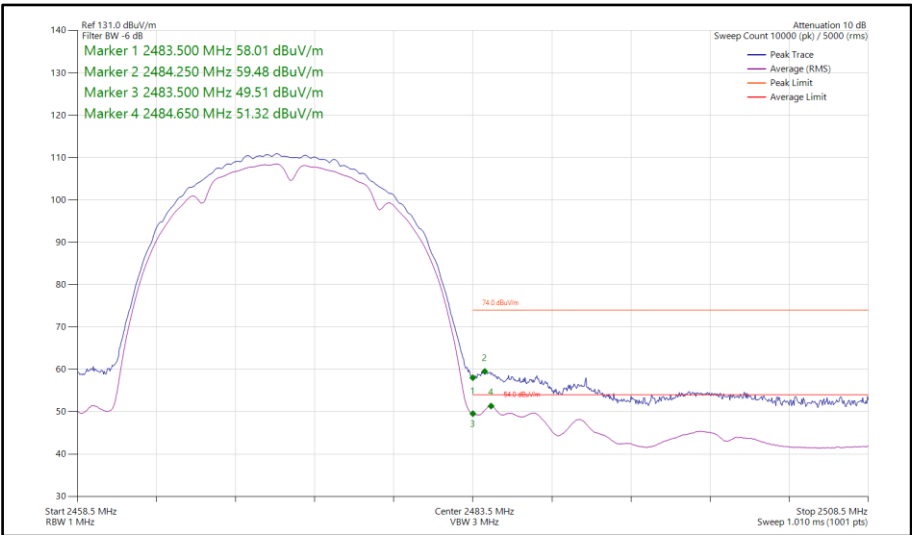
Figure 106 - 802.11b, SISO, Core 1 - 2472 MHz Band Edge Frequency 2483.5 MHz
