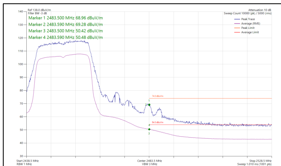
Figure 128 - 802.11ax HE20, SU, SISO, Core 1 - 2452 MHz Band Edge Frequency 2483.5 MHz
