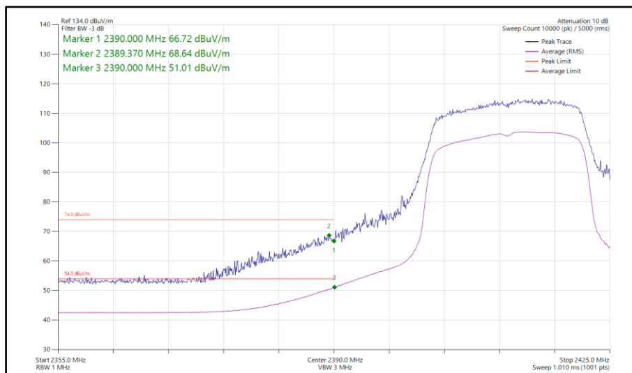
Figure 86 - 802.11ax HE20, SU, SISO, Core 1 - 2412 MHz Band Edge Frequency 2390 MHz
