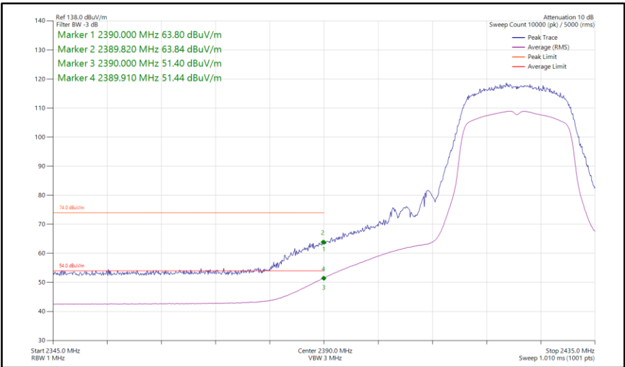
Figure 78 - 802.11g, SISO, Core 1 - 2422 MHz Band Edge Frequency 2390 MHz
