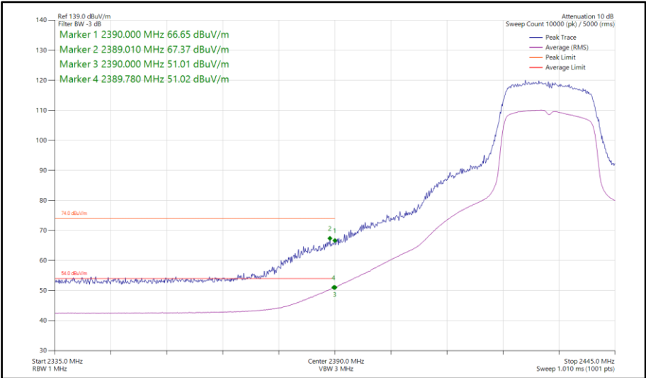
Figure 80 - 802.11g, SISO, Core 1 - 2432 MHz Band Edge Frequency 2390 MHz
