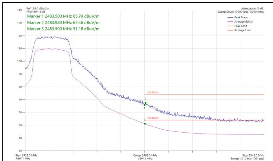
Figure 115 - 802.11n HT20, SISO, Core 1 - 2437 MHz Band Edge Frequency 2483.5 MHz
