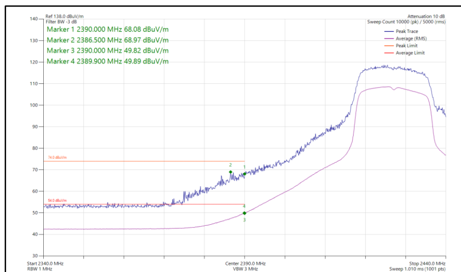
Figure 84 - 802.11n HT20, SISO, Core 1 - 2427 MHz Band Edge Frequency 2390 MHz
