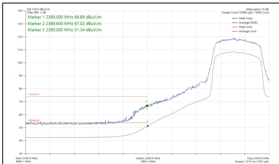
Figure 92 - 802.11ax HE20, SU, SISO, Core 1 - 2427 MHz Band Edge Frequency 2390 MHz
