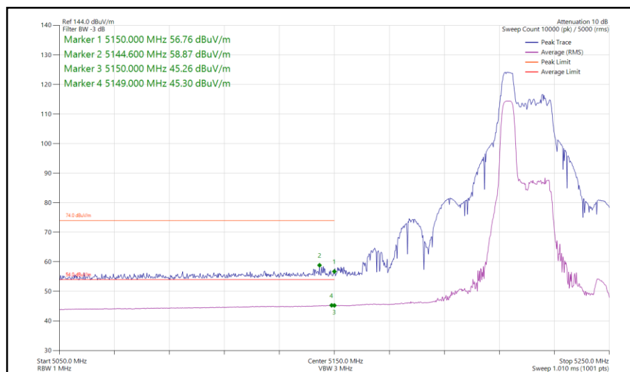
Figure 133 - 802.11ax HE40, RU 52-37, SISO, Core 0 - 5230 MHz Band Edge Frequency 5150 MHz
