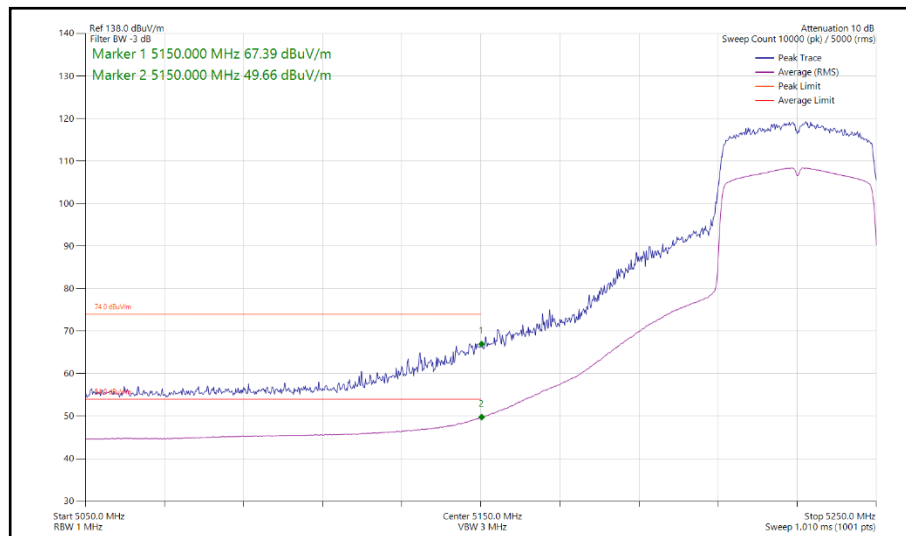
Figure 132 - 802.11ax HE40, SU, SISO, Core 0 - 5230 MHz Band Edge Frequency 5150 MHz
