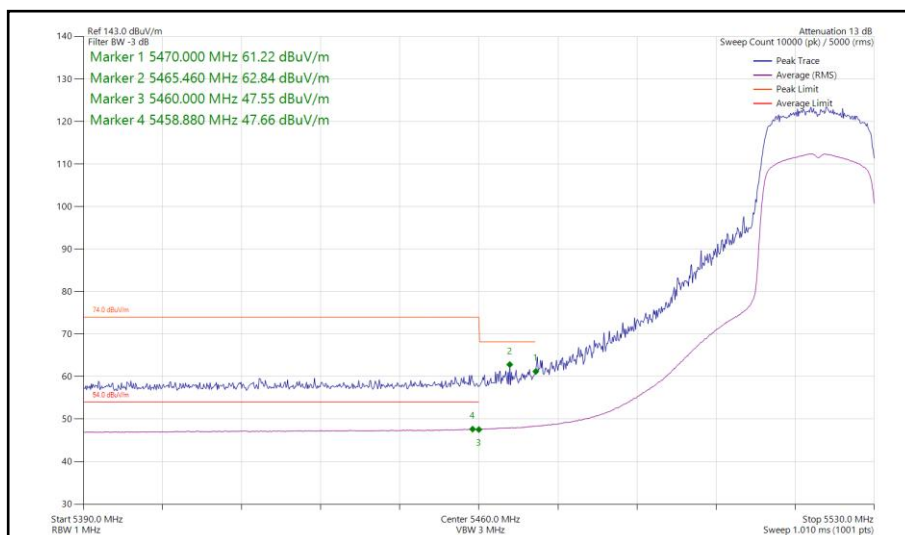
Figure 124 - 802.11ax HE20, SU, TxBF, Core 0-1 - 5520 MHz Band Edge Frequency 5460 MHz
