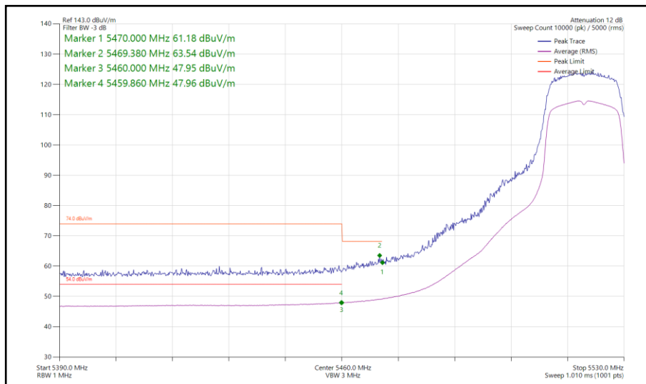
Figure 121 - 802.11ac VHT20, TxBF, Core 0-1 - 5520 MHz Band Edge Frequency 5460 MHz
