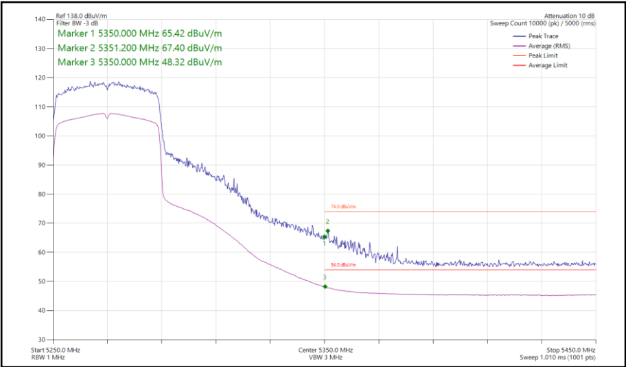
Figure 171 - 802.11ax HE40, SU, SISO, Core 1 - 5270 MHz Band Edge Frequency 5350 MHz
