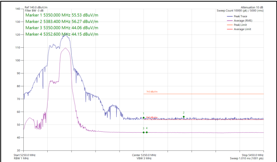
Figure 172 - 802.11ax HE40, RU 106-56, SISO, Core 1 - 5270 MHz Band Edge Frequency 5350 MHz
