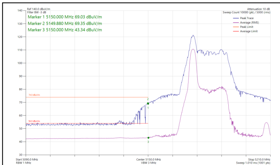
Figure 162 - 802.11ax HE40, RU 26-0, SISO, Core 1 - 5190 MHz Band Edge Frequency 5150 MHz
