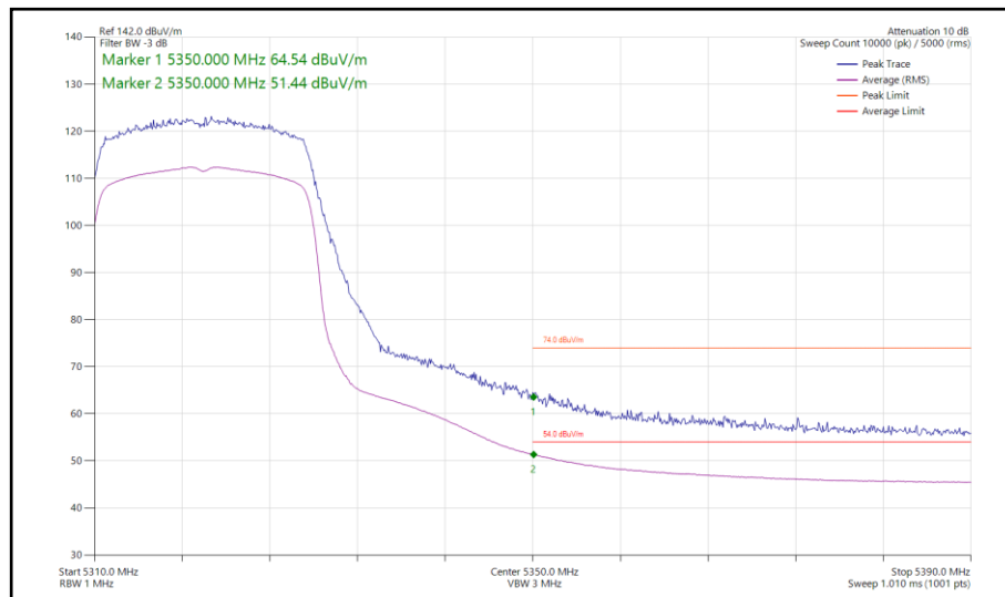
Figure 119 - 802.11ax HE20, SU, TxBF, Core 0-1 - 5320 MHz Band Edge Frequency 5350 MHz
