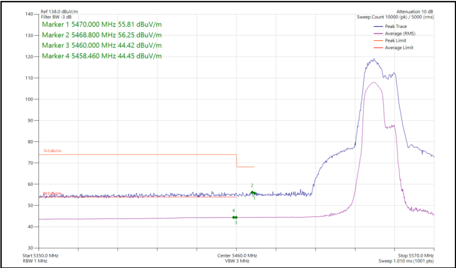
Figure 156 - 802.11be EHT40, RU 106+26-82, SISO, Core 0 - 5550 MHz Band Edge Frequency 5460 MHz
