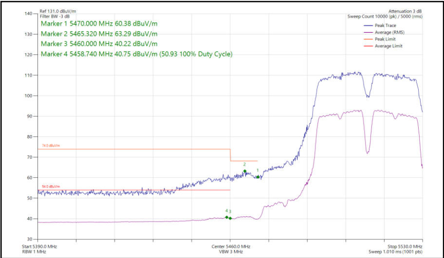
Figure 146 - 802.11a, SISO, Core 0 - 5510 MHz Band Edge Frequency 5460 MHz
