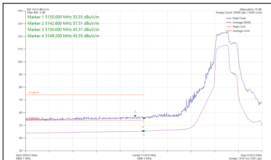
Figure 135 - 802.11be EHT40, RU 52+26-82, SISO, Core 0 - 5230 MHz Band Edge Frequency 5150 MHz
