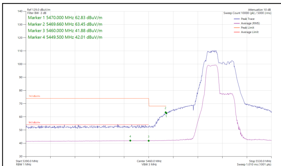
Figure 155 - 802.11be EHT40, RU 52+26-70, SISO, Core 0 - 5510 MHz Band Edge Frequency 5460 MHz
