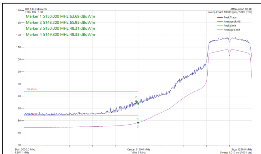
Figure 129 - 802.11n HT40, SISO, Core 0 - 5230 MHz Band Edge Frequency 5150 MHz
