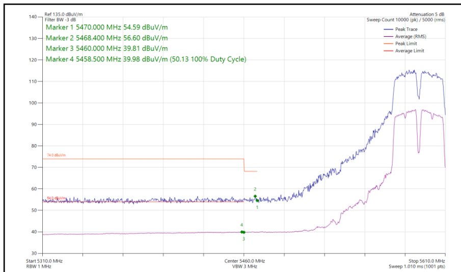
Figure 148 - 802.11a, SISO, Core 0 - 5590 MHz Band Edge Frequency 5460 MHz
