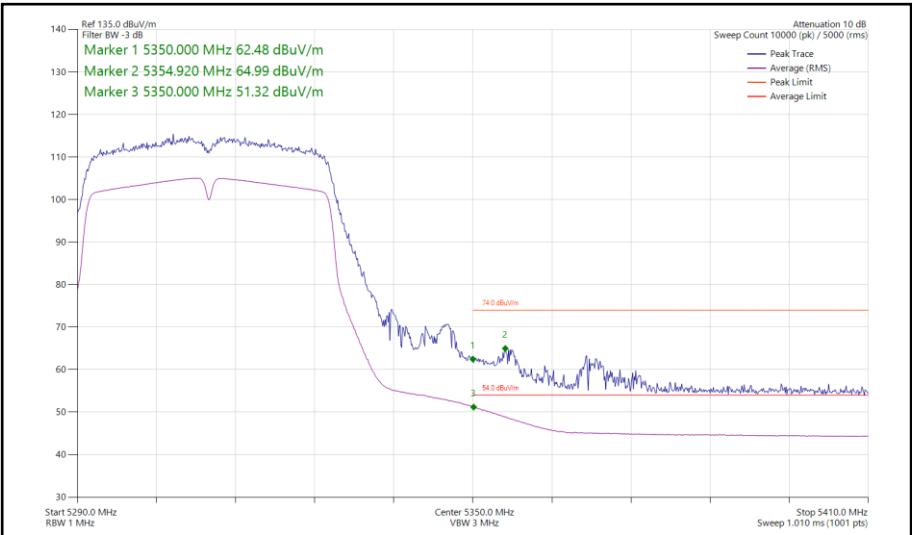
Figure 170 - 802.11n HT40, SISO, Core 1 - 5310 MHz Band Edge Frequency 5350 MHz
