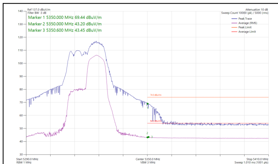
Figure 143 - 802.11ax HE40, RU 106-56, SISO, Core 0 - 5310 MHz Band Edge Frequency 5350 MHz
