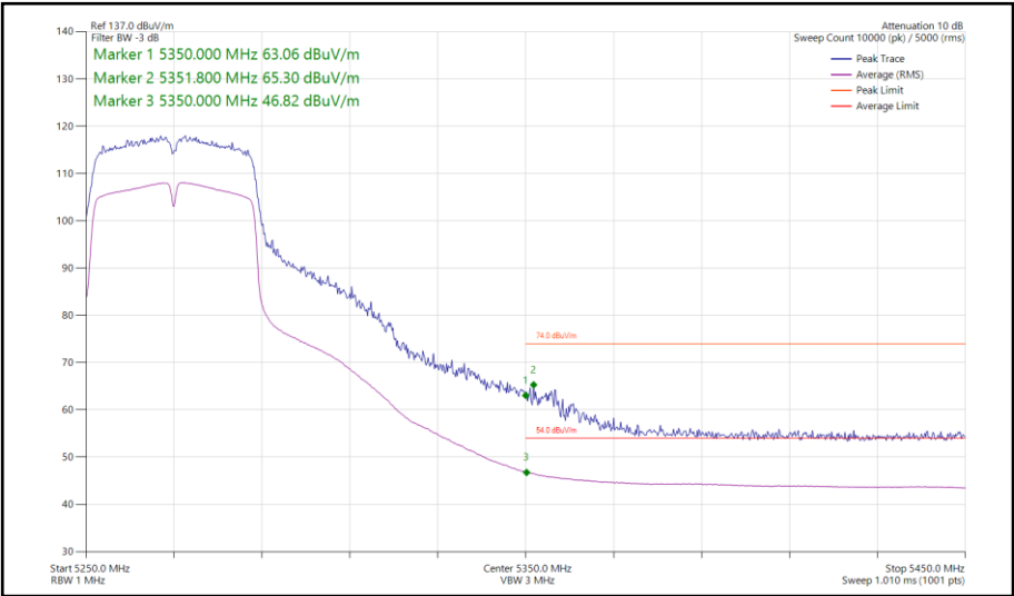
Figure 138 - 802.11n HT40, SISO, Core 0 - 5270 MHz Band Edge Frequency 5350 MHz
