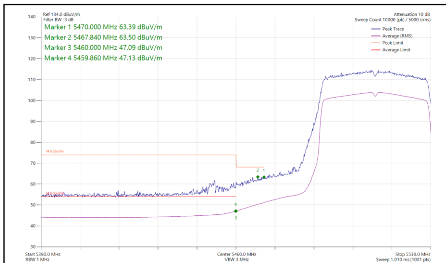
Figure 151 - 802.11ax HE40, SU, SISO, Core 0 - 5510 MHz Band Edge Frequency 5460 MHz
