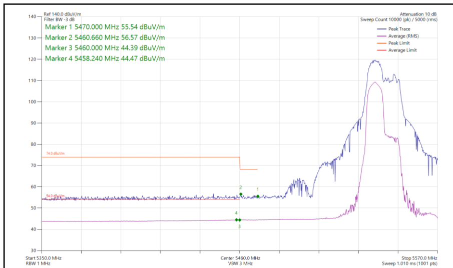
Figure 154 - 802.11ax HE40, RU 106-53, SISO, Core 0 - 5550 MHz Band Edge Frequency 5460 MHz
