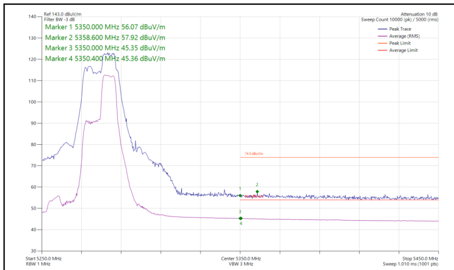
Figure 144 - 802.11be EHT40, RU 52+26-75, SISO, Core 0 - 5270 MHz Band Edge Frequency 5350 MHz
