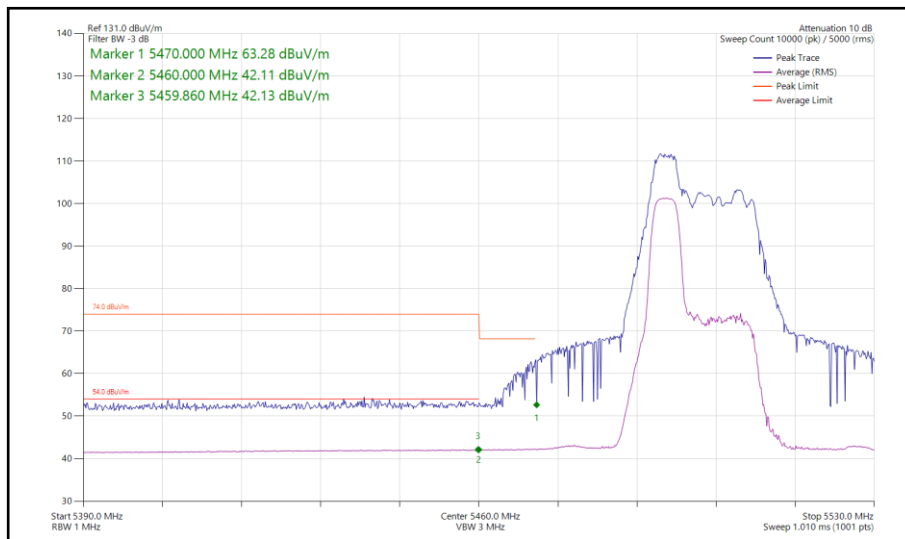
Figure 152 - 802.11ax HE40, RU 52-37, SISO, Core 0 - 5510 MHz Band Edge Frequency 5460 MHz
