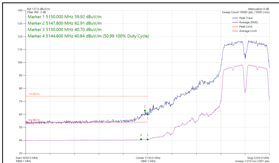
Figure 158 - 802.11a, SISO, Core 1 - 5230 MHz Band Edge Frequency 5150 MHz
