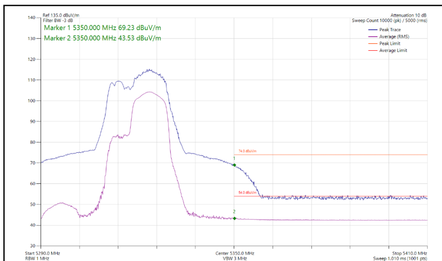
Figure 176 - 802.11be EHT40, RU 106+26-85, SISO, Core 1 - 5310 MHz Band Edge Frequency 5350 MHz
