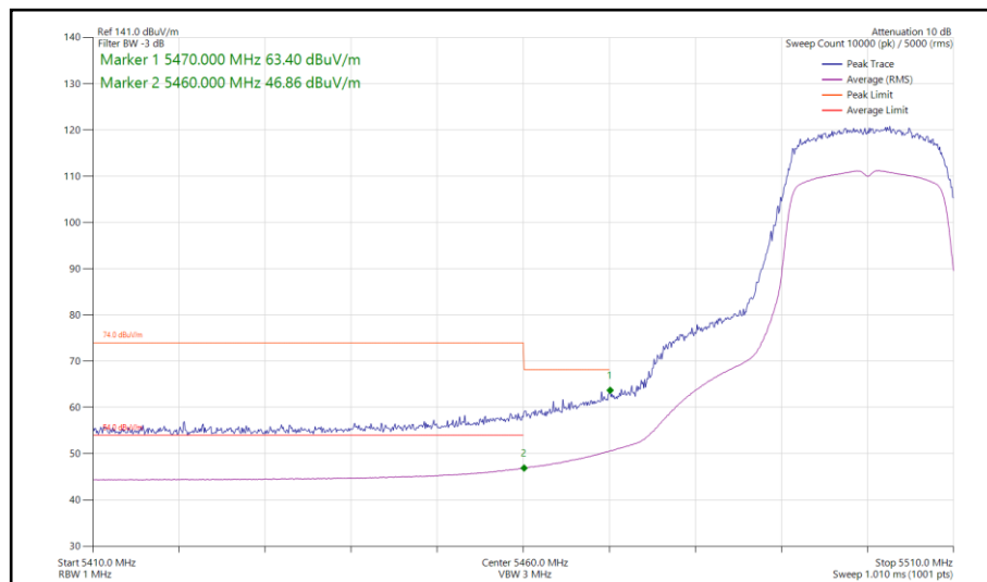
Figure 120 - 802.11ac VHT20, TxBF, Core 0-1 - 5500 MHz Band Edge Frequency 5460 MHz
