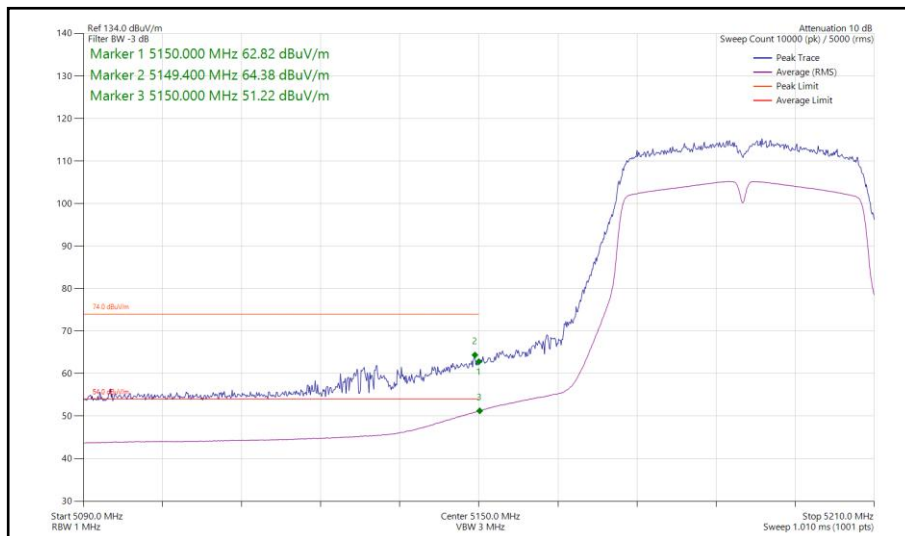
Figure 128 - 802.11n HT40, SISO, Core 0 - 5190 MHz Band Edge Frequency 5150 MHz
