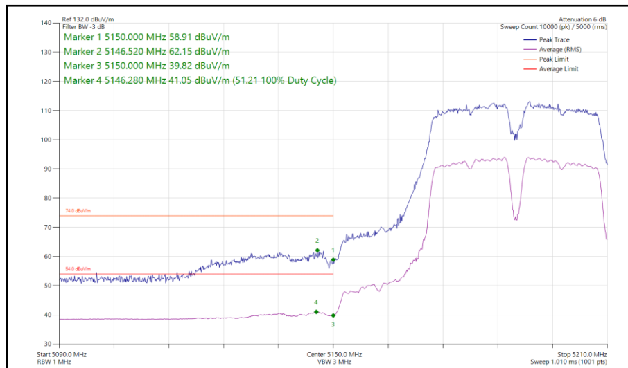
Figure 126 - 802.11a, SISO, Core 0 - 5190 MHz Band Edge Frequency 5150 MHz
