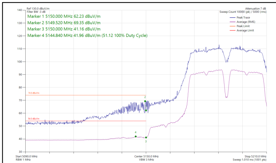
Figure 157 - 802.11a, SISO, Core 1 - 5190 MHz Band Edge Frequency 5150 MHz
