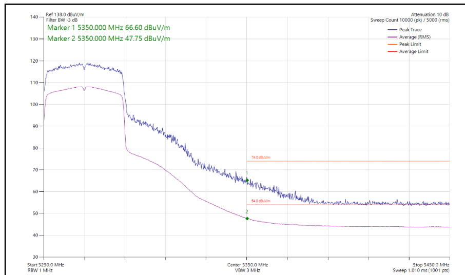
Figure 140 - 802.11ax HE40, SU, SISO, Core 0 - 5270 MHz Band Edge Frequency 5350 MHz
