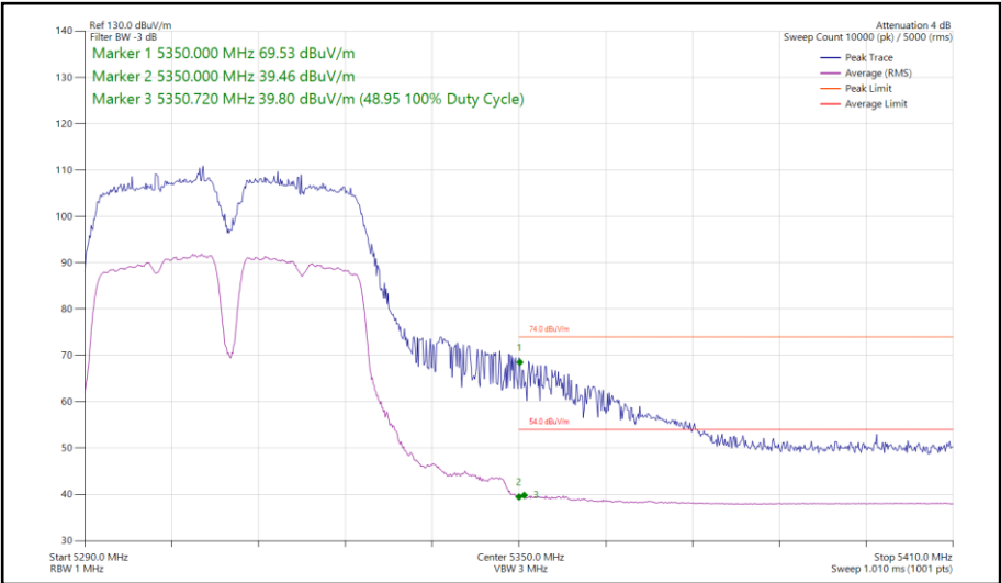
Figure 137 - 802.11a, SISO, Core 0 - 5310 MHz Band Edge Frequency 5350 MHz
