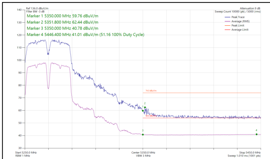
Figure 167 - 802.11a, SISO, Core 1 - 5270 MHz Band Edge Frequency 5350 MHz
