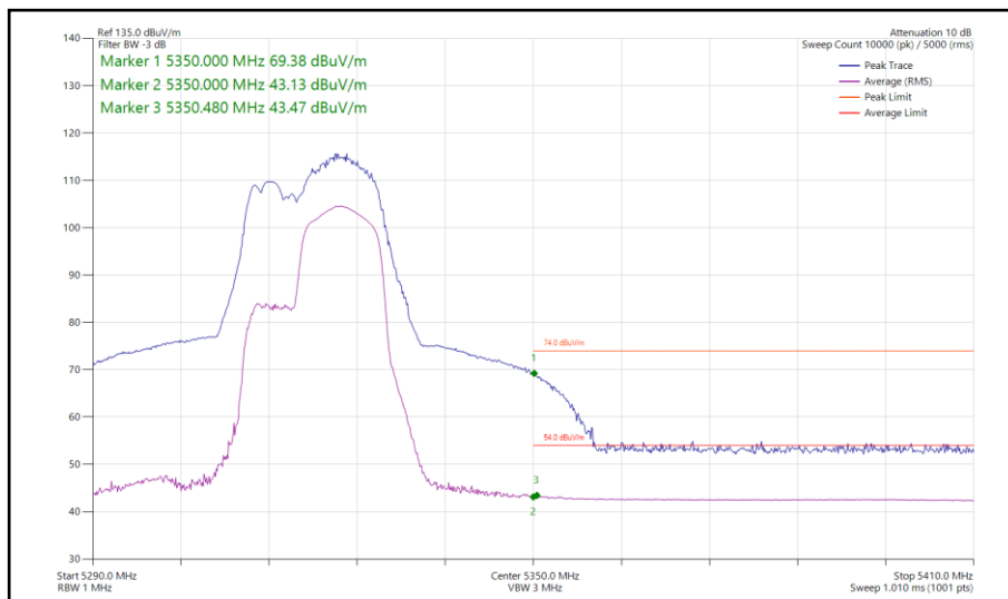
Figure 145 - 802.11be EHT40, RU 106+26-85, SISO, Core 0 - 5310 MHz Band Edge Frequency 5350 MHz
