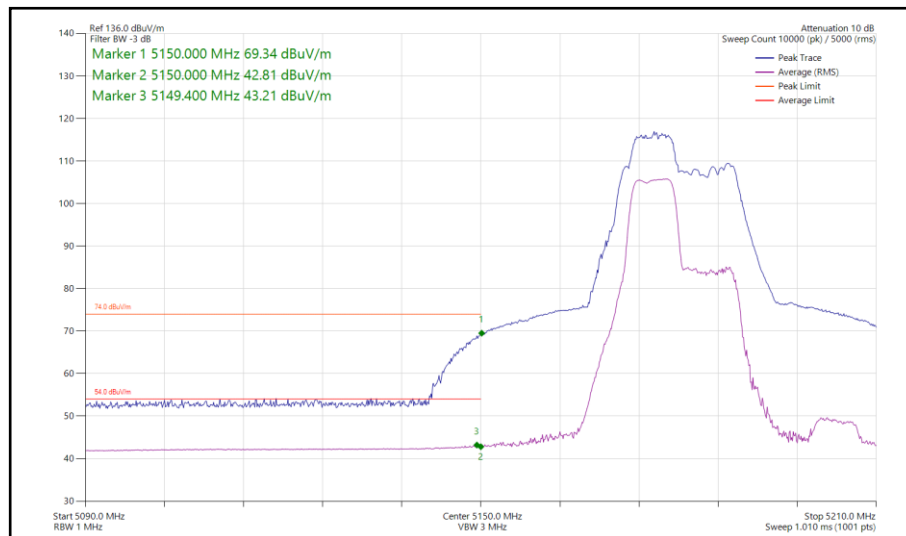
Figure 134 - 802.11be EHT40, RU 52+26-70, SISO, Core 0 - 5190 MHz Band Edge Frequency 5150 MHz
