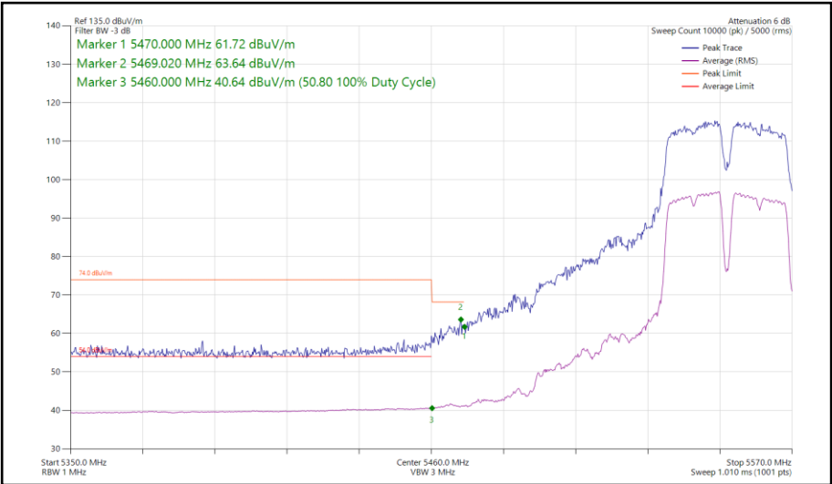
Figure 147 - 802.11a, SISO, Core 0 - 5550 MHz Band Edge Frequency 5460 MHz
