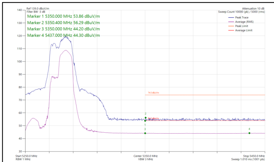
Figure 175 - 802.11be EHT40, RU 106+26-85, SISO, Core 1 - 5270 MHz Band Edge Frequency 5350 MHz
