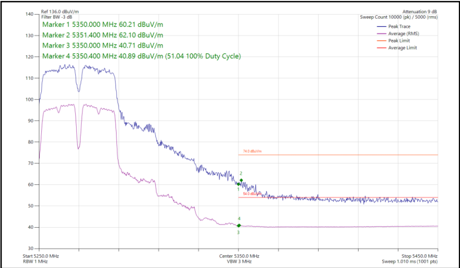
Figure 136 - 802.11a, SISO, Core 0 - 5270 MHz Band Edge Frequency 5350 MHz
