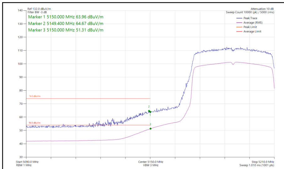
Figure 161 - 802.11ax HE40, SU, SISO, Core 1 - 5190 MHz Band Edge Frequency 5150 MHz
