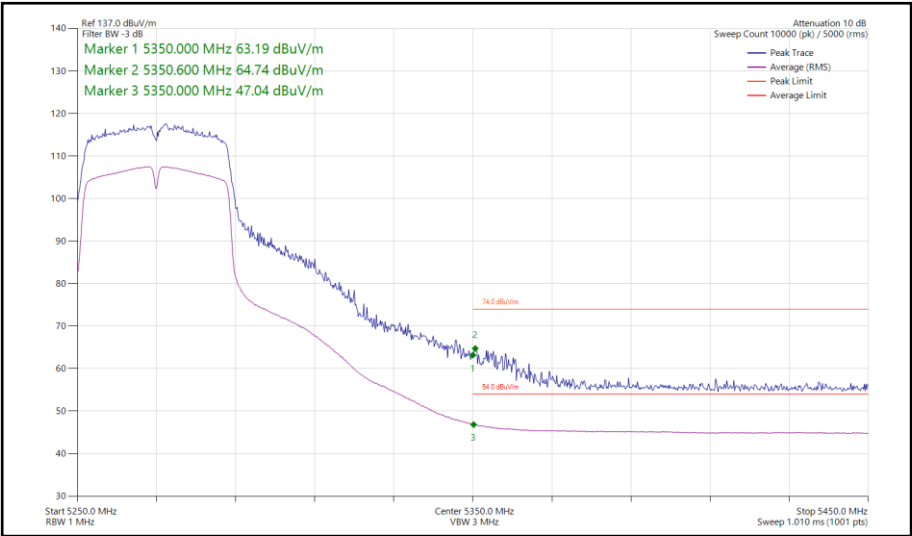
Figure 169 - 802.11n HT40, SISO, Core 1 - 5270 MHz Band Edge Frequency 5350 MHz
