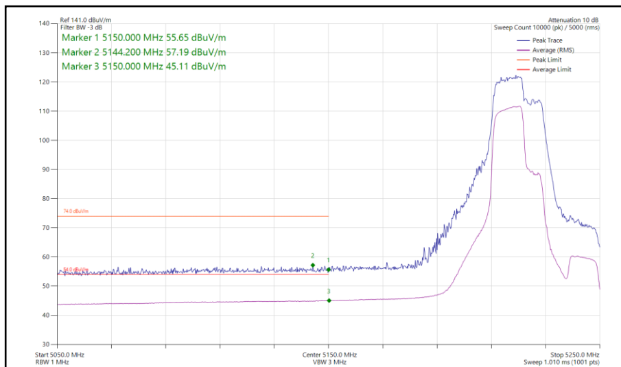
Figure 166 - 802.11be EHT40, RU 106+26-82, SISO, Core 1 - 5230 MHz Band Edge Frequency 5150 MHz
