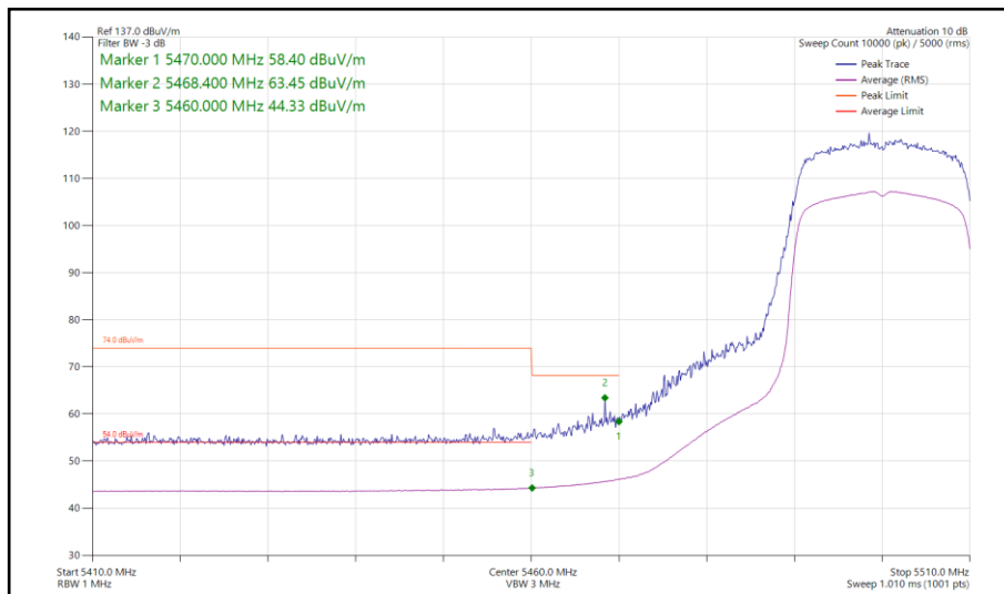
Figure 123 - 802.11ax HE20, SU, TxBF, Core 0-1 - 5500 MHz Band Edge Frequency 5460 MHz
