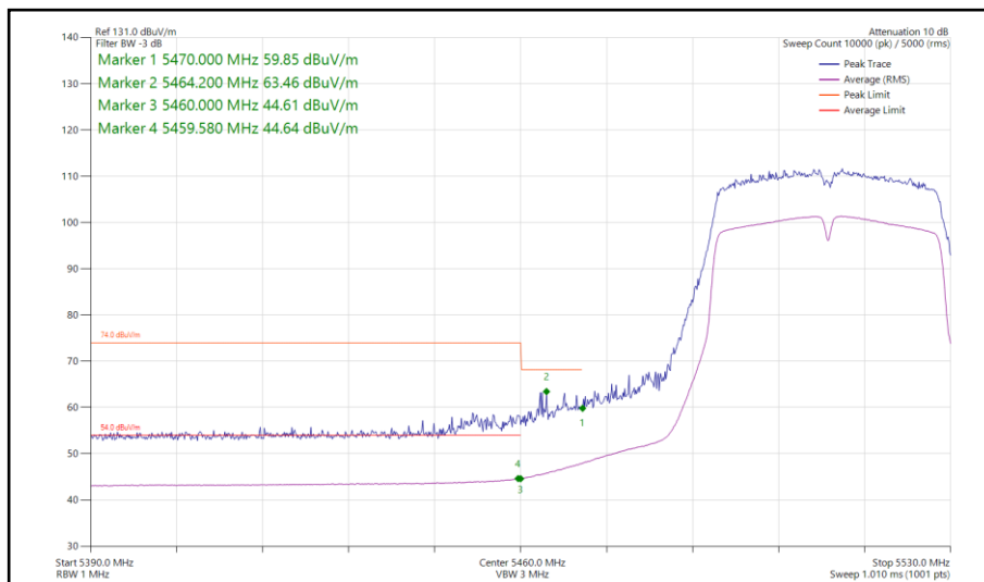
Figure 149 - 802.11n HT40, SISO, Core 0 - 5510 MHz Band Edge Frequency 5460 MHz
