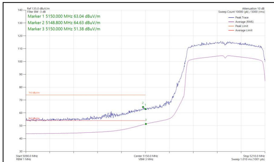
Figure 130 - 802.11ax HE40, SU, SISO, Core 0 - 5190 MHz Band Edge Frequency 5150 MHz
