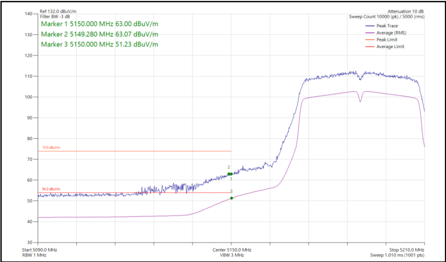
Figure 159 - 802.11n HT40, SISO, Core 1 - 5190 MHz Band Edge Frequency 5150 MHz
