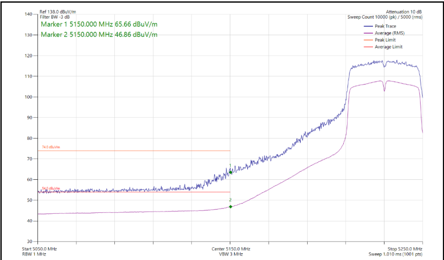
Figure 160 - 802.11n HT40, SISO, Core 1 - 5230 MHz Band Edge Frequency 5150 MHz
