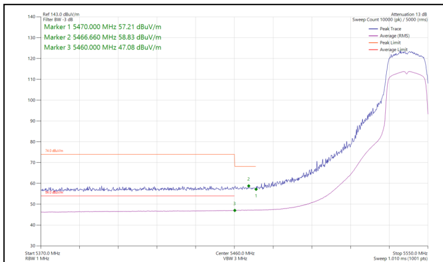
Figure 122 - 802.11ac VHT20, TxBF, Core 0-1 - 5540 MHz Band Edge Frequency 5460 MHz
