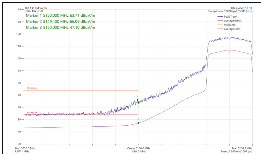
Figure 163 - 802.11ax HE40, SU, SISO, Core 1 - 5230 MHz Band Edge Frequency 5150 MHz
