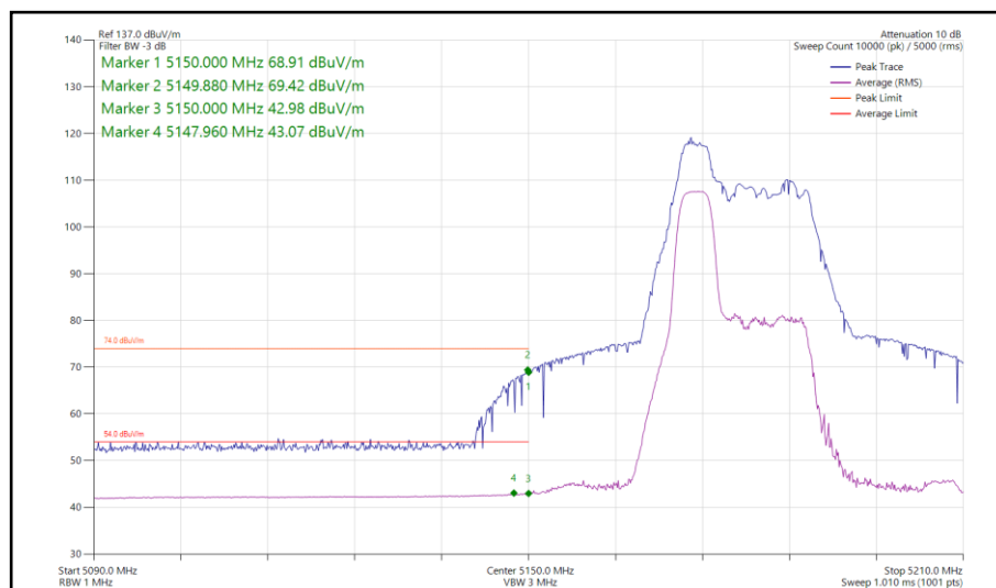
Figure 131 - 802.11ax HE40, RU 52-37, SISO, Core 0 - 5190 MHz Band Edge Frequency 5150 MHz
