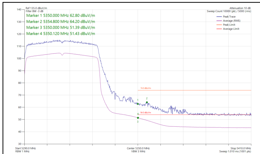
Figure 142 - 802.11ax HE40, SU, SISO, Core 0 - 5310 MHz Band Edge Frequency 5350 MHz
