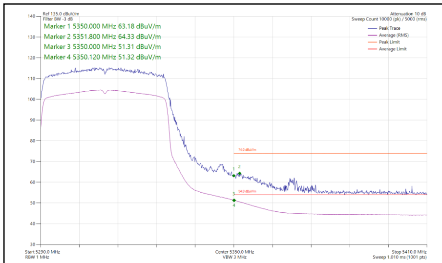
Figure 173 - 802.11ax HE40, SU, SISO, Core 1 - 5310 MHz Band Edge Frequency 5350 MHz
