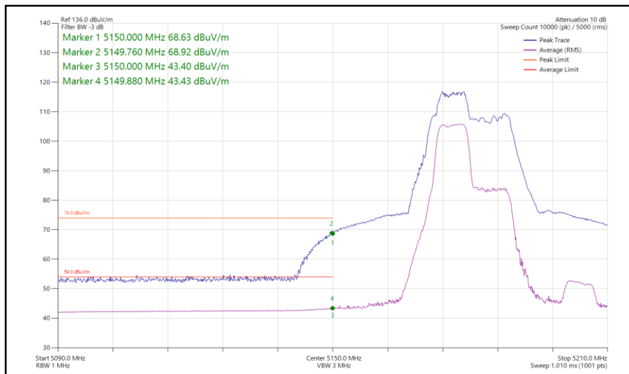
Figure 165 - 802.11be EHT40, RU 52+26-70, SISO, Core 1 - 5190 MHz Band Edge Frequency 5150 MHz
