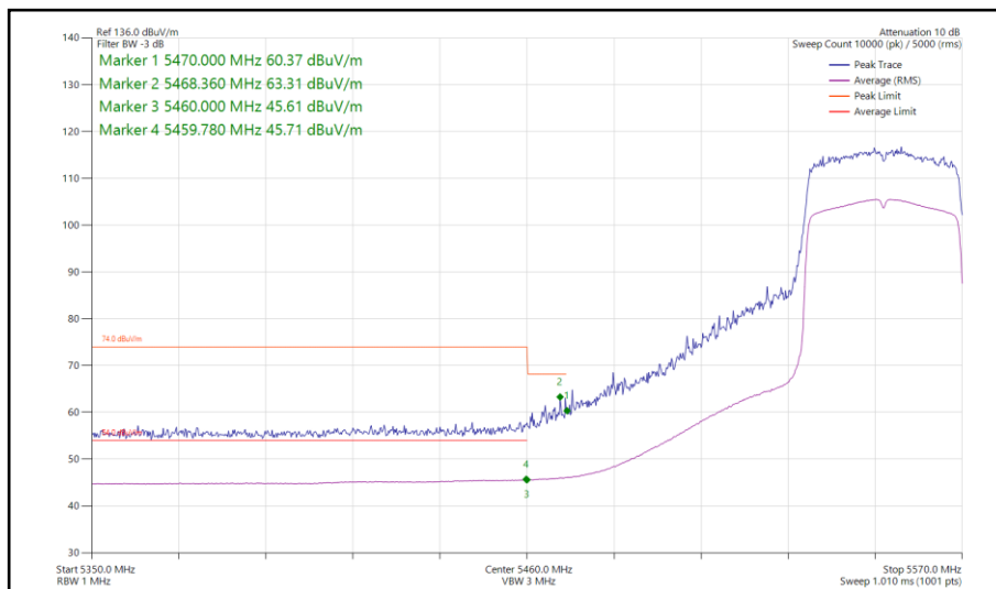
Figure 153 - 802.11ax HE40, SU, SISO, Core 0 - 5550 MHz Band Edge Frequency 5460 MHz
