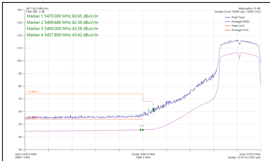
Figure 150 - 802.11n HT40, SISO, Core 0 - 5550 MHz Band Edge Frequency 5460 MHz
