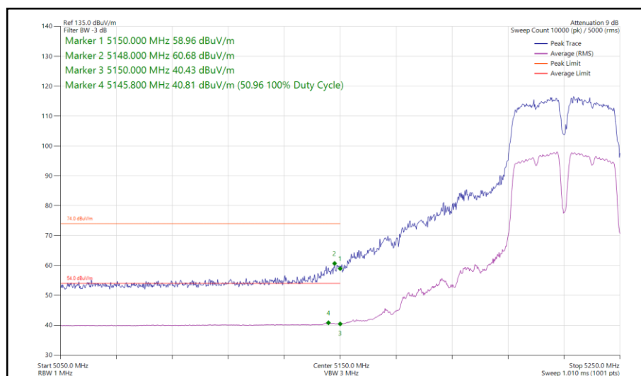
Figure 127 - 802.11a, SISO, Core 0 - 5230 MHz Band Edge Frequency 5150 MHz
