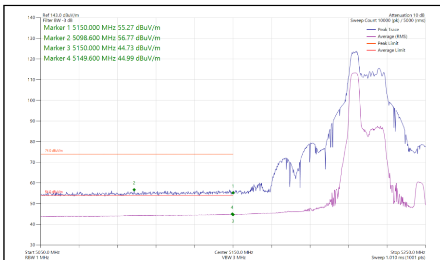
Figure 164 - 802.11ax HE40, RU 52-37, SISO, Core 1 - 5230 MHz Band Edge Frequency 5150 MHz
