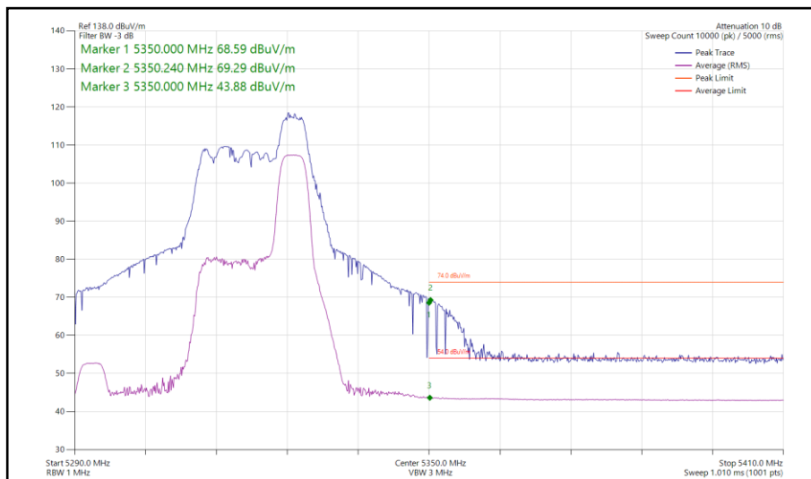
Figure 174 - 802.11ax HE40, RU 52-44, SISO, Core 1 - 5310 MHz Band Edge Frequency 5350 MHz
