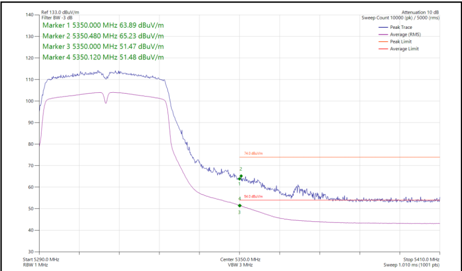
Figure 139 - 802.11n HT40, SISO, Core 0 - 5310 MHz Band Edge Frequency 5350 MHz
