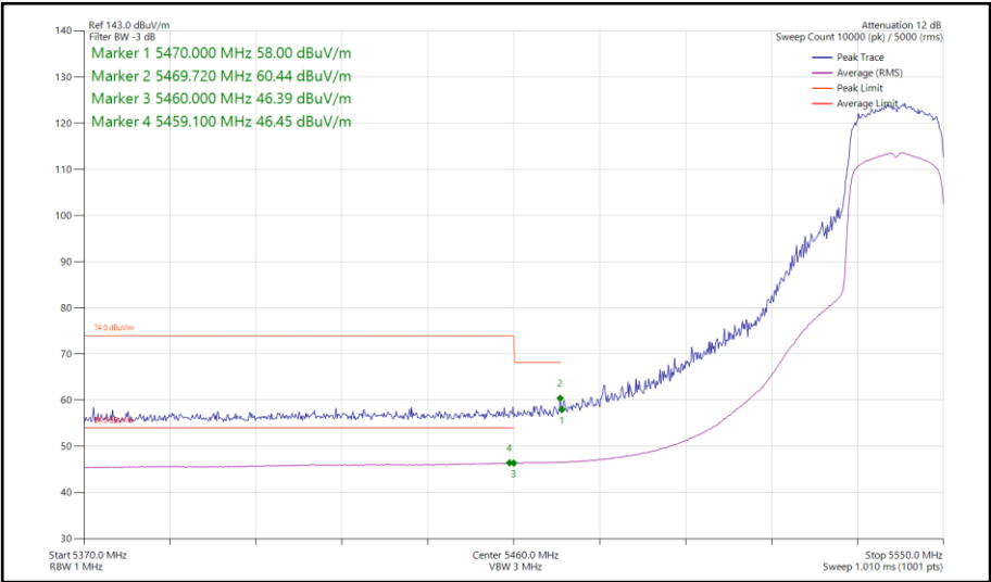
Figure 125 - 802.11ax HE20, SU, TxBF, Core 0-1 - 5540 MHz Band Edge Frequency 5460 MHz
