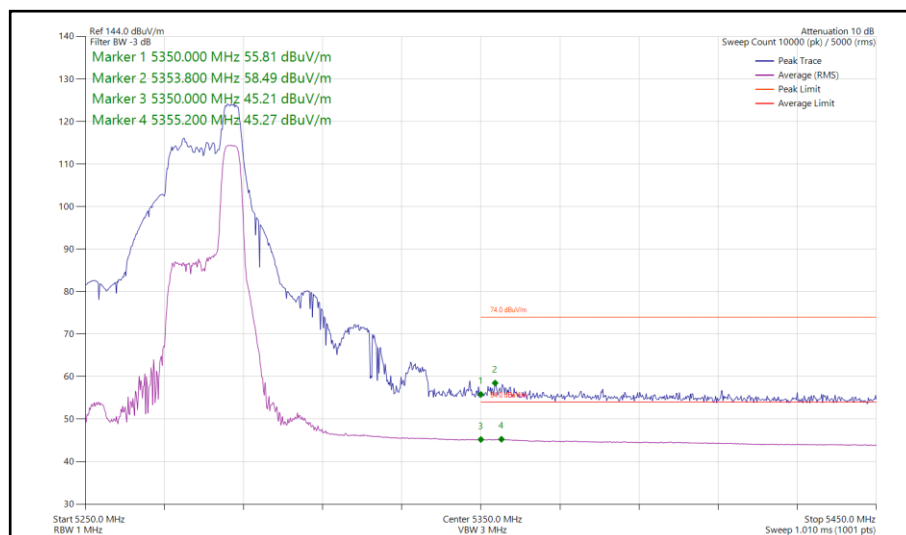
Figure 141 - 802.11ax HE40, RU 52-44, SISO, Core 0 - 5270 MHz Band Edge Frequency 5350 MHz
