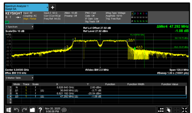
Figure 116 - 802.11a40 SP Maximum 26 dB EBW
