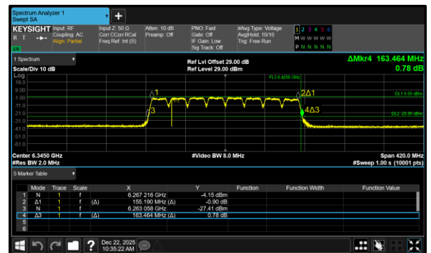
Figure 88 - 802.11a160 VLP Maximum 99% OBW
