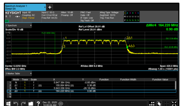
Figure 104 - 802.11a160 LPI Maximum 26 dB EBW
