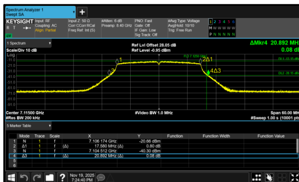
Figure 145 - 802.11a20 LPI Minimum 99% OBW
