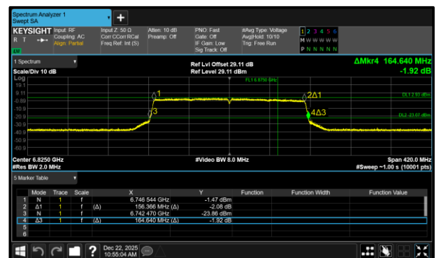
Figure 96 - 802.11ax HE160 SU VLP Maximum 99% OBW
