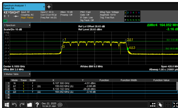
Figure 87 - 802.11a160 VLP Minimum 99% OBW
