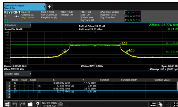
Figure 82 - 802.11a20 VLP Maximum 99% OBW
