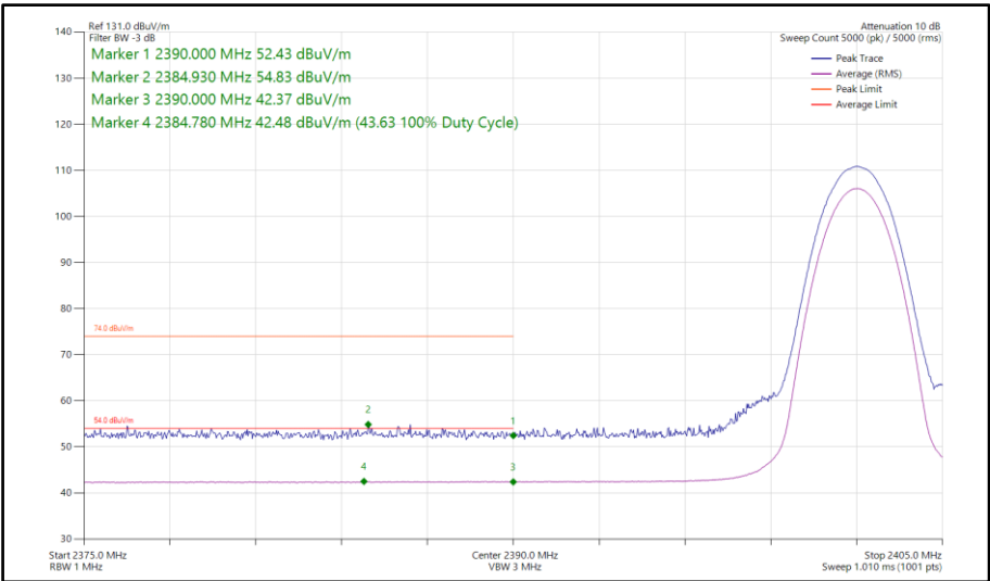
Figure 50 - Bluetooth 3DH5, MIMO, Core 0-1 - 2402 MHz Band Edge Frequency 2390 MHz
