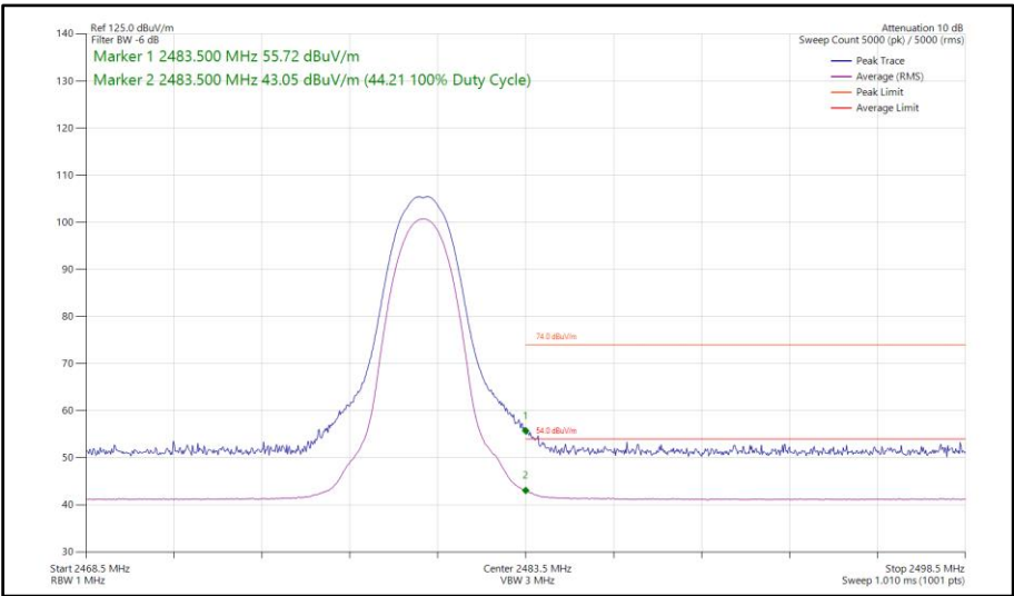
Figure 13 - Bluetooth 2DH5, SISO, Core 0 - 2480 MHz Band Edge Frequency 2483.5 MHz
