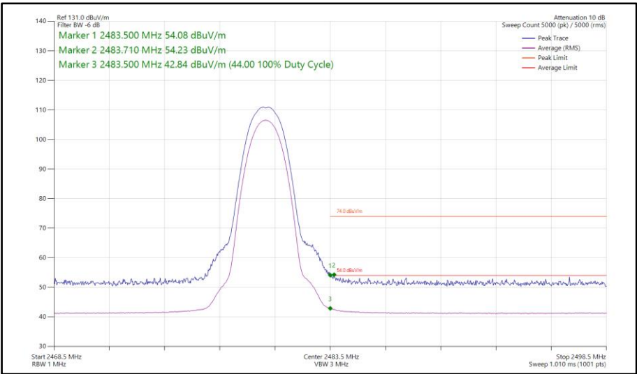
Figure 61 - Bluetooth 2DH5, MIMO, Core 0-1 - 2480 MHz Band Edge Frequency 2483.5 MHz
