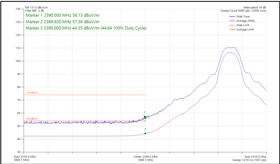
Figure 56 - Bluetooth HDT4, MIMO, Core 0-1 - 2404 MHz Band Edge Frequency 2390 MHz
