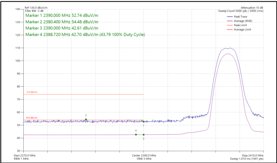
Figure 51 - Bluetooth HDR4, MIMO, Core 0-1 - 2404 MHz Band Edge Frequency 2390 MHz
