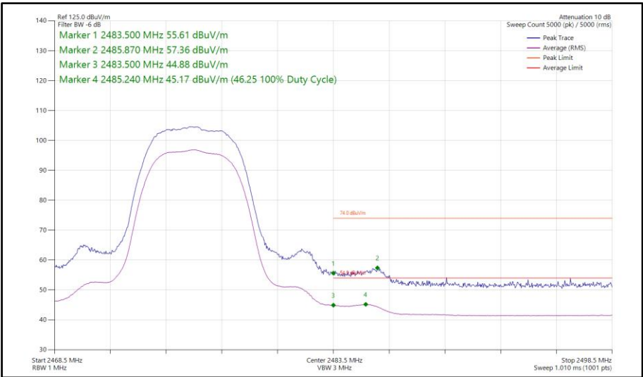
Figure 16 - Bluetooth HDR8, SISO, Core 0 - 2476 MHz Band Edge Frequency 2483.5 MHz
