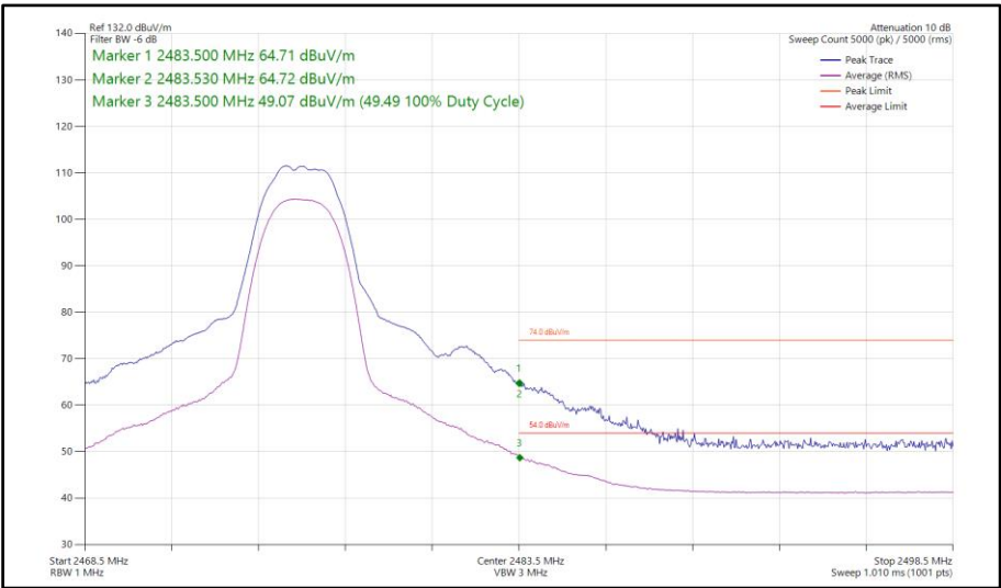
Figure 69 - Bluetooth HDT6, MIMO, Core 0-1 - 2476 MHz Band Edge Frequency 2483.5 MHz
