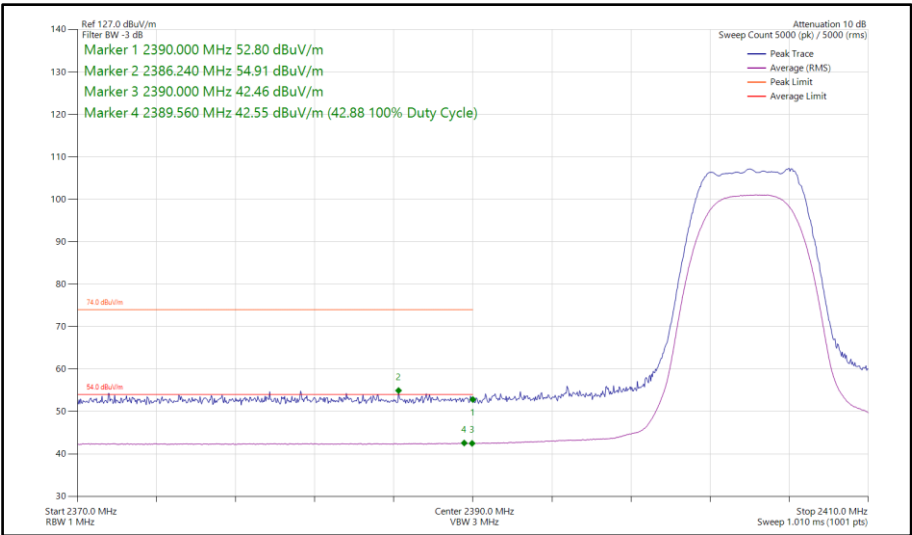
Figure 60 - Bluetooth XHDRPM8, MIMO, Core 0-1 - 2404 MHz Band Edge Frequency 2390 MHz
