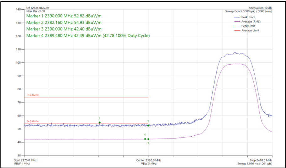
Figure 59 - Bluetooth HDRPM12, MIMO, Core 0-1 - 2404 MHz Band Edge Frequency 2390 MHz
