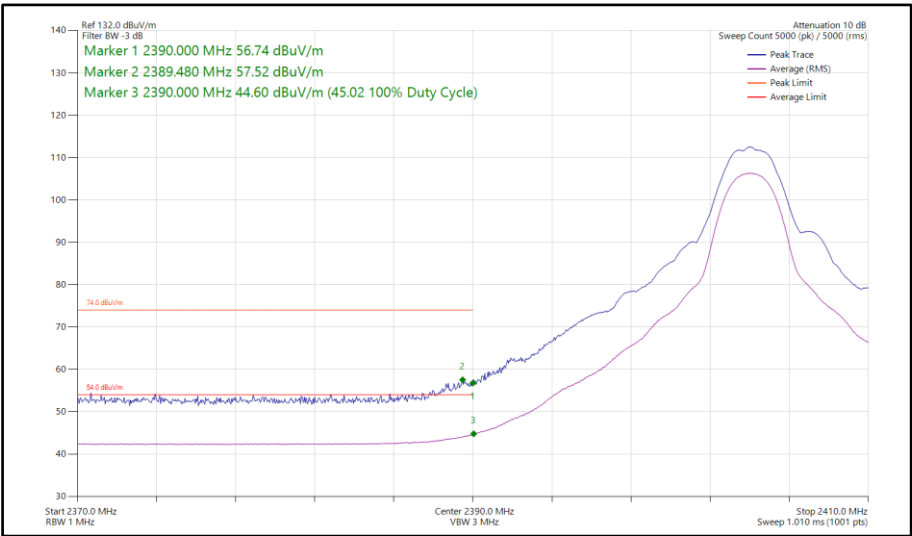
Figure 57 - Bluetooth HDT6, MIMO, Core 0-1 - 2404 MHz Band Edge Frequency 2390 MHz
