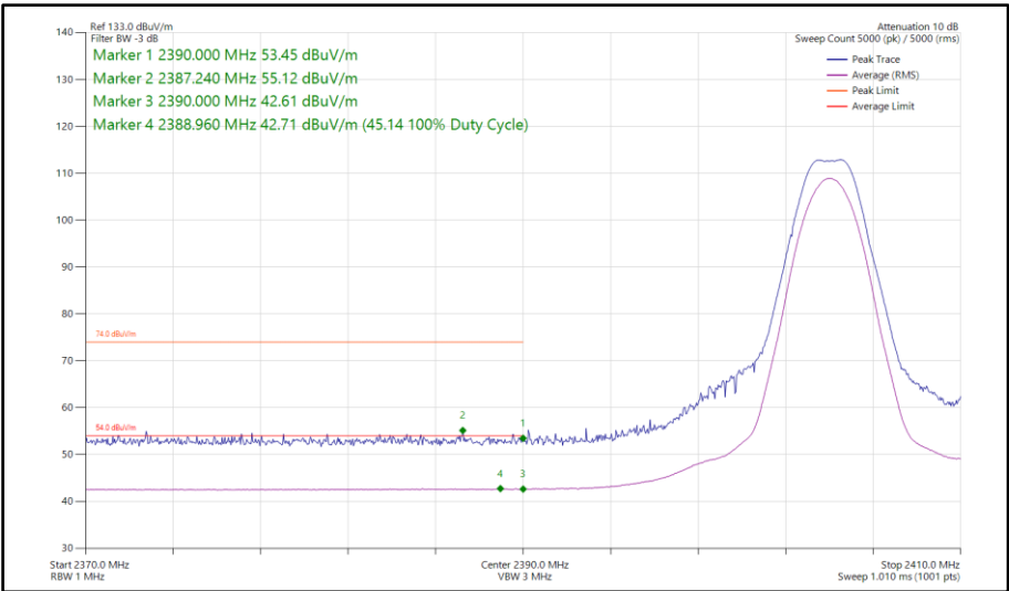
Figure 54 - Bluetooth LE2M, MIMO, Core 0-1 - 2404 MHz Band Edge Frequency 2390 MHz
