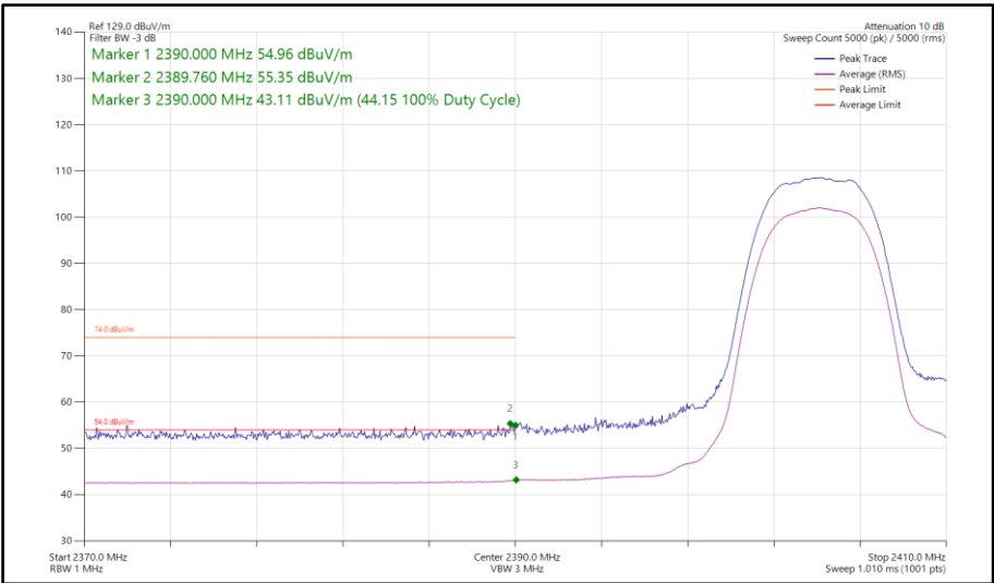
Figure 52 - Bluetooth HDR8, MIMO, Core 0-1 - 2404 MHz Band Edge Frequency 2390 MHz
