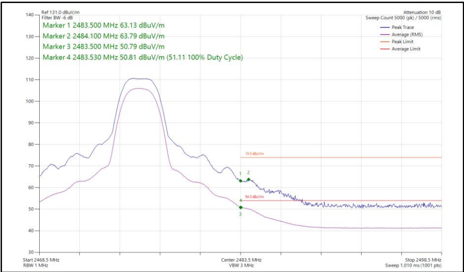
Figure 68 - Bluetooth HDT4, MIMO, Core 0-1 - 2476 MHz Band Edge Frequency 2483.5 MHz
