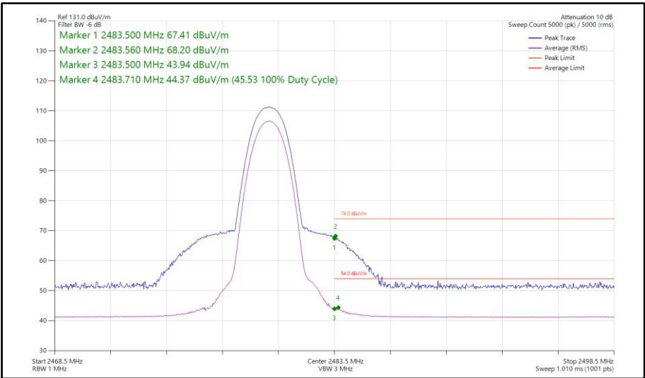
Figure 62 - Bluetooth 3DH5, MIMO, Core 0-1 - 2480 MHz Band Edge Frequency 2483.5 MHz
