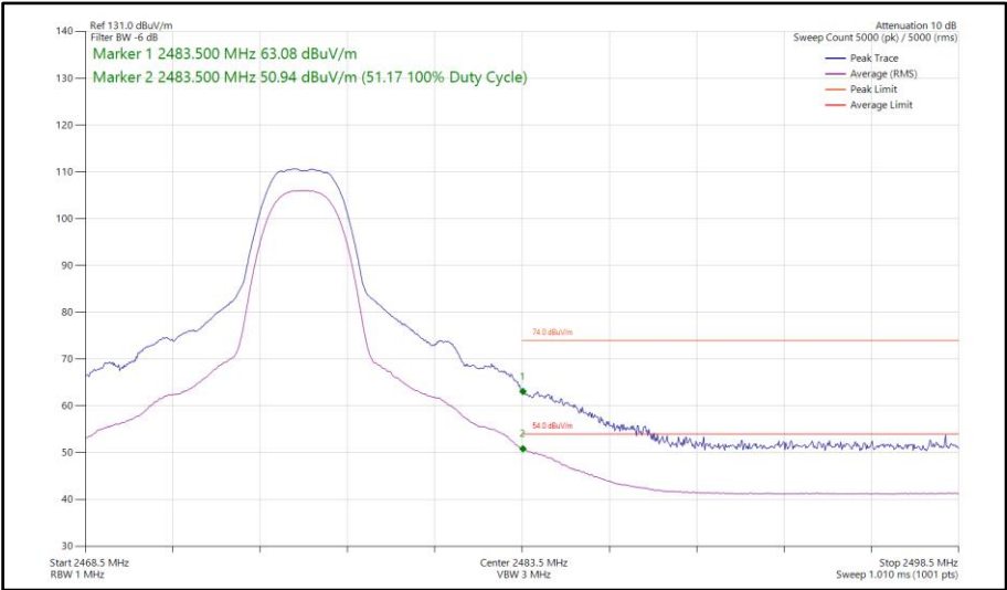
Figure 67 - Bluetooth HDT3, MIMO, Core 0-1 - 2476 MHz Band Edge Frequency 2483.5 MHz
