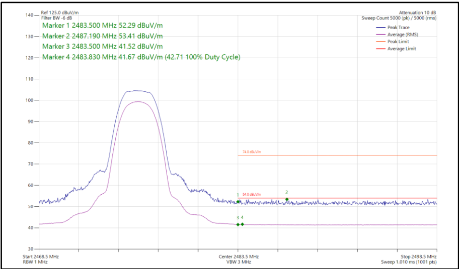
Figure 15 - Bluetooth HDR4, SISO, Core 0 - 2476 MHz Band Edge Frequency 2483.5 MHz
