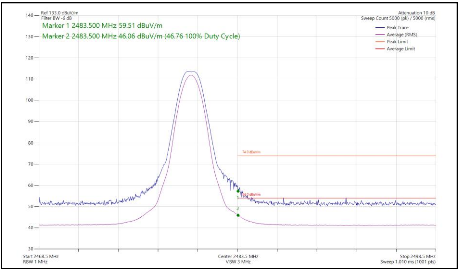
Figure 65 - Bluetooth LE1M, MIMO, Core 0-1 - 2480 MHz Band Edge Frequency 2483.5 MHz
