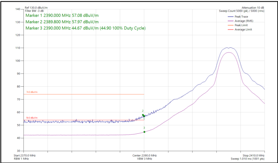
Figure 55 - Bluetooth HDT3, MIMO, Core 0-1 - 2404 MHz Band Edge Frequency 2390 MHz
