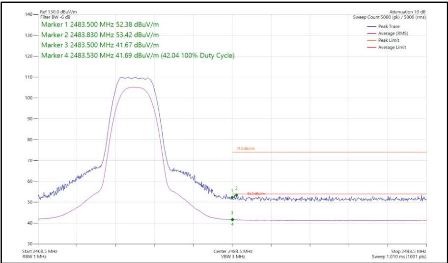
Figure 70 - Bluetooth HDRPS2, MIMO, Core 0-1 - 2476 MHz Band Edge Frequency 2483.5 MHz
