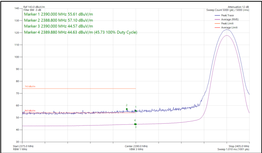
Figure 74 - Bluetooth 3DH5, SISO, Core 0 - 2402 MHz Band Edge Frequency 2390 MHz
