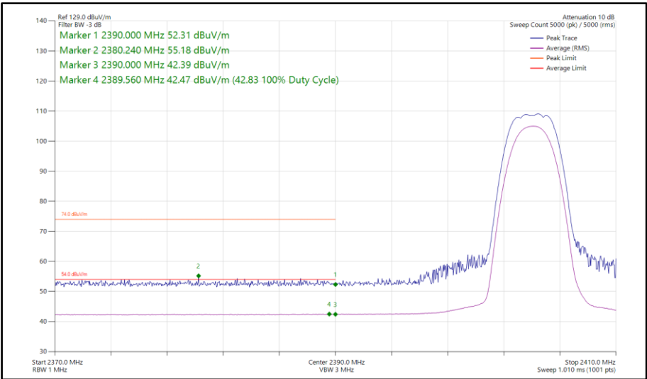
Figure 58 - Bluetooth HDRPS2, MIMO, Core 0-1 - 2404 MHz Band Edge Frequency 2390 MHz
