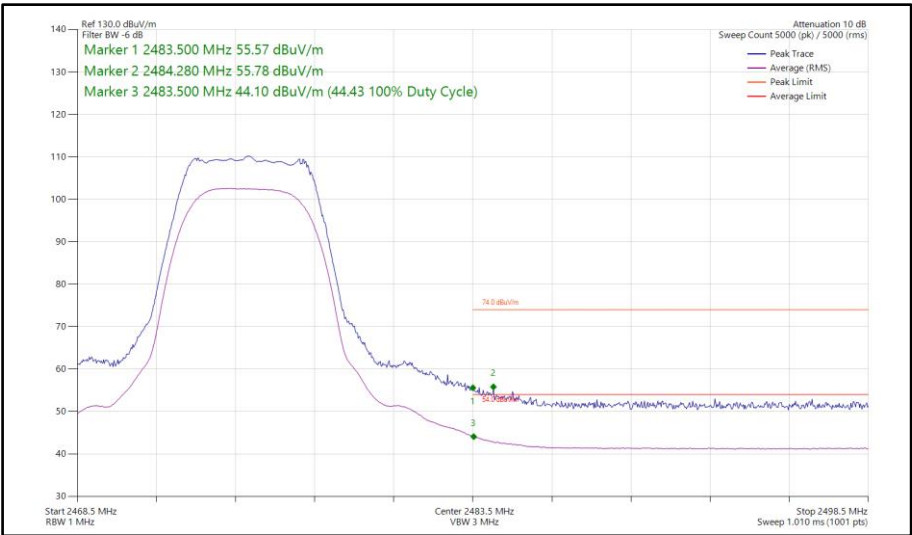
Figure 72 - Bluetooth XHDRPM8, MIMO, Core 0-1 - 2475 MHz Band Edge Frequency 2483.5 MHz
