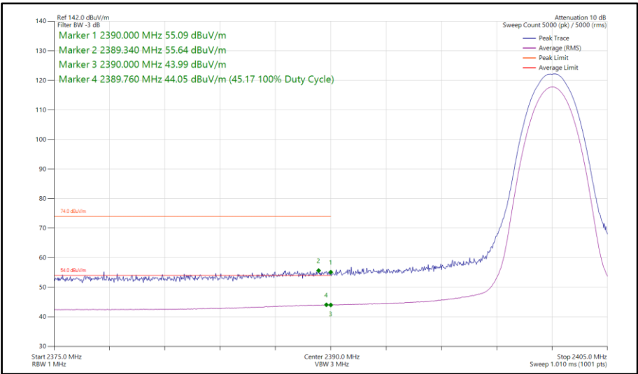
Figure 73 - Bluetooth 2DH5, SISO, Core 0 - 2402 MHz Band Edge Frequency 2390 MHz
