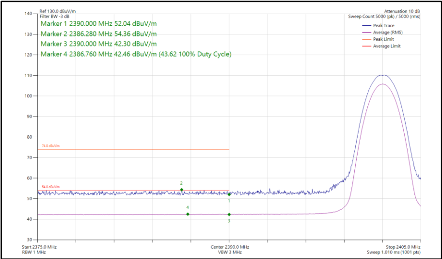
Figure 49 - Bluetooth 2DH5, MIMO, Core 0-1 - 2402 MHz Band Edge Frequency 2390 MHz
