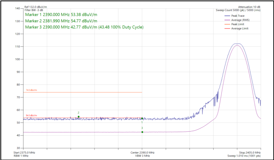
Figure 53 - Bluetooth LE1M, MIMO, Core 0-1 - 2402 MHz Band Edge Frequency 2390 MHz
