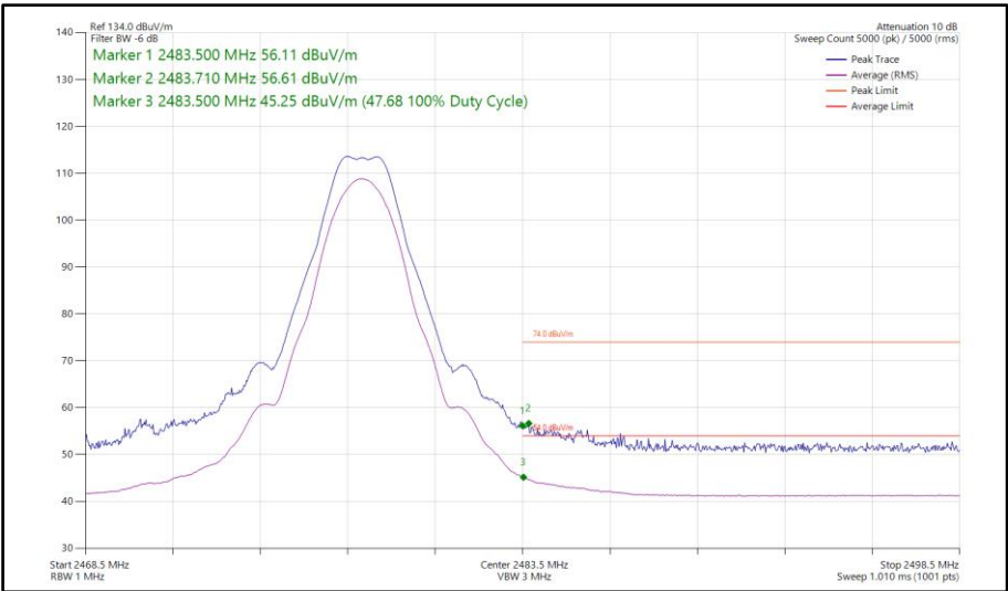
Figure 66 - Bluetooth LE2M, MIMO, Core 0-1 - 2478 MHz Band Edge Frequency 2483.5 MHz
