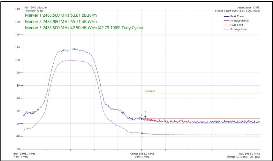
Figure 71 - Bluetooth HDRPM12, MIMO, Core 0-1 - 2475 MHz Band Edge Frequency 2483.5 MHz
