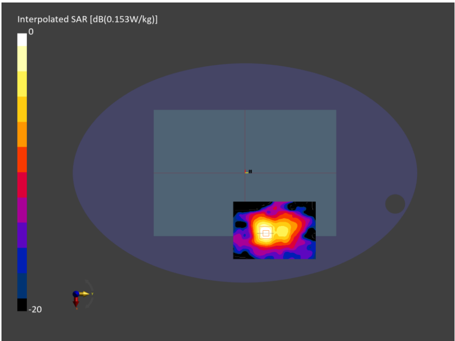
Figure C.7: SAR Testing Results for A3449 at 5788 MHz
