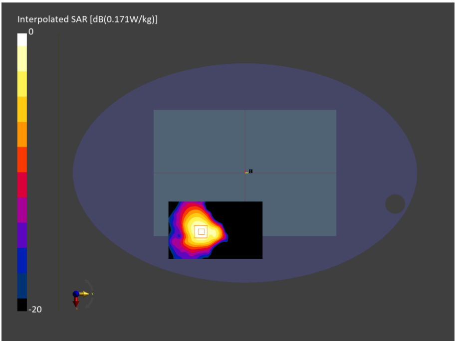
Figure C.4: SAR Testing Results for A3449 at 5150 MHz
