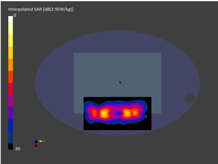
Figure C.27: SAR Testing Results for A3449 at 5690 MHz
