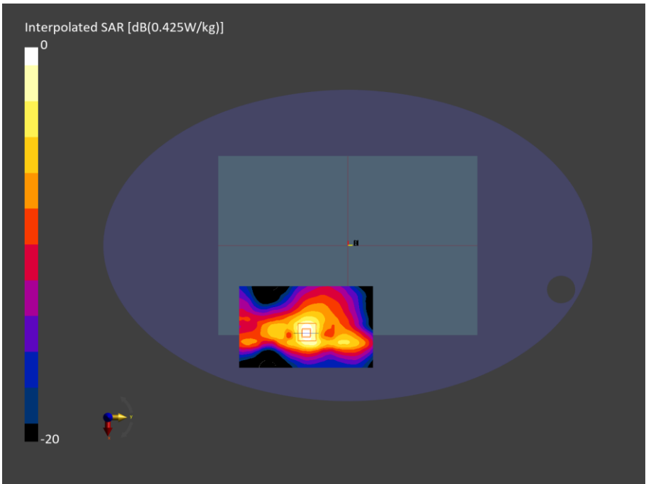
Figure C.14: SAR Testing Results for A3449 at 2437 MHz
