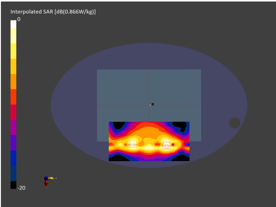
Figure C.18: SAR Testing Results for A3449 at 2437 MHz
