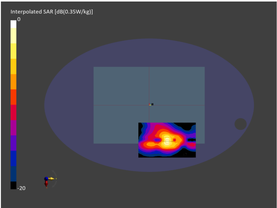
Figure C.1: SAR Testing Results for A3449 at 2441 MHz
