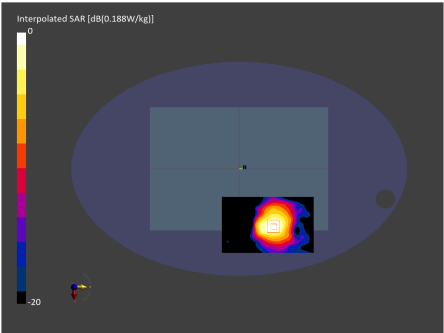
Figure C.3: SAR Testing Results for A3449 at 5250 MHz
