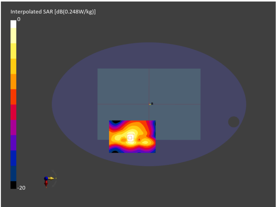
Figure C.10: SAR Testing Results for A3449 at 2405 MHz
