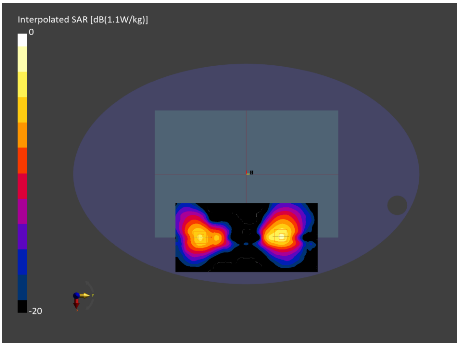
Figure C.24: SAR Testing Results for A3449 at 5270 MHz
