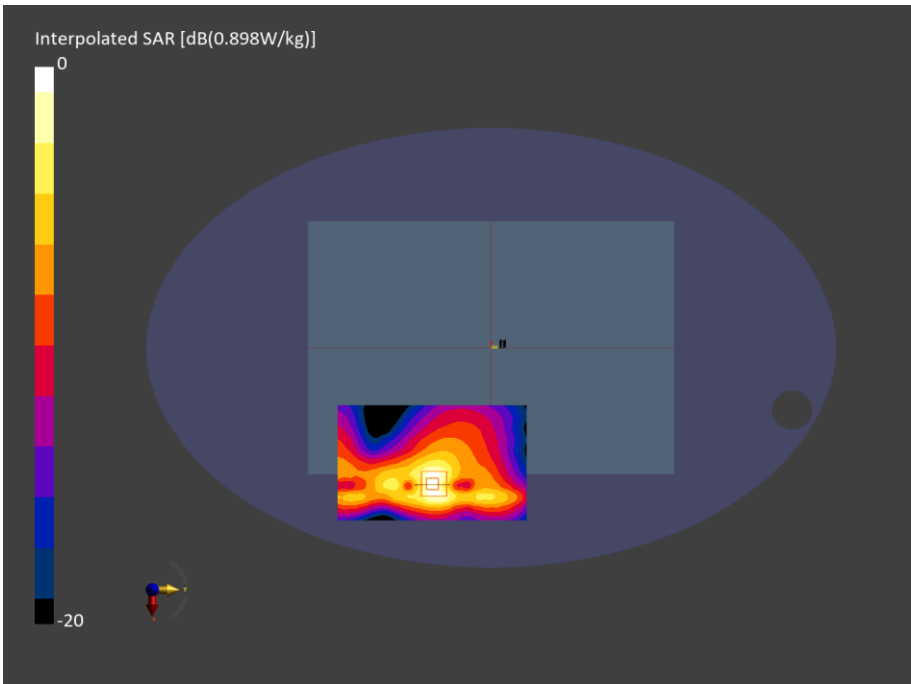
Figure C.17: SAR Testing Results for A3449 at 2437 MHz
