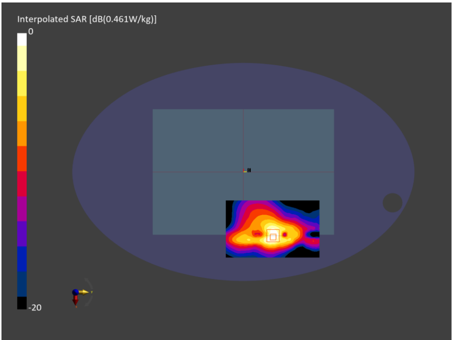
Figure C.13: SAR Testing Results for A3449 at 2462 MHz
