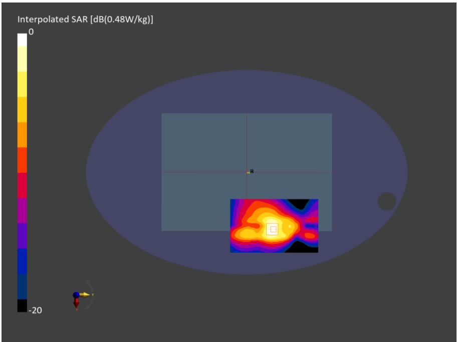
Figure C.11: SAR Testing Results for A3449 at 2440 MHz
