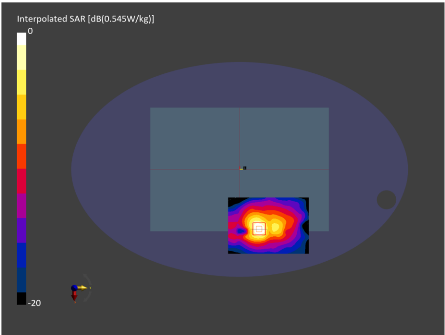
Figure C.5: SAR Testing Results for A3449 at 5850 MHz
