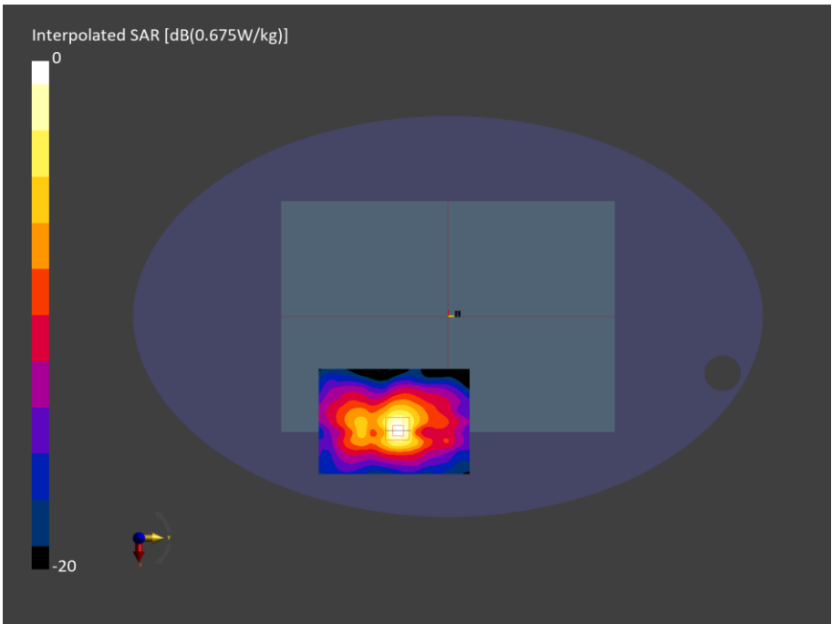
Figure C.6: SAR Testing Results for A3449 at 5788 MHz
