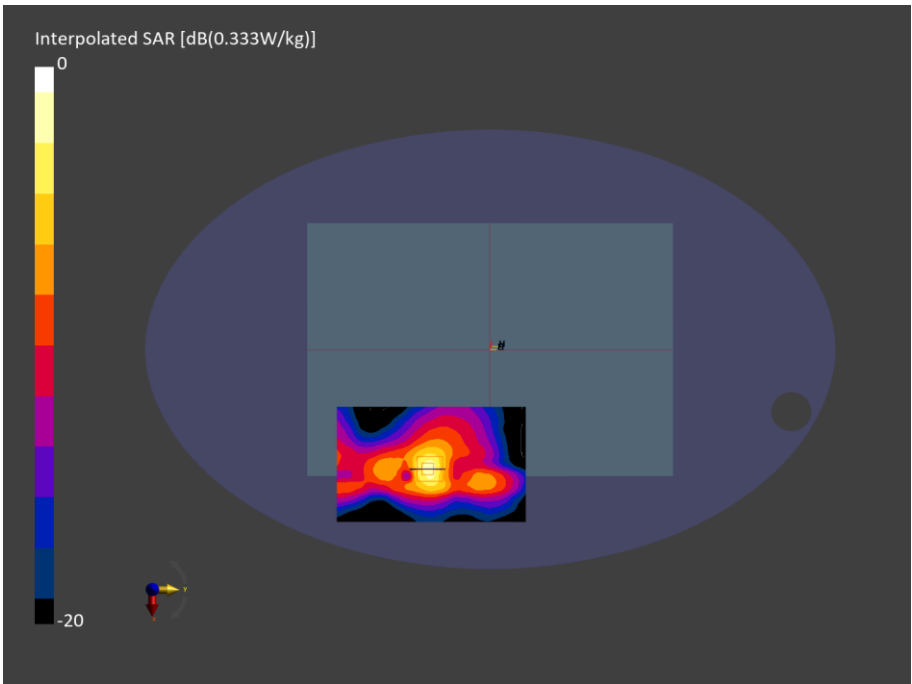
Figure C.12: SAR Testing Results for A3449 at 2405 MHz
