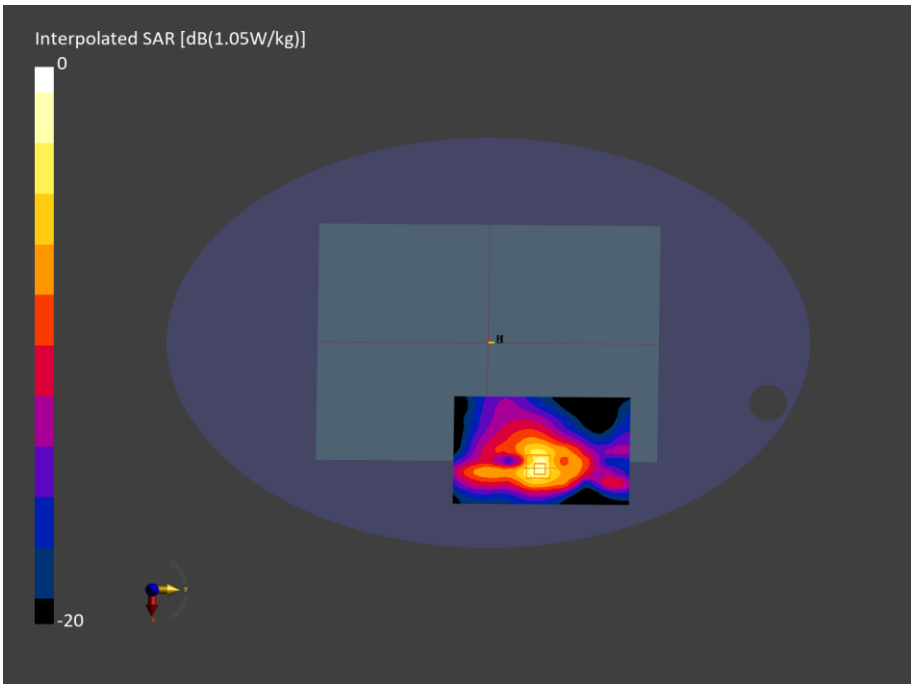
Figure C.16: SAR Testing Results for A3449 at 2437 MHz
