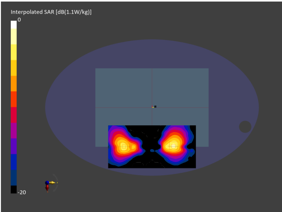
Figure C.21: SAR Testing Results for A3449 at 5230 MHz
