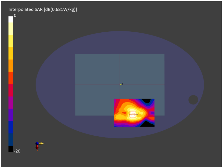
Figure C.9: SAR Testing Results for A3449 at 2440 MHz
