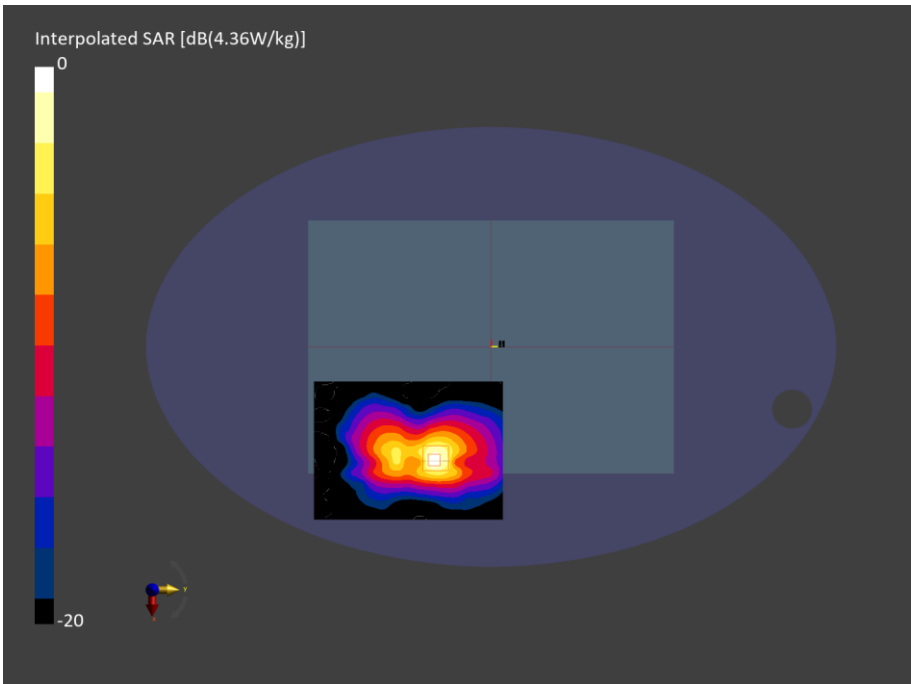
Figure C.26: SAR Testing Results for A3449 at 5690 MHz
