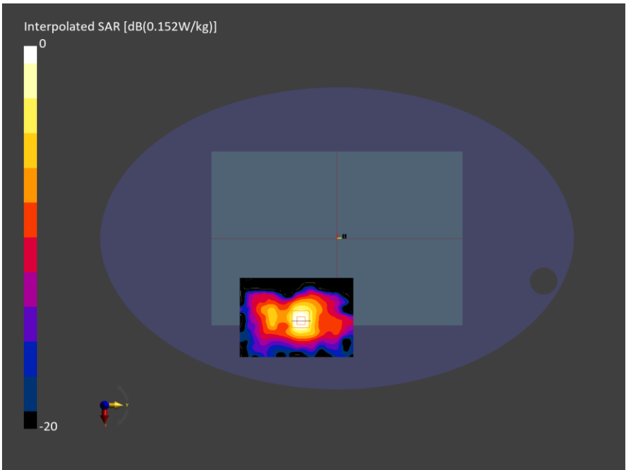
Figure C.8: SAR Testing Results for A3449 at 5788 MHz
