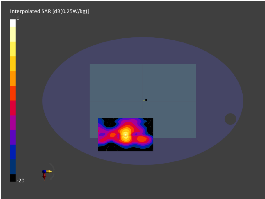
Figure C.2: SAR Testing Results for A3449 at 2441 MHz
