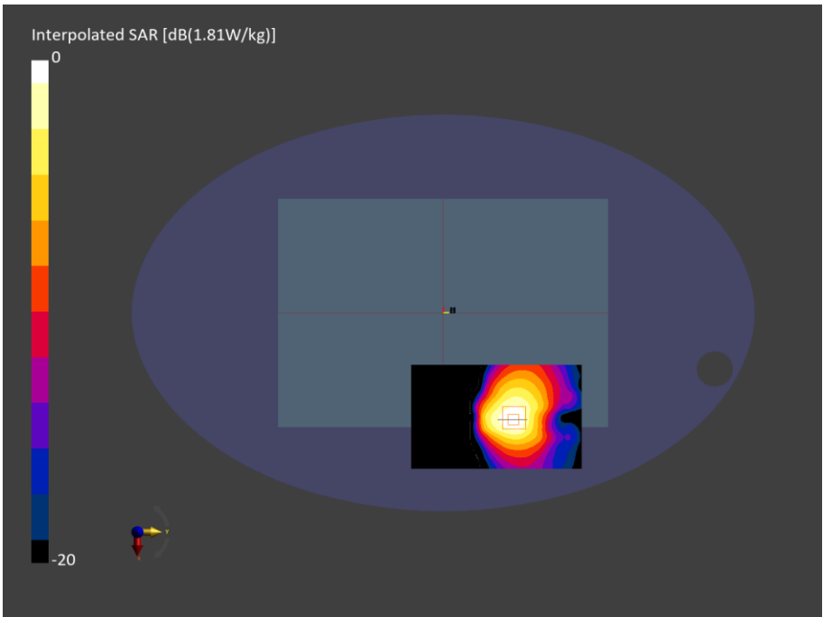
Figure C.22: SAR Testing Results for A3449 at 5300 MHz
