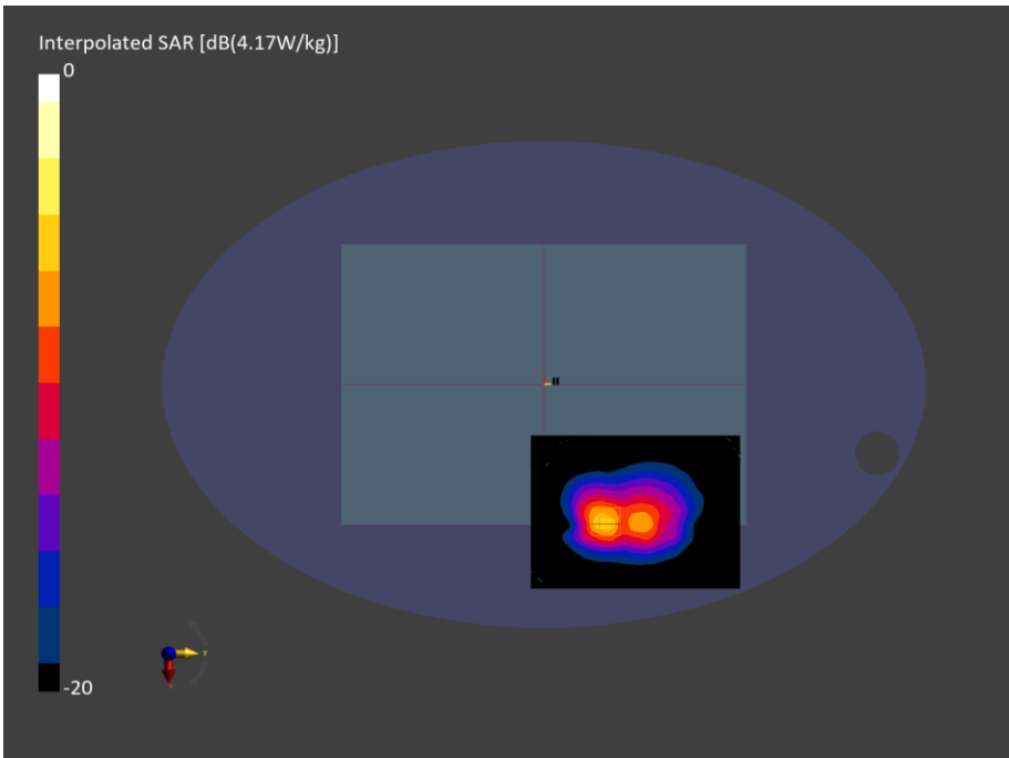
Figure C.25: SAR Testing Results for A3449 at 5690 MHz
