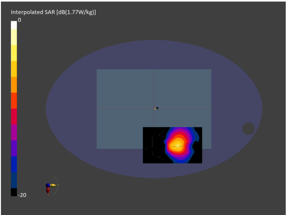
Figure C.19: SAR Testing Results for A3449 at 5200 MHz
