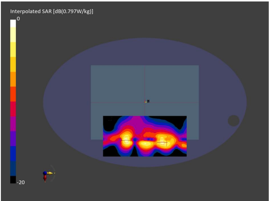
Figure C.15: SAR Testing Results for A3449 at 2417 MHz
