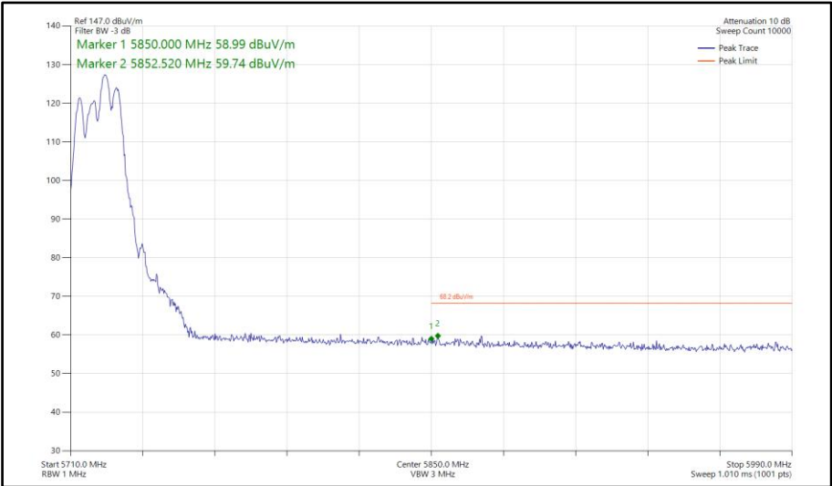
Figure 828 - 802.11be EHT20, RU 106+26-83, CDD, Core 0-1 - 5720 MHz Band Edge Frequency 5850 MHz
