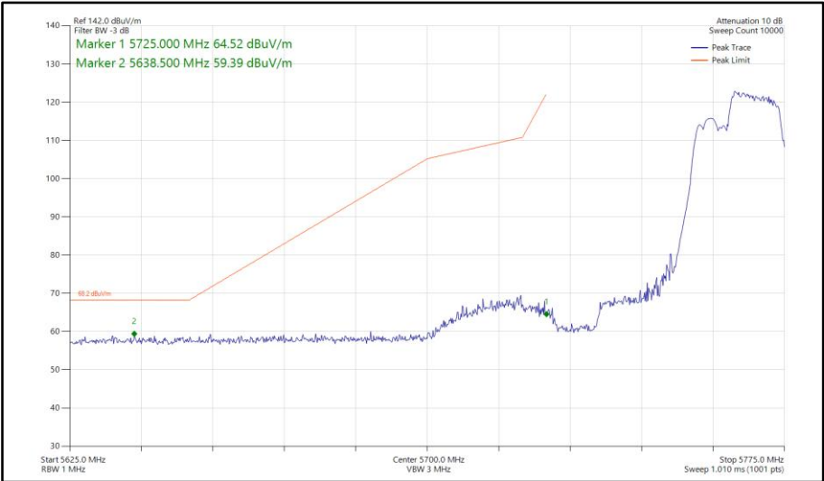
Figure 896 - 802.11be EHT40, RU 106+26-85, SISO, Core 0 - 5755 MHz Band Edge Frequency 5725 MHz
