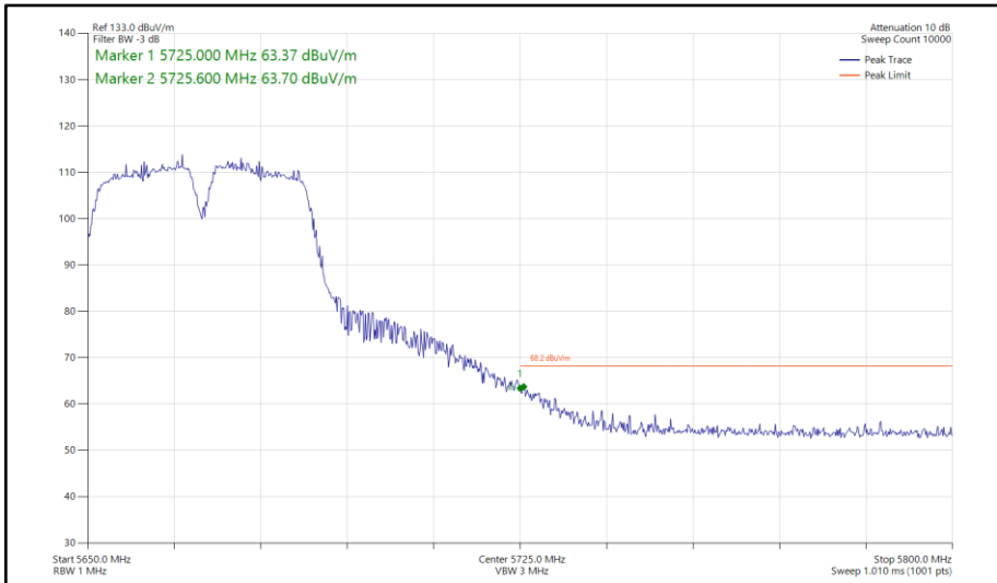
Figure 898 - 802.11a, SISO, Core 0 - 5670 MHz Band Edge Frequency 5725 MHz
