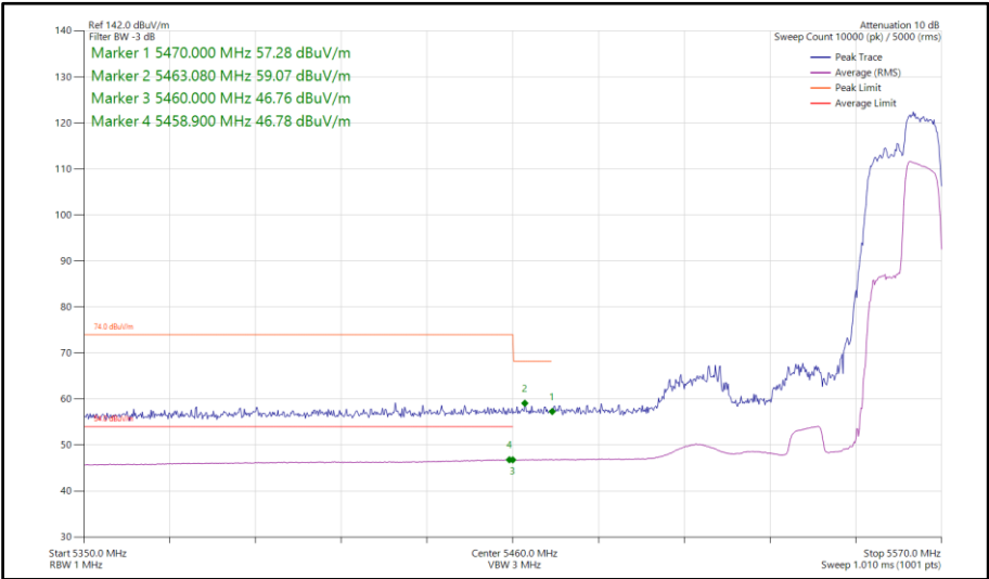
Figure 889 - 802.11ax HE40, RU 106-56, SISO, Core 0 - 5550 MHz Band Edge Frequency 5470 MHz
