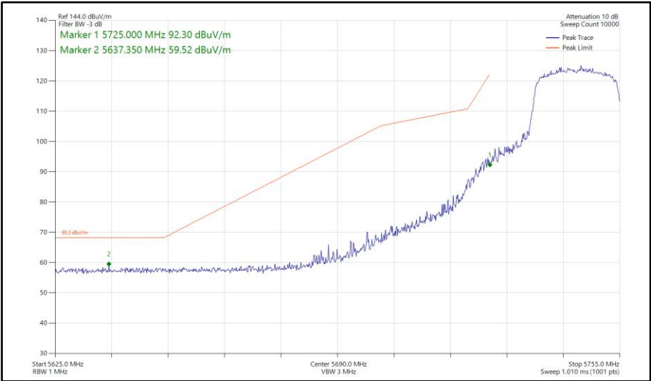
Figure 870 - 802.11ax HE20, SU, TxBF, Core 0-1 - 5745 MHz Band Edge Frequency 5725 MHz
