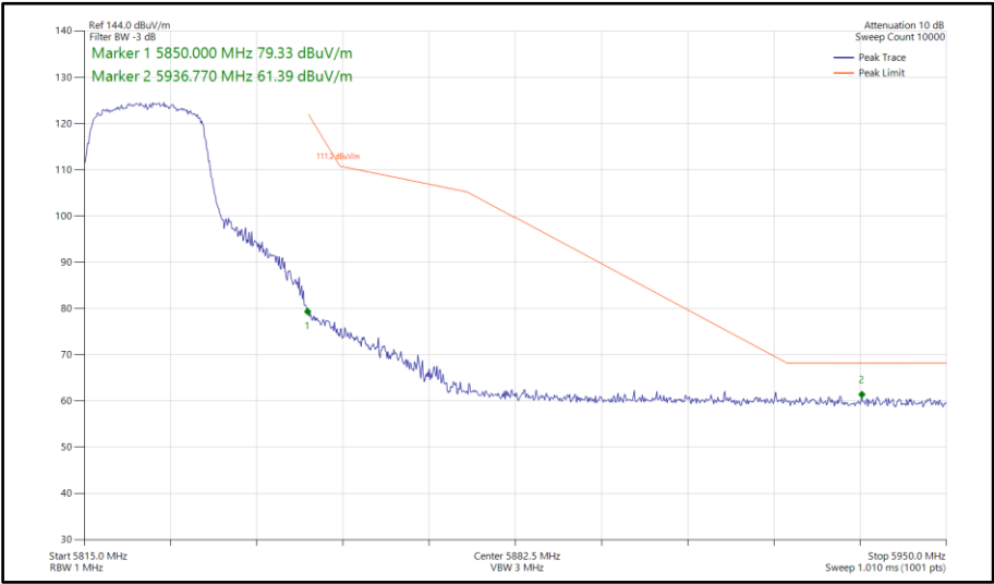
Figure 858 - 802.11n HT20, SDM, Core 0-1 - 5825 MHz Band Edge Frequency 5850 MHz
