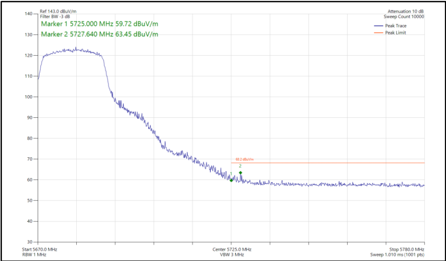
Figure 872 - 802.11ac VHT20, TxBF, Core 0-1 - 5680 MHz Band Edge Frequency 5725 MHz
