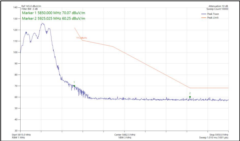
Figure 827 - 802.11ax HE20, RU 106-54, CDD, Core 0-1 - 5825 MHz Band Edge Frequency 5850 MHz
