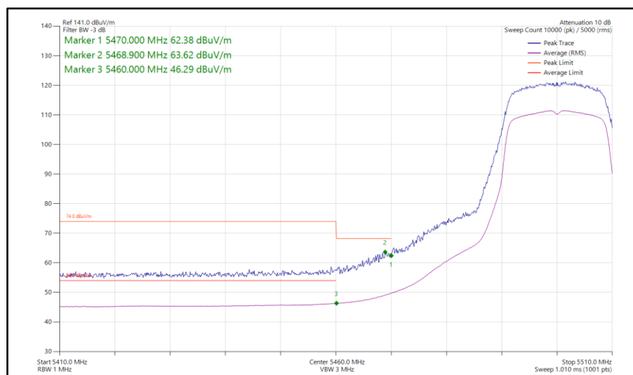
Figure 863 - 802.11ac VHT20, TxBF, Core 0-1 - 5500 MHz Band Edge Frequency 5470 MHz
