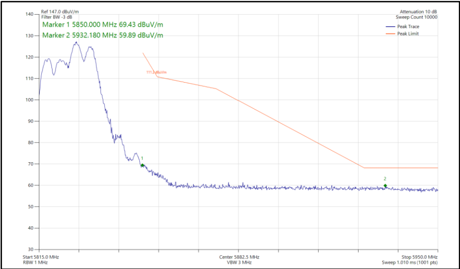
Figure 829 - 802.11be EHT20, RU 106+26-83, CDD, Core 0-1 - 5825 MHz Band Edge Frequency 5850 MHz
