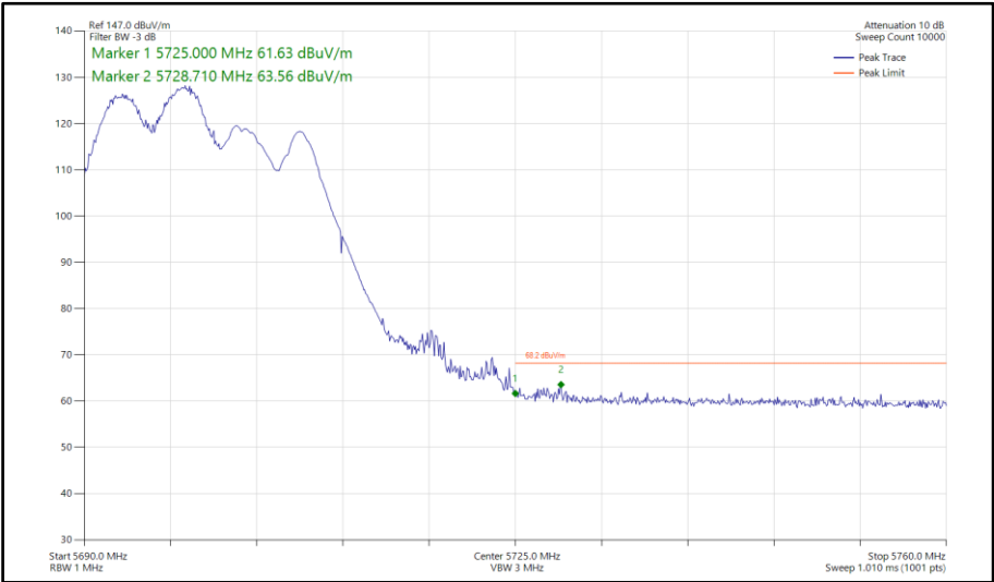
Figure 854 - 802.11be EHT20, RU 106+26-82, SDM, Core 0-1 - 5700 MHz Band Edge Frequency 5725 MHz
