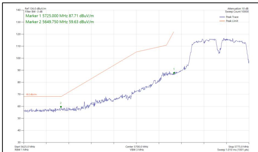
Figure 892 - 802.11a, SISO, Core 0 - 5755 MHz Band Edge Frequency 5725 MHz
