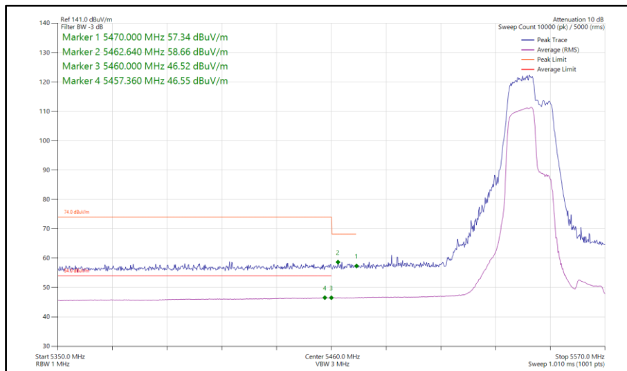
Figure 891 - 802.11be EHT40, RU 106+26-82, SISO, Core 0 - 5550 MHz Band Edge Frequency 5470 MHz
