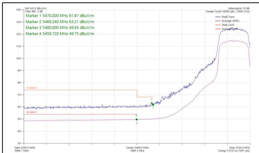
Figure 831 - 802.11n HT20, SDM, Core 0-1 - 5520 MHz Band Edge Frequency 5470 MHz
