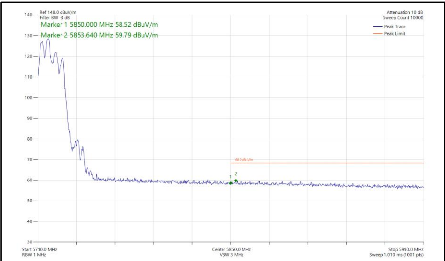
Figure 857 - 802.11ax HE20, RU 106-53, SDM, Core 0-1 - 5720 MHz Band Edge Frequency 5850 MHz
