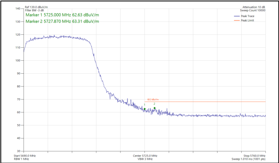
Figure 850 - 802.11ax HE20, SU, SDM, Core 0-1 - 5700 MHz Band Edge Frequency 5725 MHz
