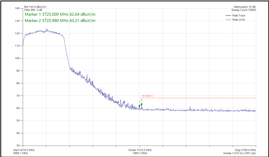
Figure 848 - 802.11ax HE20, SU, SDM, Core 0-1 - 5680 MHz Band Edge Frequency 5725 MHz
