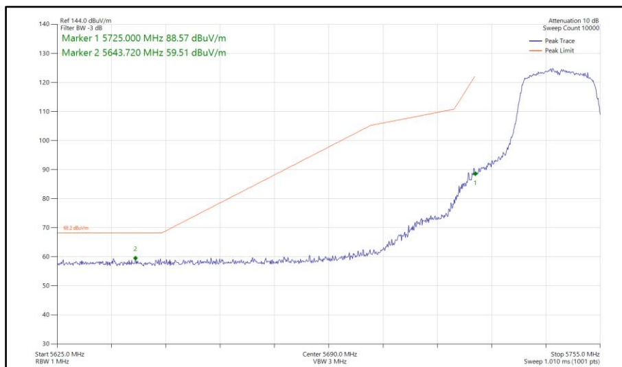
Figure 869 - 802.11ac VHT20, TxBF, Core 0-1 - 5745 MHz Band Edge Frequency 5725 MHz
