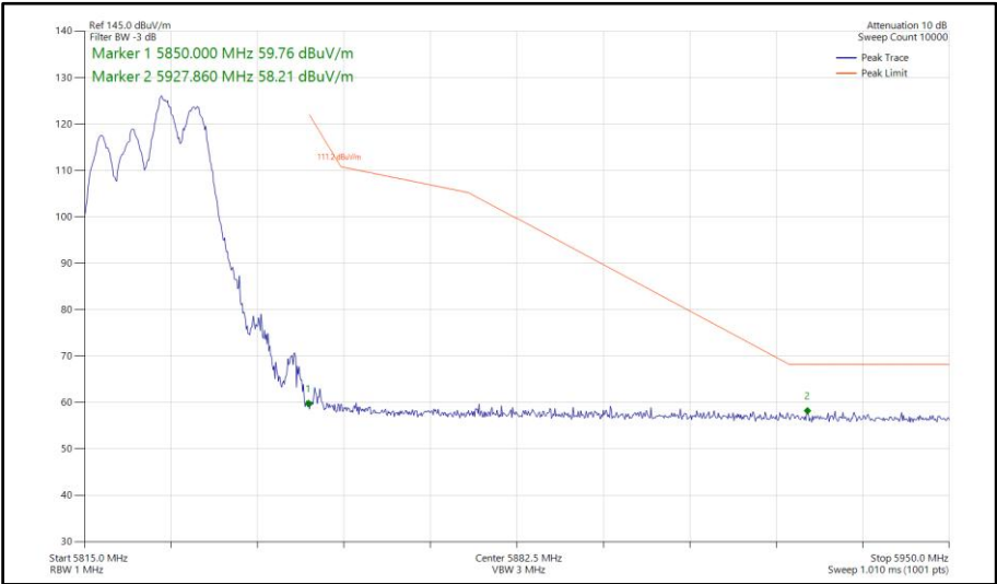
Figure 860 - 802.11ax HE20, RU 106-54, SDM, Core 0-1 - 5825 MHz Band Edge Frequency 5850 MHz
