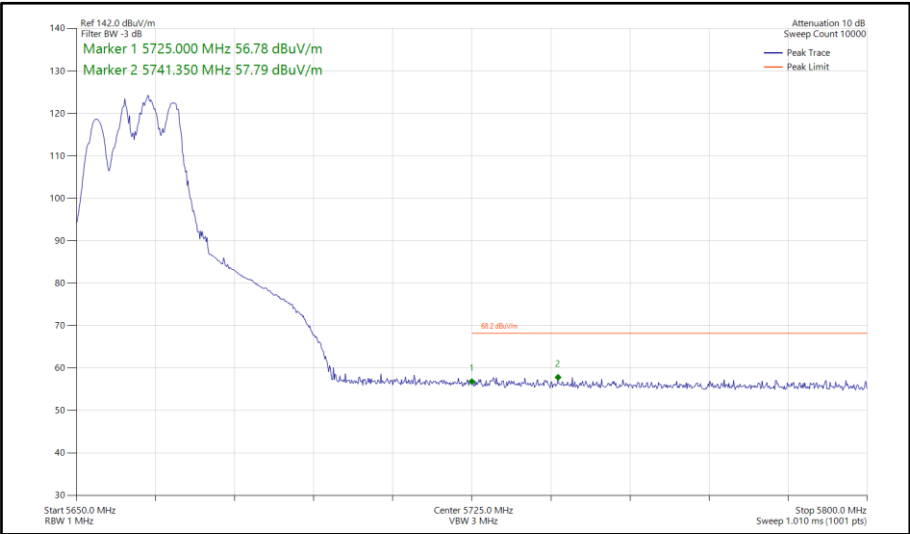
Figure 852 - 802.11be EHT20, RU 160+26-83, SDM, Core 0-1 - 5660 MHz Band Edge Frequency 5725 MHz
