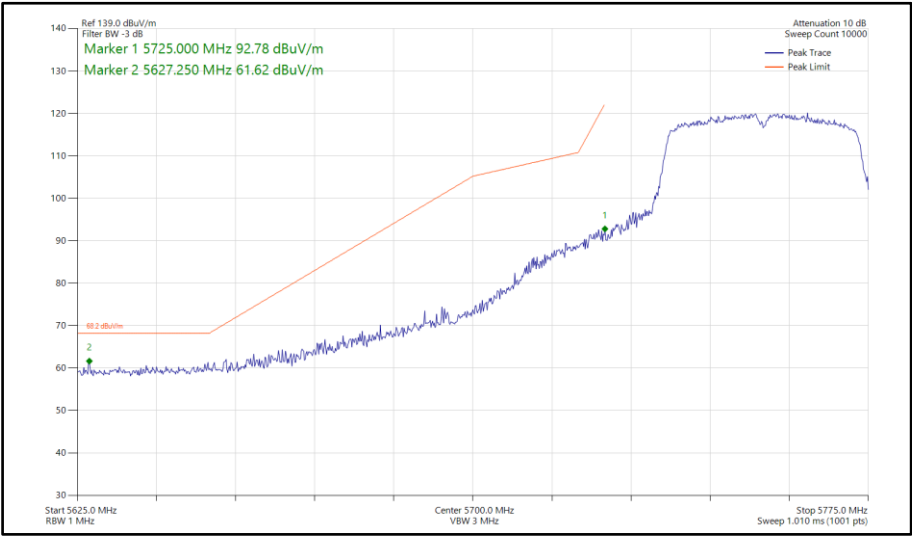
Figure 893 - 802.11n HT40, SISO, Core 0 - 5755 MHz Band Edge Frequency 5725 MHz
