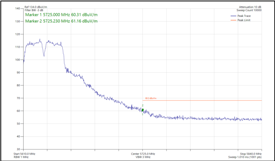
Figure 897 - 802.11a, SISO, Core 0 - 5630 MHz Band Edge Frequency 5725 MHz
