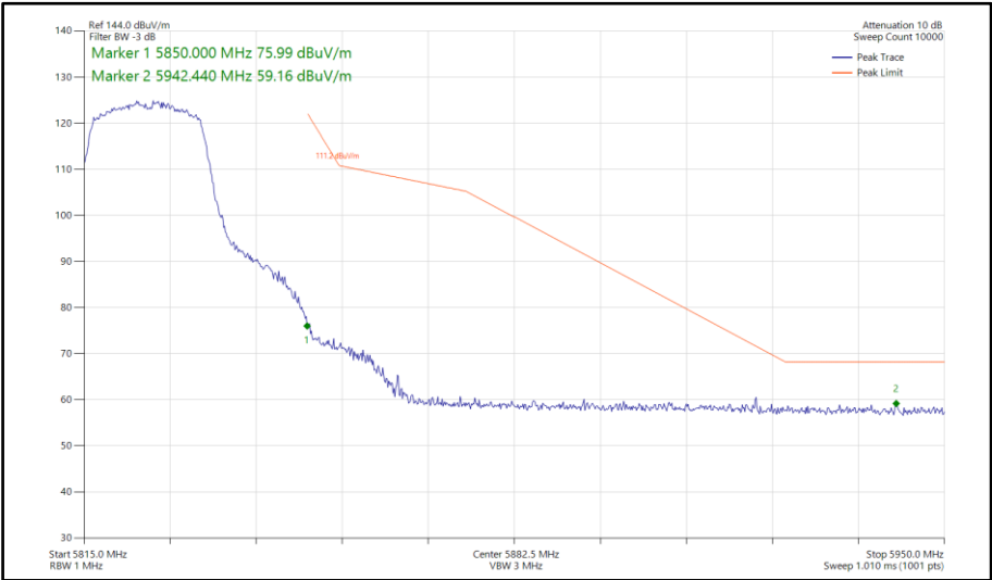
Figure 878 - 802.11ac VHT20, TxBF, Core 0-1 - 5825 MHz Band Edge Frequency 5850 MHz
