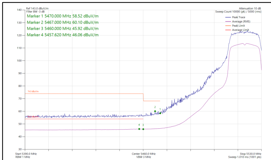
Figure 864 - 802.11ac VHT20, TxBF, Core 0-1 - 5520 MHz Band Edge Frequency 5470 MHz
