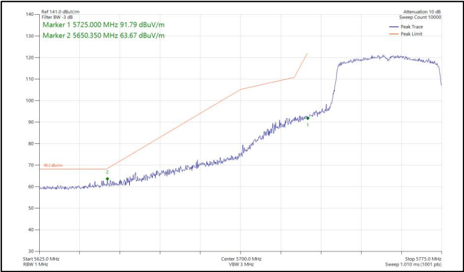
Figure 894 - 802.11ax HE40, SU, SISO, Core 0 - 5755 MHz Band Edge Frequency 5725 MHz
