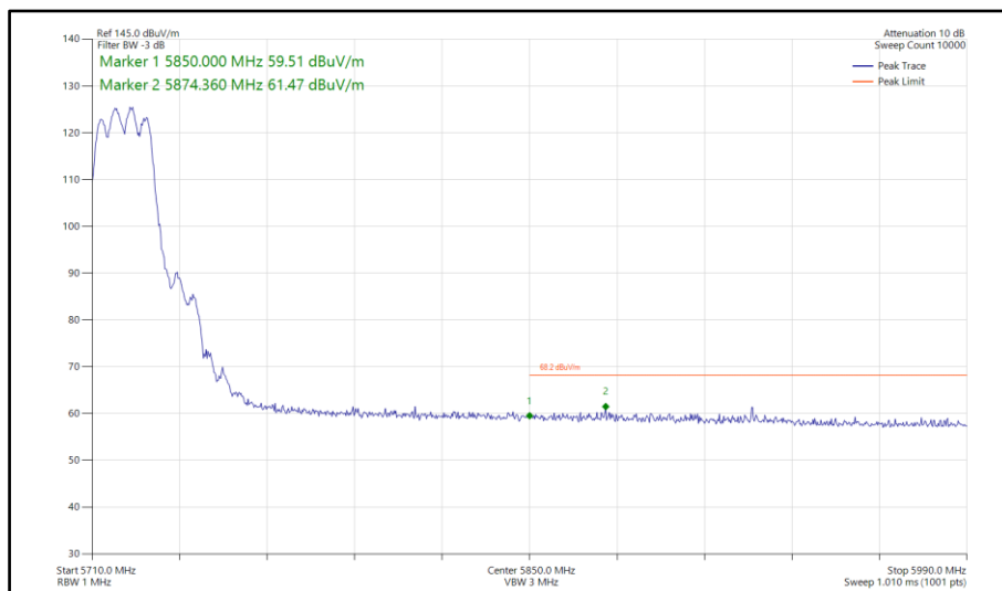
Figure 822 - 802.11n HT20, CDD, Core 0-1 - 5720 MHz Band Edge Frequency 5850 MHz
