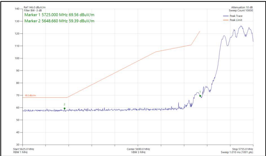
Figure 843 - 802.11be EHT20, RU 106+26-83, SDM, Core 0-1 - 5745 MHz Band Edge Frequency 5725 MHz
