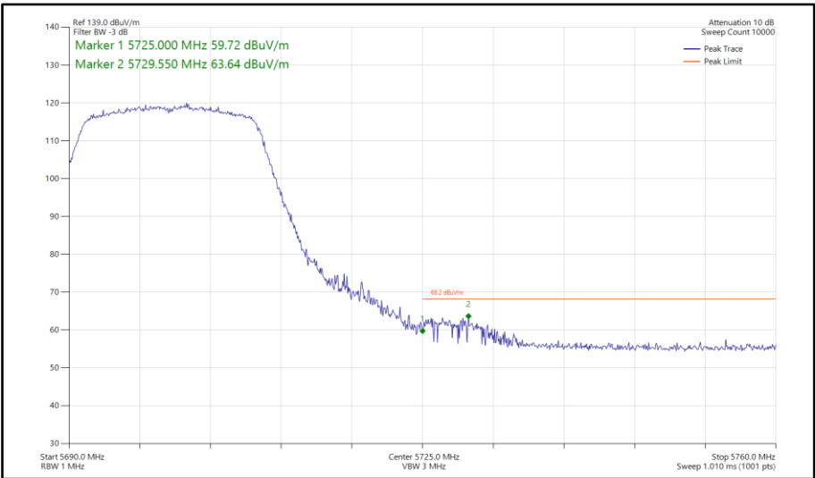
Figure 873 - 802.11ac VHT20, TxBF, Core 0-1 - 5700 MHz Band Edge Frequency 5725 MHz
