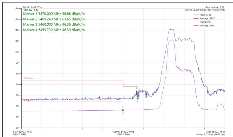
Figure 887 - 802.11ax HE40, RU 52-37, SISO, Core 0 - 5510 MHz Band Edge Frequency 5470 MHz
