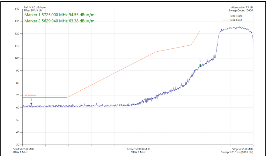
Figure 841 - 802.11ax HE20, SU, SDM, Core 0-1 - 5745 MHz Band Edge Frequency 5725 MHz
