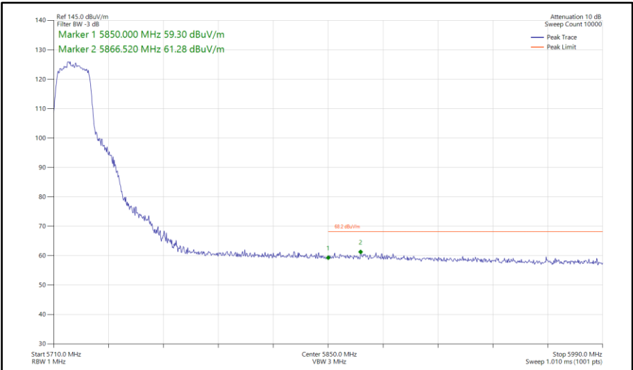
Figure 855 - 802.11n HT20, SDM, Core 0-1 - 5720 MHz Band Edge Frequency 5850 MHz
