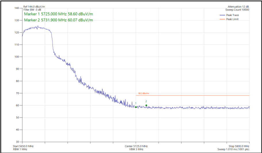
Figure 874 - 802.11ax HE20, SU, TxBF, Core 0-1 - 5660 MHz Band Edge Frequency 5725 MHz
