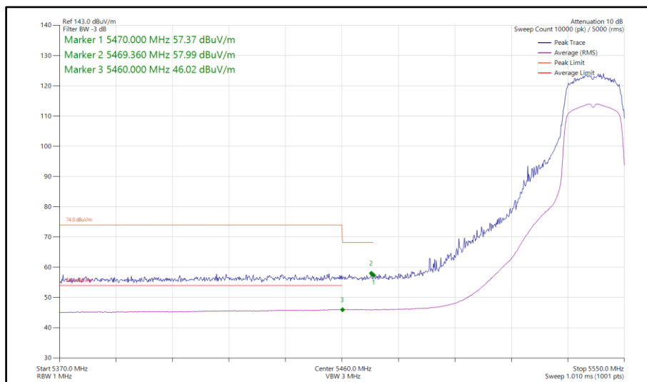
Figure 865 - 802.11ac VHT20, TxBF, Core 0-1 - 5540 MHz Band Edge Frequency 5470 MHz
