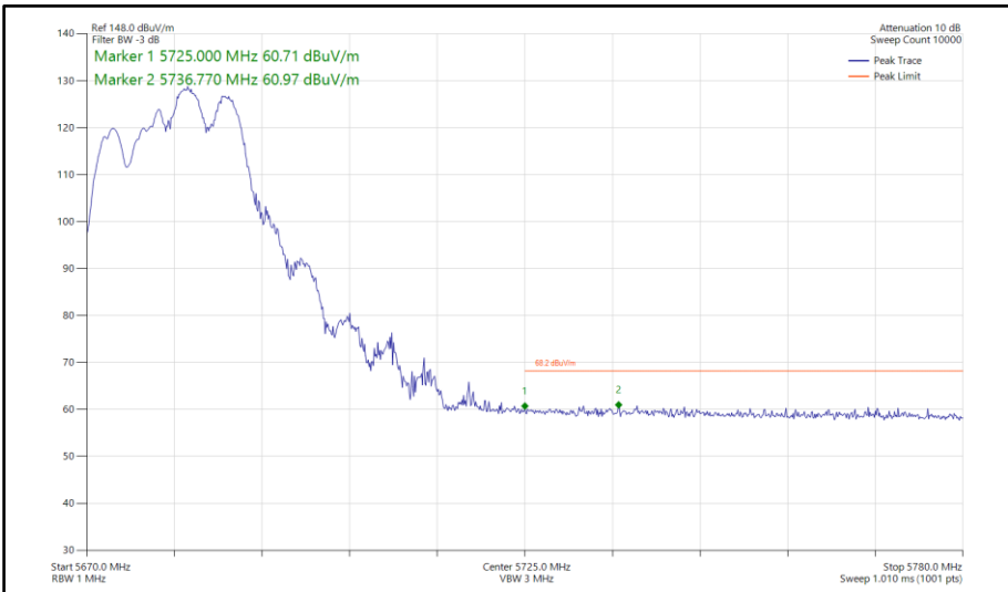
Figure 853 - 802.11be EHT20, RU 160+26-83, SDM, Core 0-1 - 5680 MHz Band Edge Frequency 5725 MHz
