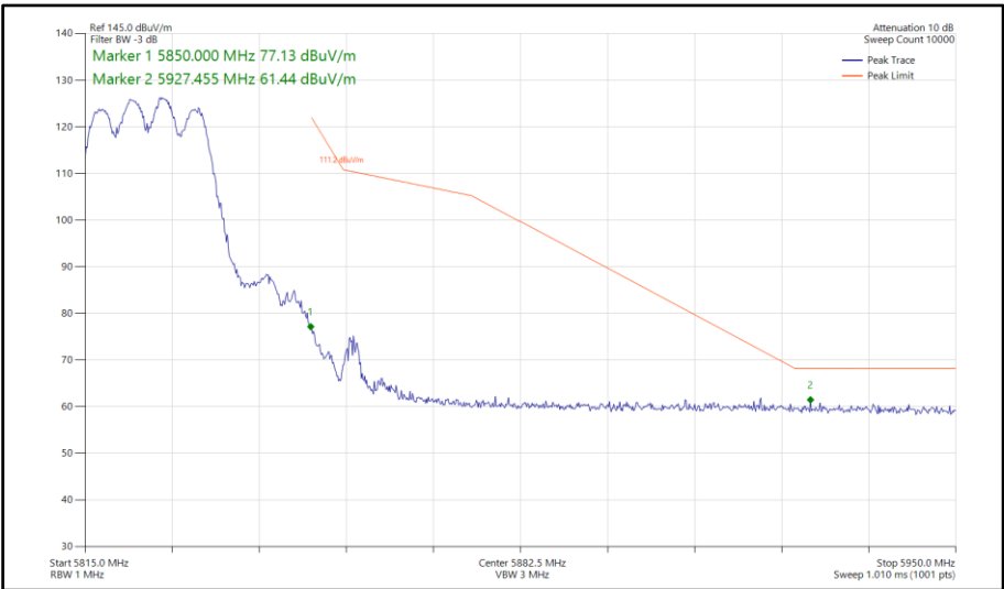
Figure 826 - 802.11ax HE20, SU, CDD, Core 0-1 - 5825 MHz Band Edge Frequency 5850 MHz
