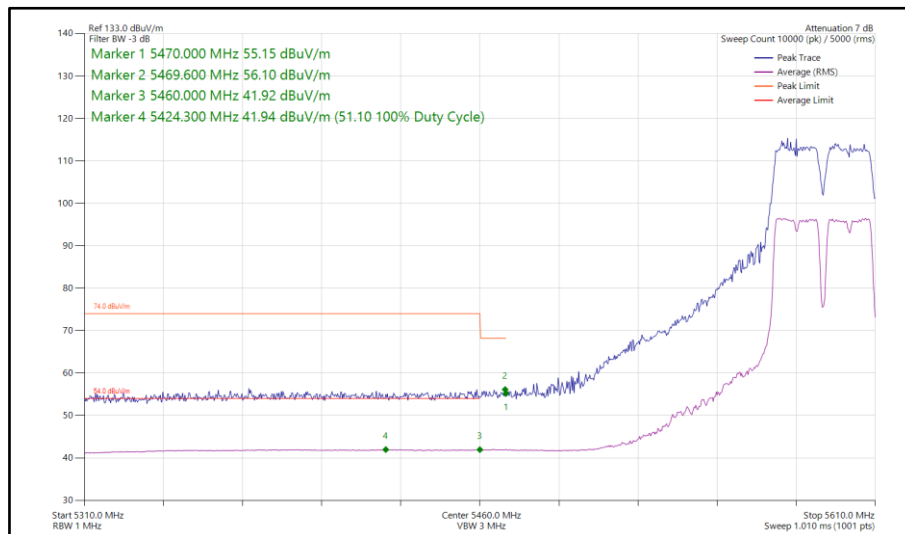
Figure 883 - 802.11a, SISO, Core 0 - 5590 MHz Band Edge Frequency 5470 MHz
