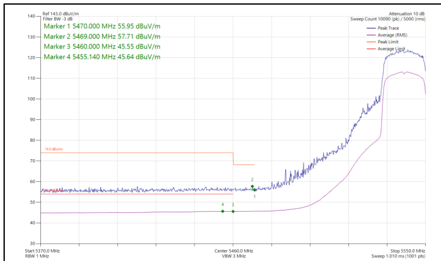
Figure 868 - 802.11ax HE20, SU, TxBF, Core 0-1 - 5540 MHz Band Edge Frequency 5470 MHz
