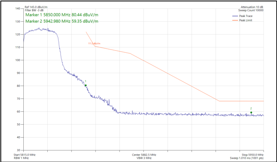
Figure 880 - 802.11ax HE20, SU, TxBF, Core 0-1 - 5825 MHz Band Edge Frequency 5850 MHz
