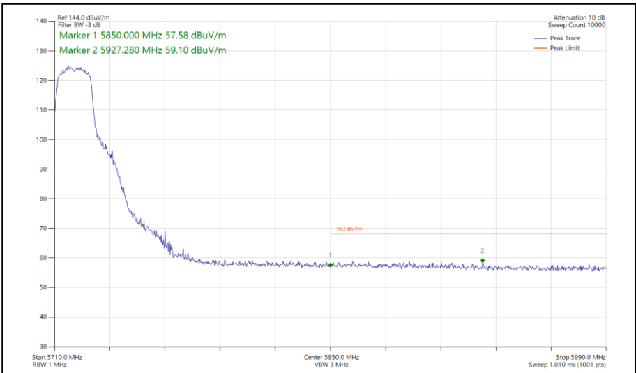
Figure 877 - 802.11ac VHT20, TxBF, Core 0-1 - 5720 MHz Band Edge Frequency 5850 MHz
