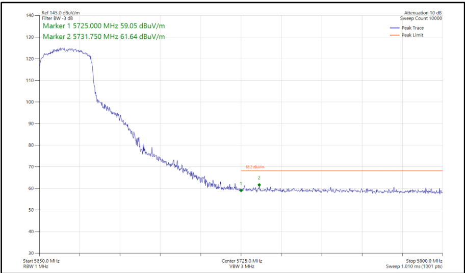
Figure 847 - 802.11ax HE20, SU, SDM, Core 0-1 - 5660 MHz Band Edge Frequency 5725 MHz
