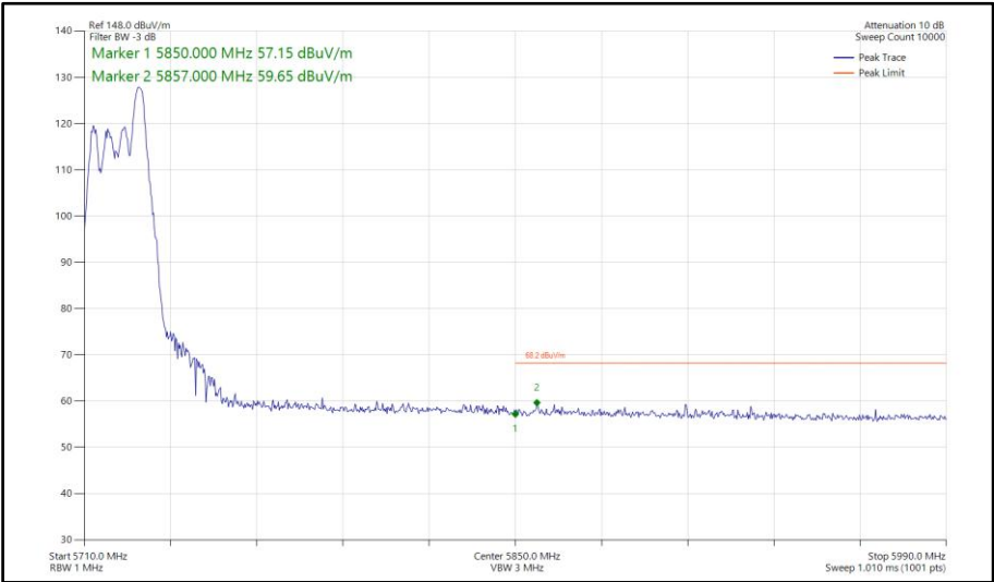
Figure 825 - 802.11ax HE20, RU 52-40, CDD, Core 0-1 - 5720 MHz Band Edge Frequency 5850 MHz
