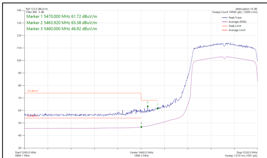
Figure 886 - 802.11ax HE40, SU, SISO, Core 0 - 5510 MHz Band Edge Frequency 5470 MHz
