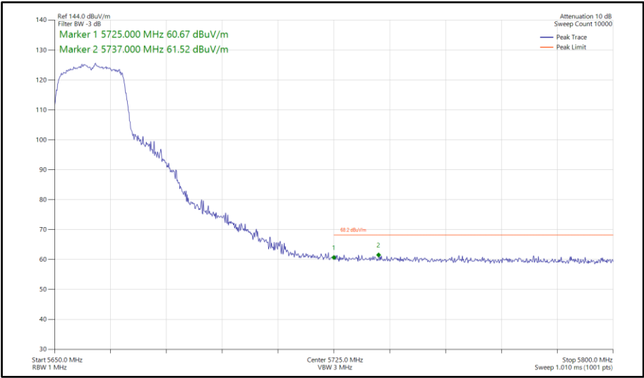
Figure 844 - 802.11n HT20, SDM, Core 0-1 - 5660 MHz Band Edge Frequency 5725 MHz
