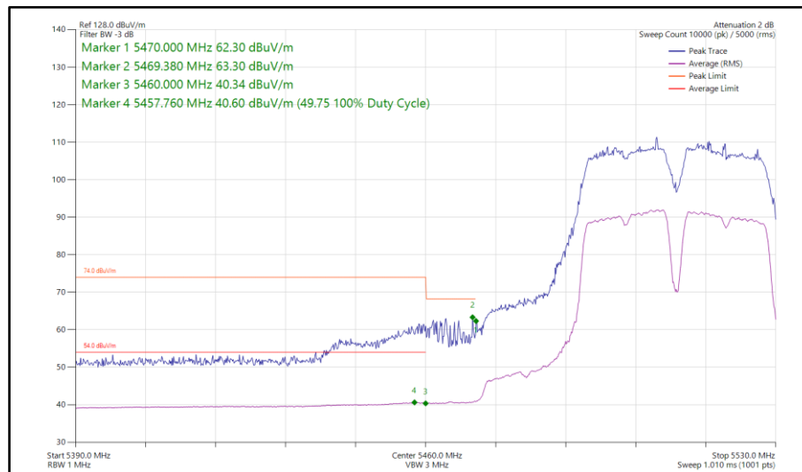
Figure 881 - 802.11a, SISO, Core 0 - 5510 MHz Band Edge Frequency 5470 MHz
