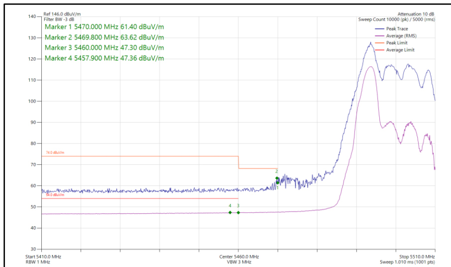
Figure 834 - 802.11ax HE20, RU 52-37, SDM, Core 0-1 - 5500 MHz Band Edge Frequency 5470 MHz
