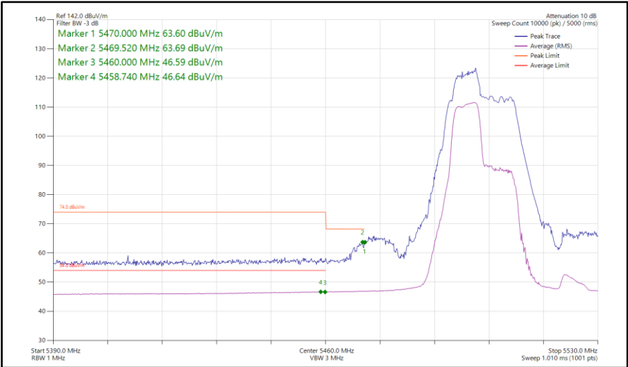
Figure 890 - 802.11be EHT40, RU 52+26-70, SISO, Core 0 - 5510 MHz Band Edge Frequency 5470 MHz
