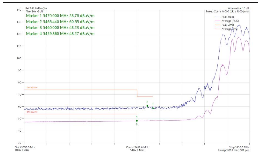
Figure 839 - 802.11be EHT20, RU 106+26-83, SDM, Core 0-1 - 5520 MHz Band Edge Frequency 5470 MHz
