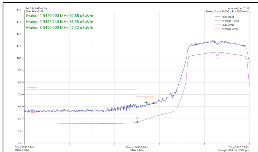
Figure 884 - 802.11n HT40, SISO, Core 0 - 5510 MHz Band Edge Frequency 5470 MHz
