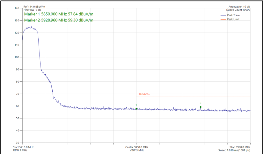
Figure 879 - 802.11ax HE20, SU, TxBF, Core 0-1 - 5720 MHz Band Edge Frequency 5850 MHz
