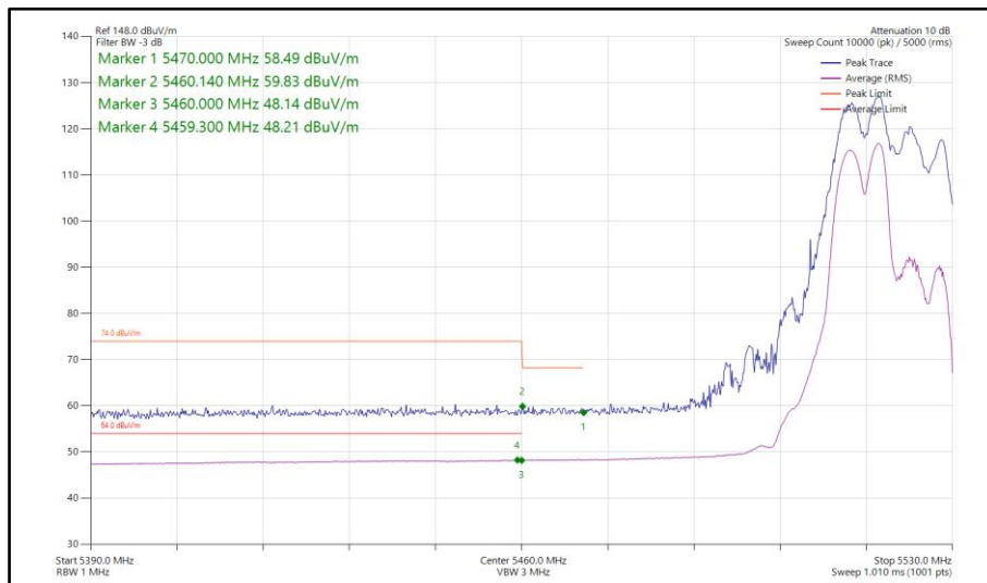
Figure 836 - 802.11ax HE20, RU 106-53, SDM, Core 0-1 - 5520 MHz Band Edge Frequency 5470 MHz
