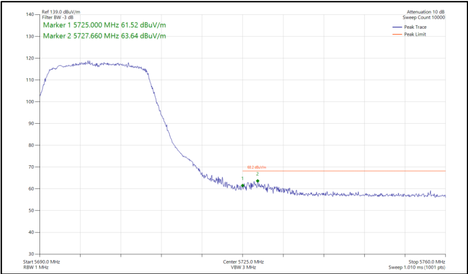
Figure 846 - 802.11n HT20, SDM, Core 0-1 - 5700 MHz Band Edge Frequency 5725 MHz
