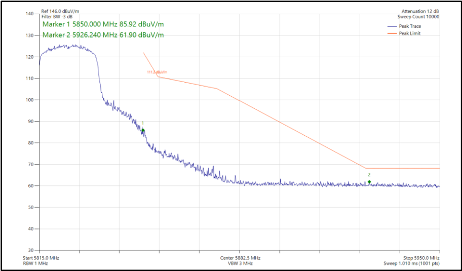
Figure 859 - 802.11ax HE20, SU, SDM, Core 0-1 - 5825 MHz Band Edge Frequency 5850 MHz
