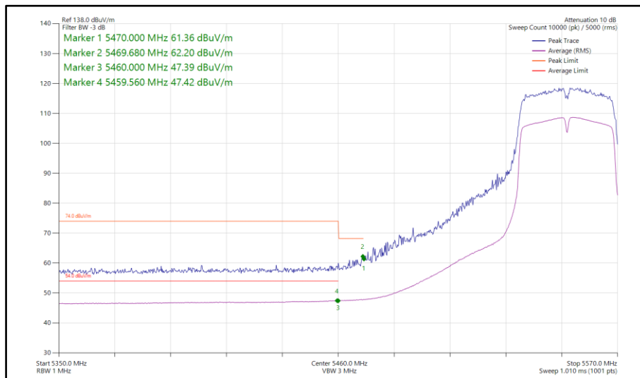
Figure 885 - 802.11n HT40, SISO, Core 0 - 5550 MHz Band Edge Frequency 5470 MHz
