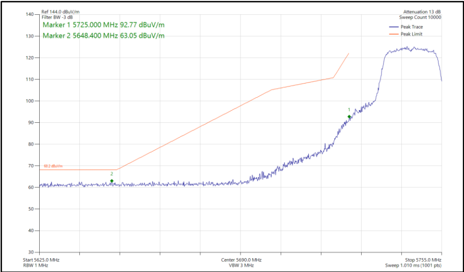
Figure 840 - 802.11n HT20, SDM, Core 0-1 - 5745 MHz Band Edge Frequency 5725 MHz
