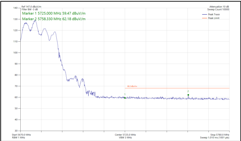
Figure 849 - 802.11ax HE20, RU 106-53, SDM, Core 0-1 - 5680 MHz Band Edge Frequency 5725 MHz
