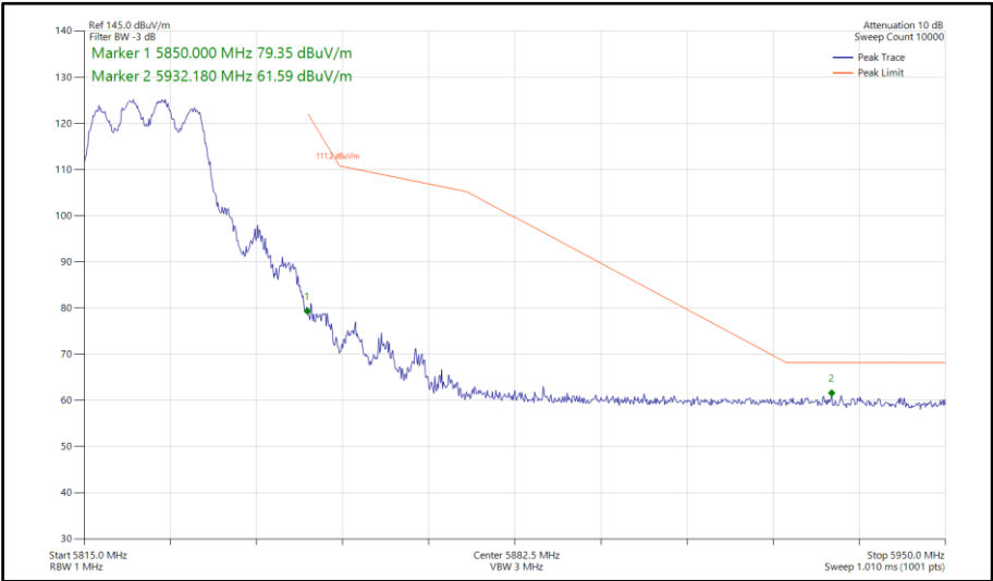
Figure 823 - 802.11n HT20, CDD, Core 0-1 - 5825 MHz Band Edge Frequency 5850 MHz
