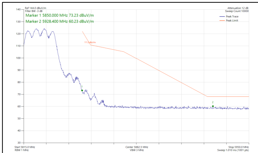
Figure 821 - 802.11a, CDD, Core 0-1 - 5825 MHz Band Edge Frequency 5850 MHz
