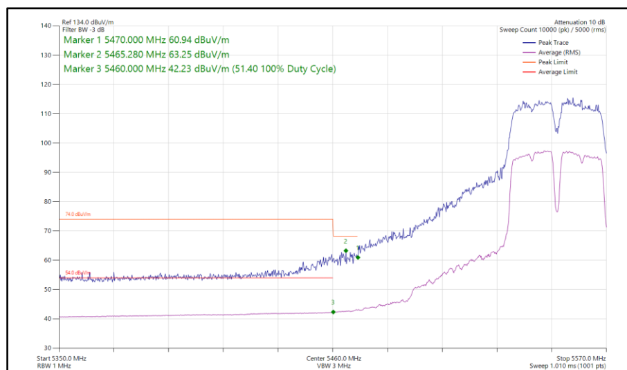
Figure 882 - 802.11a, SISO, Core 0 - 5550 MHz Band Edge Frequency 5470 MHz
