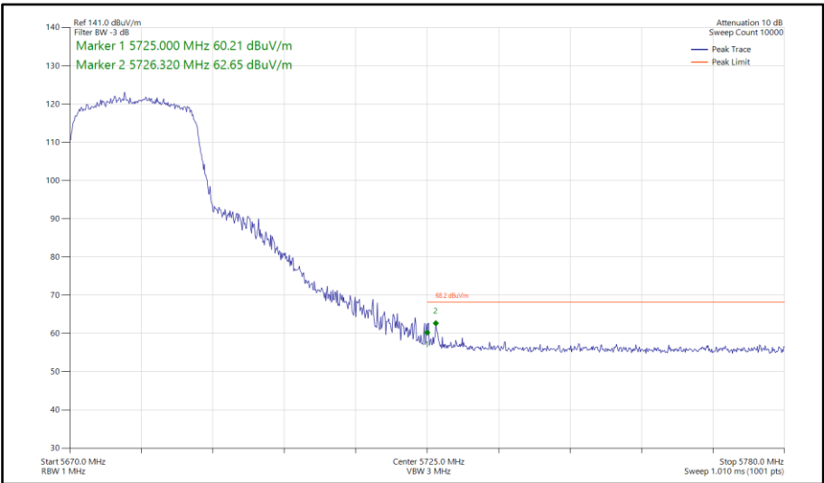
Figure 875 - 802.11ax HE20, SU, TxBF, Core 0-1 - 5680 MHz Band Edge Frequency 5725 MHz
