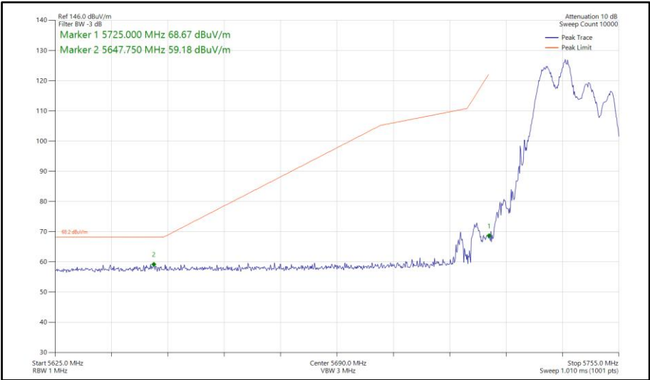
Figure 842 - 802.11ax HE20, RU 106-53, SDM, Core 0-1 - 5745 MHz Band Edge Frequency 5725 MHz
