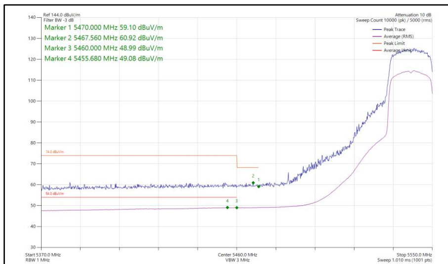
Figure 837 - 802.11ax HE20, SU, SDM, Core 0-1 - 5540 MHz Band Edge Frequency 5470 MHz
