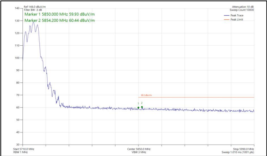
Figure 861 - 802.11be EHT20, RU 106+26-83, SDM, Core 0-1 - 5720 MHz Band Edge Frequency 5850 MHz
