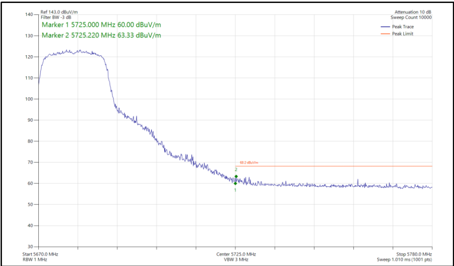
Figure 845 - 802.11n HT20, SDM, Core 0-1 - 5680 MHz Band Edge Frequency 5725 MHz
