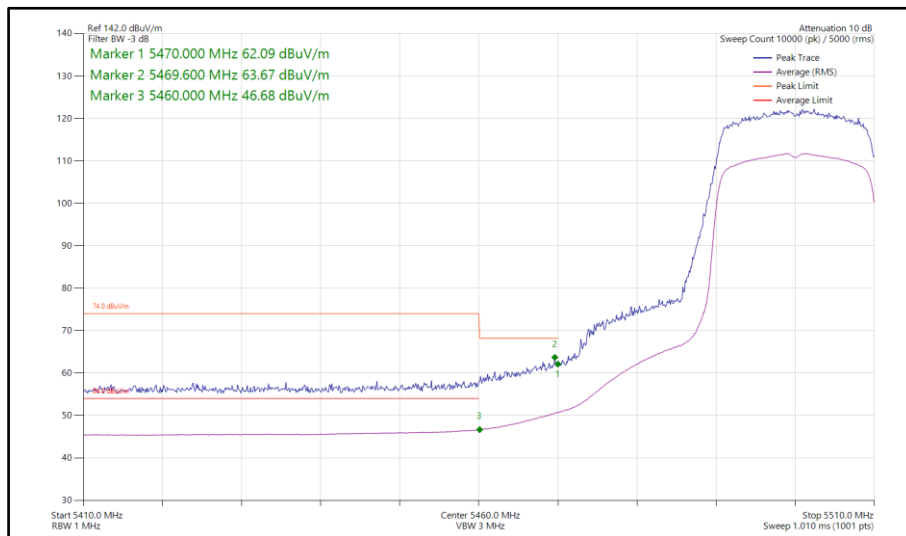
Figure 866 - 802.11ax HE20, SU, TxBF, Core 0-1 - 5500 MHz Band Edge Frequency 5470 MHz
