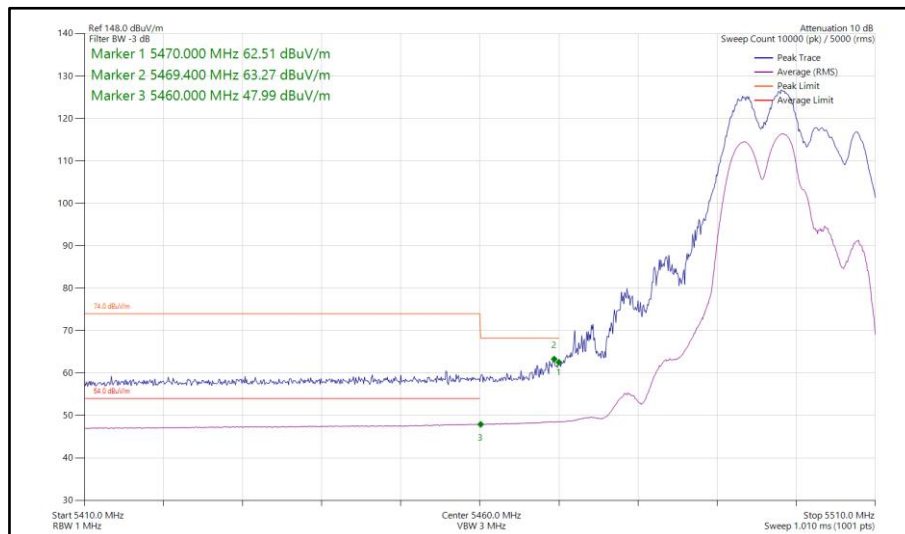
Figure 838 - 802.11be EHT20, RU 106+26-83, SDM, Core 0-1 - 5500 MHz Band Edge Frequency 5470 MHz
