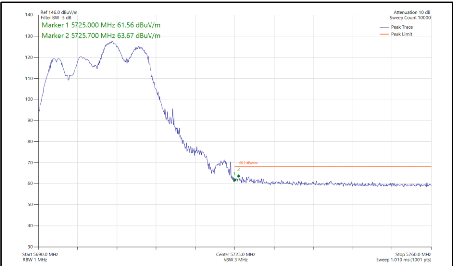
Figure 851 - 802.11ax HE20, RU 106-54, SDM, Core 0-1 - 5700 MHz Band Edge Frequency 5725 MHz
