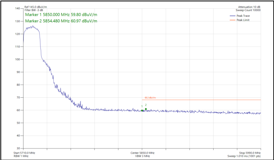
Figure 856 - 802.11ax HE20, SU, SDM, Core 0-1 - 5720 MHz Band Edge Frequency 5850 MHz
