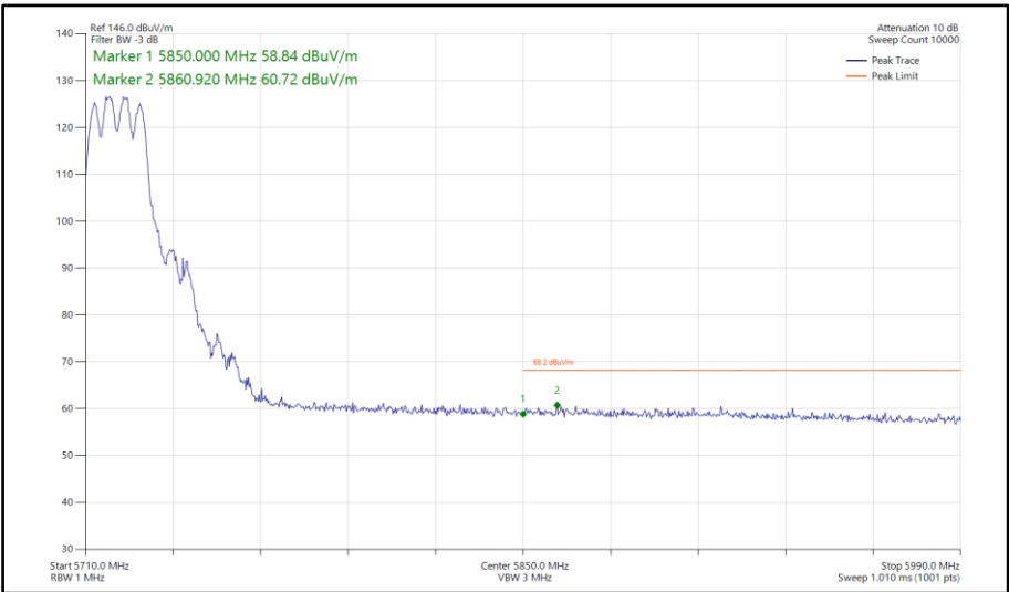
Figure 824 - 802.11ax HE20, SU, CDD, Core 0-1 - 5720 MHz Band Edge Frequency 5850 MHz
