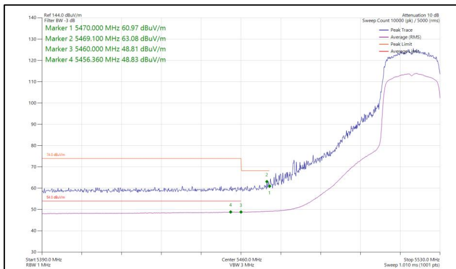
Figure 835 - 802.11ax HE20, SU, SDM, Core 0-1 - 5520 MHz Band Edge Frequency 5470 MHz
