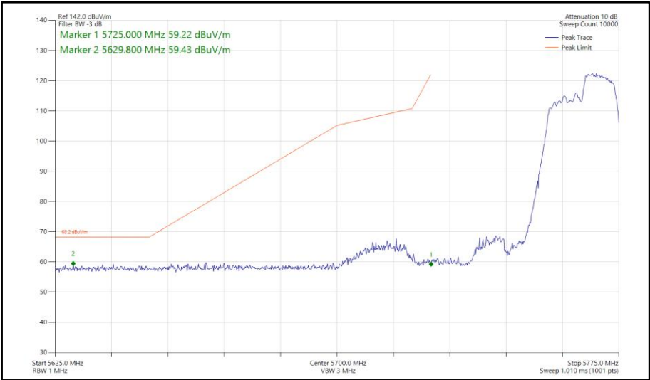
Figure 895 - 802.11ax HE40, RU 106-56, SISO, Core 0 - 5755 MHz Band Edge Frequency 5725 MHz
