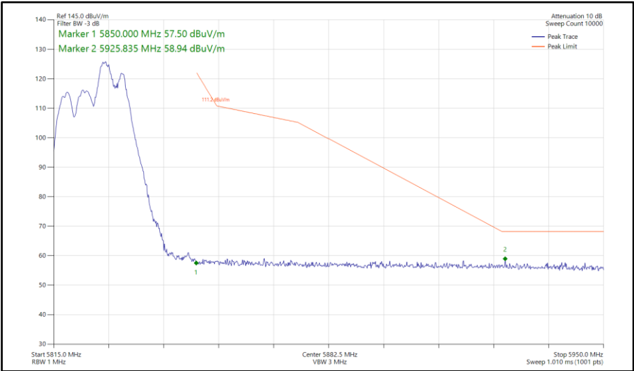
Figure 862 - 802.11be EHT20, RU 52+26-72, SDM, Core 0-1 - 5825 MHz Band Edge Frequency 5850 MHz
