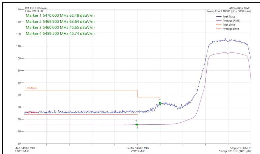
Figure 830 - 802.11n HT20, SDM, Core 0-1 - 5500 MHz Band Edge Frequency 5470 MHz
