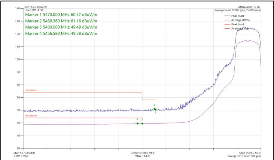
Figure 832 - 802.11n HT20, SDM, Core 0-1 - 5540 MHz Band Edge Frequency 5470 MHz
