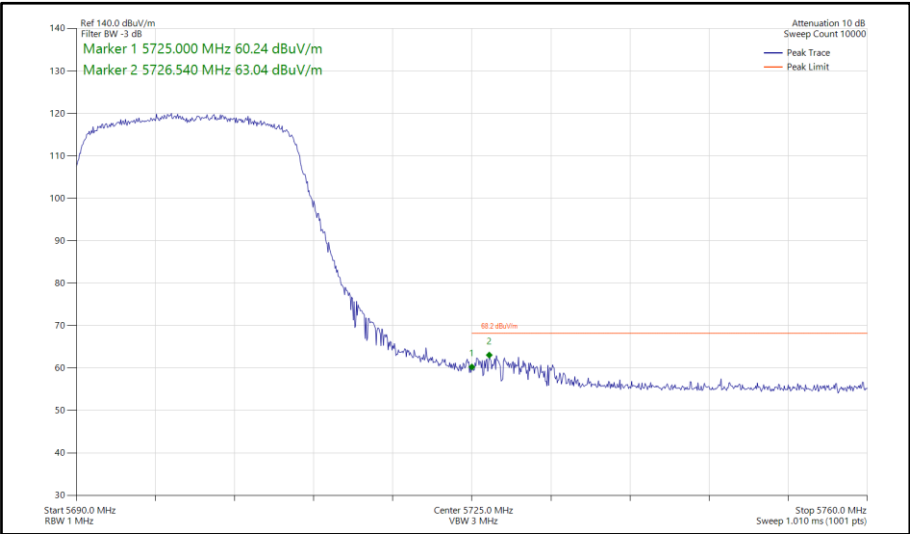
Figure 876 - 802.11ax HE20, SU, TxBF, Core 0-1 - 5700 MHz Band Edge Frequency 5725 MHz
