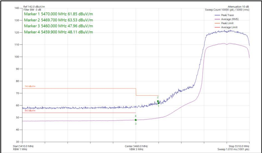
Figure 833 - 802.11ax HE20, SU, SDM, Core 0-1 - 5500 MHz Band Edge Frequency 5470 MHz
