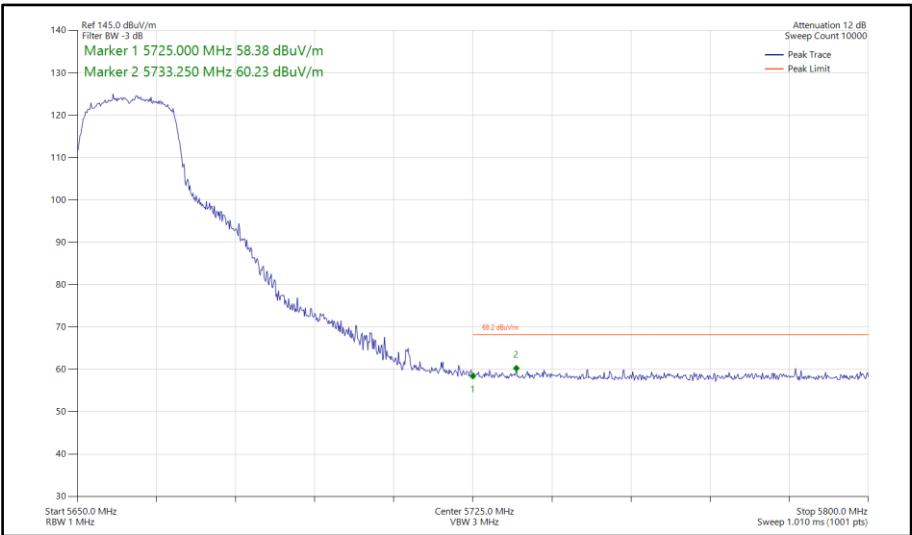
Figure 871 - 802.11ac VHT20, TxBF, Core 0-1 - 5660 MHz Band Edge Frequency 5725 MHz
