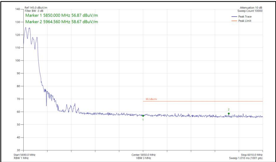
Figure 986 - 802.11ax HE40, RU 106-53, CDD, Core 0-1 - 5710 MHz Band Edge Frequency 5850 MHz
