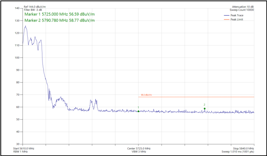
Figure 1006 - 802.11ax HE40, RU 52-37, SDM, Core 0-1 - 5630 MHz Band Edge Frequency 5725 MHz
