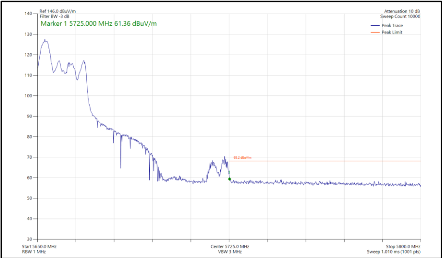
Figure 978 - 802.11ax HE40, RU 52-37, CDD, Core 0-1 - 5670 MHz Band Edge Frequency 5725 MHz
