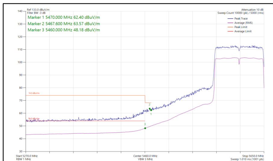
Figure 1036 - 802.11ac VHT80, SISO, Core 0 - 5610 MHz Band Edge Frequency 5470 MHz
