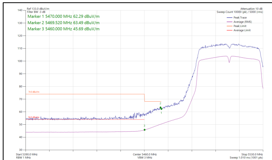
Figure 1019 - 802.11ac VHT40, TxBF, Core 0-1 - 5510 MHz Band Edge Frequency 5470 MHz
