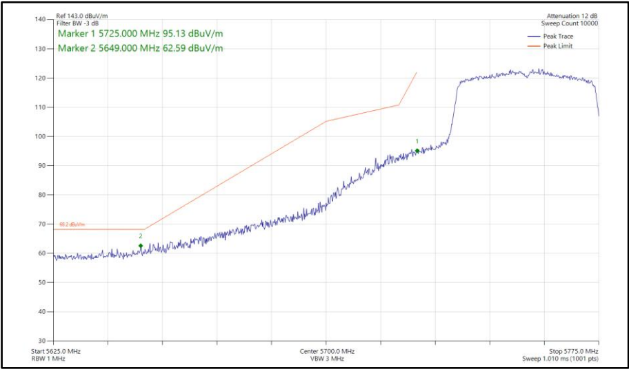
Figure 1024 - 802.11ax HE40, SU, TxBF, Core 0-1 - 5755 MHz Band Edge Frequency 5725 MHz
