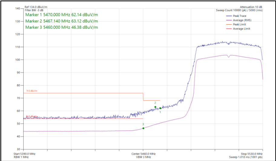
Figure 1021 - 802.11ax HE40, SU, TxBF, Core 0-1 - 5510 MHz Band Edge Frequency 5470 MHz
