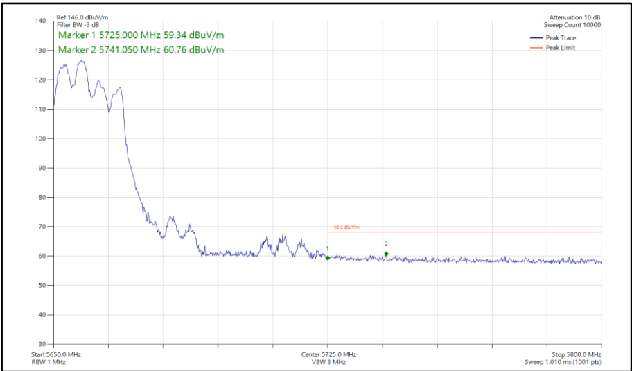
Figure 1008 - 802.11ax HE40, RU 106-53, SDM, Core 0-1 - 5670 MHz Band Edge Frequency 5725 MHz
