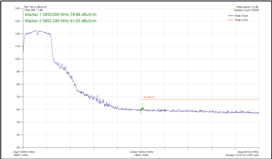
Figure 1011 - 802.11n HT40, SDM, Core 0-1 - 5710 MHz Band Edge Frequency 5850 MHz
