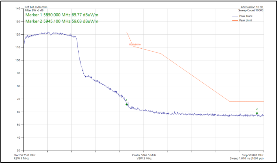
Figure 1032 - 802.11ax HE40, SU, TxBF, Core 0-1 - 5795 MHz Band Edge Frequency 5850 MHz
