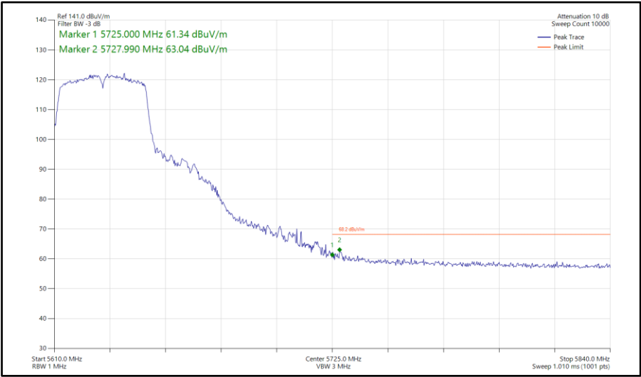
Figure 1003 - 802.11n HT40, SDM, Core 0-1 - 5630 MHz Band Edge Frequency 5725 MHz
