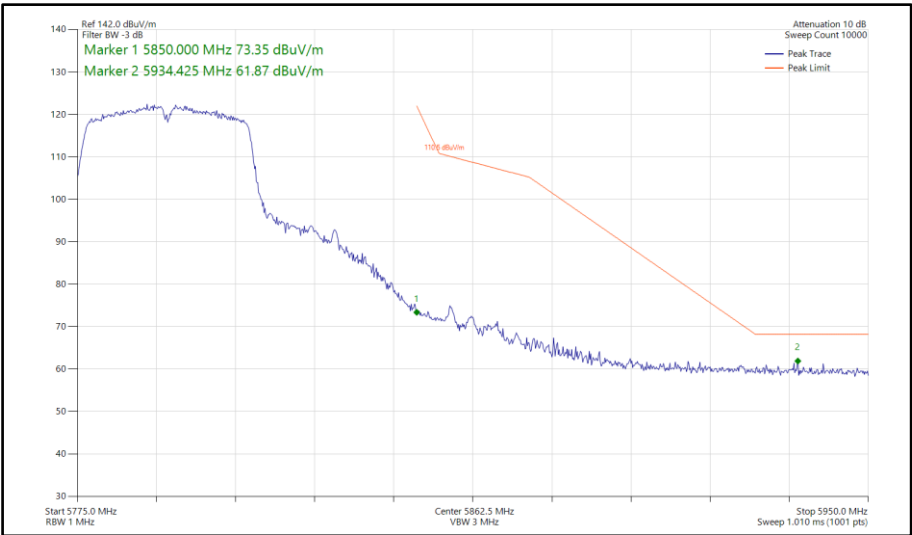
Figure 1012 - 802.11n HT40, SDM, Core 0-1 - 5795 MHz Band Edge Frequency 5850 MHz
