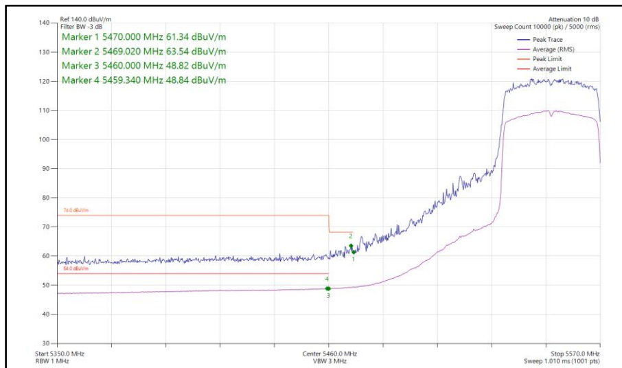
Figure 995 - 802.11ax HE40, SU, SDM, Core 0-1 - 5550 MHz Band Edge Frequency 5470 MHz
