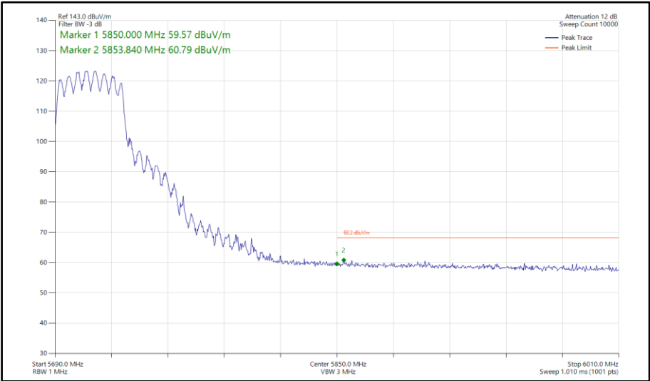
Figure 983 - 802.11n HT40, CDD, Core 0-1 - 5710 MHz Band Edge Frequency 5850 MHz
