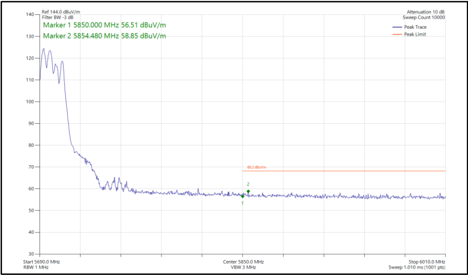
Figure 989 - 802.11be EHT40, RU 106+26-82, CDD, Core 0-1 - 5710 MHz Band Edge Frequency 5850 MHz
