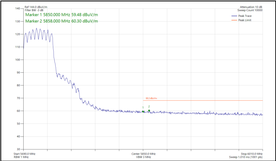
Figure 985 - 802.11ax HE40, SU, CDD, Core 0-1 - 5710 MHz Band Edge Frequency 5850 MHz
