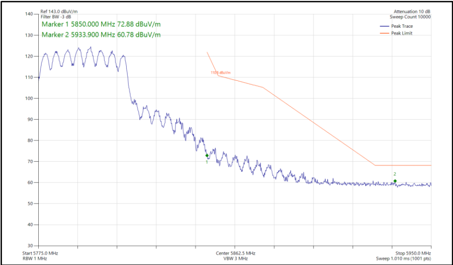
Figure 987 - 802.11ax HE40, SU, CDD, Core 0-1 - 5795 MHz Band Edge Frequency 5850 MHz
