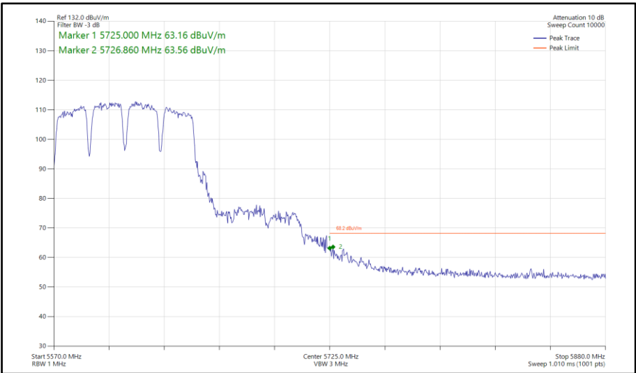
Figure 1048 - 802.11a, SISO, Core 0 - 5610 MHz Band Edge Frequency 5725 MHz
