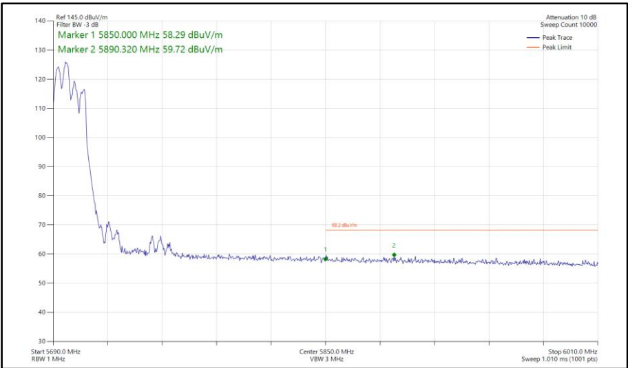
Figure 1014 - 802.11ax HE40, RU 106-53, SDM, Core 0-1 - 5710 MHz Band Edge Frequency 5850 MHz
