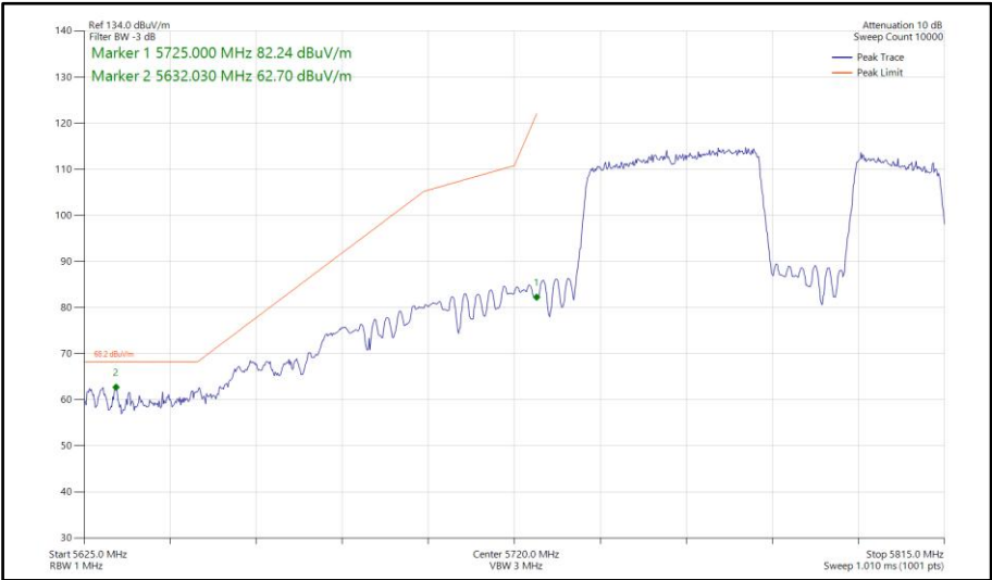
Figure 1047 - 802.11be EHT80, RU 484+242-92, SISO, Core 0 - 5775 MHz Band Edge Frequency 5725 MHz
