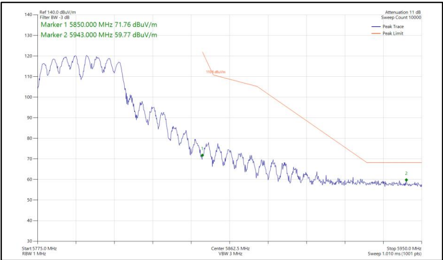
Figure 982 - 802.11a, CDD, Core 0-1 - 5795 MHz Band Edge Frequency 5850 MHz
