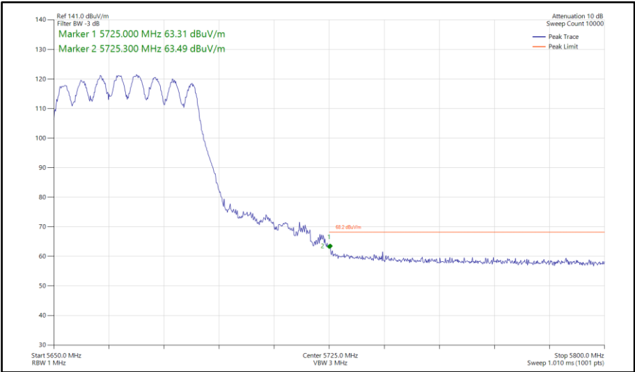
Figure 977 - 802.11ax HE40, SU, CDD, Core 0-1 - 5670 MHz Band Edge Frequency 5725 MHz
