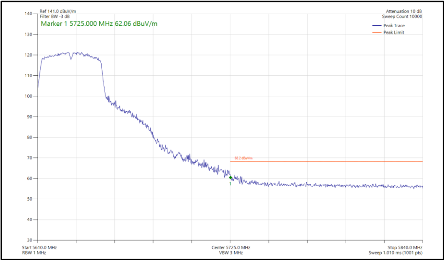
Figure 1025 - 802.11ac VHT40, TxBF, Core 0-1 - 5630 MHz Band Edge Frequency 5725 MHz
