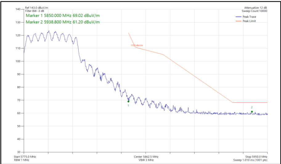
Figure 984 - 802.11n HT40, CDD, Core 0-1 - 5795 MHz Band Edge Frequency 5850 MHz
