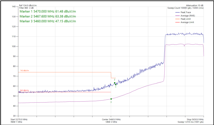
Figure 1039 - 802.11ax HE80, SU, SISO, Core 0 - 5610 MHz Band Edge Frequency 5470 MHz
