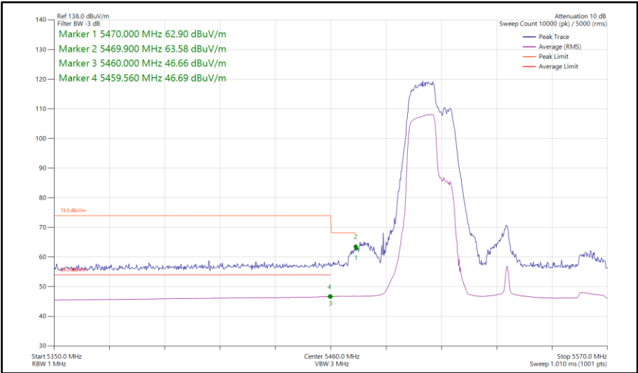
Figure 1041 - 802.11be EHT80, RU 106+26-82, SISO, Core 0 - 5530 MHz Band Edge Frequency 5470 MHz
