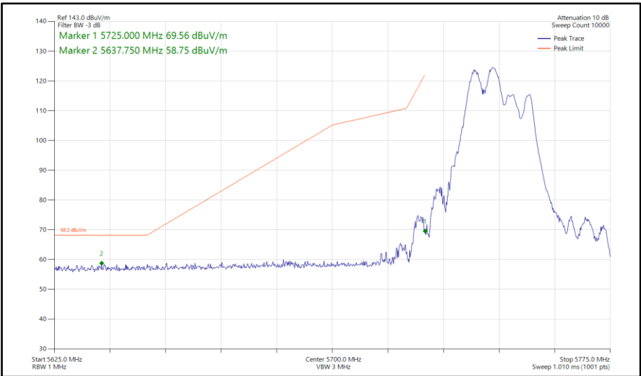
Figure 1002 - 802.11be EHT40, SDM, Core 0-1 - 5755 MHz Band Edge Frequency 5725 MHz
