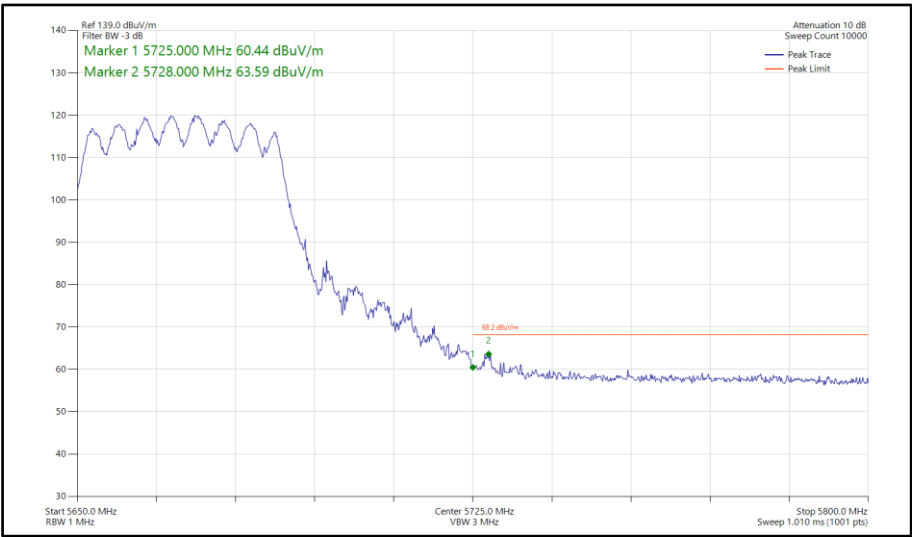
Figure 974 - 802.11n HT40, CDD, Core 0-1 - 5670 MHz Band Edge Frequency 5725 MHz
