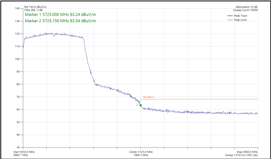
Figure 1028 - 802.11ax HE40, SU, TxBF, Core 0-1 - 5670 MHz Band Edge Frequency 5725 MHz
