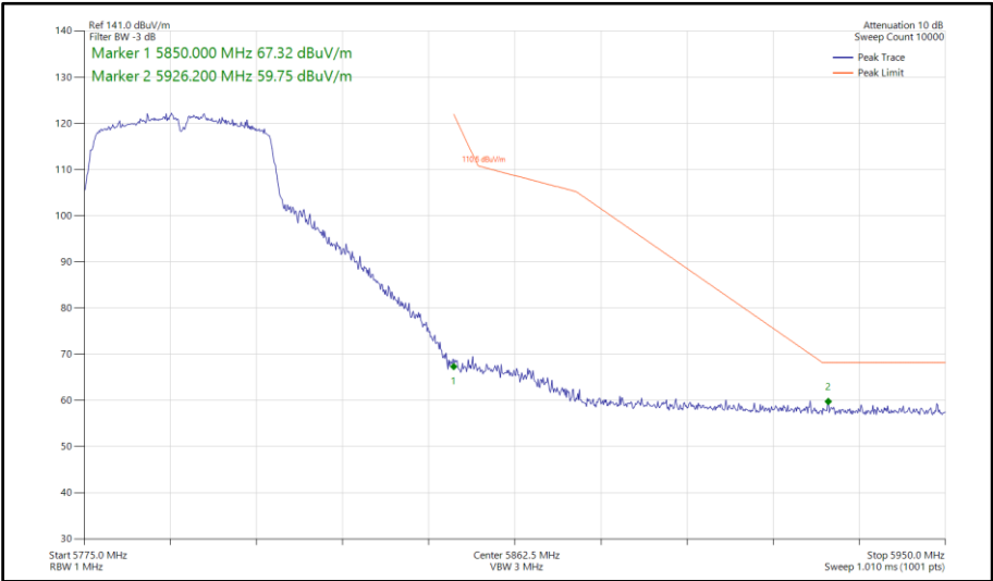
Figure 1030 - 802.11ac VHT40, TxBF, Core 0-1 - 5795 MHz Band Edge Frequency 5850 MHz
