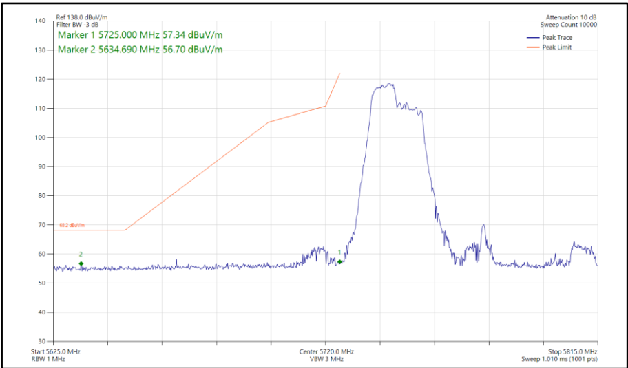
Figure 1046 - 802.11ax HE80, RU 106-53, SISO, Core 0 - 5775 MHz Band Edge Frequency 5725 MHz
