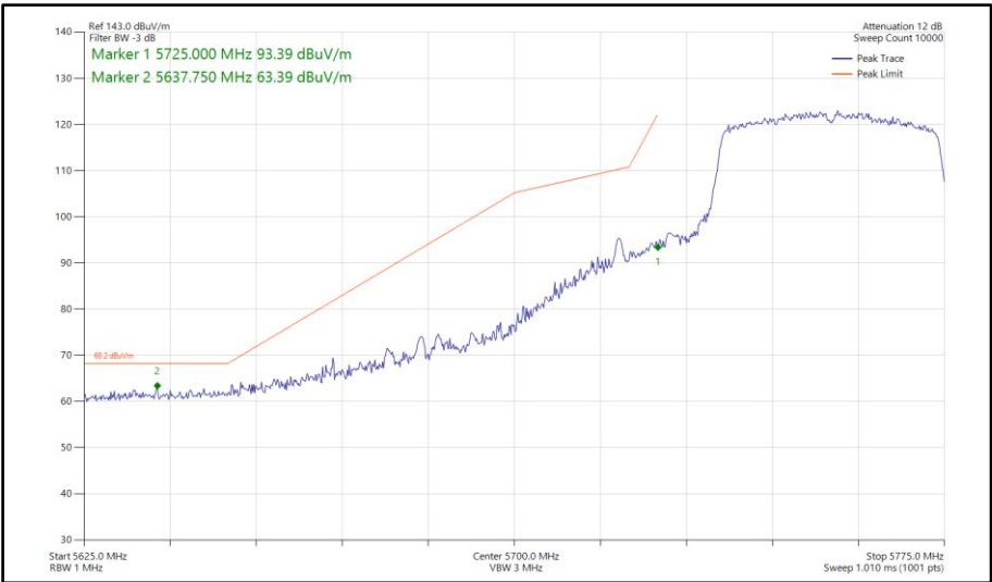
Figure 1000 - 802.11ax HE40, SU, SDM, Core 0-1 - 5755 MHz Band Edge Frequency 5725 MHz
