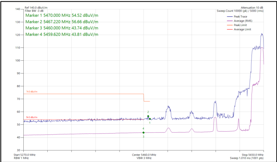
Figure 1040 - 802.11ax HE80, RU 52-52, SISO, Core 0 - 5610 MHz Band Edge Frequency 5470 MHz
