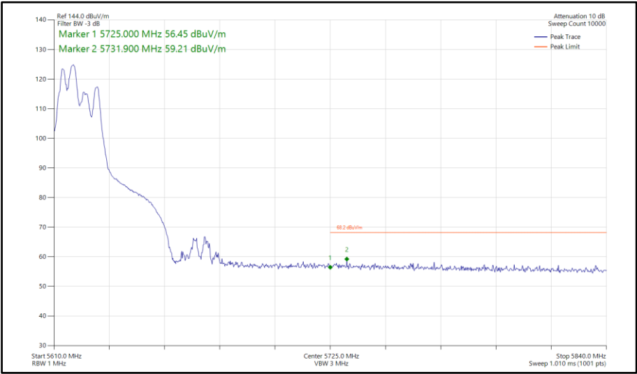
Figure 979 - 802.11be EHT40, RU 52+26-70, CDD, Core 0-1 - 5630 MHz Band Edge Frequency 5725 MHz
