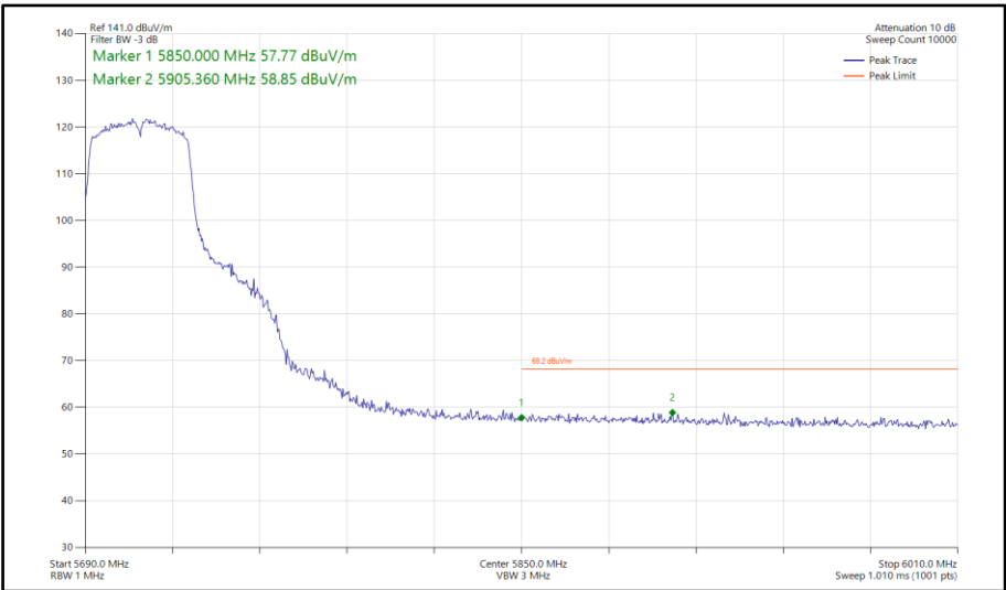
Figure 1029 - 802.11ac VHT40, TxBF, Core 0-1 - 5710 MHz Band Edge Frequency 5850 MHz
