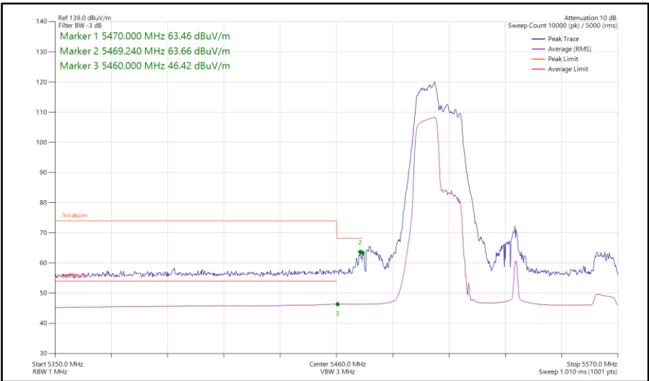
Figure 1038 - 802.11ax HE80, RU 106-53, SISO, Core 0 - 5530 MHz Band Edge Frequency 5470 MHz
