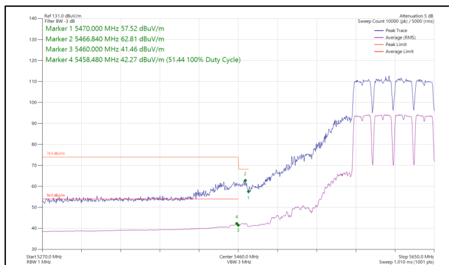
Figure 1034 - 802.11a, SISO, Core 0 - 5610 MHz Band Edge Frequency 5470 MHz
