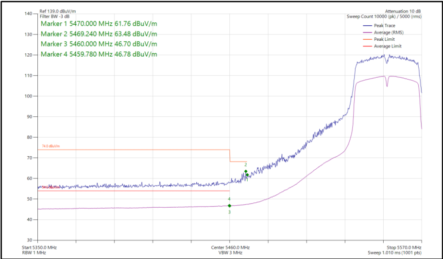
Figure 1020 - 802.11ac VHT40, TxBF, Core 0-1 - 5550 MHz Band Edge Frequency 5470 MHz
