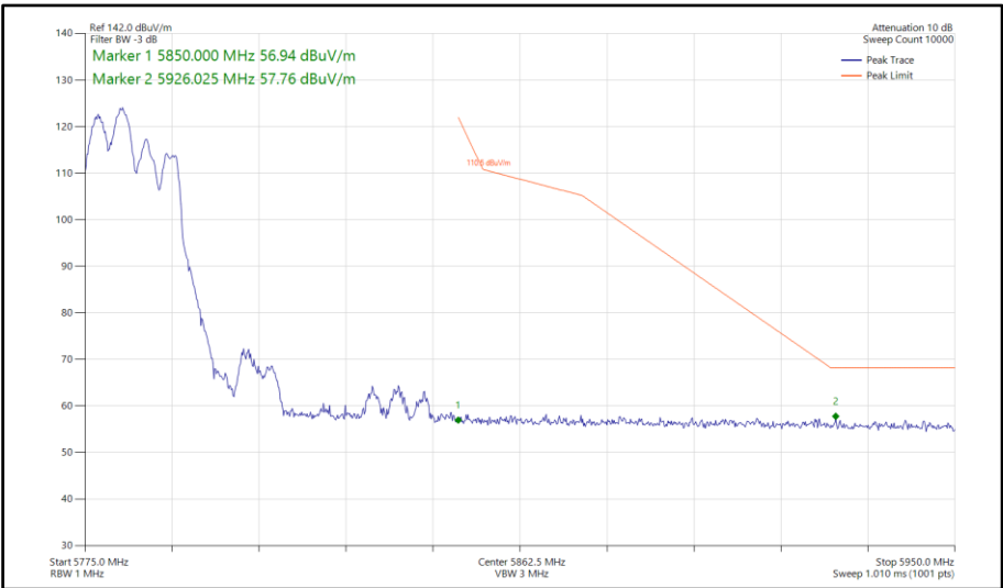
Figure 1016 - 802.11ax HE40, RU 106-53, SDM, Core 0-1 - 5795 MHz Band Edge Frequency 5850 MHz
