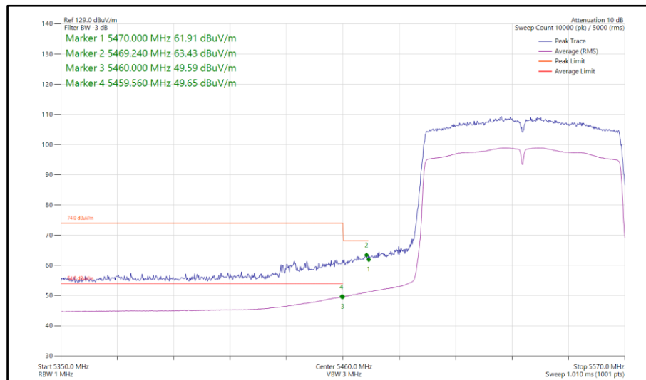
Figure 1035 - 802.11ac VHT80, SISO, Core 0 - 5530 MHz Band Edge Frequency 5470 MHz
