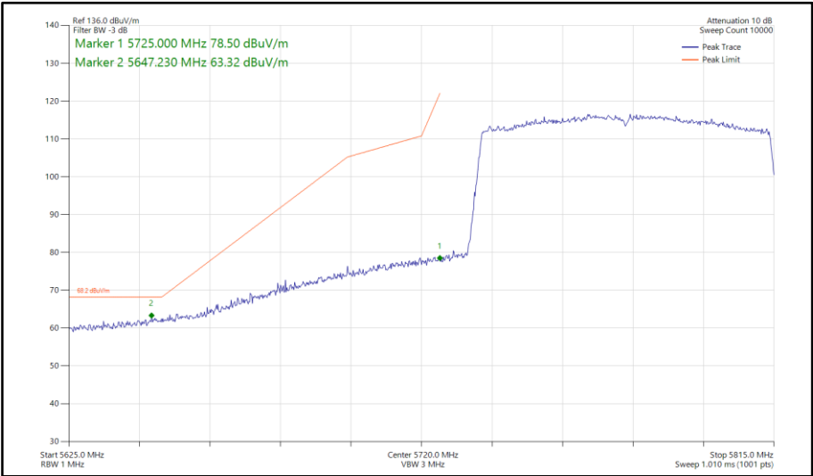
Figure 1045 - 802.11ax HE80, SU, SISO, Core 0 - 5775 MHz Band Edge Frequency 5725 MHz
