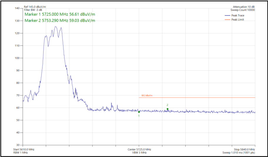
Figure 1009 - 802.11be EHT40, RU 106+26-85, SDM, Core 0-1 - 5630 MHz Band Edge Frequency 5725 MHz
