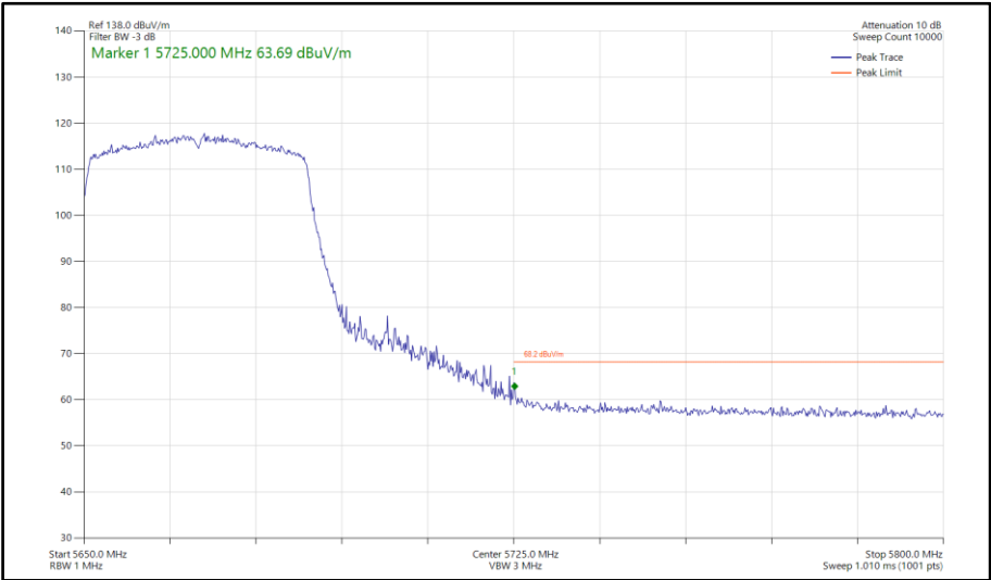
Figure 1007 - 802.11ax HE40, SU, SDM, Core 0-1 - 5670 MHz Band Edge Frequency 5725 MHz
