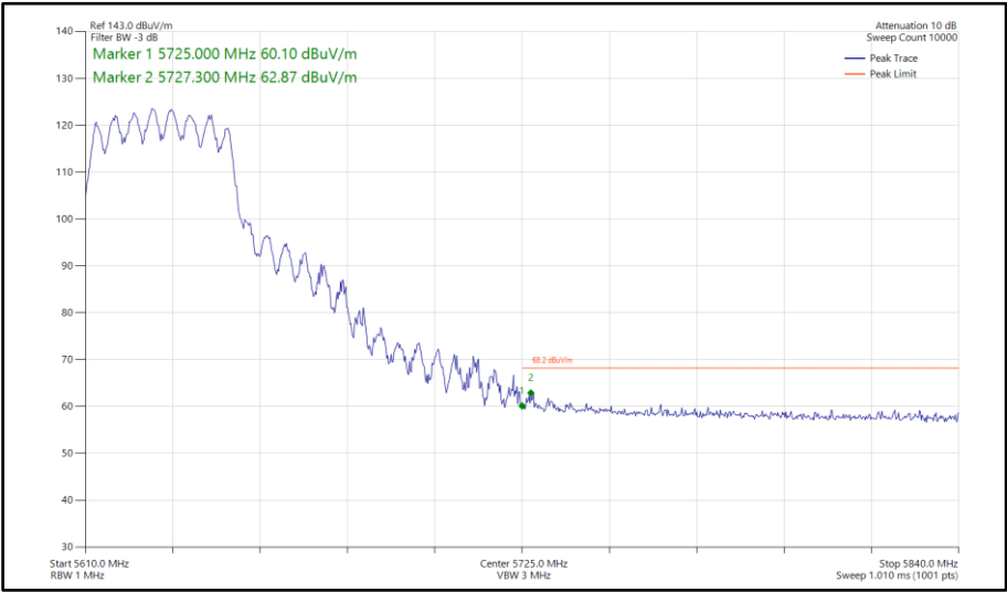
Figure 973 - 802.11n HT40, CDD, Core 0-1 - 5630 MHz Band Edge Frequency 5725 MHz
