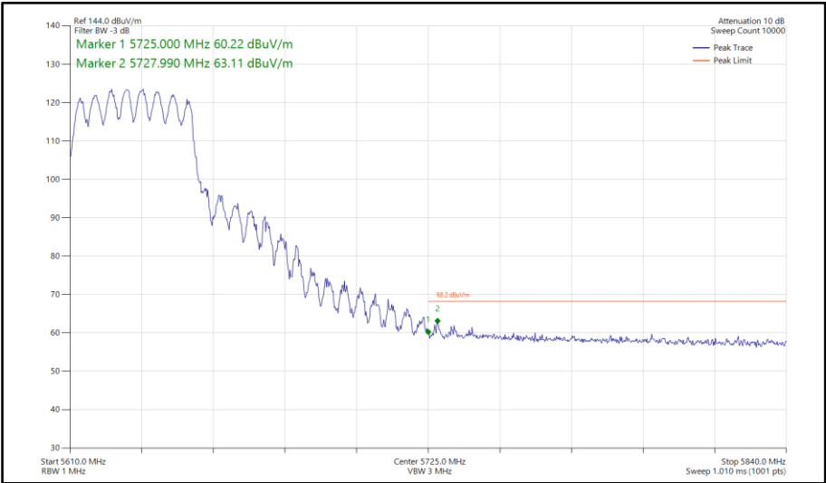
Figure 975 - 802.11ax HE40, SU, CDD, Core 0-1 - 5630 MHz Band Edge Frequency 5725 MHz
