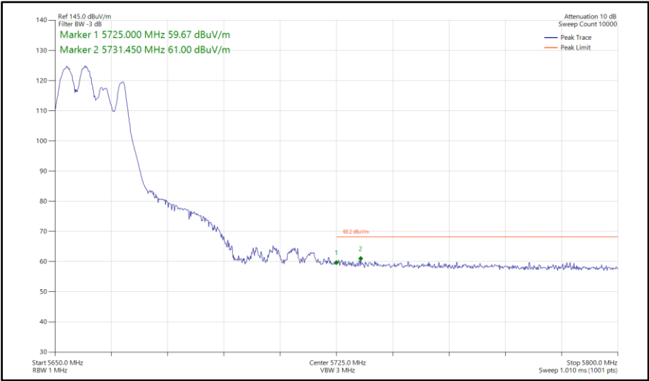
Figure 980 - 802.11be EHT40, RU 106+26-82, CDD, Core 0-1 - 5670 MHz Band Edge Frequency 5725 MHz
