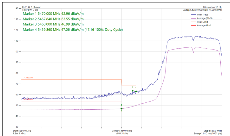
Figure 991 - 802.11n HT40, SDM, Core 0-1 - 5510 MHz Band Edge Frequency 5470 MHz
