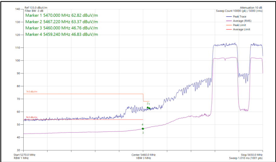
Figure 1042 - 802.11be EHT80, RU 484+242-92, SISO, Core 0 - 5610 MHz Band Edge Frequency 5470 MHz
