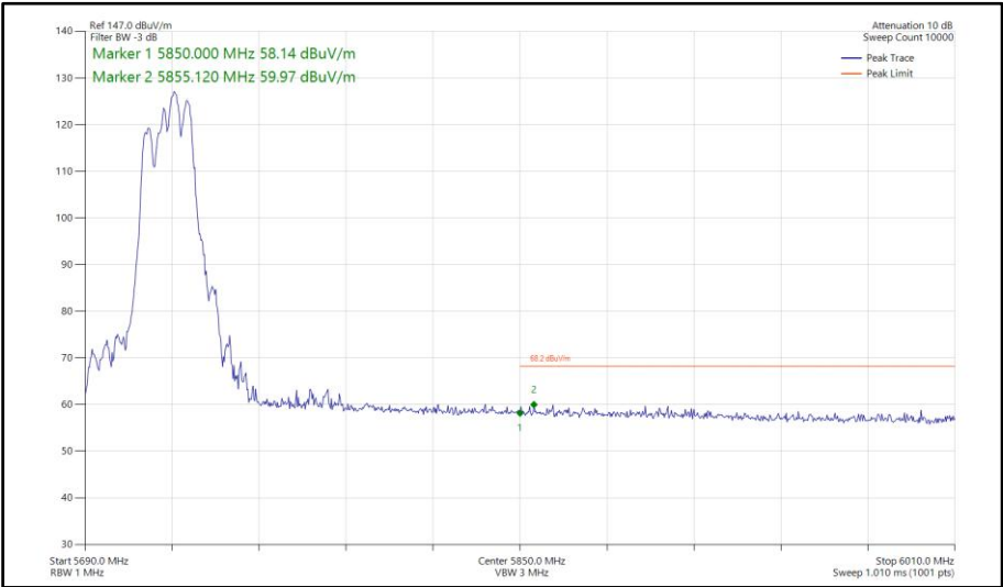
Figure 1017 - 802.11be EHT40, RU 106+26-85, SDM, Core 0-1 - 5710 MHz Band Edge Frequency 5850 MHz
