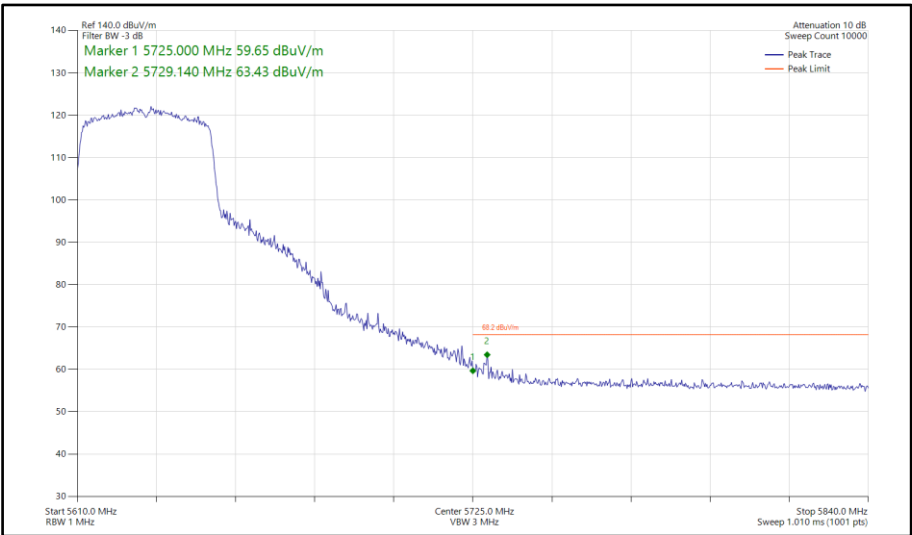
Figure 1027 - 802.11ax HE40, SU, TxBF, Core 0-1 - 5630 MHz Band Edge Frequency 5725 MHz
