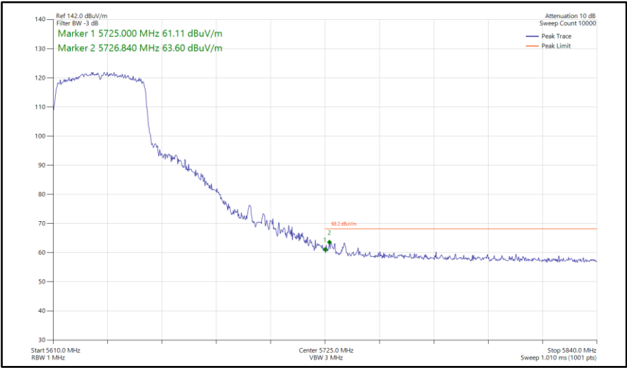
Figure 1005 - 802.11ax HE40, SU, SDM, Core 0-1 - 5630 MHz Band Edge Frequency 5725 MHz
