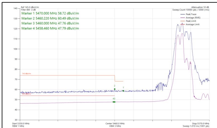
Figure 996 - 802.11ax HE40, RU 106-53, SDM, Core 0-1 - 5550 MHz Band Edge Frequency 5470 MHz
