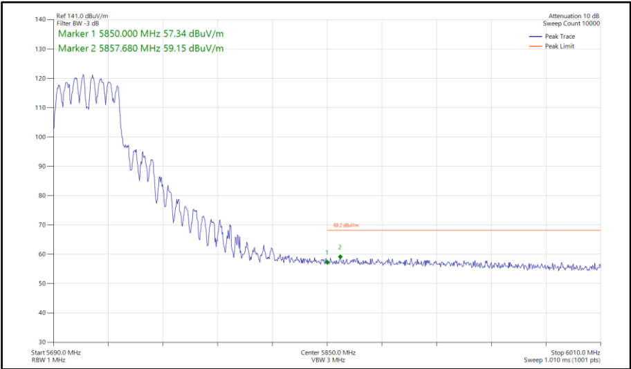
Figure 981 - 802.11a, CDD, Core 0-1 - 5710 MHz Band Edge Frequency 5850 MHz
