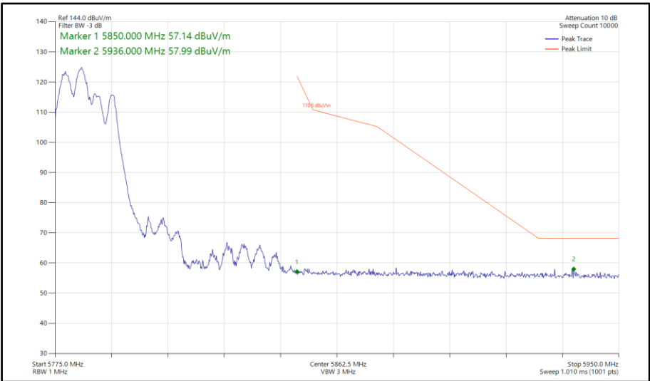
Figure 1018 - 802.11be EHT40, RU 106+26-82, SDM, Core 0-1 - 5795 MHz Band Edge Frequency 5850 MHz
