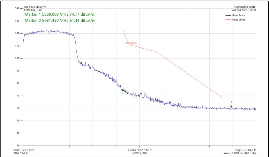
Figure 1015 - 802.11ax HE40, SU, SDM, Core 0-1 - 5795 MHz Band Edge Frequency 5850 MHz
