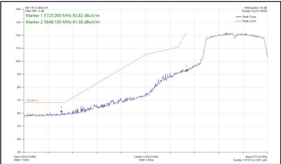
Figure 1023 - 802.11ac VHT40, TxBF, Core 0-1 - 5755 MHz Band Edge Frequency 5725 MHz
