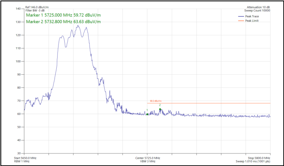
Figure 1010 - 802.11be EHT40, RU 106+26-85, SDM, Core 0-1 - 5670 MHz Band Edge Frequency 5725 MHz
