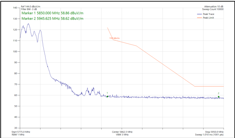
Figure 990 - 802.11be EHT40, RU 106+26-82, CDD, Core 0-1 - 5795 MHz Band Edge Frequency 5850 MHz
