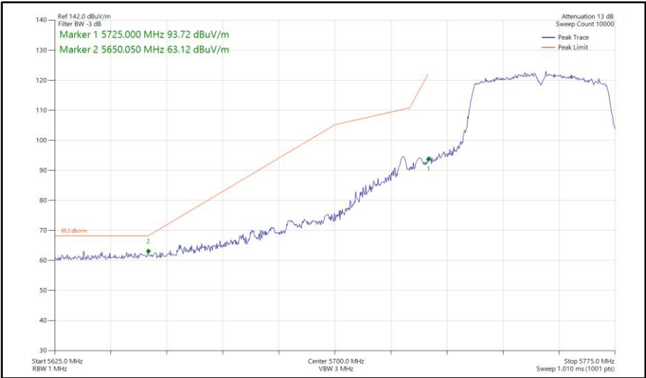
Figure 999 - 802.11n HT40, SDM, Core 0-1 - 5755 MHz Band Edge Frequency 5725 MHz
