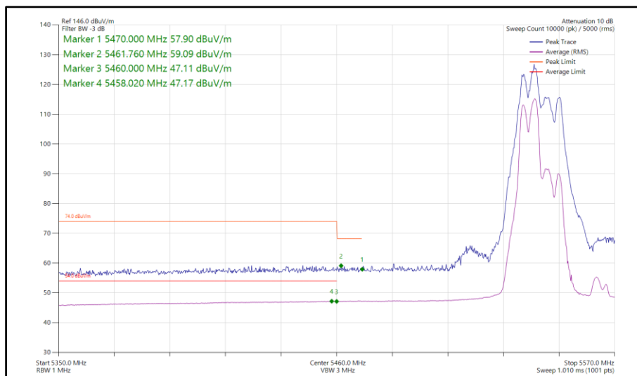
Figure 998 - 802.11be EHT40, RU 52+26-70, SDM, Core 0-1 - 5550 MHz Band Edge Frequency 5470 MHz
