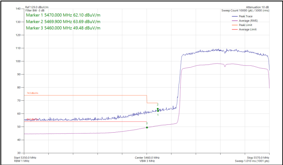
Figure 1037 - 802.11ax HE80, SU, SISO, Core 0 - 5530 MHz Band Edge Frequency 5470 MHz
