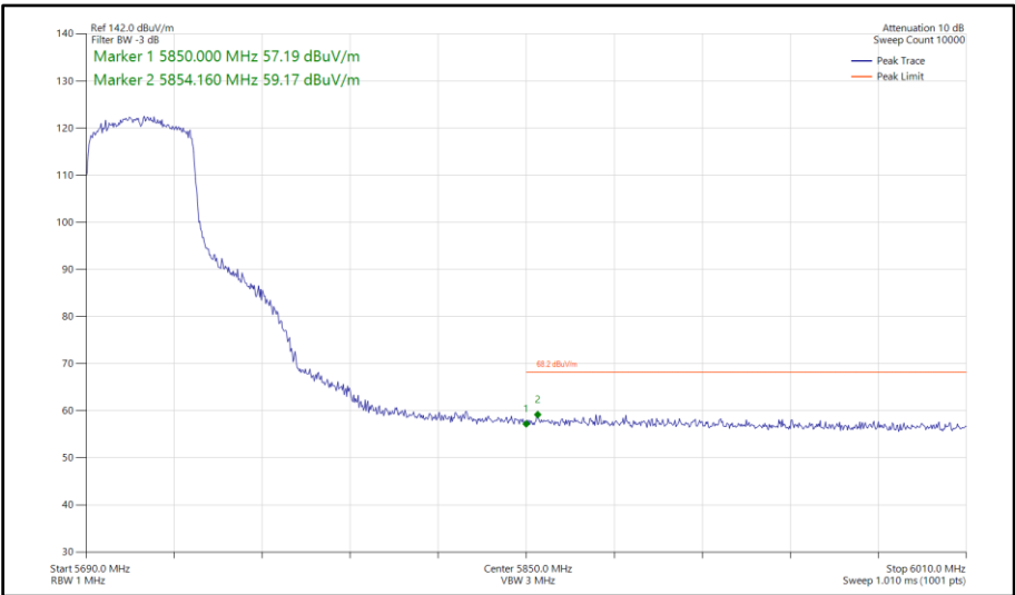
Figure 1031 - 802.11ax HE40, SU, TxBF, Core 0-1 - 5710 MHz Band Edge Frequency 5850 MHz
