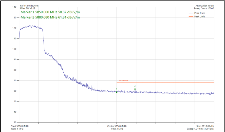
Figure 1013 - 802.11ax HE40, SU, SDM, Core 0-1 - 5710 MHz Band Edge Frequency 5850 MHz
