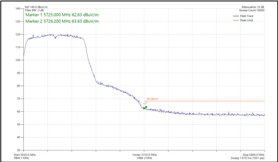
Figure 1026 - 802.11ac VHT40, TxBF, Core 0-1 - 5670 MHz Band Edge Frequency 5725 MHz
