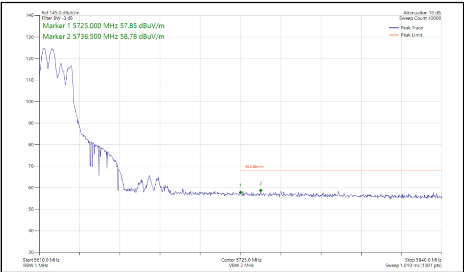
Figure 976 - 802.11ax HE40, RU 106-53, CDD, Core 0-1 - 5630 MHz Band Edge Frequency 5725 MHz
