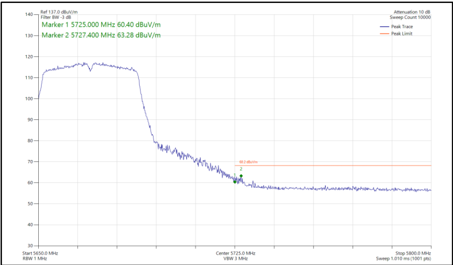
Figure 1004 - 802.11n HT40, SDM, Core 0-1 - 5670 MHz Band Edge Frequency 5725 MHz
