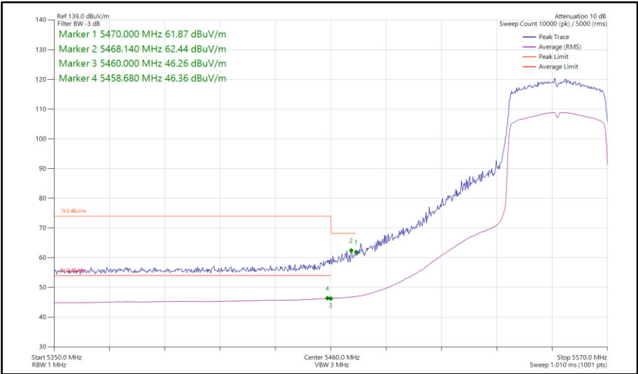
Figure 1022 - 802.11ax HE40, SU, TxBF, Core 0-1 - 5550 MHz Band Edge Frequency 5470 MHz
