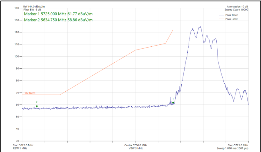
Figure 1001 - 802.11ax HE40, RU 106-53, SDM, Core 0-1 - 5755 MHz Band Edge Frequency 5725 MHz
