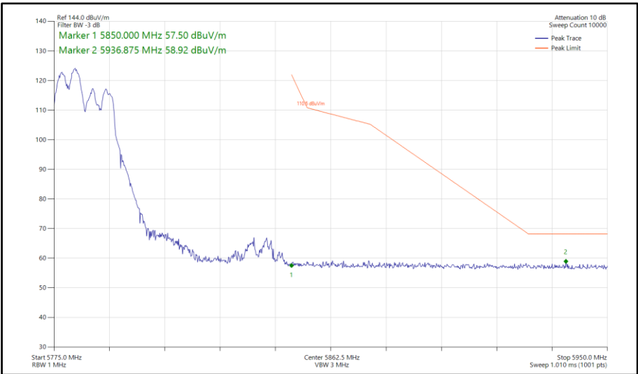
Figure 988 - 802.11ax HE40, RU 106-53, CDD, Core 0-1 - 5795 MHz Band Edge Frequency 5850 MHz
